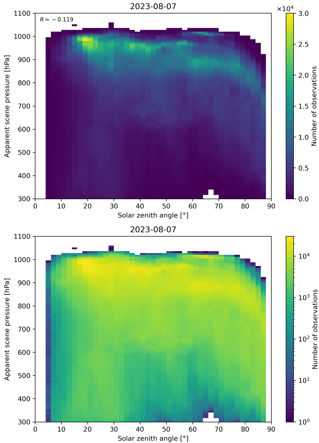
Figure 118: Scatter density plot of “Solar zenith angle” against “Apparent scene pressure” for 2023-08-06 to 2023-08-08.
