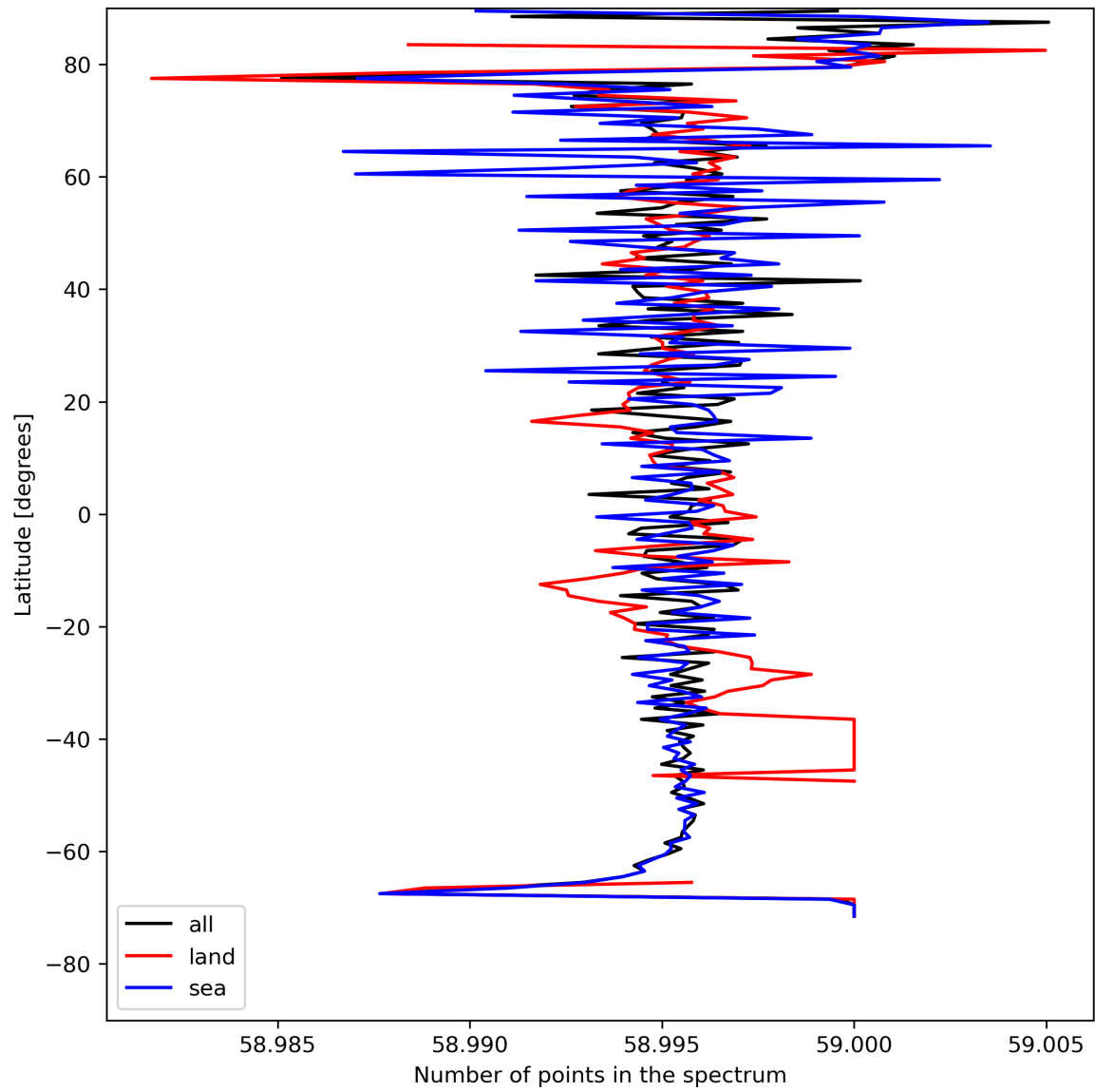
Figure 27: Zonal average of “Number of points in the spectrum” for 2023-08-06 to 2023-08-08.
