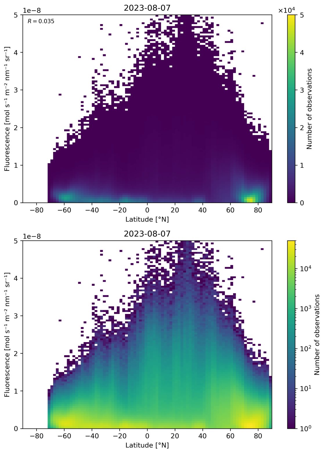
Figure 101: Scatter density plot of “Latitude” against “Fluorescence” for 2023-08-06 to 2023-08-08.
