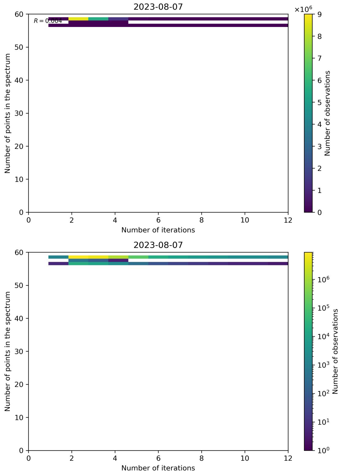
Figure 108: Scatter density plot of “Number of iterations” against “Number of points in the spectrum” for 2023-08-06 to 2023-08-08.
