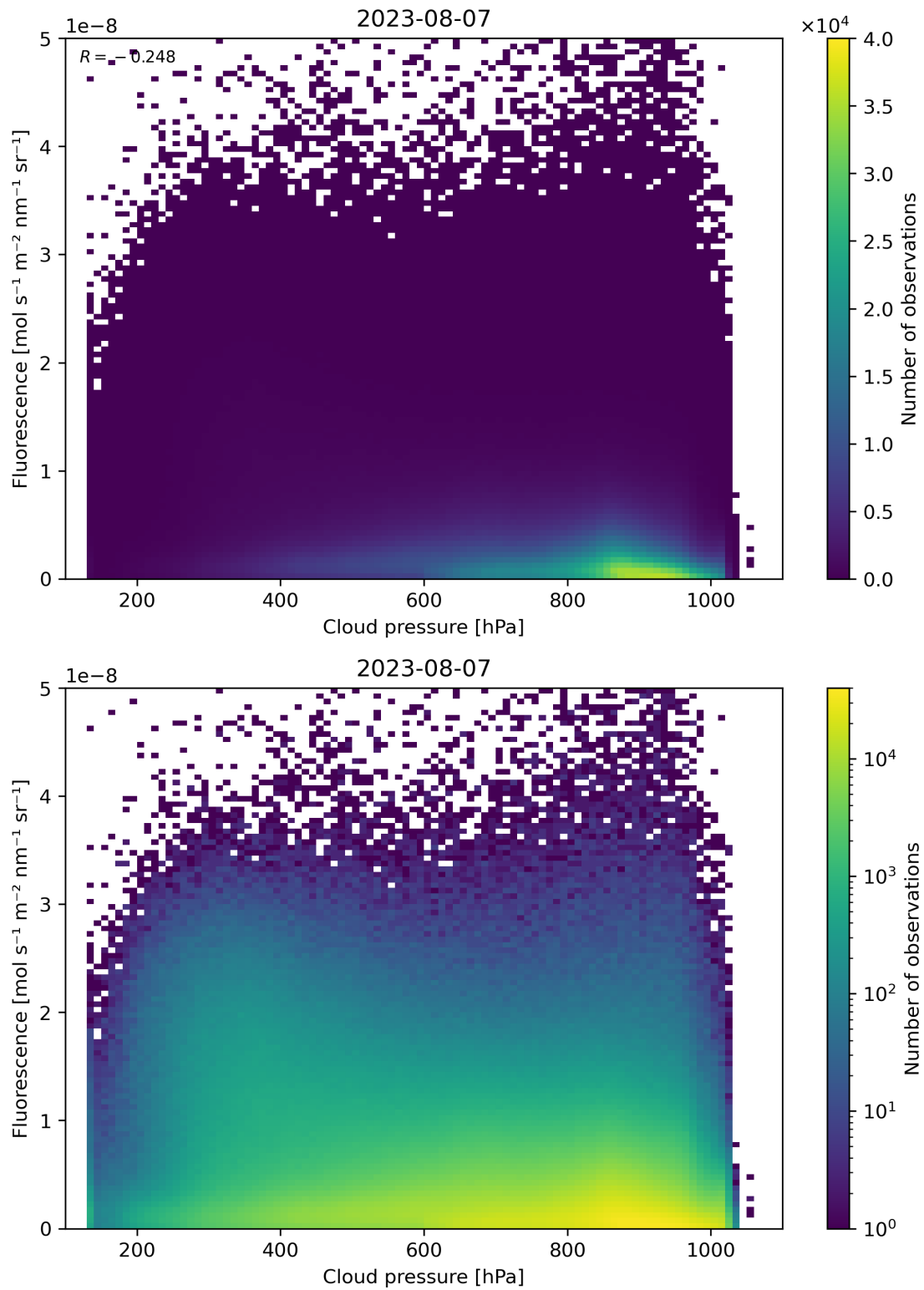
Figure 88: Scatter density plot of “Cloud pressure” against “Fluorescence” for 2023-08-06 to 2023-08-08.
