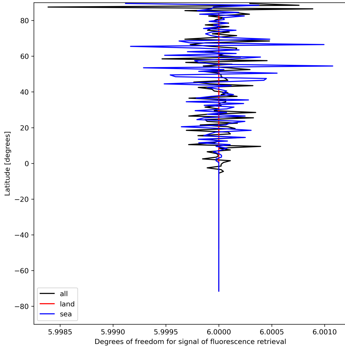
Figure 26: Zonal average of “Degrees of freedom for signal of fluorescence retrieval” for 2023-08-06 to 2023-08-08.
