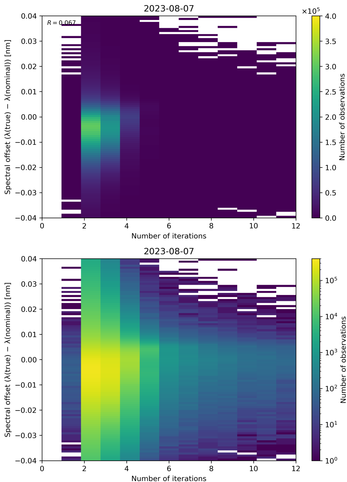
Figure 109: Scatter density plot of “Number of iterations” against “Spectral offset ( \lambda(\text{true}) - \lambda(\text{nominal}) )” for 2023-08-06 to 2023-08-08.
