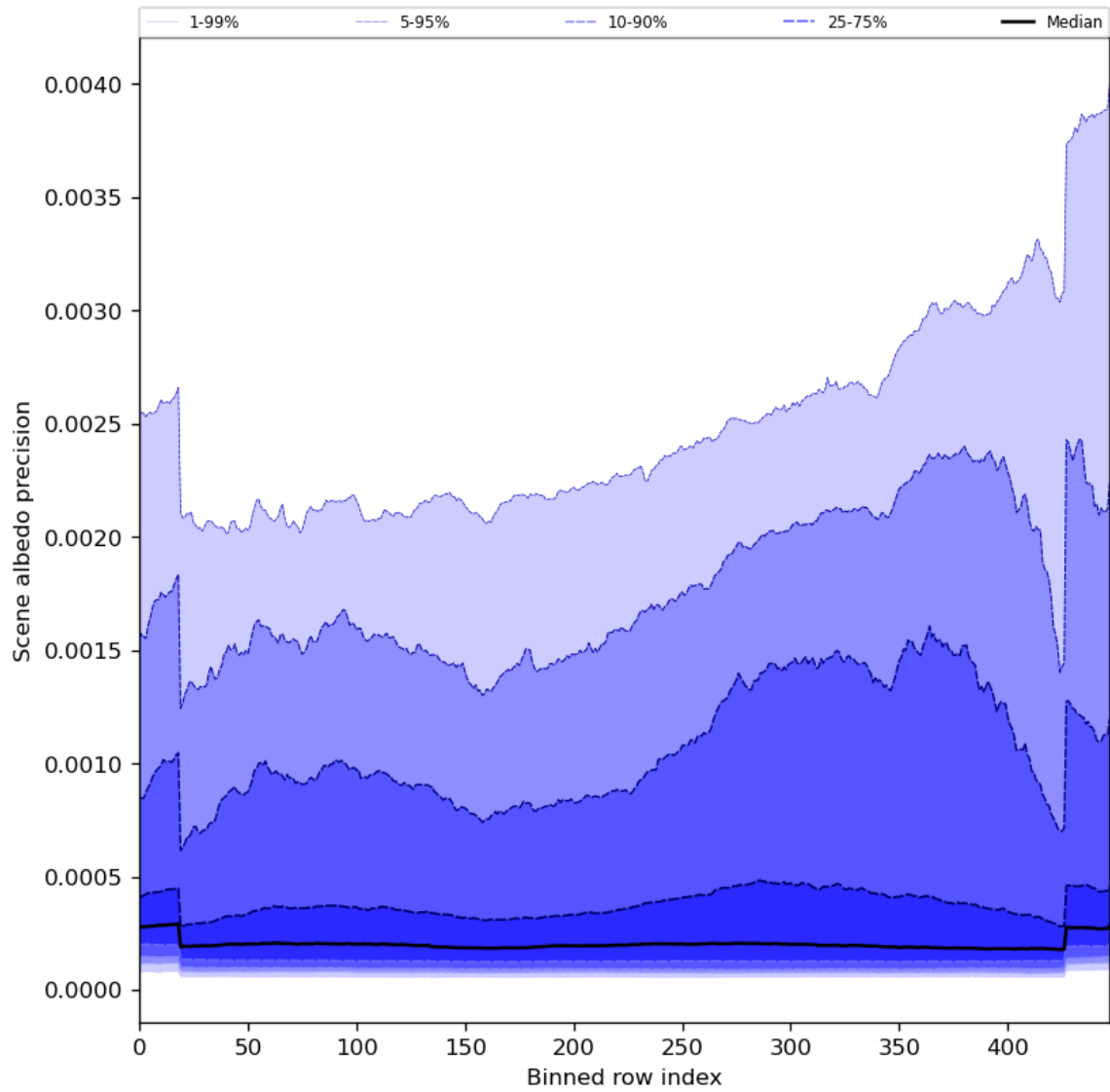
Figure 52: Along track statistics of “Scene albedo precision” for 2023-08-06 to 2023-08-08
