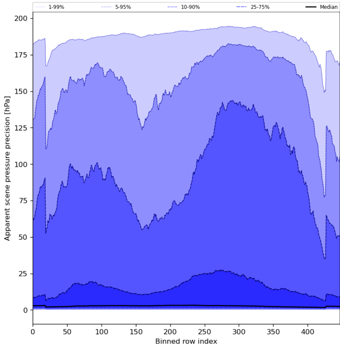
Figure 54: Along track statistics of “Apparent scene pressure precision” for 2023-08-06 to 2023-08-08
