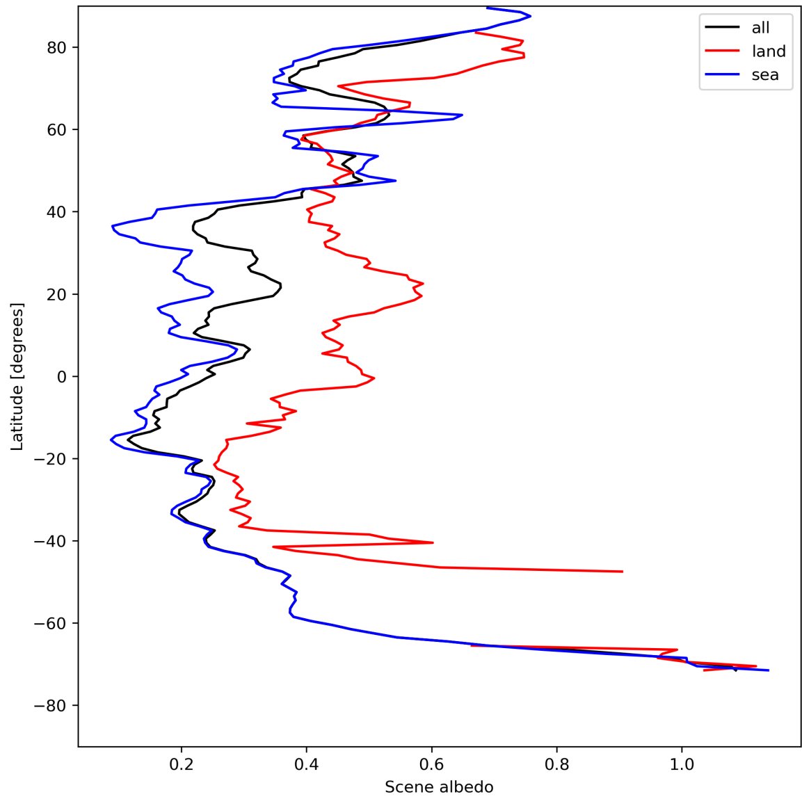
Figure 17: Zonal average of “Scene albedo” for 2023-08-06 to 2023-08-08.
