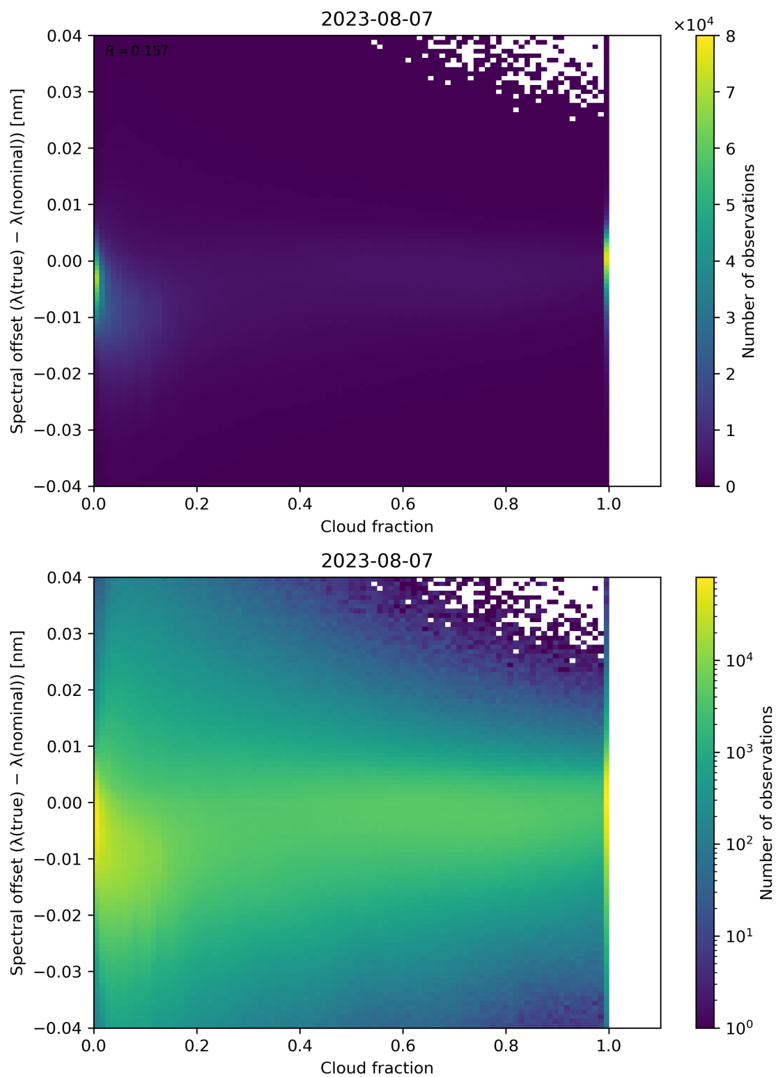
Figure 83: Scatter density plot of “Cloud fraction” against “Spectral offset ( \lambda(\text{true}) - \lambda(\text{nominal}) )” for 2023-08-06 to 2023-08-08.
