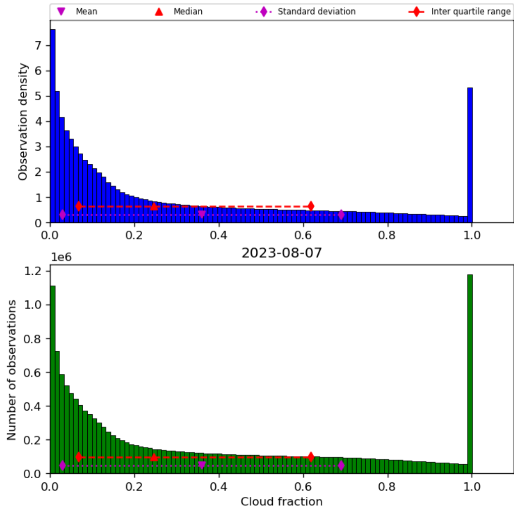
Figure 32: Histogram of “Cloud fraction” for 2023-08-06 to 2023-08-08
