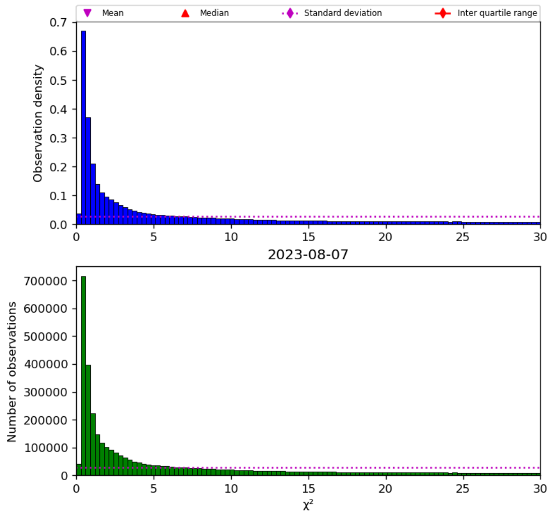
Figure 38: Histogram of “ \chi^2 ” for 2023-08-06 to 2023-08-08
