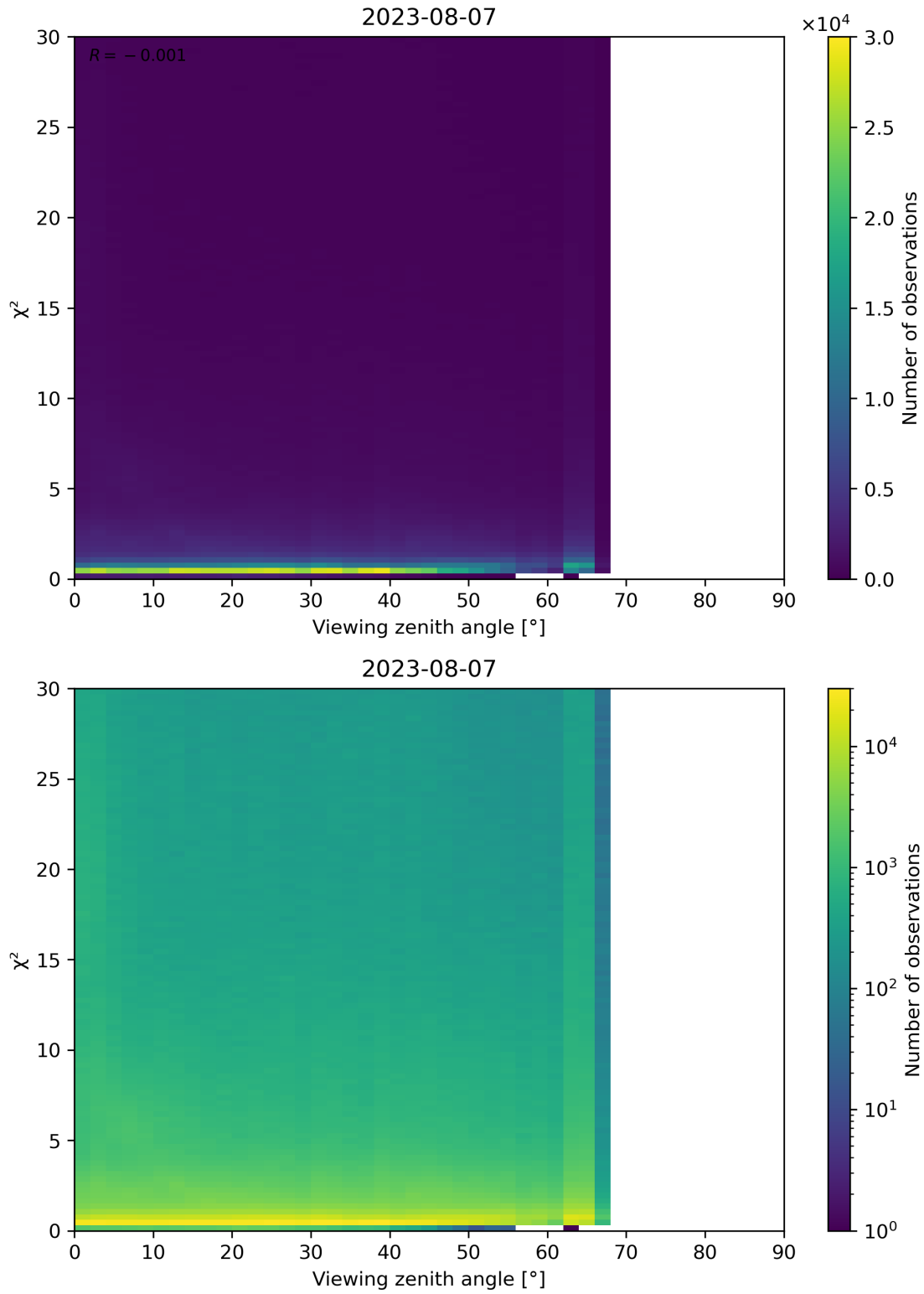
Figure 130: Scatter density plot of “Viewing zenith angle” against “ \chi^2 ” for 2023-08-06 to 2023-08-08.
