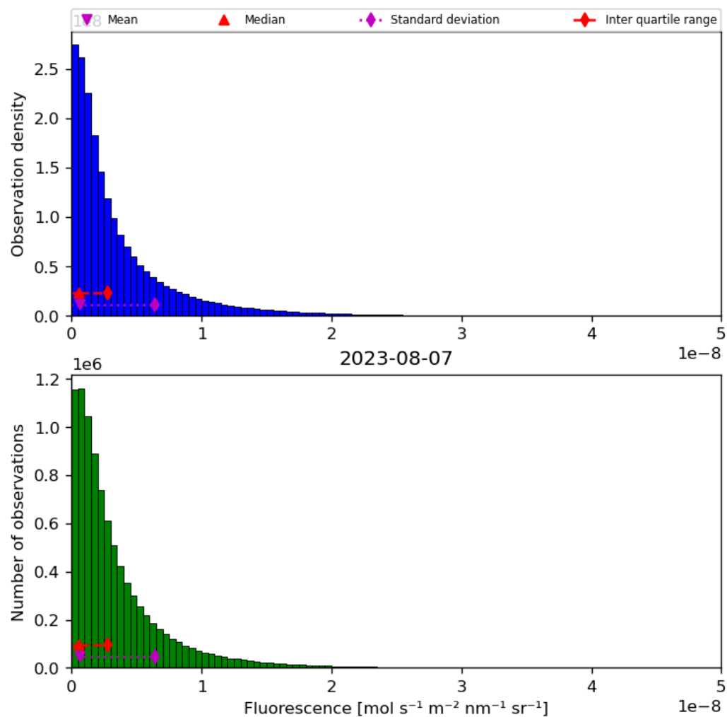
Figure 40: Histogram of “Fluorescence” for 2023-08-06 to 2023-08-08
