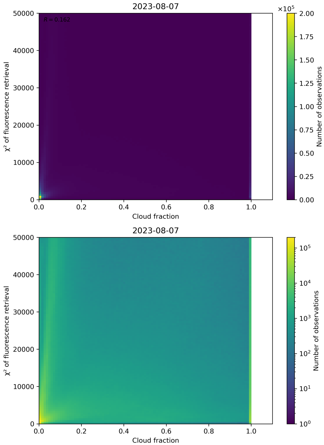
Figure 78: Scatter density plot of “Cloud fraction” against “ \chi^2 of fluorescence retrieval” for 2023-08-06 to 2023-08-08.
