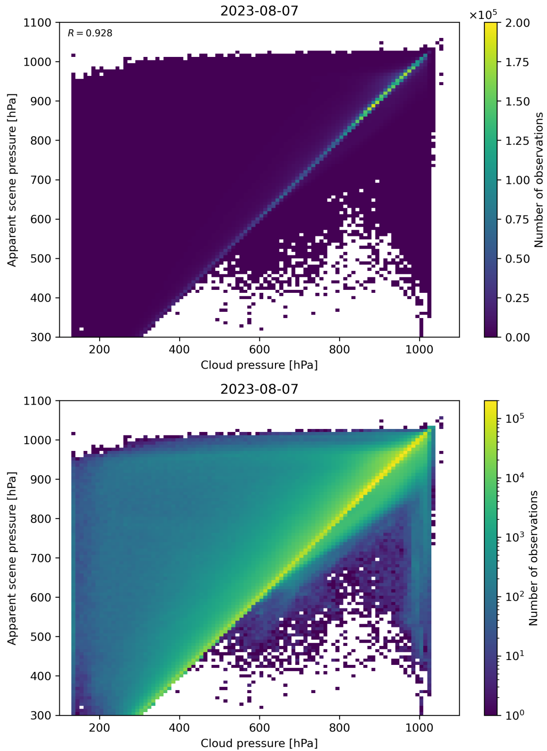
Figure 84: Scatter density plot of “Cloud pressure” against “Apparent scene pressure” for 2023-08-06 to 2023-08-08.
