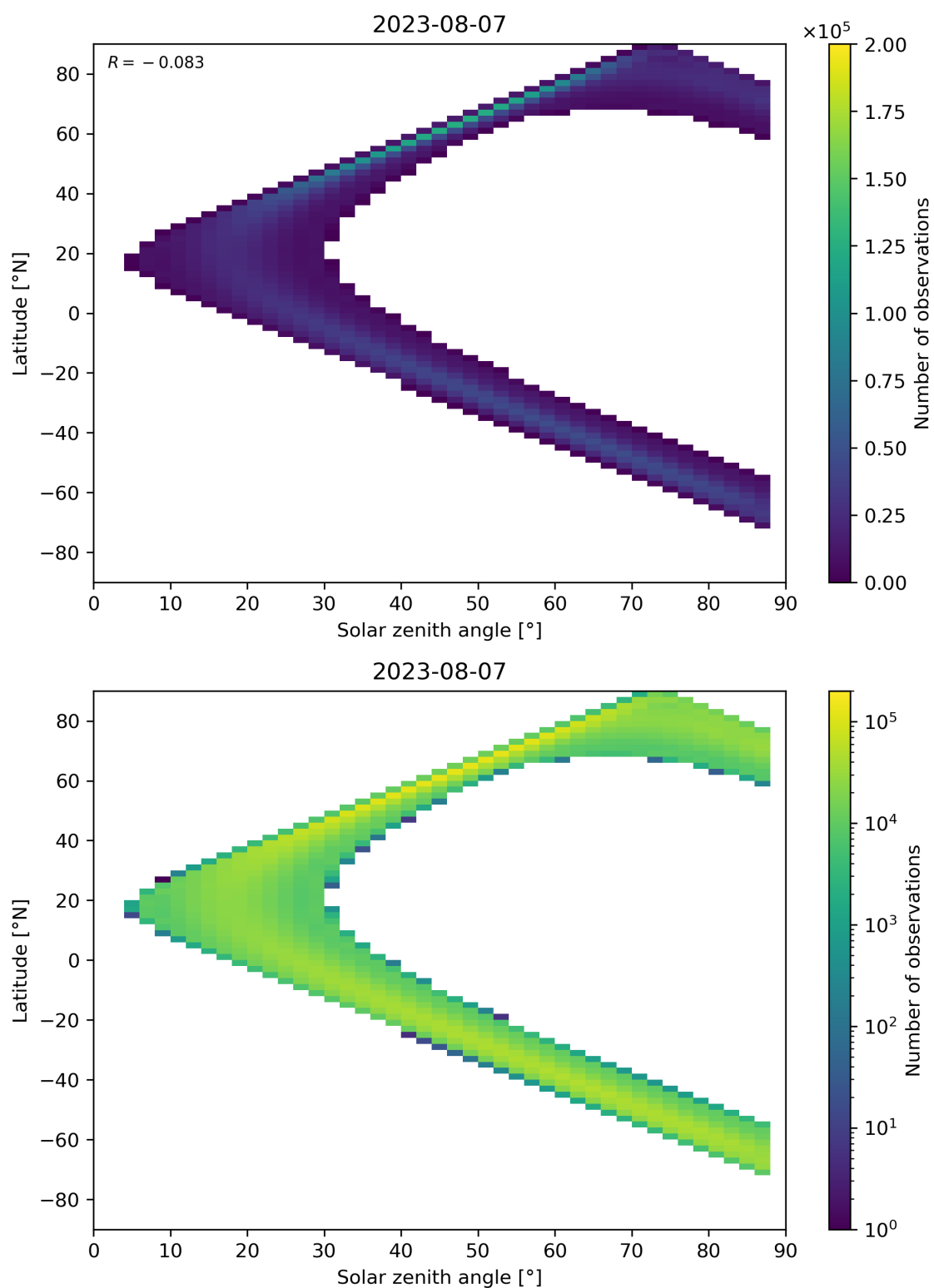
Figure 124: Scatter density plot of “Solar zenith angle” against “Latitude” for 2023-08-06 to 2023-08-08.
