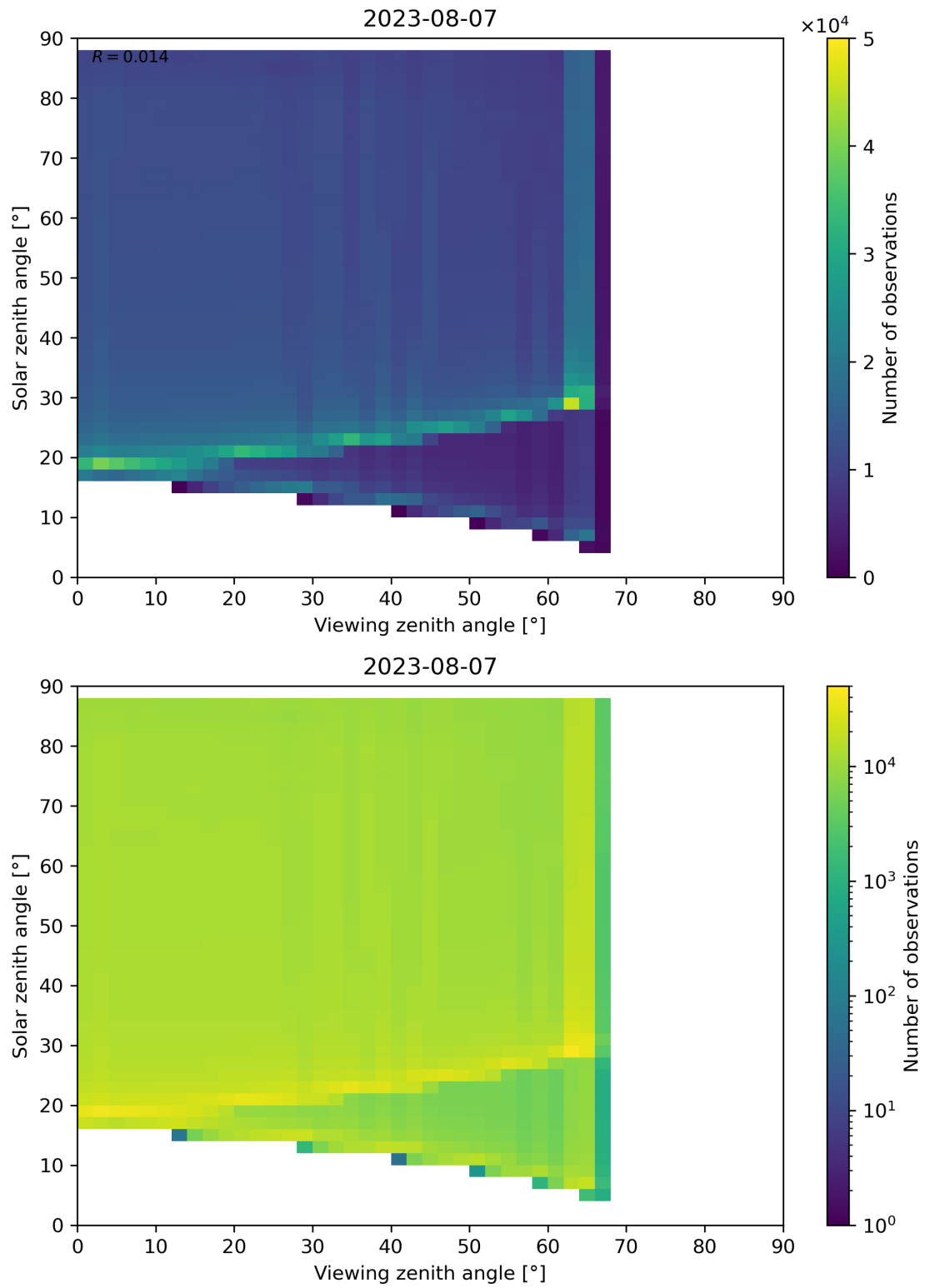
Figure 139: Scatter density plot of “Viewing zenith angle” against “Solar zenith angle” for 2023-08-06 to 2023-08-08.
