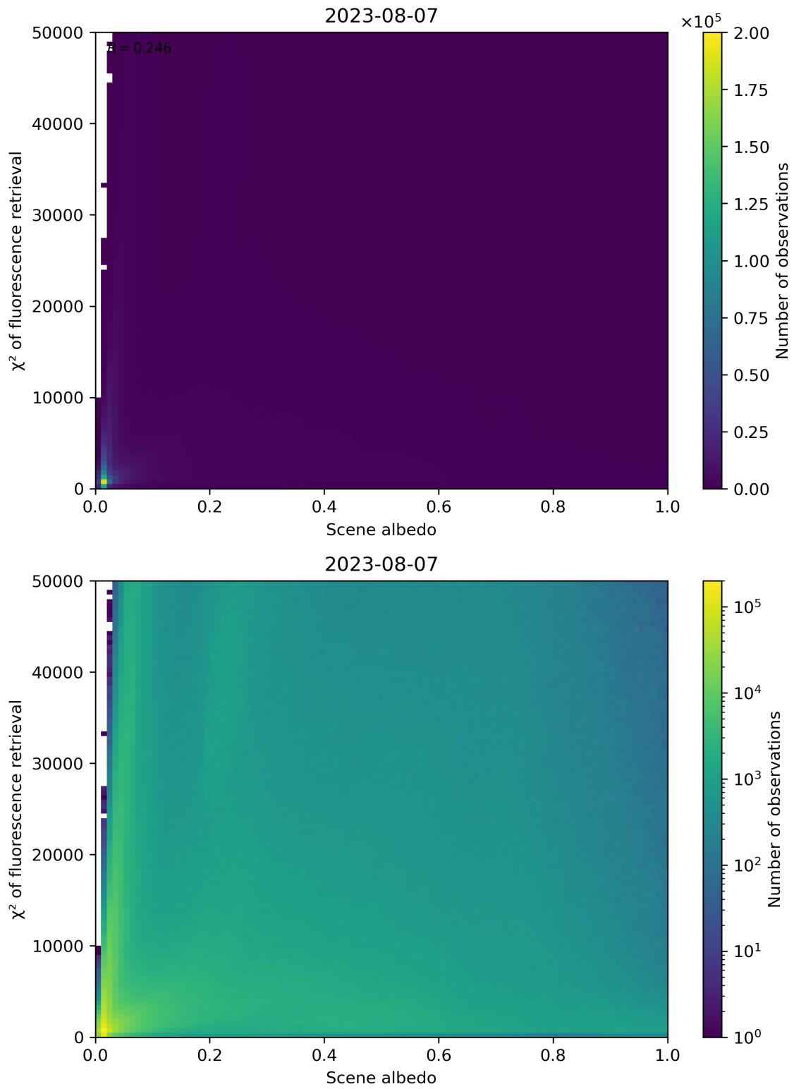
Figure 113: Scatter density plot of “Scene albedo” against “ \chi^2 of fluorescence retrieval” for 2023-08-06 to 2023-08-08.
