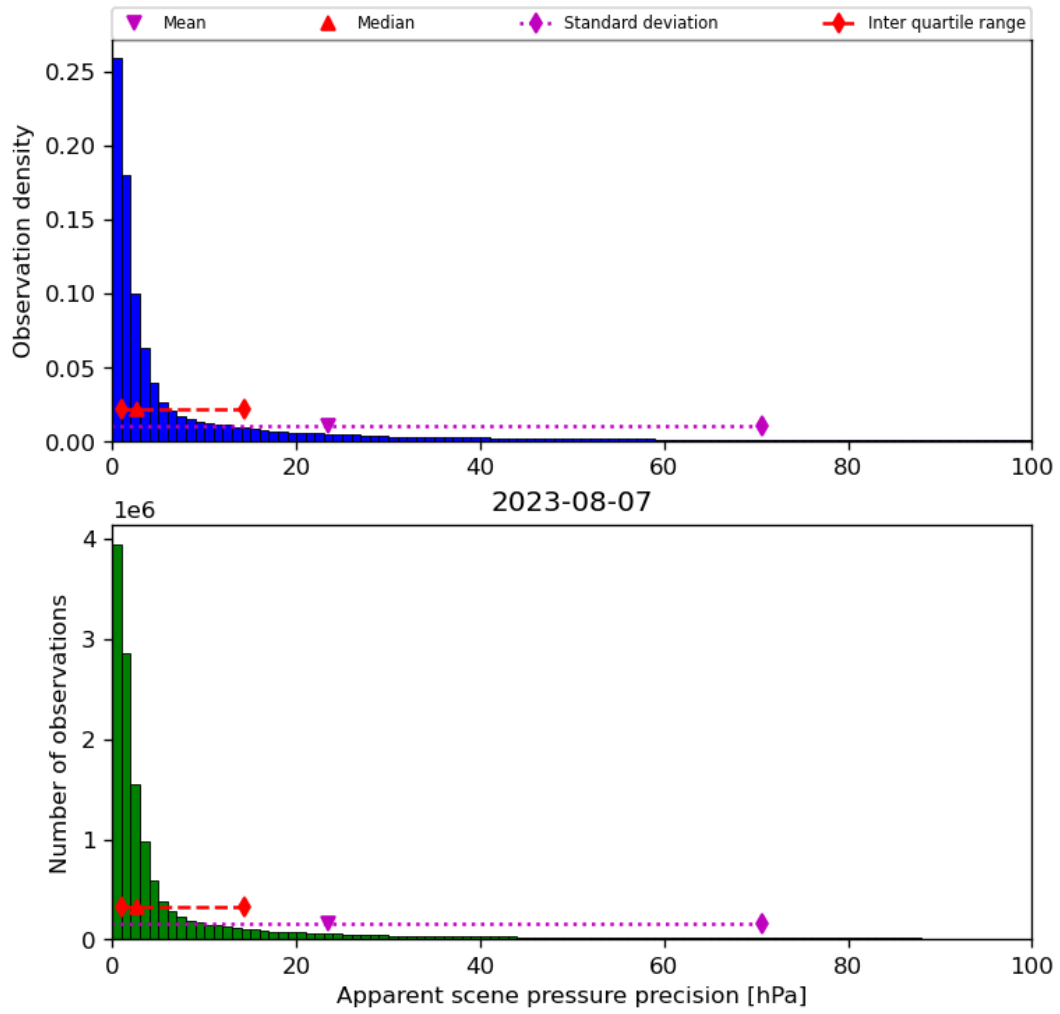
Figure 37: Histogram of “Apparent scene pressure precision” for 2023-08-06 to 2023-08-08
