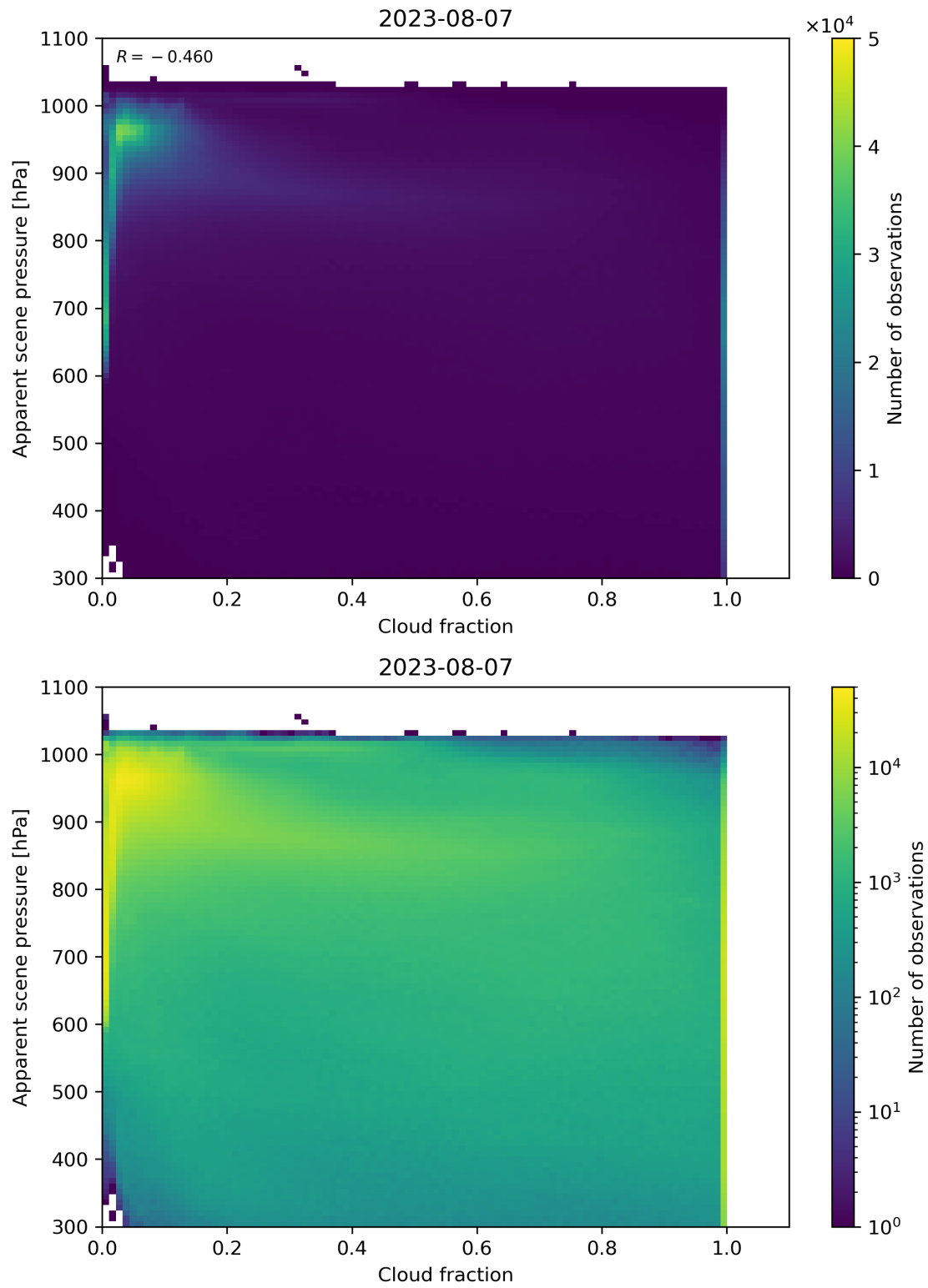
Figure 76: Scatter density plot of “Cloud fraction” against “Apparent scene pressure” for 2023-08-06 to 2023-08-08.
