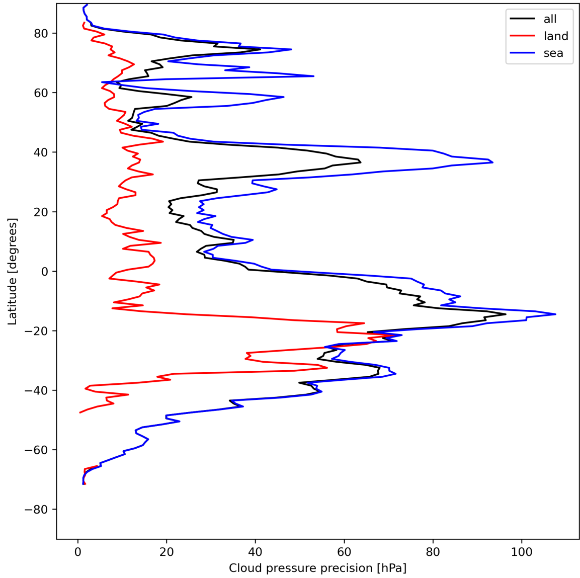
Figure 14: Zonal average of “Cloud pressure precision” for 2023-08-06 to 2023-08-08.
