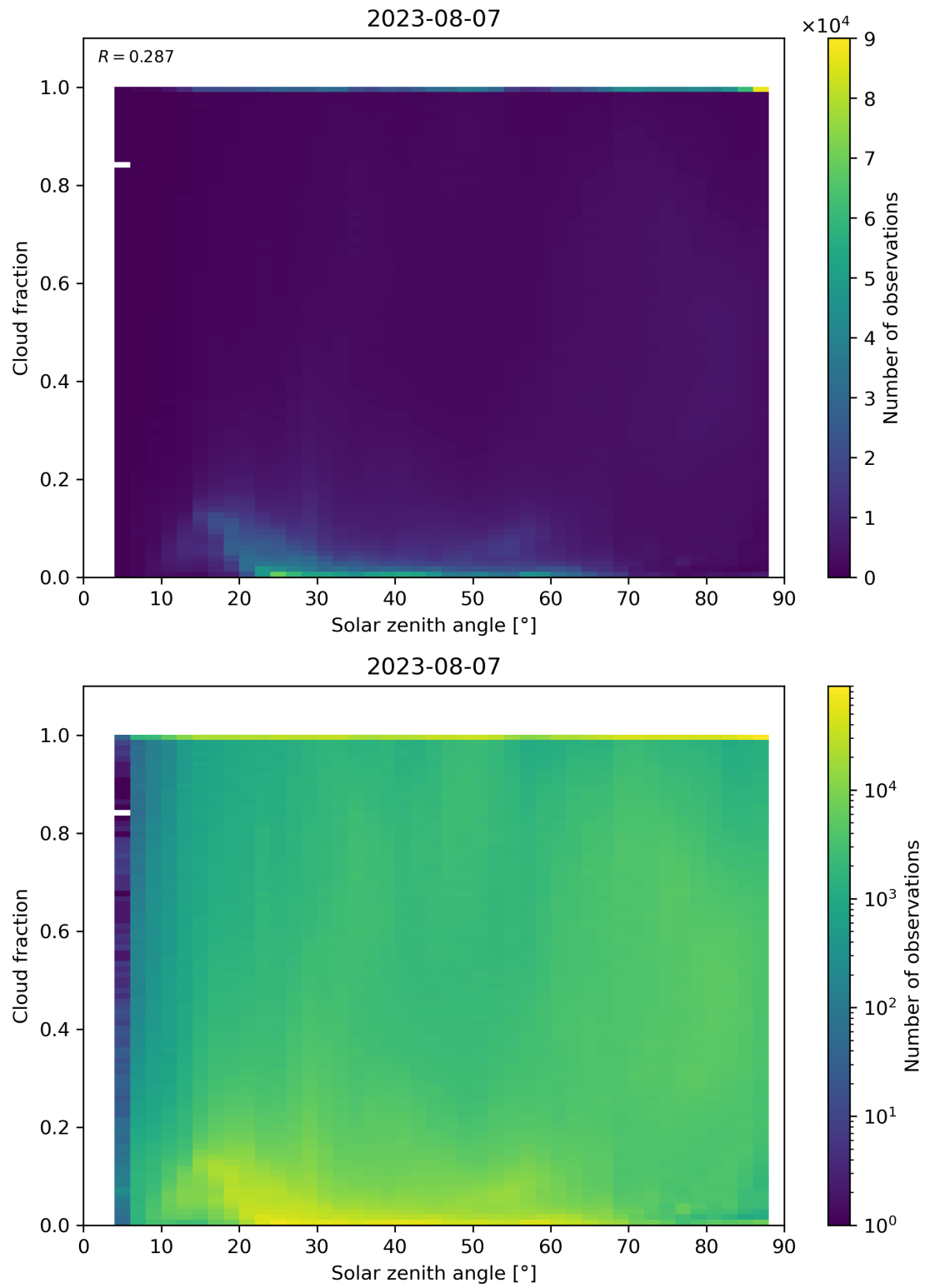
Figure 121: Scatter density plot of “Solar zenith angle” against “Cloud fraction” for 2023-08-06 to 2023-08-08.
