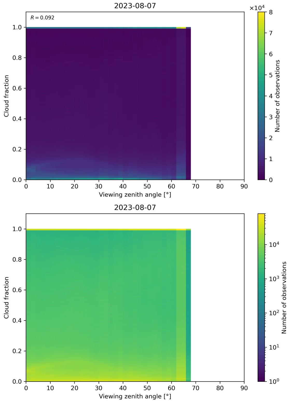
Figure 132: Scatter density plot of “Viewing zenith angle” against “Cloud fraction” for 2023-08-06 to 2023-08-08.
