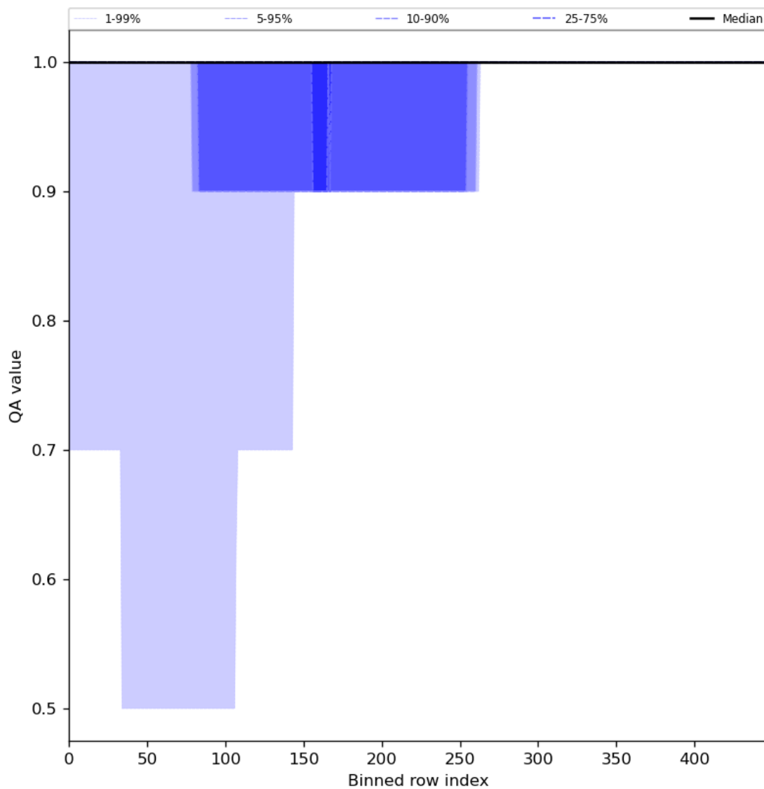
Figure 46: Along track statistics of “QA value” for 2023-08-06 to 2023-08-08
