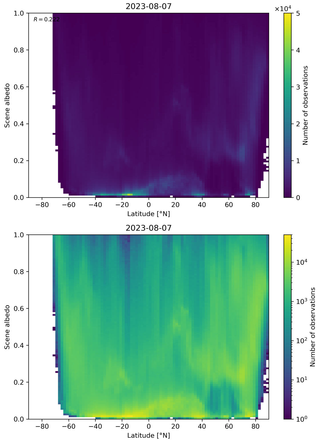
Figure 104: Scatter density plot of “Latitude” against “Scene albedo” for 2023-08-06 to 2023-08-08.
