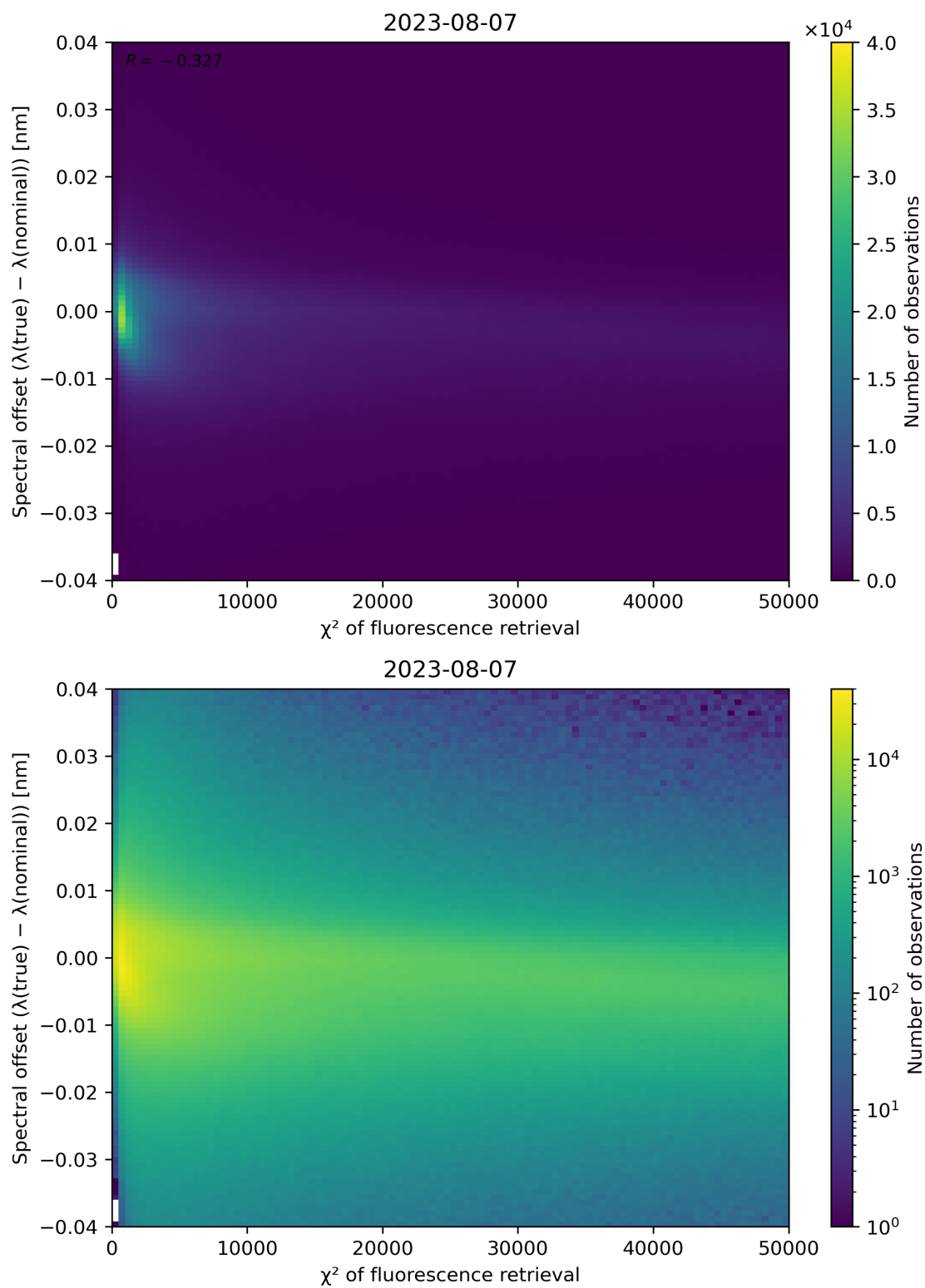
Figure 72: Scatter density plot of " \chi^2 of fluorescence retrieval" against "Spectral offset ( \lambda(\text{true}) - \lambda(\text{nominal}) )" for 2023-08-06 to 2023-08-08.
