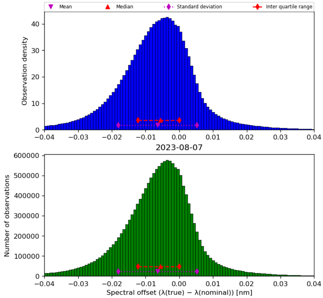
Figure 45: Histogram of “Spectral offset ( \lambda(\text{true}) - \lambda(\text{nominal}) )” for 2023-08-06 to 2023-08-08
