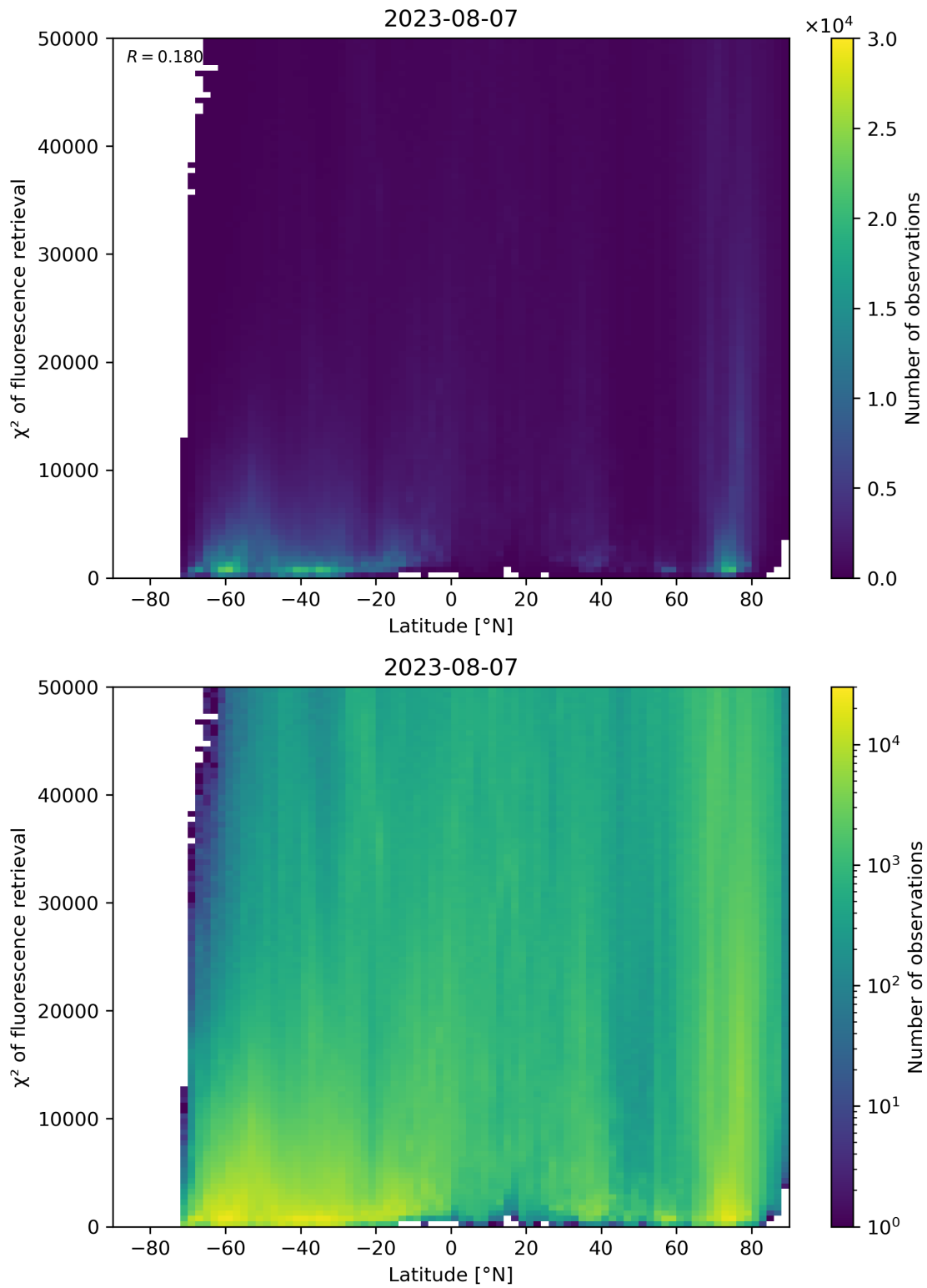
Figure 98: Scatter density plot of “Latitude” against “ \chi^2 of fluorescence retrieval” for 2023-08-06 to 2023-08-08.
