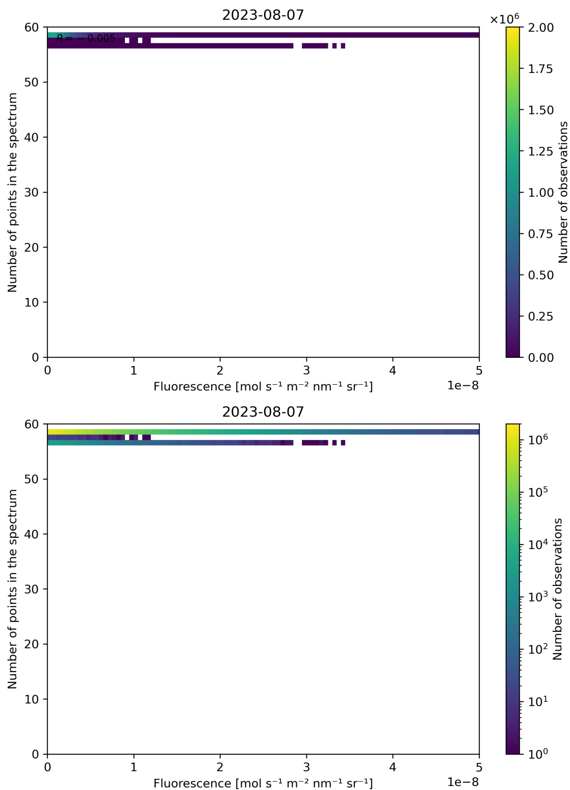
Figure 94: Scatter density plot of “Fluorescence” against “Number of points in the spectrum” for 2023-08-06 to 2023-08-08.
