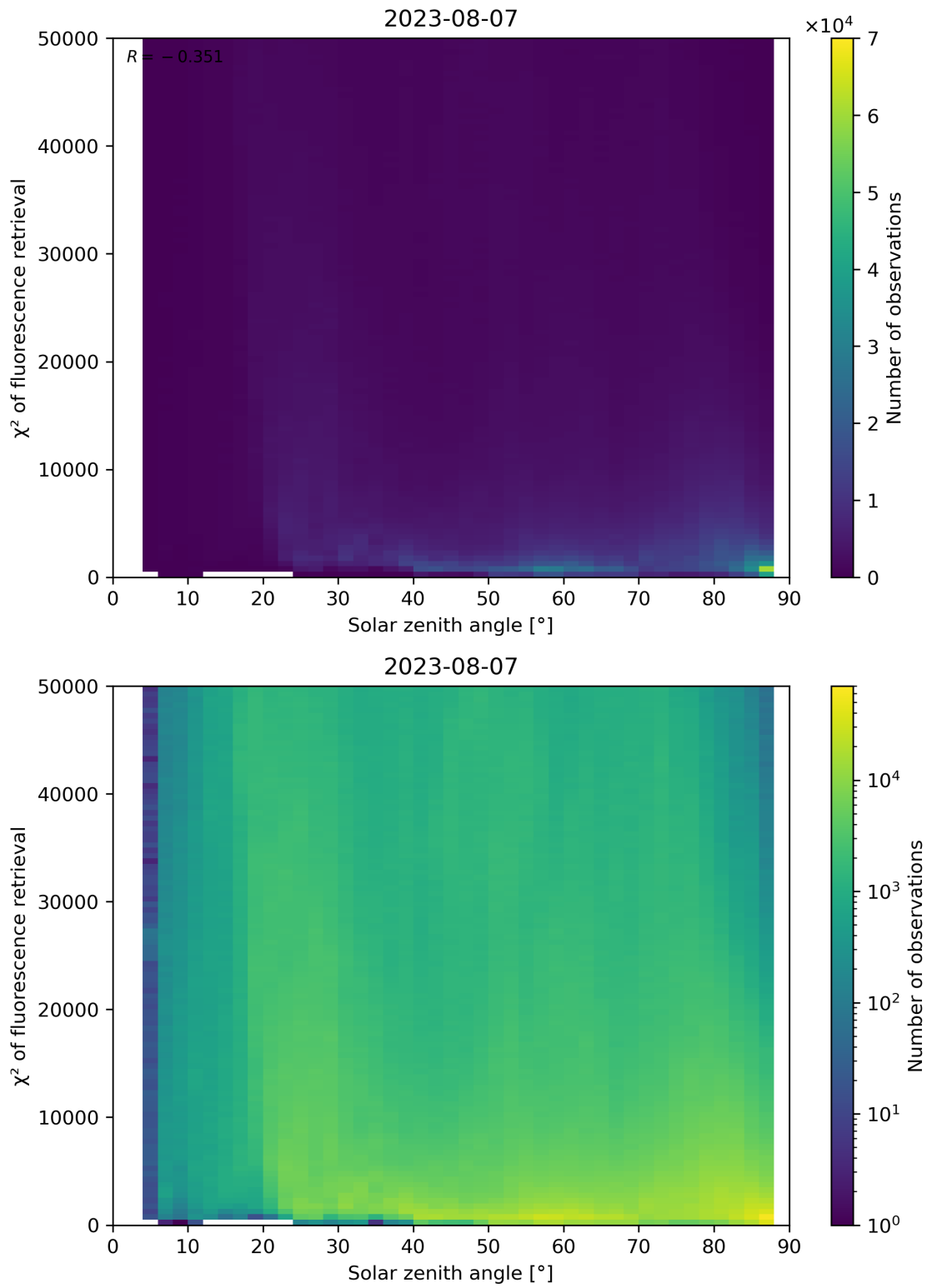
Figure 120: Scatter density plot of “Solar zenith angle” against “ \chi^2 of fluorescence retrieval” for 2023-08-06 to 2023-08-08.
