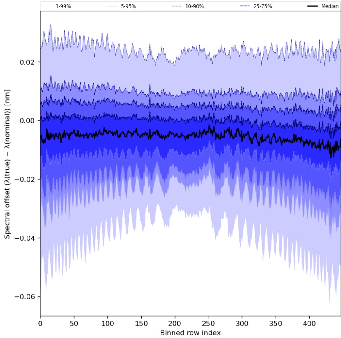
Figure 62: Along track statistics of “Spectral offset ( \lambda(\text{true}) - \lambda(\text{nominal}) )” for 2023-08-06 to 2023-08-08
