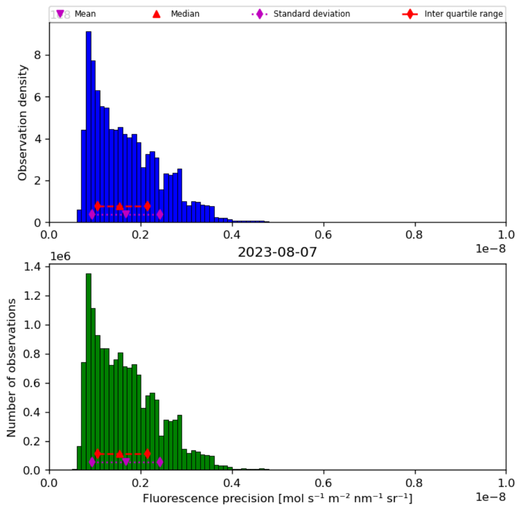
Figure 41: Histogram of “Fluorescence precision” for 2023-08-06 to 2023-08-08
