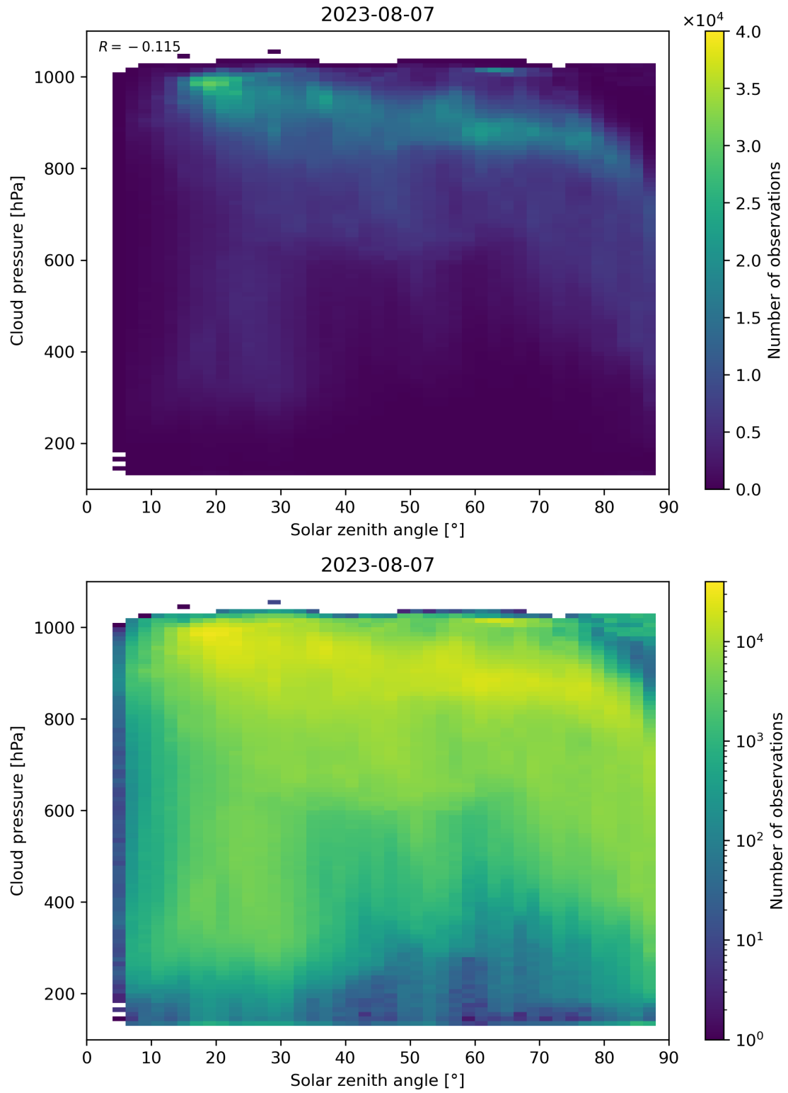
Figure 122: Scatter density plot of “Solar zenith angle” against “Cloud pressure” for 2023-08-06 to 2023-08-08.
