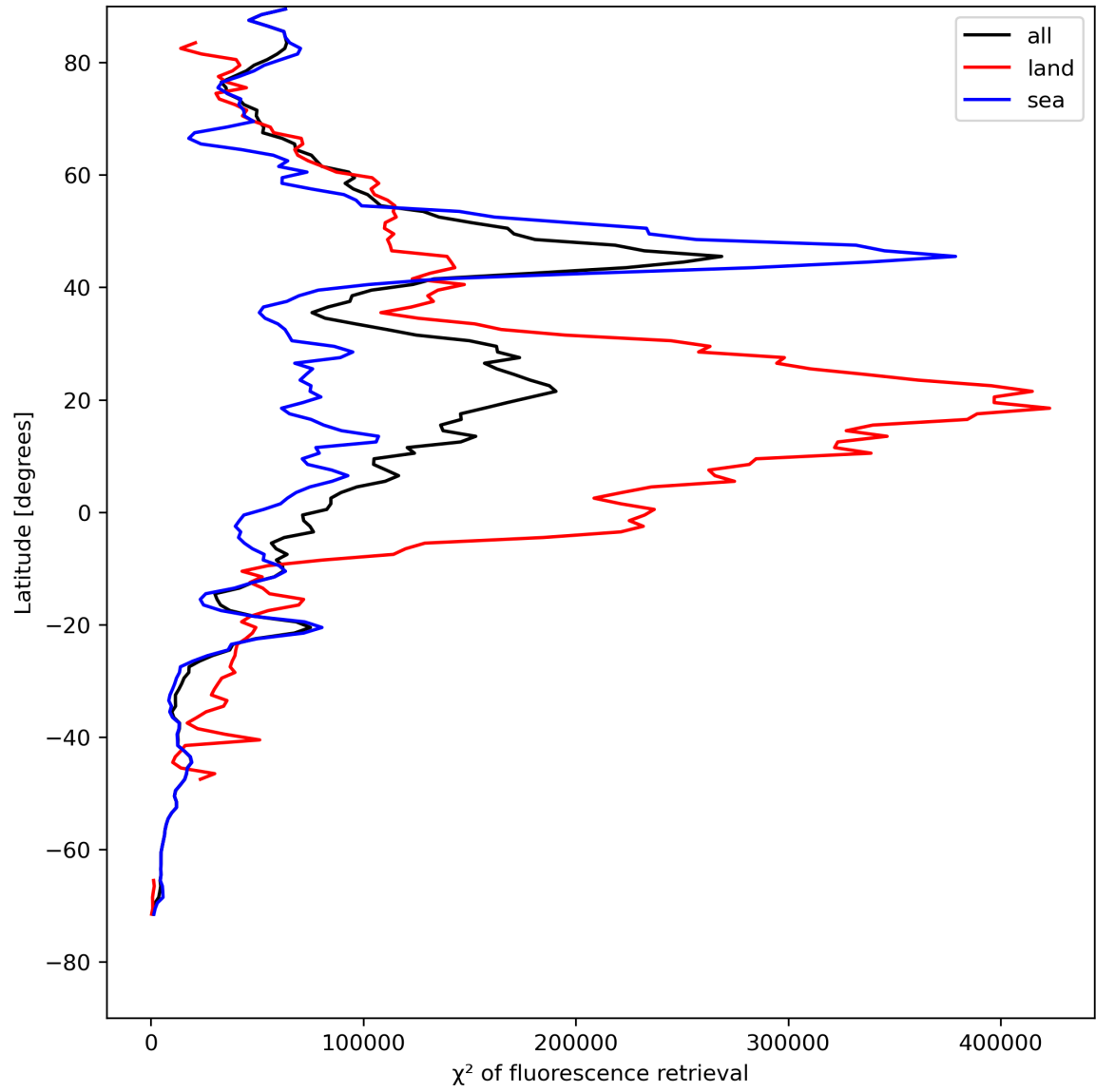
Figure 25: Zonal average of “ \chi^2 of fluorescence retrieval” for 2023-08-06 to 2023-08-08.
