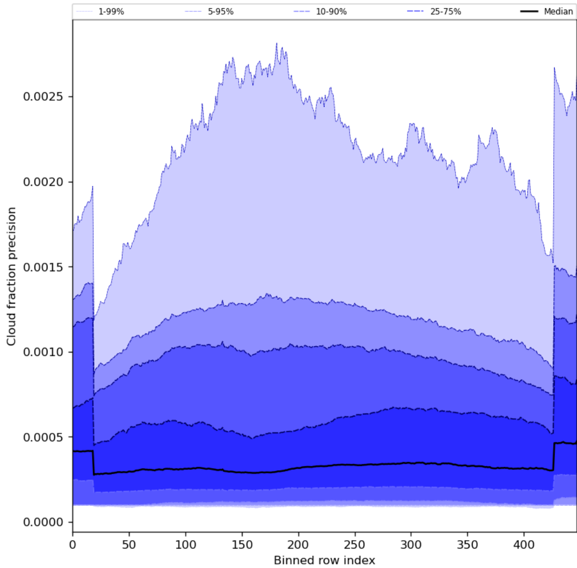
Figure 50: Along track statistics of “Cloud fraction precision” for 2023-08-06 to 2023-08-08
