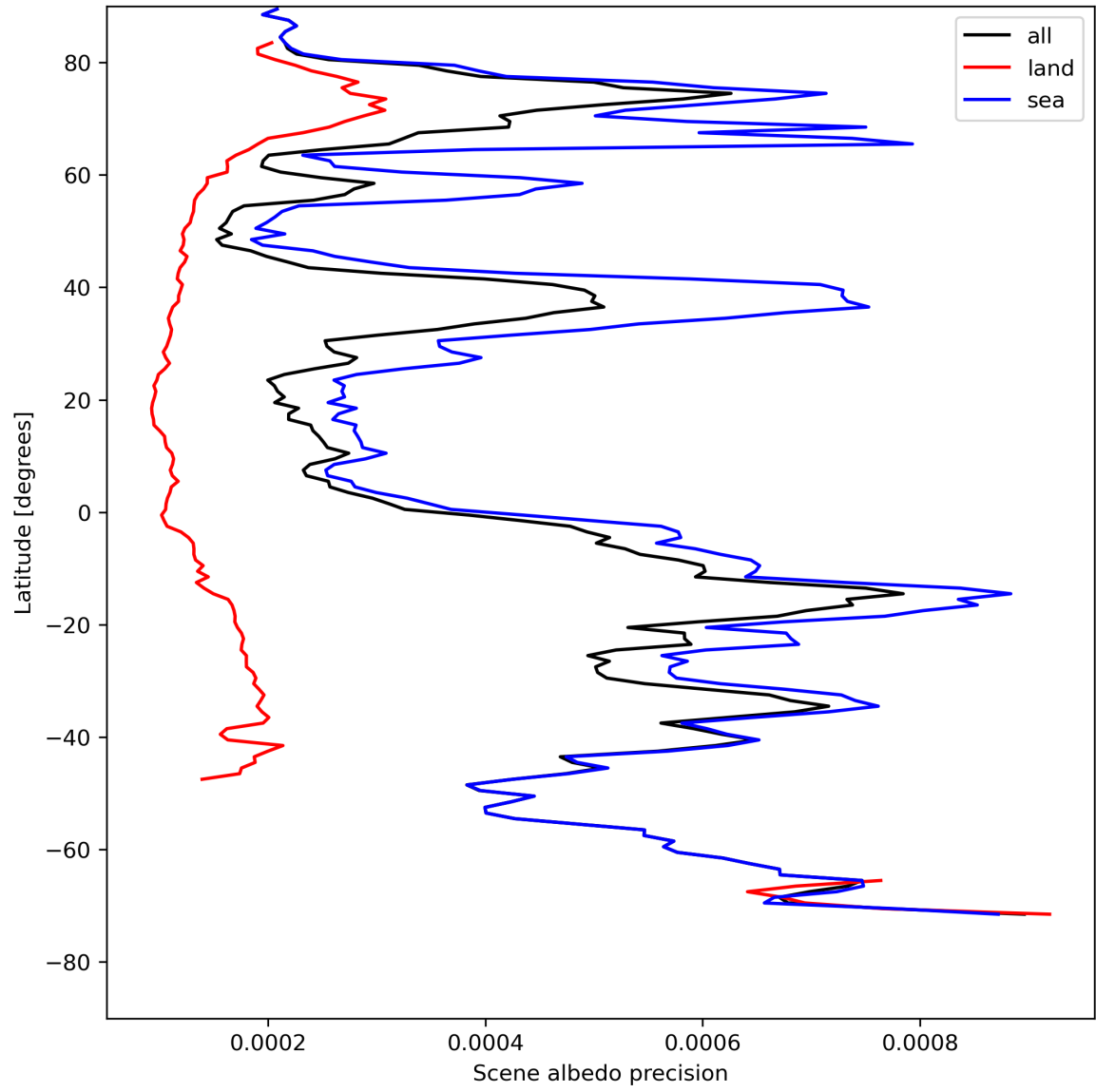
Figure 18: Zonal average of “Scene albedo precision” for 2023-08-06 to 2023-08-08.
