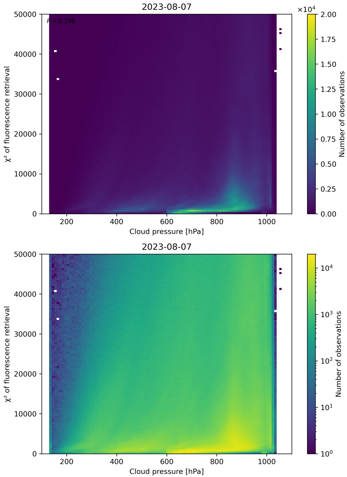
Figure 86: Scatter density plot of “Cloud pressure” against “ \chi^2 of fluorescence retrieval” for 2023-08-06 to 2023-08-08.
