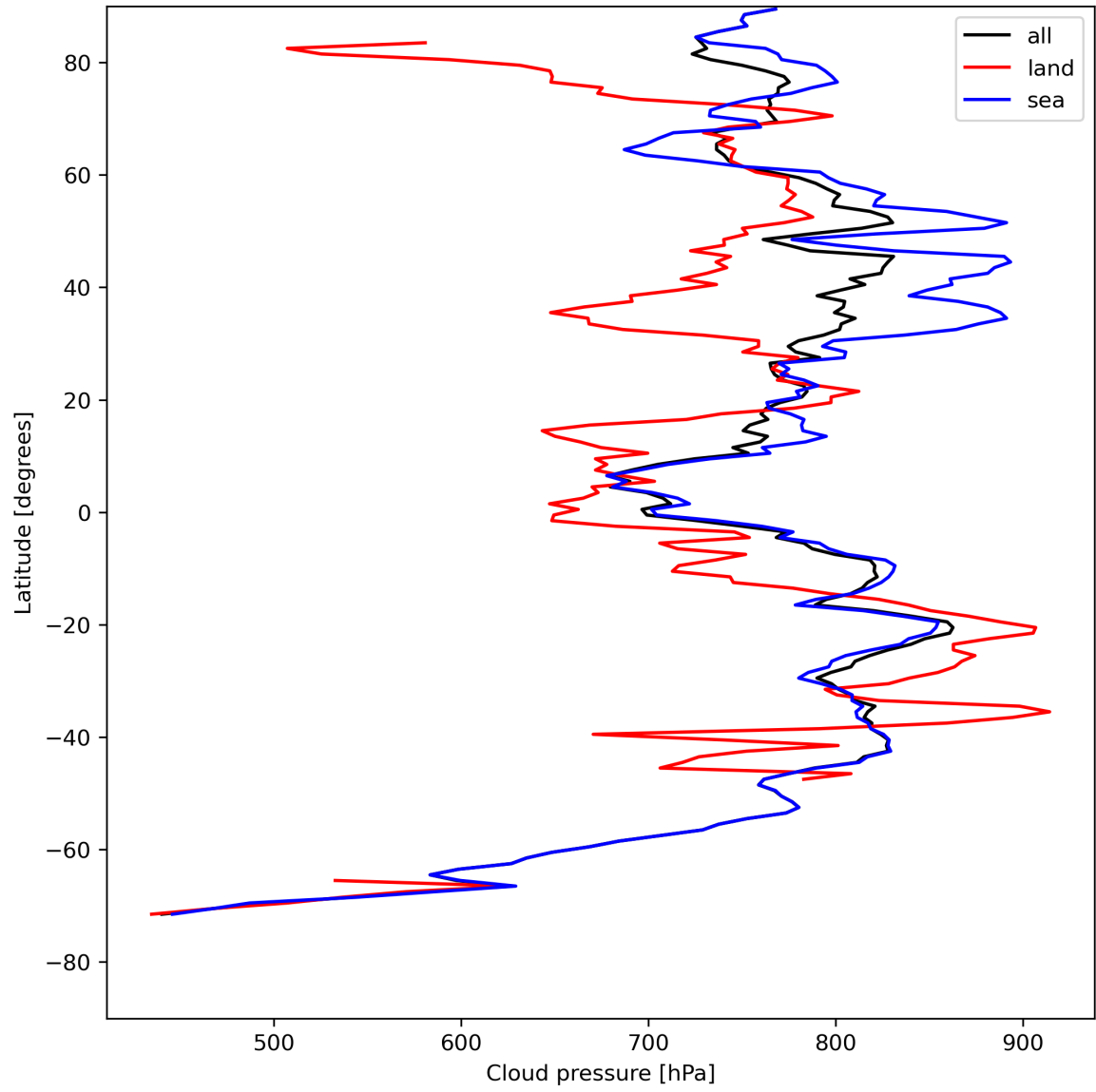
Figure 13: Zonal average of “Cloud pressure” for 2023-08-06 to 2023-08-08.
