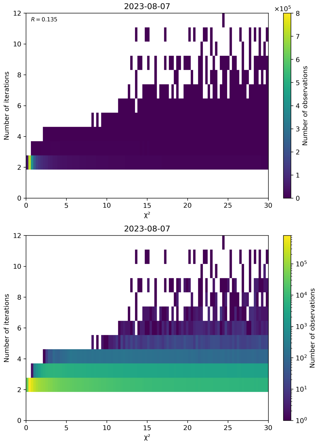
Figure 73: Scatter density plot of “ \chi^2 ” against “Number of iterations” for 2023-08-06 to 2023-08-08.
