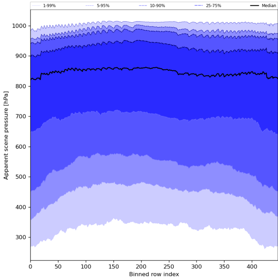
Figure 53: Along track statistics of “Apparent scene pressure” for 2023-08-06 to 2023-08-08
