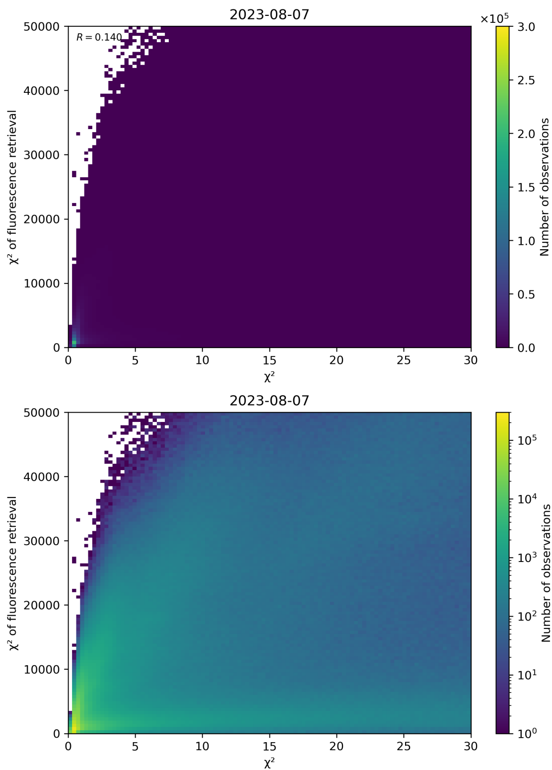
Figure 69: Scatter density plot of “ \chi^2 ” against “ \chi^2 of fluorescence retrieval” for 2023-08-06 to 2023-08-08.
