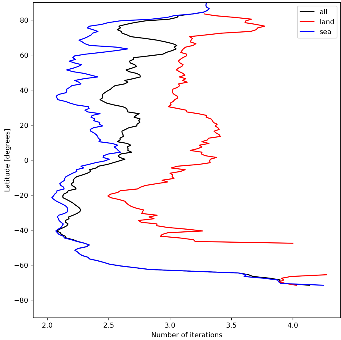
Figure 22: Zonal average of “Number of iterations” for 2023-08-06 to 2023-08-08.
