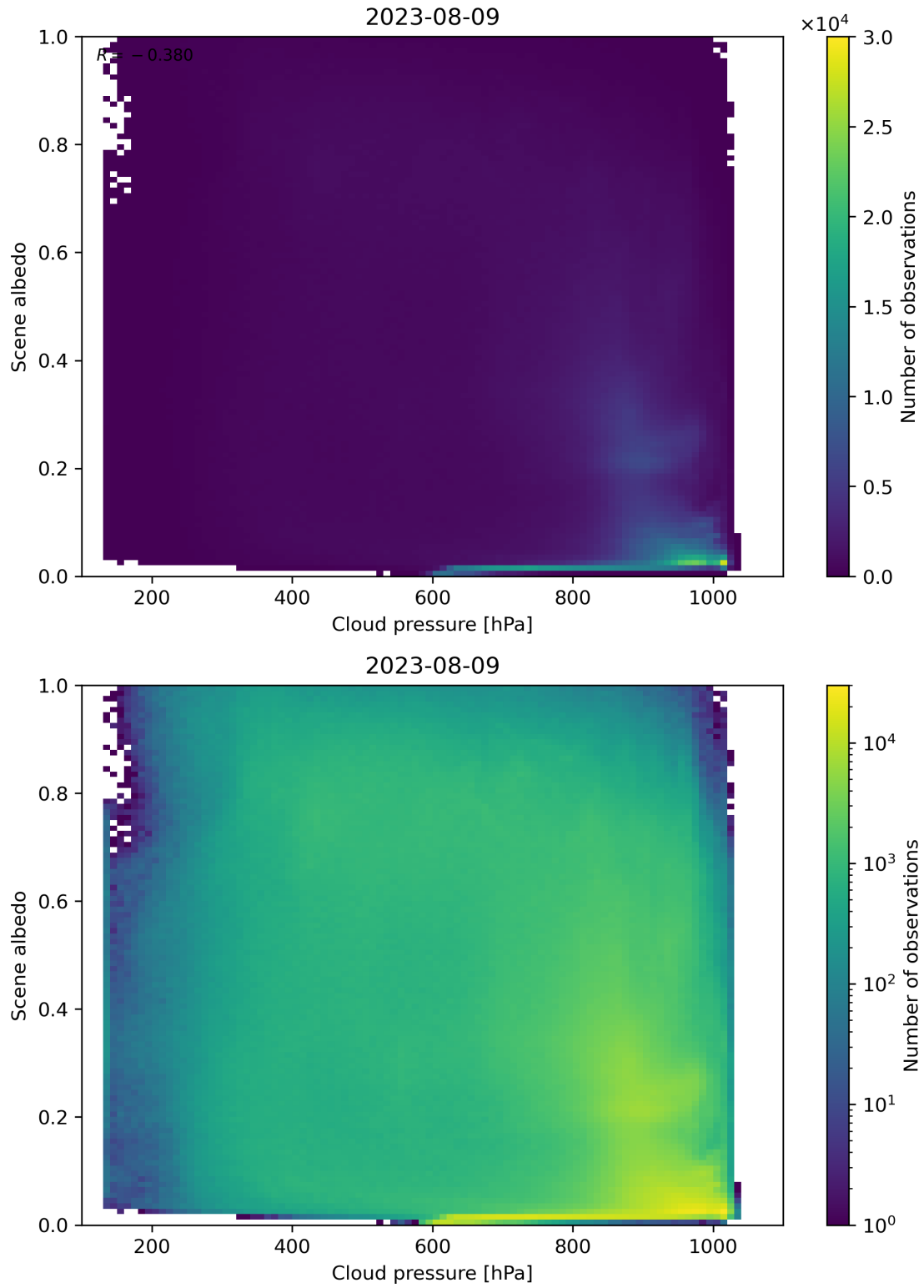
Figure 91: Scatter density plot of “Cloud pressure” against “Scene albedo” for 2023-08-09 to 2023-08-10.
