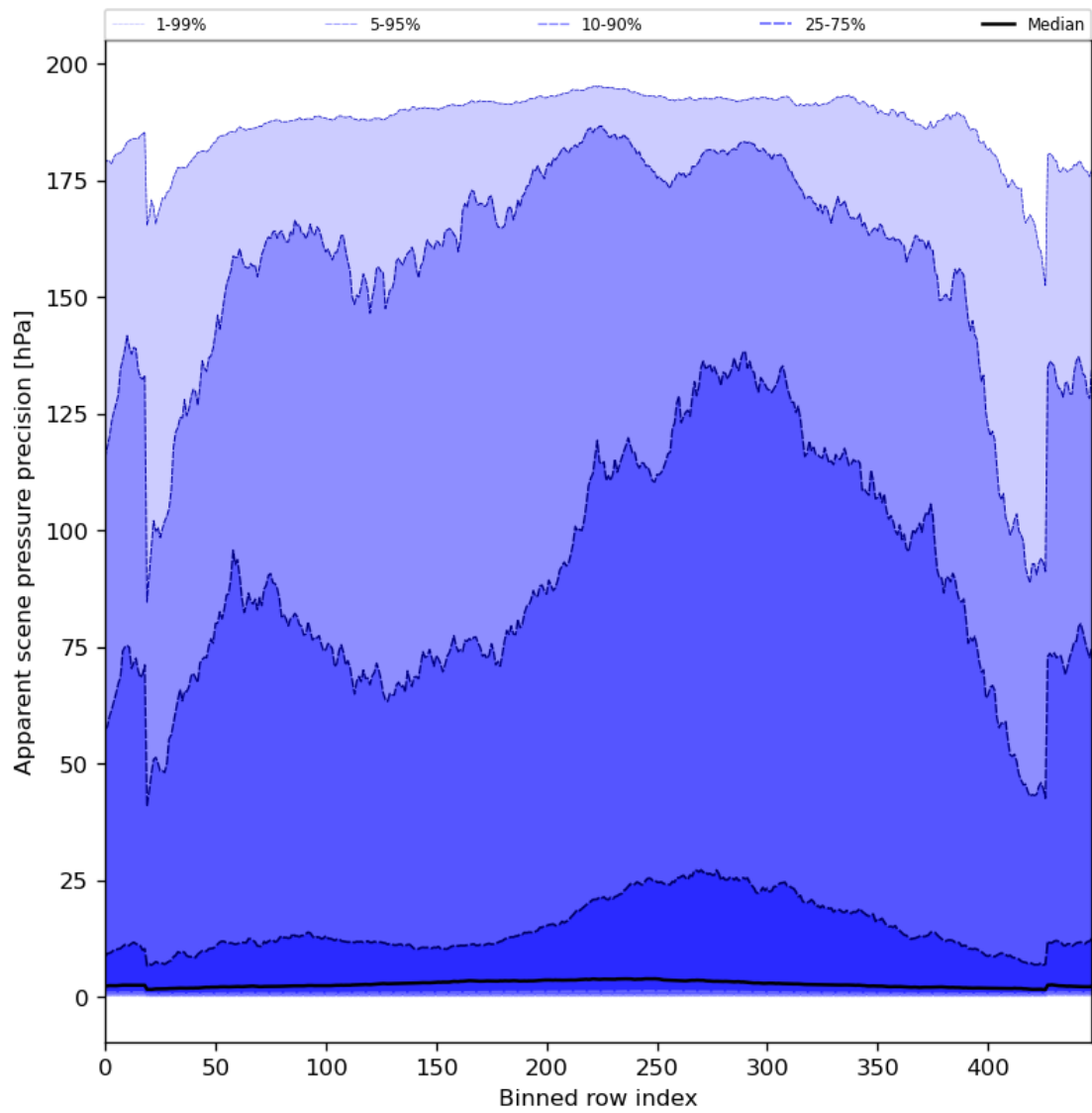
Figure 54: Along track statistics of “Apparent scene pressure precision” for 2023-08-09 to 2023-08-10
