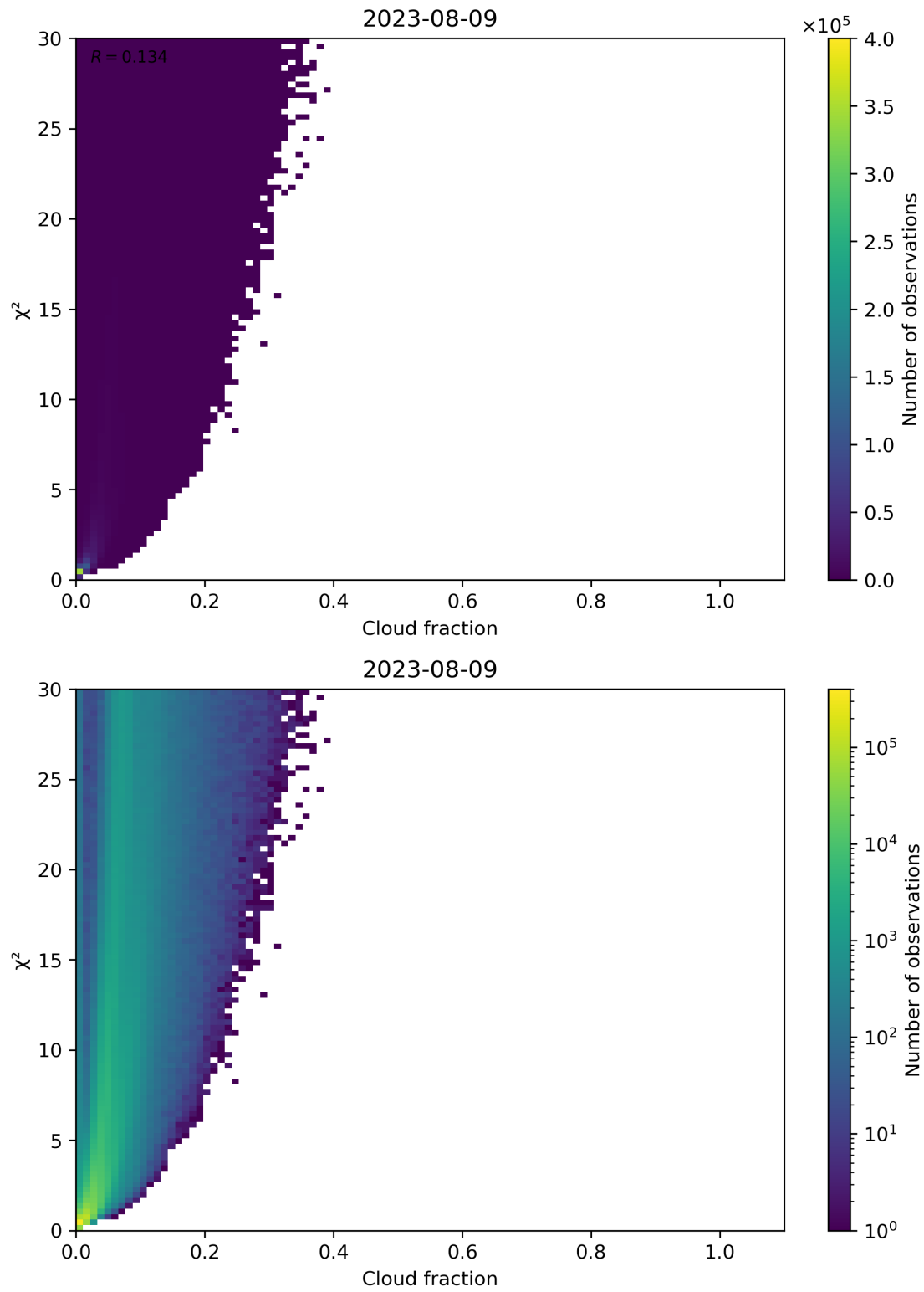
Figure 77: Scatter density plot of “Cloud fraction” against “ \chi^2 ” for 2023-08-09 to 2023-08-10.
