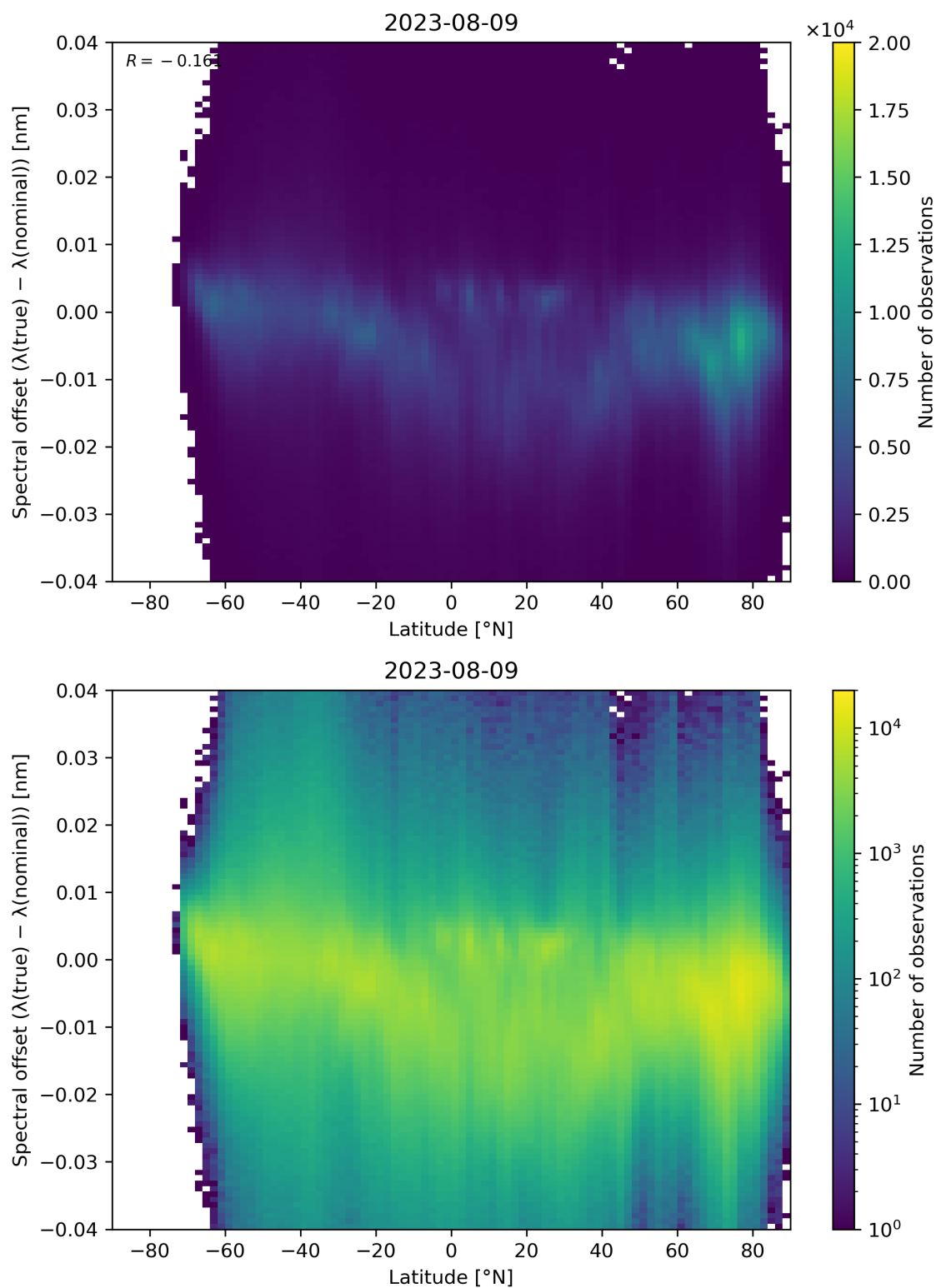
Figure 105: Scatter density plot of “Latitude” against “Spectral offset ( \lambda(\text{true}) - \lambda(\text{nominal}) )” for 2023-08-09 to 2023-08-10.
