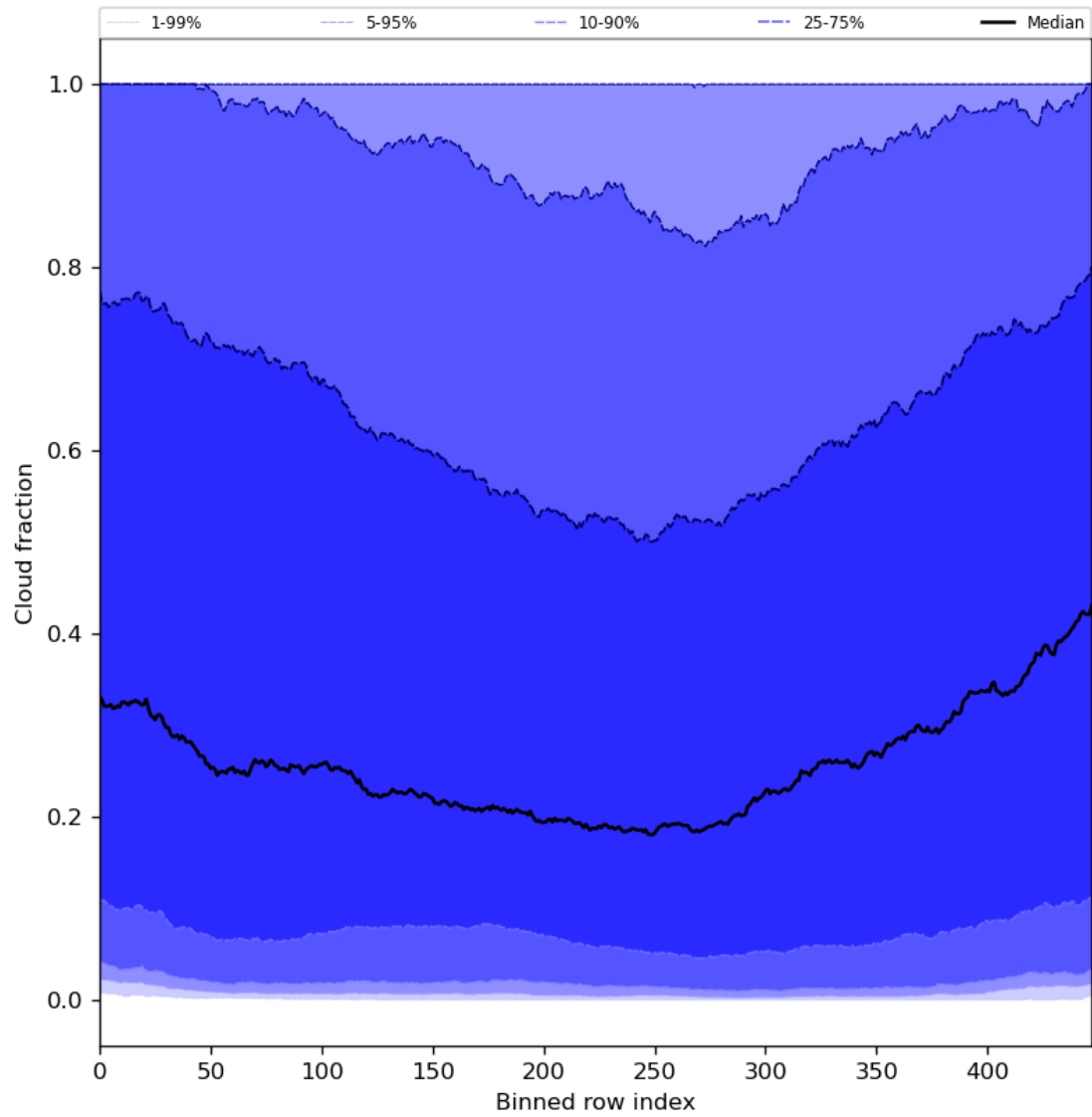
Figure 49: Along track statistics of “Cloud fraction” for 2023-08-09 to 2023-08-10
