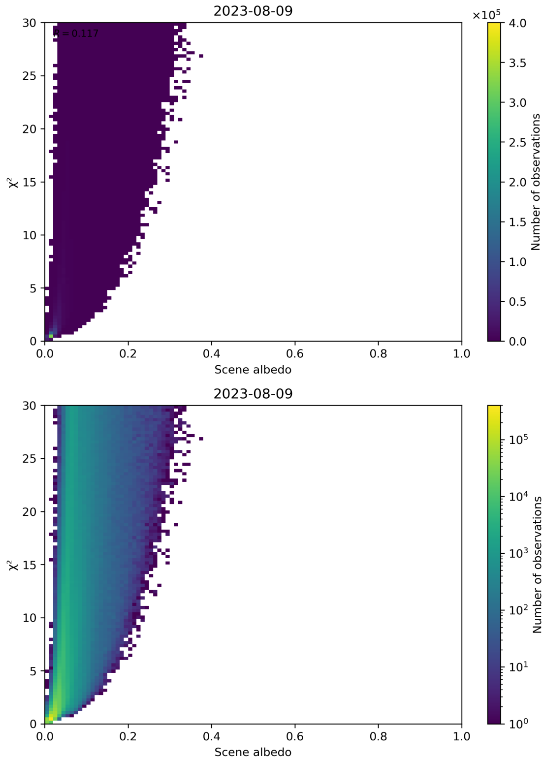
Figure 112: Scatter density plot of “Scene albedo” against “ \chi^2 ” for 2023-08-09 to 2023-08-10.
