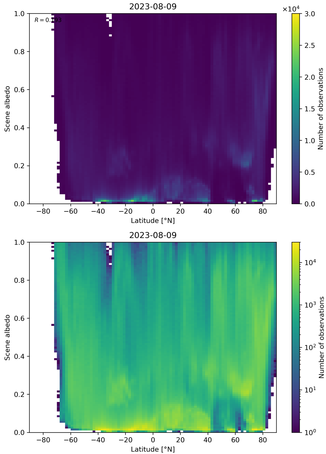
Figure 104: Scatter density plot of “Latitude” against “Scene albedo” for 2023-08-09 to 2023-08-10.
