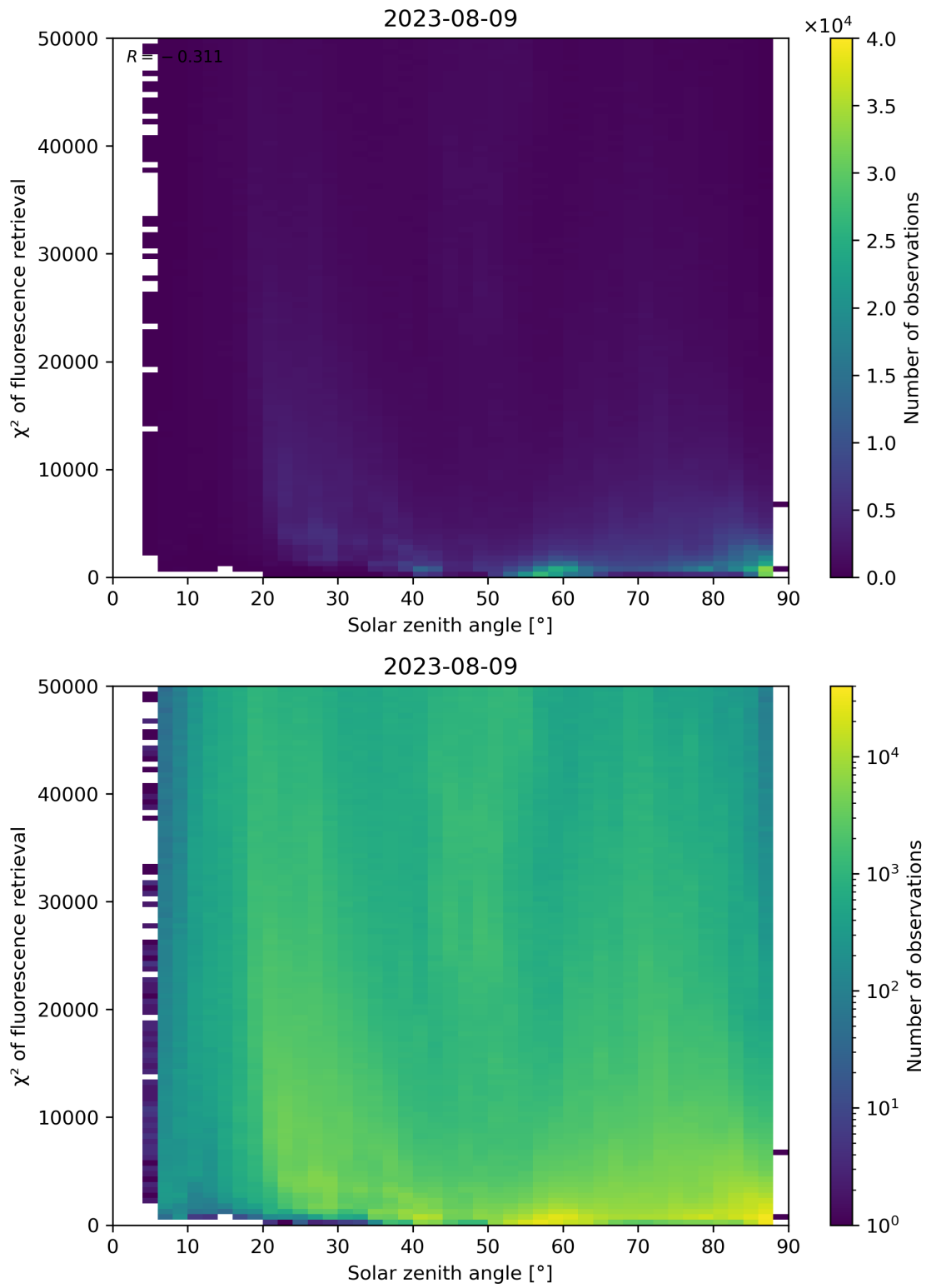
Figure 120: Scatter density plot of “Solar zenith angle” against “ \chi^2 of fluorescence retrieval” for 2023-08-09 to 2023-08-10.
