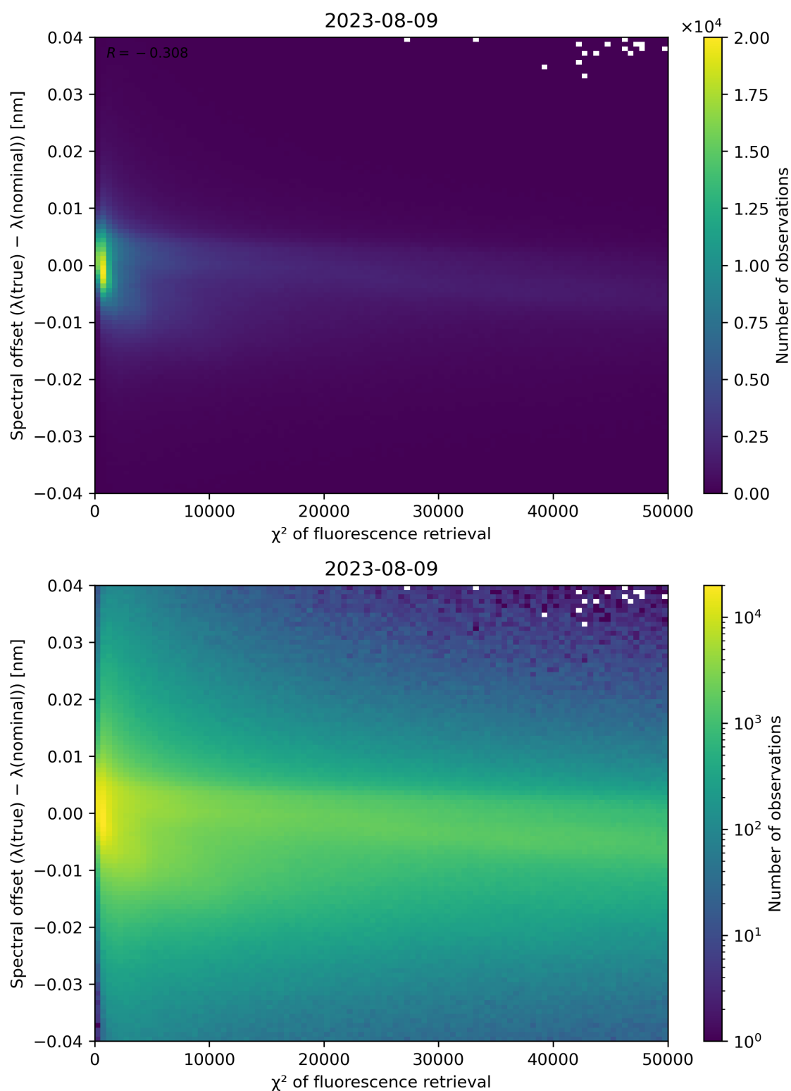
Figure 72: Scatter density plot of " \chi^2 of fluorescence retrieval" against "Spectral offset ( \lambda(\text{true}) - \lambda(\text{nominal})) " for 2023-08-09 to 2023-08-10.
