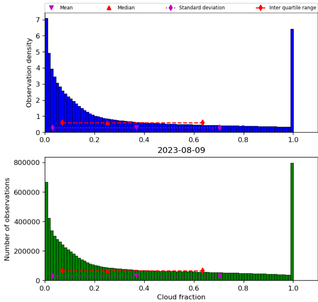
Figure 32: Histogram of “Cloud fraction” for 2023-08-09 to 2023-08-10
