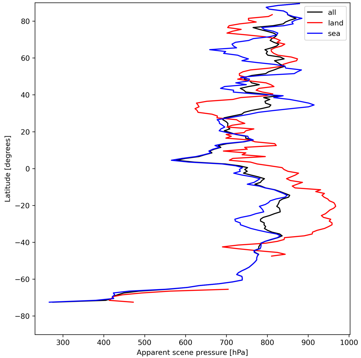
Figure 19: Zonal average of “Apparent scene pressure” for 2023-08-09 to 2023-08-10.
