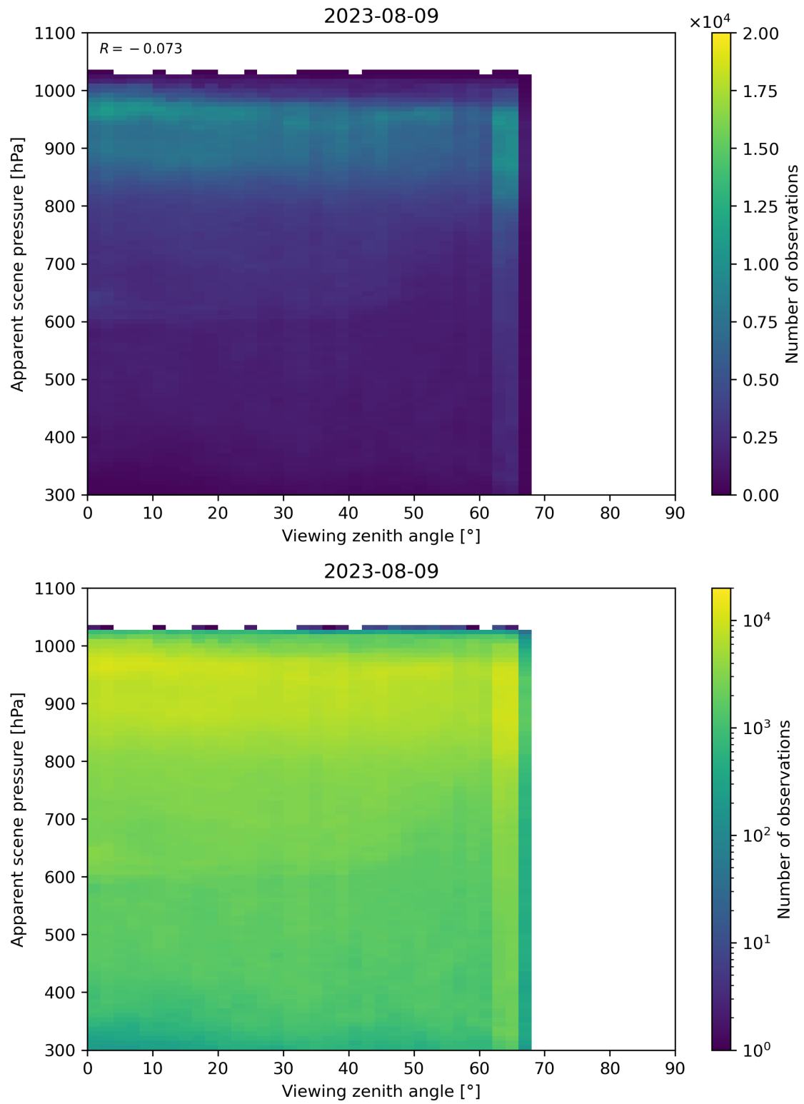
Figure 129: Scatter density plot of “Viewing zenith angle” against “Apparent scene pressure” for 2023-08-09 to 2023-08-10.
