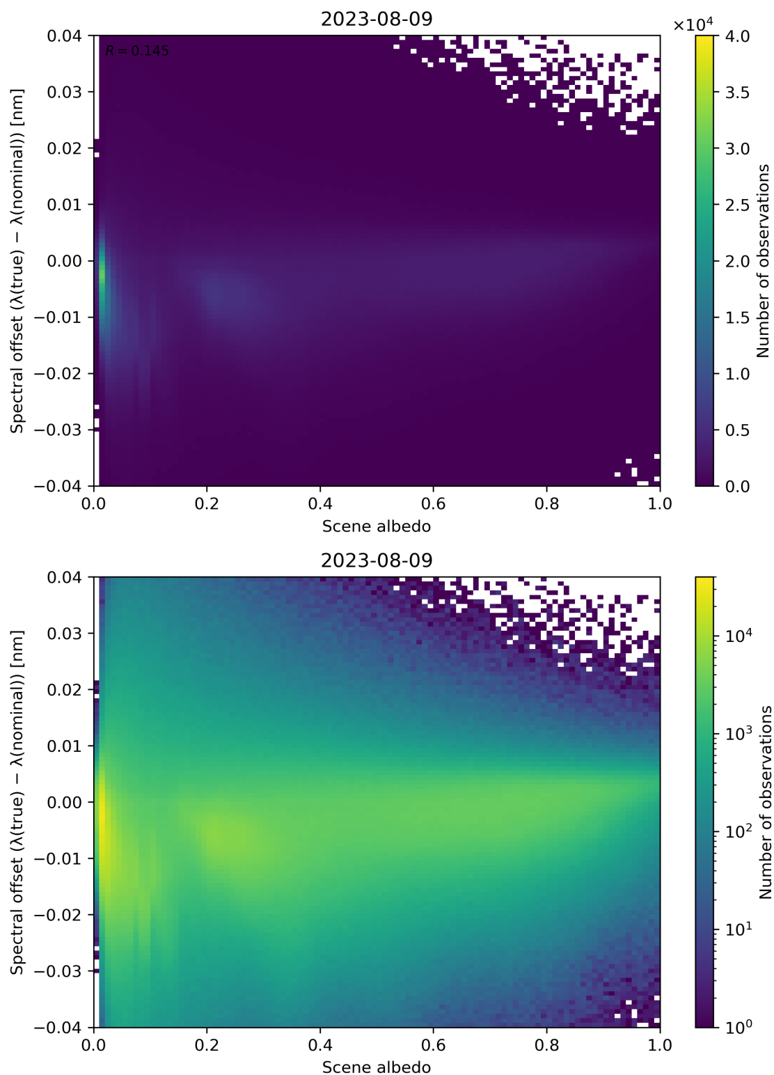
Figure 117: Scatter density plot of “Scene albedo” against “Spectral offset ( \lambda(\text{true}) - \lambda(\text{nominal}) )” for 2023-08-09 to 2023-08-10.
