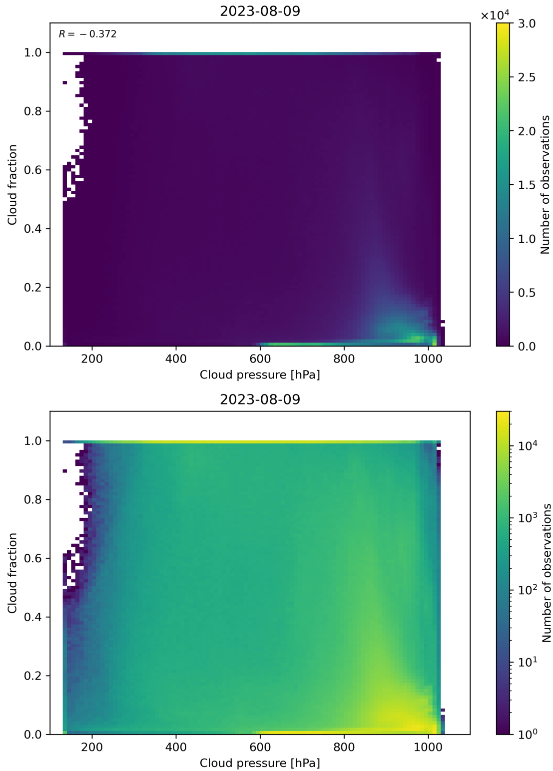
Figure 87: Scatter density plot of “Cloud pressure” against “Cloud fraction” for 2023-08-09 to 2023-08-10.
