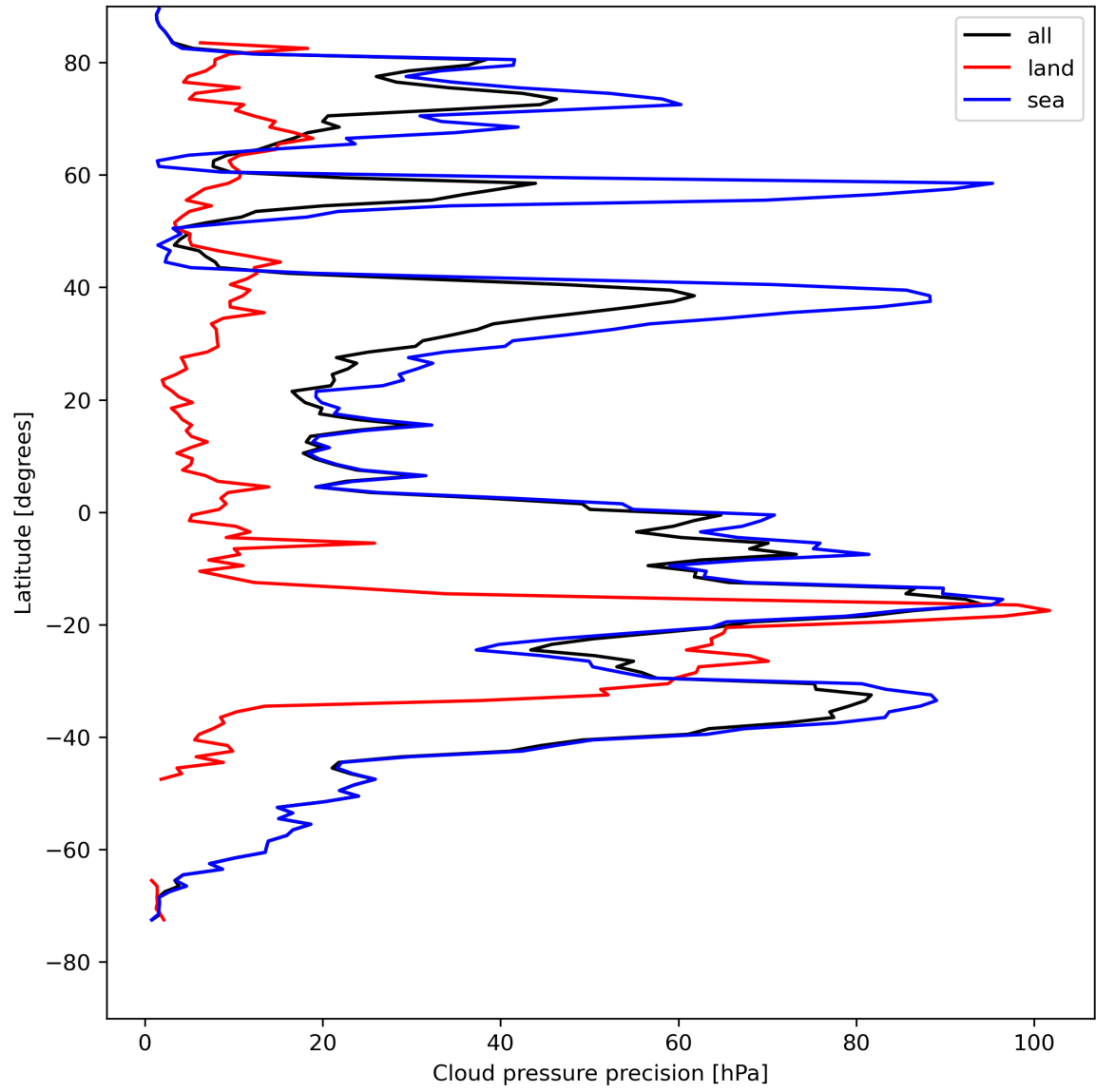
Figure 14: Zonal average of “Cloud pressure precision” for 2023-08-09 to 2023-08-10.
