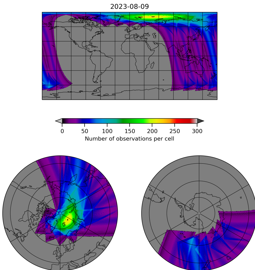
Figure 11: Map of the number of observations for 2023-08-09 to 2023-08-10
