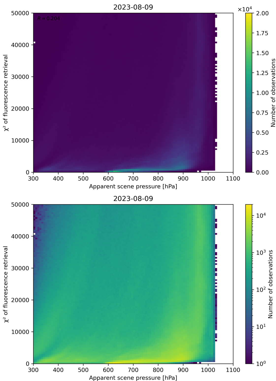
Figure 64: Scatter density plot of “Apparent scene pressure” against “ \chi^2 of fluorescence retrieval” for 2023-08-09 to 2023-08-10.
