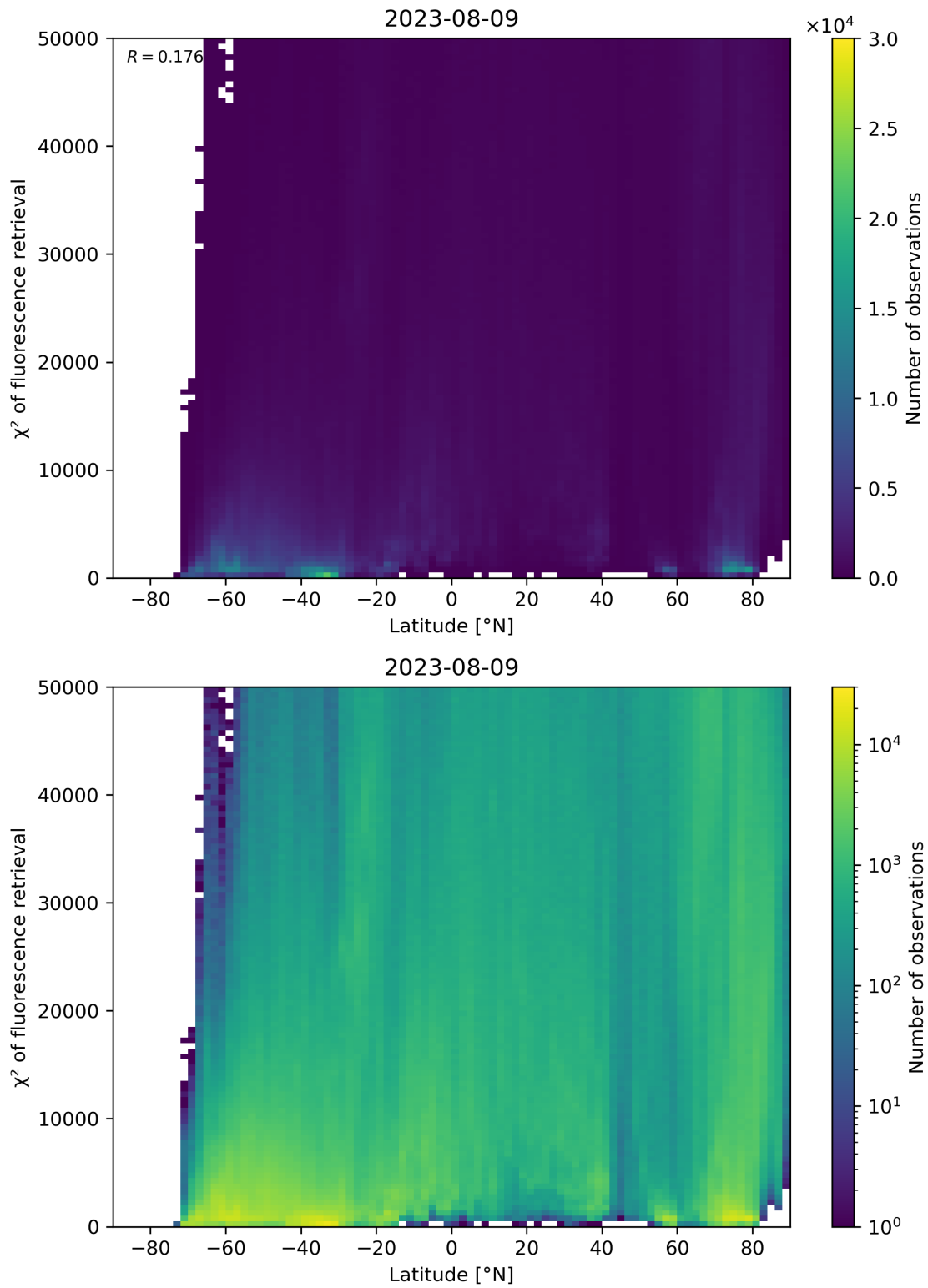
Figure 98: Scatter density plot of “Latitude” against “ \chi^2 of fluorescence retrieval” for 2023-08-09 to 2023-08-10.
