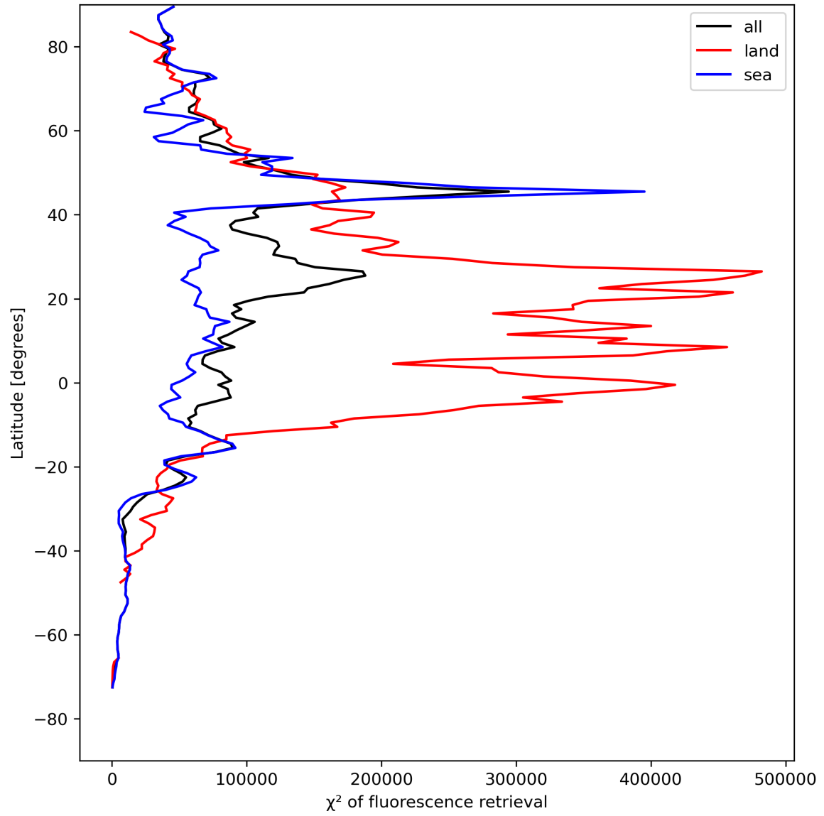
Figure 25: Zonal average of “ \chi^2 of fluorescence retrieval” for 2023-08-09 to 2023-08-10.
