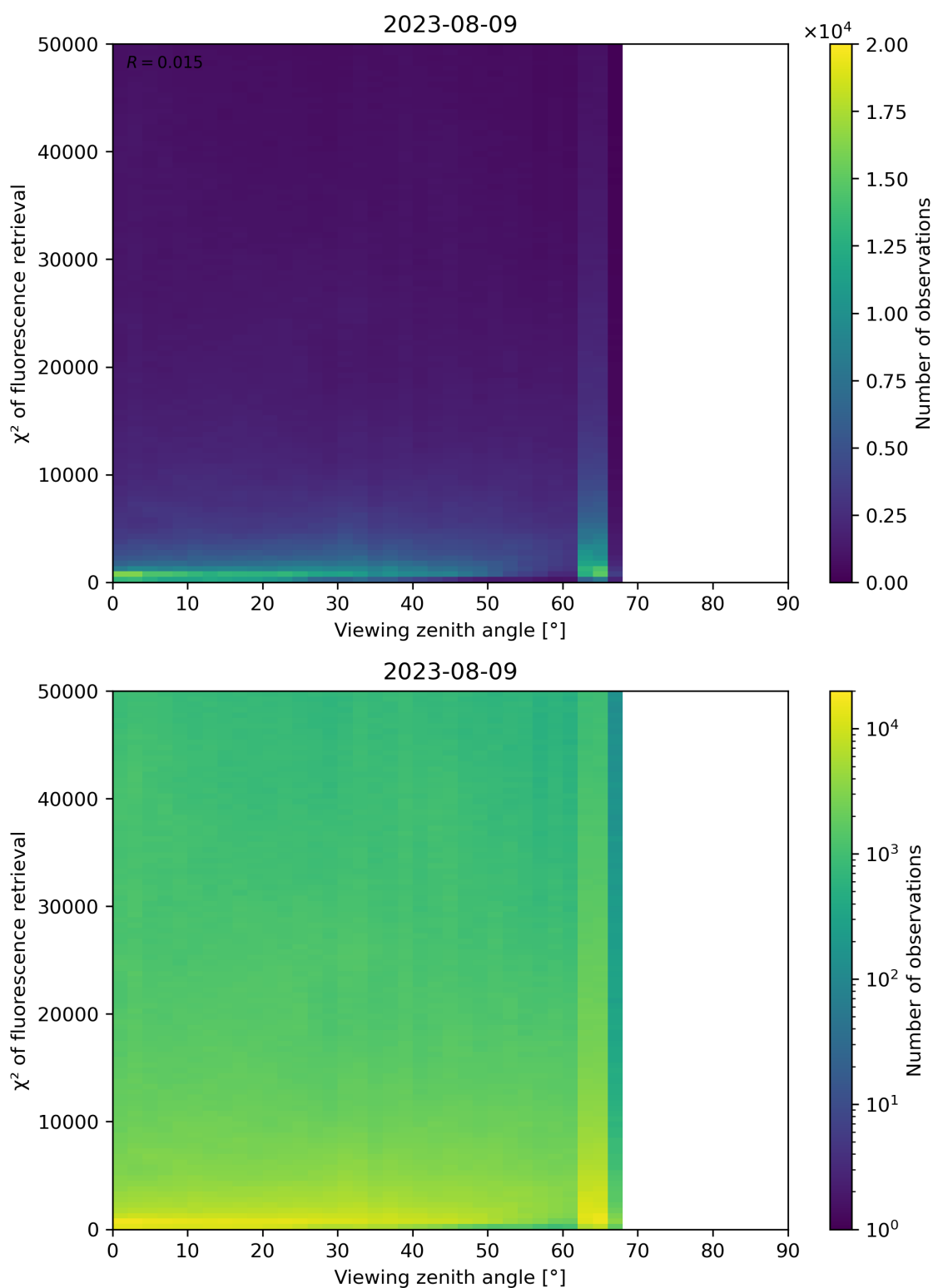
Figure 131: Scatter density plot of “Viewing zenith angle” against “ \chi^2 of fluorescence retrieval” for 2023-08-09 to 2023-08-10.
