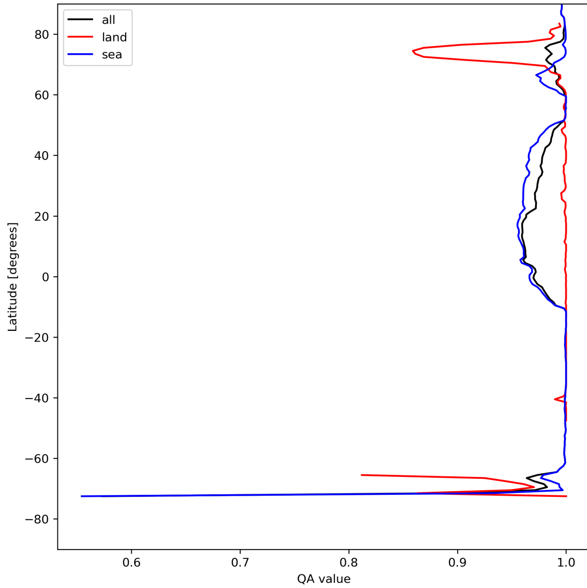
Figure 12: Zonal average of “QA value” for 2023-08-09 to 2023-08-10.
