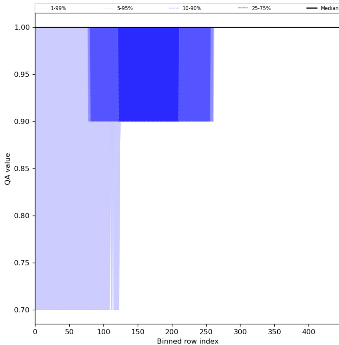
Figure 46: Along track statistics of “QA value” for 2023-08-09 to 2023-08-10
