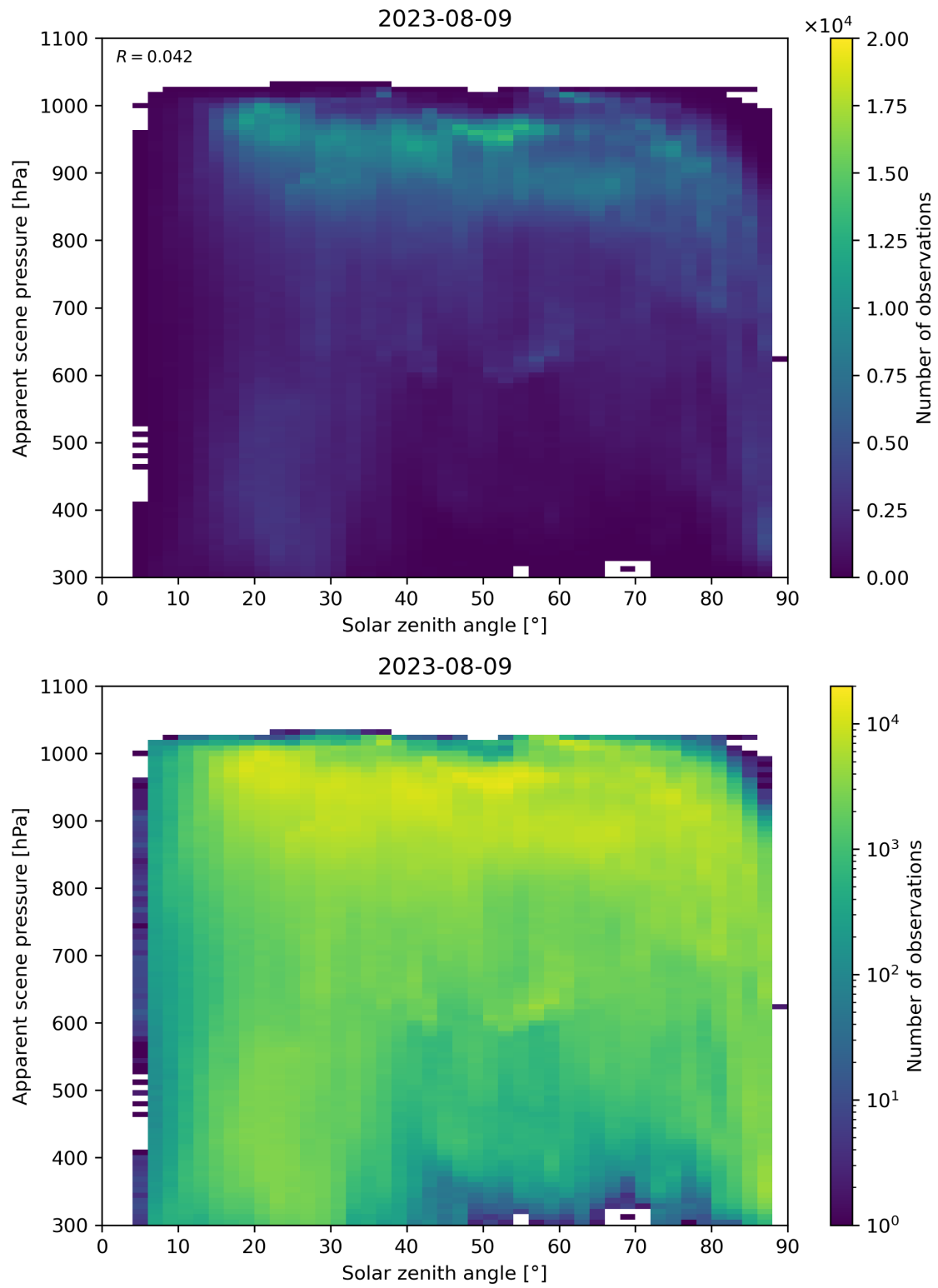
Figure 118: Scatter density plot of “Solar zenith angle” against “Apparent scene pressure” for 2023-08-09 to 2023-08-10.
