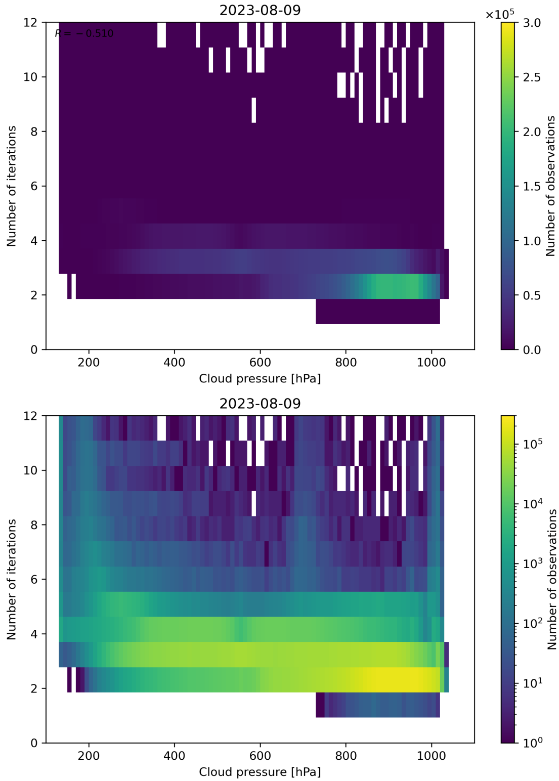
Figure 89: Scatter density plot of “Cloud pressure” against “Number of iterations” for 2023-08-09 to 2023-08-10.
