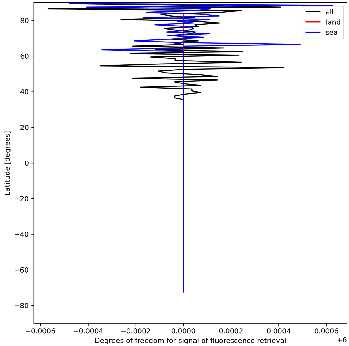
Figure 26: Zonal average of “Degrees of freedom for signal of fluorescence retrieval” for 2023-08-09 to 2023-08-10.
