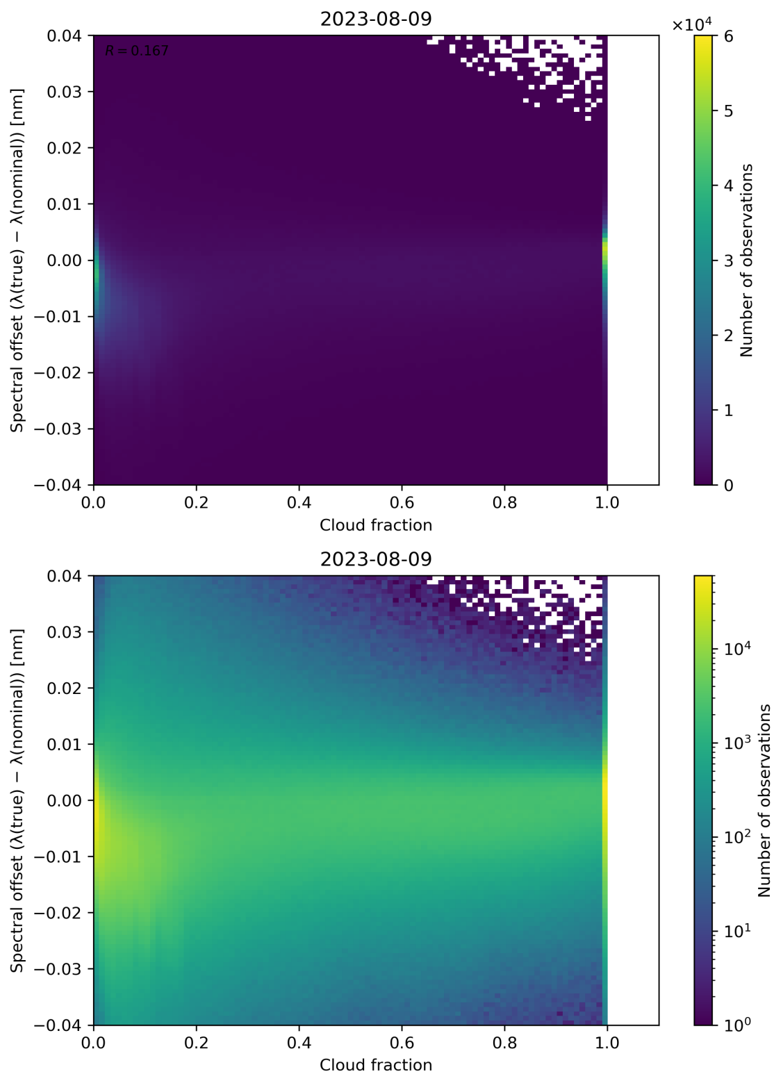
Figure 83: Scatter density plot of “Cloud fraction” against “Spectral offset ( \lambda(\text{true}) - \lambda(\text{nominal}) )” for 2023-08-09 to 2023-08-10.
