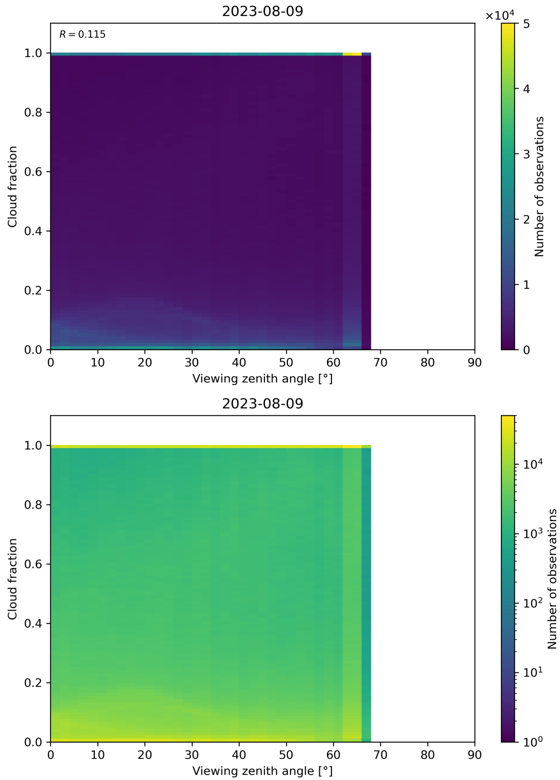
Figure 132: Scatter density plot of “Viewing zenith angle” against “Cloud fraction” for 2023-08-09 to 2023-08-10.
