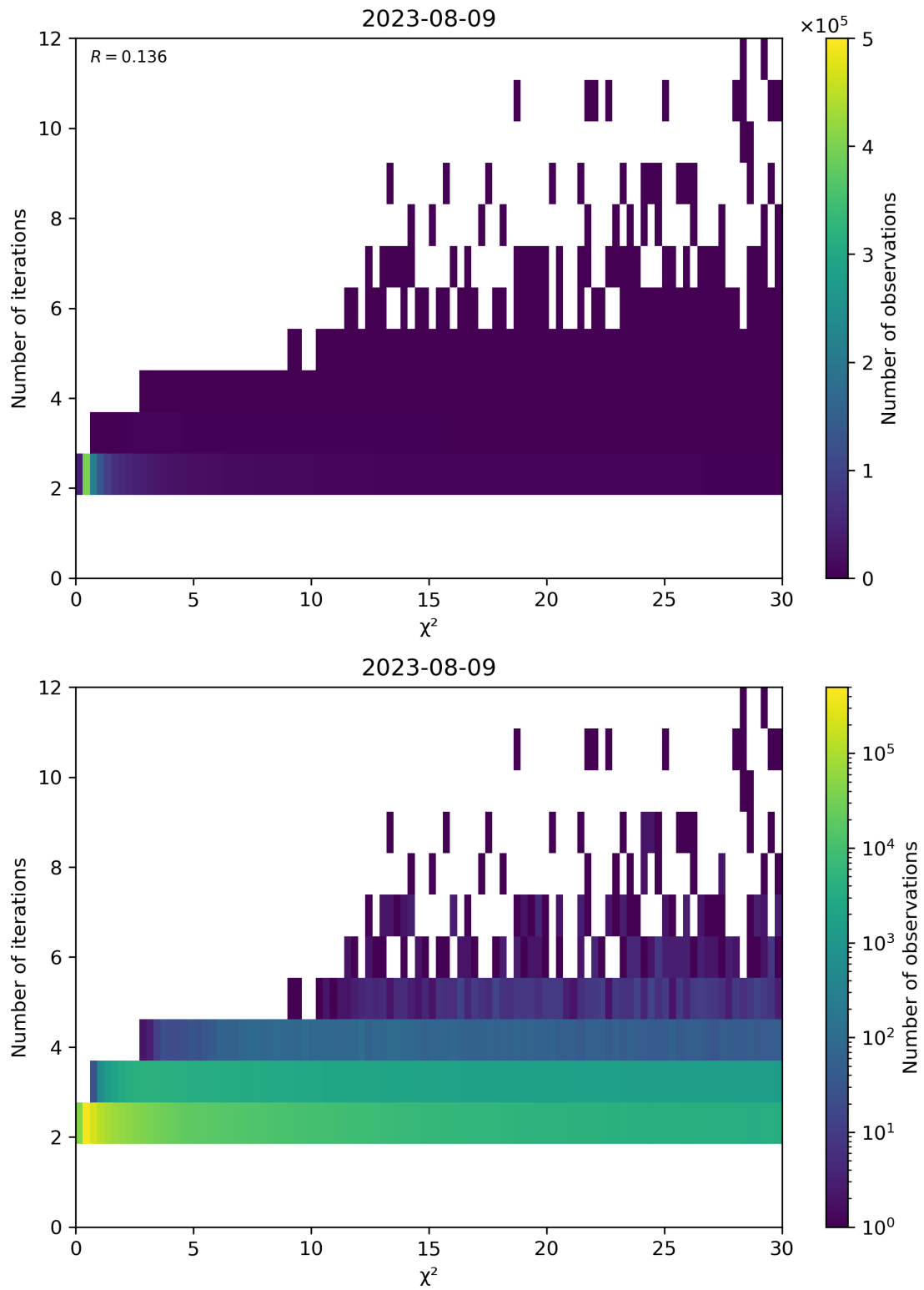
Figure 73: Scatter density plot of “ \chi^2 ” against “Number of iterations” for 2023-08-09 to 2023-08-10.
