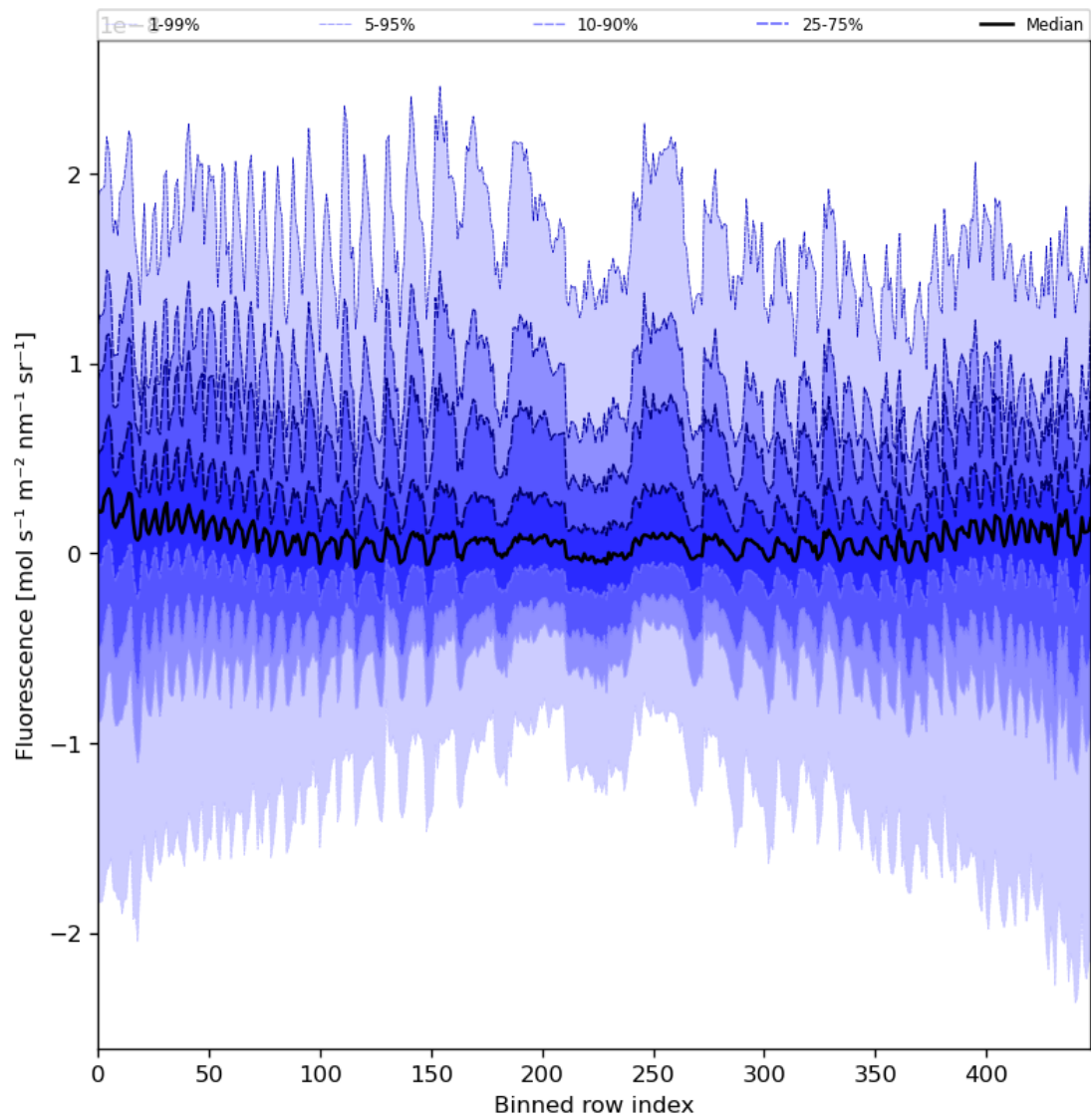
Figure 57: Along track statistics of “Fluorescence” for 2023-08-09 to 2023-08-10
