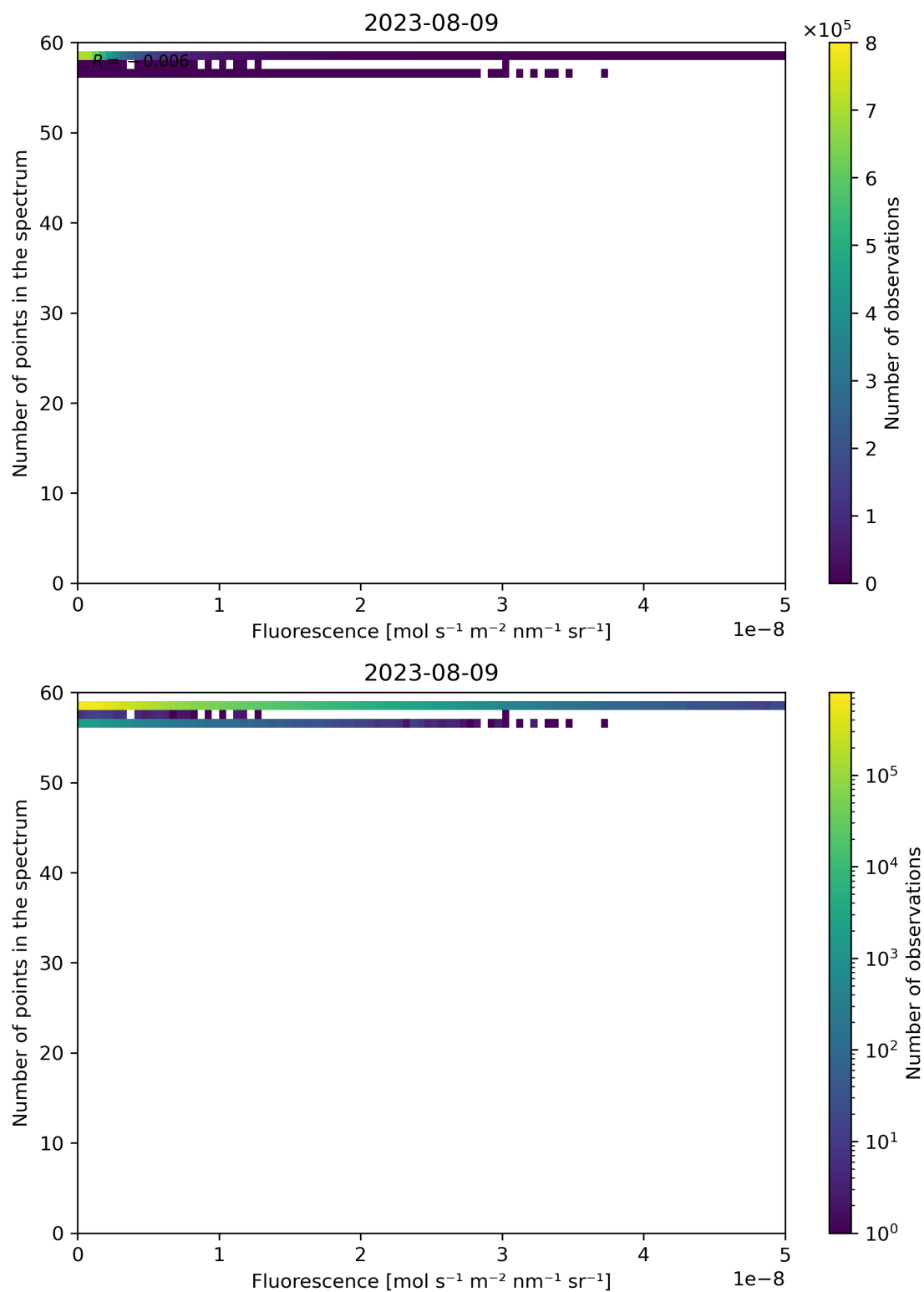
Figure 94: Scatter density plot of “Fluorescence” against “Number of points in the spectrum” for 2023-08-09 to 2023-08-10.
