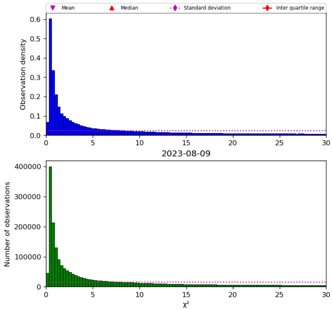
Figure 38: Histogram of " \chi^2 " for 2023-08-09 to 2023-08-10
