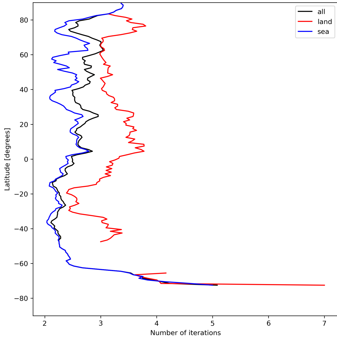
Figure 22: Zonal average of “Number of iterations” for 2023-08-09 to 2023-08-10.
