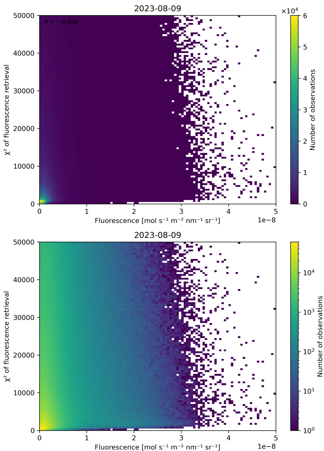
Figure 93: Scatter density plot of “Fluorescence” against “ \chi^2 of fluorescence retrieval” for 2023-08-09 to 2023-08-10.
