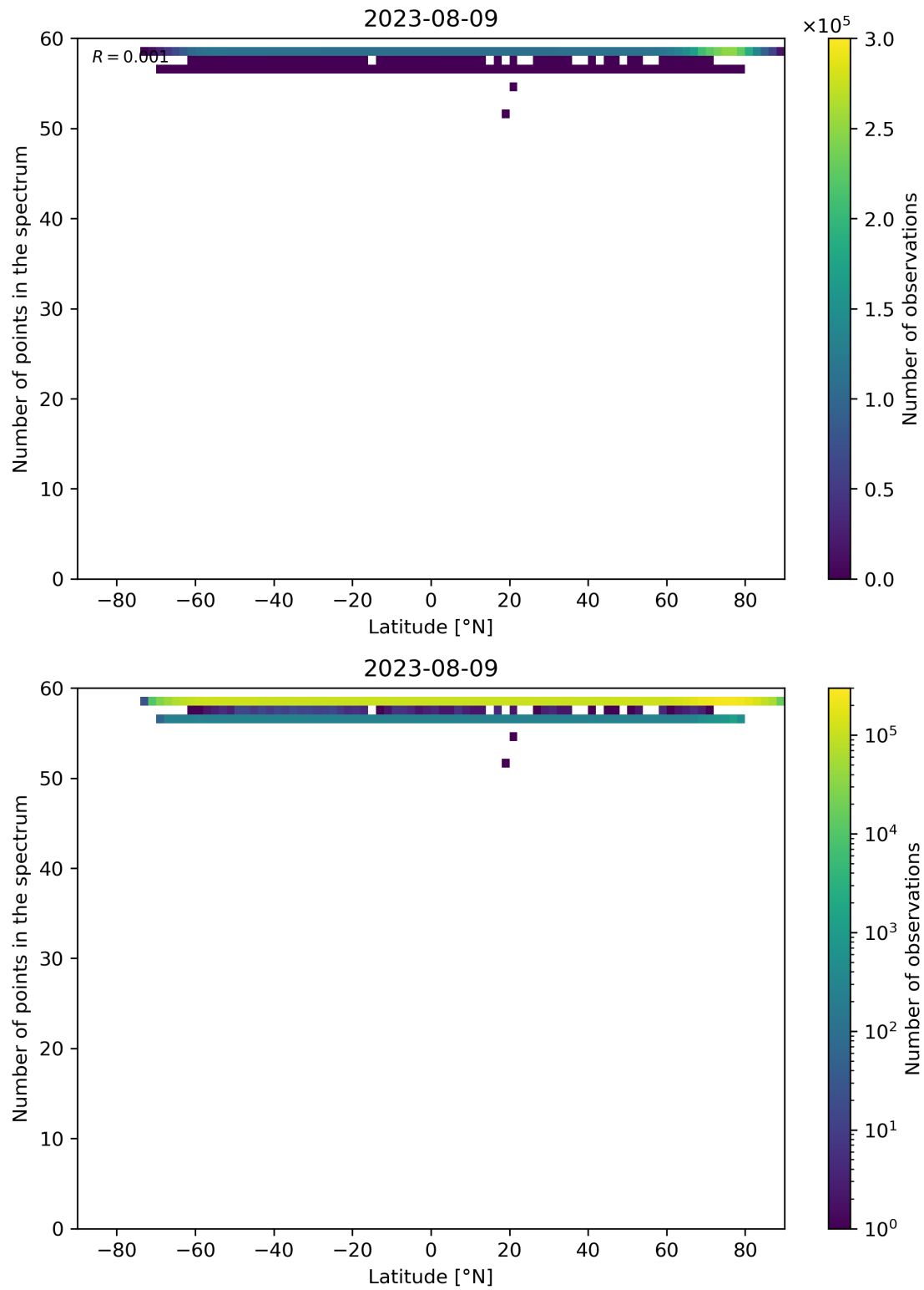
Figure 103: Scatter density plot of “Latitude” against “Number of points in the spectrum” for 2023-08-09 to 2023-08-10.
