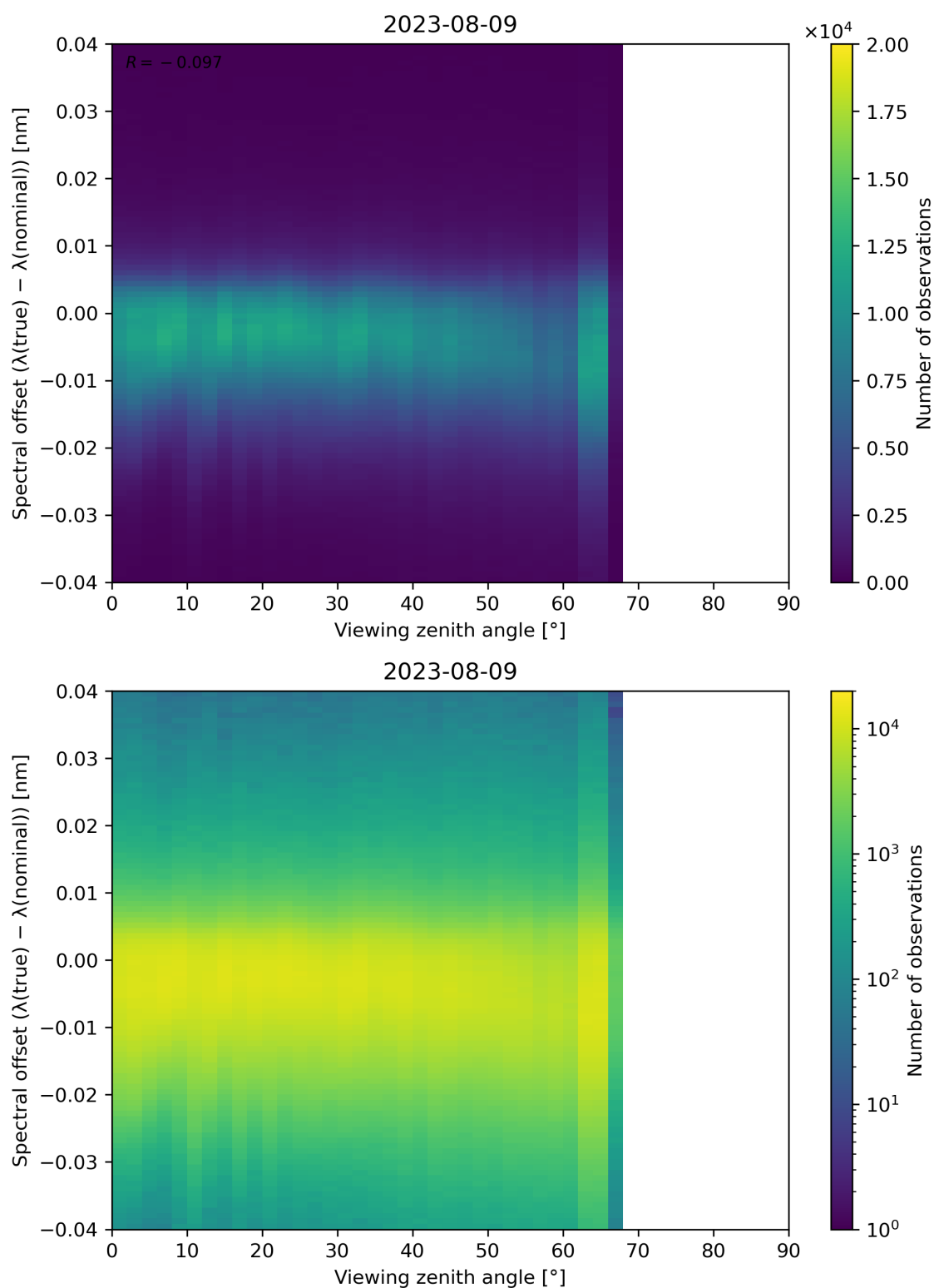
Figure 140: Scatter density plot of “Viewing zenith angle” against “Spectral offset ( \lambda(\text{true}) - \lambda(\text{nominal}) )” for 2023-08-09 to 2023-08-10.
