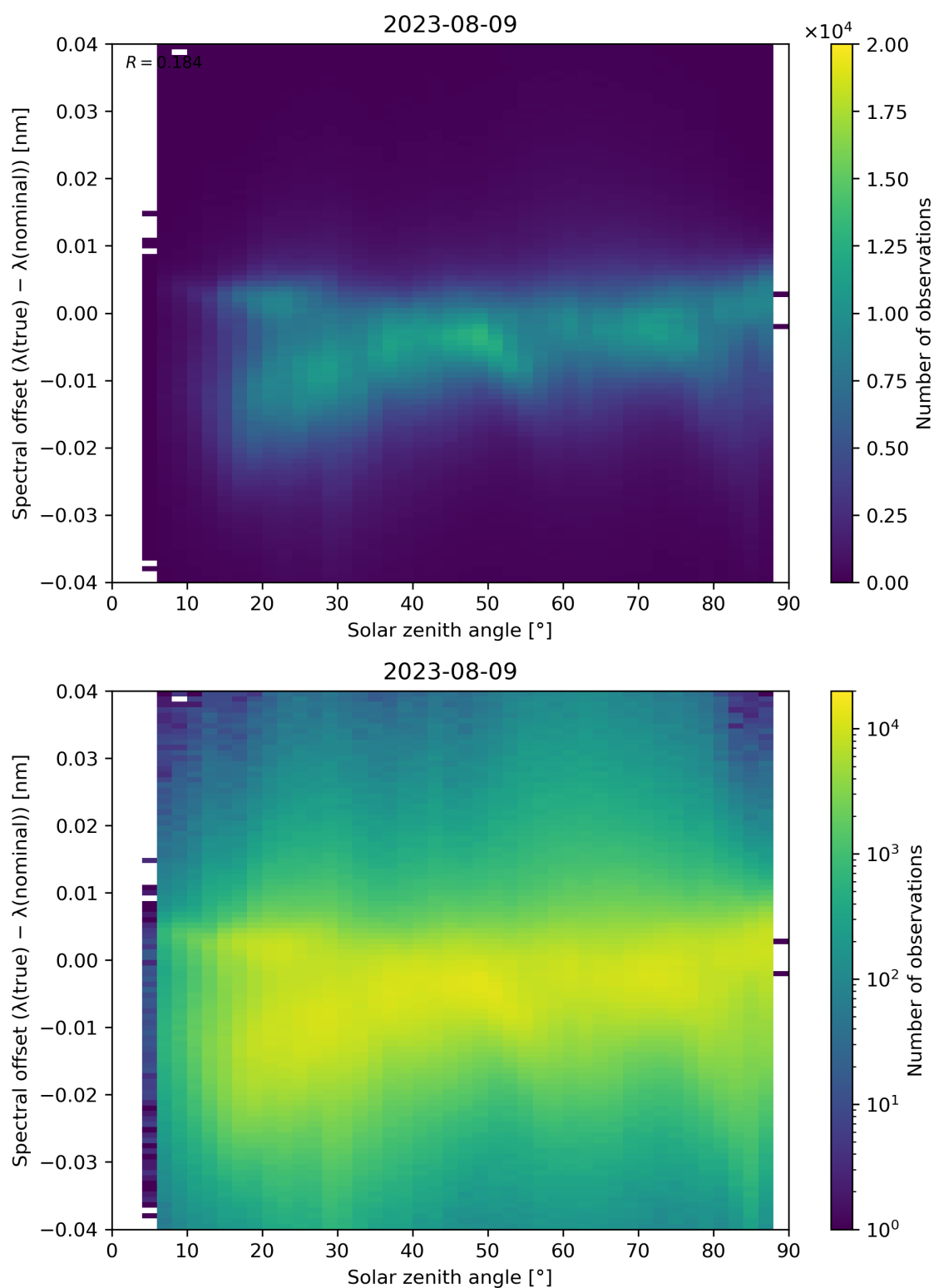
Figure 128: Scatter density plot of “Solar zenith angle” against “Spectral offset ( \lambda(\text{true}) - \lambda(\text{nominal}) )” for 2023-08-09 to 2023-08-10.
