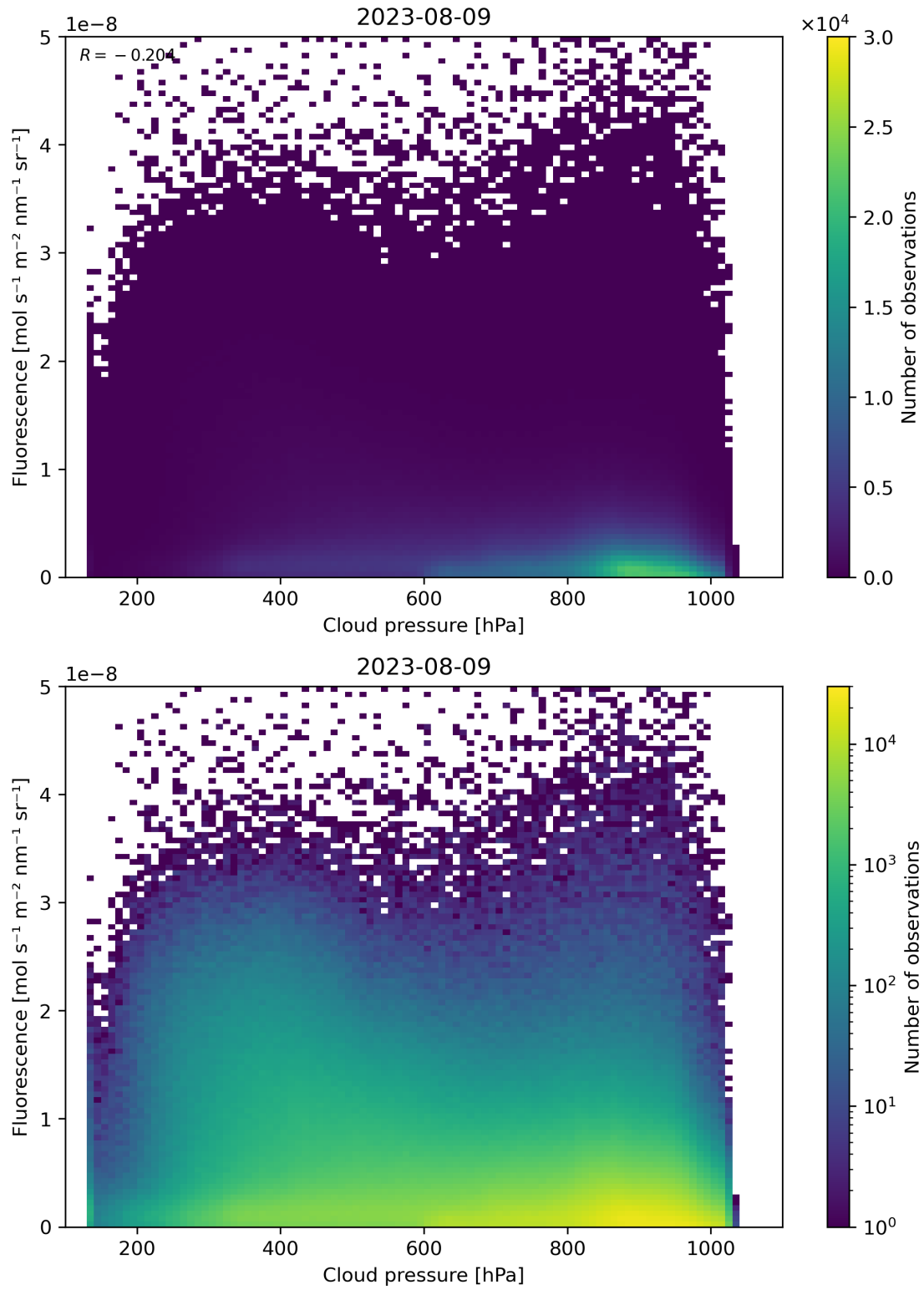
Figure 88: Scatter density plot of “Cloud pressure” against “Fluorescence” for 2023-08-09 to 2023-08-10.
