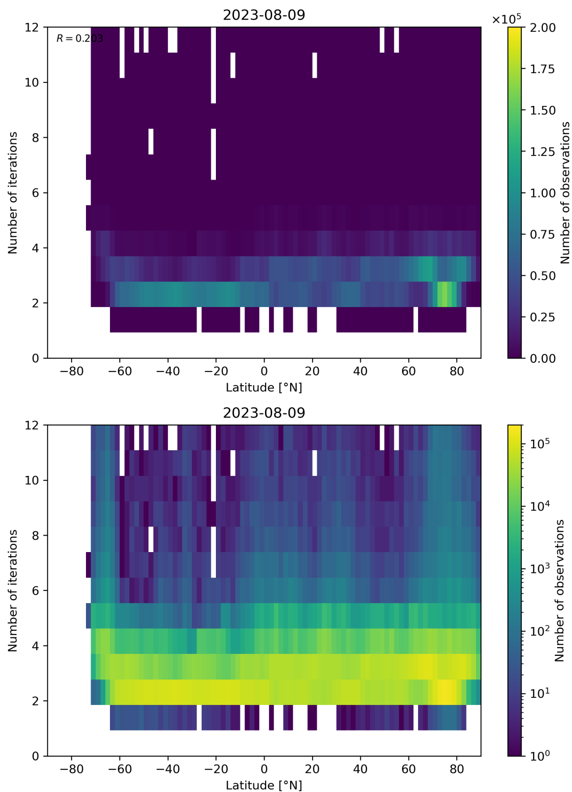
Figure 102: Scatter density plot of “Latitude” against “Number of iterations” for 2023-08-09 to 2023-08-10.
