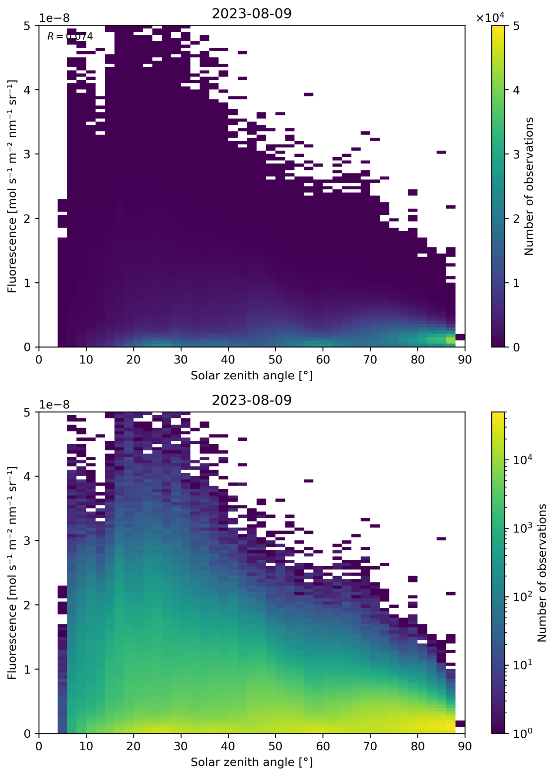
Figure 123: Scatter density plot of “Solar zenith angle” against “Fluorescence” for 2023-08-09 to 2023-08-10.
