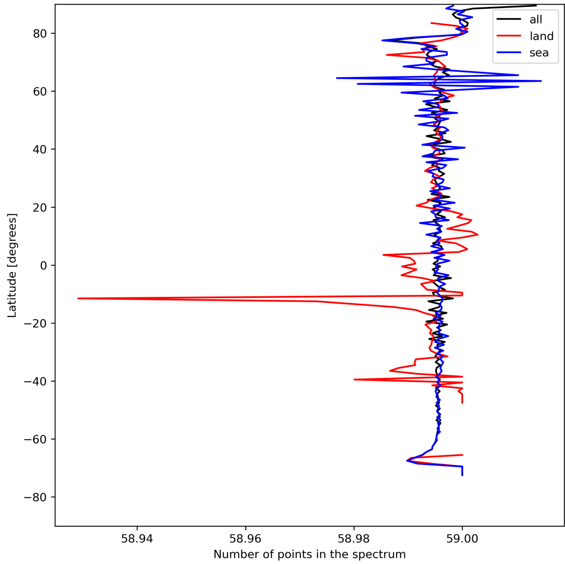
Figure 27: Zonal average of “Number of points in the spectrum” for 2023-08-09 to 2023-08-10.
