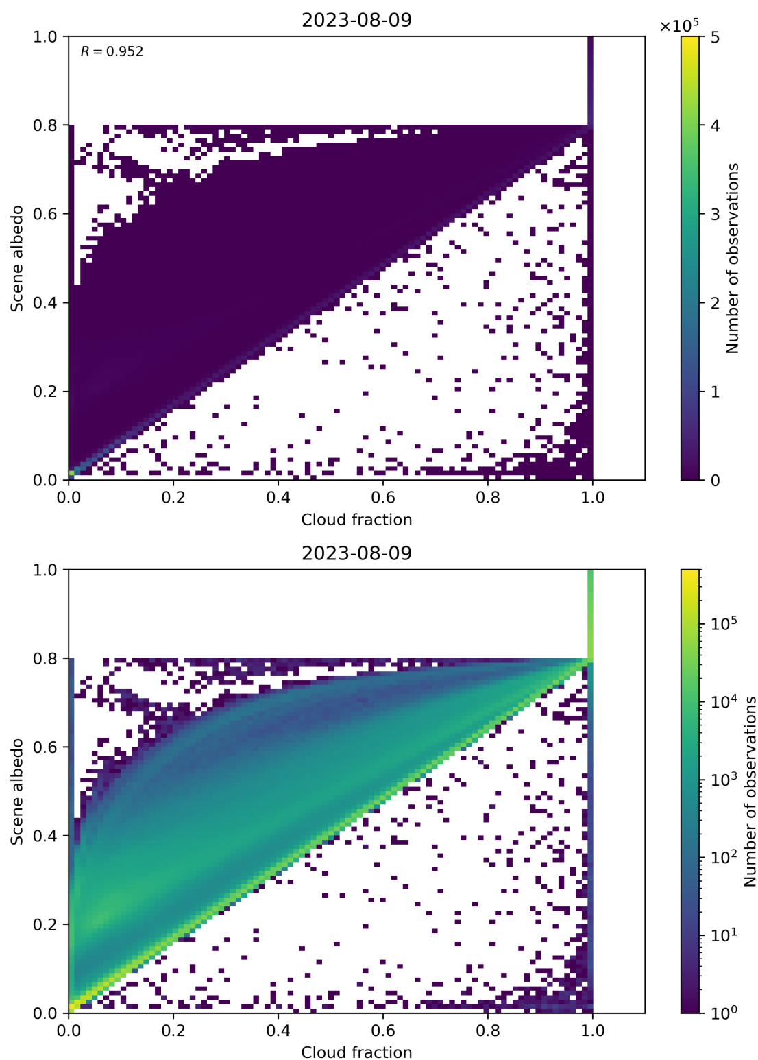
Figure 82: Scatter density plot of “Cloud fraction” against “Scene albedo” for 2023-08-09 to 2023-08-10.
