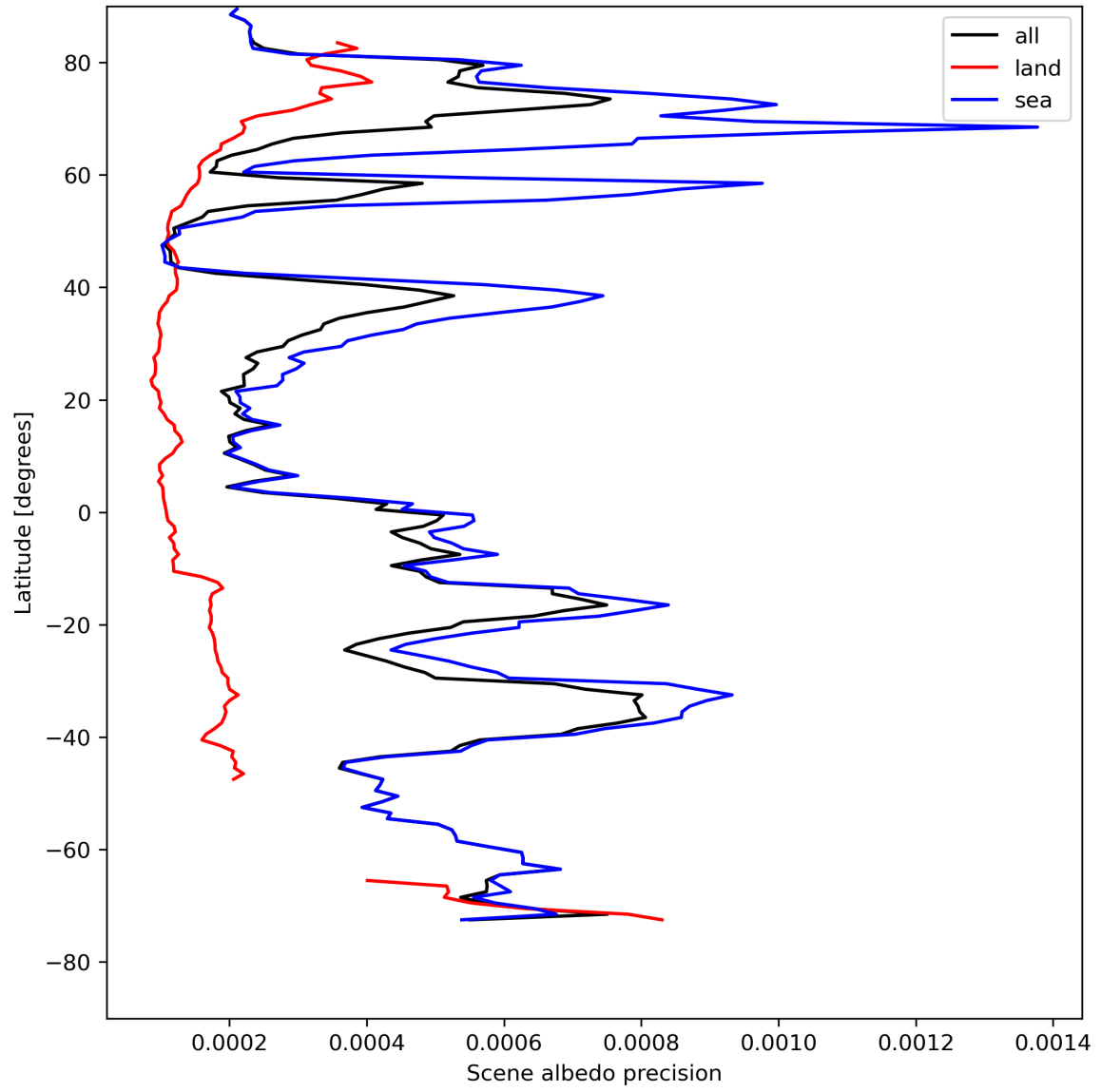
Figure 18: Zonal average of “Scene albedo precision” for 2023-08-09 to 2023-08-10.
