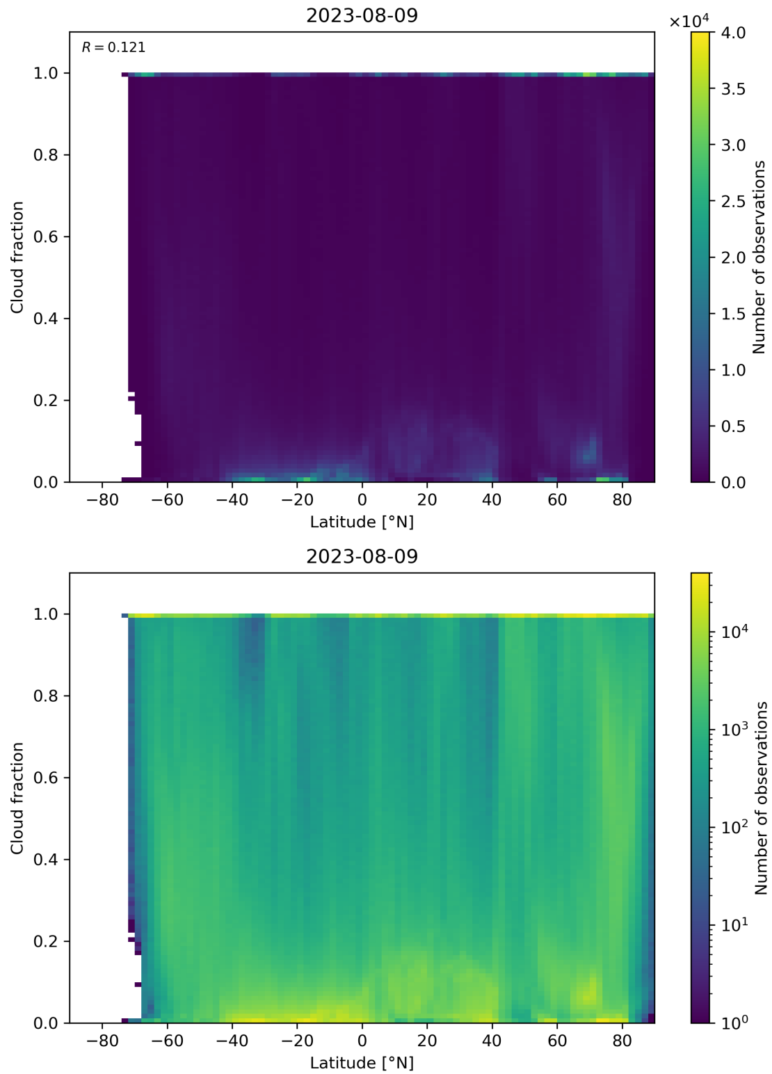
Figure 99: Scatter density plot of “Latitude” against “Cloud fraction” for 2023-08-09 to 2023-08-10.
