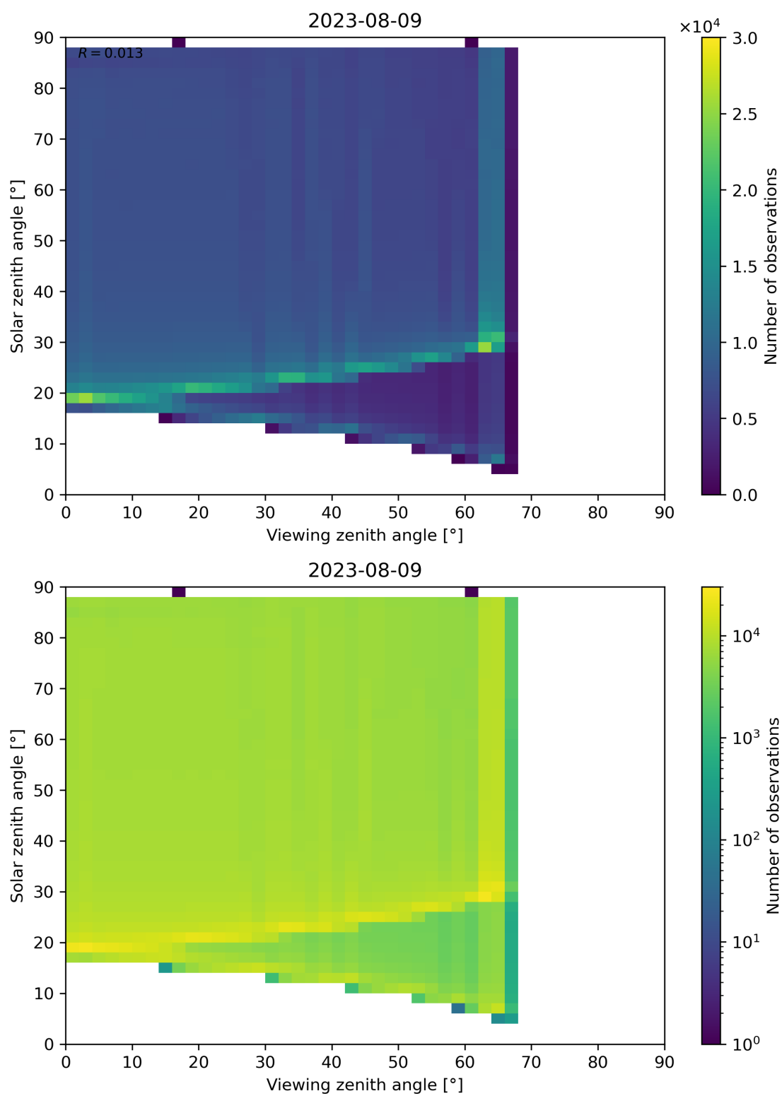
Figure 139: Scatter density plot of “Viewing zenith angle” against “Solar zenith angle” for 2023-08-09 to 2023-08-10.
