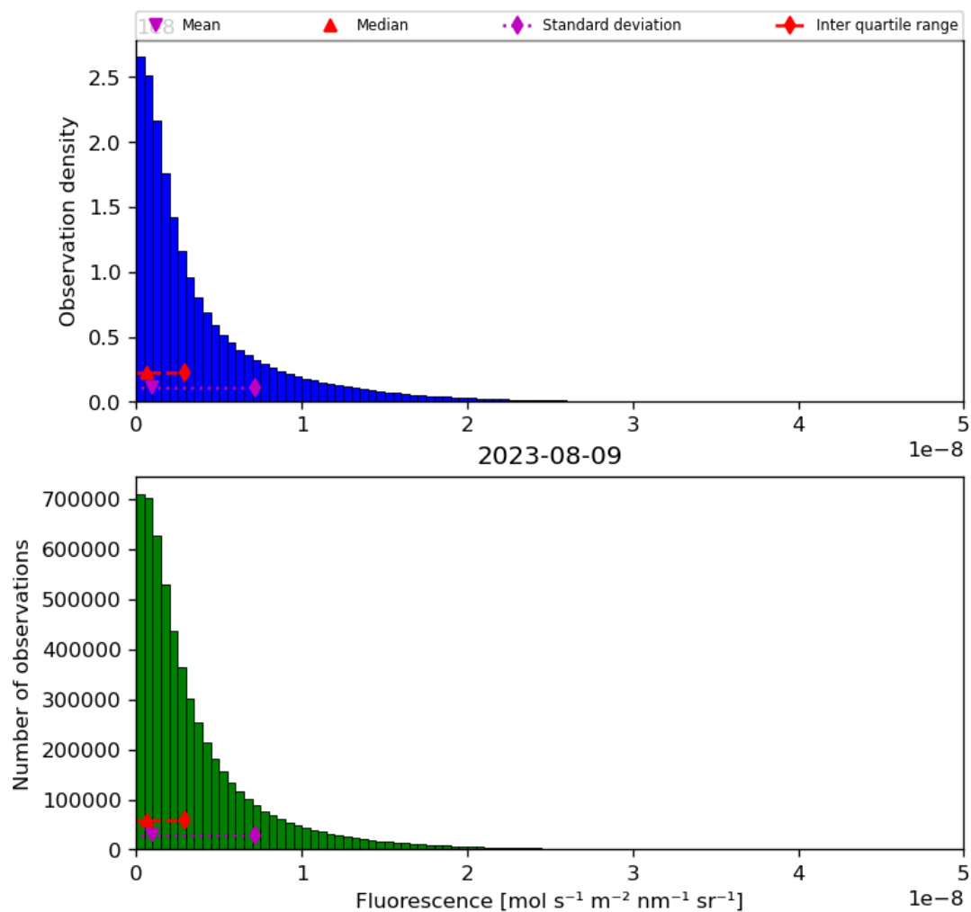
Figure 40: Histogram of “Fluorescence” for 2023-08-09 to 2023-08-10
