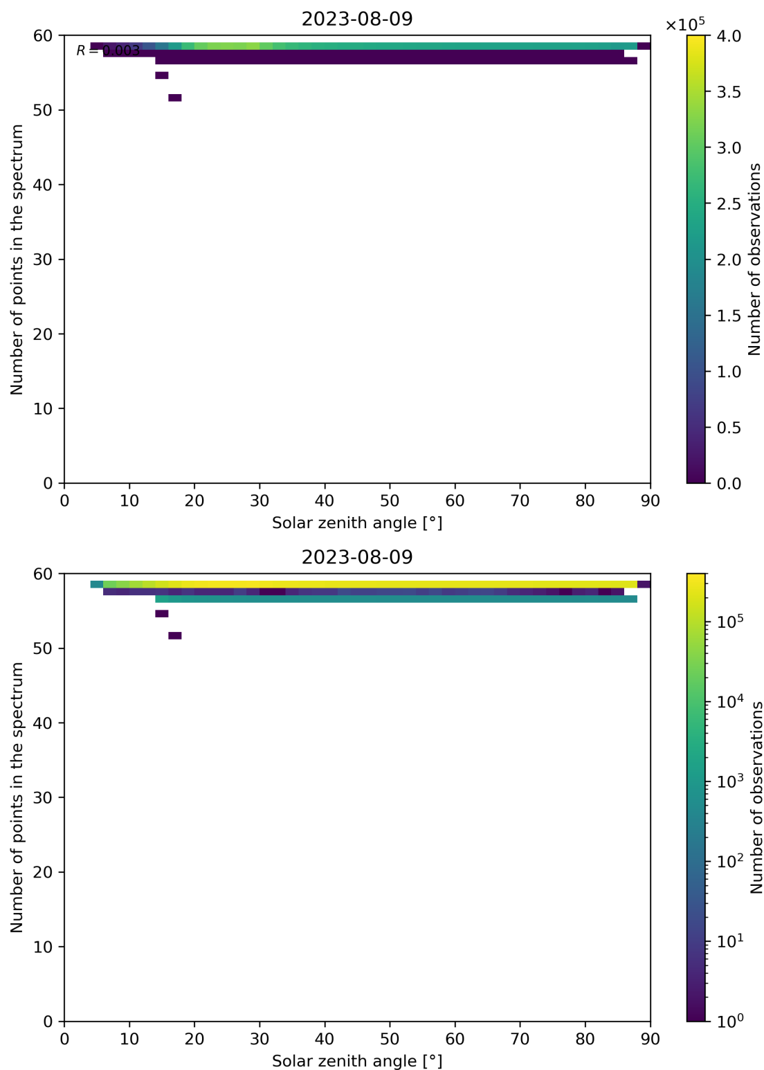
Figure 126: Scatter density plot of “Solar zenith angle” against “Number of points in the spectrum” for 2023-08-09 to 2023-08-10.
