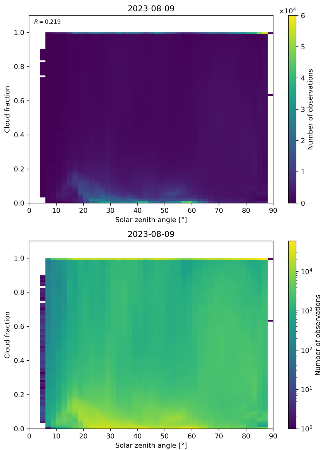
Figure 121: Scatter density plot of “Solar zenith angle” against “Cloud fraction” for 2023-08-09 to 2023-08-10.
