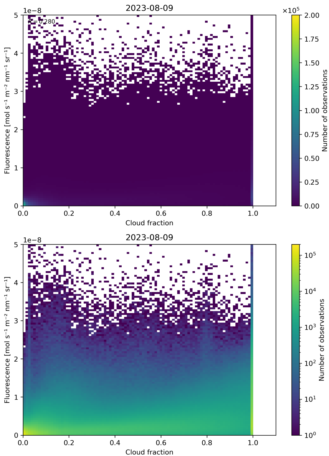
Figure 79: Scatter density plot of “Cloud fraction” against “Fluorescence” for 2023-08-09 to 2023-08-10.
