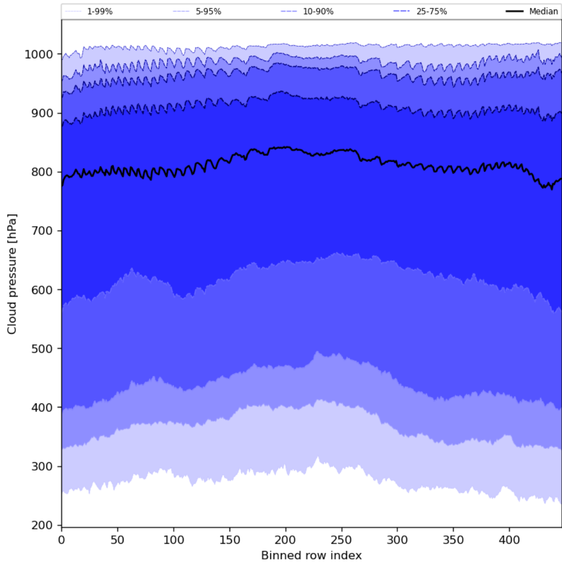
Figure 47: Along track statistics of “Cloud pressure” for 2023-08-09 to 2023-08-10
