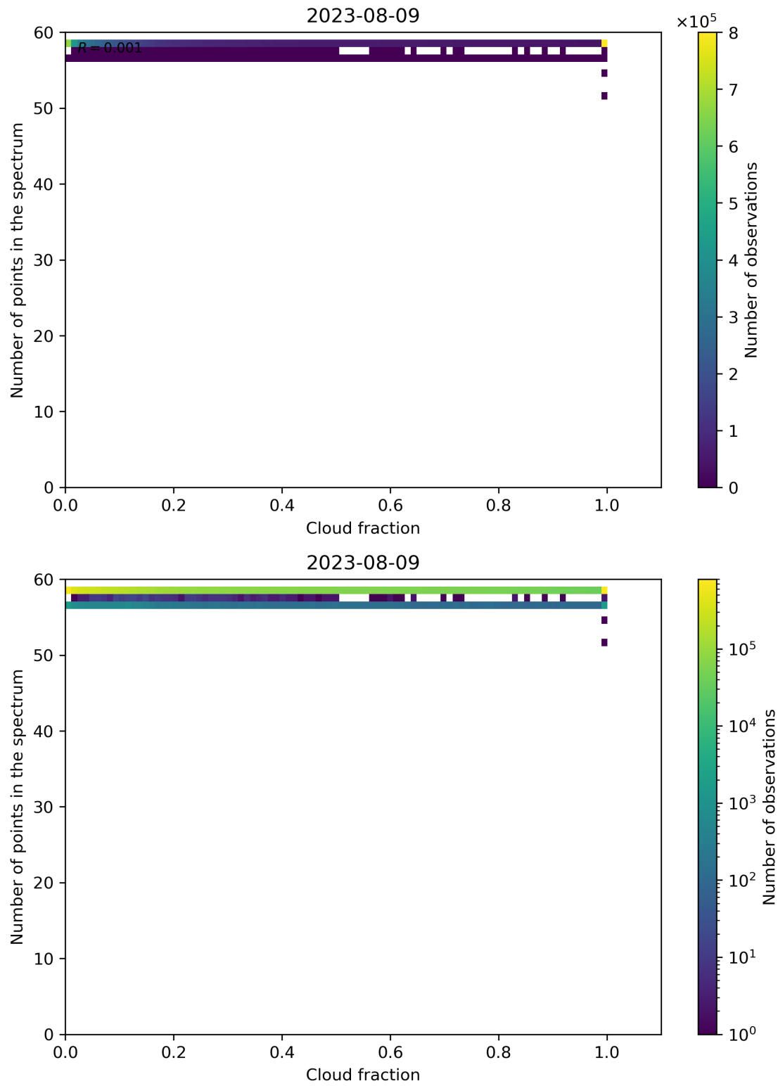
Figure 81: Scatter density plot of “Cloud fraction” against “Number of points in the spectrum” for 2023-08-09 to 2023-08-10.
