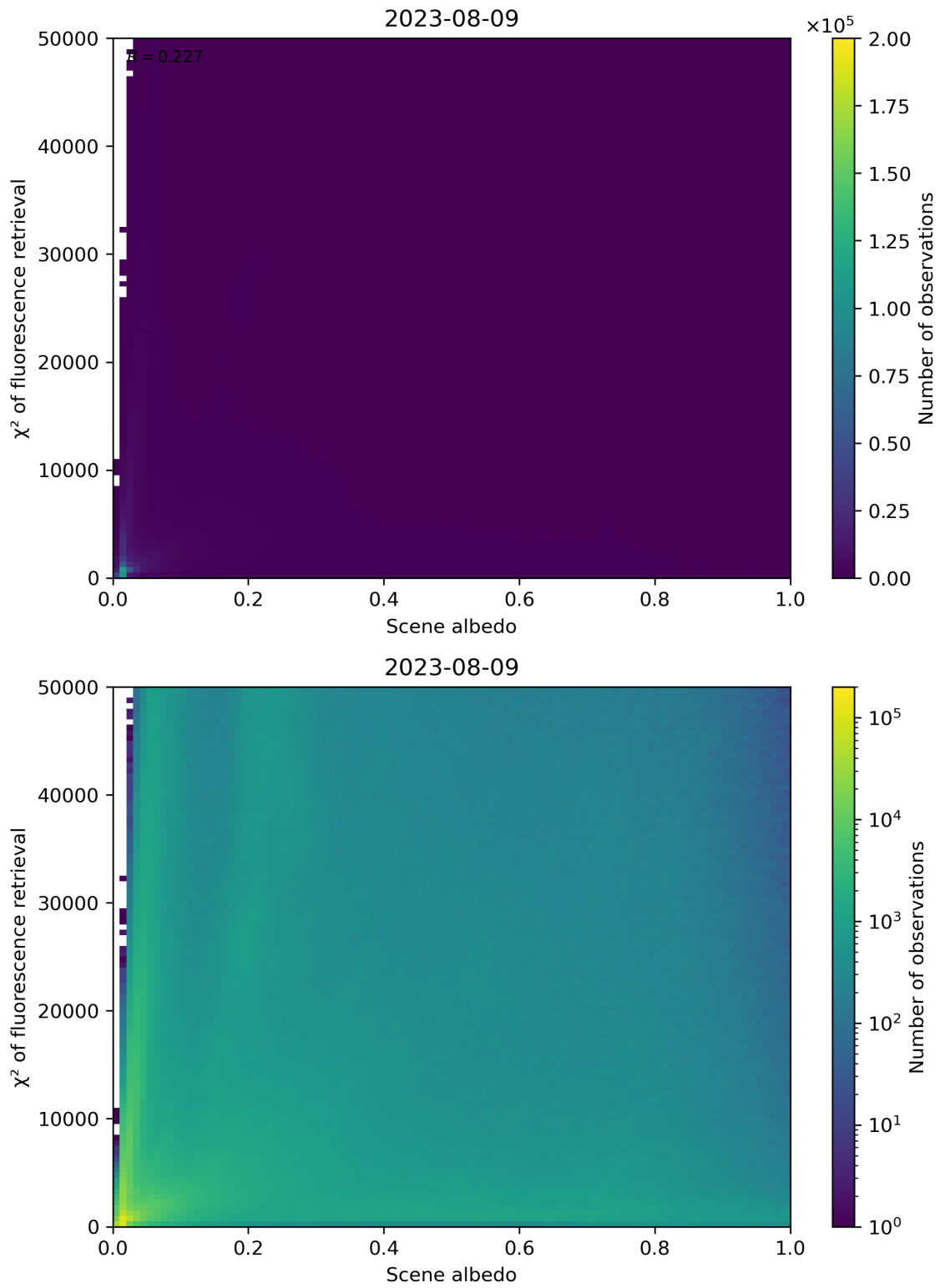
Figure 113: Scatter density plot of “Scene albedo” against “ \chi^2 of fluorescence retrieval” for 2023-08-09 to 2023-08-10.
