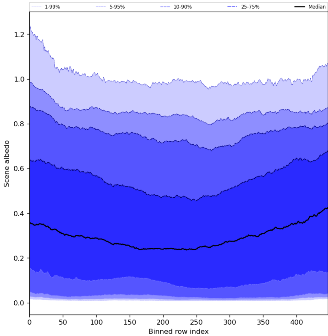
Figure 51: Along track statistics of “Scene albedo” for 2023-08-09 to 2023-08-10
