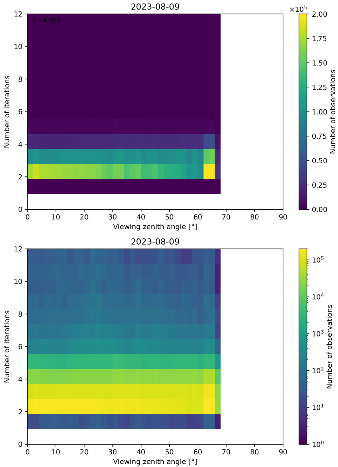
Figure 136: Scatter density plot of “Viewing zenith angle” against “Number of iterations” for 2023-08-09 to 2023-08-10.
