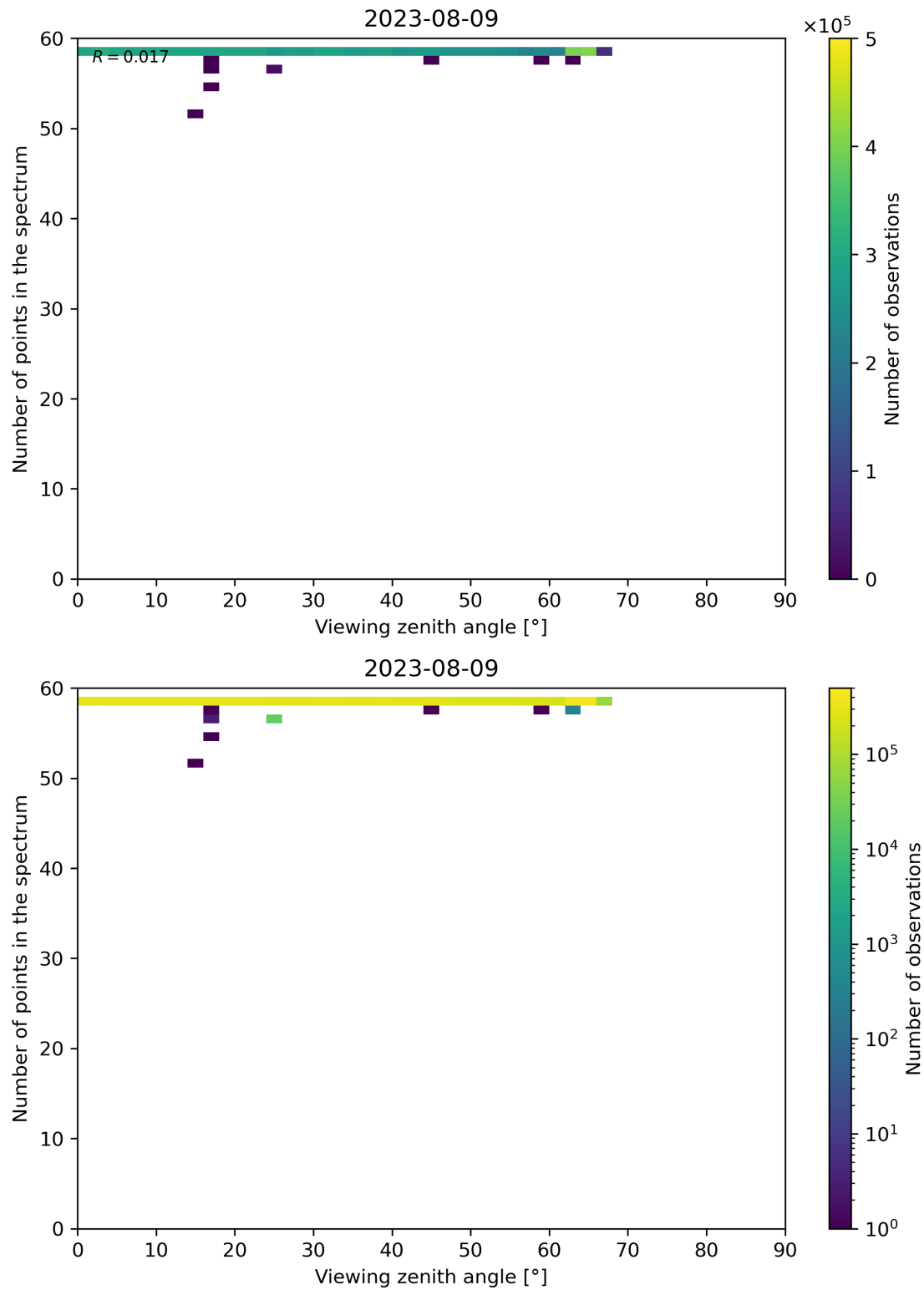
Figure 137: Scatter density plot of “Viewing zenith angle” against “Number of points in the spectrum” for 2023-08-09 to 2023-08-10.
