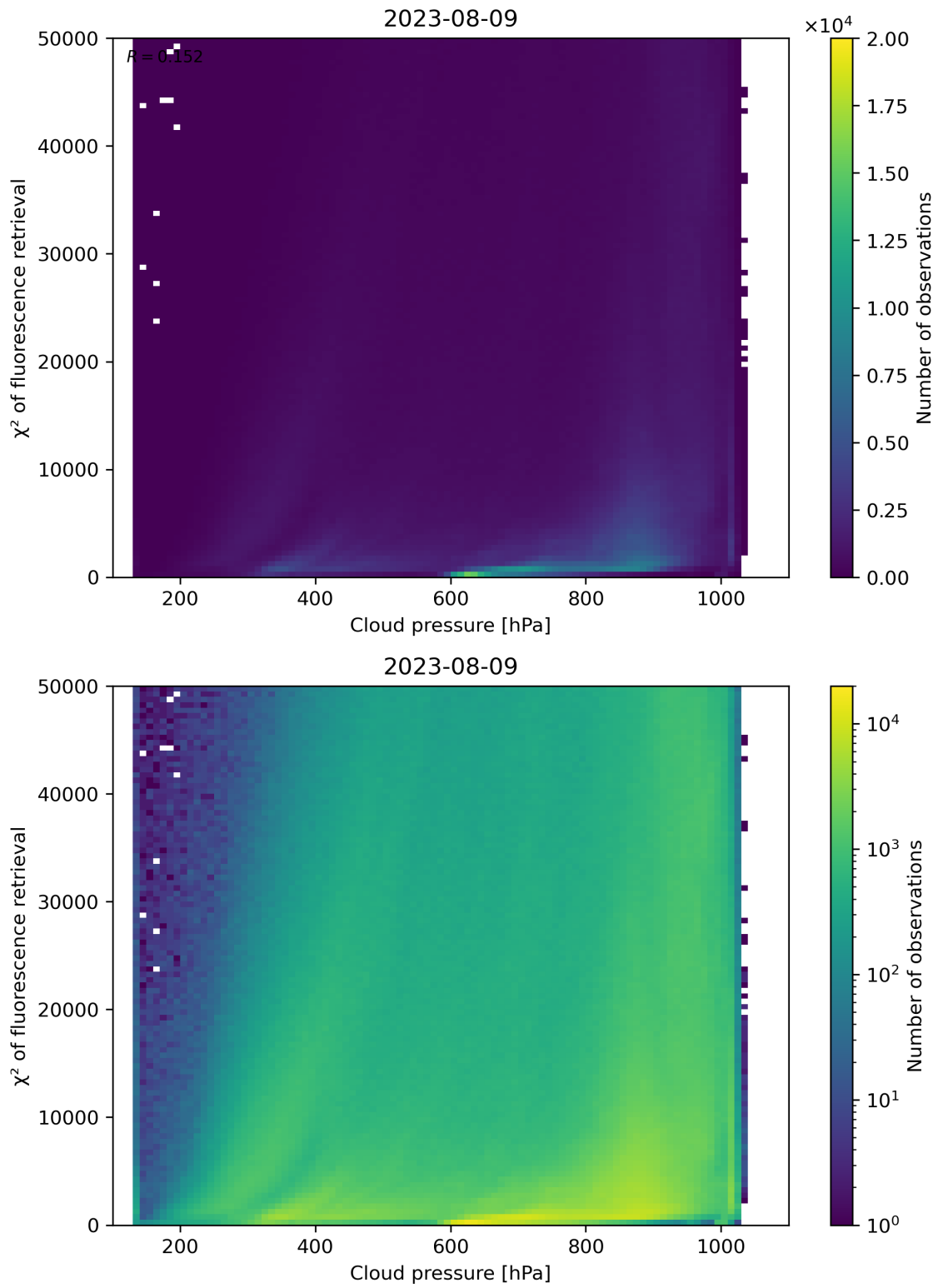
Figure 86: Scatter density plot of “Cloud pressure” against “ \chi^2 of fluorescence retrieval” for 2023-08-09 to 2023-08-10.
