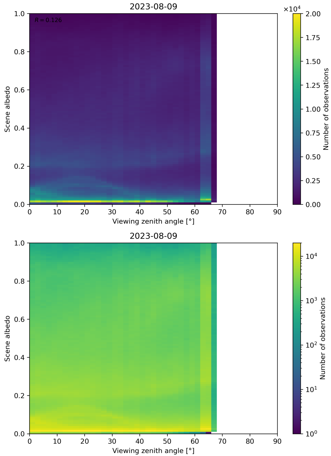
Figure 138: Scatter density plot of “Viewing zenith angle” against “Scene albedo” for 2023-08-09 to 2023-08-10.
