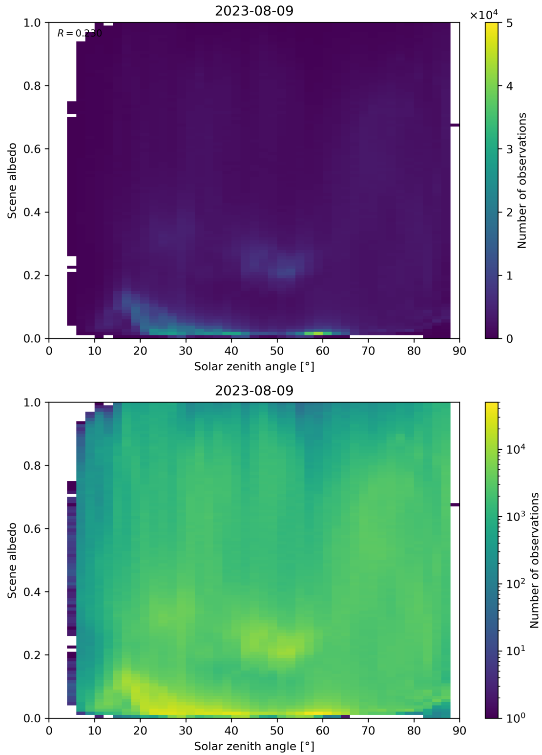
Figure 127: Scatter density plot of “Solar zenith angle” against “Scene albedo” for 2023-08-09 to 2023-08-10.
