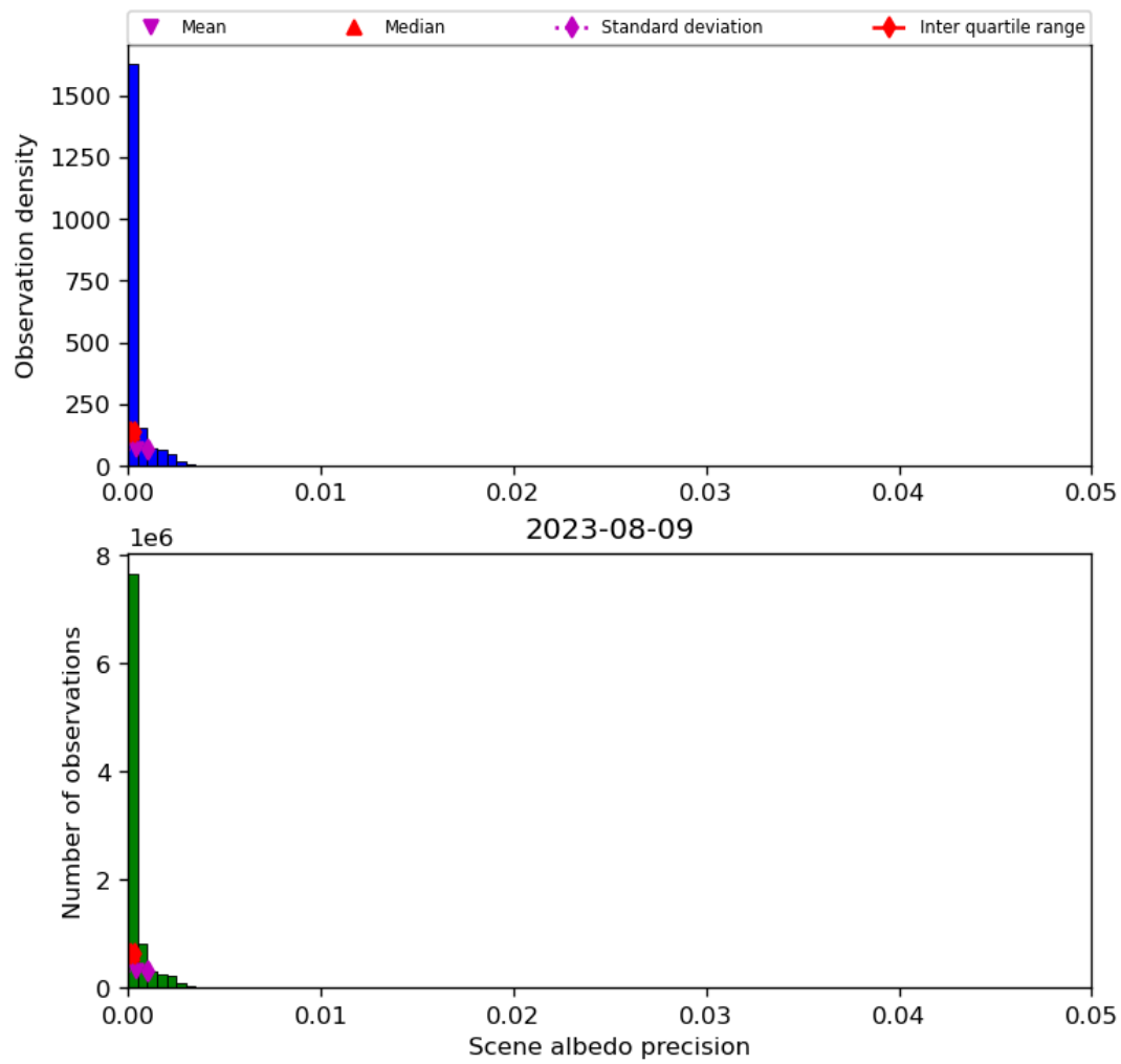
Figure 35: Histogram of “Scene albedo precision” for 2023-08-09 to 2023-08-10
