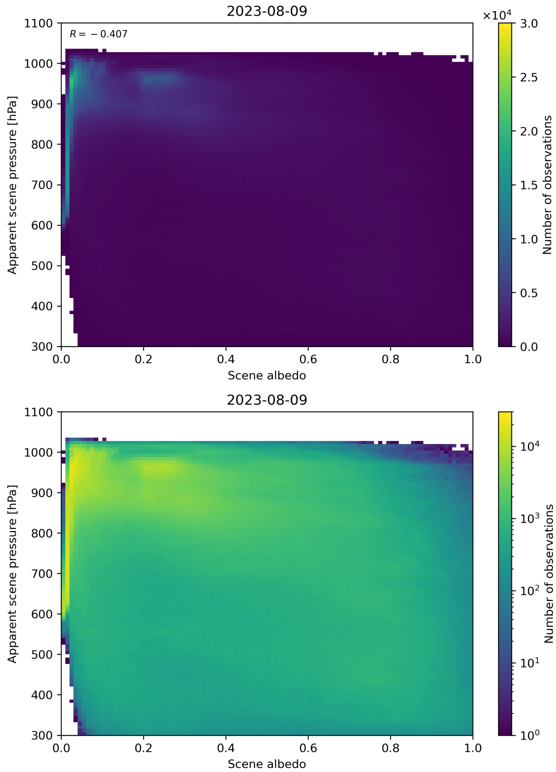
Figure 111: Scatter density plot of “Scene albedo” against “Apparent scene pressure” for 2023-08-09 to 2023-08-10.
