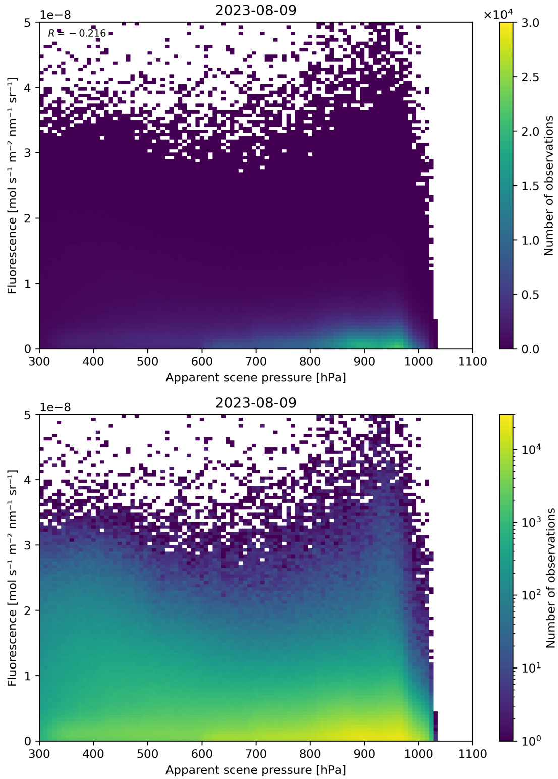
Figure 65: Scatter density plot of “Apparent scene pressure” against “Fluorescence” for 2023-08-09 to 2023-08-10.
