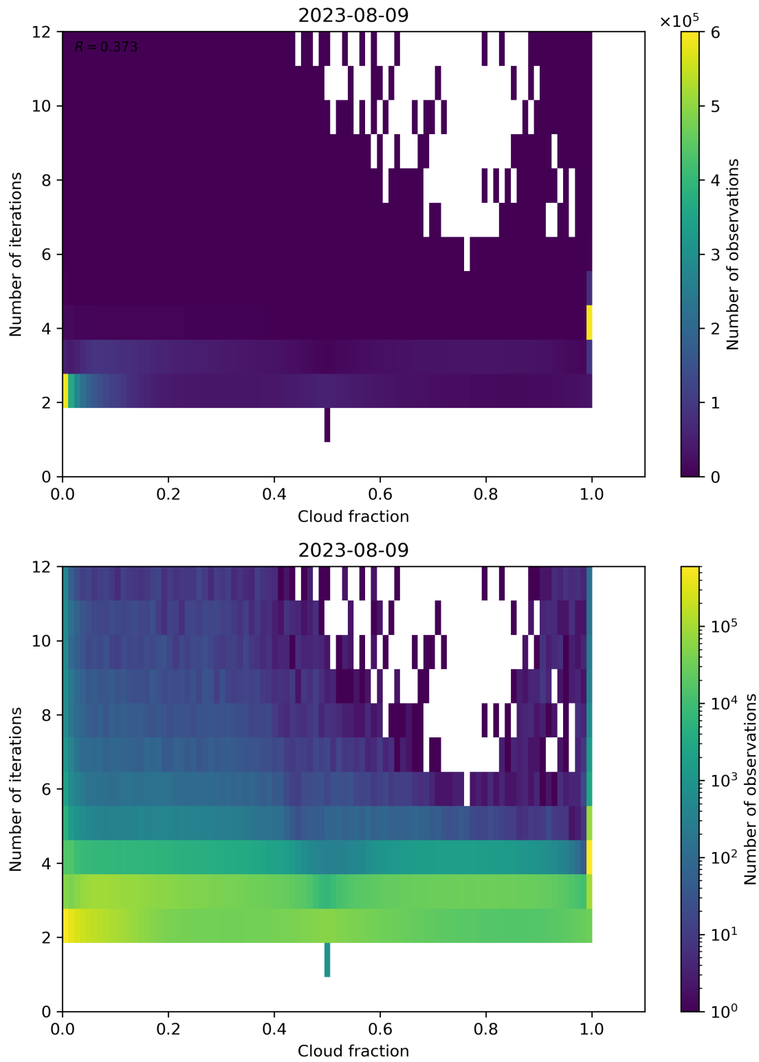
Figure 80: Scatter density plot of “Cloud fraction” against “Number of iterations” for 2023-08-09 to 2023-08-10.
