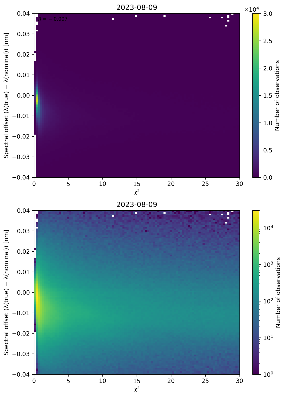
Figure 75: Scatter density plot of " \chi^2 " against "Spectral offset ( \lambda(\text{true}) - \lambda(\text{nominal}) )" for 2023-08-09 to 2023-08-10.
