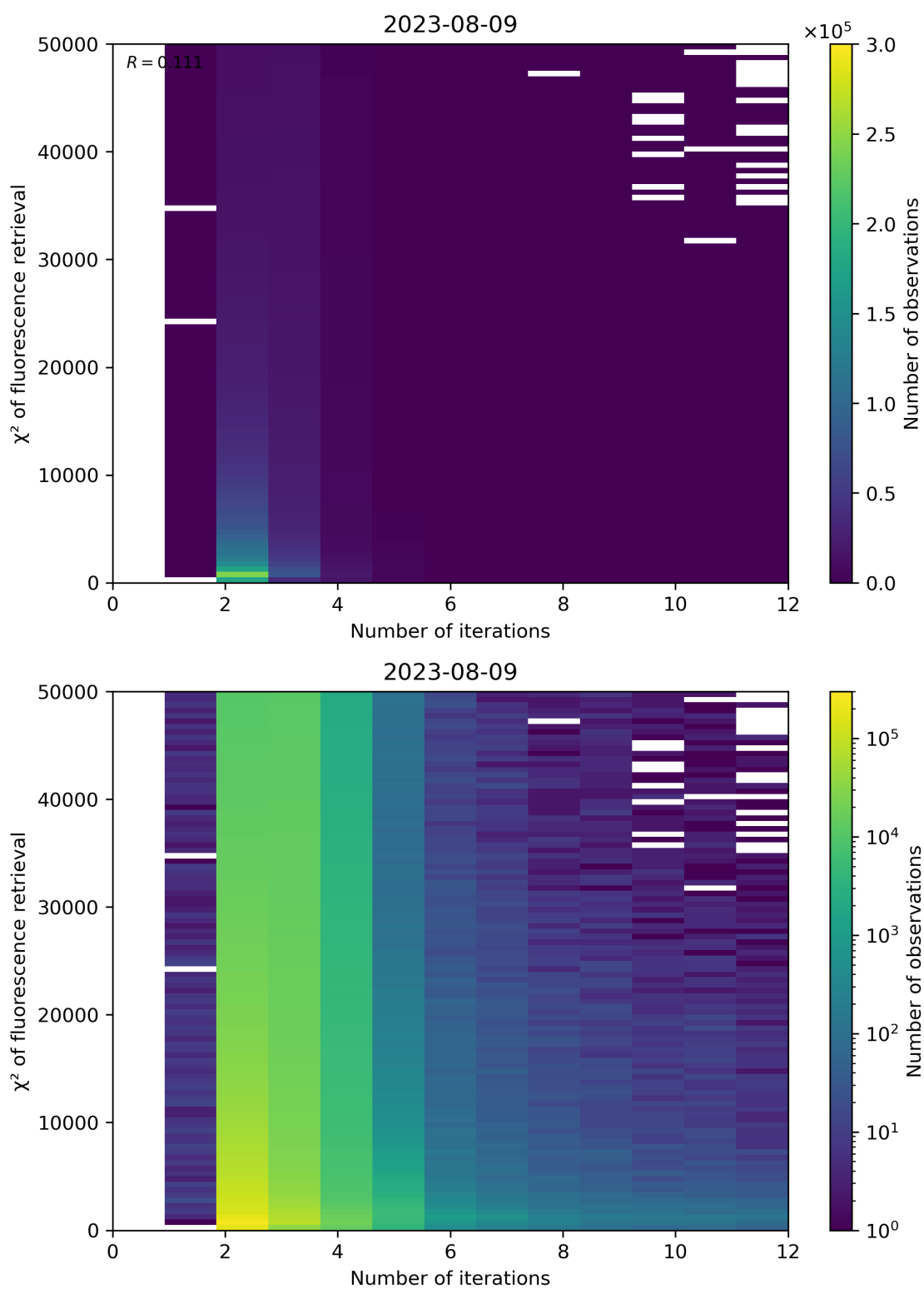
Figure 106: Scatter density plot of “Number of iterations” against “ \chi^2 of fluorescence retrieval” for 2023-08-09 to 2023-08-10.
