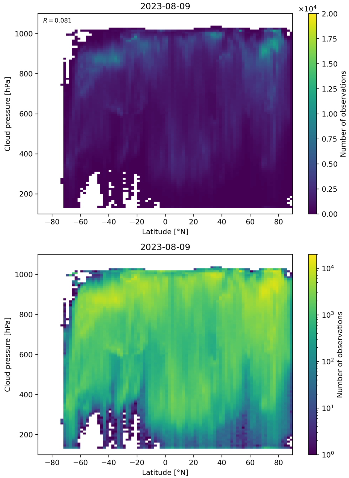
Figure 100: Scatter density plot of “Latitude” against “Cloud pressure” for 2023-08-09 to 2023-08-10.
