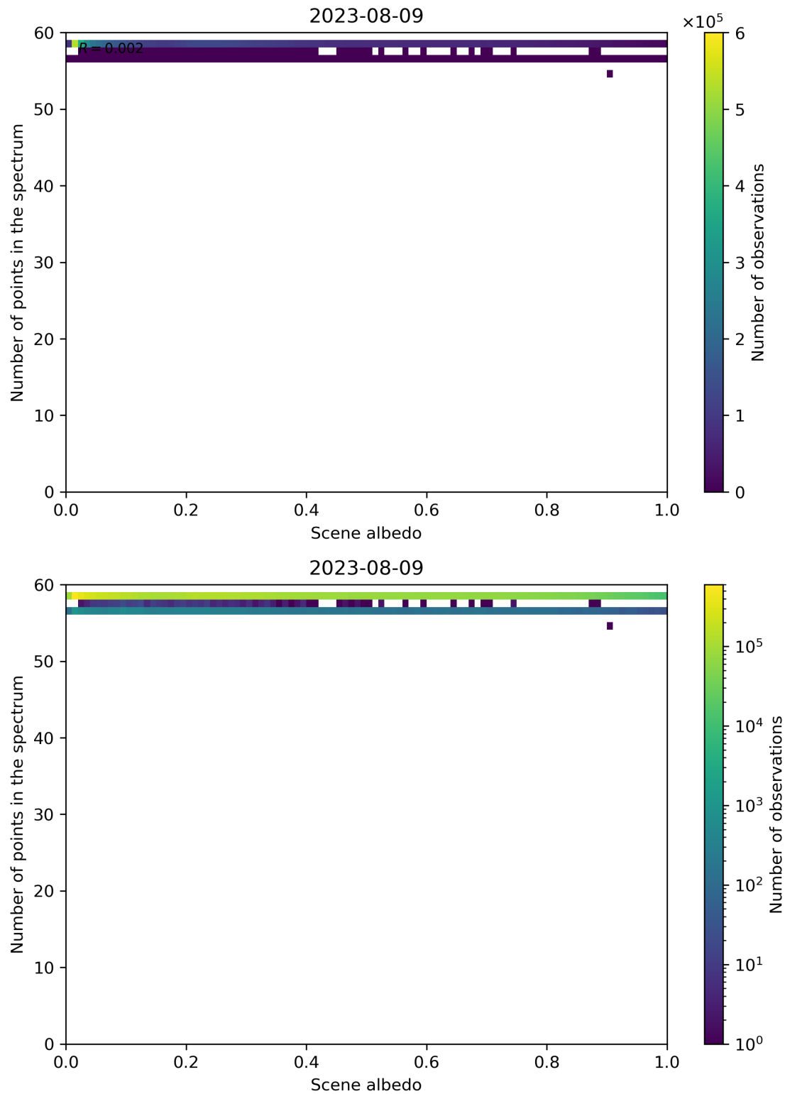
Figure 116: Scatter density plot of “Scene albedo” against “Number of points in the spectrum” for 2023-08-09 to 2023-08-10.
