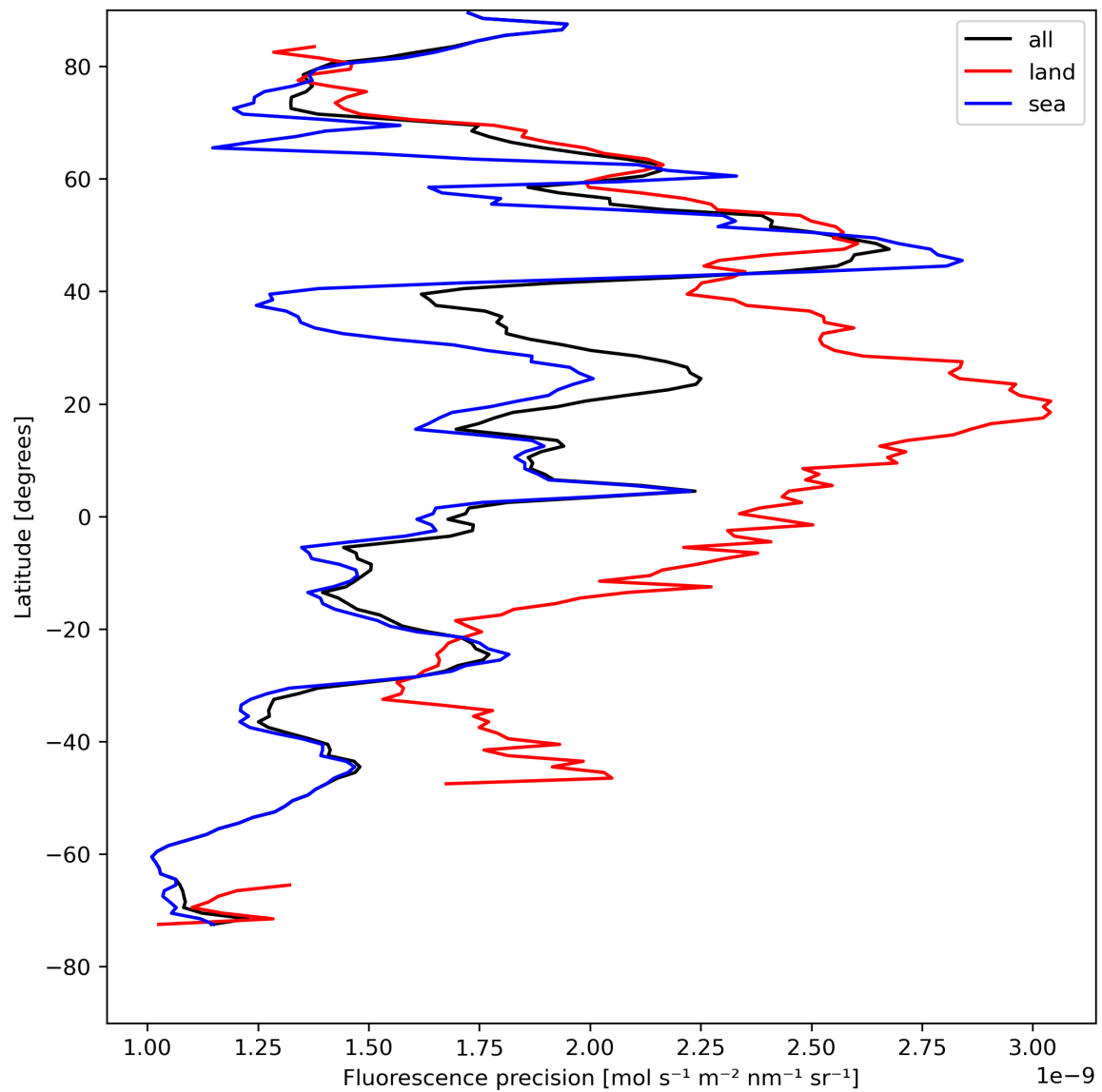
Figure 24: Zonal average of “Fluorescence precision” for 2023-08-09 to 2023-08-10.
