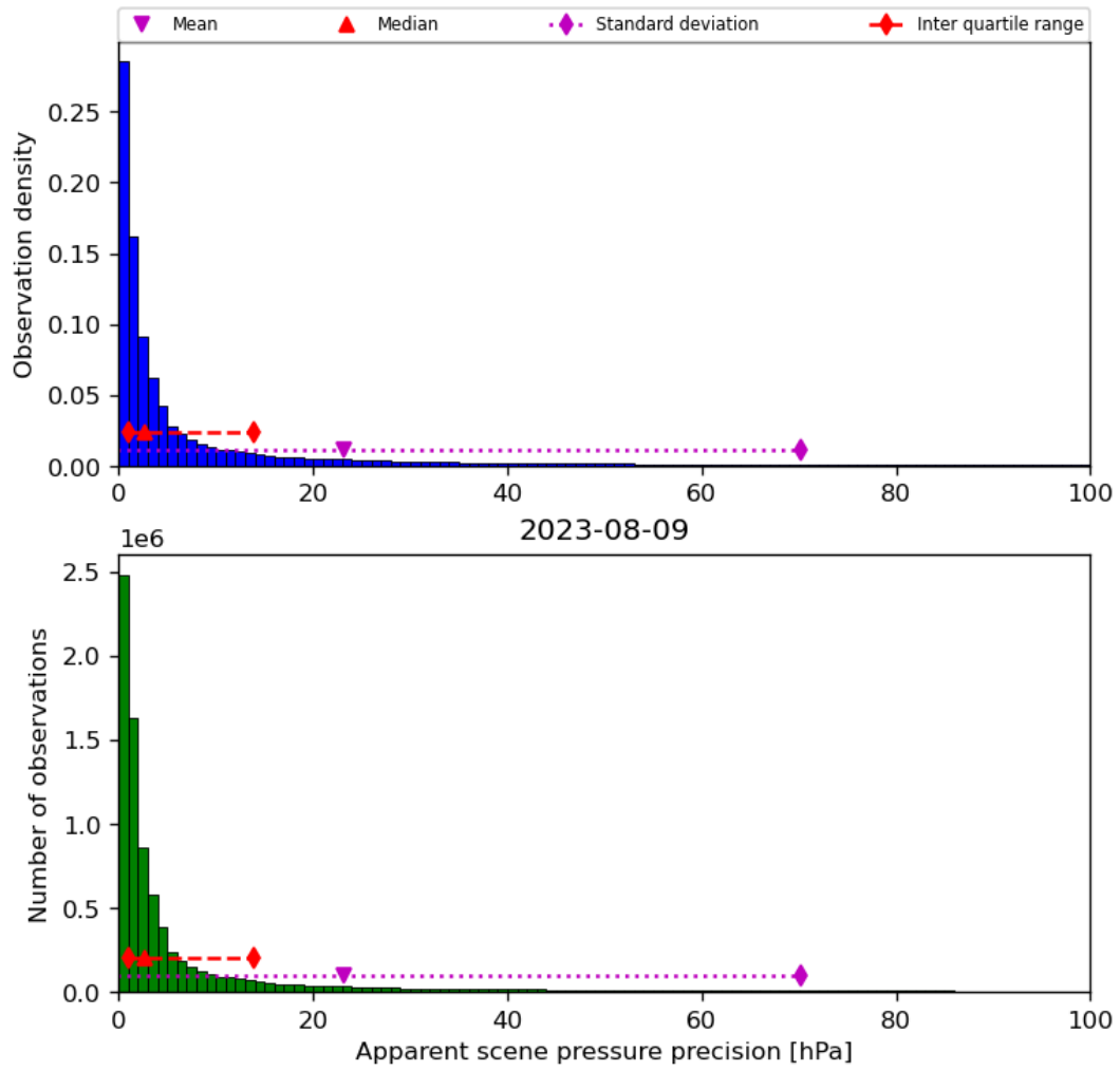
Figure 37: Histogram of “Apparent scene pressure precision” for 2023-08-09 to 2023-08-10
