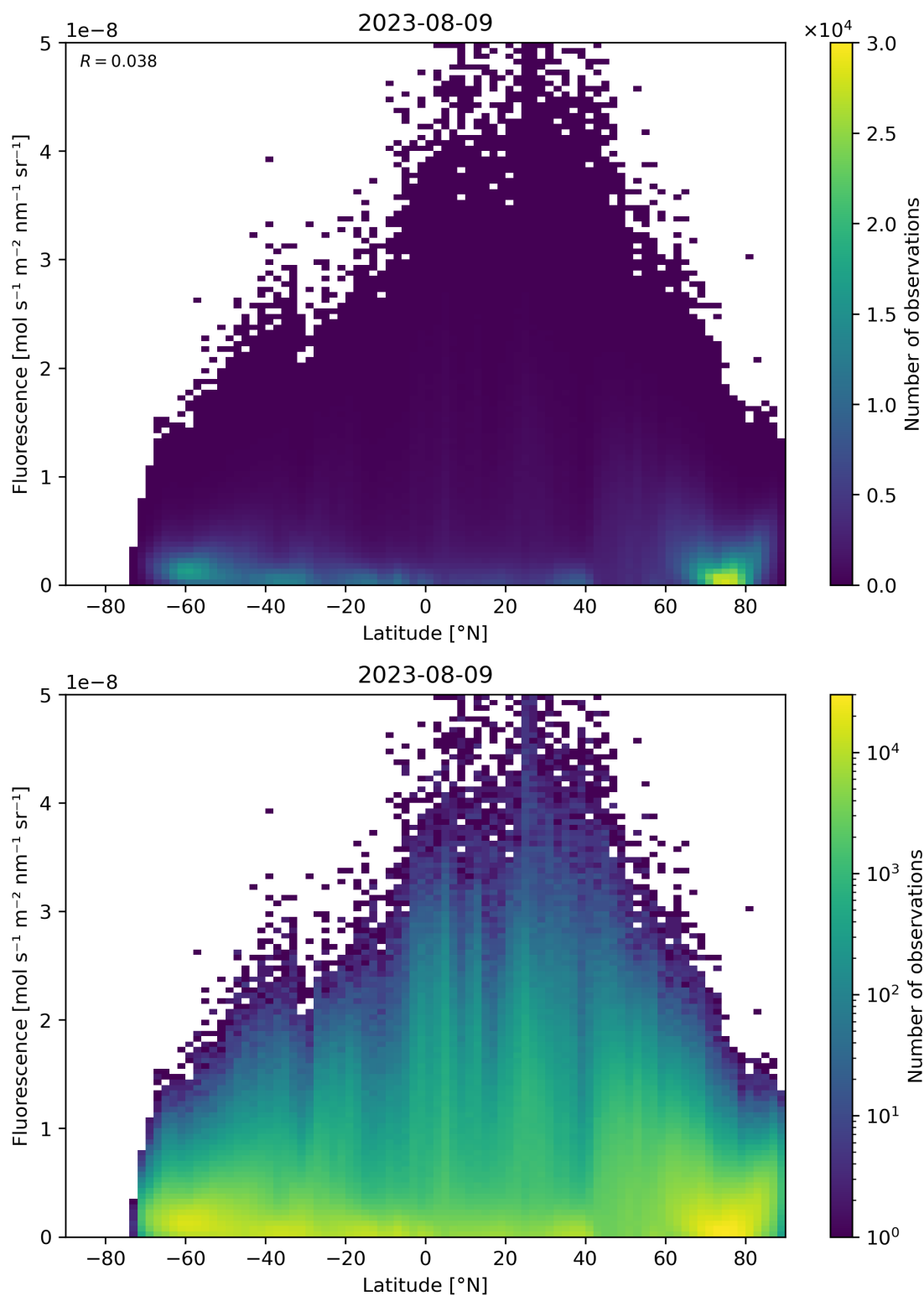
Figure 101: Scatter density plot of “Latitude” against “Fluorescence” for 2023-08-09 to 2023-08-10.
