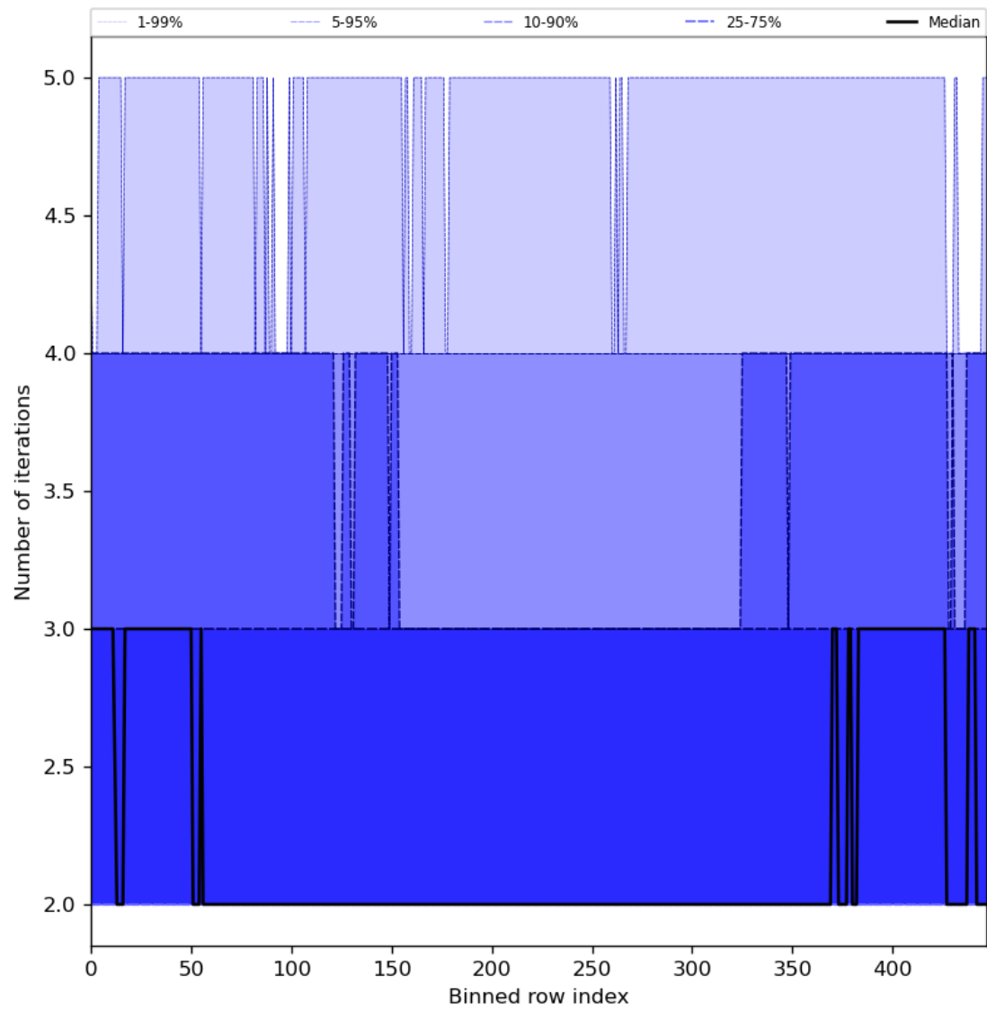
Figure 56: Along track statistics of “Number of iterations” for 2023-08-09 to 2023-08-10
