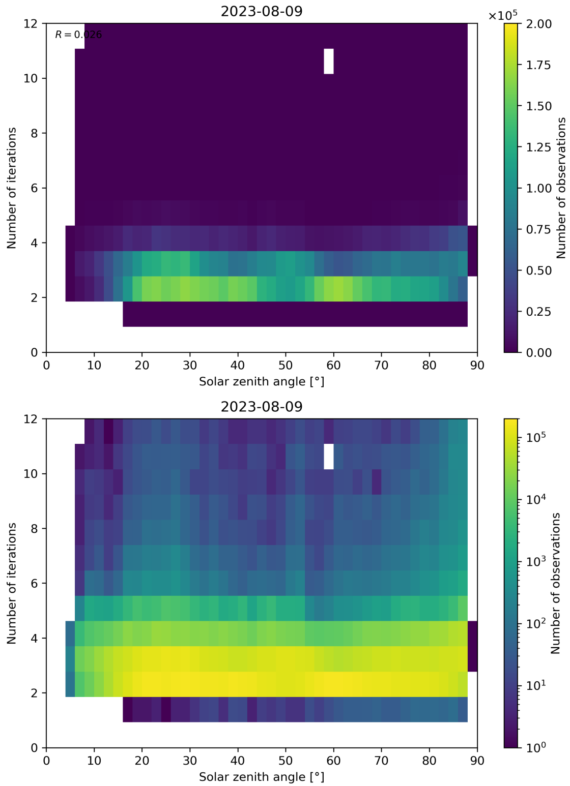
Figure 125: Scatter density plot of “Solar zenith angle” against “Number of iterations” for 2023-08-09 to 2023-08-10.
