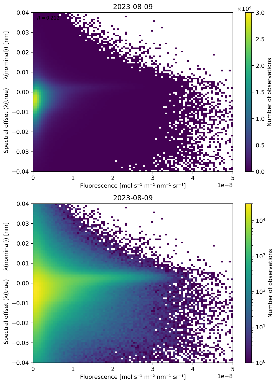
Figure 95: Scatter density plot of “Fluorescence” against “Spectral offset ( \lambda(\text{true}) - \lambda(\text{nominal}) )” for 2023-08-09 to 2023-08-10.
