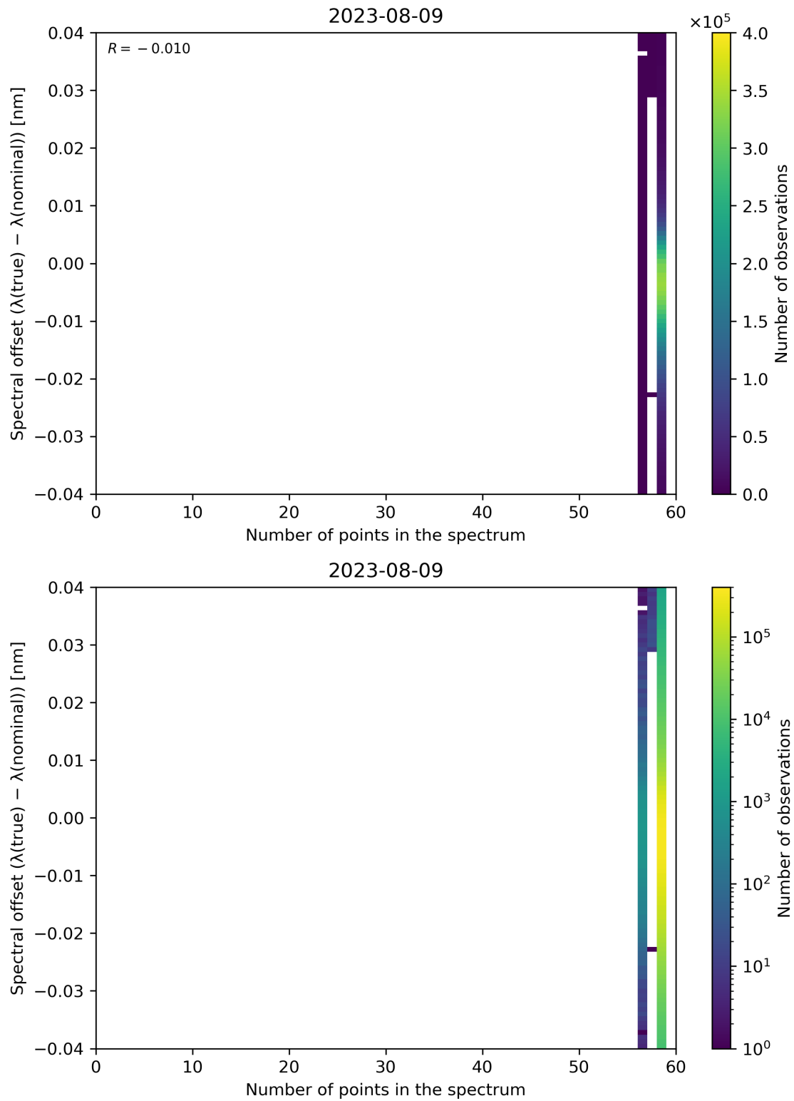
Figure 110: Scatter density plot of “Number of points in the spectrum” against “Spectral offset ( \lambda(\text{true}) - \lambda(\text{nominal}) )” for 2023-08-09 to 2023-08-10.
