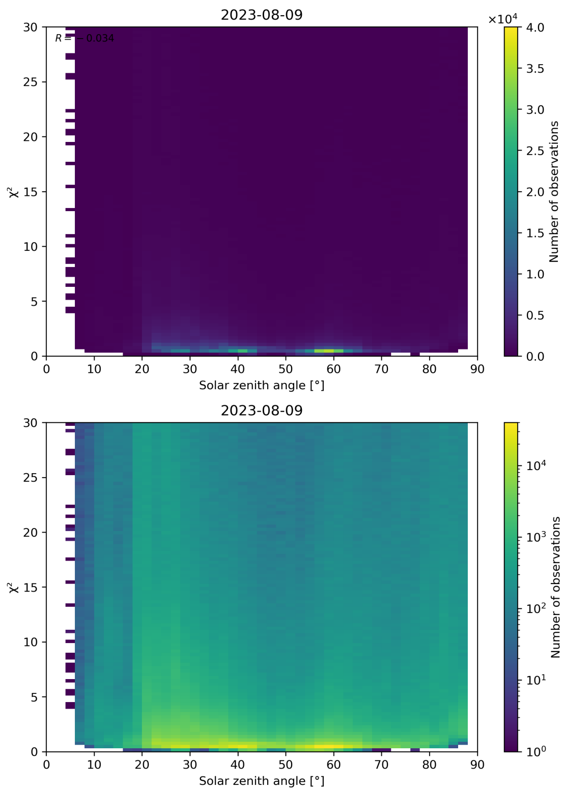
Figure 119: Scatter density plot of “Solar zenith angle” against “ \chi^2 ” for 2023-08-09 to 2023-08-10.
