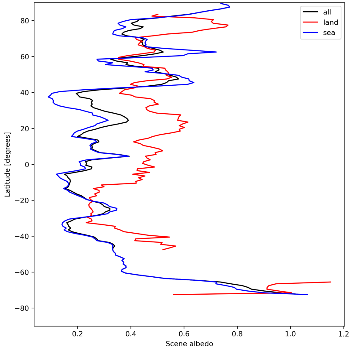
Figure 17: Zonal average of "Scene albedo" for 2023-08-09 to 2023-08-10.
