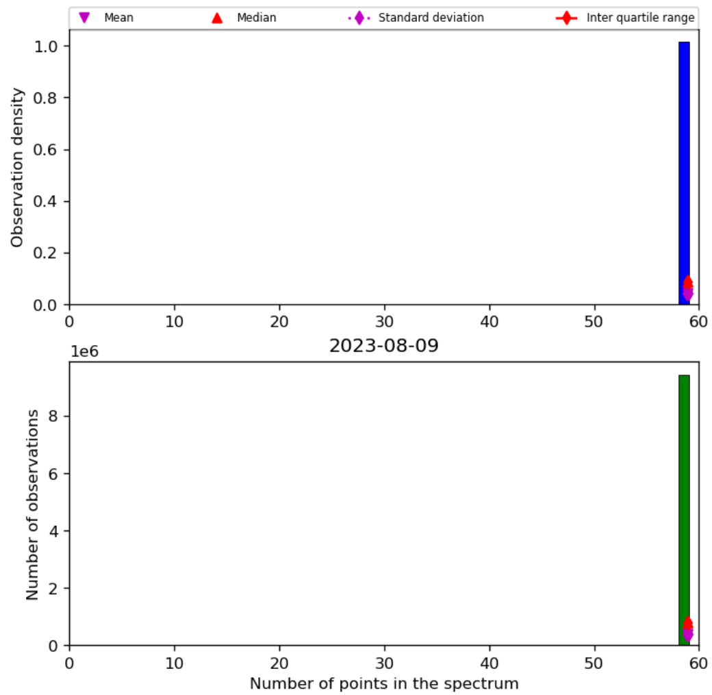
Figure 44: Histogram of “Number of points in the spectrum” for 2023-08-09 to 2023-08-10
