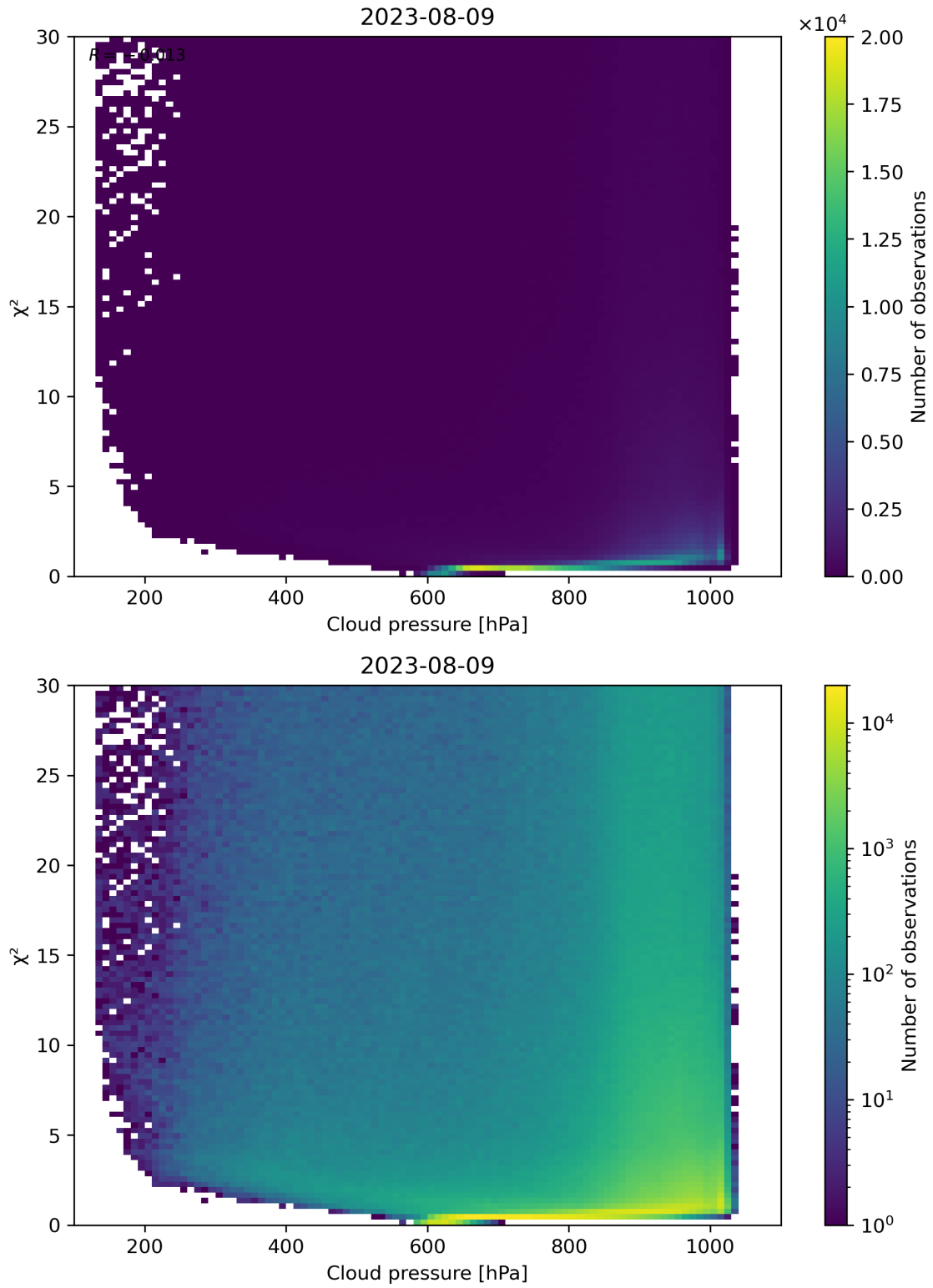
Figure 85: Scatter density plot of “Cloud pressure” against “ \chi^2 ” for 2023-08-09 to 2023-08-10.
