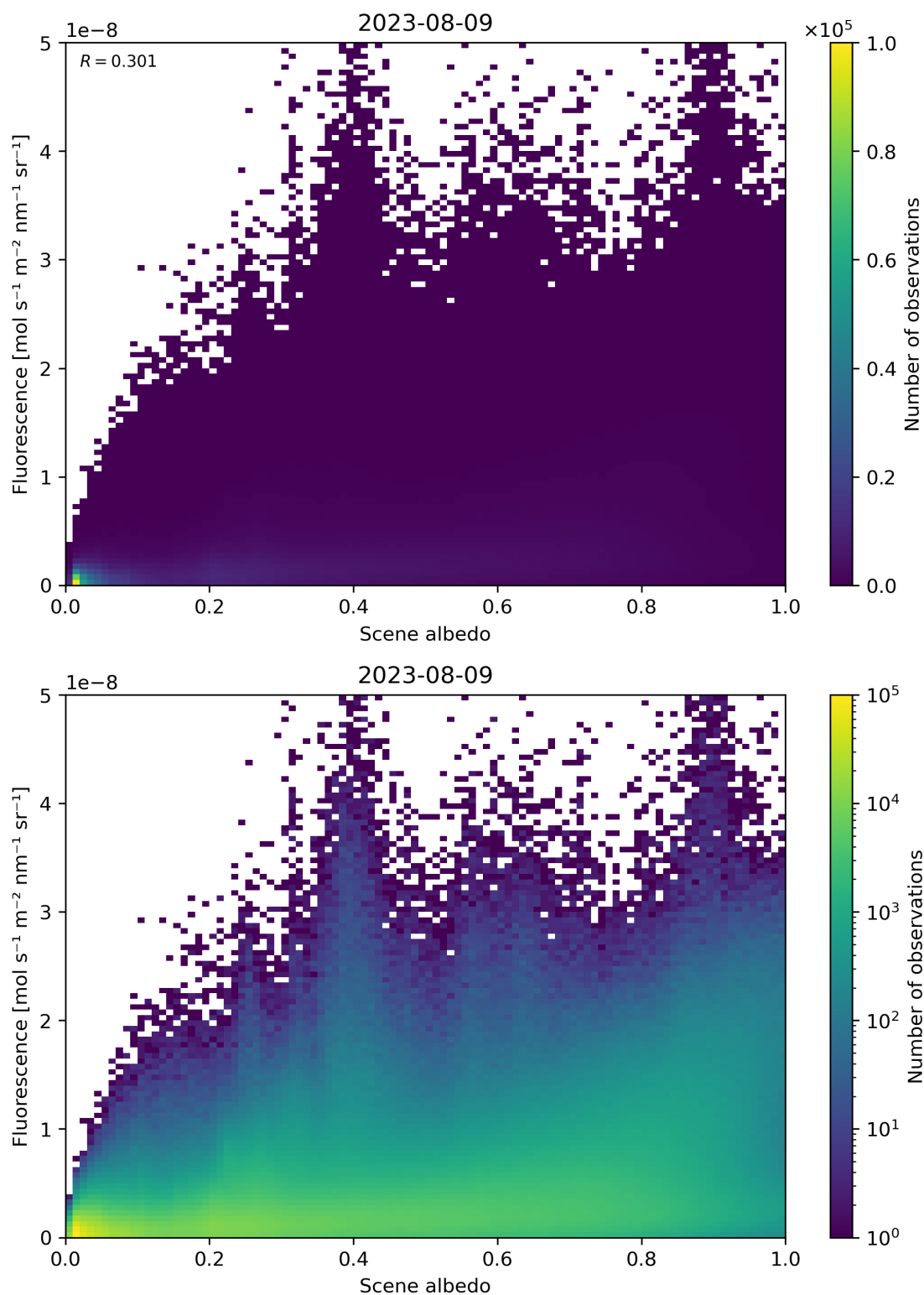
Figure 114: Scatter density plot of “Scene albedo” against “Fluorescence” for 2023-08-09 to 2023-08-10.
