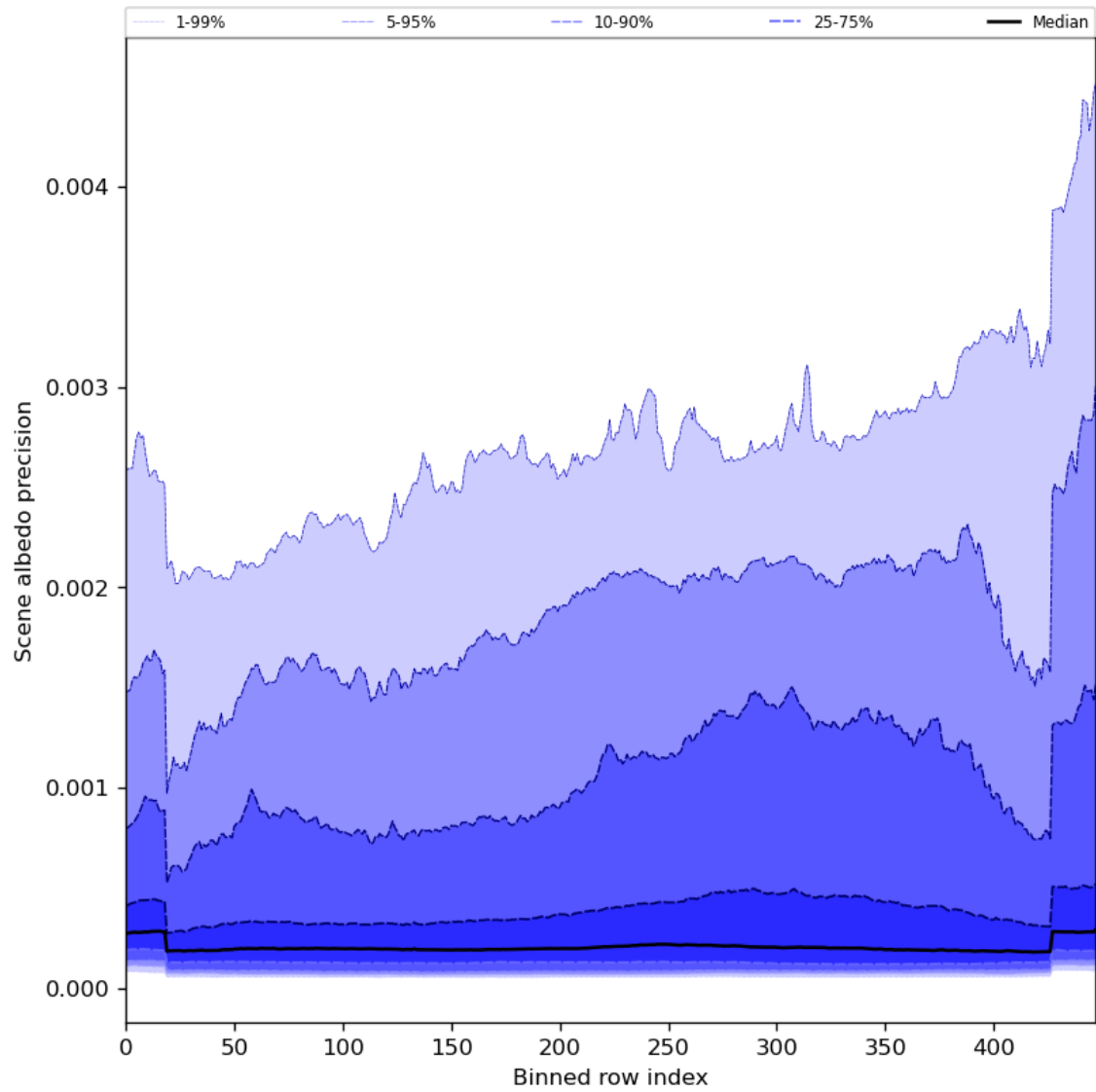
Figure 52: Along track statistics of “Scene albedo precision” for 2023-08-09 to 2023-08-10
