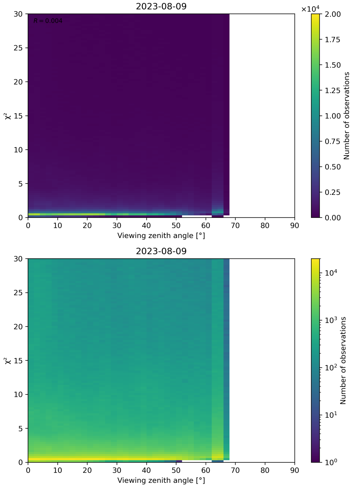
Figure 130: Scatter density plot of “Viewing zenith angle” against “ \chi^2 ” for 2023-08-09 to 2023-08-10.
