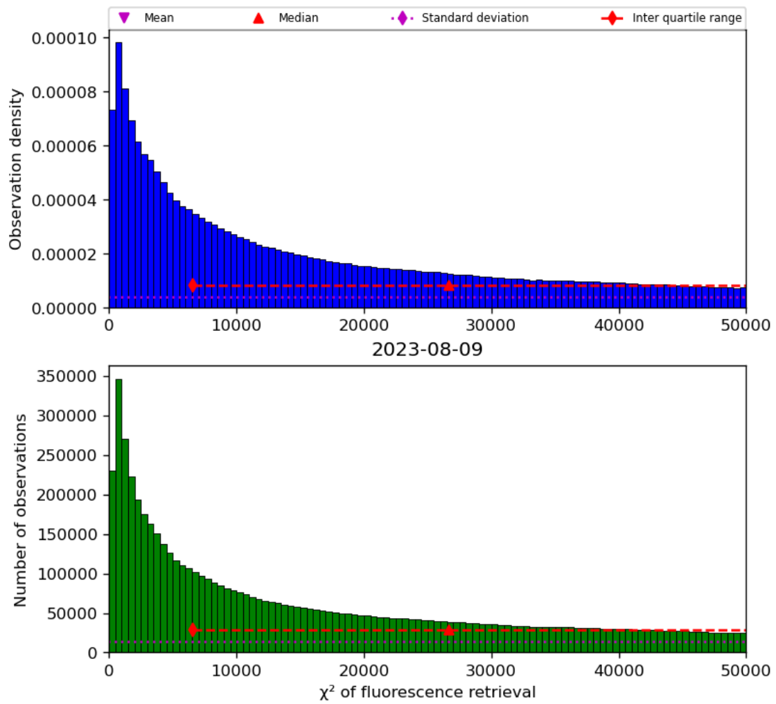
Figure 42: Histogram of “ \chi^2 of fluorescence retrieval” for 2023-08-09 to 2023-08-10
