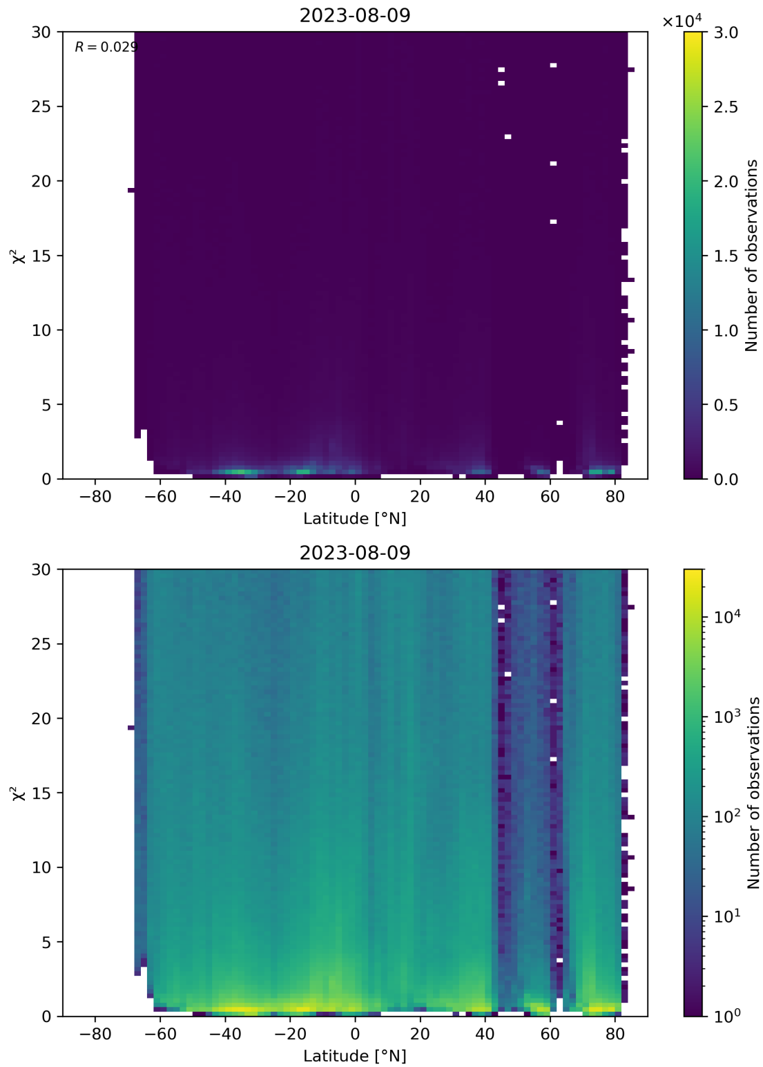
Figure 97: Scatter density plot of “Latitude” against “ \chi^2 ” for 2023-08-09 to 2023-08-10.
