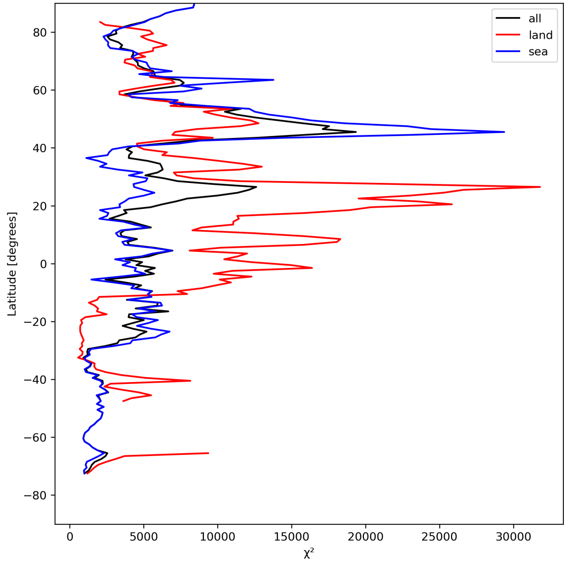
Figure 21: Zonal average of “ \chi^2 ” for 2023-08-09 to 2023-08-10.
