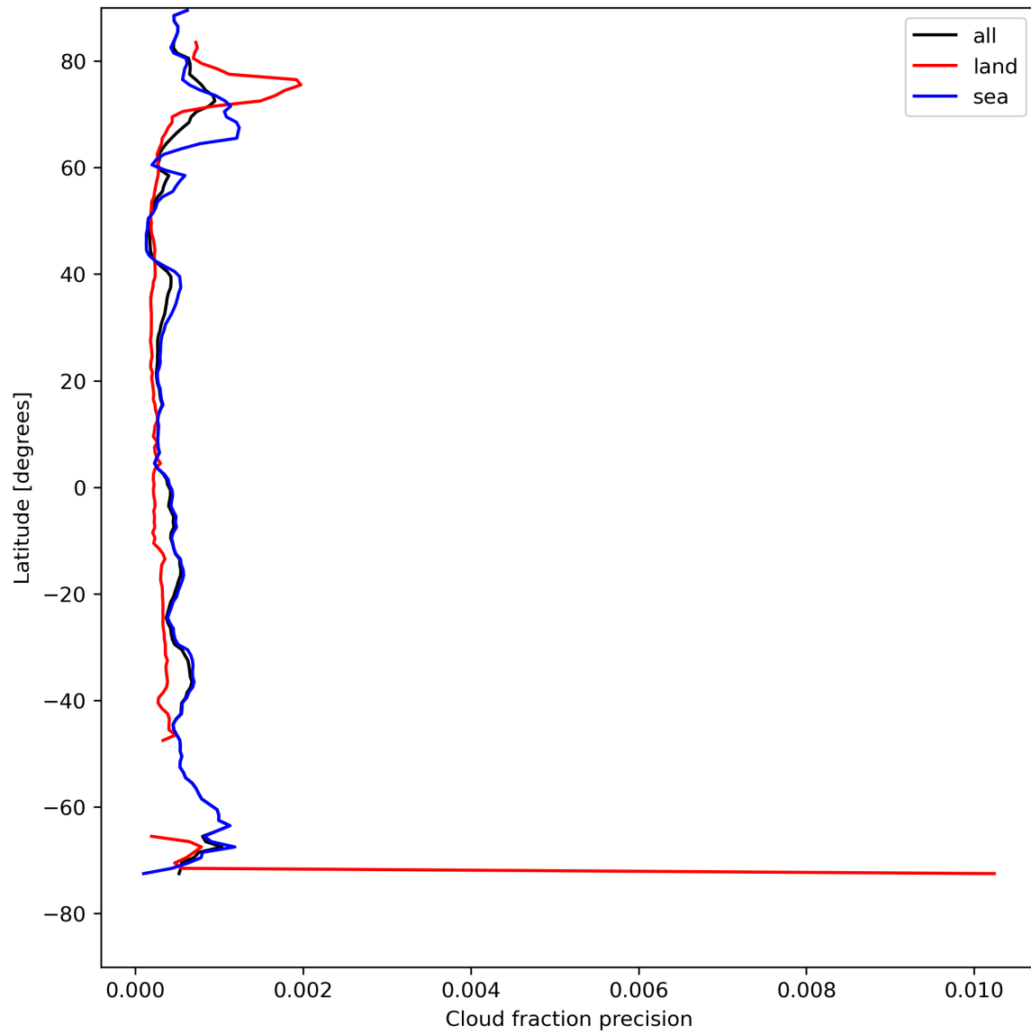
Figure 16: Zonal average of “Cloud fraction precision” for 2023-08-09 to 2023-08-10.
