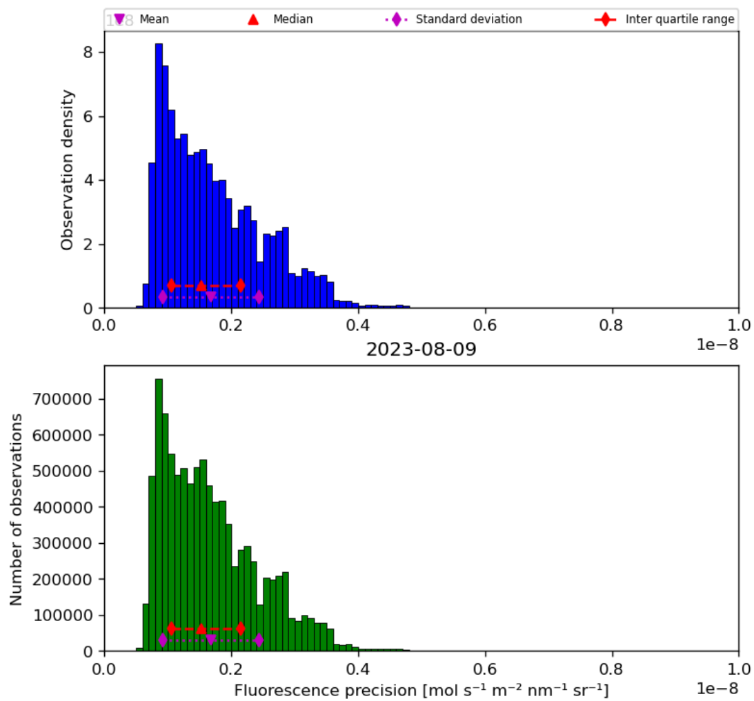
Figure 41: Histogram of “Fluorescence precision” for 2023-08-09 to 2023-08-10
