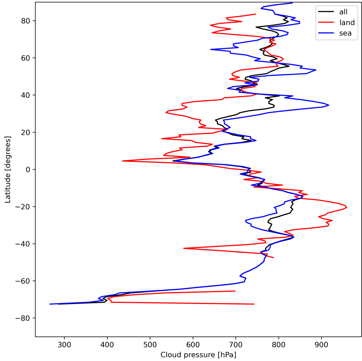
Figure 13: Zonal average of “Cloud pressure” for 2023-08-09 to 2023-08-10.
