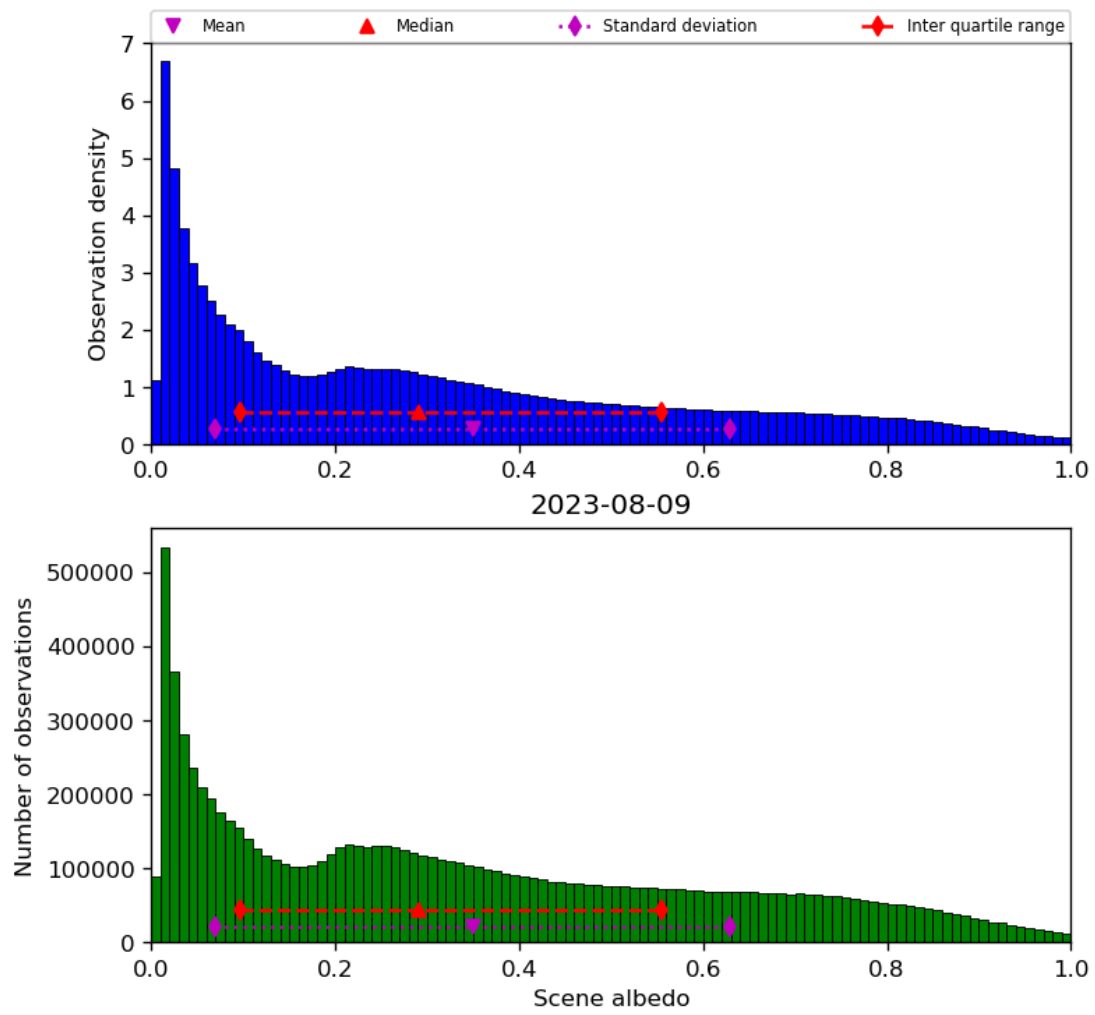
Figure 34: Histogram of “Scene albedo” for 2023-08-09 to 2023-08-10
