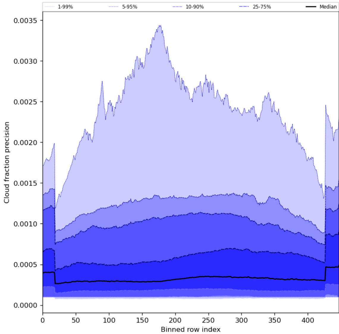
Figure 50: Along track statistics of “Cloud fraction precision” for 2023-08-09 to 2023-08-10
