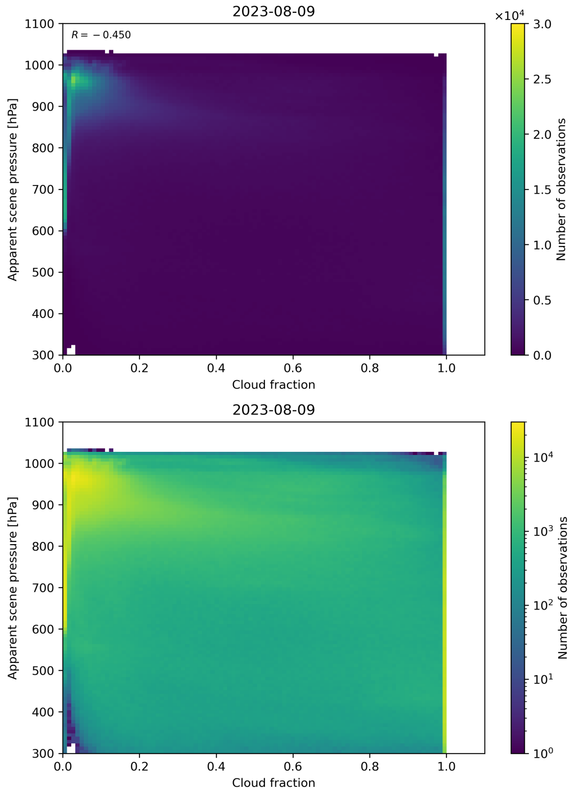
Figure 76: Scatter density plot of “Cloud fraction” against “Apparent scene pressure” for 2023-08-09 to 2023-08-10.
