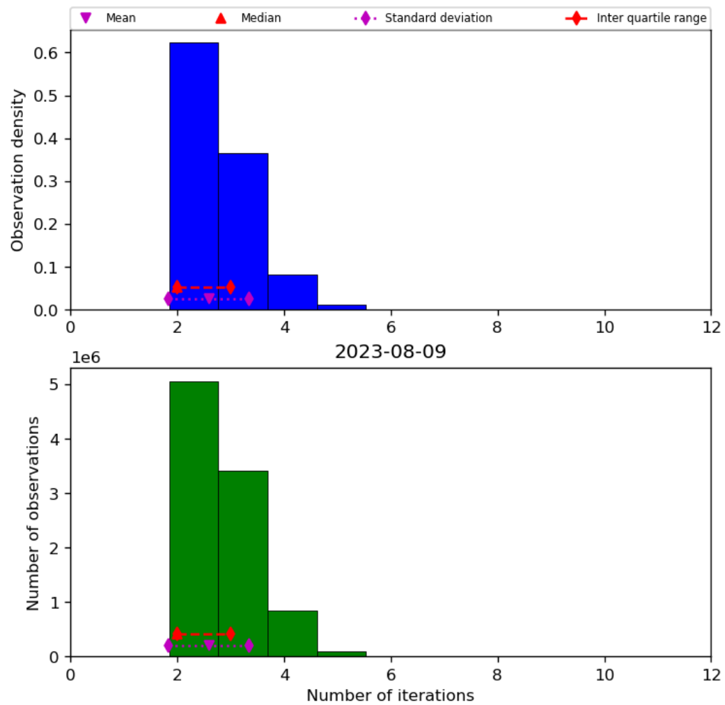
Figure 39: Histogram of “Number of iterations” for 2023-08-09 to 2023-08-10
