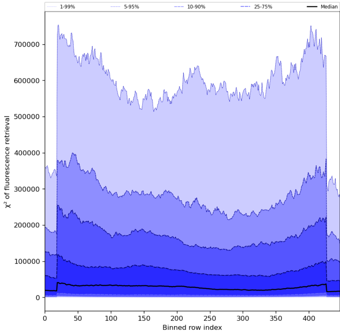
Figure 59: Along track statistics of “ \chi^2 of fluorescence retrieval” for 2023-08-09 to 2023-08-10
