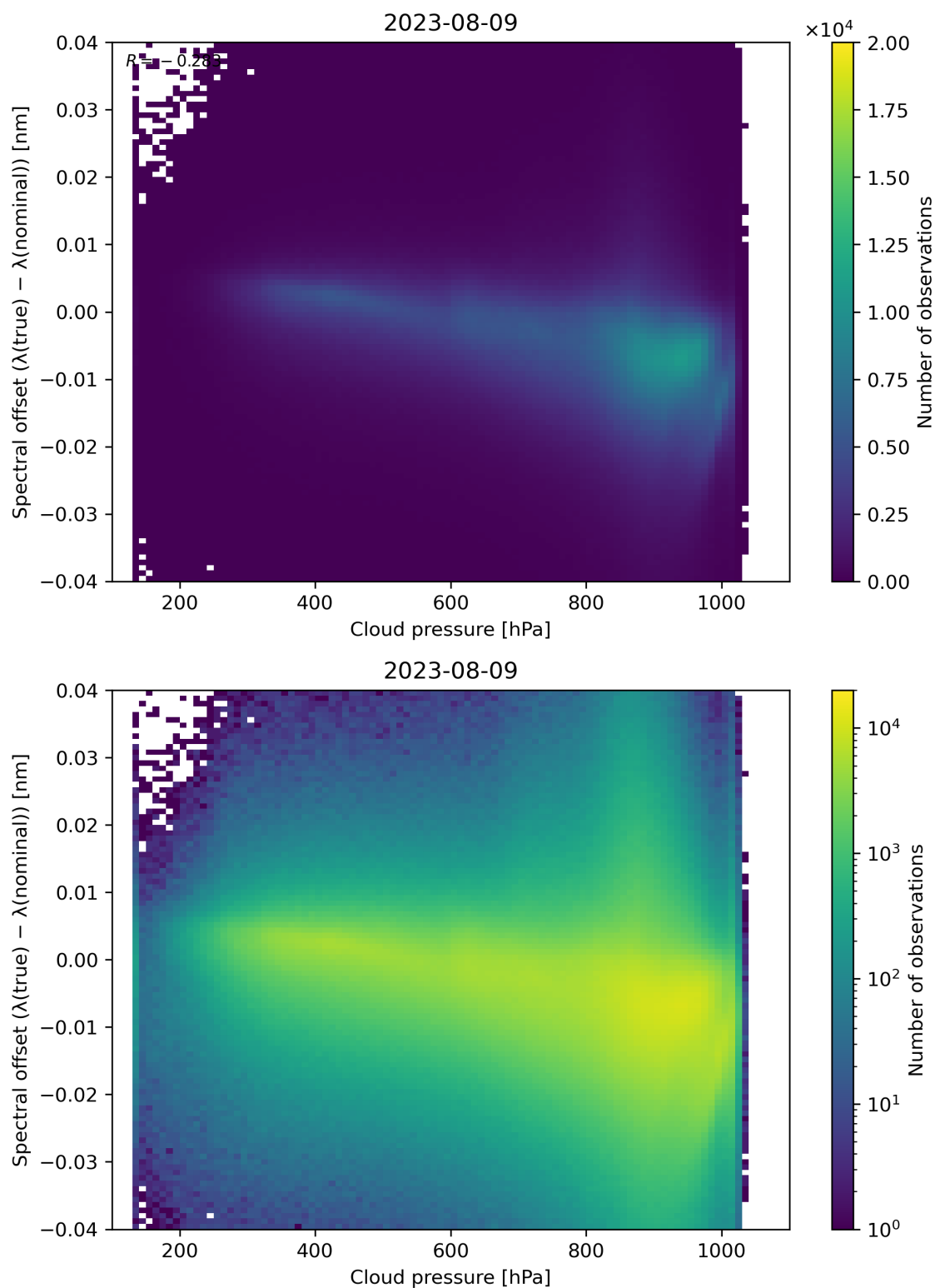
Figure 92: Scatter density plot of “Cloud pressure” against “Spectral offset ( \lambda(\text{true}) - \lambda(\text{nominal}) )” for 2023-08-09 to 2023-08-10.
