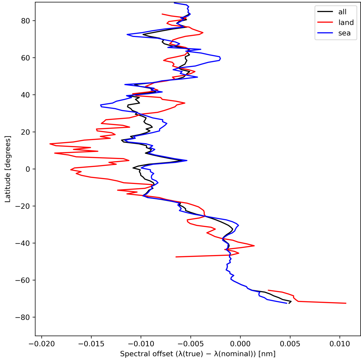
Figure 28: Zonal average of “Spectral offset ( \lambda(\text{true}) - \lambda(\text{nominal}) )” for 2023-08-09 to 2023-08-10.
