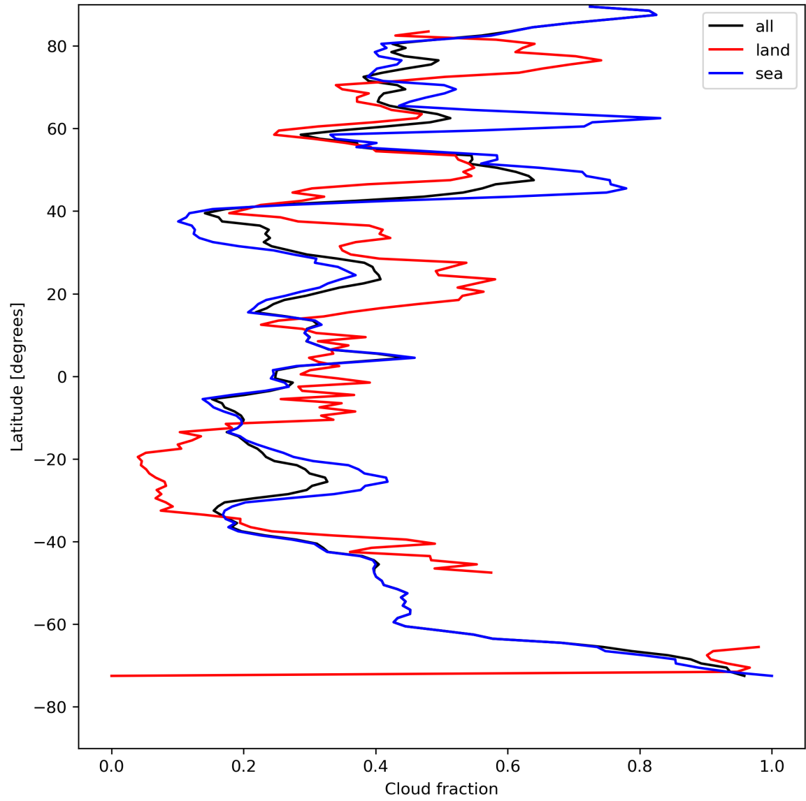
Figure 15: Zonal average of “Cloud fraction” for 2023-08-09 to 2023-08-10.
