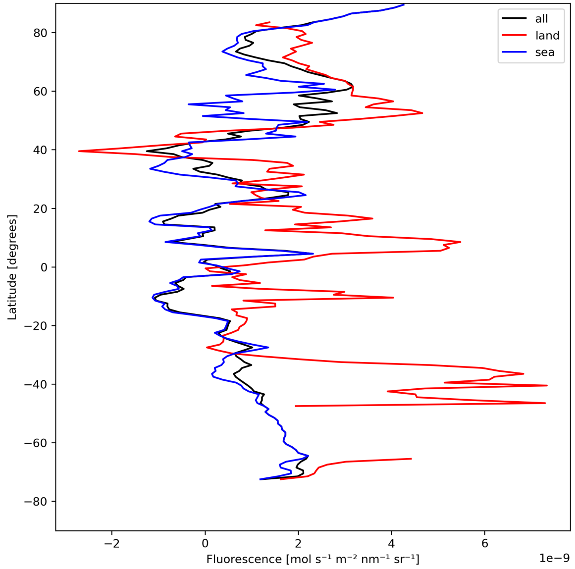
Figure 23: Zonal average of “Fluorescence” for 2023-08-09 to 2023-08-10.
