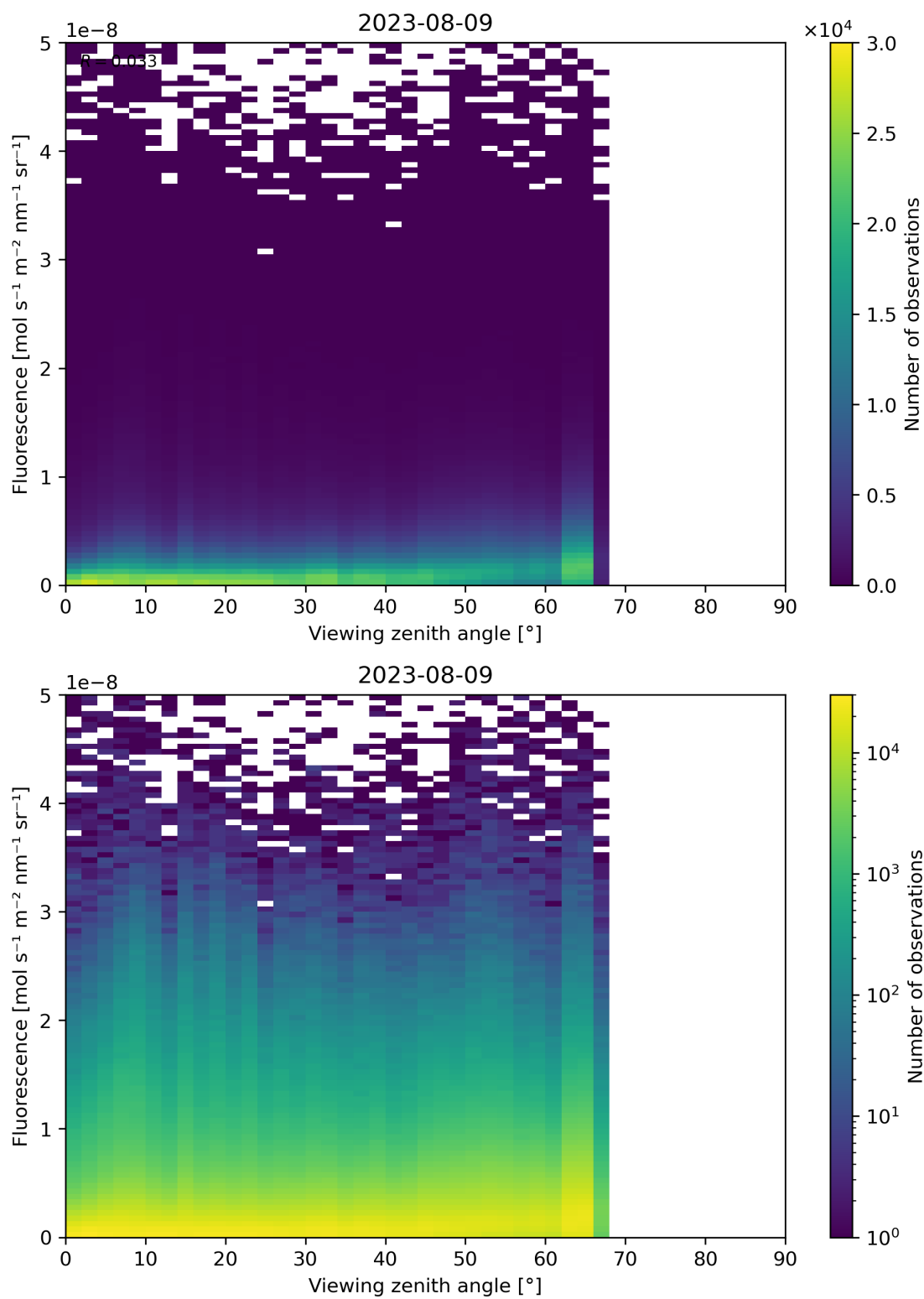
Figure 134: Scatter density plot of “Viewing zenith angle” against “Fluorescence” for 2023-08-09 to 2023-08-10.
