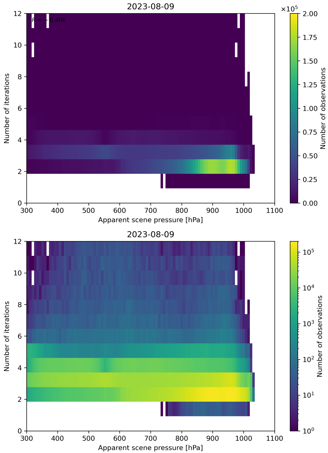
Figure 66: Scatter density plot of “Apparent scene pressure” against “Number of iterations” for 2023-08-09 to 2023-08-10.
