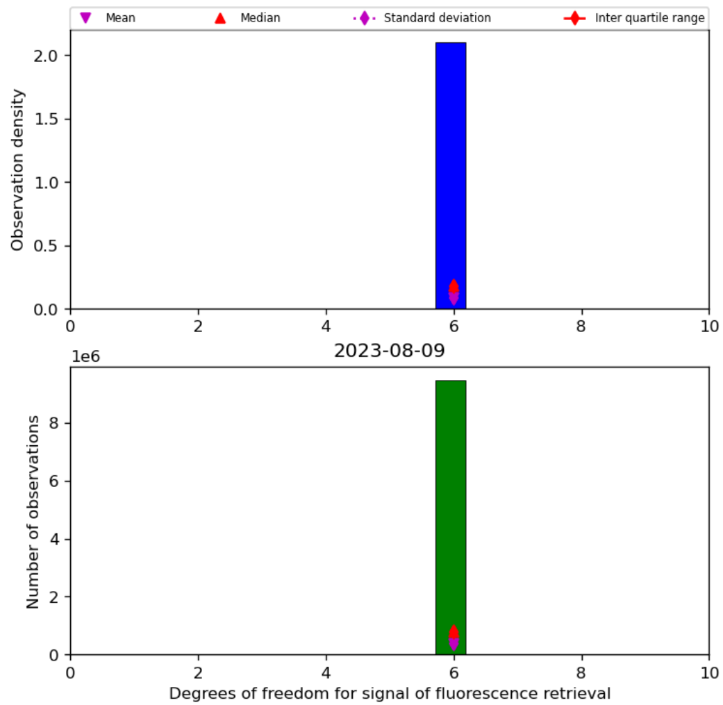
Figure 43: Histogram of “Degrees of freedom for signal of fluorescence retrieval” for 2023-08-09 to 2023-08-10
