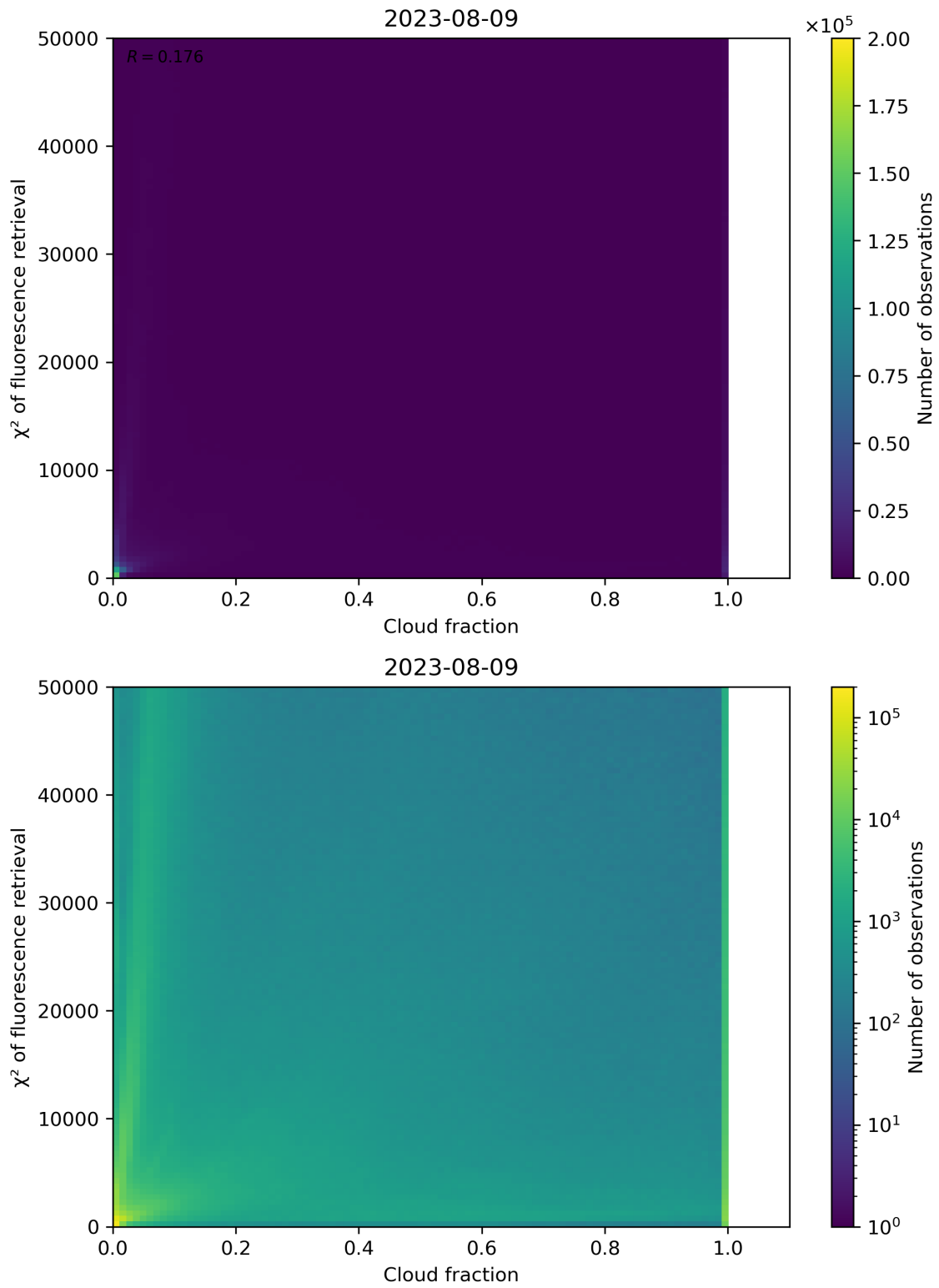
Figure 78: Scatter density plot of “Cloud fraction” against “ \chi^2 of fluorescence retrieval” for 2023-08-09 to 2023-08-10.
