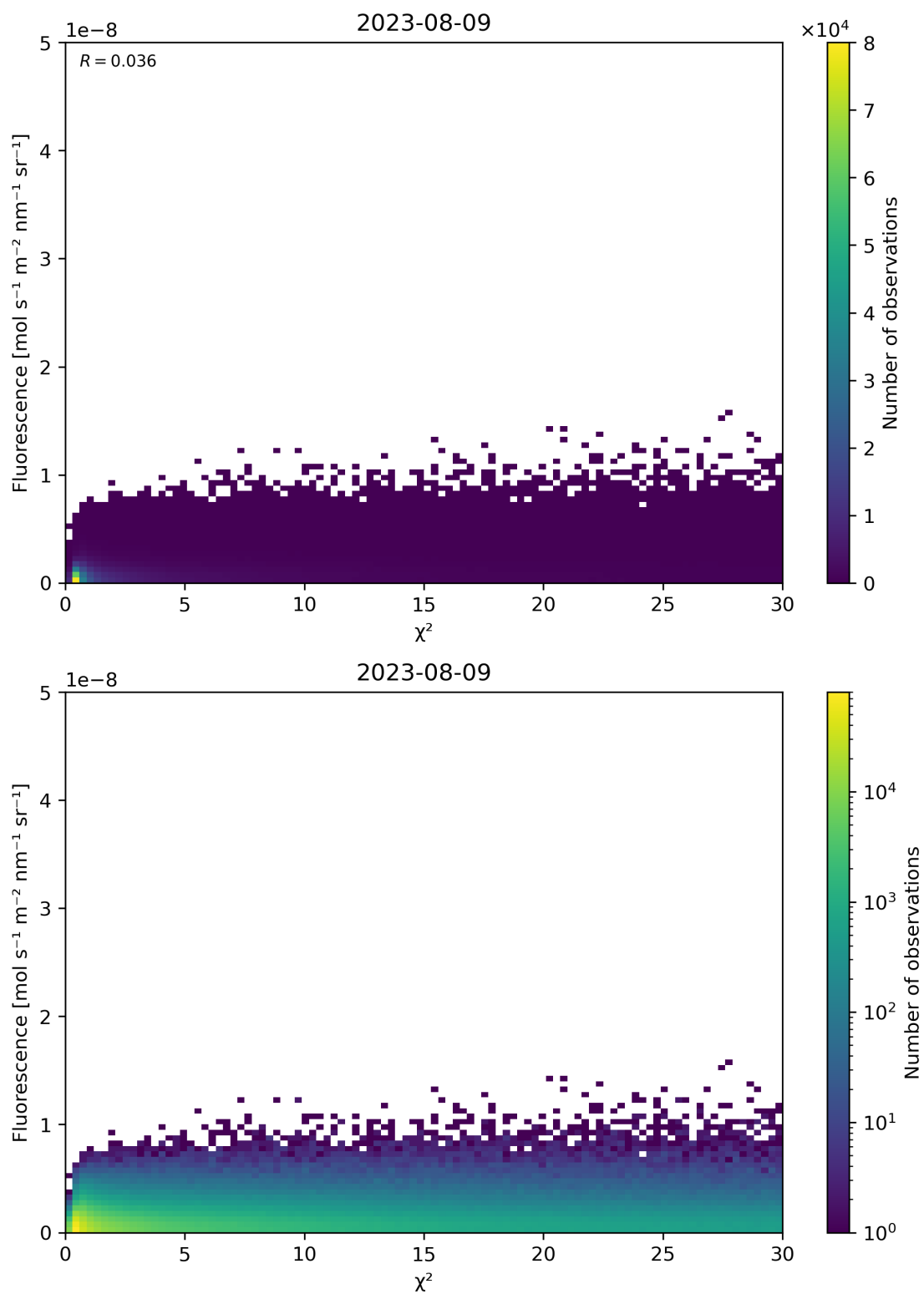
Figure 70: Scatter density plot of “ \chi^2 ” against “Fluorescence” for 2023-08-09 to 2023-08-10.
