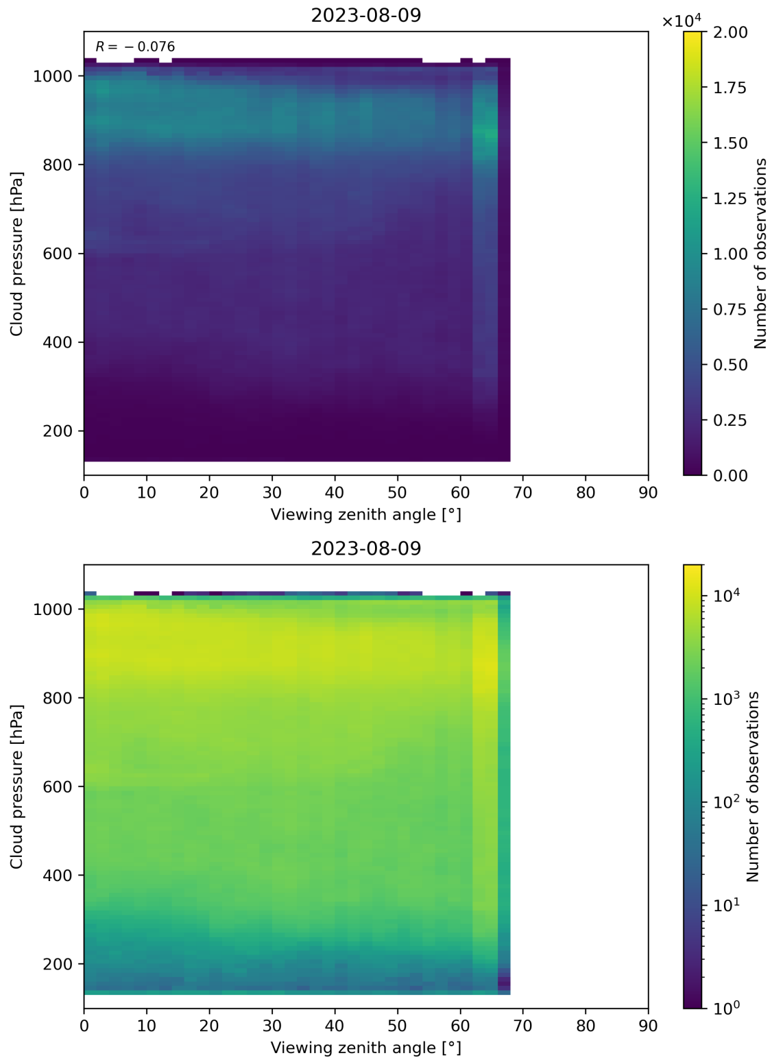
Figure 133: Scatter density plot of “Viewing zenith angle” against “Cloud pressure” for 2023-08-09 to 2023-08-10.
