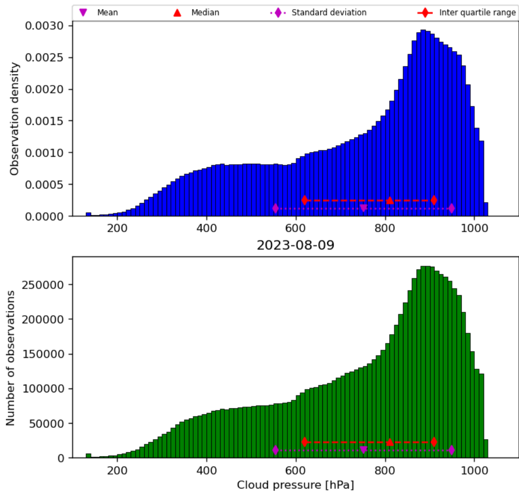
Figure 30: Histogram of “Cloud pressure” for 2023-08-09 to 2023-08-10
