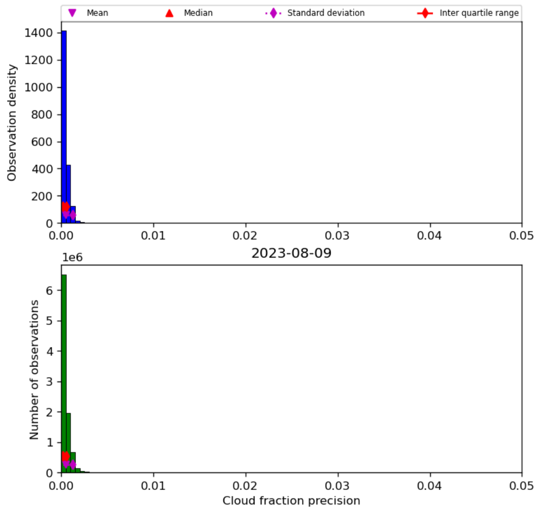
Figure 33: Histogram of “Cloud fraction precision” for 2023-08-09 to 2023-08-10
