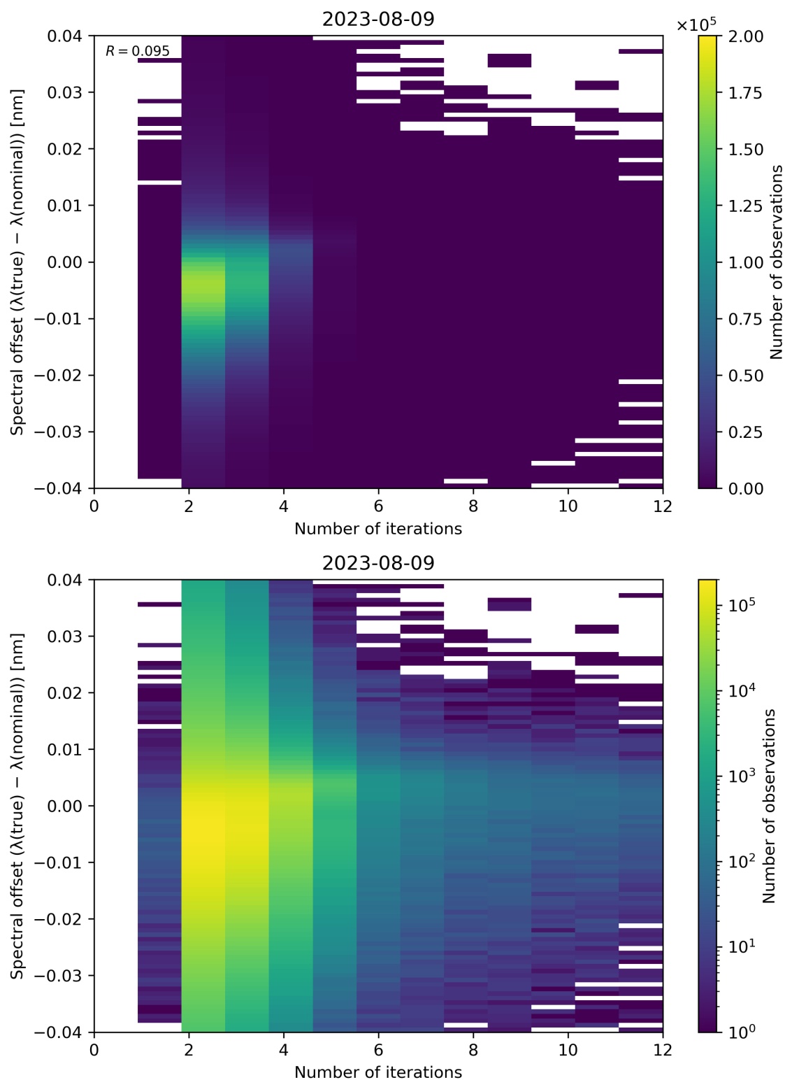
Figure 109: Scatter density plot of “Number of iterations” against “Spectral offset ( \lambda(\text{true}) - \lambda(\text{nominal}) )” for 2023-08-09 to 2023-08-10.
