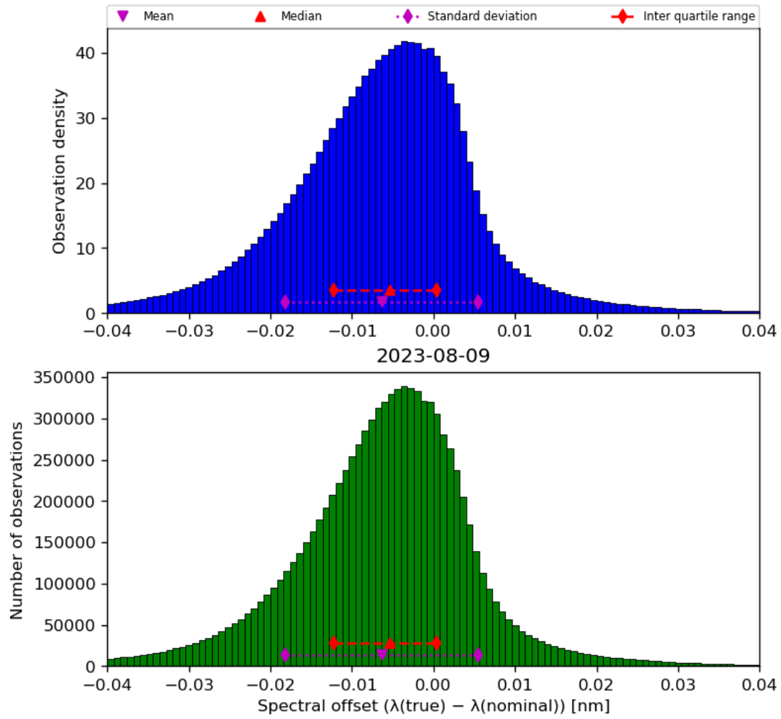
Figure 45: Histogram of “Spectral offset ( \lambda(\text{true}) - \lambda(\text{nominal}) )” for 2023-08-09 to 2023-08-10
