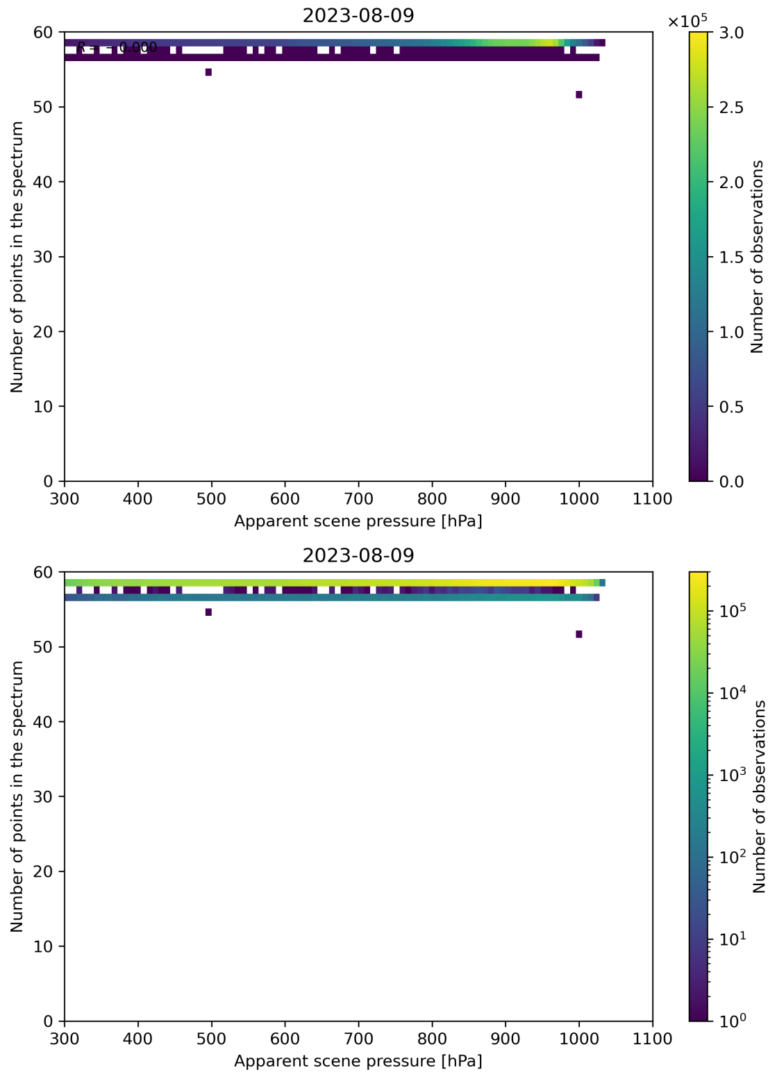
Figure 67: Scatter density plot of “Apparent scene pressure” against “Number of points in the spectrum” for 2023-08-09 to 2023-08-10.
