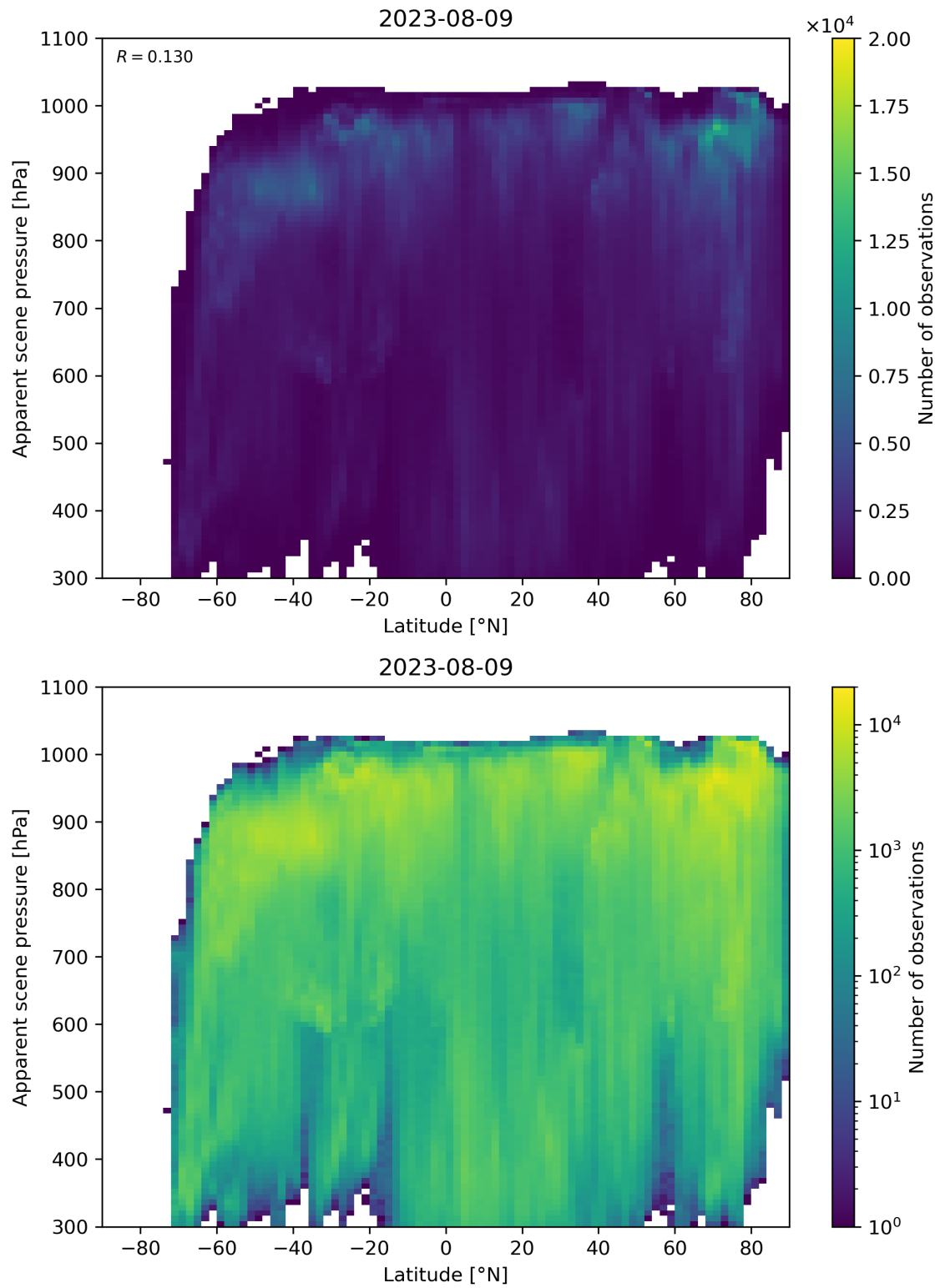
Figure 96: Scatter density plot of “Latitude” against “Apparent scene pressure” for 2023-08-09 to 2023-08-10.
