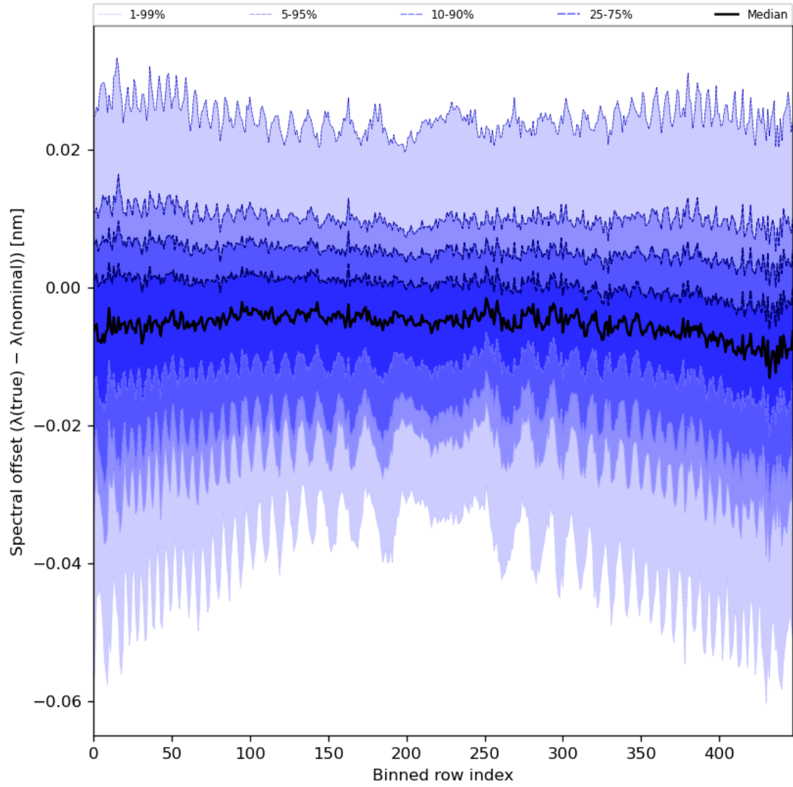
Figure 62: Along track statistics of “Spectral offset ( \lambda(\text{true}) - \lambda(\text{nominal}) )” for 2023-08-09 to 2023-08-10
