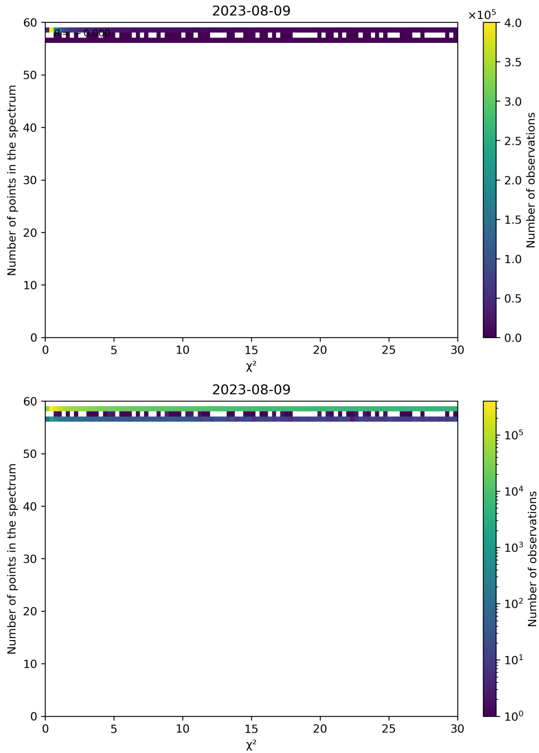
Figure 74: Scatter density plot of " \chi^2 " against "Number of points in the spectrum" for 2023-08-09 to 2023-08-10.
