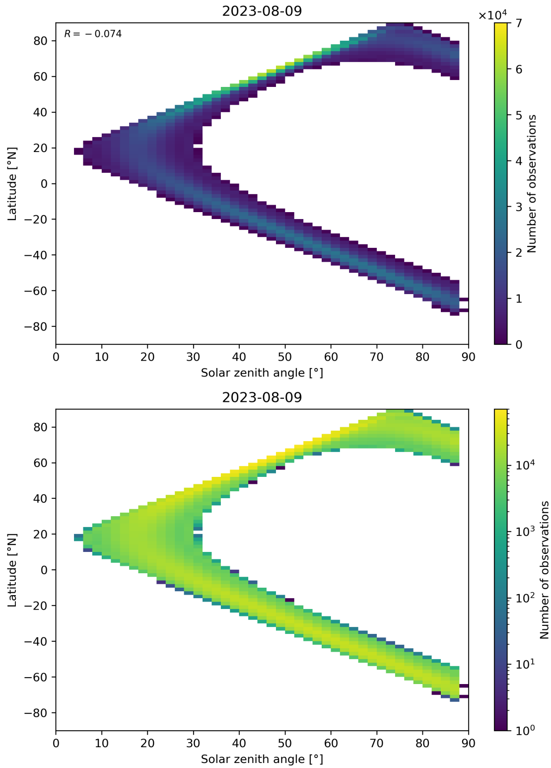
Figure 124: Scatter density plot of “Solar zenith angle” against “Latitude” for 2023-08-09 to 2023-08-10.
