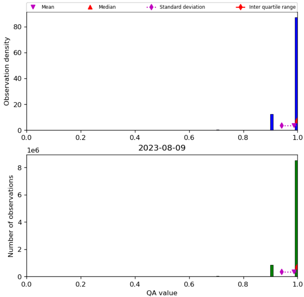
Figure 29: Histogram of “QA value” for 2023-08-09 to 2023-08-10
