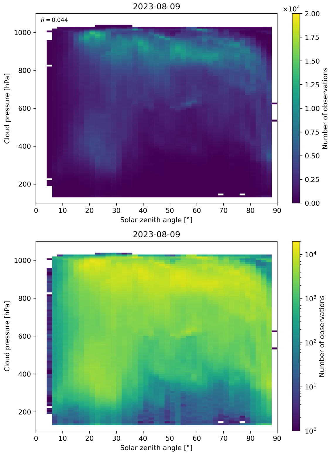
Figure 122: Scatter density plot of “Solar zenith angle” against “Cloud pressure” for 2023-08-09 to 2023-08-10.
