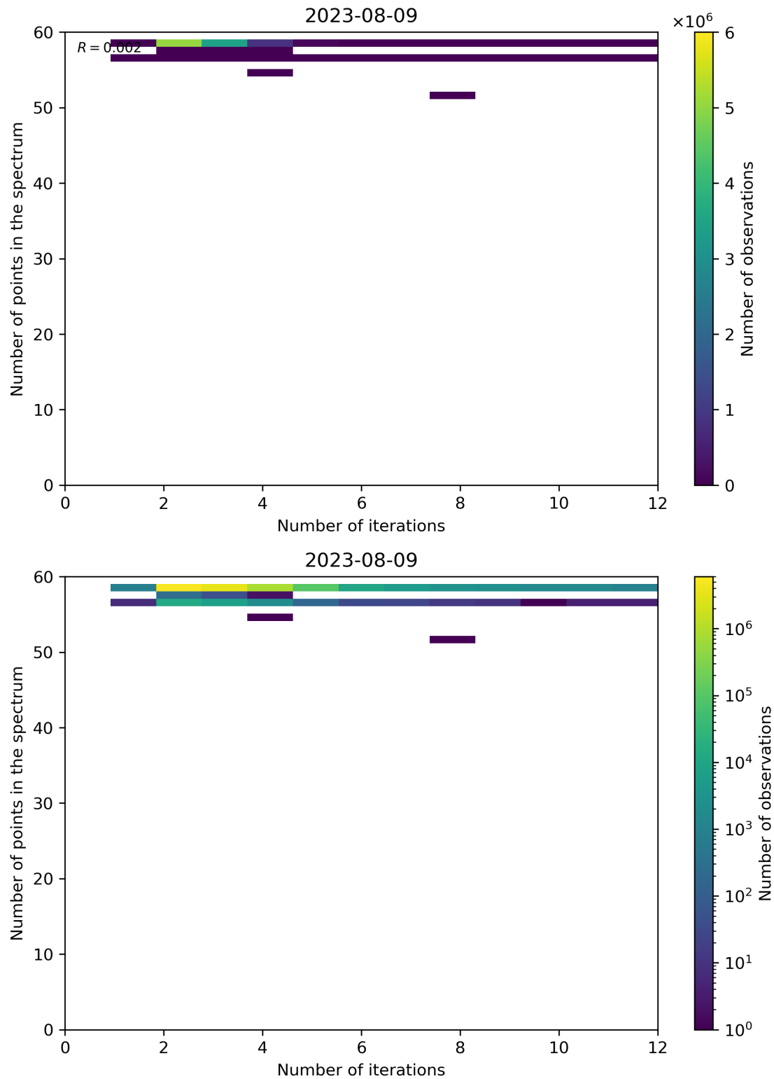
Figure 108: Scatter density plot of “Number of iterations” against “Number of points in the spectrum” for 2023-08-09 to 2023-08-10.
