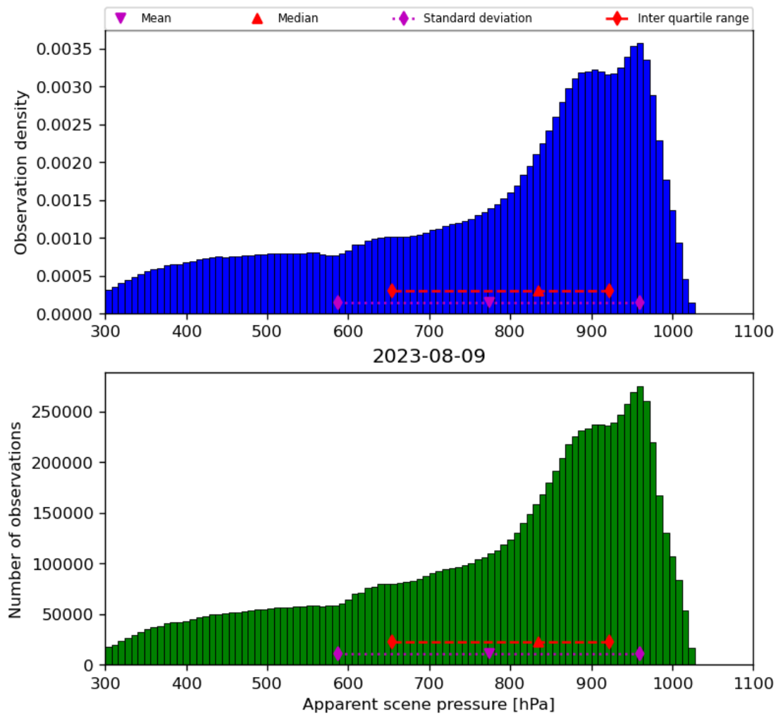
Figure 36: Histogram of “Apparent scene pressure” for 2023-08-09 to 2023-08-10
