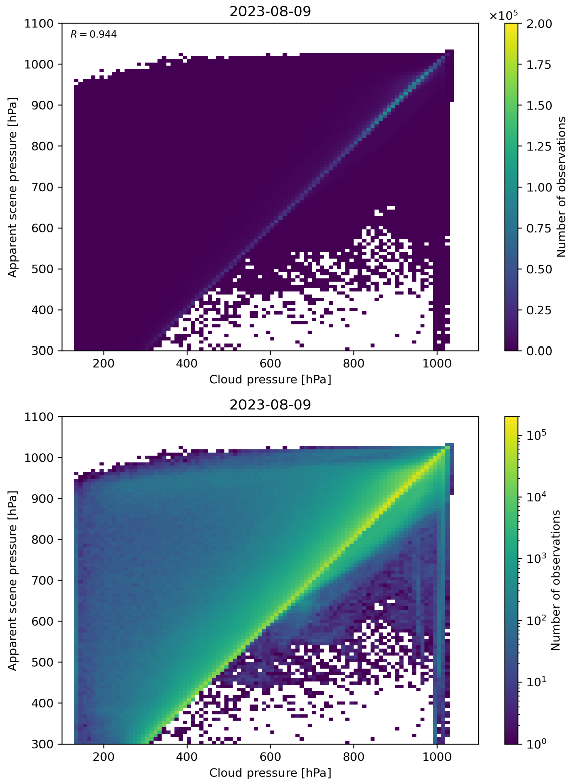
Figure 84: Scatter density plot of “Cloud pressure” against “Apparent scene pressure” for 2023-08-09 to 2023-08-10.
