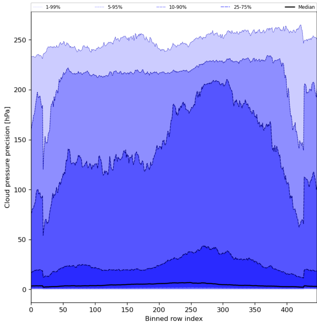
Figure 48: Along track statistics of “Cloud pressure precision” for 2023-08-09 to 2023-08-10
