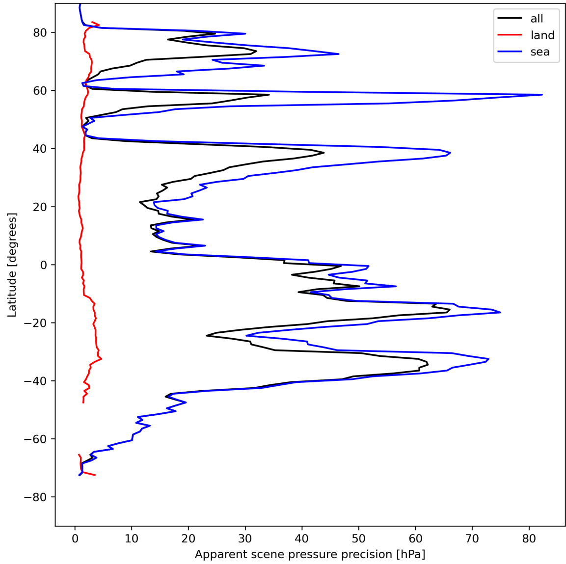
Figure 20: Zonal average of “Apparent scene pressure precision” for 2023-08-09 to 2023-08-10.
