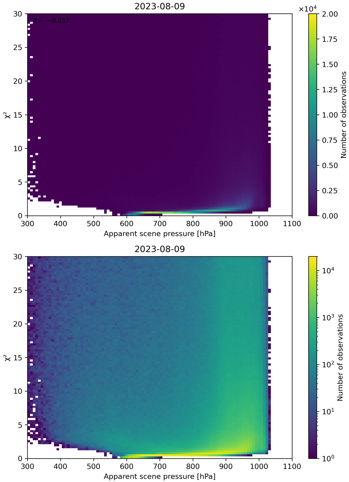
Figure 63: Scatter density plot of “Apparent scene pressure” against “ \chi^2 ” for 2023-08-09 to 2023-08-10.
