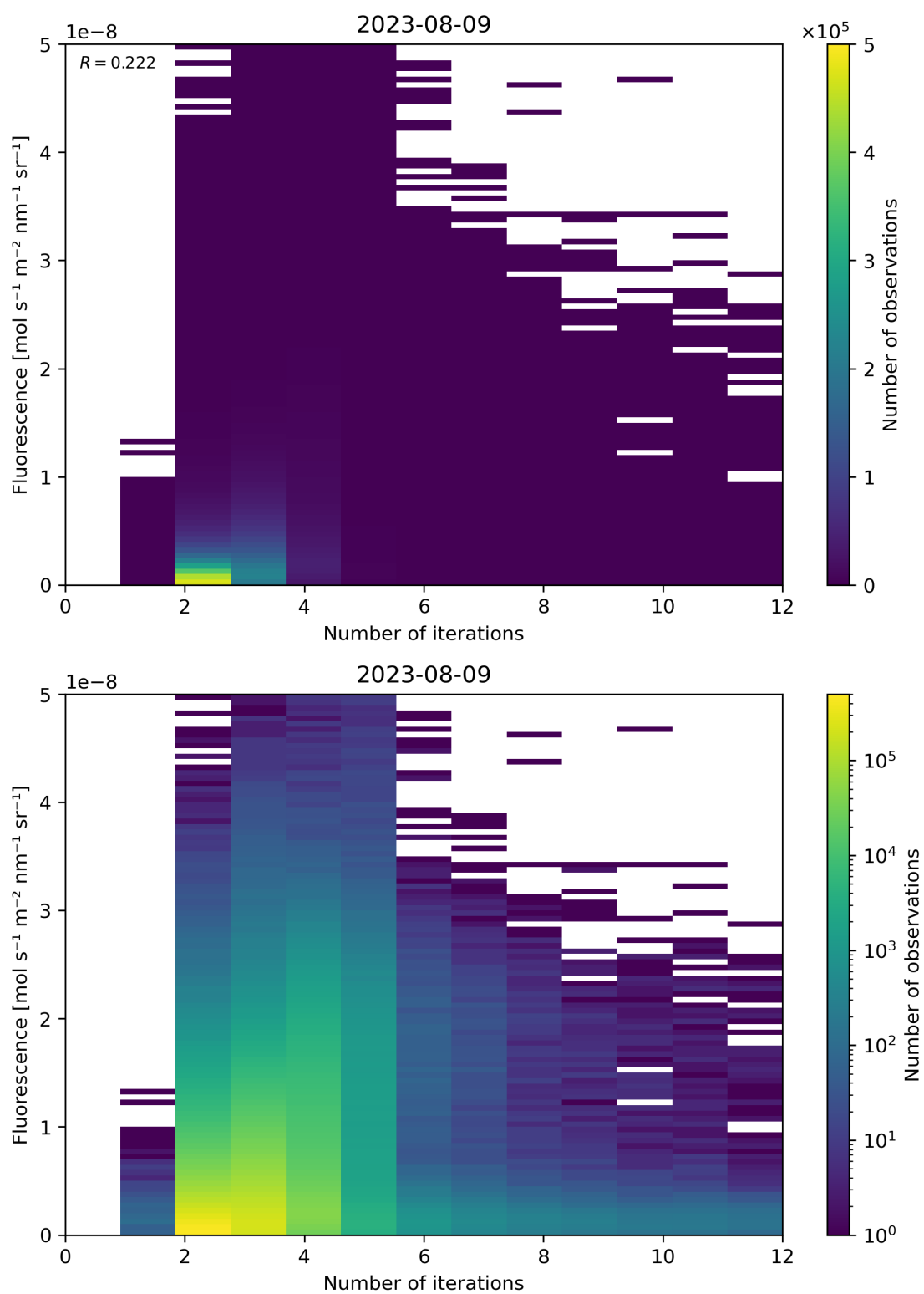
Figure 107: Scatter density plot of “Number of iterations” against “Fluorescence” for 2023-08-09 to 2023-08-10.
