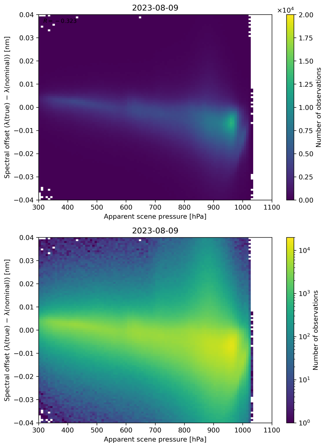
Figure 68: Scatter density plot of “Apparent scene pressure” against “Spectral offset ( \lambda(\text{true}) - \lambda(\text{nominal}) )” for 2023-08-09 to 2023-08-10.
