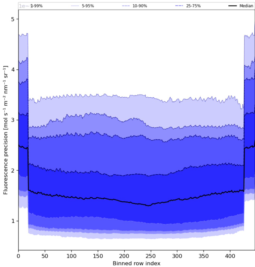
Figure 58: Along track statistics of “Fluorescence precision” for 2023-08-09 to 2023-08-10
