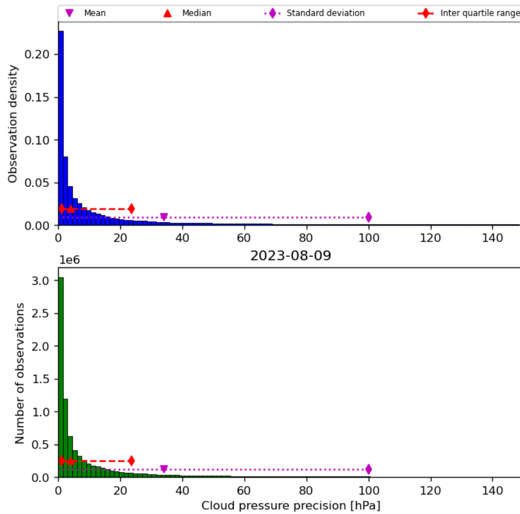
Figure 31: Histogram of “Cloud pressure precision” for 2023-08-09 to 2023-08-10
