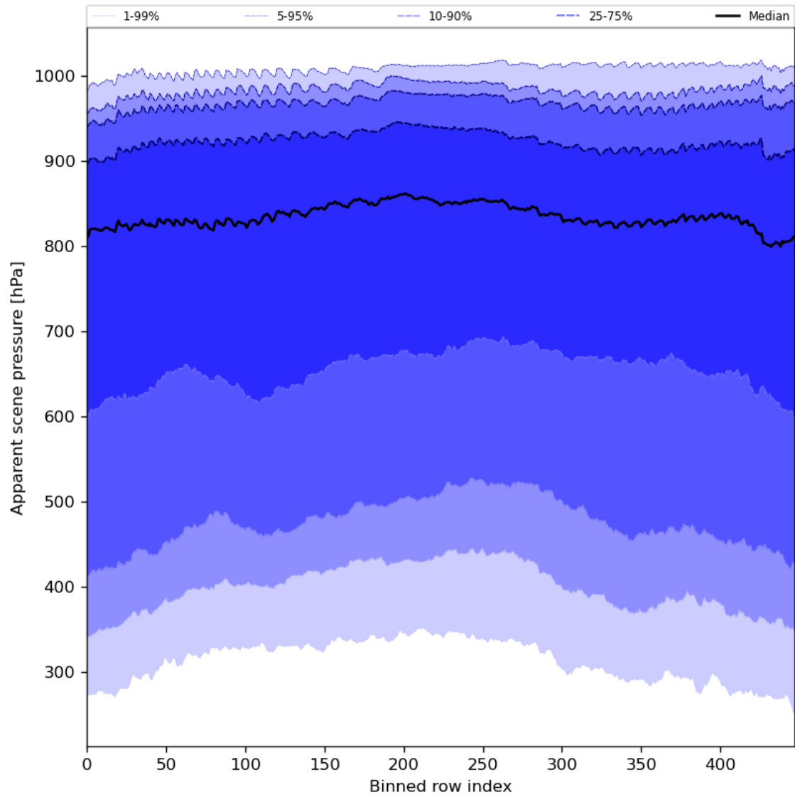
Figure 53: Along track statistics of “Apparent scene pressure” for 2023-08-09 to 2023-08-10
