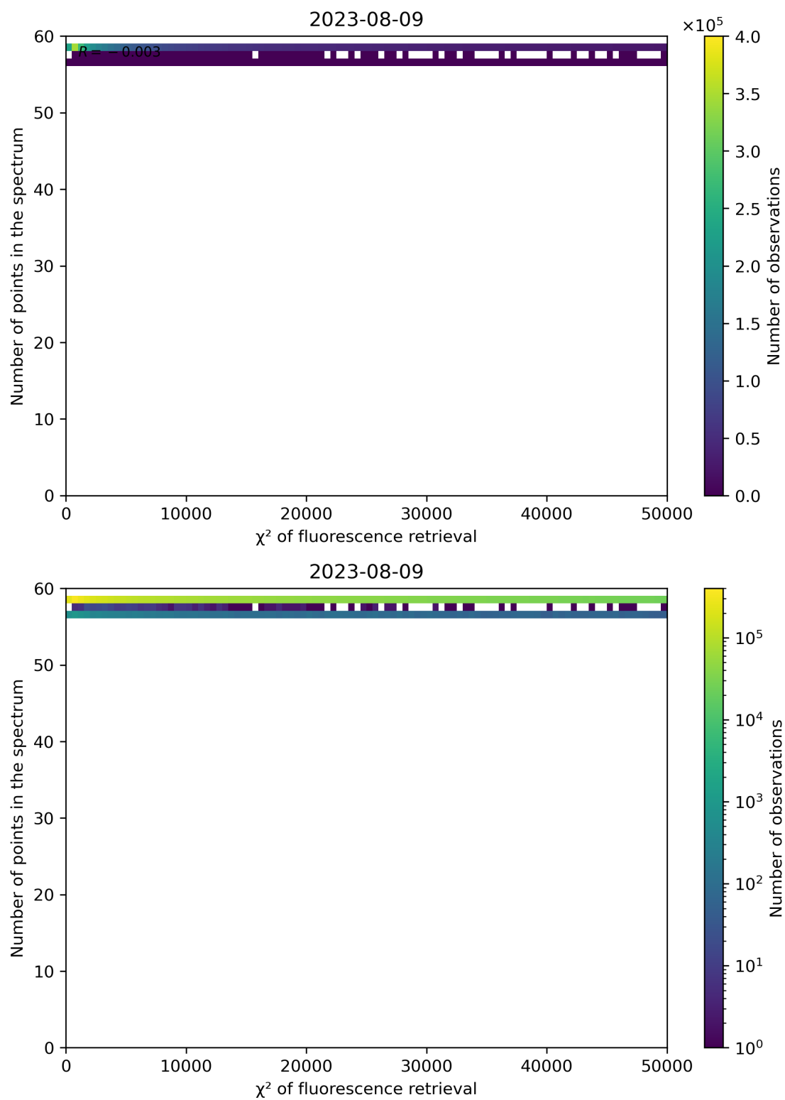
Figure 71: Scatter density plot of “ \chi^2 of fluorescence retrieval” against “Number of points in the spectrum” for 2023-08-09 to 2023-08-10.
