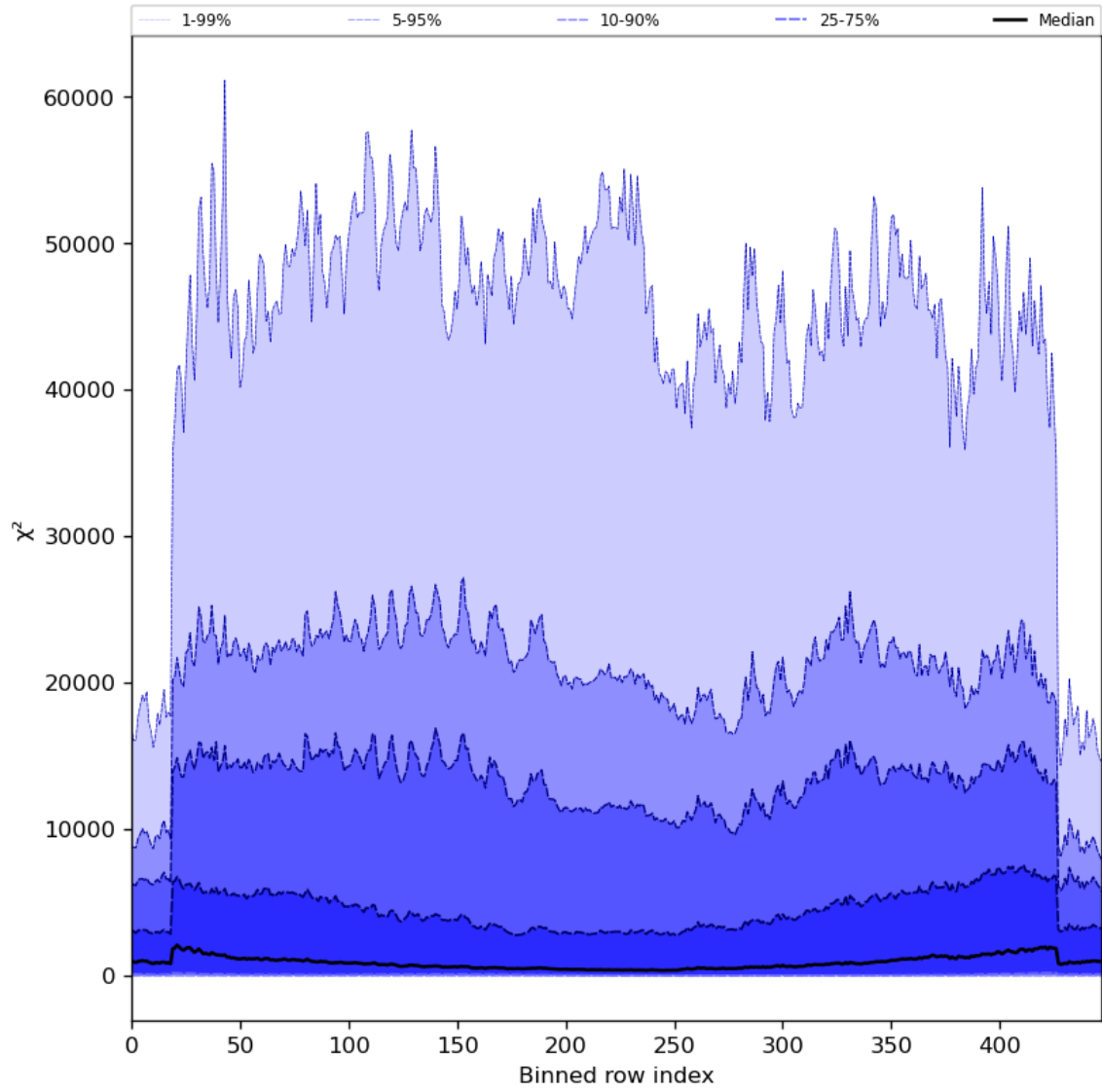
Figure 55: Along track statistics of “ \chi^2 ” for 2023-08-09 to 2023-08-10
