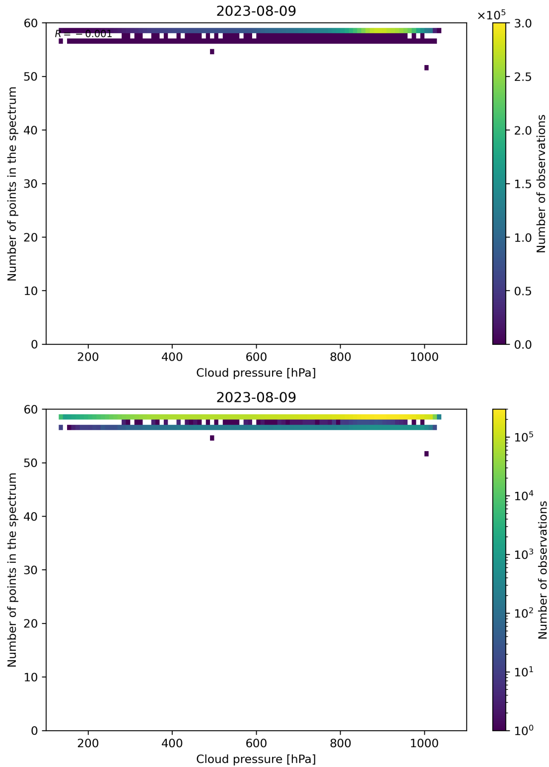
Figure 90: Scatter density plot of “Cloud pressure” against “Number of points in the spectrum” for 2023-08-09 to 2023-08-10.
