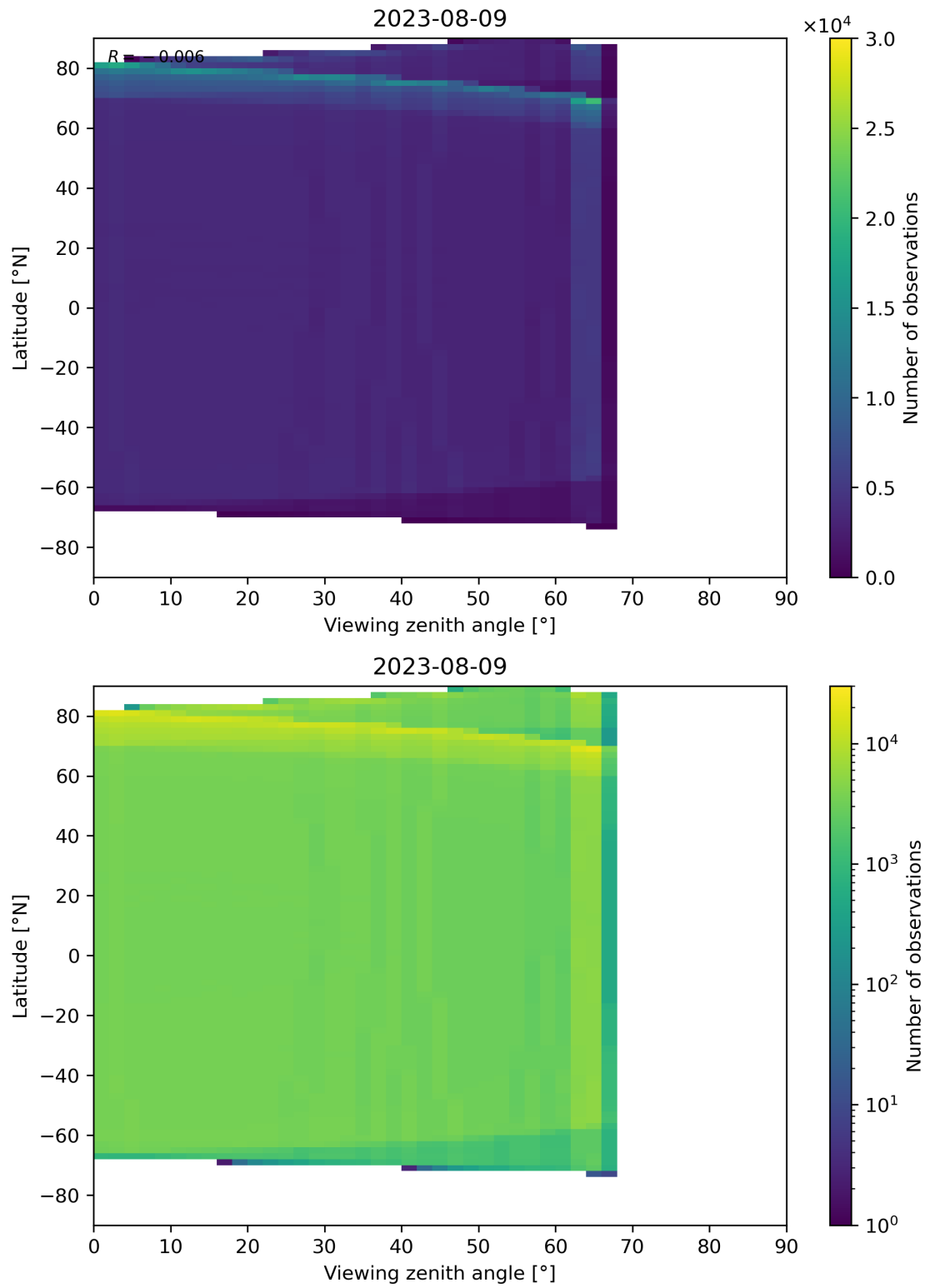
Figure 135: Scatter density plot of “Viewing zenith angle” against “Latitude” for 2023-08-09 to 2023-08-10.
