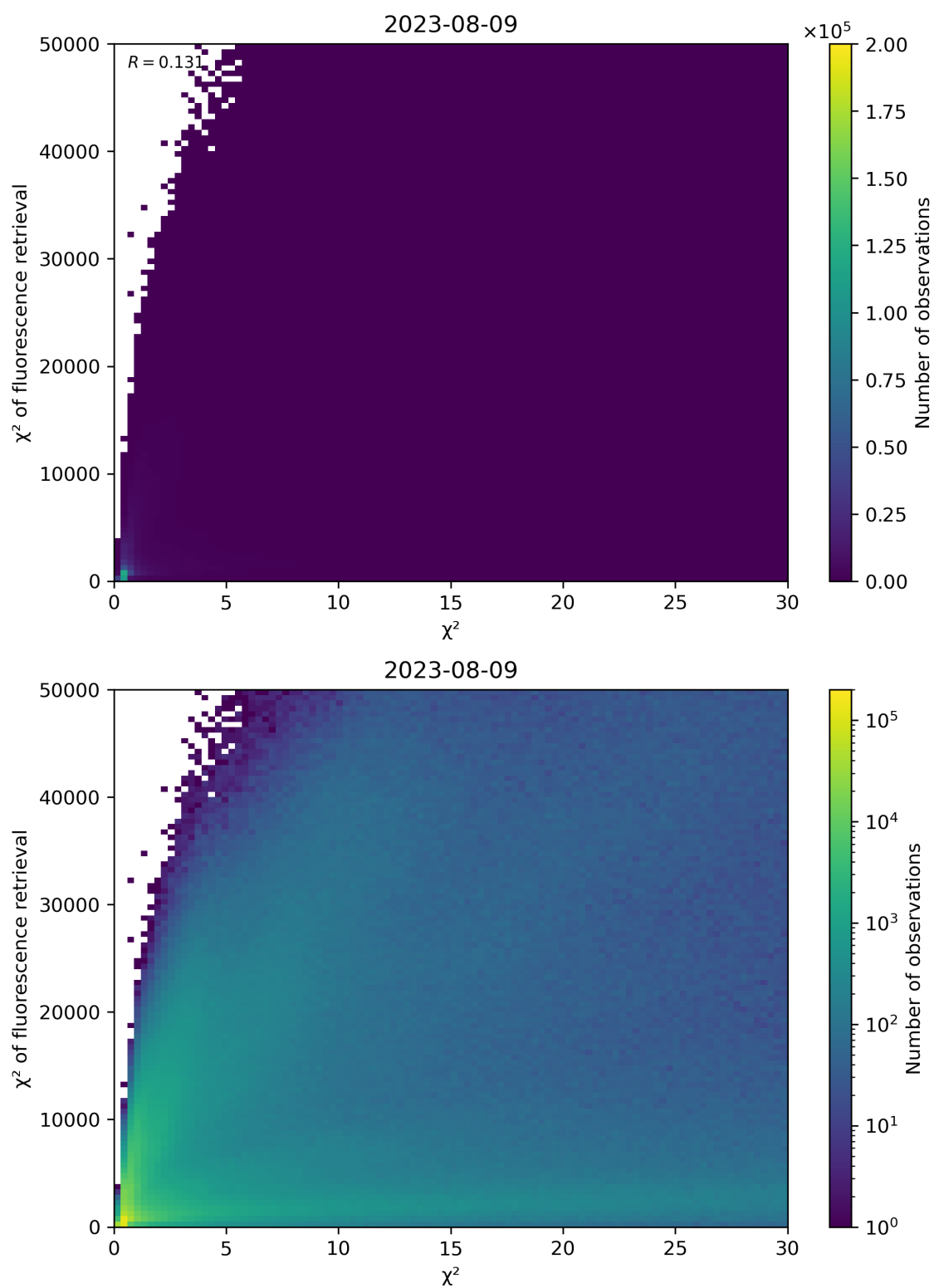
Figure 69: Scatter density plot of “ \chi^2 ” against “ \chi^2 of fluorescence retrieval” for 2023-08-09 to 2023-08-10.
