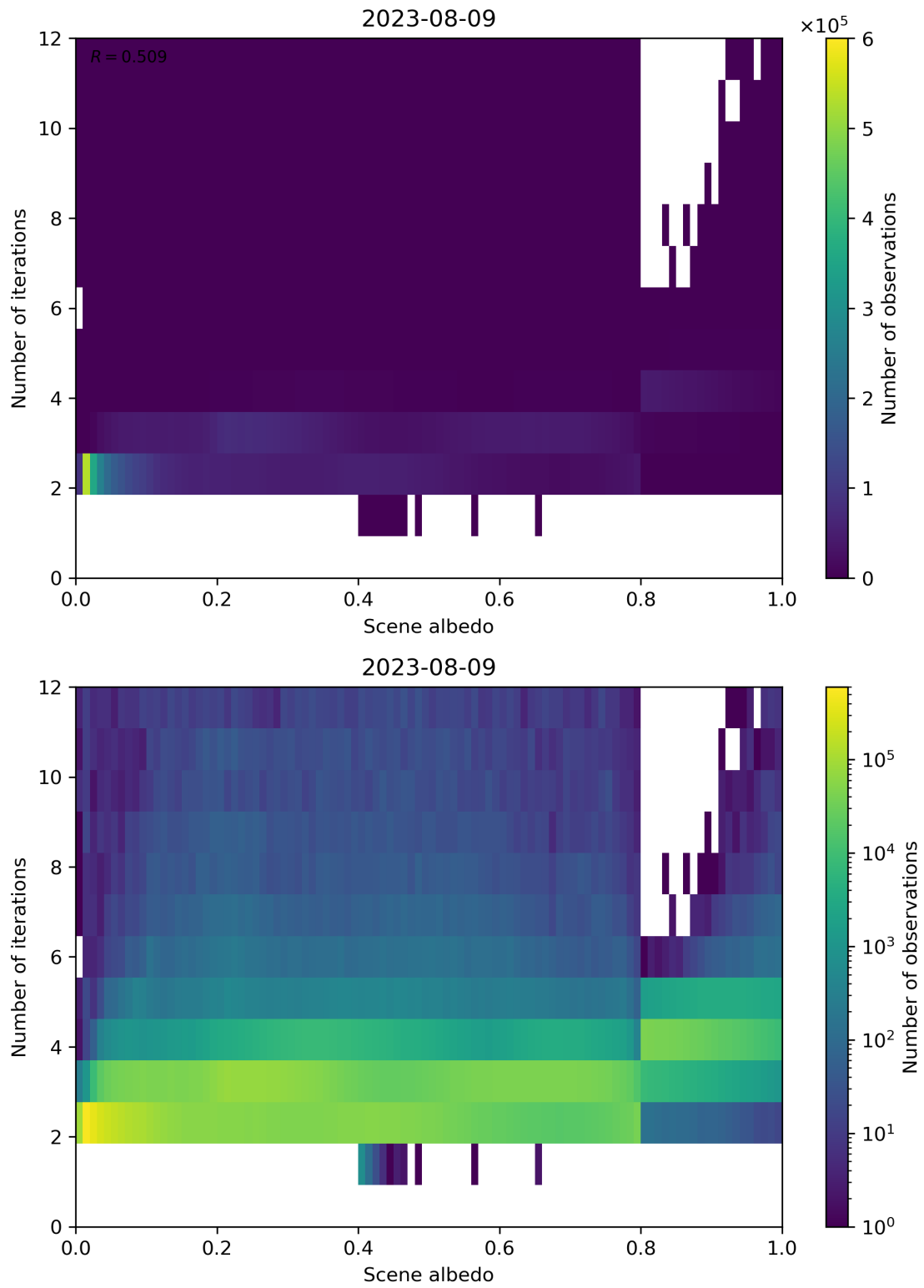
Figure 115: Scatter density plot of “Scene albedo” against “Number of iterations” for 2023-08-09 to 2023-08-10.
