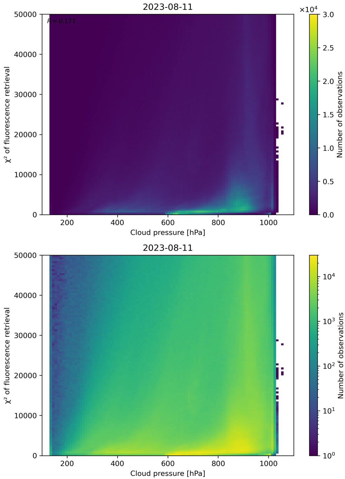
Figure 86: Scatter density plot of “Cloud pressure” against “ \chi^2 of fluorescence retrieval” for 2023-08-10 to 2023-08-12.
