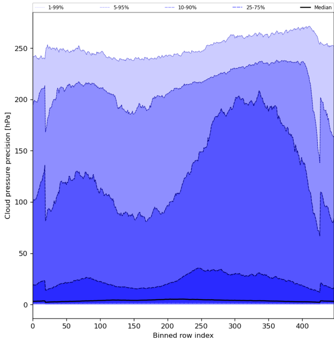
Figure 48: Along track statistics of “Cloud pressure precision” for 2023-08-10 to 2023-08-12
