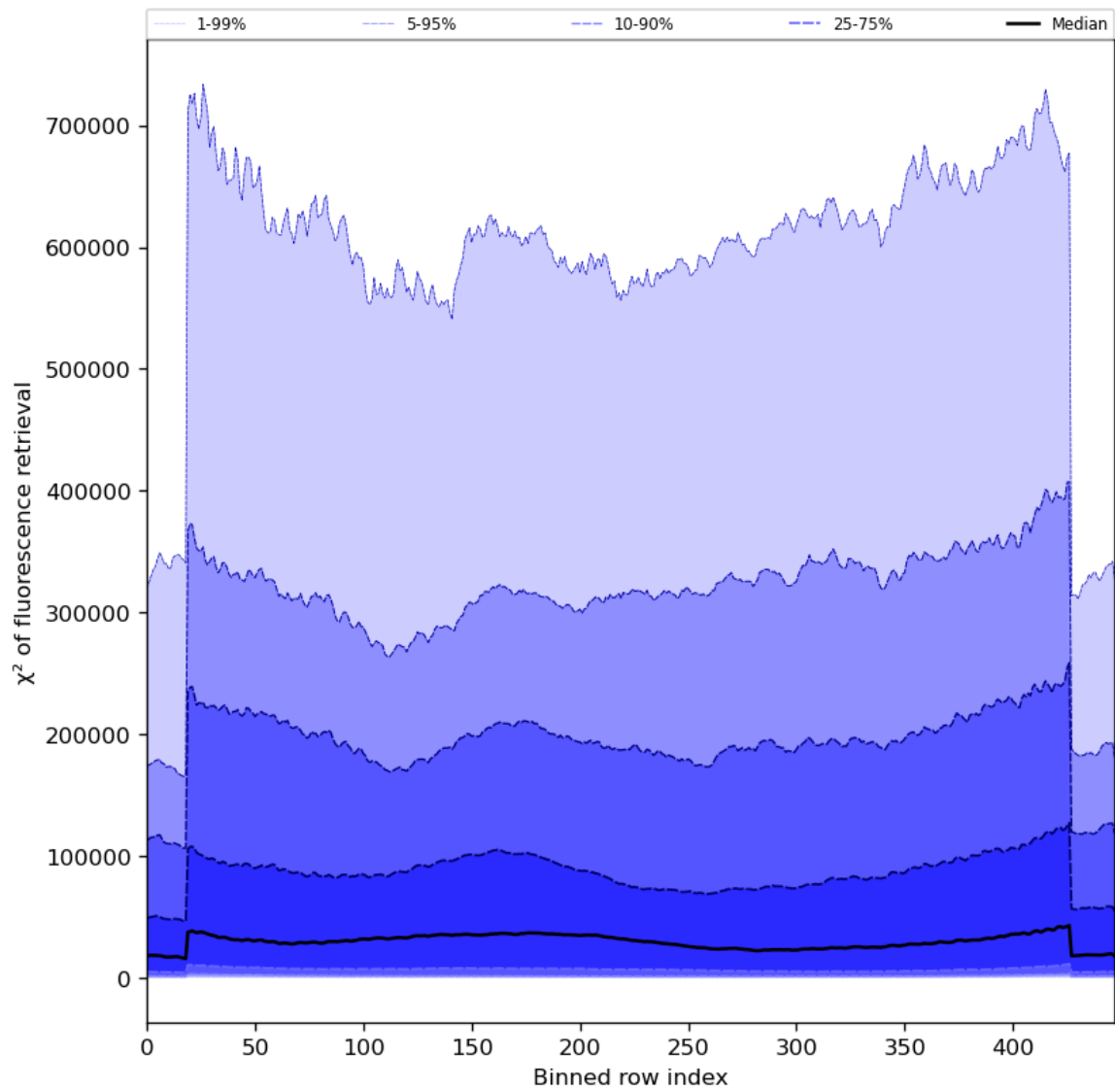
Figure 59: Along track statistics of “ \chi^2 of fluorescence retrieval” for 2023-08-10 to 2023-08-12
