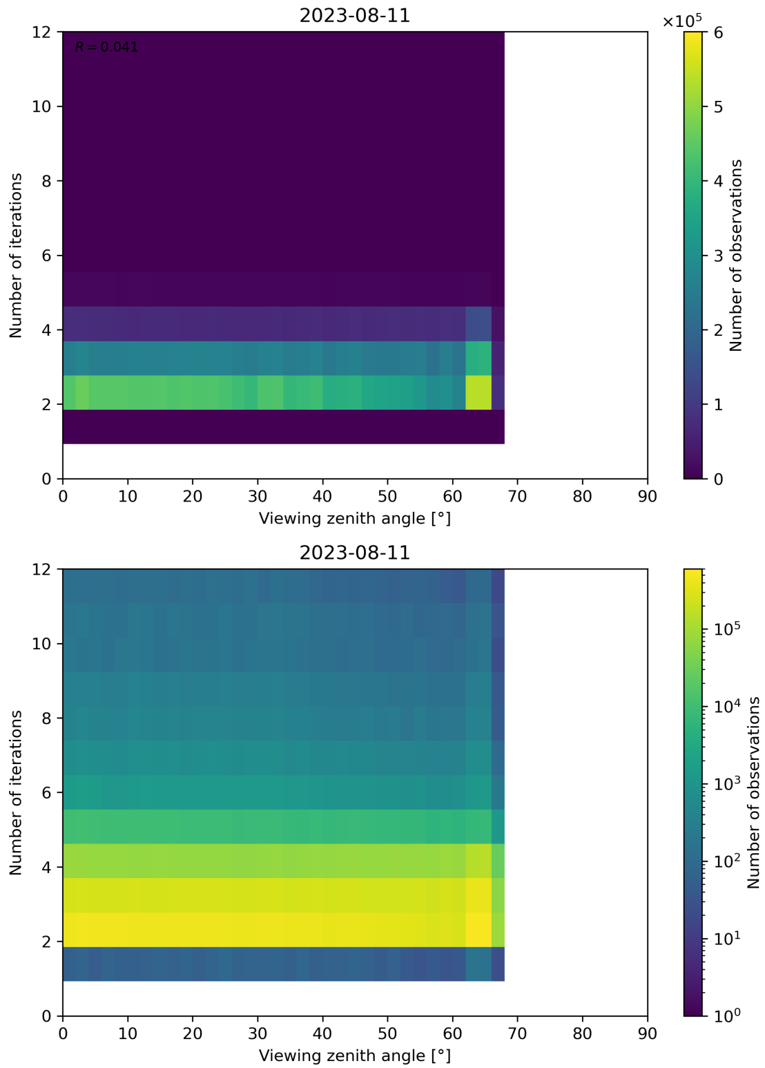
Figure 136: Scatter density plot of “Viewing zenith angle” against “Number of iterations” for 2023-08-10 to 2023-08-12.
