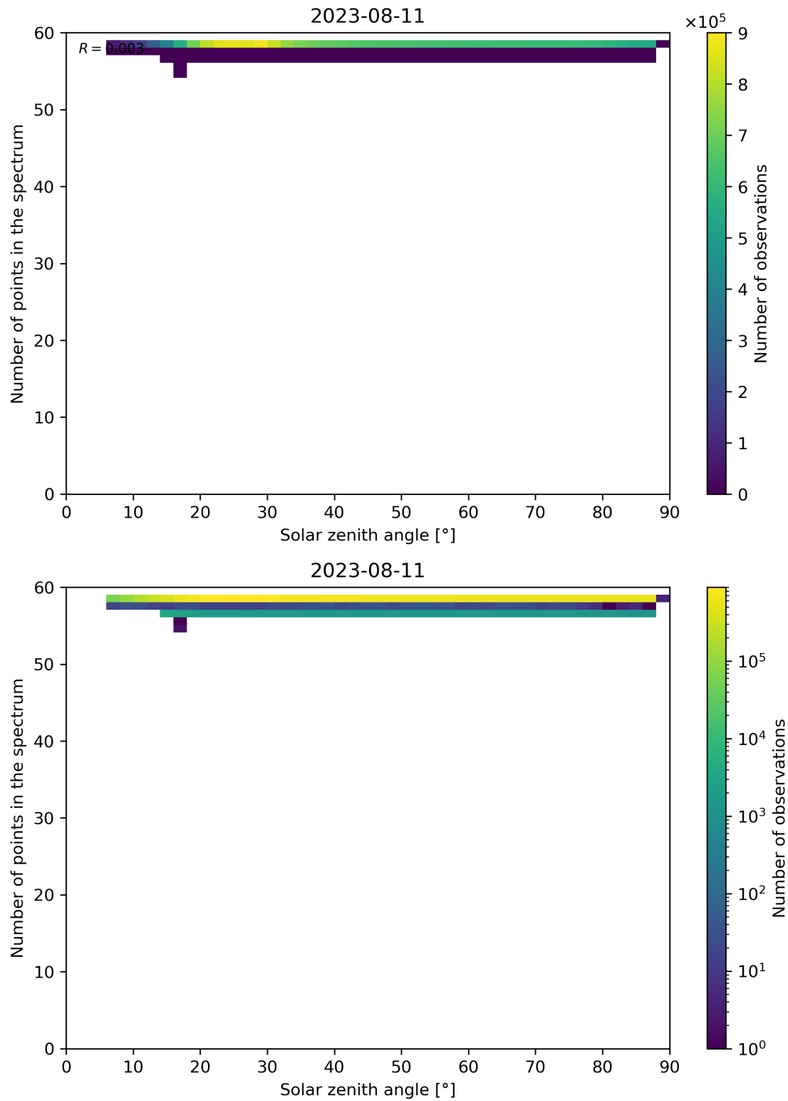
Figure 126: Scatter density plot of “Solar zenith angle” against “Number of points in the spectrum” for 2023-08-10 to 2023-08-12.
