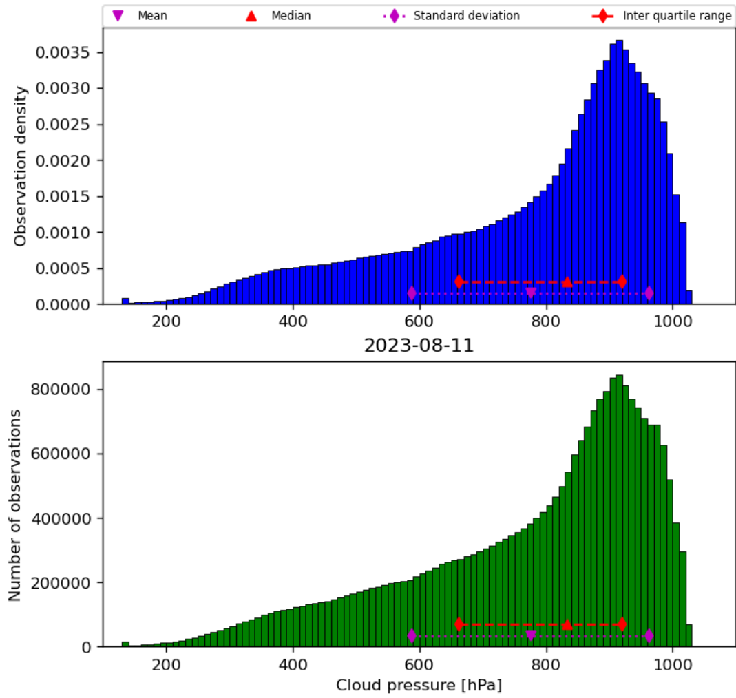
Figure 30: Histogram of “Cloud pressure” for 2023-08-10 to 2023-08-12
