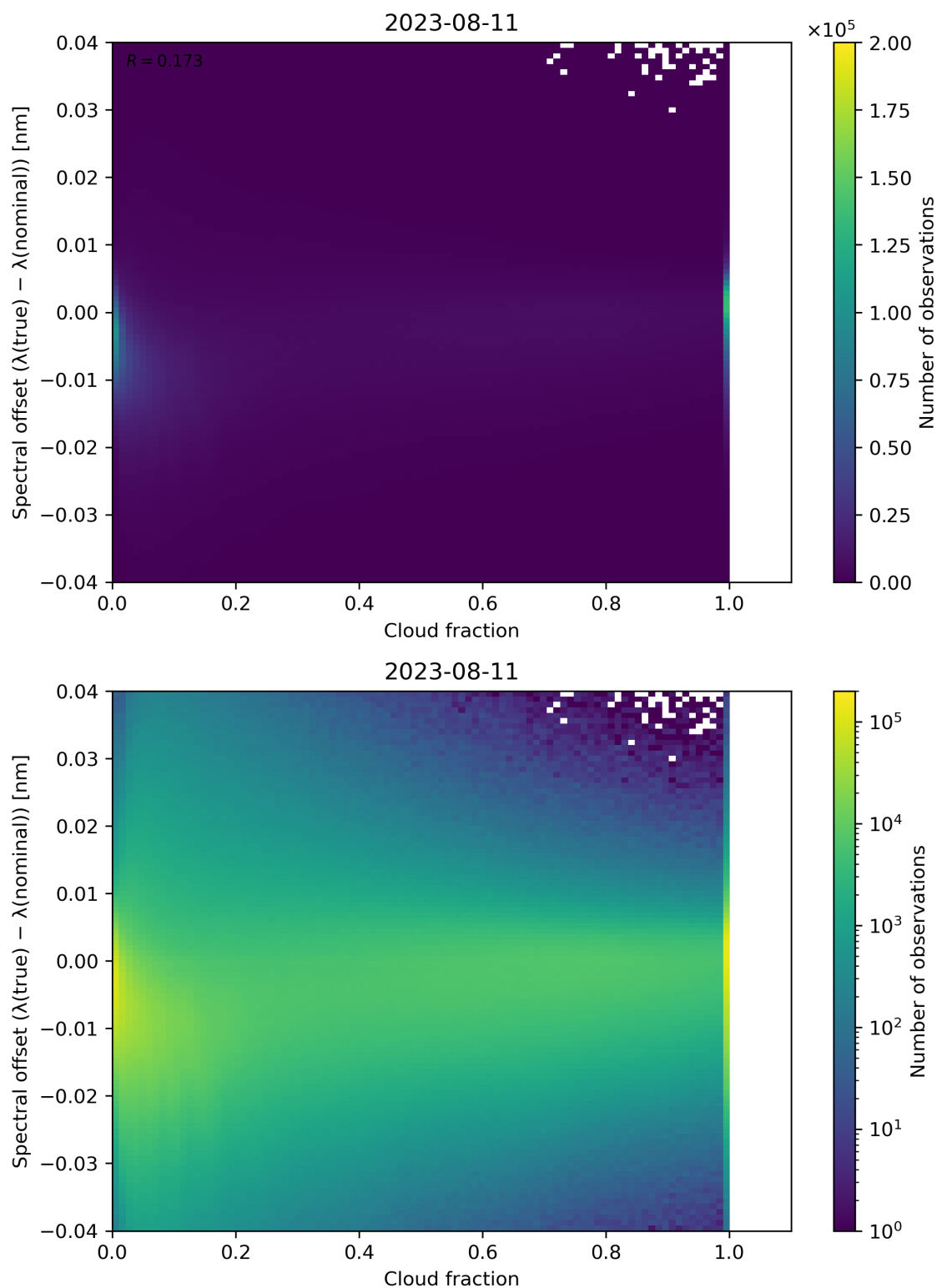
Figure 83: Scatter density plot of “Cloud fraction” against “Spectral offset ( \lambda(\text{true}) - \lambda(\text{nominal}) )” for 2023-08-10 to 2023-08-12.
