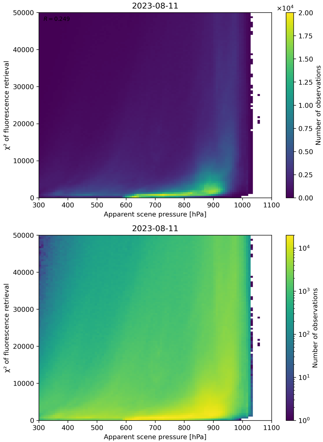
Figure 64: Scatter density plot of “Apparent scene pressure” against “ \chi^2 of fluorescence retrieval” for 2023-08-10 to 2023-08-12.
