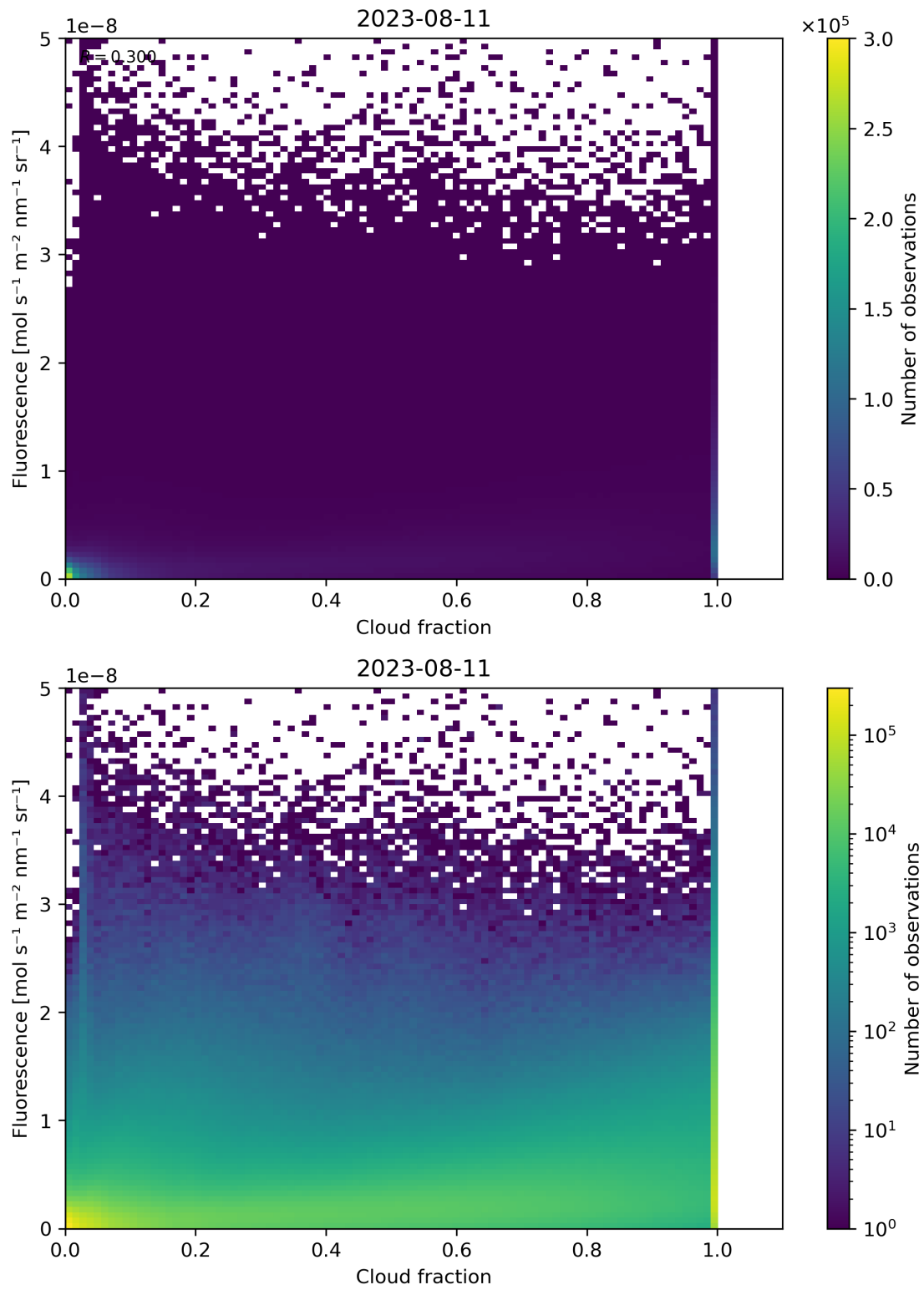
Figure 79: Scatter density plot of “Cloud fraction” against “Fluorescence” for 2023-08-10 to 2023-08-12.
