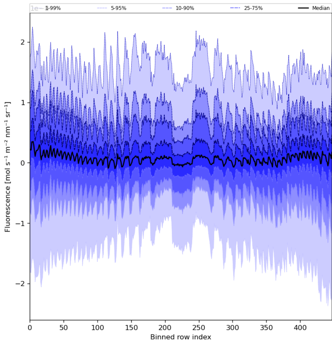
Figure 57: Along track statistics of “Fluorescence” for 2023-08-10 to 2023-08-12
