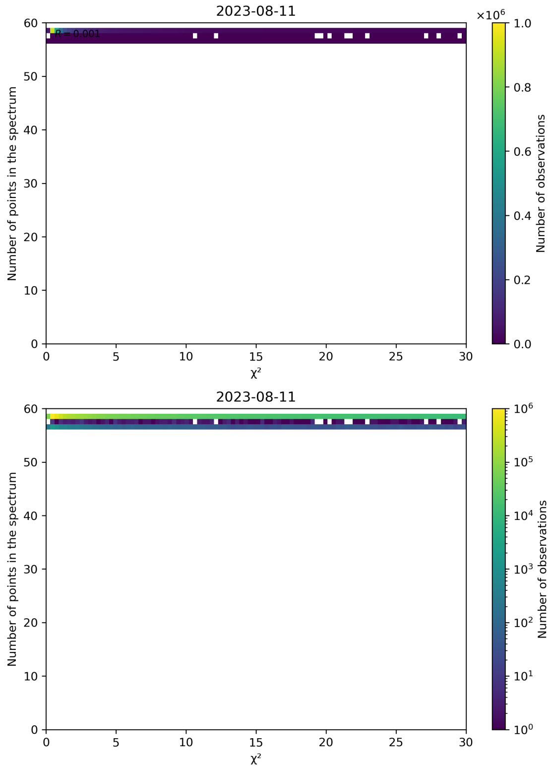
Figure 74: Scatter density plot of “ \chi^2 ” against “Number of points in the spectrum” for 2023-08-10 to 2023-08-12.
