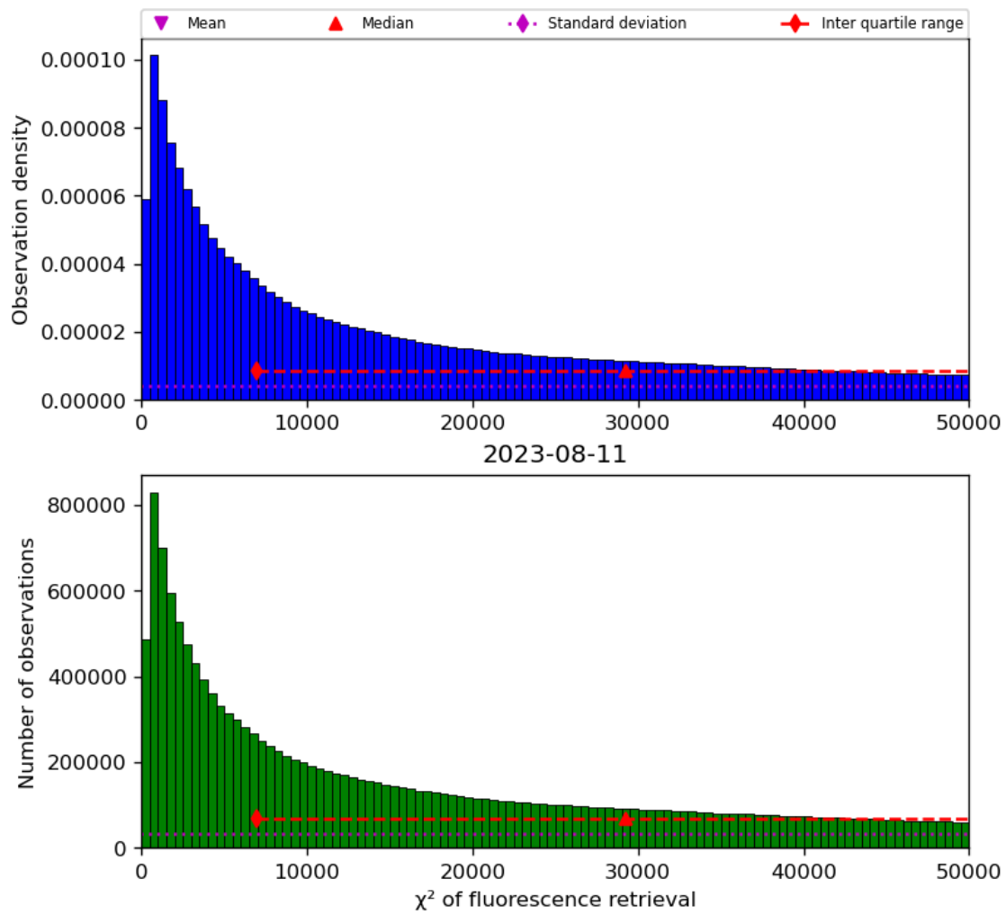
Figure 42: Histogram of “ \chi^2 of fluorescence retrieval” for 2023-08-10 to 2023-08-12
