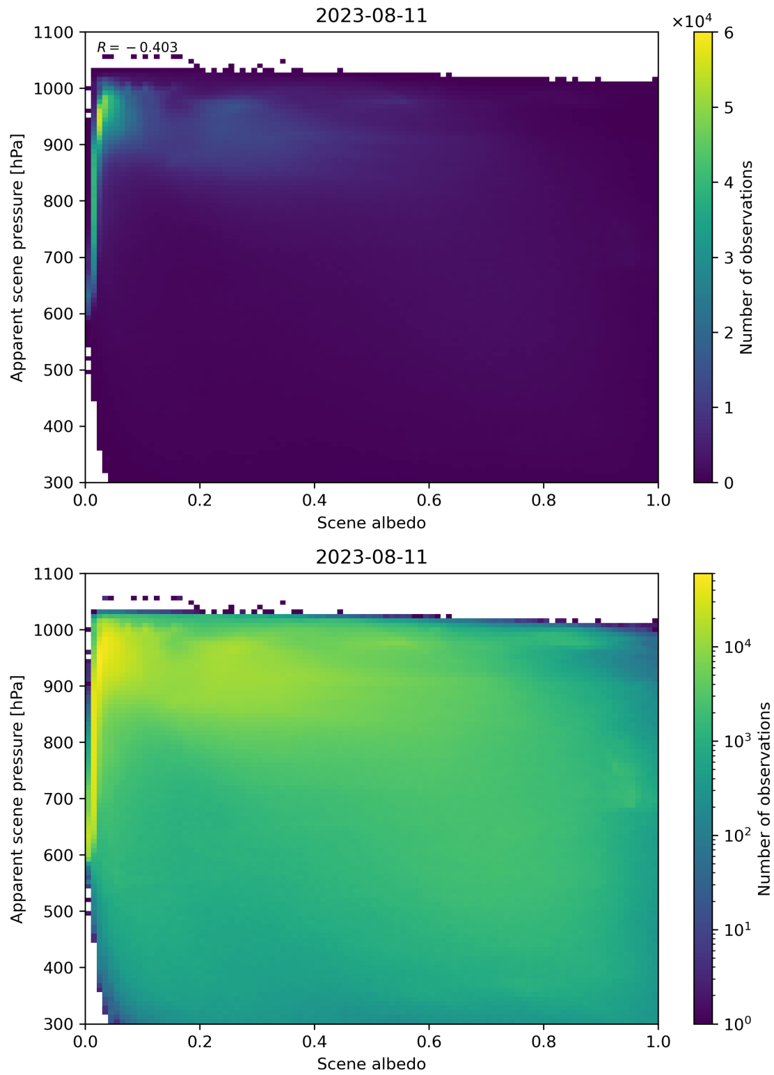
Figure 111: Scatter density plot of “Scene albedo” against “Apparent scene pressure” for 2023-08-10 to 2023-08-12.
