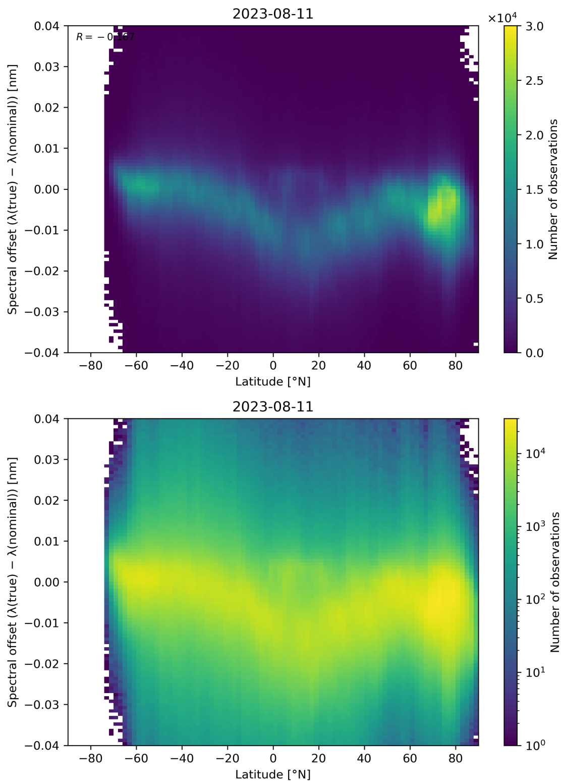
Figure 105: Scatter density plot of “Latitude” against “Spectral offset ( \lambda(\text{true}) - \lambda(\text{nominal}) )” for 2023-08-10 to 2023-08-12.
