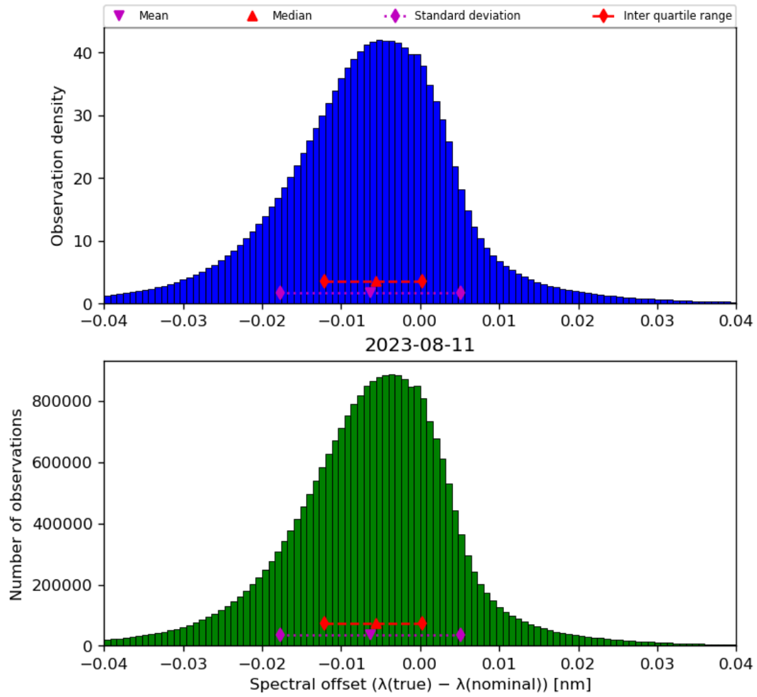
Figure 45: Histogram of “Spectral offset ( \lambda(\text{true}) - \lambda(\text{nominal}) )” for 2023-08-10 to 2023-08-12
