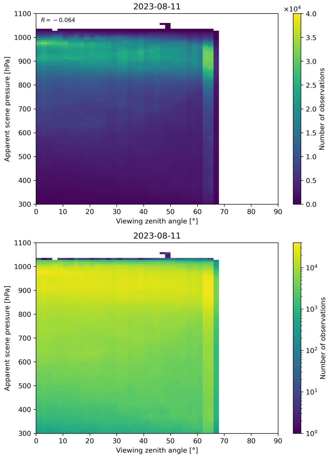
Figure 129: Scatter density plot of “Viewing zenith angle” against “Apparent scene pressure” for 2023-08-10 to 2023-08-12.
