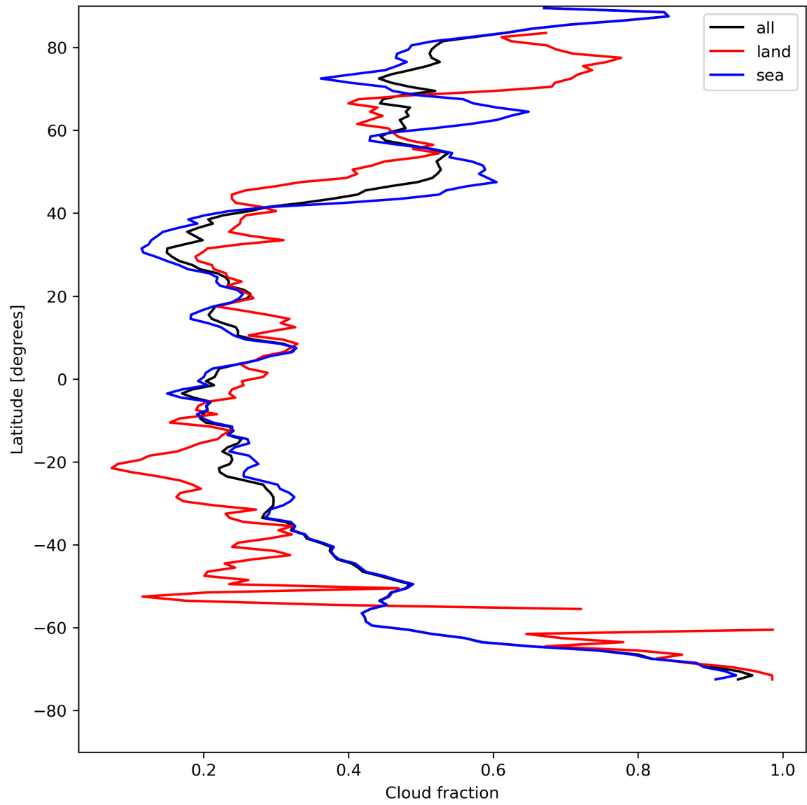
Figure 15: Zonal average of “Cloud fraction” for 2023-08-10 to 2023-08-12.
