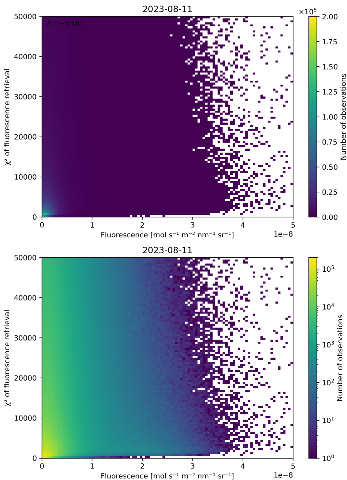
Figure 93: Scatter density plot of “Fluorescence” against “ \chi^2 of fluorescence retrieval” for 2023-08-10 to 2023-08-12.
