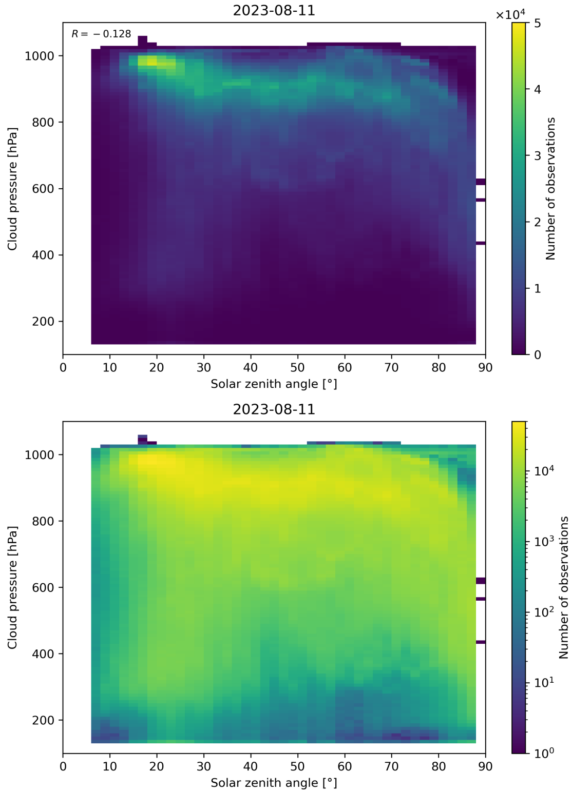
Figure 122: Scatter density plot of “Solar zenith angle” against “Cloud pressure” for 2023-08-10 to 2023-08-12.
