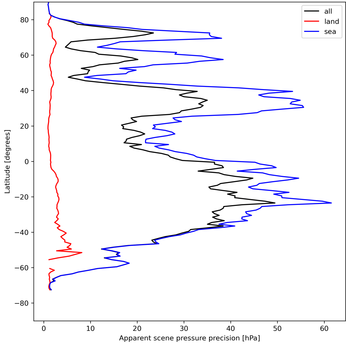
Figure 20: Zonal average of “Apparent scene pressure precision” for 2023-08-10 to 2023-08-12.
