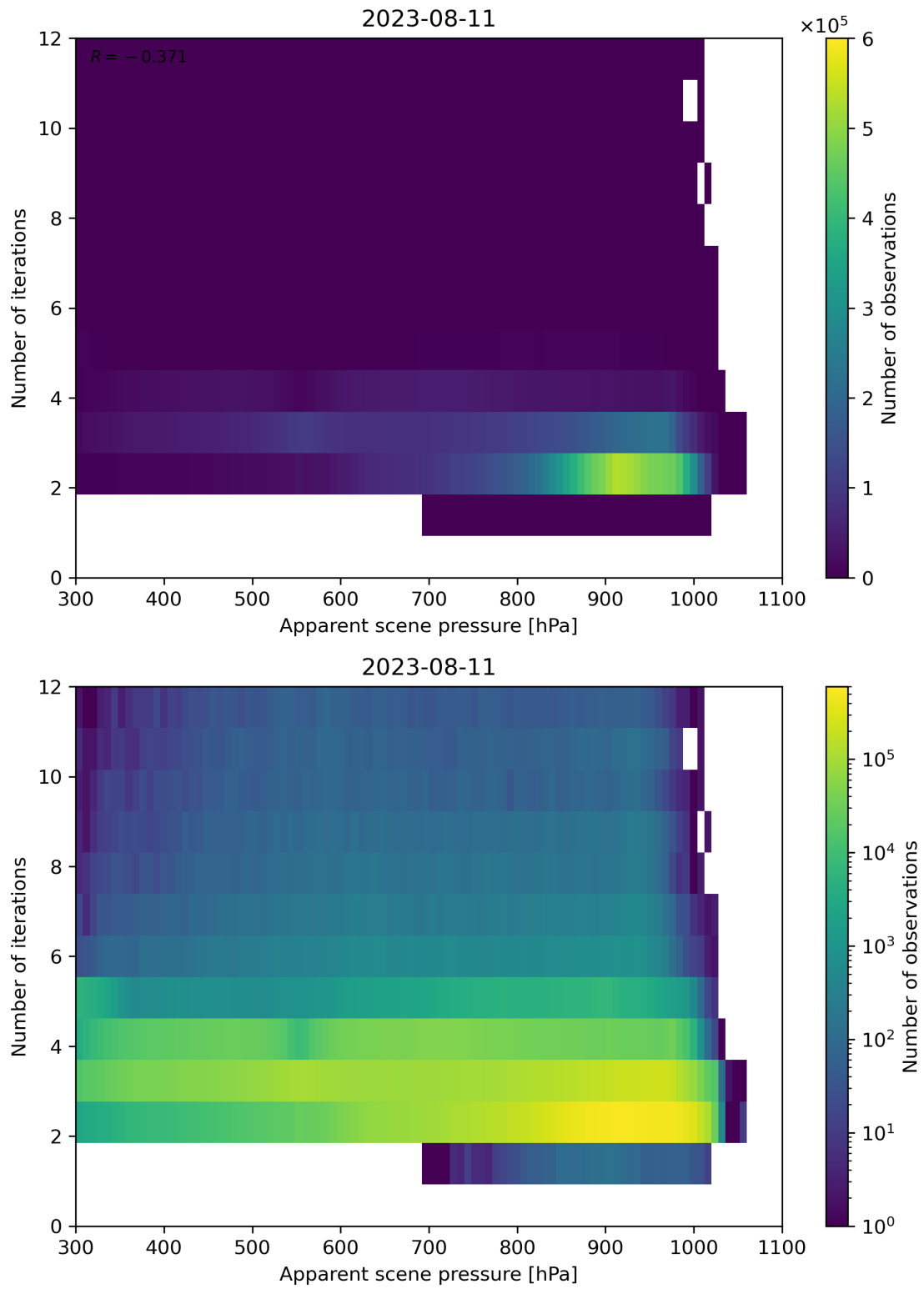
Figure 66: Scatter density plot of “Apparent scene pressure” against “Number of iterations” for 2023-08-10 to 2023-08-12.
