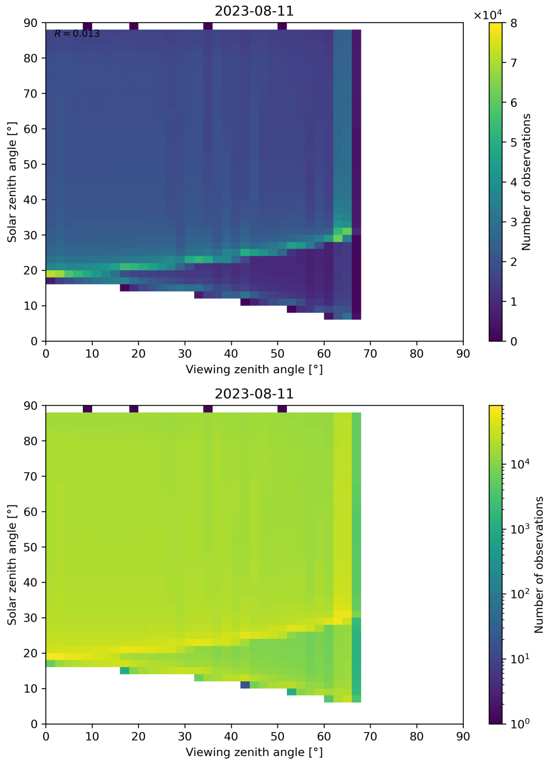
Figure 139: Scatter density plot of “Viewing zenith angle” against “Solar zenith angle” for 2023-08-10 to 2023-08-12.
