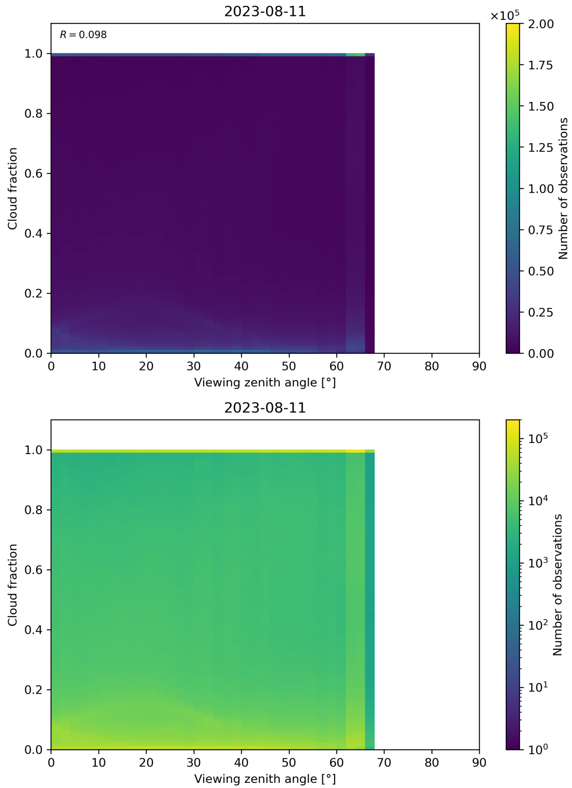
Figure 132: Scatter density plot of “Viewing zenith angle” against “Cloud fraction” for 2023-08-10 to 2023-08-12.
