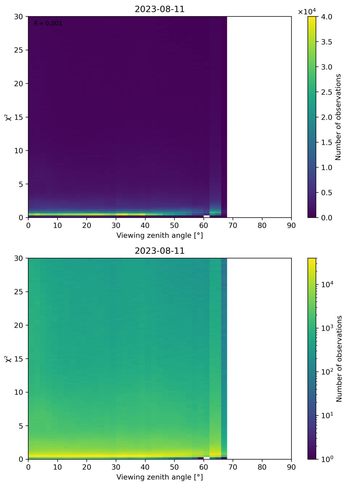
Figure 130: Scatter density plot of “Viewing zenith angle” against “ \chi^2 ” for 2023-08-10 to 2023-08-12.
