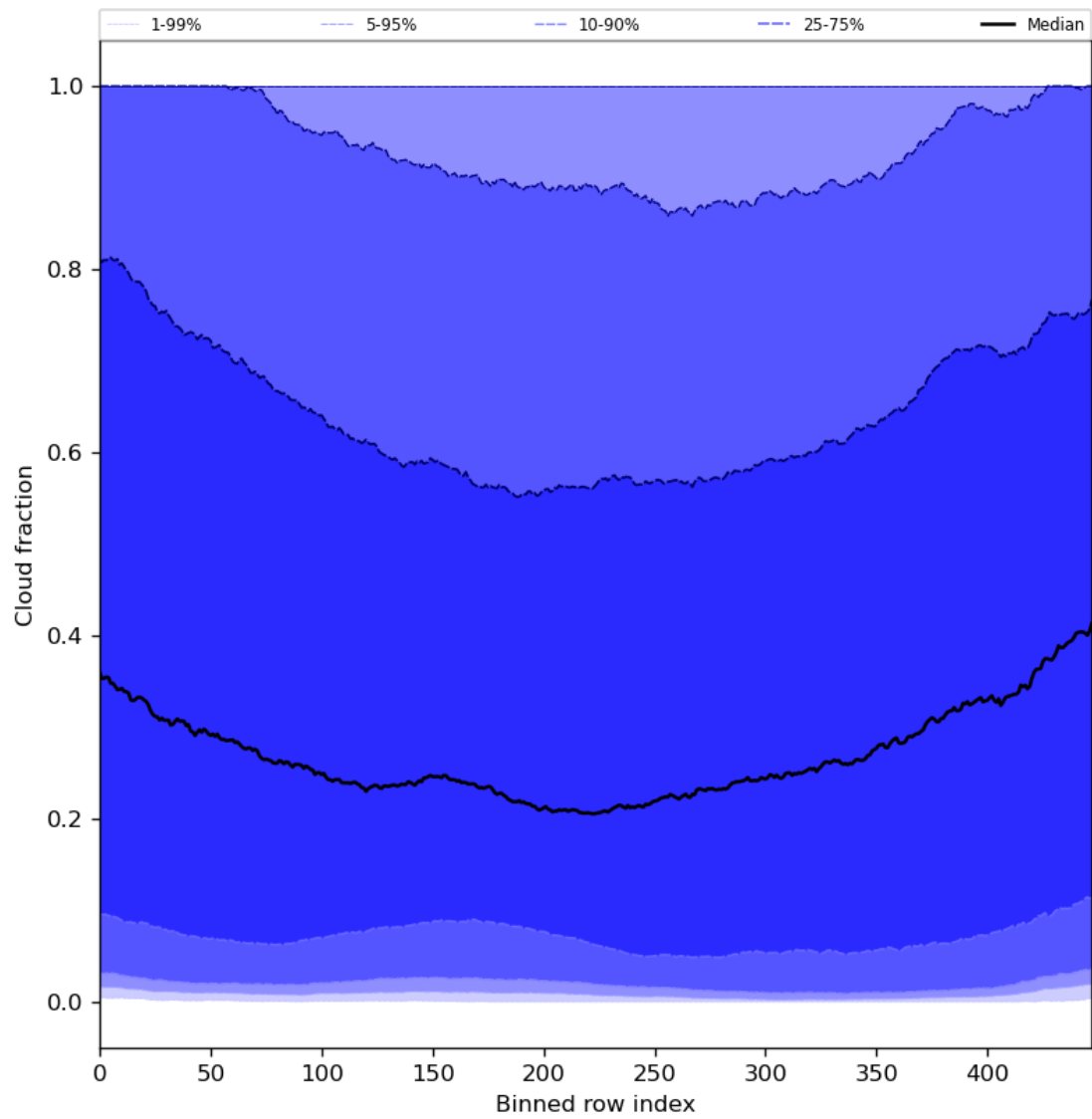
Figure 49: Along track statistics of “Cloud fraction” for 2023-08-10 to 2023-08-12
