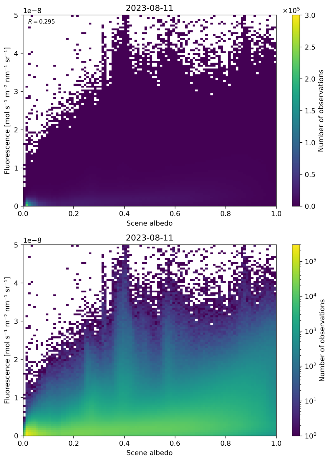
Figure 114: Scatter density plot of “Scene albedo” against “Fluorescence” for 2023-08-10 to 2023-08-12.
