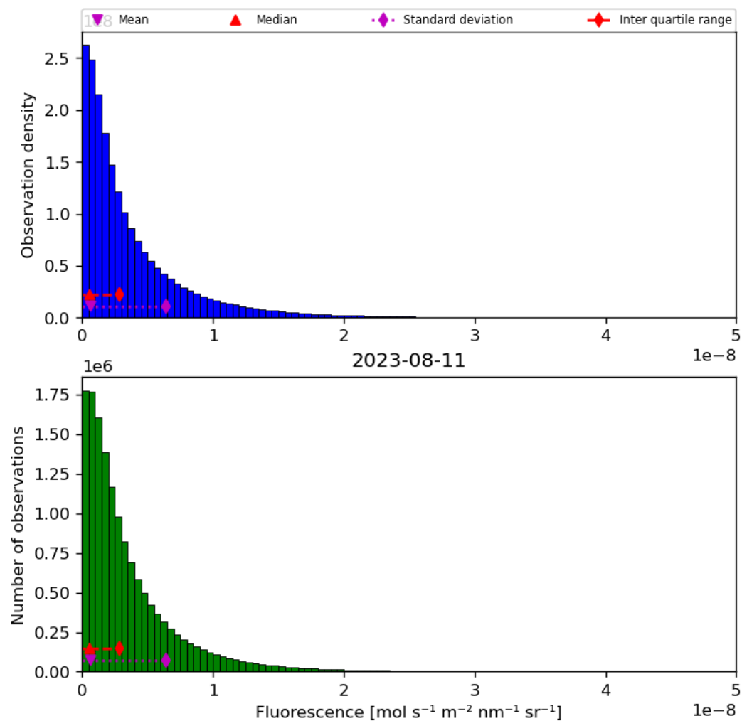
Figure 40: Histogram of “Fluorescence” for 2023-08-10 to 2023-08-12
