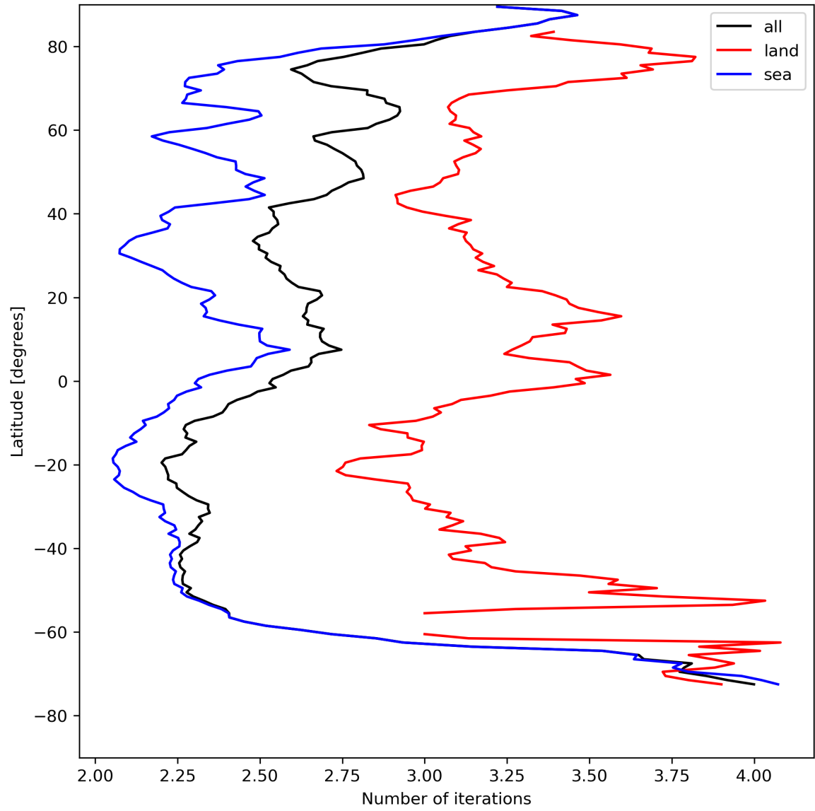
Figure 22: Zonal average of “Number of iterations” for 2023-08-10 to 2023-08-12.
