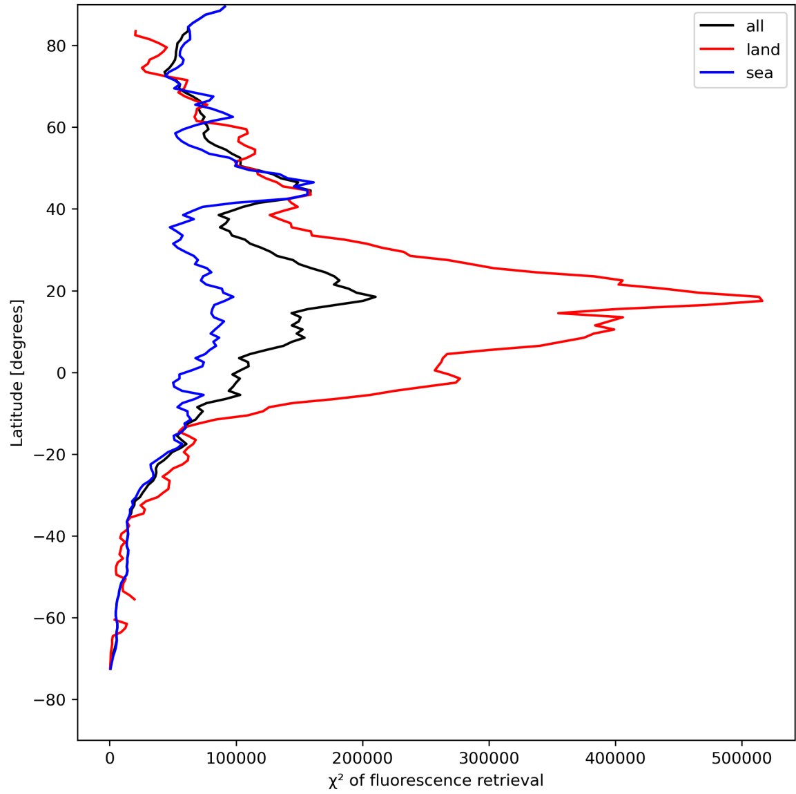
Figure 25: Zonal average of “ \chi^2 of fluorescence retrieval” for 2023-08-10 to 2023-08-12.
