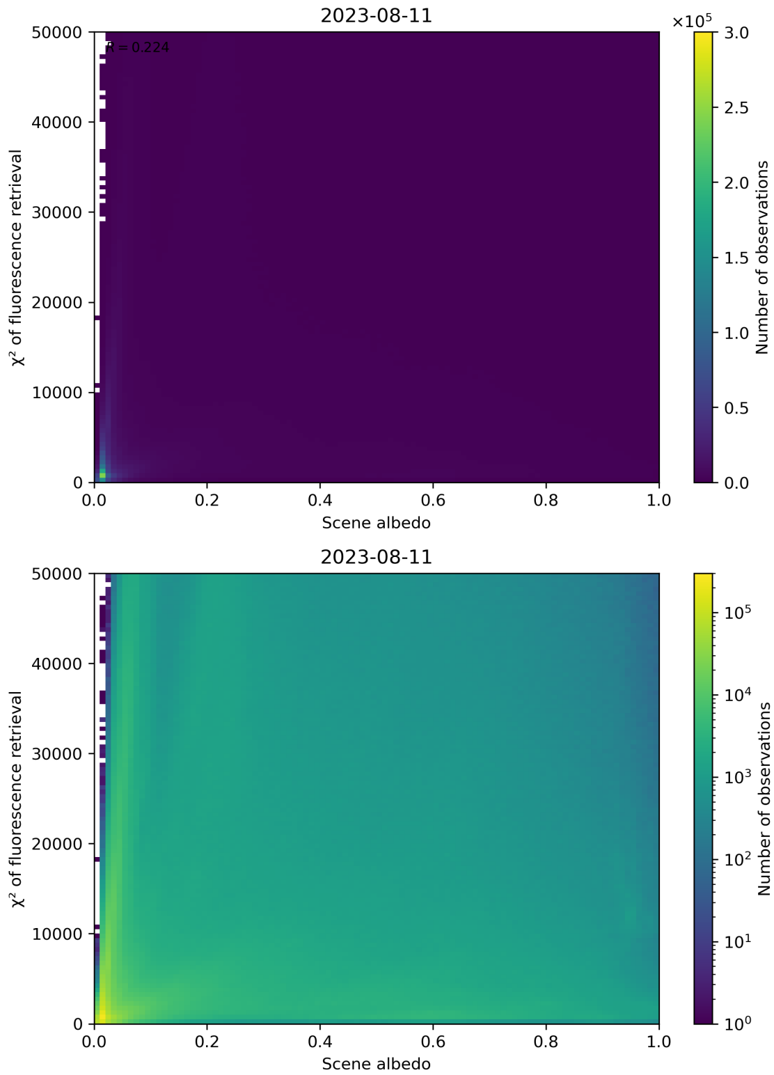
Figure 113: Scatter density plot of “Scene albedo” against “ \chi^2 of fluorescence retrieval” for 2023-08-10 to 2023-08-12.
