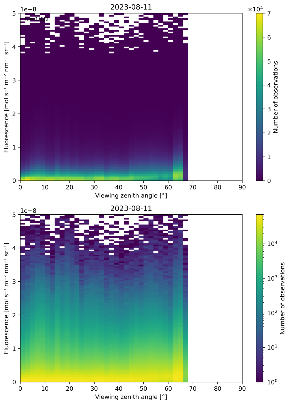
Figure 134: Scatter density plot of “Viewing zenith angle” against “Fluorescence” for 2023-08-10 to 2023-08-12.
