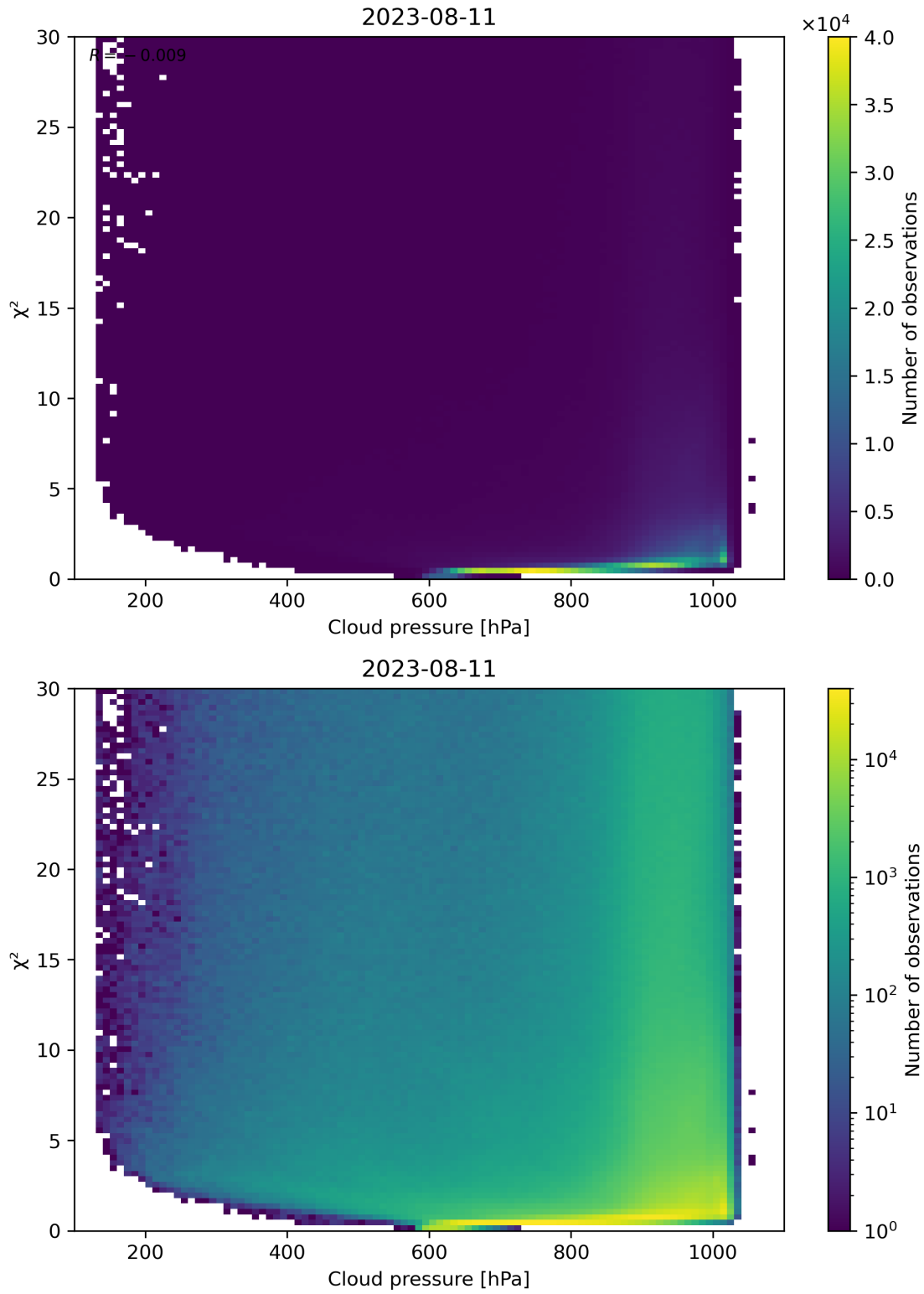
Figure 85: Scatter density plot of “Cloud pressure” against “ \chi^2 ” for 2023-08-10 to 2023-08-12.
