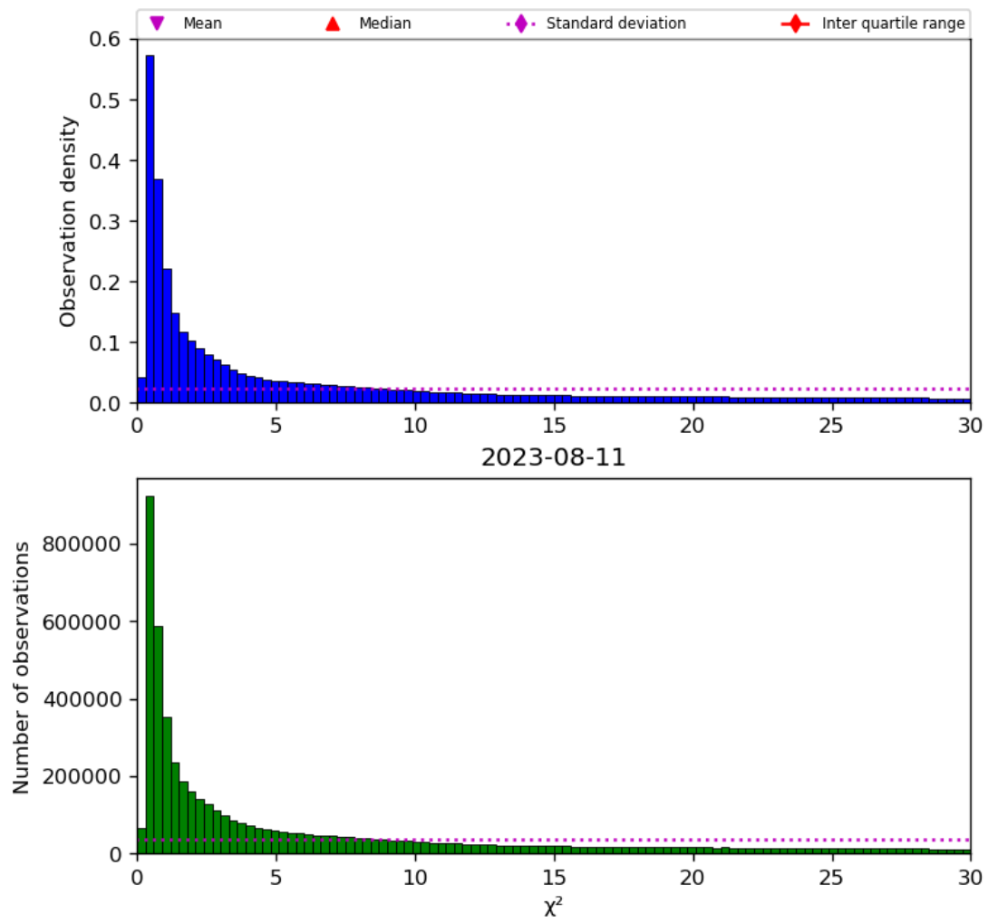
Figure 38: Histogram of “ \chi^2 ” for 2023-08-10 to 2023-08-12
