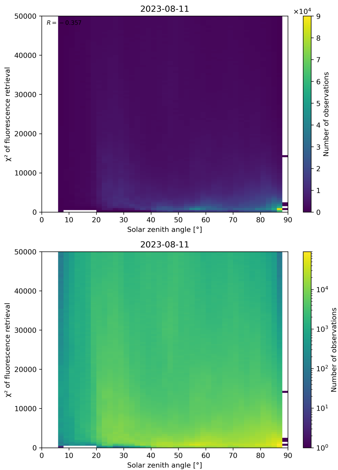
Figure 120: Scatter density plot of “Solar zenith angle” against “ \chi^2 of fluorescence retrieval” for 2023-08-10 to 2023-08-12.
