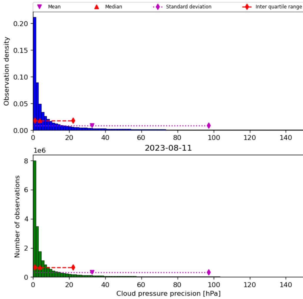
Figure 31: Histogram of “Cloud pressure precision” for 2023-08-10 to 2023-08-12
