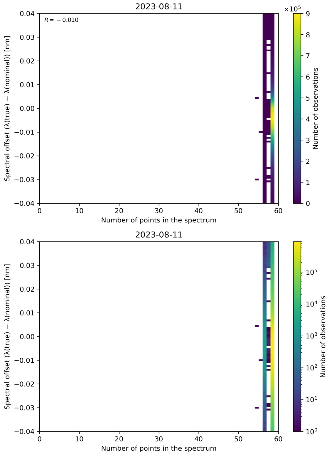
Figure 110: Scatter density plot of “Number of points in the spectrum” against “Spectral offset ( \lambda(\text{true}) - \lambda(\text{nominal}) )” for 2023-08-10 to 2023-08-12.
