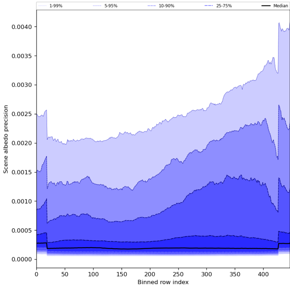
Figure 52: Along track statistics of “Scene albedo precision” for 2023-08-10 to 2023-08-12
