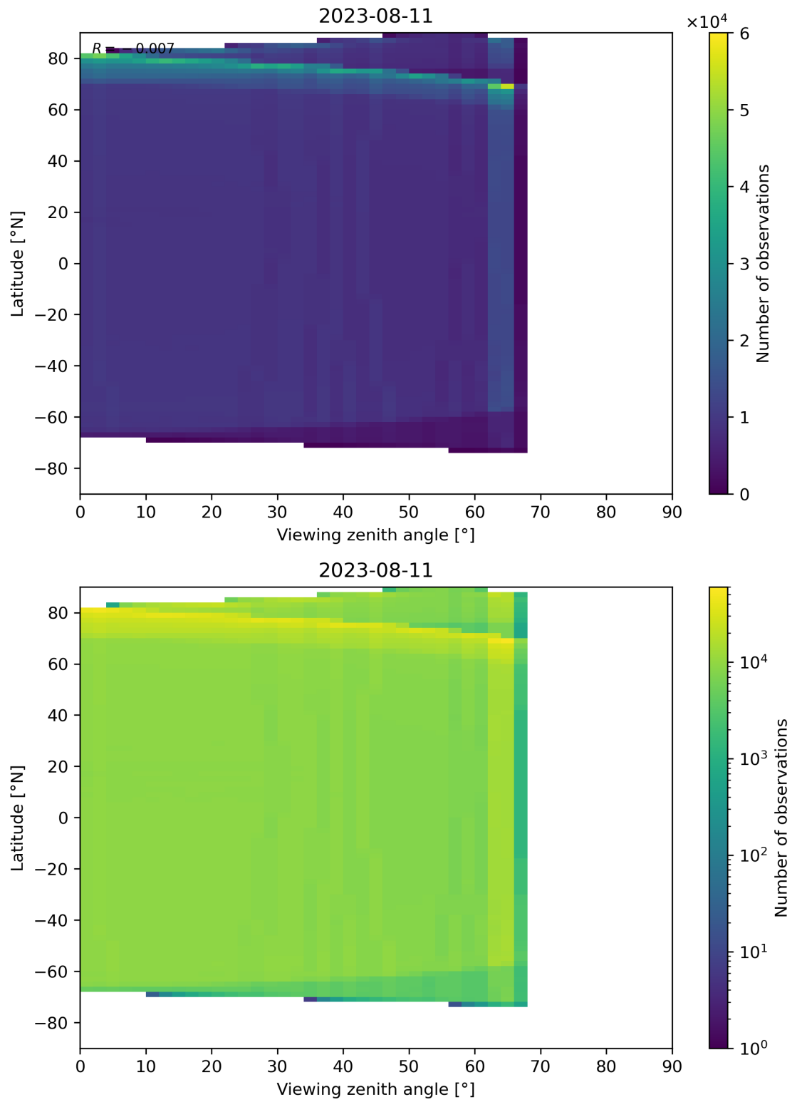
Figure 135: Scatter density plot of “Viewing zenith angle” against “Latitude” for 2023-08-10 to 2023-08-12.
