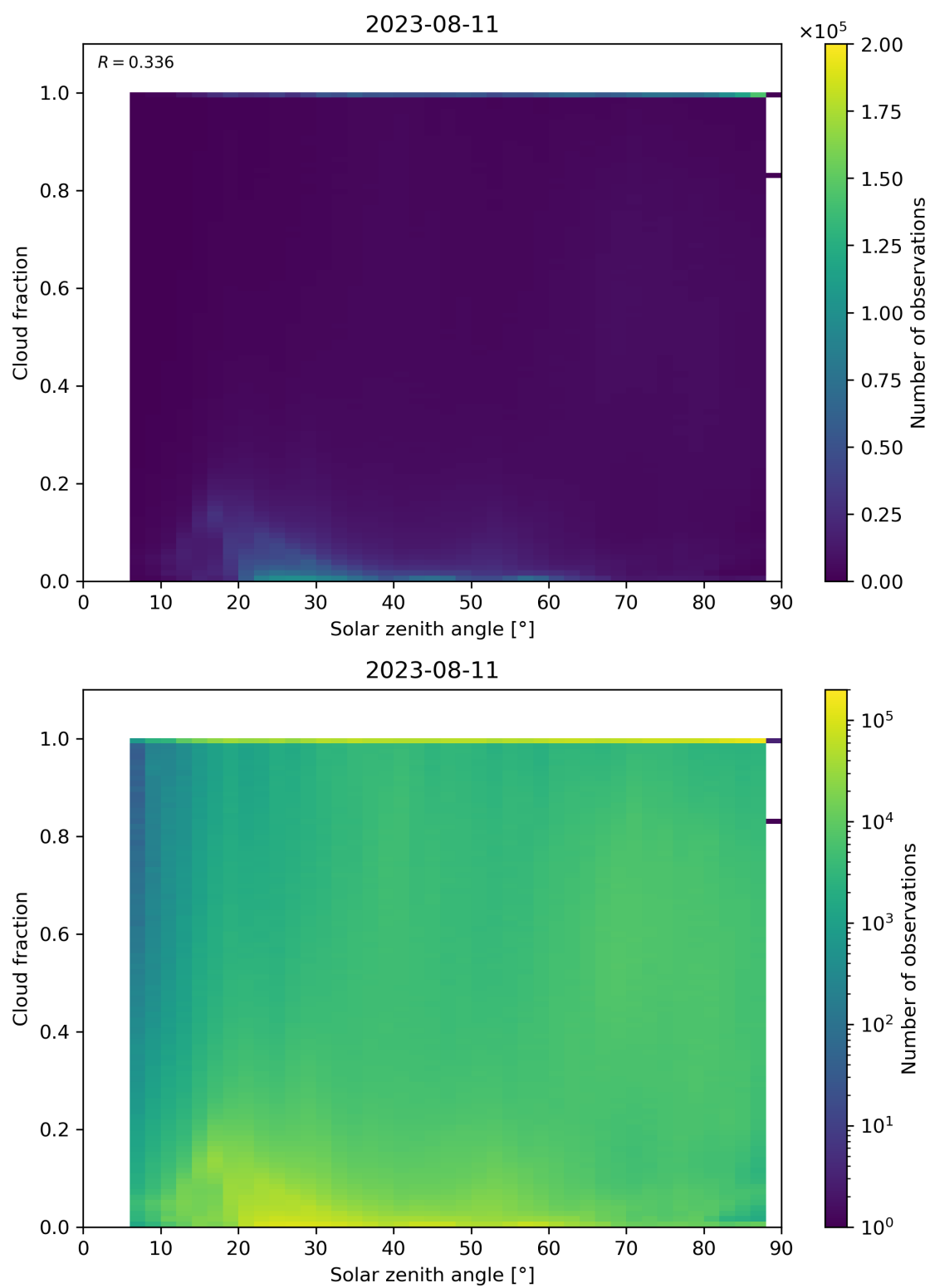
Figure 121: Scatter density plot of “Solar zenith angle” against “Cloud fraction” for 2023-08-10 to 2023-08-12.
