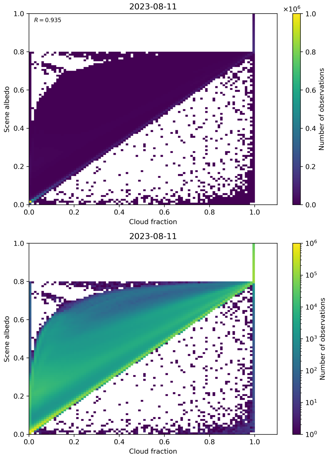
Figure 82: Scatter density plot of “Cloud fraction” against “Scene albedo” for 2023-08-10 to 2023-08-12.
