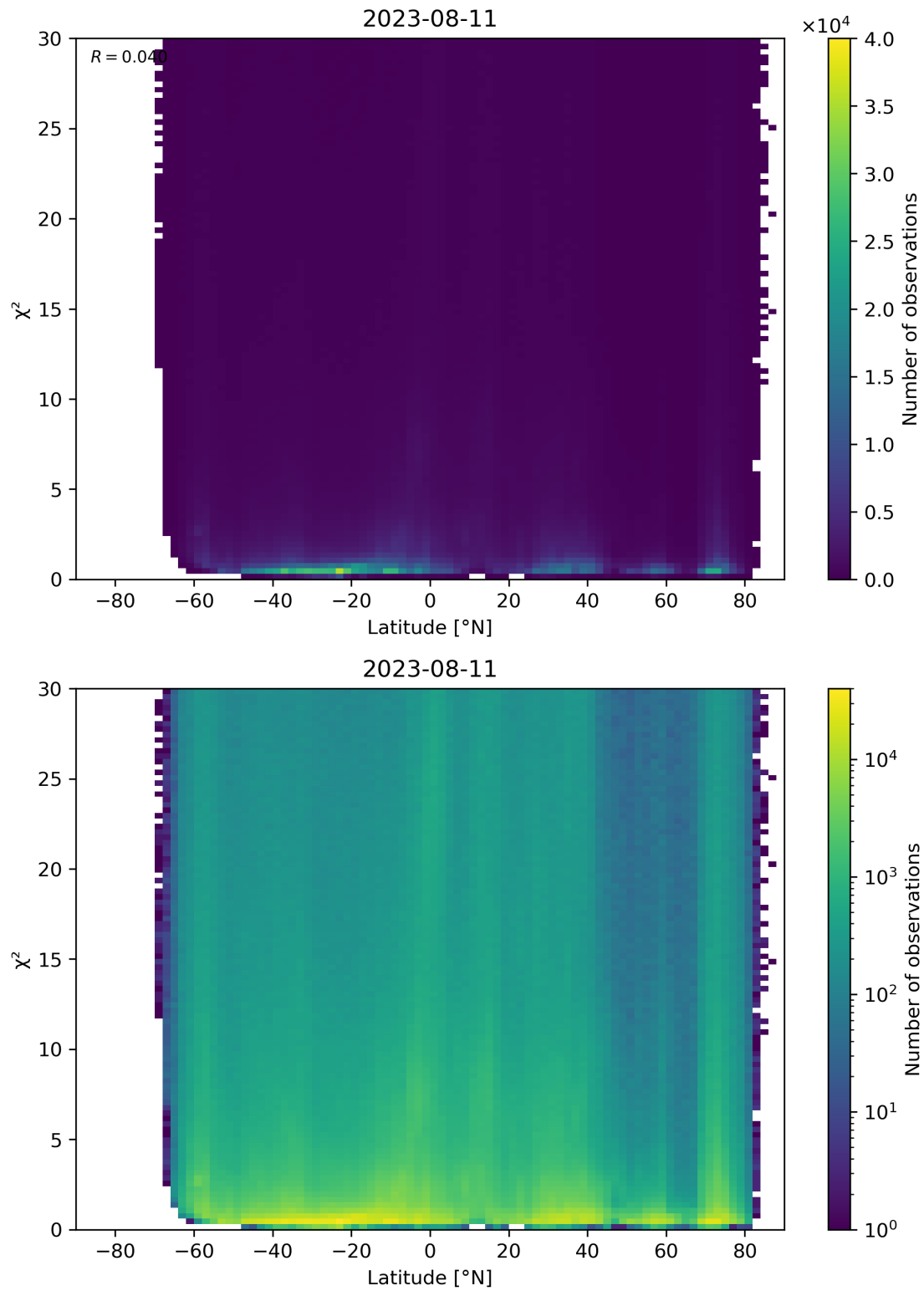
Figure 97: Scatter density plot of “Latitude” against “ \chi^2 ” for 2023-08-10 to 2023-08-12.
