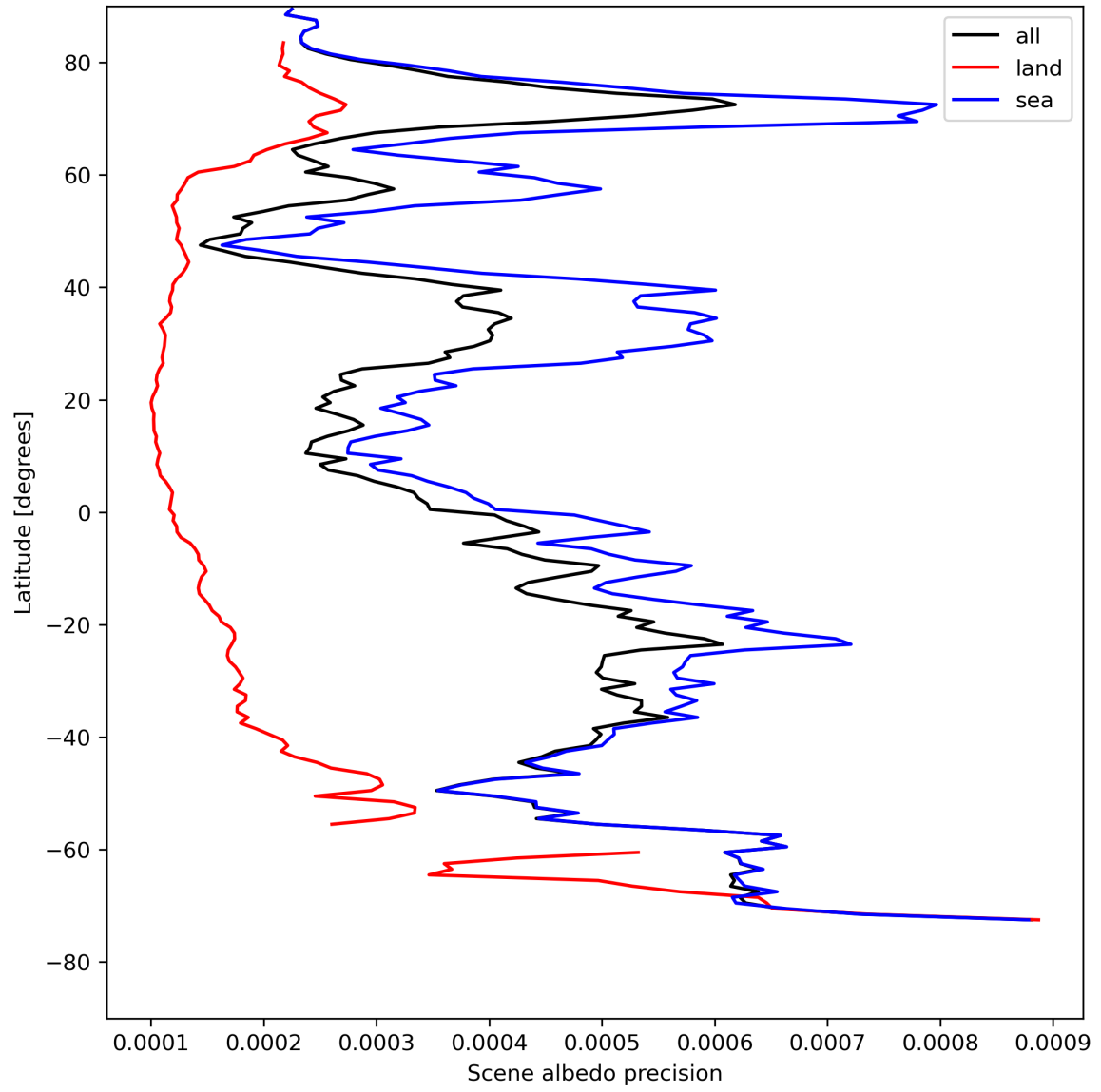
Figure 18: Zonal average of “Scene albedo precision” for 2023-08-10 to 2023-08-12.
