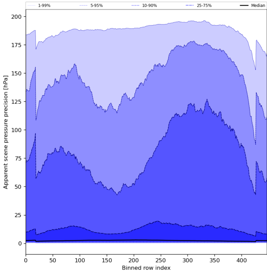
Figure 54: Along track statistics of “Apparent scene pressure precision” for 2023-08-10 to 2023-08-12
