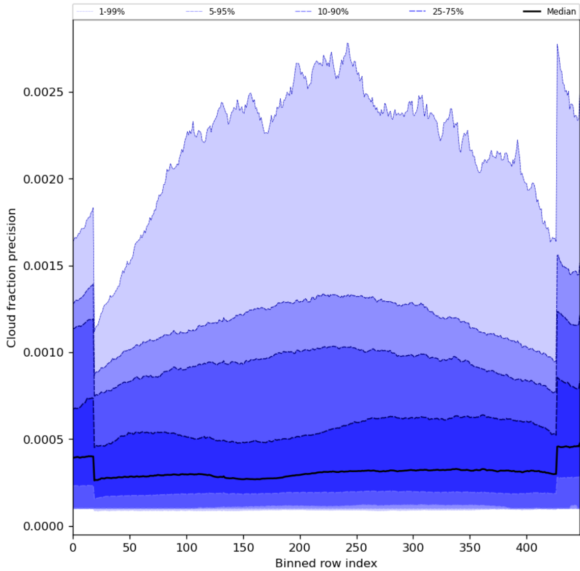
Figure 50: Along track statistics of “Cloud fraction precision” for 2023-08-10 to 2023-08-12
