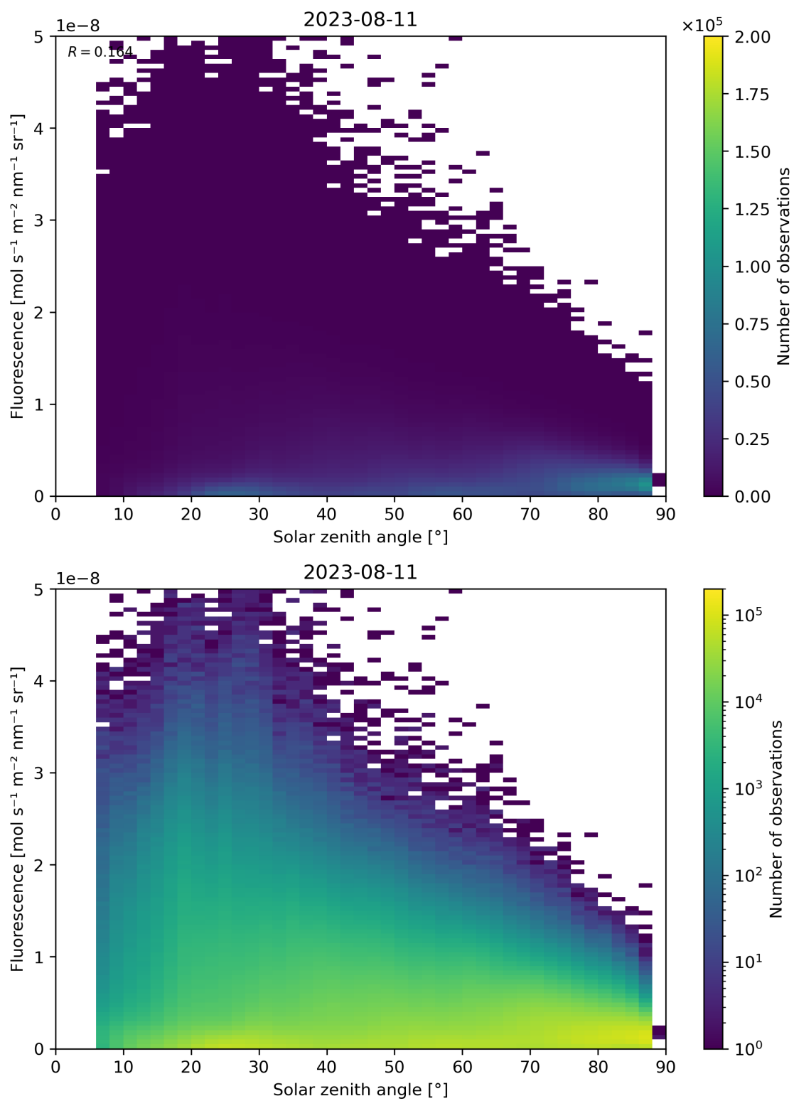
Figure 123: Scatter density plot of “Solar zenith angle” against “Fluorescence” for 2023-08-10 to 2023-08-12.
