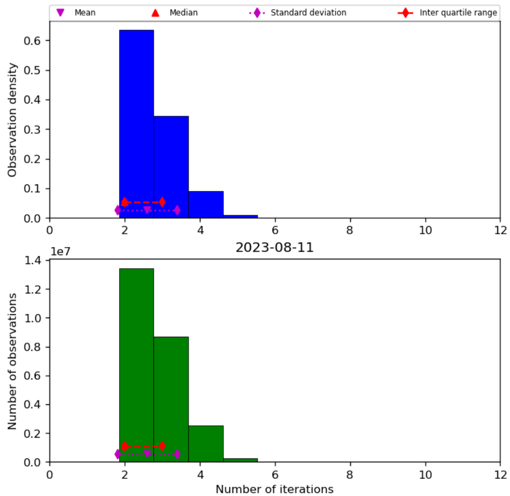
Figure 39: Histogram of “Number of iterations” for 2023-08-10 to 2023-08-12
