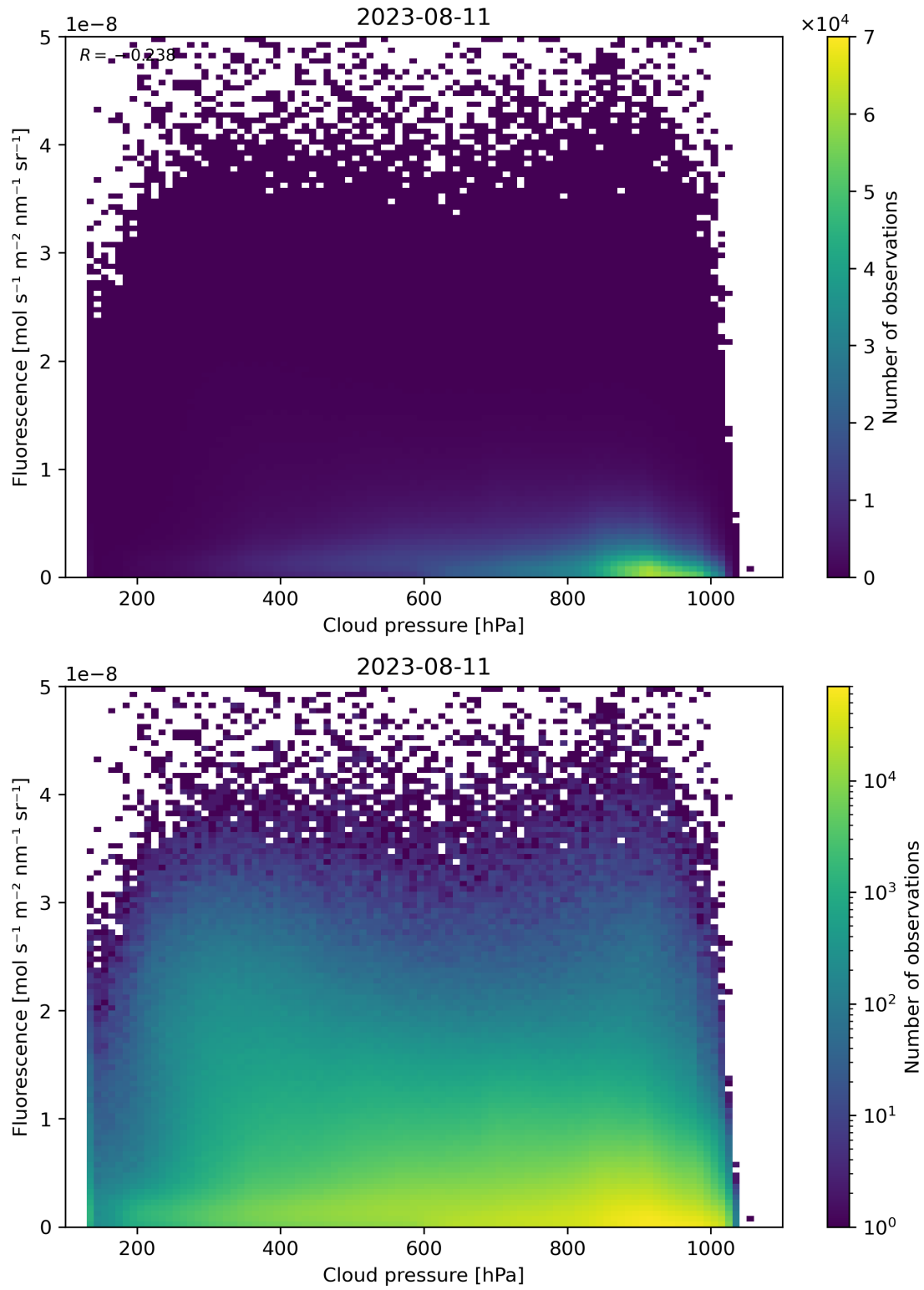
Figure 88: Scatter density plot of “Cloud pressure” against “Fluorescence” for 2023-08-10 to 2023-08-12.
