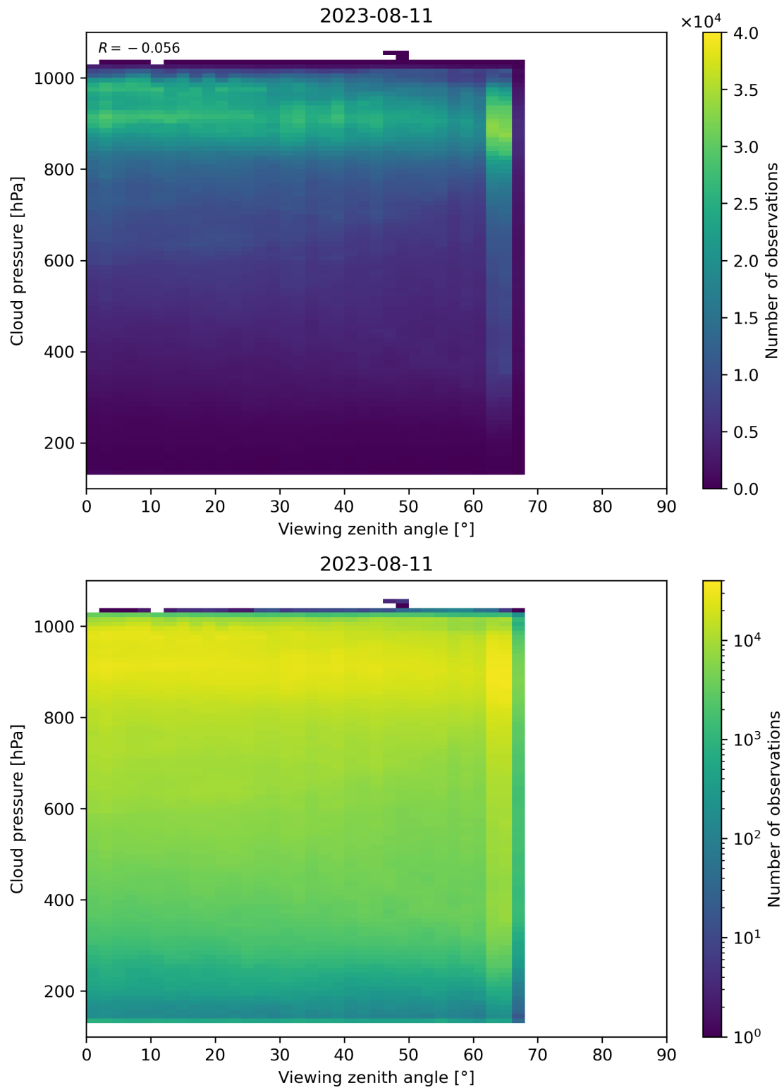
Figure 133: Scatter density plot of “Viewing zenith angle” against “Cloud pressure” for 2023-08-10 to 2023-08-12.
