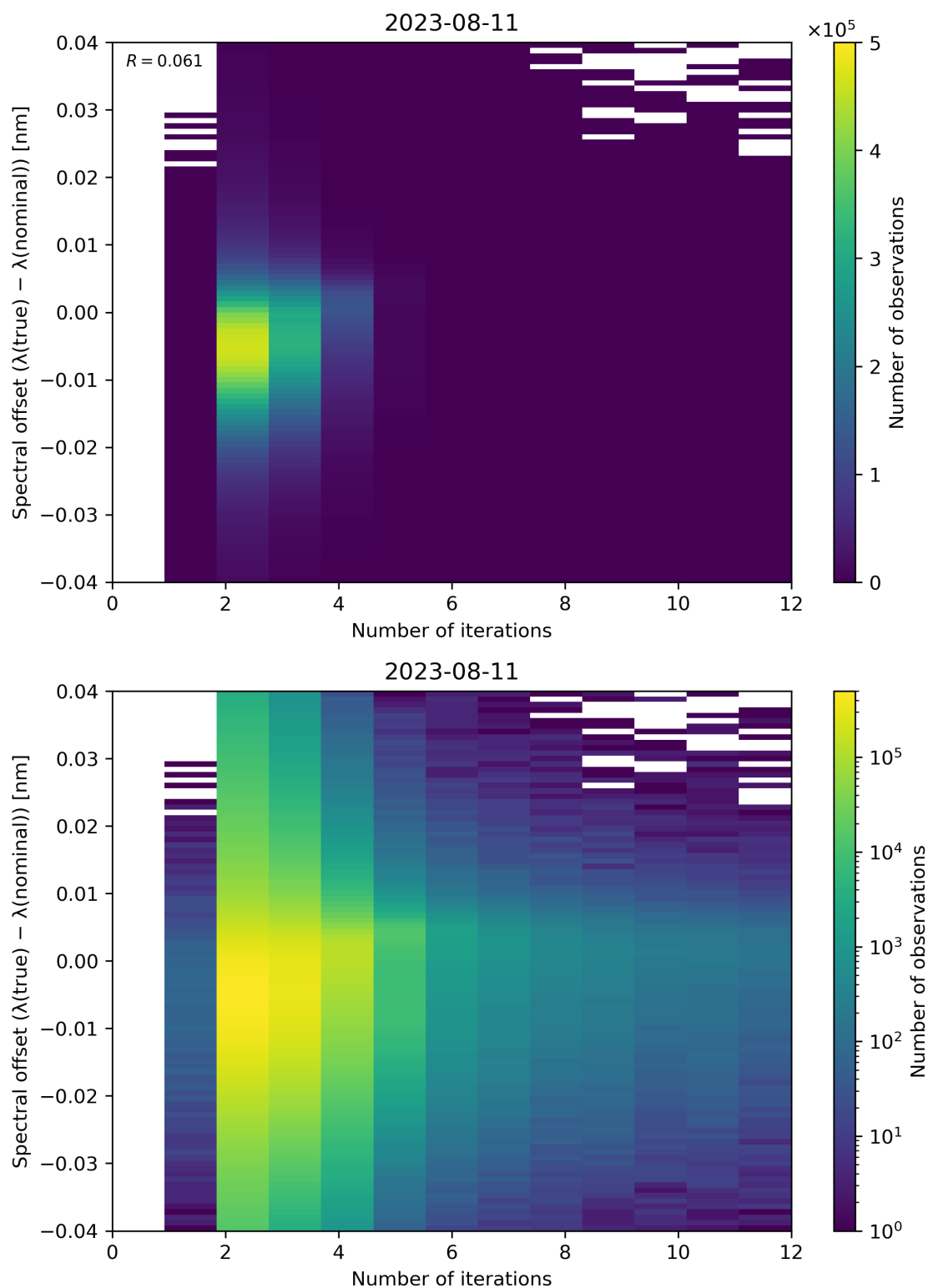
Figure 109: Scatter density plot of “Number of iterations” against “Spectral offset ( \lambda(\text{true}) - \lambda(\text{nominal}) )” for 2023-08-10 to 2023-08-12.
