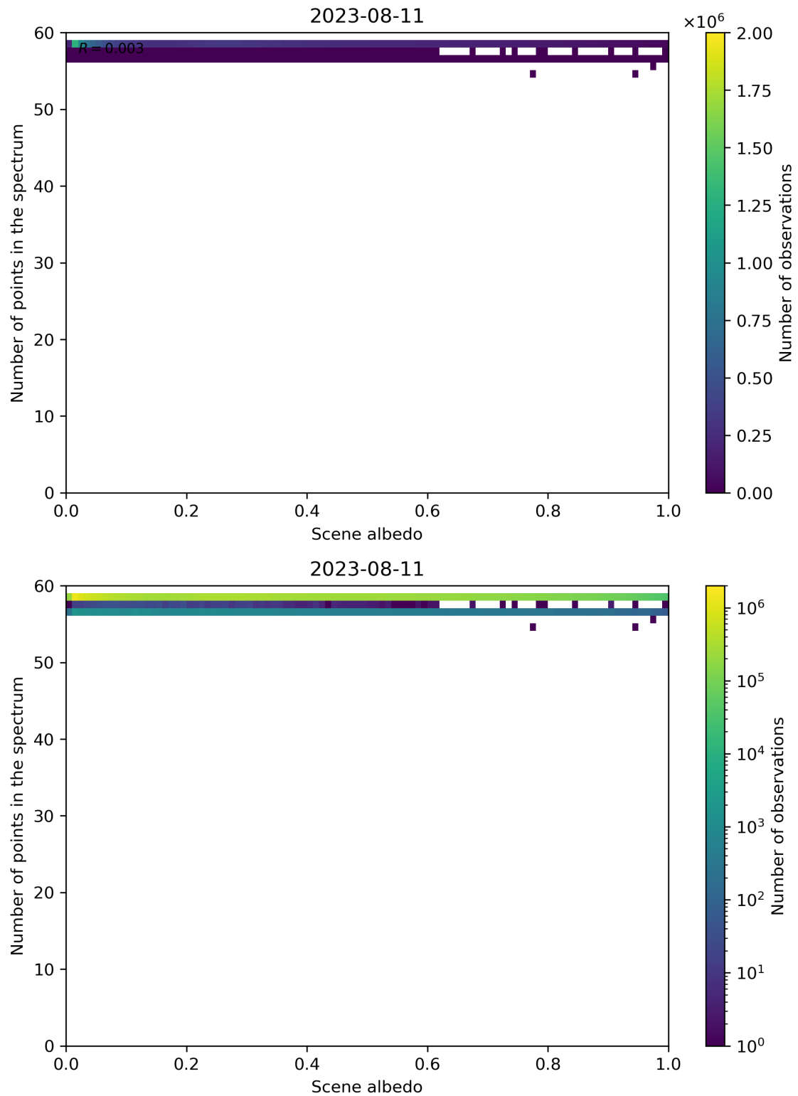
Figure 116: Scatter density plot of “Scene albedo” against “Number of points in the spectrum” for 2023-08-10 to 2023-08-12.
