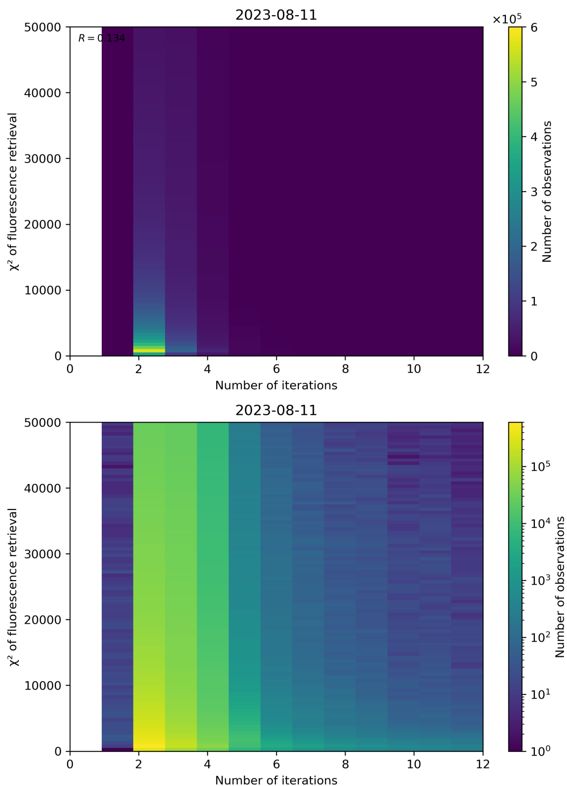
Figure 106: Scatter density plot of “Number of iterations” against “ \chi^2 of fluorescence retrieval” for 2023-08-10 to 2023-08-12.
