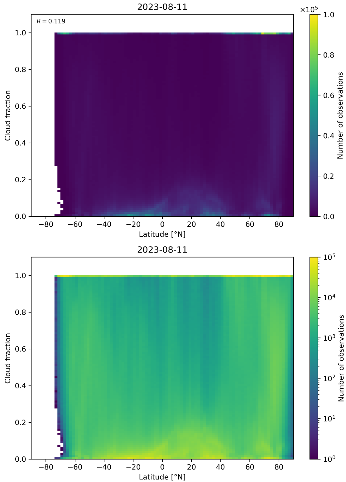
Figure 99: Scatter density plot of “Latitude” against “Cloud fraction” for 2023-08-10 to 2023-08-12.
