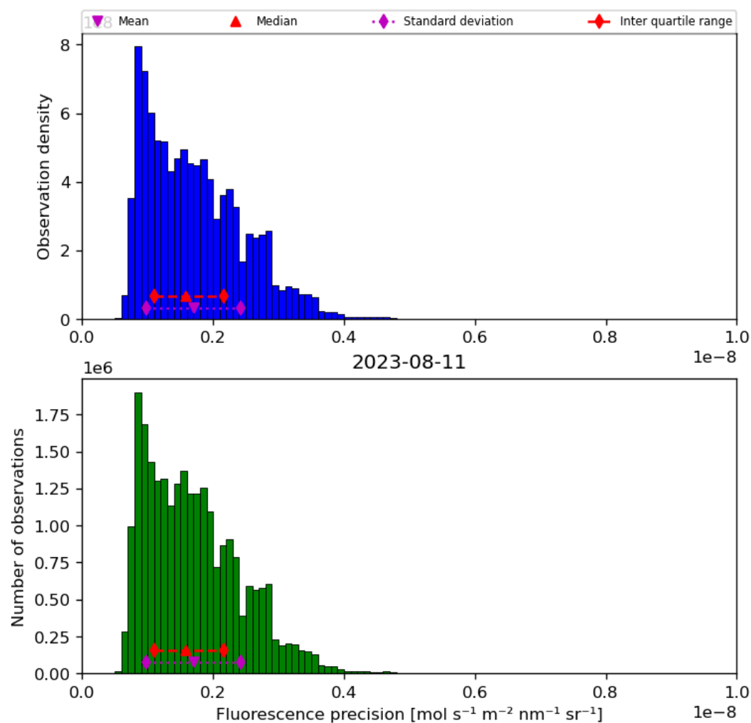
Figure 41: Histogram of “Fluorescence precision” for 2023-08-10 to 2023-08-12
