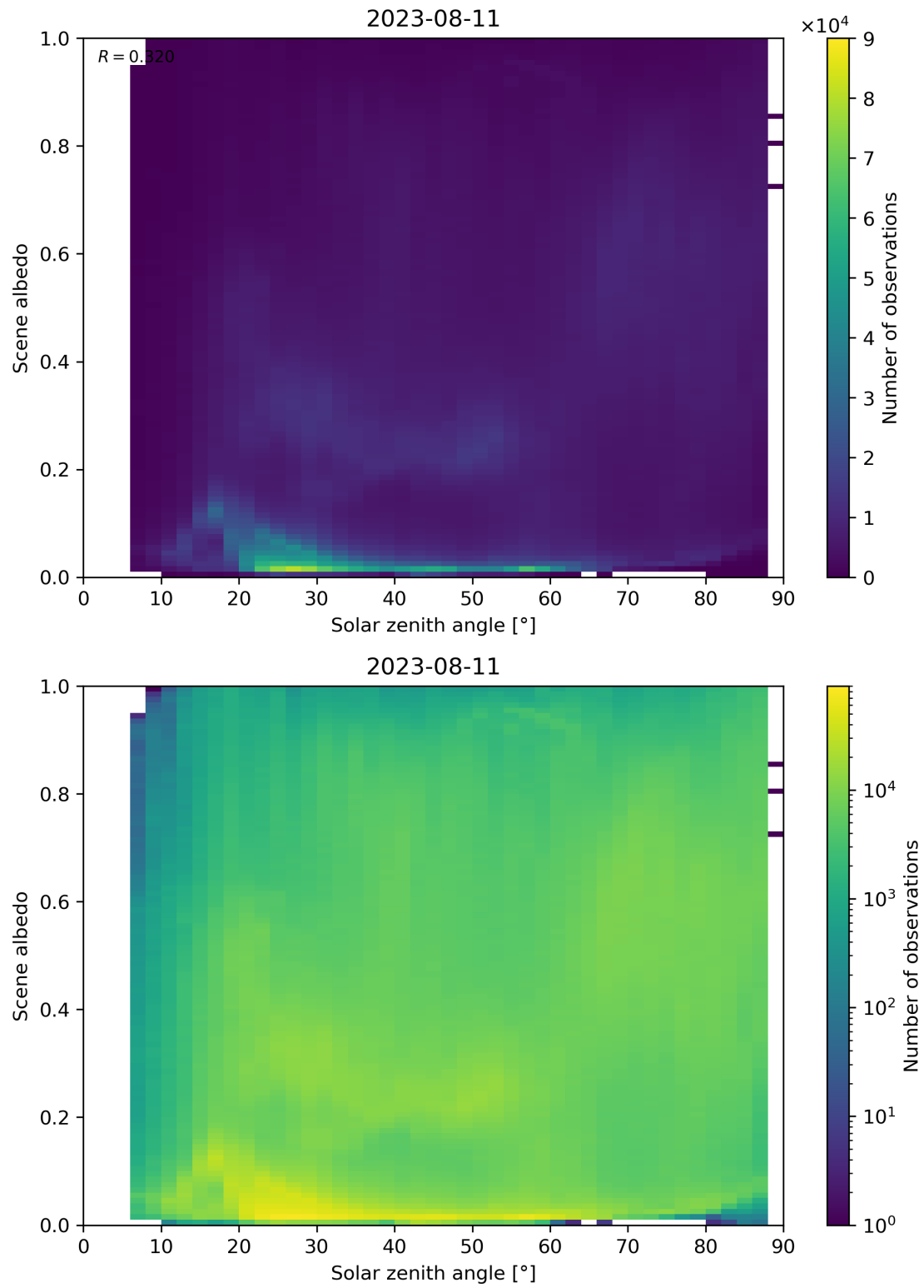
Figure 127: Scatter density plot of “Solar zenith angle” against “Scene albedo” for 2023-08-10 to 2023-08-12.
