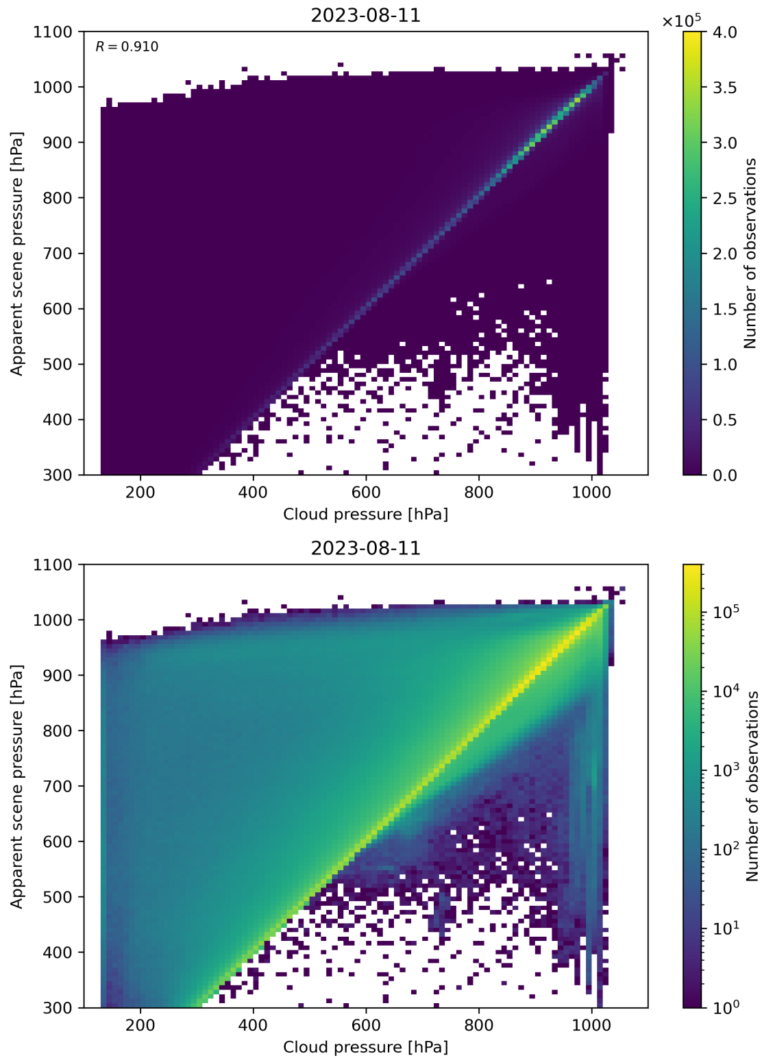
Figure 84: Scatter density plot of “Cloud pressure” against “Apparent scene pressure” for 2023-08-10 to 2023-08-12.
