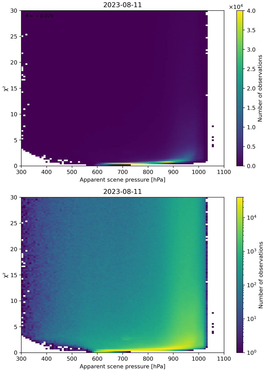
Figure 63: Scatter density plot of “Apparent scene pressure” against “ \chi^2 ” for 2023-08-10 to 2023-08-12.
