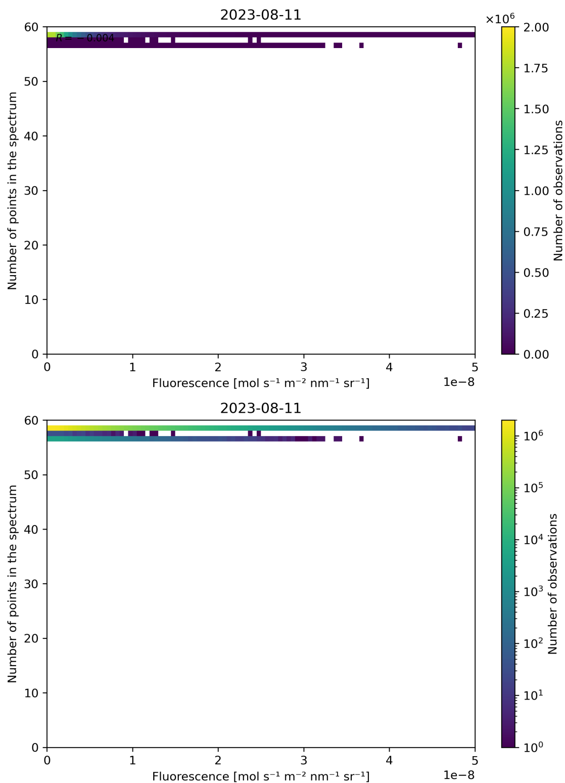
Figure 94: Scatter density plot of “Fluorescence” against “Number of points in the spectrum” for 2023-08-10 to 2023-08-12.
