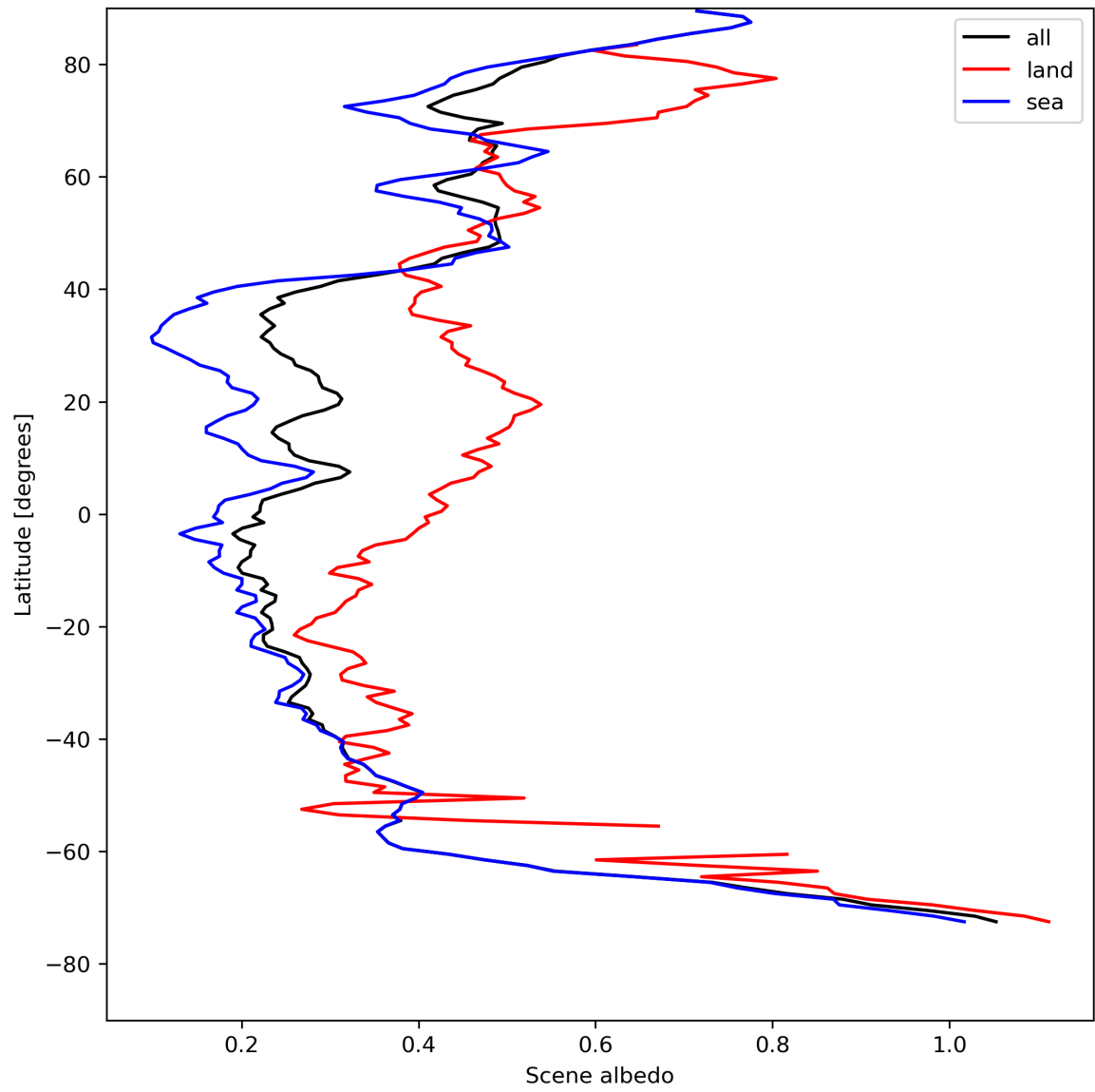
Figure 17: Zonal average of “Scene albedo” for 2023-08-10 to 2023-08-12.
