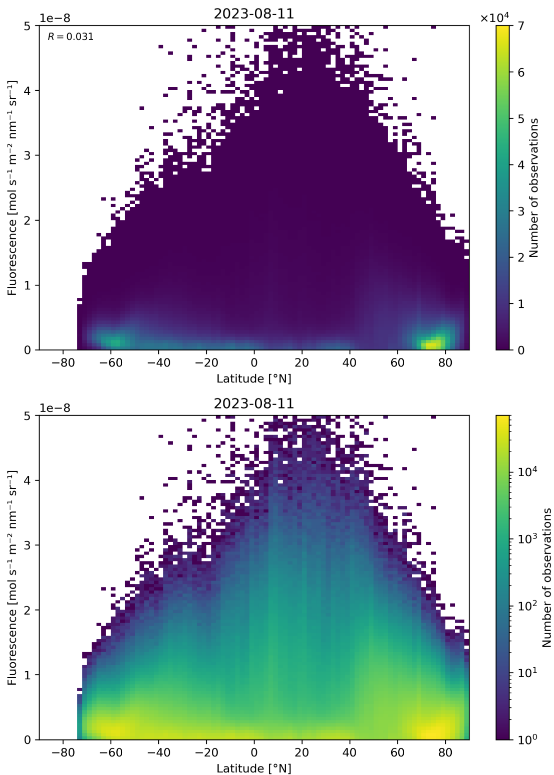
Figure 101: Scatter density plot of “Latitude” against “Fluorescence” for 2023-08-10 to 2023-08-12.
