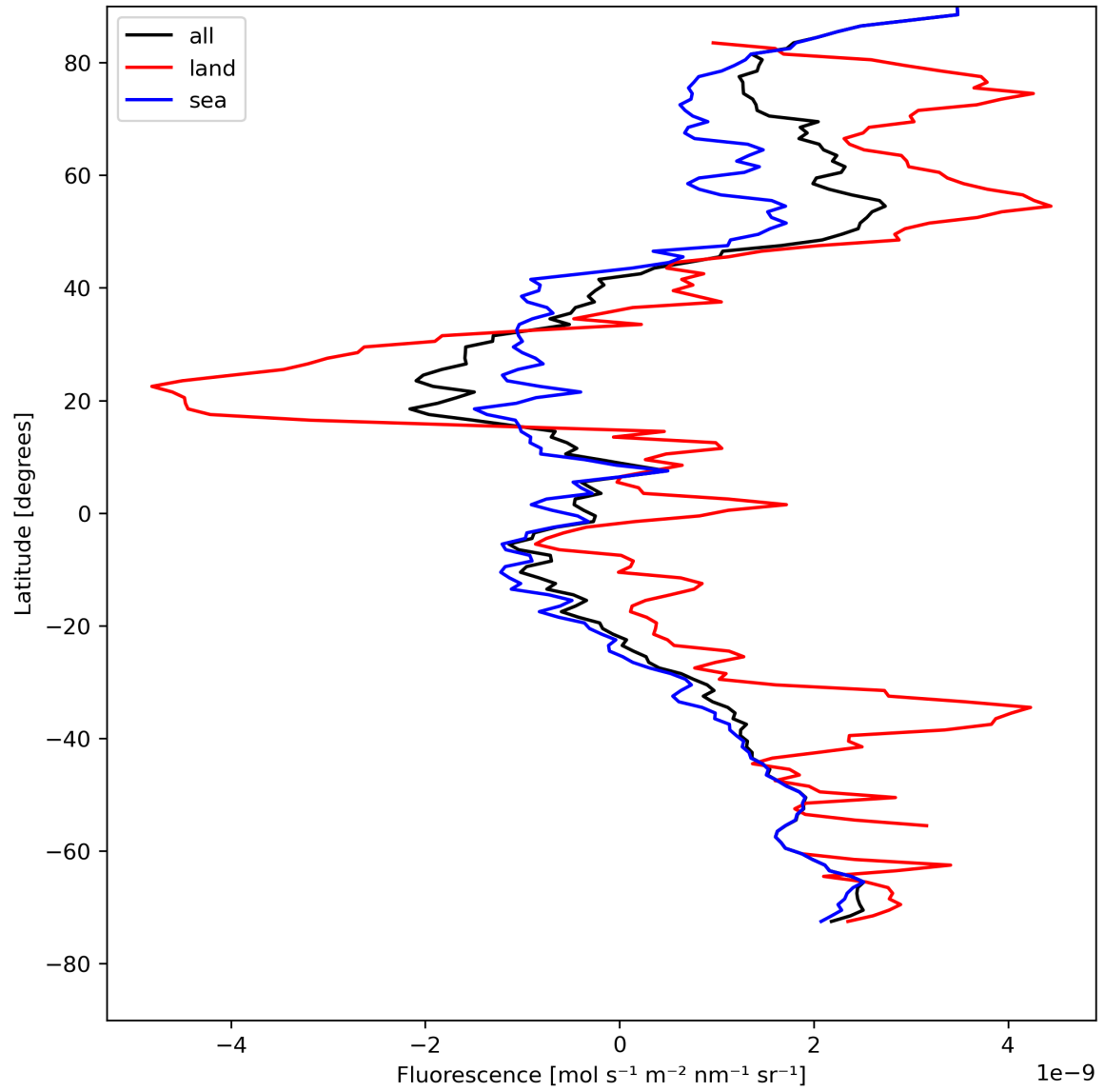
Figure 23: Zonal average of “Fluorescence” for 2023-08-10 to 2023-08-12.
