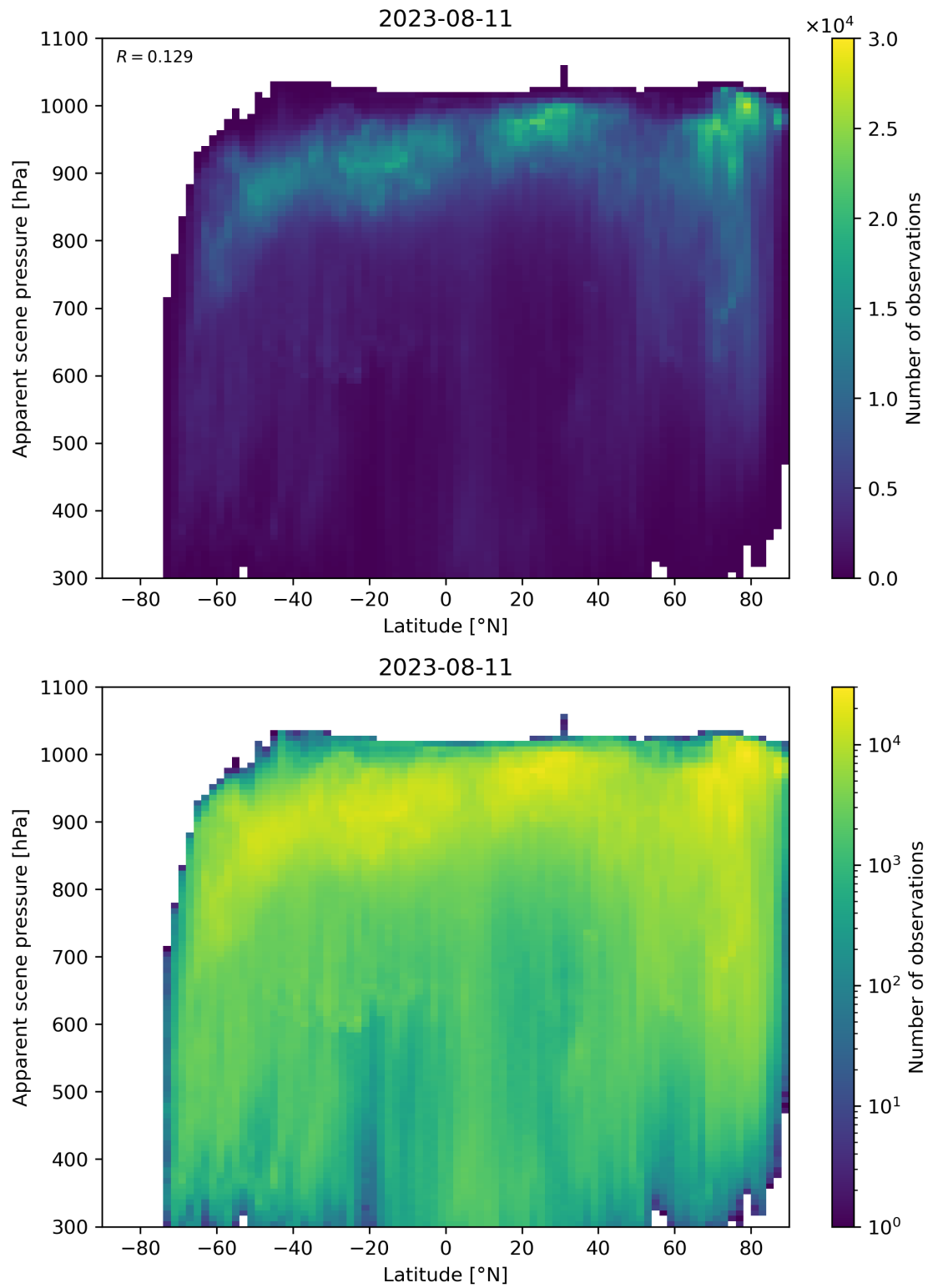
Figure 96: Scatter density plot of “Latitude” against “Apparent scene pressure” for 2023-08-10 to 2023-08-12.
