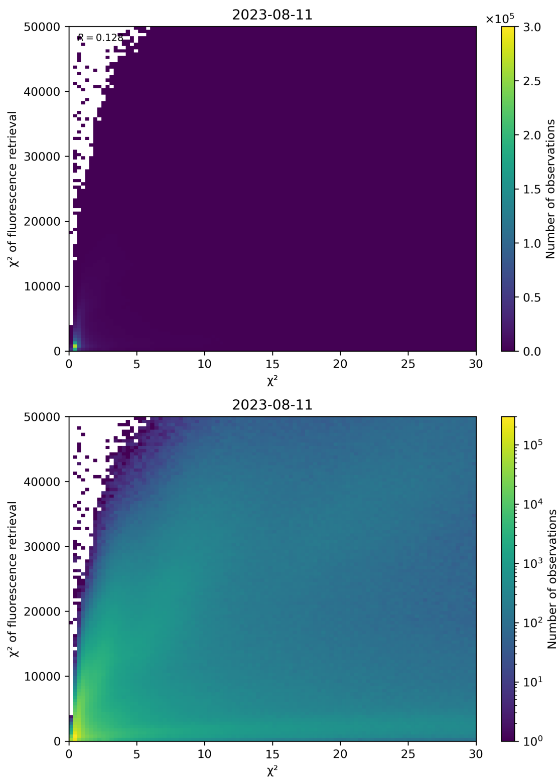
Figure 69: Scatter density plot of “ \chi^2 ” against “ \chi^2 of fluorescence retrieval” for 2023-08-10 to 2023-08-12.
