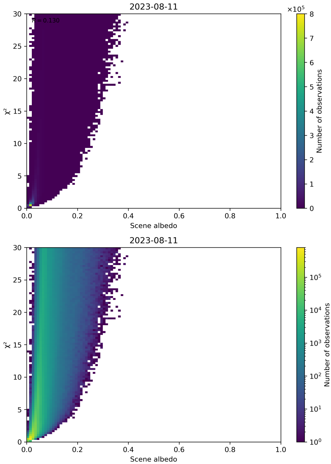
Figure 112: Scatter density plot of “Scene albedo” against “ \chi^2 ” for 2023-08-10 to 2023-08-12.
