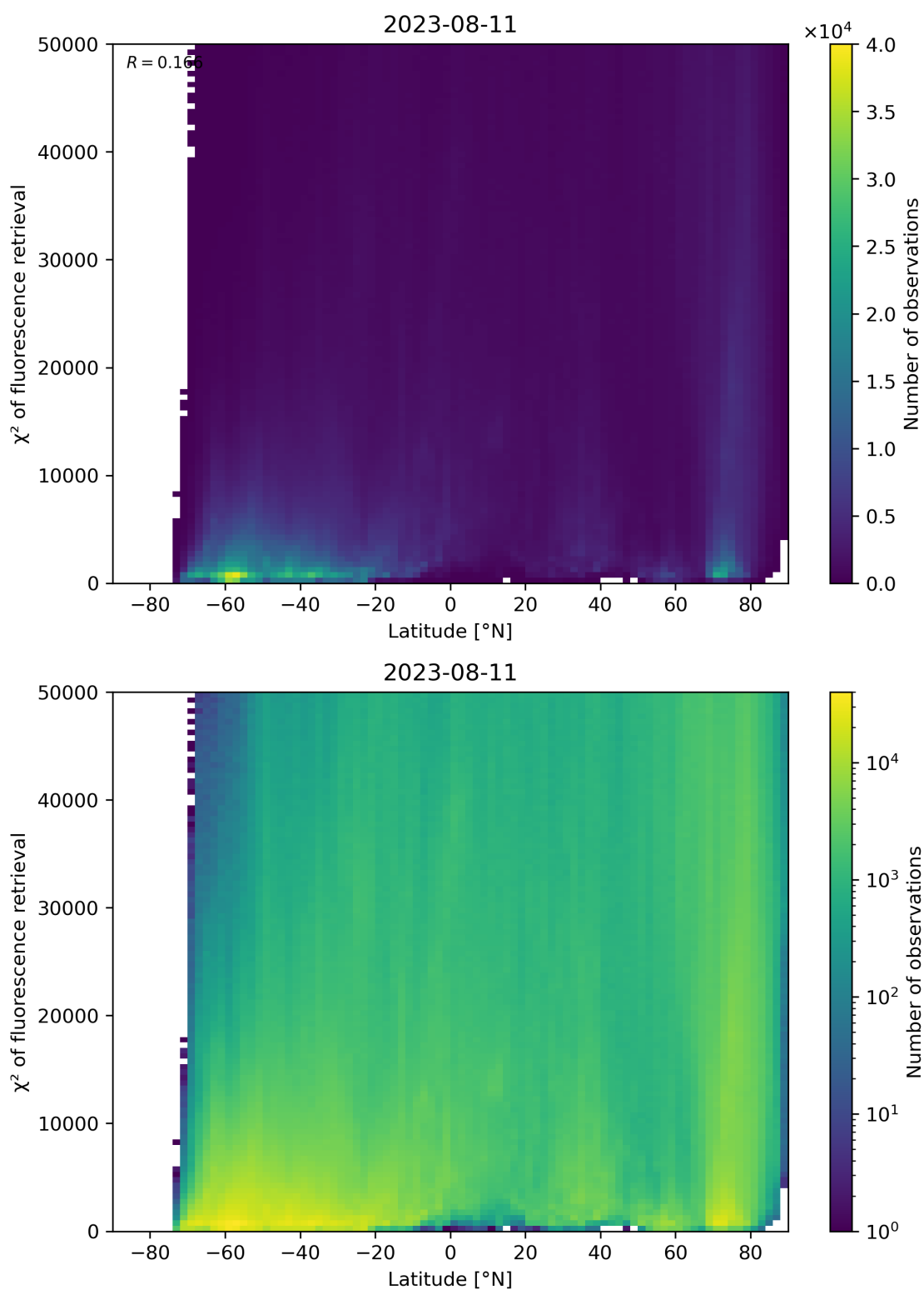
Figure 98: Scatter density plot of “Latitude” against “ \chi^2 of fluorescence retrieval” for 2023-08-10 to 2023-08-12.
