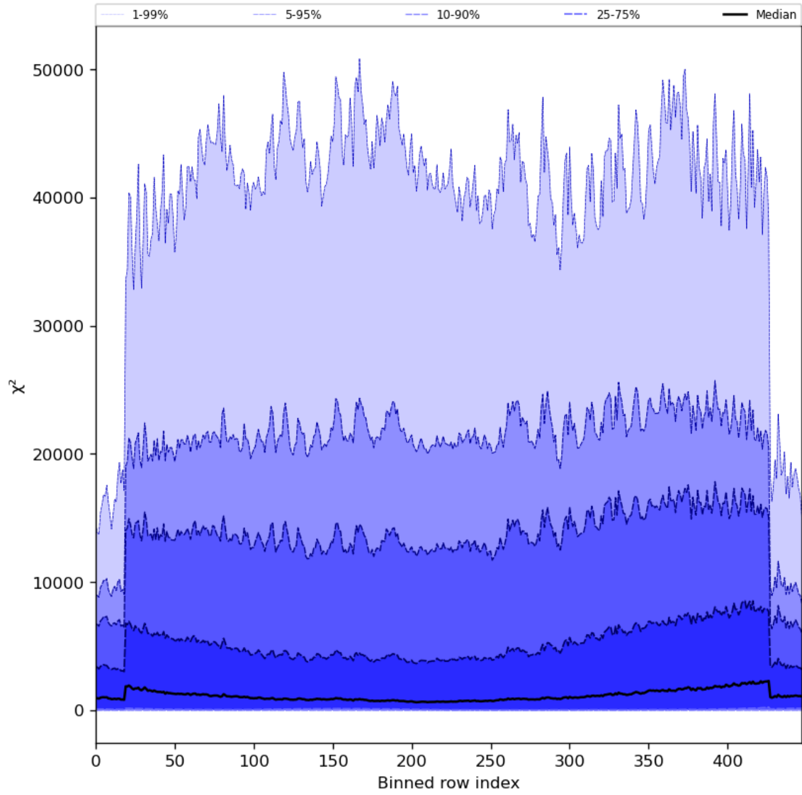
Figure 55: Along track statistics of “ \chi^2 ” for 2023-08-10 to 2023-08-12
