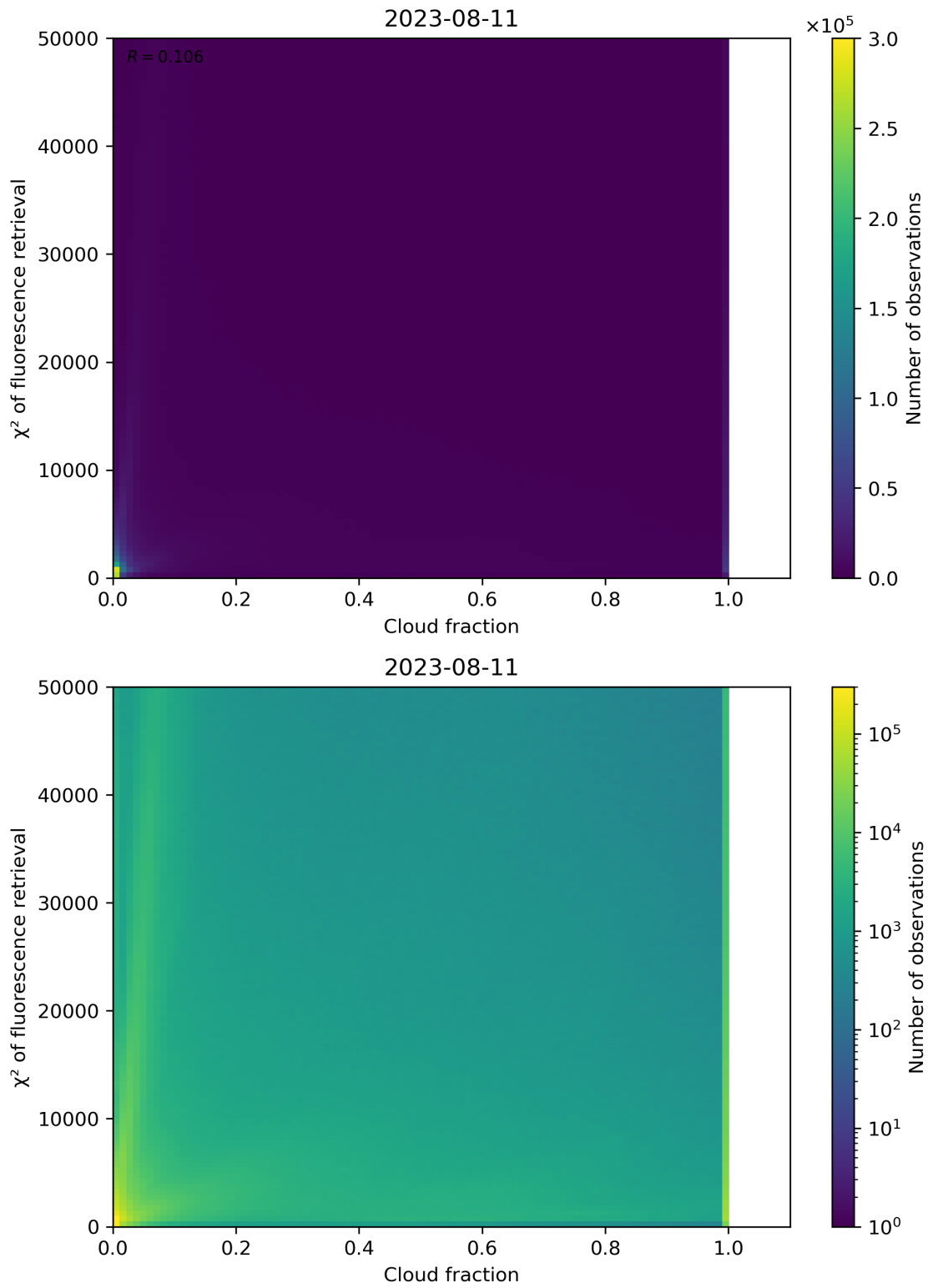
Figure 78: Scatter density plot of “Cloud fraction” against “ \chi^2 of fluorescence retrieval” for 2023-08-10 to 2023-08-12.
