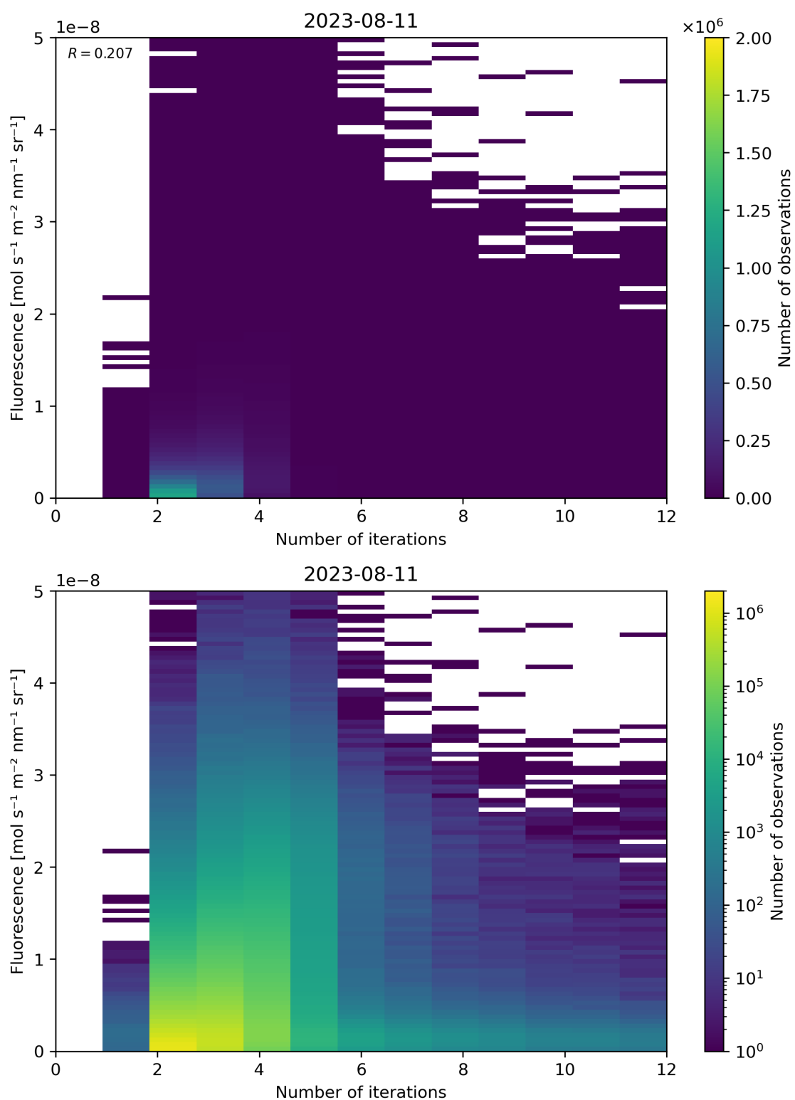
Figure 107: Scatter density plot of “Number of iterations” against “Fluorescence” for 2023-08-10 to 2023-08-12.
