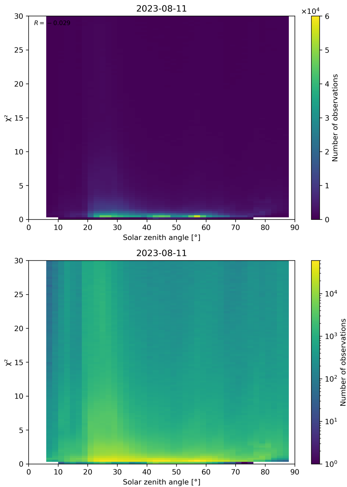
Figure 119: Scatter density plot of “Solar zenith angle” against “ \chi^2 ” for 2023-08-10 to 2023-08-12.
