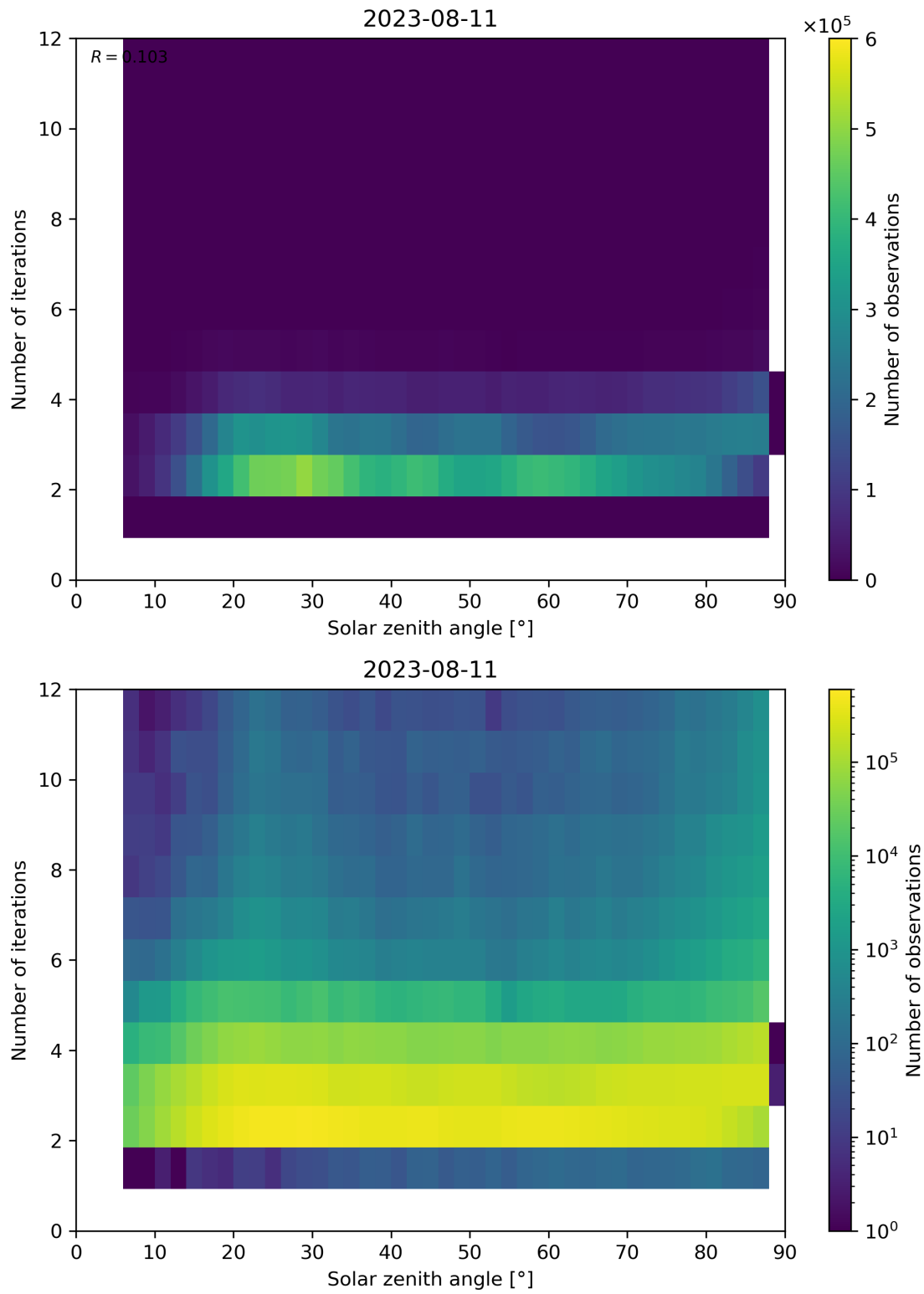
Figure 125: Scatter density plot of “Solar zenith angle” against “Number of iterations” for 2023-08-10 to 2023-08-12.
