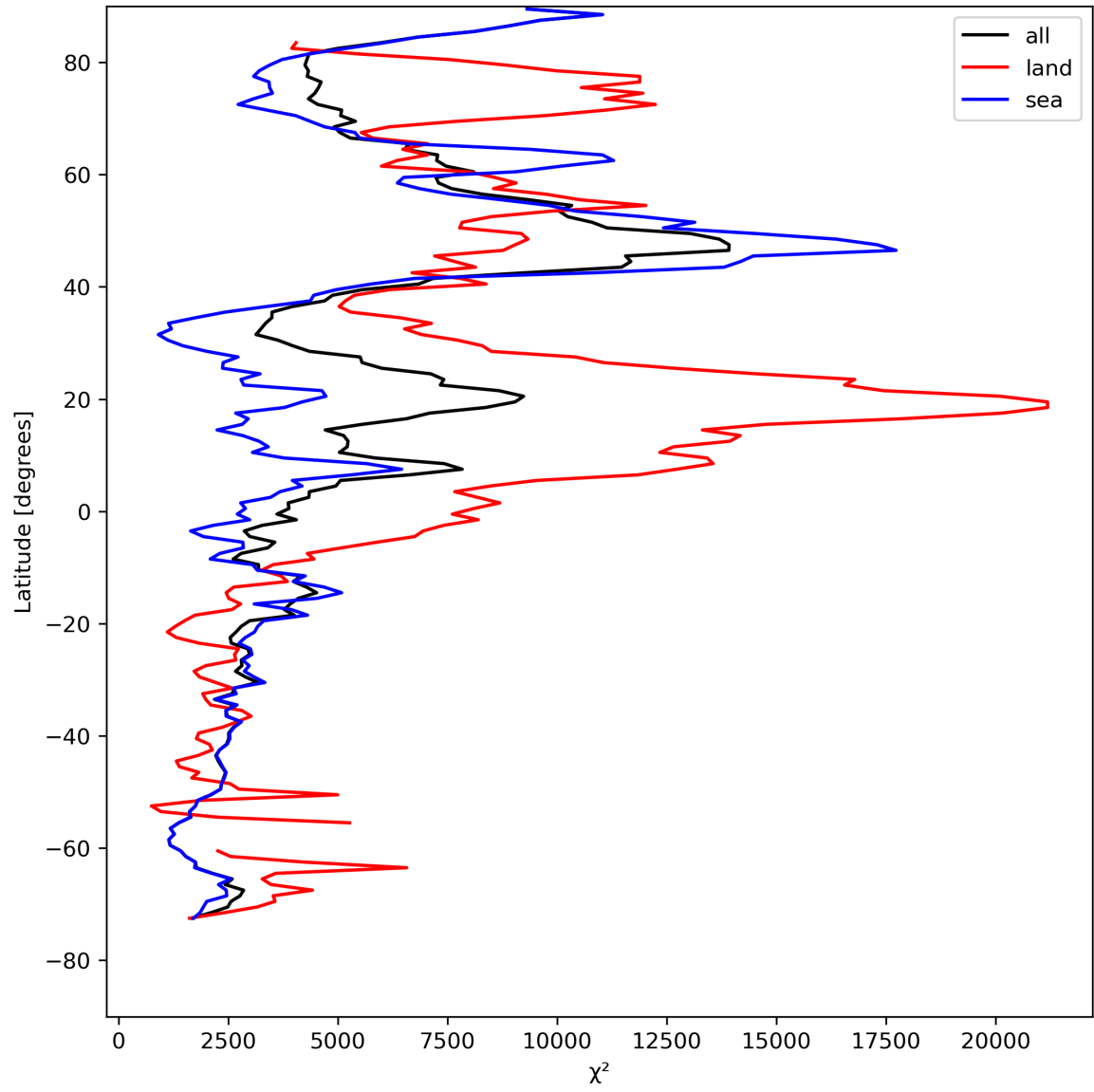
Figure 21: Zonal average of “ \chi^2 ” for 2023-08-10 to 2023-08-12.
