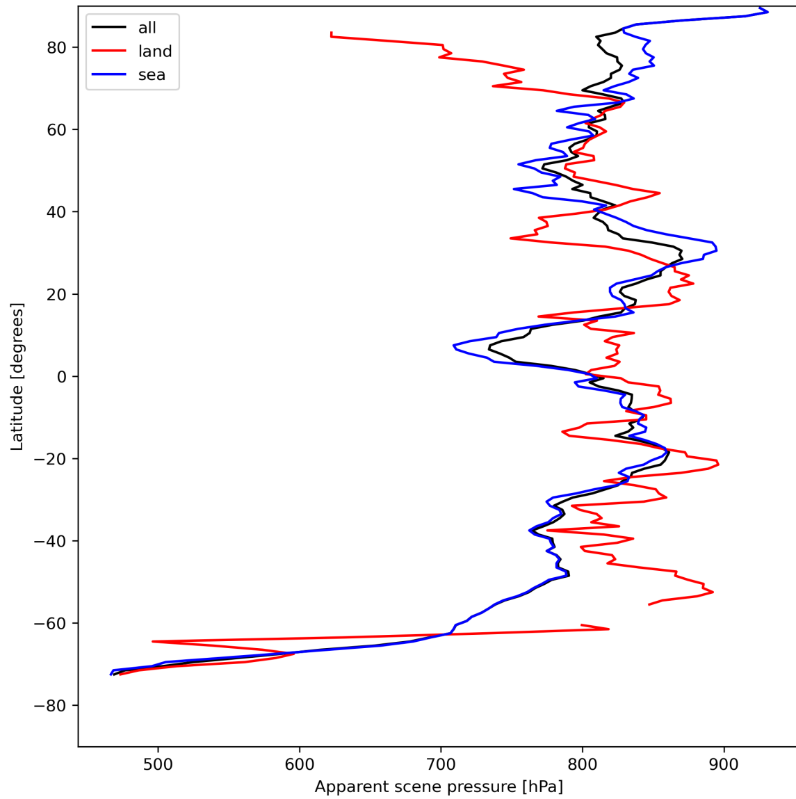
Figure 19: Zonal average of “Apparent scene pressure” for 2023-08-10 to 2023-08-12.
