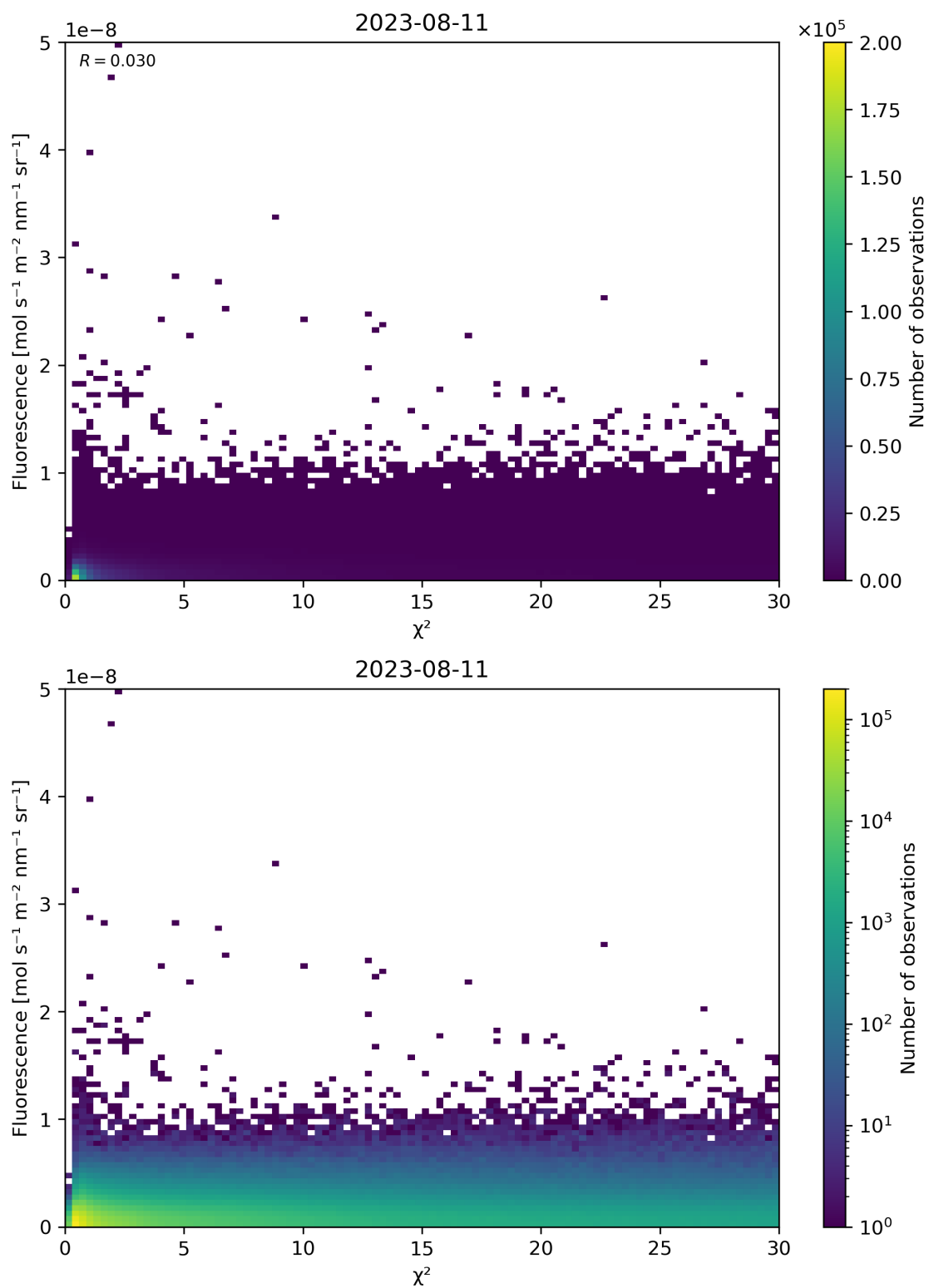
Figure 70: Scatter density plot of “ \chi^2 ” against “Fluorescence” for 2023-08-10 to 2023-08-12.
