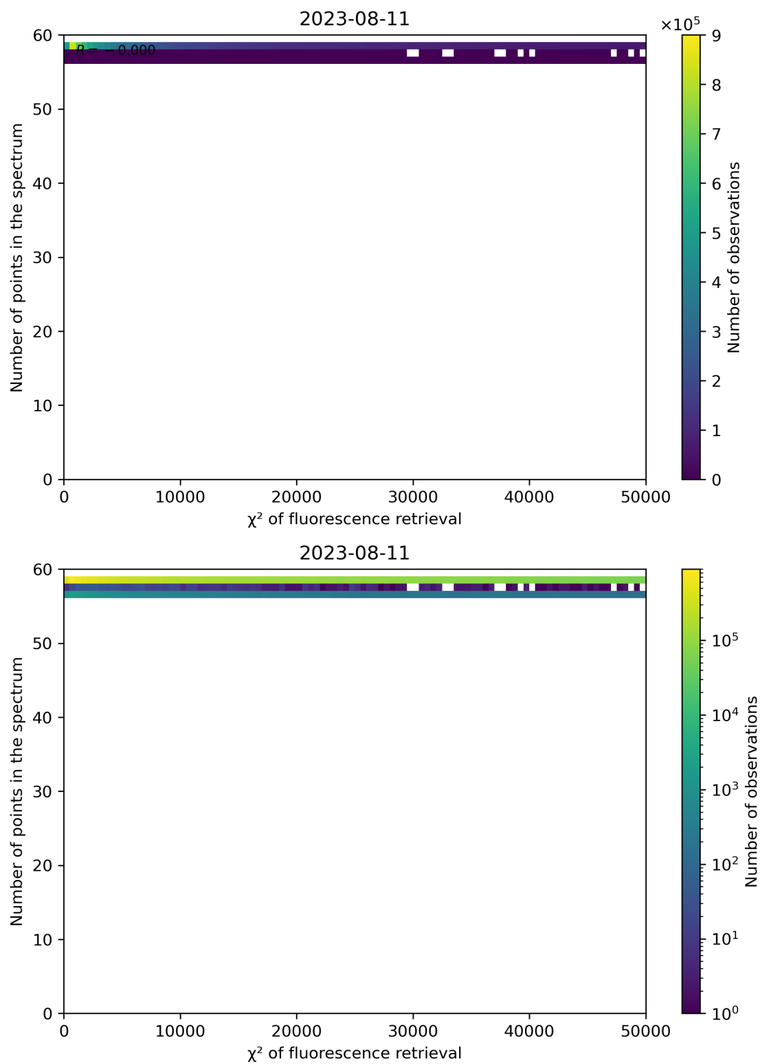
Figure 71: Scatter density plot of " \chi^2 of fluorescence retrieval" against "Number of points in the spectrum" for 2023-08-10 to 2023-08-12.
