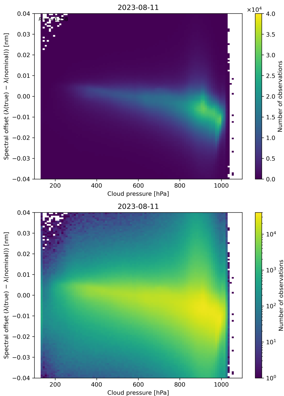
Figure 92: Scatter density plot of “Cloud pressure” against “Spectral offset ( \lambda(\text{true}) - \lambda(\text{nominal}) )” for 2023-08-10 to 2023-08-12.
