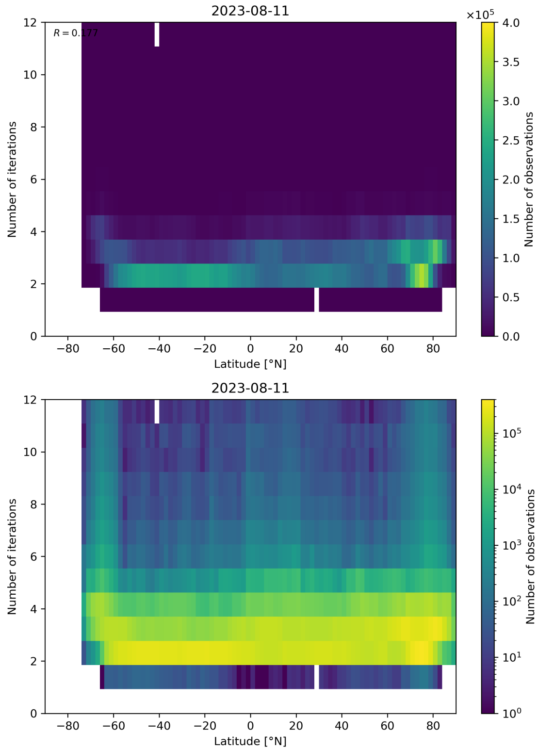
Figure 102: Scatter density plot of “Latitude” against “Number of iterations” for 2023-08-10 to 2023-08-12.
