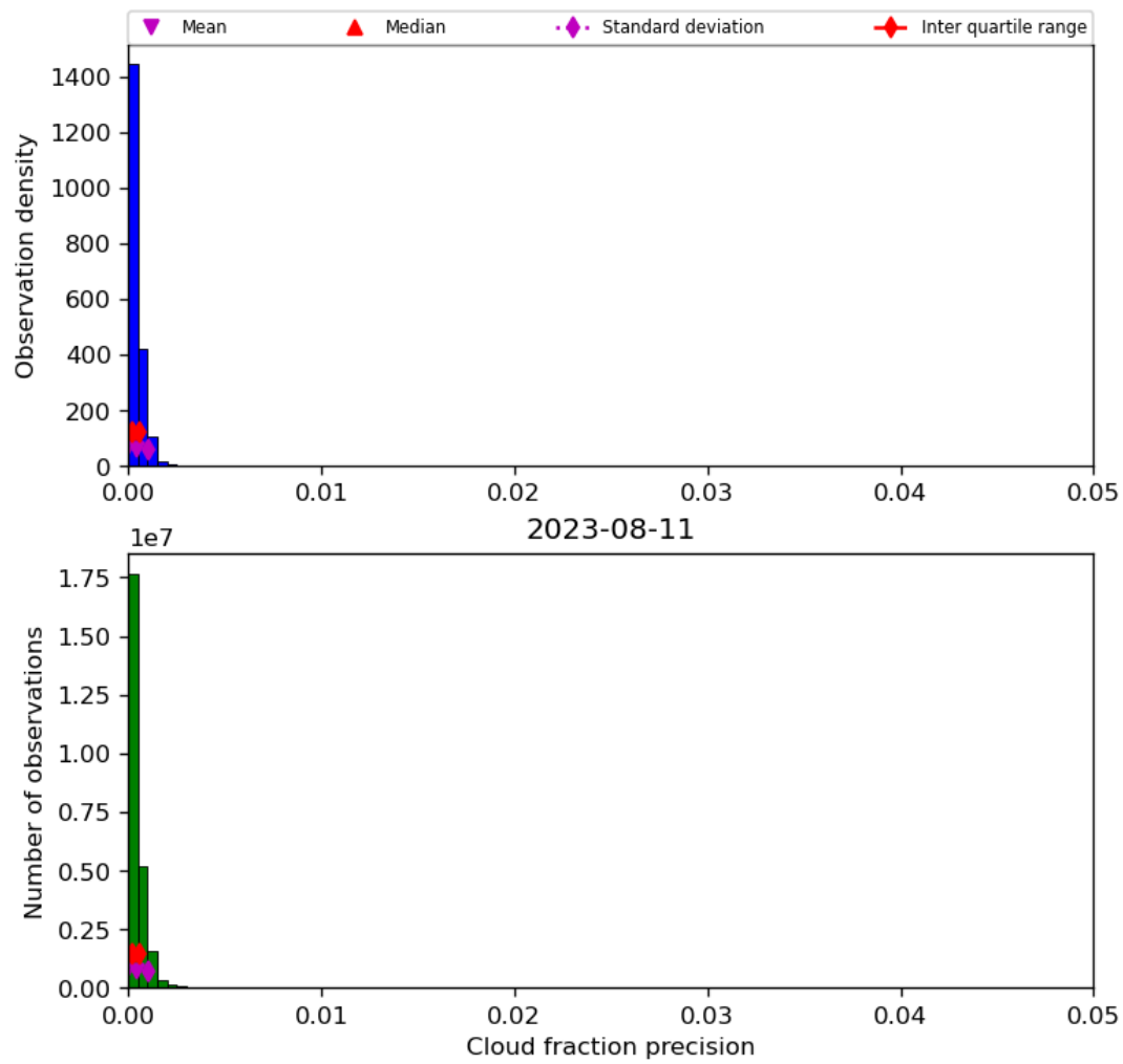
Figure 33: Histogram of “Cloud fraction precision” for 2023-08-10 to 2023-08-12
