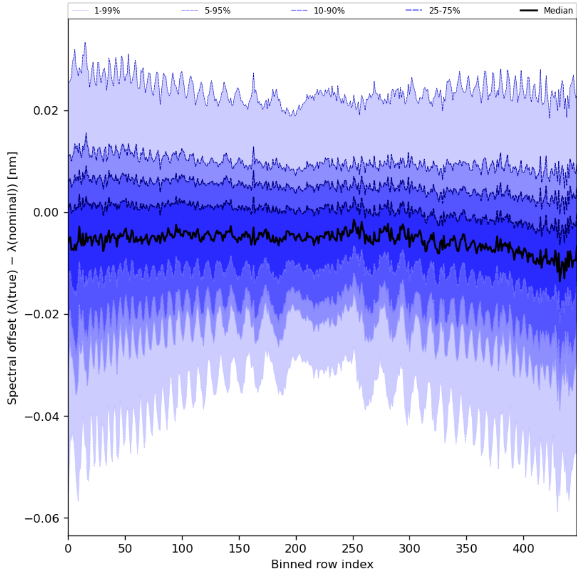
Figure 62: Along track statistics of “Spectral offset ( \lambda(\text{true}) - \lambda(\text{nominal}) )” for 2023-08-10 to 2023-08-12
