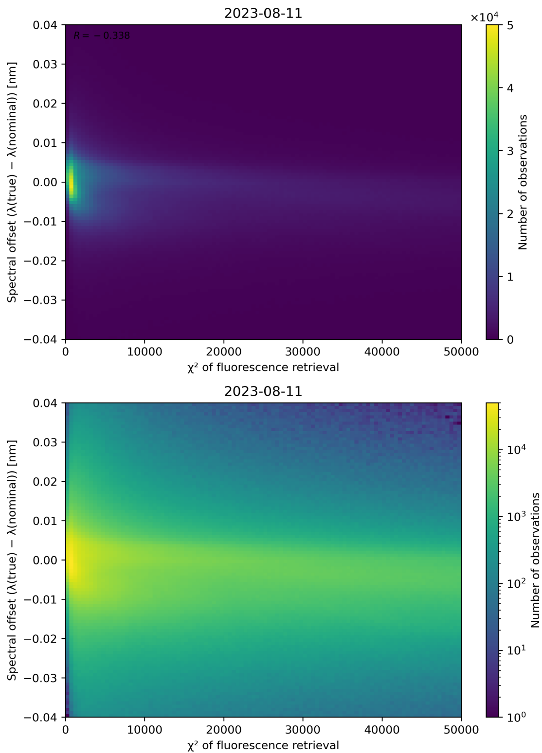
Figure 72: Scatter density plot of “ \chi^2 of fluorescence retrieval” against “Spectral offset ( \lambda(\text{true}) - \lambda(\text{nominal}) )” for 2023-08-10 to 2023-08-12.
