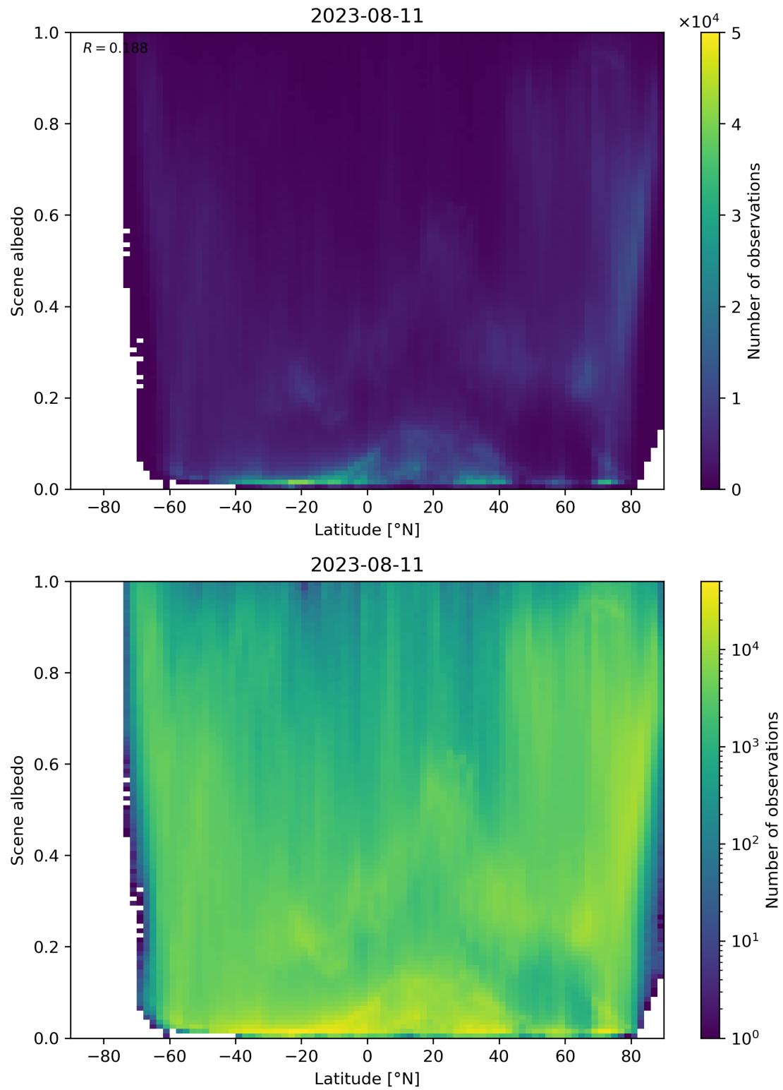
Figure 104: Scatter density plot of “Latitude” against “Scene albedo” for 2023-08-10 to 2023-08-12.
