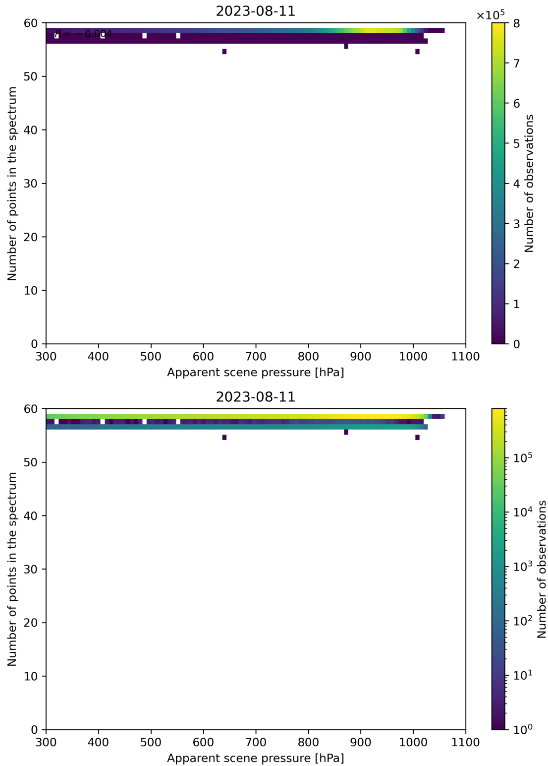
Figure 67: Scatter density plot of “Apparent scene pressure” against “Number of points in the spectrum” for 2023-08-10 to 2023-08-12.
