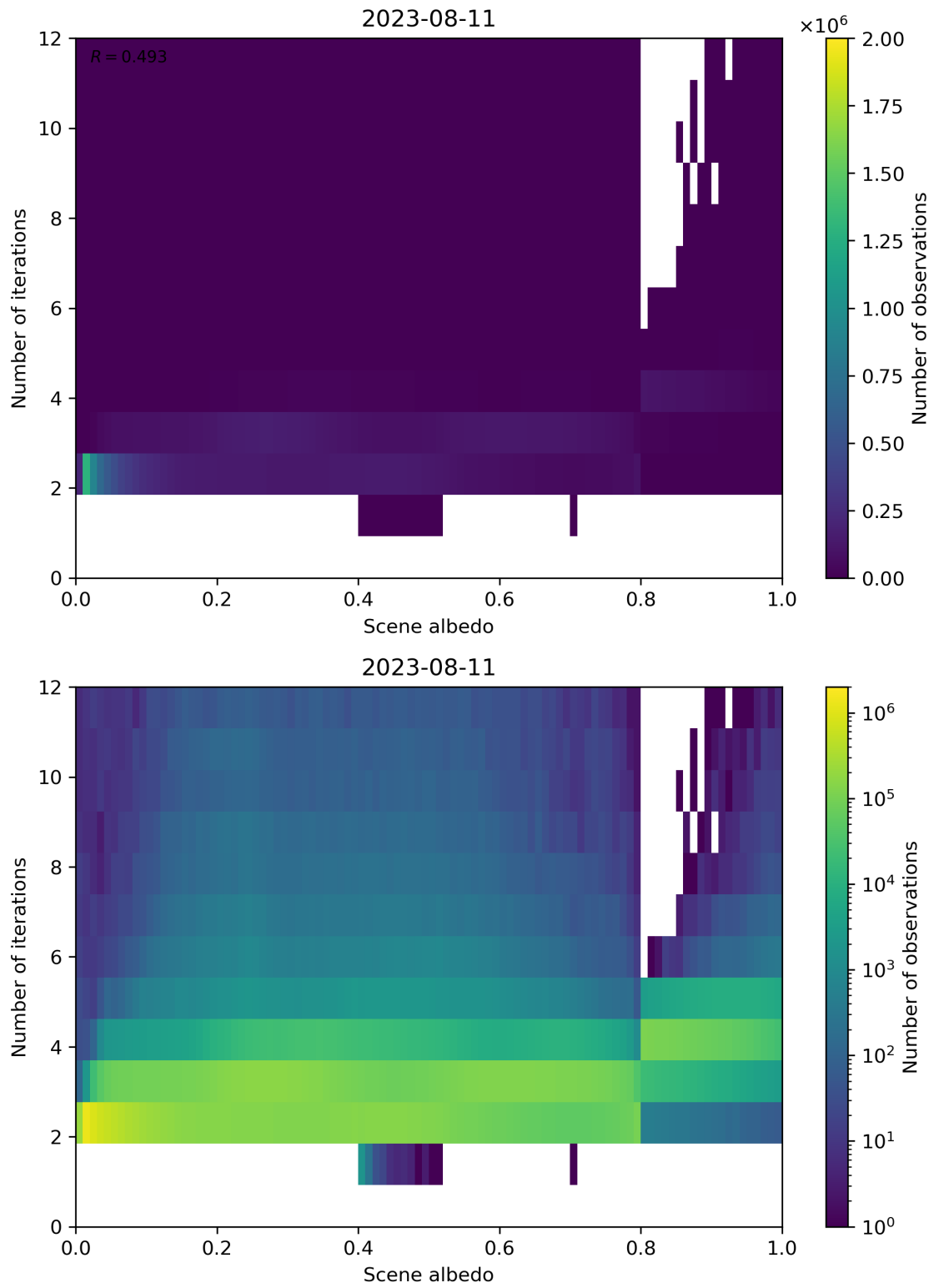
Figure 115: Scatter density plot of “Scene albedo” against “Number of iterations” for 2023-08-10 to 2023-08-12.
