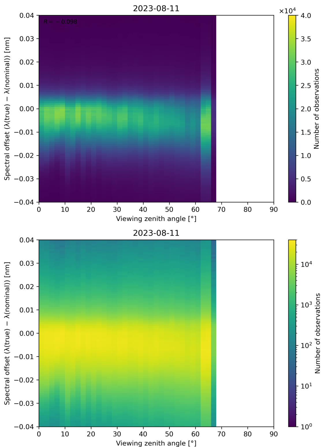
Figure 140: Scatter density plot of “Viewing zenith angle” against “Spectral offset ( \lambda(\text{true}) - \lambda(\text{nominal}) )” for 2023-08-10 to 2023-08-12.
