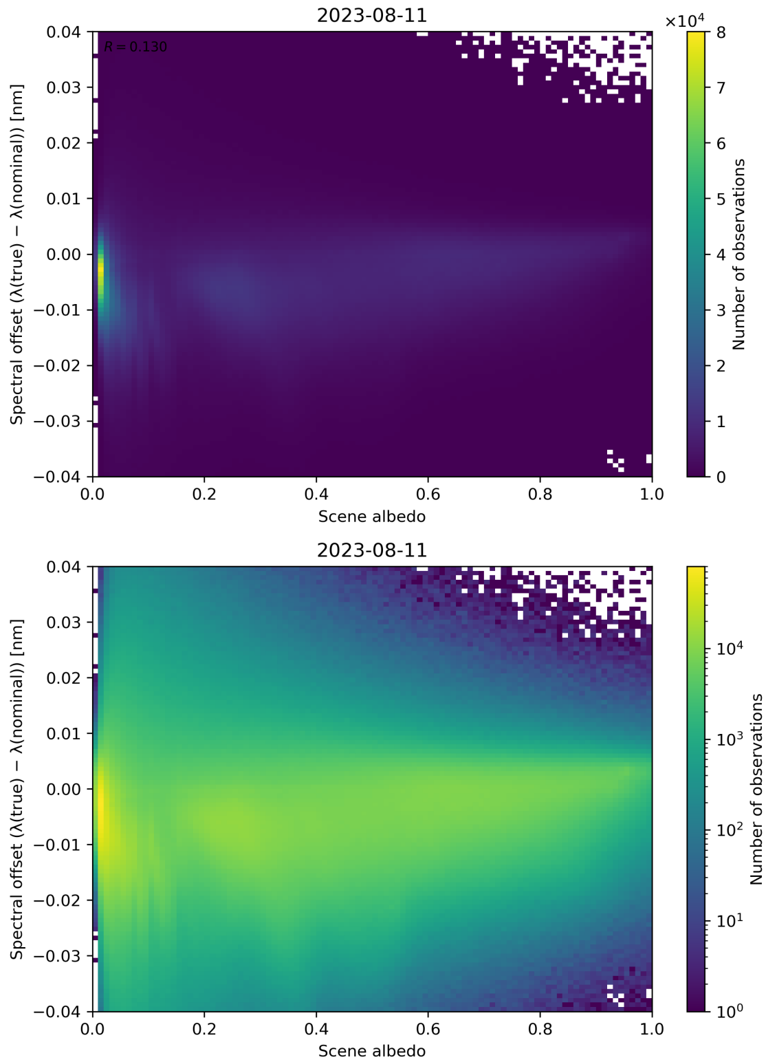
Figure 117: Scatter density plot of “Scene albedo” against “Spectral offset ( \lambda(\text{true}) - \lambda(\text{nominal}) )” for 2023-08-10 to 2023-08-12.
