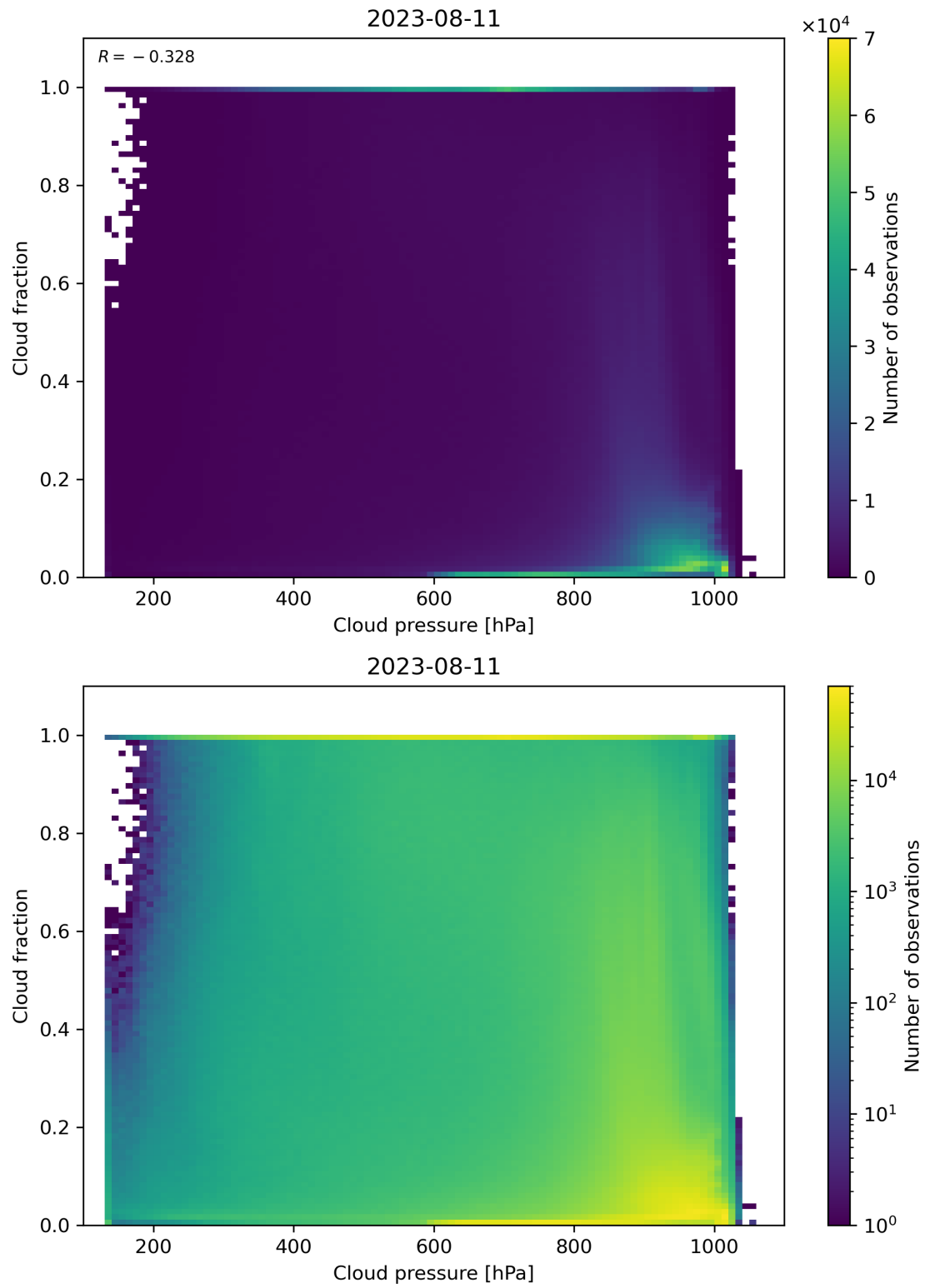
Figure 87: Scatter density plot of “Cloud pressure” against “Cloud fraction” for 2023-08-10 to 2023-08-12.
