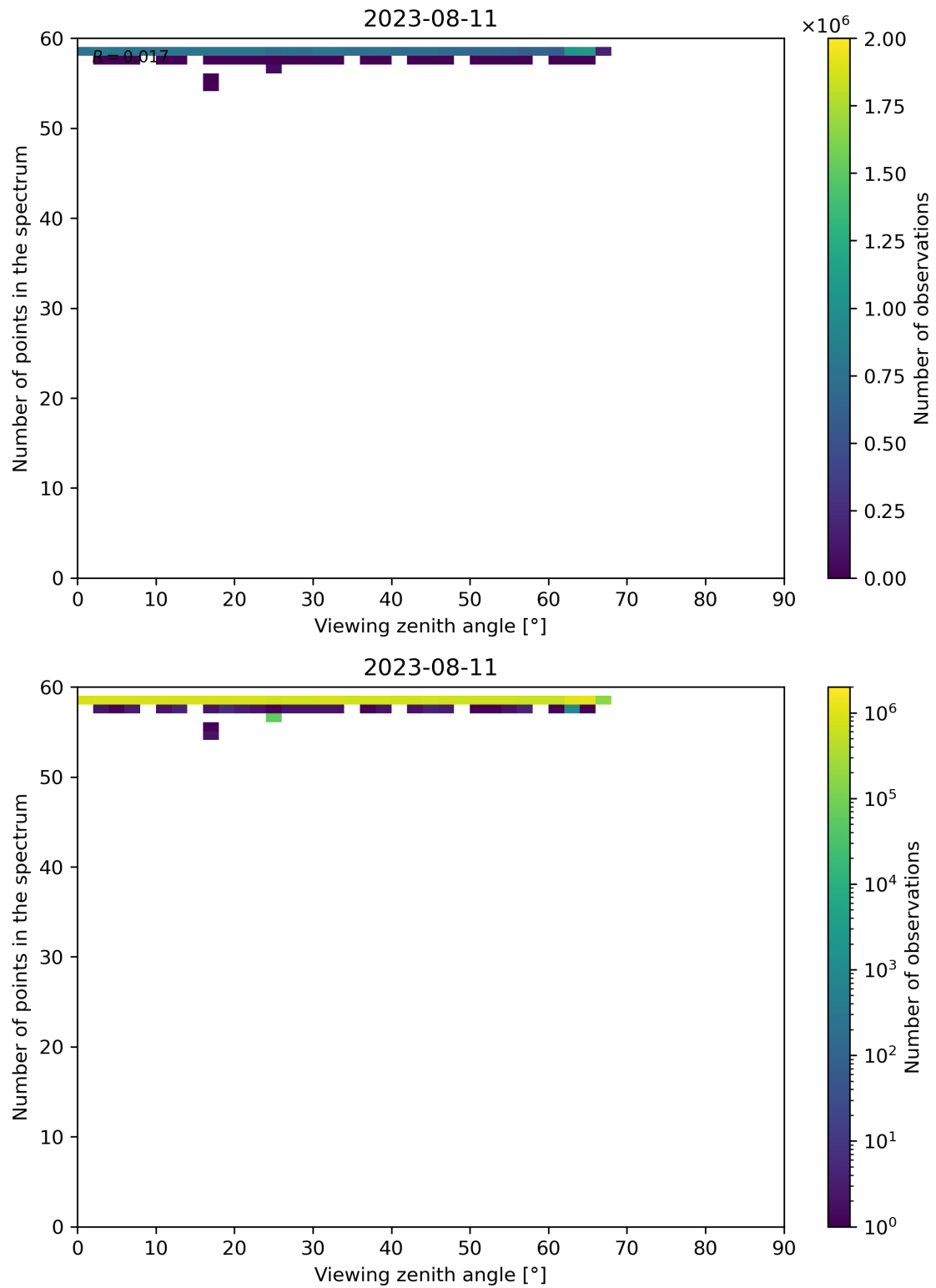
Figure 137: Scatter density plot of “Viewing zenith angle” against “Number of points in the spectrum” for 2023-08-10 to 2023-08-12.
