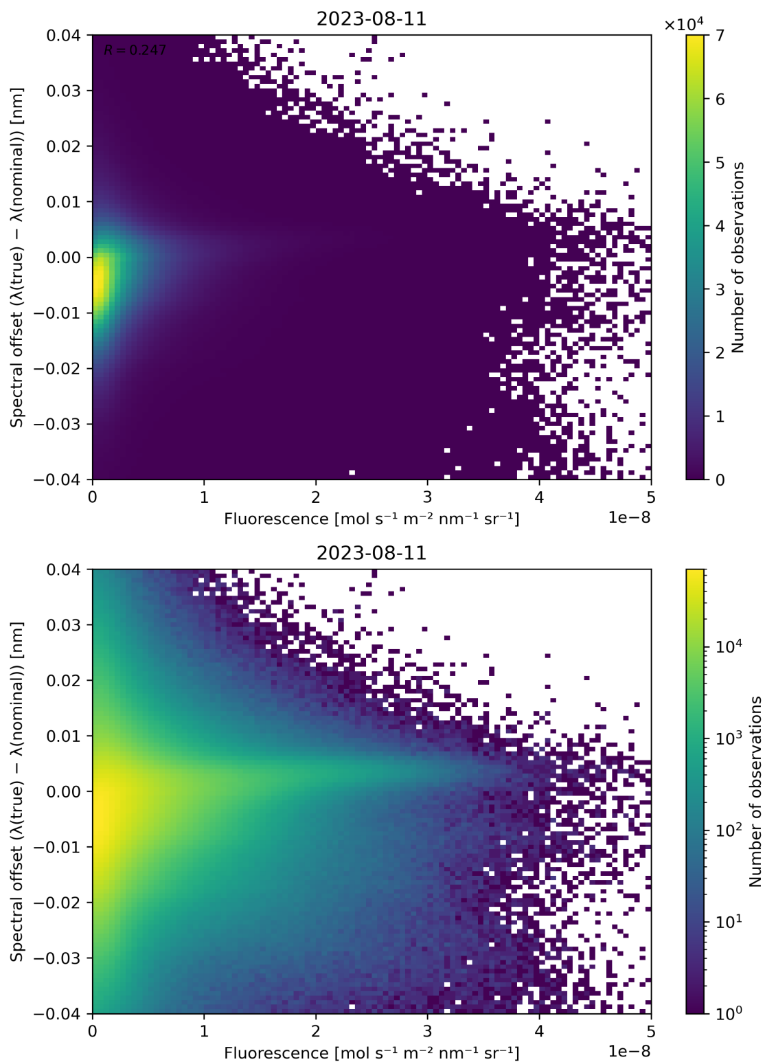
Figure 95: Scatter density plot of “Fluorescence” against “Spectral offset ( \lambda(\text{true}) - \lambda(\text{nominal}) )” for 2023-08-10 to 2023-08-12.
