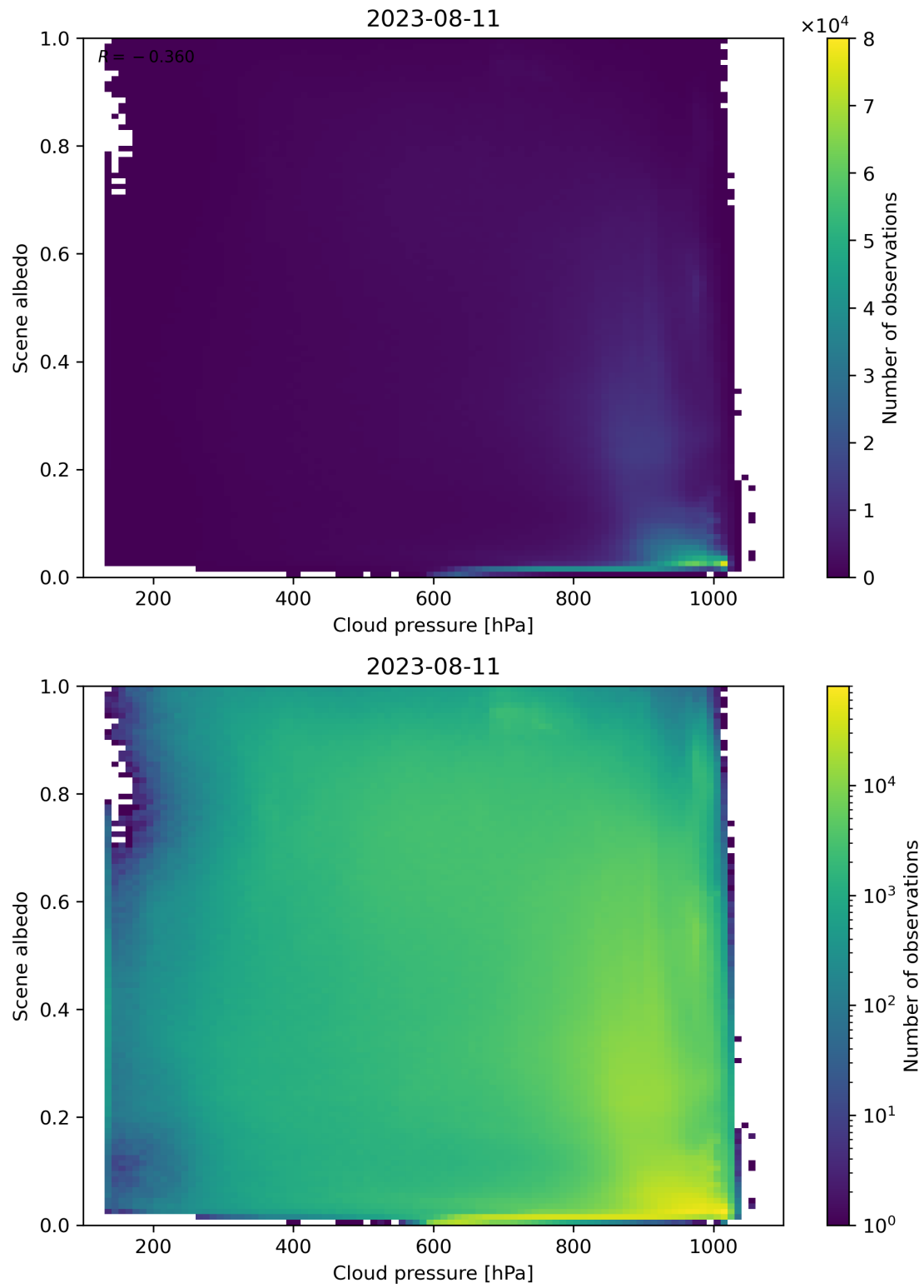
Figure 91: Scatter density plot of “Cloud pressure” against “Scene albedo” for 2023-08-10 to 2023-08-12.
