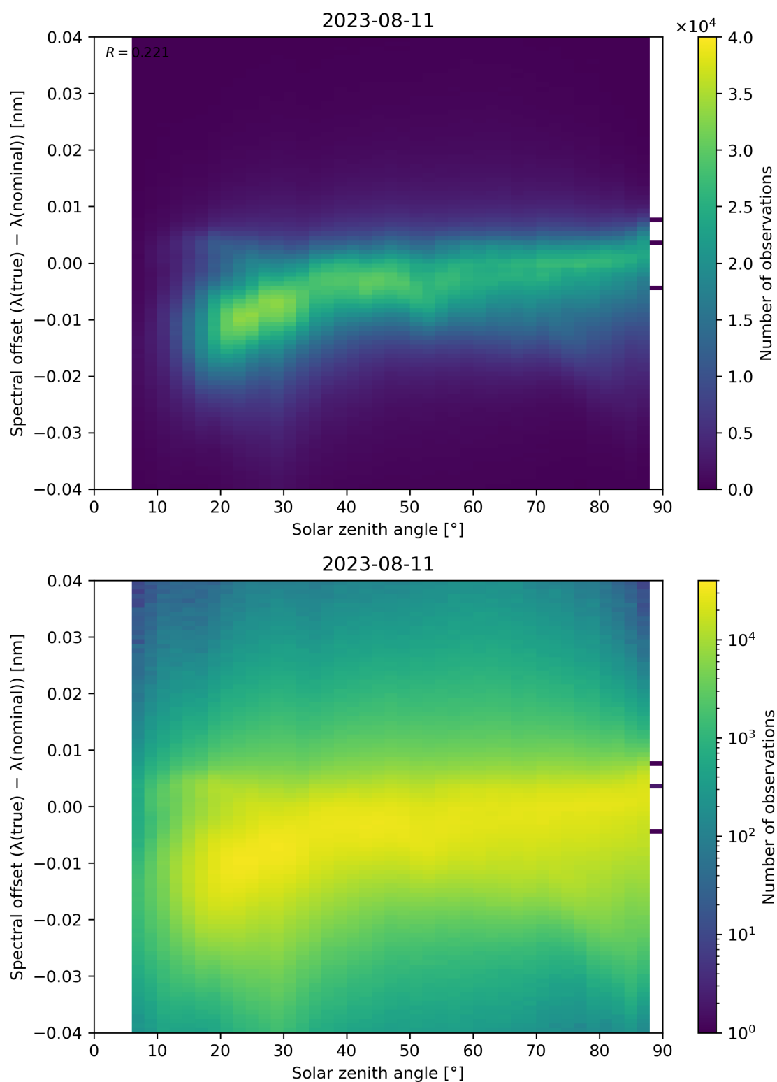
Figure 128: Scatter density plot of “Solar zenith angle” against “Spectral offset ( \lambda(\text{true}) - \lambda(\text{nominal}) )” for 2023-08-10 to 2023-08-12.
