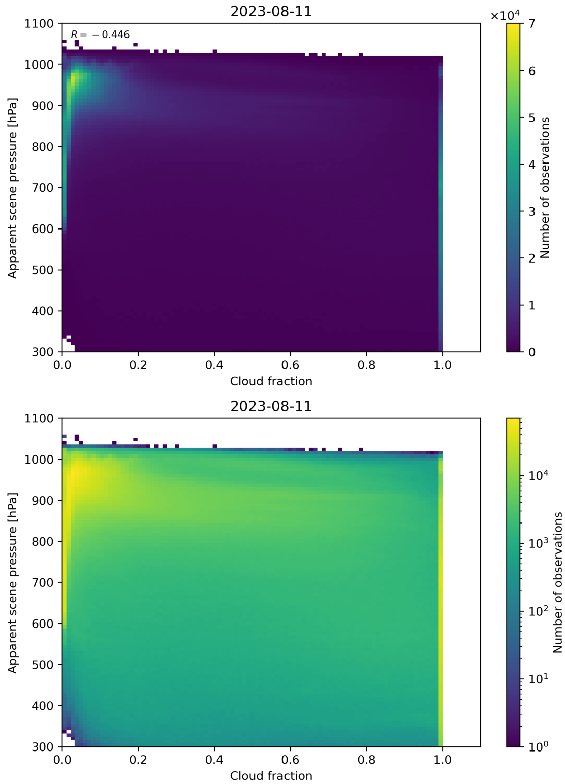
Figure 76: Scatter density plot of “Cloud fraction” against “Apparent scene pressure” for 2023-08-10 to 2023-08-12.
