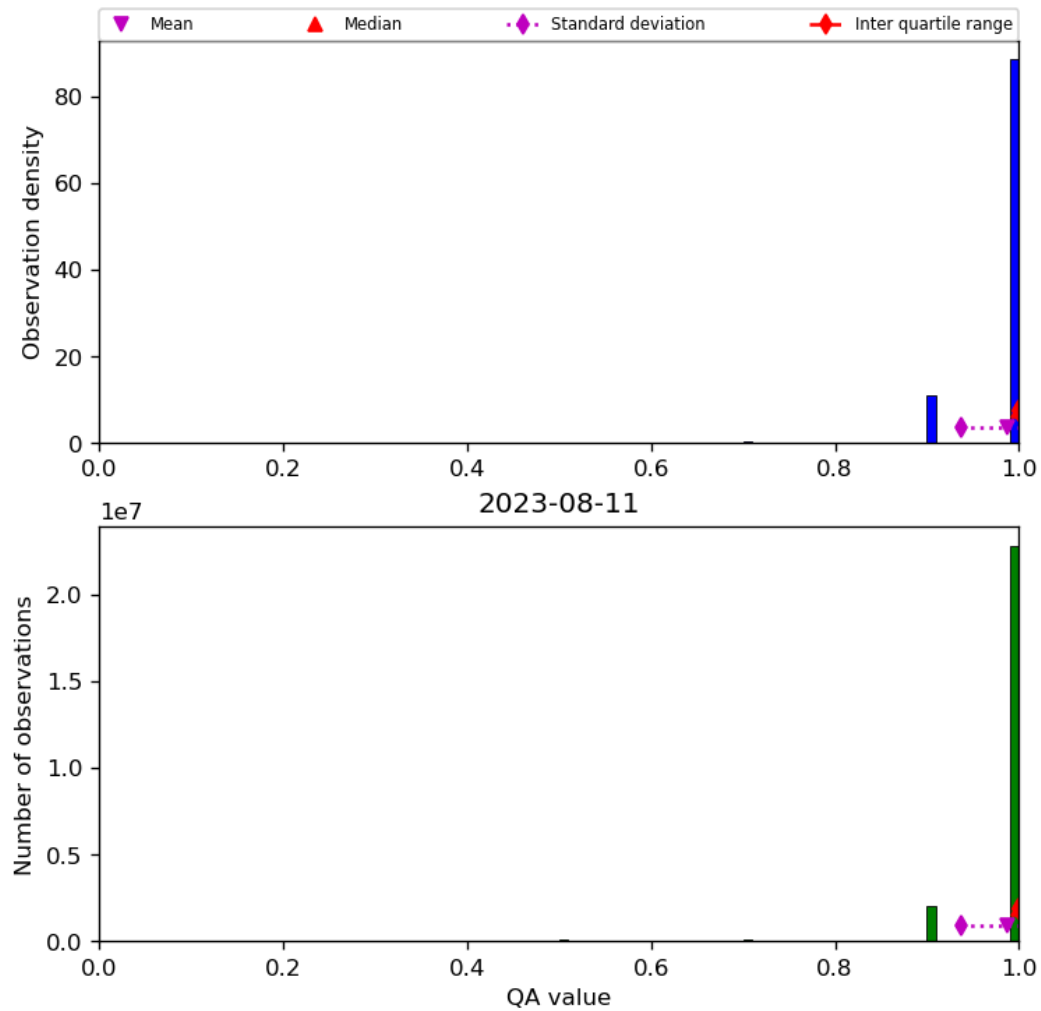
Figure 29: Histogram of “QA value” for 2023-08-10 to 2023-08-12
