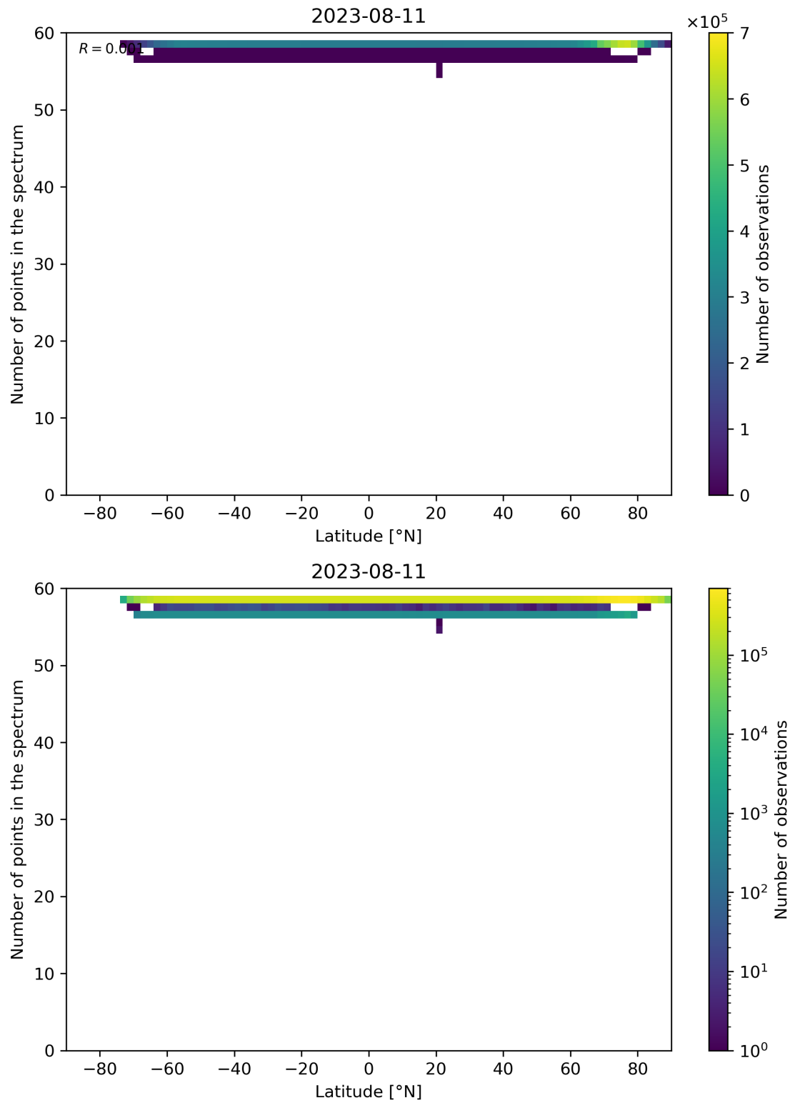
Figure 103: Scatter density plot of “Latitude” against “Number of points in the spectrum” for 2023-08-10 to 2023-08-12.
