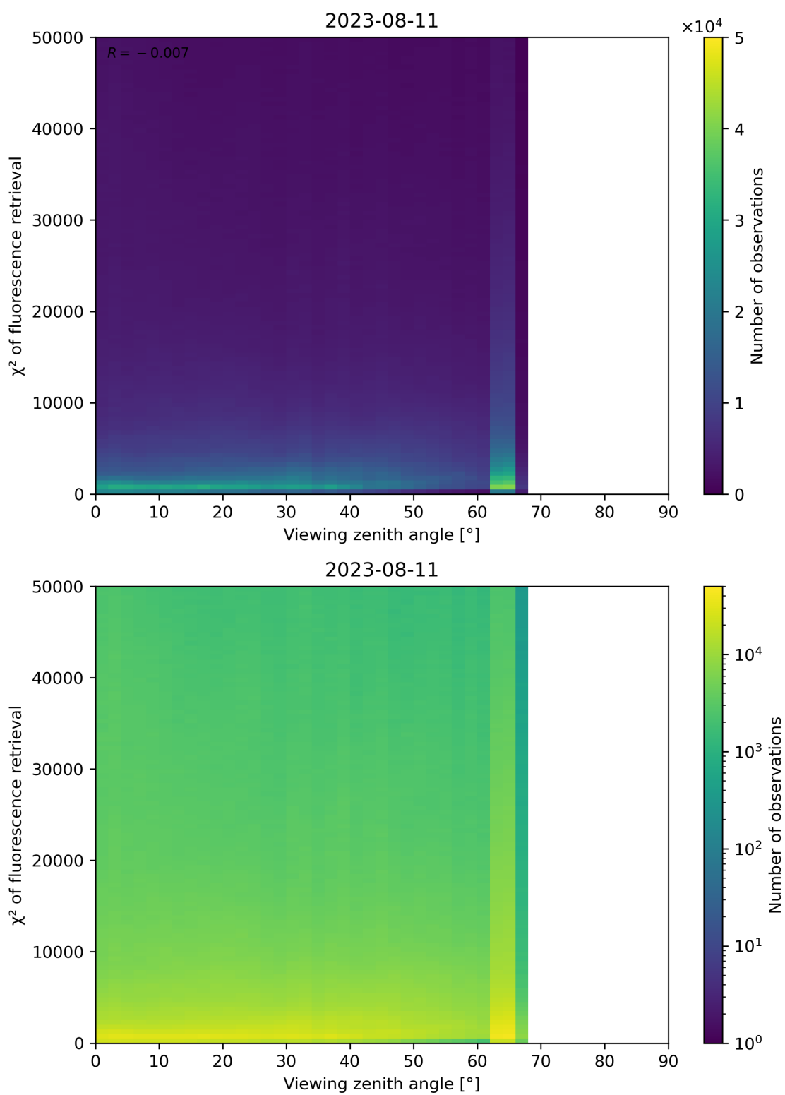
Figure 131: Scatter density plot of “Viewing zenith angle” against “ \chi^2 of fluorescence retrieval” for 2023-08-10 to 2023-08-12.
