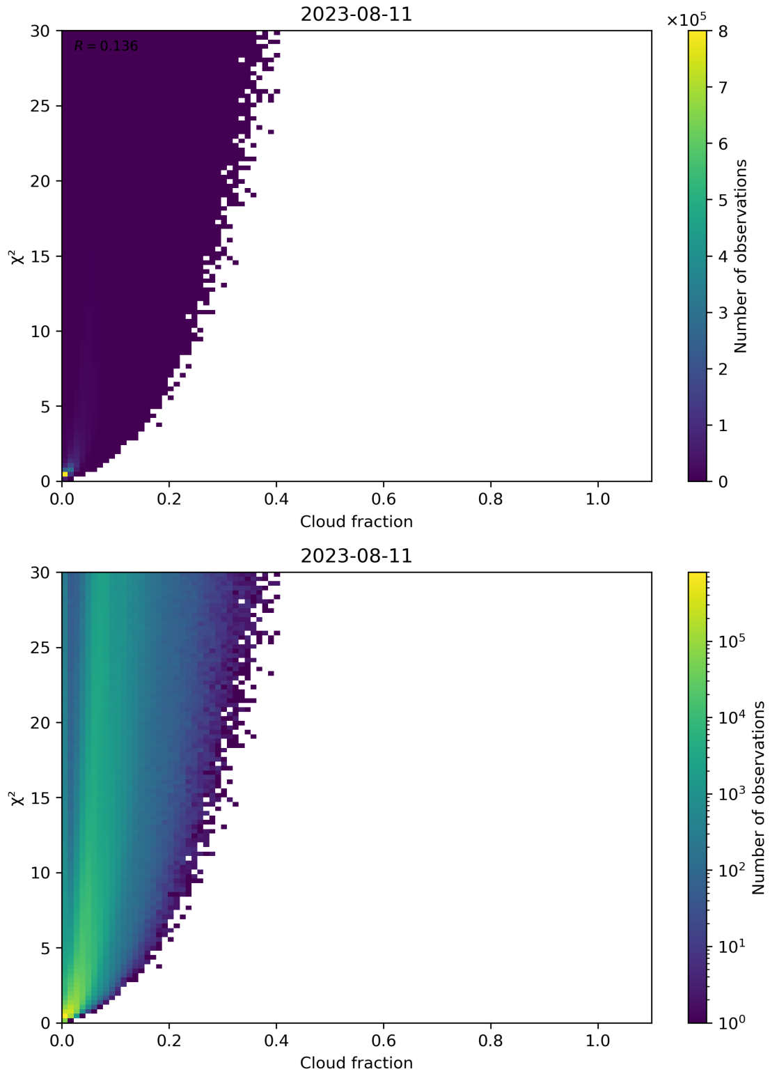
Figure 77: Scatter density plot of “Cloud fraction” against “ \chi^2 ” for 2023-08-10 to 2023-08-12.
