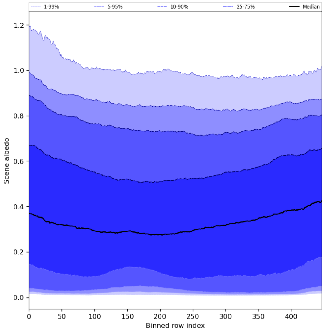
Figure 51: Along track statistics of “Scene albedo” for 2023-08-10 to 2023-08-12
