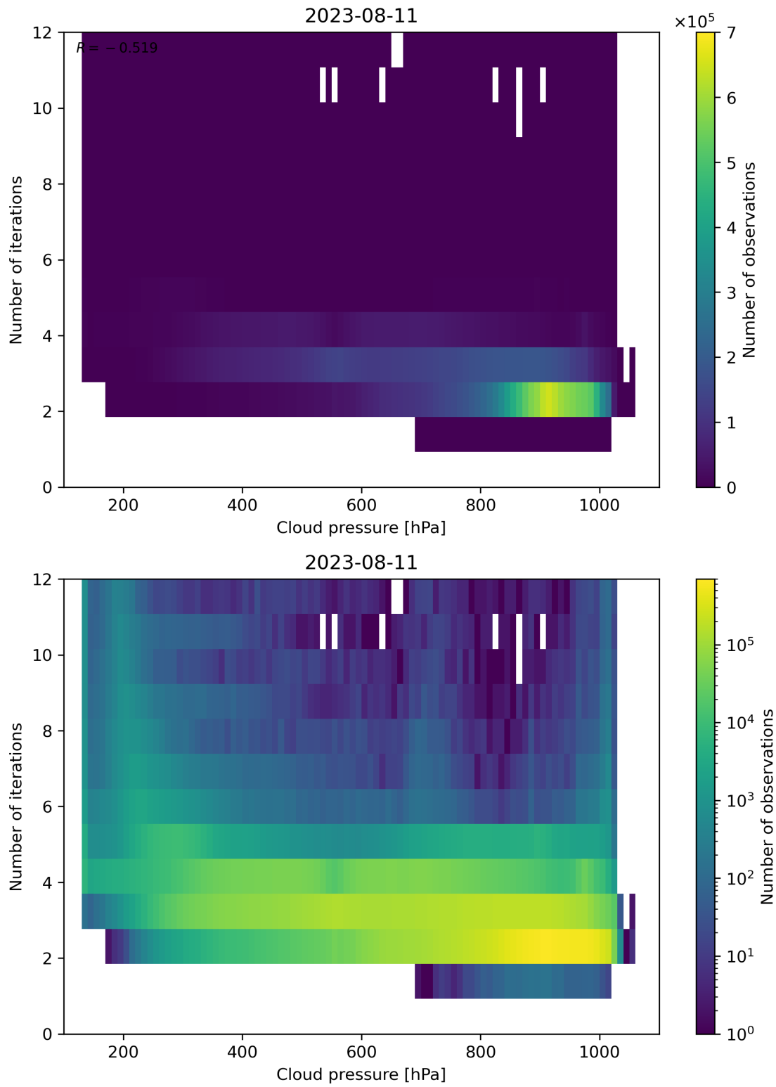
Figure 89: Scatter density plot of “Cloud pressure” against “Number of iterations” for 2023-08-10 to 2023-08-12.
