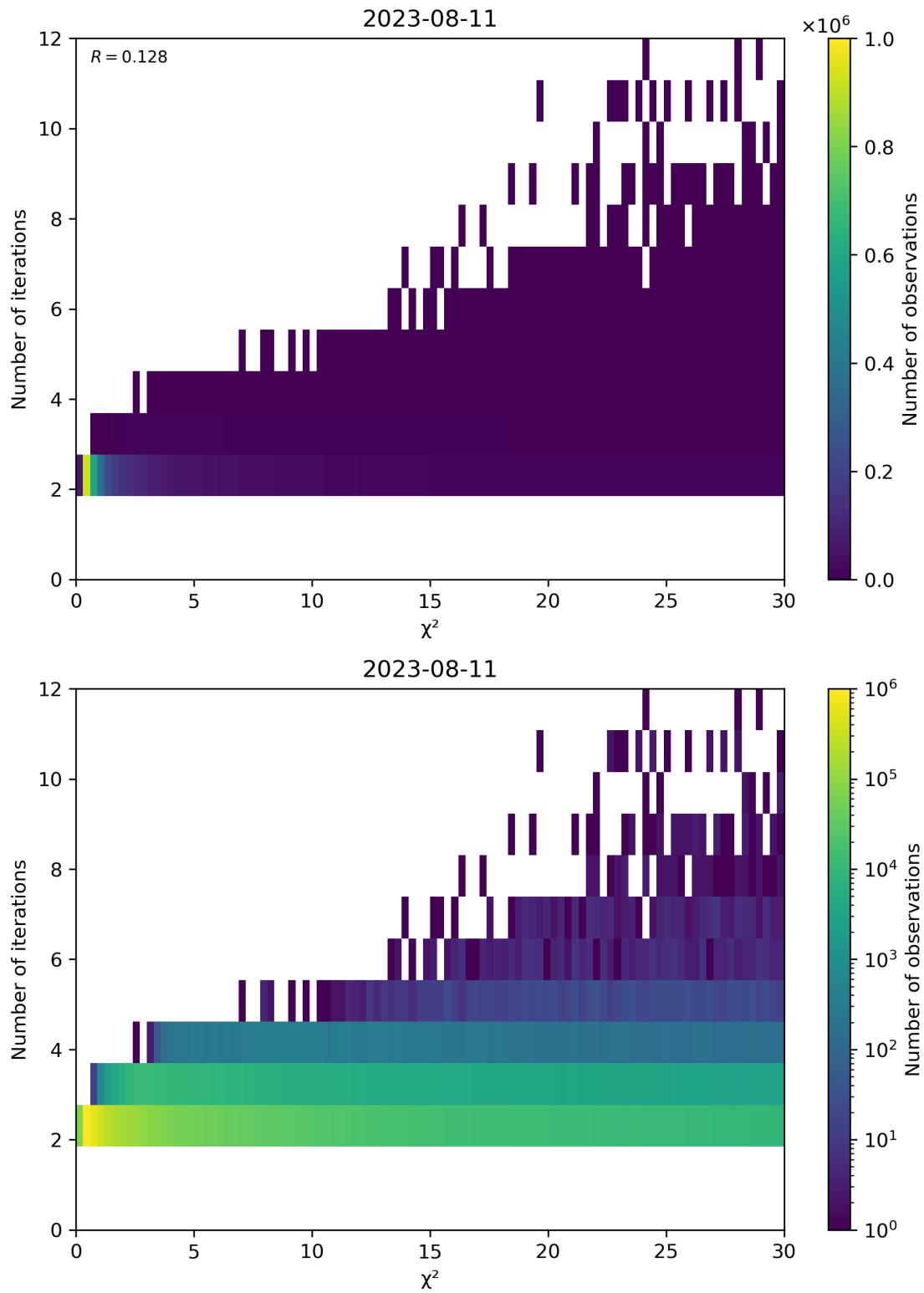
Figure 73: Scatter density plot of “ \chi^2 ” against “Number of iterations” for 2023-08-10 to 2023-08-12.
