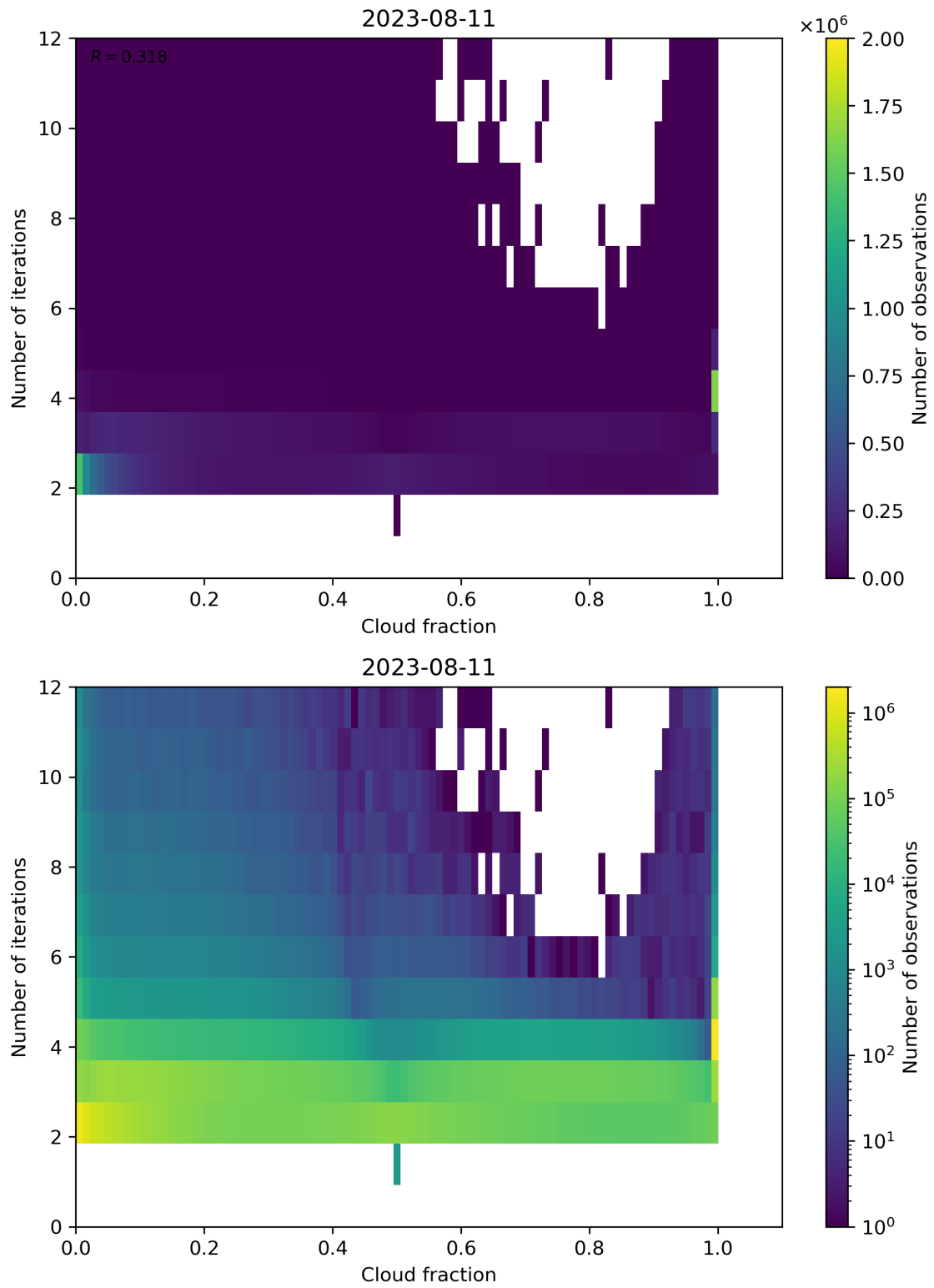
Figure 80: Scatter density plot of “Cloud fraction” against “Number of iterations” for 2023-08-10 to 2023-08-12.
