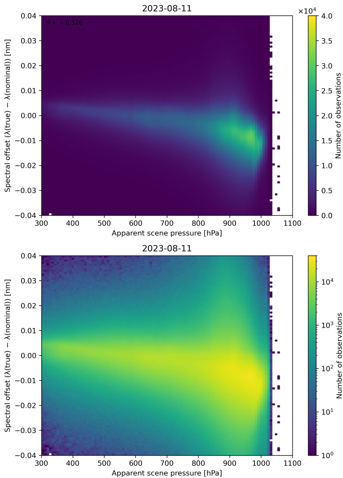
Figure 68: Scatter density plot of “Apparent scene pressure” against “Spectral offset ( \lambda(\text{true}) - \lambda(\text{nominal}) )” for 2023-08-10 to 2023-08-12.
