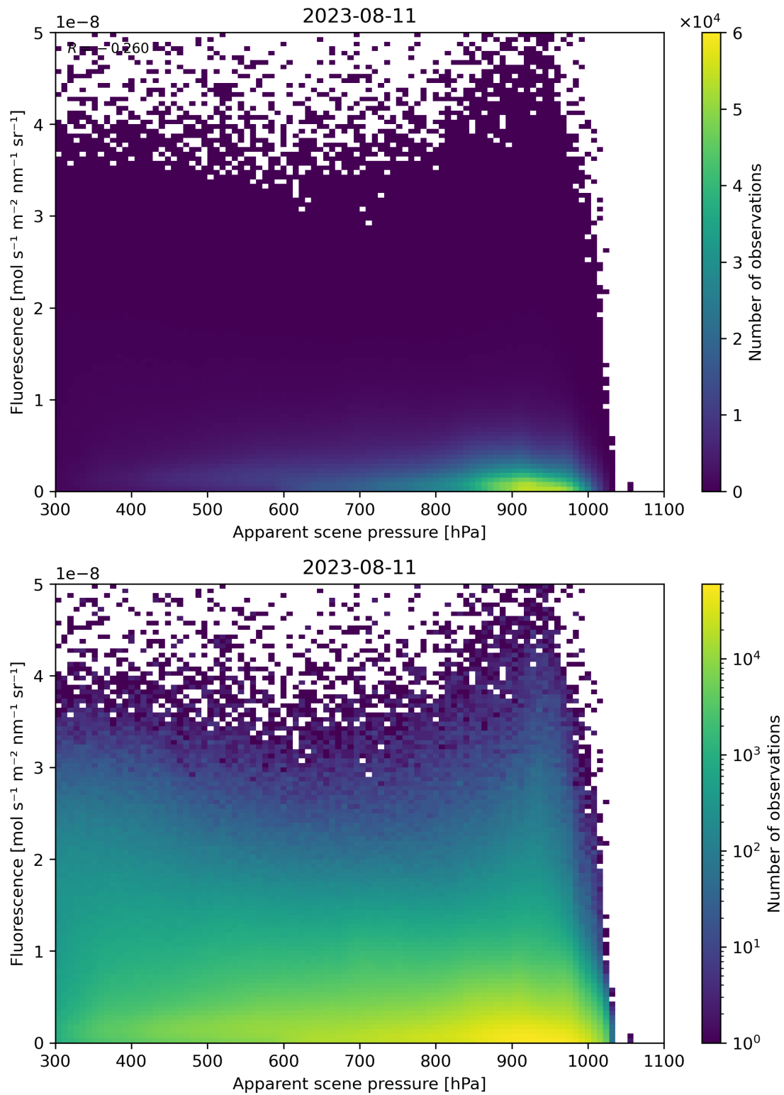
Figure 65: Scatter density plot of “Apparent scene pressure” against “Fluorescence” for 2023-08-10 to 2023-08-12.
