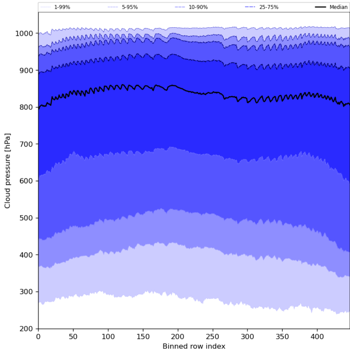
Figure 47: Along track statistics of “Cloud pressure” for 2023-08-10 to 2023-08-12
