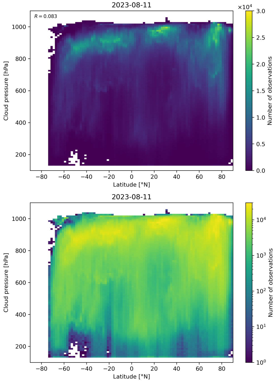
Figure 100: Scatter density plot of “Latitude” against “Cloud pressure” for 2023-08-10 to 2023-08-12.
