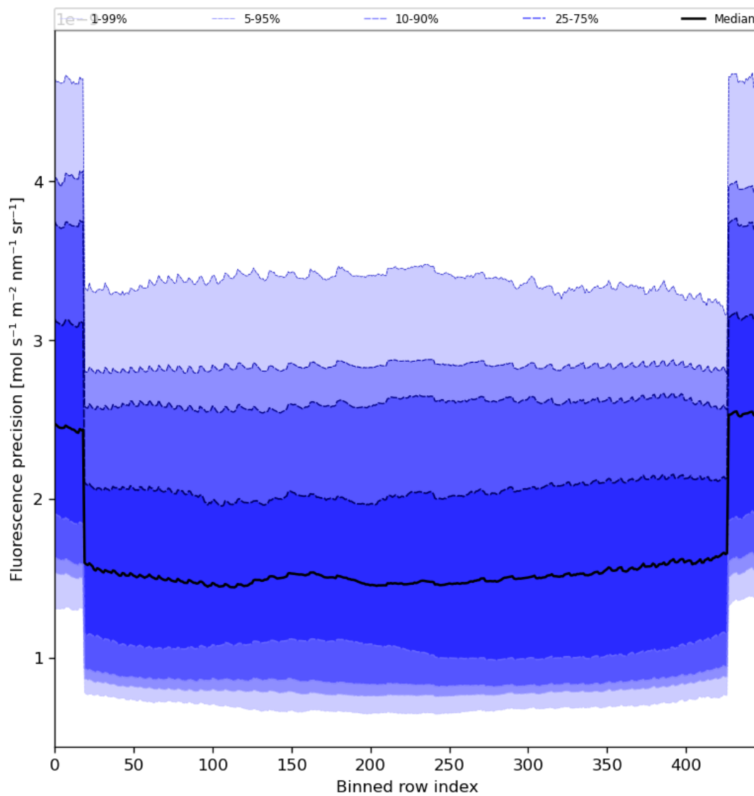
Figure 58: Along track statistics of “Fluorescence precision” for 2023-08-10 to 2023-08-12
