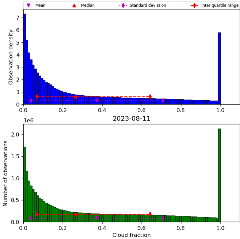
Figure 32: Histogram of “Cloud fraction” for 2023-08-10 to 2023-08-12
