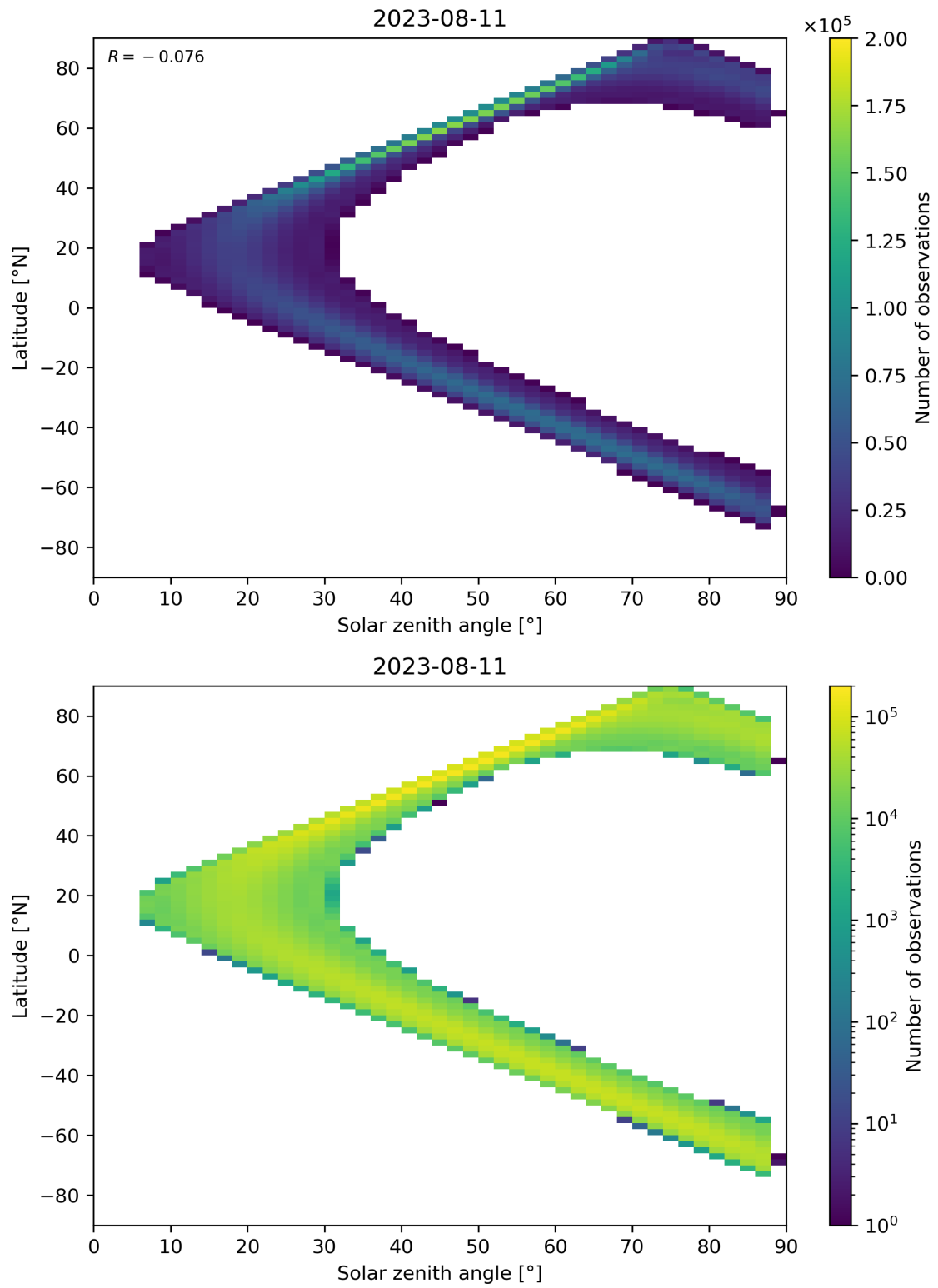
Figure 124: Scatter density plot of “Solar zenith angle” against “Latitude” for 2023-08-10 to 2023-08-12.
