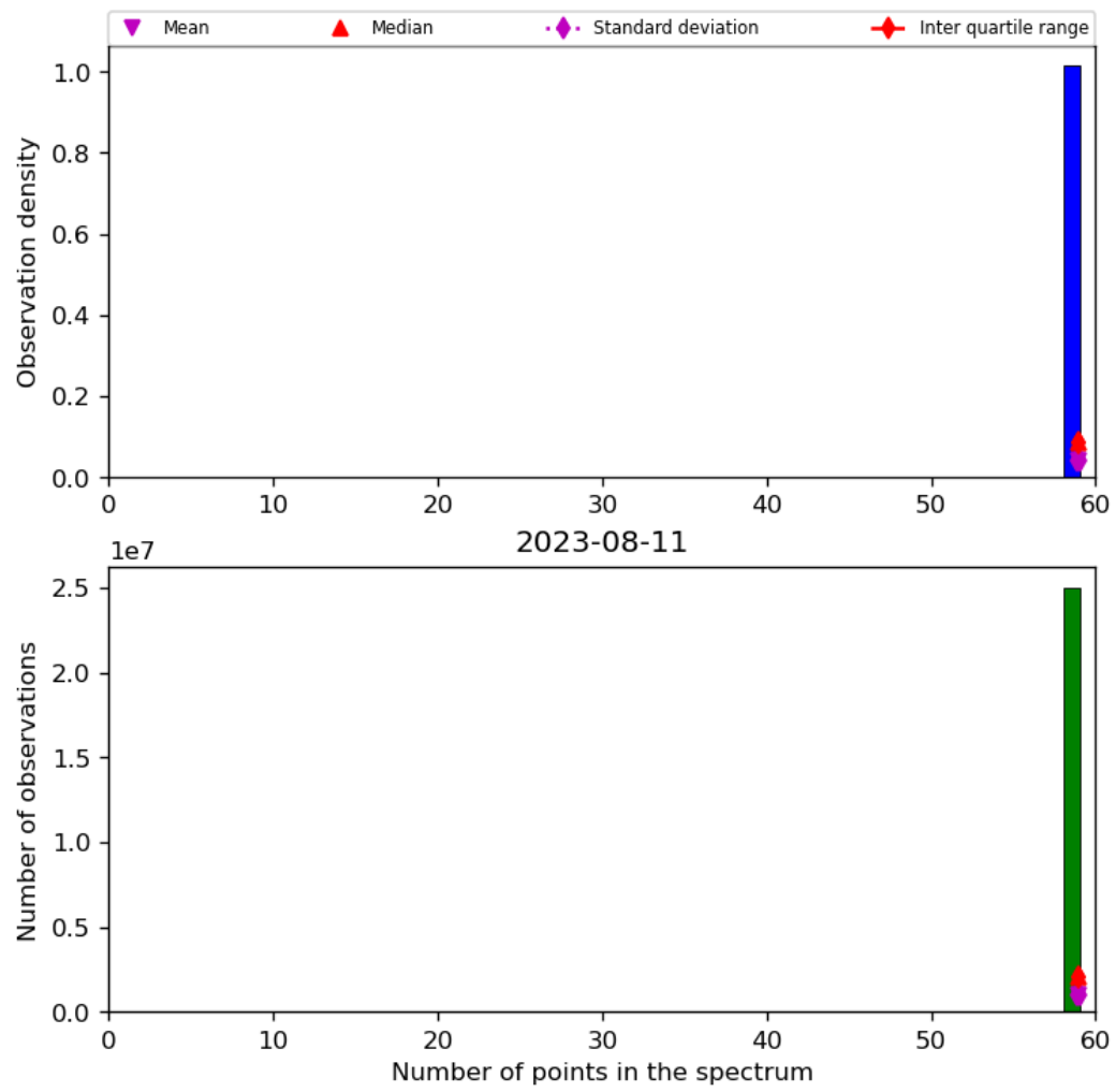
Figure 44: Histogram of “Number of points in the spectrum” for 2023-08-10 to 2023-08-12
