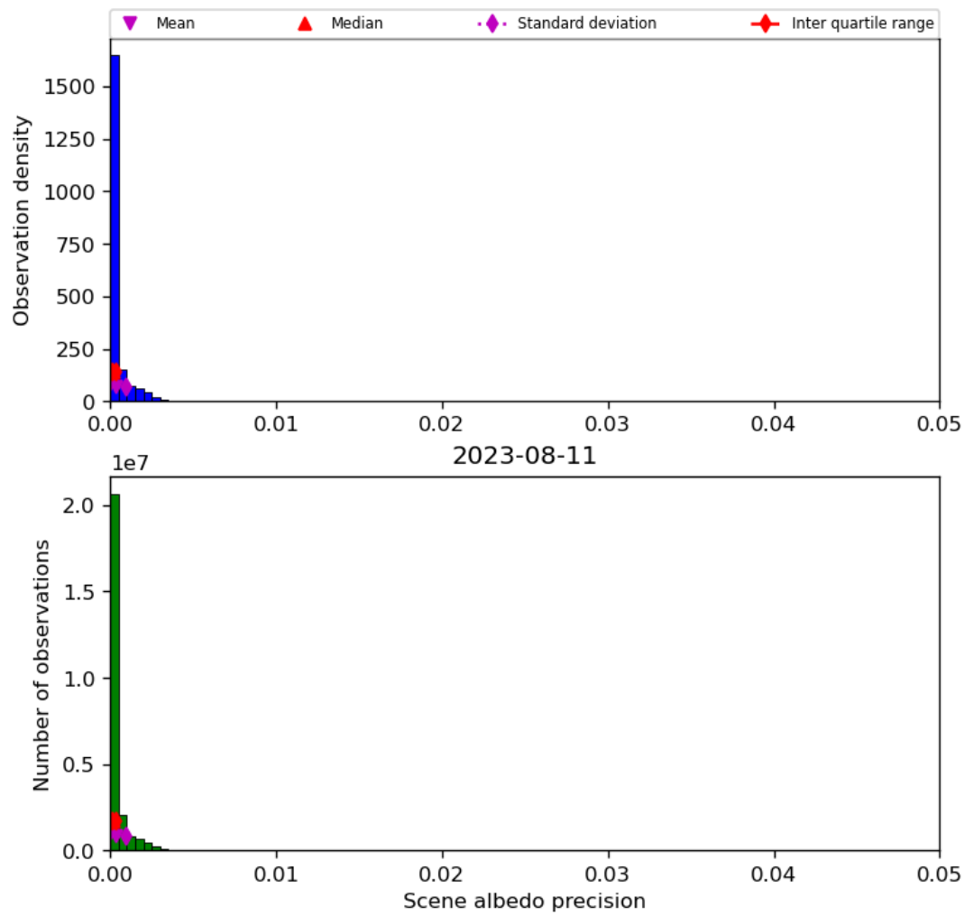
Figure 35: Histogram of “Scene albedo precision” for 2023-08-10 to 2023-08-12
