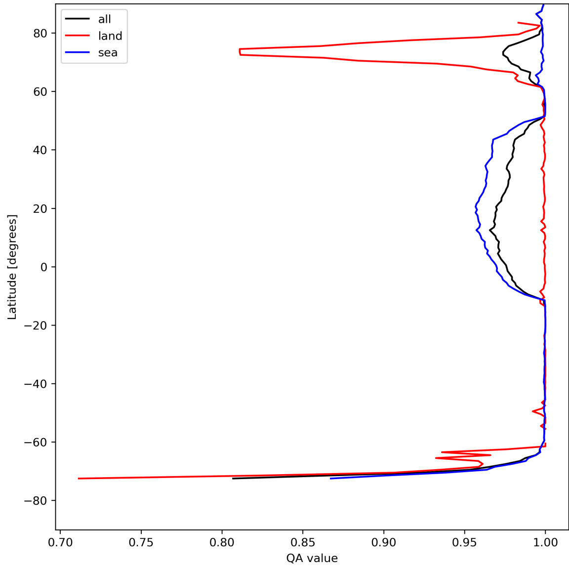
Figure 12: Zonal average of "QA value" for 2023-08-10 to 2023-08-12.
