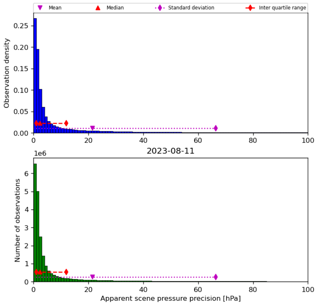
Figure 37: Histogram of “Apparent scene pressure precision” for 2023-08-10 to 2023-08-12
