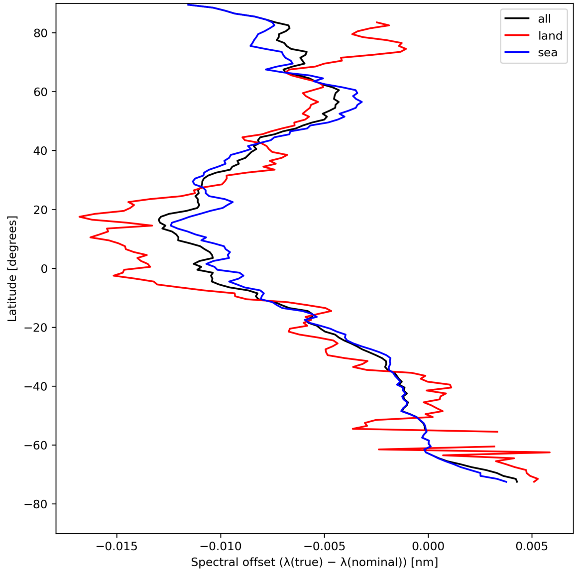
Figure 28: Zonal average of “Spectral offset ( \lambda(\text{true}) - \lambda(\text{nominal}) )” for 2023-08-10 to 2023-08-12.
