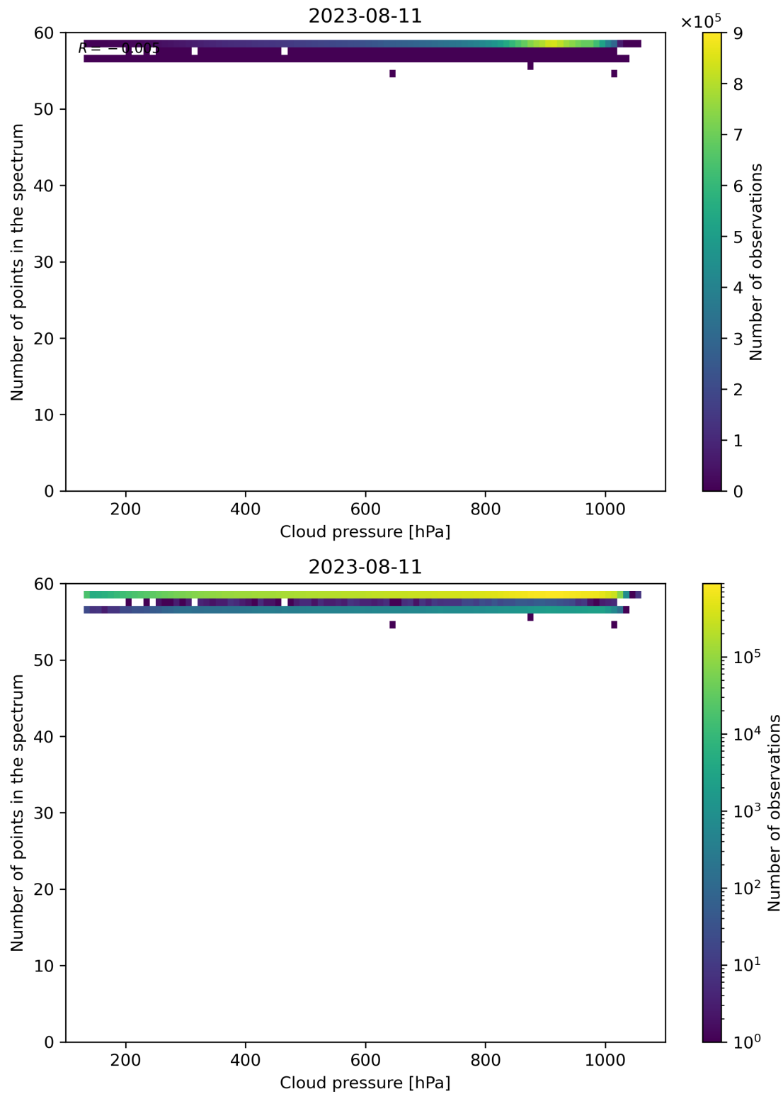
Figure 90: Scatter density plot of “Cloud pressure” against “Number of points in the spectrum” for 2023-08-10 to 2023-08-12.
