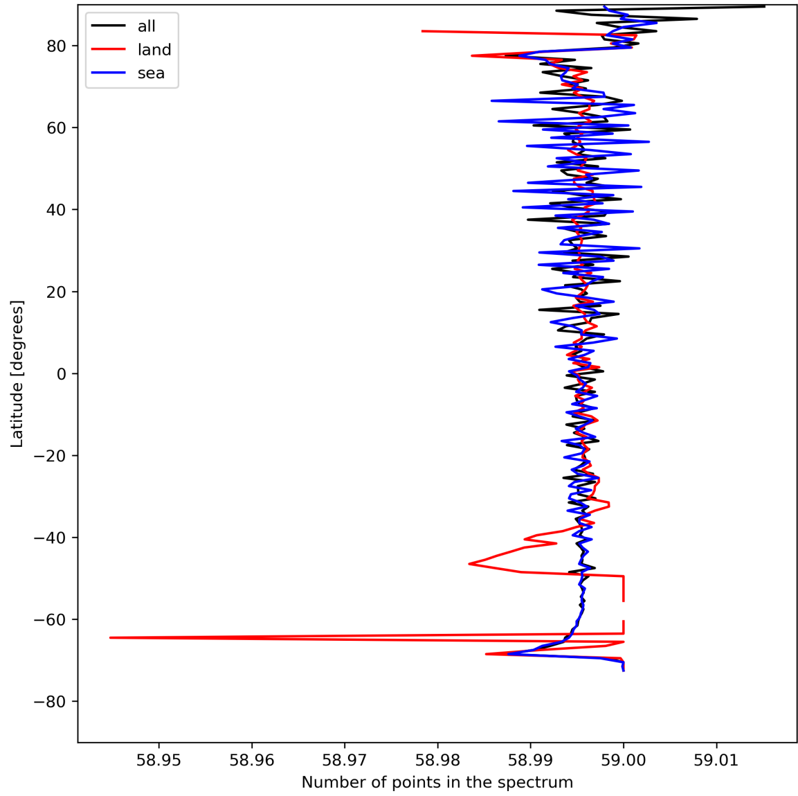
Figure 27: Zonal average of “Number of points in the spectrum” for 2023-08-10 to 2023-08-12.
