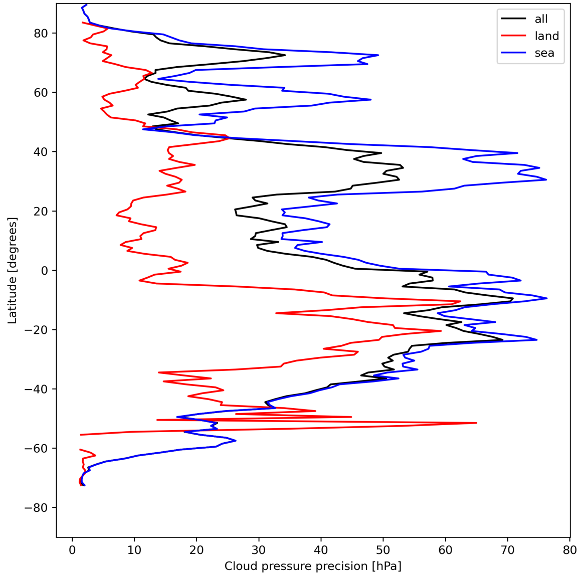
Figure 14: Zonal average of “Cloud pressure precision” for 2023-08-10 to 2023-08-12.
