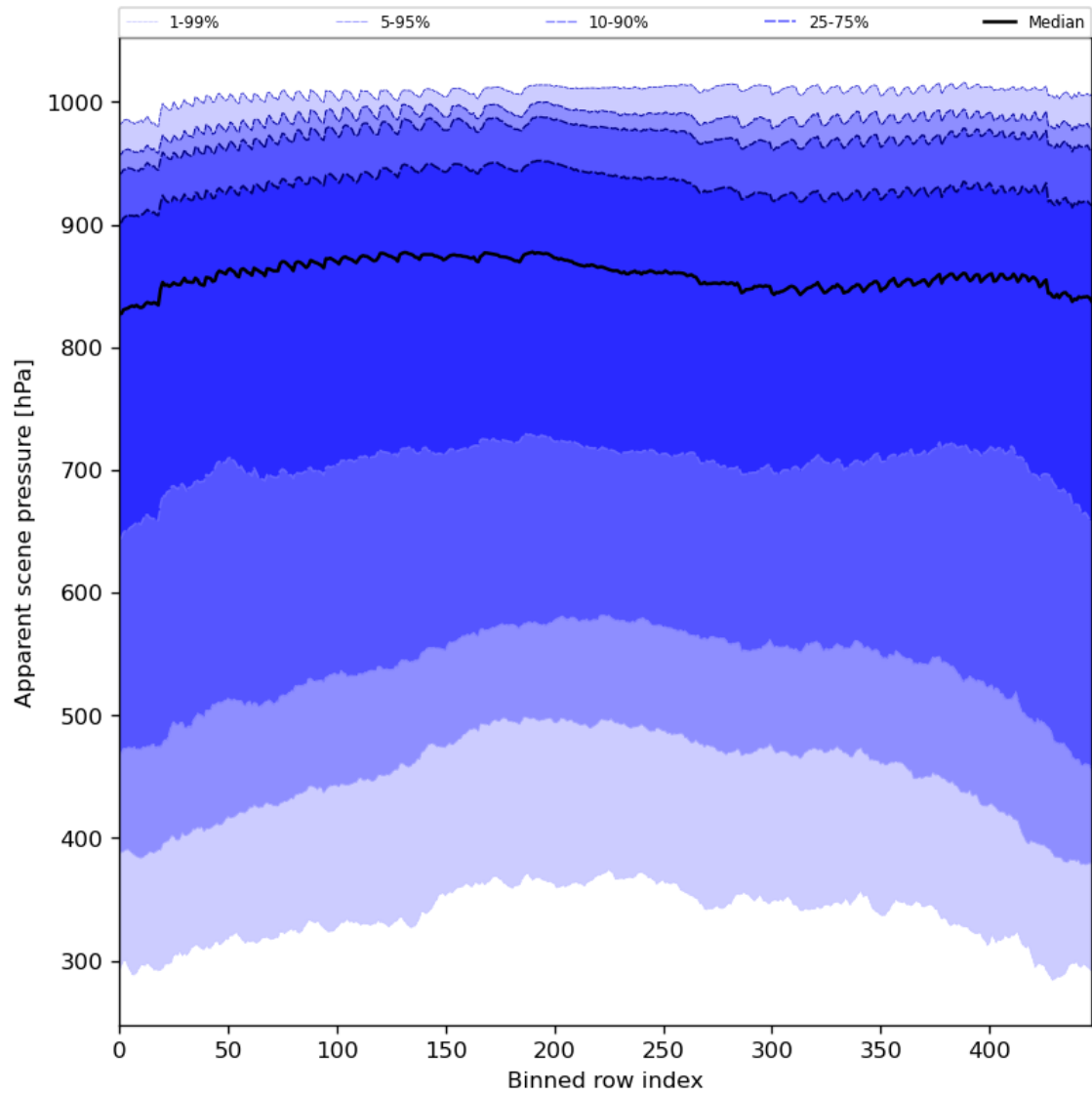
Figure 53: Along track statistics of “Apparent scene pressure” for 2023-08-10 to 2023-08-12
