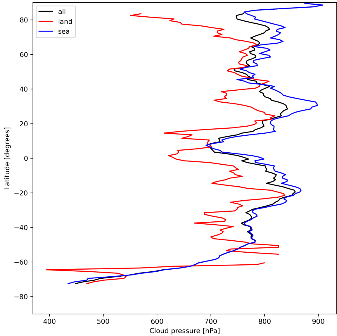
Figure 13: Zonal average of “Cloud pressure” for 2023-08-10 to 2023-08-12.
