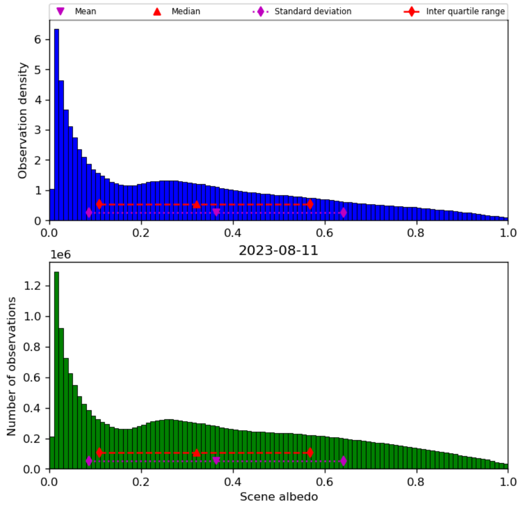
Figure 34: Histogram of “Scene albedo” for 2023-08-10 to 2023-08-12
