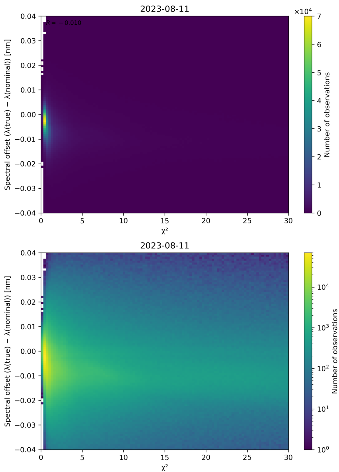
Figure 75: Scatter density plot of " \chi^2 " against "Spectral offset ( \lambda(\text{true}) - \lambda(\text{nominal}) )" for 2023-08-10 to 2023-08-12.
