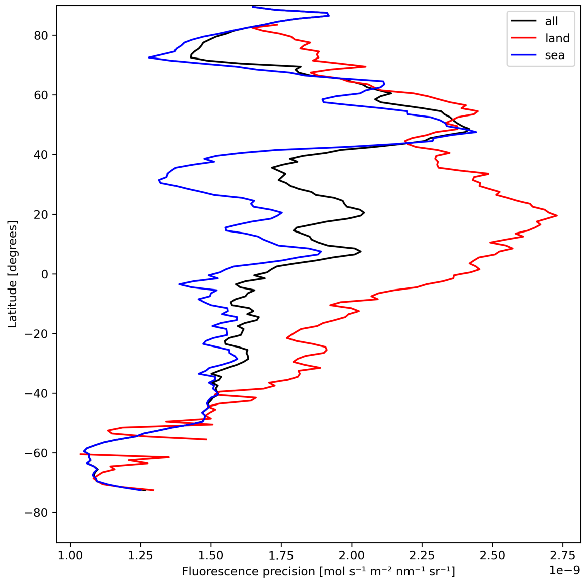
Figure 24: Zonal average of “Fluorescence precision” for 2023-08-10 to 2023-08-12.
