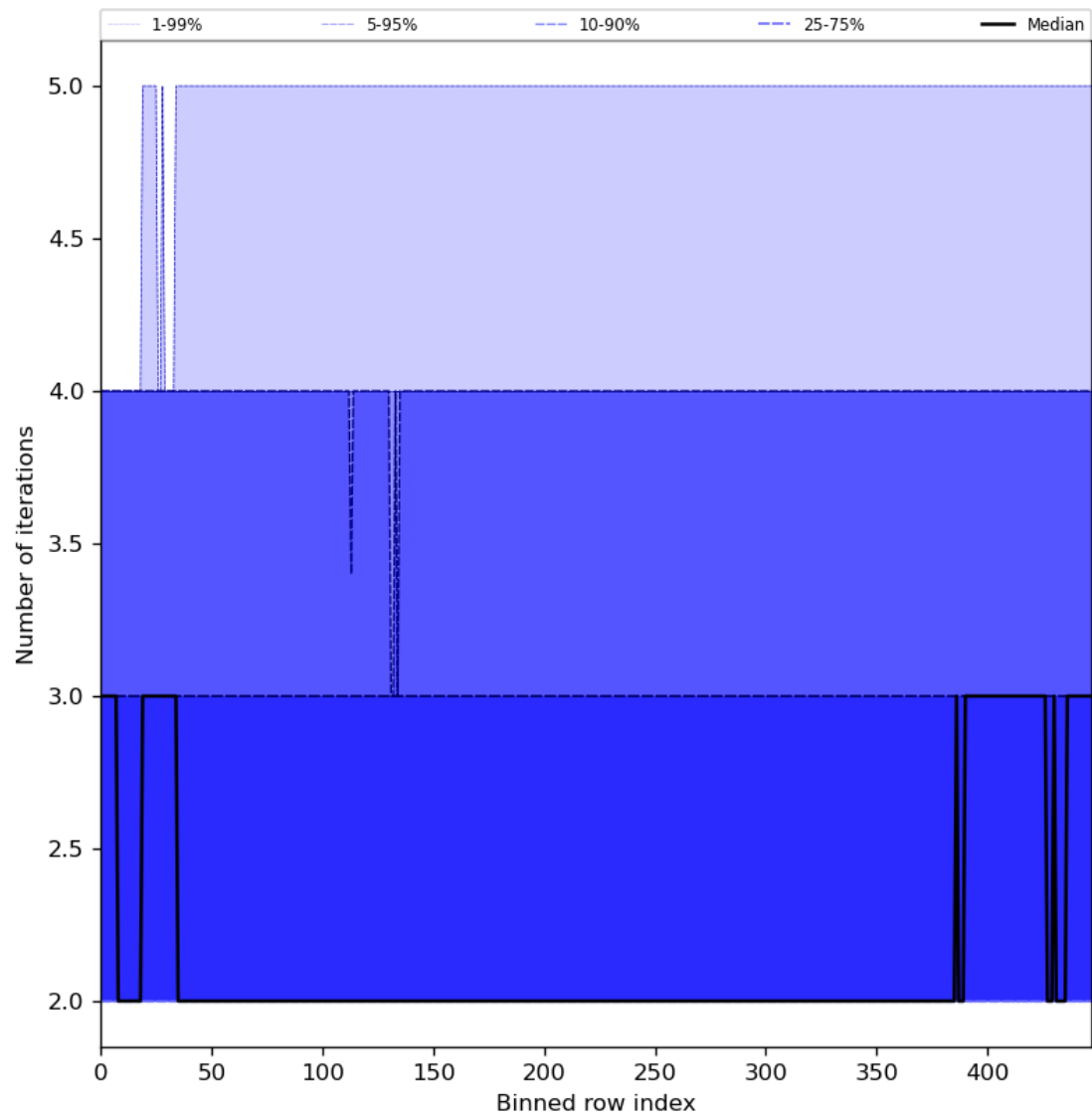
Figure 56: Along track statistics of "Number of iterations" for 2023-08-10 to 2023-08-12
