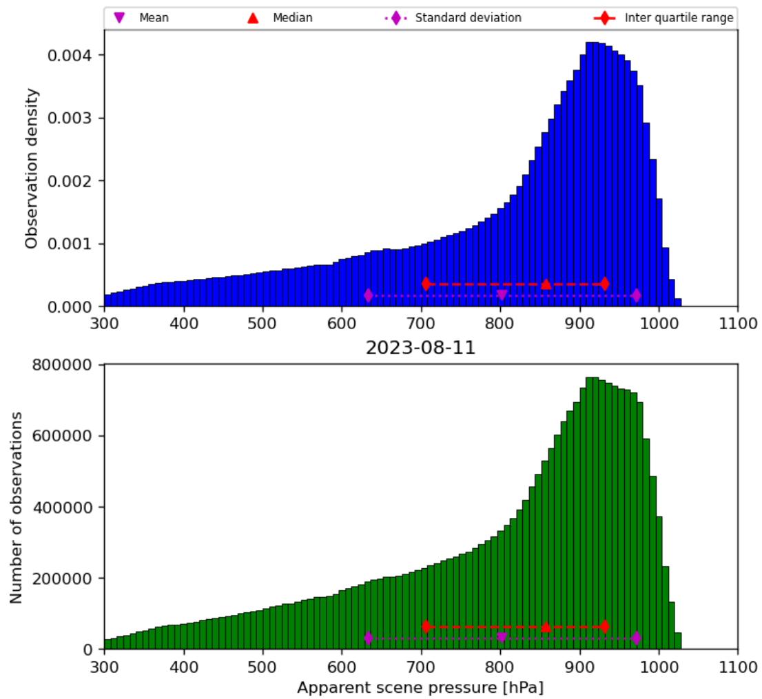
Figure 36: Histogram of “Apparent scene pressure” for 2023-08-10 to 2023-08-12
