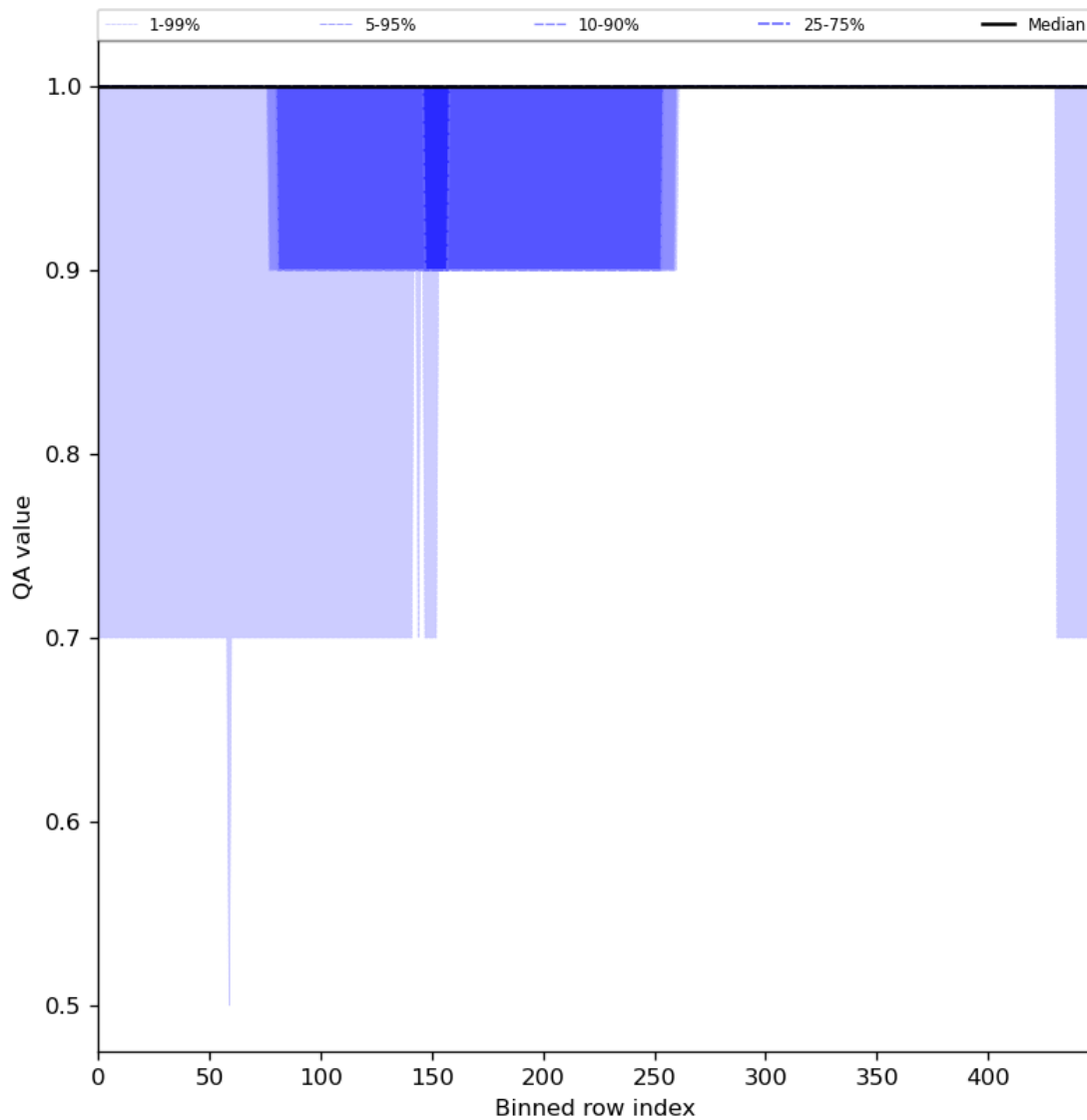
Figure 46: Along track statistics of “QA value” for 2023-08-10 to 2023-08-12
