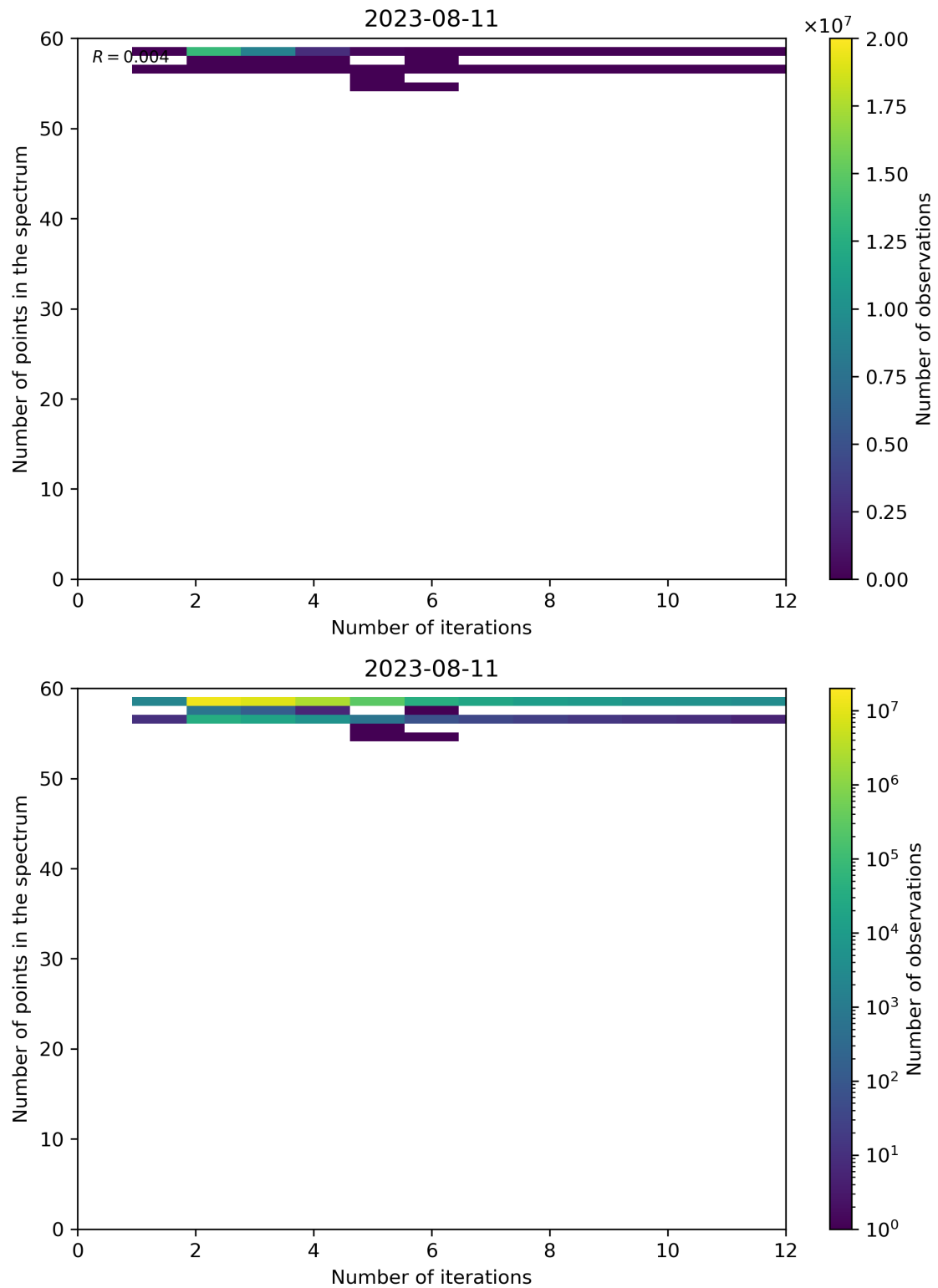
Figure 108: Scatter density plot of “Number of iterations” against “Number of points in the spectrum” for 2023-08-10 to 2023-08-12.
