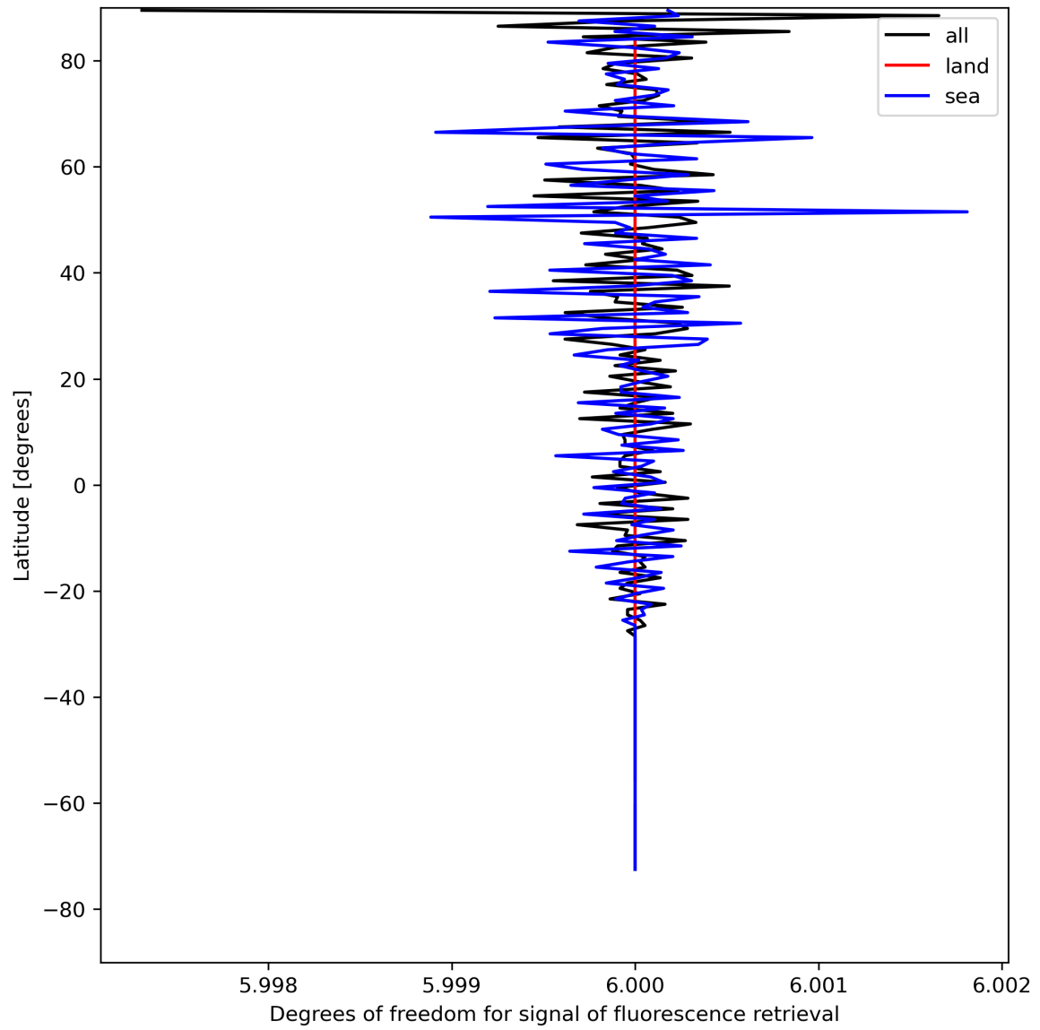
Figure 26: Zonal average of “Degrees of freedom for signal of fluorescence retrieval” for 2023-08-10 to 2023-08-12.
