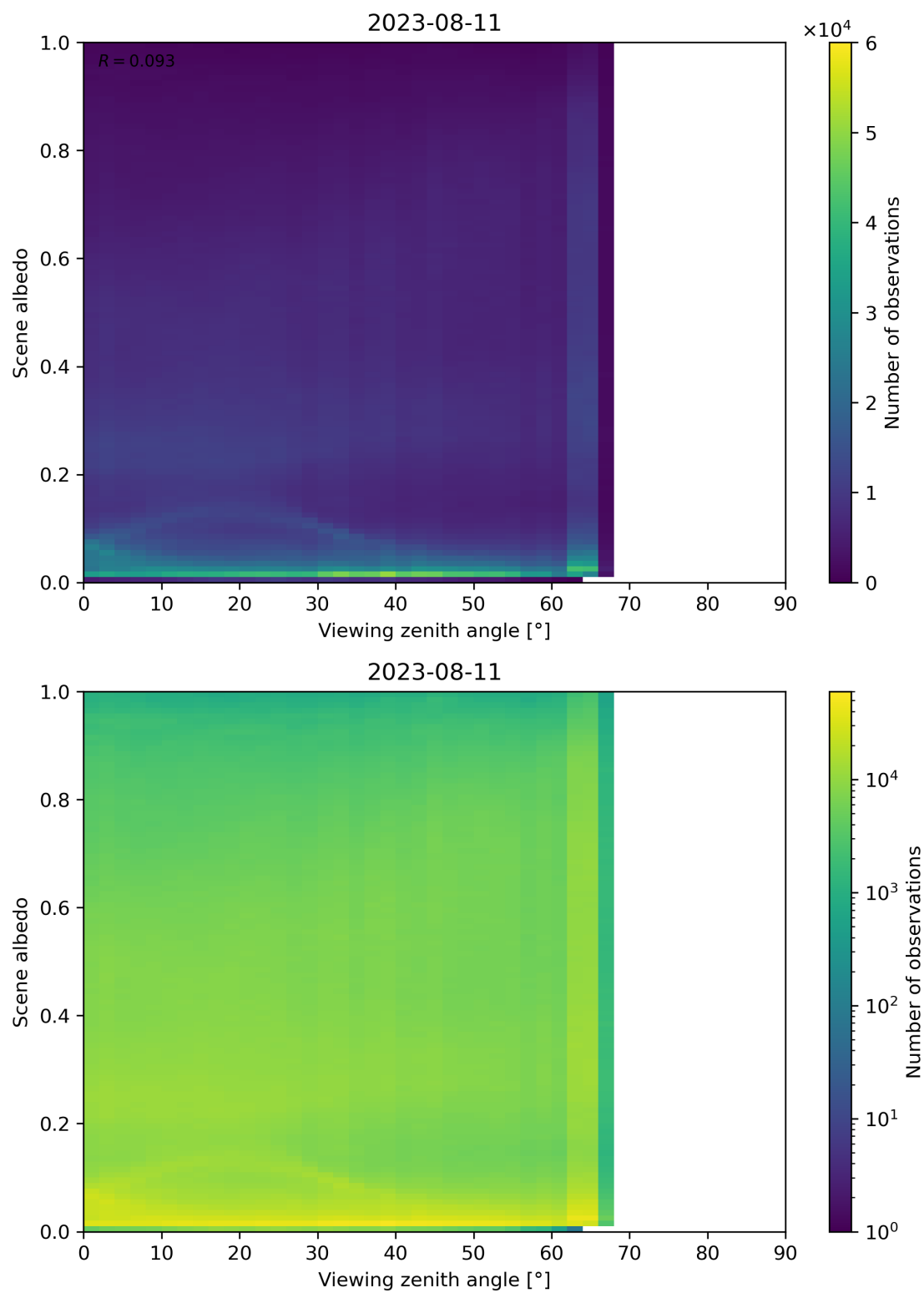
Figure 138: Scatter density plot of “Viewing zenith angle” against “Scene albedo” for 2023-08-10 to 2023-08-12.
