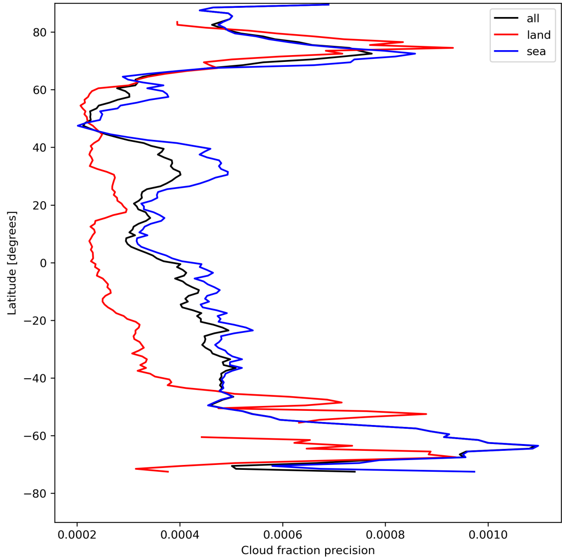
Figure 16: Zonal average of “Cloud fraction precision” for 2023-08-10 to 2023-08-12.
