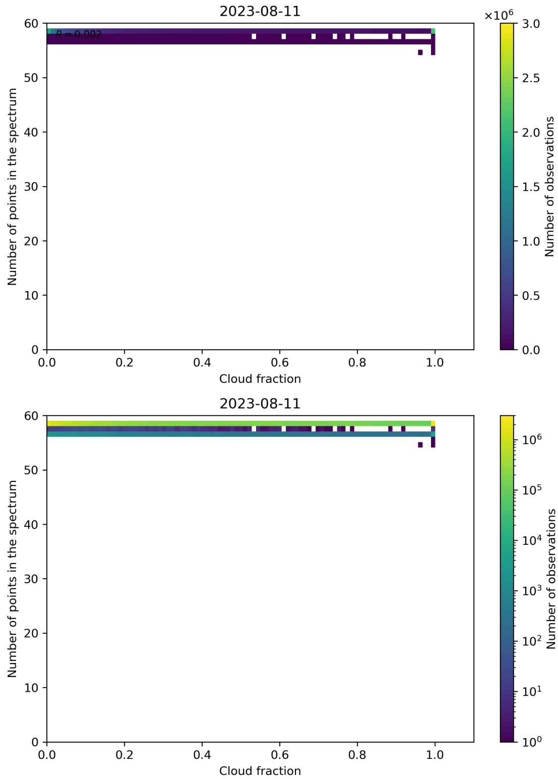
Figure 81: Scatter density plot of “Cloud fraction” against “Number of points in the spectrum” for 2023-08-10 to 2023-08-12.
