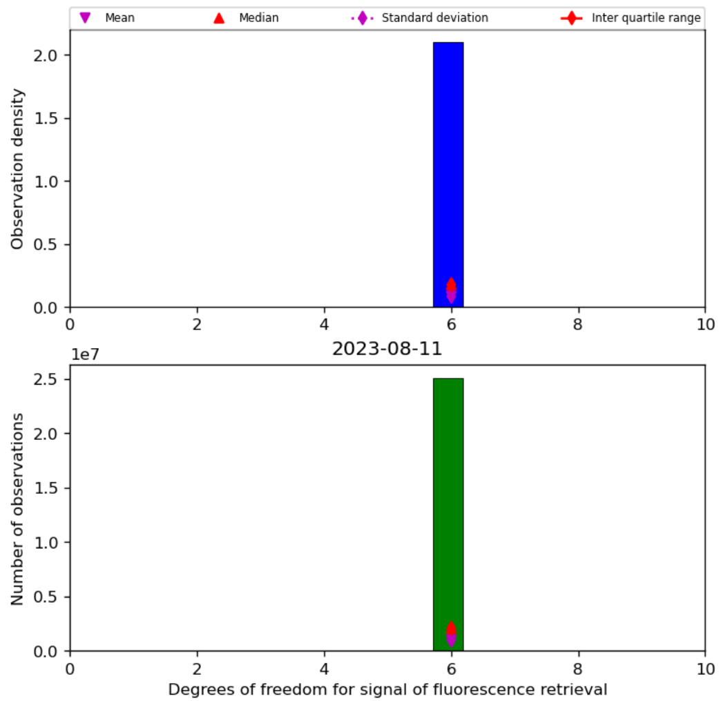
Figure 43: Histogram of “Degrees of freedom for signal of fluorescence retrieval” for 2023-08-10 to 2023-08-12
