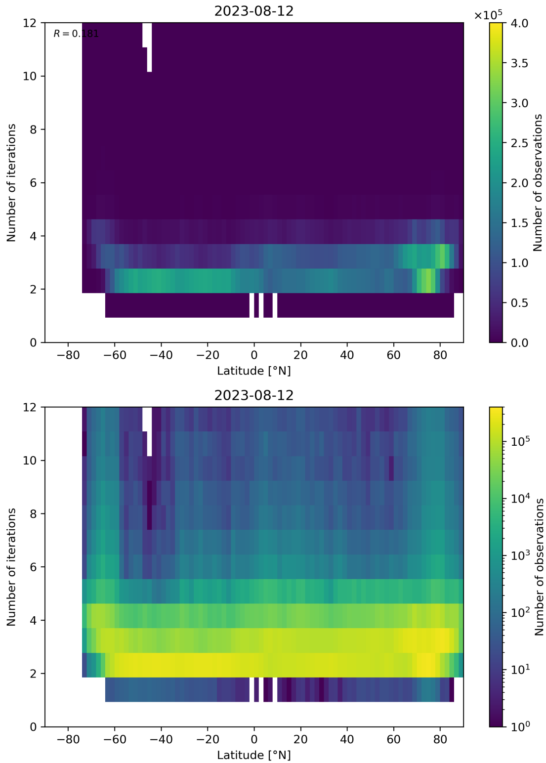
Figure 102: Scatter density plot of “Latitude” against “Number of iterations” for 2023-08-11 to 2023-08-13.
