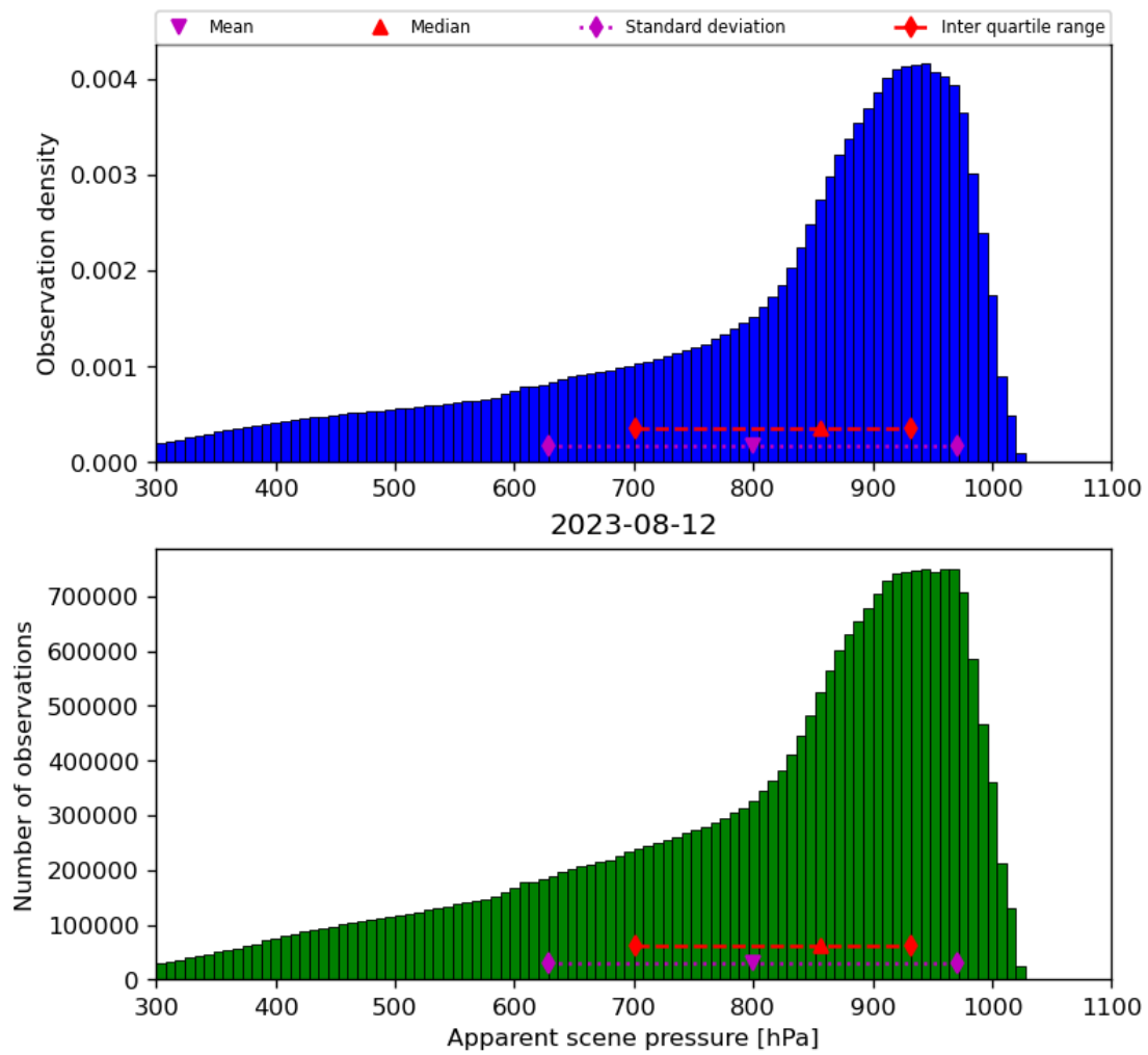
Figure 36: Histogram of “Apparent scene pressure” for 2023-08-11 to 2023-08-13
