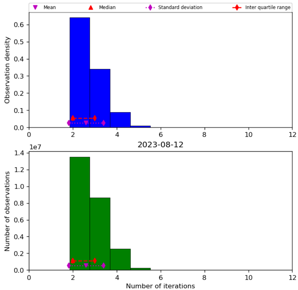
Figure 39: Histogram of “Number of iterations” for 2023-08-11 to 2023-08-13
