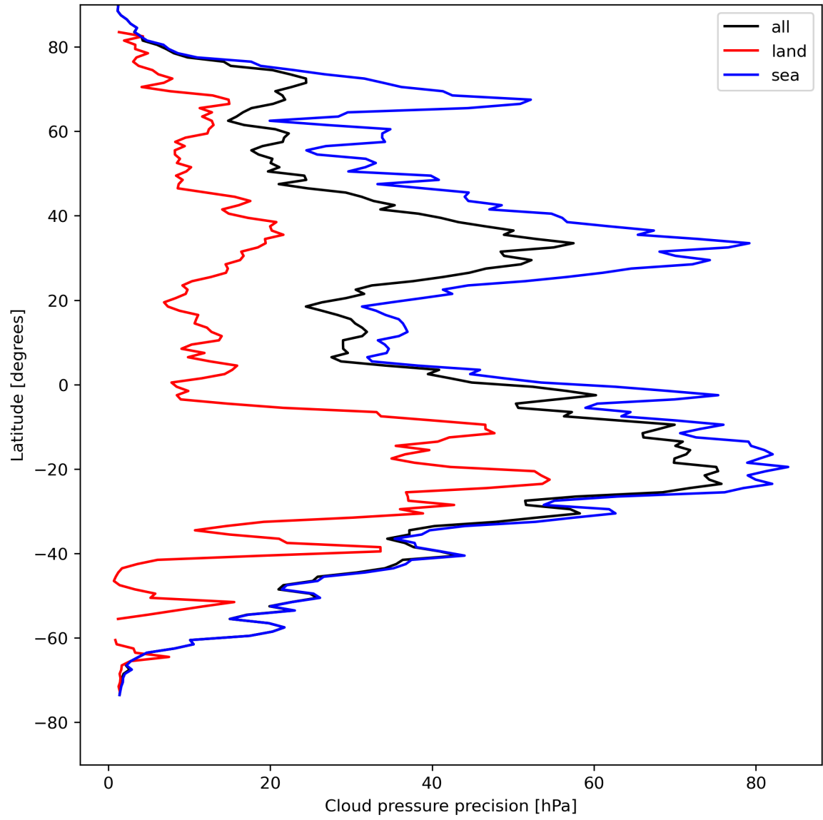
Figure 14: Zonal average of “Cloud pressure precision” for 2023-08-11 to 2023-08-13.
