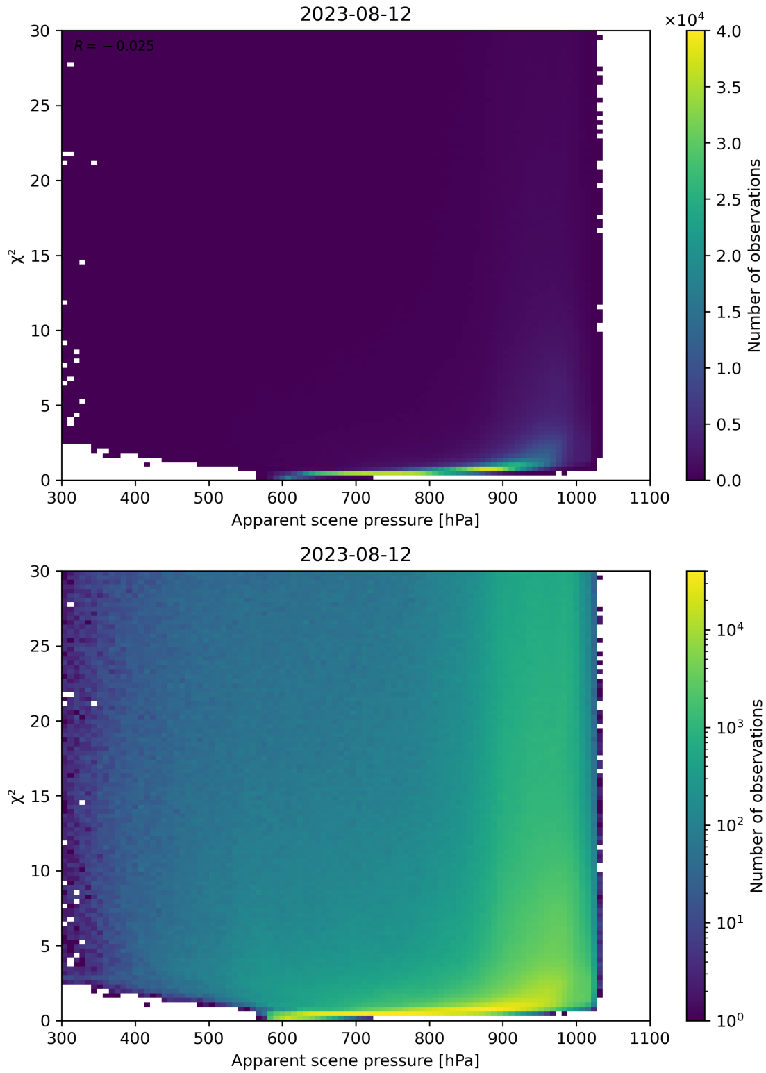
Figure 63: Scatter density plot of “Apparent scene pressure” against “ \chi^2 ” for 2023-08-11 to 2023-08-13.
