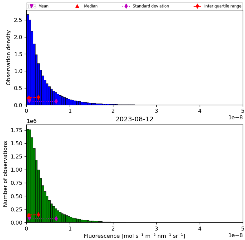
Figure 40: Histogram of “Fluorescence” for 2023-08-11 to 2023-08-13
