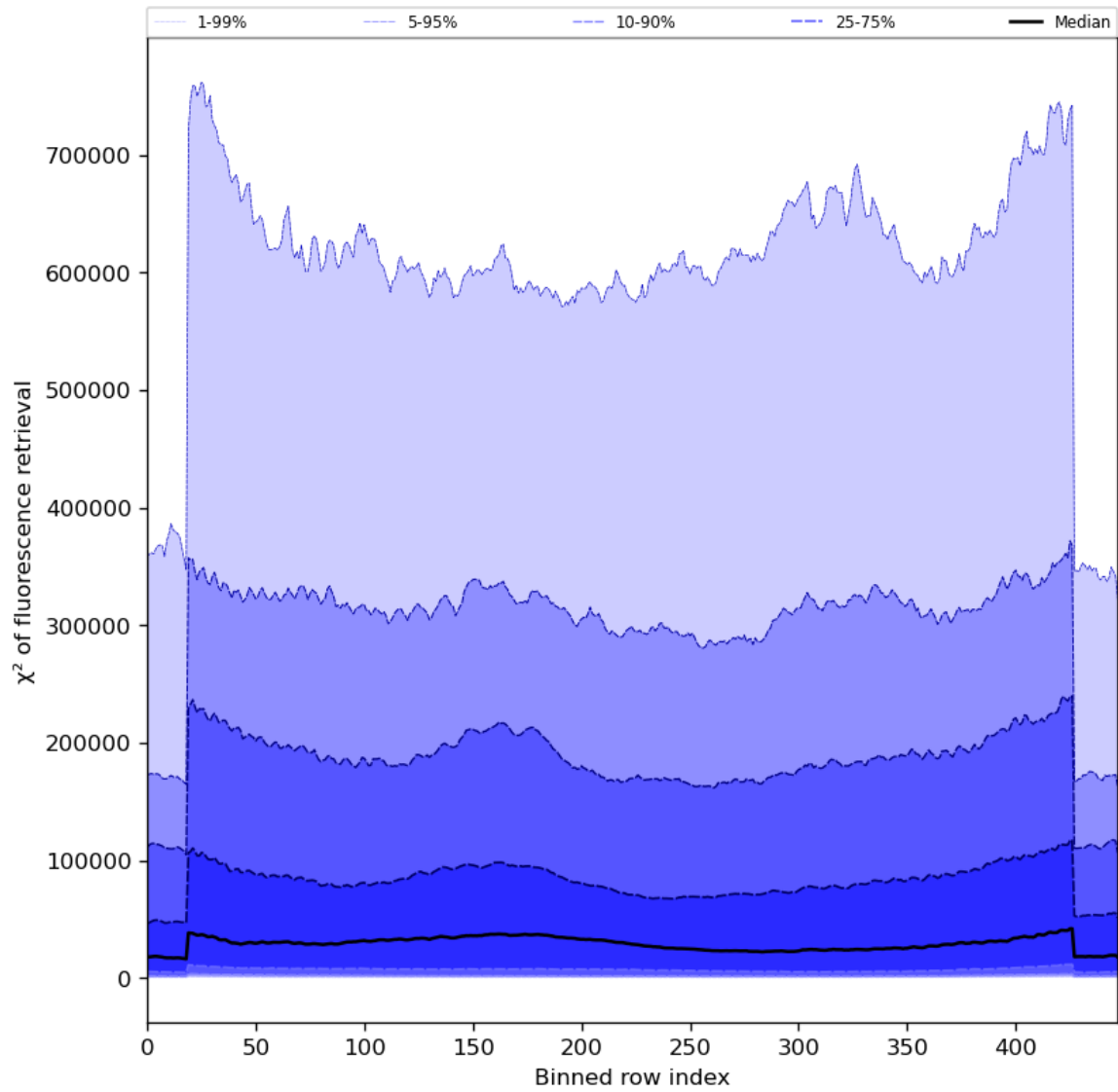
Figure 59: Along track statistics of “ \chi^2 of fluorescence retrieval” for 2023-08-11 to 2023-08-13
