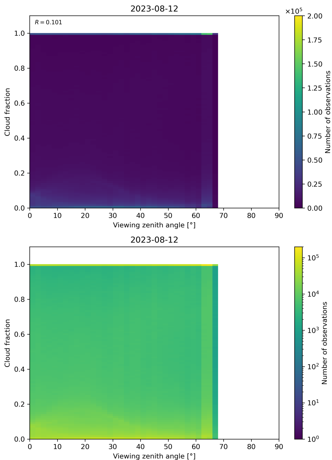
Figure 132: Scatter density plot of “Viewing zenith angle” against “Cloud fraction” for 2023-08-11 to 2023-08-13.
