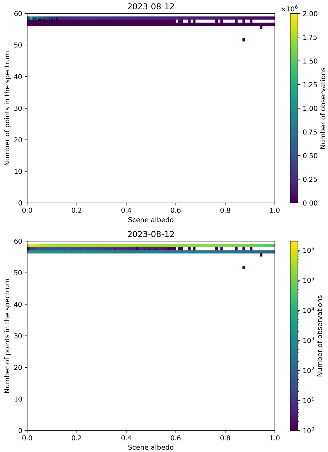
Figure 116: Scatter density plot of “Scene albedo” against “Number of points in the spectrum” for 2023-08-11 to 2023-08-13.
