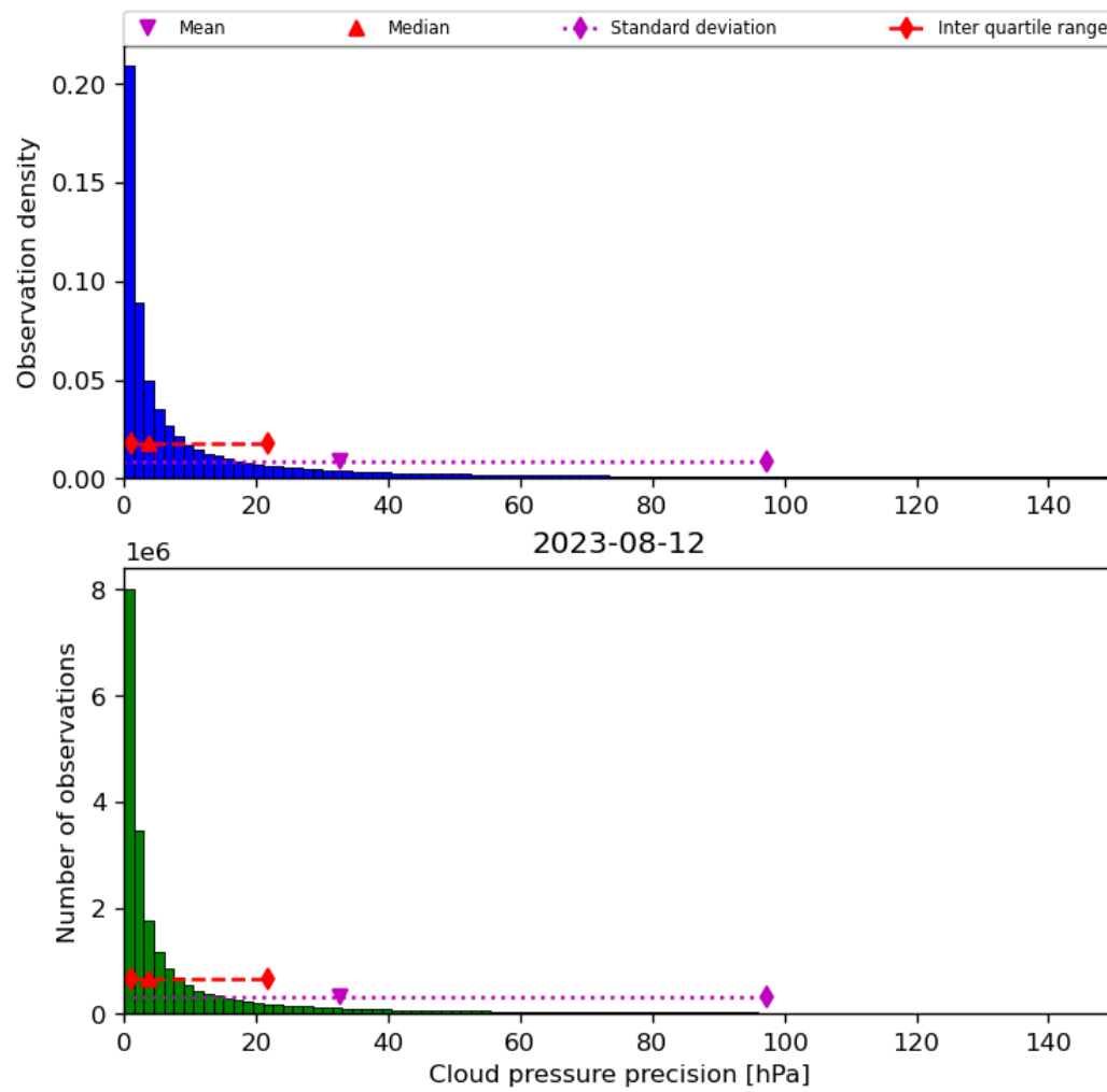
Figure 31: Histogram of “Cloud pressure precision” for 2023-08-11 to 2023-08-13
