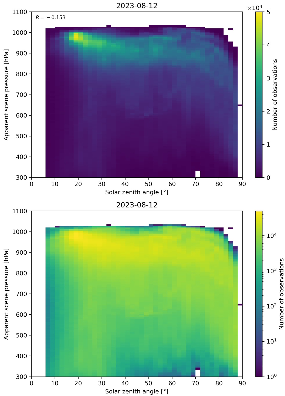
Figure 118: Scatter density plot of “Solar zenith angle” against “Apparent scene pressure” for 2023-08-11 to 2023-08-13.
