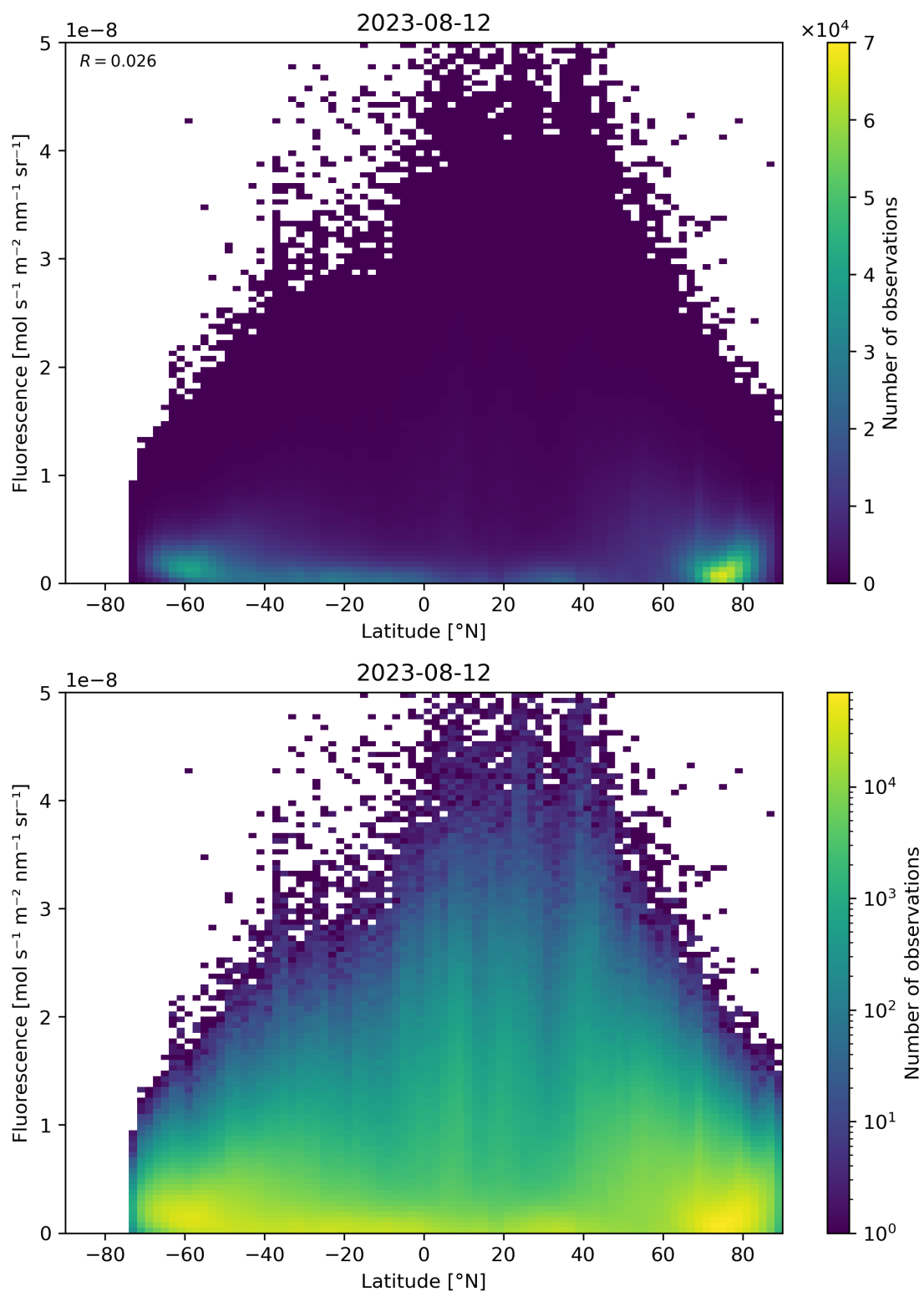
Figure 101: Scatter density plot of “Latitude” against “Fluorescence” for 2023-08-11 to 2023-08-13.
