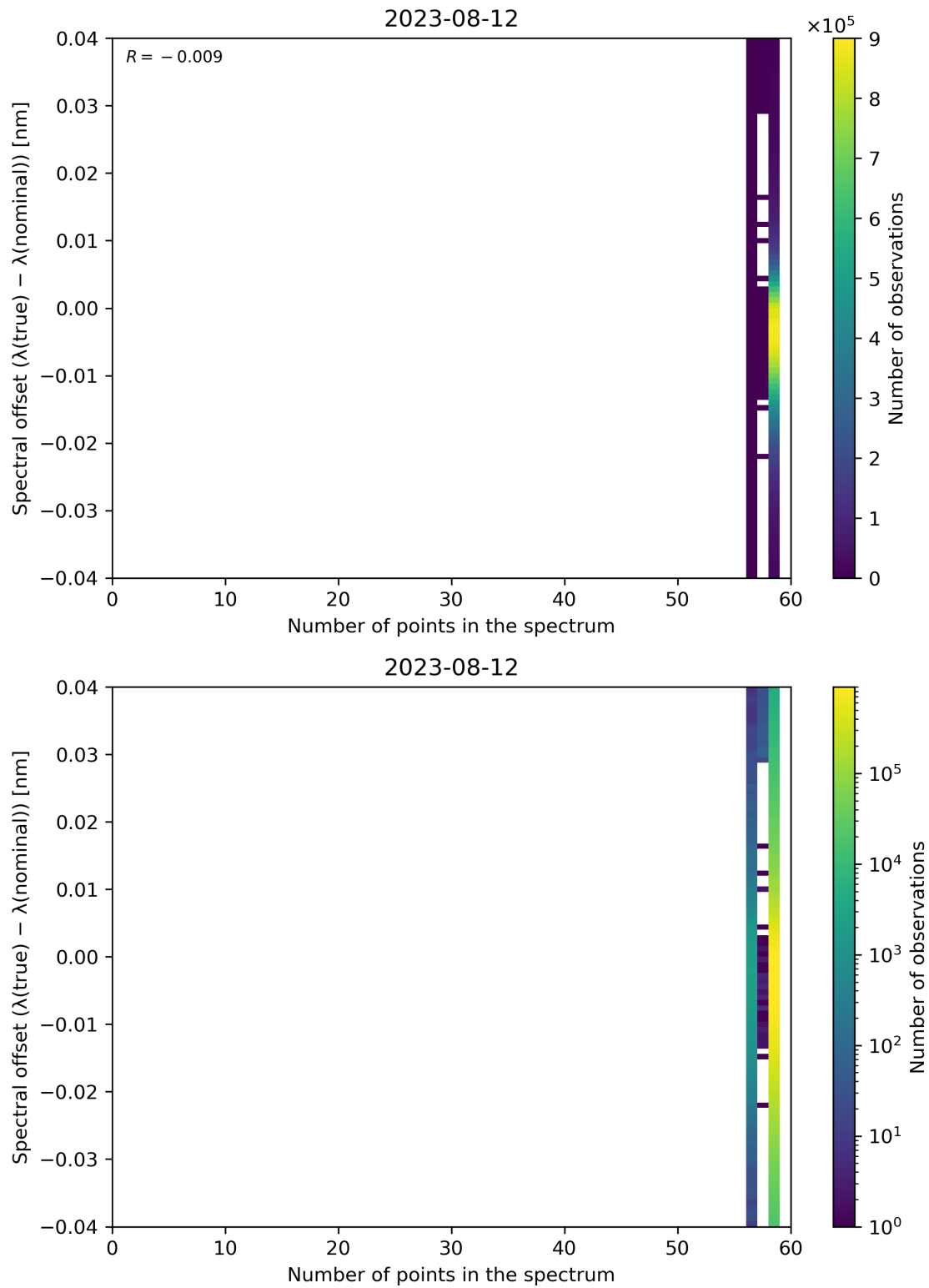
Figure 110: Scatter density plot of “Number of points in the spectrum” against “Spectral offset ( \lambda(\text{true}) - \lambda(\text{nominal}) )” for 2023-08-11 to 2023-08-13.
