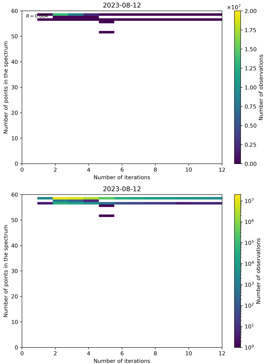
Figure 108: Scatter density plot of “Number of iterations” against “Number of points in the spectrum” for 2023-08-11 to 2023-08-13.
