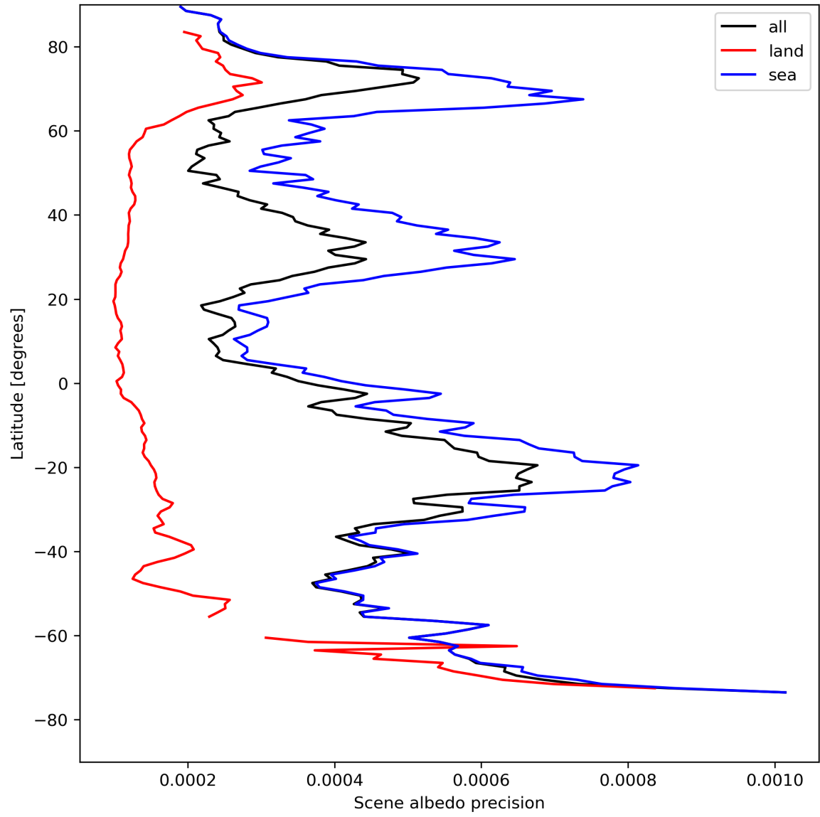
Figure 18: Zonal average of “Scene albedo precision” for 2023-08-11 to 2023-08-13.
