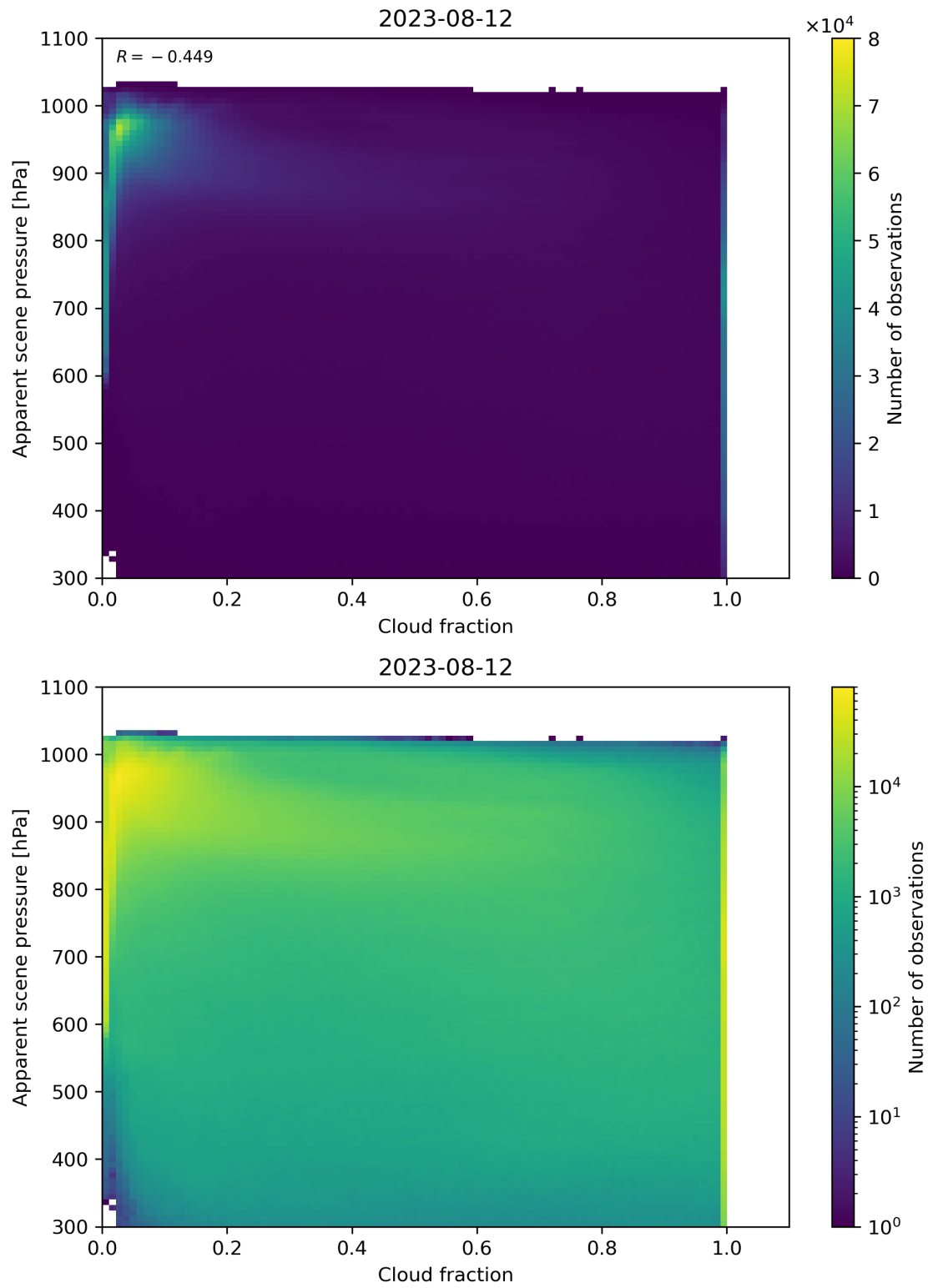
Figure 76: Scatter density plot of “Cloud fraction” against “Apparent scene pressure” for 2023-08-11 to 2023-08-13.
