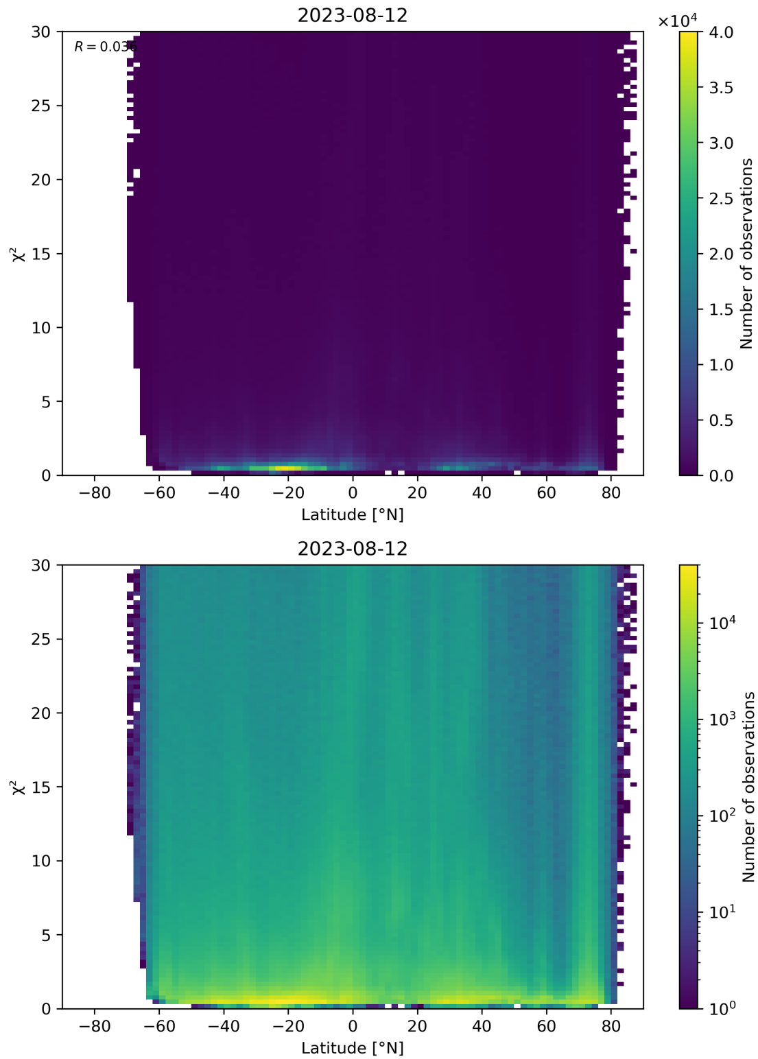
Figure 97: Scatter density plot of “Latitude” against “ \chi^2 ” for 2023-08-11 to 2023-08-13.
