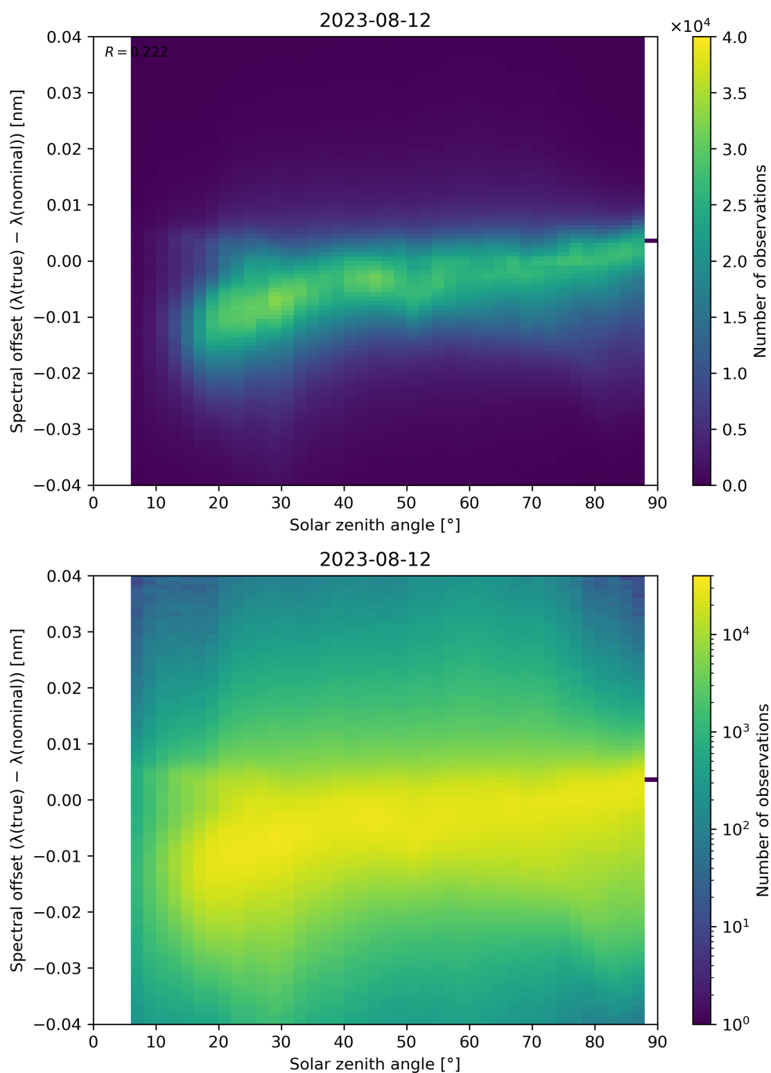
Figure 128: Scatter density plot of “Solar zenith angle” against “Spectral offset ( \lambda(\text{true}) - \lambda(\text{nominal}) )” for 2023-08-11 to 2023-08-13.
