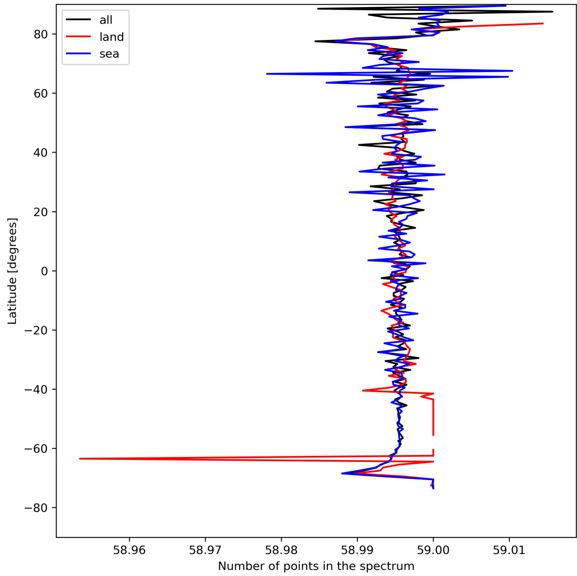
Figure 27: Zonal average of “Number of points in the spectrum” for 2023-08-11 to 2023-08-13.
