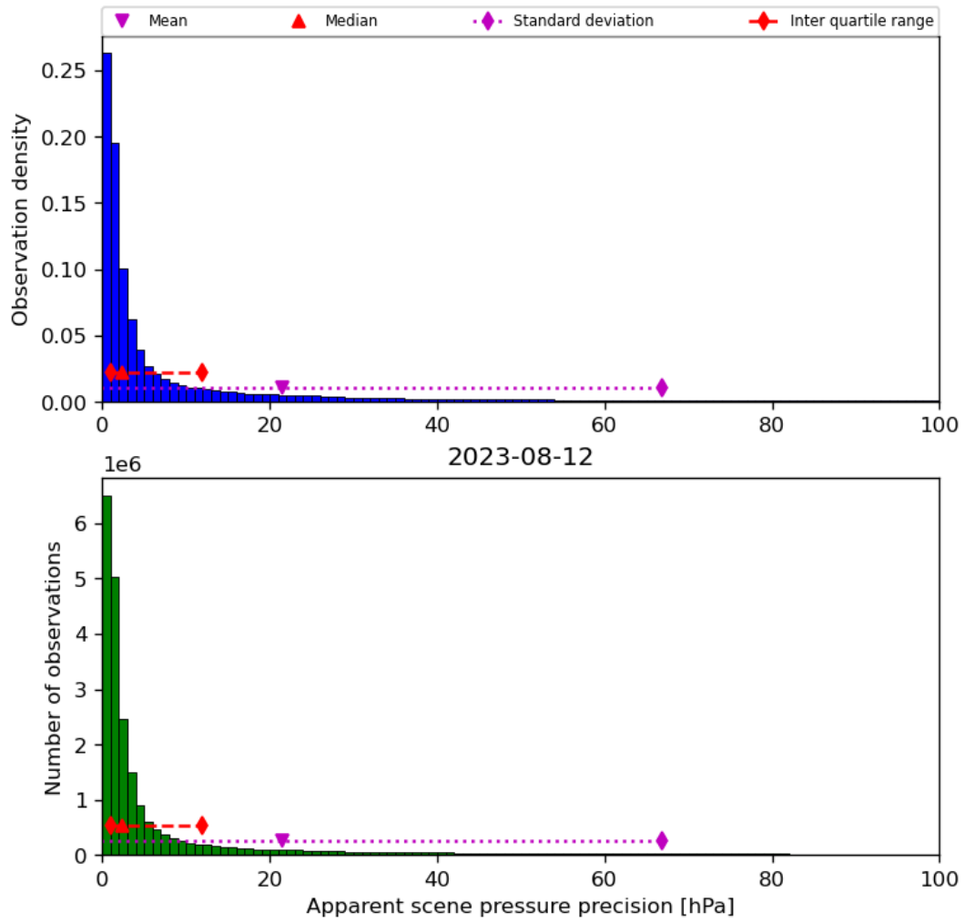
Figure 37: Histogram of “Apparent scene pressure precision” for 2023-08-11 to 2023-08-13
