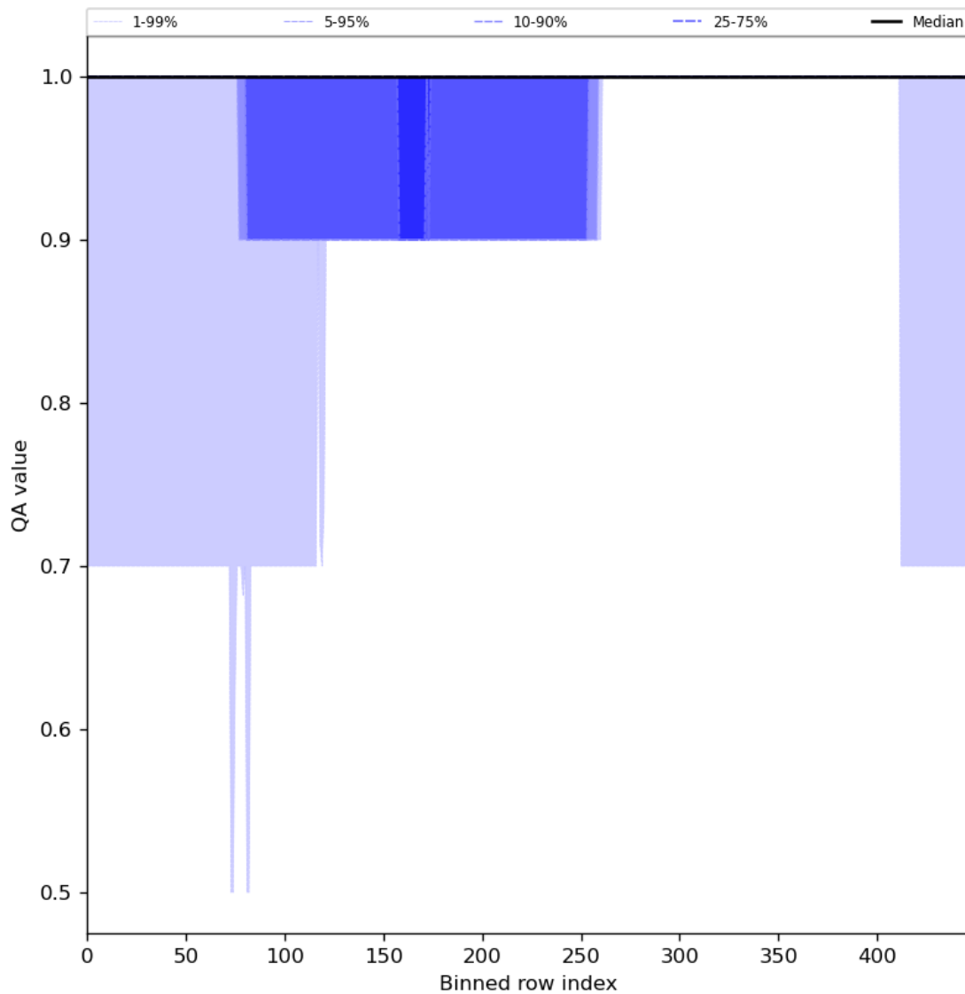
Figure 46: Along track statistics of “QA value” for 2023-08-11 to 2023-08-13
