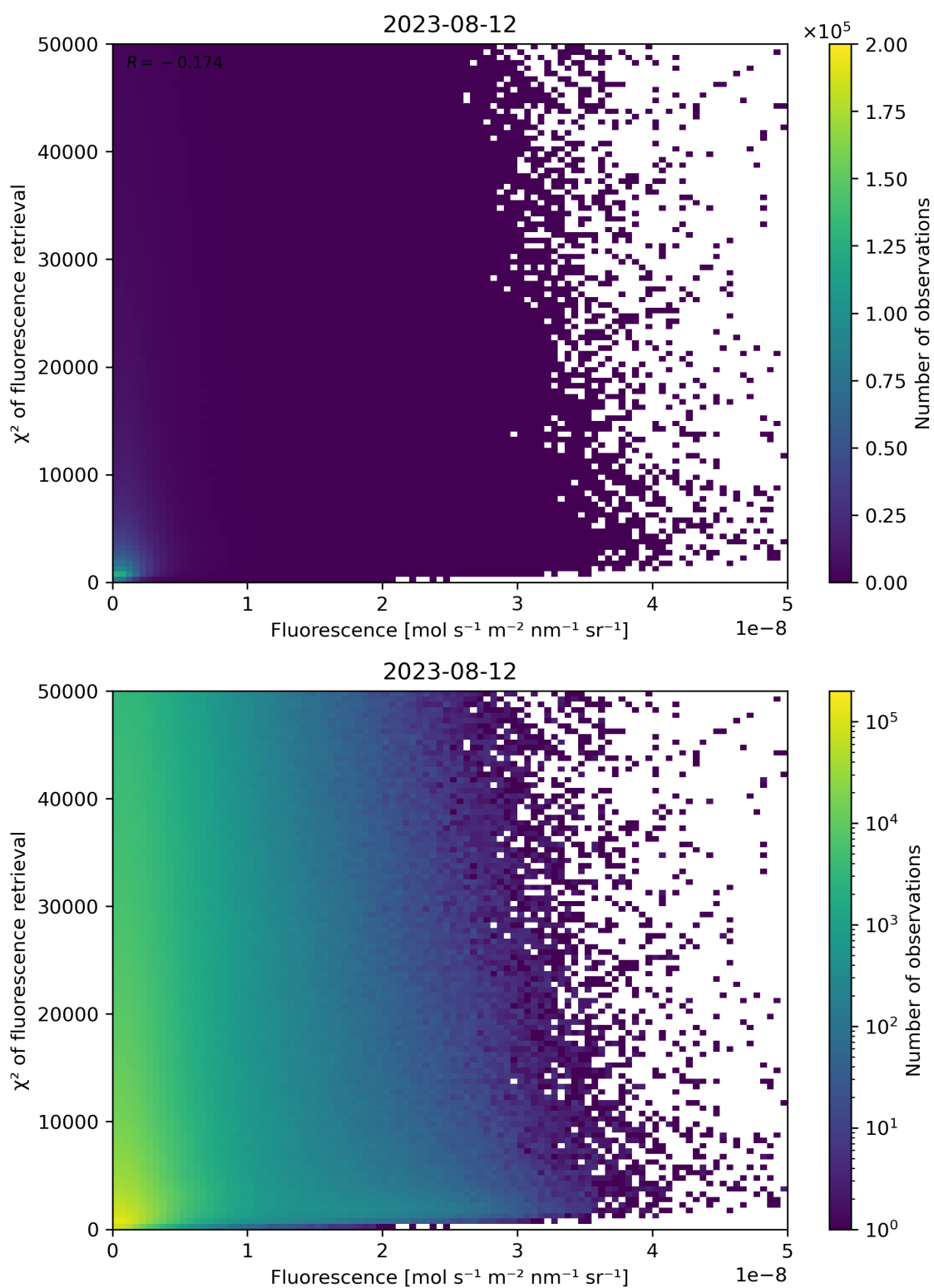
Figure 93: Scatter density plot of “Fluorescence” against “ \chi^2 of fluorescence retrieval” for 2023-08-11 to 2023-08-13.
