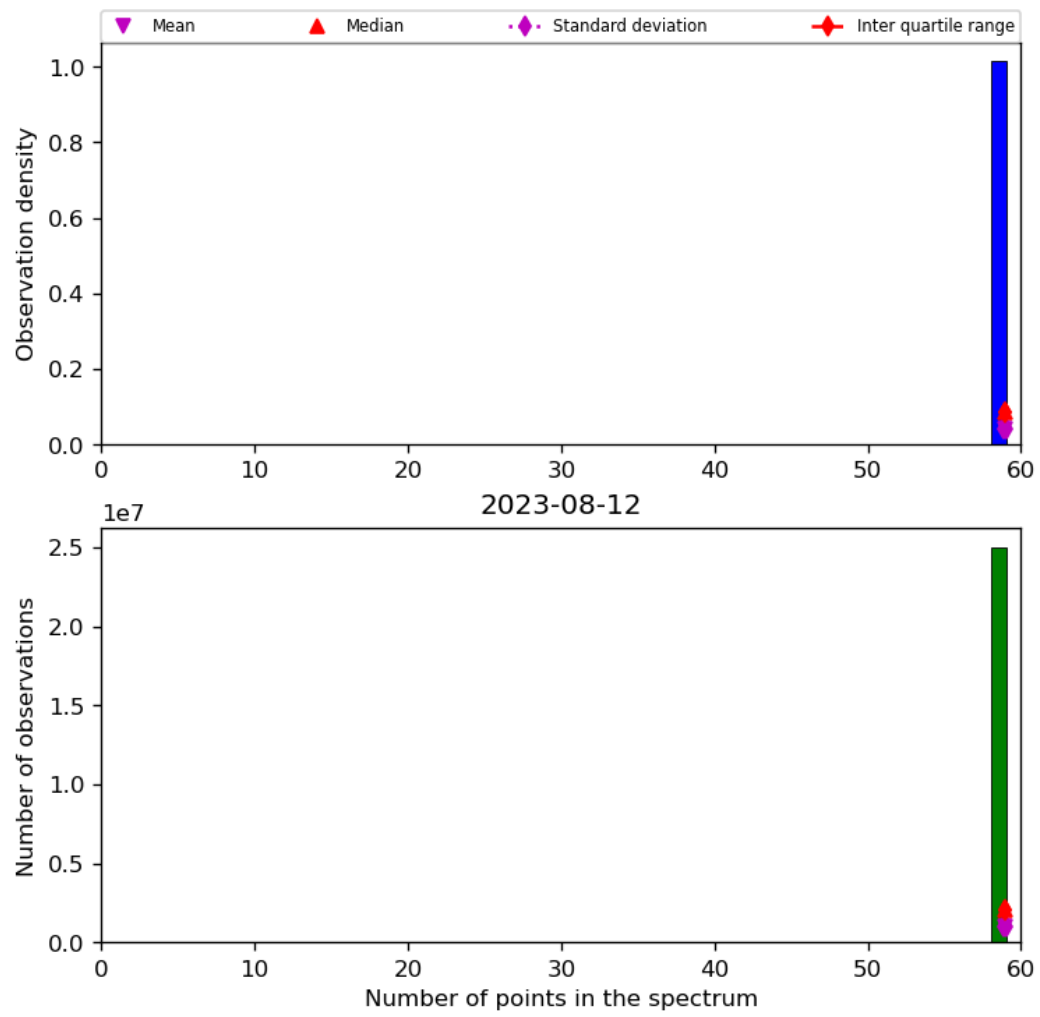
Figure 44: Histogram of “Number of points in the spectrum” for 2023-08-11 to 2023-08-13
