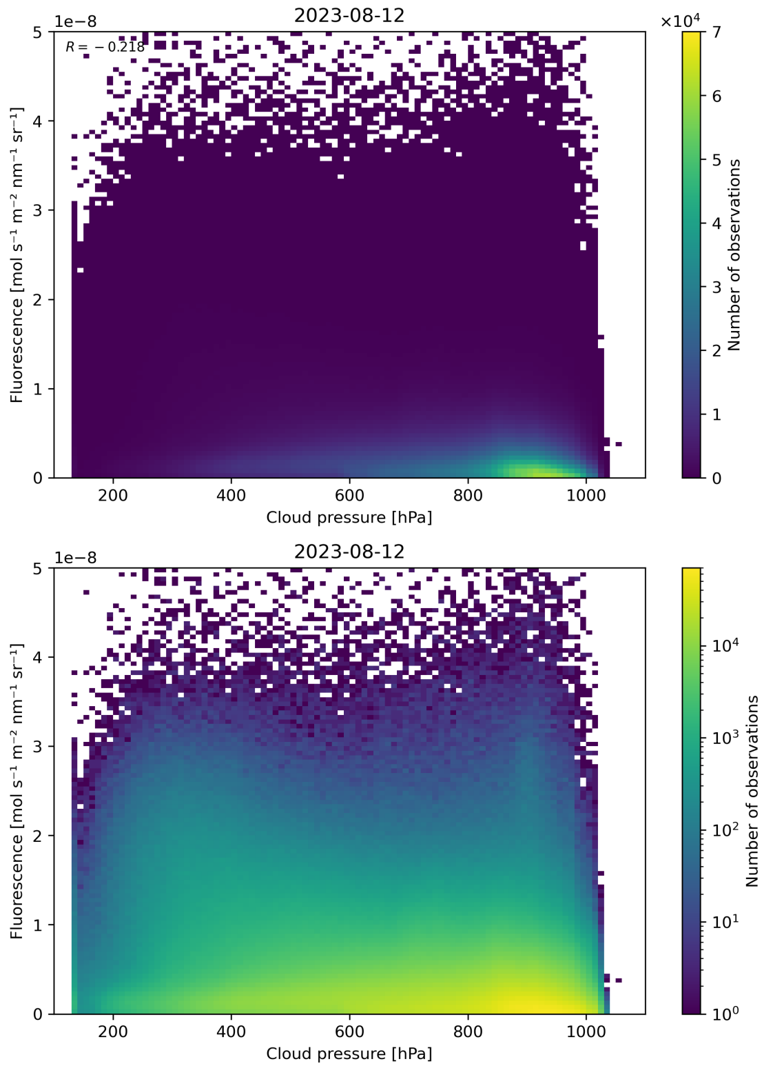
Figure 88: Scatter density plot of “Cloud pressure” against “Fluorescence” for 2023-08-11 to 2023-08-13.
