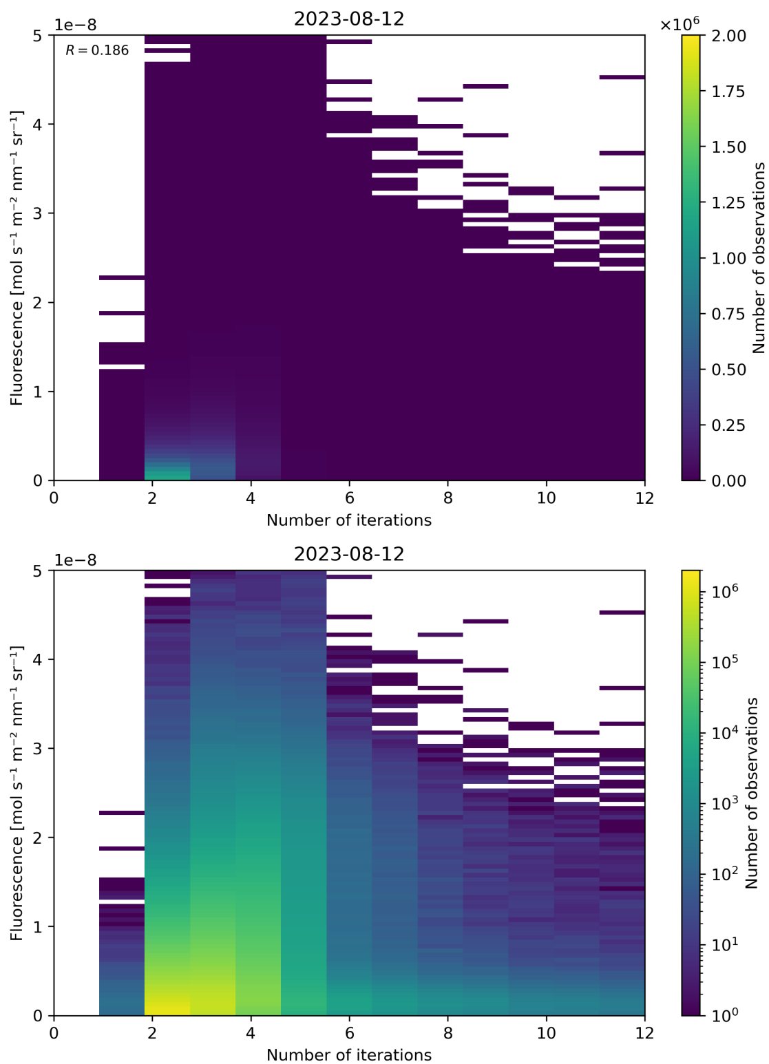
Figure 107: Scatter density plot of “Number of iterations” against “Fluorescence” for 2023-08-11 to 2023-08-13.
