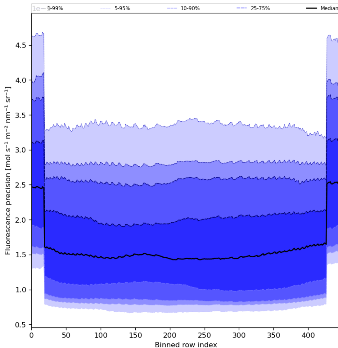
Figure 58: Along track statistics of “Fluorescence precision” for 2023-08-11 to 2023-08-13
