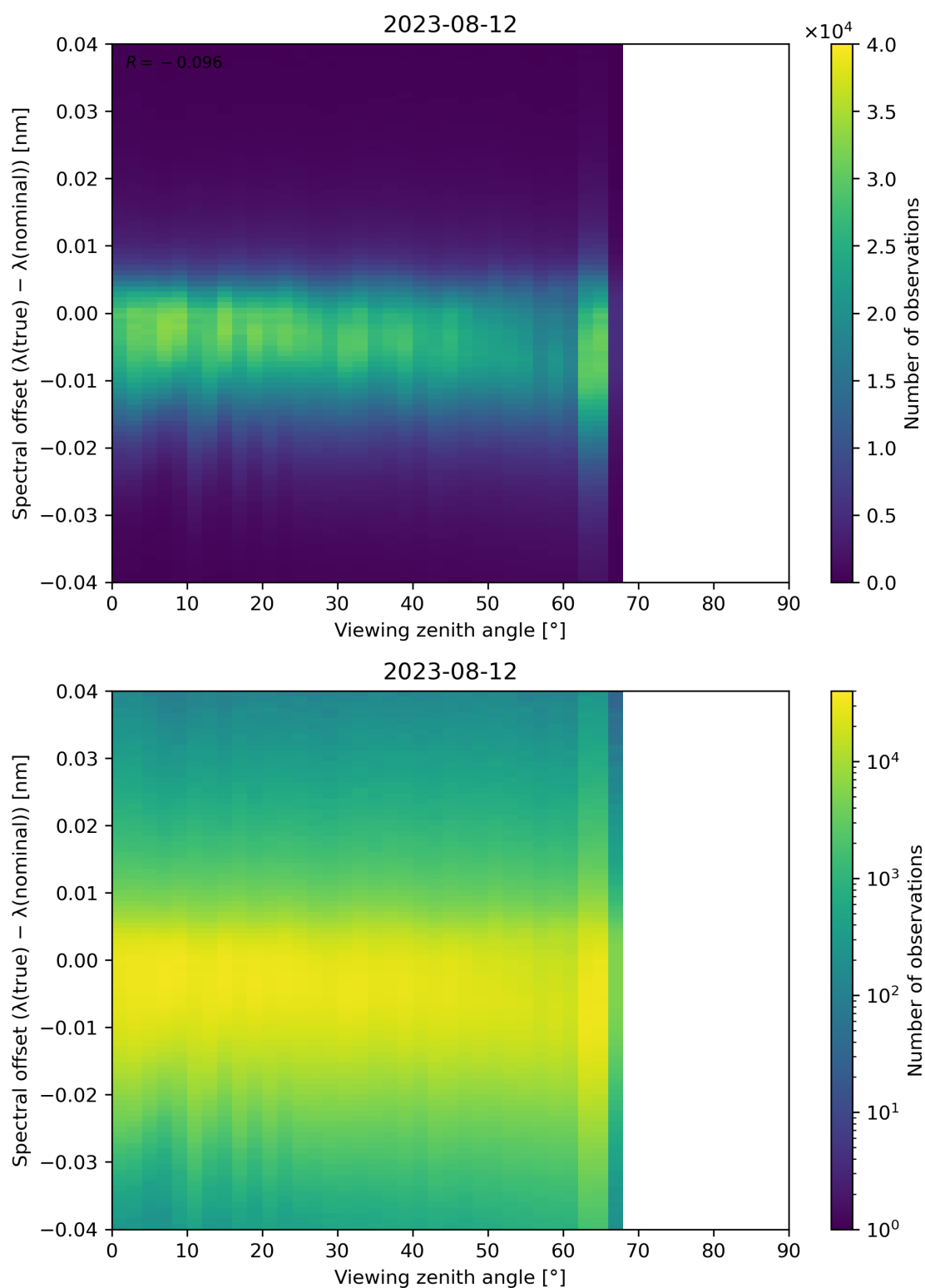
Figure 140: Scatter density plot of “Viewing zenith angle” against “Spectral offset ( \lambda(\text{true}) - \lambda(\text{nominal}) )” for 2023-08-11 to 2023-08-13.
