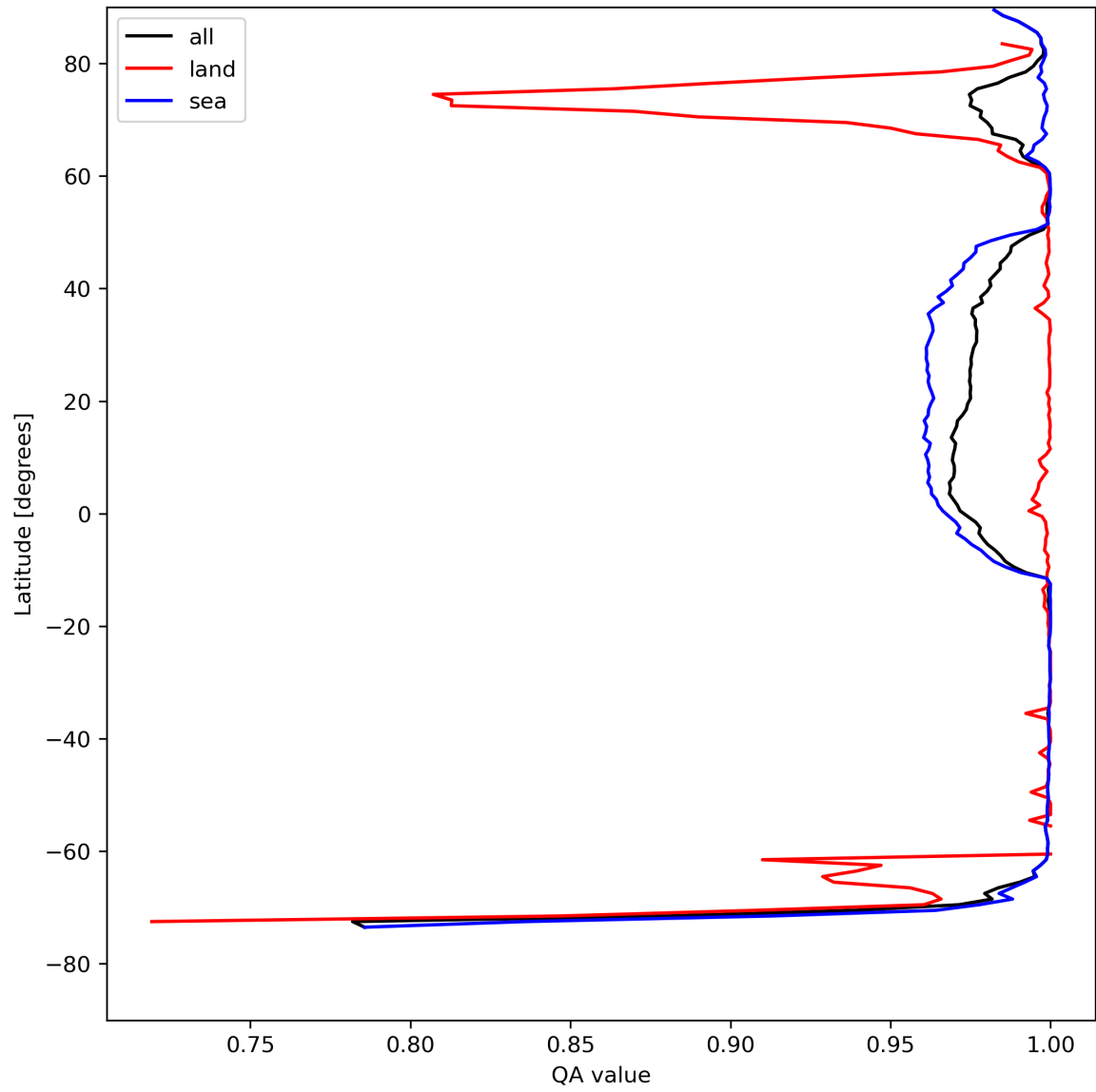
Figure 12: Zonal average of "QA value" for 2023-08-11 to 2023-08-13.
