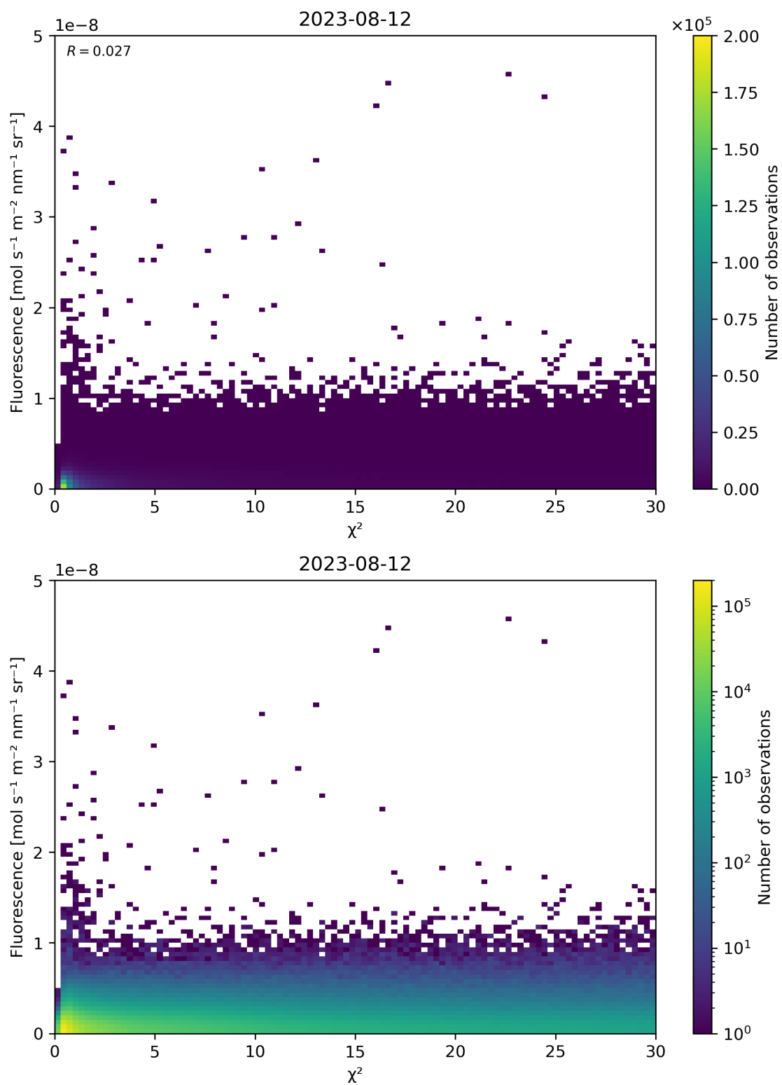
Figure 70: Scatter density plot of “ \chi^2 ” against “Fluorescence” for 2023-08-11 to 2023-08-13.
