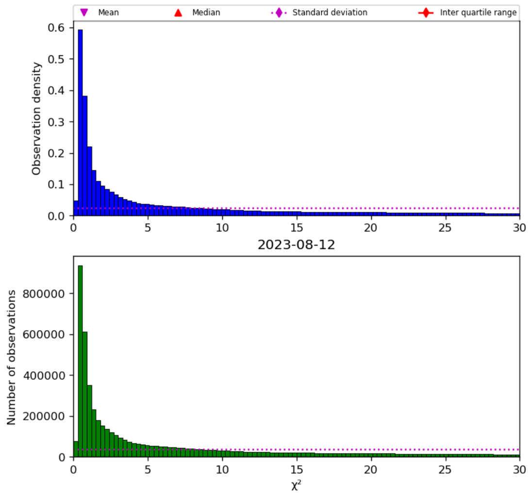
Figure 38: Histogram of “ \chi^2 ” for 2023-08-11 to 2023-08-13
