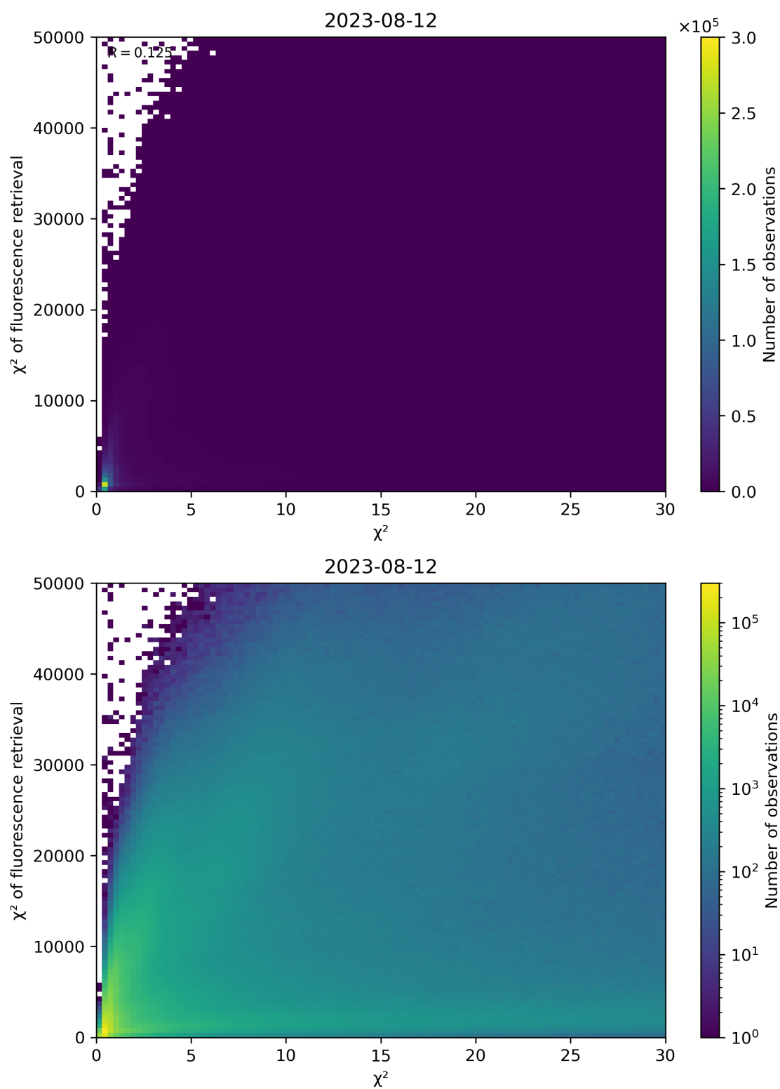
Figure 69: Scatter density plot of “ \chi^2 ” against “ \chi^2 of fluorescence retrieval” for 2023-08-11 to 2023-08-13.
