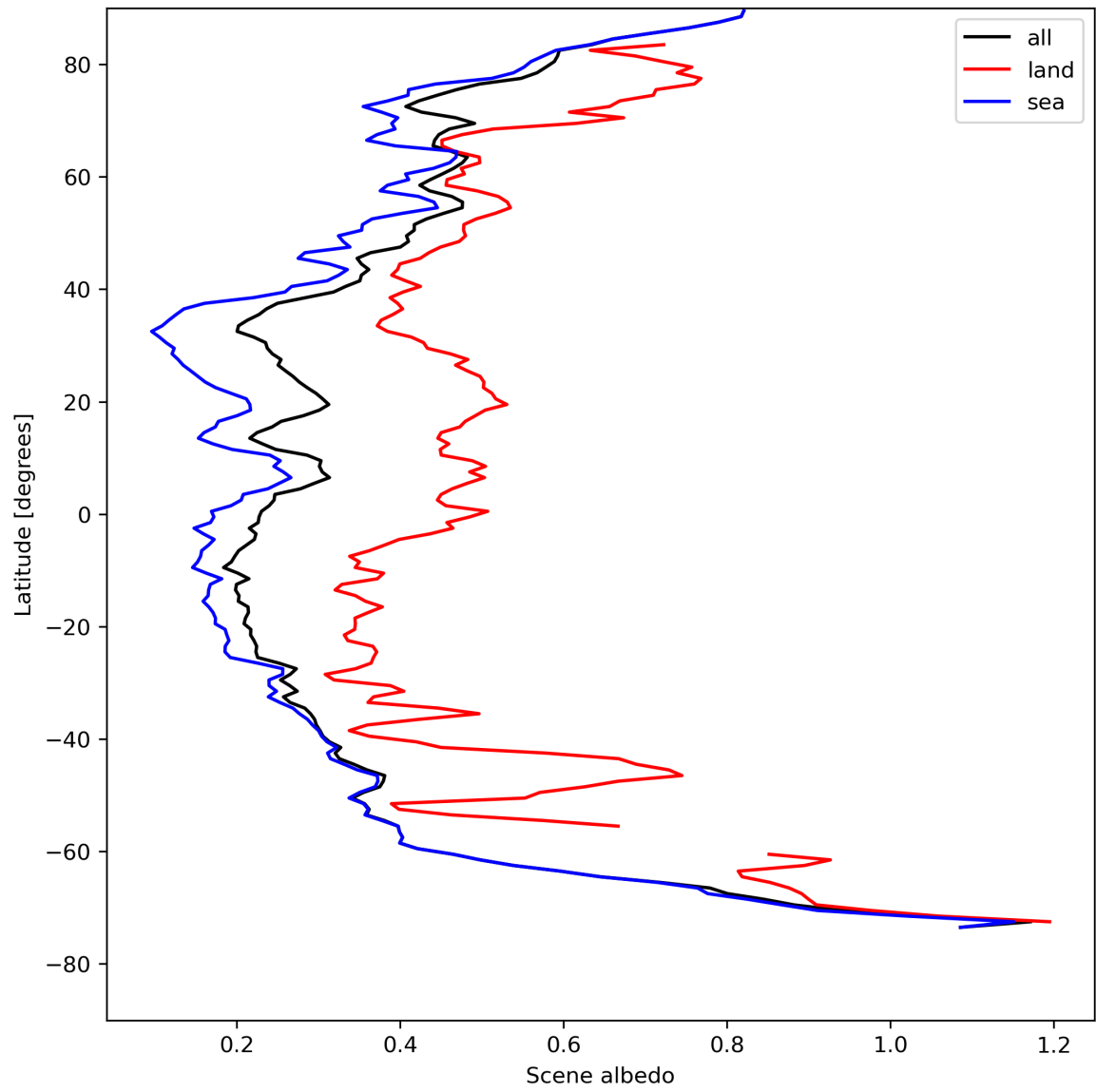
Figure 17: Zonal average of “Scene albedo” for 2023-08-11 to 2023-08-13.
