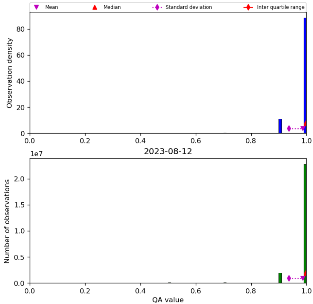
Figure 29: Histogram of “QA value” for 2023-08-11 to 2023-08-13
