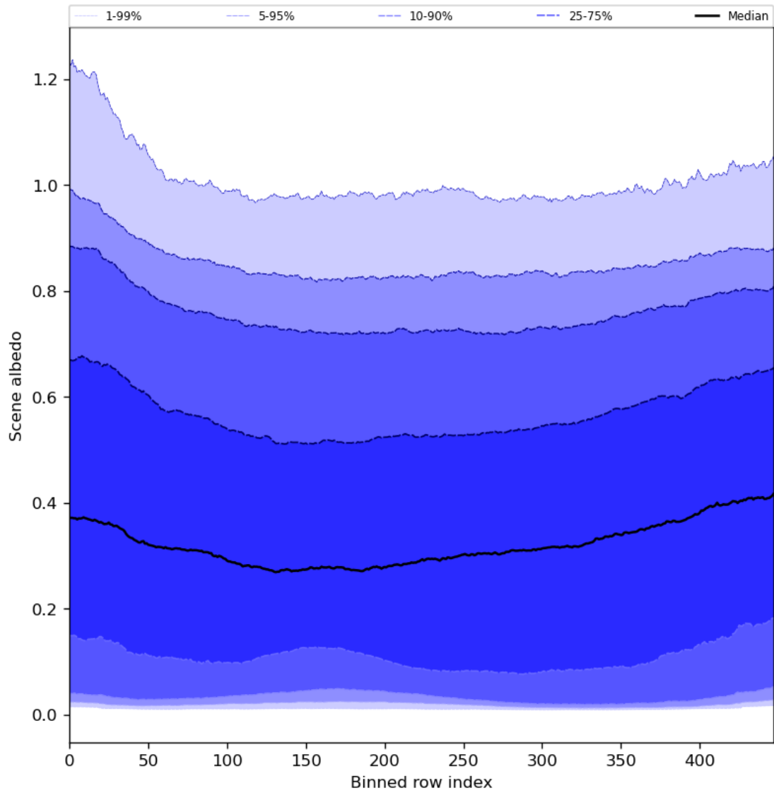
Figure 51: Along track statistics of “Scene albedo” for 2023-08-11 to 2023-08-13
