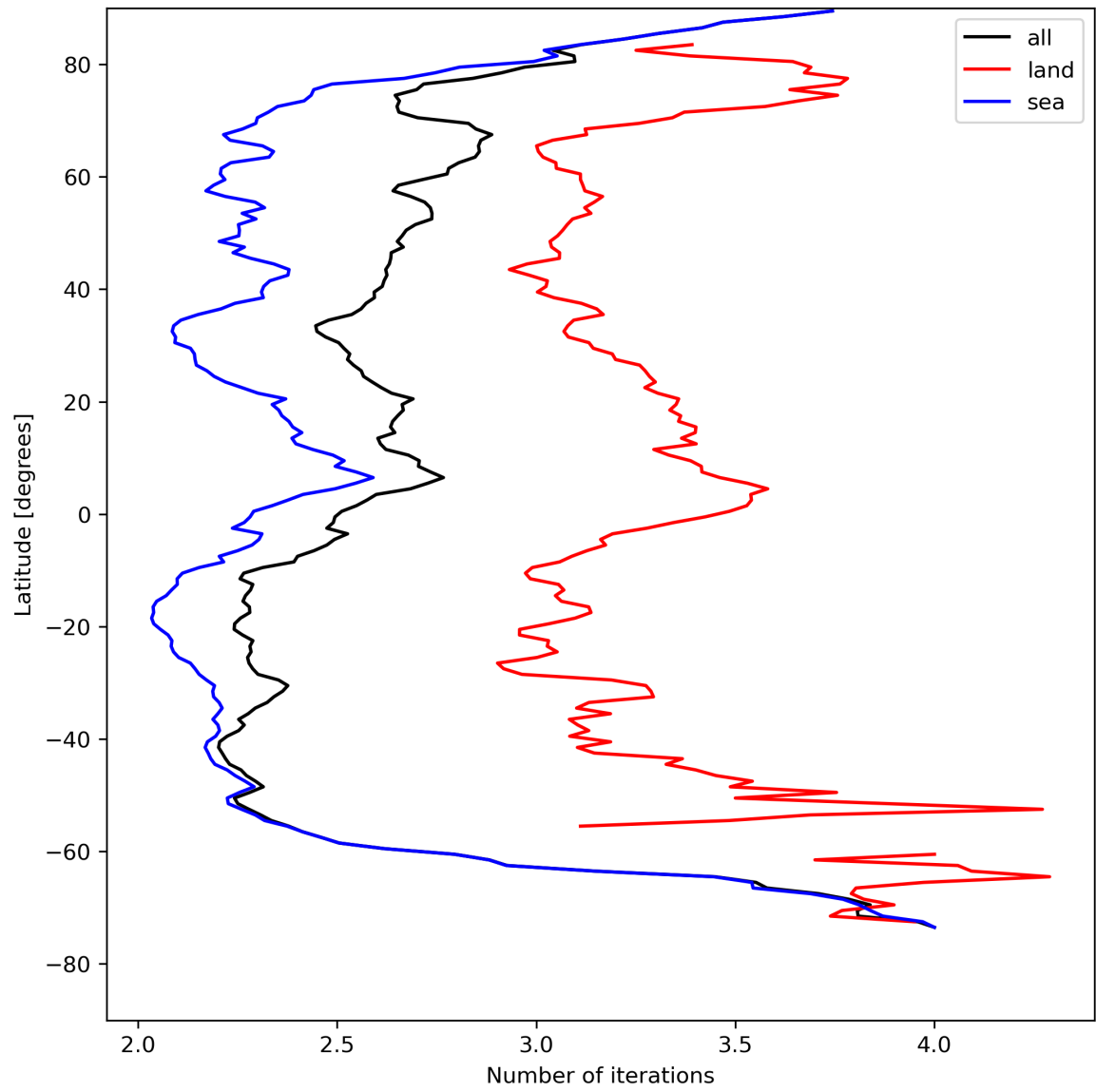
Figure 22: Zonal average of “Number of iterations” for 2023-08-11 to 2023-08-13.
