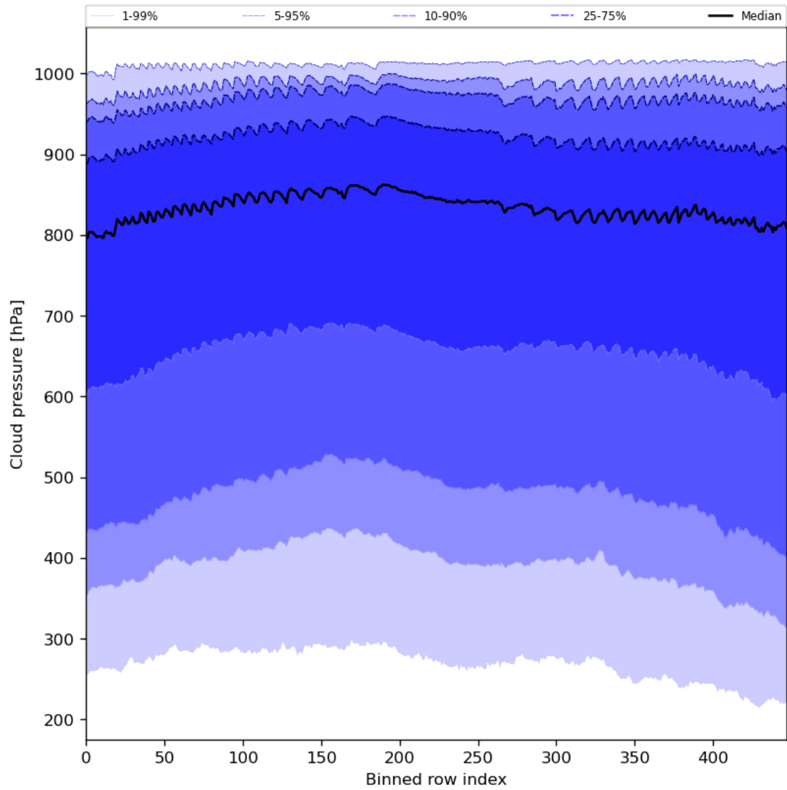
Figure 47: Along track statistics of “Cloud pressure” for 2023-08-11 to 2023-08-13
