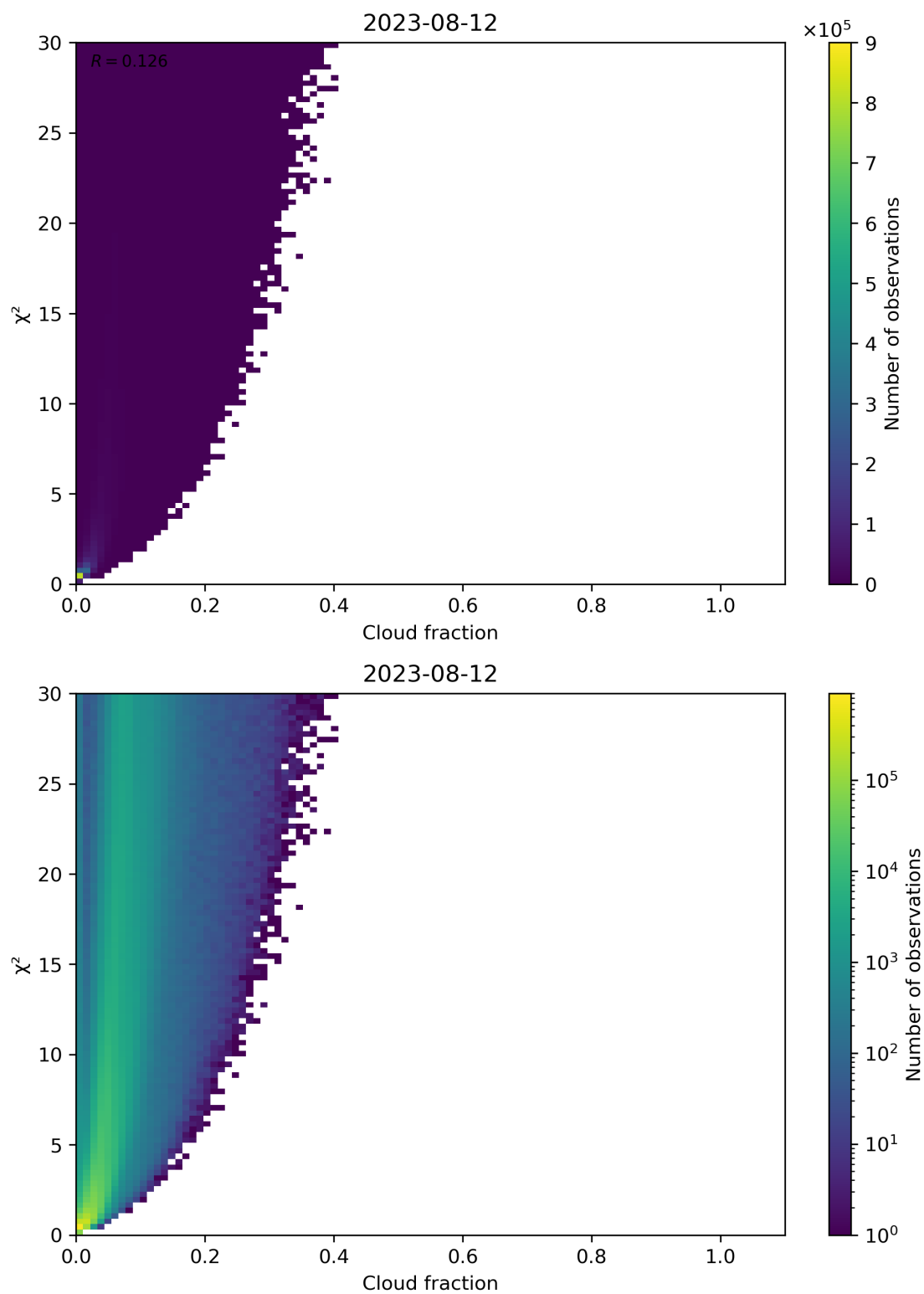
Figure 77: Scatter density plot of “Cloud fraction” against “ \chi^2 ” for 2023-08-11 to 2023-08-13.
