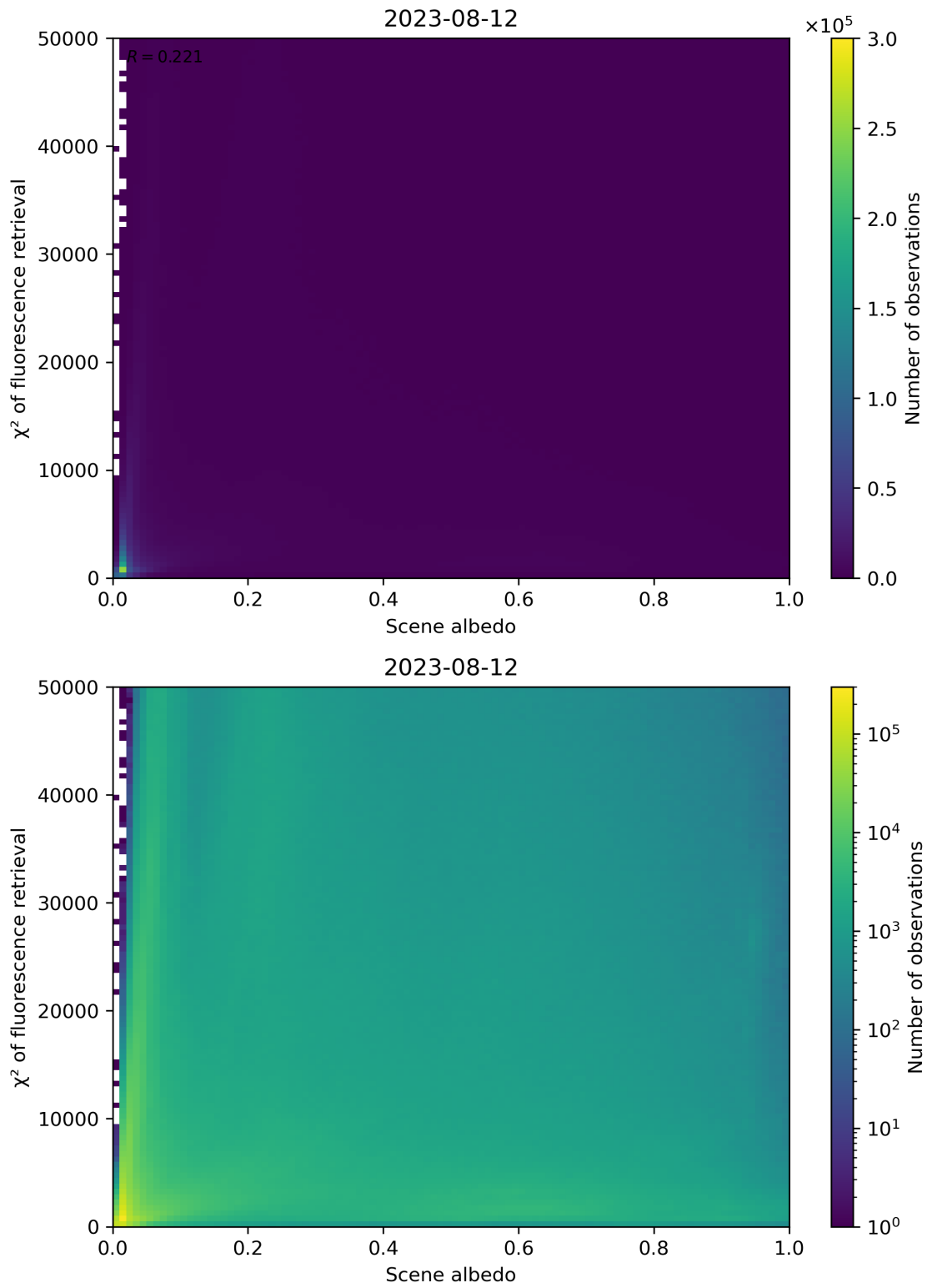
Figure 113: Scatter density plot of “Scene albedo” against “ \chi^2 of fluorescence retrieval” for 2023-08-11 to 2023-08-13.
