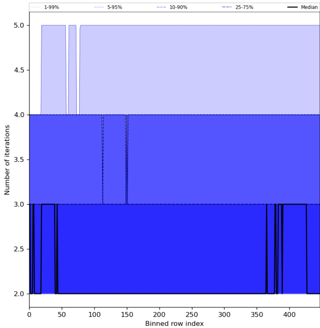
Figure 56: Along track statistics of “Number of iterations” for 2023-08-11 to 2023-08-13
