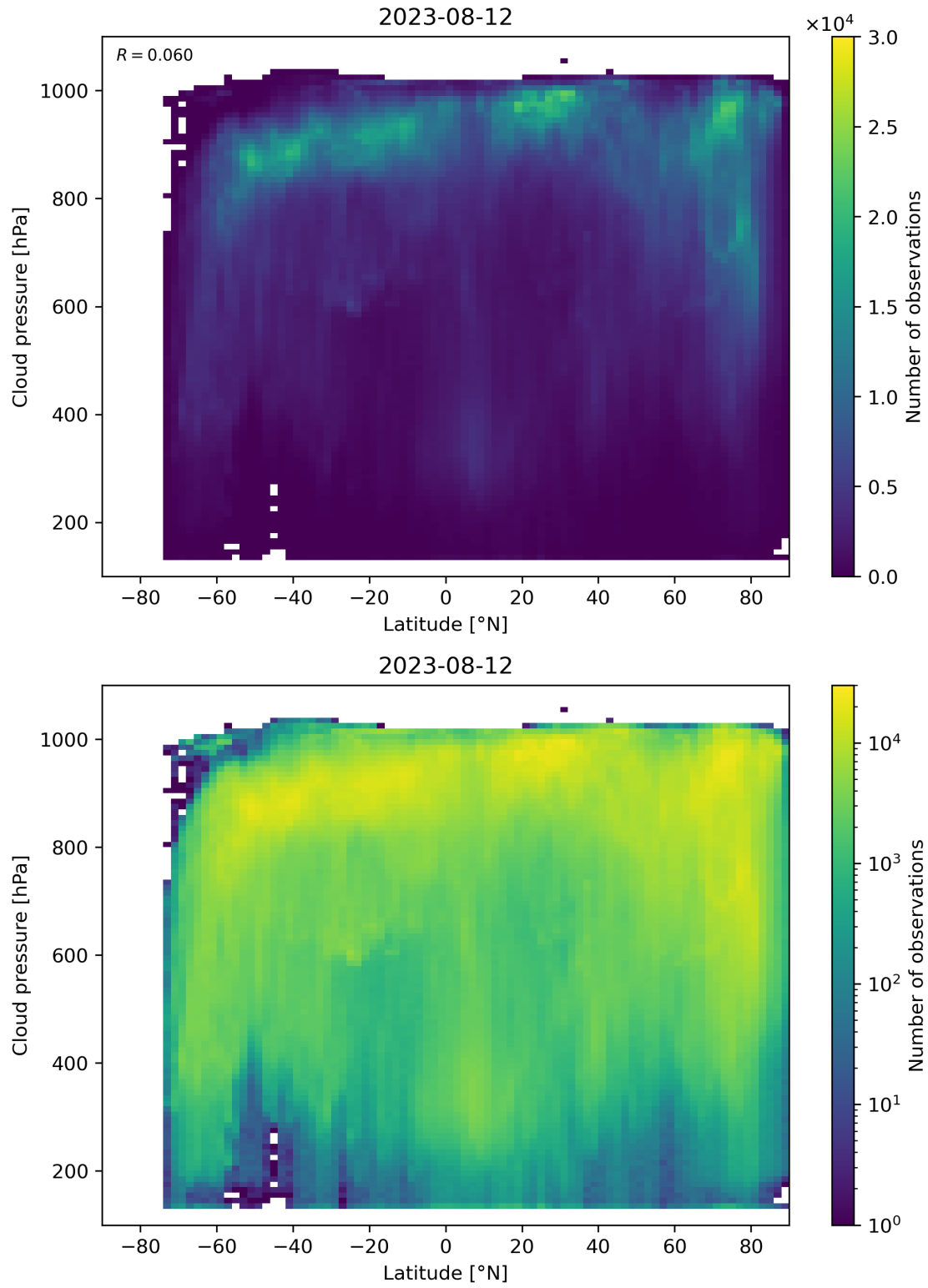
Figure 100: Scatter density plot of “Latitude” against “Cloud pressure” for 2023-08-11 to 2023-08-13.
