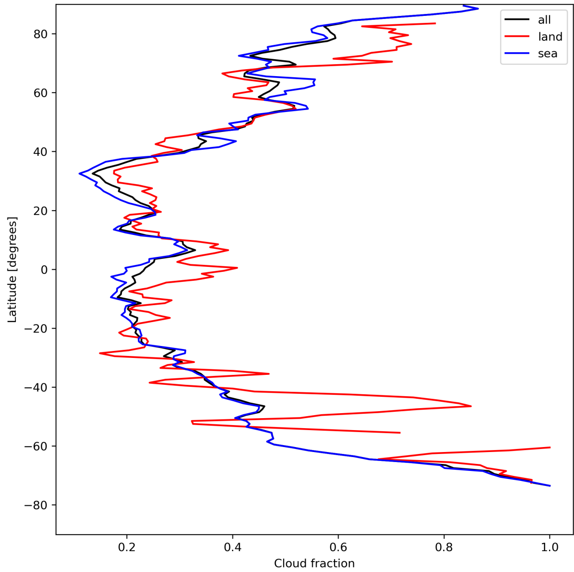
Figure 15: Zonal average of “Cloud fraction” for 2023-08-11 to 2023-08-13.
