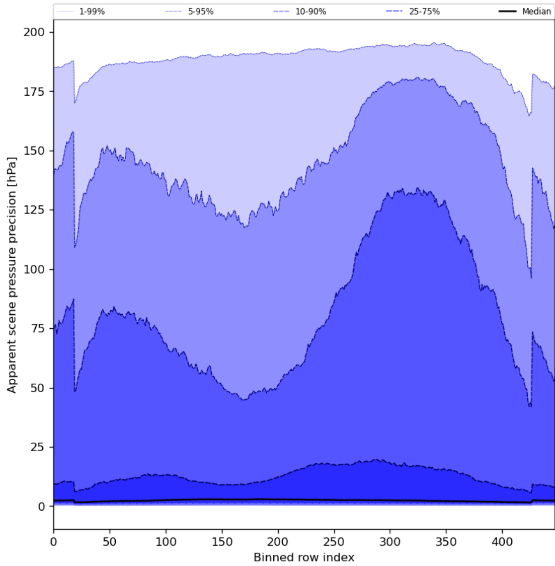
Figure 54: Along track statistics of “Apparent scene pressure precision” for 2023-08-11 to 2023-08-13
