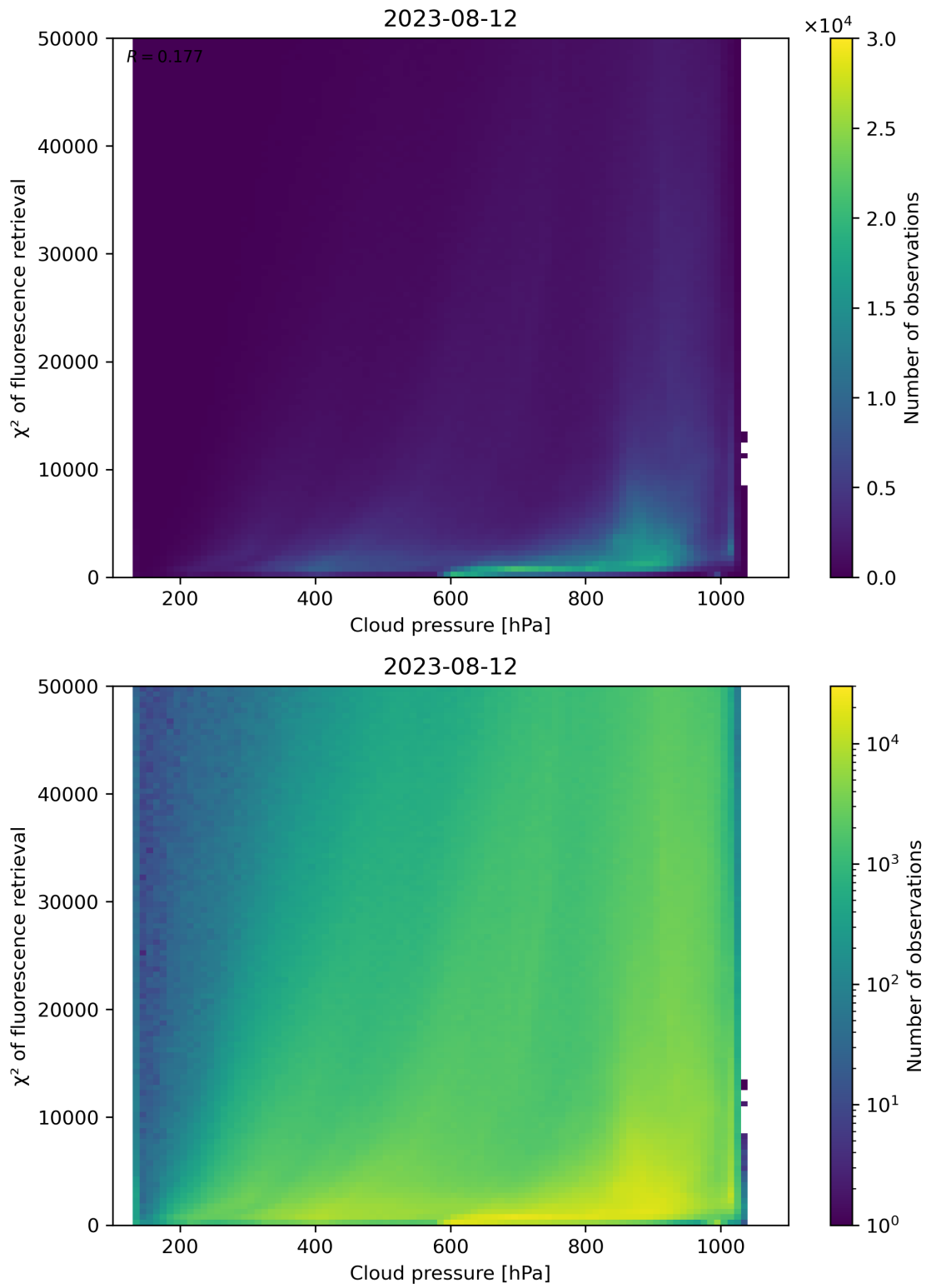
Figure 86: Scatter density plot of “Cloud pressure” against “ \chi^2 of fluorescence retrieval” for 2023-08-11 to 2023-08-13.
