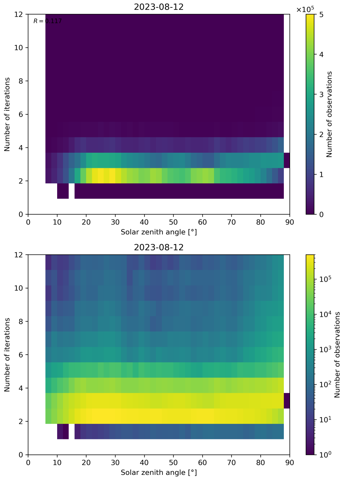
Figure 125: Scatter density plot of “Solar zenith angle” against “Number of iterations” for 2023-08-11 to 2023-08-13.
