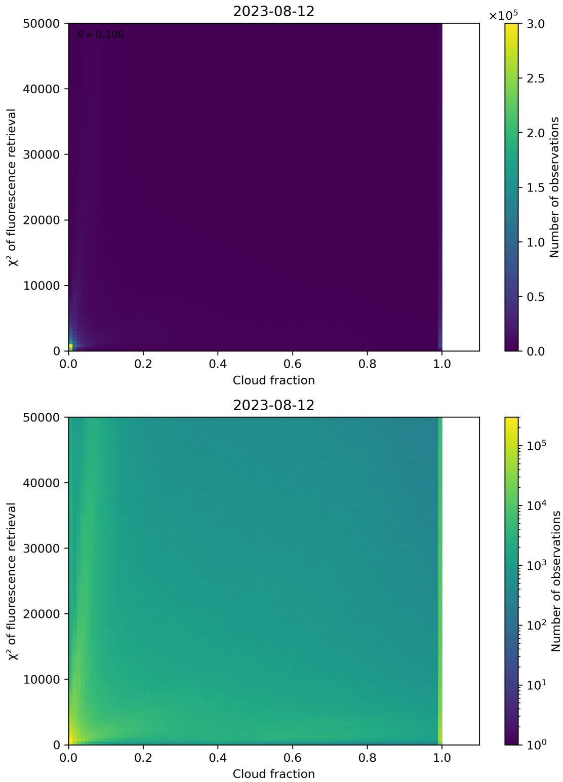
Figure 78: Scatter density plot of “Cloud fraction” against “ \chi^2 of fluorescence retrieval” for 2023-08-11 to 2023-08-13.
