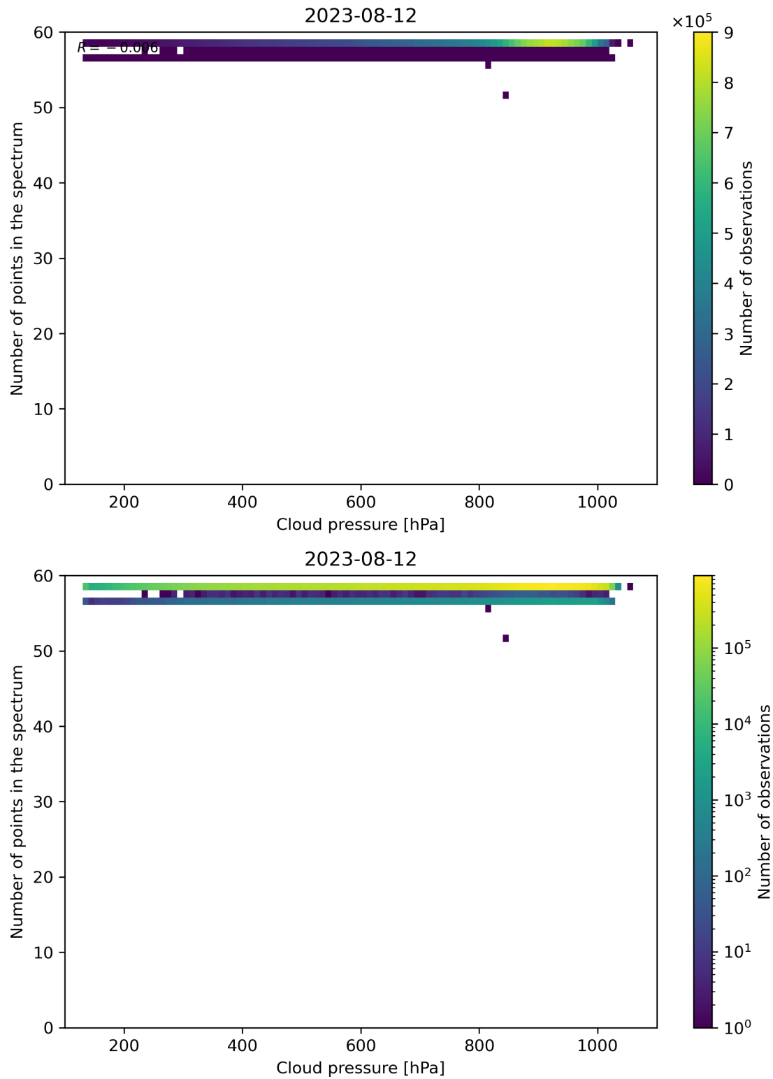
Figure 90: Scatter density plot of “Cloud pressure” against “Number of points in the spectrum” for 2023-08-11 to 2023-08-13.
