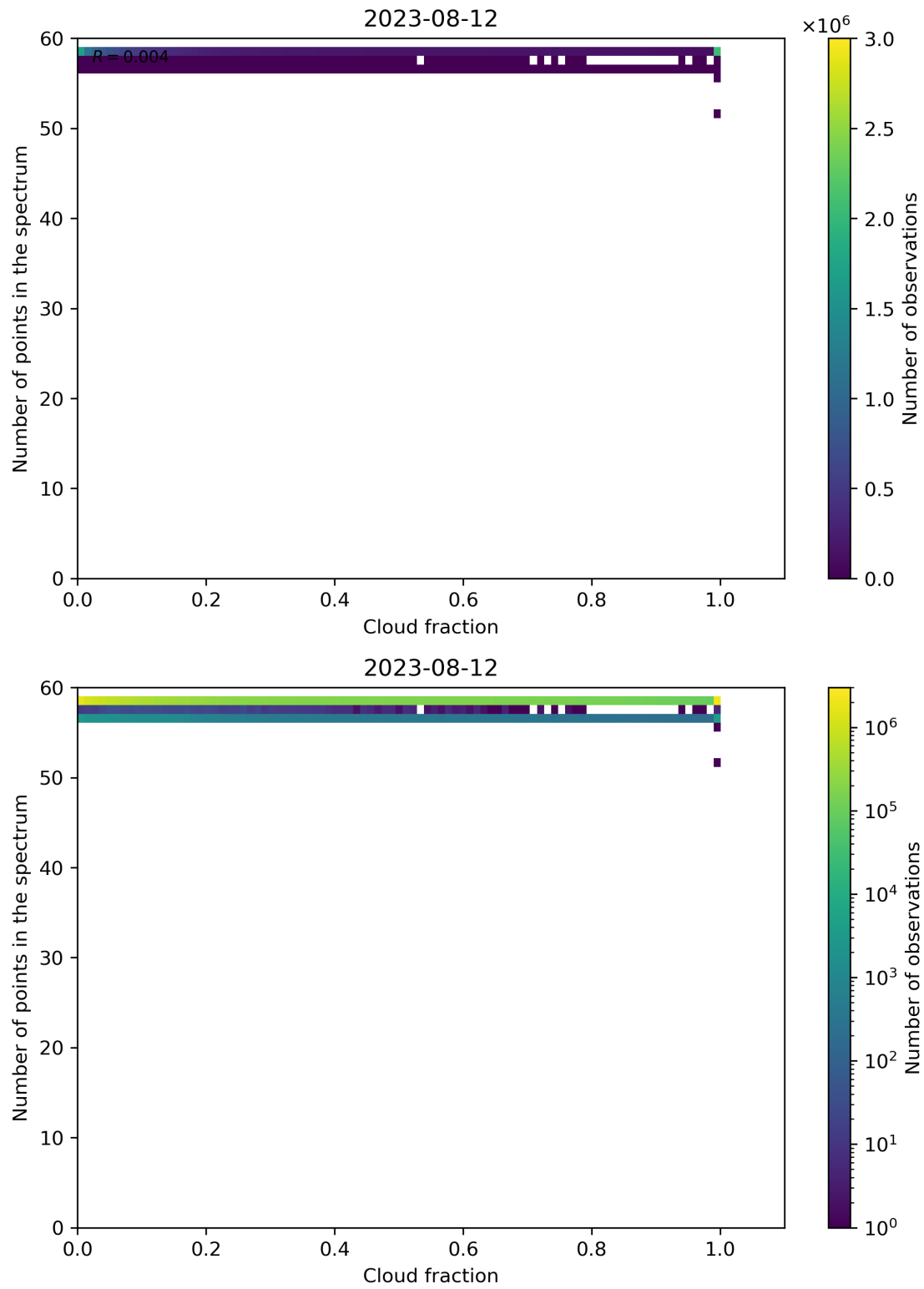
Figure 81: Scatter density plot of “Cloud fraction” against “Number of points in the spectrum” for 2023-08-11 to 2023-08-13.
