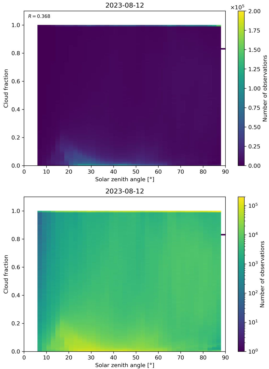
Figure 121: Scatter density plot of “Solar zenith angle” against “Cloud fraction” for 2023-08-11 to 2023-08-13.
