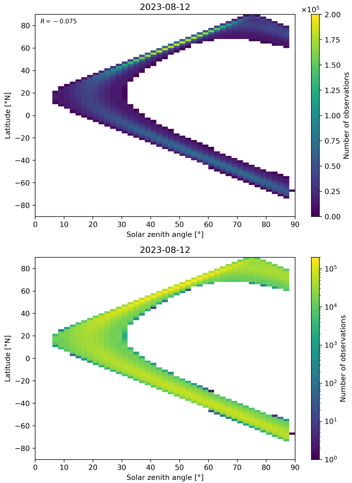
Figure 124: Scatter density plot of “Solar zenith angle” against “Latitude” for 2023-08-11 to 2023-08-13.
