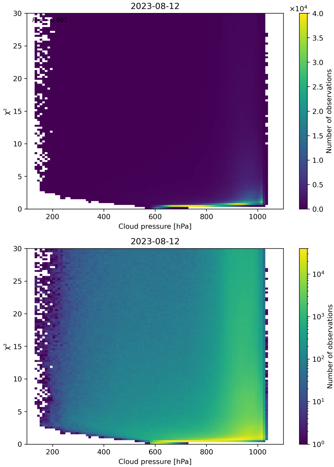
Figure 85: Scatter density plot of “Cloud pressure” against “ \chi^2 ” for 2023-08-11 to 2023-08-13.
