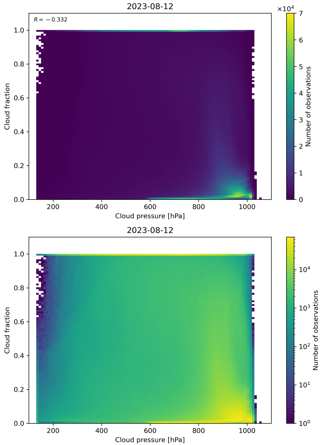
Figure 87: Scatter density plot of “Cloud pressure” against “Cloud fraction” for 2023-08-11 to 2023-08-13.
