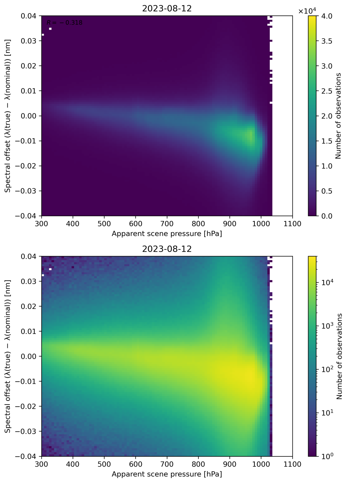
Figure 68: Scatter density plot of “Apparent scene pressure” against “Spectral offset ( \lambda(\text{true}) - \lambda(\text{nominal}) )” for 2023-08-11 to 2023-08-13.
