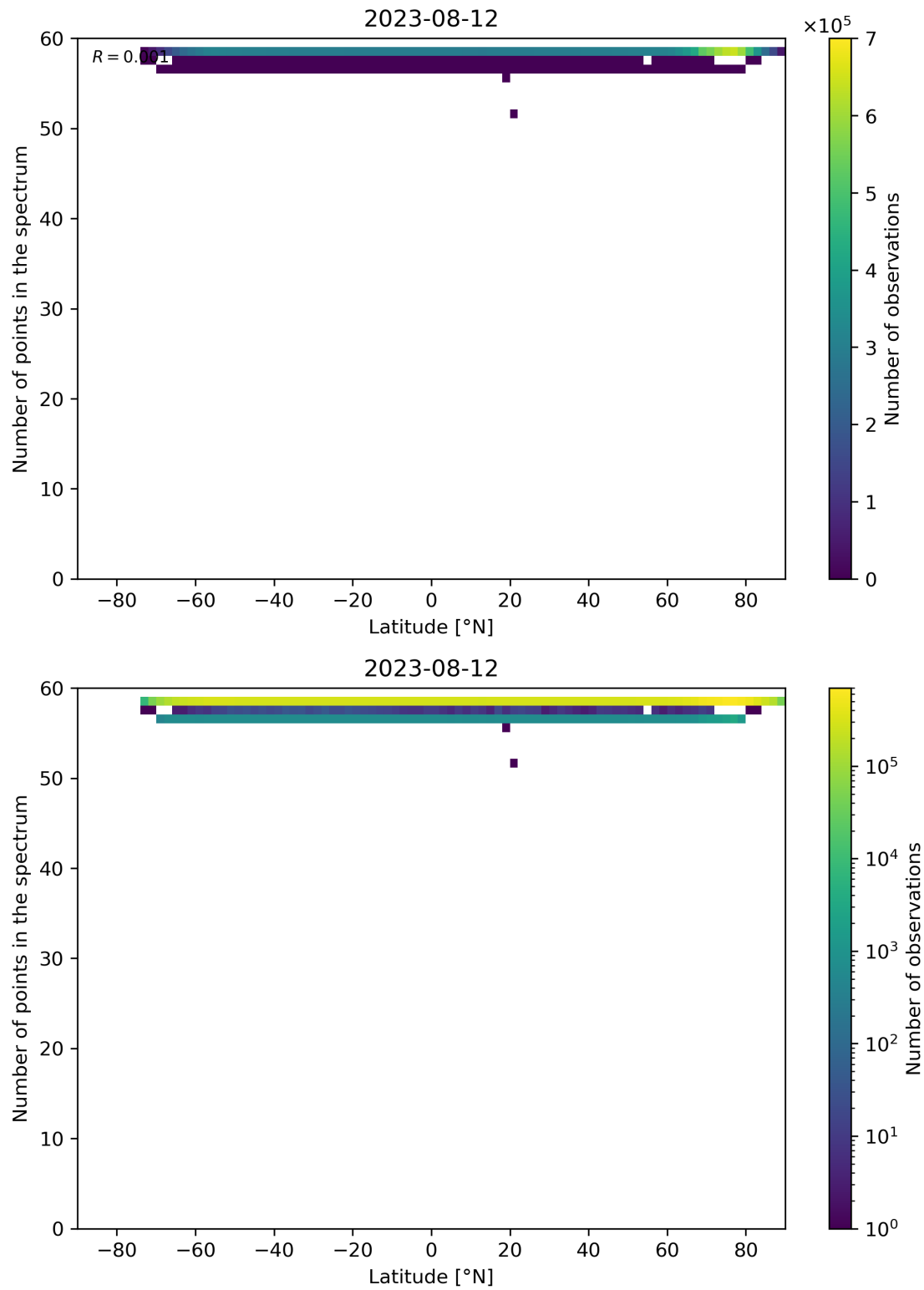
Figure 103: Scatter density plot of “Latitude” against “Number of points in the spectrum” for 2023-08-11 to 2023-08-13.
