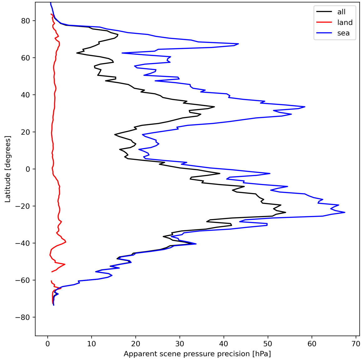
Figure 20: Zonal average of “Apparent scene pressure precision” for 2023-08-11 to 2023-08-13.
