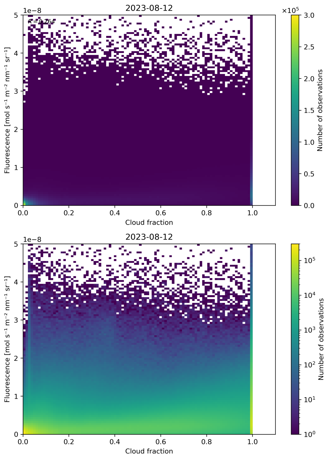
Figure 79: Scatter density plot of “Cloud fraction” against “Fluorescence” for 2023-08-11 to 2023-08-13.
