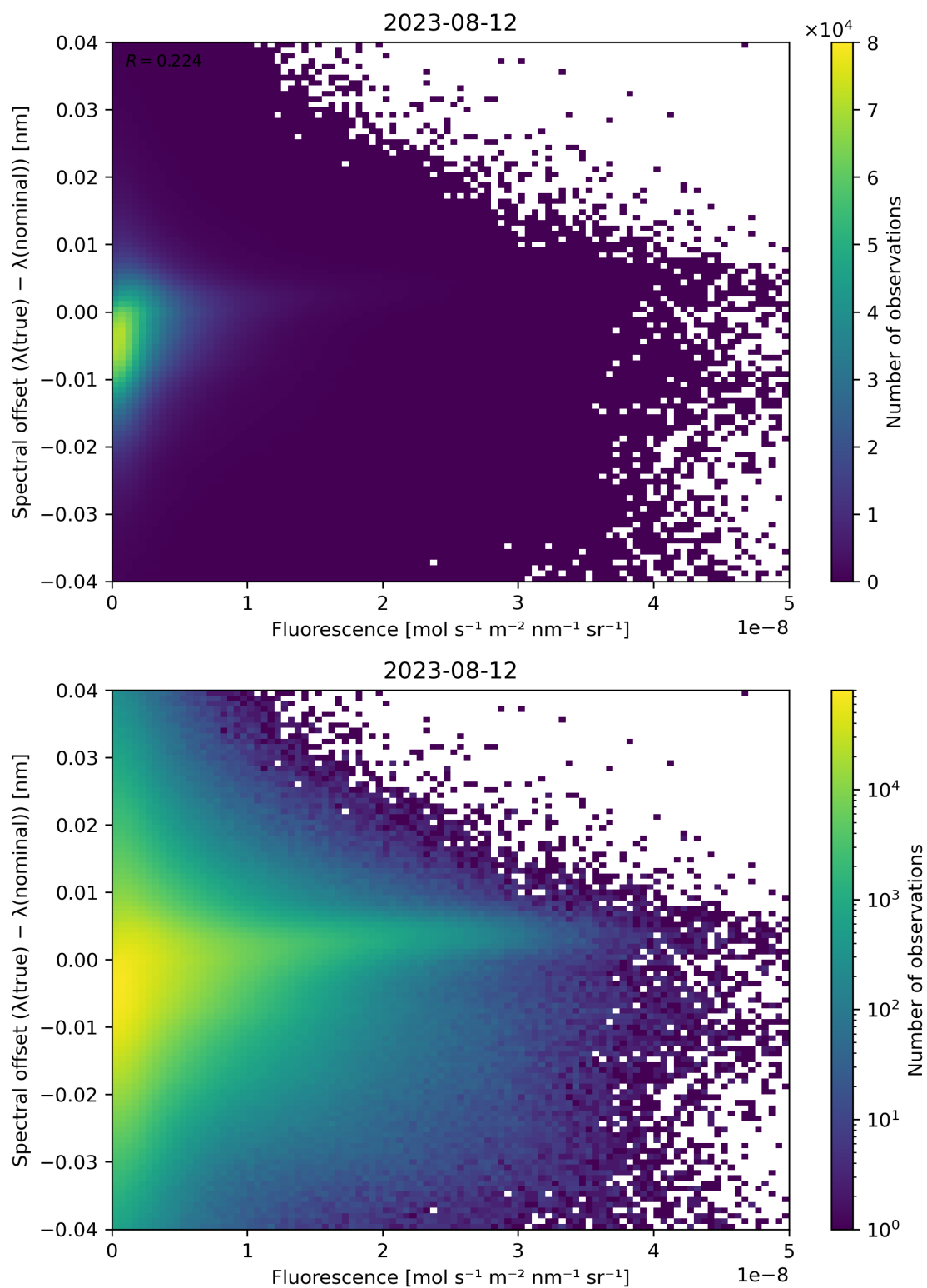
Figure 95: Scatter density plot of “Fluorescence” against “Spectral offset ( \lambda(\text{true}) - \lambda(\text{nominal}) )” for 2023-08-11 to 2023-08-13.
