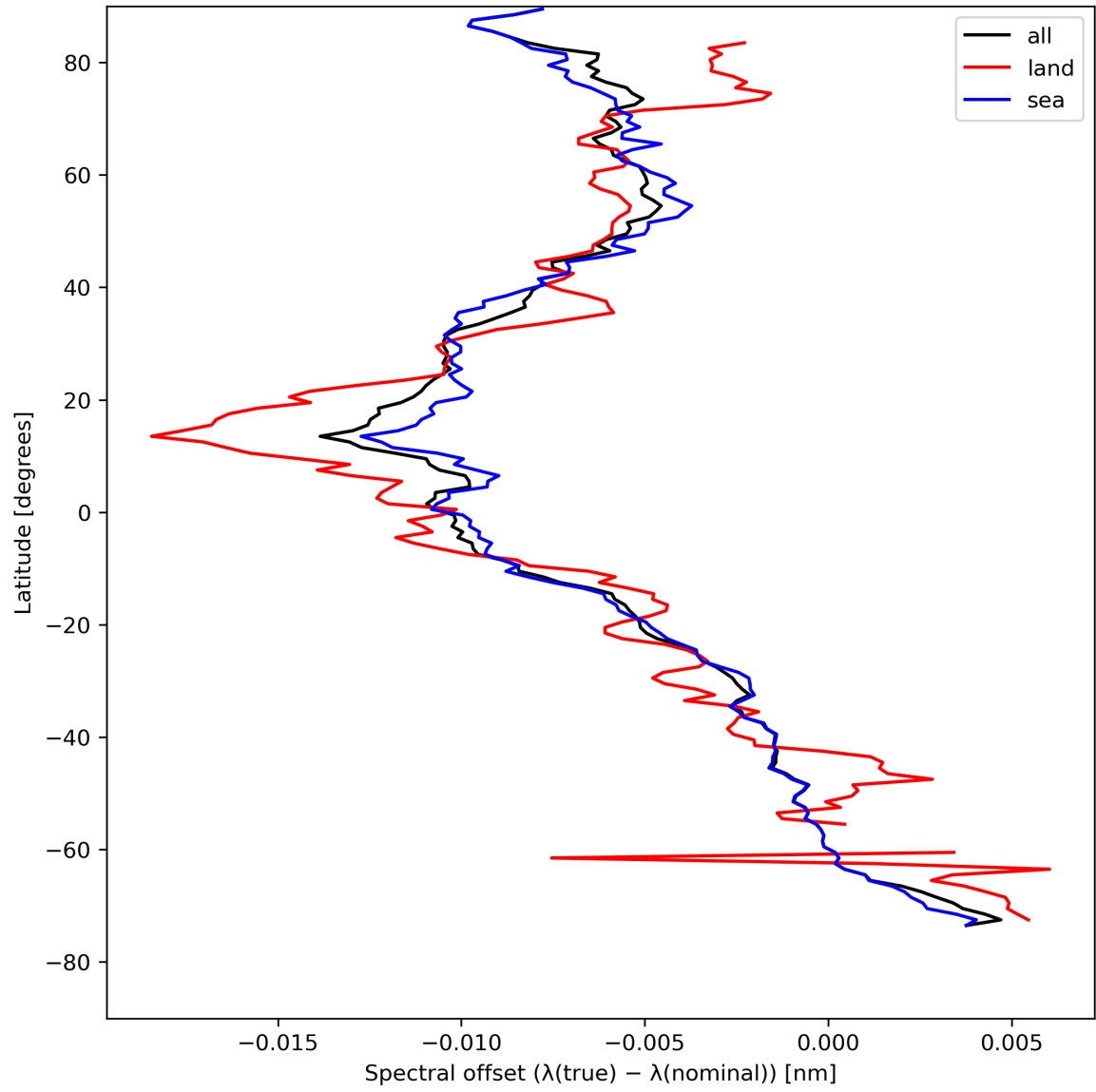
Figure 28: Zonal average of “Spectral offset ( \lambda(\text{true}) - \lambda(\text{nominal}) )” for 2023-08-11 to 2023-08-13.
