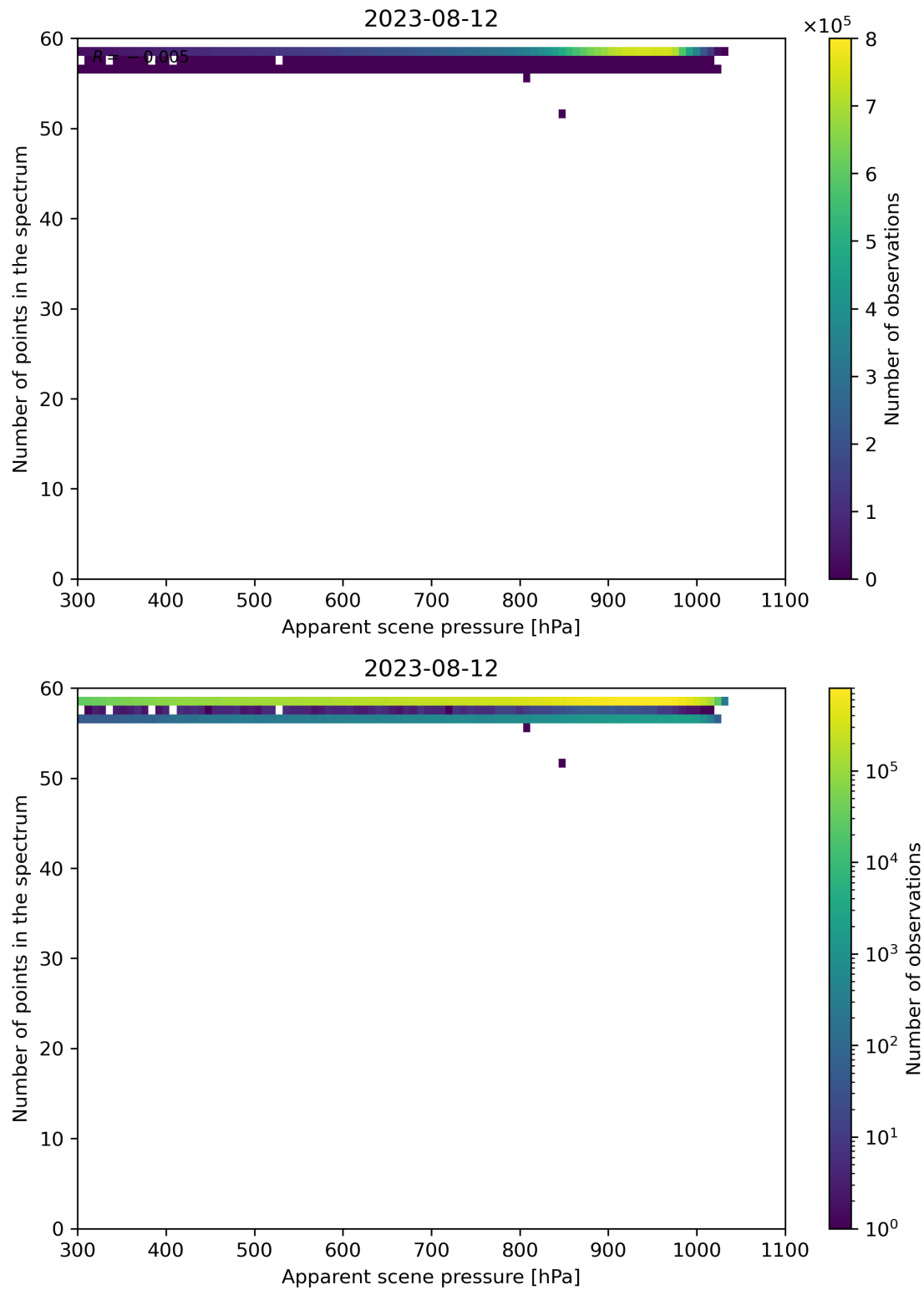
Figure 67: Scatter density plot of “Apparent scene pressure” against “Number of points in the spectrum” for 2023-08-11 to 2023-08-13.
