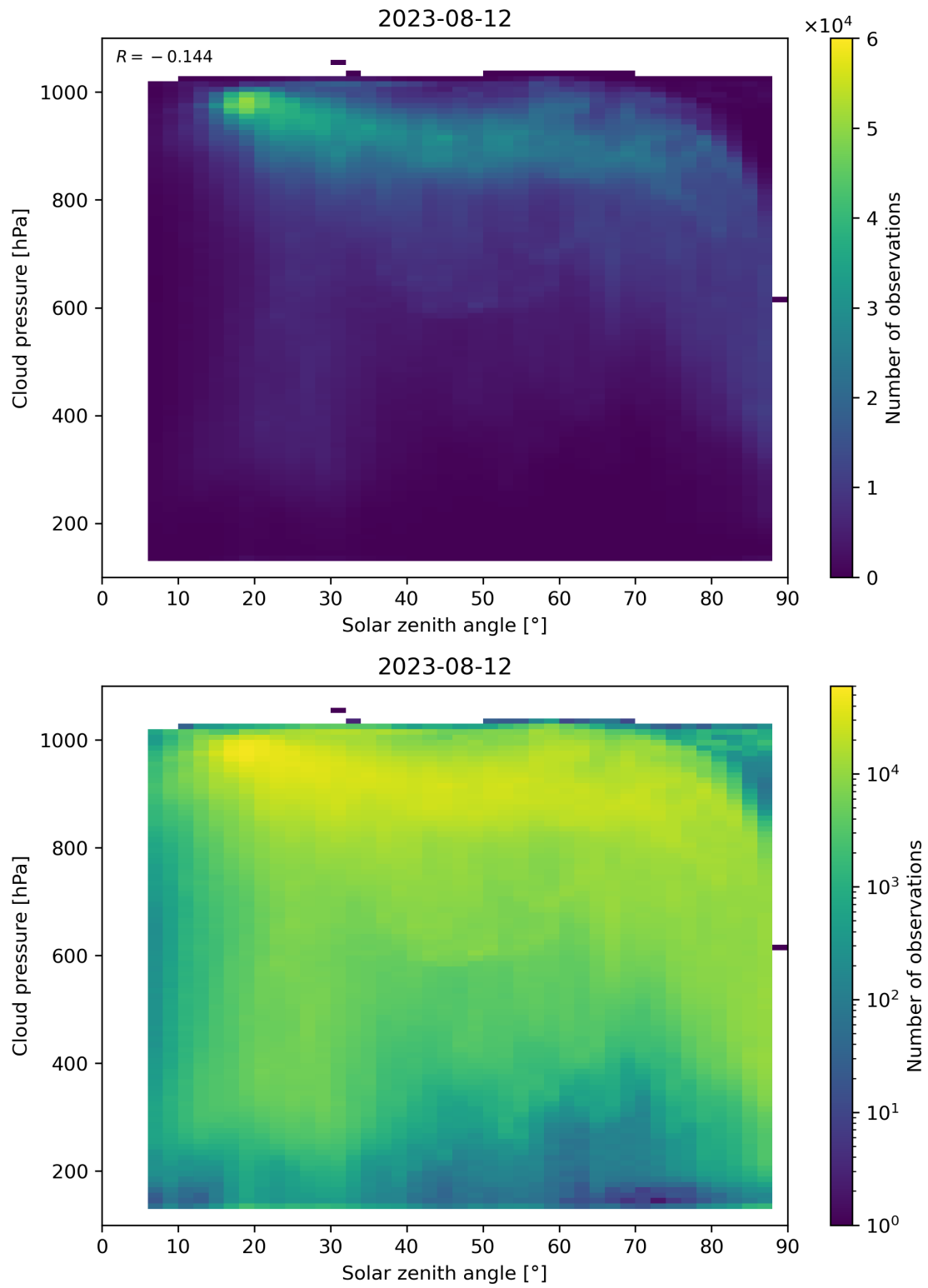
Figure 122: Scatter density plot of “Solar zenith angle” against “Cloud pressure” for 2023-08-11 to 2023-08-13.
