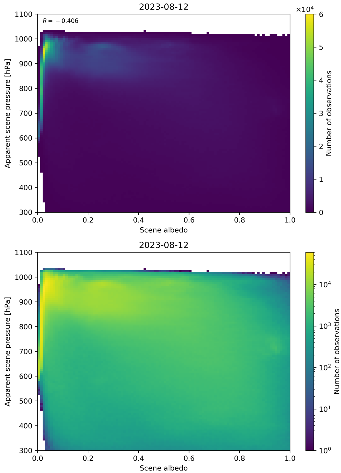
Figure 111: Scatter density plot of “Scene albedo” against “Apparent scene pressure” for 2023-08-11 to 2023-08-13.
