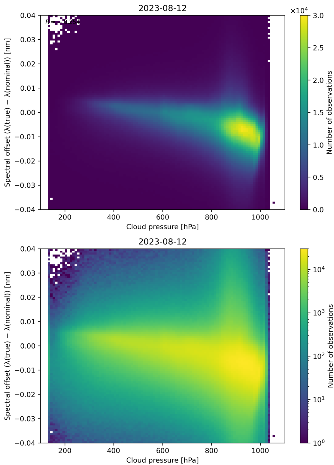
Figure 92: Scatter density plot of “Cloud pressure” against “Spectral offset ( \lambda(\text{true}) - \lambda(\text{nominal}) )” for 2023-08-11 to 2023-08-13.
