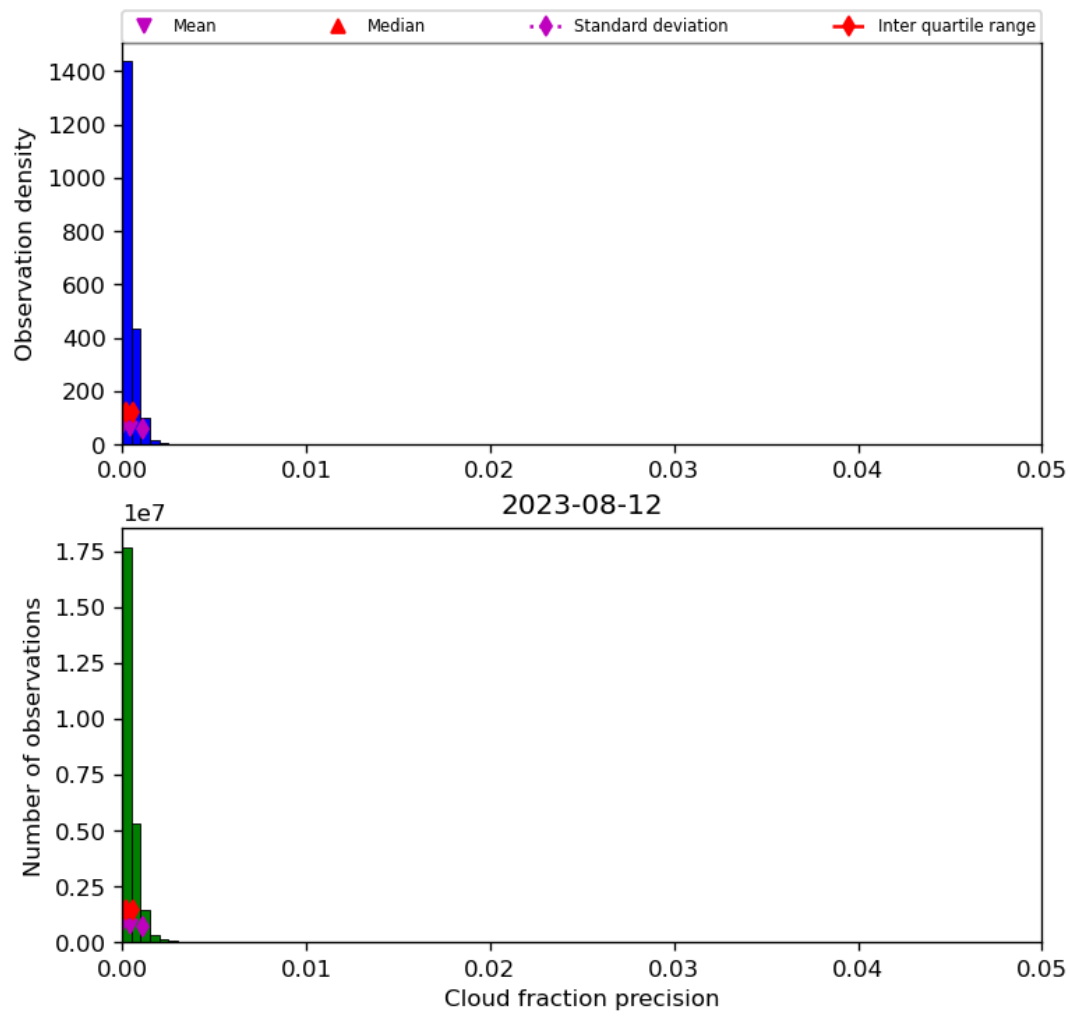
Figure 33: Histogram of “Cloud fraction precision” for 2023-08-11 to 2023-08-13
