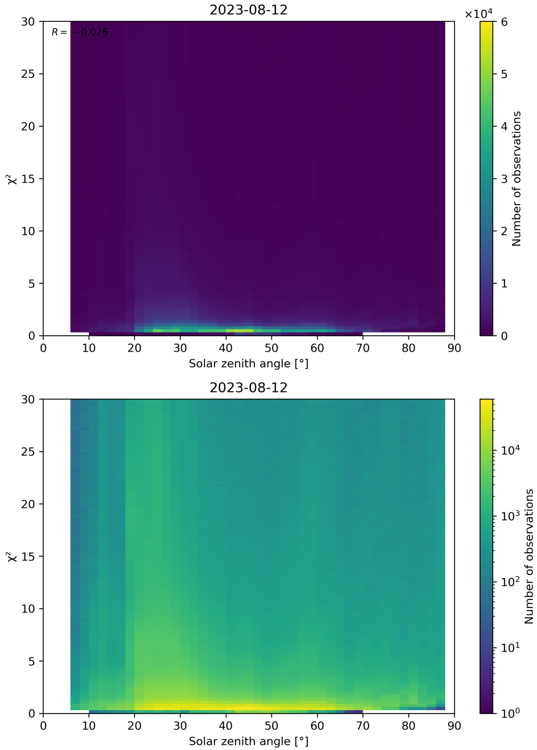
Figure 119: Scatter density plot of “Solar zenith angle” against “ \chi^2 ” for 2023-08-11 to 2023-08-13.
