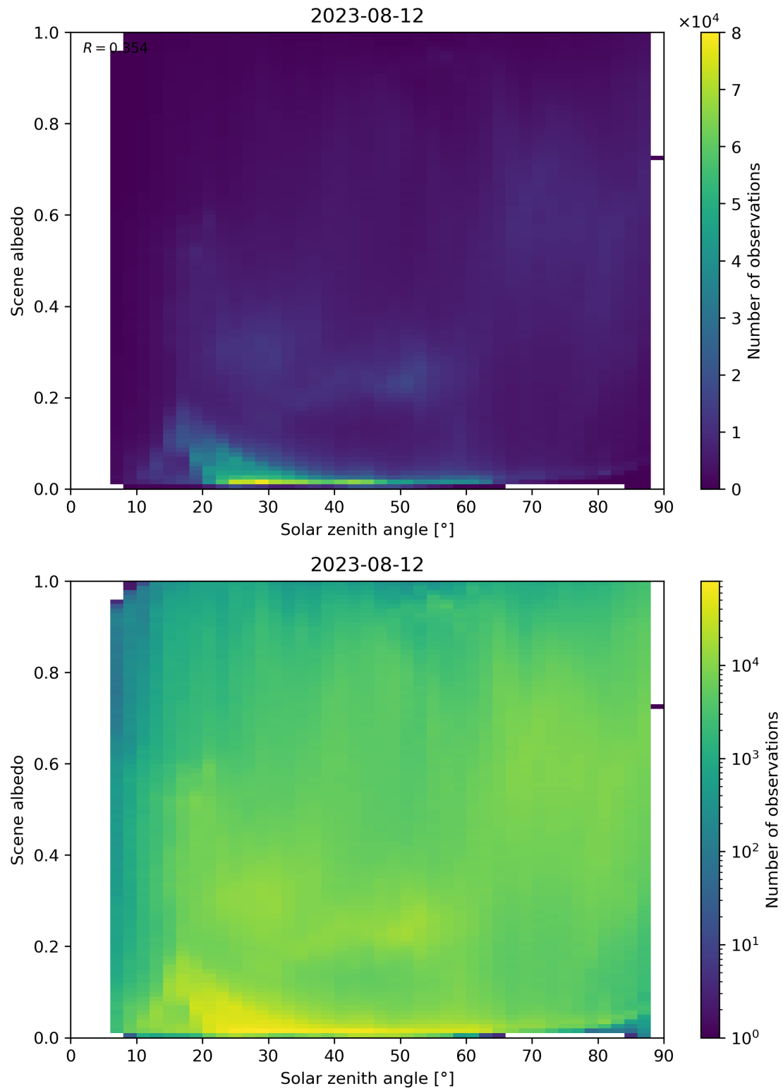
Figure 127: Scatter density plot of “Solar zenith angle” against “Scene albedo” for 2023-08-11 to 2023-08-13.
