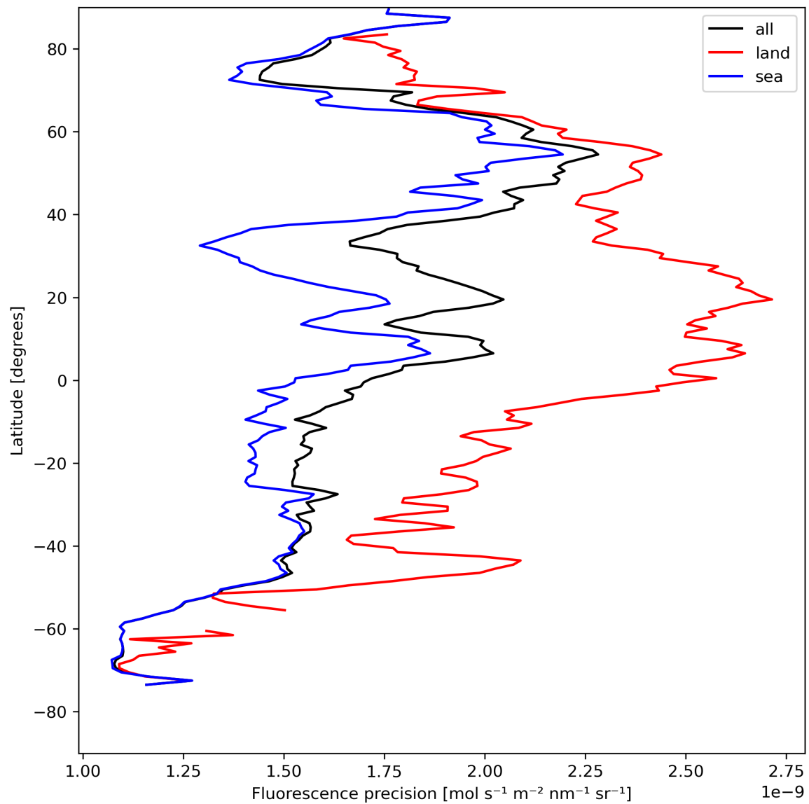
Figure 24: Zonal average of “Fluorescence precision” for 2023-08-11 to 2023-08-13.
