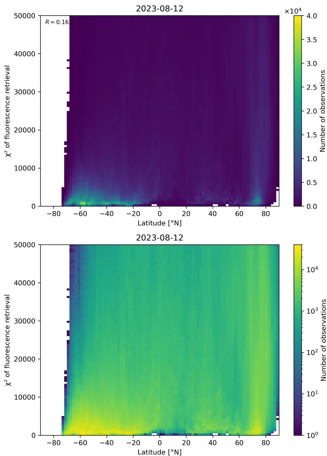
Figure 98: Scatter density plot of “Latitude” against “ \chi^2 of fluorescence retrieval” for 2023-08-11 to 2023-08-13.
