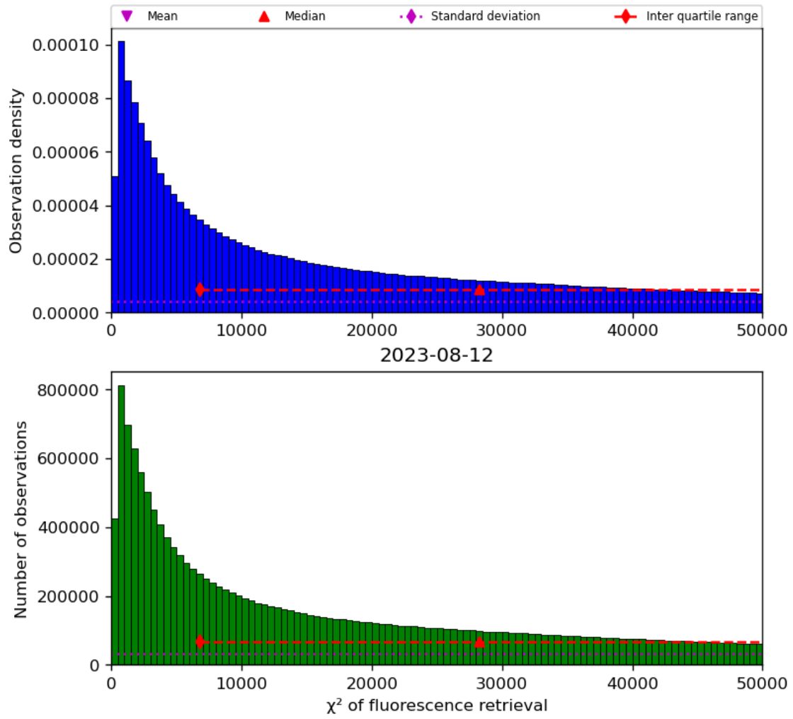
Figure 42: Histogram of “ \chi^2 of fluorescence retrieval” for 2023-08-11 to 2023-08-13
