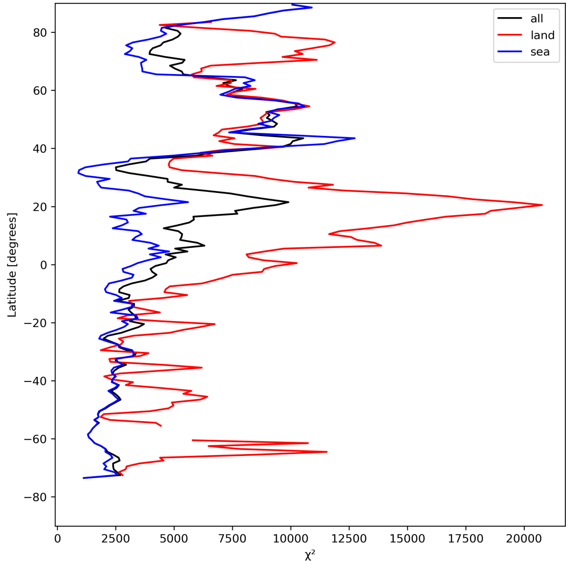
Figure 21: Zonal average of “ \chi^2 ” for 2023-08-11 to 2023-08-13.
