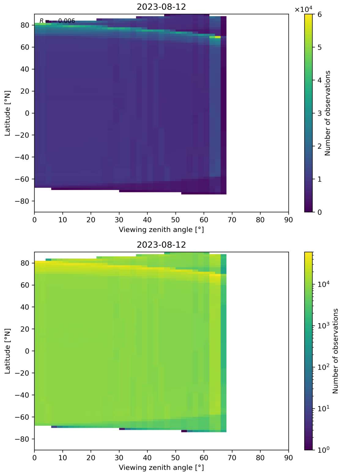
Figure 135: Scatter density plot of “Viewing zenith angle” against “Latitude” for 2023-08-11 to 2023-08-13.
