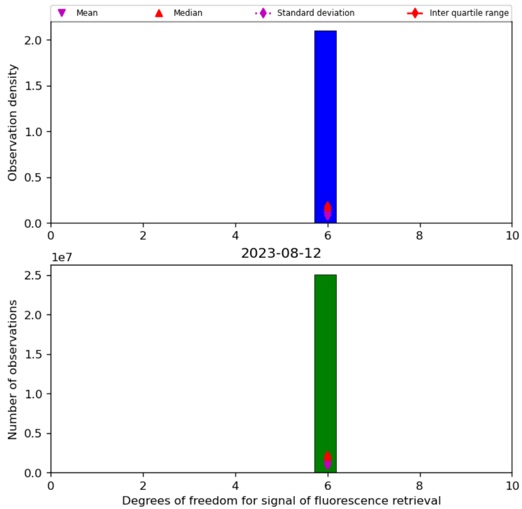
Figure 43: Histogram of “Degrees of freedom for signal of fluorescence retrieval” for 2023-08-11 to 2023-08-13
