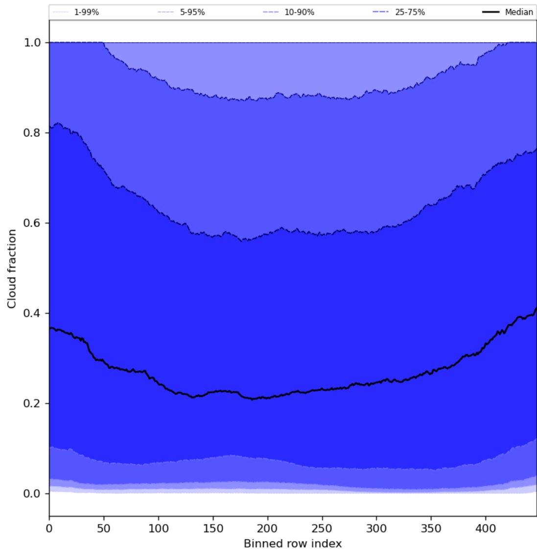
Figure 49: Along track statistics of “Cloud fraction” for 2023-08-11 to 2023-08-13
