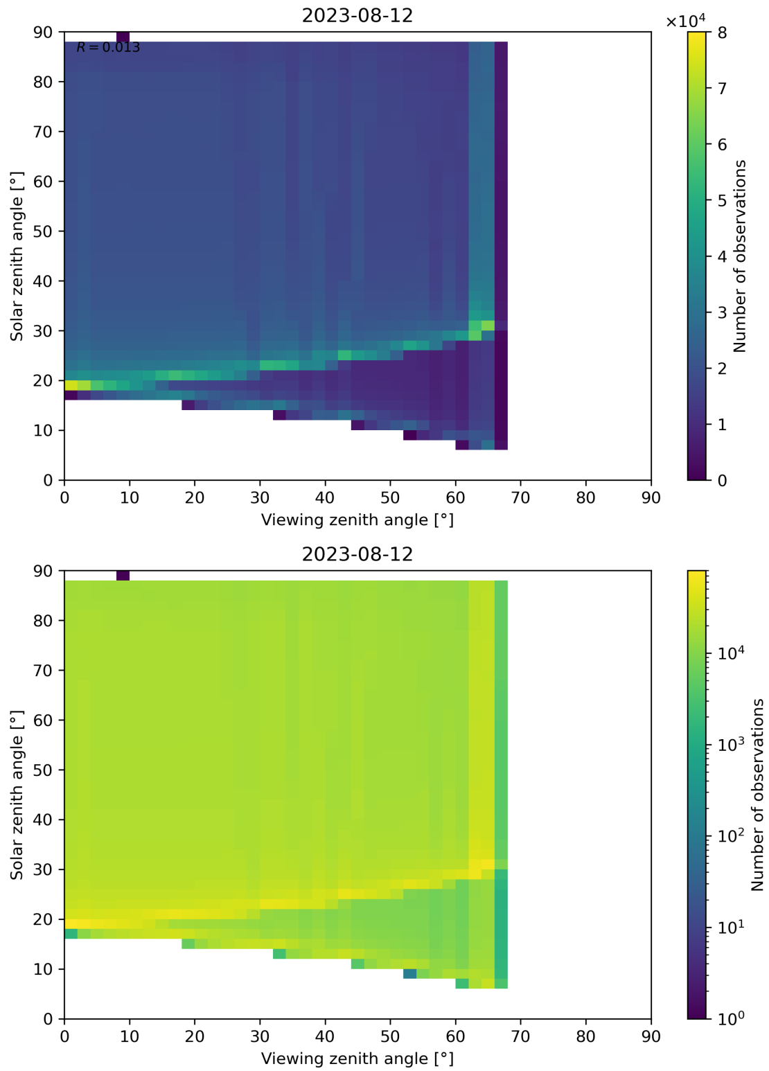
Figure 139: Scatter density plot of “Viewing zenith angle” against “Solar zenith angle” for 2023-08-11 to 2023-08-13.
