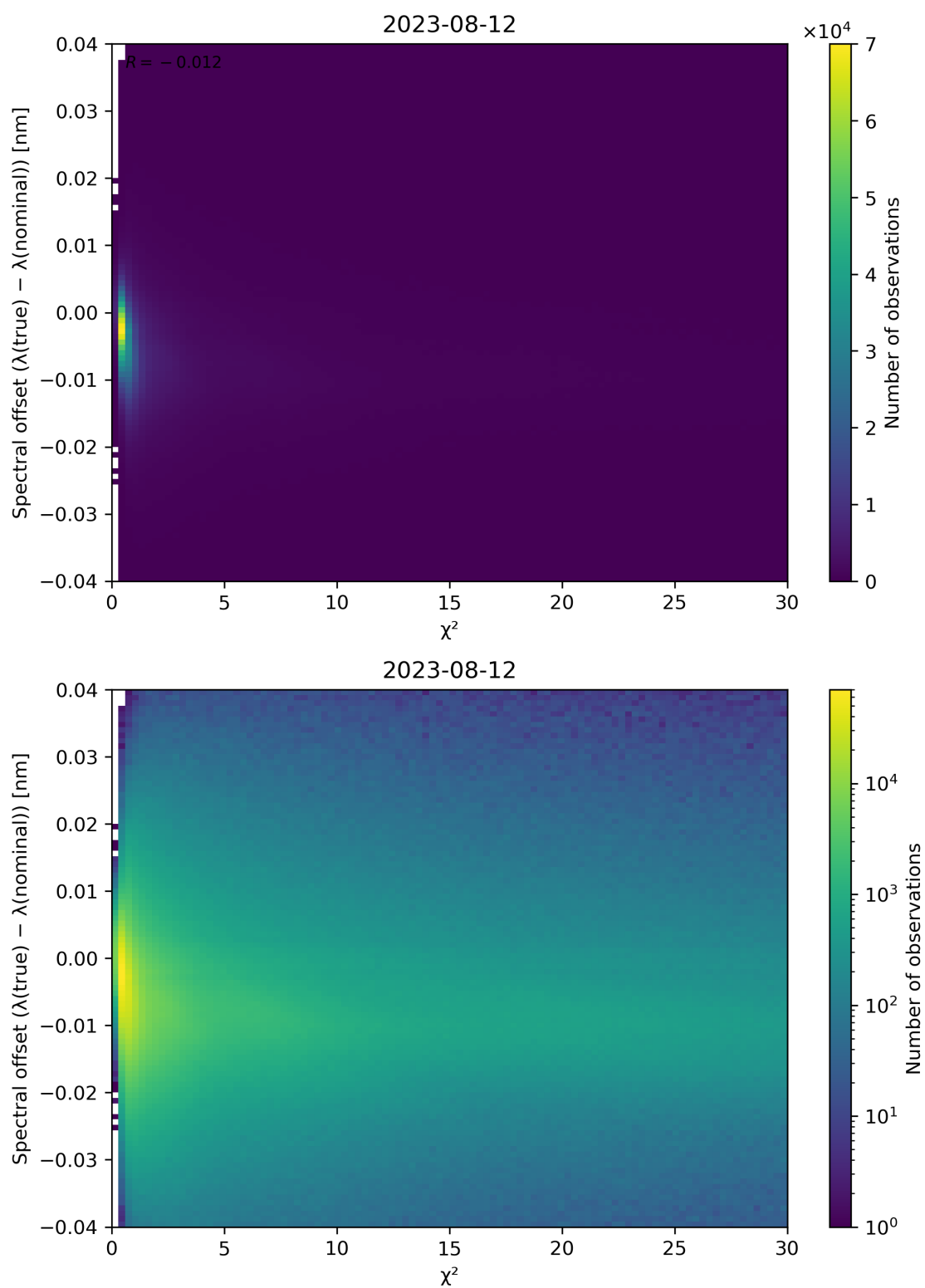
Figure 75: Scatter density plot of " \chi^2 " against "Spectral offset ( \lambda(\text{true}) - \lambda(\text{nominal}) )" for 2023-08-11 to 2023-08-13.
