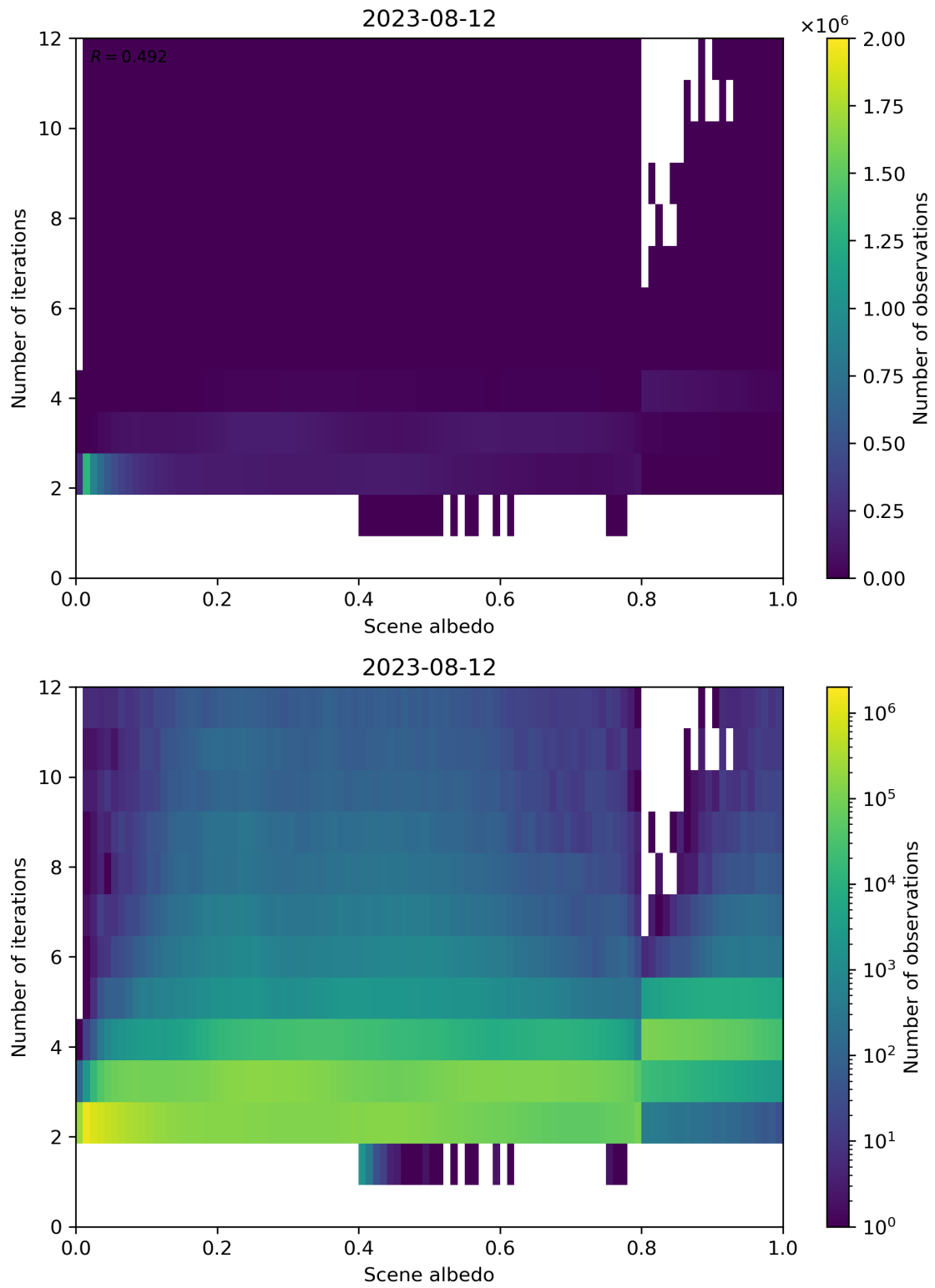
Figure 115: Scatter density plot of “Scene albedo” against “Number of iterations” for 2023-08-11 to 2023-08-13.
