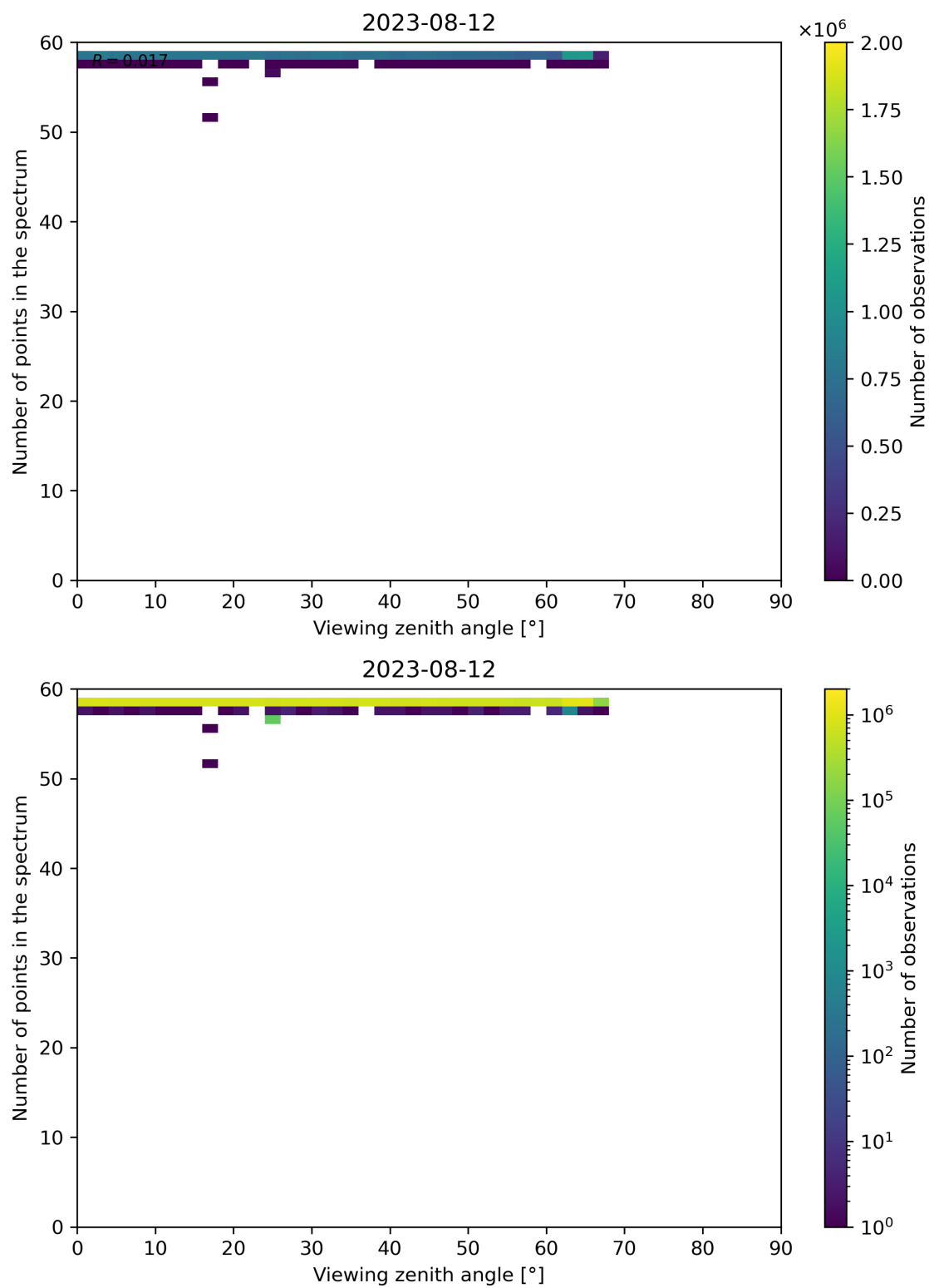
Figure 137: Scatter density plot of “Viewing zenith angle” against “Number of points in the spectrum” for 2023-08-11 to 2023-08-13.
