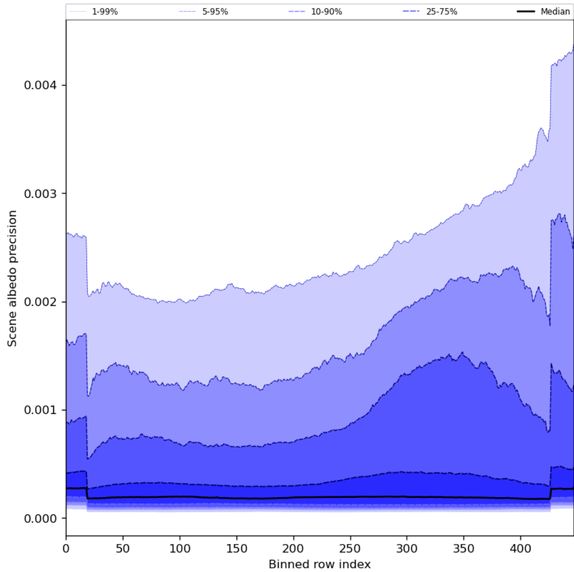
Figure 52: Along track statistics of “Scene albedo precision” for 2023-08-11 to 2023-08-13
