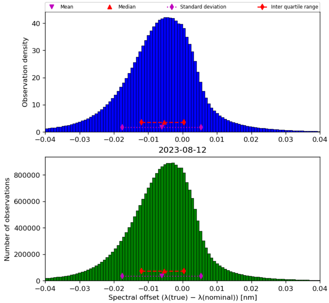
Figure 45: Histogram of “Spectral offset ( \lambda(\text{true}) - \lambda(\text{nominal}) )” for 2023-08-11 to 2023-08-13
