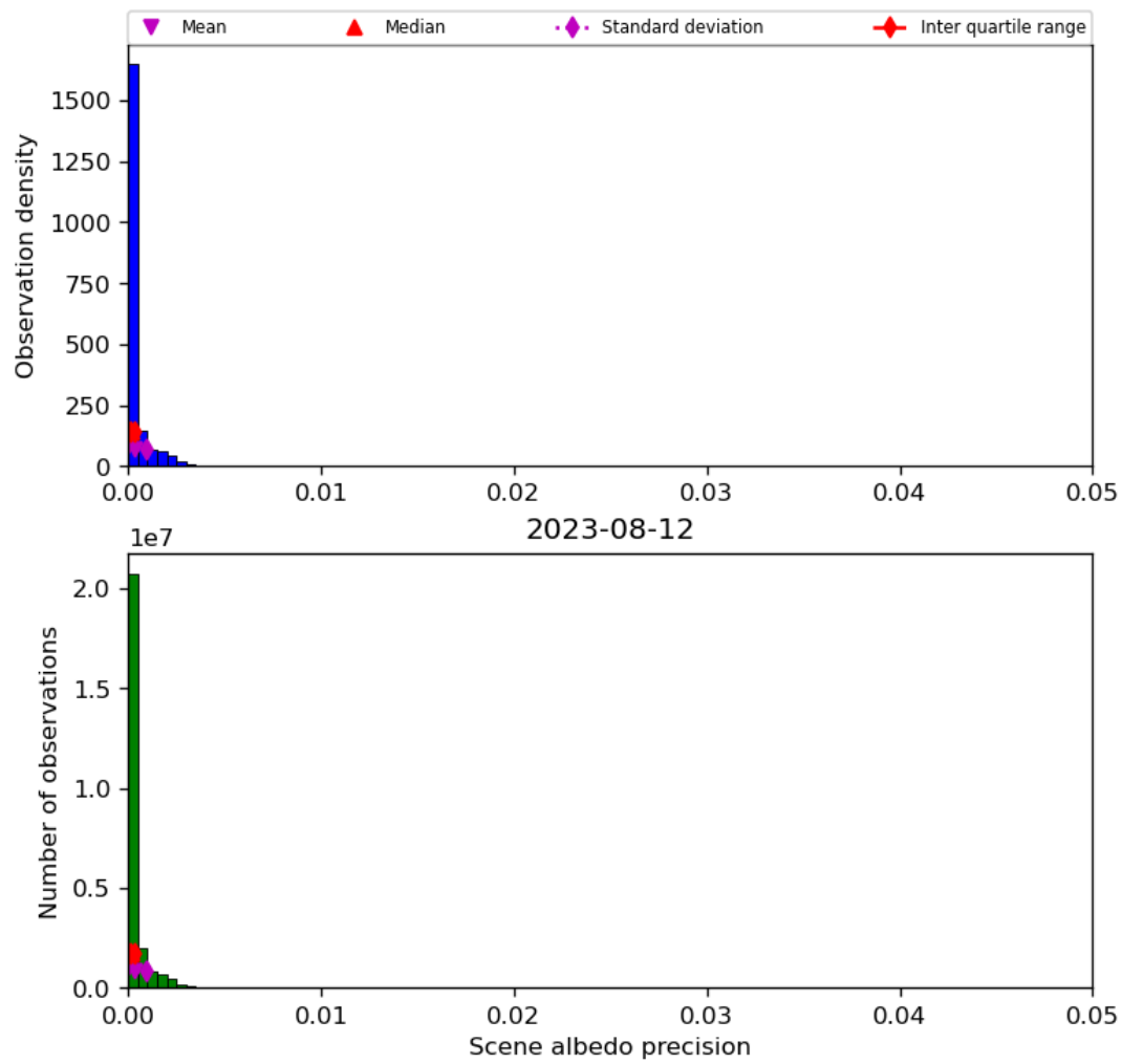
Figure 35: Histogram of “Scene albedo precision” for 2023-08-11 to 2023-08-13
