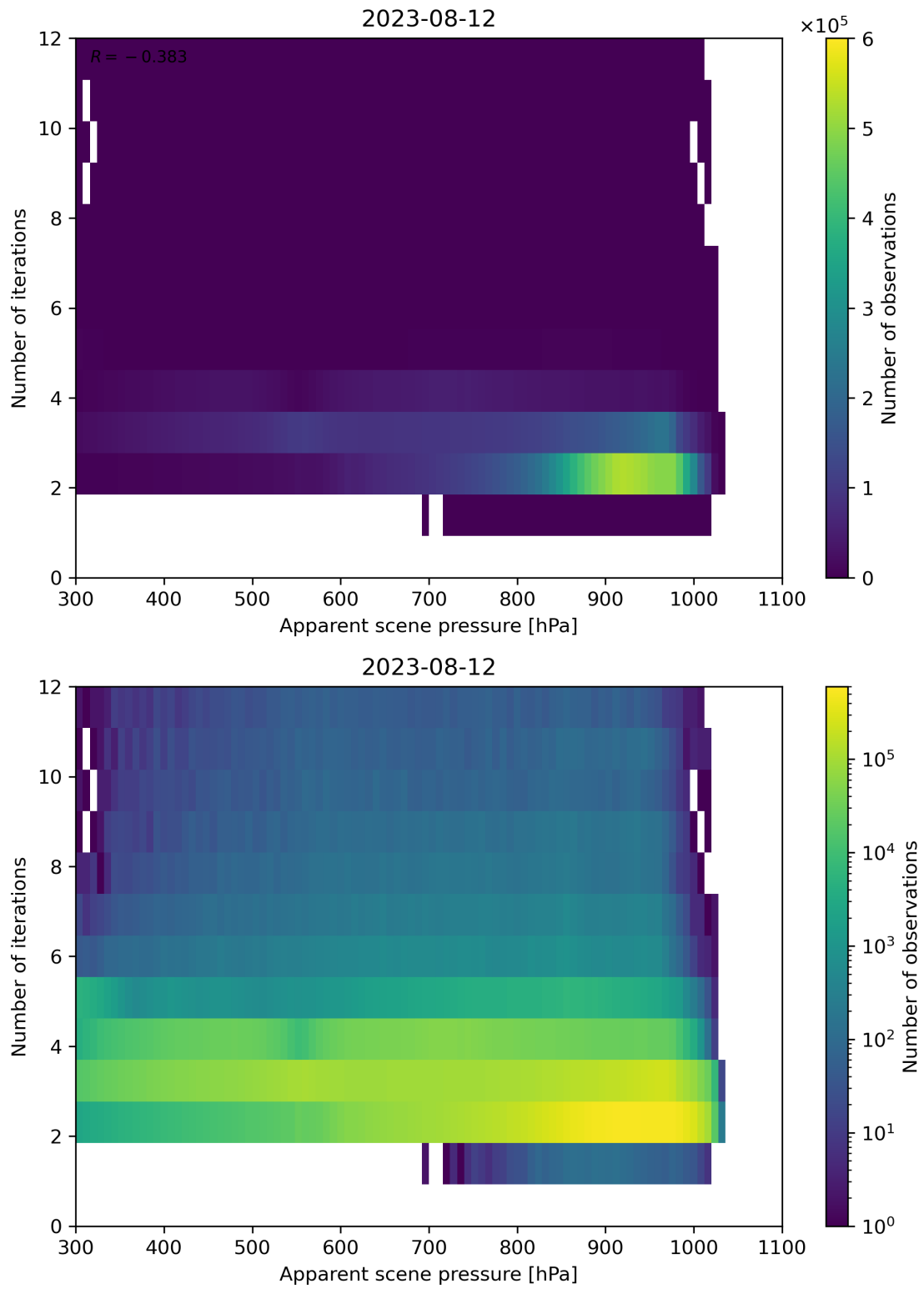
Figure 66: Scatter density plot of “Apparent scene pressure” against “Number of iterations” for 2023-08-11 to 2023-08-13.
