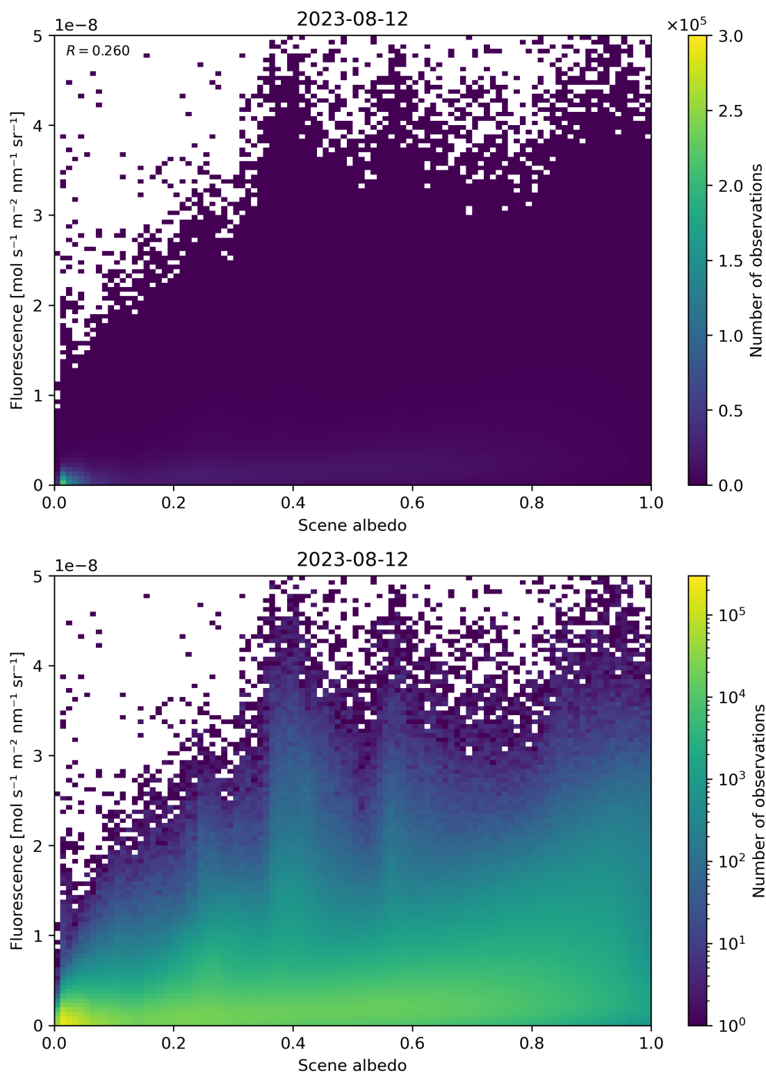
Figure 114: Scatter density plot of “Scene albedo” against “Fluorescence” for 2023-08-11 to 2023-08-13.
