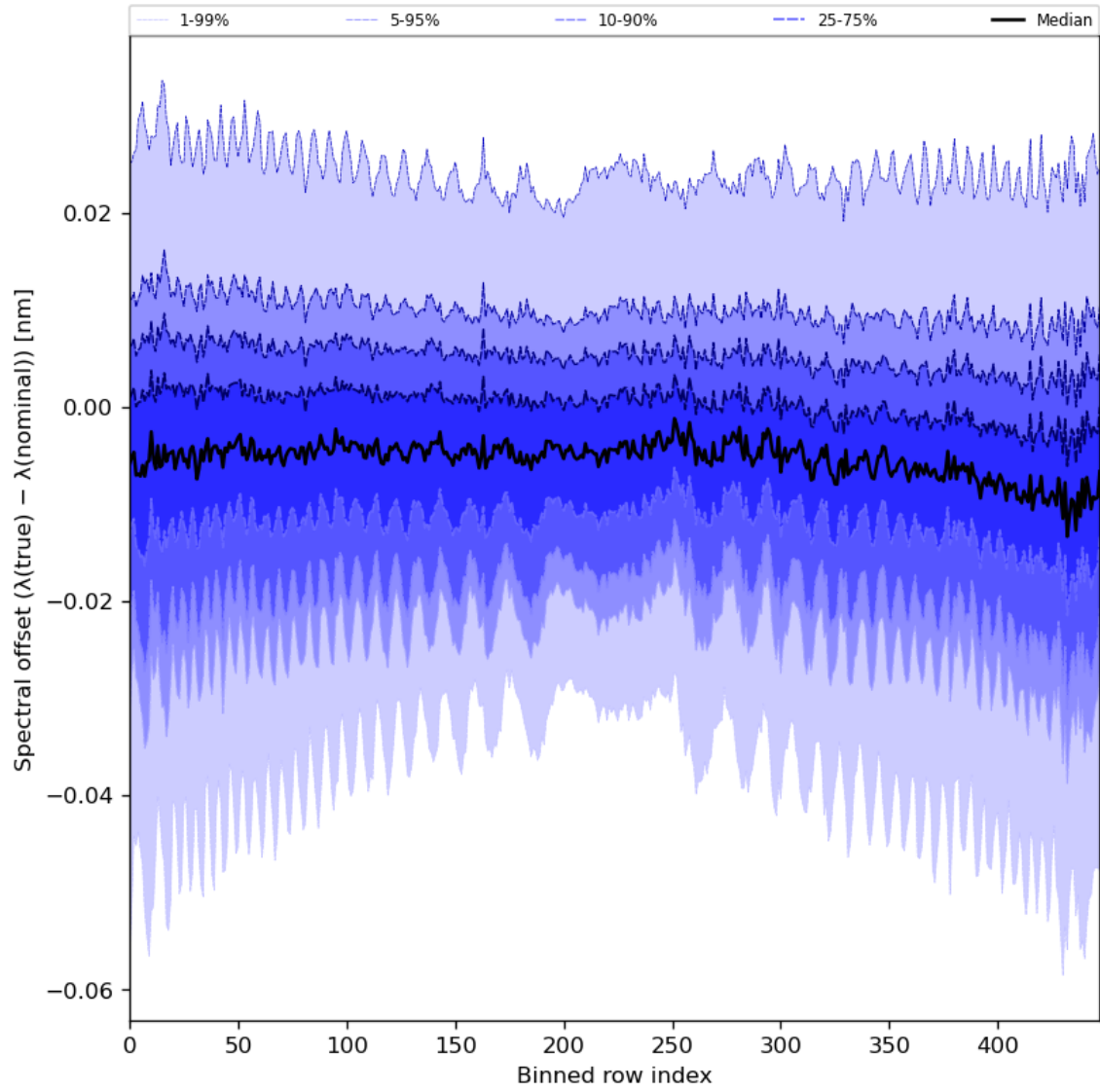
Figure 62: Along track statistics of “Spectral offset ( \lambda(\text{true}) - \lambda(\text{nominal}) )” for 2023-08-11 to 2023-08-13
