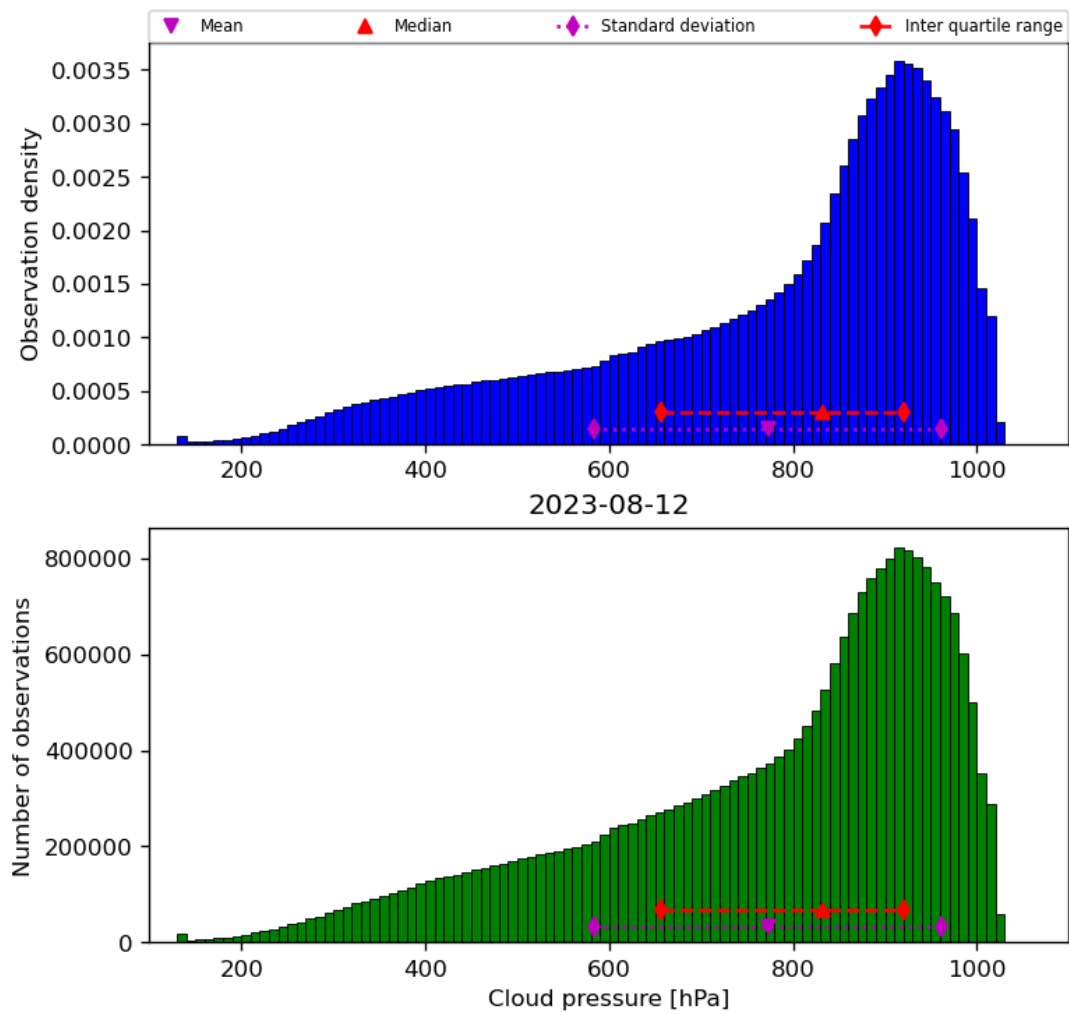
Figure 30: Histogram of “Cloud pressure” for 2023-08-11 to 2023-08-13
