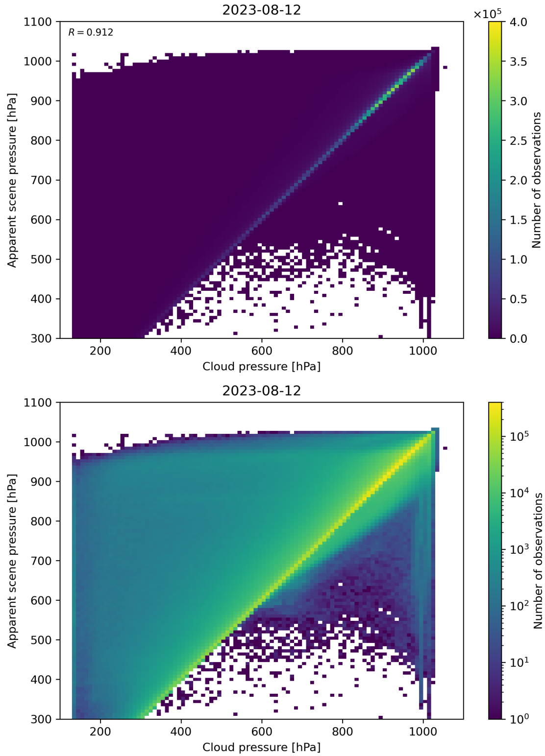
Figure 84: Scatter density plot of “Cloud pressure” against “Apparent scene pressure” for 2023-08-11 to 2023-08-13.
