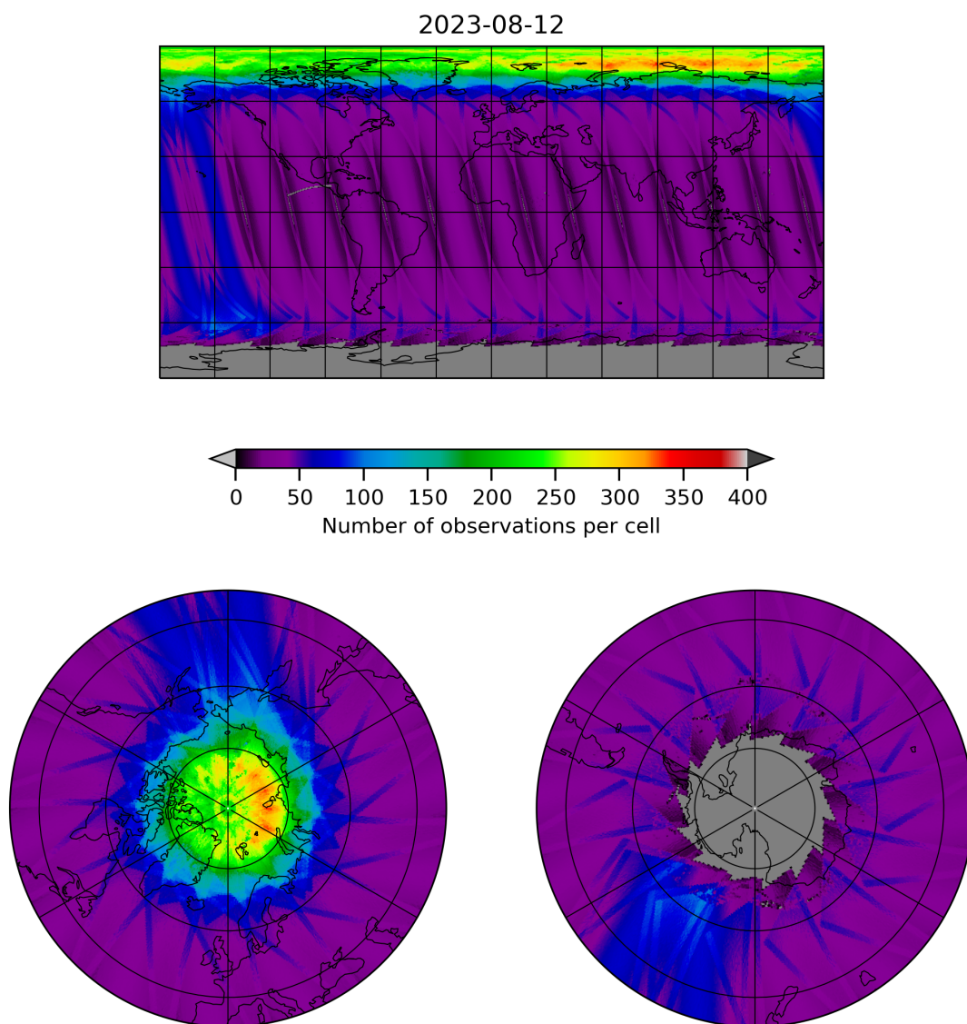
Figure 11: Map of the number of observations for 2023-08-11 to 2023-08-13
