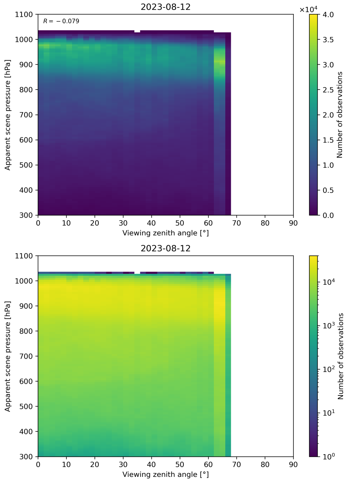
Figure 129: Scatter density plot of “Viewing zenith angle” against “Apparent scene pressure” for 2023-08-11 to 2023-08-13.
