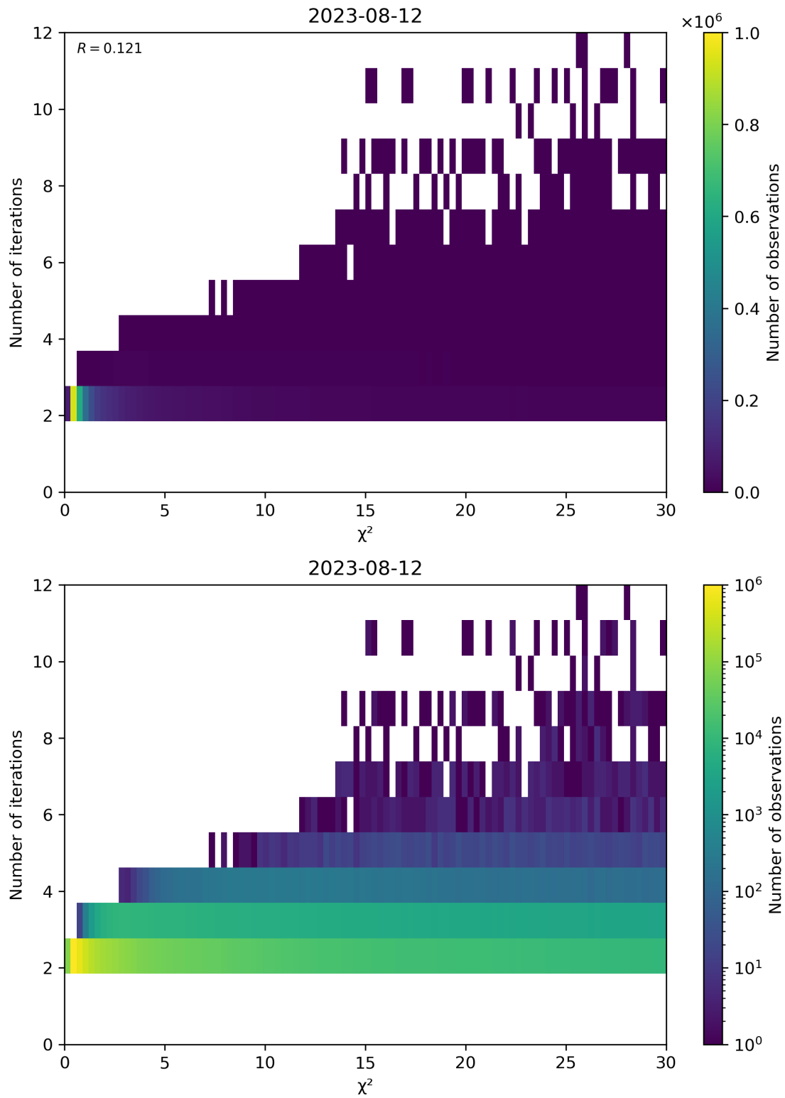
Figure 73: Scatter density plot of “ \chi^2 ” against “Number of iterations” for 2023-08-11 to 2023-08-13.
