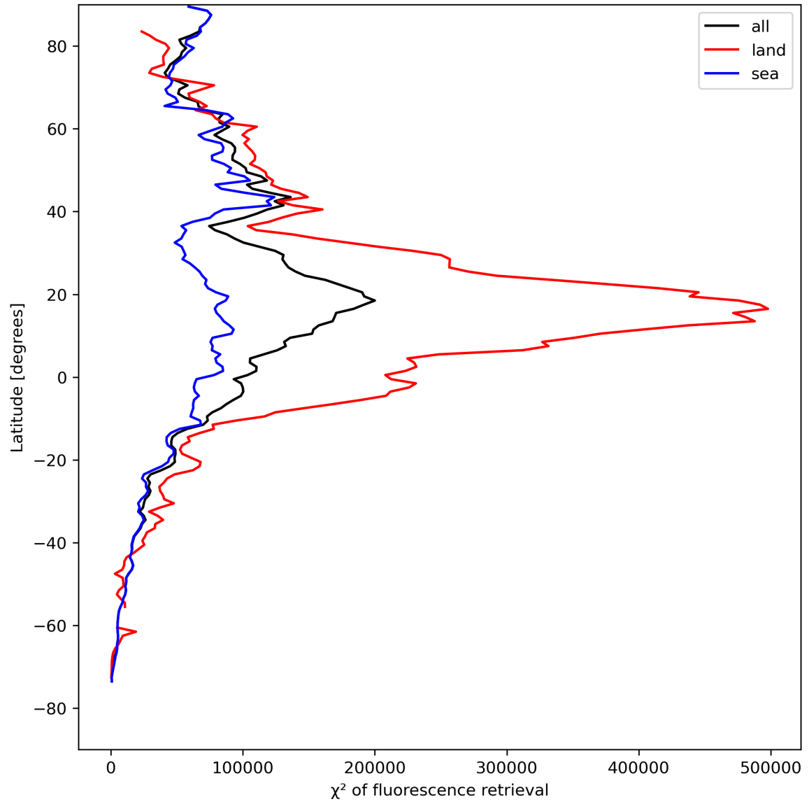
Figure 25: Zonal average of “ \chi^2 of fluorescence retrieval” for 2023-08-11 to 2023-08-13.
