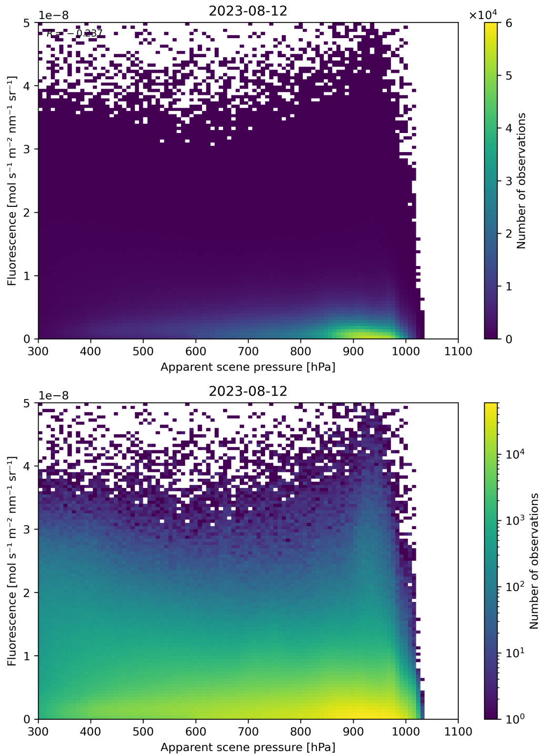
Figure 65: Scatter density plot of “Apparent scene pressure” against “Fluorescence” for 2023-08-11 to 2023-08-13.
