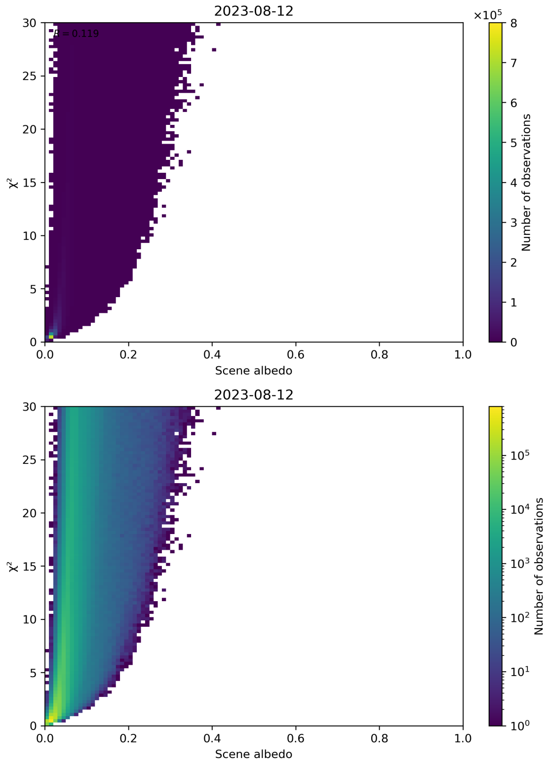
Figure 112: Scatter density plot of “Scene albedo” against “ \chi^2 ” for 2023-08-11 to 2023-08-13.
