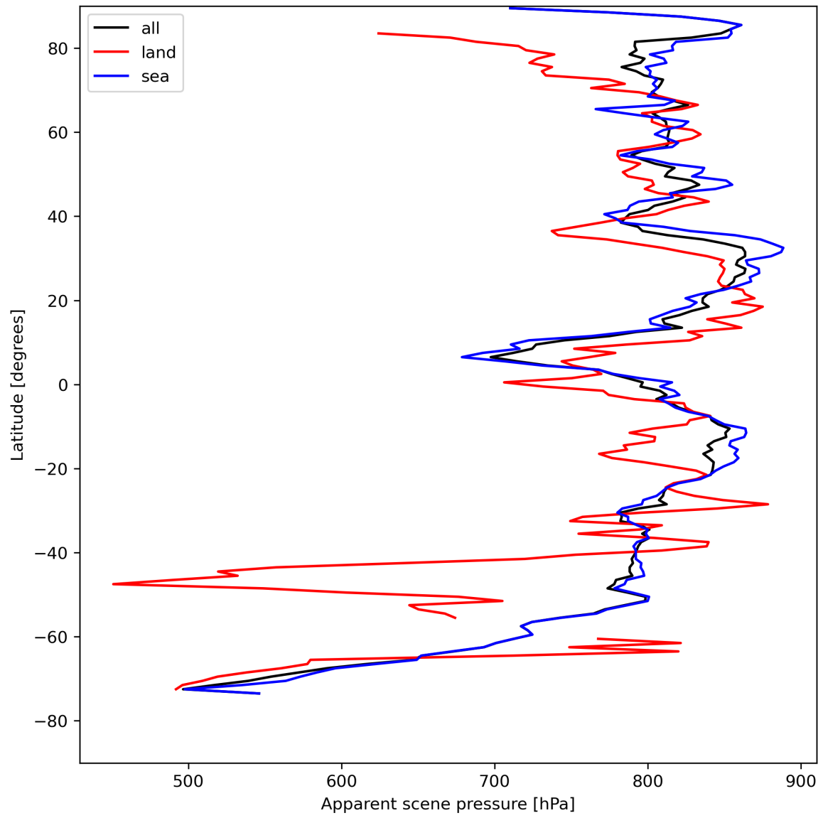
Figure 19: Zonal average of “Apparent scene pressure” for 2023-08-11 to 2023-08-13.
