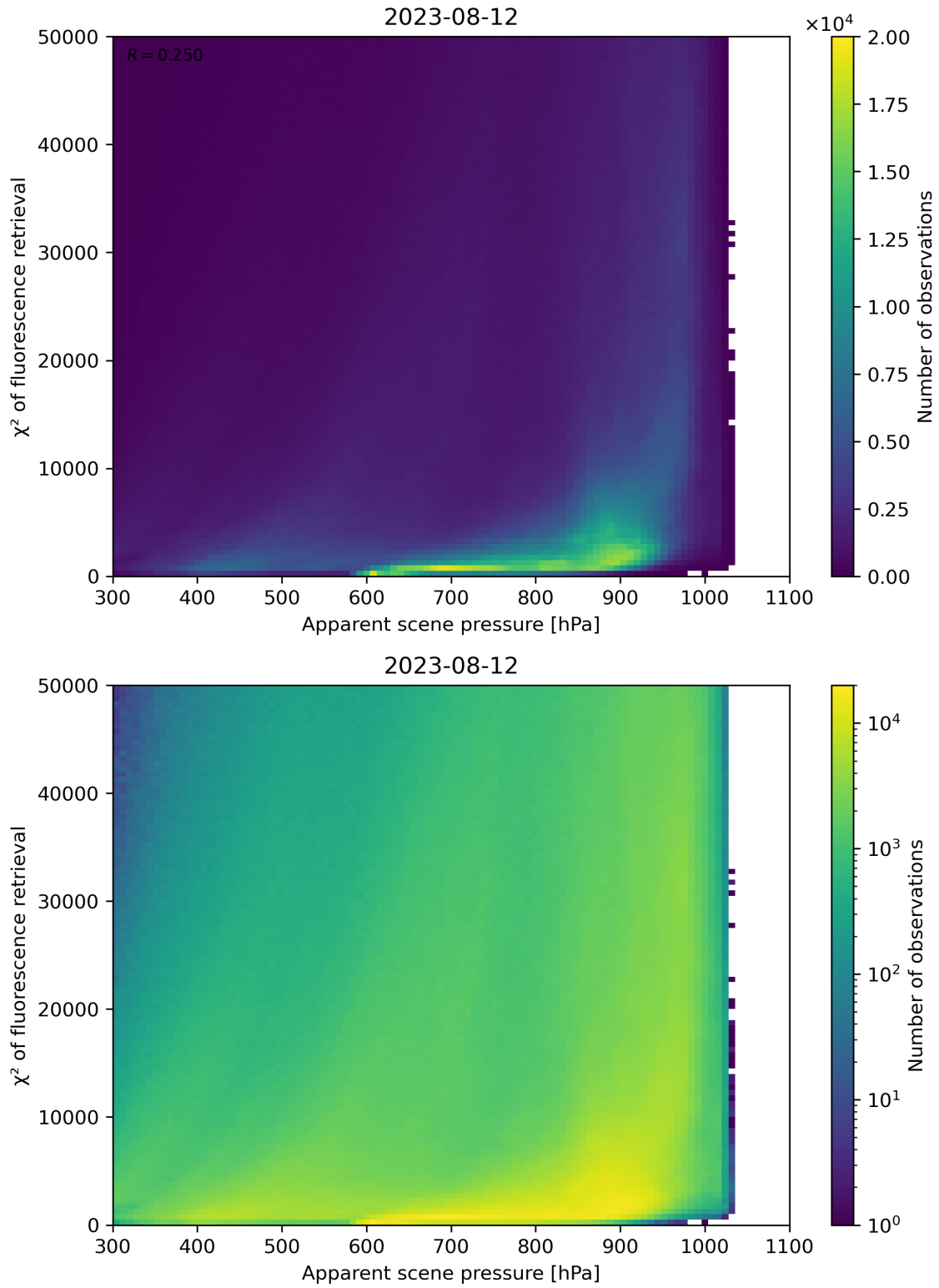
Figure 64: Scatter density plot of “Apparent scene pressure” against “ \chi^2 of fluorescence retrieval” for 2023-08-11 to 2023-08-13.
