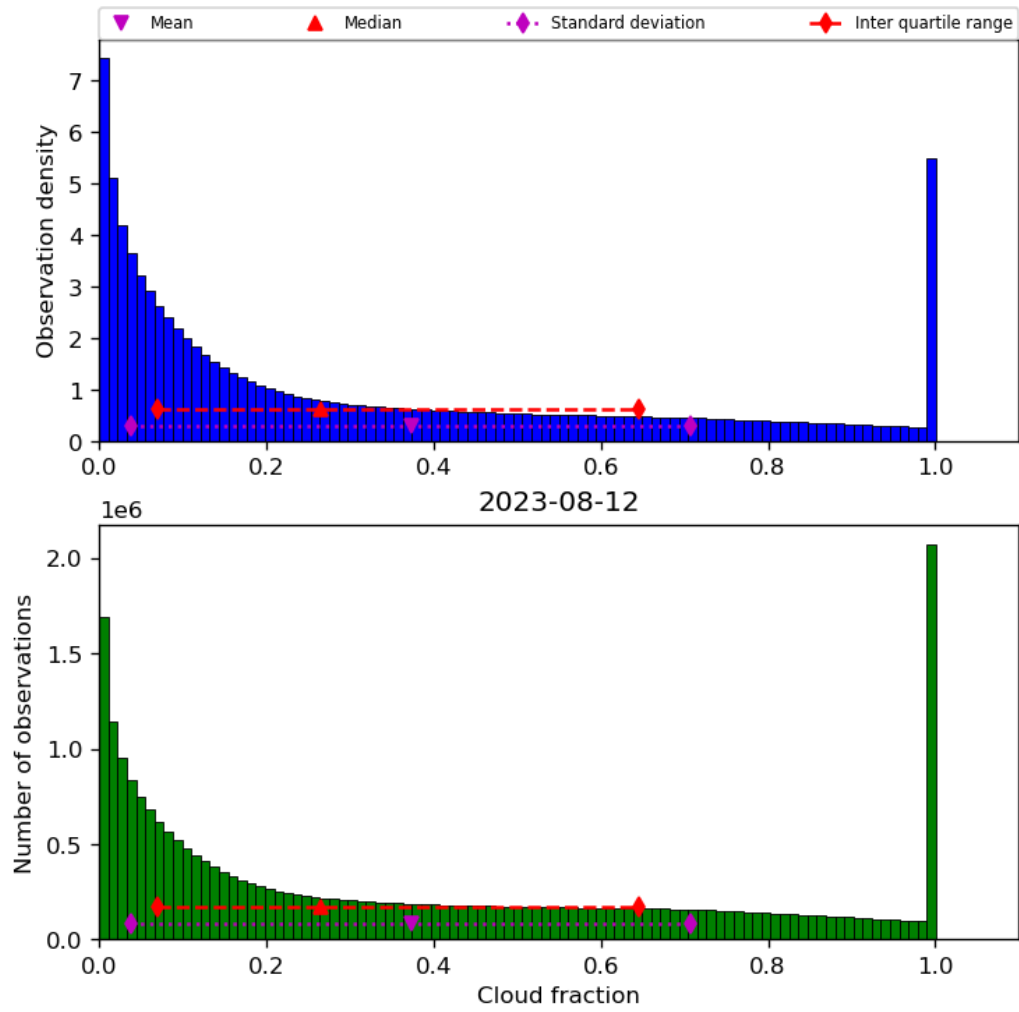
Figure 32: Histogram of “Cloud fraction” for 2023-08-11 to 2023-08-13
