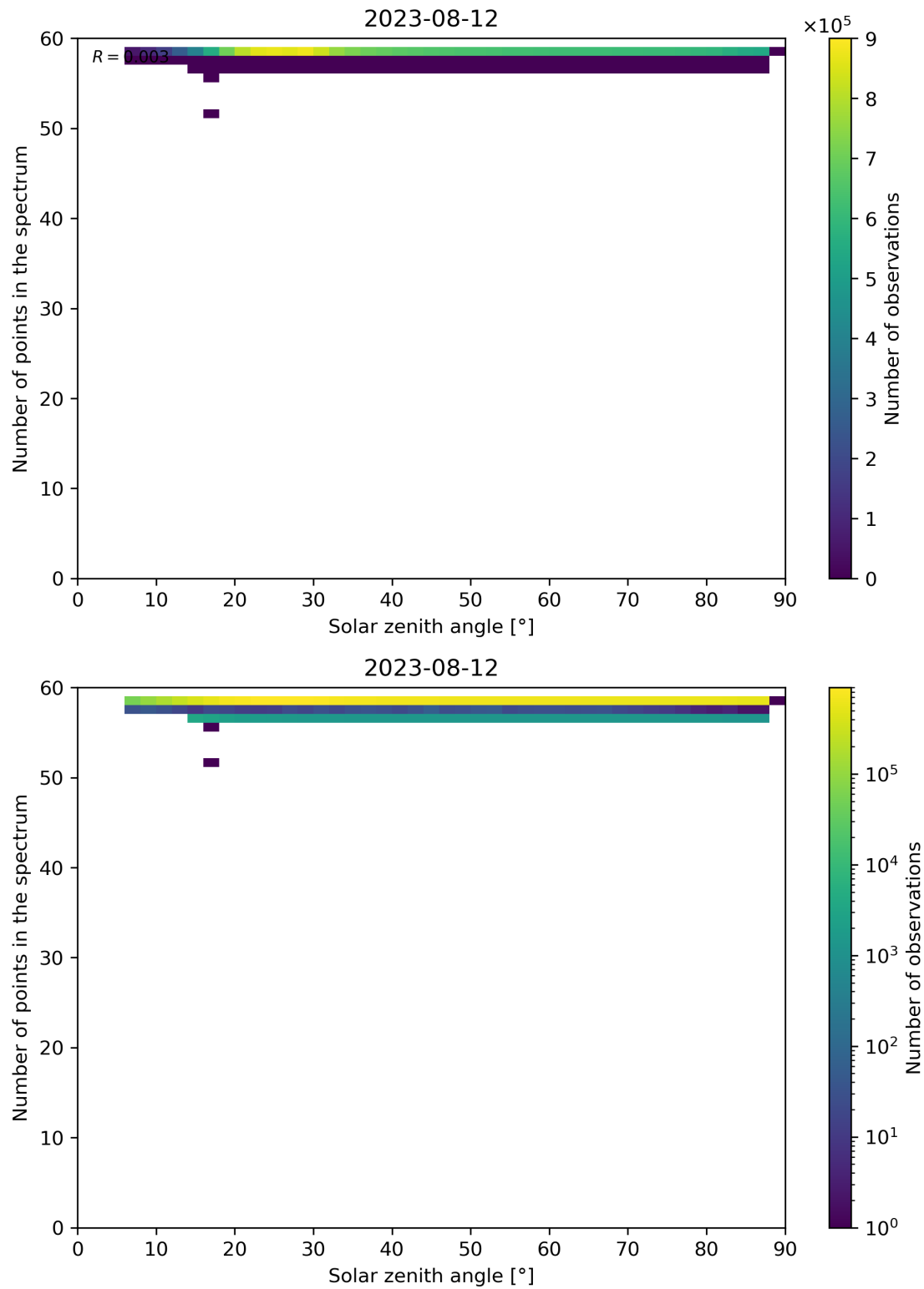
Figure 126: Scatter density plot of “Solar zenith angle” against “Number of points in the spectrum” for 2023-08-11 to 2023-08-13.
