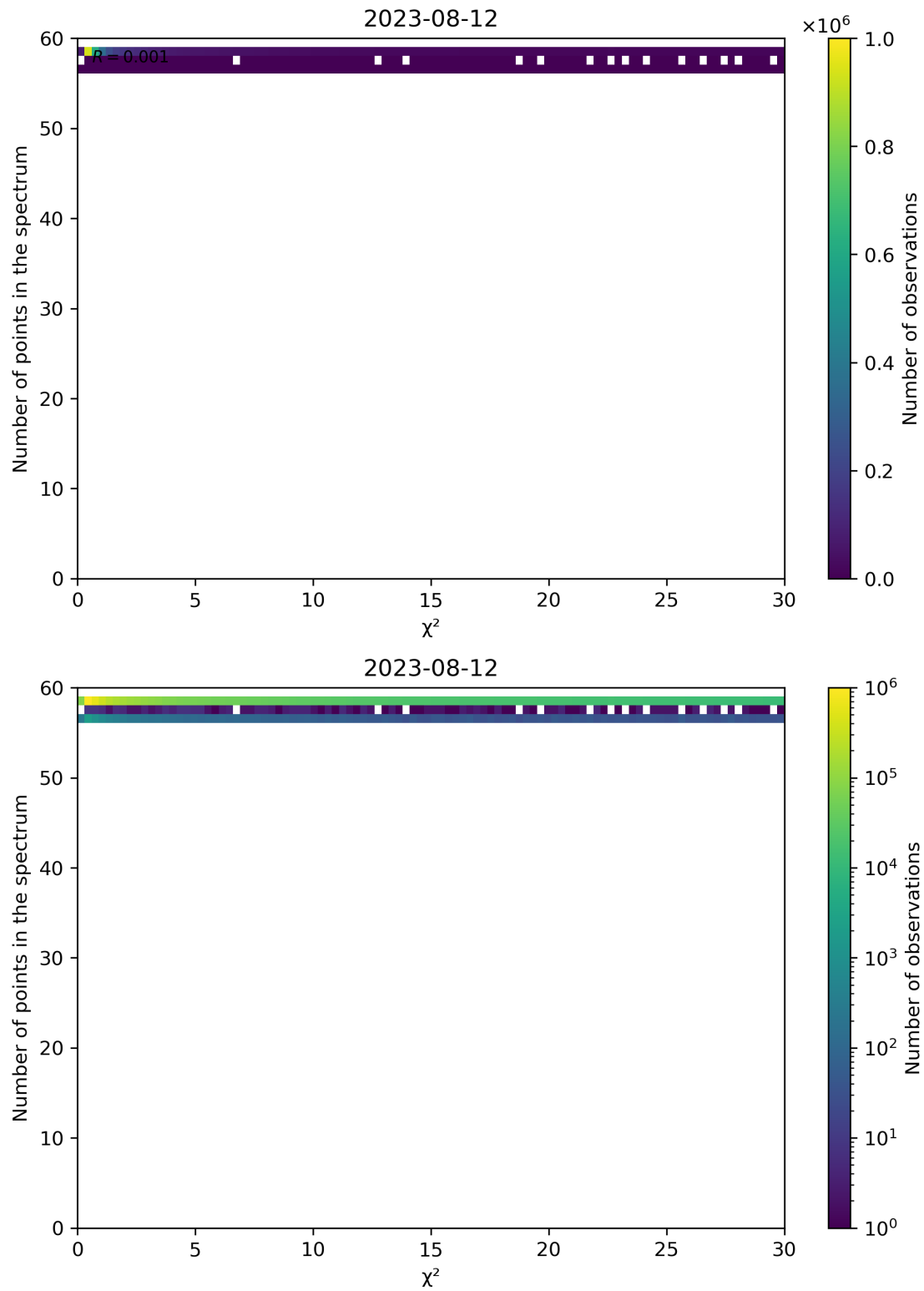
Figure 74: Scatter density plot of " \chi^2 " against "Number of points in the spectrum" for 2023-08-11 to 2023-08-13.
