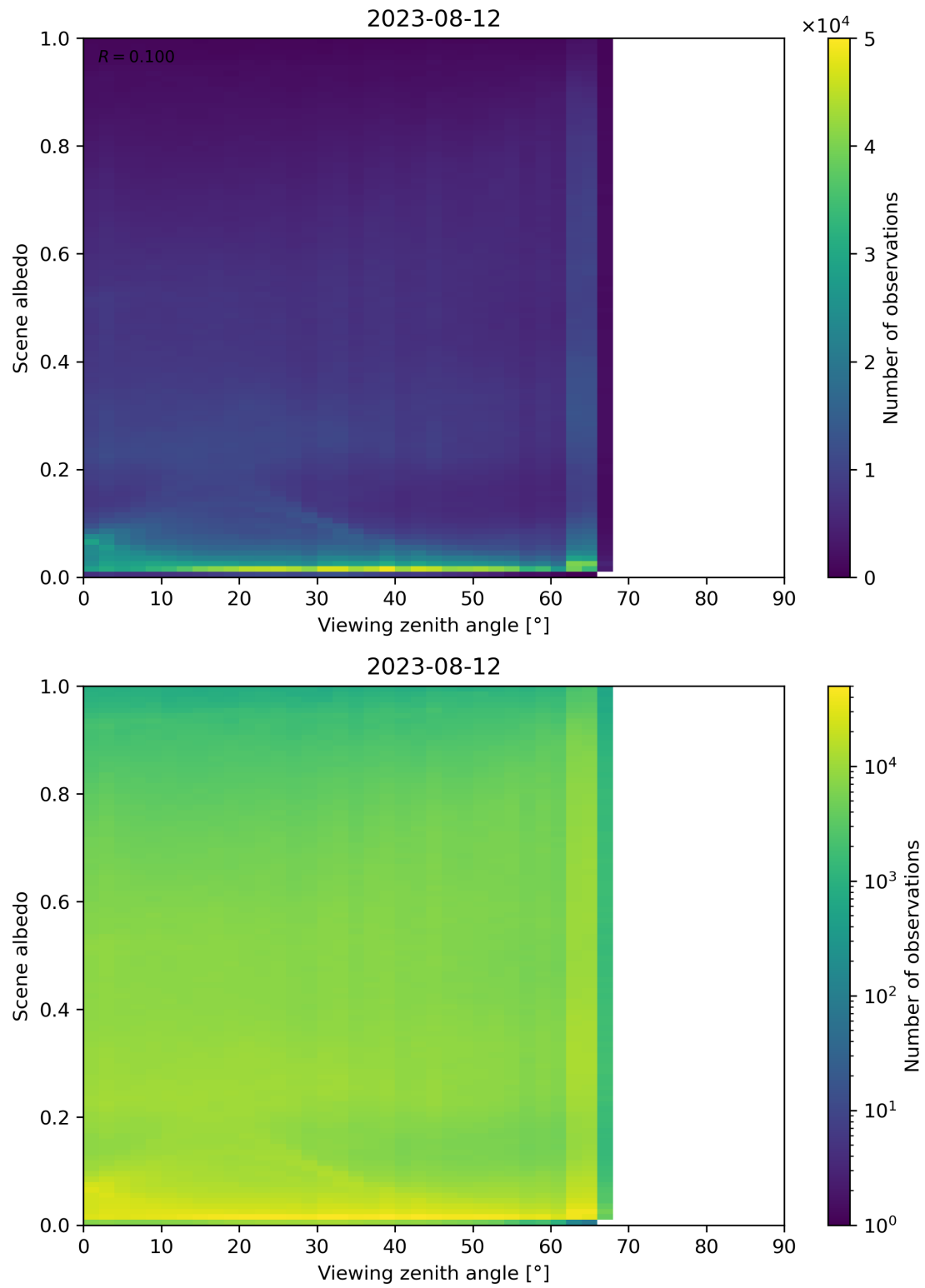
Figure 138: Scatter density plot of “Viewing zenith angle” against “Scene albedo” for 2023-08-11 to 2023-08-13.
