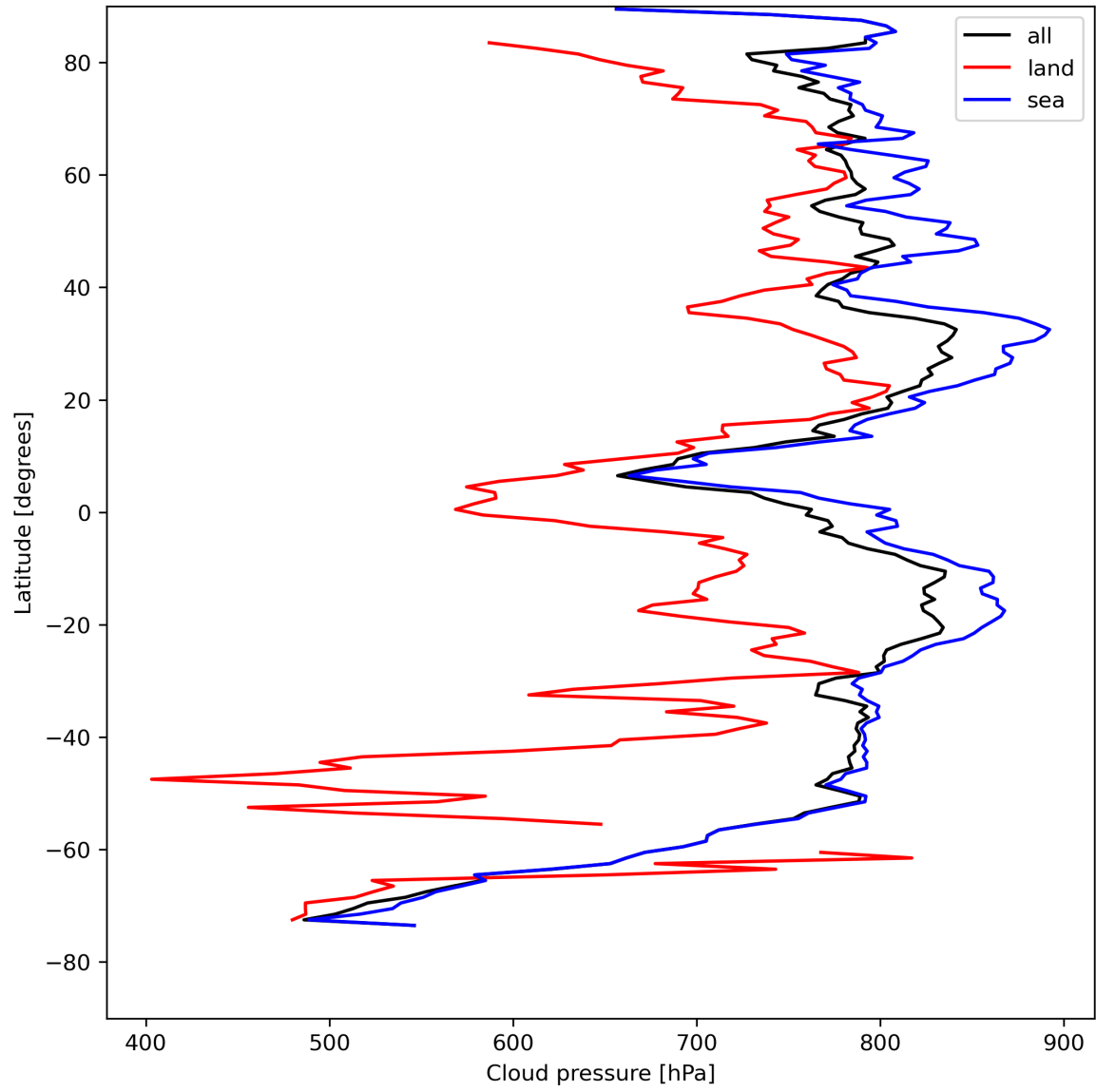
Figure 13: Zonal average of “Cloud pressure” for 2023-08-11 to 2023-08-13.
