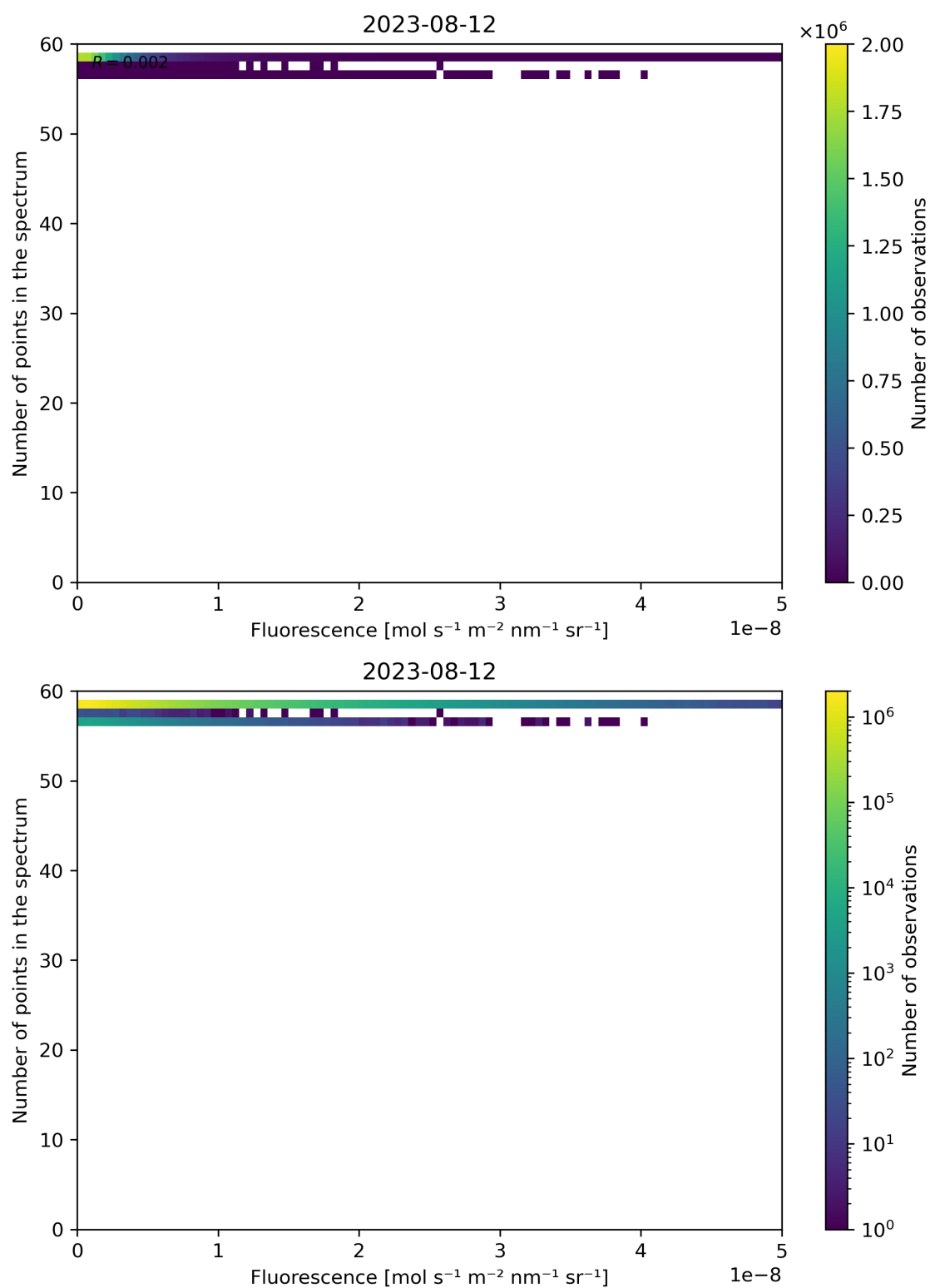
Figure 94: Scatter density plot of “Fluorescence” against “Number of points in the spectrum” for 2023-08-11 to 2023-08-13.
