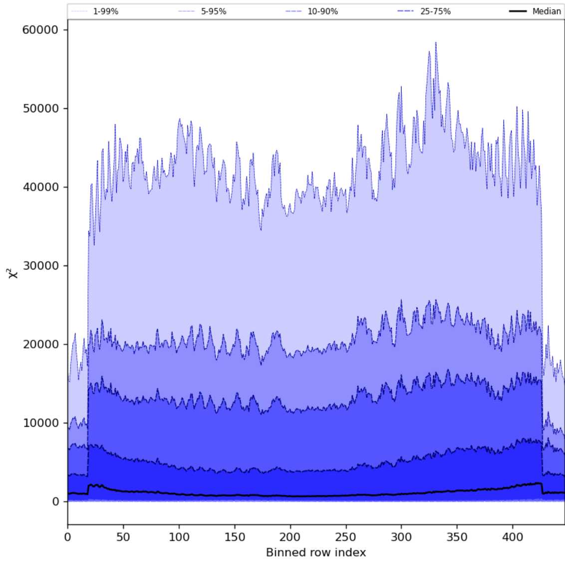
Figure 55: Along track statistics of “ \chi^2 ” for 2023-08-11 to 2023-08-13
