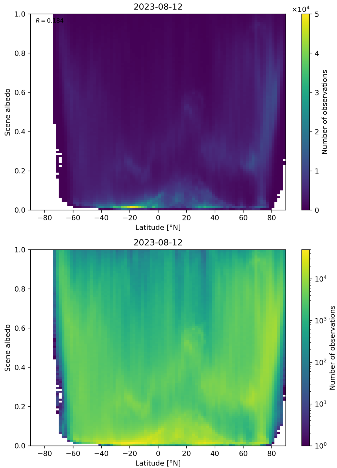
Figure 104: Scatter density plot of “Latitude” against “Scene albedo” for 2023-08-11 to 2023-08-13.
