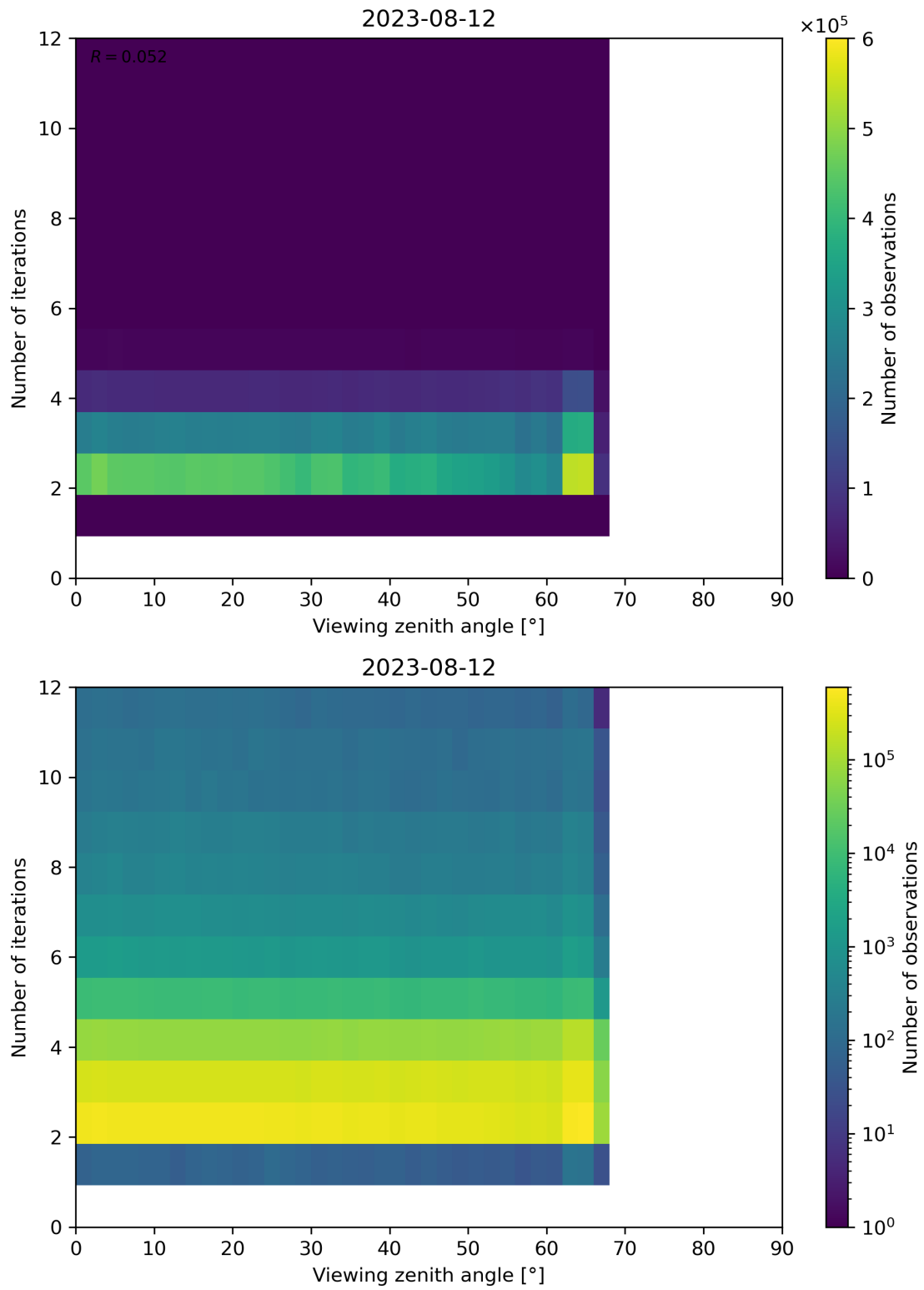
Figure 136: Scatter density plot of “Viewing zenith angle” against “Number of iterations” for 2023-08-11 to 2023-08-13.
