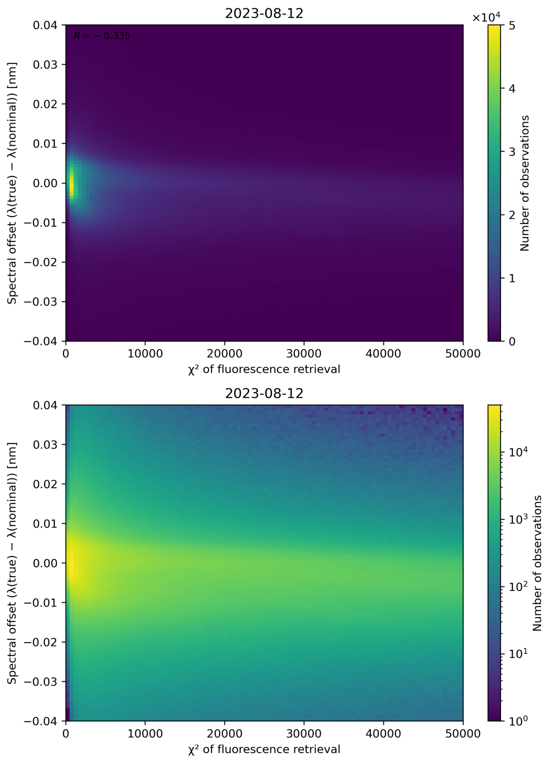
Figure 72: Scatter density plot of " \chi^2 of fluorescence retrieval" against "Spectral offset ( \lambda(\text{true}) - \lambda(\text{nominal})) " for 2023-08-11 to 2023-08-13.
