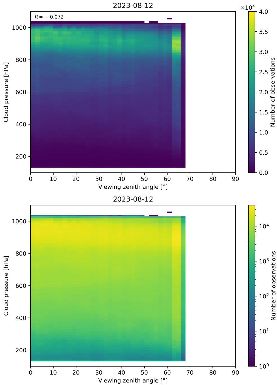
Figure 133: Scatter density plot of “Viewing zenith angle” against “Cloud pressure” for 2023-08-11 to 2023-08-13.
