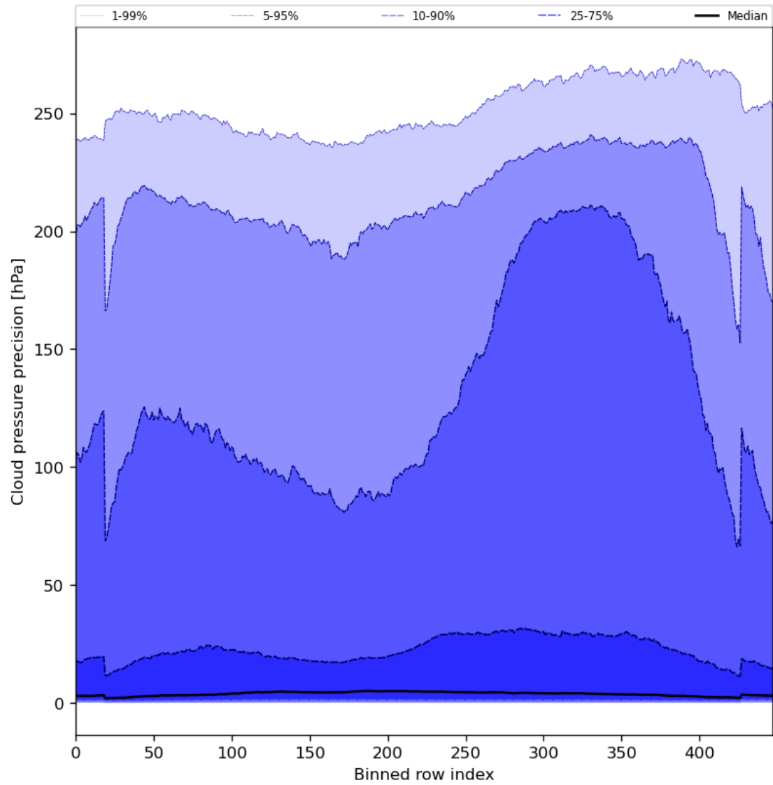
Figure 48: Along track statistics of “Cloud pressure precision” for 2023-08-11 to 2023-08-13
