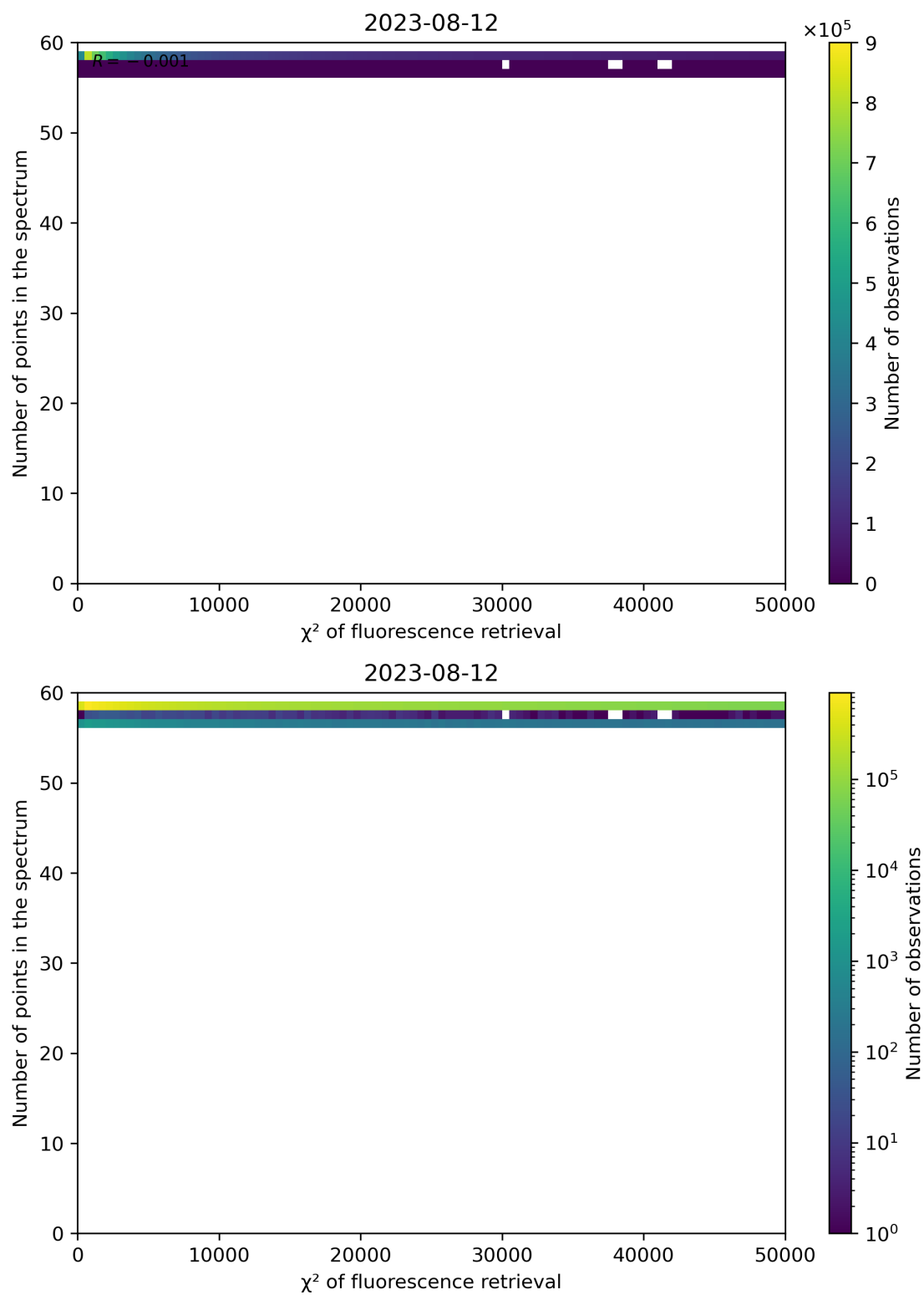
Figure 71: Scatter density plot of " \chi^2 of fluorescence retrieval" against "Number of points in the spectrum" for 2023-08-11 to 2023-08-13.
