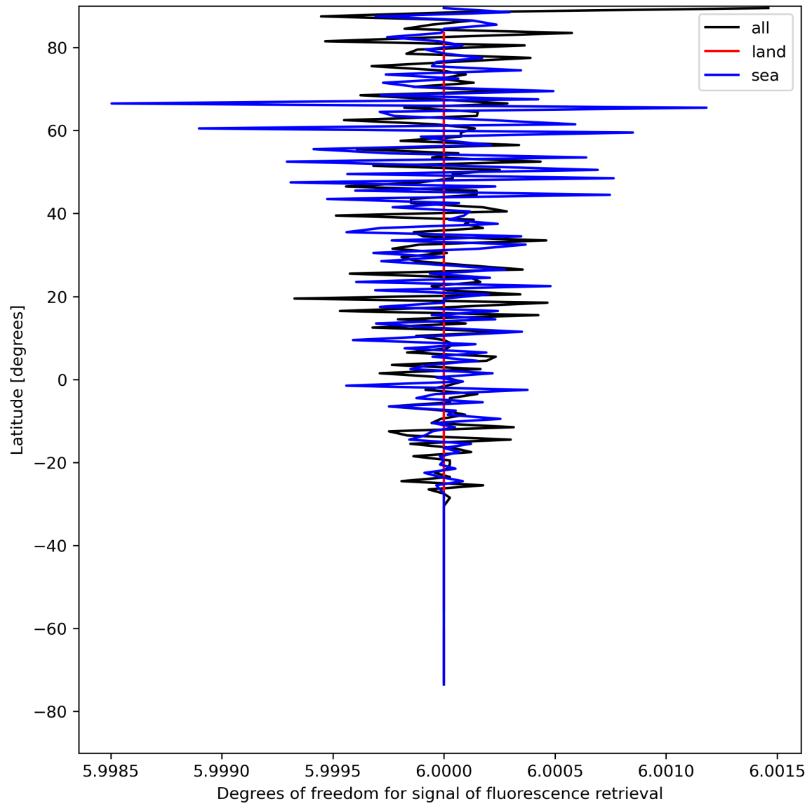
Figure 26: Zonal average of “Degrees of freedom for signal of fluorescence retrieval” for 2023-08-11 to 2023-08-13.
