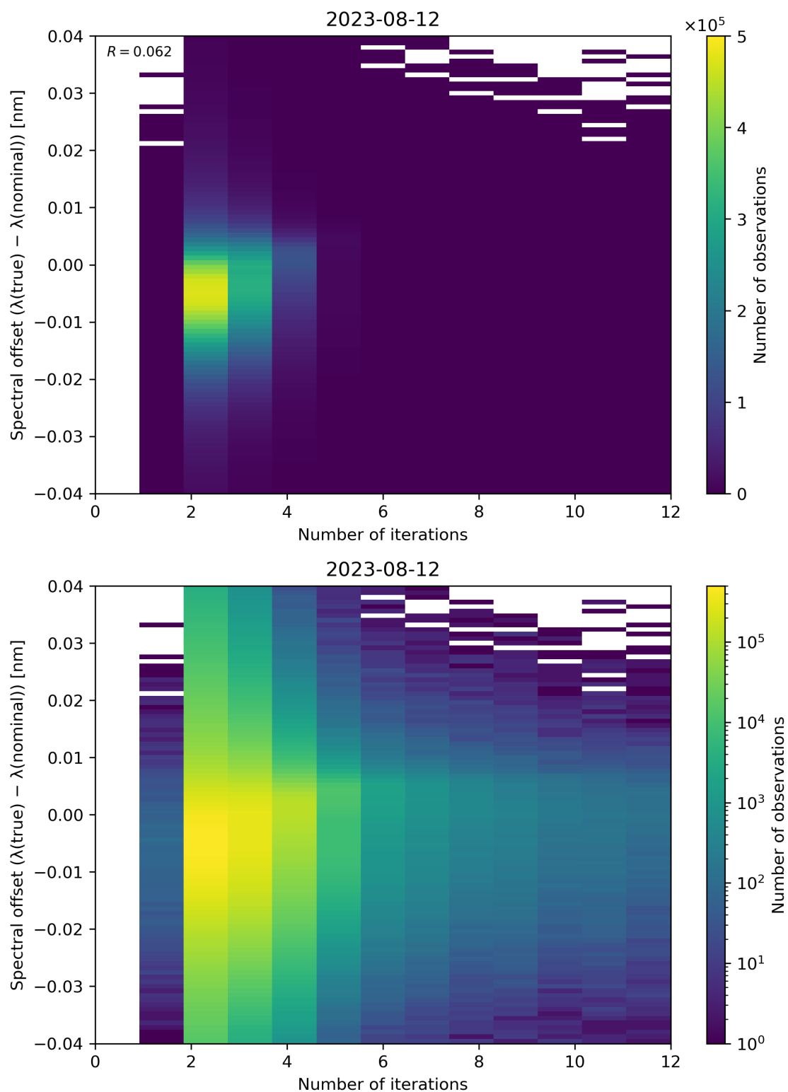
Figure 109: Scatter density plot of “Number of iterations” against “Spectral offset ( \lambda(\text{true}) - \lambda(\text{nominal}) )” for 2023-08-11 to 2023-08-13.
