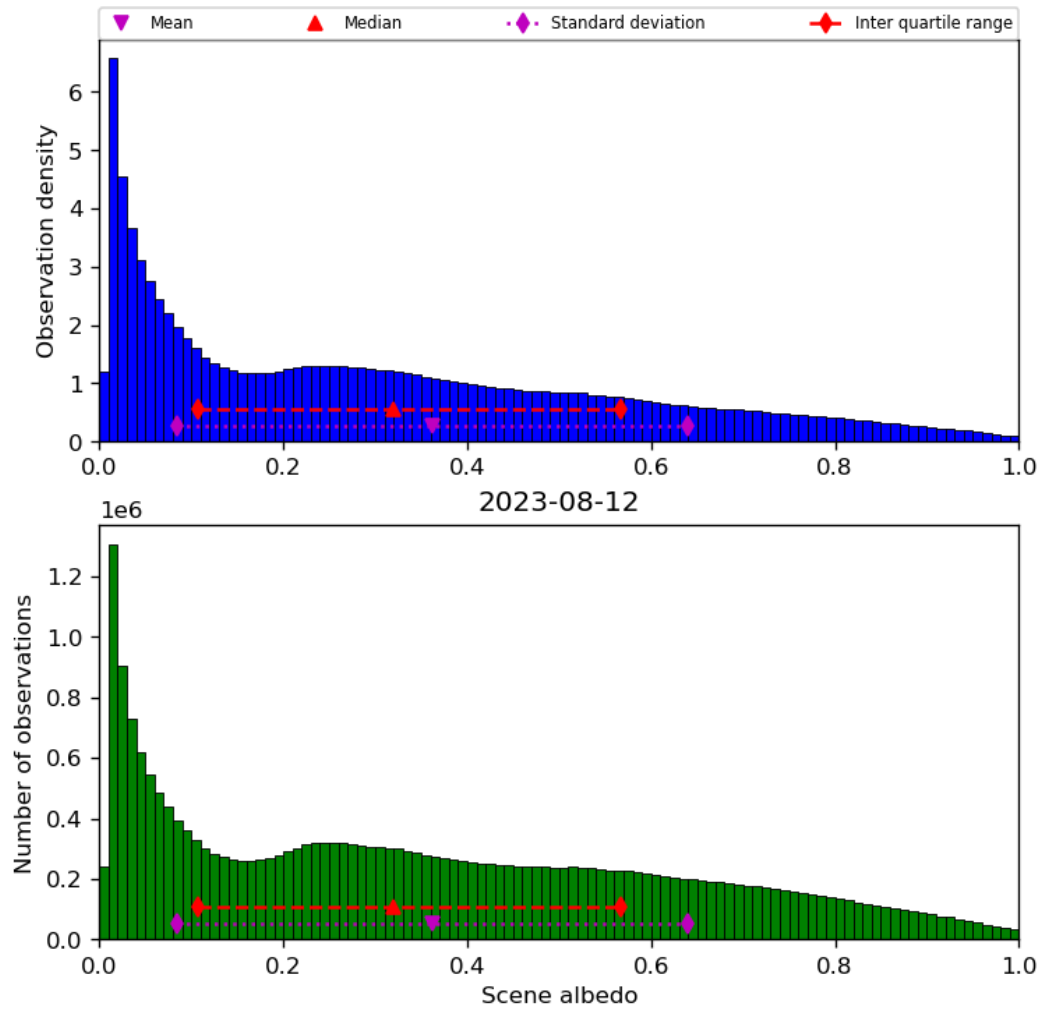
Figure 34: Histogram of “Scene albedo” for 2023-08-11 to 2023-08-13
