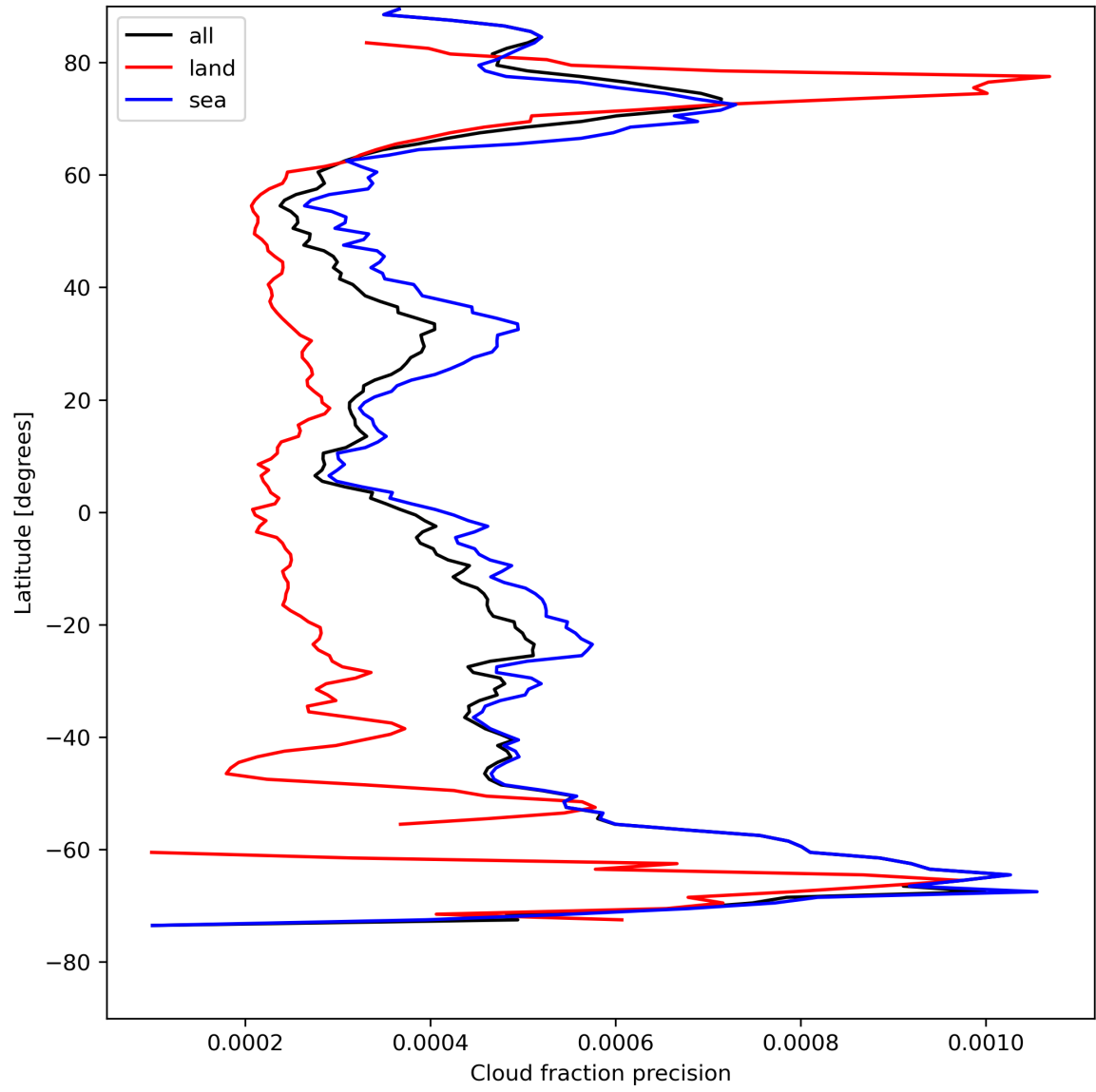
Figure 16: Zonal average of “Cloud fraction precision” for 2023-08-11 to 2023-08-13.
