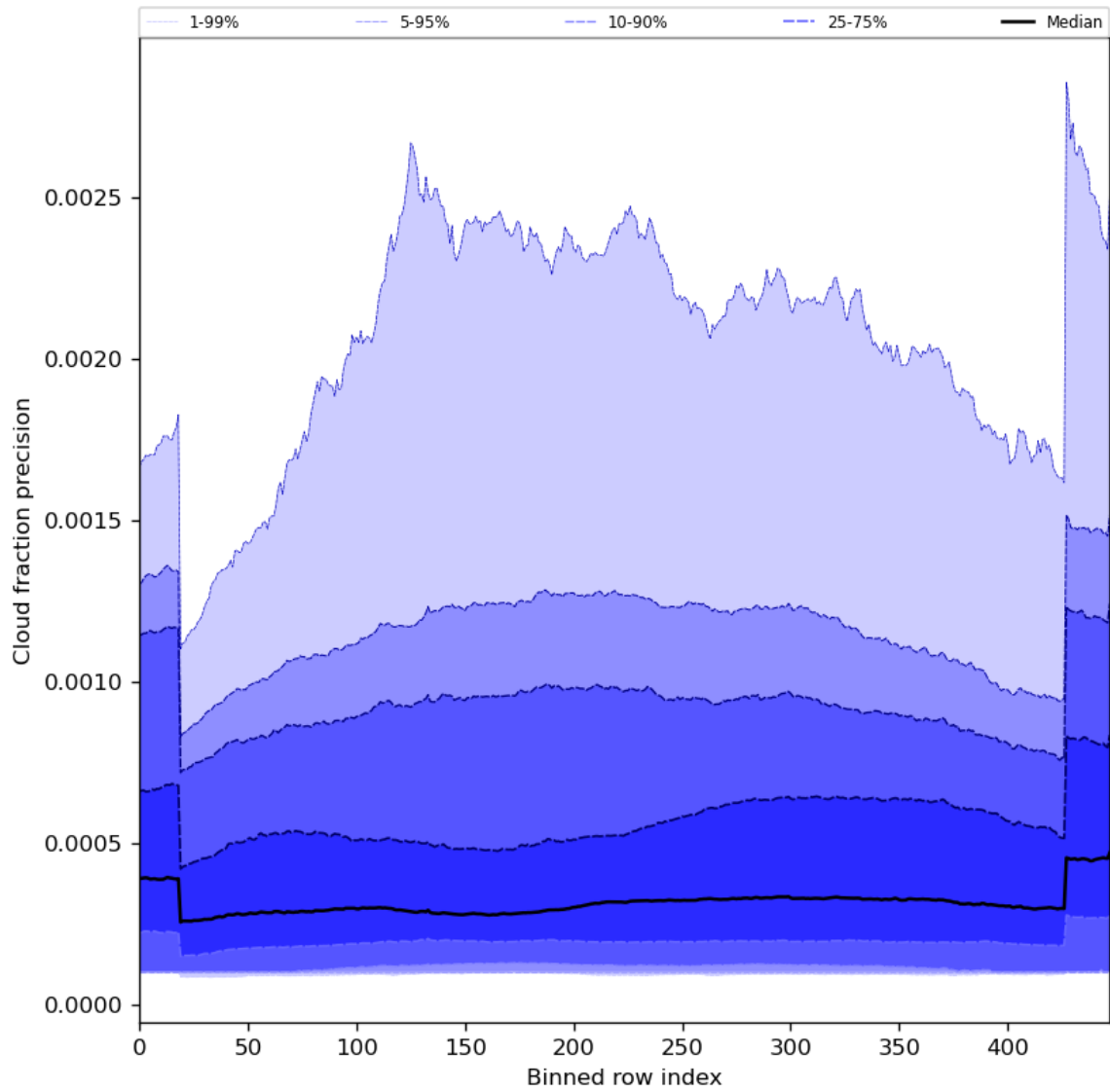
Figure 50: Along track statistics of “Cloud fraction precision” for 2023-08-11 to 2023-08-13
