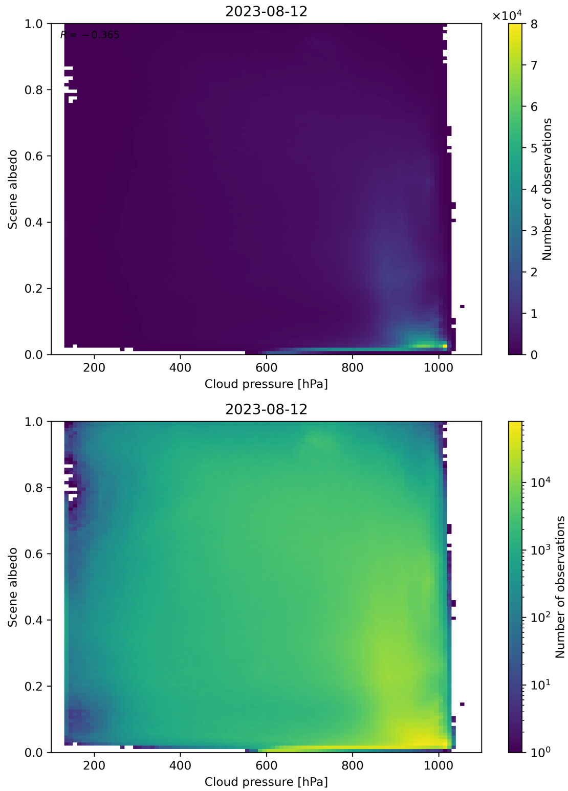
Figure 91: Scatter density plot of “Cloud pressure” against “Scene albedo” for 2023-08-11 to 2023-08-13.
