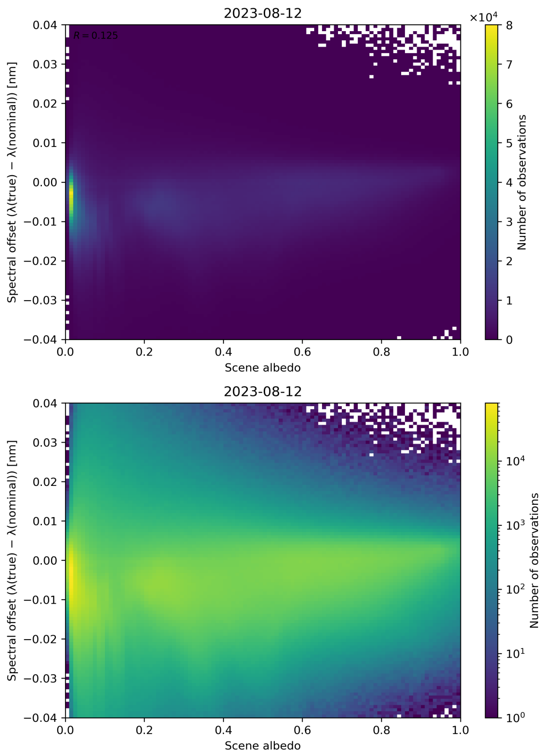
Figure 117: Scatter density plot of “Scene albedo” against “Spectral offset ( \lambda(\text{true}) - \lambda(\text{nominal}) )” for 2023-08-11 to 2023-08-13.
