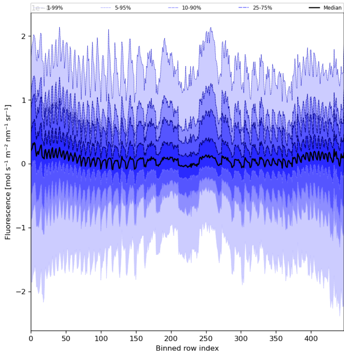
Figure 57: Along track statistics of “Fluorescence” for 2023-08-11 to 2023-08-13
