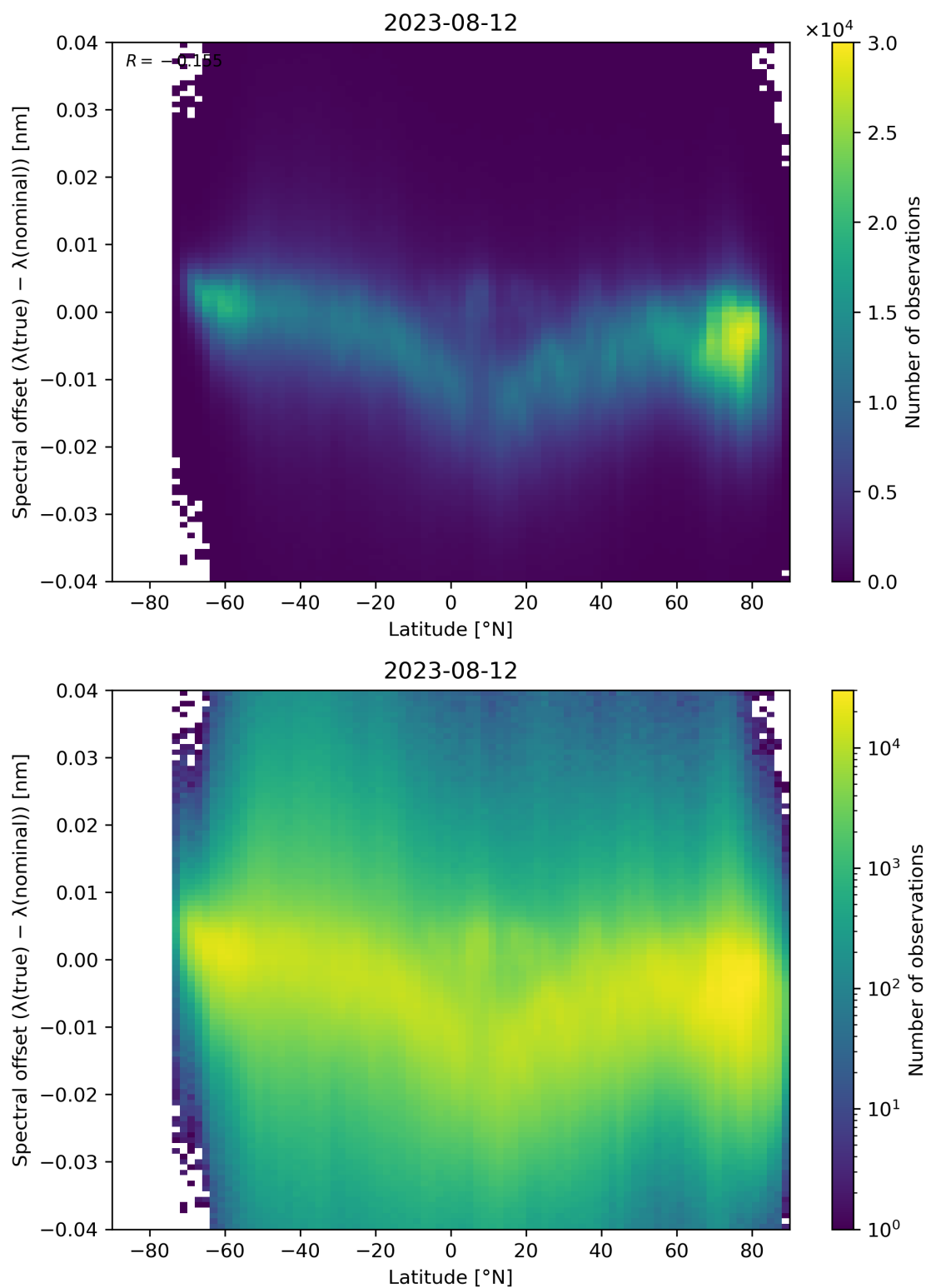
Figure 105: Scatter density plot of “Latitude” against “Spectral offset ( \lambda(\text{true}) - \lambda(\text{nominal}) )” for 2023-08-11 to 2023-08-13.
