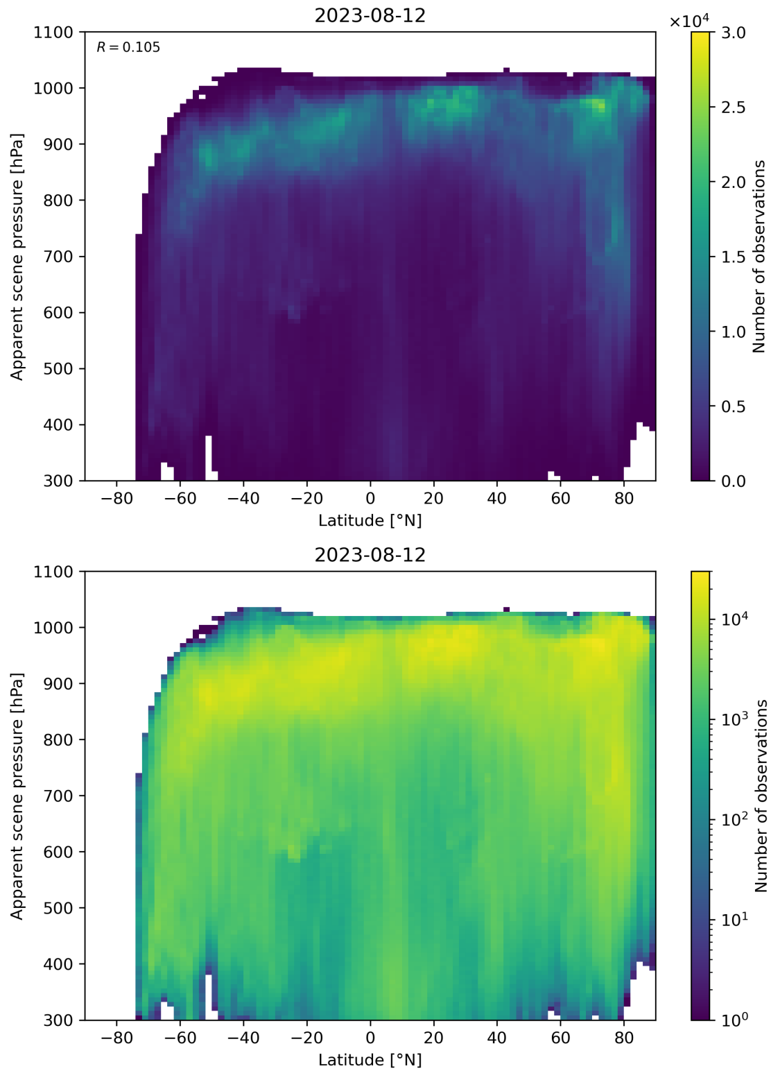
Figure 96: Scatter density plot of “Latitude” against “Apparent scene pressure” for 2023-08-11 to 2023-08-13.
