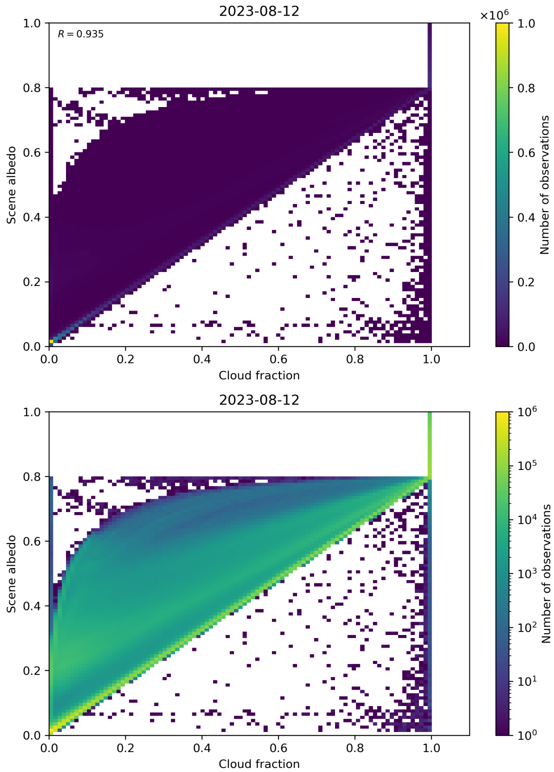
Figure 82: Scatter density plot of “Cloud fraction” against “Scene albedo” for 2023-08-11 to 2023-08-13.
