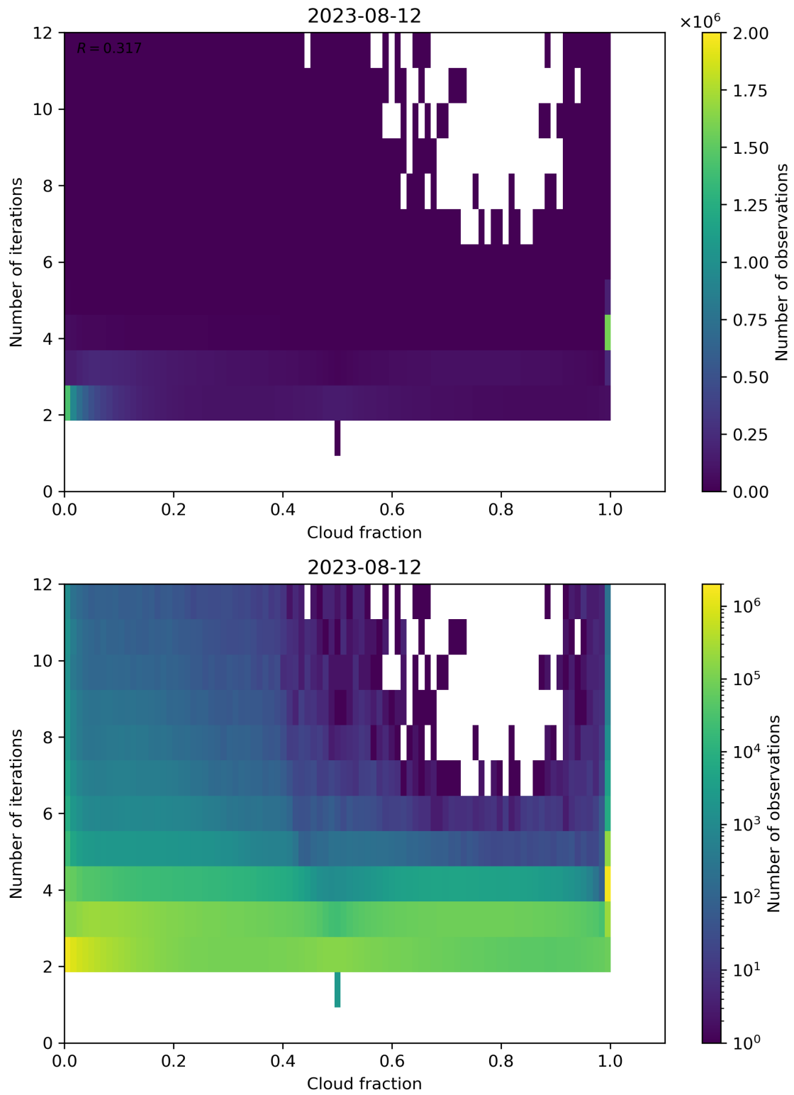
Figure 80: Scatter density plot of “Cloud fraction” against “Number of iterations” for 2023-08-11 to 2023-08-13.
