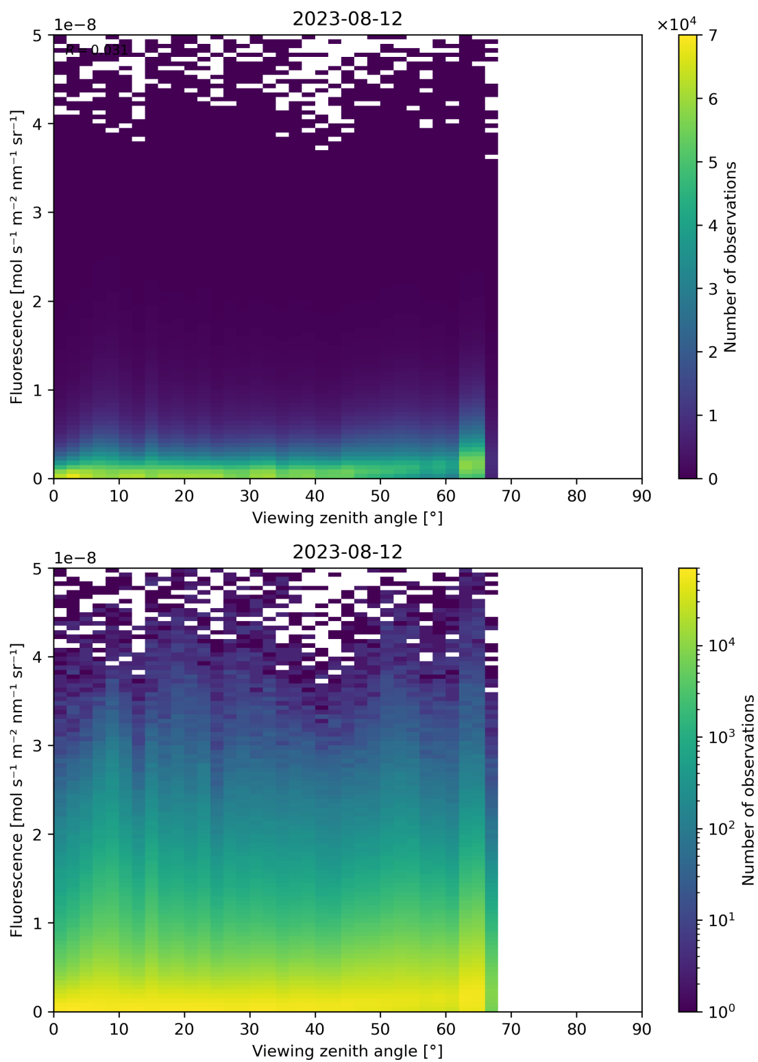
Figure 134: Scatter density plot of “Viewing zenith angle” against “Fluorescence” for 2023-08-11 to 2023-08-13.
