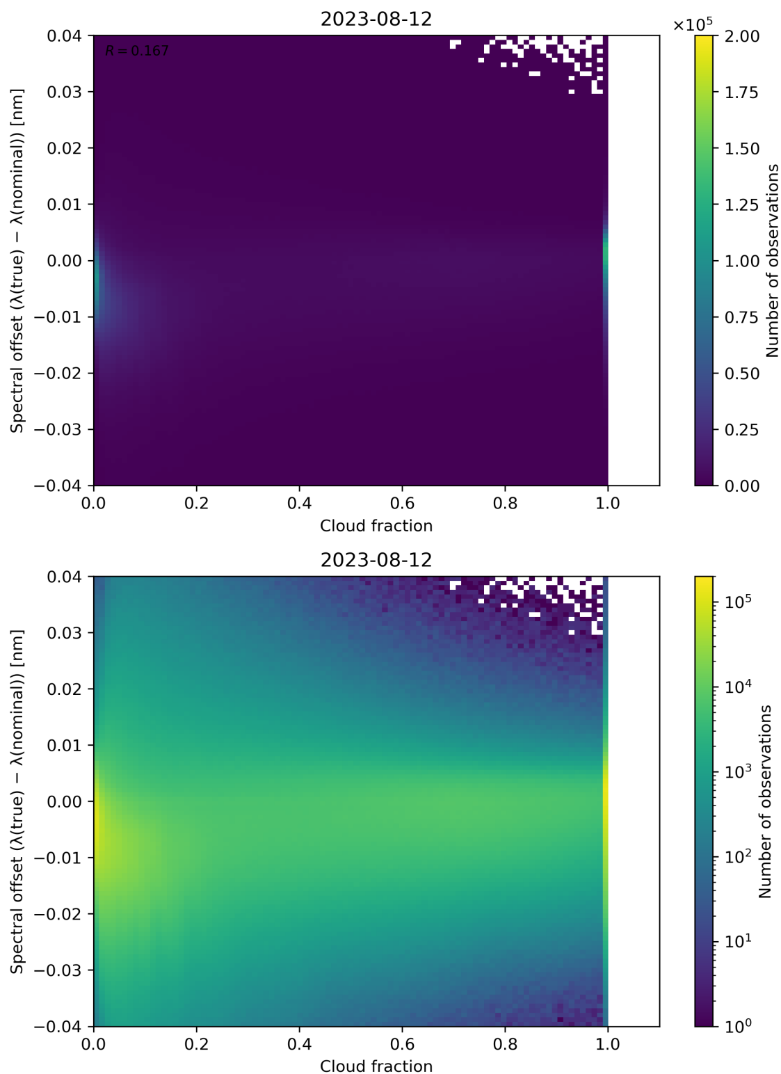
Figure 83: Scatter density plot of “Cloud fraction” against “Spectral offset ( \lambda(\text{true}) - \lambda(\text{nominal}) )” for 2023-08-11 to 2023-08-13.
