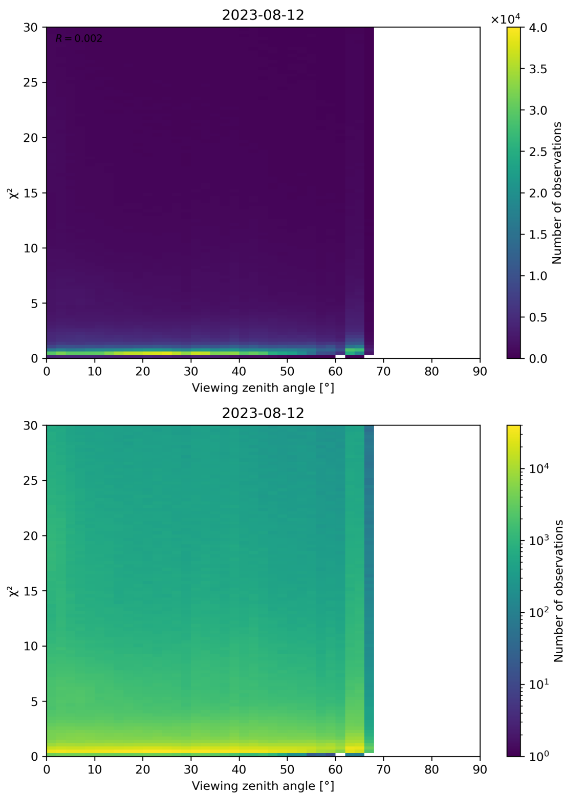
Figure 130: Scatter density plot of “Viewing zenith angle” against “ \chi^2 ” for 2023-08-11 to 2023-08-13.
