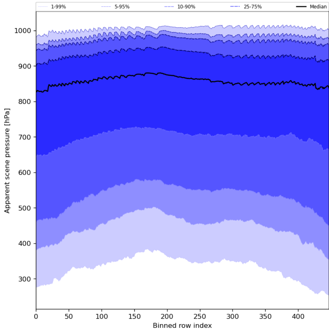
Figure 53: Along track statistics of “Apparent scene pressure” for 2023-08-11 to 2023-08-13
