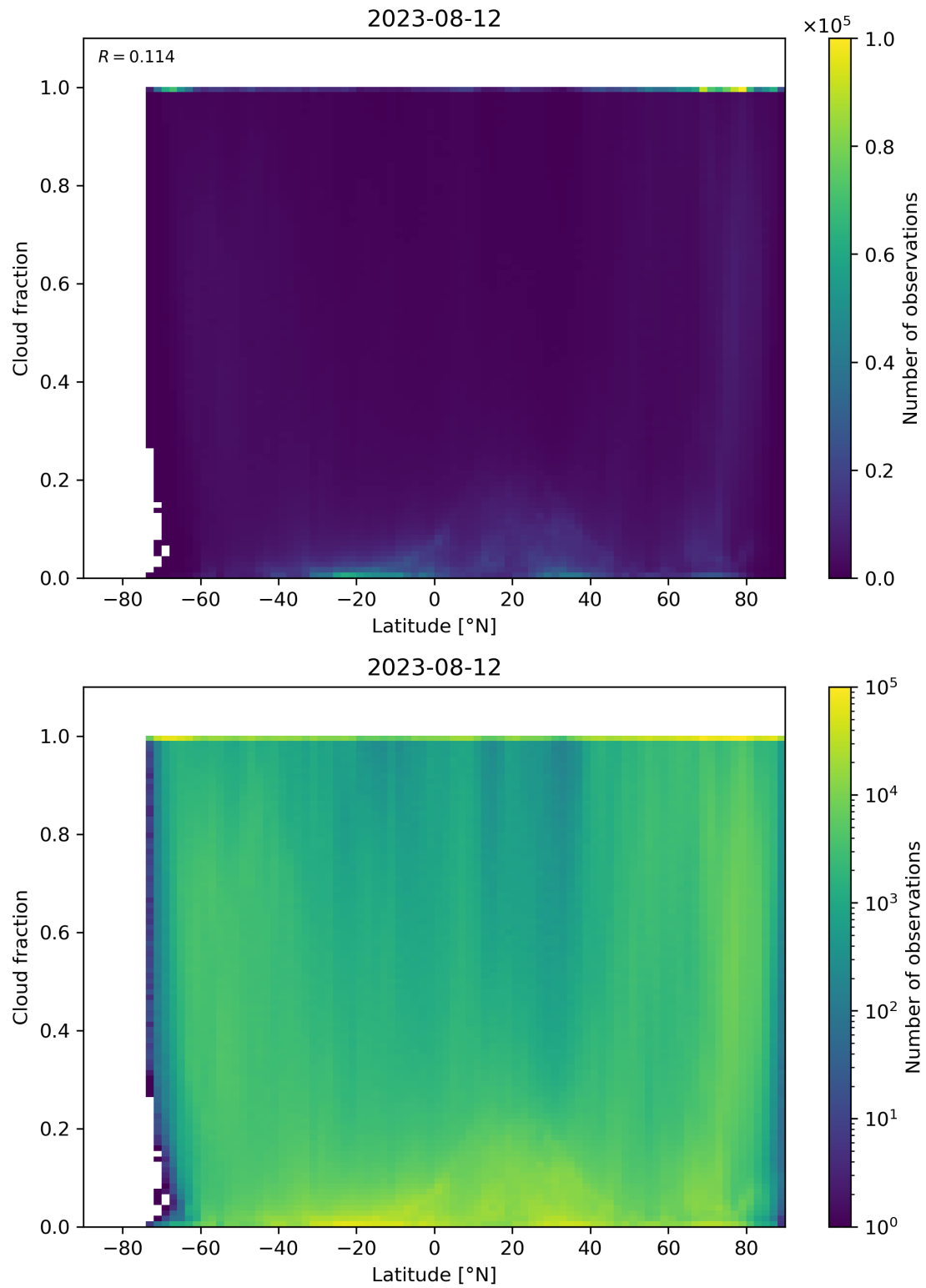
Figure 99: Scatter density plot of “Latitude” against “Cloud fraction” for 2023-08-11 to 2023-08-13.
