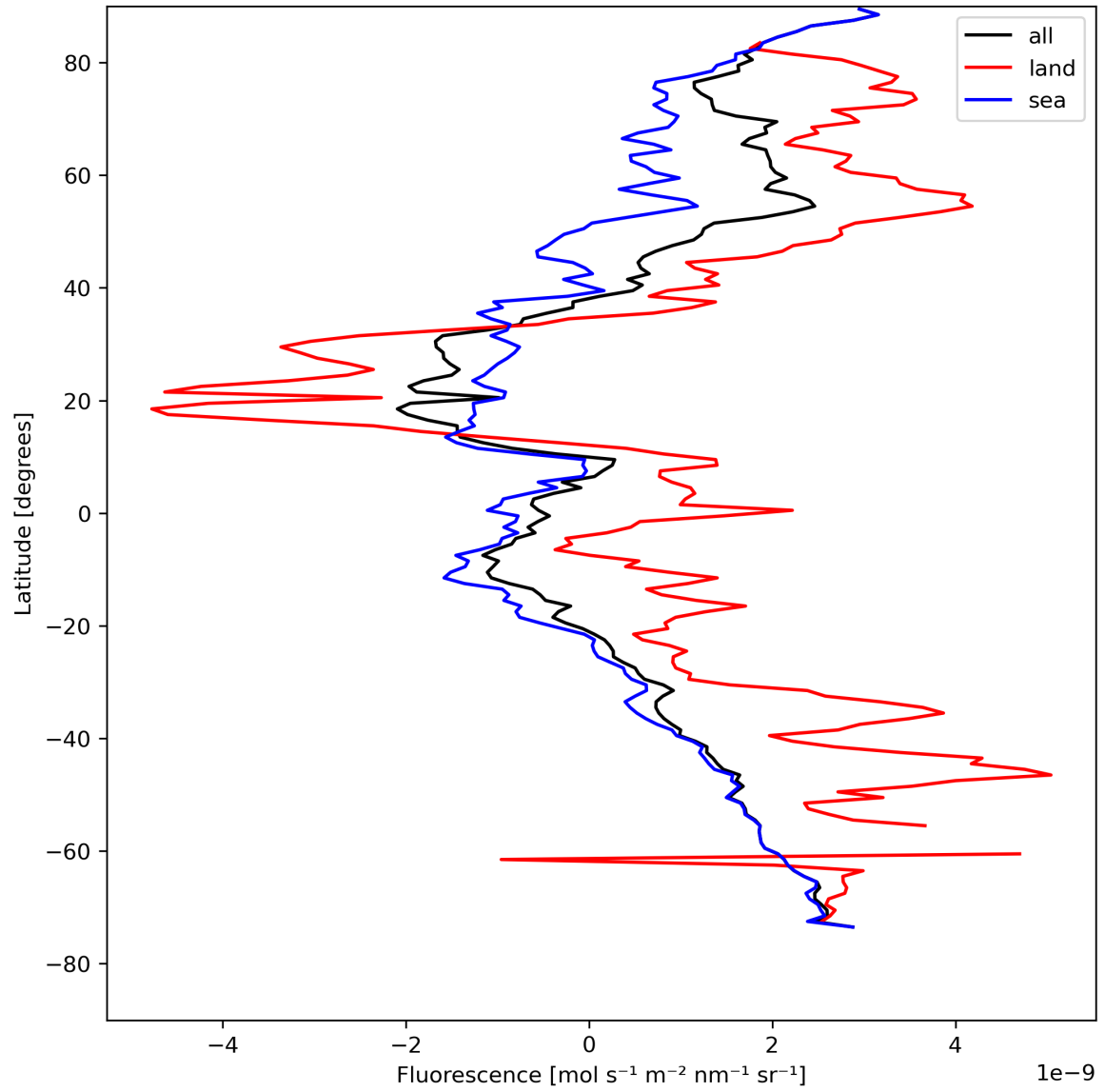
Figure 23: Zonal average of “Fluorescence” for 2023-08-11 to 2023-08-13.
