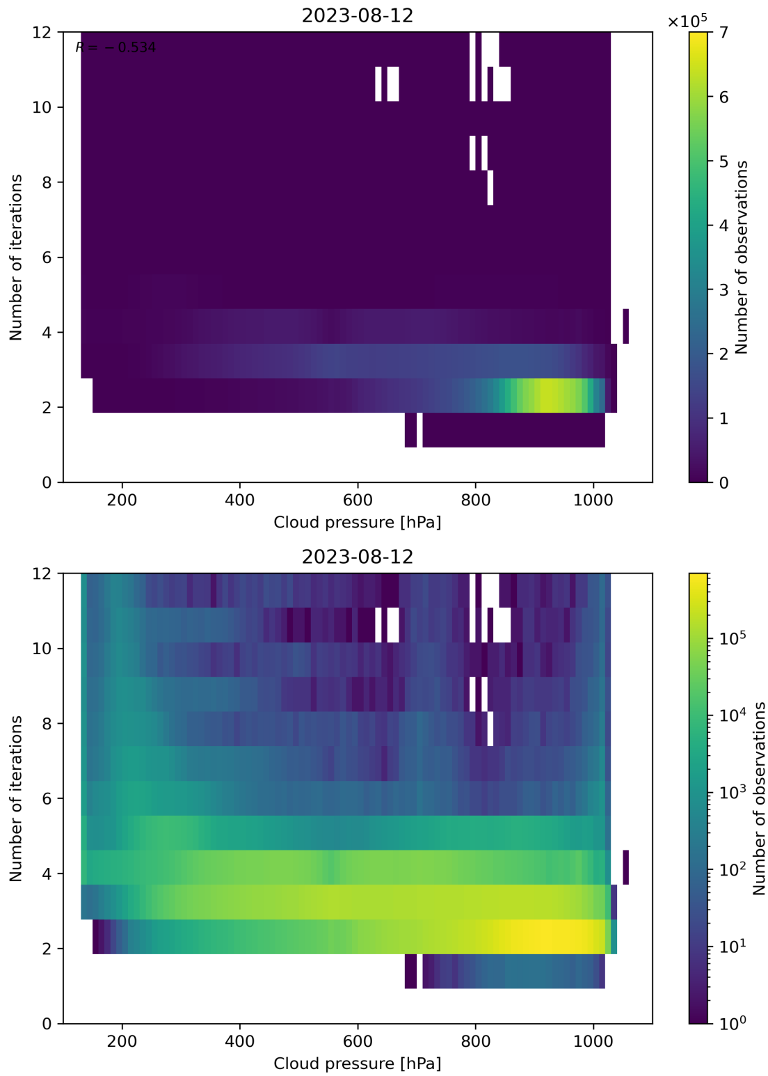
Figure 89: Scatter density plot of “Cloud pressure” against “Number of iterations” for 2023-08-11 to 2023-08-13.
