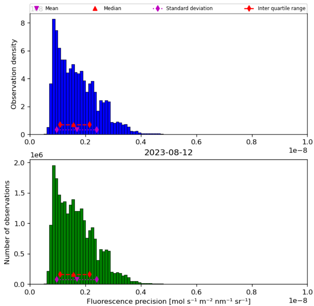
Figure 41: Histogram of “Fluorescence precision” for 2023-08-11 to 2023-08-13
