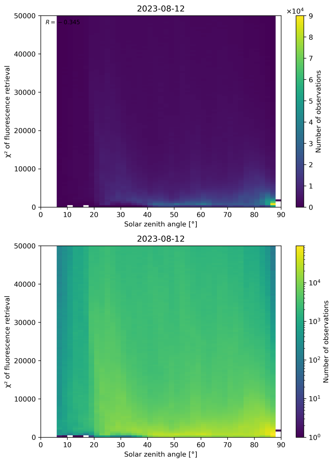
Figure 120: Scatter density plot of “Solar zenith angle” against “ \chi^2 of fluorescence retrieval” for 2023-08-11 to 2023-08-13.
