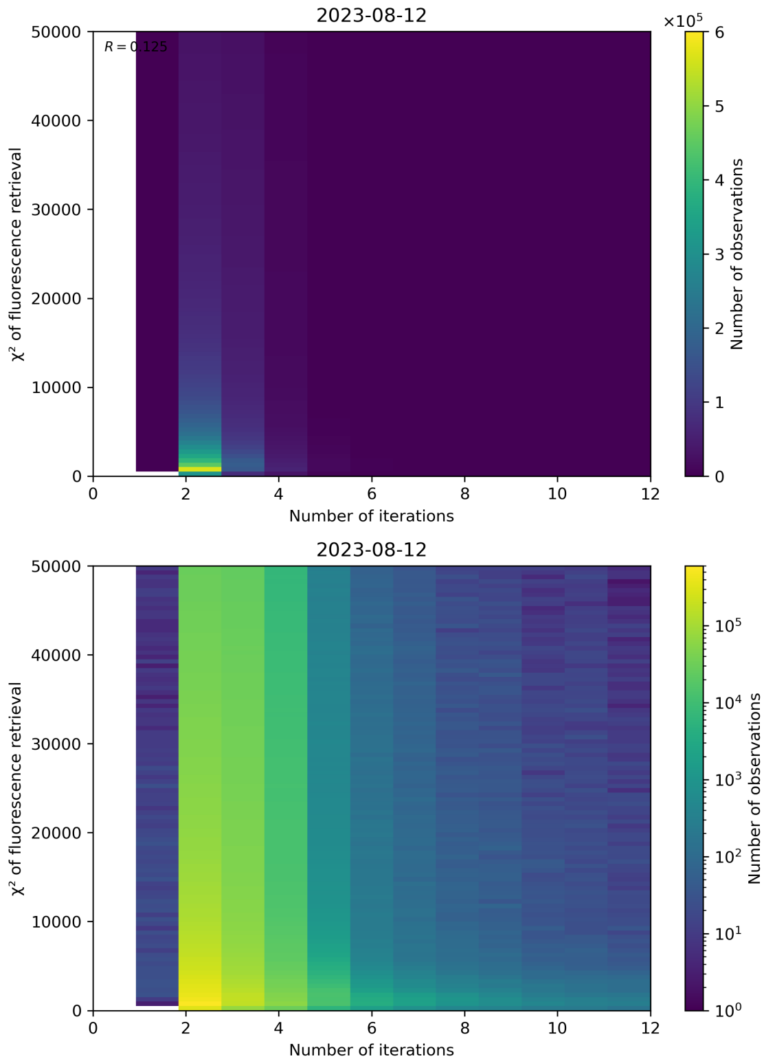
Figure 106: Scatter density plot of “Number of iterations” against “ \chi^2 of fluorescence retrieval” for 2023-08-11 to 2023-08-13.
