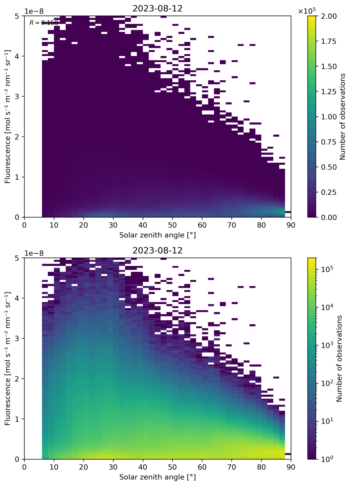
Figure 123: Scatter density plot of “Solar zenith angle” against “Fluorescence” for 2023-08-11 to 2023-08-13.
