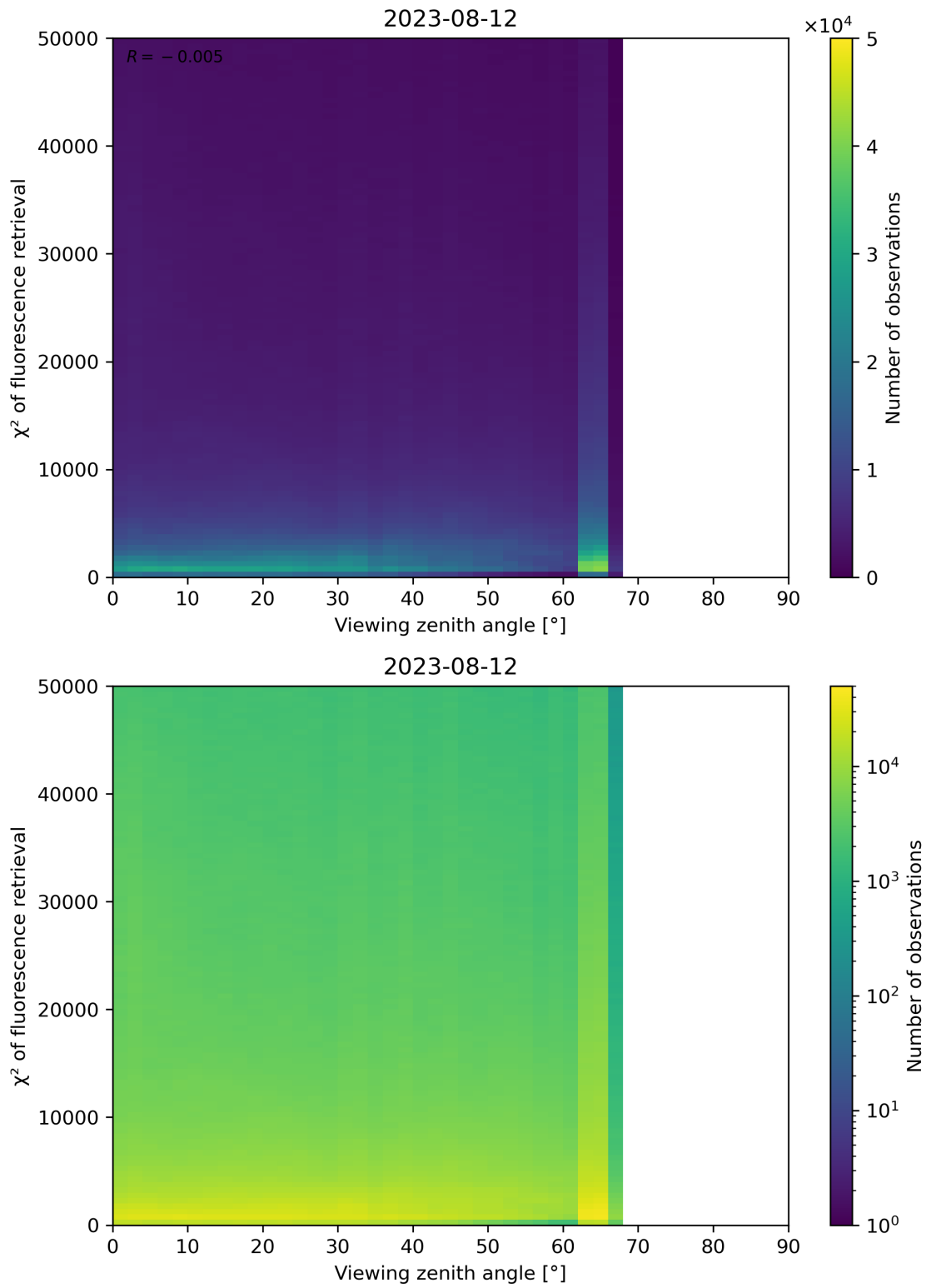
Figure 131: Scatter density plot of “Viewing zenith angle” against “ \chi^2 of fluorescence retrieval” for 2023-08-11 to 2023-08-13.
