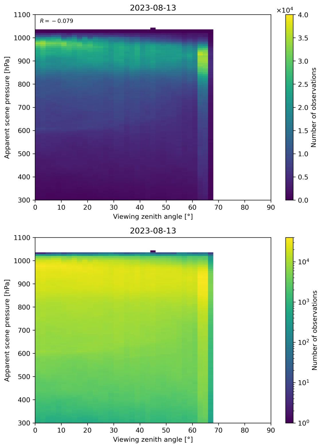
Figure 129: Scatter density plot of “Viewing zenith angle” against “Apparent scene pressure” for 2023-08-12 to 2023-08-14.
