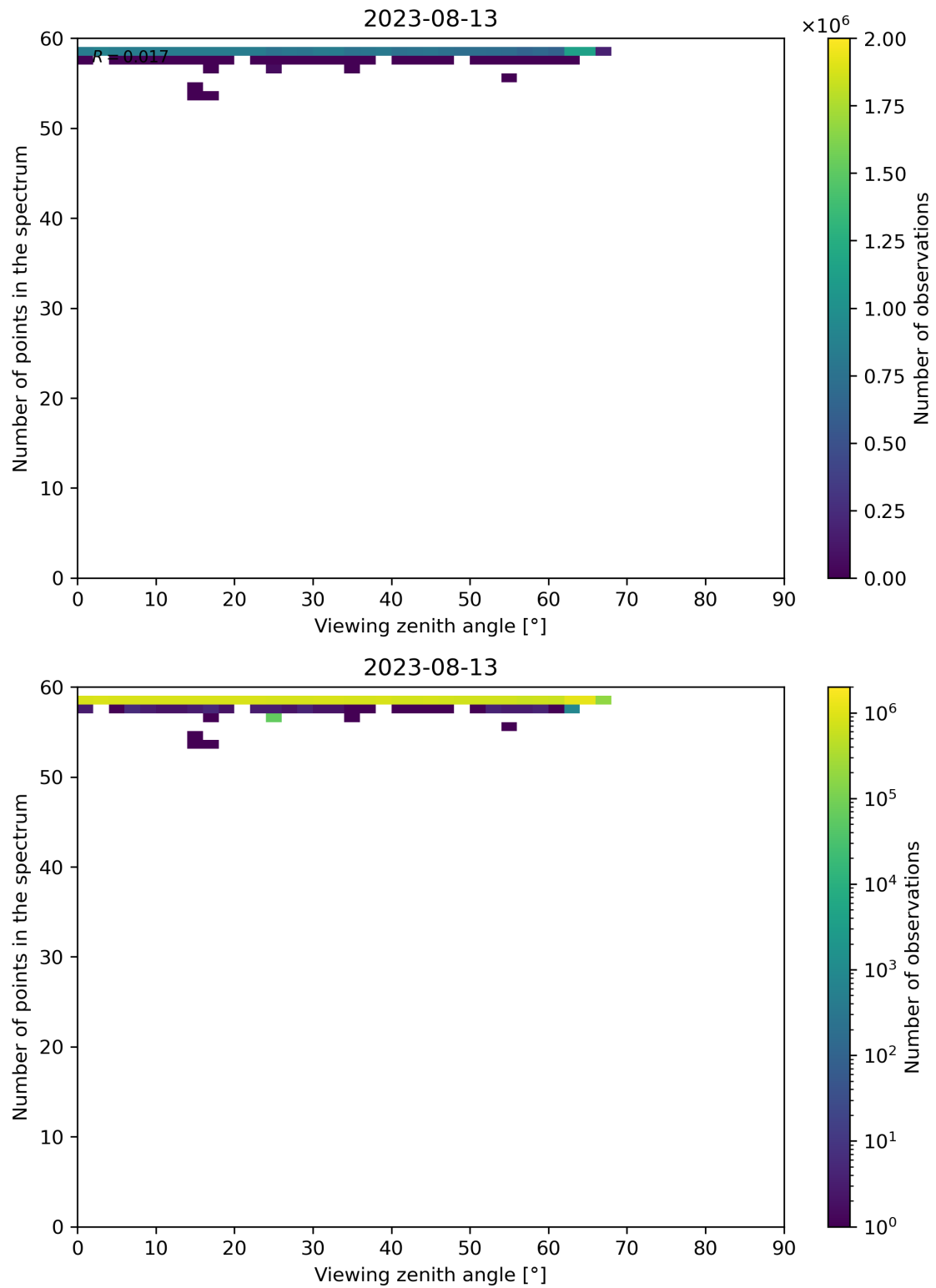
Figure 137: Scatter density plot of “Viewing zenith angle” against “Number of points in the spectrum” for 2023-08-12 to 2023-08-14.
