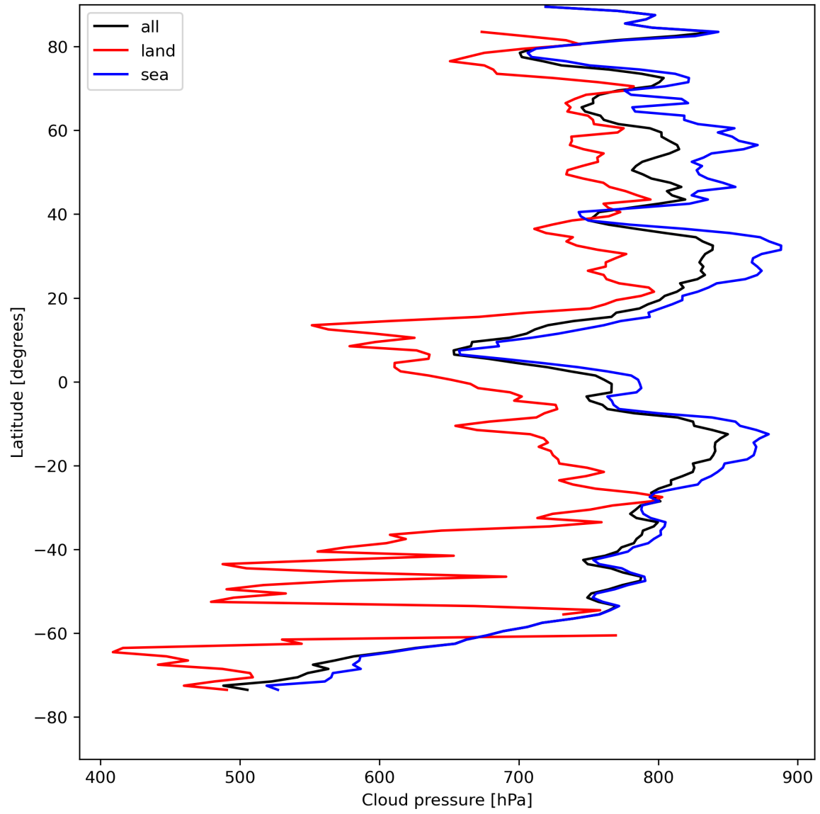
Figure 13: Zonal average of “Cloud pressure” for 2023-08-12 to 2023-08-14.
