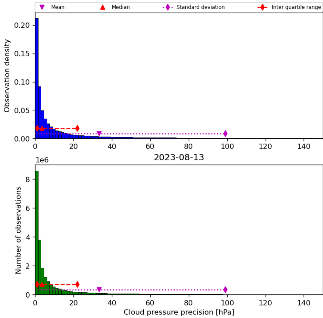
Figure 31: Histogram of “Cloud pressure precision” for 2023-08-12 to 2023-08-14
