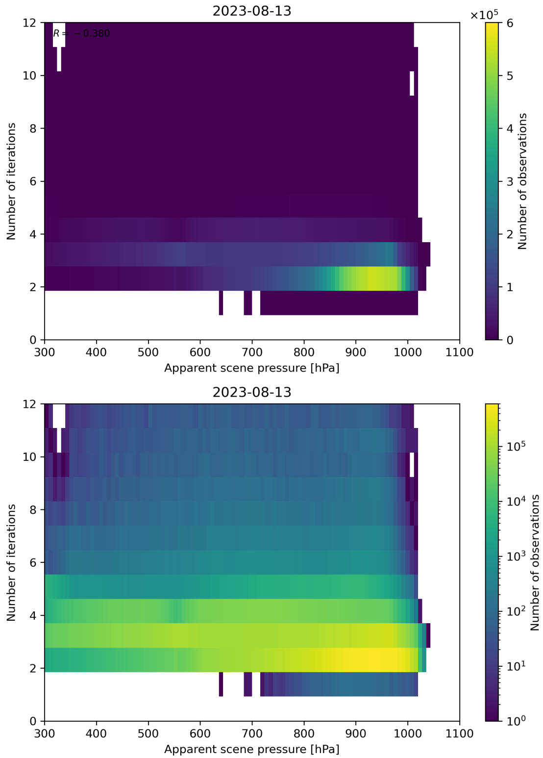
Figure 66: Scatter density plot of “Apparent scene pressure” against “Number of iterations” for 2023-08-12 to 2023-08-14.
