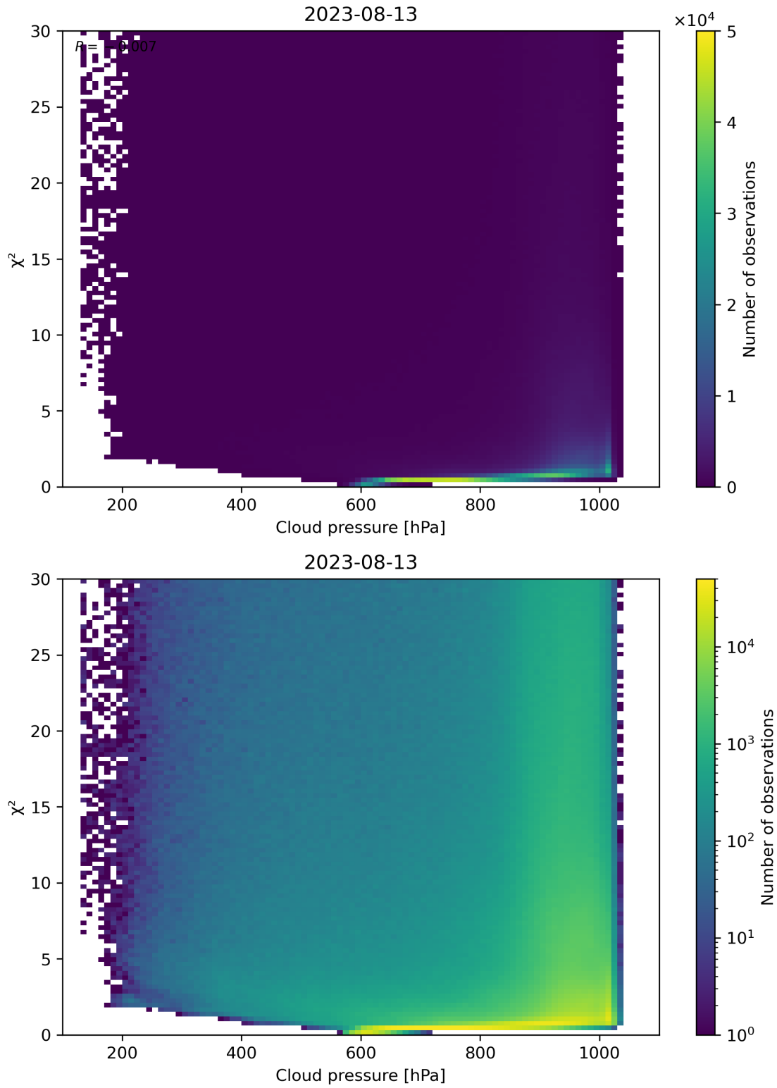
Figure 85: Scatter density plot of “Cloud pressure” against “ \chi^2 ” for 2023-08-12 to 2023-08-14.
