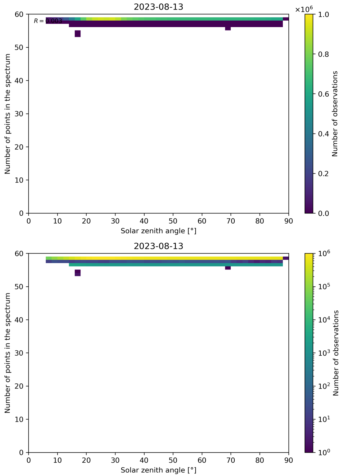
Figure 126: Scatter density plot of “Solar zenith angle” against “Number of points in the spectrum” for 2023-08-12 to 2023-08-14.
