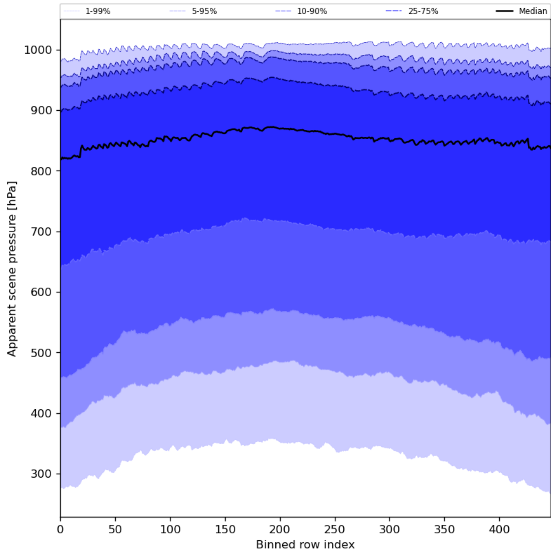
Figure 53: Along track statistics of “Apparent scene pressure” for 2023-08-12 to 2023-08-14
