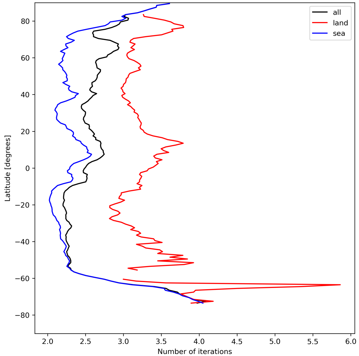
Figure 22: Zonal average of “Number of iterations” for 2023-08-12 to 2023-08-14.
