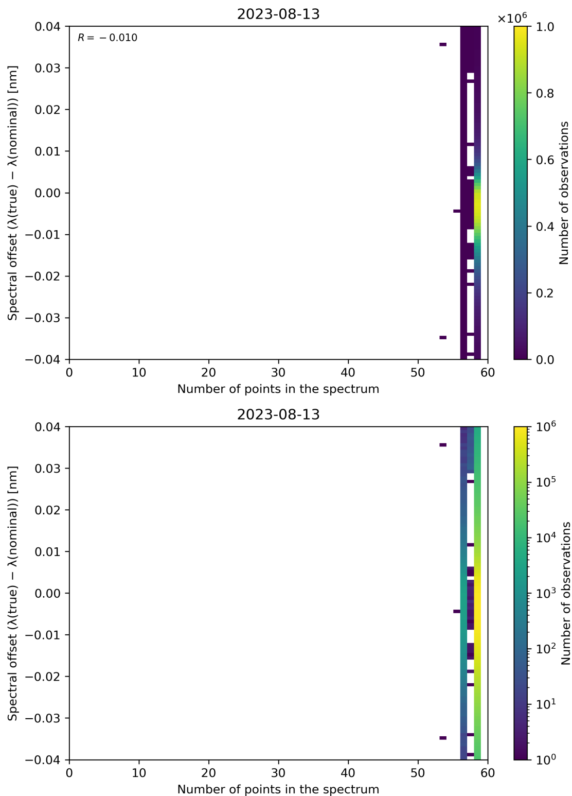
Figure 110: Scatter density plot of “Number of points in the spectrum” against “Spectral offset ( \lambda(\text{true}) - \lambda(\text{nominal}) )” for 2023-08-12 to 2023-08-14.
