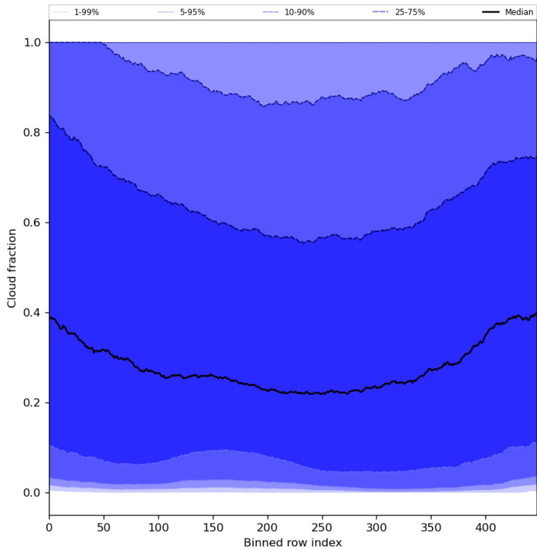
Figure 49: Along track statistics of “Cloud fraction” for 2023-08-12 to 2023-08-14
