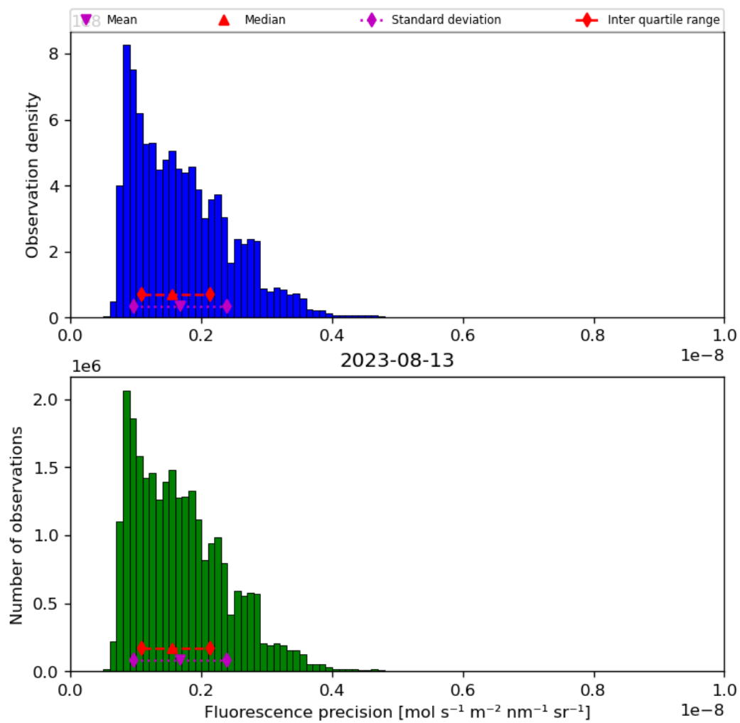
Figure 41: Histogram of “Fluorescence precision” for 2023-08-12 to 2023-08-14
