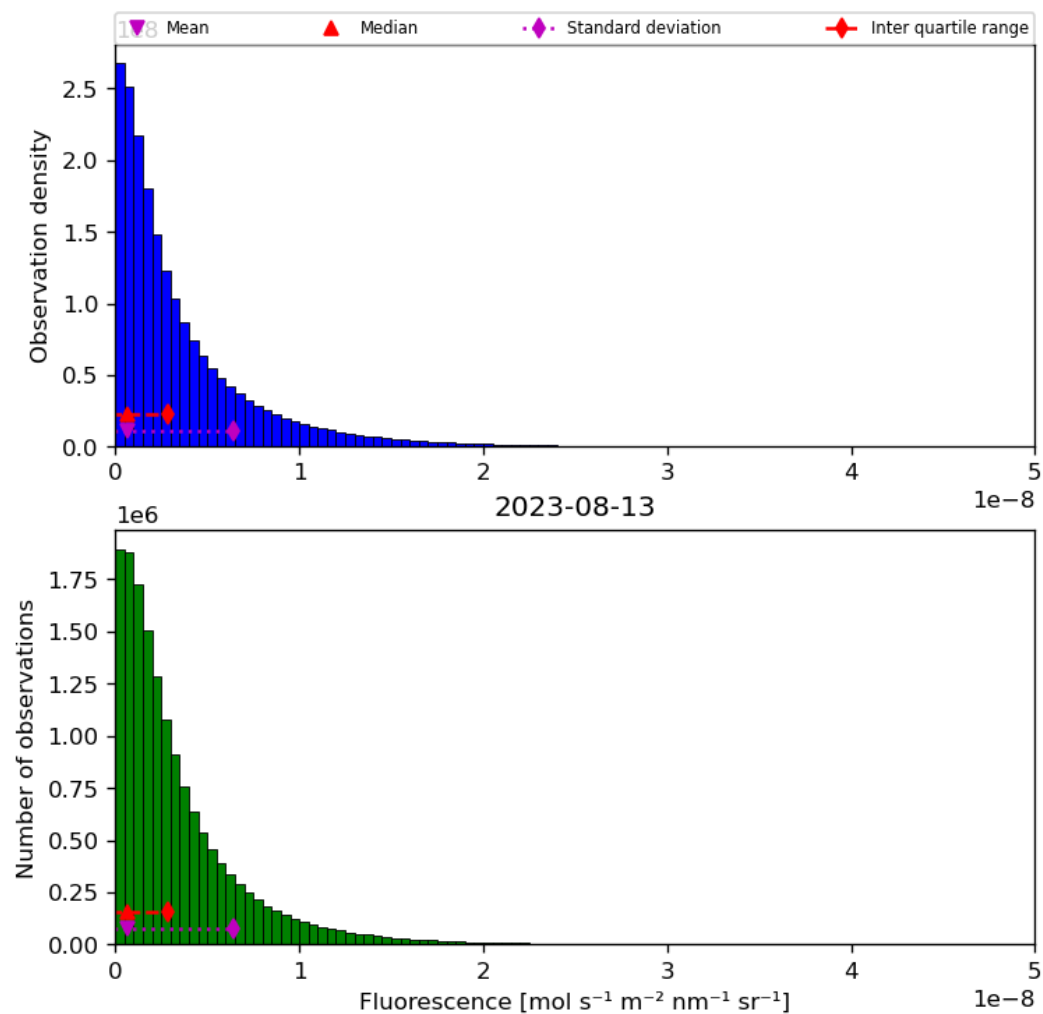
Figure 40: Histogram of “Fluorescence” for 2023-08-12 to 2023-08-14
