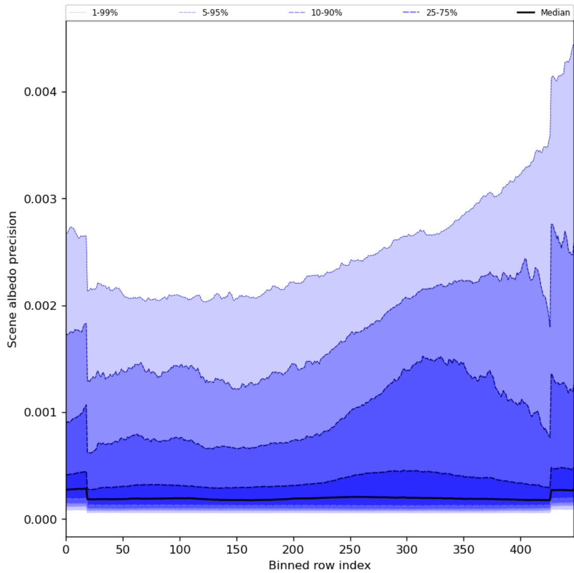
Figure 52: Along track statistics of “Scene albedo precision” for 2023-08-12 to 2023-08-14
