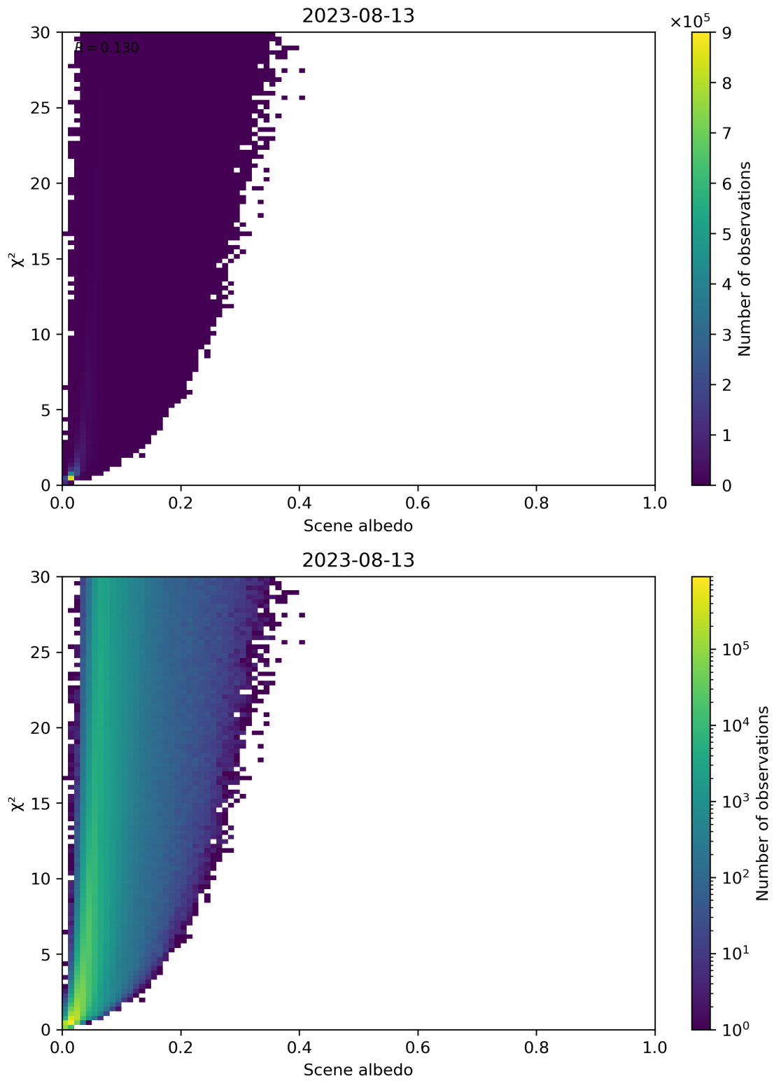
Figure 112: Scatter density plot of “Scene albedo” against “ \chi^2 ” for 2023-08-12 to 2023-08-14.
