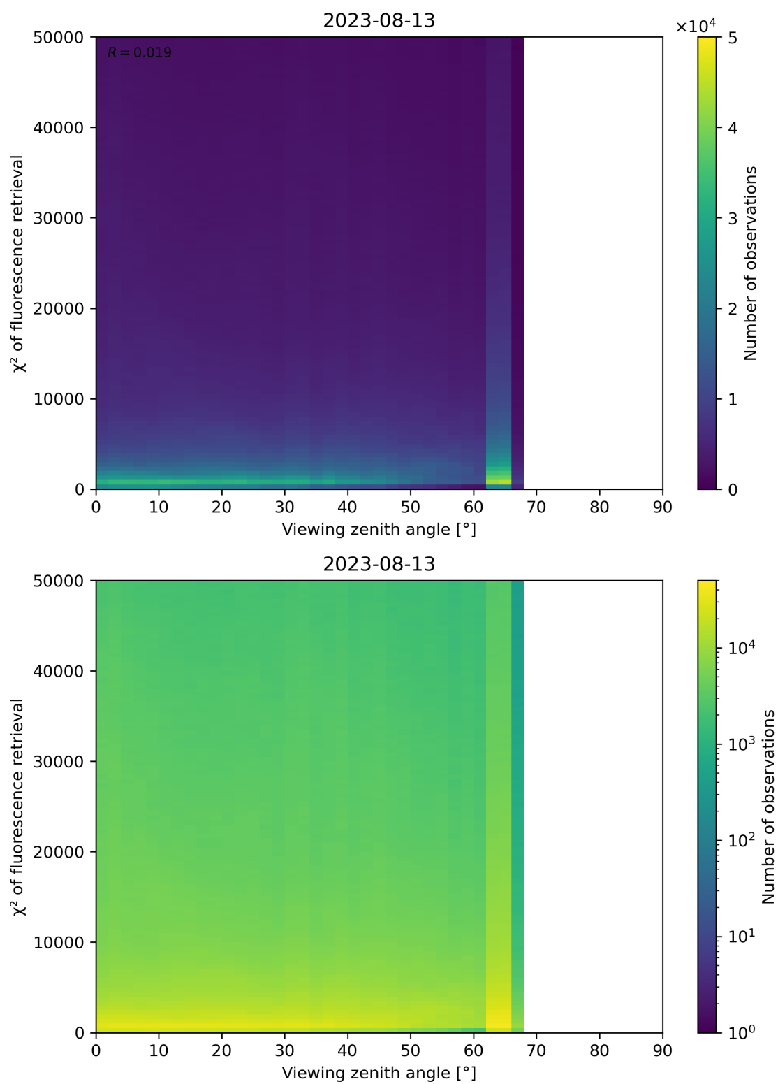
Figure 131: Scatter density plot of “Viewing zenith angle” against “ \chi^2 of fluorescence retrieval” for 2023-08-12 to 2023-08-14.
