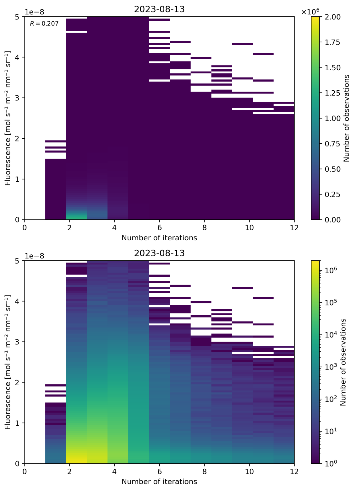
Figure 107: Scatter density plot of “Number of iterations” against “Fluorescence” for 2023-08-12 to 2023-08-14.
