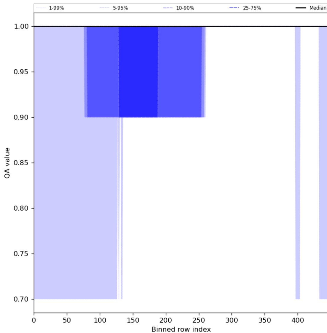
Figure 46: Along track statistics of “QA value” for 2023-08-12 to 2023-08-14
