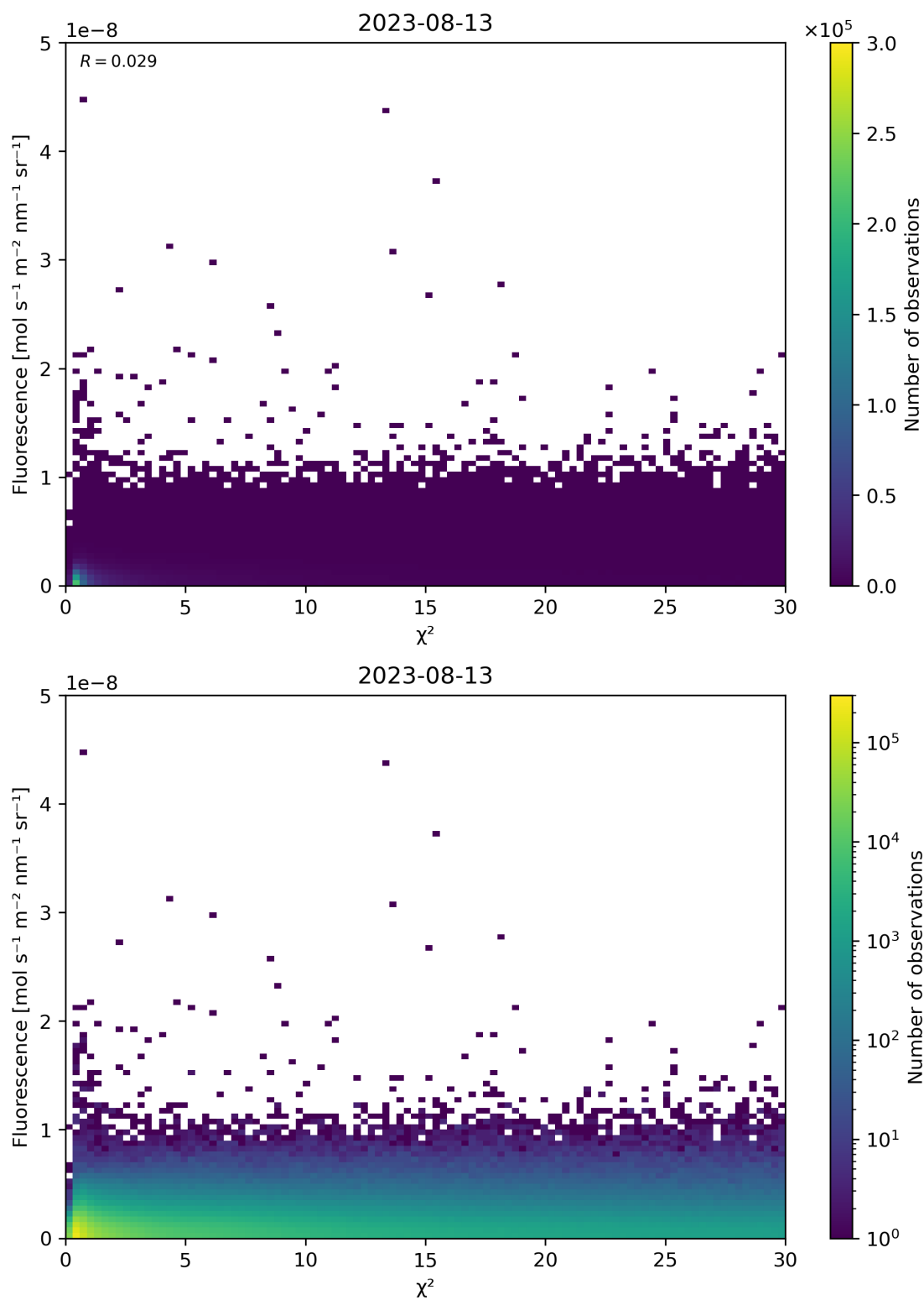
Figure 70: Scatter density plot of “ \chi^2 ” against “Fluorescence” for 2023-08-12 to 2023-08-14.
