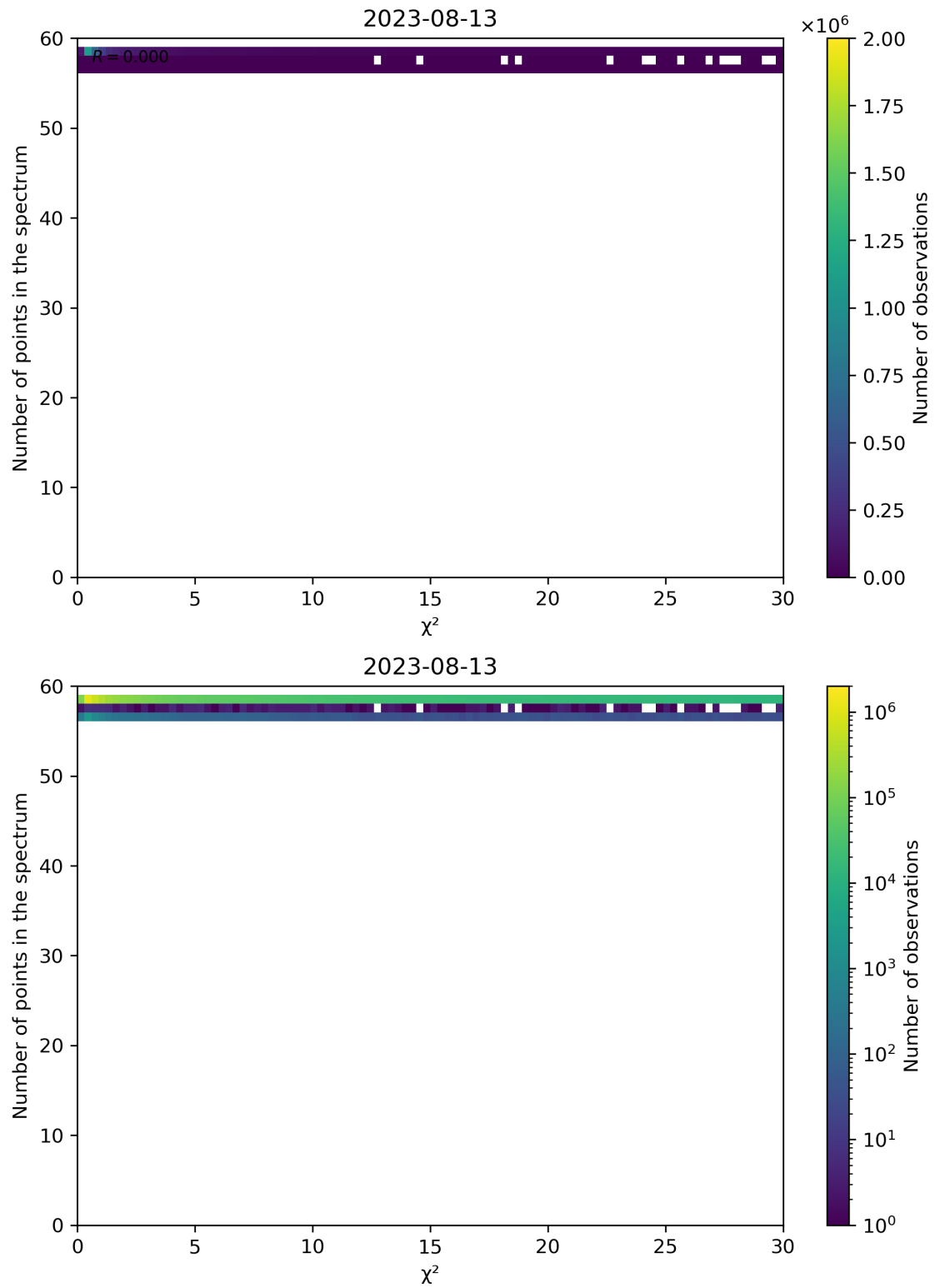
Figure 74: Scatter density plot of " \chi^2 " against "Number of points in the spectrum" for 2023-08-12 to 2023-08-14.
