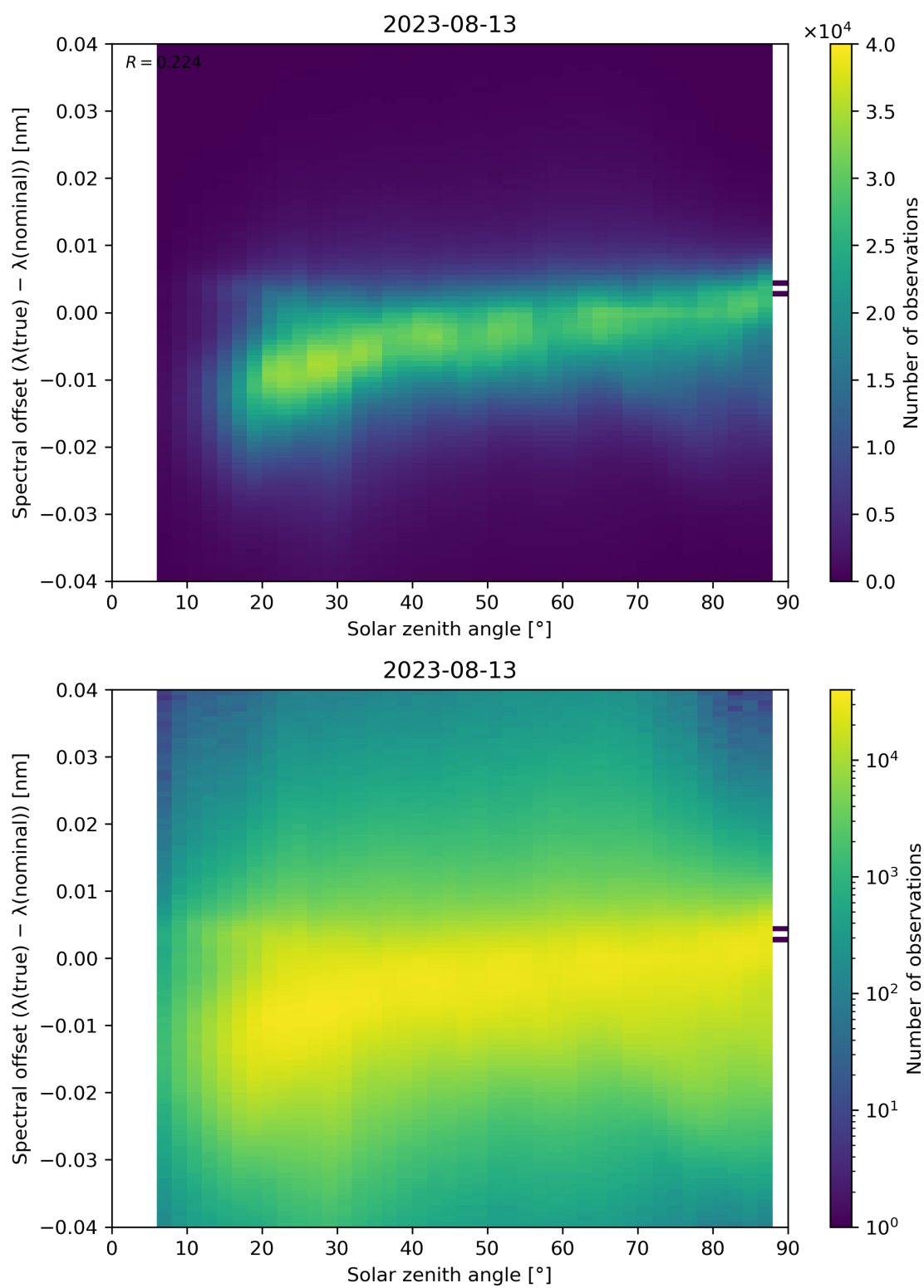
Figure 128: Scatter density plot of “Solar zenith angle” against “Spectral offset ( \lambda(\text{true}) - \lambda(\text{nominal}) )” for 2023-08-12 to 2023-08-14.
