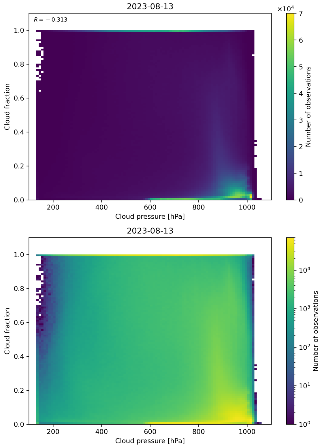
Figure 87: Scatter density plot of “Cloud pressure” against “Cloud fraction” for 2023-08-12 to 2023-08-14.
