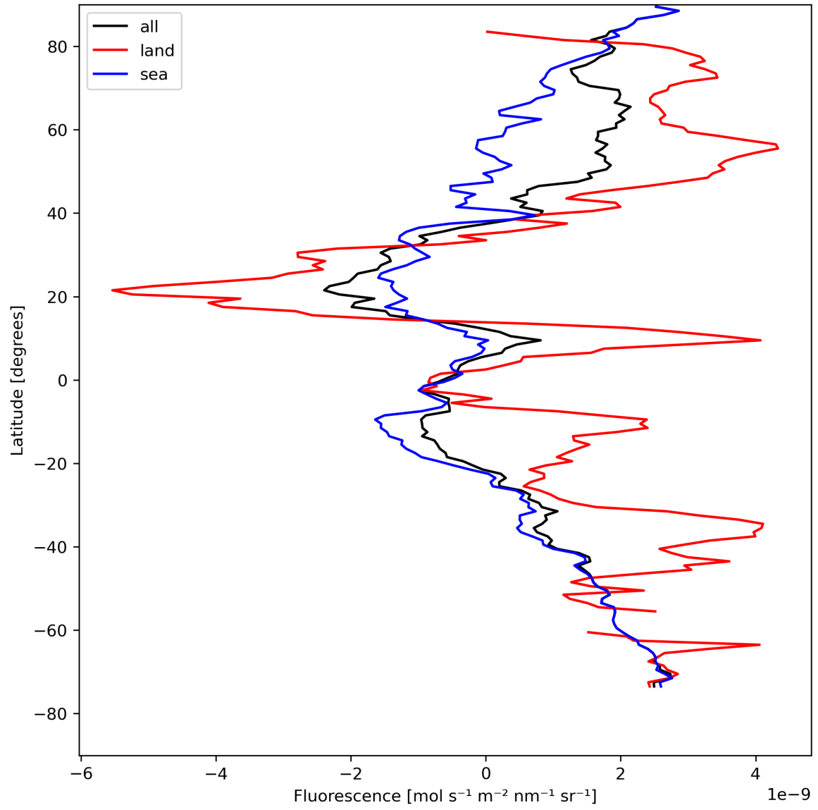
Figure 23: Zonal average of “Fluorescence” for 2023-08-12 to 2023-08-14.
