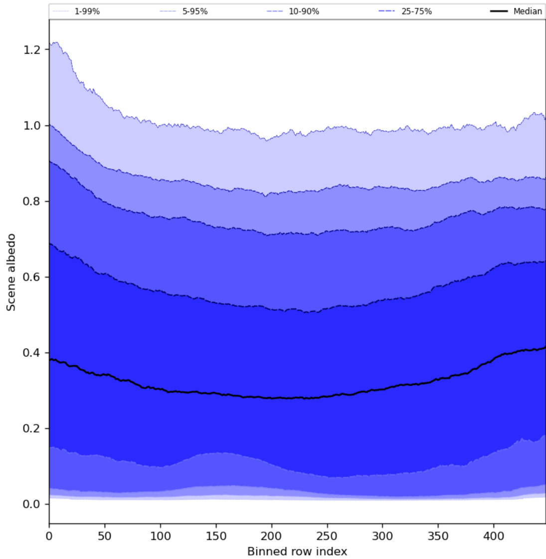
Figure 51: Along track statistics of “Scene albedo” for 2023-08-12 to 2023-08-14
