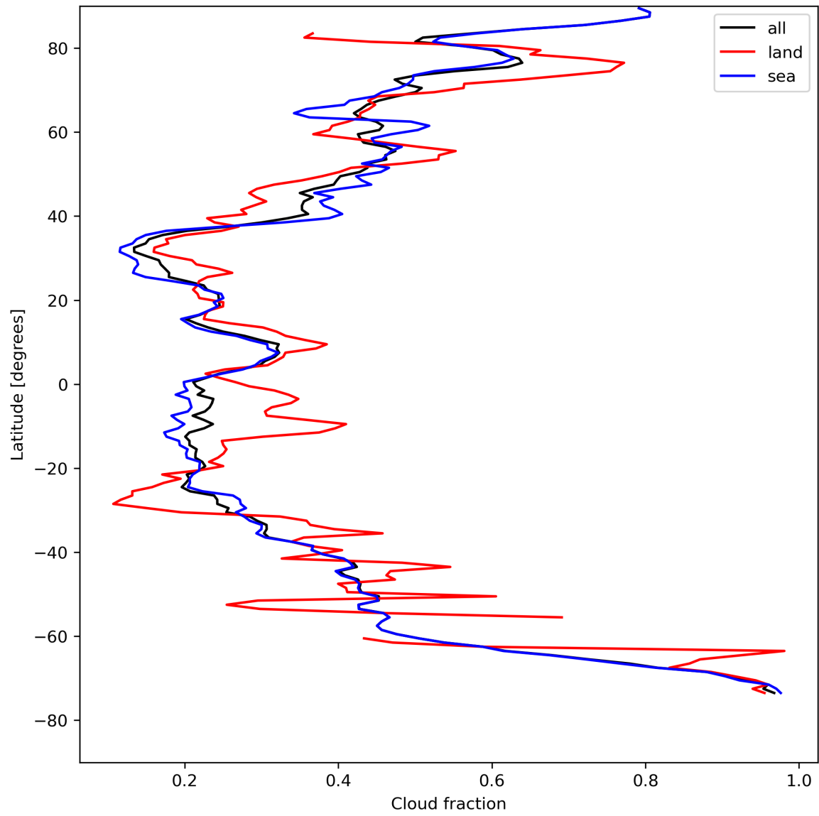
Figure 15: Zonal average of “Cloud fraction” for 2023-08-12 to 2023-08-14.
