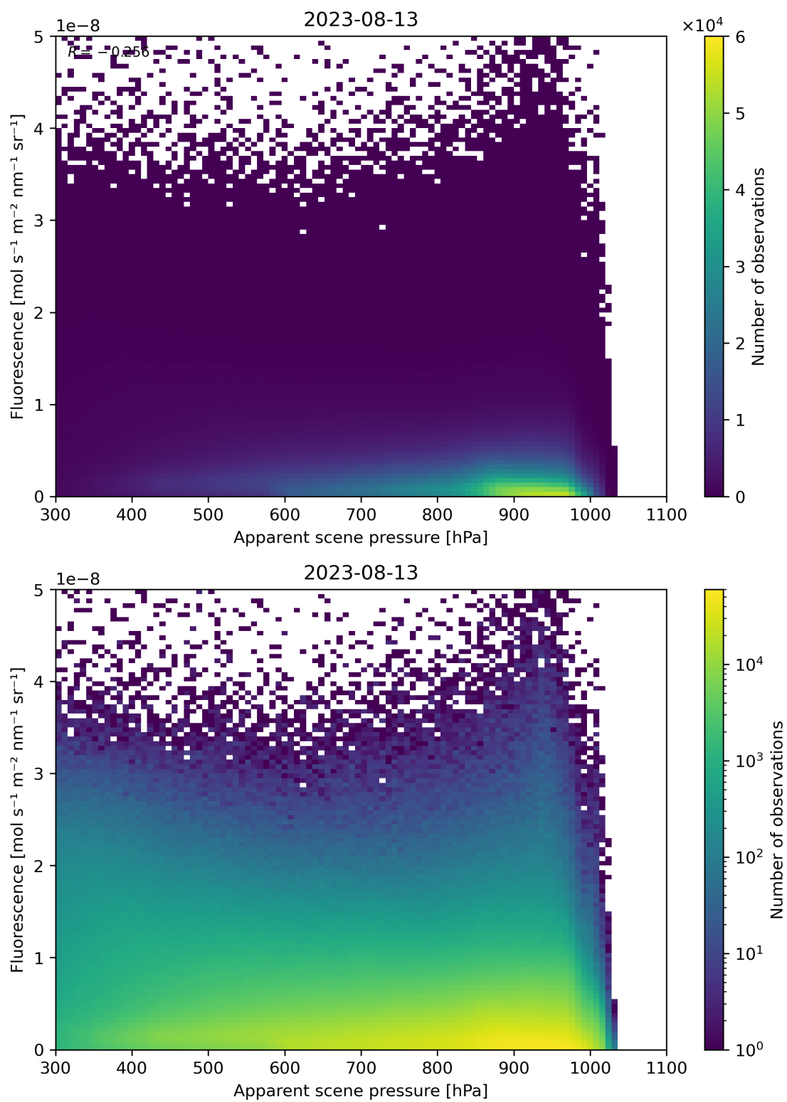
Figure 65: Scatter density plot of “Apparent scene pressure” against “Fluorescence” for 2023-08-12 to 2023-08-14.
