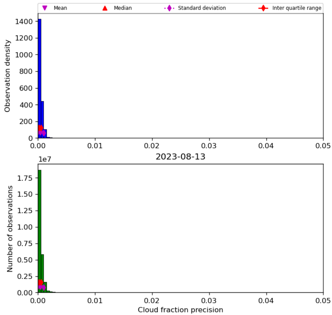
Figure 33: Histogram of “Cloud fraction precision” for 2023-08-12 to 2023-08-14
