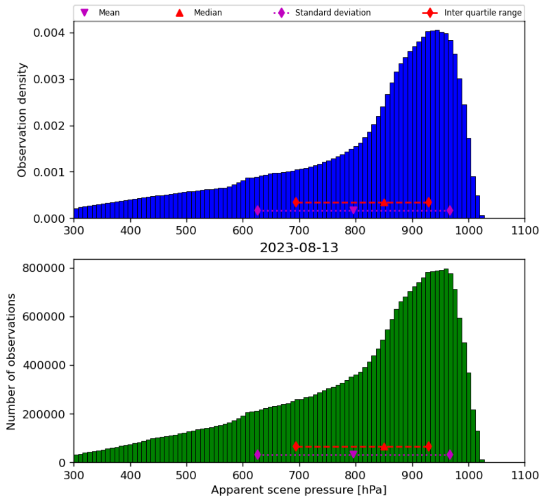
Figure 36: Histogram of “Apparent scene pressure” for 2023-08-12 to 2023-08-14
