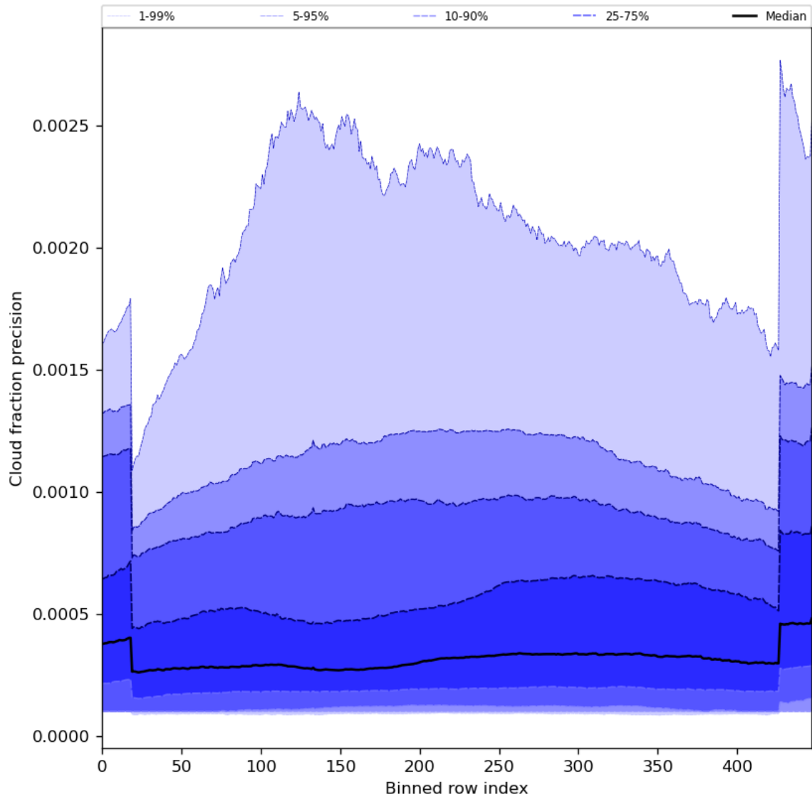
Figure 50: Along track statistics of “Cloud fraction precision” for 2023-08-12 to 2023-08-14
