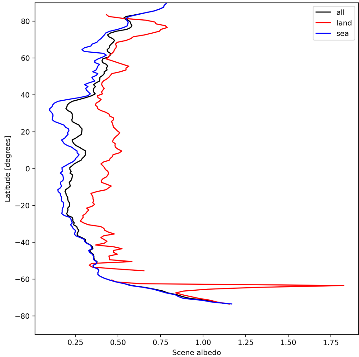
Figure 17: Zonal average of “Scene albedo” for 2023-08-12 to 2023-08-14.
