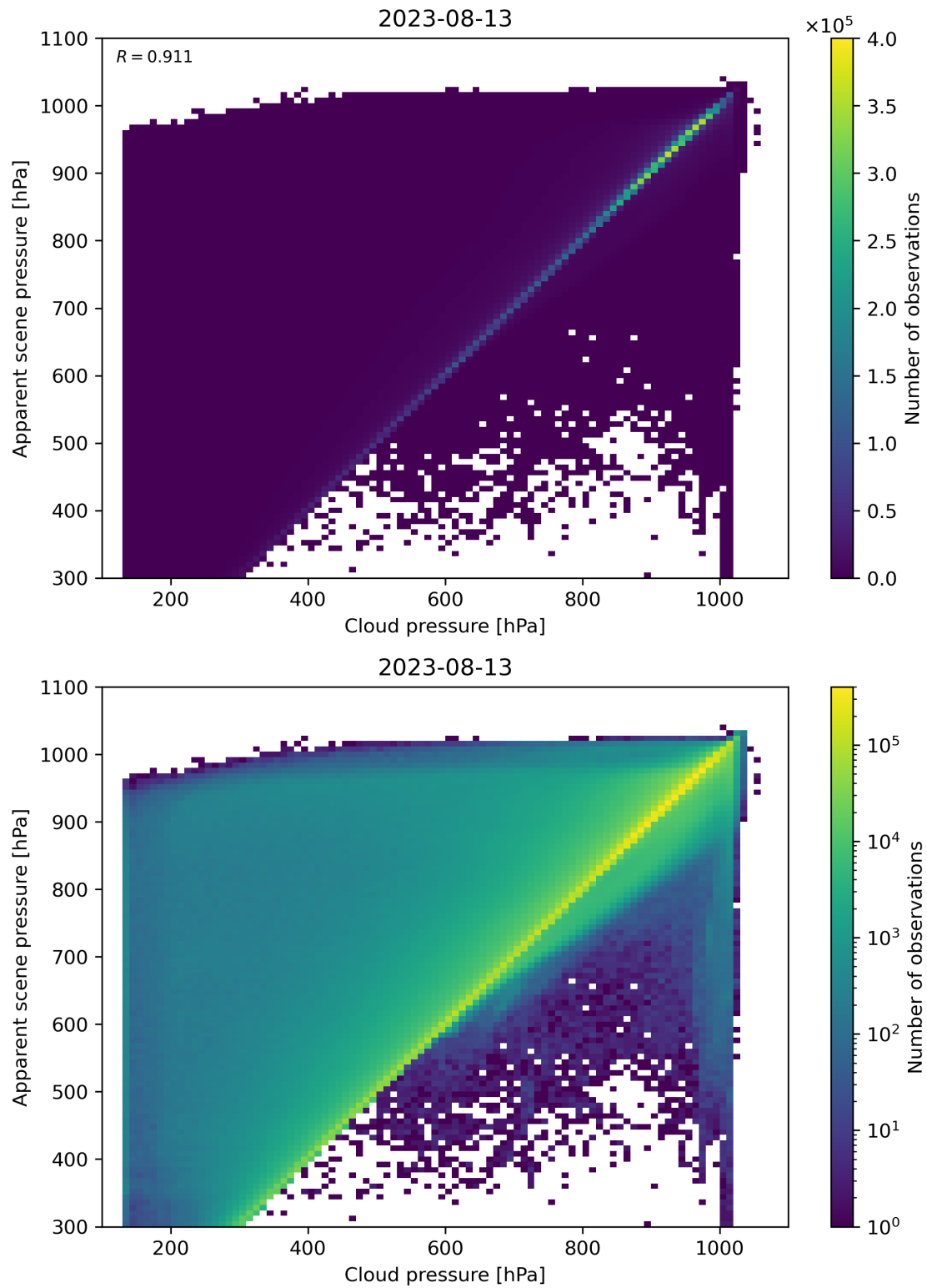
Figure 84: Scatter density plot of “Cloud pressure” against “Apparent scene pressure” for 2023-08-12 to 2023-08-14.
