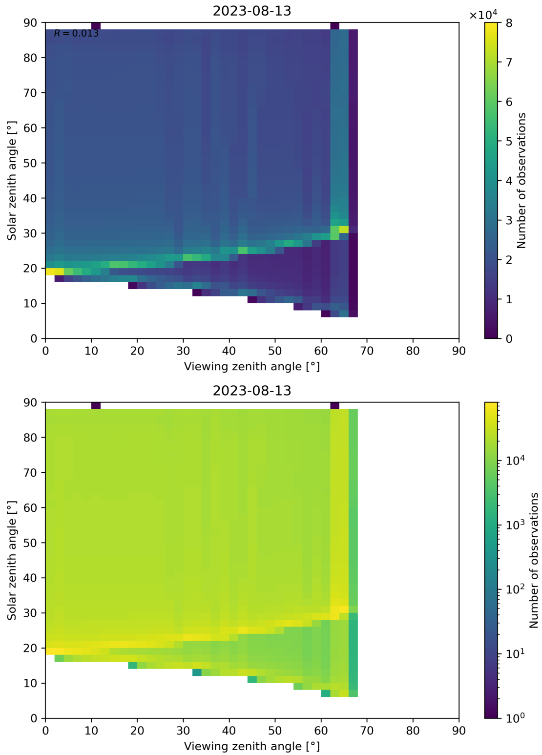
Figure 139: Scatter density plot of “Viewing zenith angle” against “Solar zenith angle” for 2023-08-12 to 2023-08-14.
