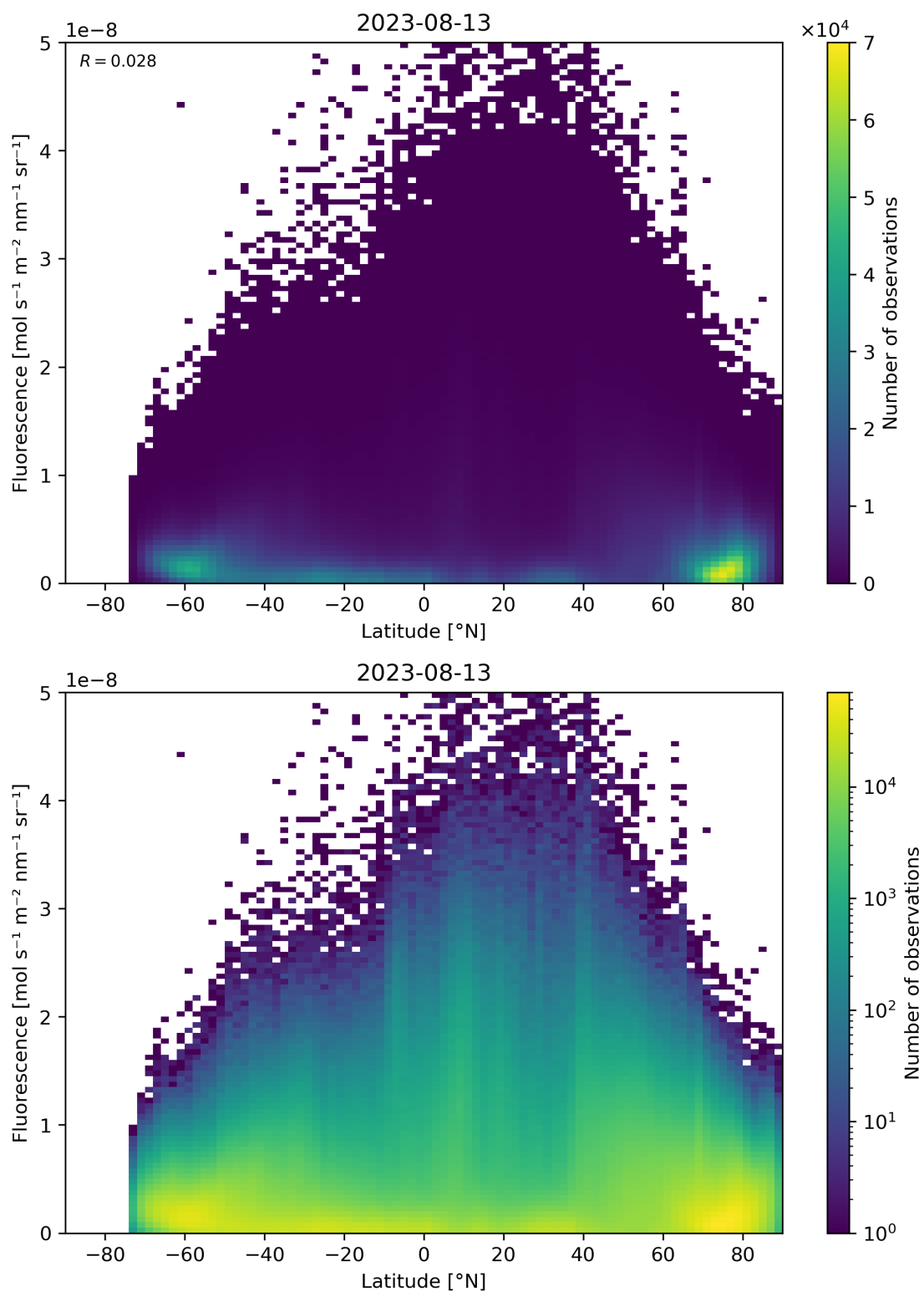
Figure 101: Scatter density plot of “Latitude” against “Fluorescence” for 2023-08-12 to 2023-08-14.
