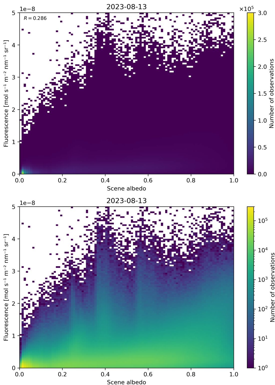
Figure 114: Scatter density plot of “Scene albedo” against “Fluorescence” for 2023-08-12 to 2023-08-14.
