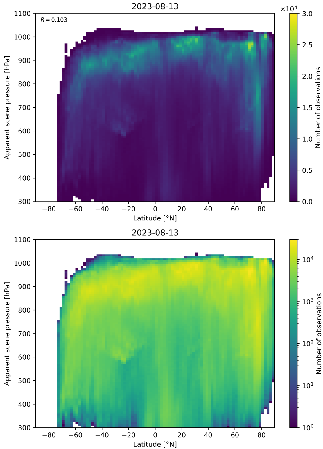
Figure 96: Scatter density plot of “Latitude” against “Apparent scene pressure” for 2023-08-12 to 2023-08-14.
