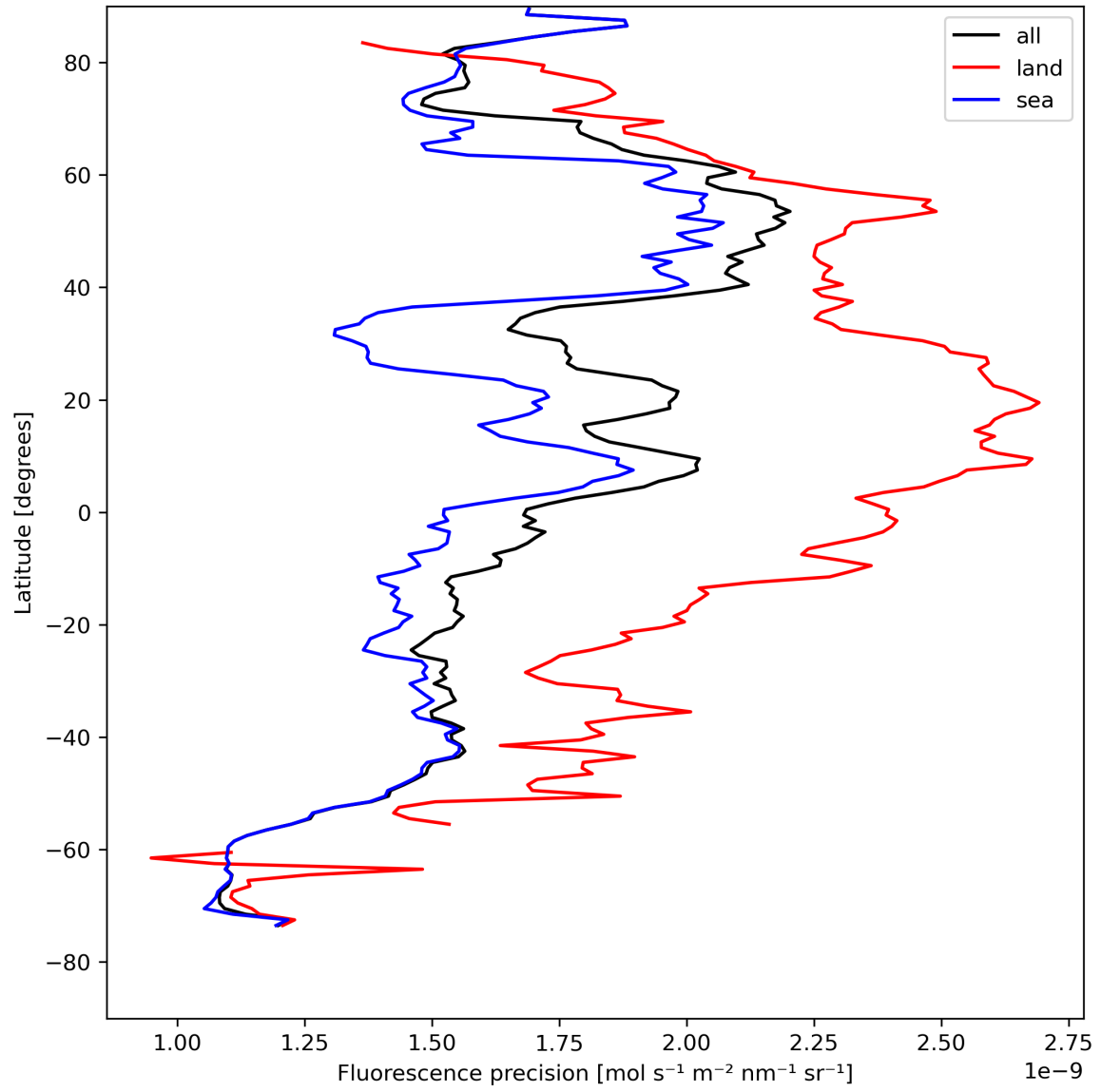
Figure 24: Zonal average of “Fluorescence precision” for 2023-08-12 to 2023-08-14.
