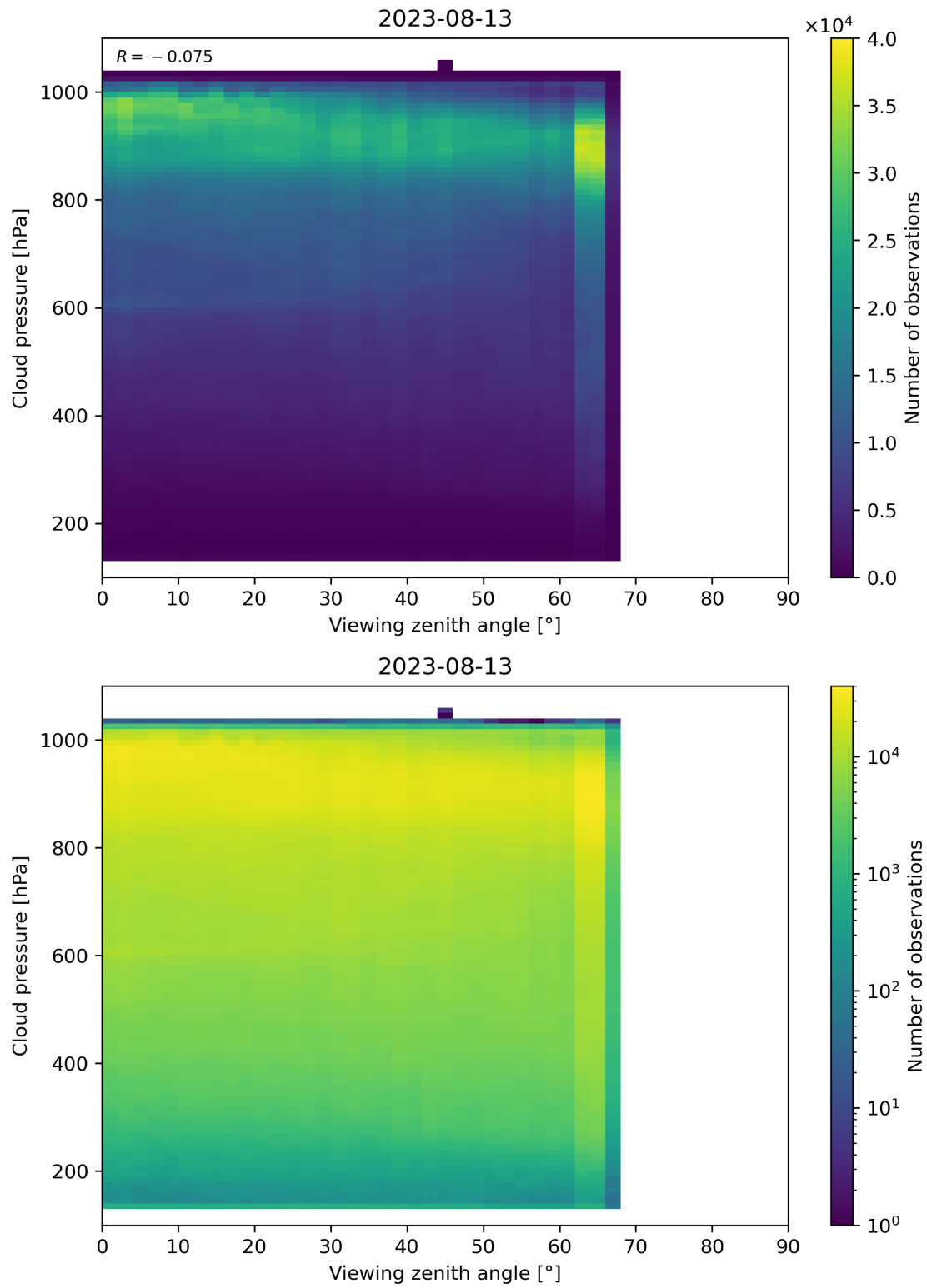
Figure 133: Scatter density plot of “Viewing zenith angle” against “Cloud pressure” for 2023-08-12 to 2023-08-14.
