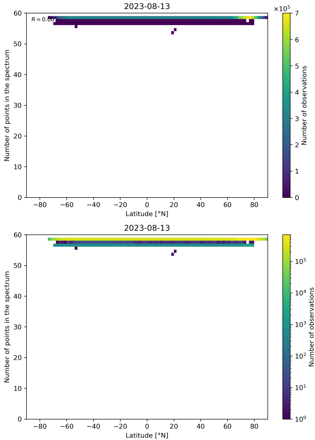
Figure 103: Scatter density plot of “Latitude” against “Number of points in the spectrum” for 2023-08-12 to 2023-08-14.
