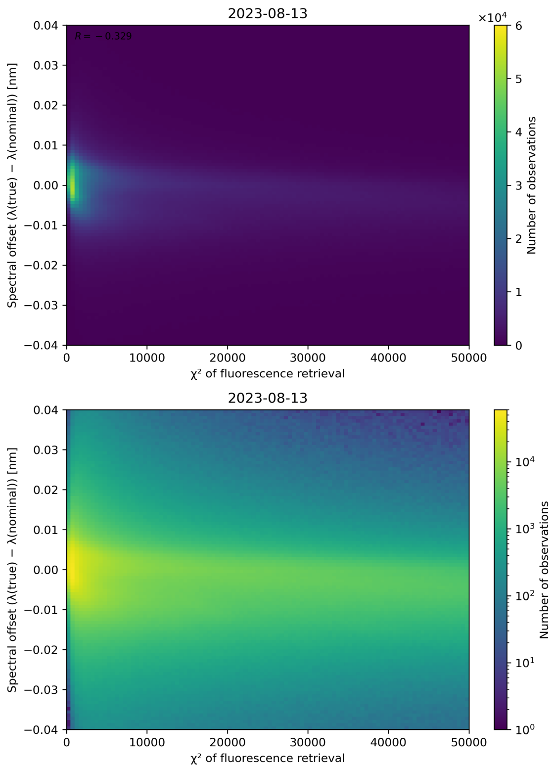
Figure 72: Scatter density plot of " \chi^2 of fluorescence retrieval" against "Spectral offset ( \lambda(\text{true}) - \lambda(\text{nominal})) " for 2023-08-12 to 2023-08-14.
