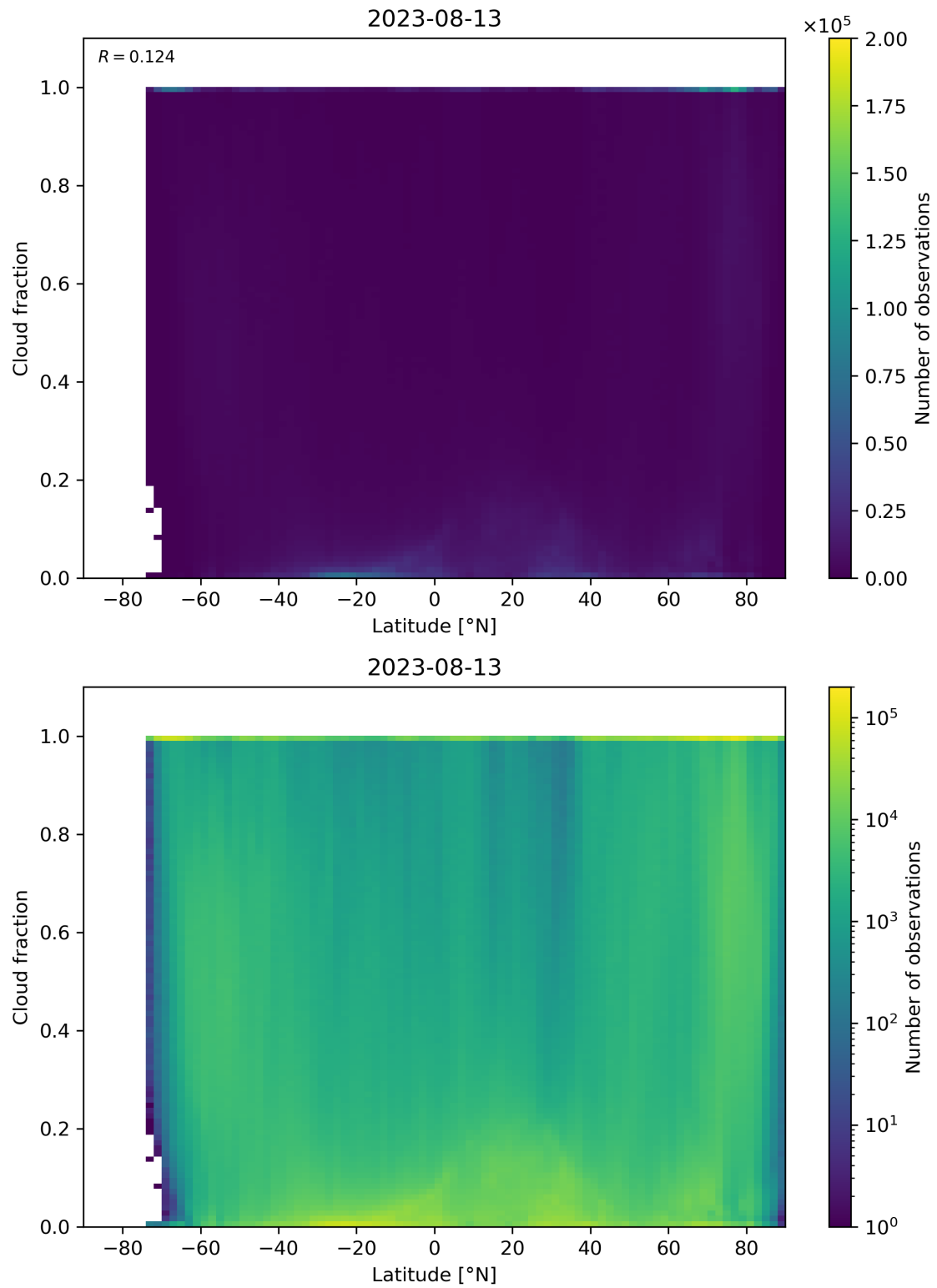
Figure 99: Scatter density plot of “Latitude” against “Cloud fraction” for 2023-08-12 to 2023-08-14.
