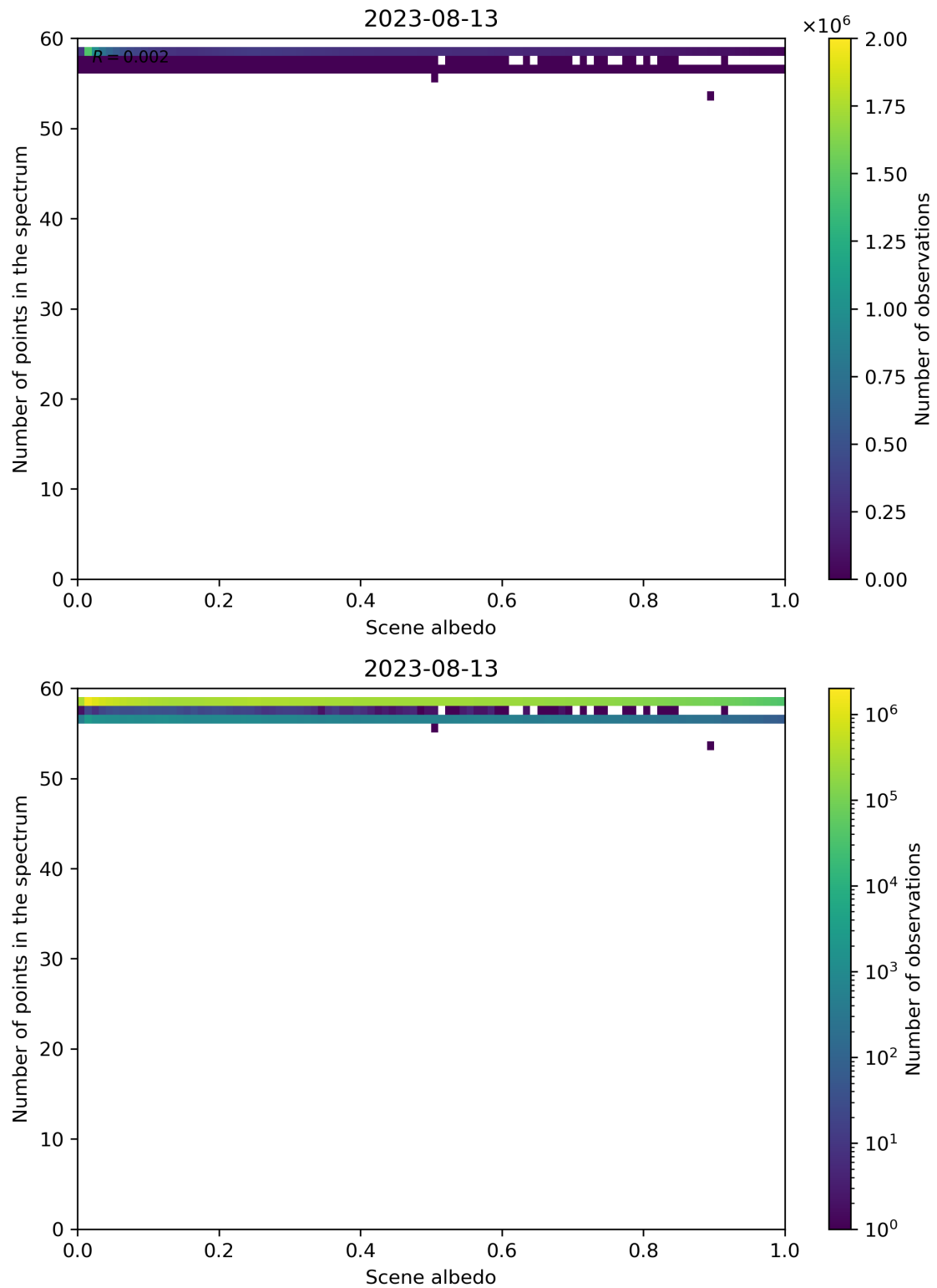
Figure 116: Scatter density plot of “Scene albedo” against “Number of points in the spectrum” for 2023-08-12 to 2023-08-14.
