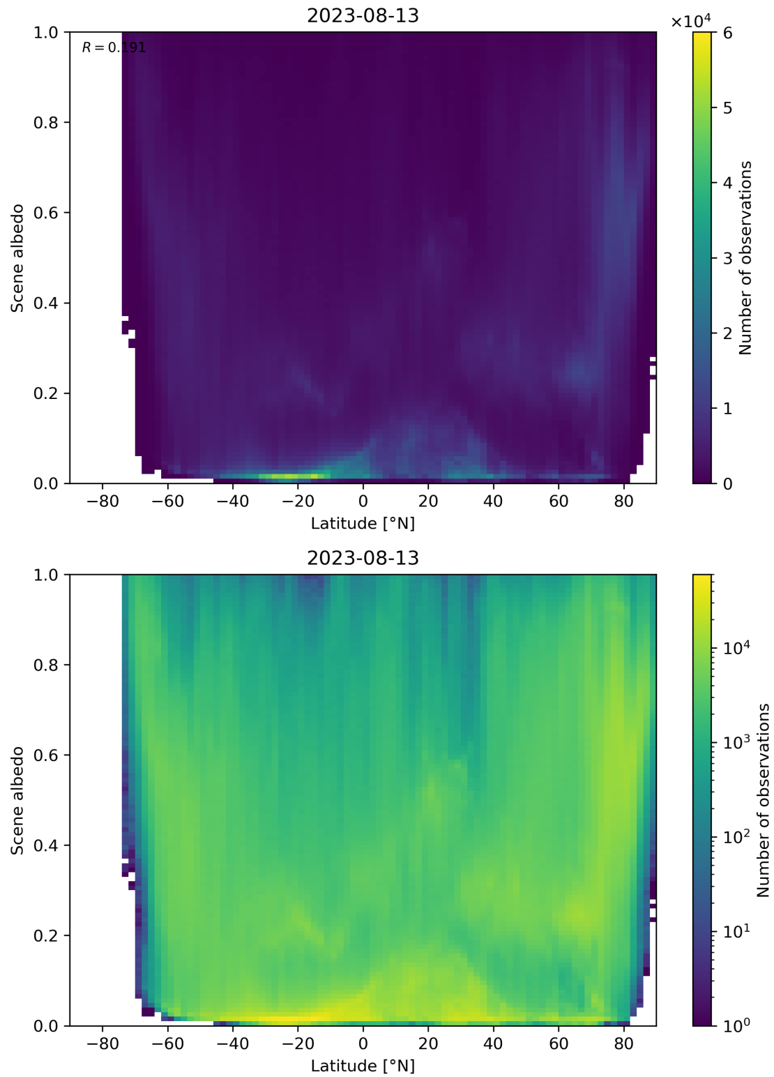
Figure 104: Scatter density plot of “Latitude” against “Scene albedo” for 2023-08-12 to 2023-08-14.
