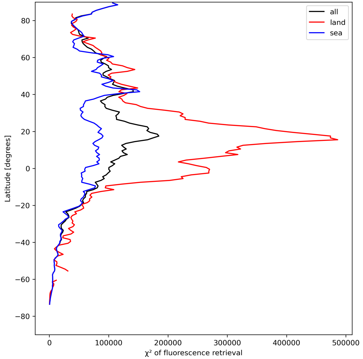
Figure 25: Zonal average of “ \chi^2 of fluorescence retrieval” for 2023-08-12 to 2023-08-14.
