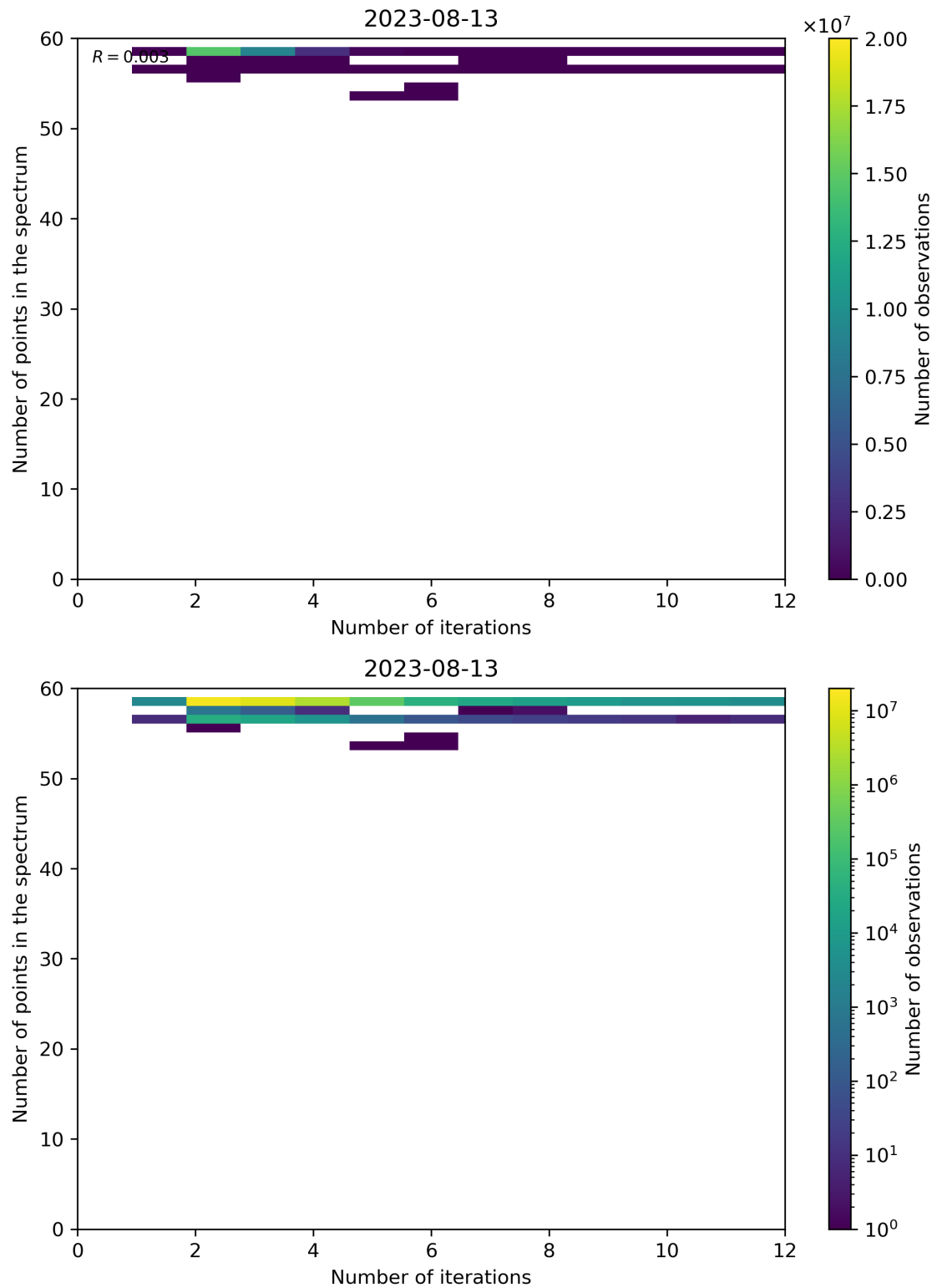
Figure 108: Scatter density plot of “Number of iterations” against “Number of points in the spectrum” for 2023-08-12 to 2023-08-14.
