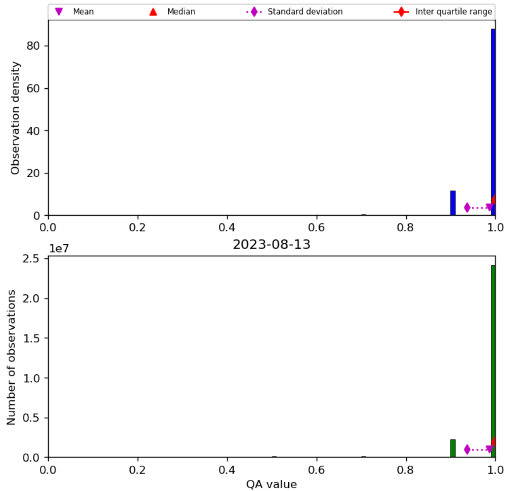
Figure 29: Histogram of “QA value” for 2023-08-12 to 2023-08-14
