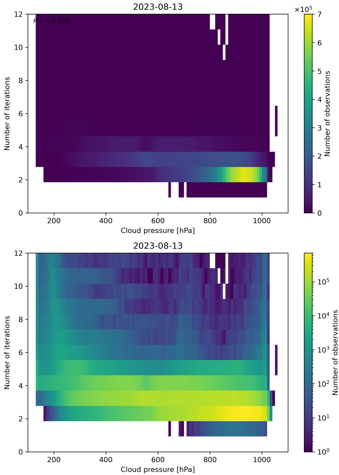
Figure 89: Scatter density plot of “Cloud pressure” against “Number of iterations” for 2023-08-12 to 2023-08-14.
