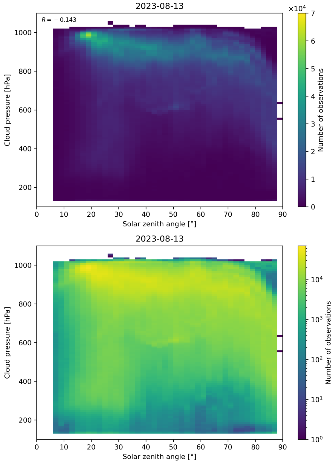
Figure 122: Scatter density plot of “Solar zenith angle” against “Cloud pressure” for 2023-08-12 to 2023-08-14.
