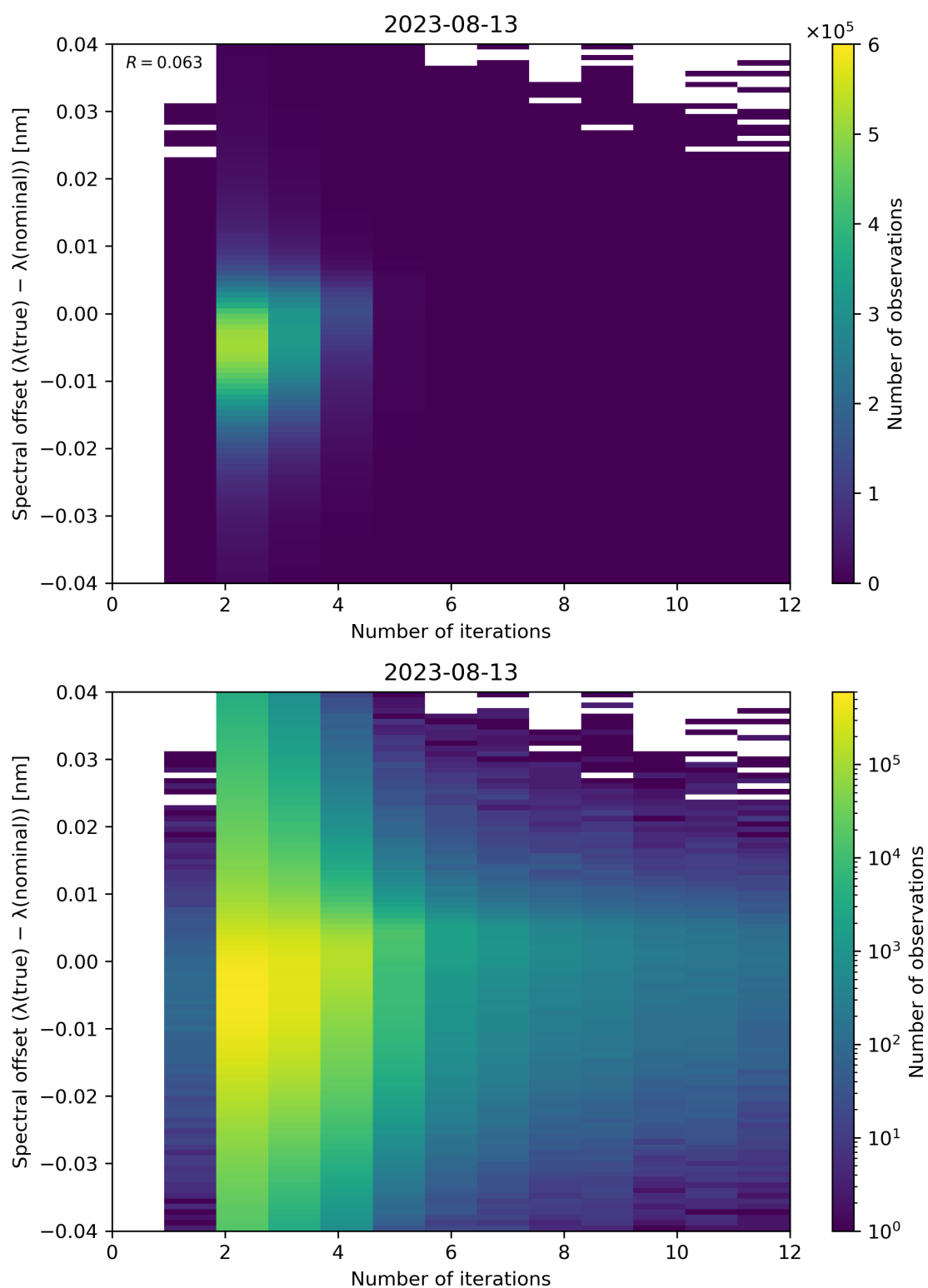
Figure 109: Scatter density plot of “Number of iterations” against “Spectral offset ( \lambda(\text{true}) - \lambda(\text{nominal}) )” for 2023-08-12 to 2023-08-14.
