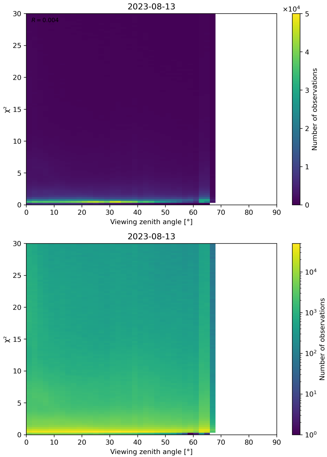
Figure 130: Scatter density plot of “Viewing zenith angle” against “ \chi^2 ” for 2023-08-12 to 2023-08-14.
