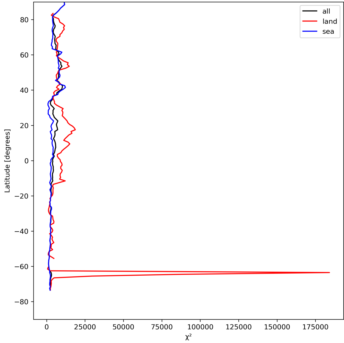
Figure 21: Zonal average of “ \chi^2 ” for 2023-08-12 to 2023-08-14.
