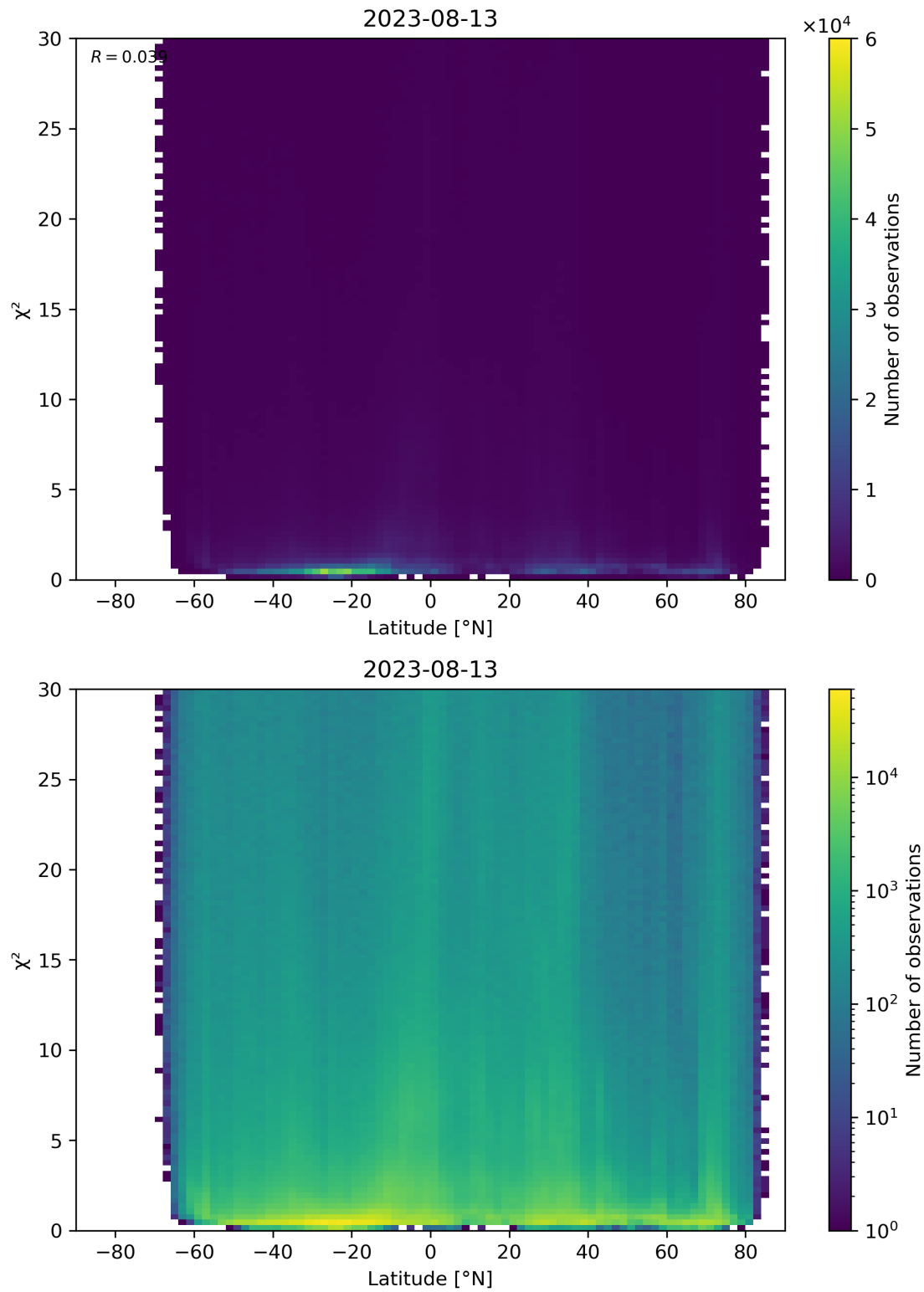
Figure 97: Scatter density plot of “Latitude” against “ \chi^2 ” for 2023-08-12 to 2023-08-14.
