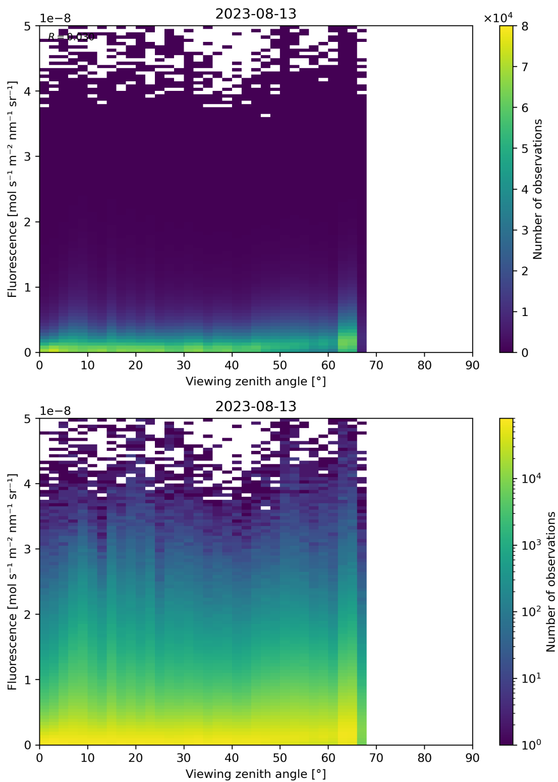
Figure 134: Scatter density plot of “Viewing zenith angle” against “Fluorescence” for 2023-08-12 to 2023-08-14.
