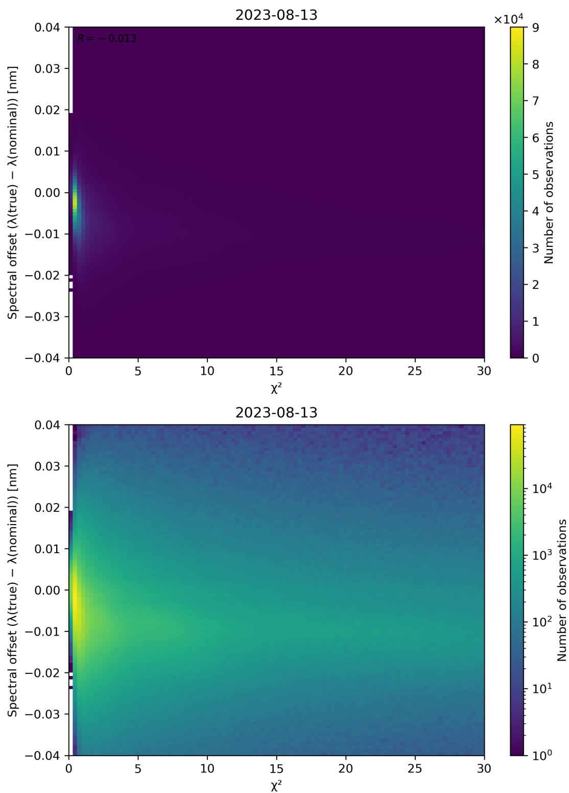
Figure 75: Scatter density plot of “ \chi^2 ” against “Spectral offset ( \lambda(\text{true}) - \lambda(\text{nominal}) )” for 2023-08-12 to 2023-08-14.
