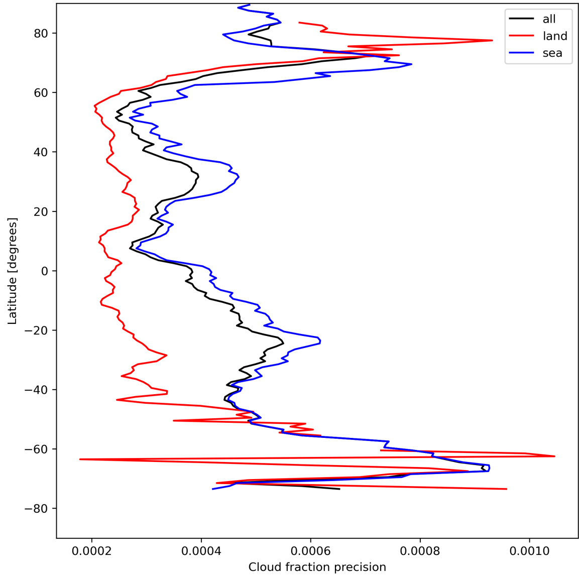
Figure 16: Zonal average of “Cloud fraction precision” for 2023-08-12 to 2023-08-14.
