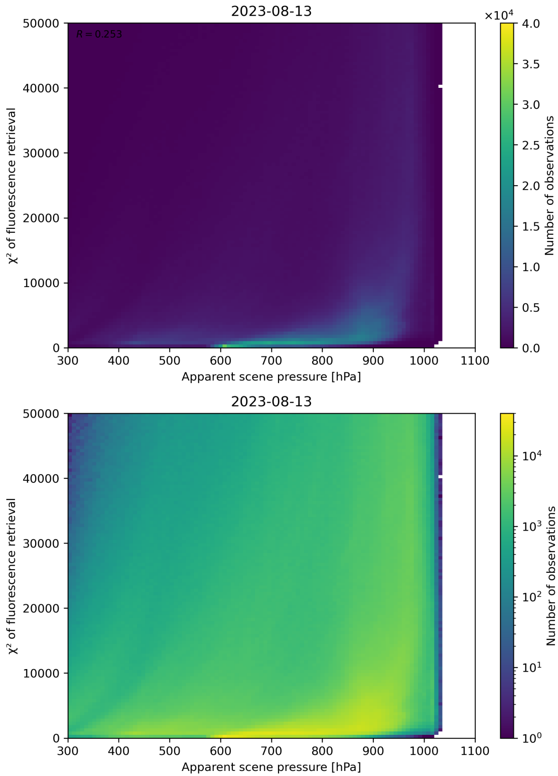
Figure 64: Scatter density plot of “Apparent scene pressure” against “ \chi^2 of fluorescence retrieval” for 2023-08-12 to 2023-08-14.
