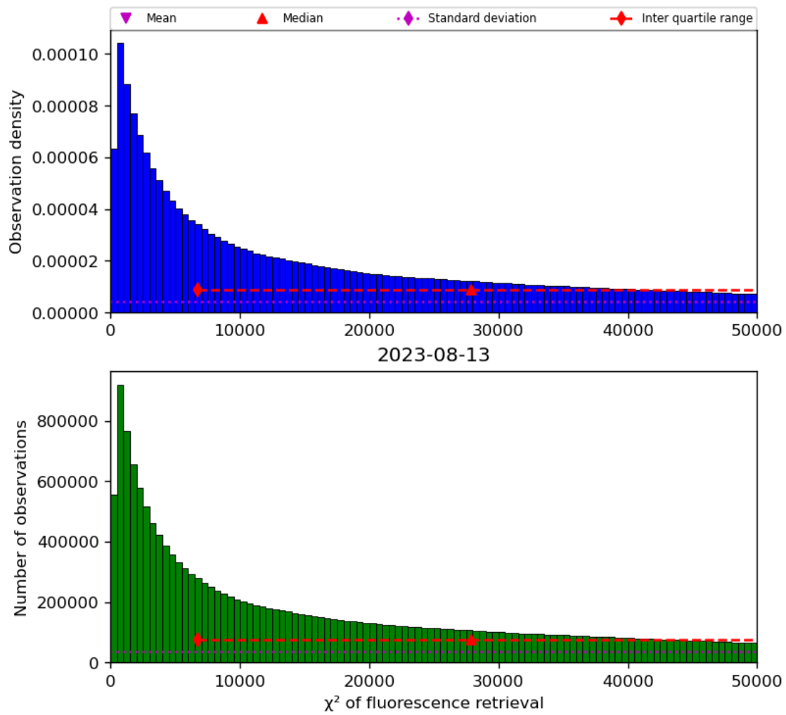
Figure 42: Histogram of “ \chi^2 of fluorescence retrieval” for 2023-08-12 to 2023-08-14
