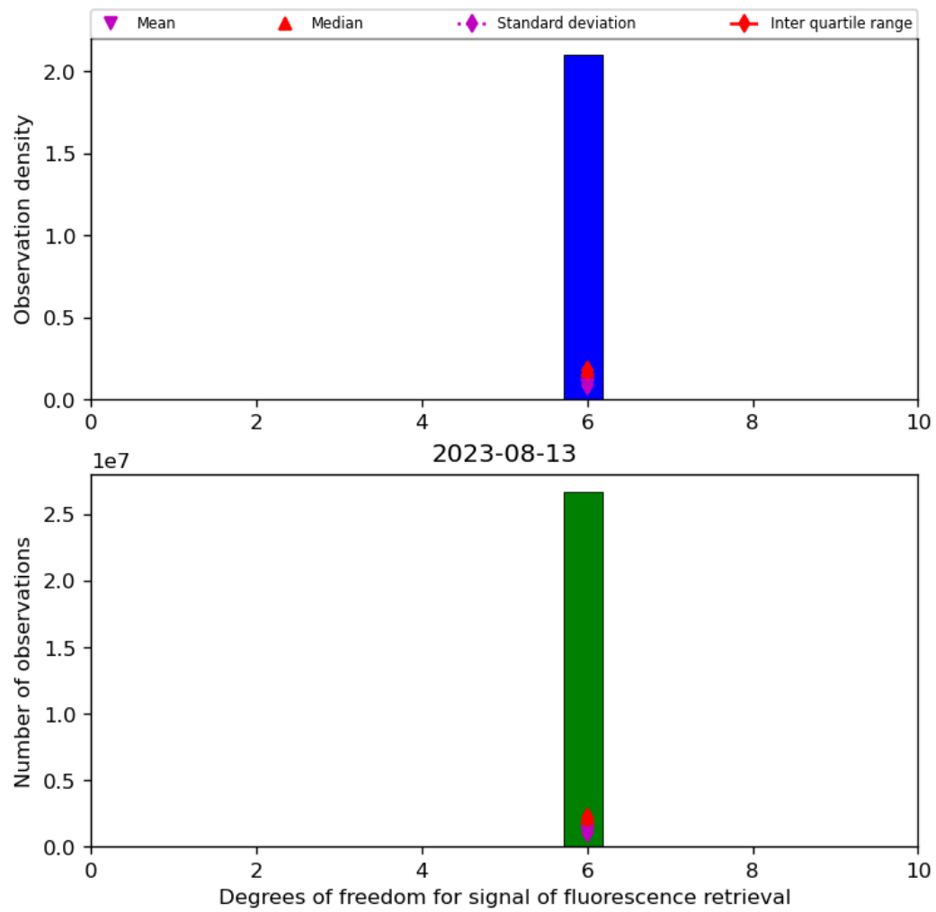
Figure 43: Histogram of “Degrees of freedom for signal of fluorescence retrieval” for 2023-08-12 to 2023-08-14
