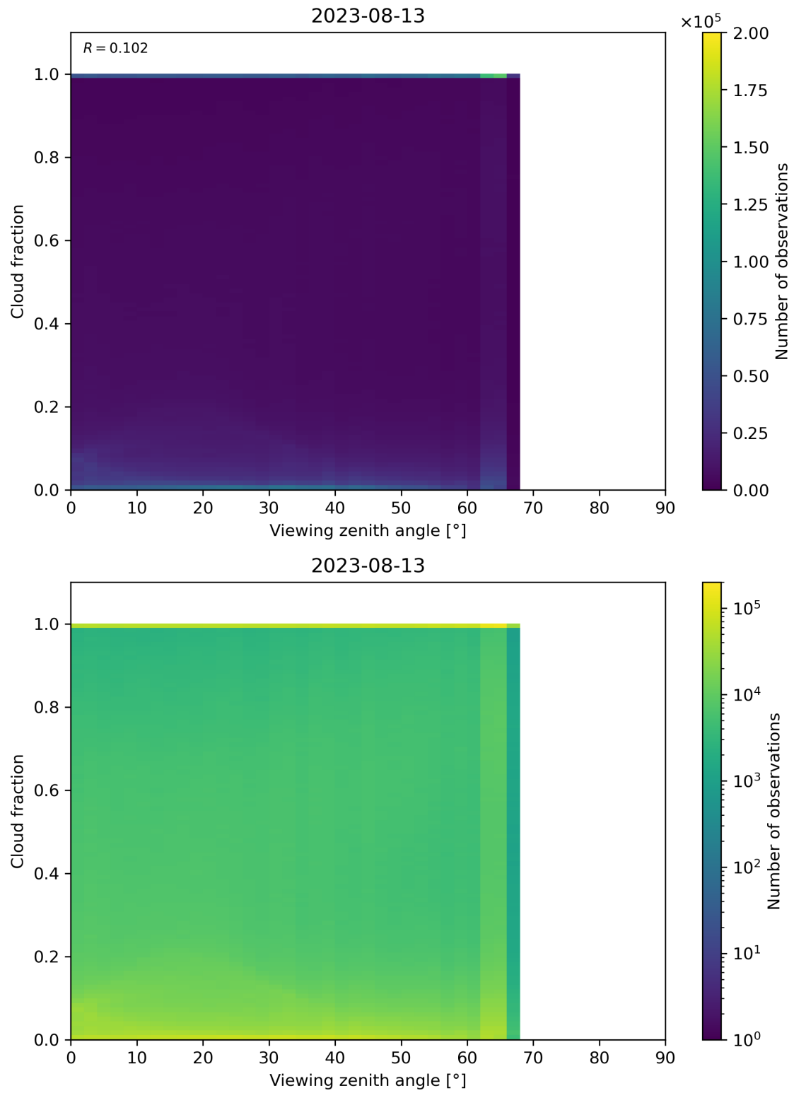
Figure 132: Scatter density plot of “Viewing zenith angle” against “Cloud fraction” for 2023-08-12 to 2023-08-14.
