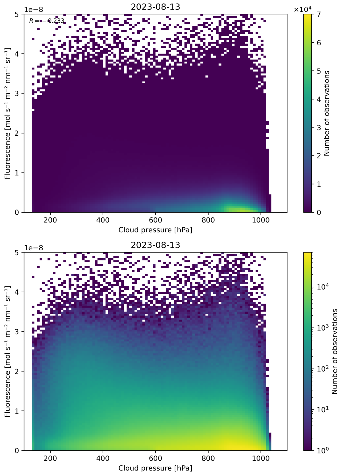
Figure 88: Scatter density plot of “Cloud pressure” against “Fluorescence” for 2023-08-12 to 2023-08-14.
