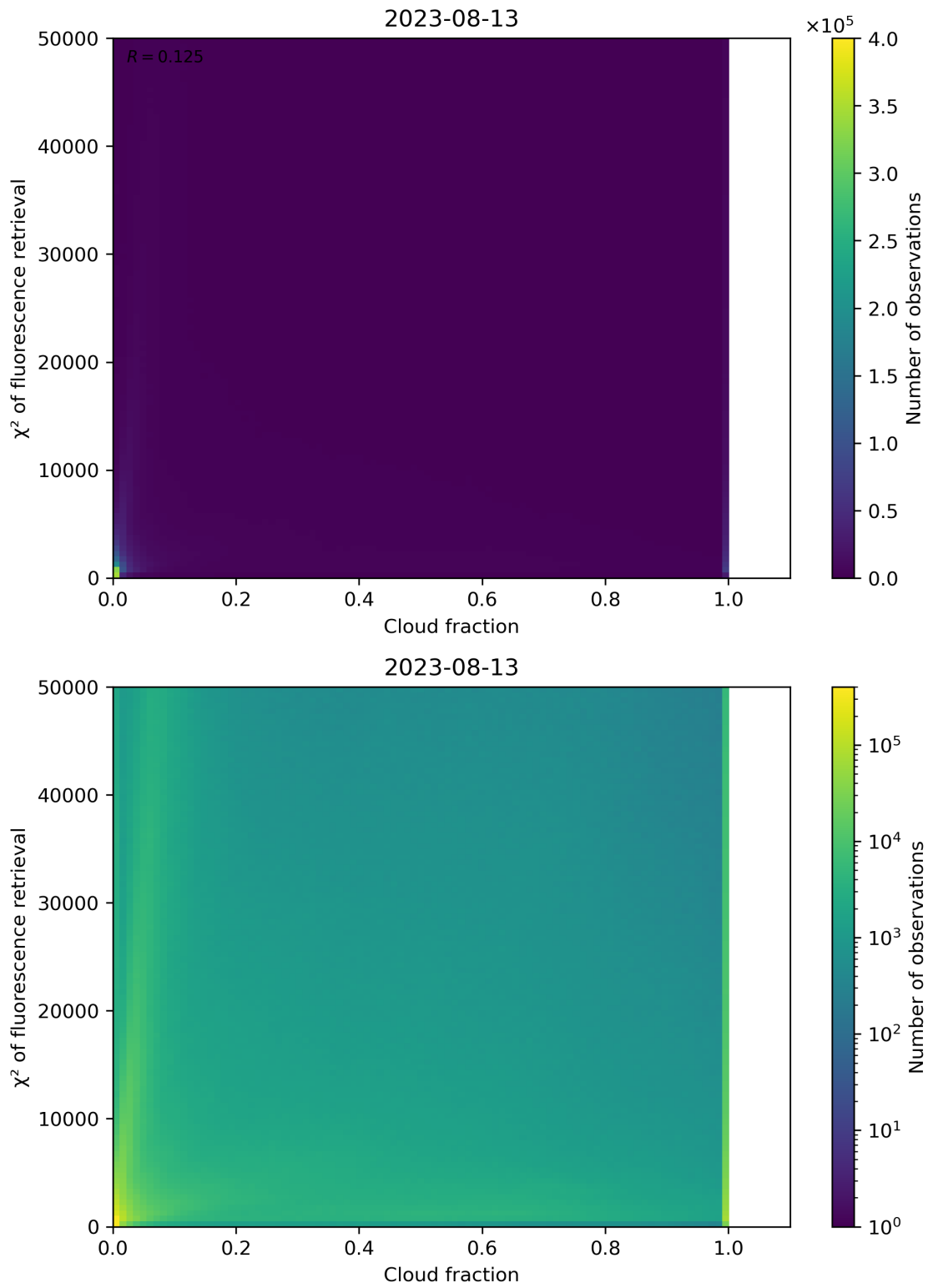
Figure 78: Scatter density plot of “Cloud fraction” against “ \chi^2 of fluorescence retrieval” for 2023-08-12 to 2023-08-14.
