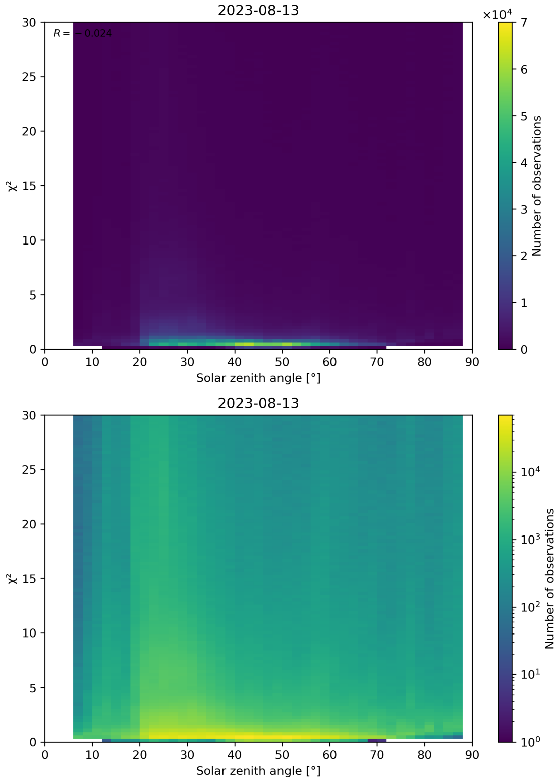
Figure 119: Scatter density plot of “Solar zenith angle” against “ \chi^2 ” for 2023-08-12 to 2023-08-14.
