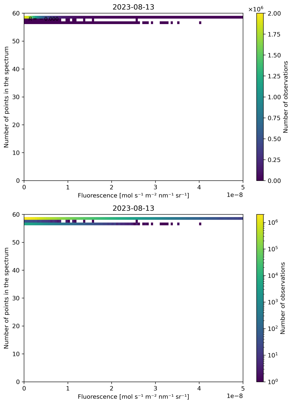
Figure 94: Scatter density plot of “Fluorescence” against “Number of points in the spectrum” for 2023-08-12 to 2023-08-14.
