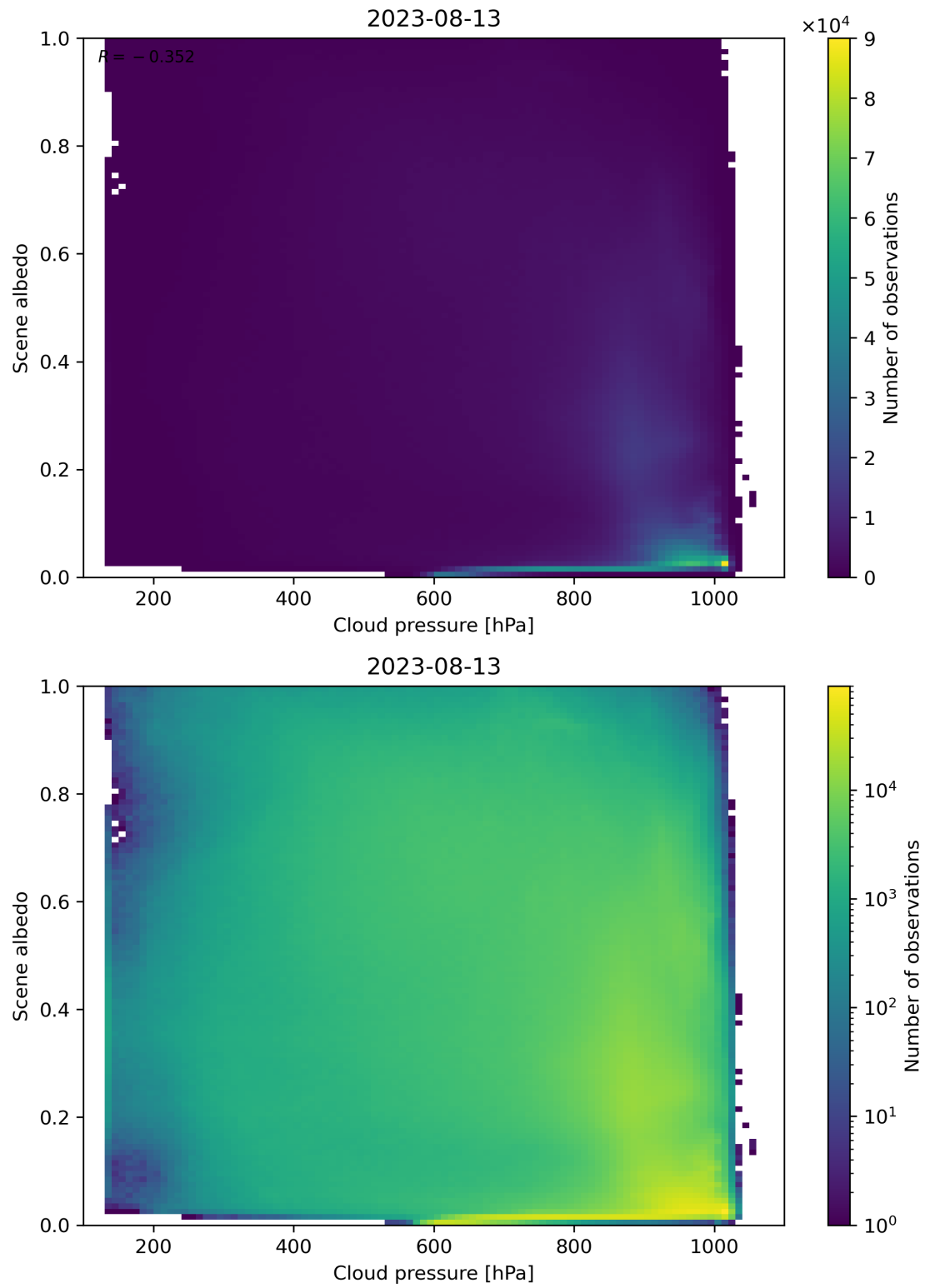
Figure 91: Scatter density plot of “Cloud pressure” against “Scene albedo” for 2023-08-12 to 2023-08-14.
