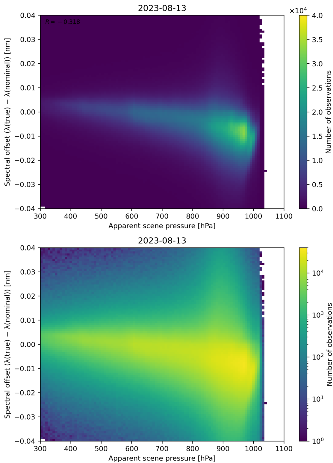
Figure 68: Scatter density plot of “Apparent scene pressure” against “Spectral offset ( \lambda(\text{true}) - \lambda(\text{nominal}) )” for 2023-08-12 to 2023-08-14.
