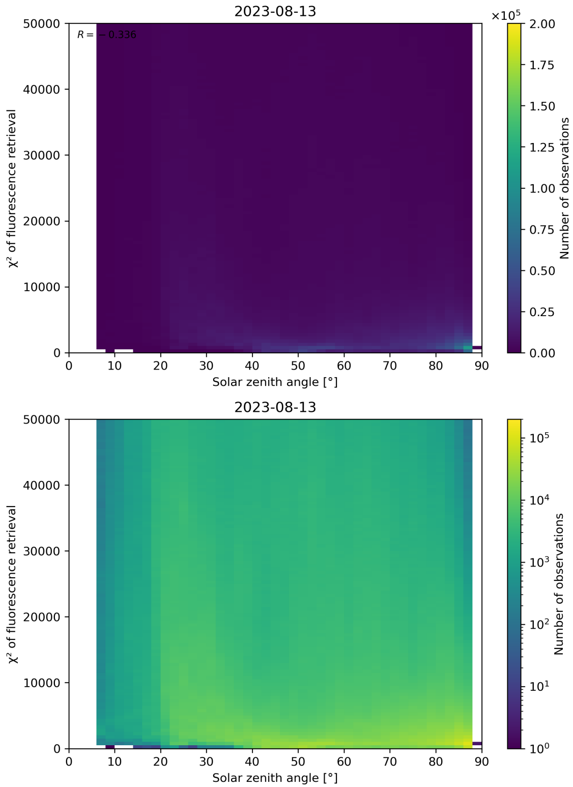
Figure 120: Scatter density plot of “Solar zenith angle” against “ \chi^2 of fluorescence retrieval” for 2023-08-12 to 2023-08-14.
