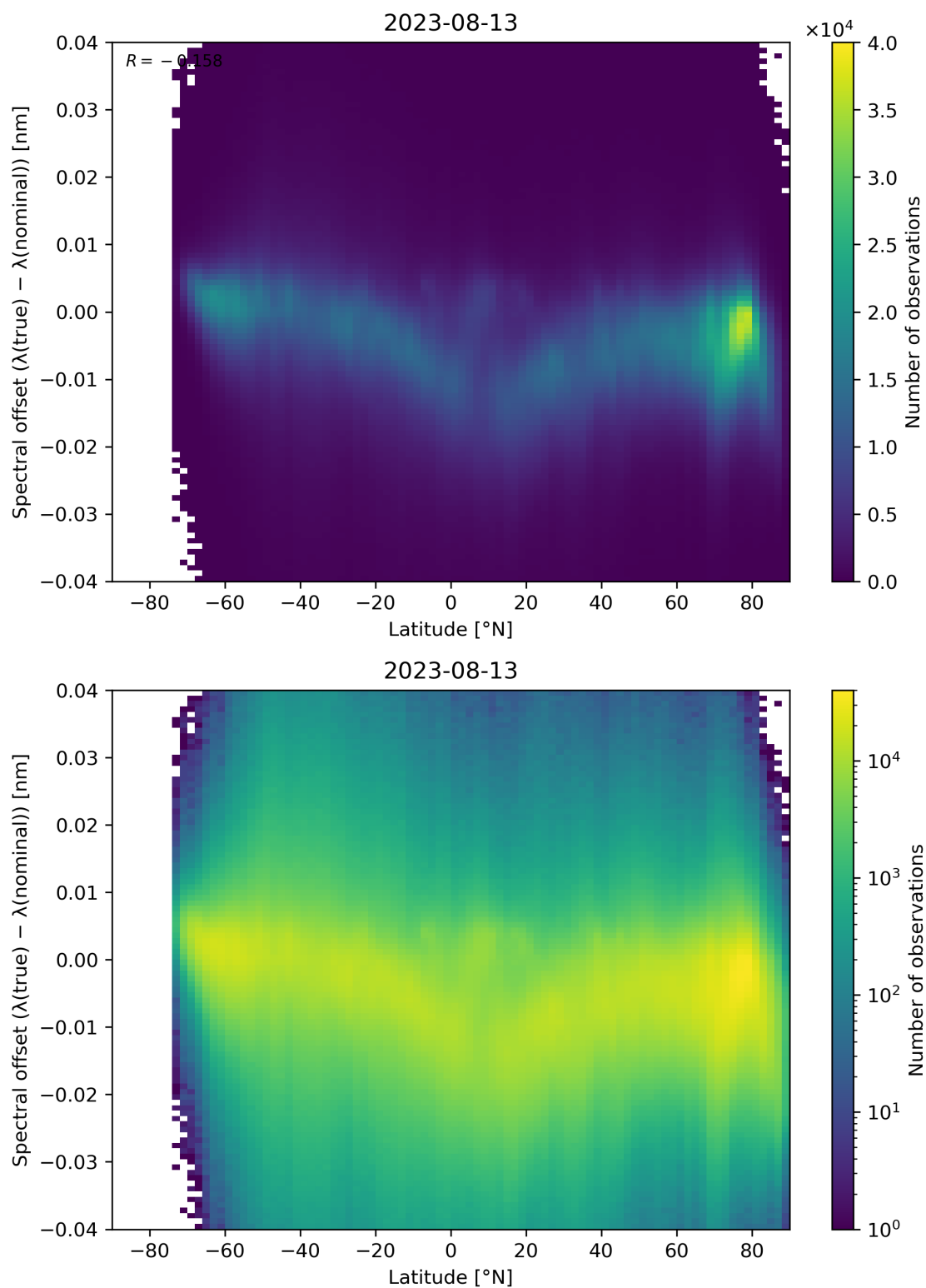
Figure 105: Scatter density plot of “Latitude” against “Spectral offset ( \lambda(\text{true}) - \lambda(\text{nominal}) )” for 2023-08-12 to 2023-08-14.
