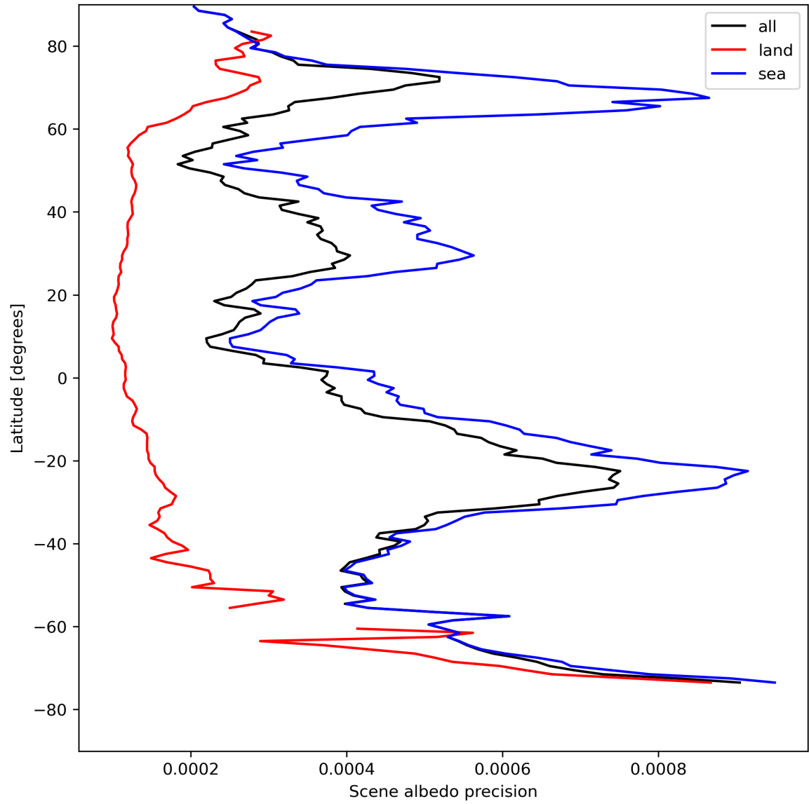
Figure 18: Zonal average of “Scene albedo precision” for 2023-08-12 to 2023-08-14.
