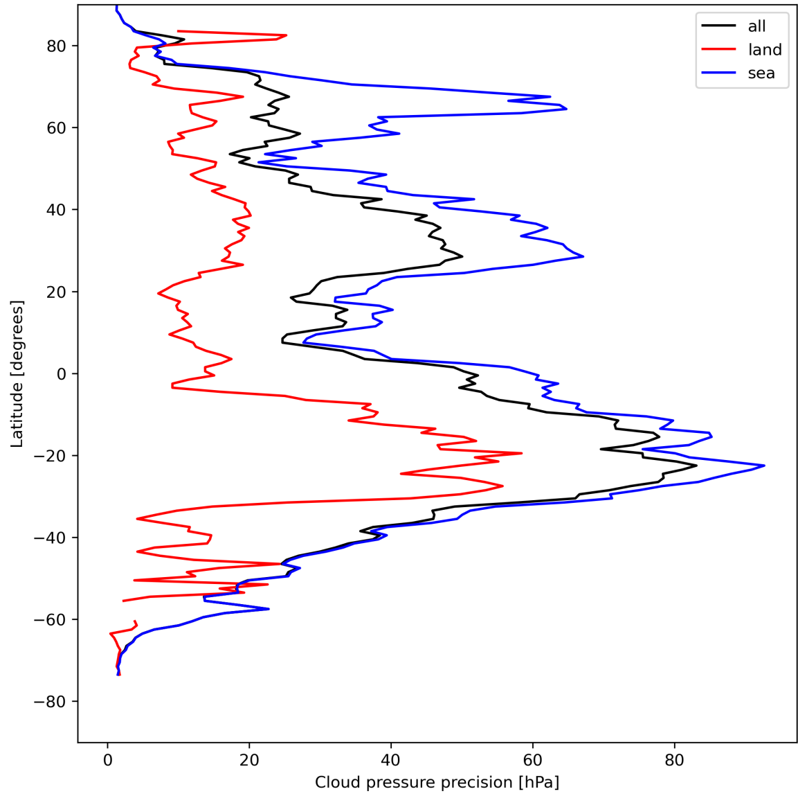
Figure 14: Zonal average of “Cloud pressure precision” for 2023-08-12 to 2023-08-14.
