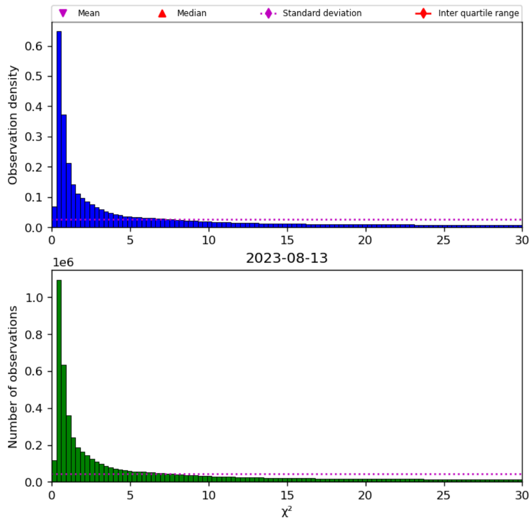
Figure 38: Histogram of “ \chi^2 ” for 2023-08-12 to 2023-08-14
