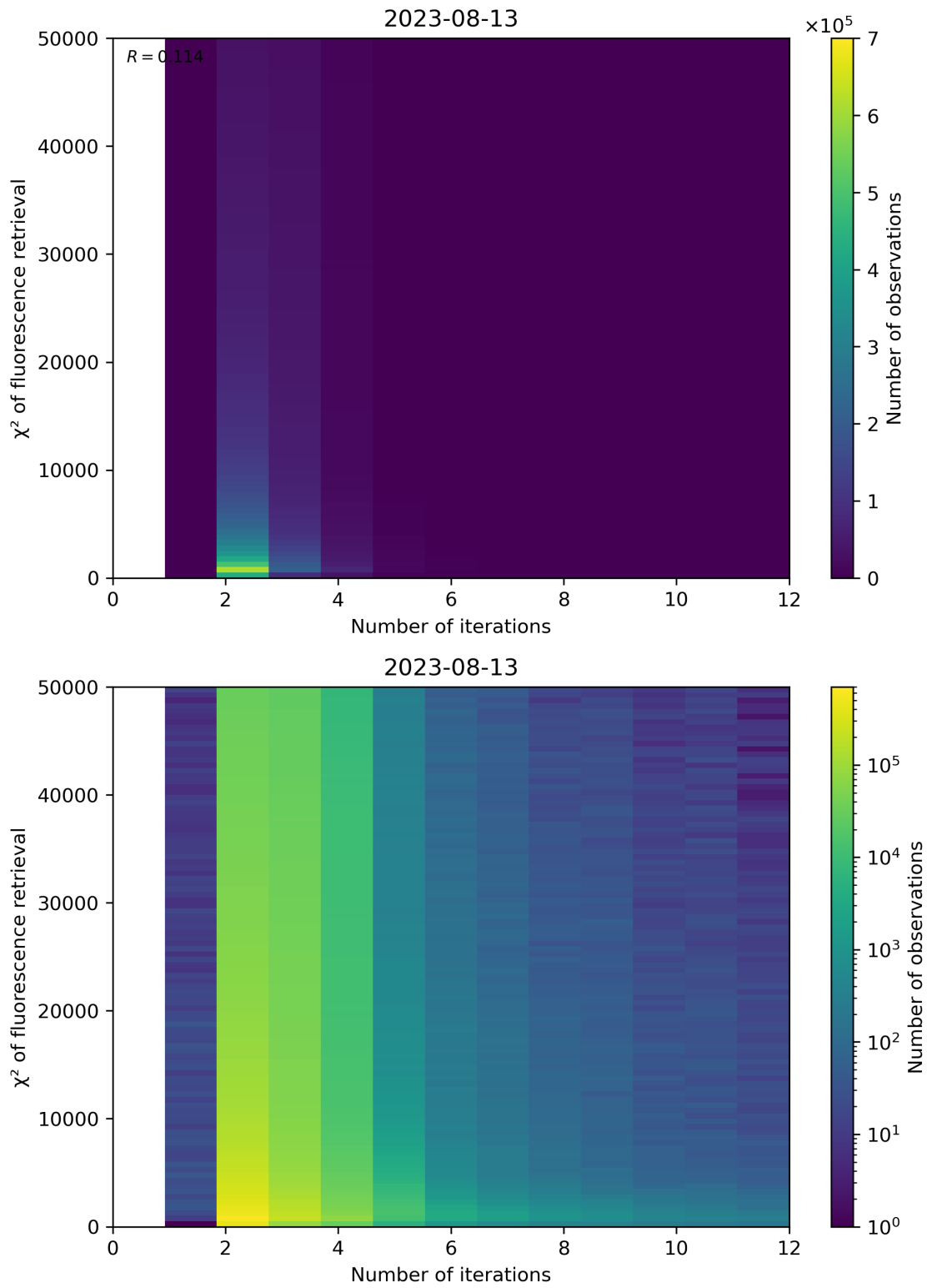
Figure 106: Scatter density plot of “Number of iterations” against “ \chi^2 of fluorescence retrieval” for 2023-08-12 to 2023-08-14.
