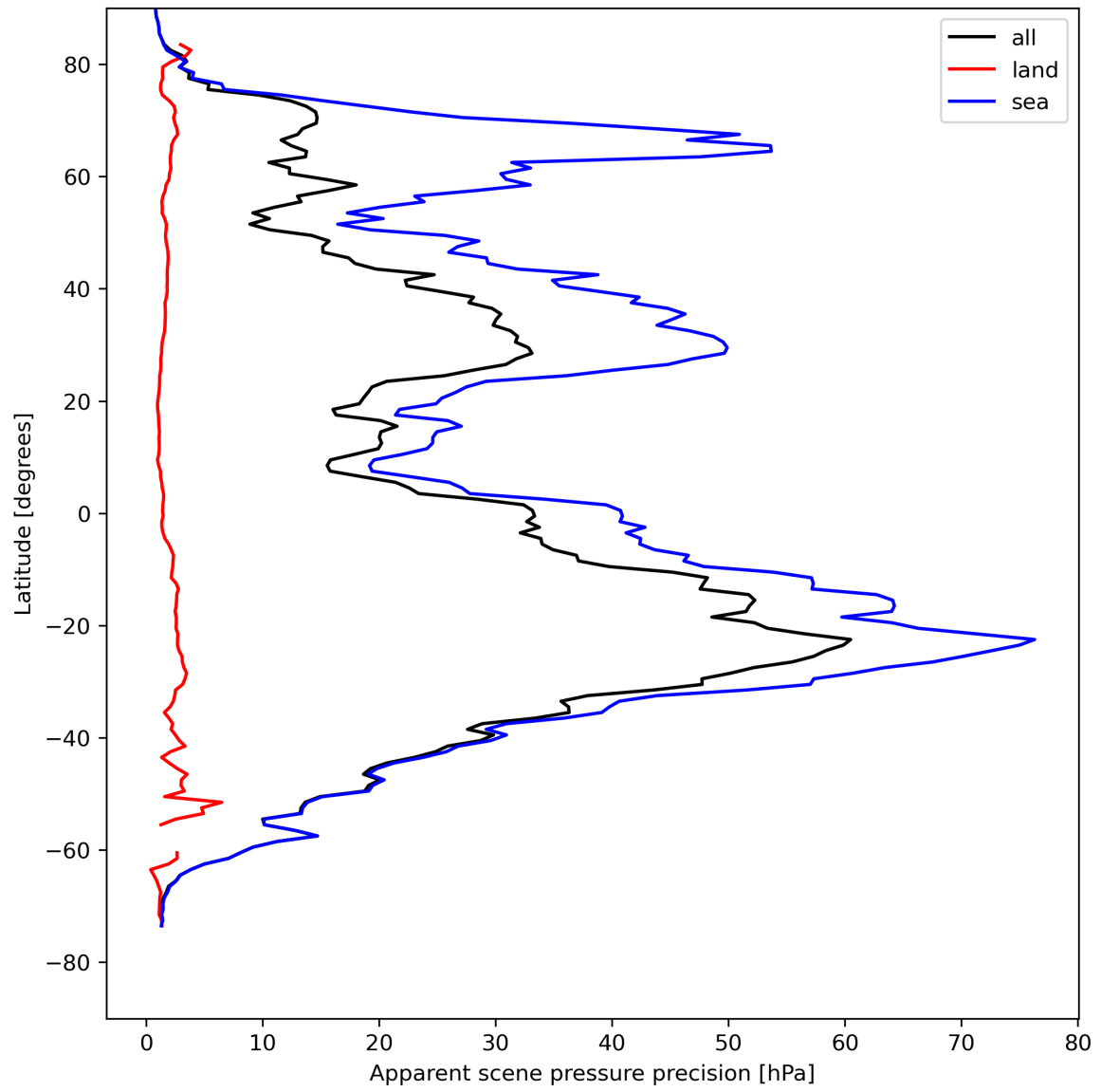
Figure 20: Zonal average of “Apparent scene pressure precision” for 2023-08-12 to 2023-08-14.
