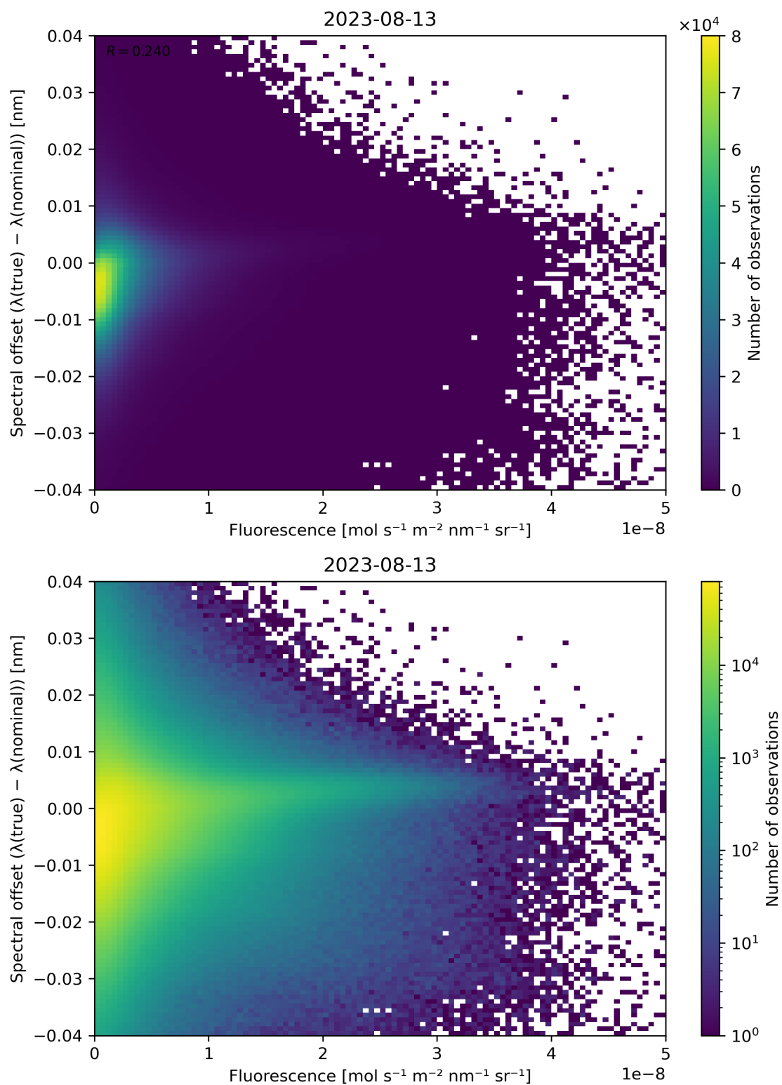
Figure 95: Scatter density plot of “Fluorescence” against “Spectral offset ( \lambda(\text{true}) - \lambda(\text{nominal}) )” for 2023-08-12 to 2023-08-14.
