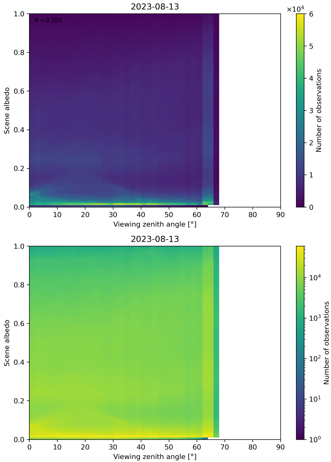
Figure 138: Scatter density plot of “Viewing zenith angle” against “Scene albedo” for 2023-08-12 to 2023-08-14.
