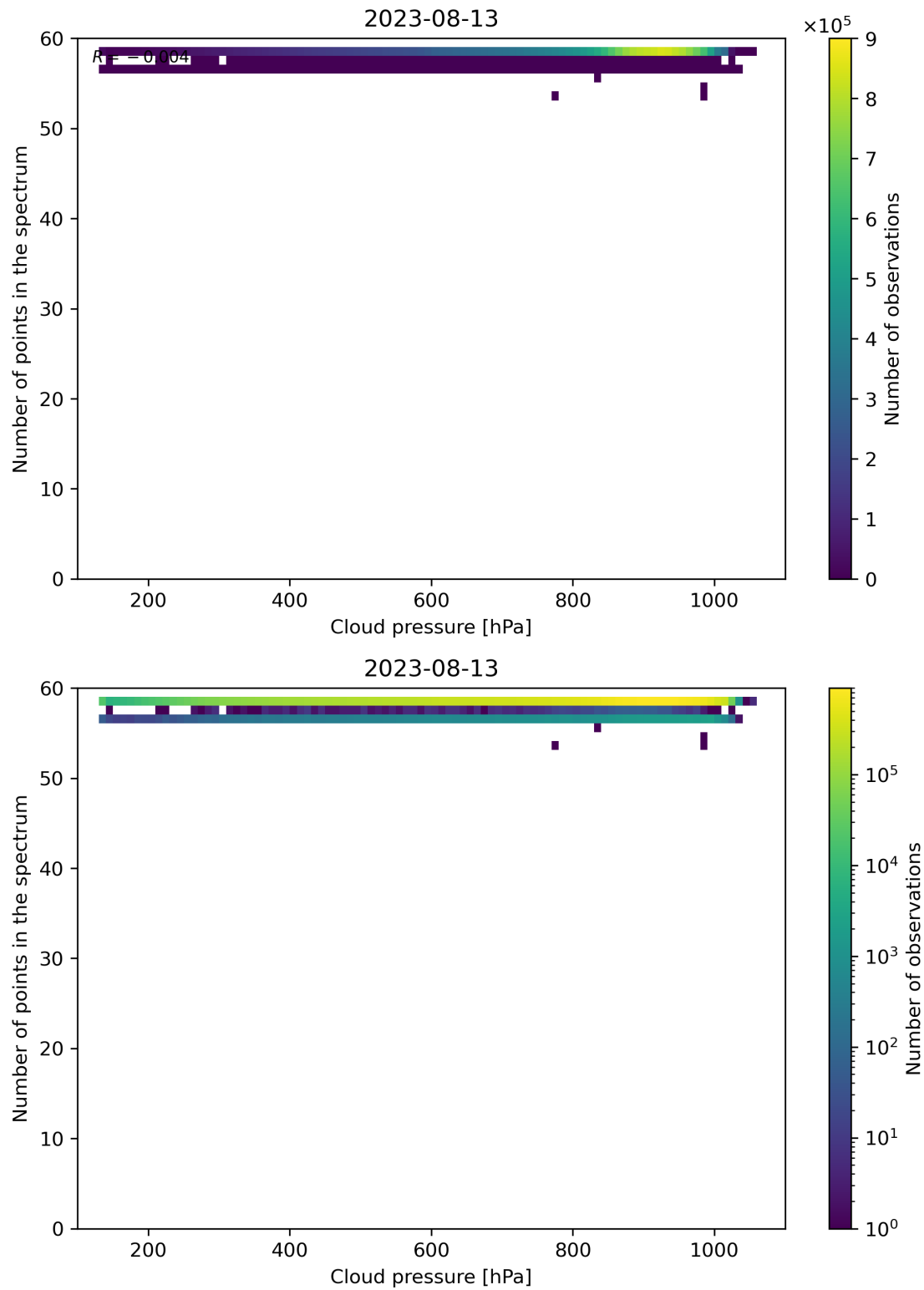
Figure 90: Scatter density plot of “Cloud pressure” against “Number of points in the spectrum” for 2023-08-12 to 2023-08-14.
