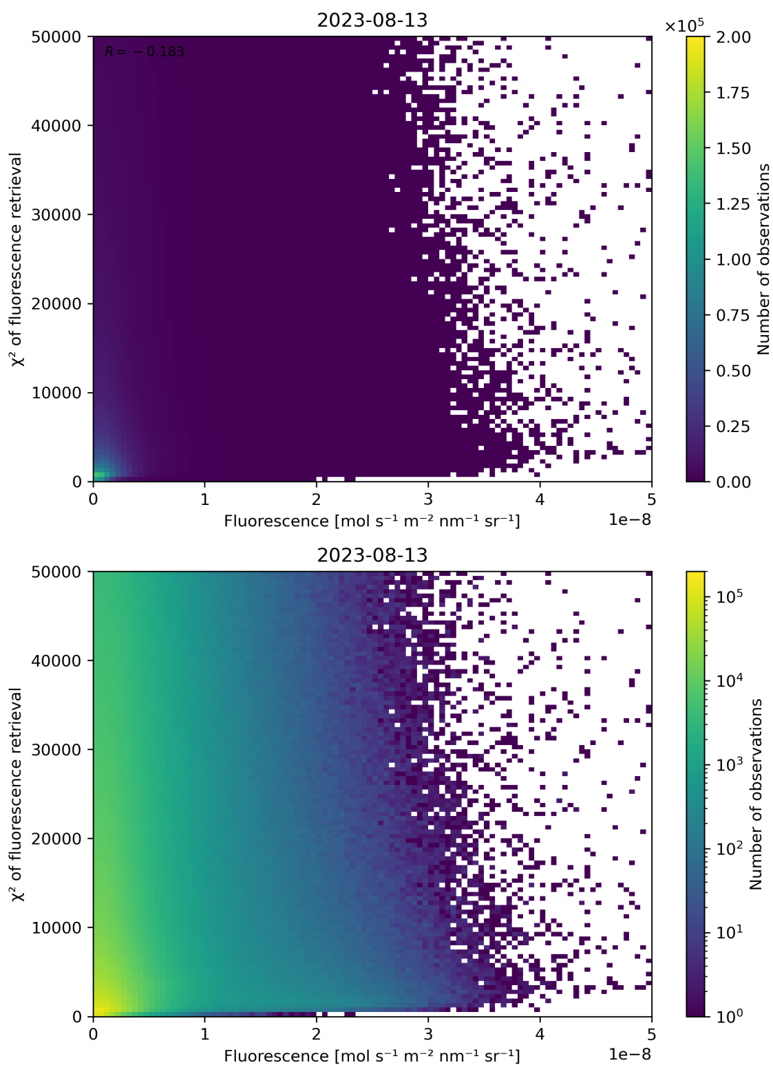
Figure 93: Scatter density plot of “Fluorescence” against “ \chi^2 of fluorescence retrieval” for 2023-08-12 to 2023-08-14.
