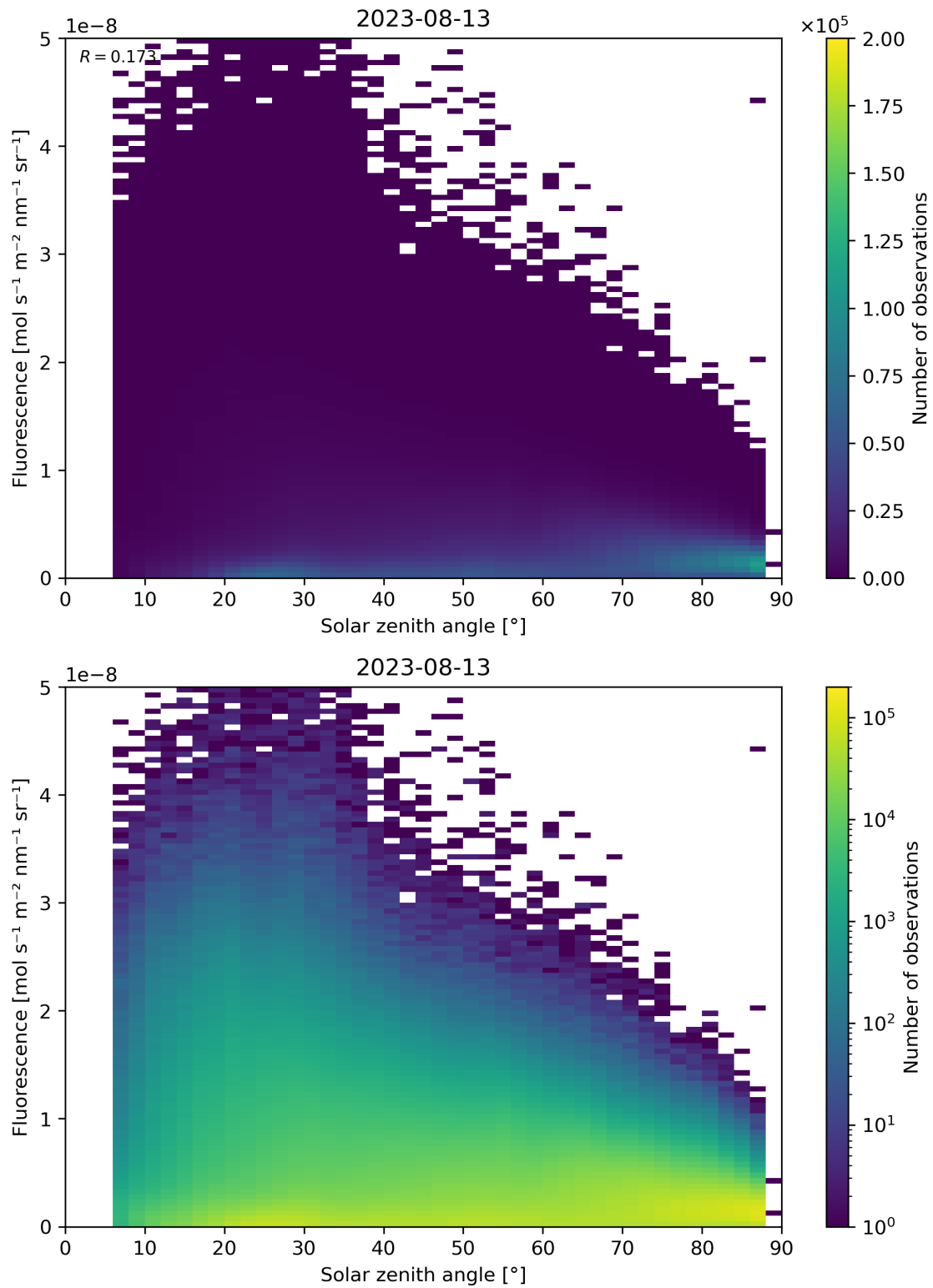
Figure 123: Scatter density plot of “Solar zenith angle” against “Fluorescence” for 2023-08-12 to 2023-08-14.
