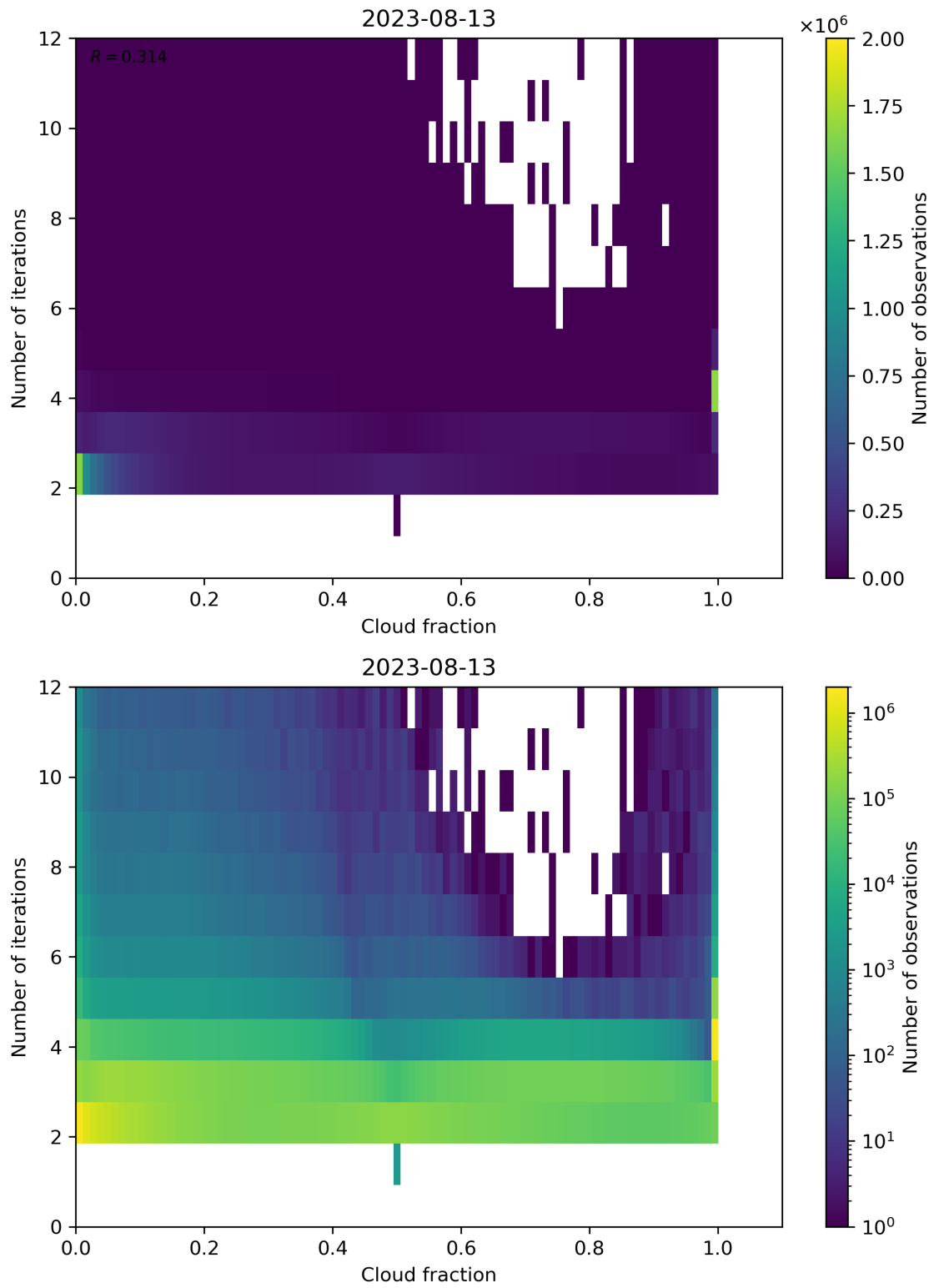
Figure 80: Scatter density plot of “Cloud fraction” against “Number of iterations” for 2023-08-12 to 2023-08-14.
