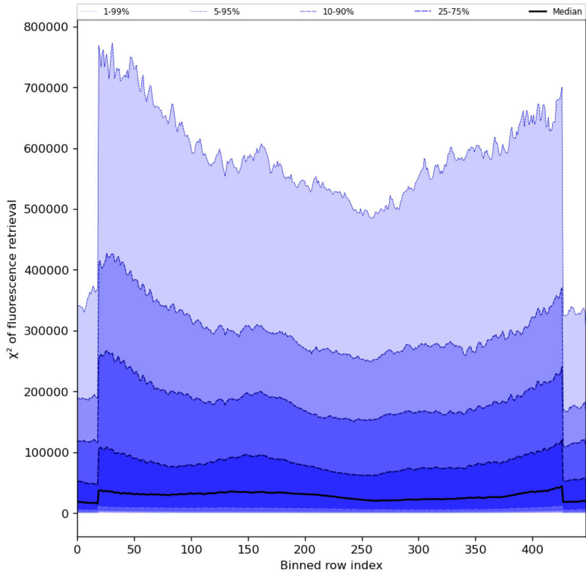
Figure 59: Along track statistics of “ \chi^2 of fluorescence retrieval” for 2023-08-12 to 2023-08-14
