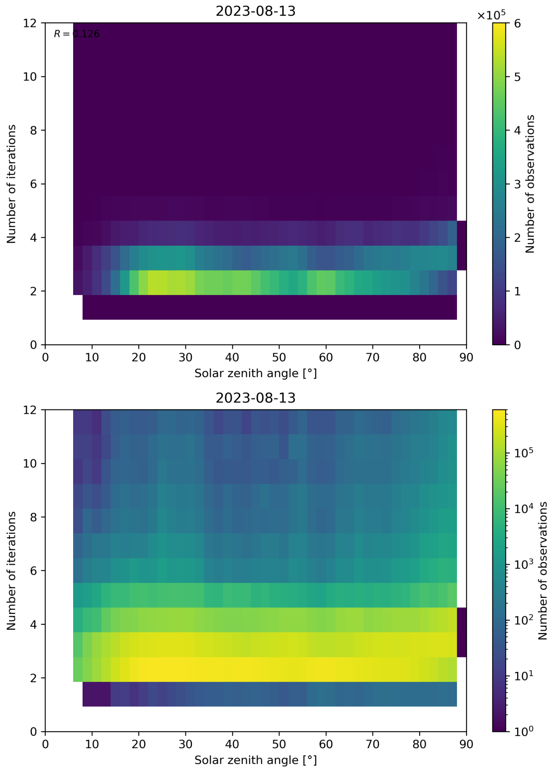
Figure 125: Scatter density plot of “Solar zenith angle” against “Number of iterations” for 2023-08-12 to 2023-08-14.
