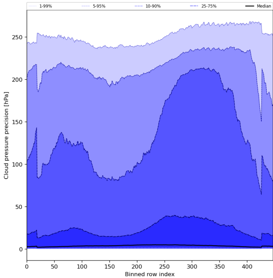
Figure 48: Along track statistics of “Cloud pressure precision” for 2023-08-12 to 2023-08-14
