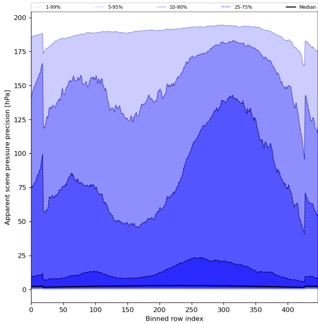
Figure 54: Along track statistics of “Apparent scene pressure precision” for 2023-08-12 to 2023-08-14
