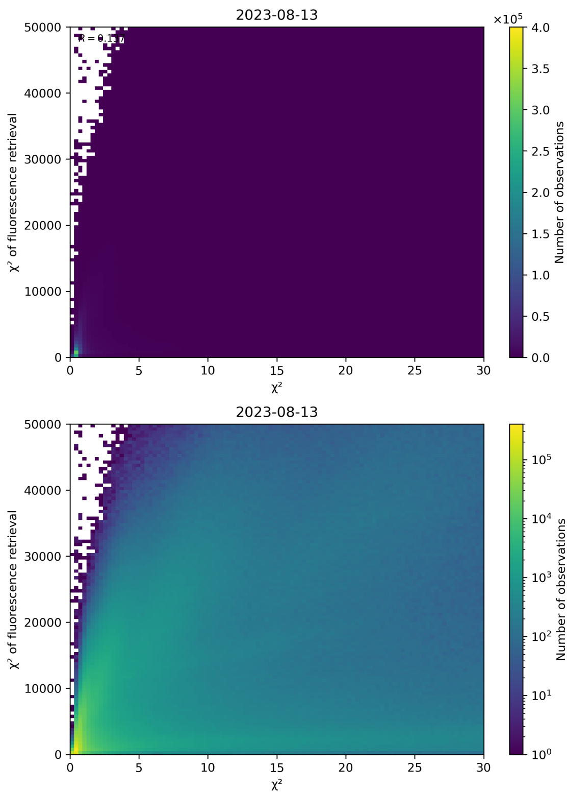
Figure 69: Scatter density plot of “ \chi^2 ” against “ \chi^2 of fluorescence retrieval” for 2023-08-12 to 2023-08-14.
