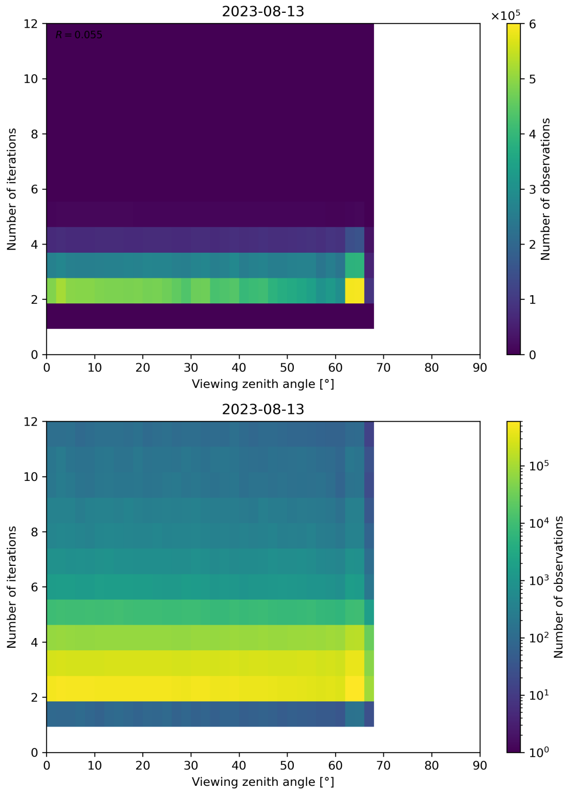
Figure 136: Scatter density plot of “Viewing zenith angle” against “Number of iterations” for 2023-08-12 to 2023-08-14.
