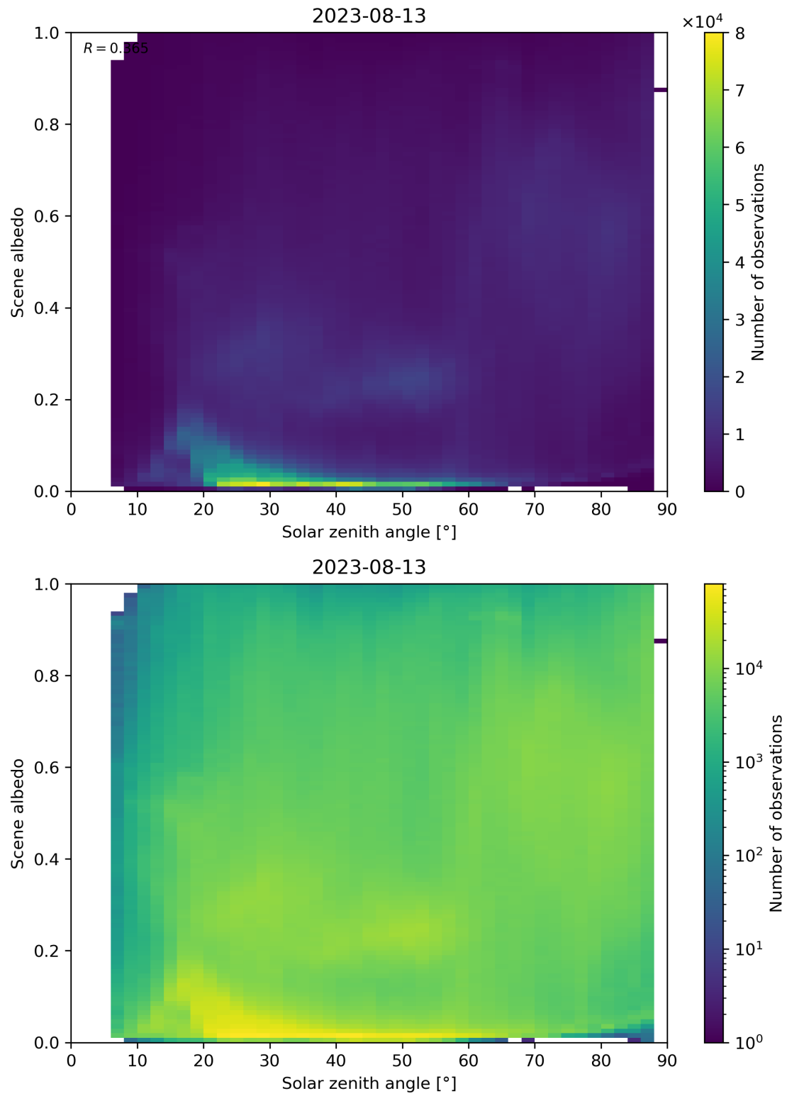
Figure 127: Scatter density plot of “Solar zenith angle” against “Scene albedo” for 2023-08-12 to 2023-08-14.
