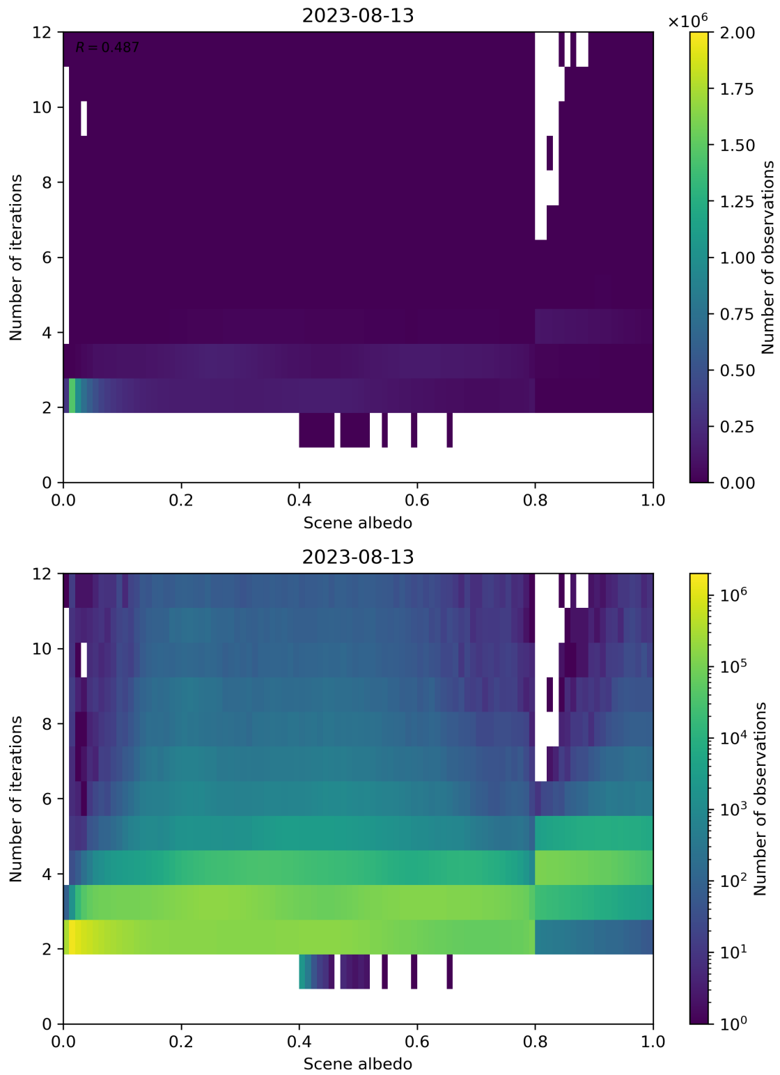
Figure 115: Scatter density plot of “Scene albedo” against “Number of iterations” for 2023-08-12 to 2023-08-14.
