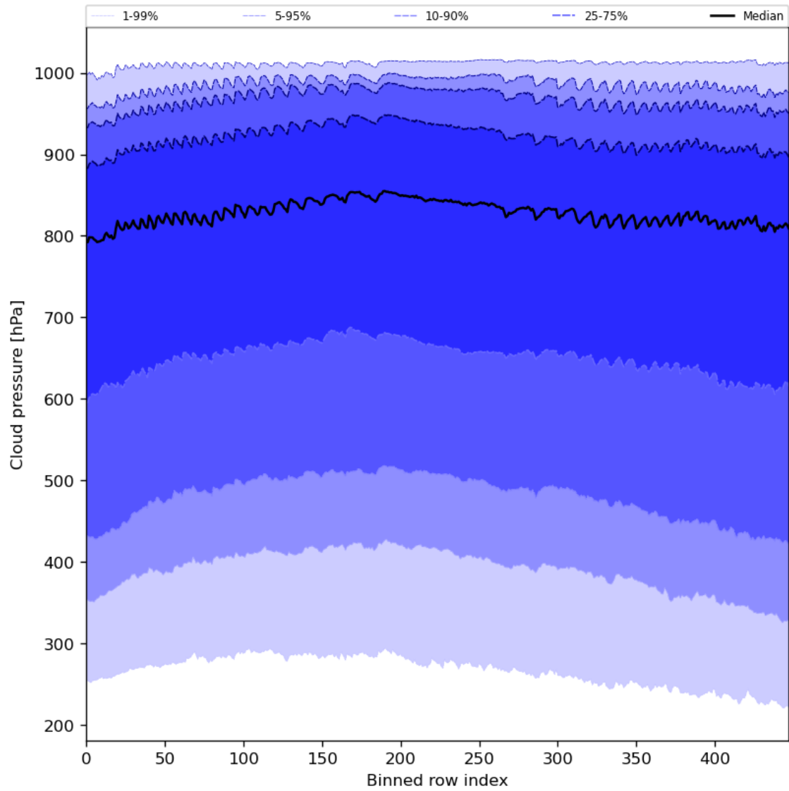
Figure 47: Along track statistics of “Cloud pressure” for 2023-08-12 to 2023-08-14
