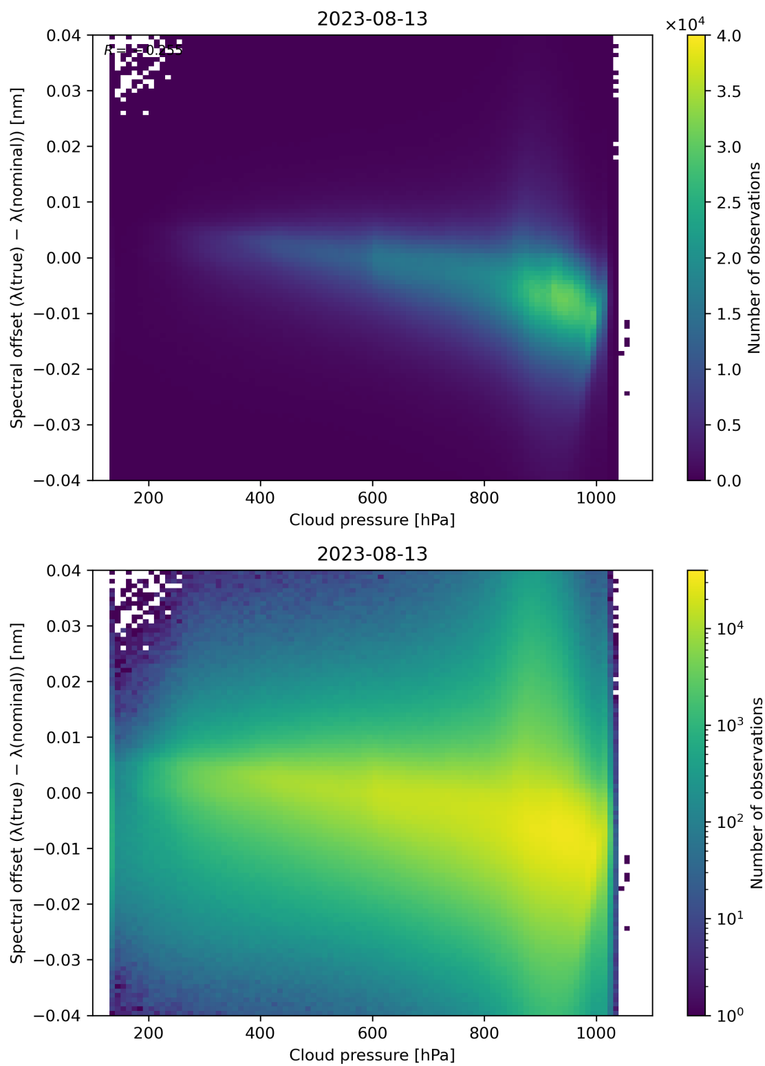
Figure 92: Scatter density plot of “Cloud pressure” against “Spectral offset ( \lambda(\text{true}) - \lambda(\text{nominal}) )” for 2023-08-12 to 2023-08-14.
