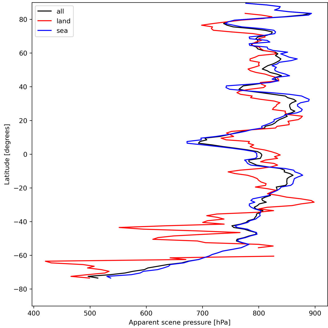
Figure 19: Zonal average of “Apparent scene pressure” for 2023-08-12 to 2023-08-14.
