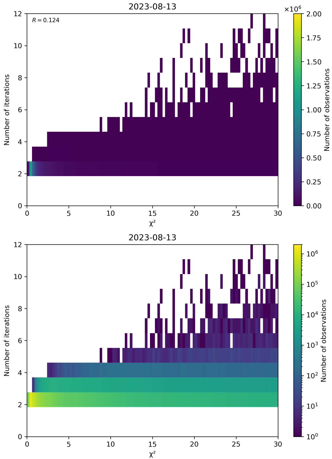
Figure 73: Scatter density plot of “ \chi^2 ” against “Number of iterations” for 2023-08-12 to 2023-08-14.
