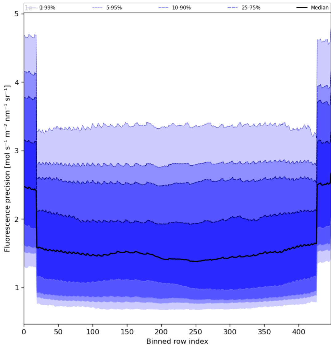
Figure 58: Along track statistics of “Fluorescence precision” for 2023-08-12 to 2023-08-14
