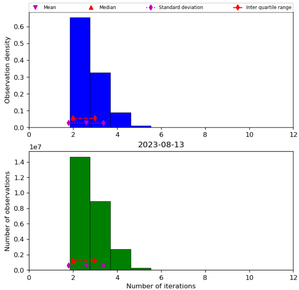
Figure 39: Histogram of “Number of iterations” for 2023-08-12 to 2023-08-14
