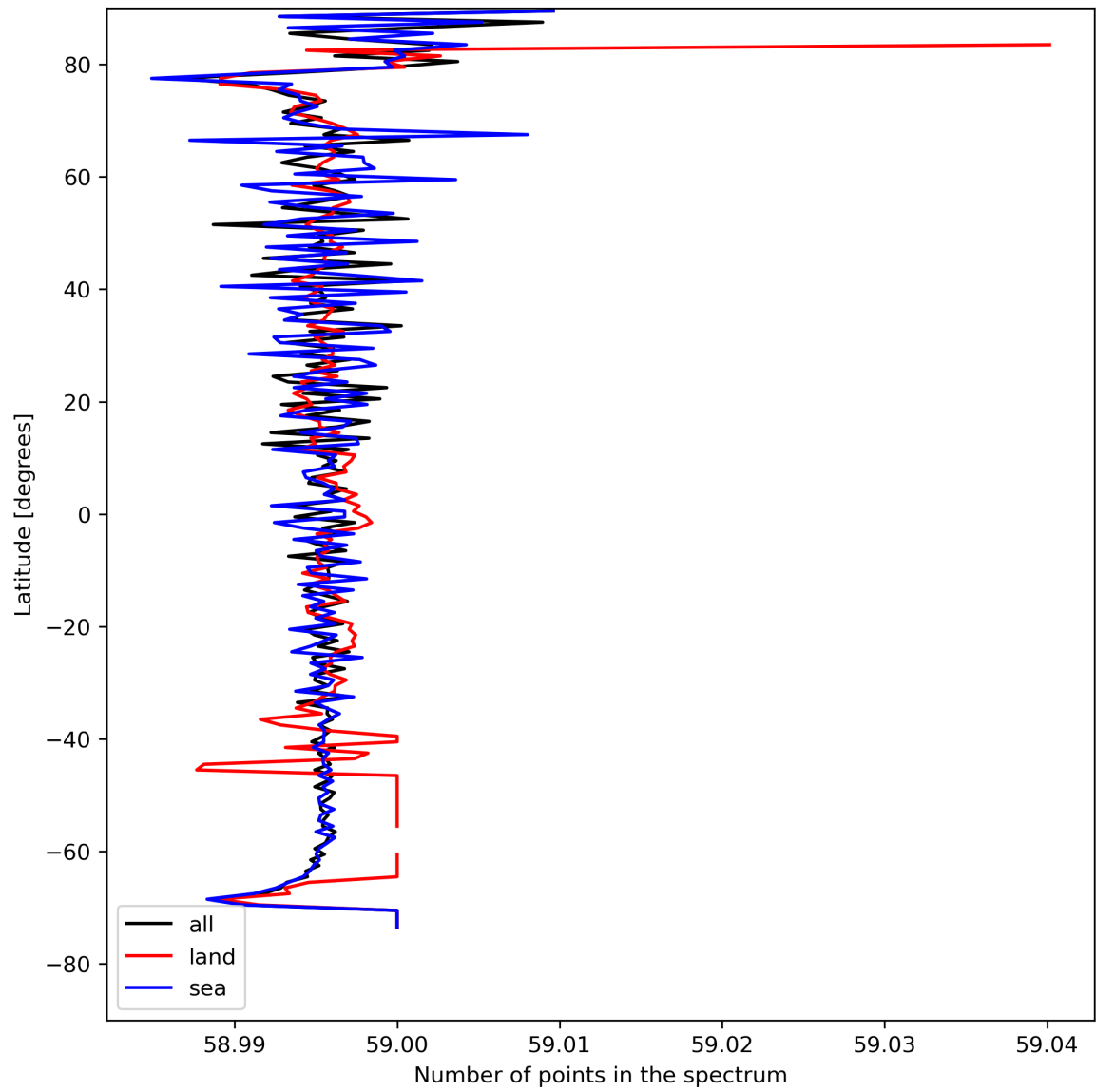
Figure 27: Zonal average of “Number of points in the spectrum” for 2023-08-12 to 2023-08-14.
