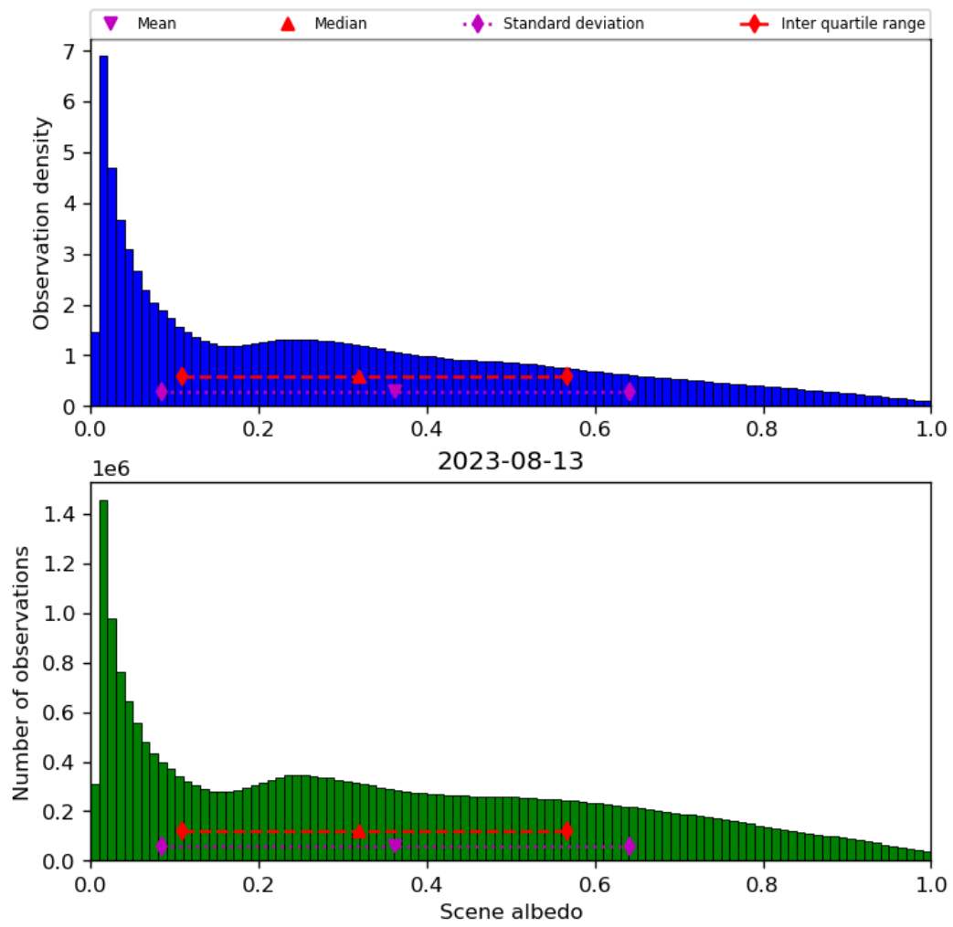
Figure 34: Histogram of “Scene albedo” for 2023-08-12 to 2023-08-14
