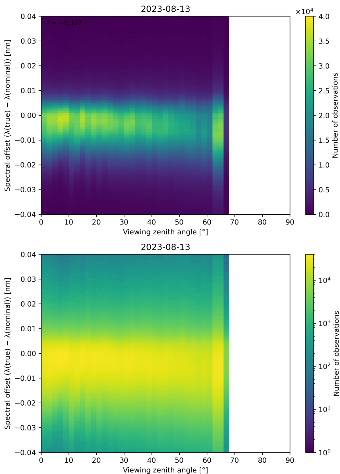
Figure 140: Scatter density plot of “Viewing zenith angle” against “Spectral offset ( \lambda(\text{true}) - \lambda(\text{nominal}) )” for 2023-08-12 to 2023-08-14.
