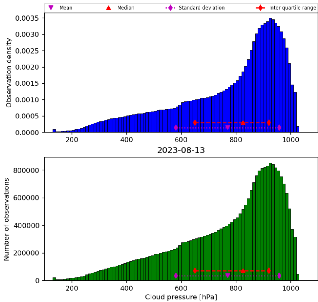
Figure 30: Histogram of “Cloud pressure” for 2023-08-12 to 2023-08-14
