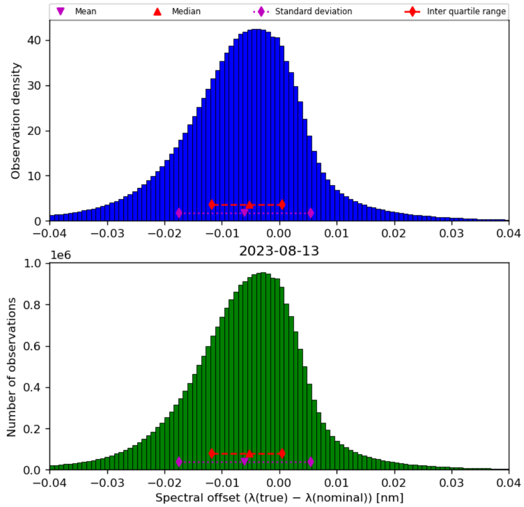
Figure 45: Histogram of “Spectral offset ( \lambda(\text{true}) - \lambda(\text{nominal}) )” for 2023-08-12 to 2023-08-14
