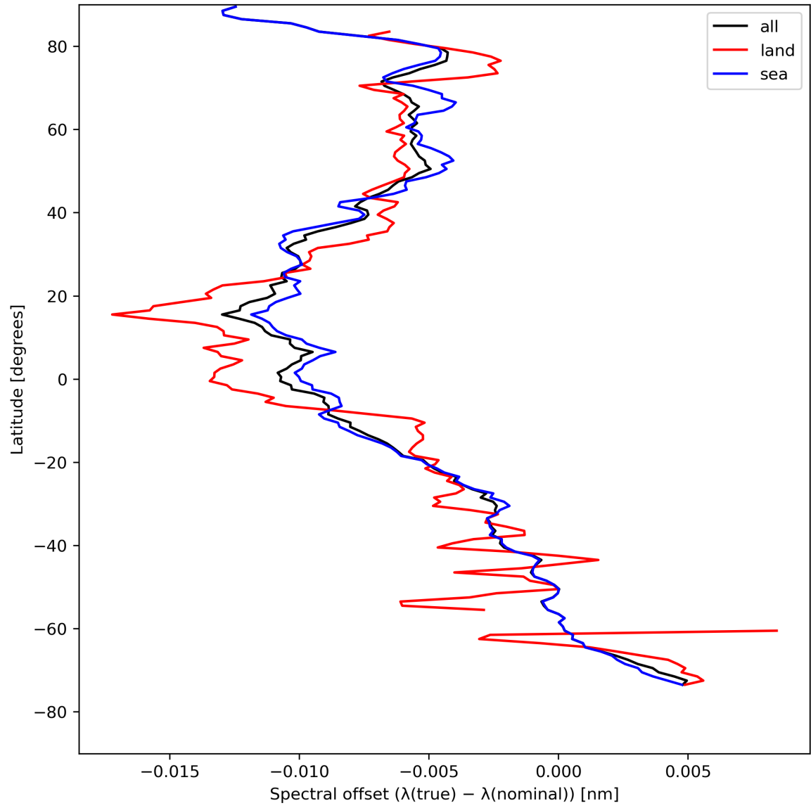
Figure 28: Zonal average of “Spectral offset ( \lambda(\text{true}) - \lambda(\text{nominal}) )” for 2023-08-12 to 2023-08-14.
