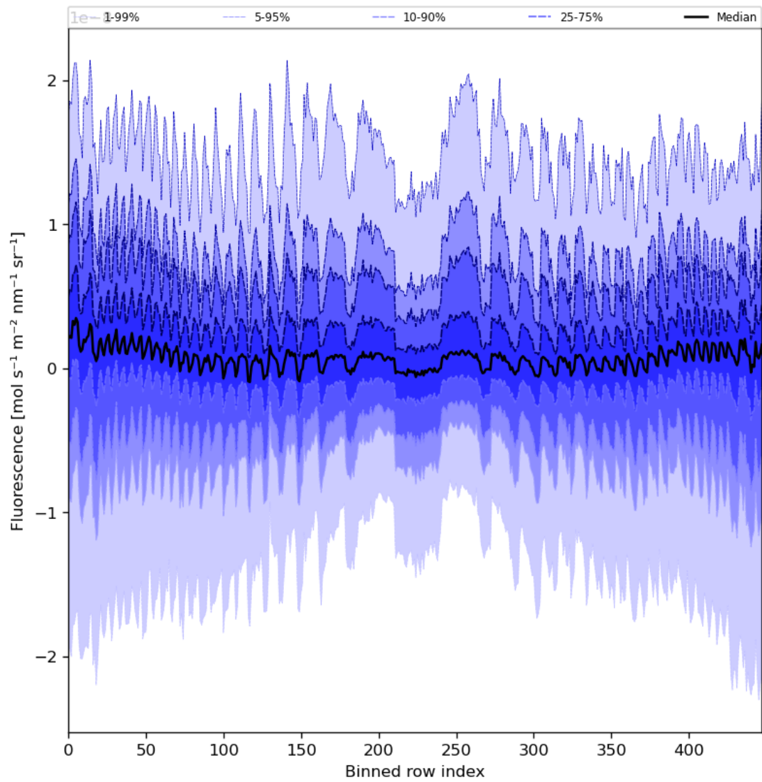
Figure 57: Along track statistics of “Fluorescence” for 2023-08-12 to 2023-08-14
