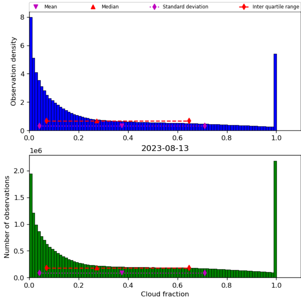
Figure 32: Histogram of “Cloud fraction” for 2023-08-12 to 2023-08-14
