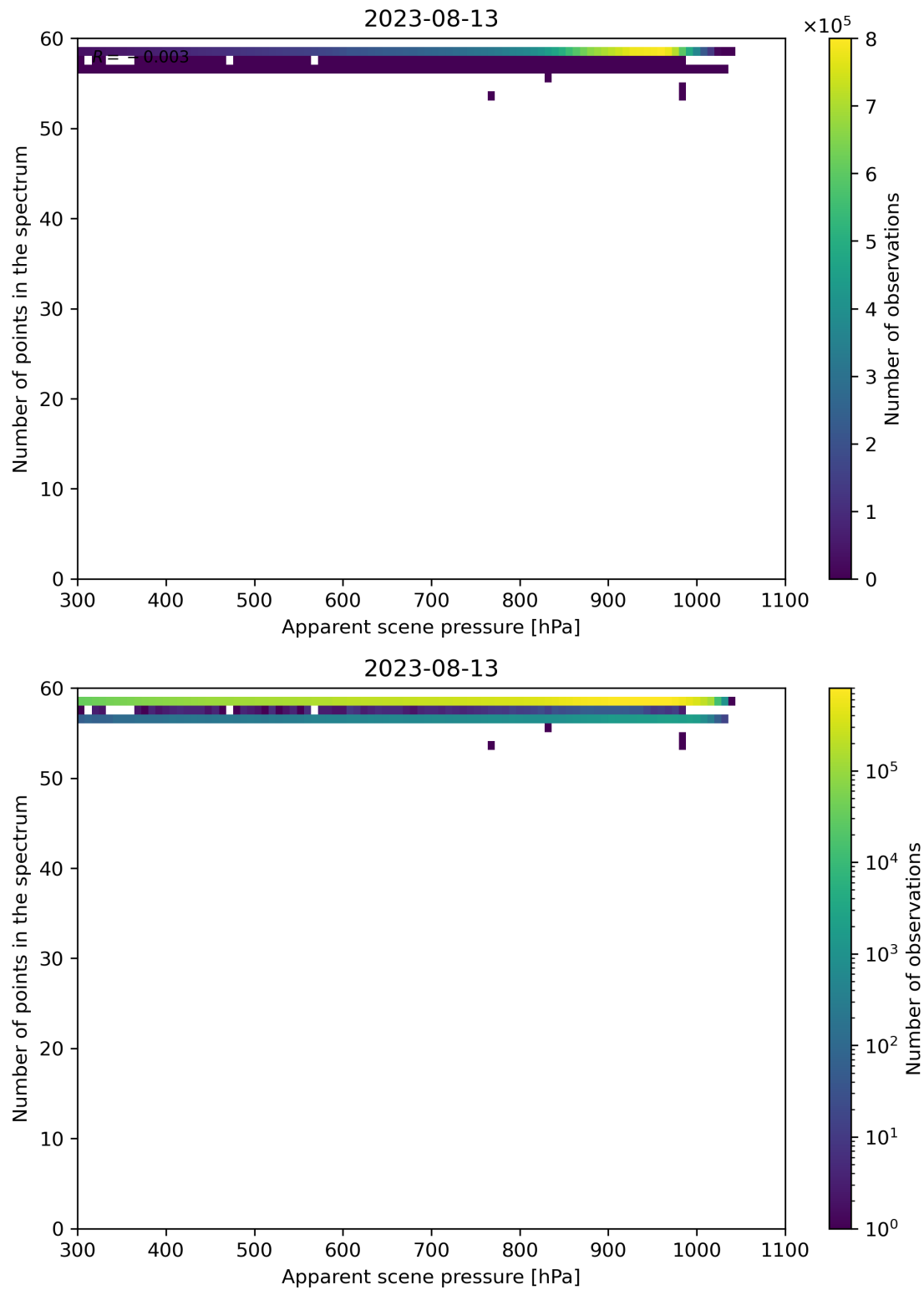
Figure 67: Scatter density plot of “Apparent scene pressure” against “Number of points in the spectrum” for 2023-08-12 to 2023-08-14.
