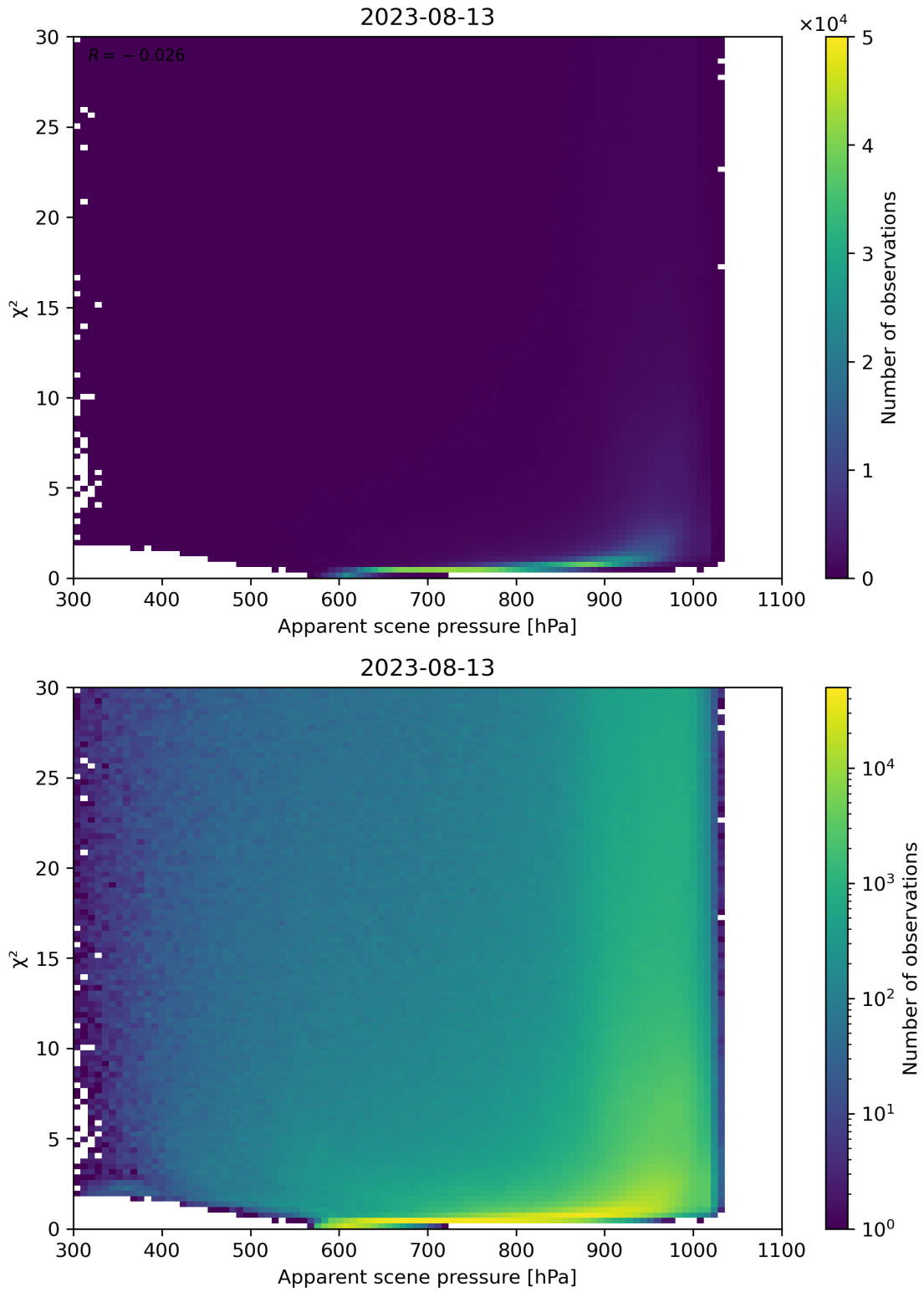
Figure 63: Scatter density plot of “Apparent scene pressure” against “ \chi^2 ” for 2023-08-12 to 2023-08-14.
