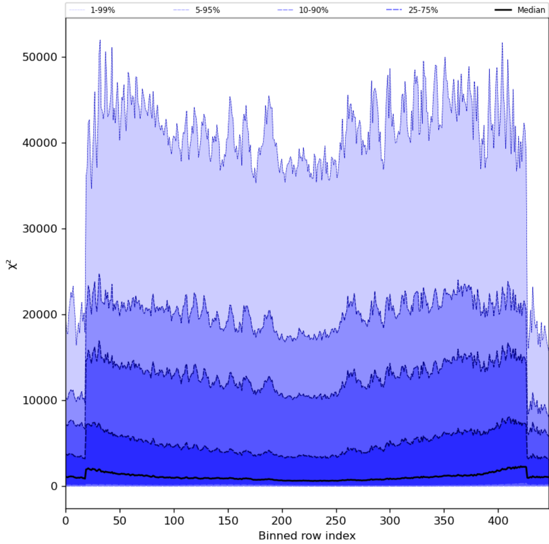
Figure 55: Along track statistics of “ \chi^2 ” for 2023-08-12 to 2023-08-14
