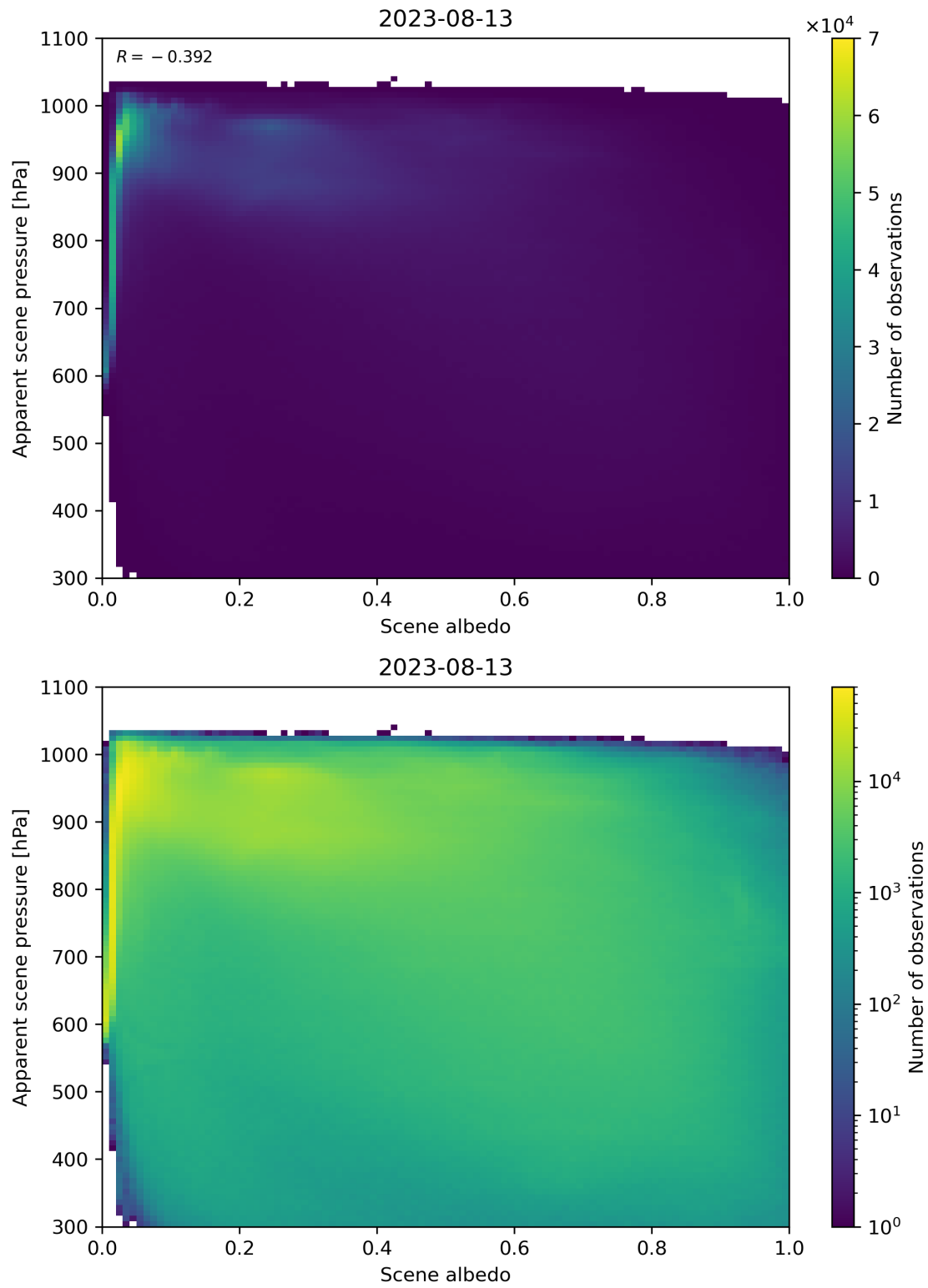
Figure 111: Scatter density plot of “Scene albedo” against “Apparent scene pressure” for 2023-08-12 to 2023-08-14.
