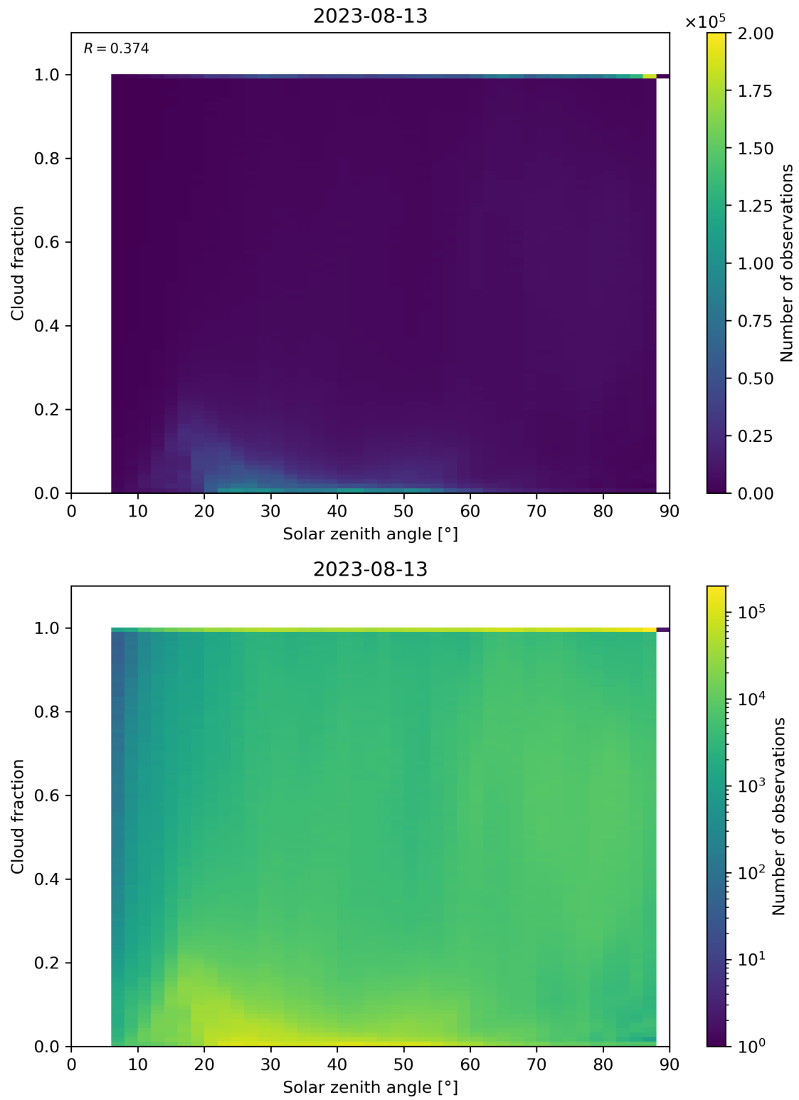
Figure 121: Scatter density plot of “Solar zenith angle” against “Cloud fraction” for 2023-08-12 to 2023-08-14.
