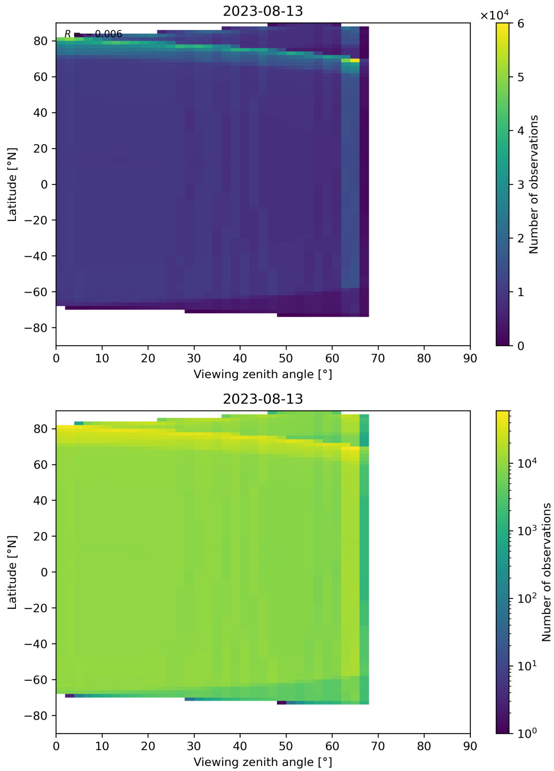
Figure 135: Scatter density plot of “Viewing zenith angle” against “Latitude” for 2023-08-12 to 2023-08-14.
