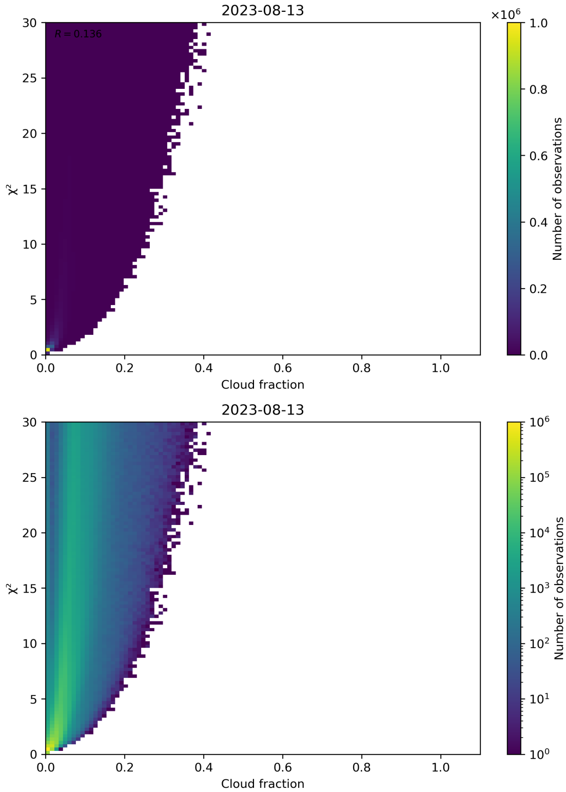
Figure 77: Scatter density plot of “Cloud fraction” against “ \chi^2 ” for 2023-08-12 to 2023-08-14.
