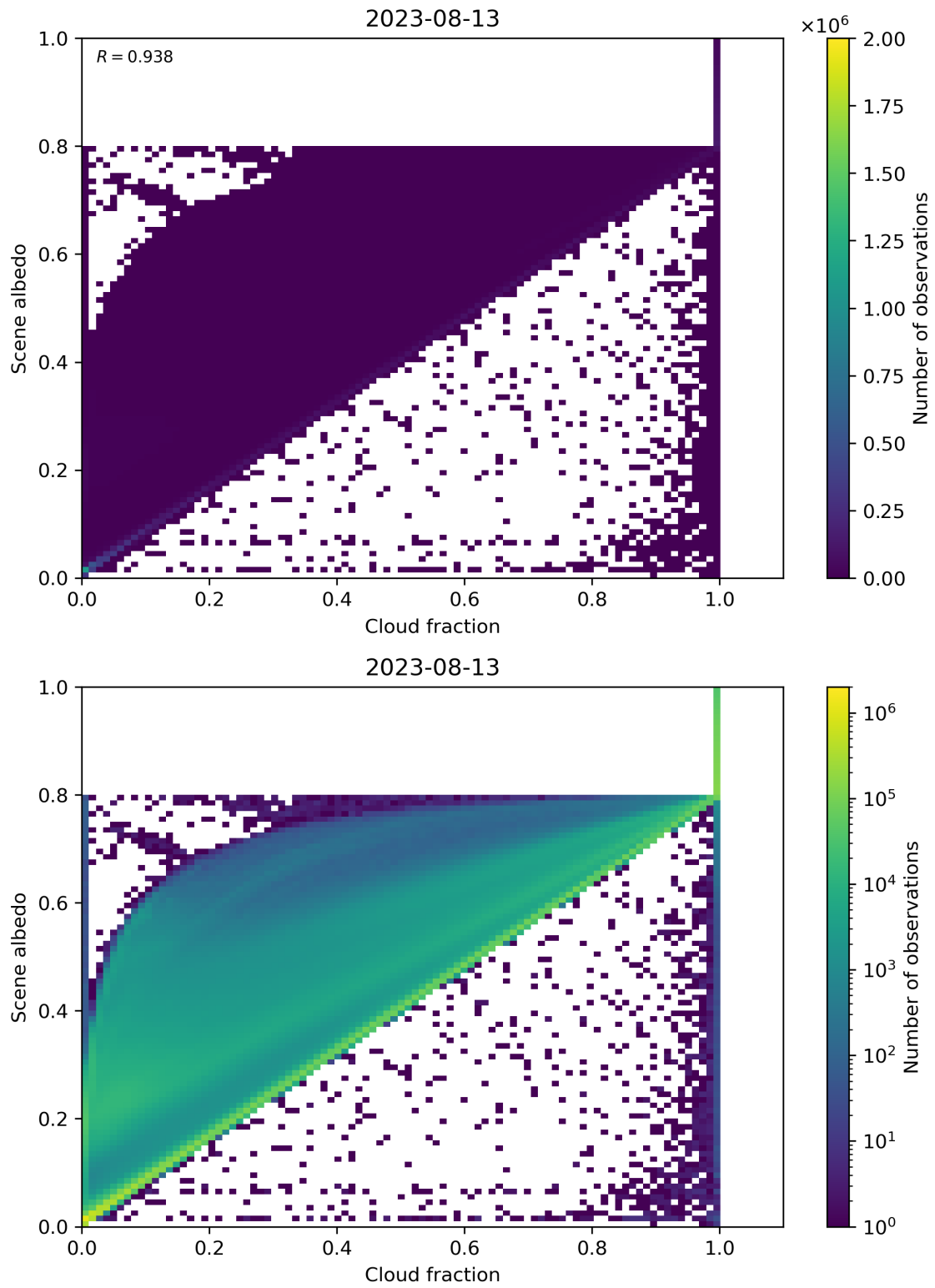
Figure 82: Scatter density plot of “Cloud fraction” against “Scene albedo” for 2023-08-12 to 2023-08-14.
