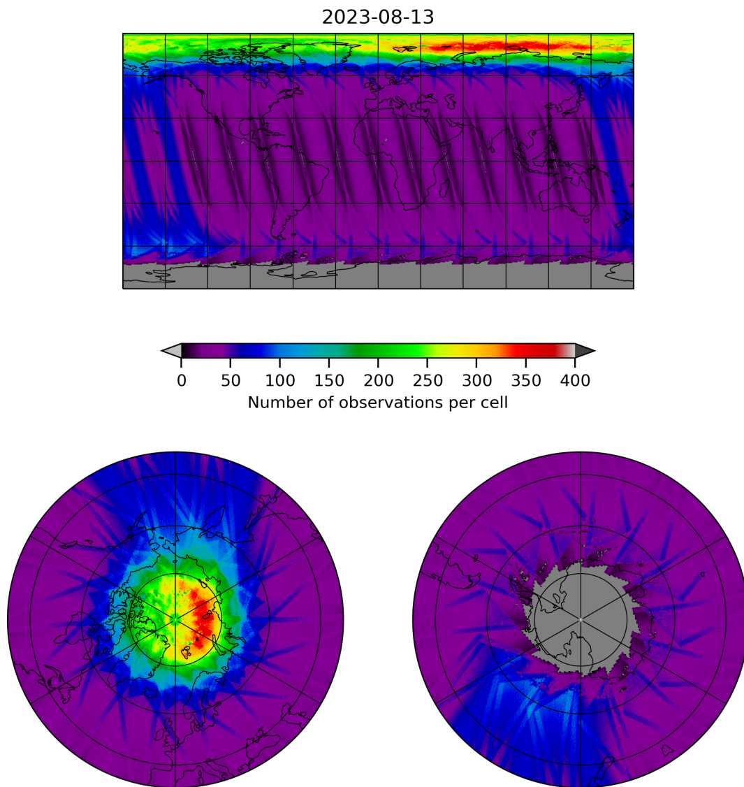
Figure 11: Map of the number of observations for 2023-08-12 to 2023-08-14
