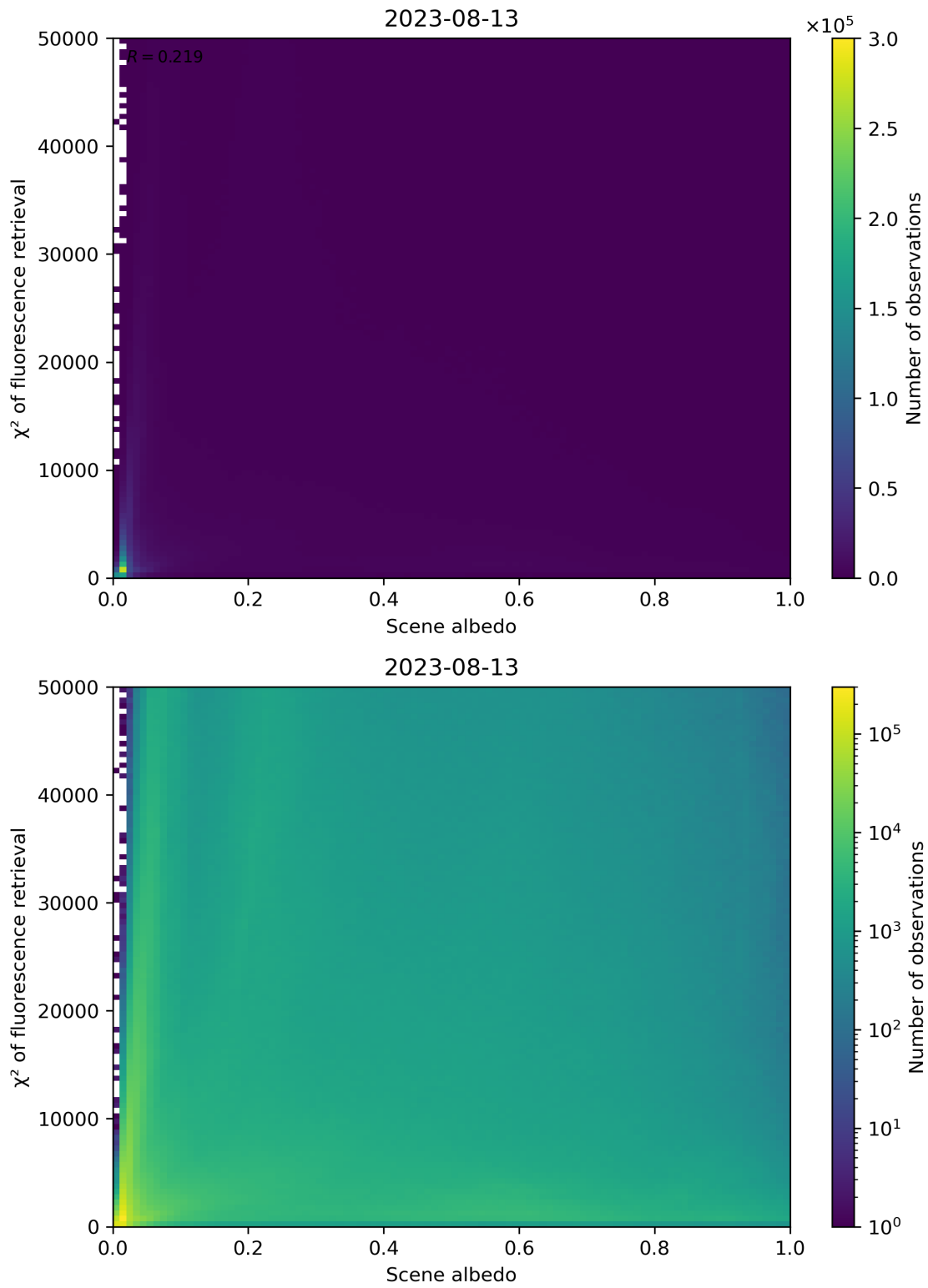
Figure 113: Scatter density plot of “Scene albedo” against “ \chi^2 of fluorescence retrieval” for 2023-08-12 to 2023-08-14.
