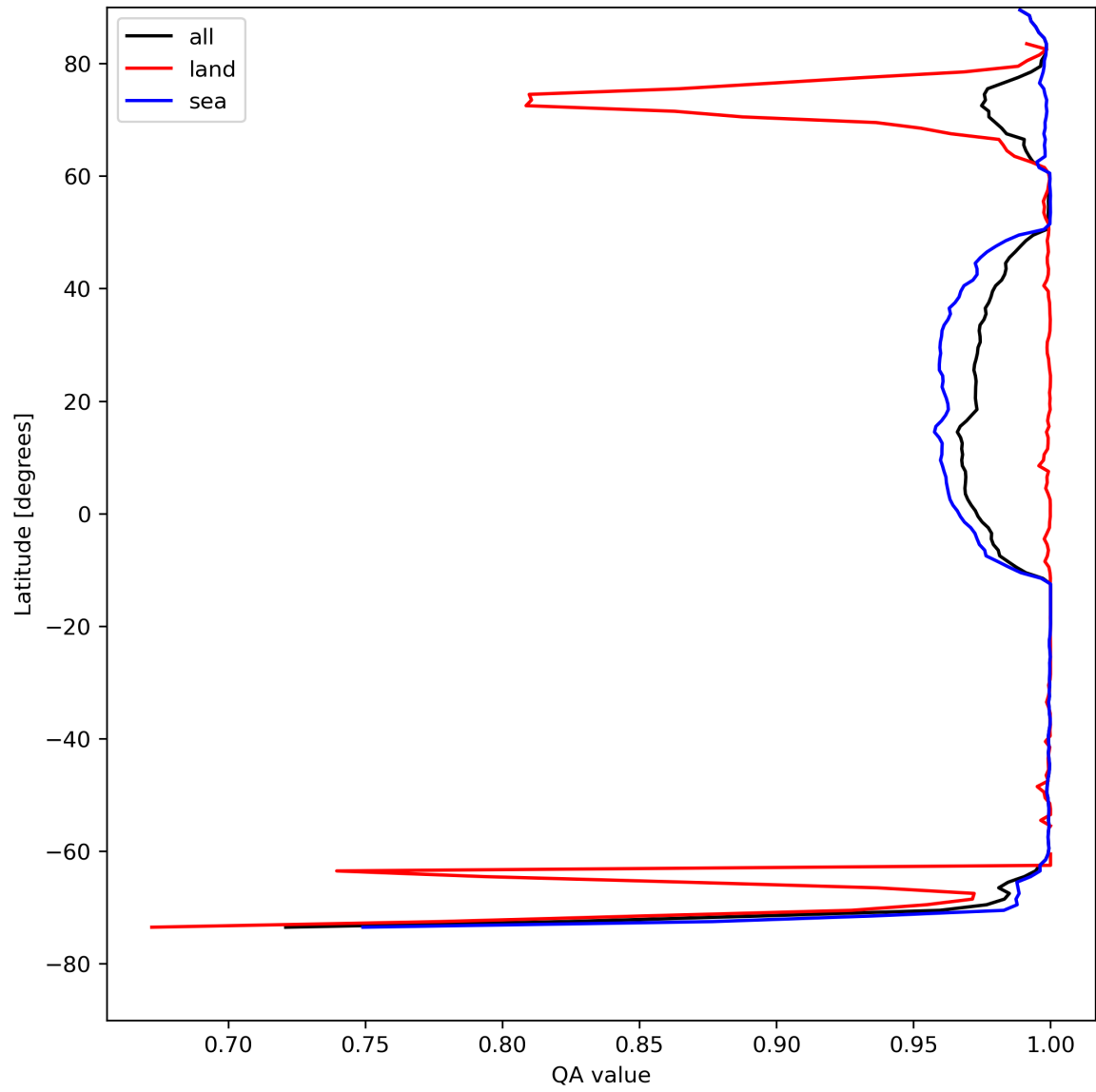
Figure 12: Zonal average of "QA value" for 2023-08-12 to 2023-08-14.
