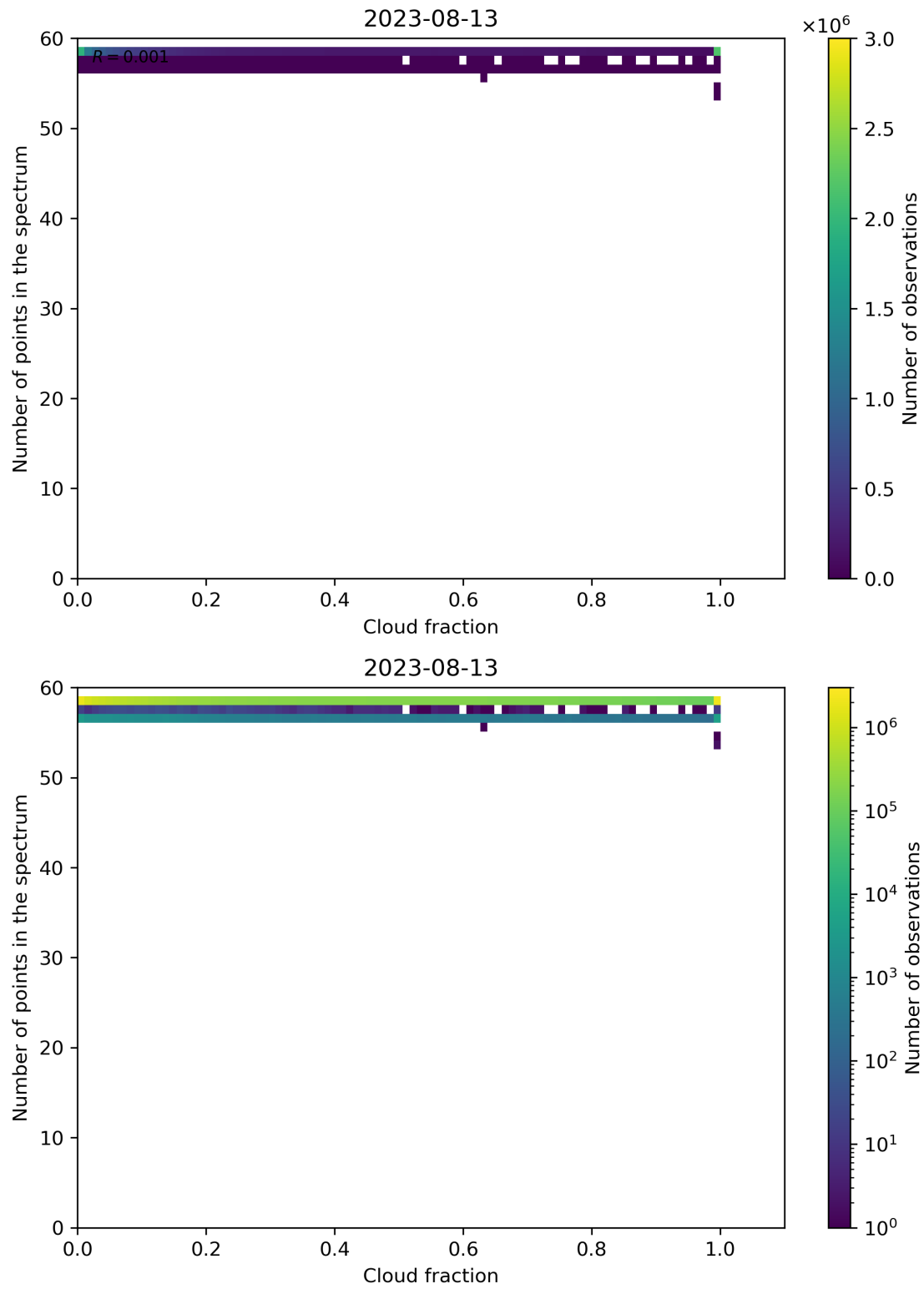
Figure 81: Scatter density plot of “Cloud fraction” against “Number of points in the spectrum” for 2023-08-12 to 2023-08-14.
