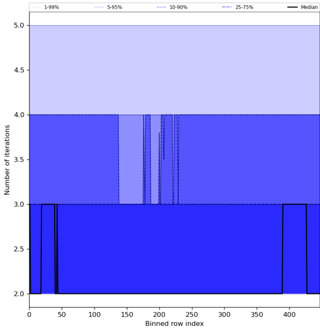
Figure 56: Along track statistics of “Number of iterations” for 2023-08-12 to 2023-08-14
