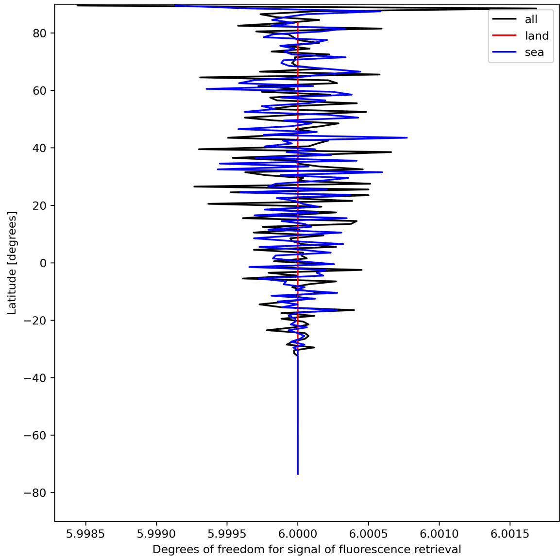
Figure 26: Zonal average of “Degrees of freedom for signal of fluorescence retrieval” for 2023-08-12 to 2023-08-14.
