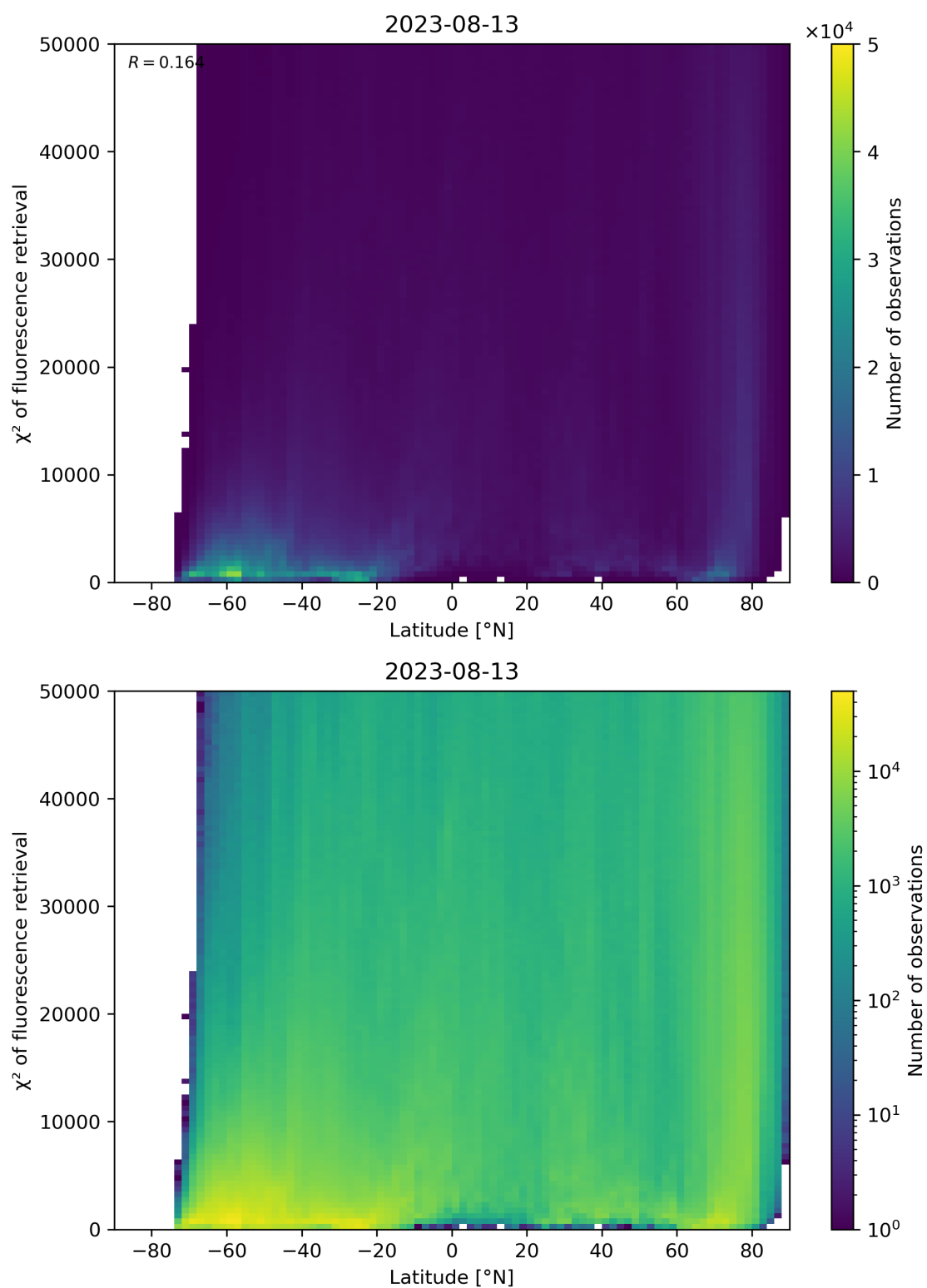
Figure 98: Scatter density plot of “Latitude” against “ \chi^2 of fluorescence retrieval” for 2023-08-12 to 2023-08-14.
