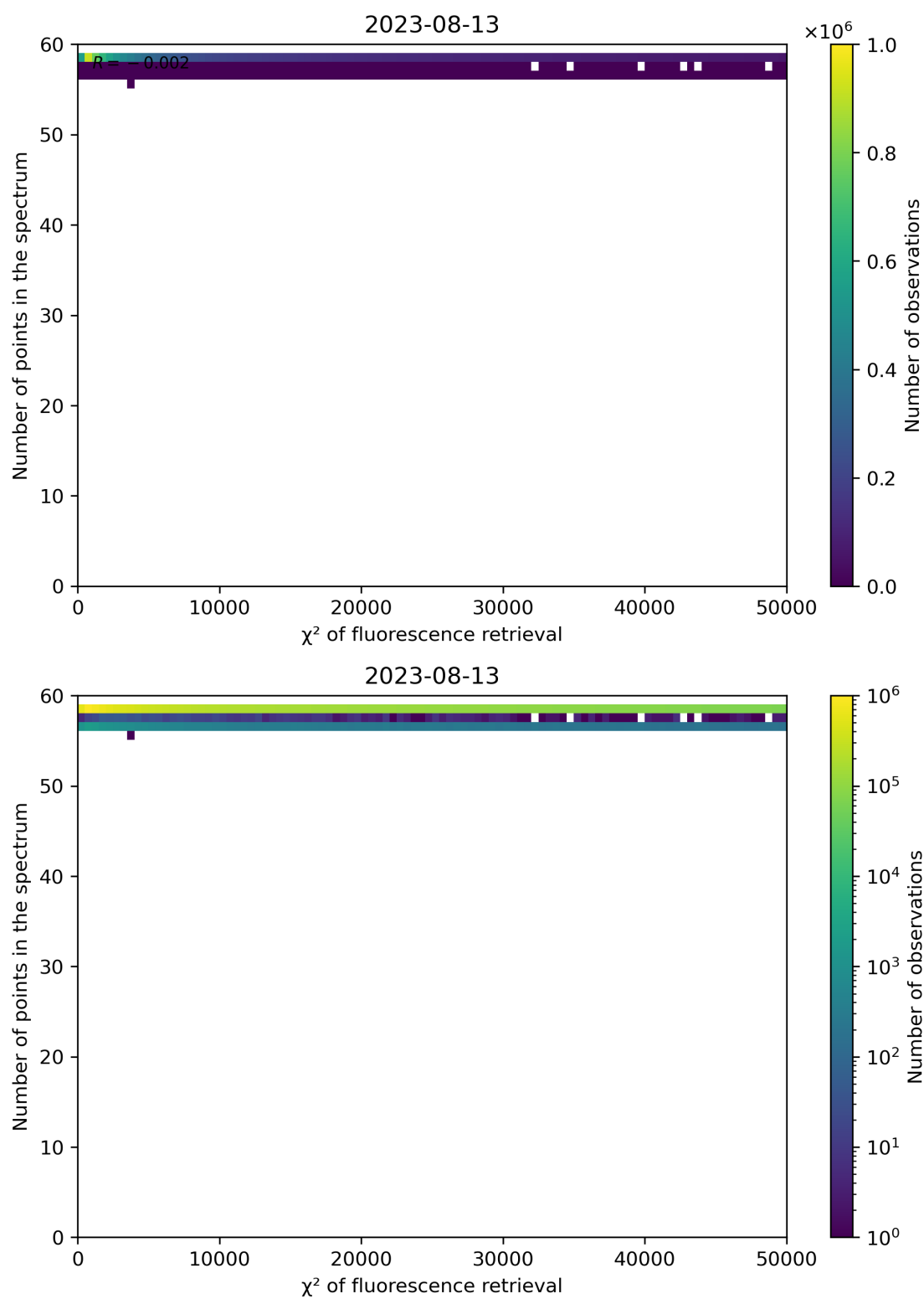
Figure 71: Scatter density plot of “ \chi^2 of fluorescence retrieval” against “Number of points in the spectrum” for 2023-08-12 to 2023-08-14.
