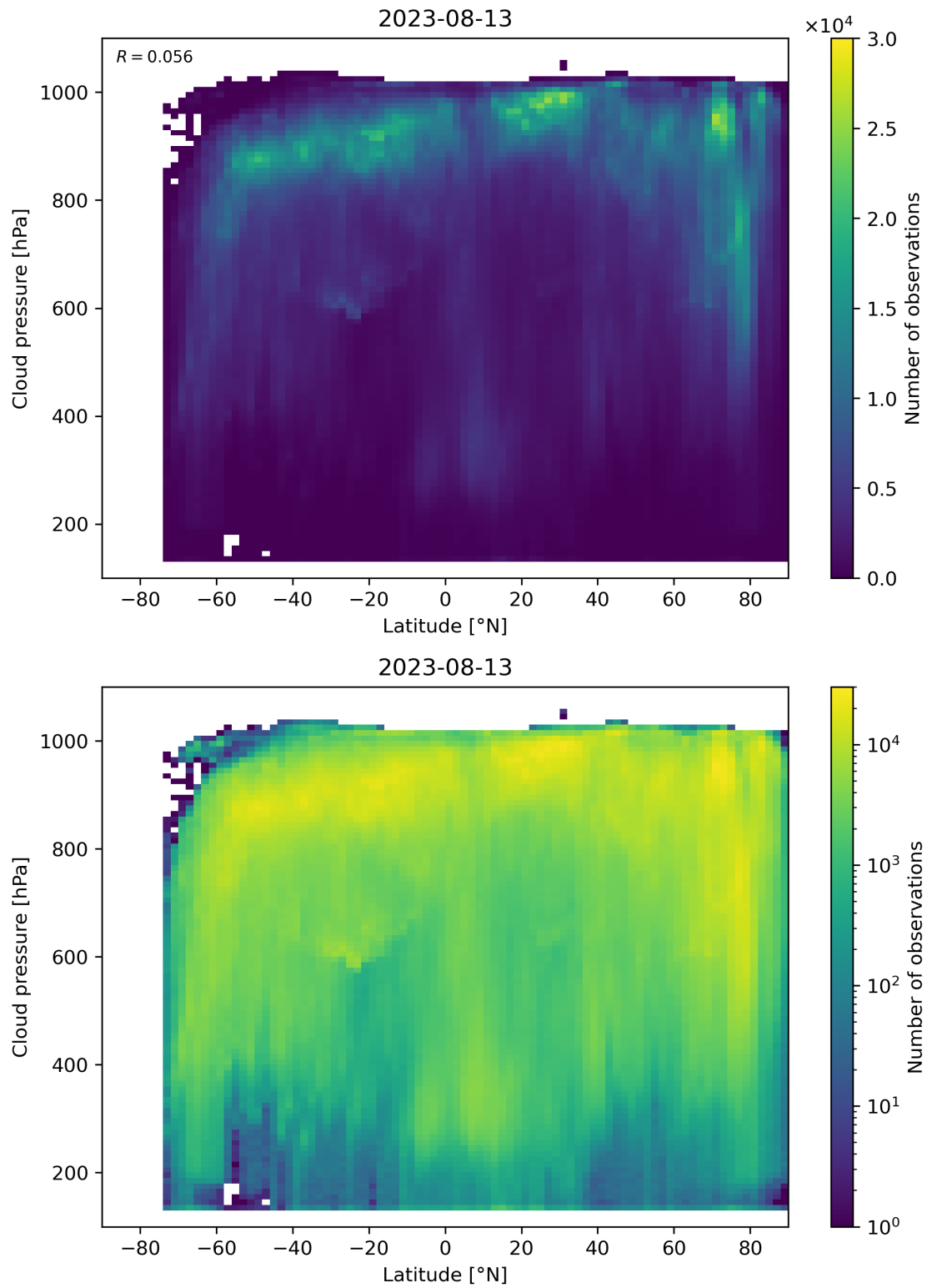
Figure 100: Scatter density plot of “Latitude” against “Cloud pressure” for 2023-08-12 to 2023-08-14.
