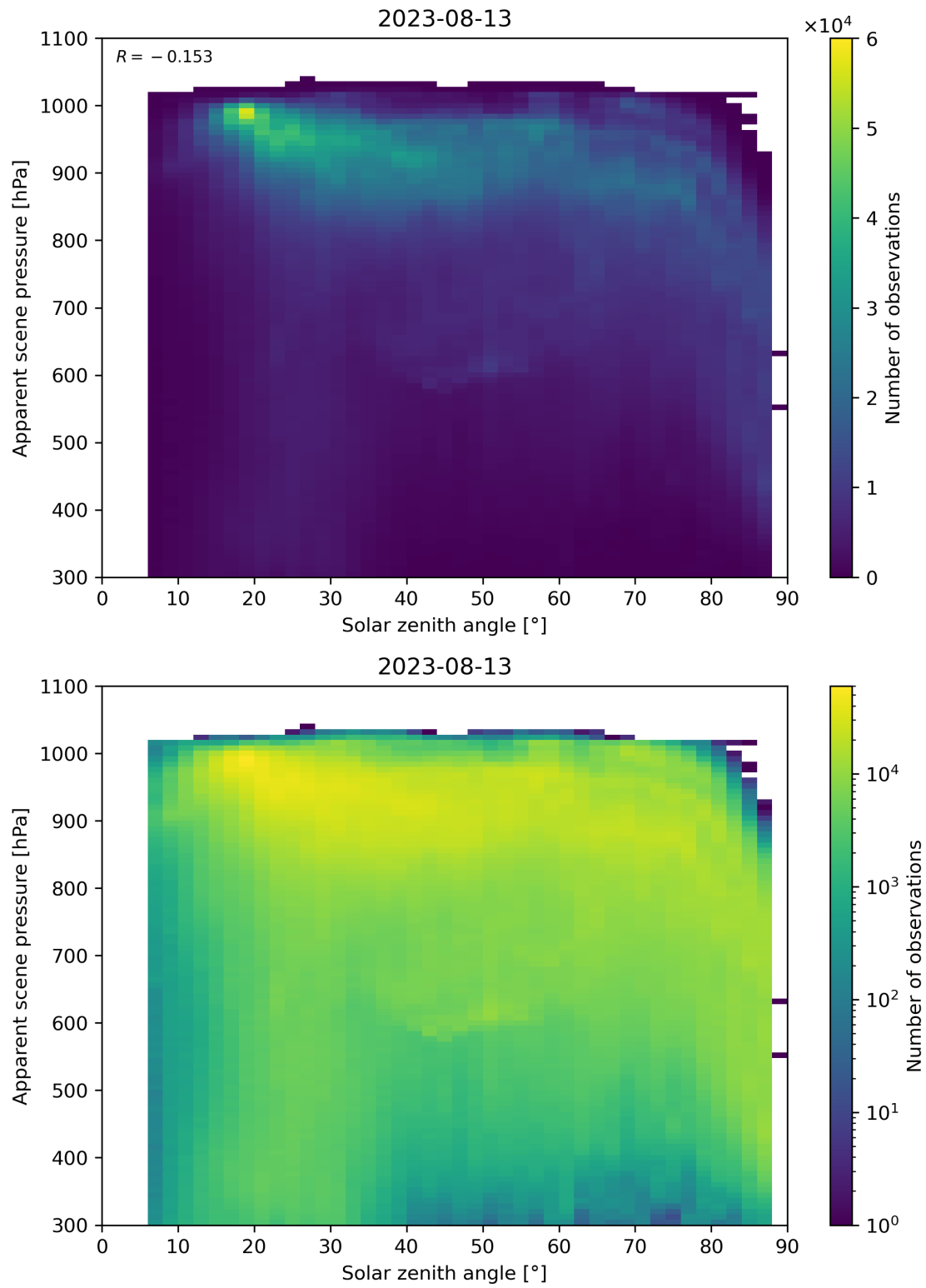
Figure 118: Scatter density plot of “Solar zenith angle” against “Apparent scene pressure” for 2023-08-12 to 2023-08-14.
