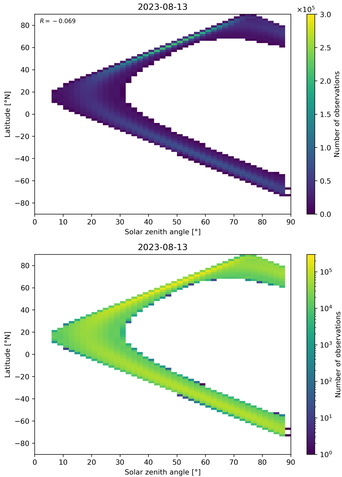
Figure 124: Scatter density plot of “Solar zenith angle” against “Latitude” for 2023-08-12 to 2023-08-14.
