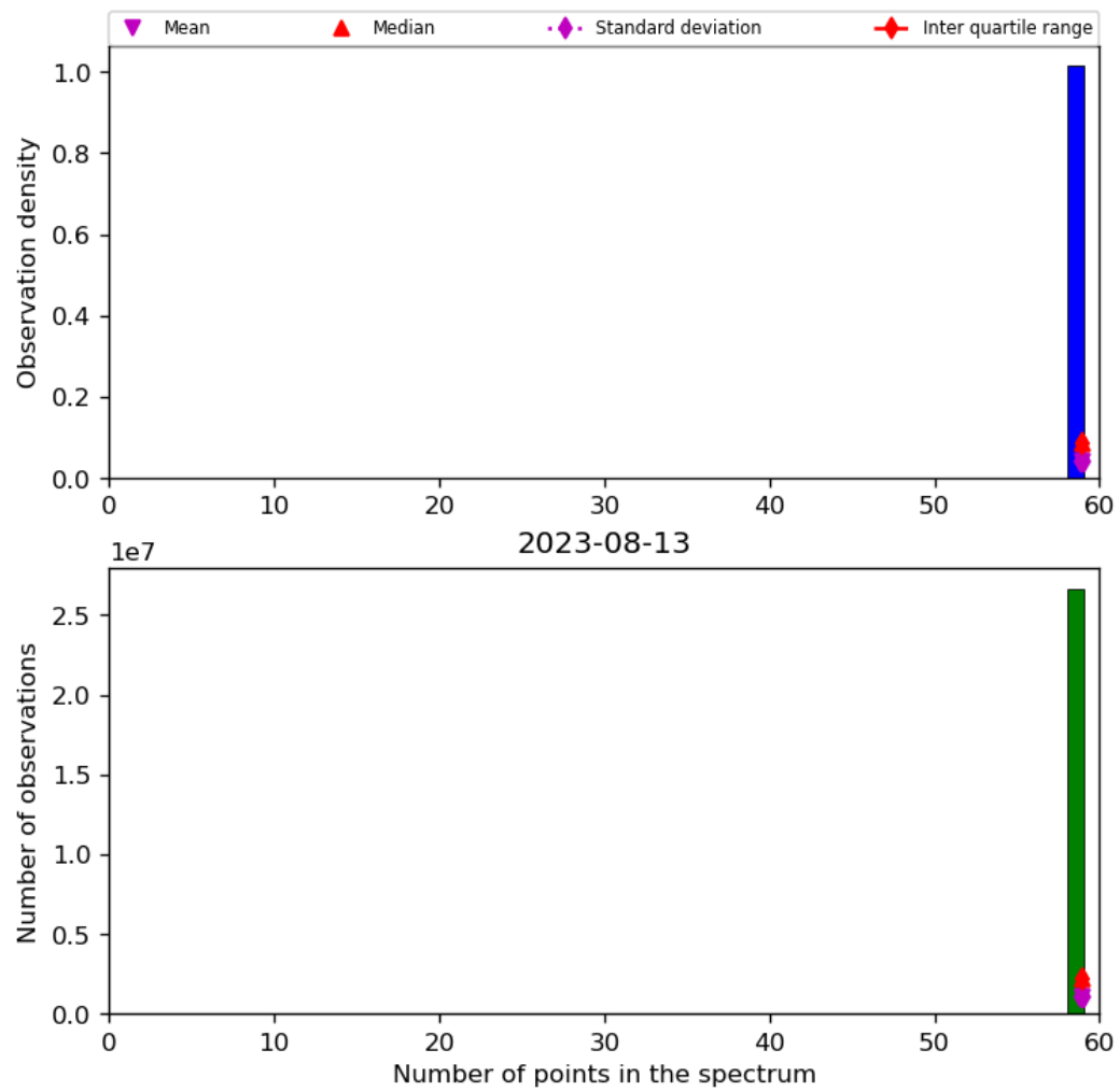
Figure 44: Histogram of “Number of points in the spectrum” for 2023-08-12 to 2023-08-14
