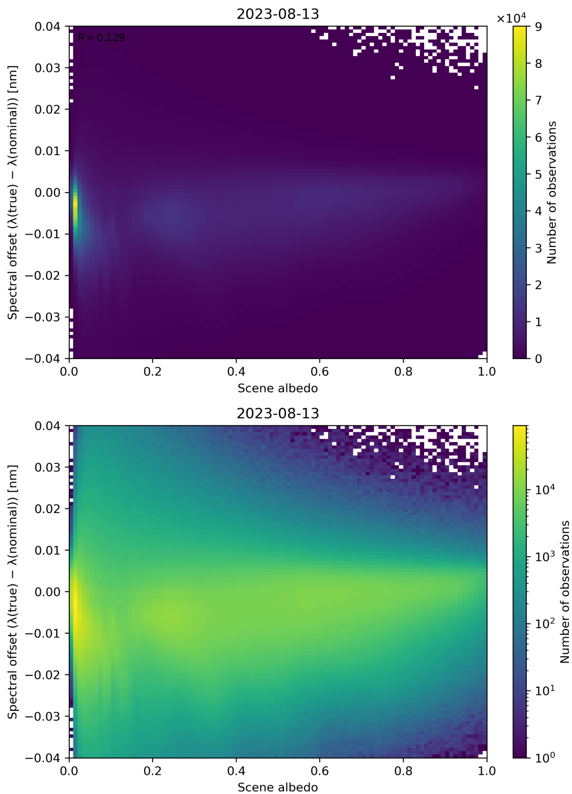
Figure 117: Scatter density plot of “Scene albedo” against “Spectral offset ( \lambda(\text{true}) - \lambda(\text{nominal}) )” for 2023-08-12 to 2023-08-14.
