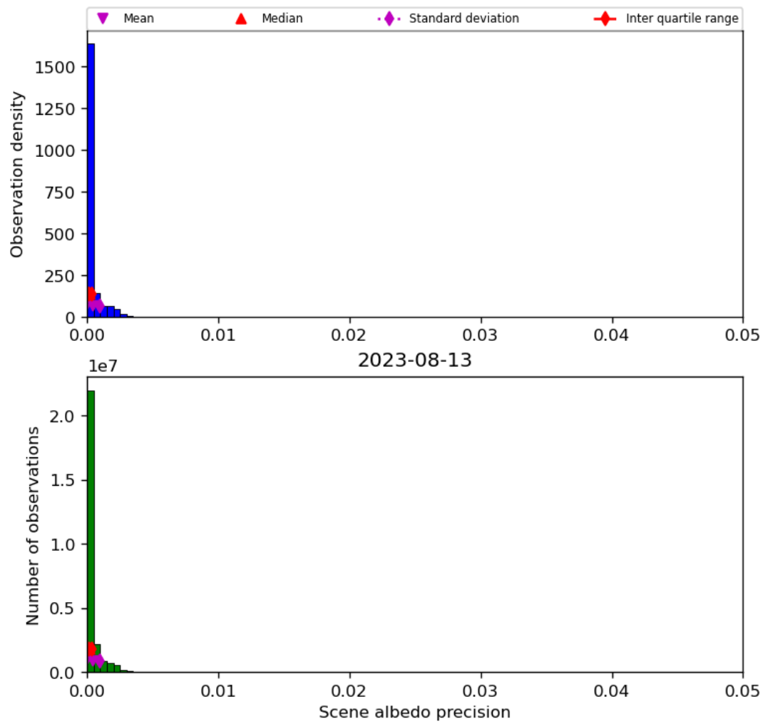
Figure 35: Histogram of “Scene albedo precision” for 2023-08-12 to 2023-08-14
