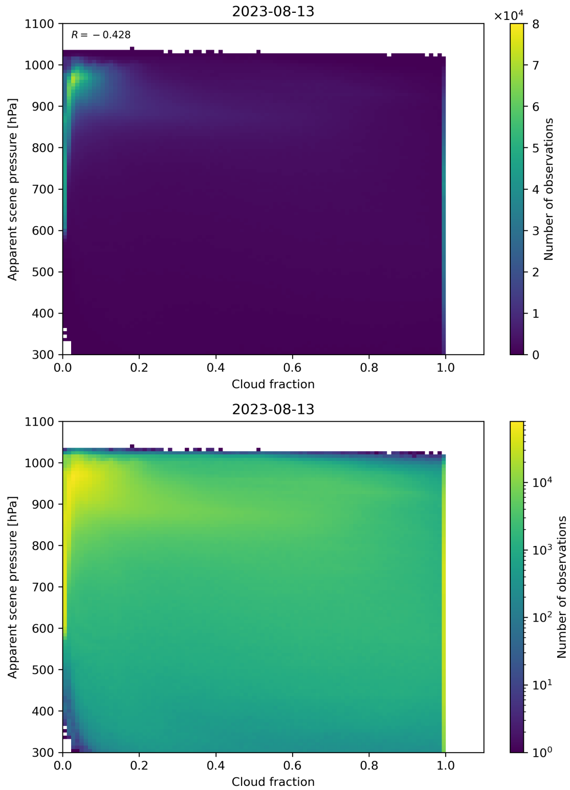
Figure 76: Scatter density plot of “Cloud fraction” against “Apparent scene pressure” for 2023-08-12 to 2023-08-14.
