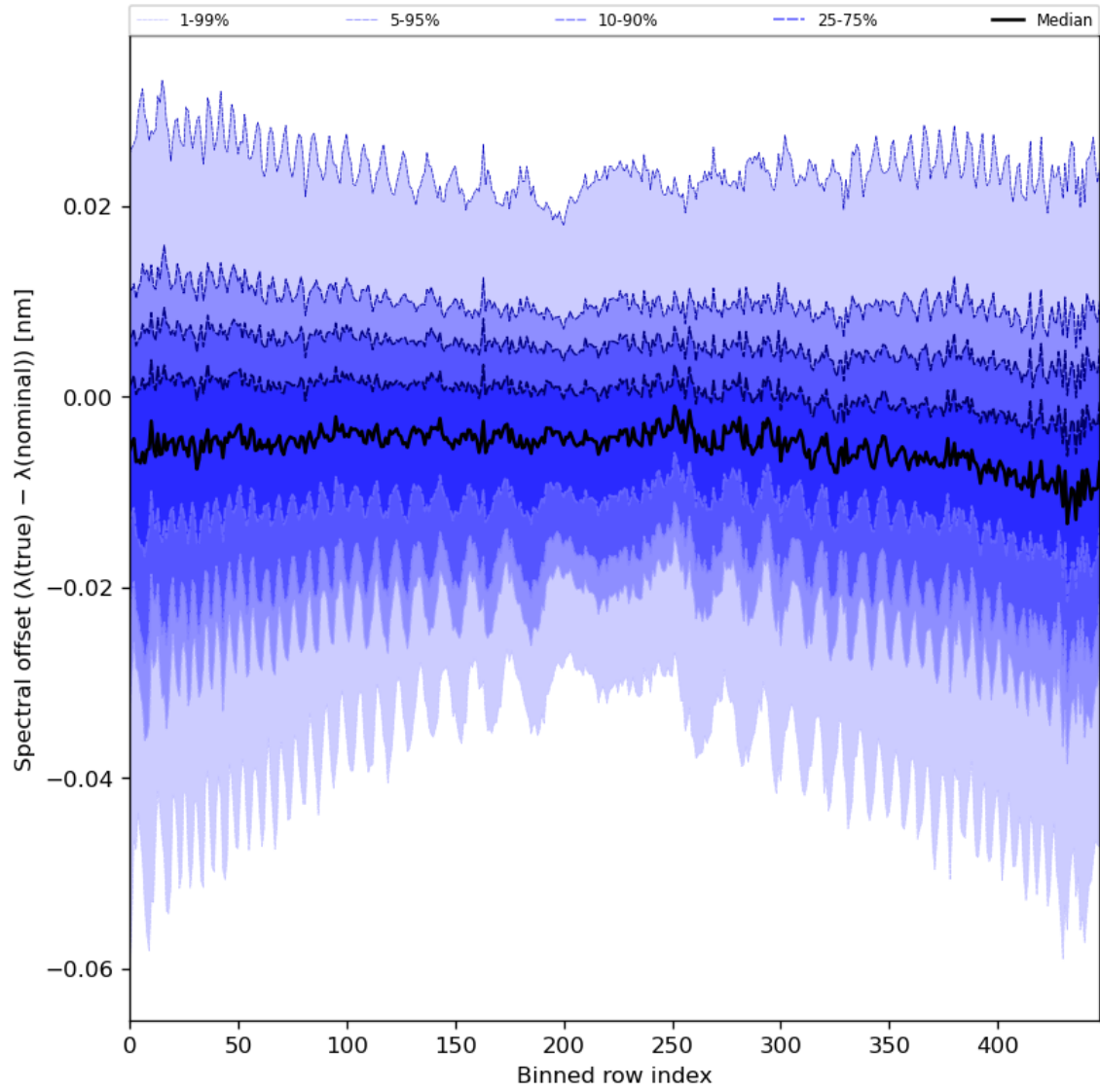
Figure 62: Along track statistics of “Spectral offset ( \lambda(\text{true}) - \lambda(\text{nominal}) )” for 2023-08-12 to 2023-08-14
