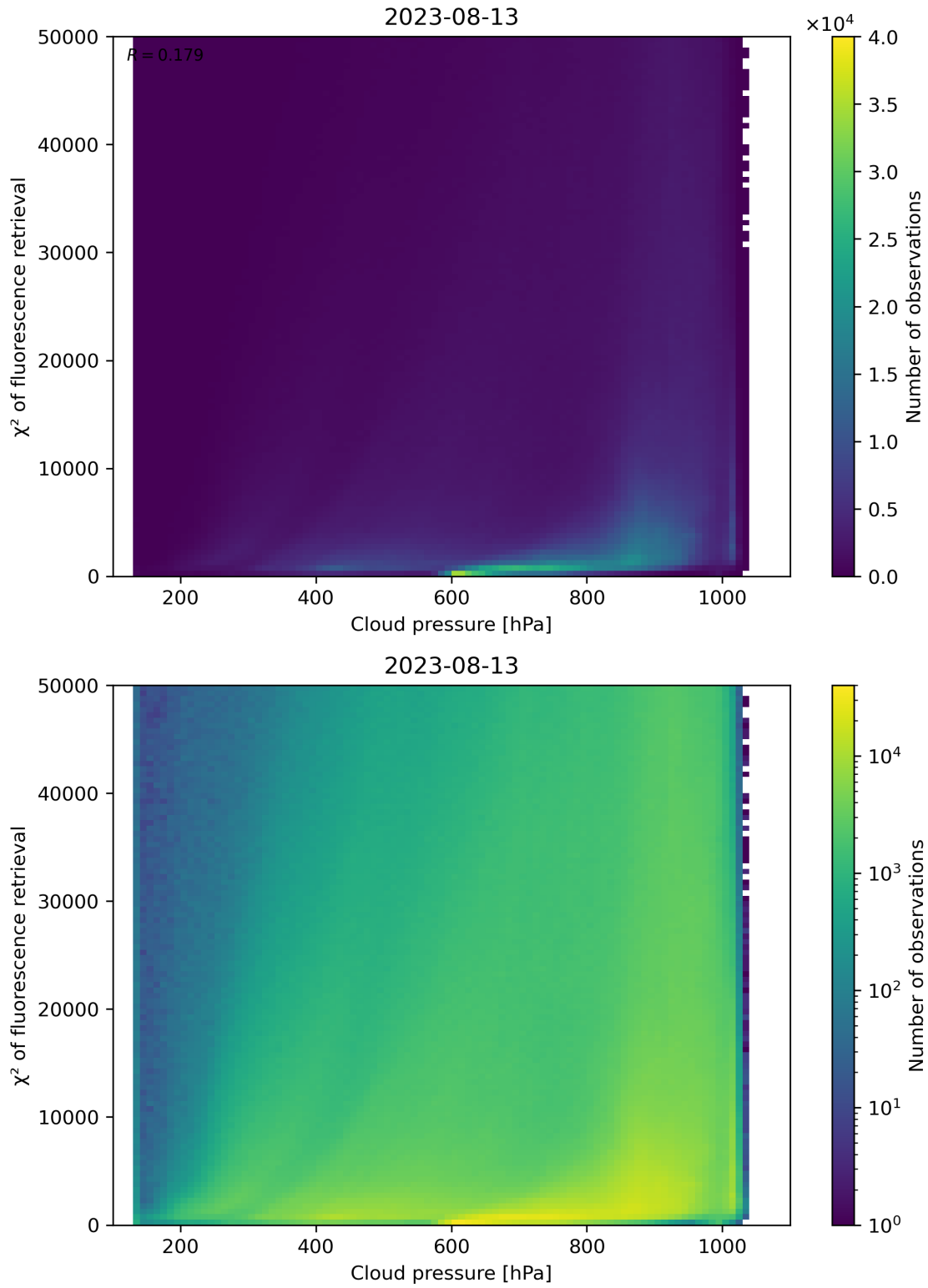
Figure 86: Scatter density plot of “Cloud pressure” against “ \chi^2 of fluorescence retrieval” for 2023-08-12 to 2023-08-14.
