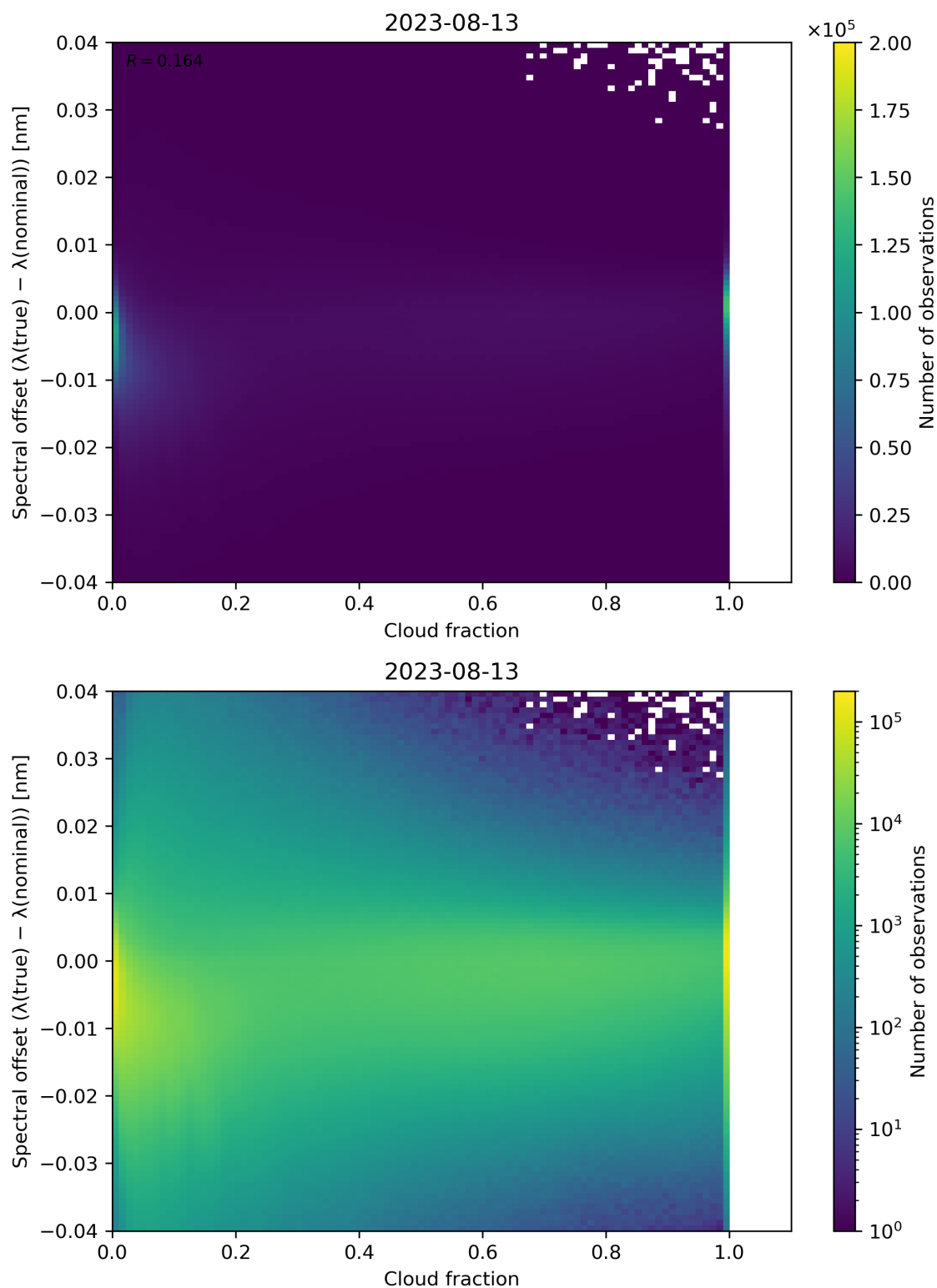
Figure 83: Scatter density plot of “Cloud fraction” against “Spectral offset ( \lambda(\text{true}) - \lambda(\text{nominal}) )” for 2023-08-12 to 2023-08-14.
