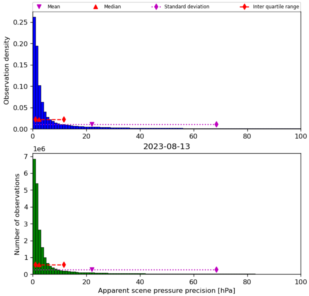
Figure 37: Histogram of “Apparent scene pressure precision” for 2023-08-12 to 2023-08-14
