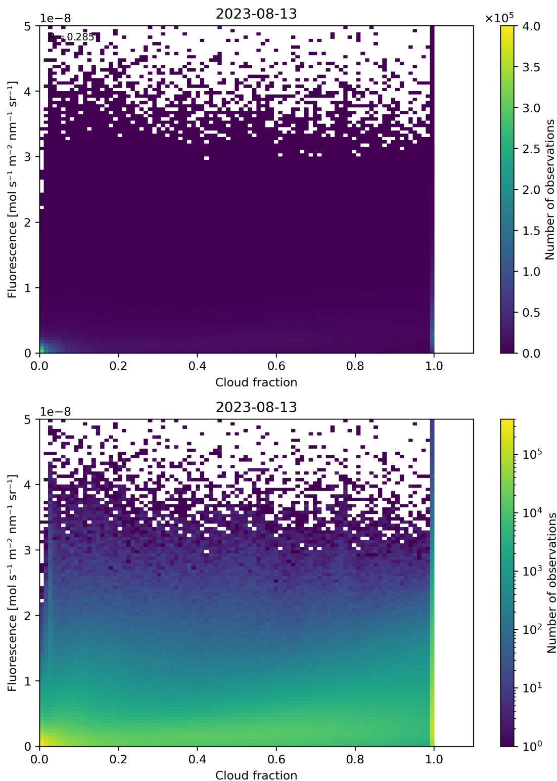
Figure 79: Scatter density plot of “Cloud fraction” against “Fluorescence” for 2023-08-12 to 2023-08-14.
