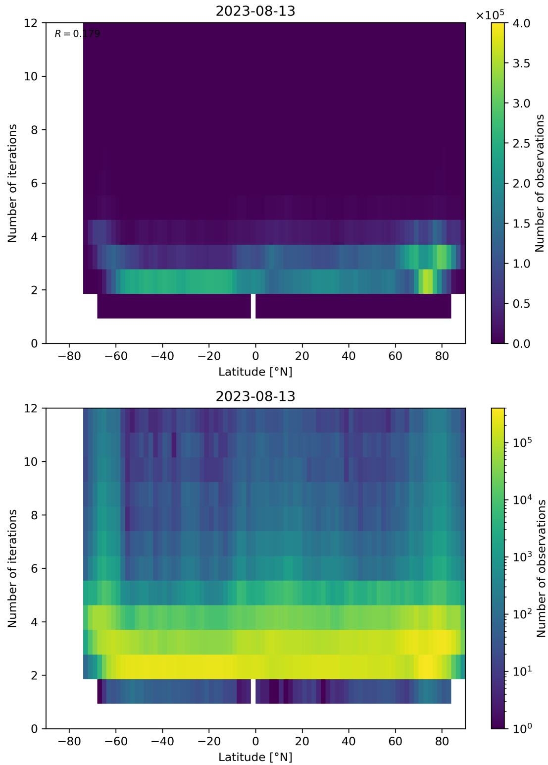
Figure 102: Scatter density plot of “Latitude” against “Number of iterations” for 2023-08-12 to 2023-08-14.
