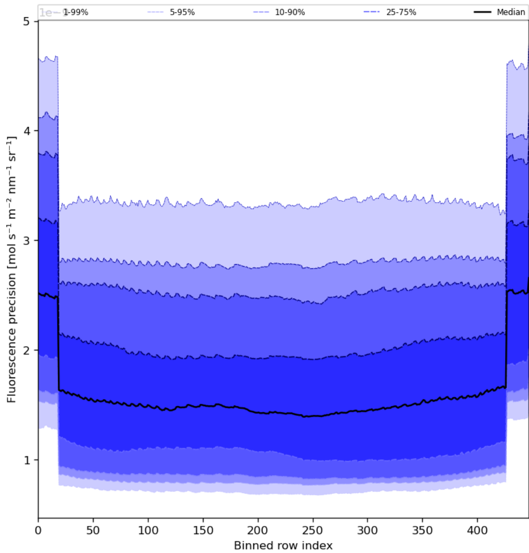
Figure 58: Along track statistics of “Fluorescence precision” for 2023-08-14 to 2023-08-15
