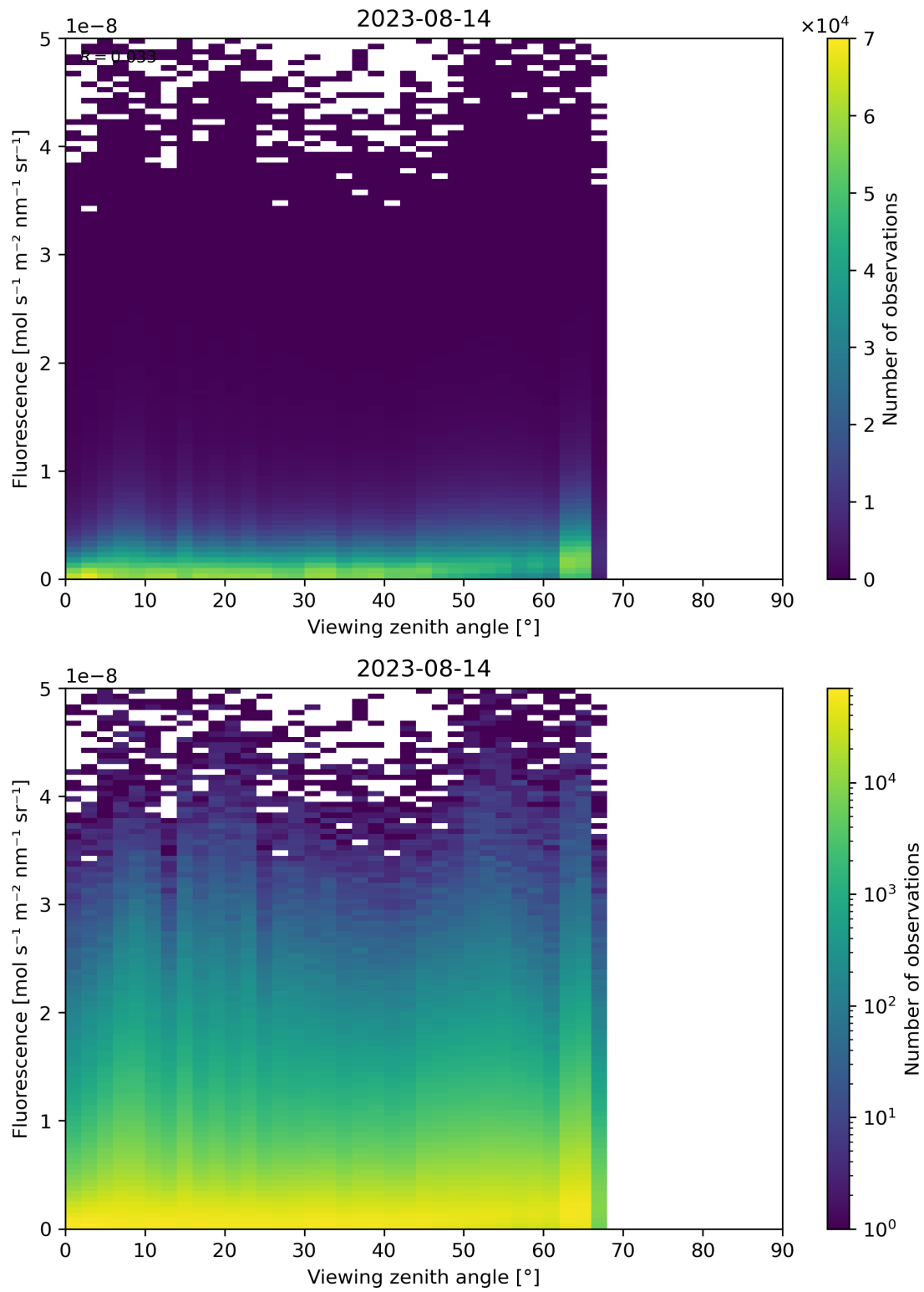
Figure 134: Scatter density plot of “Viewing zenith angle” against “Fluorescence” for 2023-08-14 to 2023-08-15.
