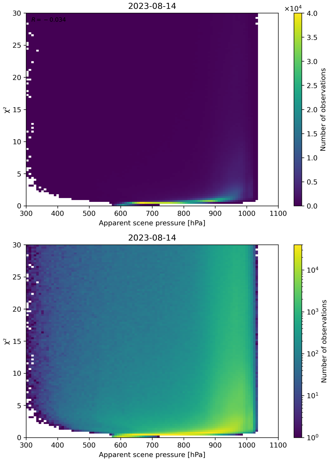
Figure 63: Scatter density plot of “Apparent scene pressure” against “ \chi^2 ” for 2023-08-14 to 2023-08-15.
