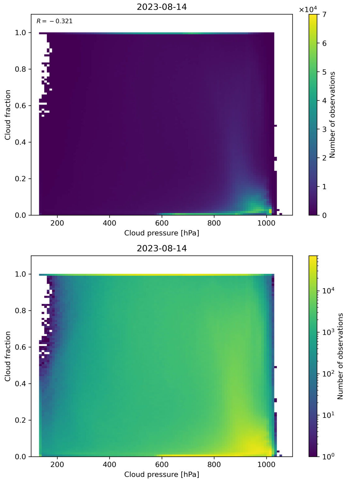
Figure 87: Scatter density plot of “Cloud pressure” against “Cloud fraction” for 2023-08-14 to 2023-08-15.
