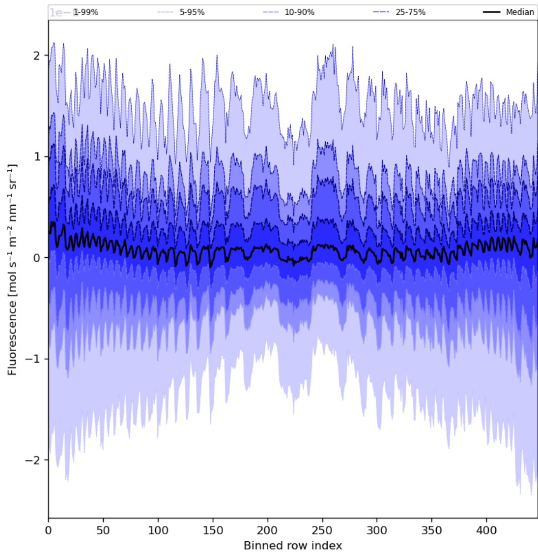
Figure 57: Along track statistics of “Fluorescence” for 2023-08-14 to 2023-08-15
