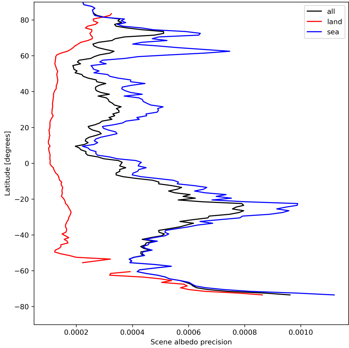
Figure 18: Zonal average of “Scene albedo precision” for 2023-08-14 to 2023-08-15.
