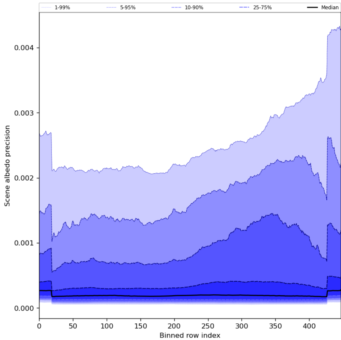
Figure 52: Along track statistics of “Scene albedo precision” for 2023-08-14 to 2023-08-15
