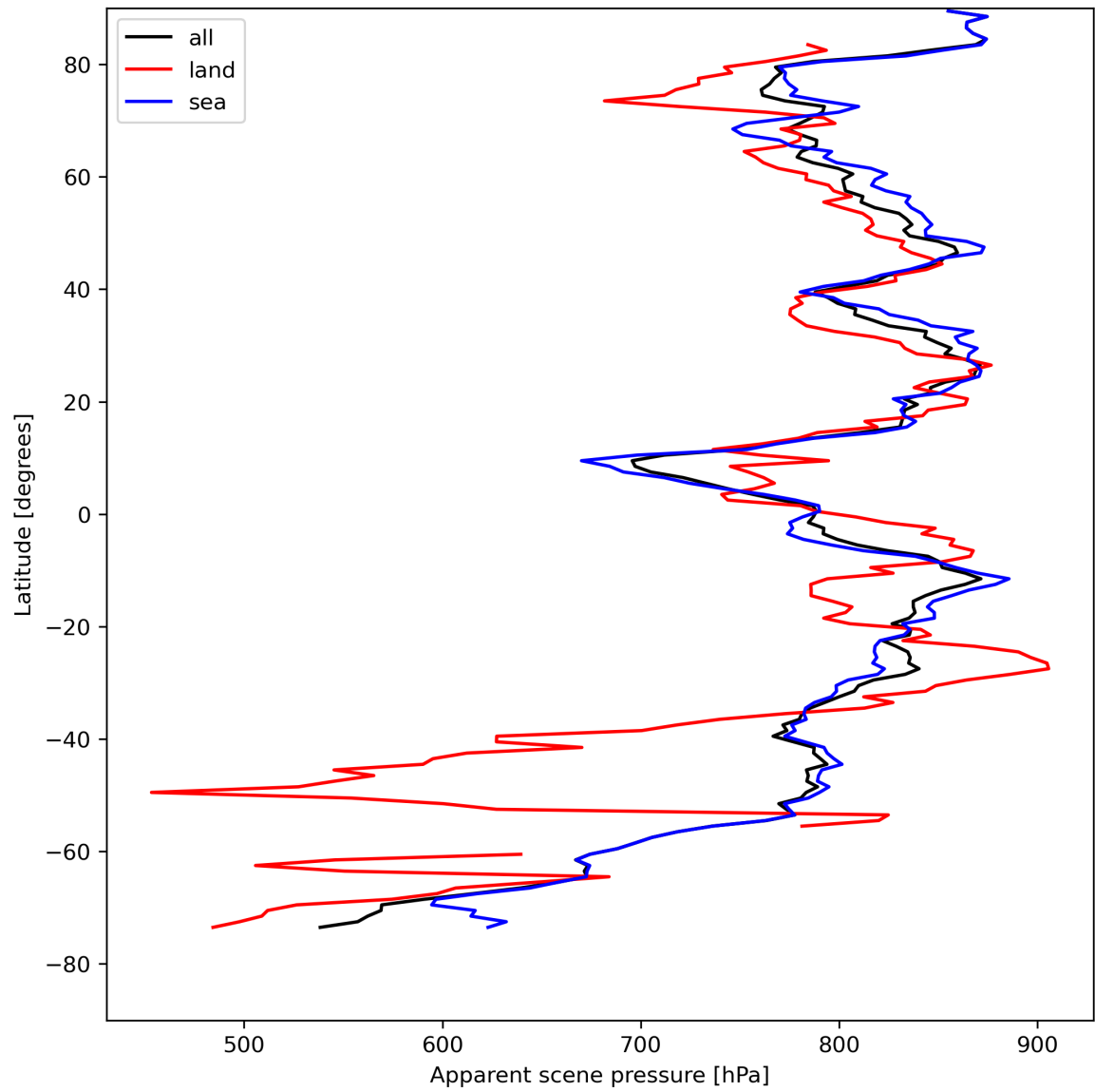
Figure 19: Zonal average of “Apparent scene pressure” for 2023-08-14 to 2023-08-15.
