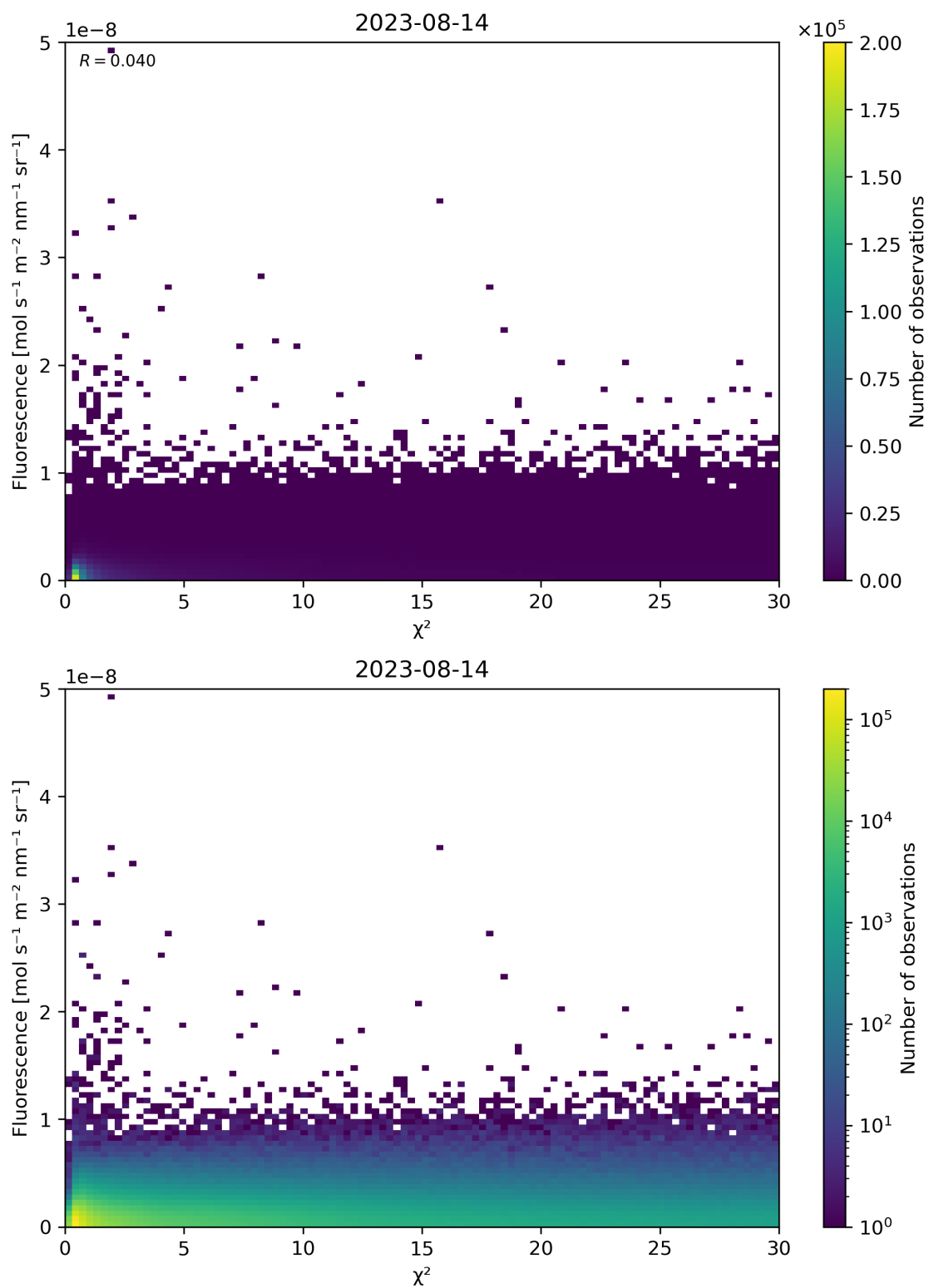
Figure 70: Scatter density plot of “ \chi^2 ” against “Fluorescence” for 2023-08-14 to 2023-08-15.
