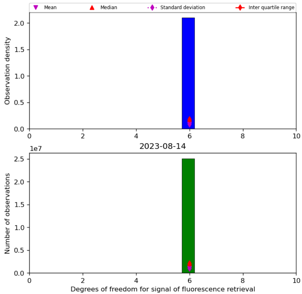
Figure 43: Histogram of “Degrees of freedom for signal of fluorescence retrieval” for 2023-08-14 to 2023-08-15
