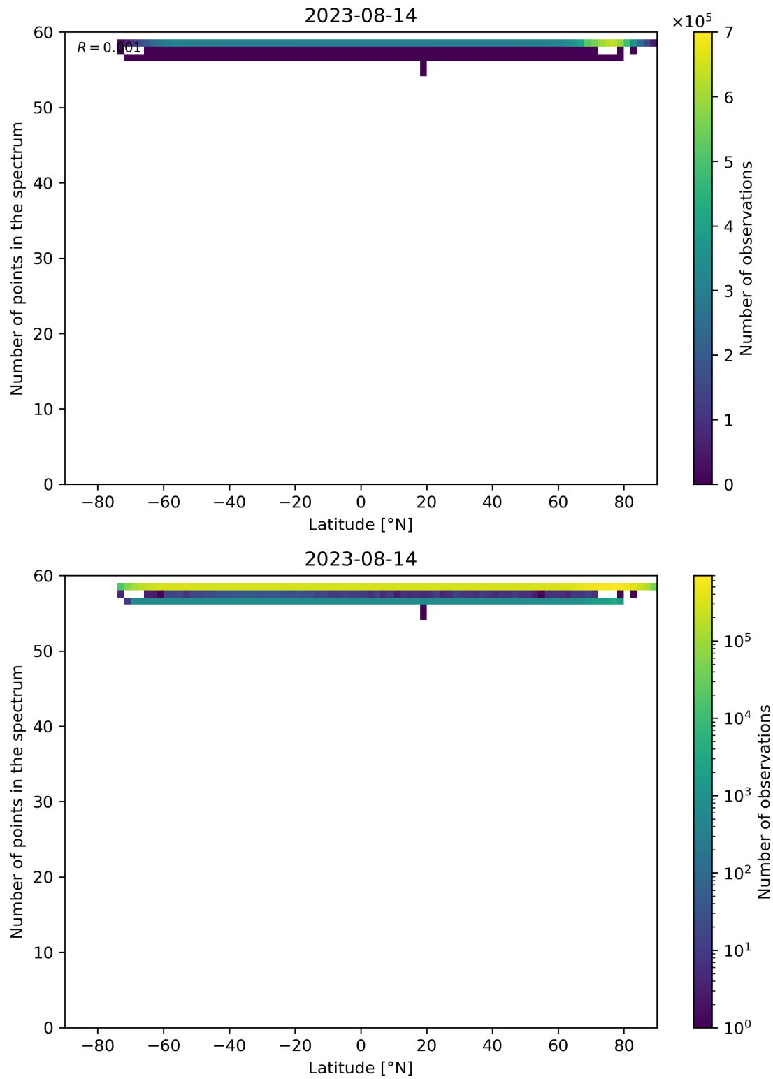
Figure 103: Scatter density plot of “Latitude” against “Number of points in the spectrum” for 2023-08-14 to 2023-08-15.
