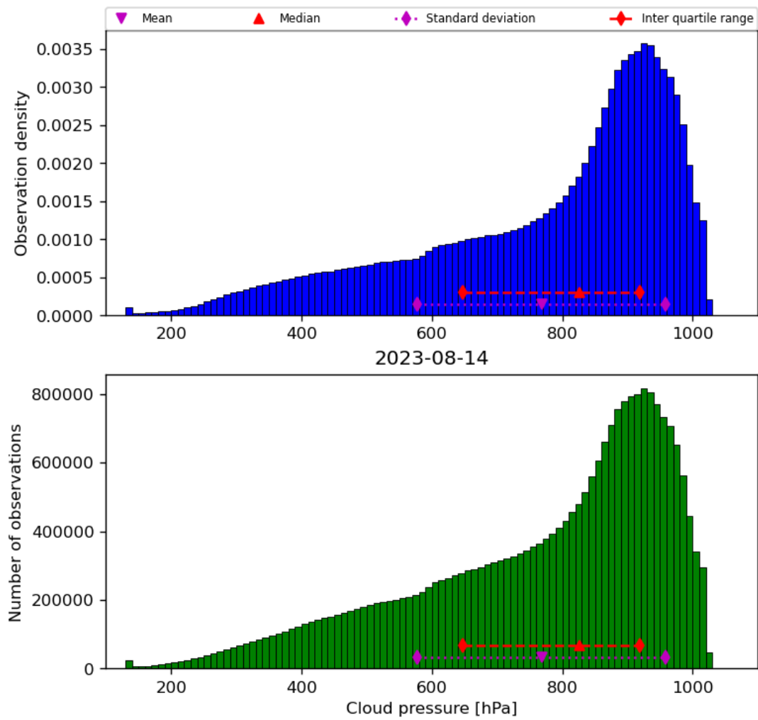
Figure 30: Histogram of “Cloud pressure” for 2023-08-14 to 2023-08-15
