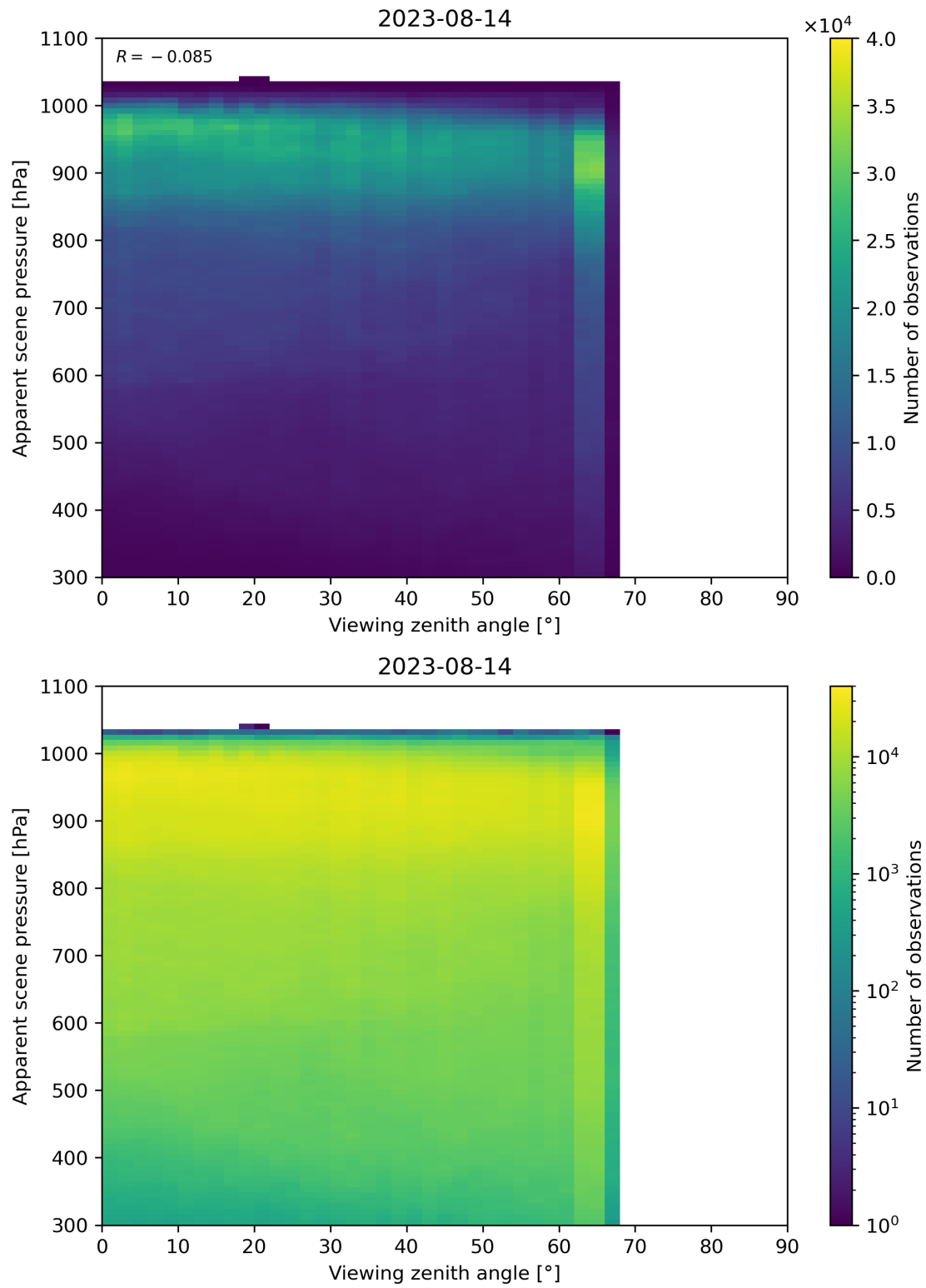
Figure 129: Scatter density plot of “Viewing zenith angle” against “Apparent scene pressure” for 2023-08-14 to 2023-08-15.
