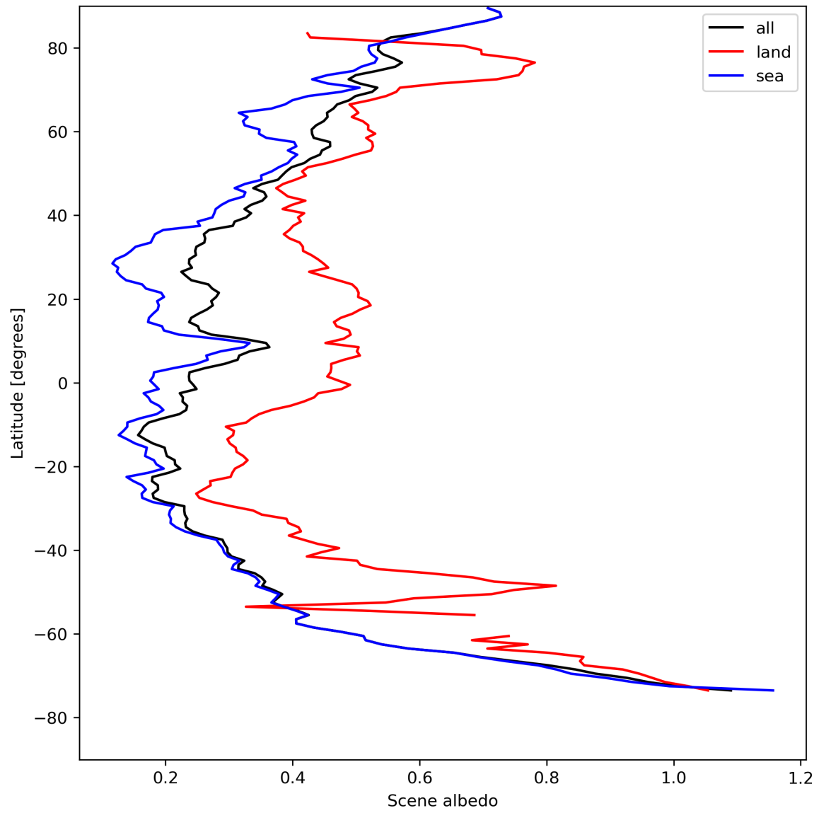
Figure 17: Zonal average of “Scene albedo” for 2023-08-14 to 2023-08-15.
