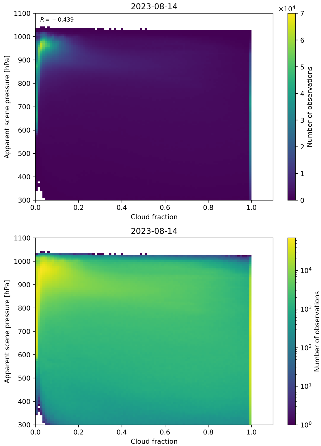
Figure 76: Scatter density plot of “Cloud fraction” against “Apparent scene pressure” for 2023-08-14 to 2023-08-15.
