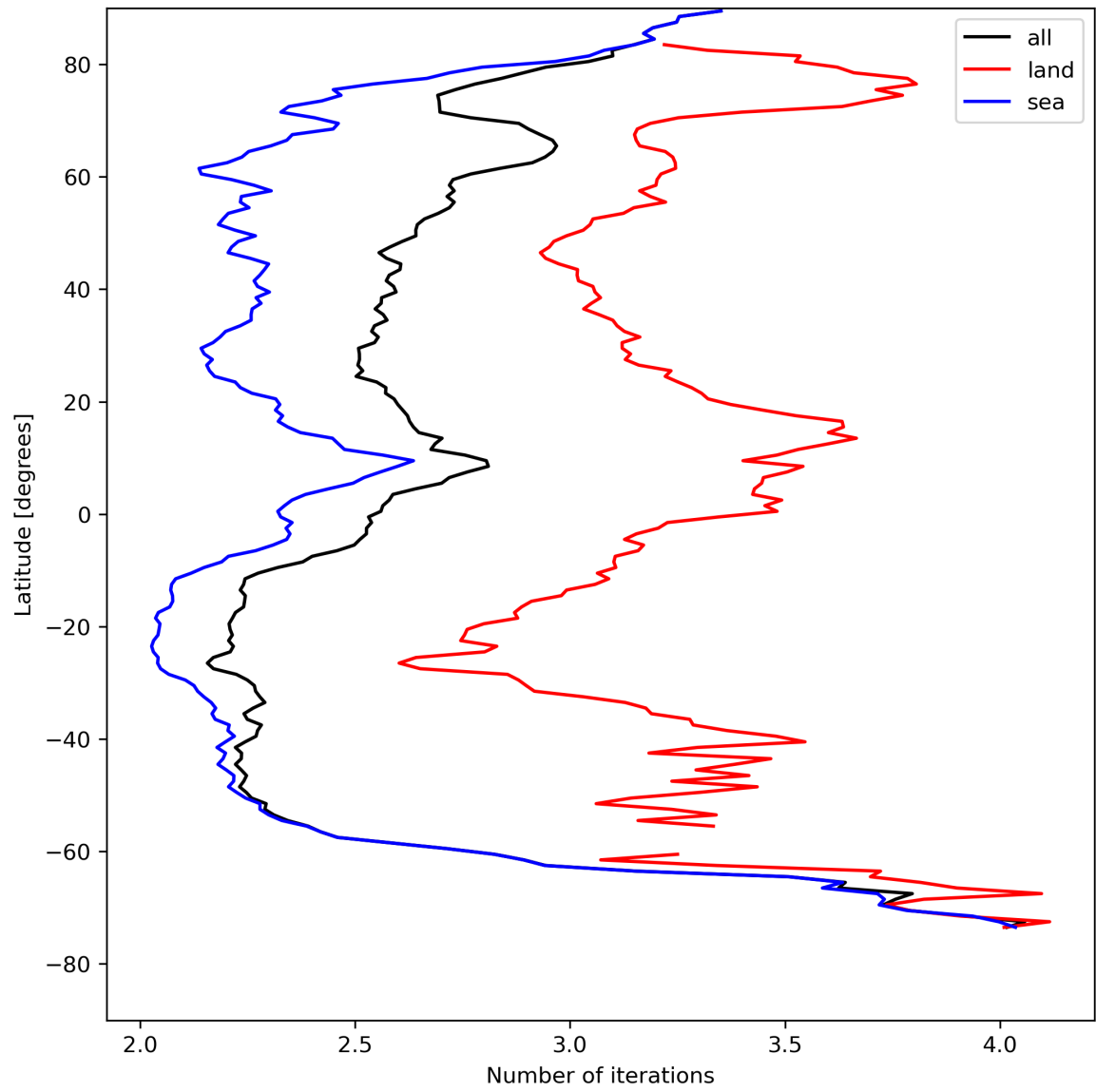
Figure 22: Zonal average of “Number of iterations” for 2023-08-14 to 2023-08-15.
