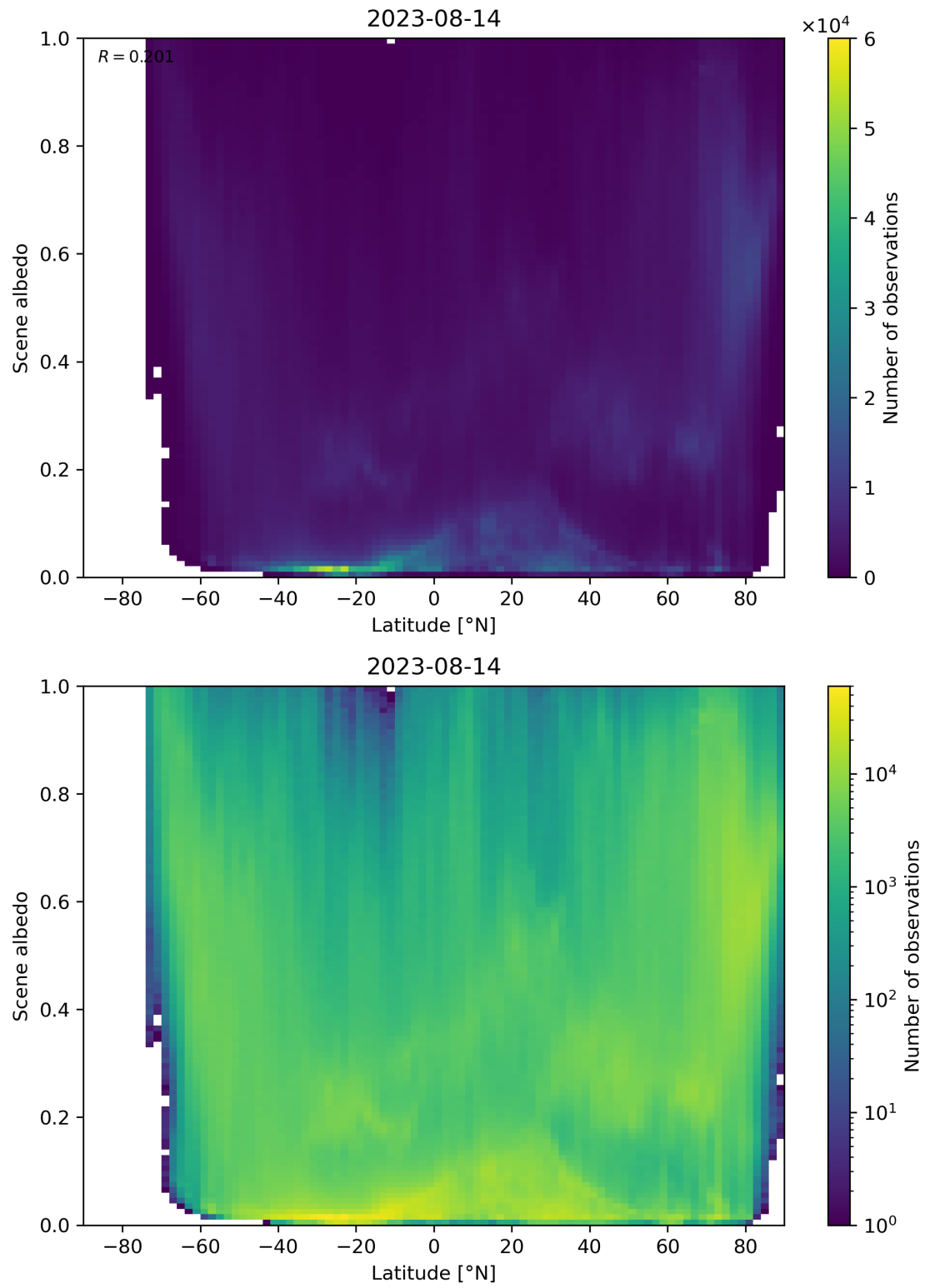
Figure 104: Scatter density plot of “Latitude” against “Scene albedo” for 2023-08-14 to 2023-08-15.
