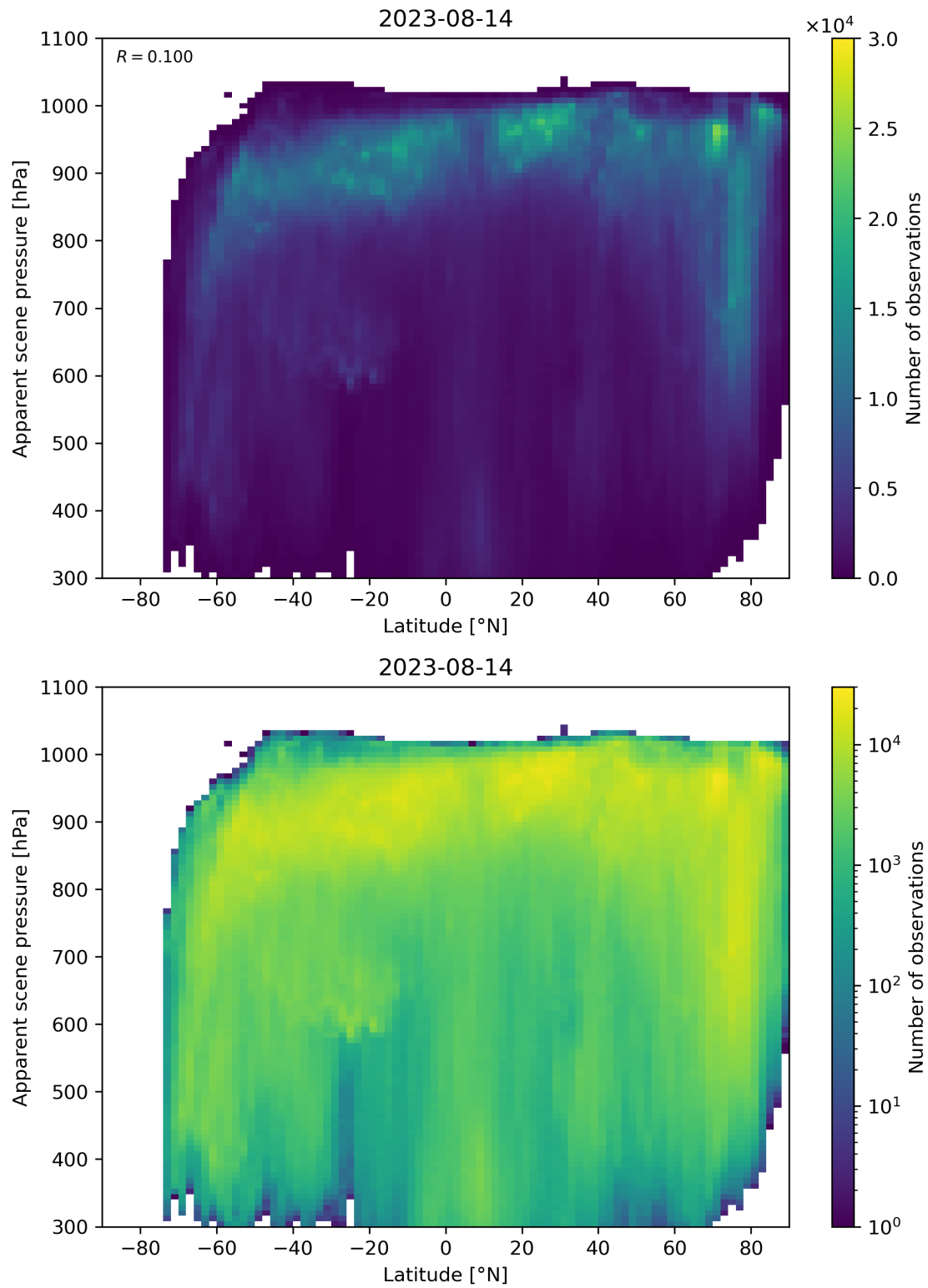
Figure 96: Scatter density plot of “Latitude” against “Apparent scene pressure” for 2023-08-14 to 2023-08-15.
