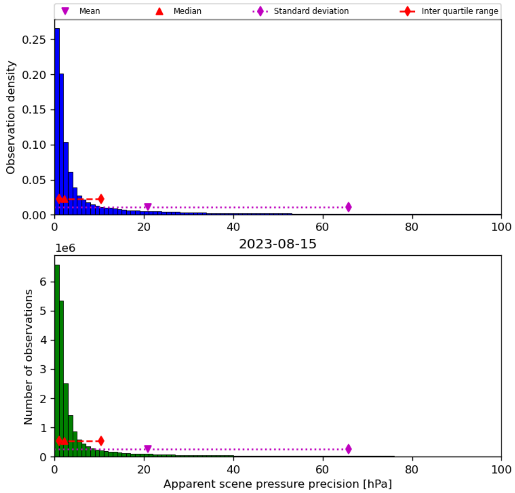
Figure 37: Histogram of “Apparent scene pressure precision” for 2023-08-14 to 2023-08-16
