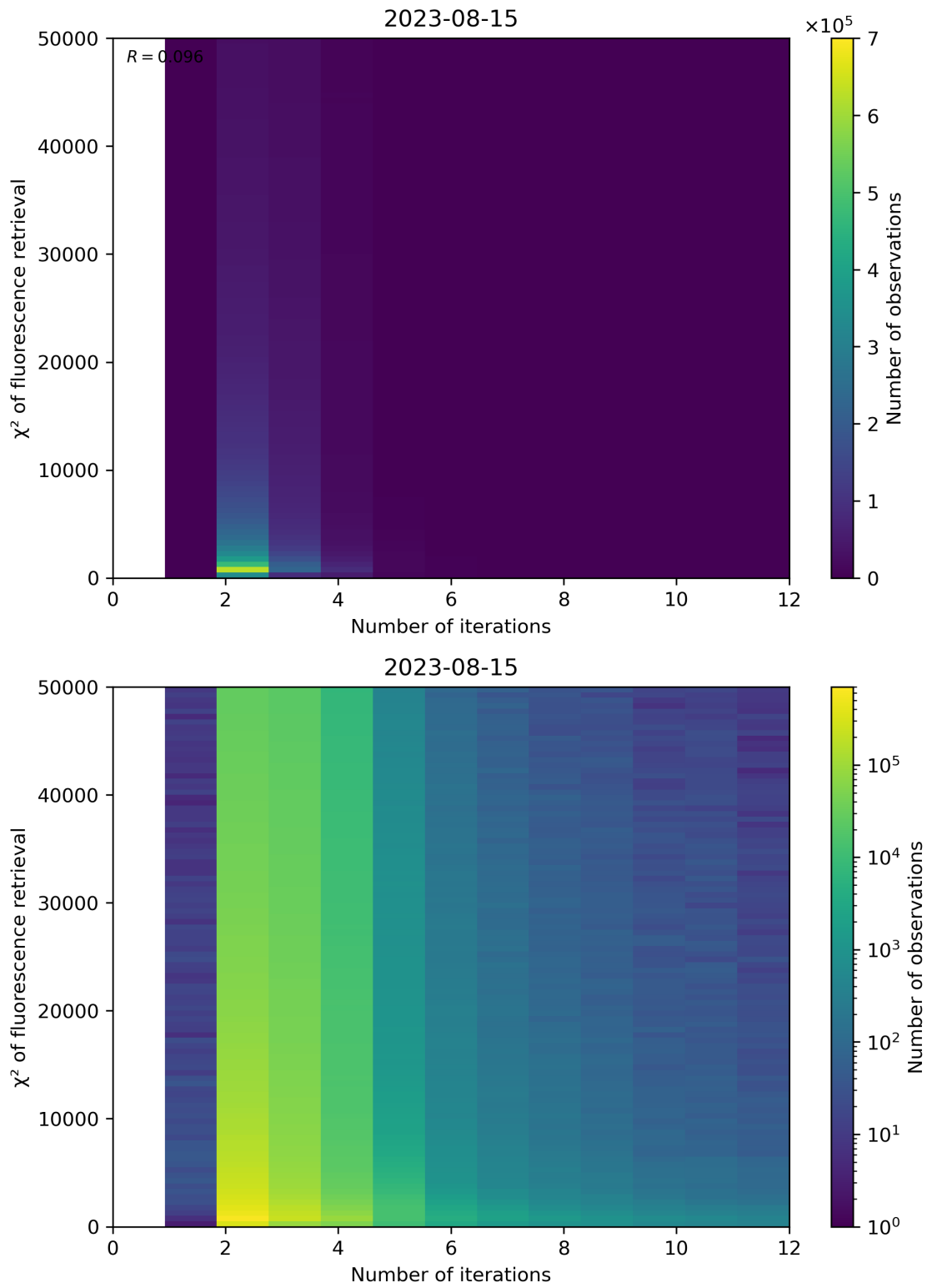
Figure 106: Scatter density plot of “Number of iterations” against “ \chi^2 of fluorescence retrieval” for 2023-08-14 to 2023-08-16.
