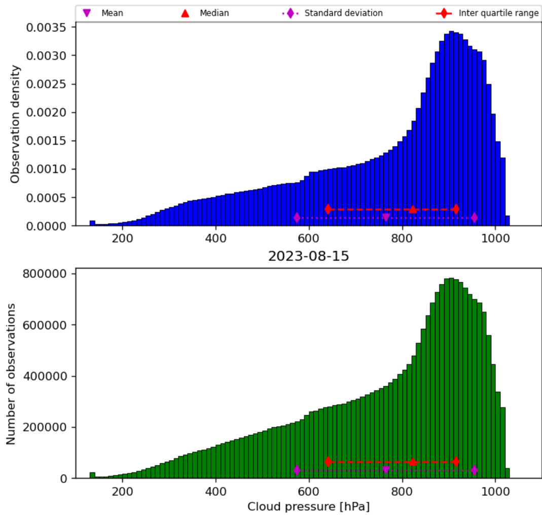
Figure 30: Histogram of “Cloud pressure” for 2023-08-14 to 2023-08-16
