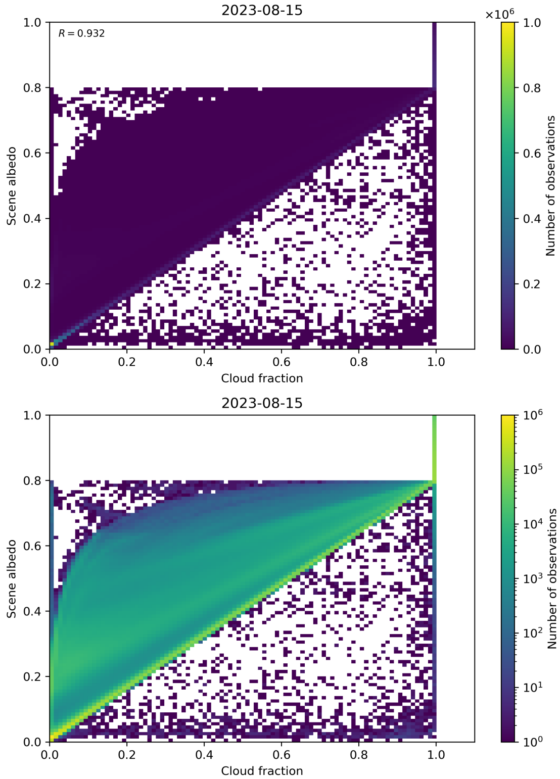
Figure 82: Scatter density plot of “Cloud fraction” against “Scene albedo” for 2023-08-14 to 2023-08-16.
