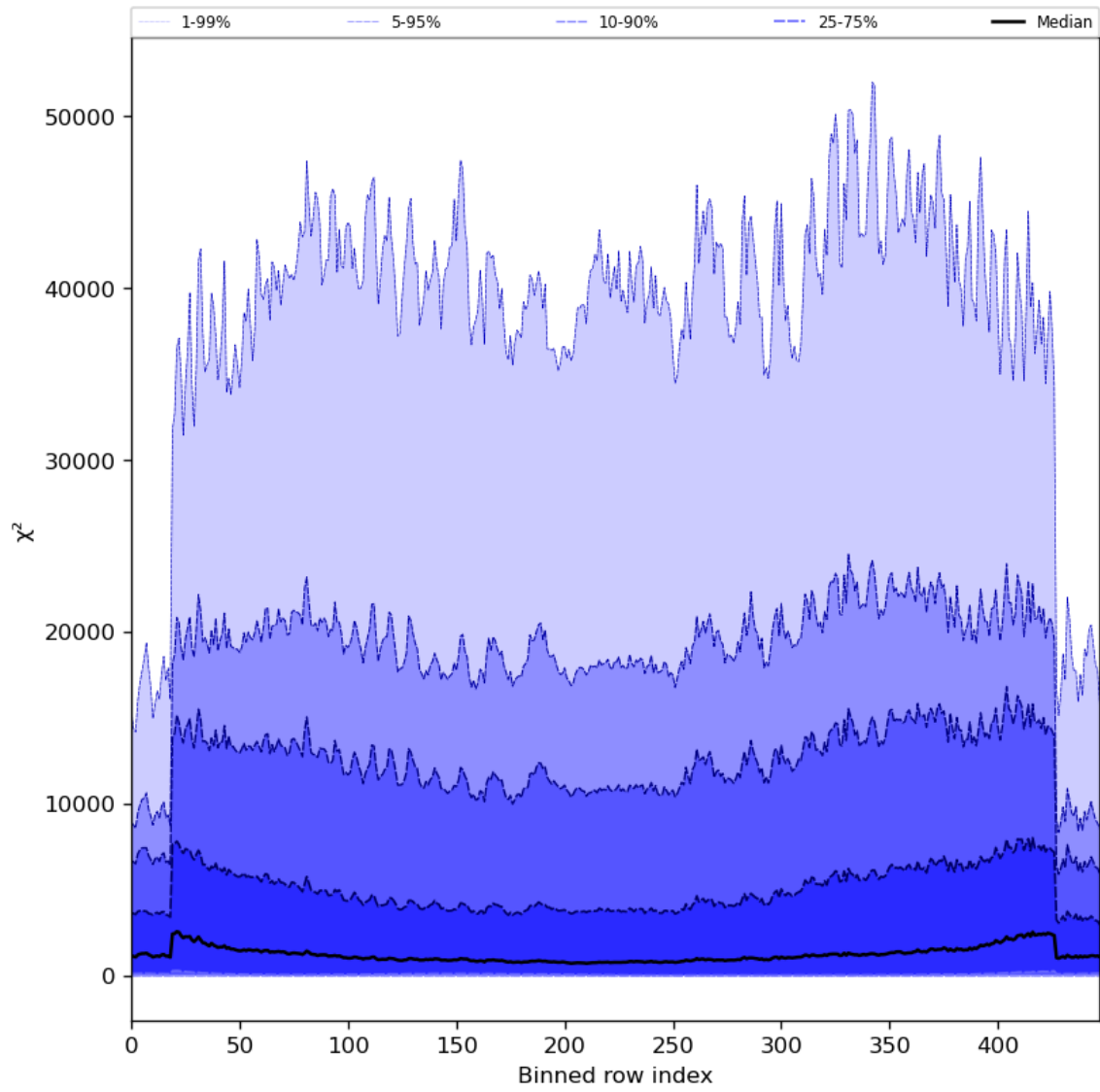
Figure 55: Along track statistics of “ \chi^2 ” for 2023-08-14 to 2023-08-16
