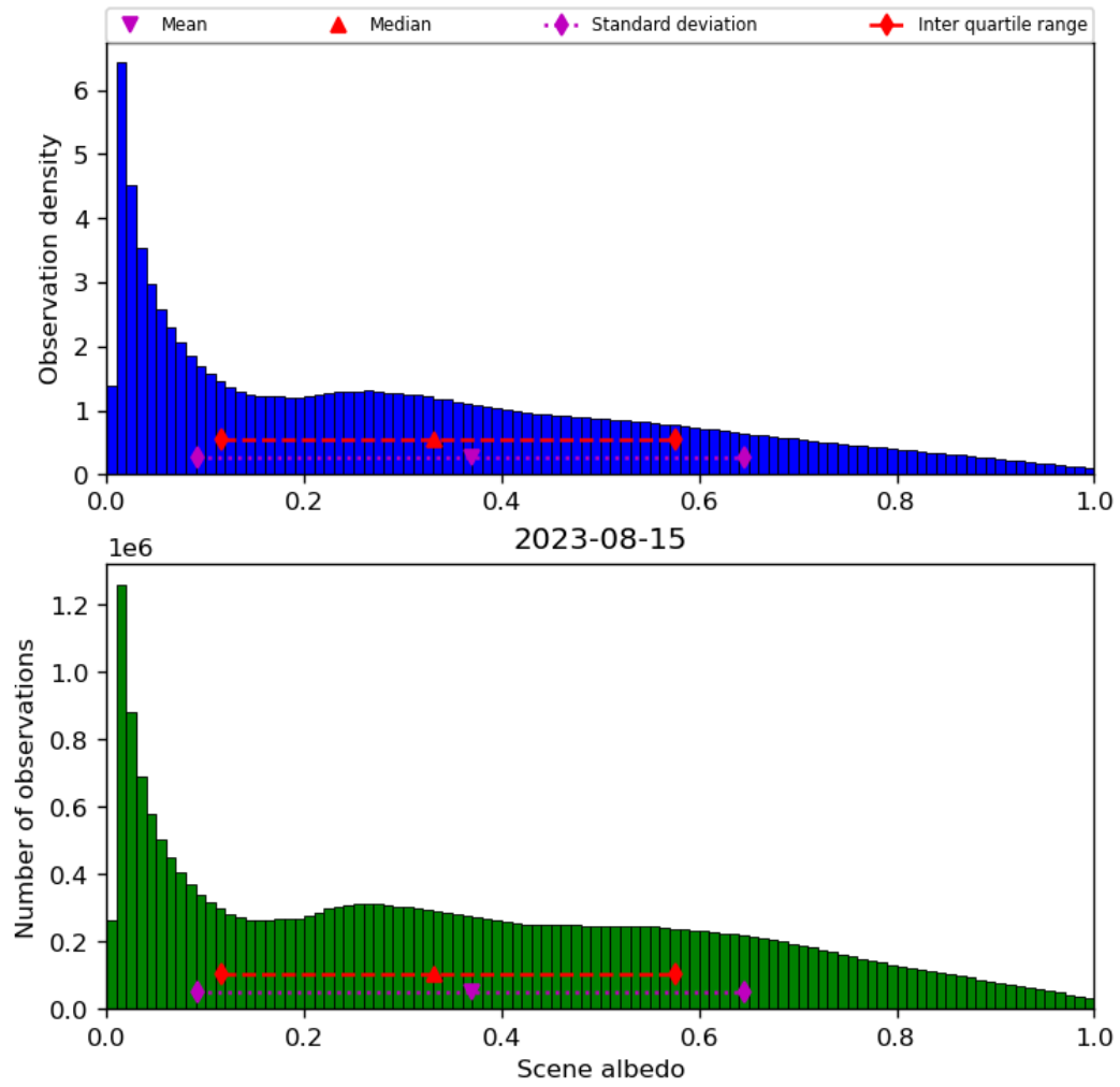
Figure 34: Histogram of “Scene albedo” for 2023-08-14 to 2023-08-16
