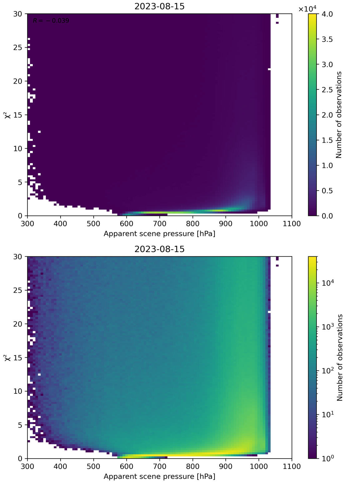
Figure 63: Scatter density plot of “Apparent scene pressure” against “ \chi^2 ” for 2023-08-14 to 2023-08-16.
