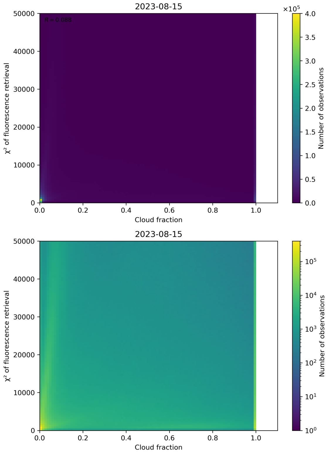
Figure 78: Scatter density plot of “Cloud fraction” against “ \chi^2 of fluorescence retrieval” for 2023-08-14 to 2023-08-16.
