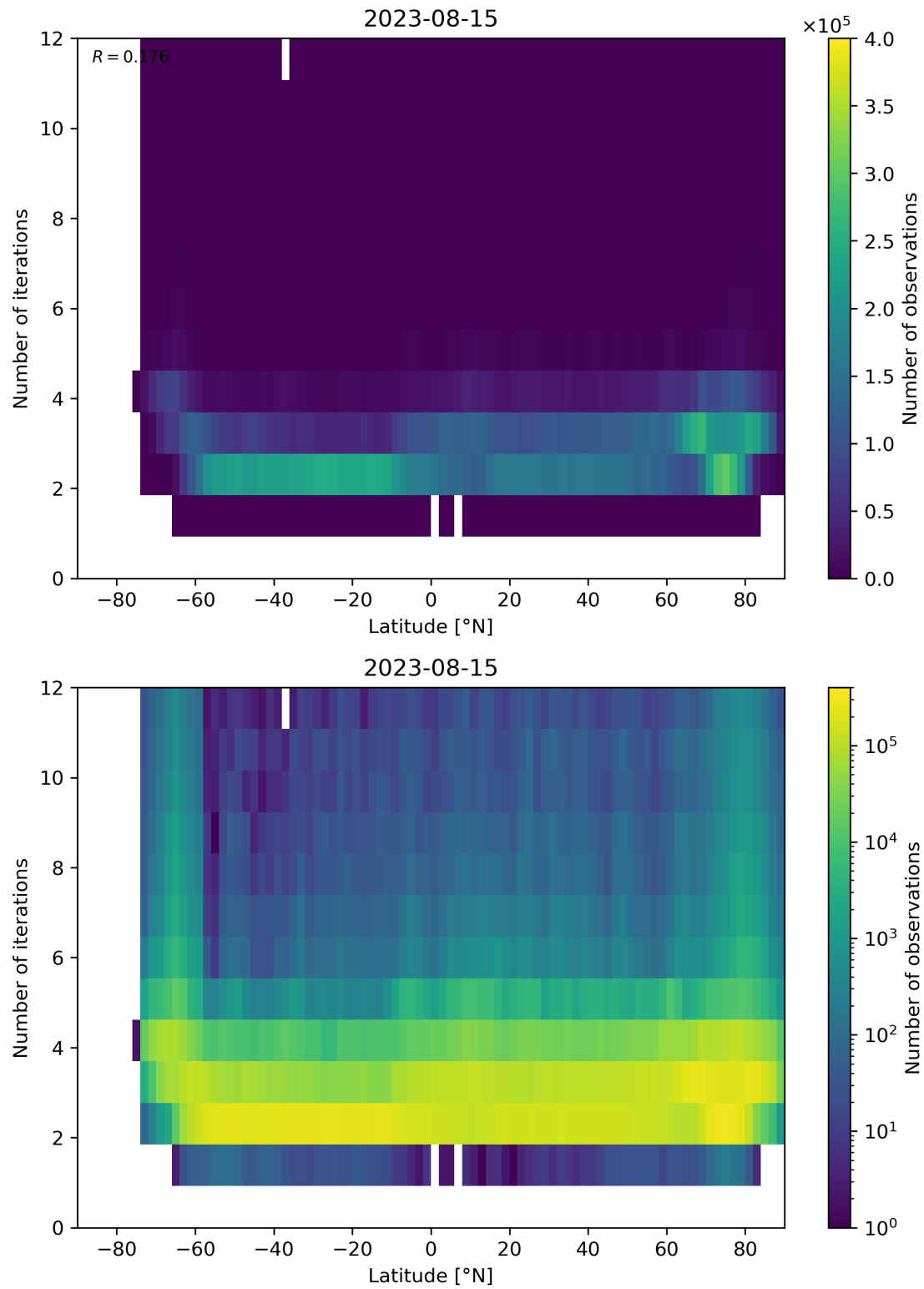
Figure 102: Scatter density plot of “Latitude” against “Number of iterations” for 2023-08-14 to 2023-08-16.
