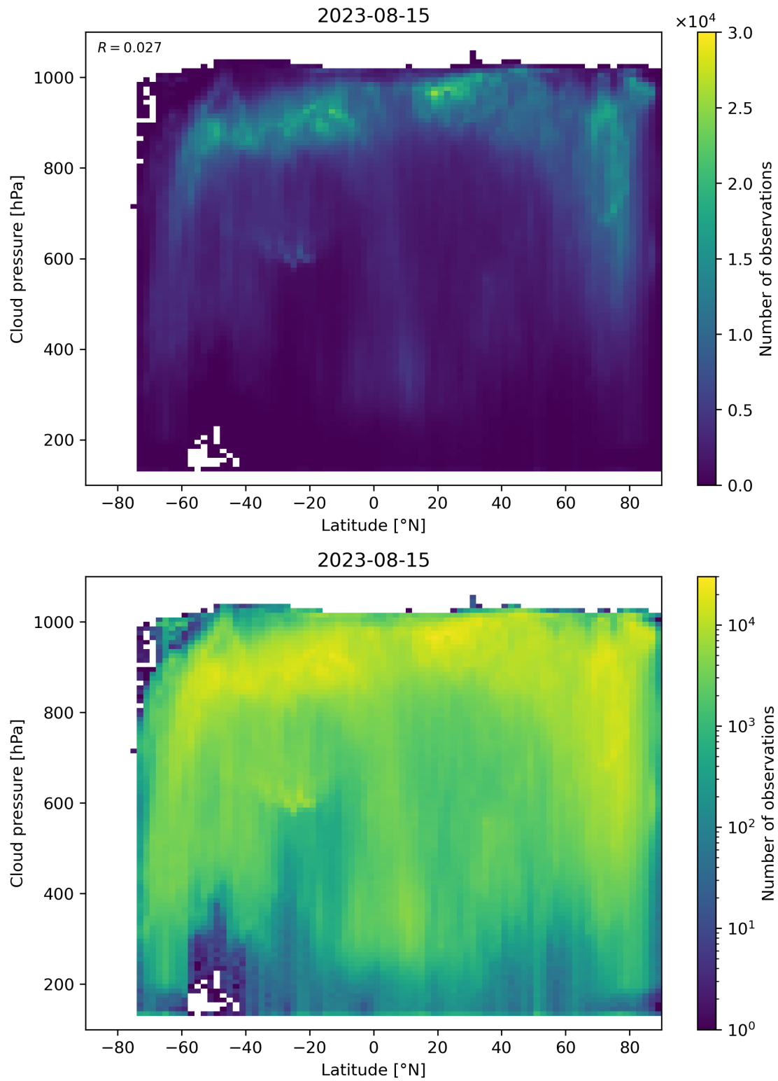
Figure 100: Scatter density plot of “Latitude” against “Cloud pressure” for 2023-08-14 to 2023-08-16.
