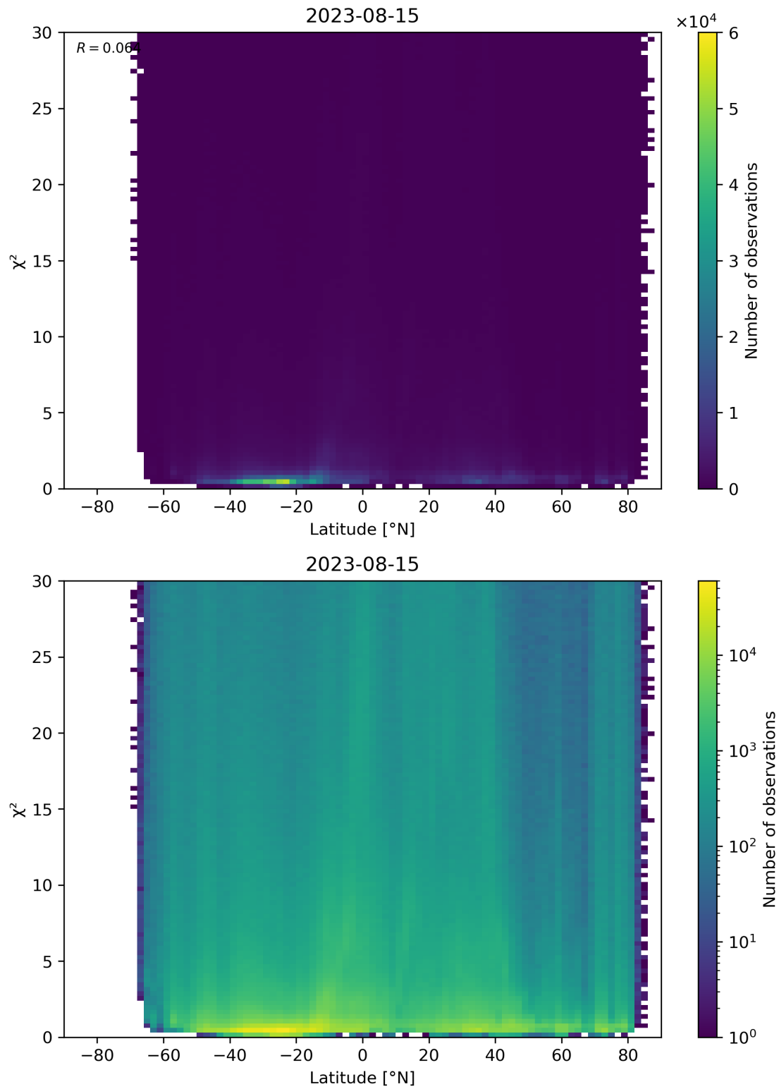
Figure 97: Scatter density plot of “Latitude” against “ \chi^2 ” for 2023-08-14 to 2023-08-16.
