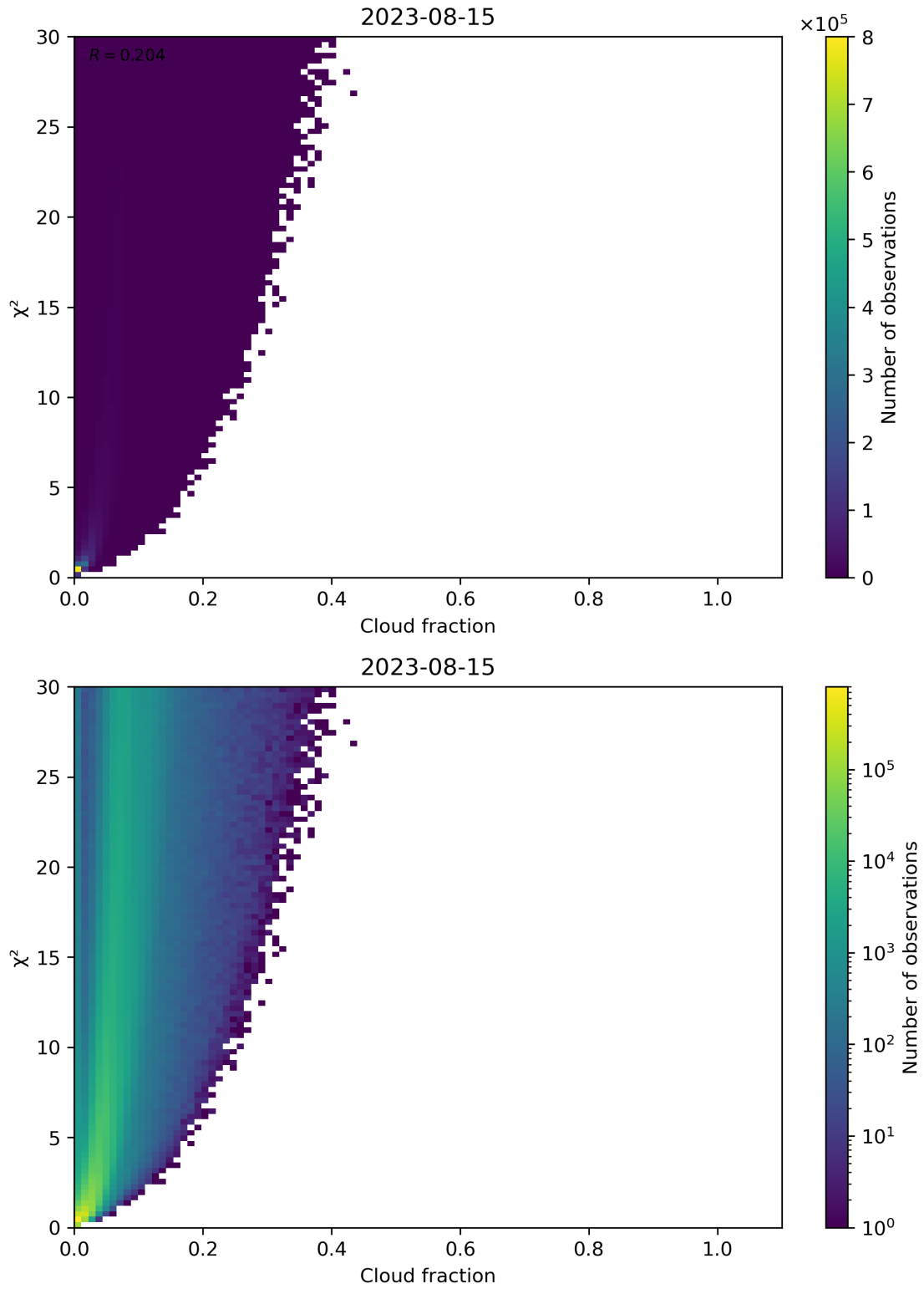
Figure 77: Scatter density plot of “Cloud fraction” against “ \chi^2 ” for 2023-08-14 to 2023-08-16.
