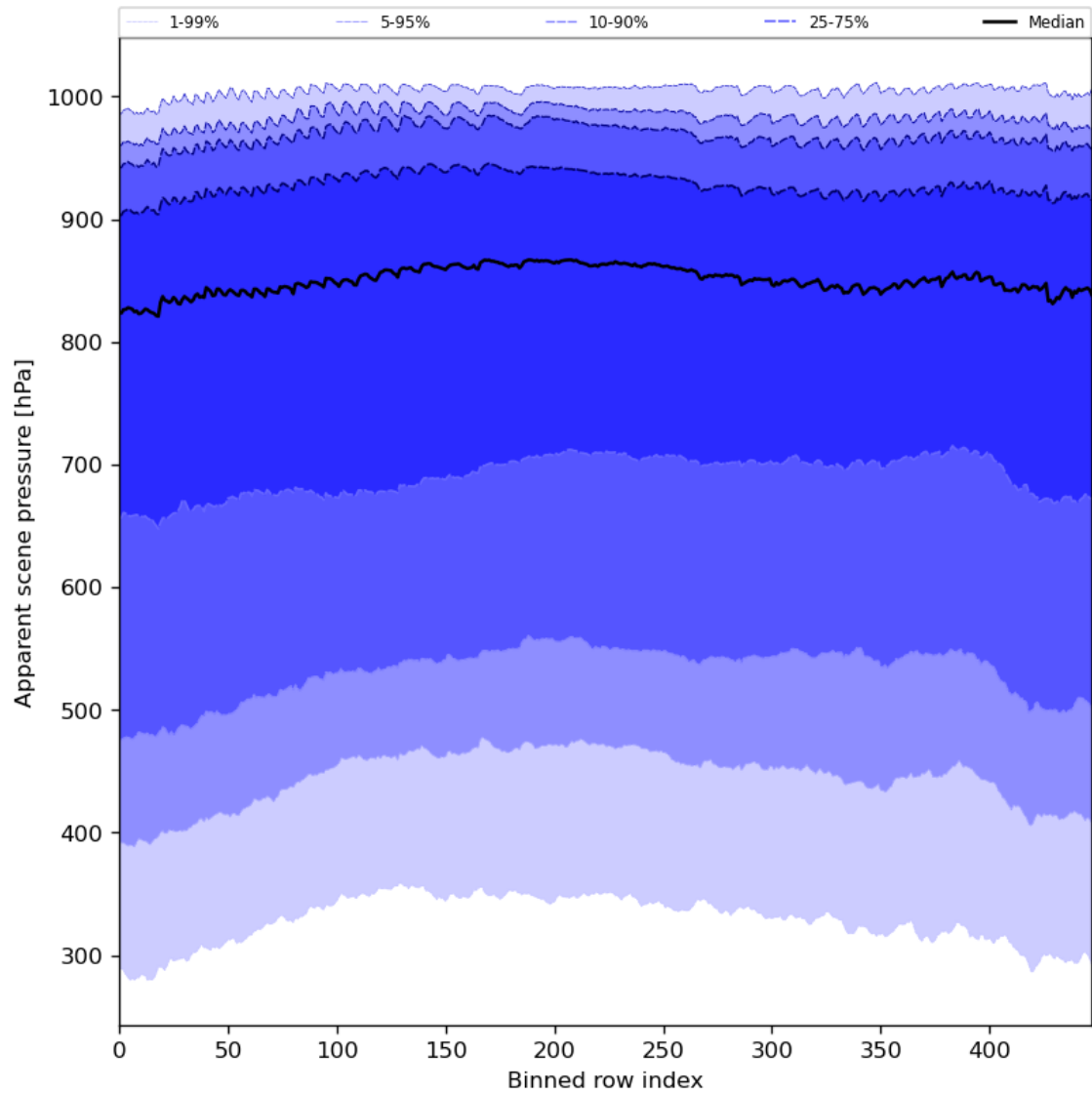
Figure 53: Along track statistics of “Apparent scene pressure” for 2023-08-14 to 2023-08-16
