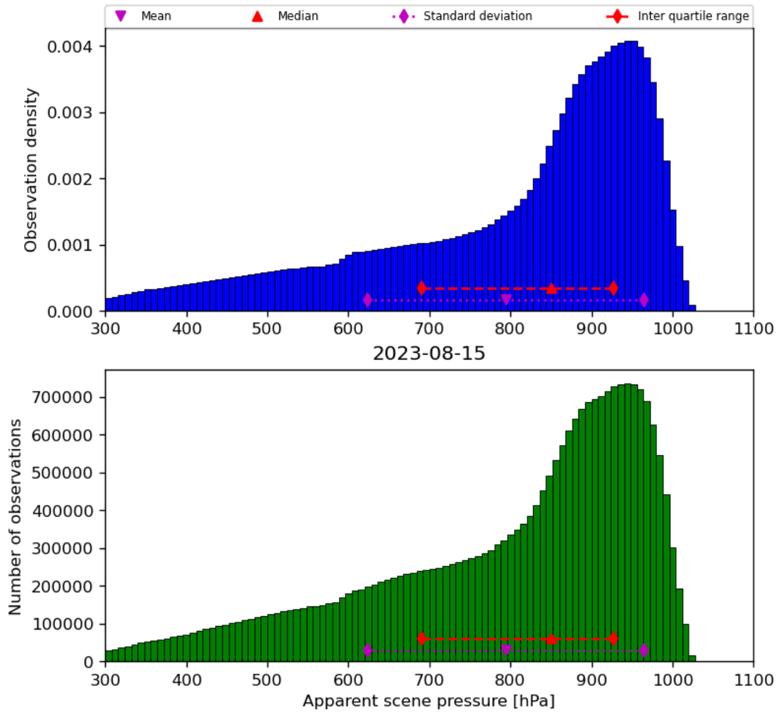
Figure 36: Histogram of “Apparent scene pressure” for 2023-08-14 to 2023-08-16
