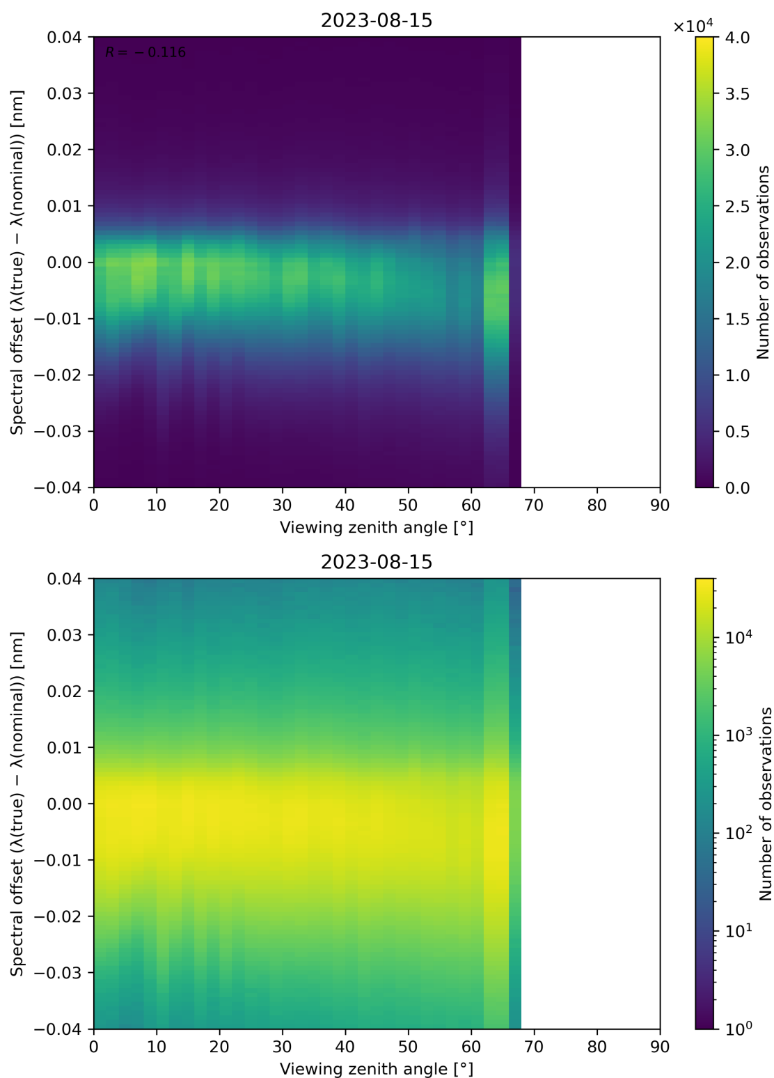
Figure 140: Scatter density plot of “Viewing zenith angle” against “Spectral offset ( \lambda(\text{true}) - \lambda(\text{nominal}) )” for 2023-08-14 to 2023-08-16.
