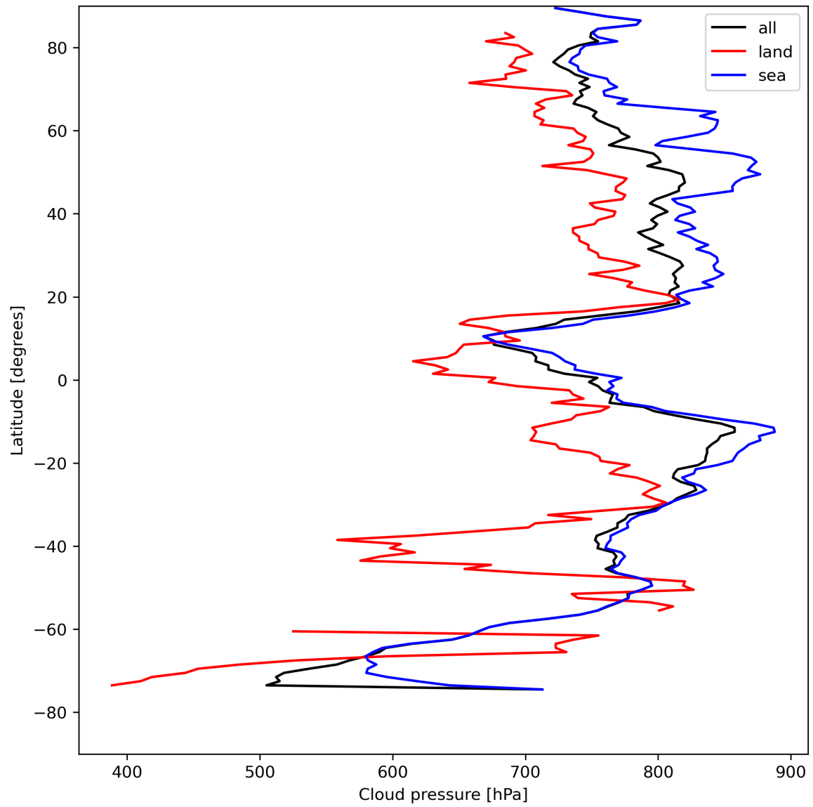
Figure 13: Zonal average of “Cloud pressure” for 2023-08-14 to 2023-08-16.
