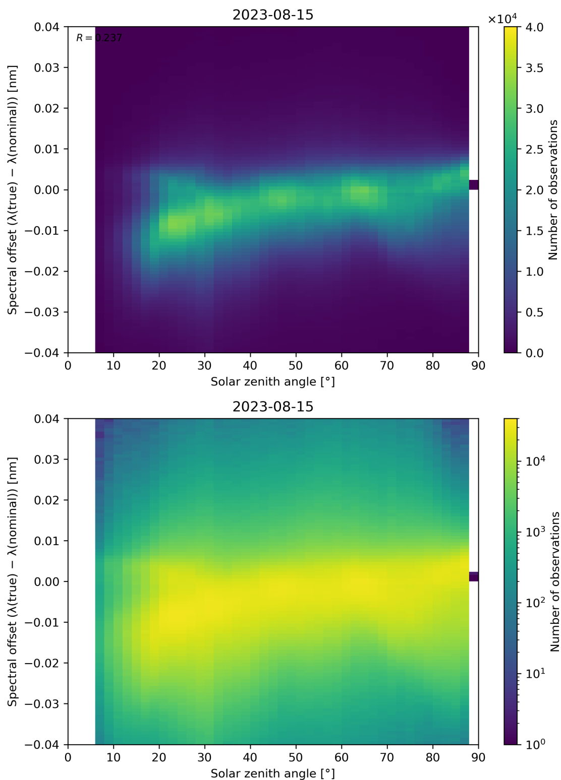
Figure 128: Scatter density plot of “Solar zenith angle” against “Spectral offset ( \lambda(\text{true}) - \lambda(\text{nominal}) )” for 2023-08-14 to 2023-08-16.
