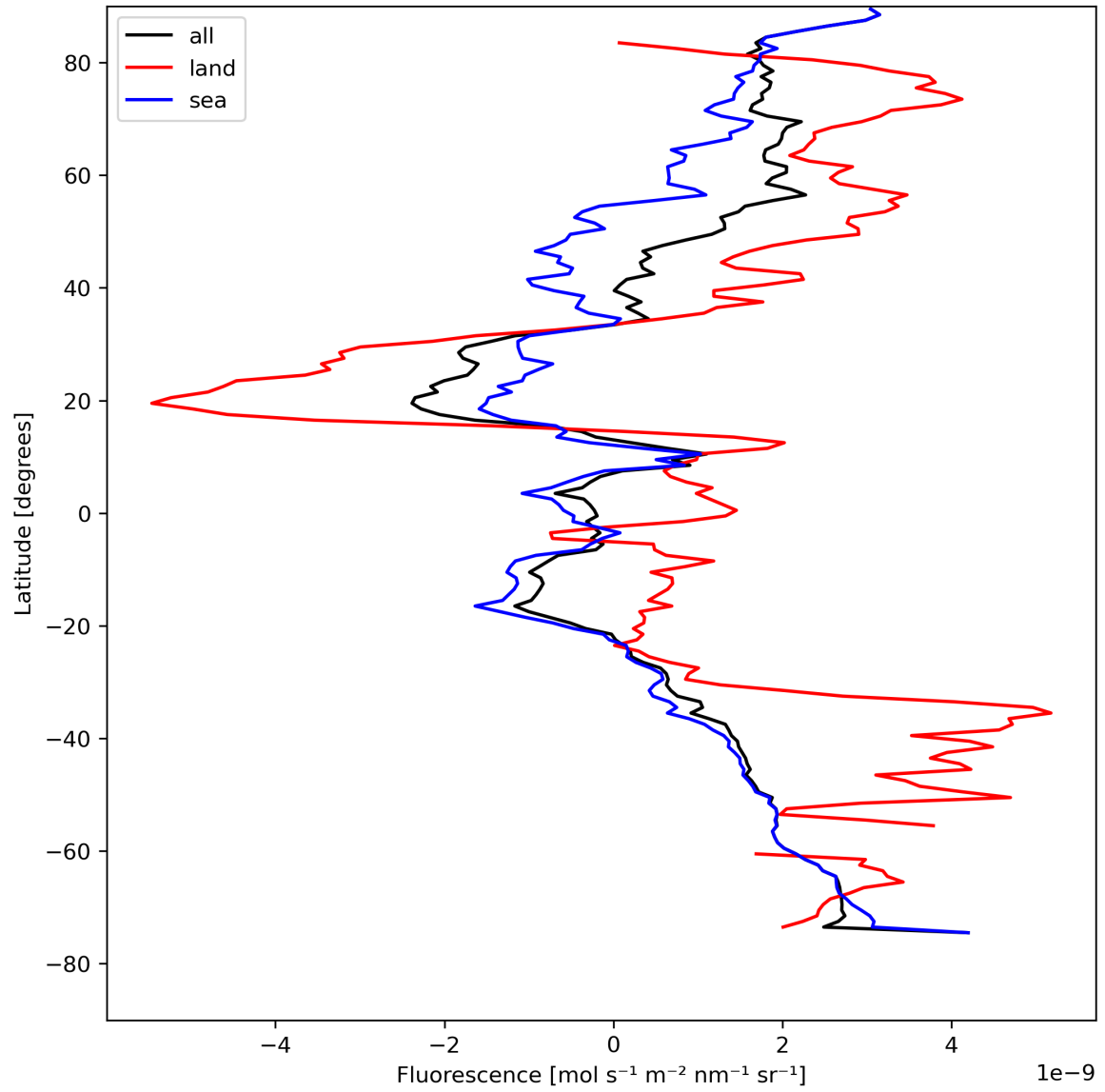
Figure 23: Zonal average of “Fluorescence” for 2023-08-14 to 2023-08-16.
