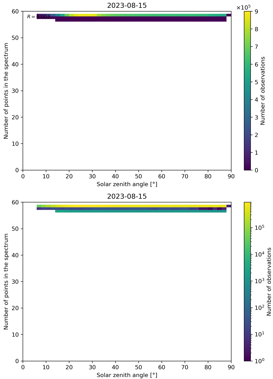
Figure 126: Scatter density plot of “Solar zenith angle” against “Number of points in the spectrum” for 2023-08-14 to 2023-08-16.
