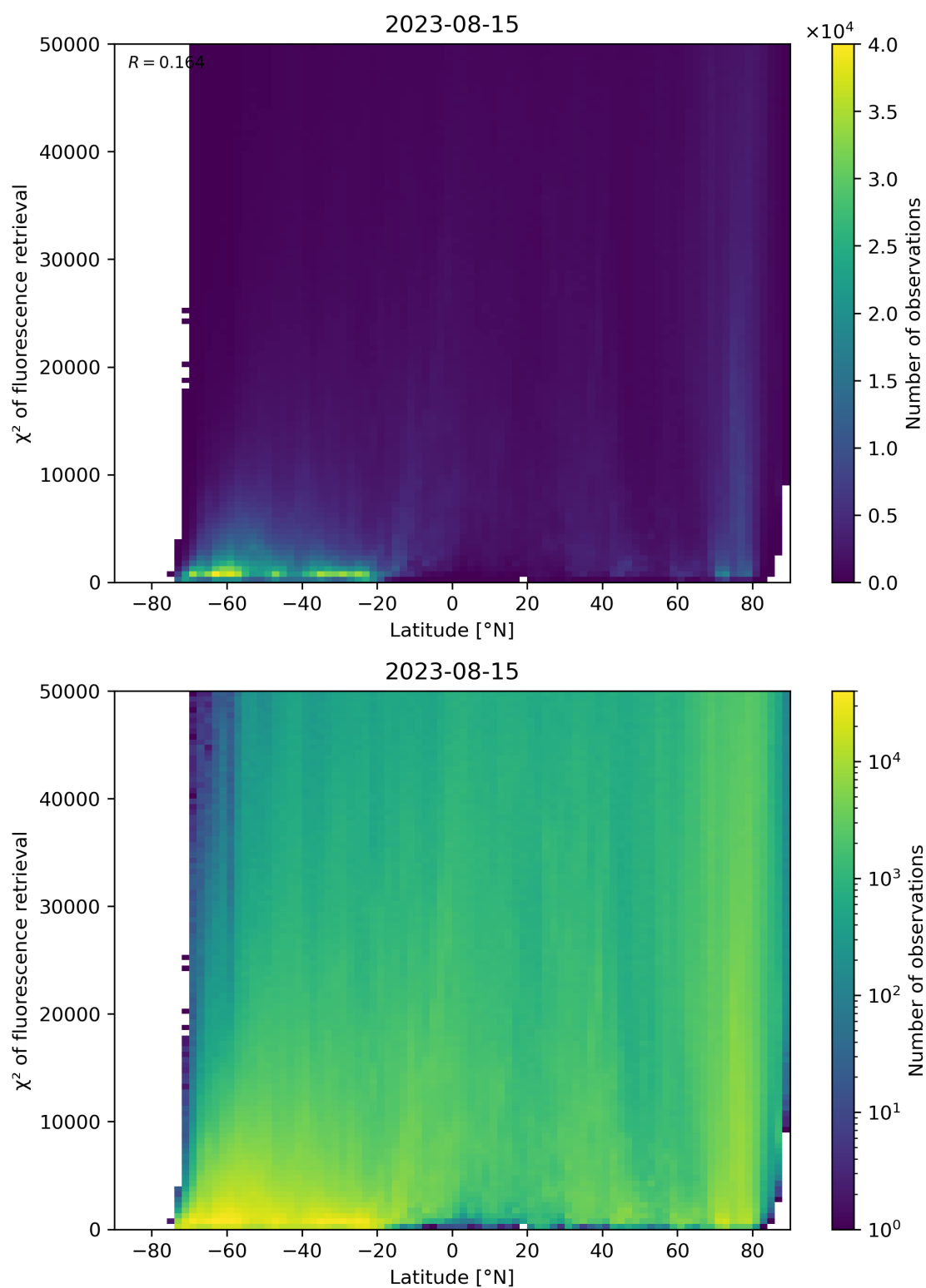
Figure 98: Scatter density plot of “Latitude” against “ \chi^2 of fluorescence retrieval” for 2023-08-14 to 2023-08-16.
