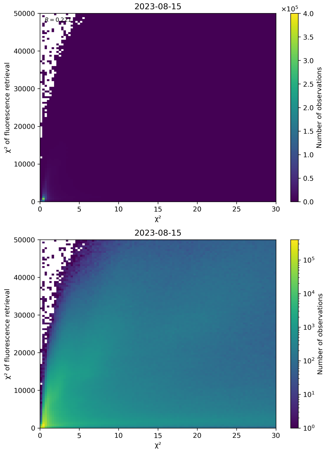
Figure 69: Scatter density plot of “ \chi^2 ” against “ \chi^2 of fluorescence retrieval” for 2023-08-14 to 2023-08-16.
