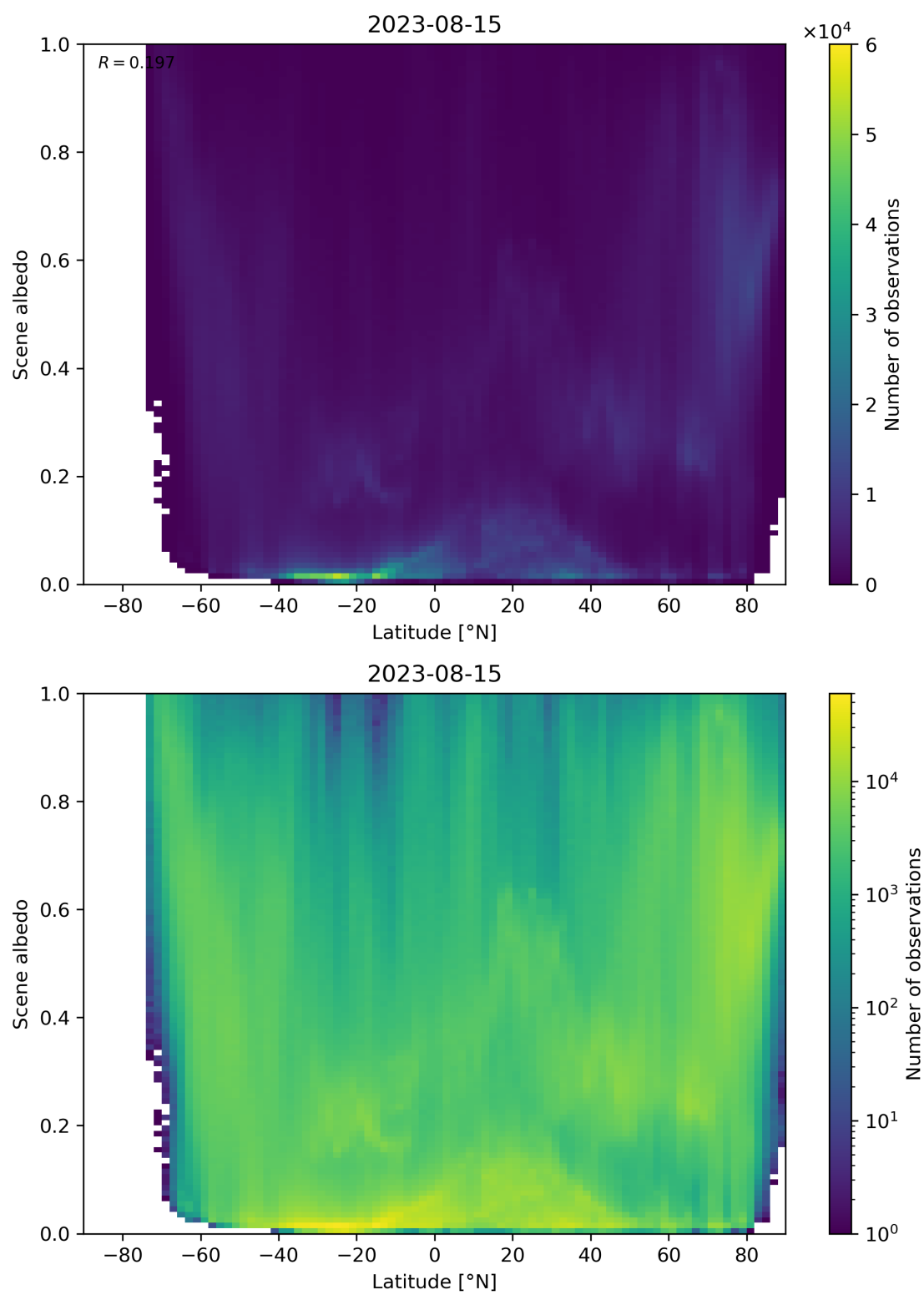
Figure 104: Scatter density plot of “Latitude” against “Scene albedo” for 2023-08-14 to 2023-08-16.
