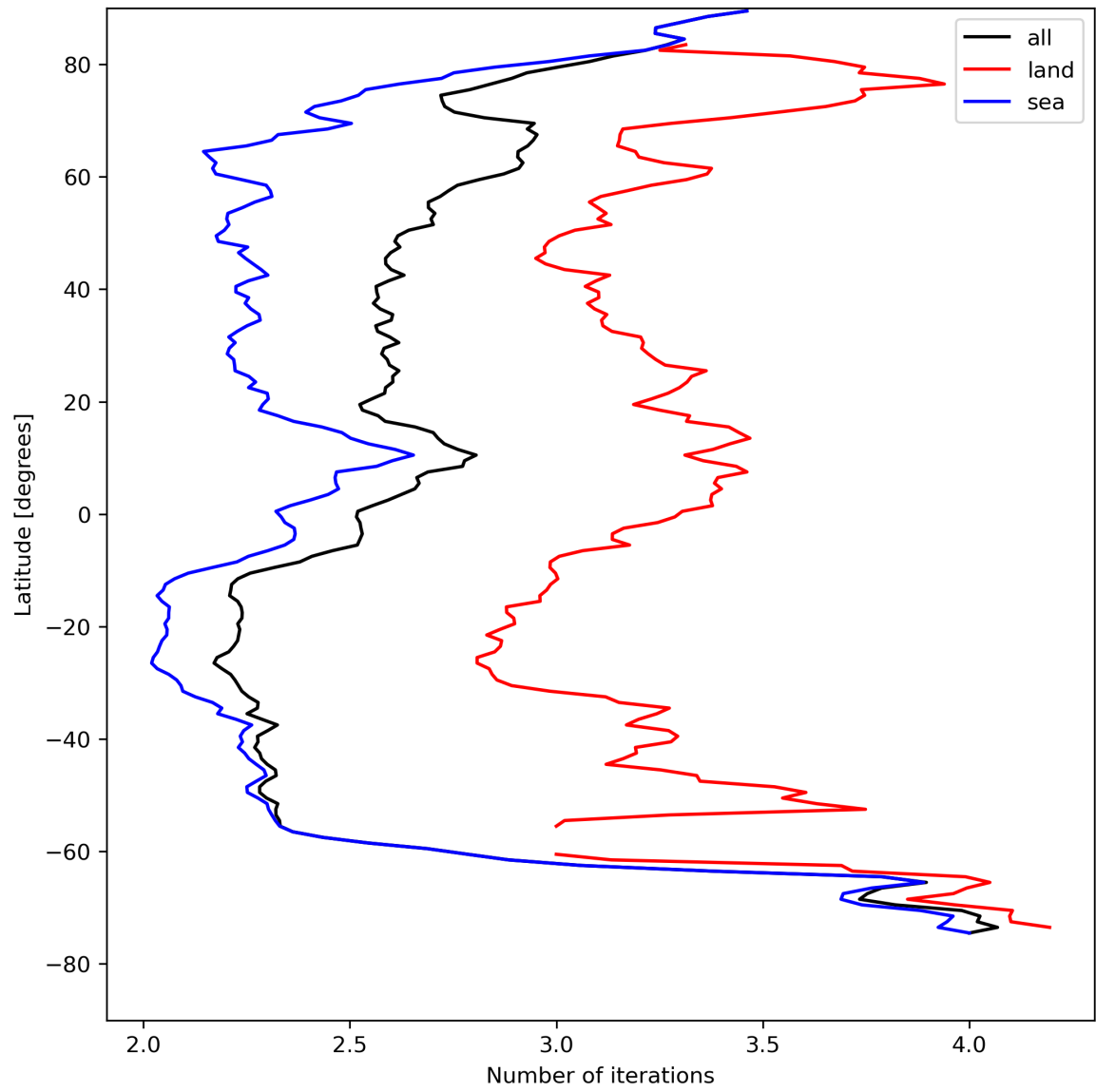
Figure 22: Zonal average of “Number of iterations” for 2023-08-14 to 2023-08-16.
