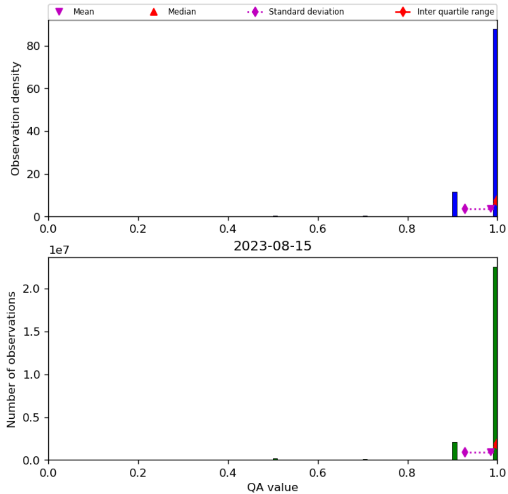
Figure 29: Histogram of “QA value” for 2023-08-14 to 2023-08-16
