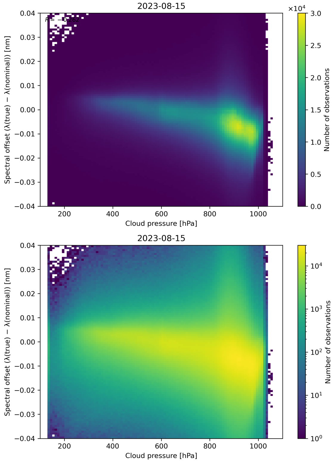
Figure 92: Scatter density plot of “Cloud pressure” against “Spectral offset ( \lambda(\text{true}) - \lambda(\text{nominal}) )” for 2023-08-14 to 2023-08-16.
