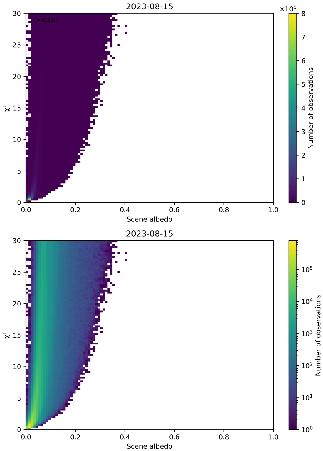
Figure 112: Scatter density plot of “Scene albedo” against “ \chi^2 ” for 2023-08-14 to 2023-08-16.
