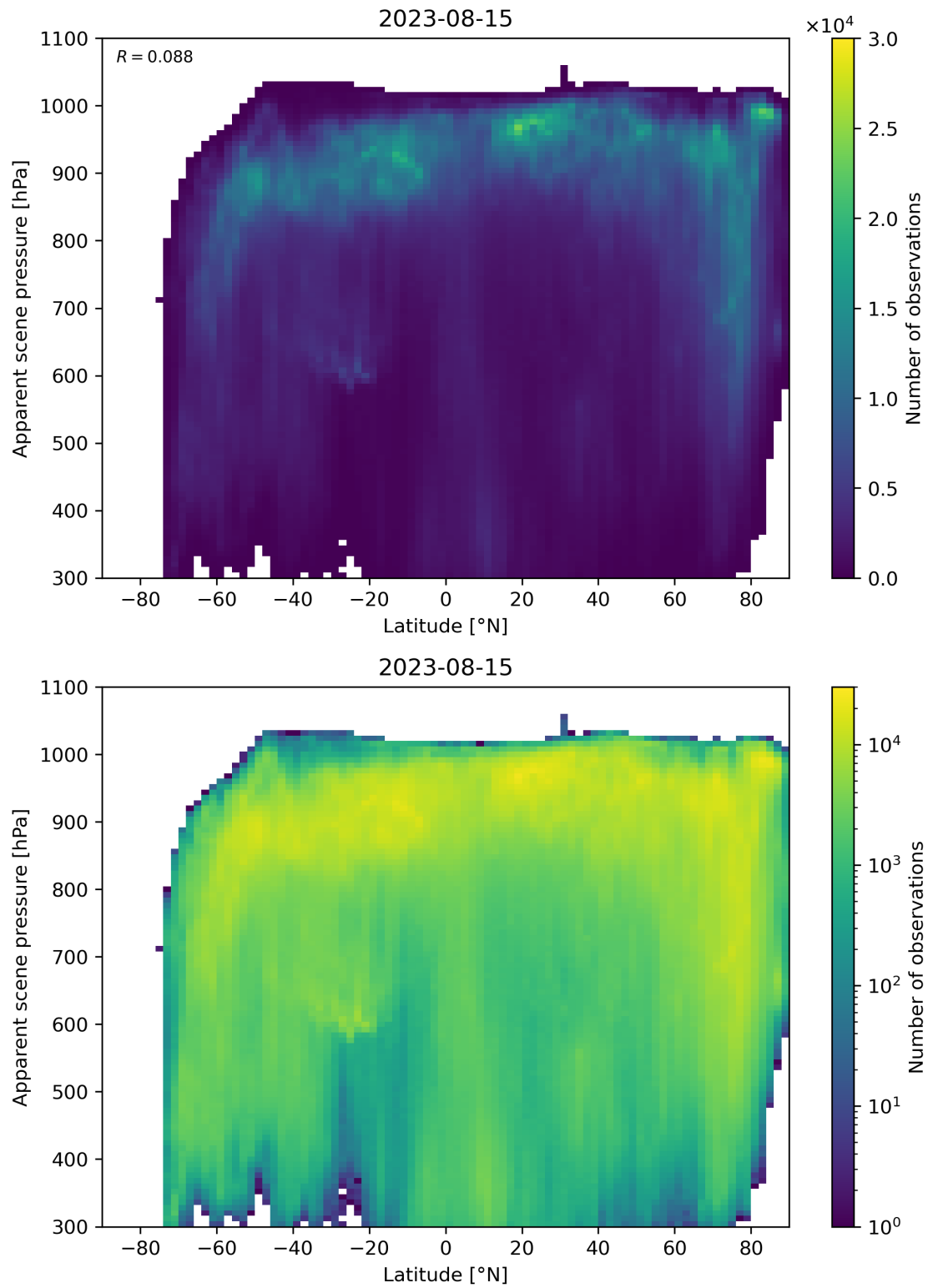
Figure 96: Scatter density plot of “Latitude” against “Apparent scene pressure” for 2023-08-14 to 2023-08-16.
