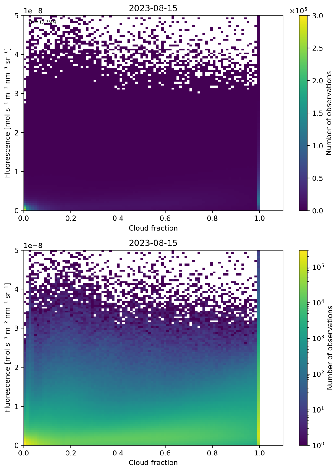
Figure 79: Scatter density plot of “Cloud fraction” against “Fluorescence” for 2023-08-14 to 2023-08-16.
