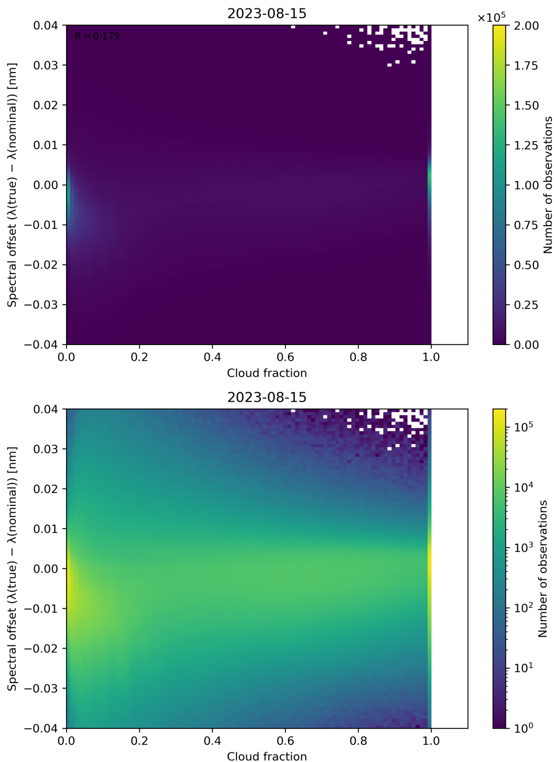
Figure 83: Scatter density plot of “Cloud fraction” against “Spectral offset ( \lambda(\text{true}) - \lambda(\text{nominal}) )” for 2023-08-14 to 2023-08-16.
