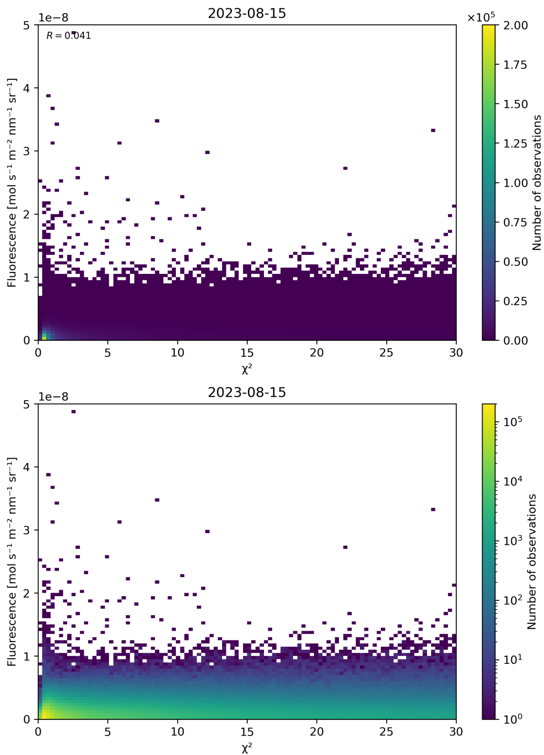
Figure 70: Scatter density plot of “ \chi^2 ” against “Fluorescence” for 2023-08-14 to 2023-08-16.
