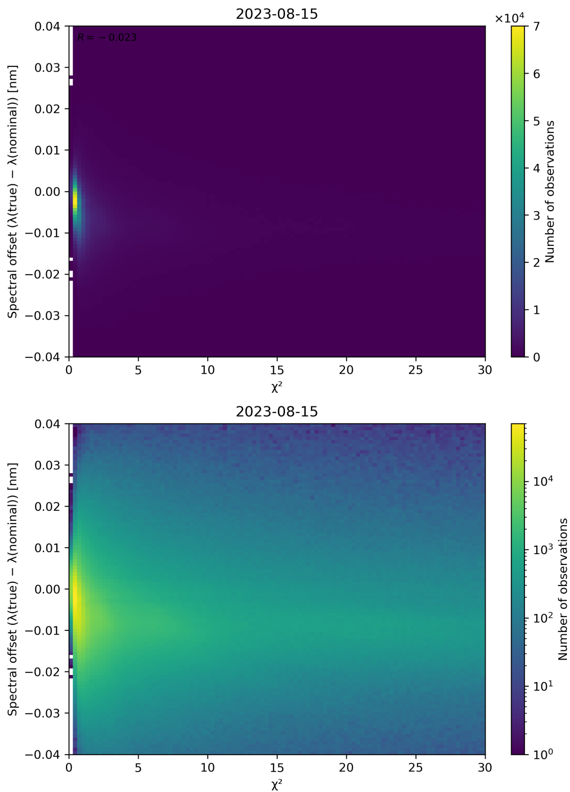
Figure 75: Scatter density plot of “ \chi^2 ” against “Spectral offset ( \lambda(\text{true}) - \lambda(\text{nominal}) )” for 2023-08-14 to 2023-08-16.
