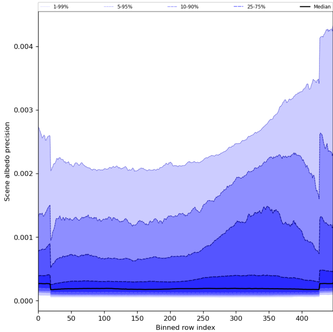
Figure 52: Along track statistics of “Scene albedo precision” for 2023-08-14 to 2023-08-16
