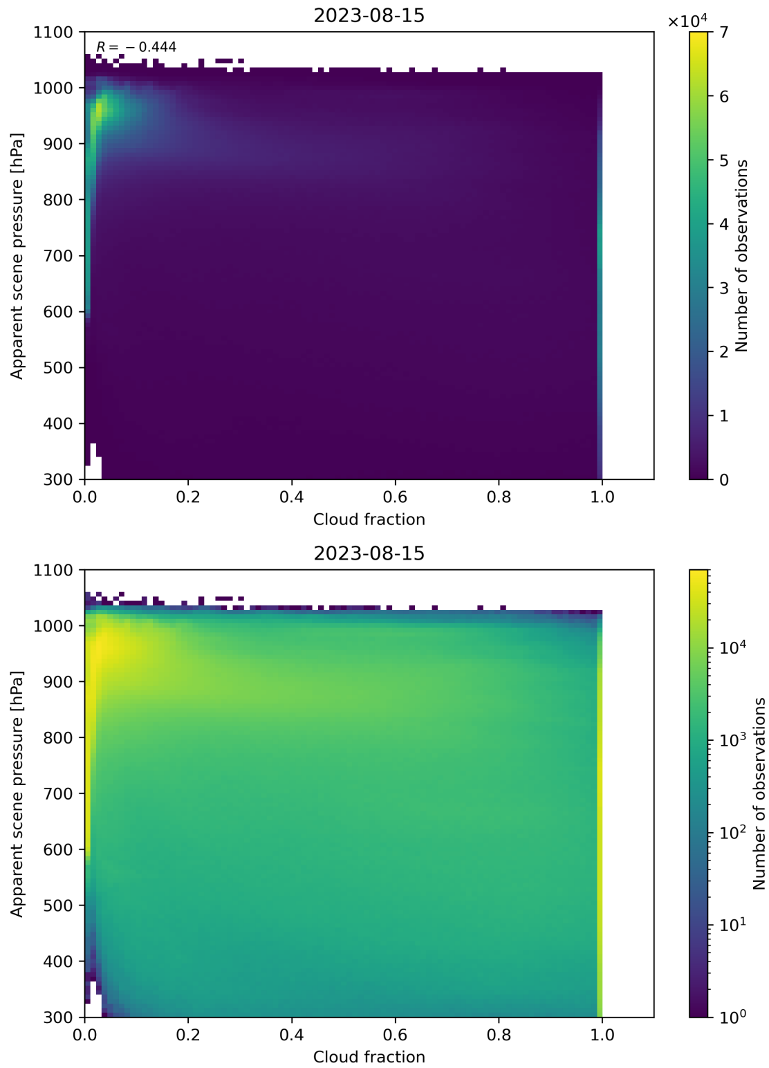
Figure 76: Scatter density plot of “Cloud fraction” against “Apparent scene pressure” for 2023-08-14 to 2023-08-16.
