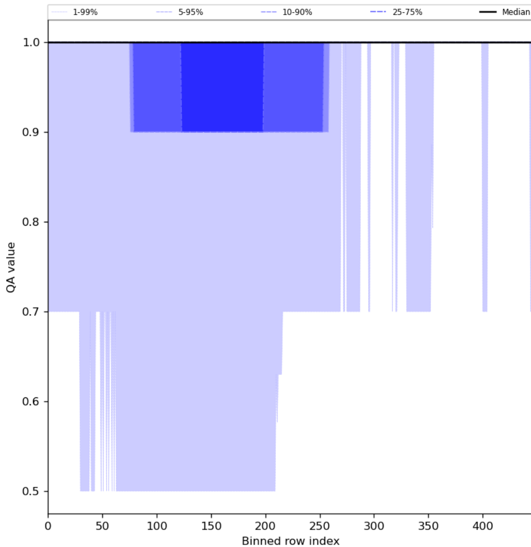
Figure 46: Along track statistics of “QA value” for 2023-08-14 to 2023-08-16
