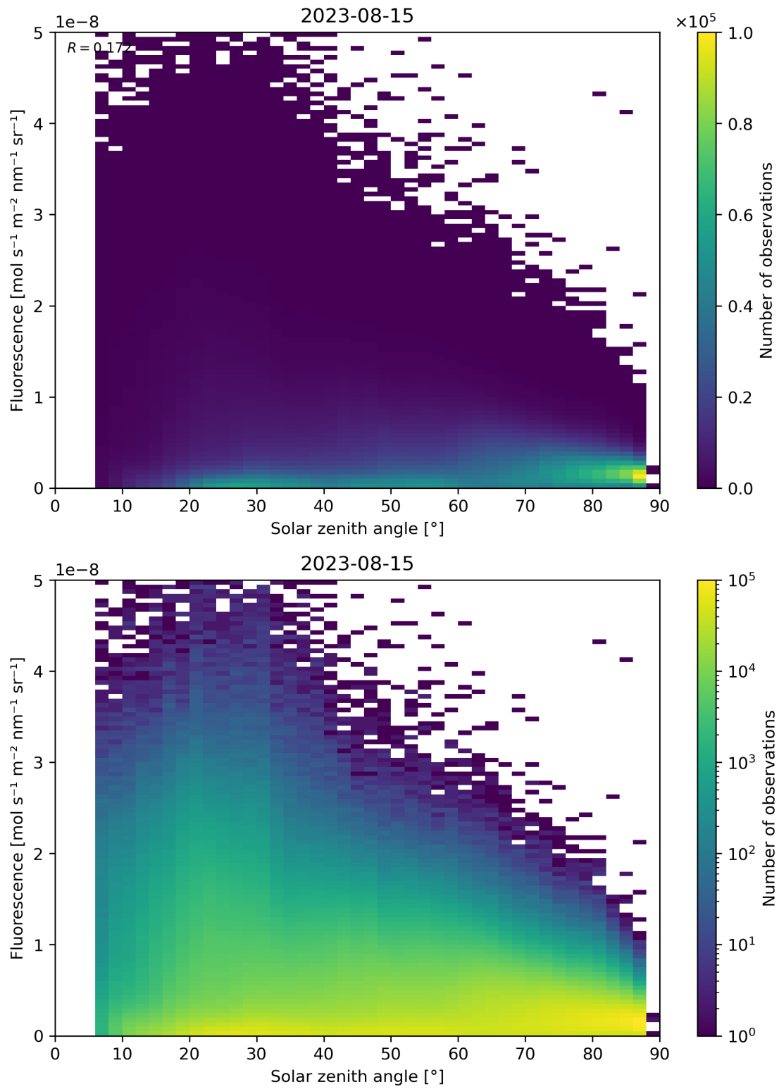
Figure 123: Scatter density plot of “Solar zenith angle” against “Fluorescence” for 2023-08-14 to 2023-08-16.
