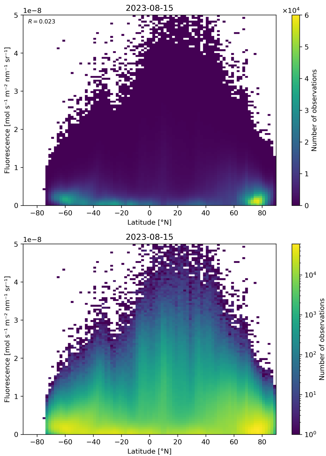
Figure 101: Scatter density plot of “Latitude” against “Fluorescence” for 2023-08-14 to 2023-08-16.
