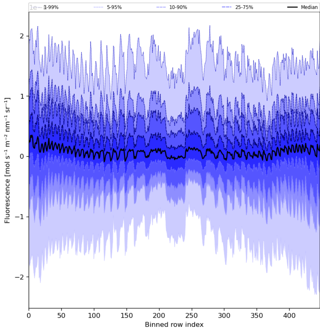
Figure 57: Along track statistics of “Fluorescence” for 2023-08-14 to 2023-08-16
