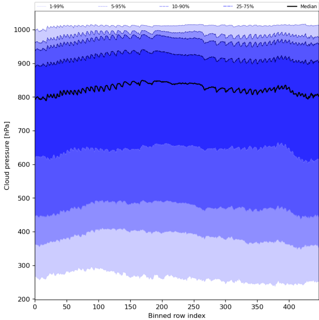
Figure 47: Along track statistics of “Cloud pressure” for 2023-08-14 to 2023-08-16
