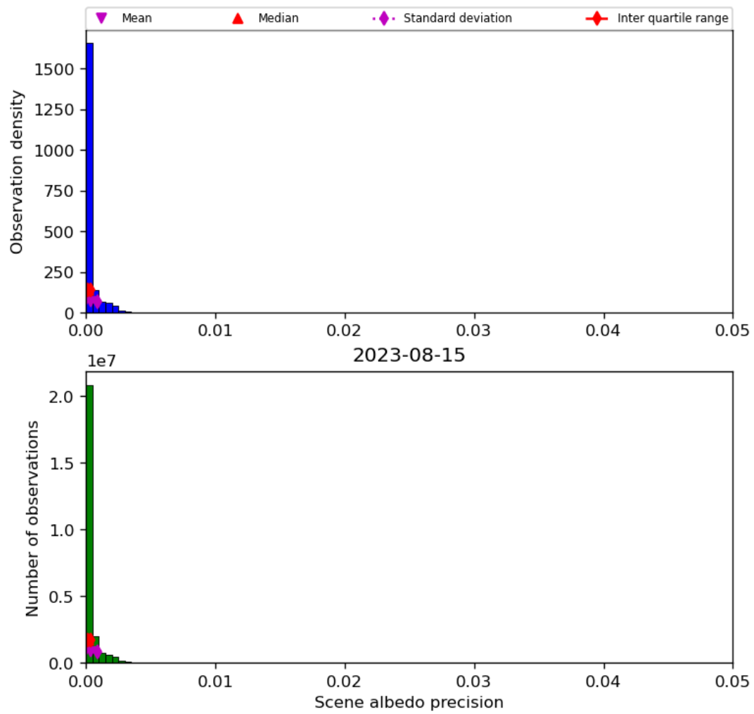
Figure 35: Histogram of “Scene albedo precision” for 2023-08-14 to 2023-08-16
