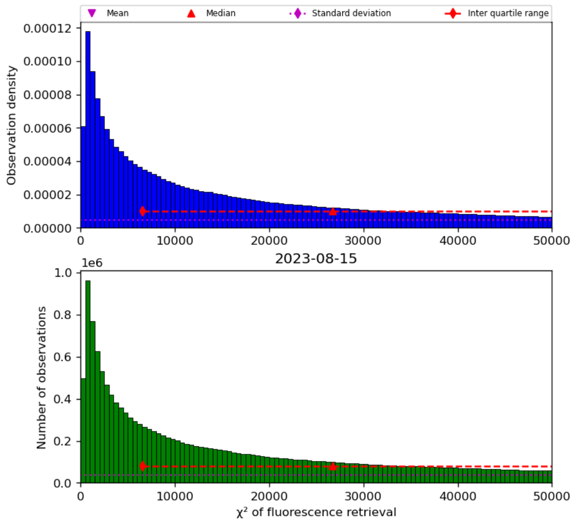
Figure 42: Histogram of “ \chi^2 of fluorescence retrieval” for 2023-08-14 to 2023-08-16
