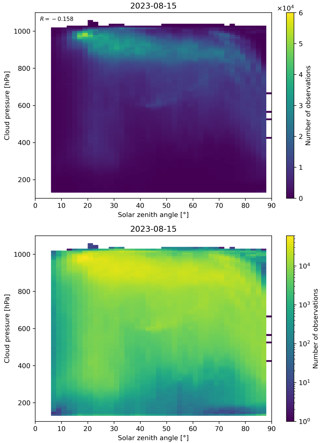
Figure 122: Scatter density plot of “Solar zenith angle” against “Cloud pressure” for 2023-08-14 to 2023-08-16.
