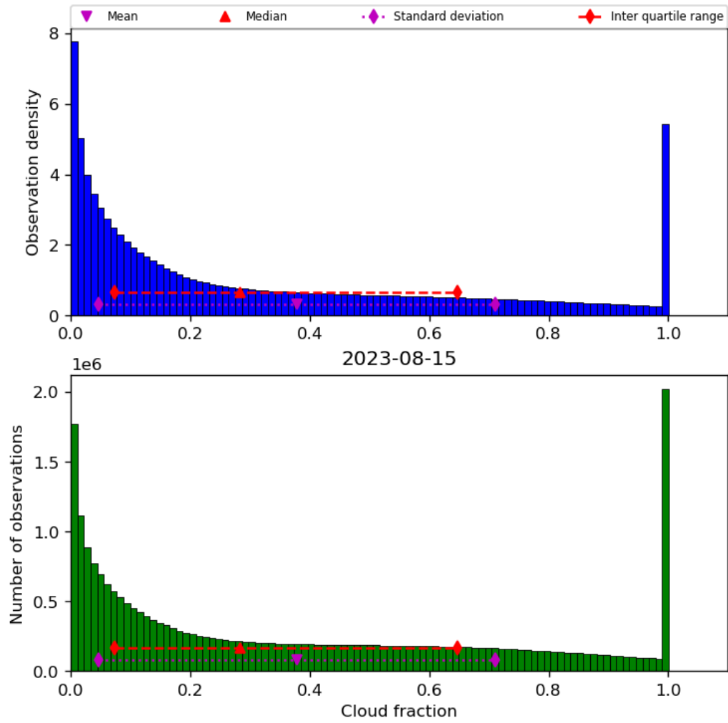
Figure 32: Histogram of “Cloud fraction” for 2023-08-14 to 2023-08-16
