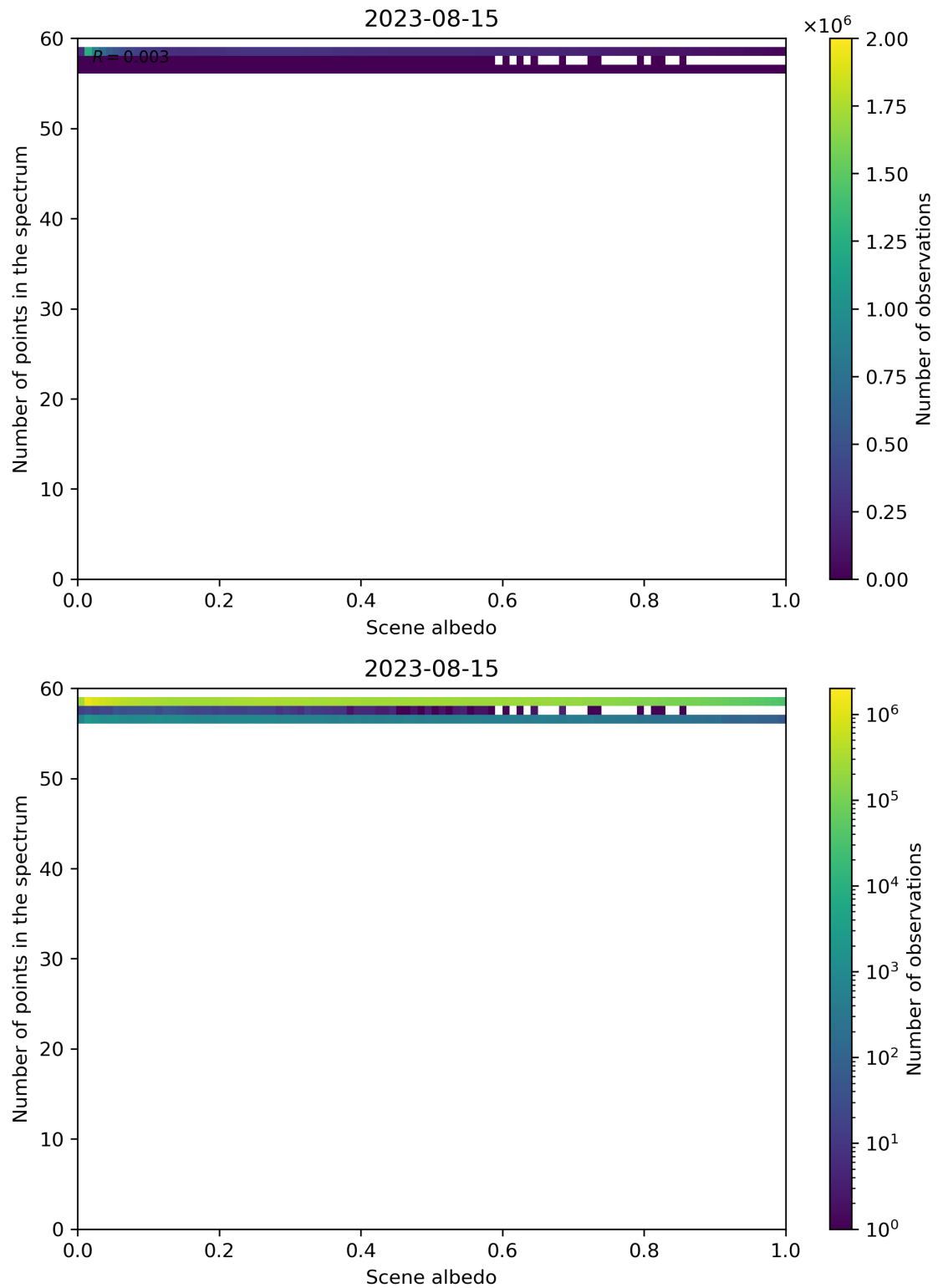
Figure 116: Scatter density plot of “Scene albedo” against “Number of points in the spectrum” for 2023-08-14 to 2023-08-16.
