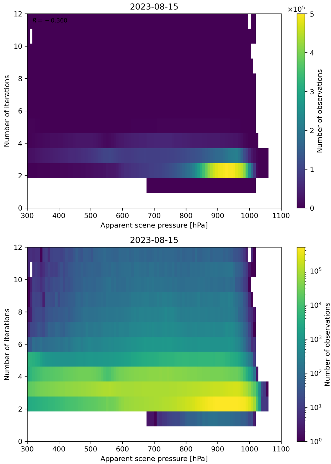
Figure 66: Scatter density plot of “Apparent scene pressure” against “Number of iterations” for 2023-08-14 to 2023-08-16.
