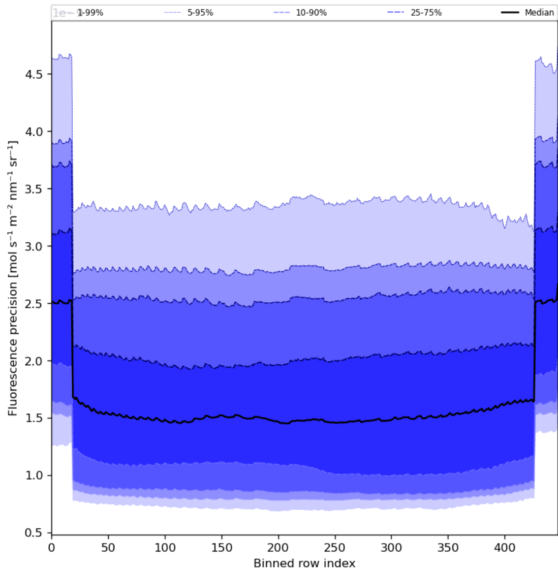
Figure 58: Along track statistics of “Fluorescence precision” for 2023-08-14 to 2023-08-16
