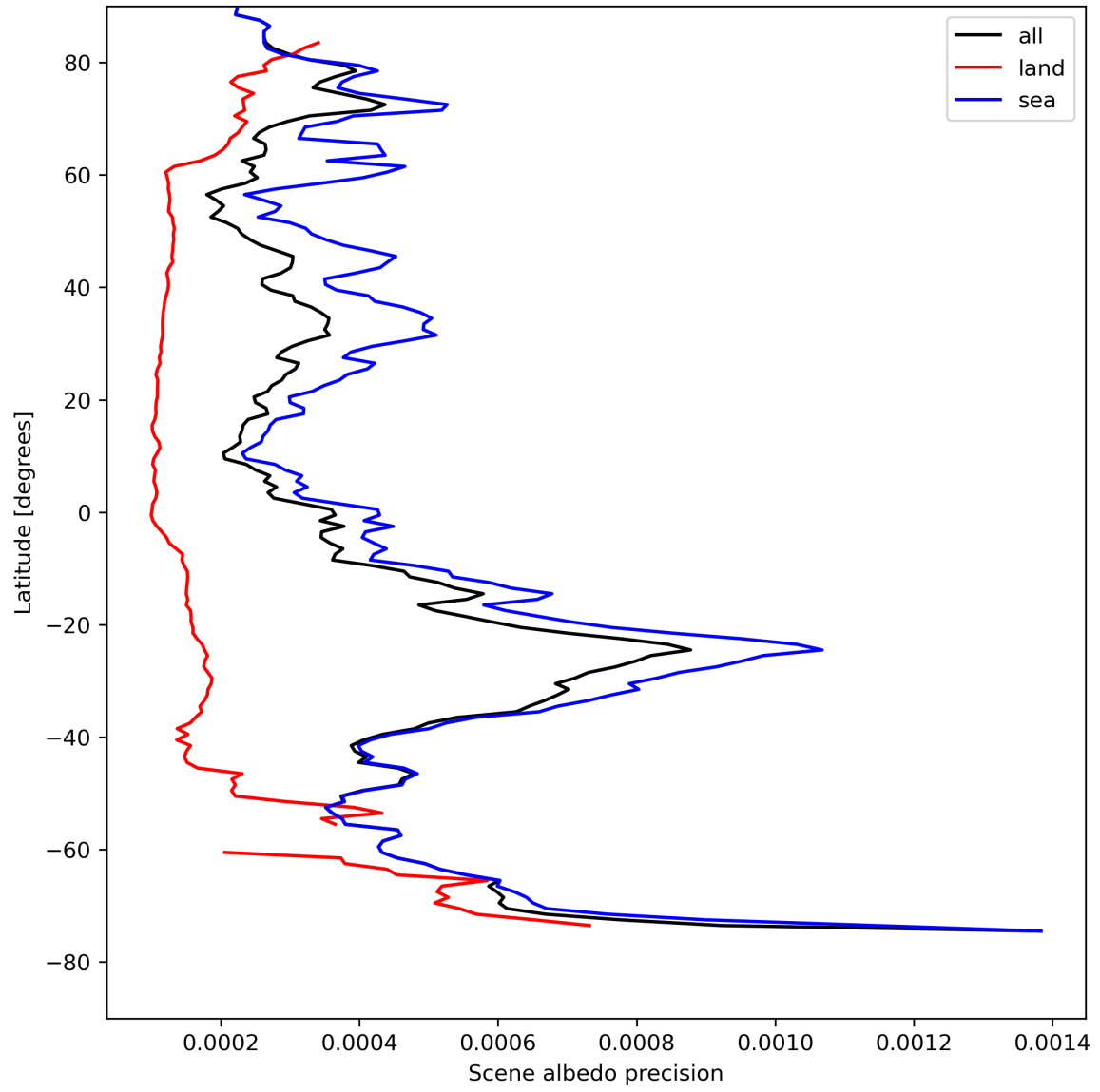
Figure 18: Zonal average of “Scene albedo precision” for 2023-08-14 to 2023-08-16.
