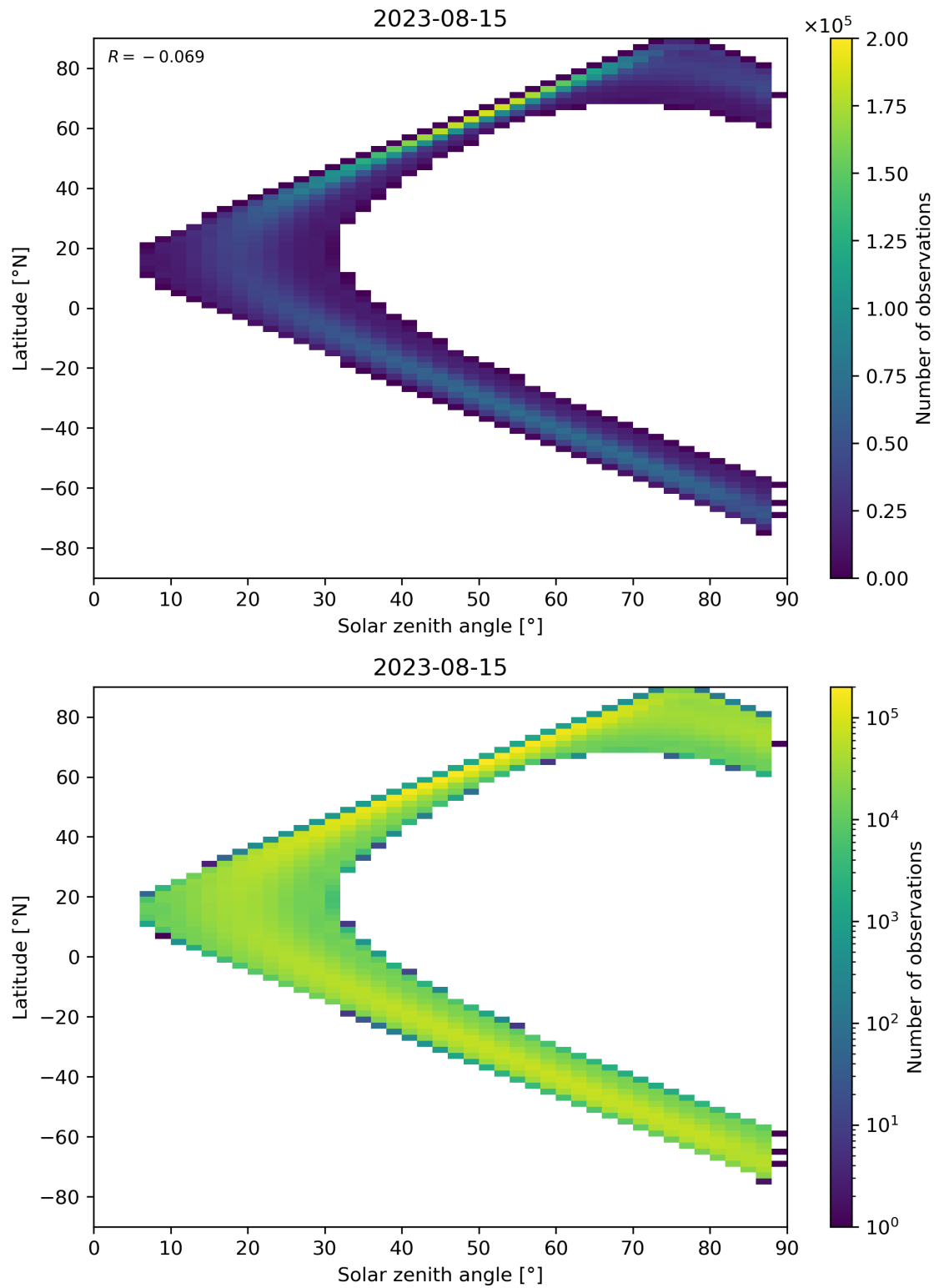
Figure 124: Scatter density plot of “Solar zenith angle” against “Latitude” for 2023-08-14 to 2023-08-16.
