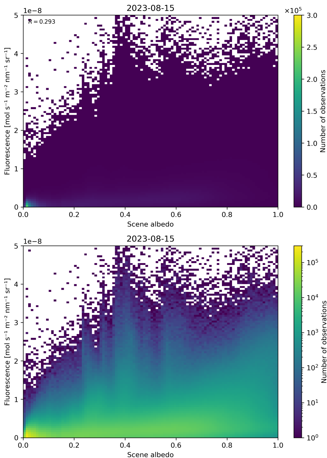
Figure 114: Scatter density plot of “Scene albedo” against “Fluorescence” for 2023-08-14 to 2023-08-16.
