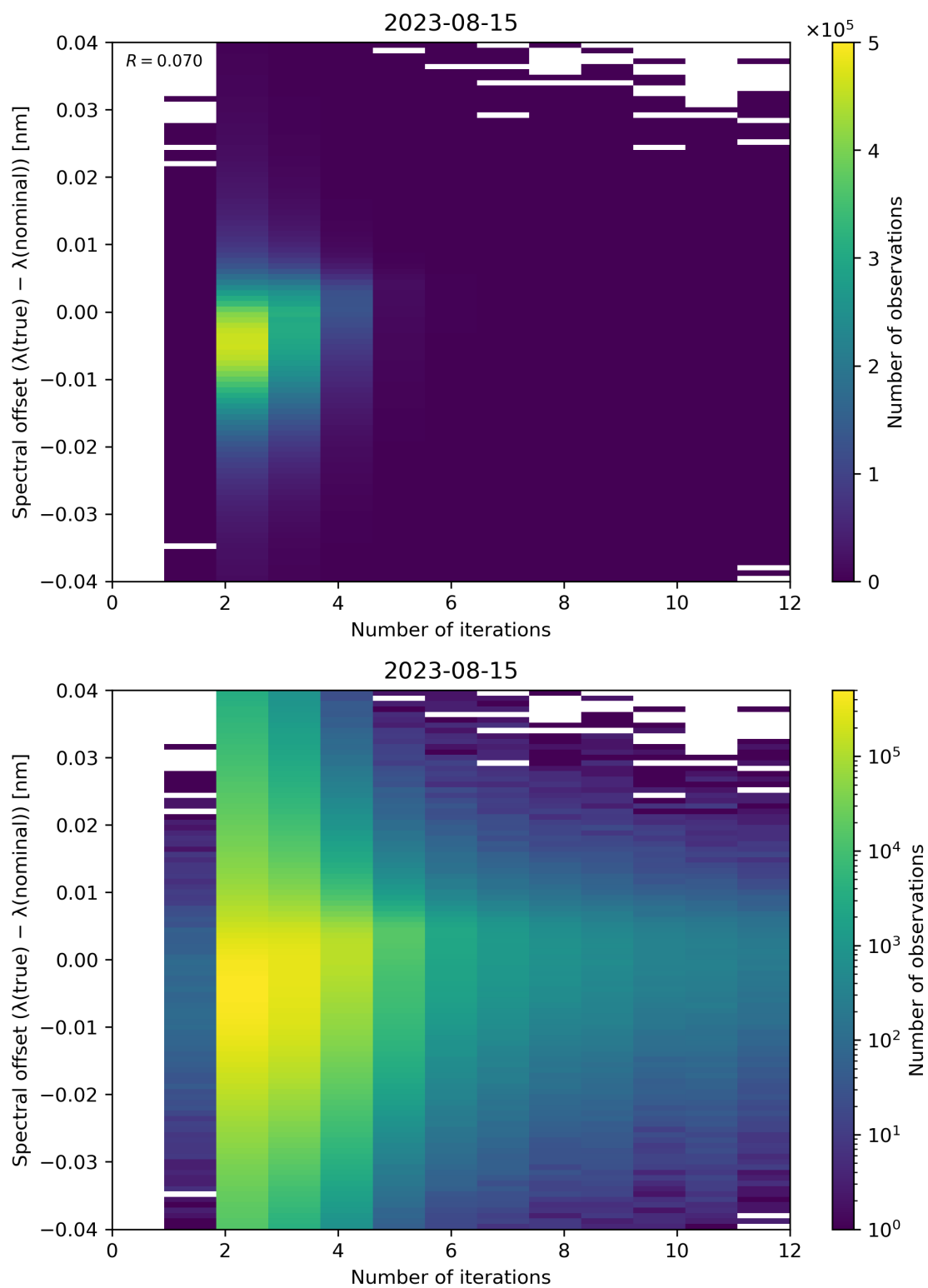
Figure 109: Scatter density plot of “Number of iterations” against “Spectral offset ( \lambda(\text{true}) - \lambda(\text{nominal}) )” for 2023-08-14 to 2023-08-16.
