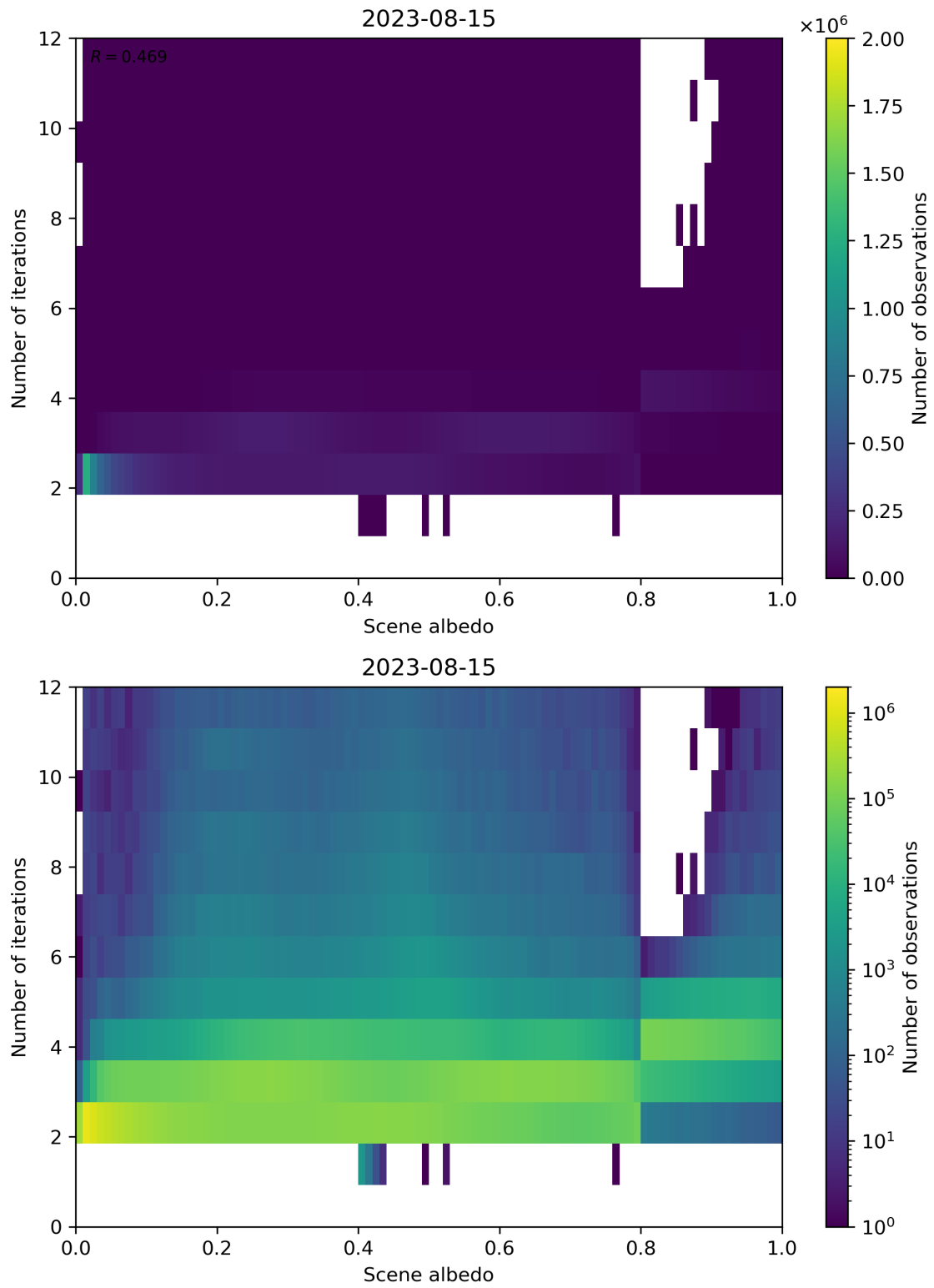
Figure 115: Scatter density plot of “Scene albedo” against “Number of iterations” for 2023-08-14 to 2023-08-16.
