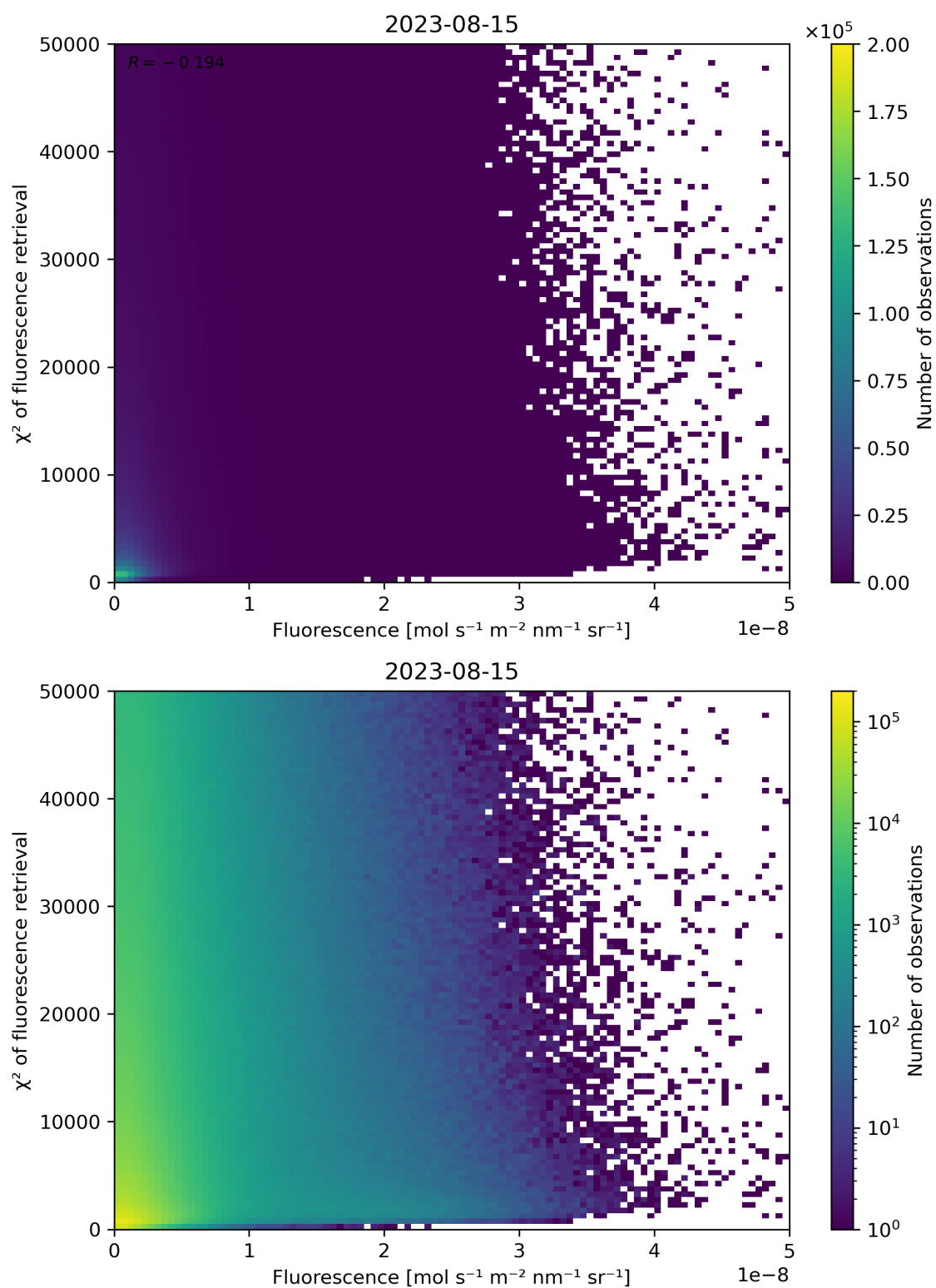
Figure 93: Scatter density plot of “Fluorescence” against “ \chi^2 of fluorescence retrieval” for 2023-08-14 to 2023-08-16.
