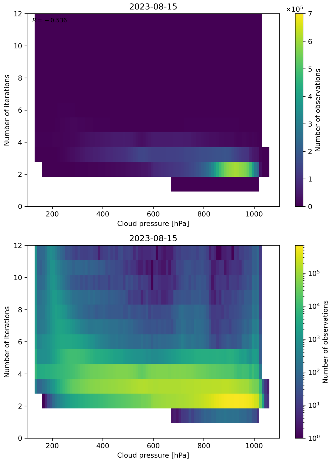
Figure 89: Scatter density plot of “Cloud pressure” against “Number of iterations” for 2023-08-14 to 2023-08-16.
