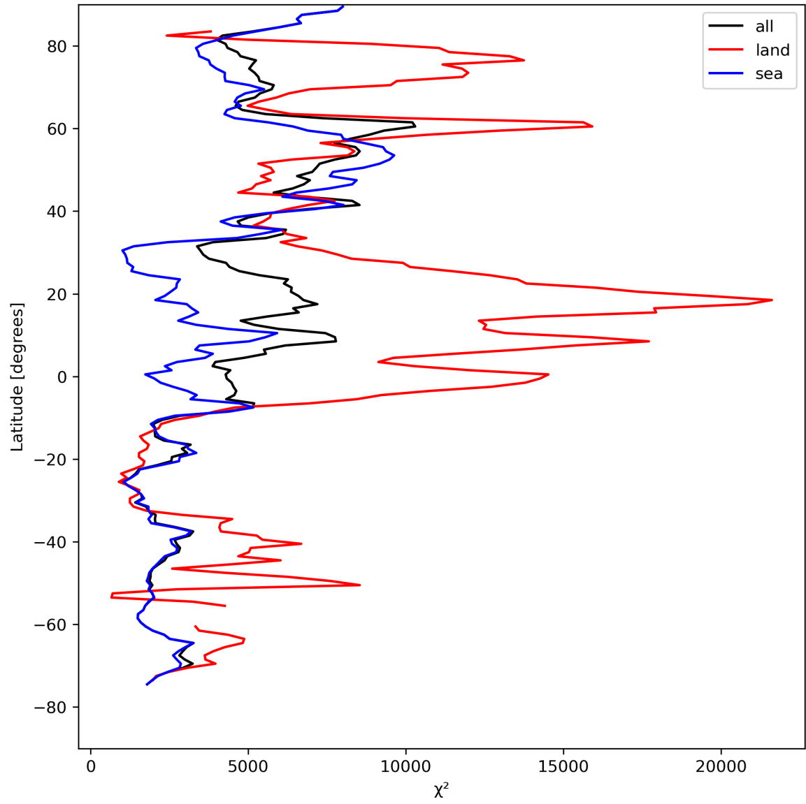
Figure 21: Zonal average of “ \chi^2 ” for 2023-08-14 to 2023-08-16.
