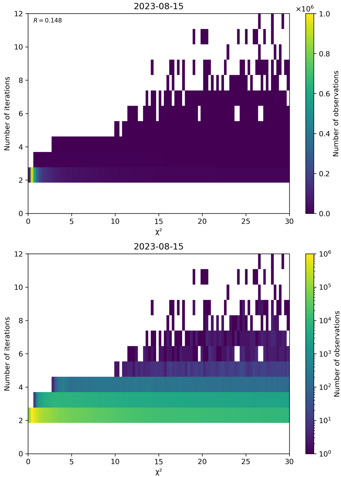
Figure 73: Scatter density plot of “ \chi^2 ” against “Number of iterations” for 2023-08-14 to 2023-08-16.
