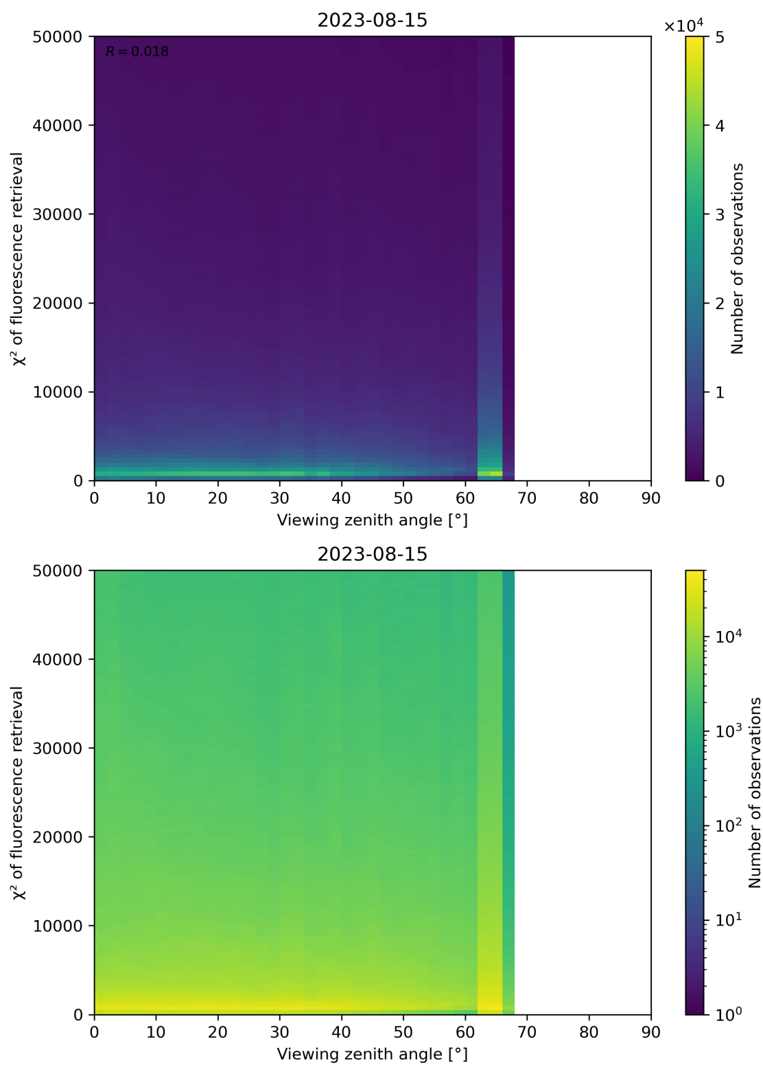
Figure 131: Scatter density plot of “Viewing zenith angle” against “ \chi^2 of fluorescence retrieval” for 2023-08-14 to 2023-08-16.
