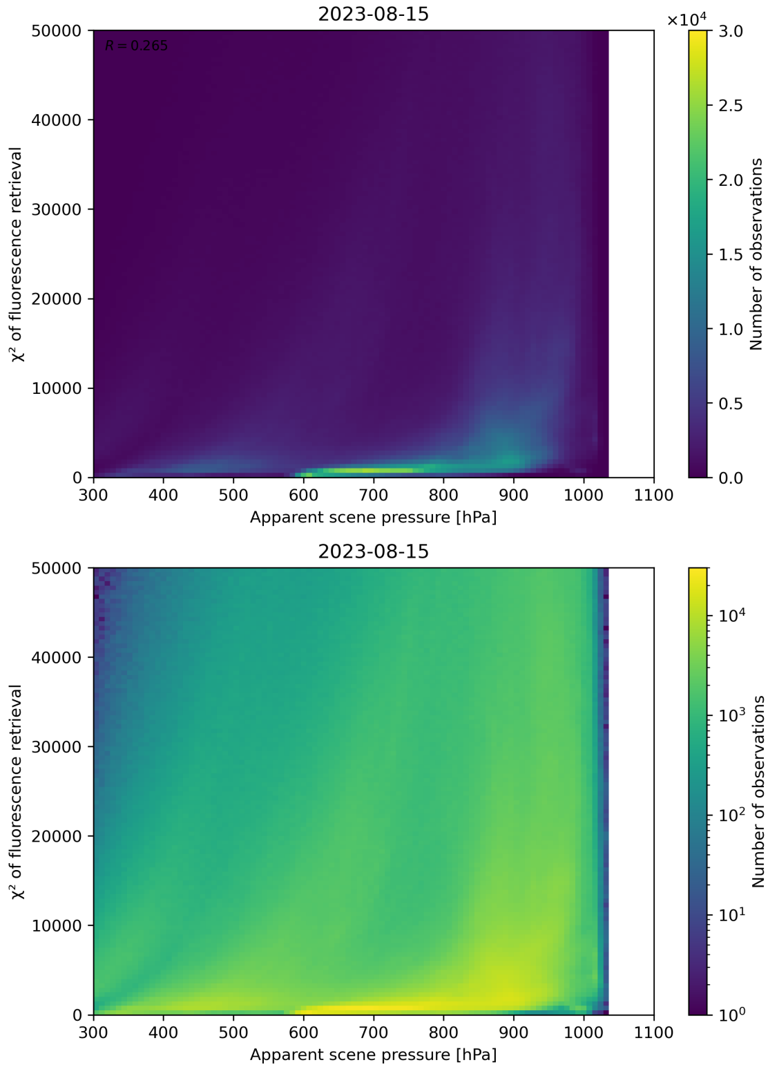
Figure 64: Scatter density plot of “Apparent scene pressure” against “ \chi^2 of fluorescence retrieval” for 2023-08-14 to 2023-08-16.
