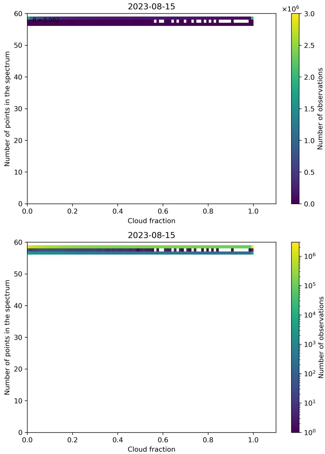
Figure 81: Scatter density plot of “Cloud fraction” against “Number of points in the spectrum” for 2023-08-14 to 2023-08-16.
