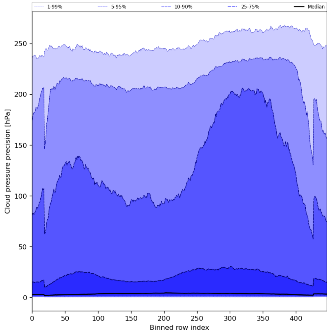
Figure 48: Along track statistics of “Cloud pressure precision” for 2023-08-14 to 2023-08-16
