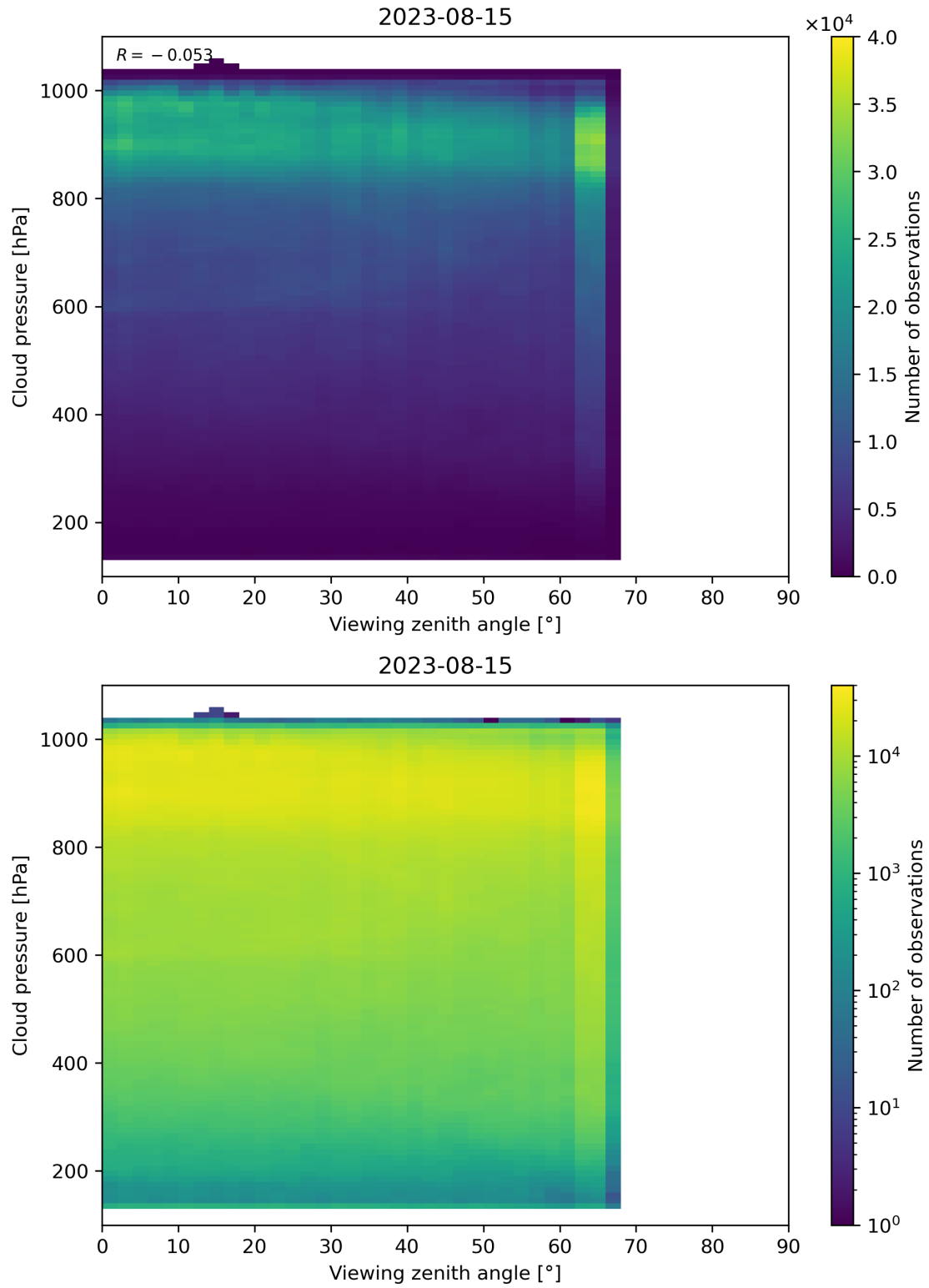
Figure 133: Scatter density plot of “Viewing zenith angle” against “Cloud pressure” for 2023-08-14 to 2023-08-16.
