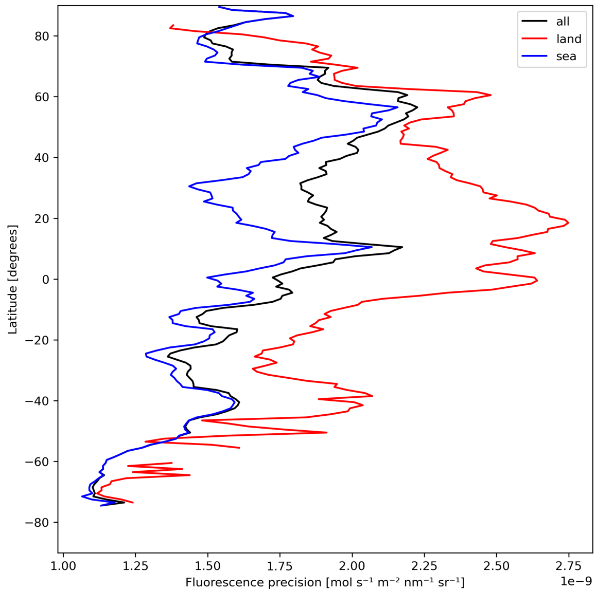
Figure 24: Zonal average of “Fluorescence precision” for 2023-08-14 to 2023-08-16.
