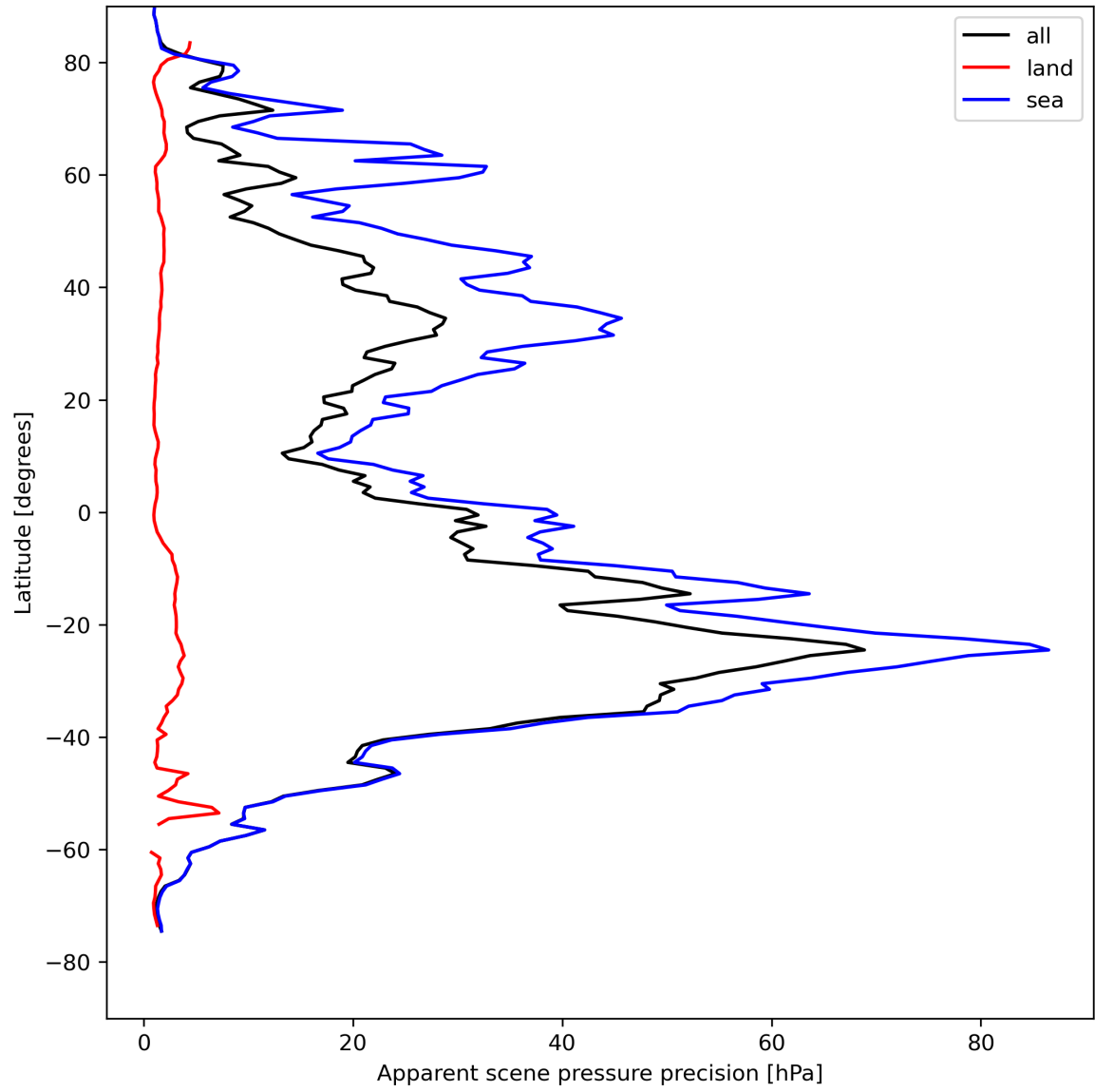
Figure 20: Zonal average of “Apparent scene pressure precision” for 2023-08-14 to 2023-08-16.
