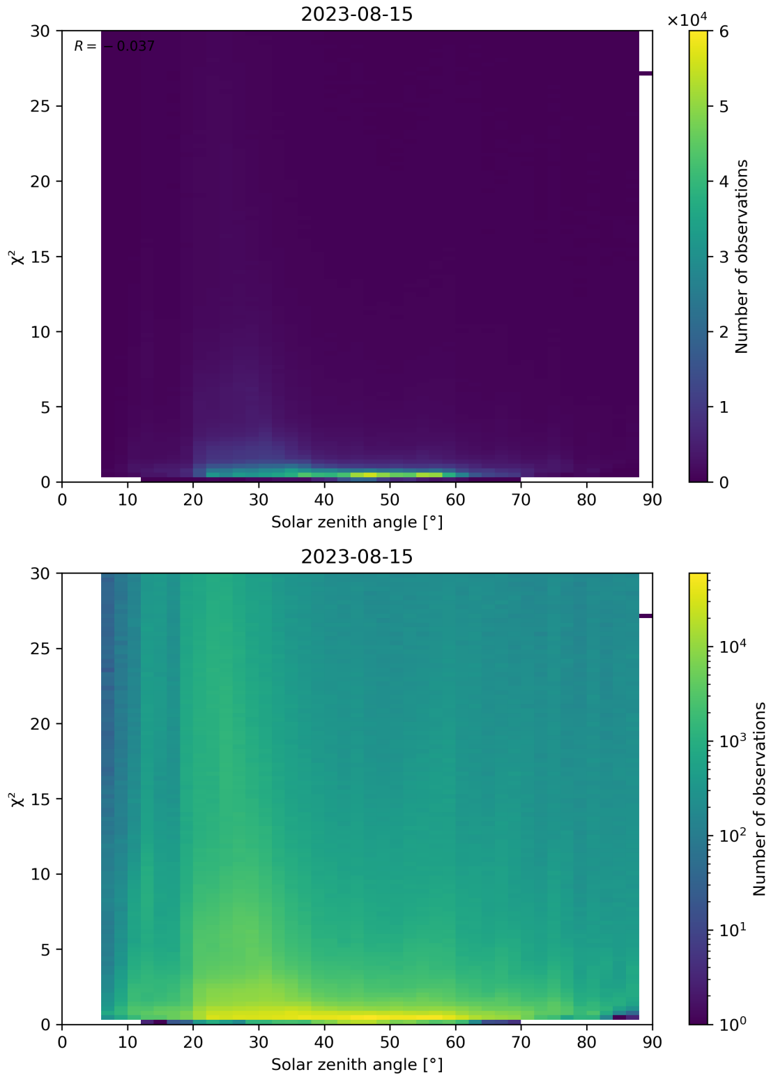
Figure 119: Scatter density plot of “Solar zenith angle” against “ \chi^2 ” for 2023-08-14 to 2023-08-16.
