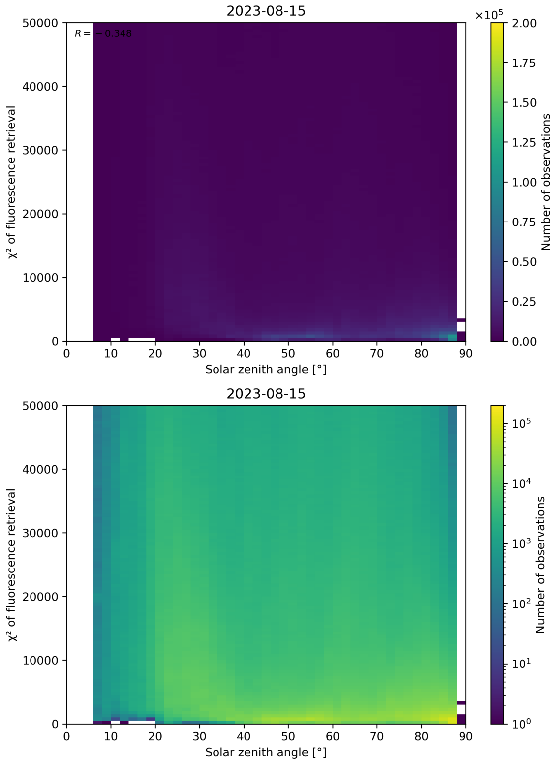
Figure 120: Scatter density plot of “Solar zenith angle” against “ \chi^2 of fluorescence retrieval” for 2023-08-14 to 2023-08-16.
