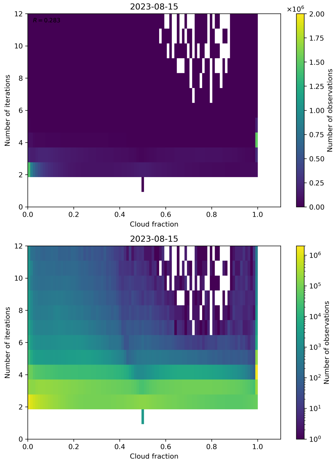
Figure 80: Scatter density plot of “Cloud fraction” against “Number of iterations” for 2023-08-14 to 2023-08-16.
