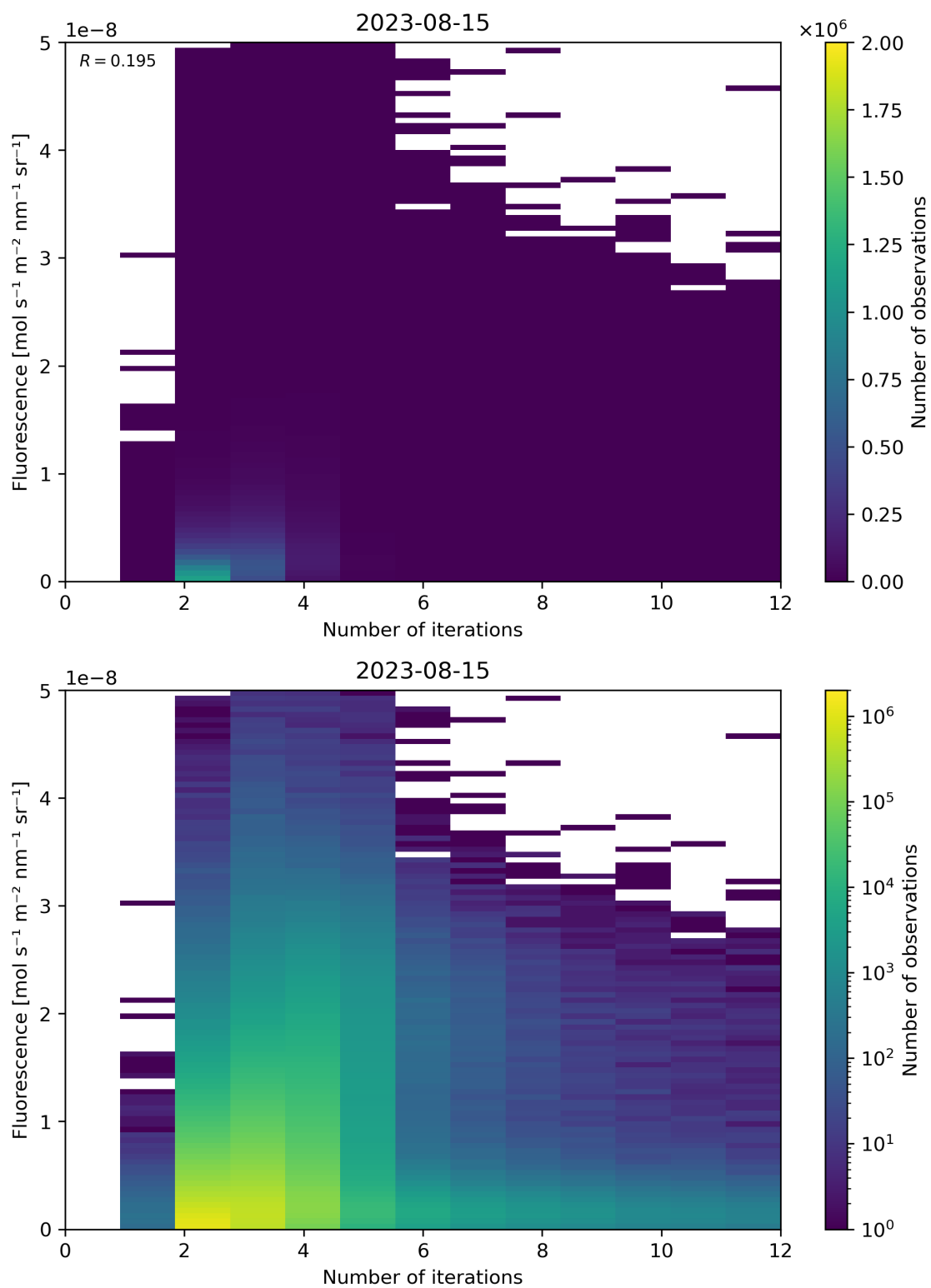
Figure 107: Scatter density plot of “Number of iterations” against “Fluorescence” for 2023-08-14 to 2023-08-16.
