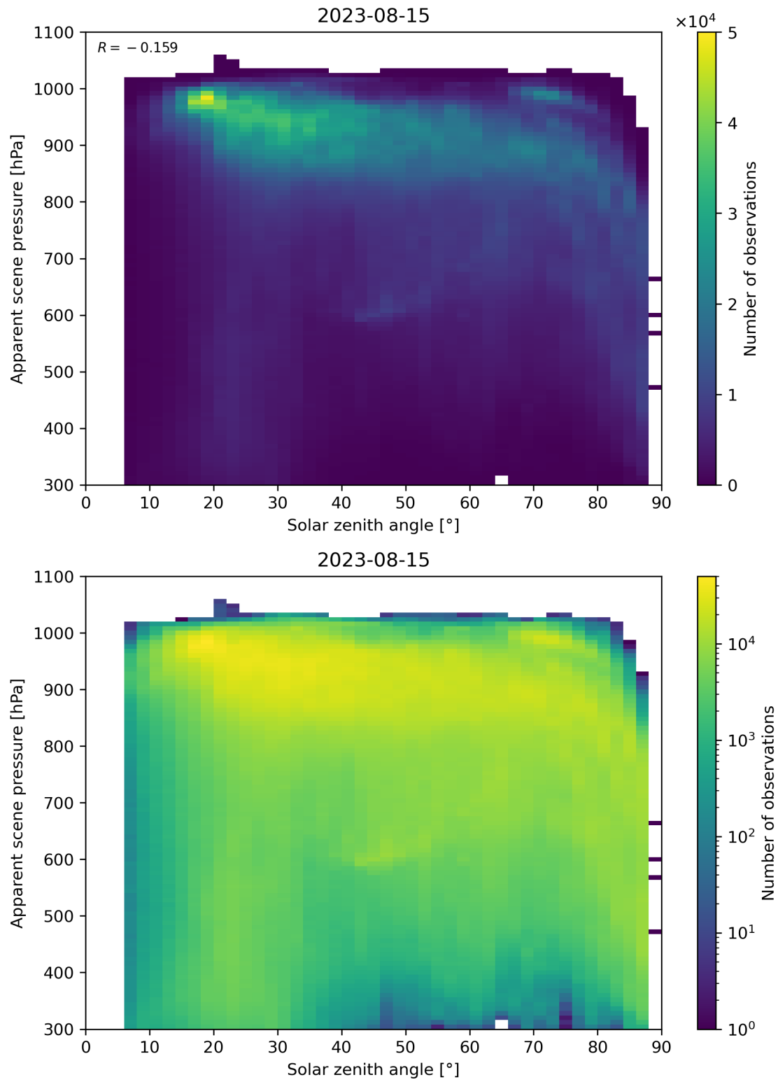
Figure 118: Scatter density plot of “Solar zenith angle” against “Apparent scene pressure” for 2023-08-14 to 2023-08-16.
