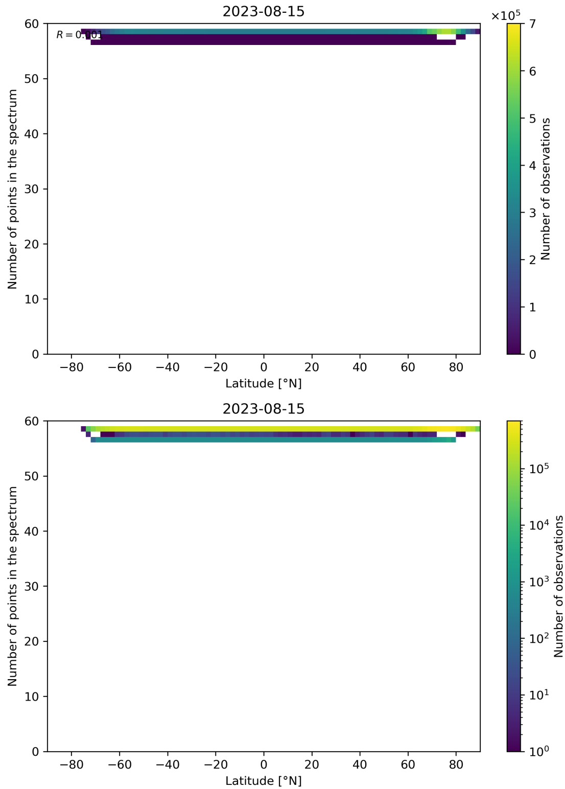
Figure 103: Scatter density plot of “Latitude” against “Number of points in the spectrum” for 2023-08-14 to 2023-08-16.
