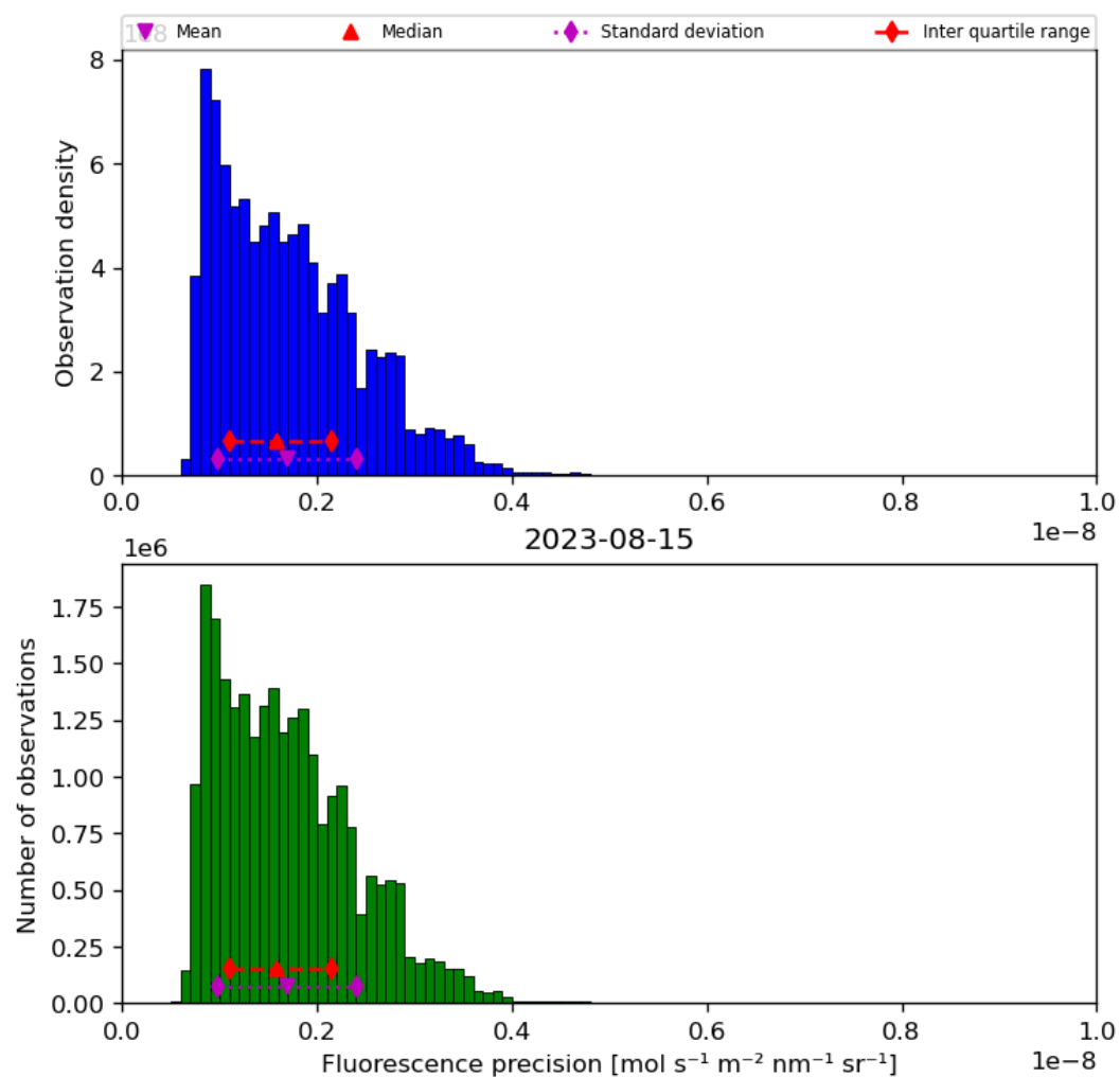
Figure 41: Histogram of “Fluorescence precision” for 2023-08-14 to 2023-08-16
