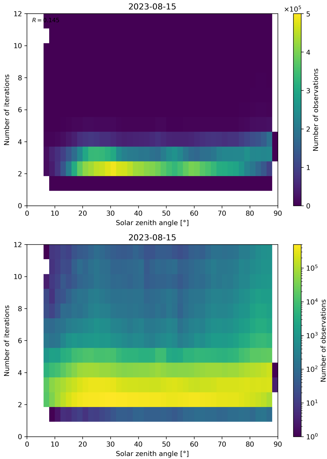
Figure 125: Scatter density plot of “Solar zenith angle” against “Number of iterations” for 2023-08-14 to 2023-08-16.
