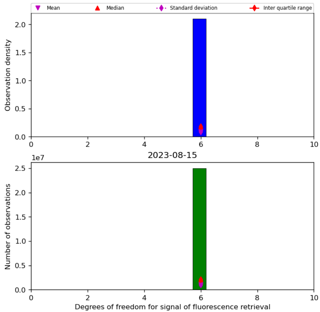
Figure 43: Histogram of “Degrees of freedom for signal of fluorescence retrieval” for 2023-08-14 to 2023-08-16
