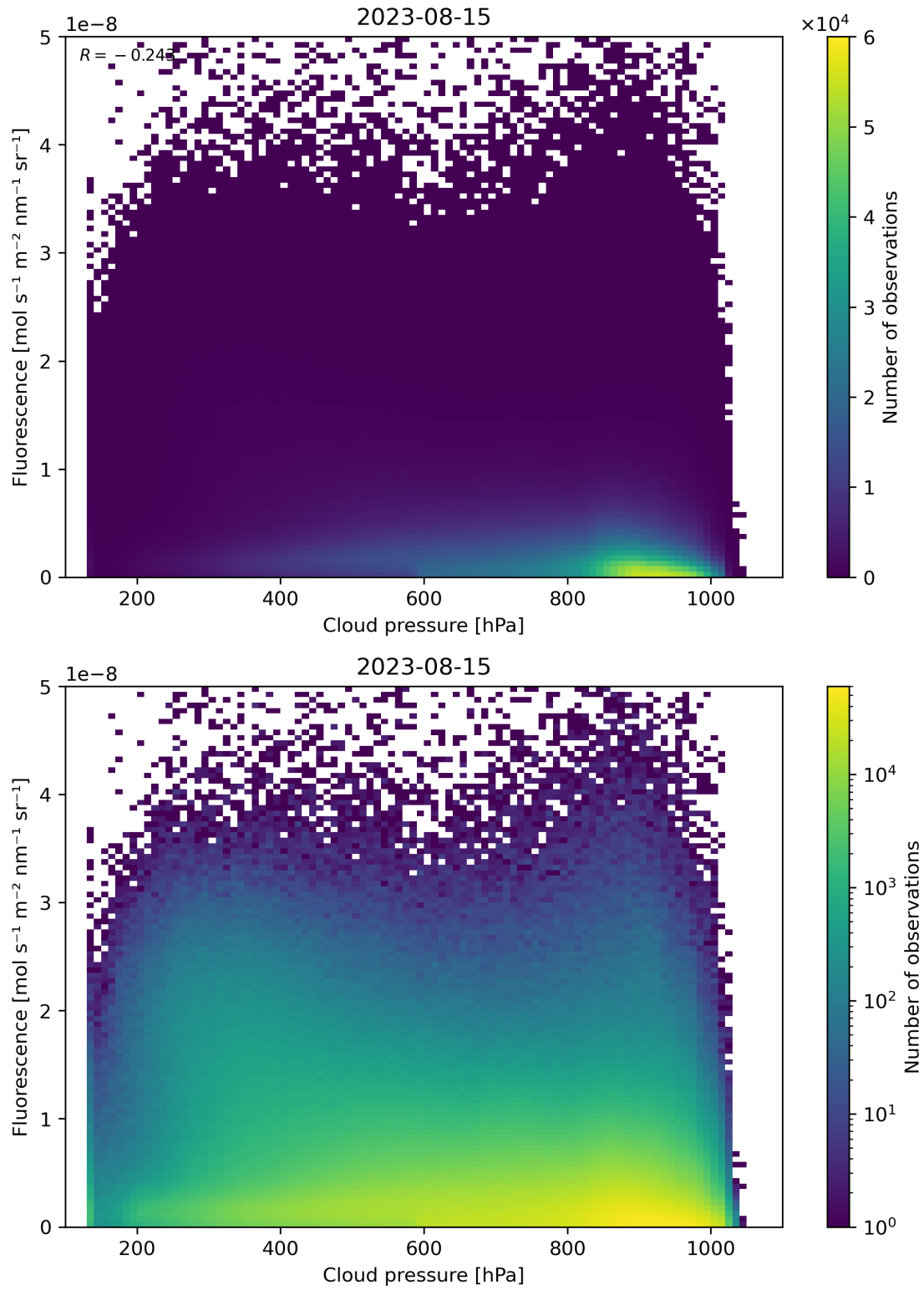
Figure 88: Scatter density plot of “Cloud pressure” against “Fluorescence” for 2023-08-14 to 2023-08-16.
