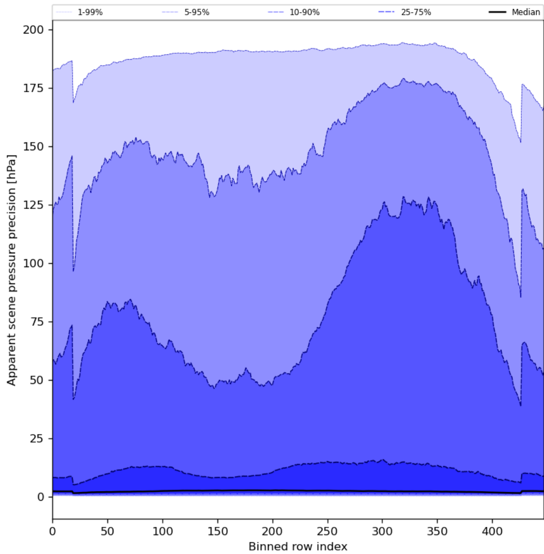
Figure 54: Along track statistics of “Apparent scene pressure precision” for 2023-08-14 to 2023-08-16
