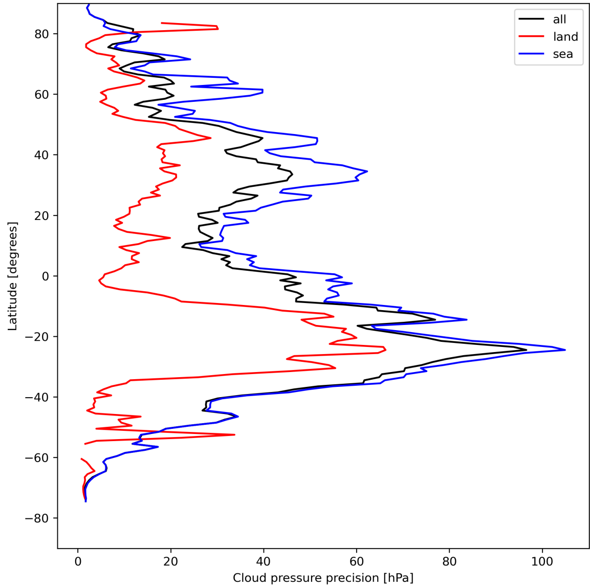
Figure 14: Zonal average of “Cloud pressure precision” for 2023-08-14 to 2023-08-16.
