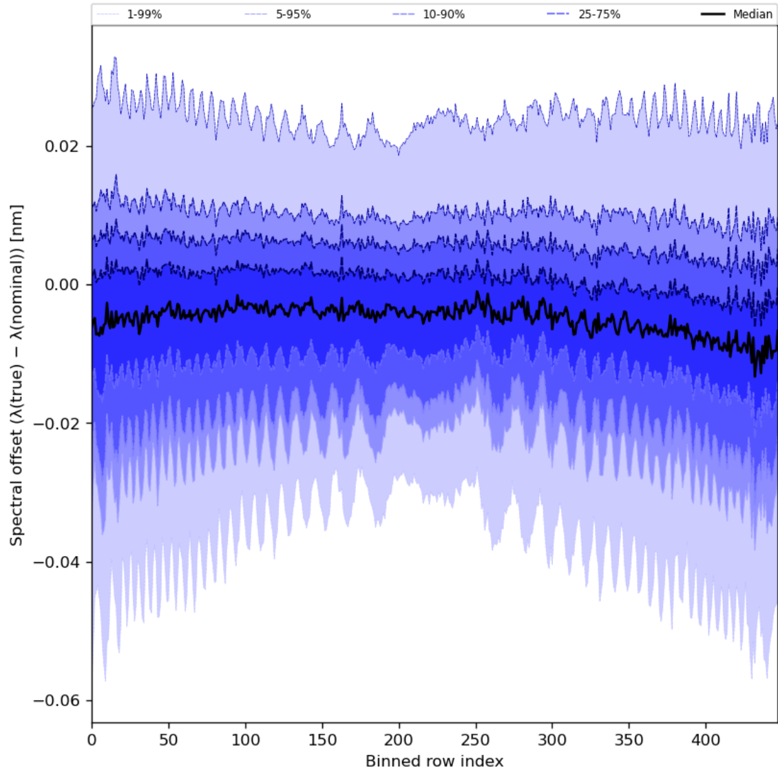
Figure 62: Along track statistics of “Spectral offset ( \lambda(\text{true}) - \lambda(\text{nominal}) )” for 2023-08-14 to 2023-08-16
