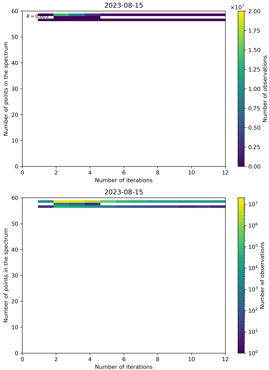
Figure 108: Scatter density plot of “Number of iterations” against “Number of points in the spectrum” for 2023-08-14 to 2023-08-16.
