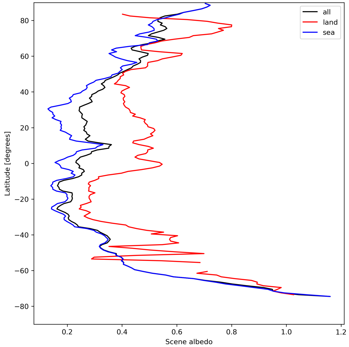
Figure 17: Zonal average of “Scene albedo” for 2023-08-14 to 2023-08-16.
