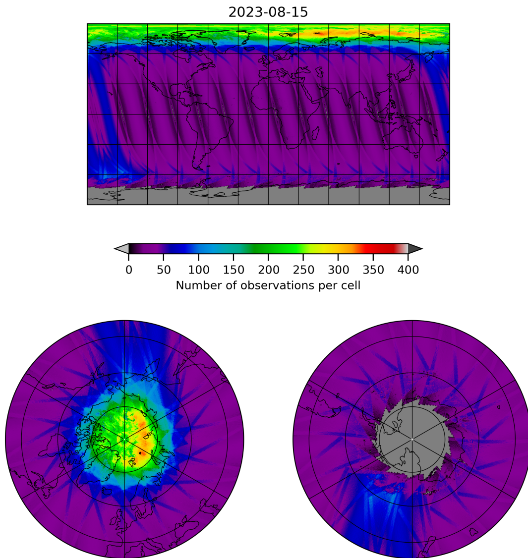
Figure 11: Map of the number of observations for 2023-08-14 to 2023-08-16
