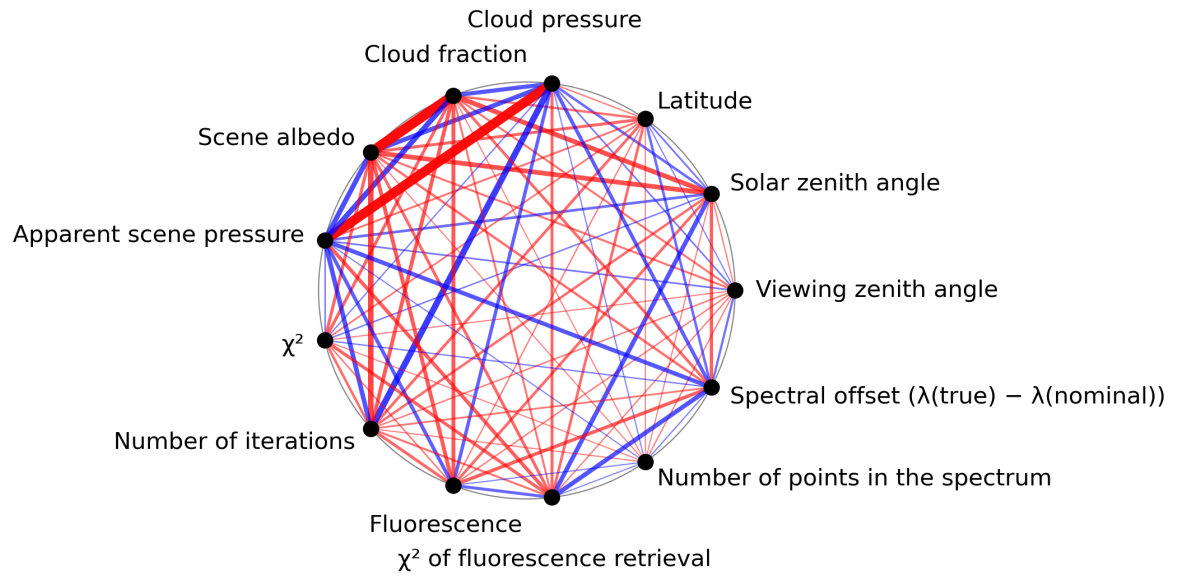
Figure 1: Map of correlation graph for 2023-08-14 to 2023-08-16.
