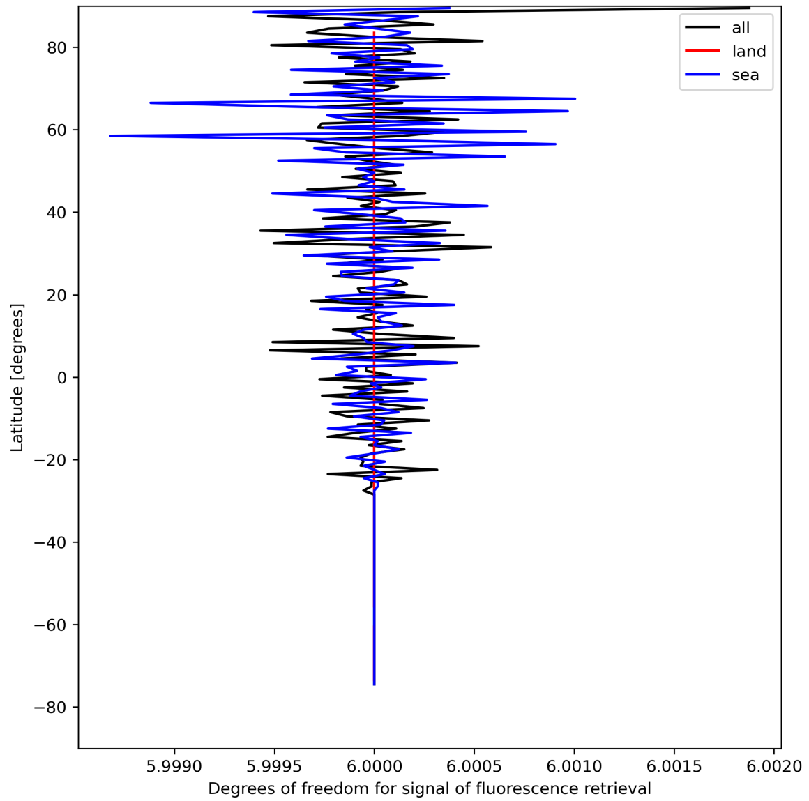
Figure 26: Zonal average of “Degrees of freedom for signal of fluorescence retrieval” for 2023-08-14 to 2023-08-16.
