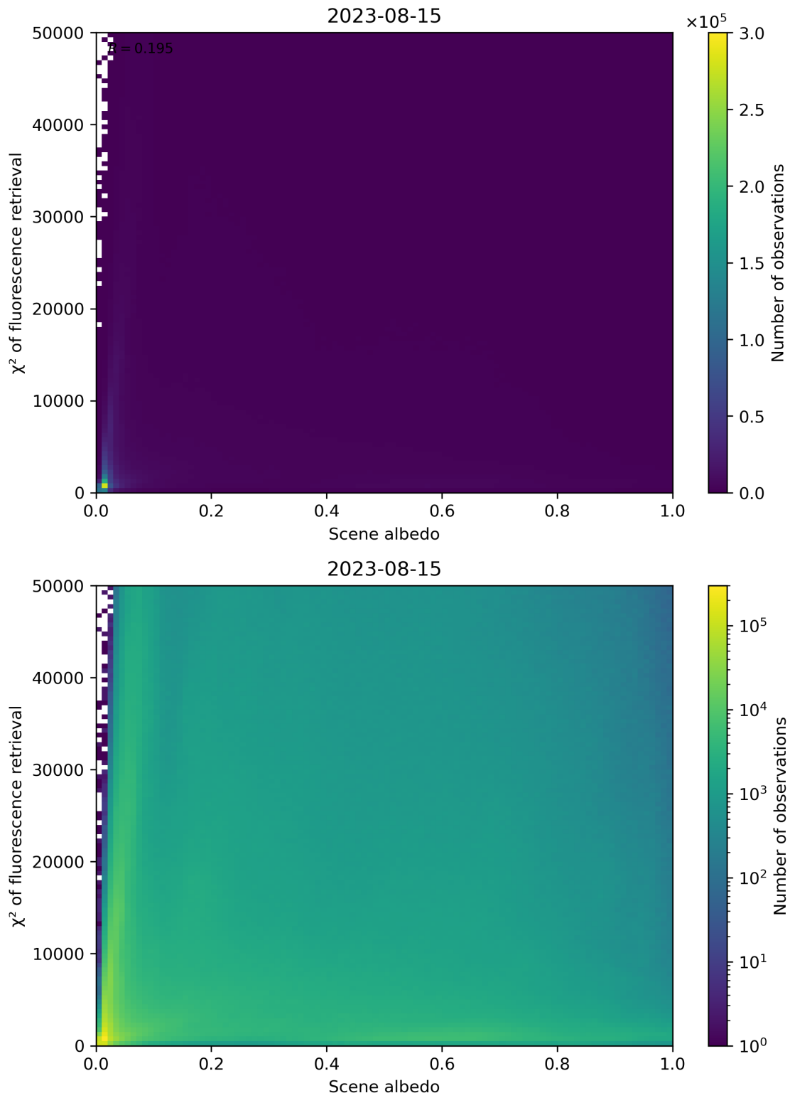
Figure 113: Scatter density plot of “Scene albedo” against “ \chi^2 of fluorescence retrieval” for 2023-08-14 to 2023-08-16.
