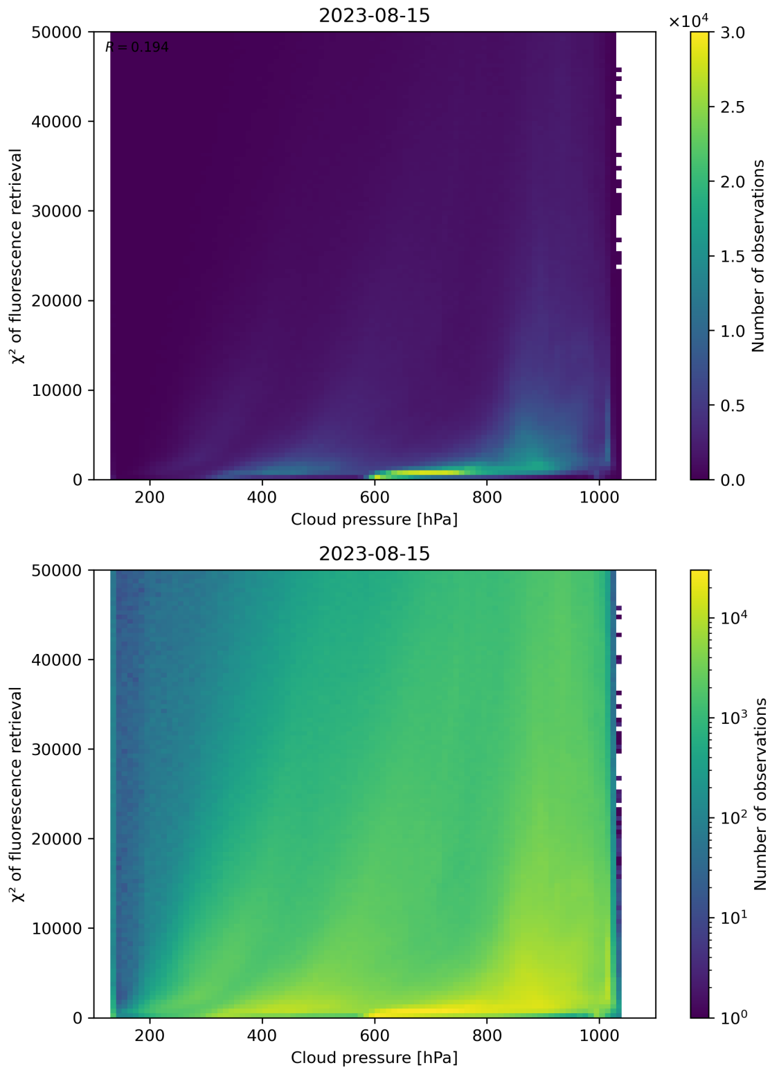
Figure 86: Scatter density plot of “Cloud pressure” against “ \chi^2 of fluorescence retrieval” for 2023-08-14 to 2023-08-16.
