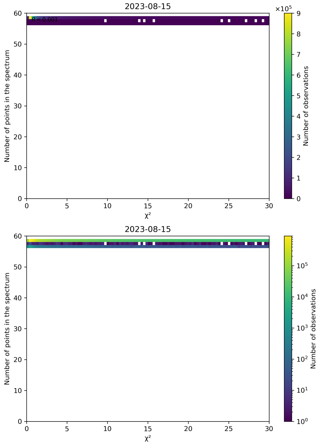
Figure 74: Scatter density plot of “ \chi^2 ” against “Number of points in the spectrum” for 2023-08-14 to 2023-08-16.
