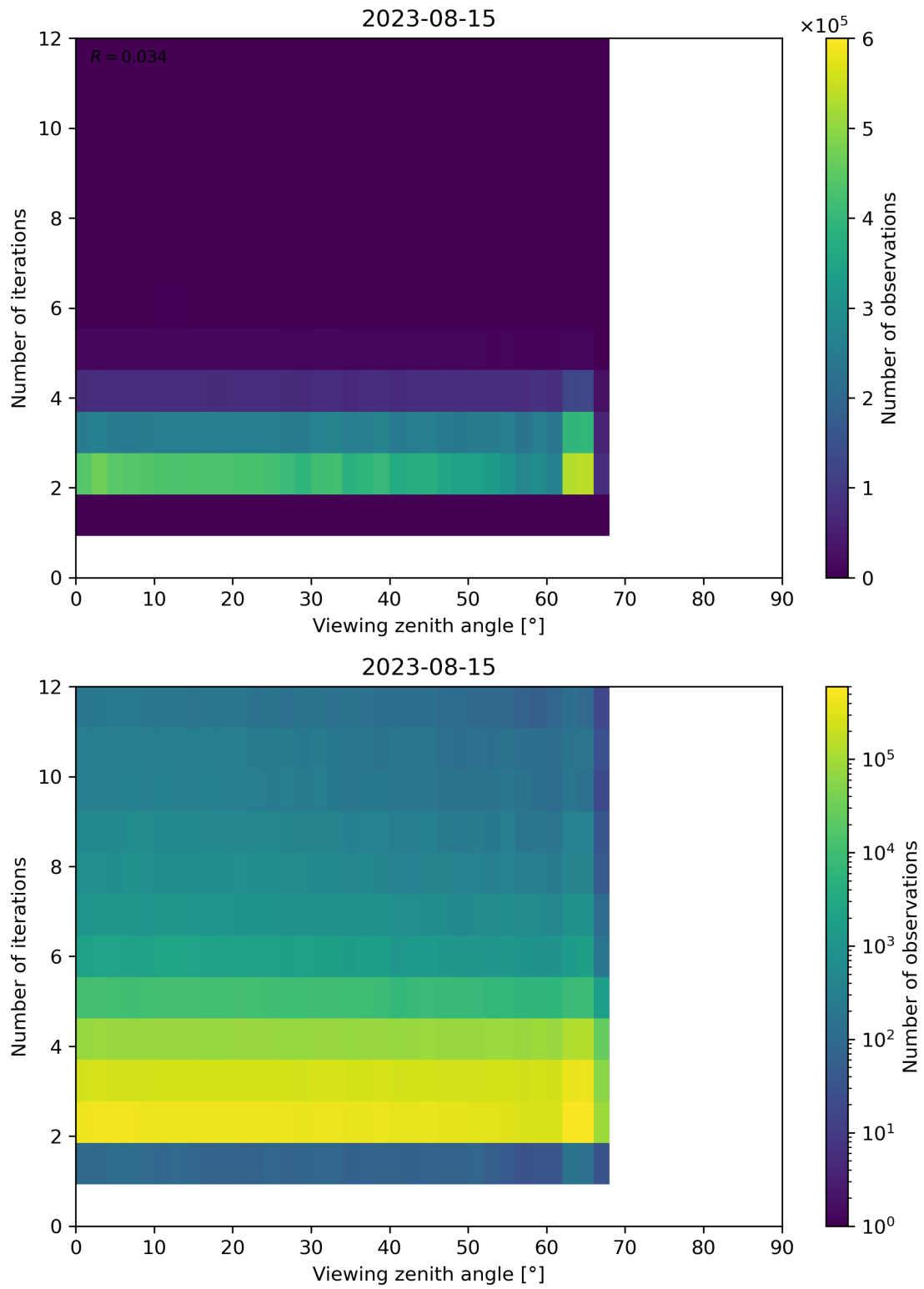
Figure 136: Scatter density plot of “Viewing zenith angle” against “Number of iterations” for 2023-08-14 to 2023-08-16.
