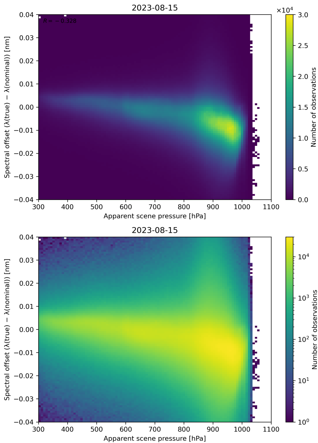
Figure 68: Scatter density plot of “Apparent scene pressure” against “Spectral offset ( \lambda(\text{true}) - \lambda(\text{nominal}) )” for 2023-08-14 to 2023-08-16.
