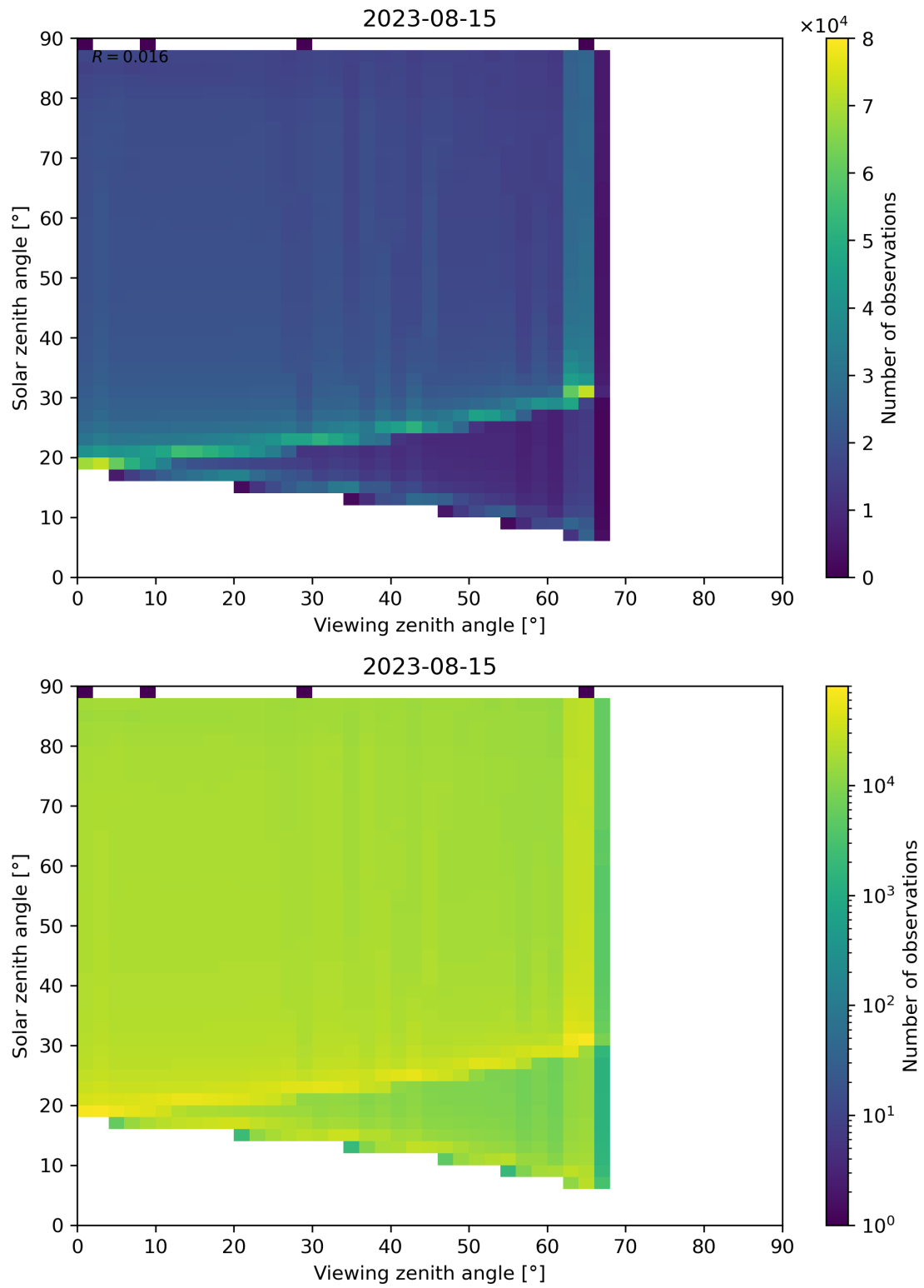
Figure 139: Scatter density plot of “Viewing zenith angle” against “Solar zenith angle” for 2023-08-14 to 2023-08-16.
