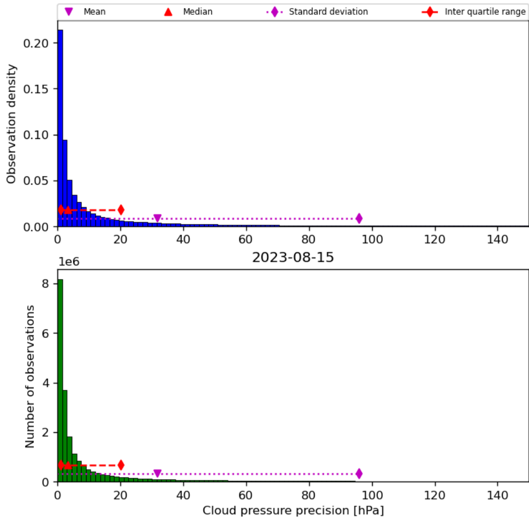
Figure 31: Histogram of “Cloud pressure precision” for 2023-08-14 to 2023-08-16
