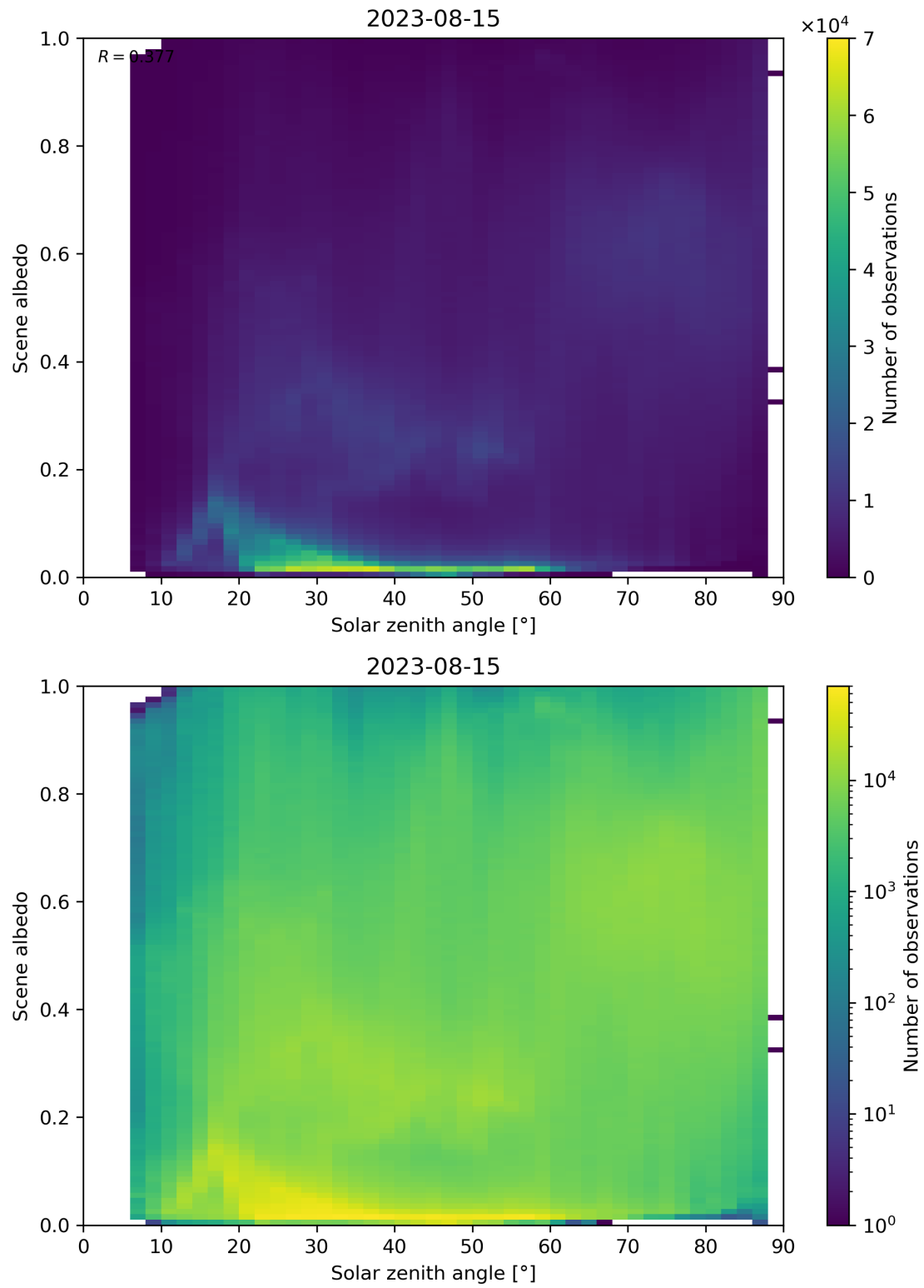
Figure 127: Scatter density plot of “Solar zenith angle” against “Scene albedo” for 2023-08-14 to 2023-08-16.
