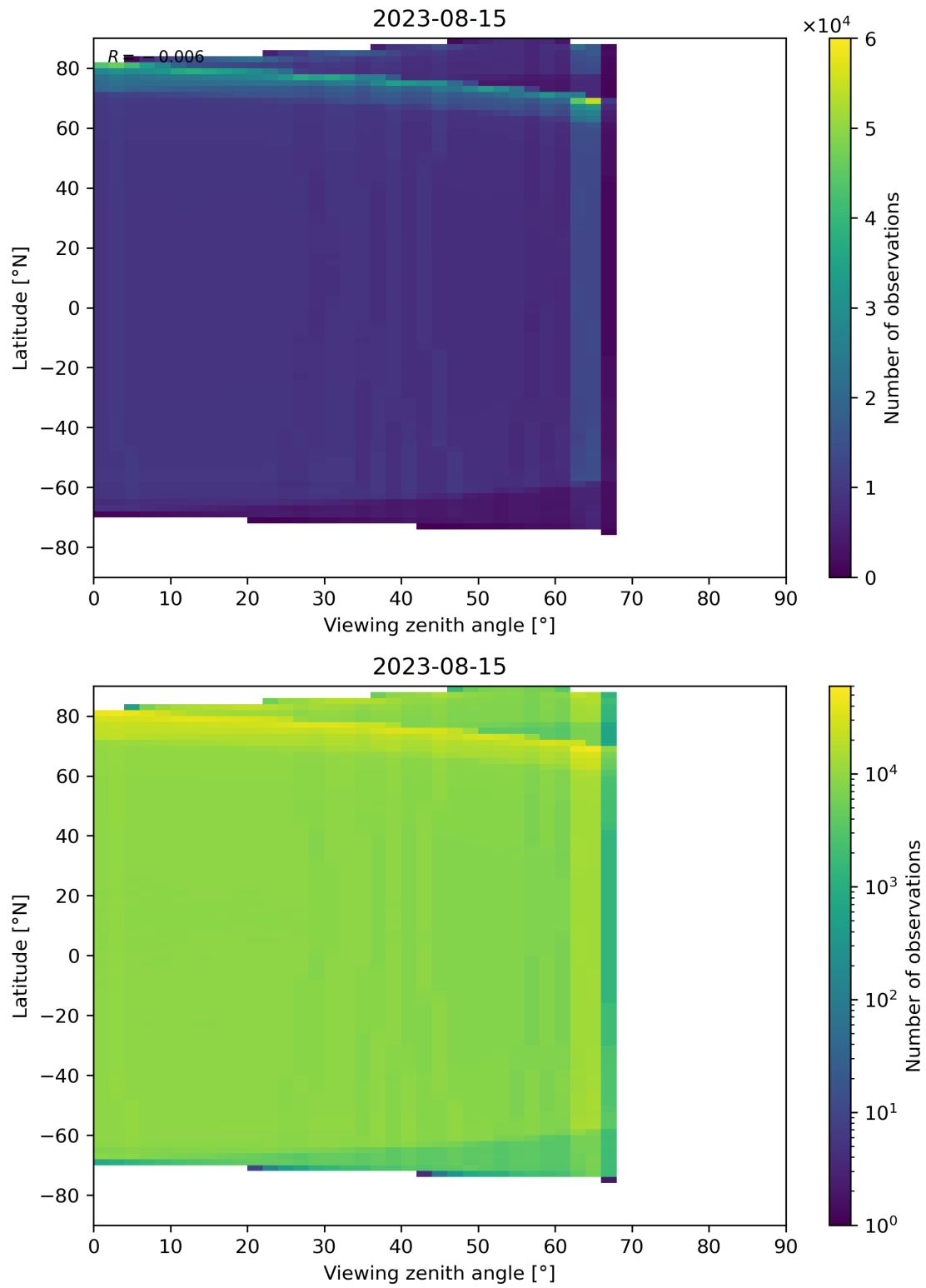
Figure 135: Scatter density plot of “Viewing zenith angle” against “Latitude” for 2023-08-14 to 2023-08-16.
