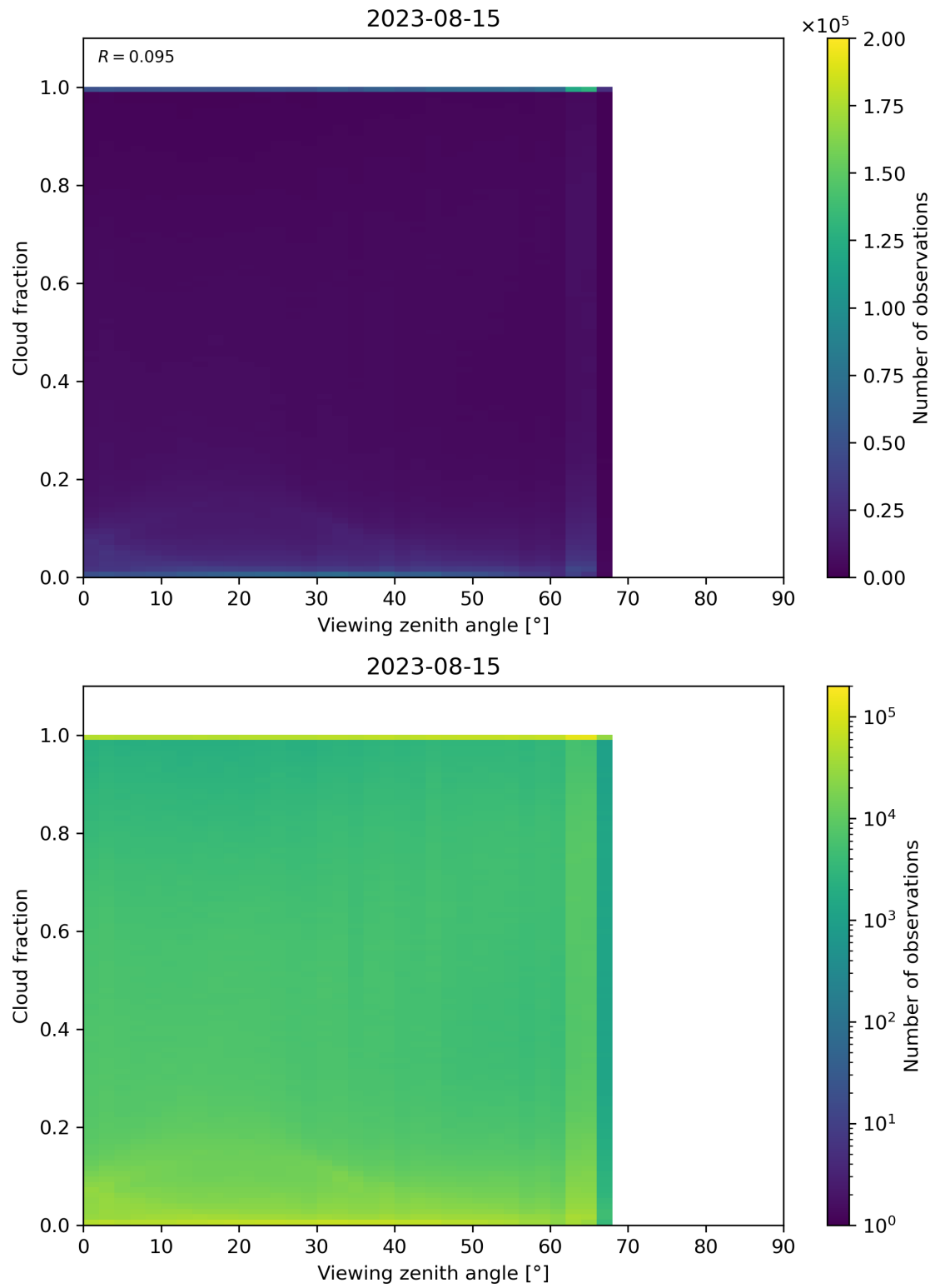
Figure 132: Scatter density plot of “Viewing zenith angle” against “Cloud fraction” for 2023-08-14 to 2023-08-16.
