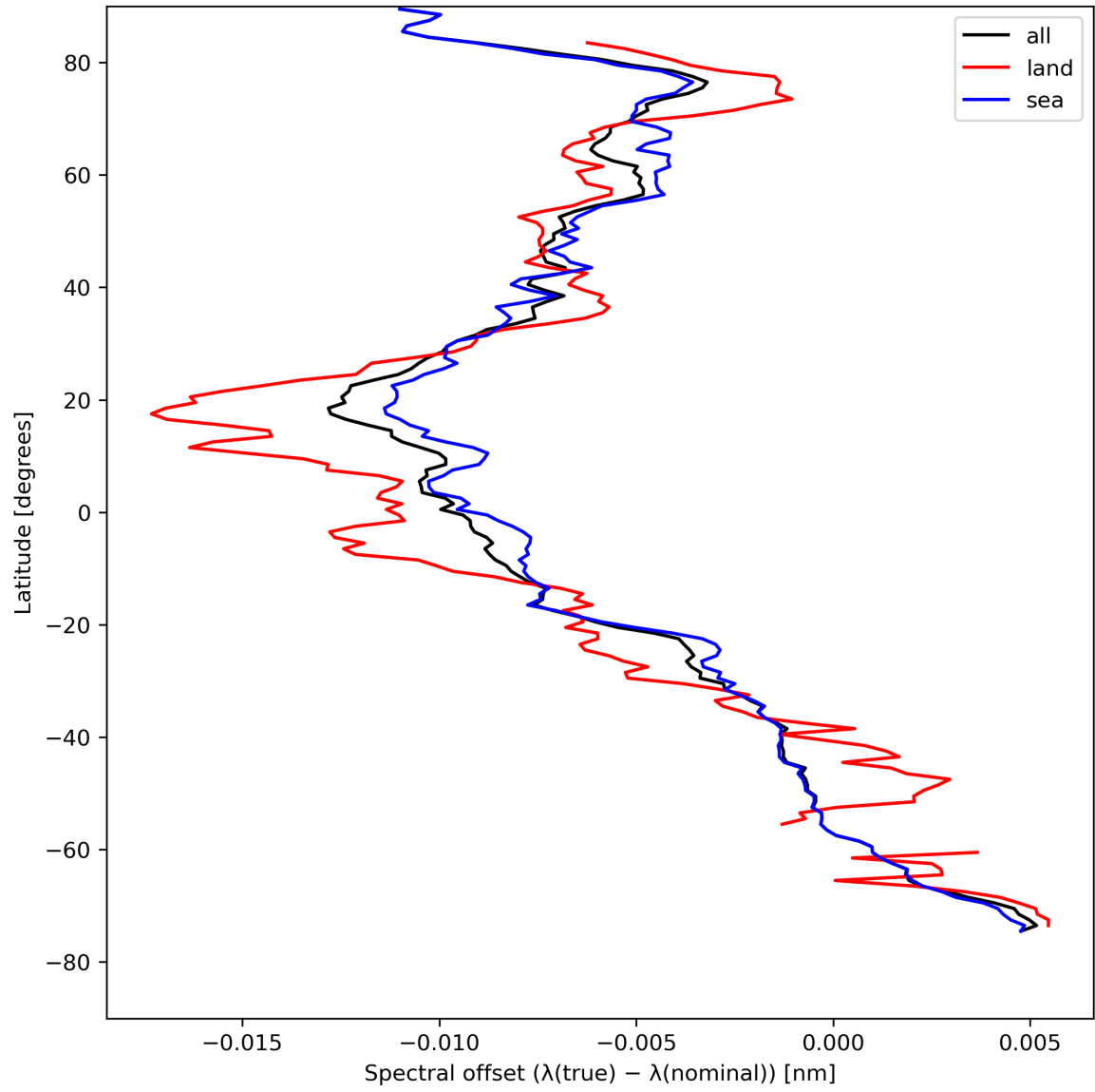
Figure 28: Zonal average of “Spectral offset ( \lambda(\text{true}) - \lambda(\text{nominal}) )” for 2023-08-14 to 2023-08-16.
