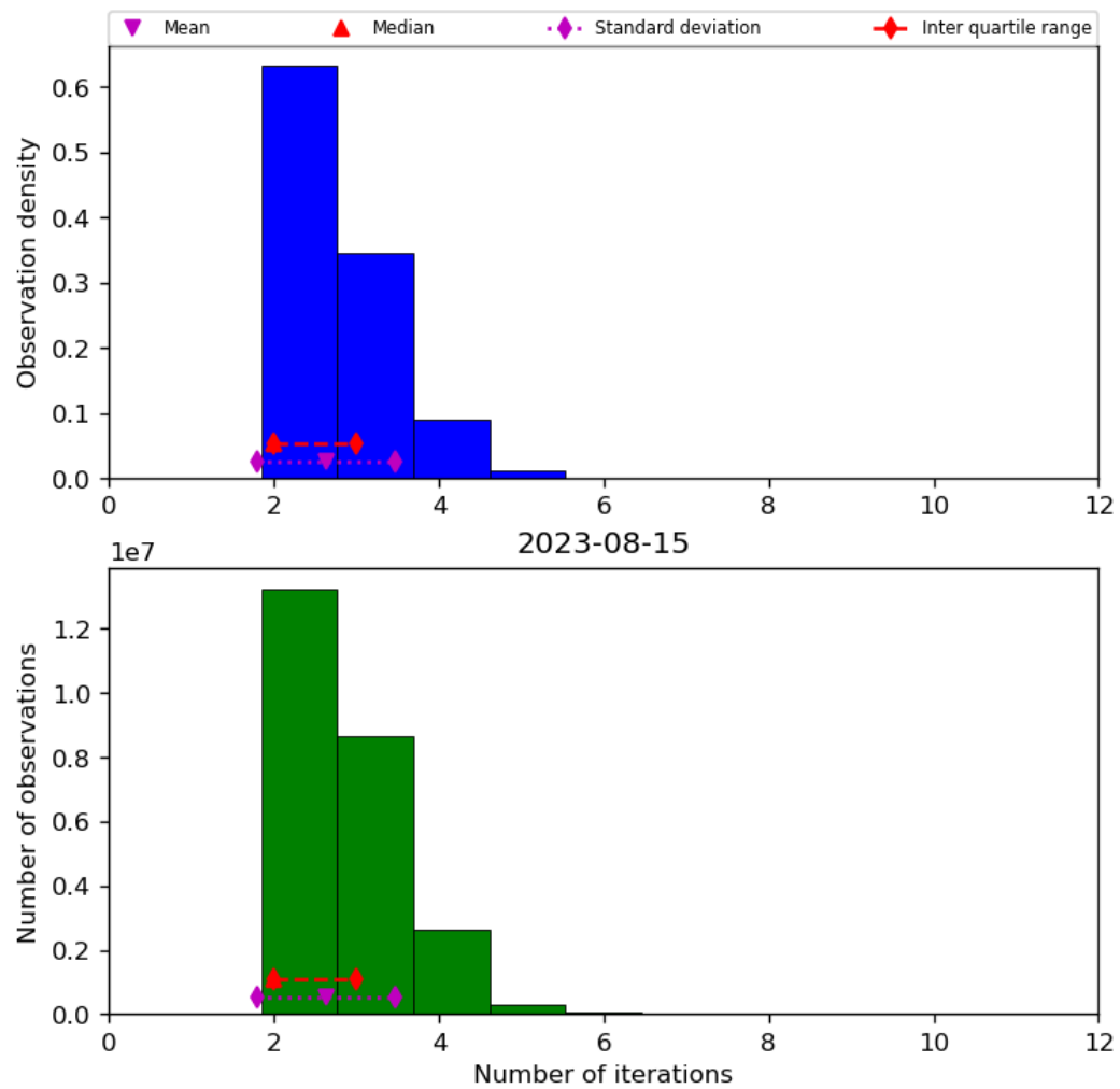
Figure 39: Histogram of “Number of iterations” for 2023-08-14 to 2023-08-16
