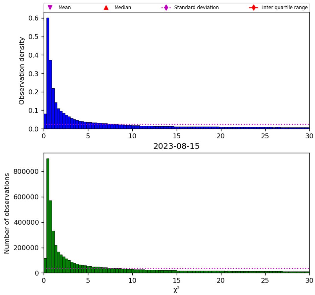
Figure 38: Histogram of “ \chi^2 ” for 2023-08-14 to 2023-08-16
