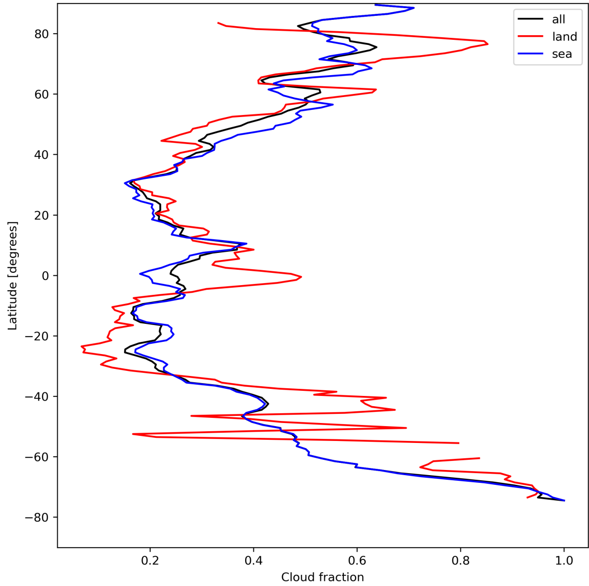
Figure 15: Zonal average of “Cloud fraction” for 2023-08-14 to 2023-08-16.
