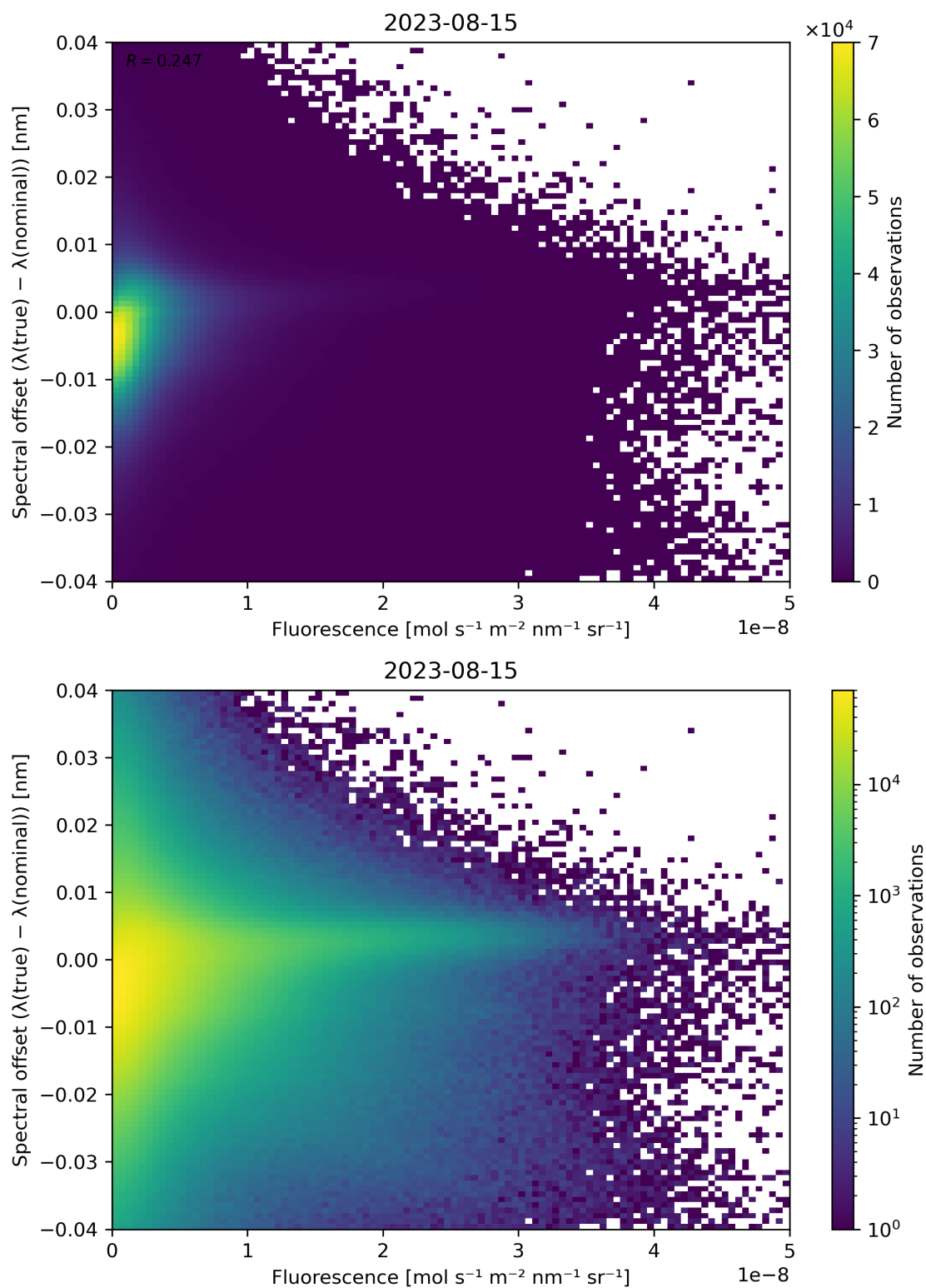
Figure 95: Scatter density plot of “Fluorescence” against “Spectral offset ( \lambda(\text{true}) - \lambda(\text{nominal}) )” for 2023-08-14 to 2023-08-16.
