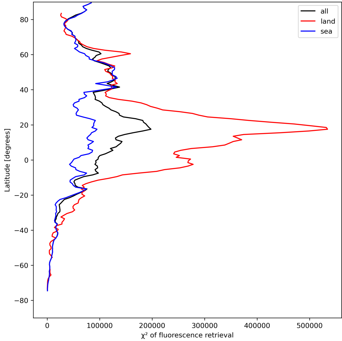
Figure 25: Zonal average of “ \chi^2 of fluorescence retrieval” for 2023-08-14 to 2023-08-16.
