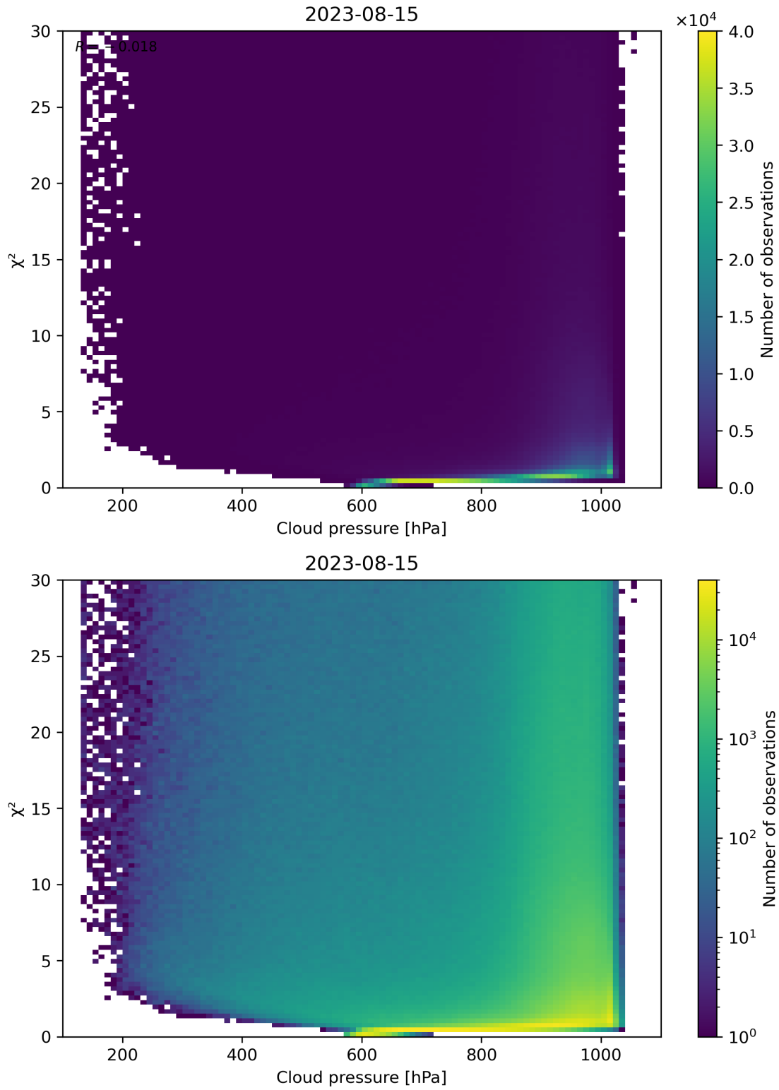
Figure 85: Scatter density plot of “Cloud pressure” against “ \chi^2 ” for 2023-08-14 to 2023-08-16.
