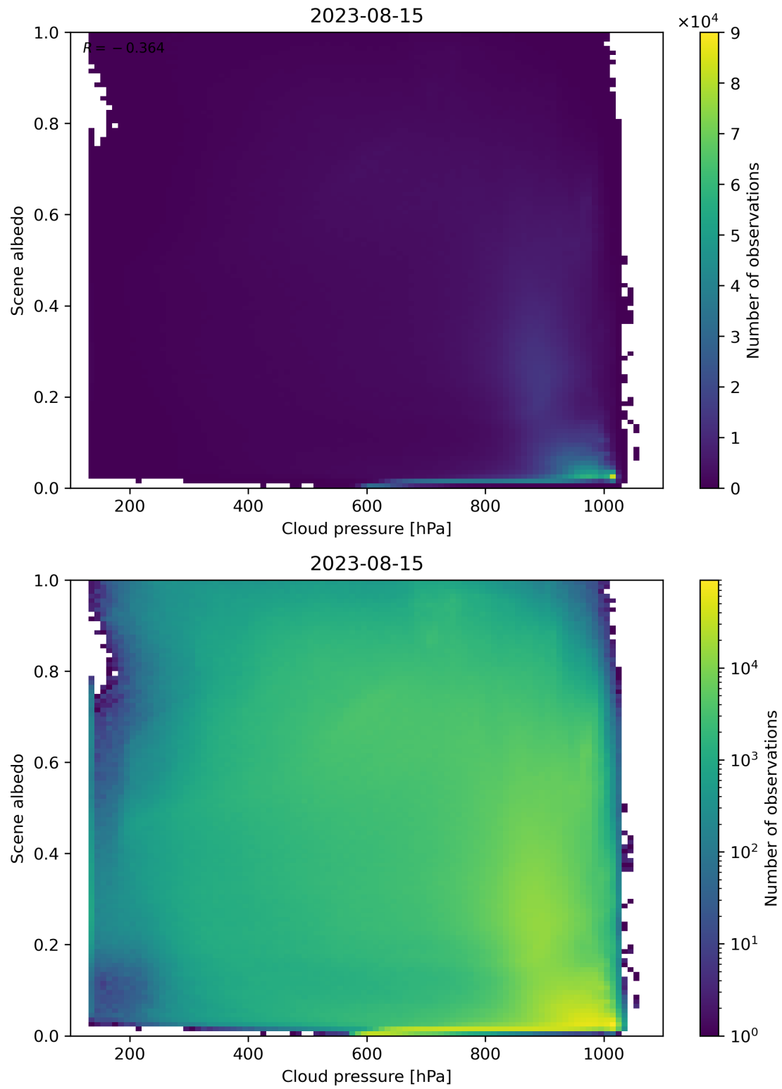
Figure 91: Scatter density plot of “Cloud pressure” against “Scene albedo” for 2023-08-14 to 2023-08-16.
