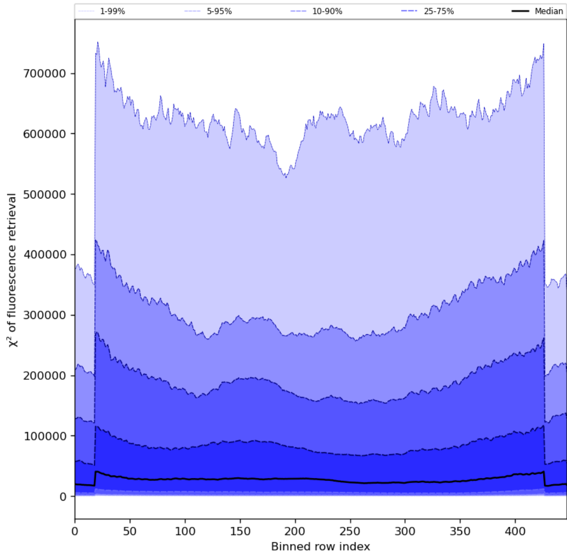
Figure 59: Along track statistics of “ \chi^2 of fluorescence retrieval” for 2023-08-14 to 2023-08-16
