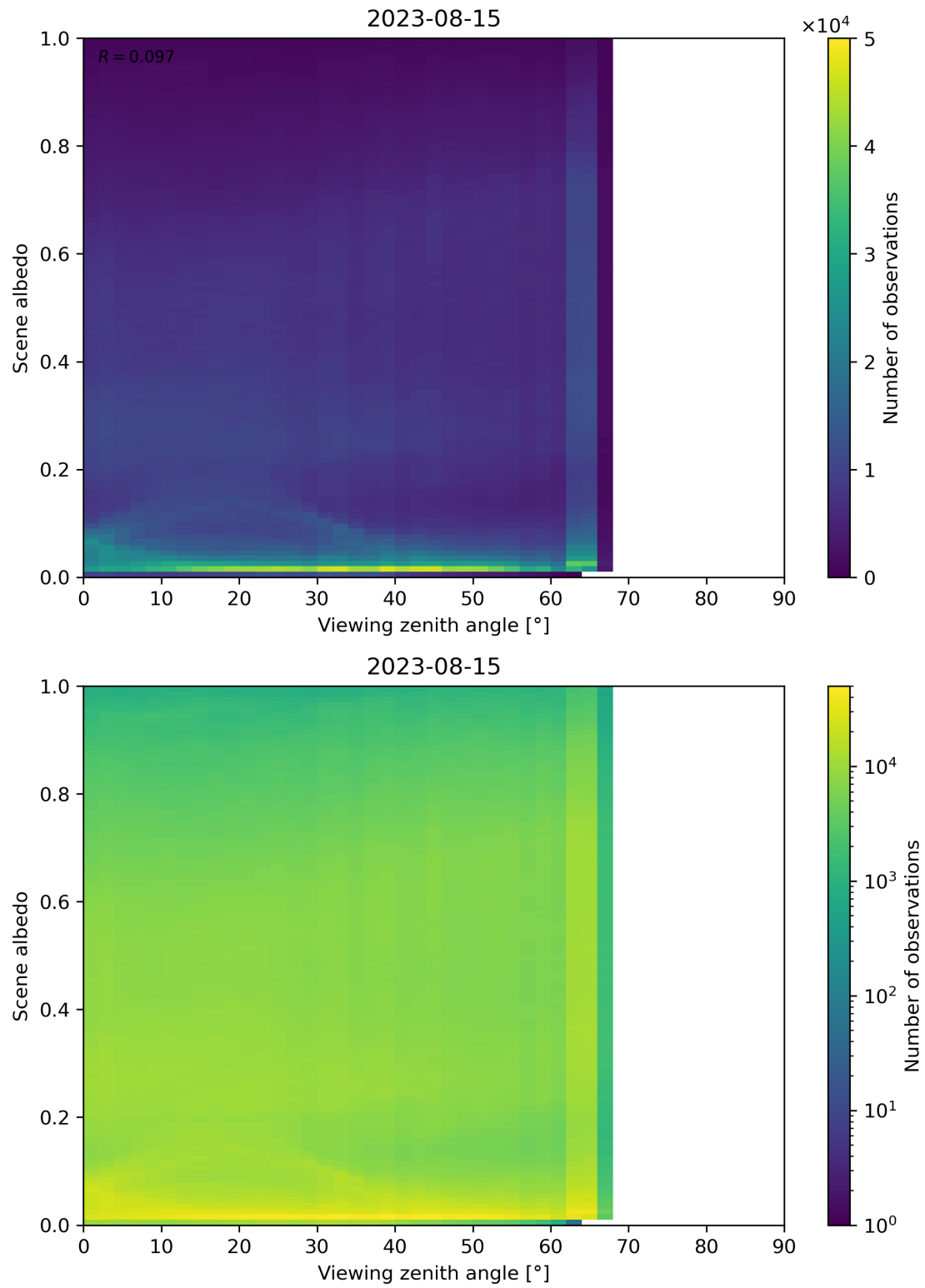
Figure 138: Scatter density plot of “Viewing zenith angle” against “Scene albedo” for 2023-08-14 to 2023-08-16.
