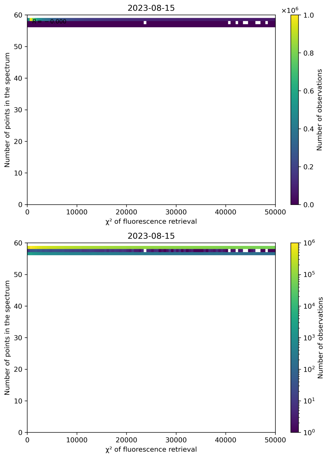
Figure 71: Scatter density plot of " \chi^2 of fluorescence retrieval" against "Number of points in the spectrum" for 2023-08-14 to 2023-08-16.
