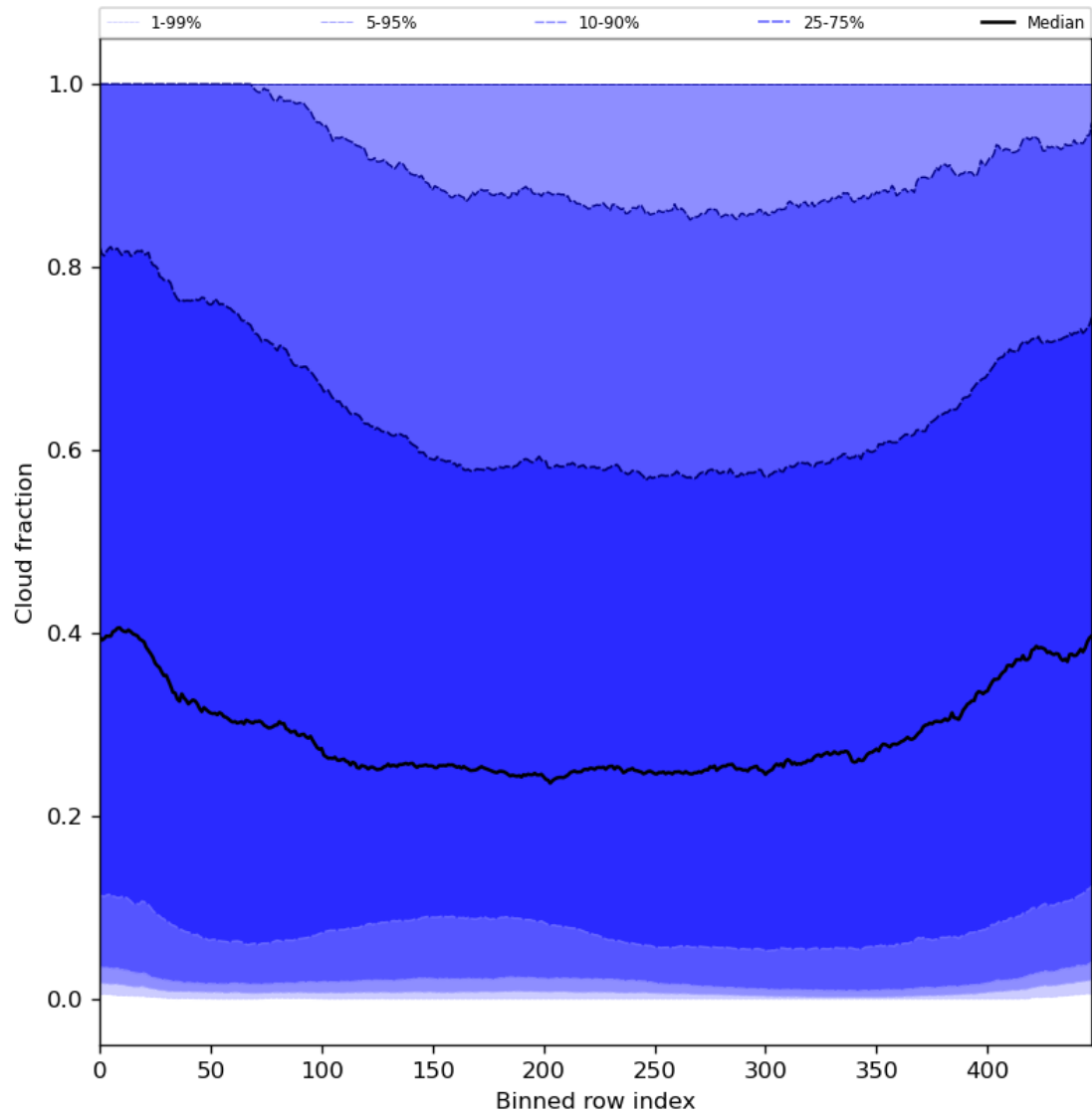
Figure 49: Along track statistics of “Cloud fraction” for 2023-08-14 to 2023-08-16
