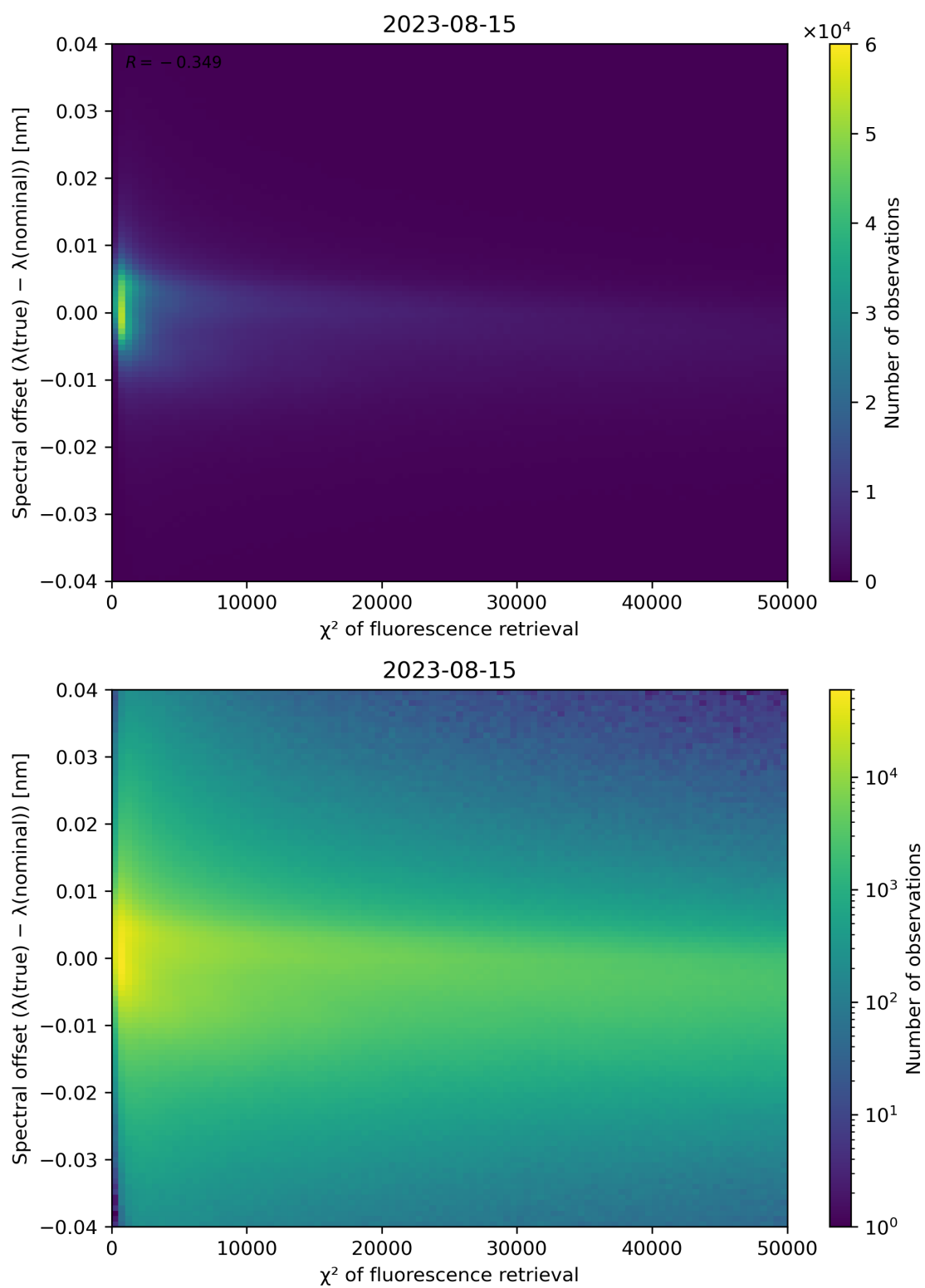
Figure 72: Scatter density plot of " \chi^2 of fluorescence retrieval" against "Spectral offset ( \lambda(\text{true}) - \lambda(\text{nominal})) " for 2023-08-14 to 2023-08-16.
