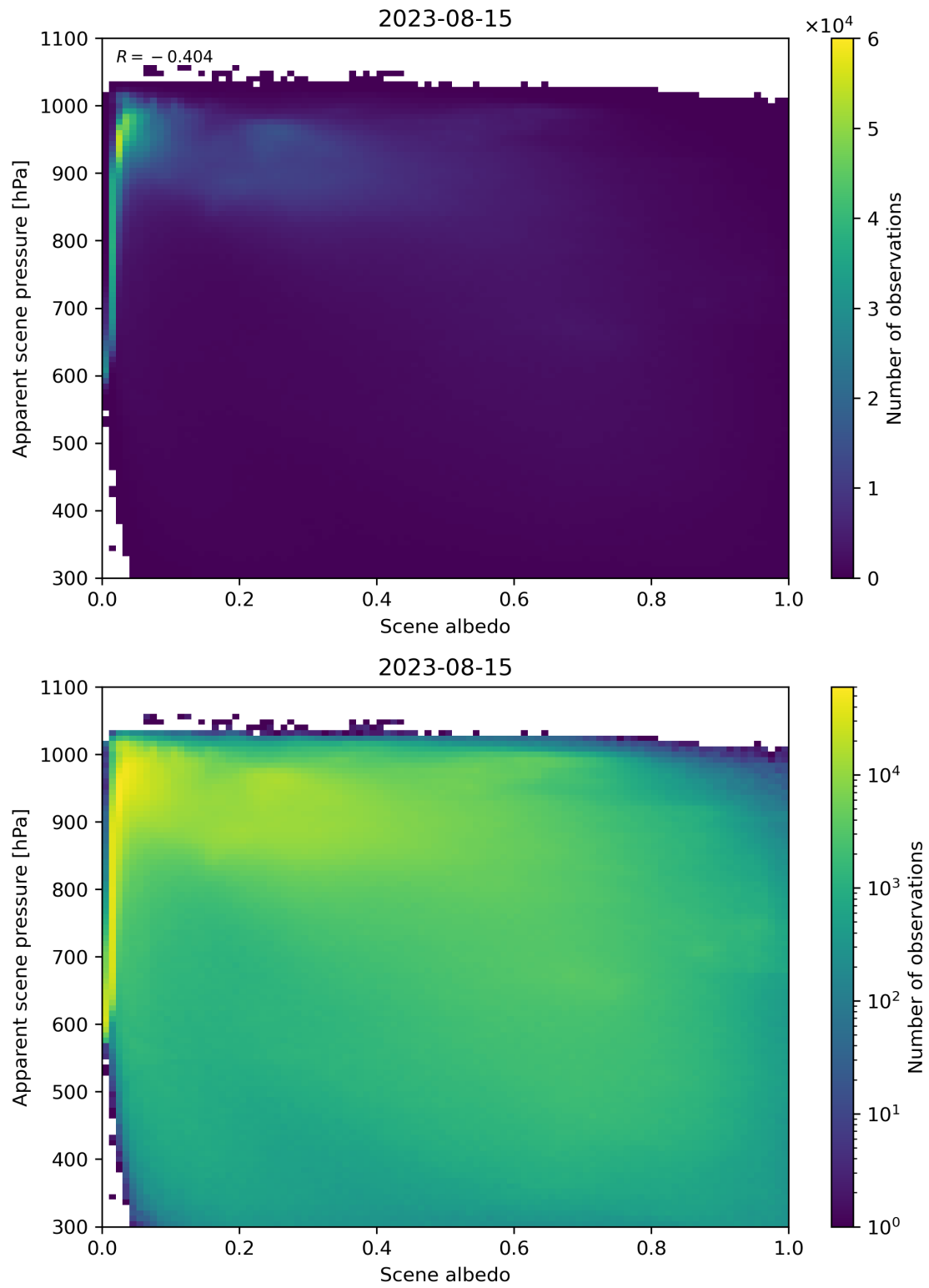
Figure 111: Scatter density plot of “Scene albedo” against “Apparent scene pressure” for 2023-08-14 to 2023-08-16.
