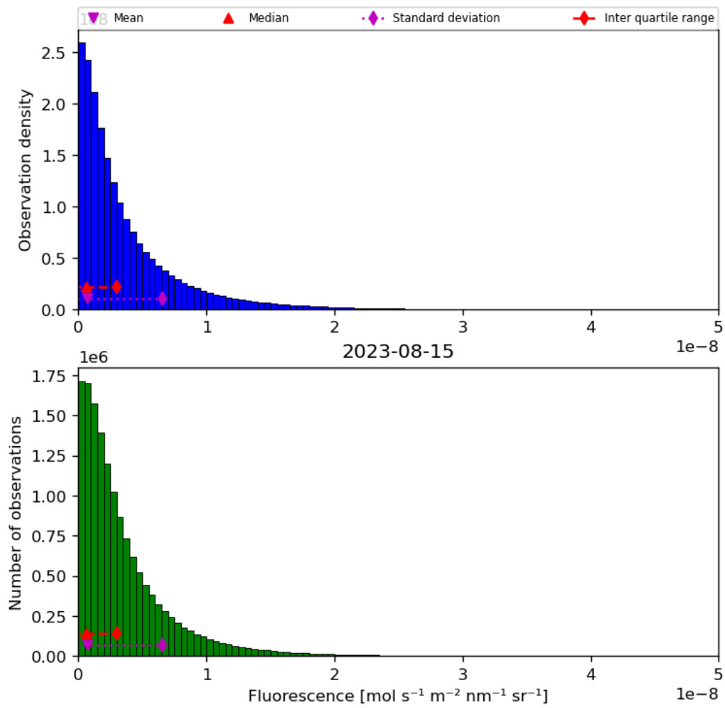
Figure 40: Histogram of “Fluorescence” for 2023-08-14 to 2023-08-16
