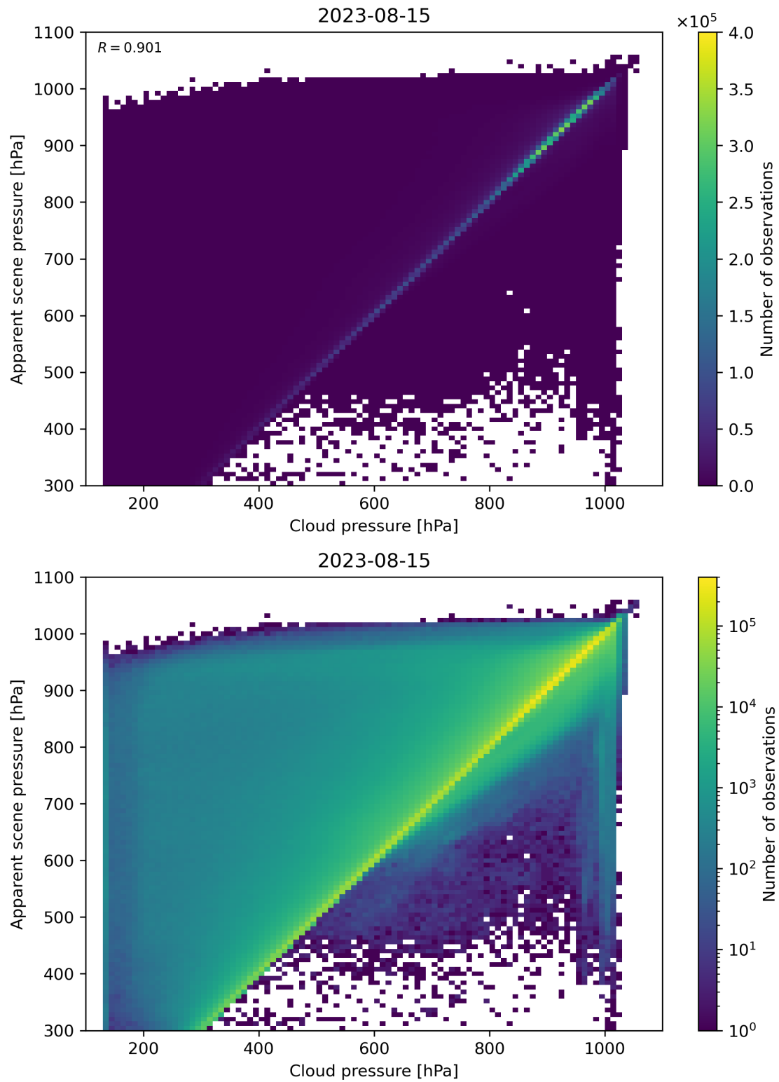
Figure 84: Scatter density plot of “Cloud pressure” against “Apparent scene pressure” for 2023-08-14 to 2023-08-16.
