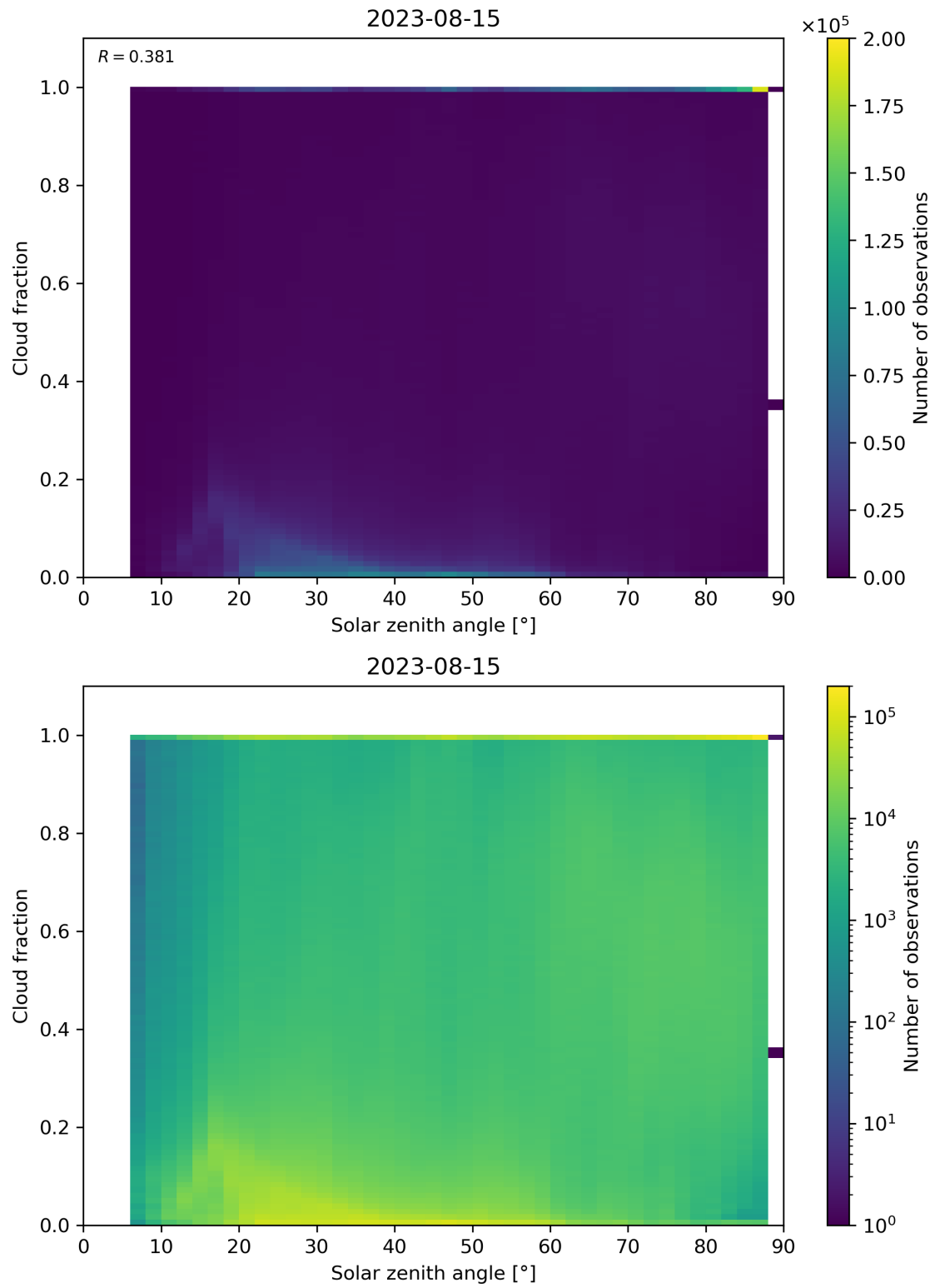
Figure 121: Scatter density plot of “Solar zenith angle” against “Cloud fraction” for 2023-08-14 to 2023-08-16.
