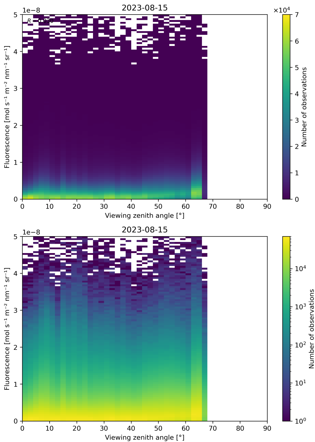
Figure 134: Scatter density plot of “Viewing zenith angle” against “Fluorescence” for 2023-08-14 to 2023-08-16.
