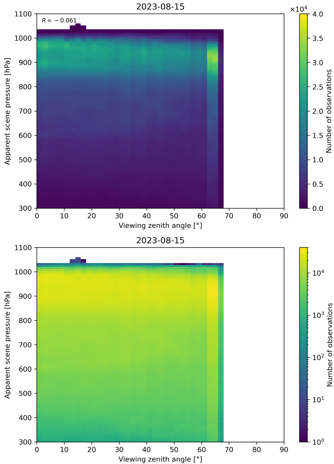
Figure 129: Scatter density plot of “Viewing zenith angle” against “Apparent scene pressure” for 2023-08-14 to 2023-08-16.
