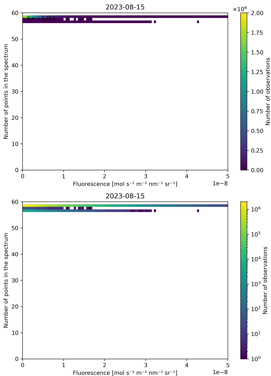
Figure 94: Scatter density plot of “Fluorescence” against “Number of points in the spectrum” for 2023-08-14 to 2023-08-16.
