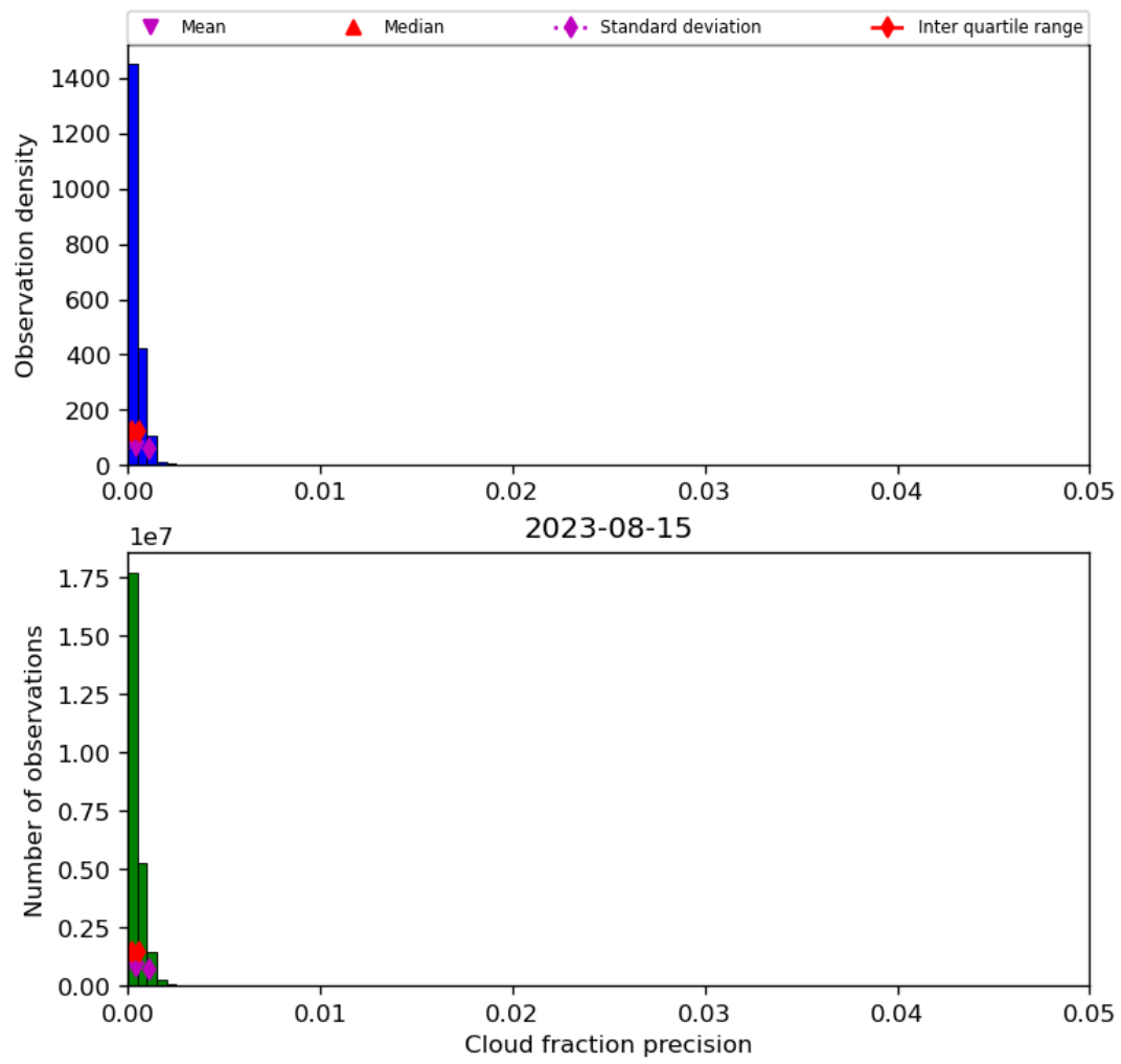
Figure 33: Histogram of “Cloud fraction precision” for 2023-08-14 to 2023-08-16
