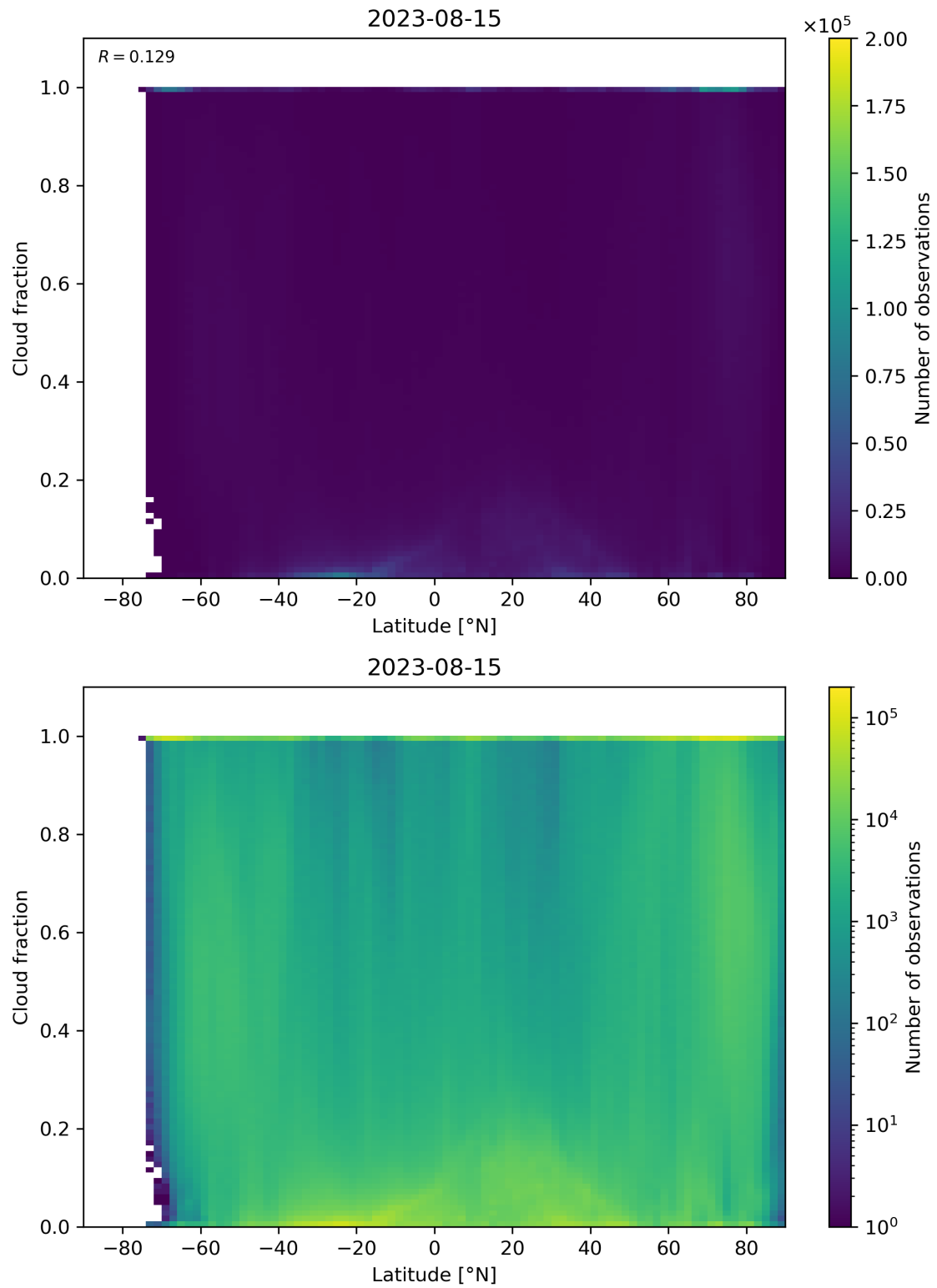
Figure 99: Scatter density plot of “Latitude” against “Cloud fraction” for 2023-08-14 to 2023-08-16.
