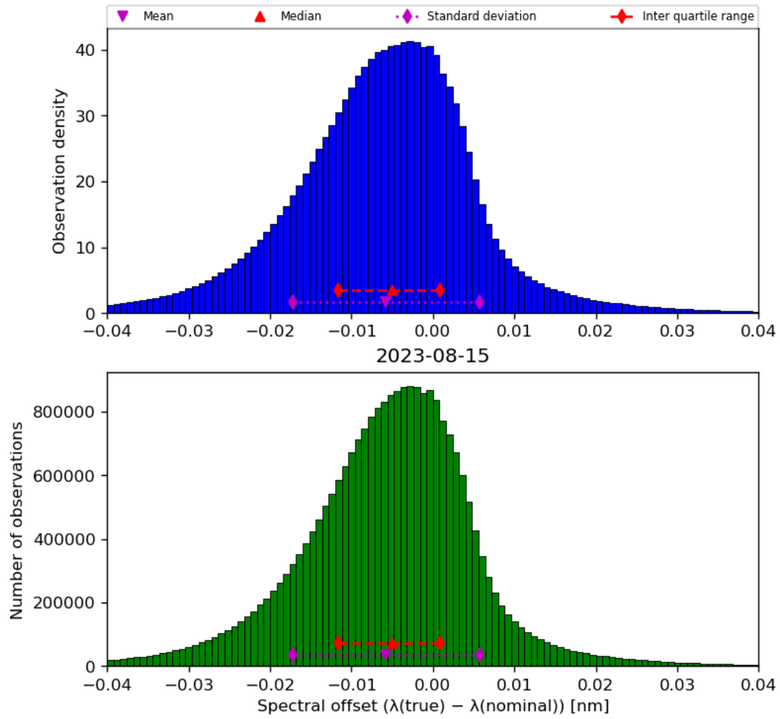
Figure 45: Histogram of “Spectral offset ( \lambda(\text{true}) - \lambda(\text{nominal}) )” for 2023-08-14 to 2023-08-16
