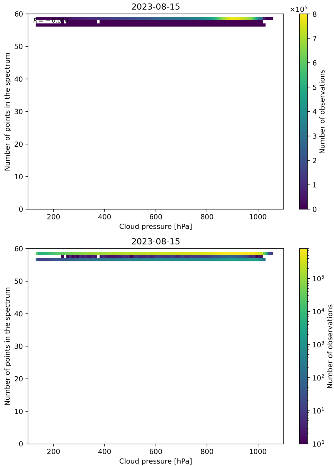
Figure 90: Scatter density plot of “Cloud pressure” against “Number of points in the spectrum” for 2023-08-14 to 2023-08-16.
