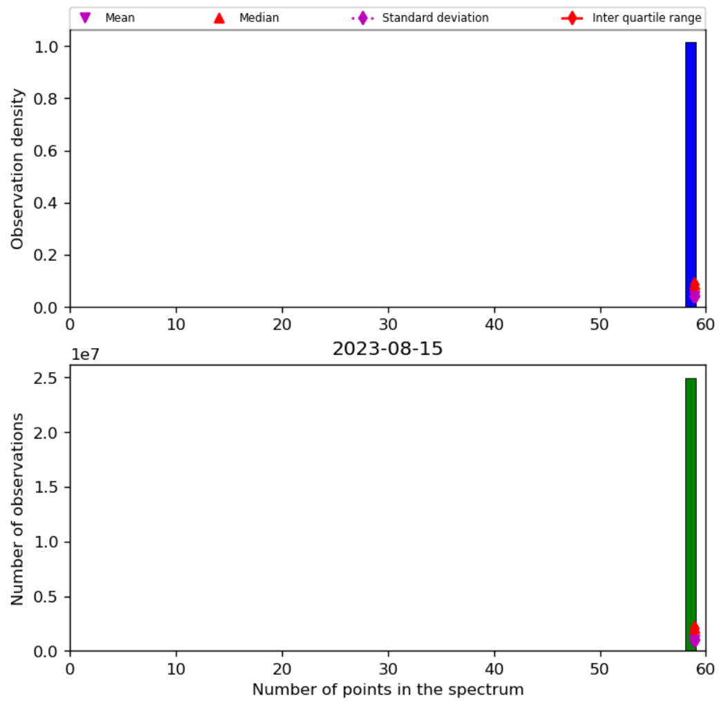
Figure 44: Histogram of “Number of points in the spectrum” for 2023-08-14 to 2023-08-16
