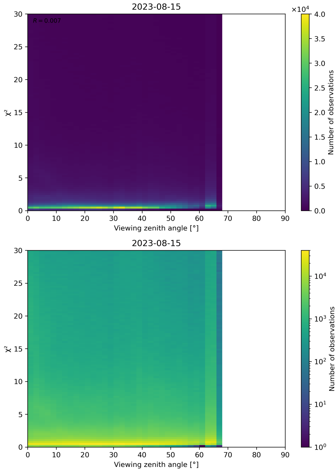
Figure 130: Scatter density plot of “Viewing zenith angle” against “ \chi^2 ” for 2023-08-14 to 2023-08-16.
