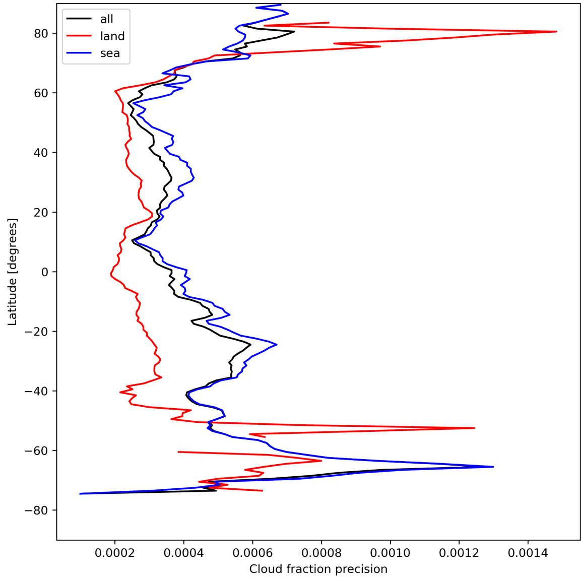
Figure 16: Zonal average of “Cloud fraction precision” for 2023-08-14 to 2023-08-16.
