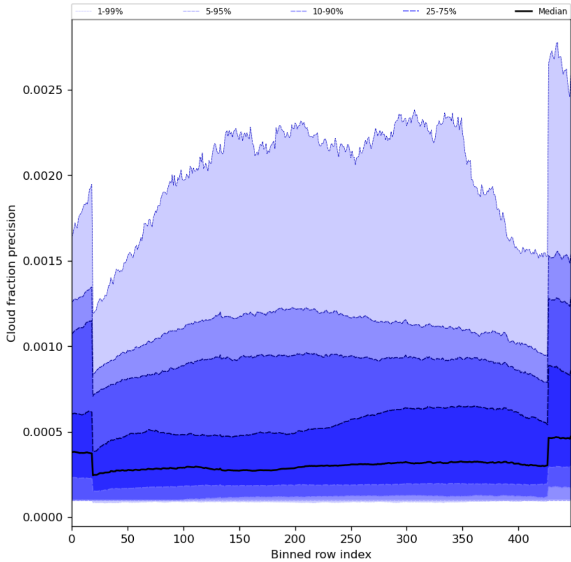
Figure 50: Along track statistics of “Cloud fraction precision” for 2023-08-14 to 2023-08-16
