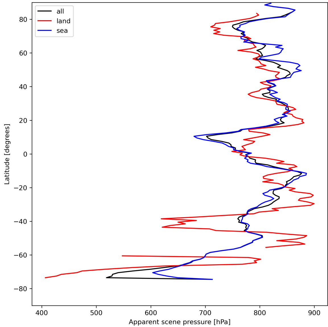
Figure 19: Zonal average of “Apparent scene pressure” for 2023-08-14 to 2023-08-16.
