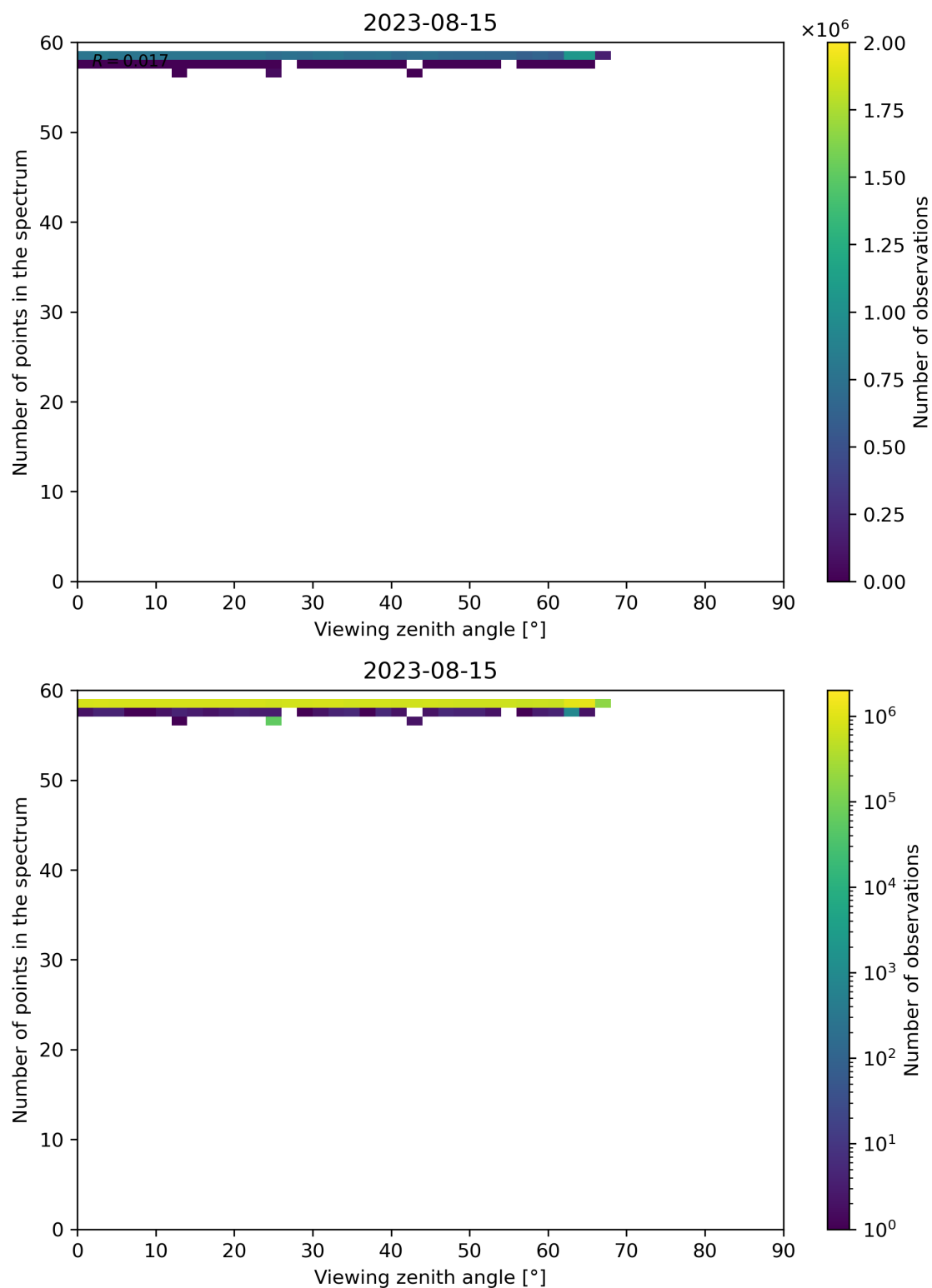
Figure 137: Scatter density plot of “Viewing zenith angle” against “Number of points in the spectrum” for 2023-08-14 to 2023-08-16.
