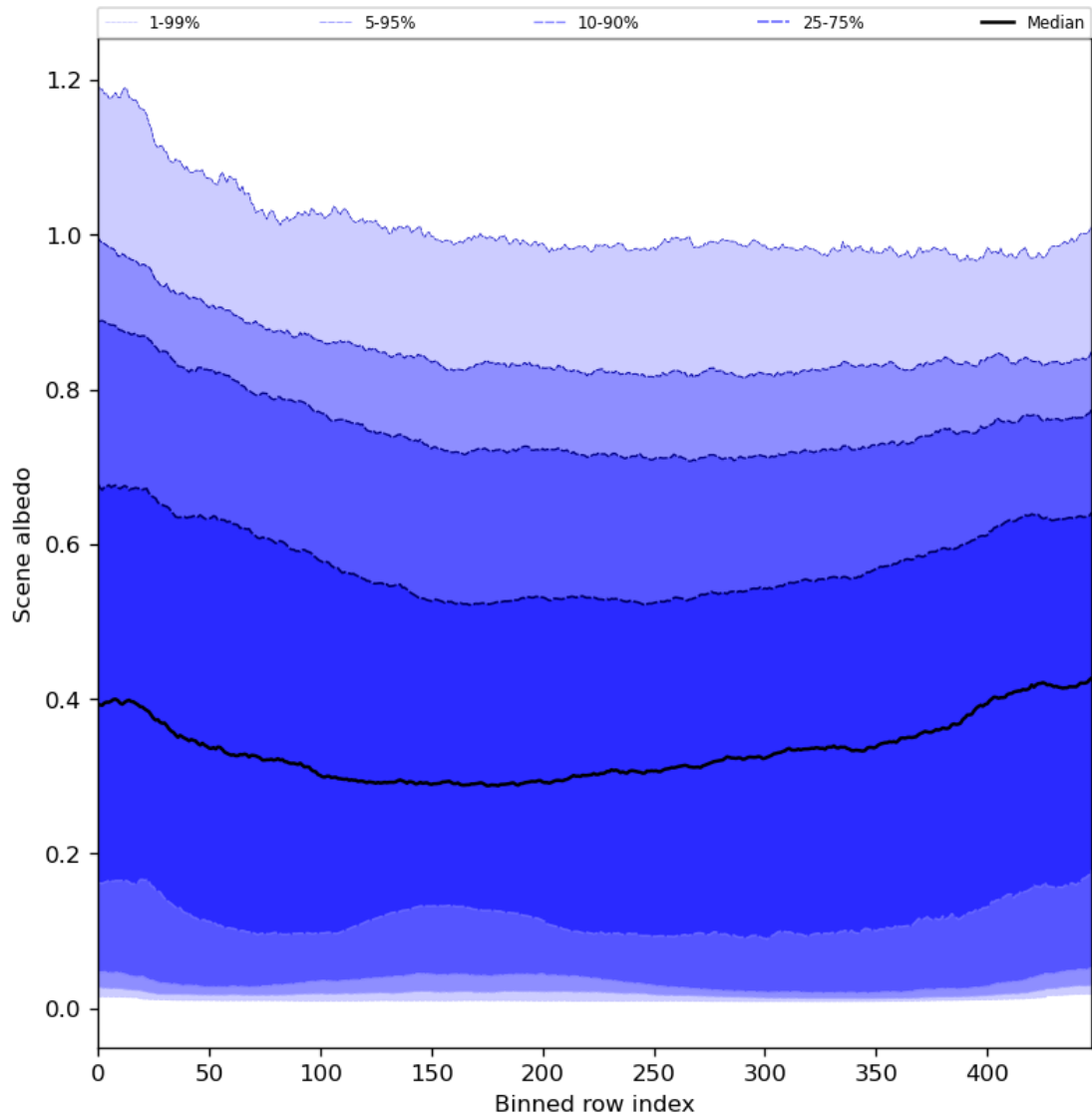
Figure 51: Along track statistics of “Scene albedo” for 2023-08-14 to 2023-08-16
