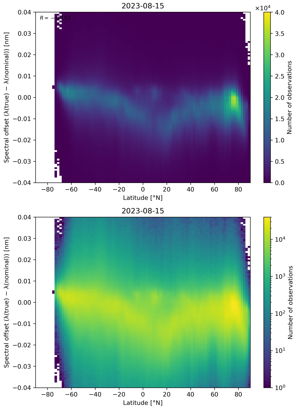
Figure 105: Scatter density plot of “Latitude” against “Spectral offset ( \lambda(\text{true}) - \lambda(\text{nominal}) )” for 2023-08-14 to 2023-08-16.
