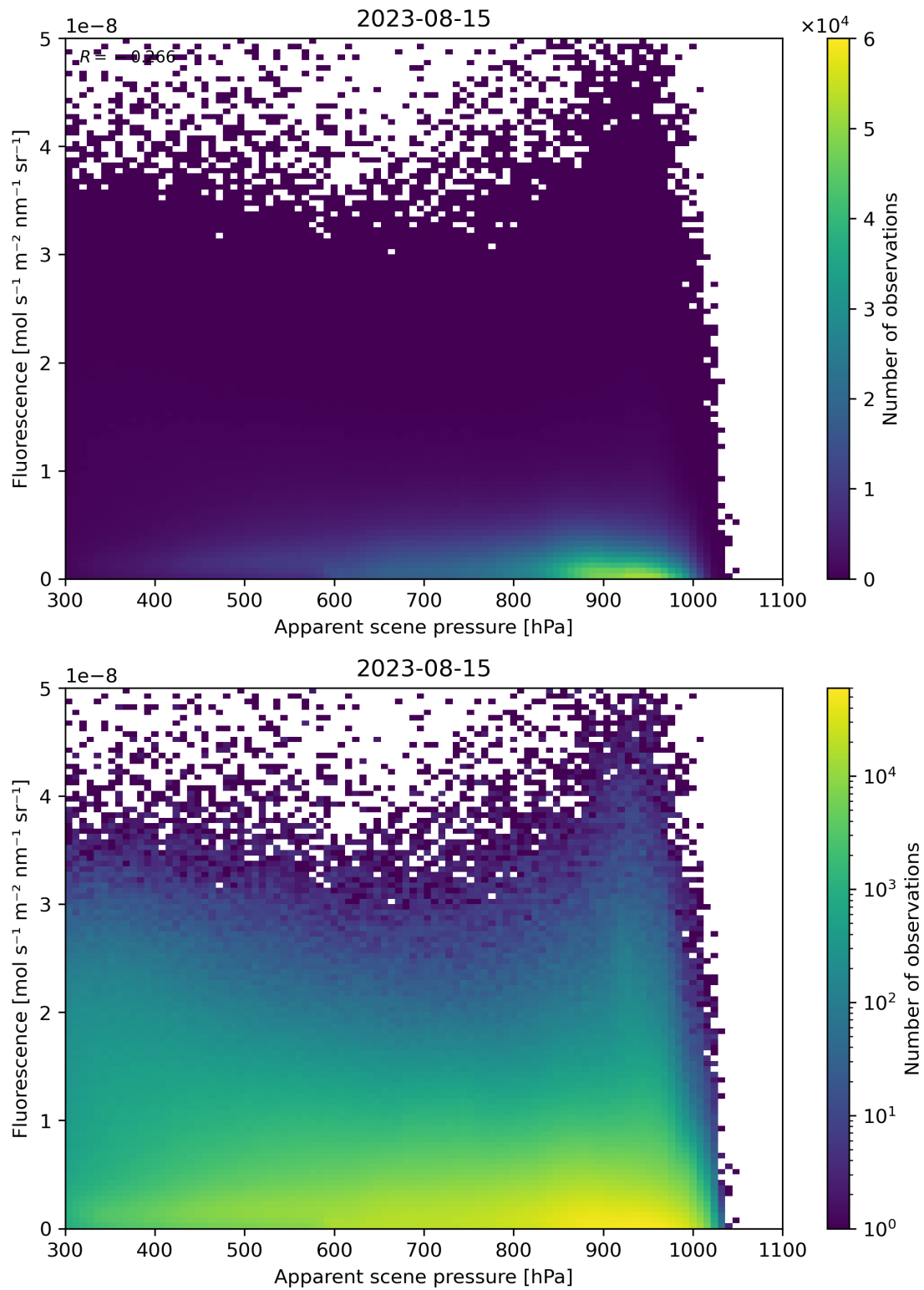
Figure 65: Scatter density plot of “Apparent scene pressure” against “Fluorescence” for 2023-08-14 to 2023-08-16.
