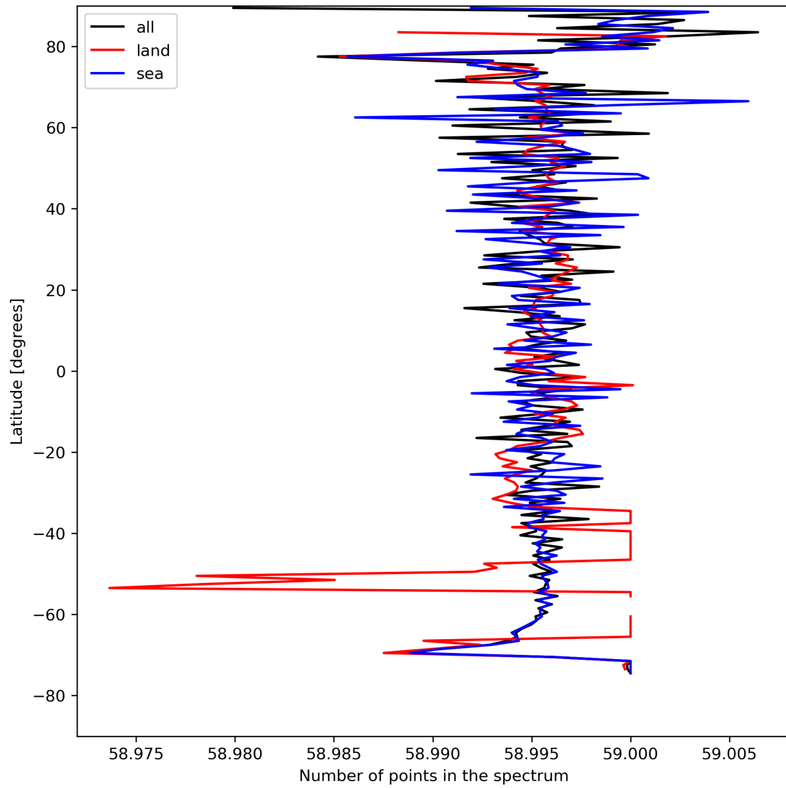
Figure 27: Zonal average of “Number of points in the spectrum” for 2023-08-14 to 2023-08-16.
