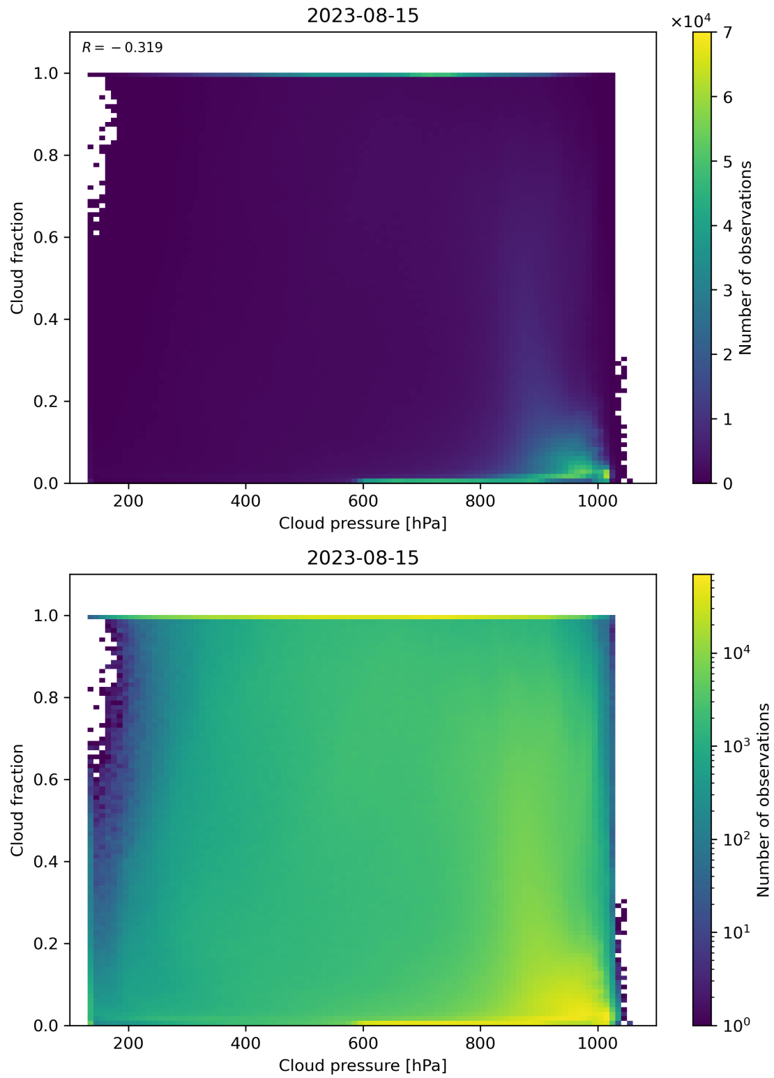
Figure 87: Scatter density plot of “Cloud pressure” against “Cloud fraction” for 2023-08-14 to 2023-08-16.
