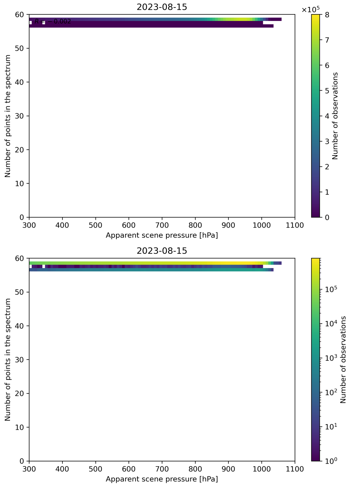
Figure 67: Scatter density plot of “Apparent scene pressure” against “Number of points in the spectrum” for 2023-08-14 to 2023-08-16.
