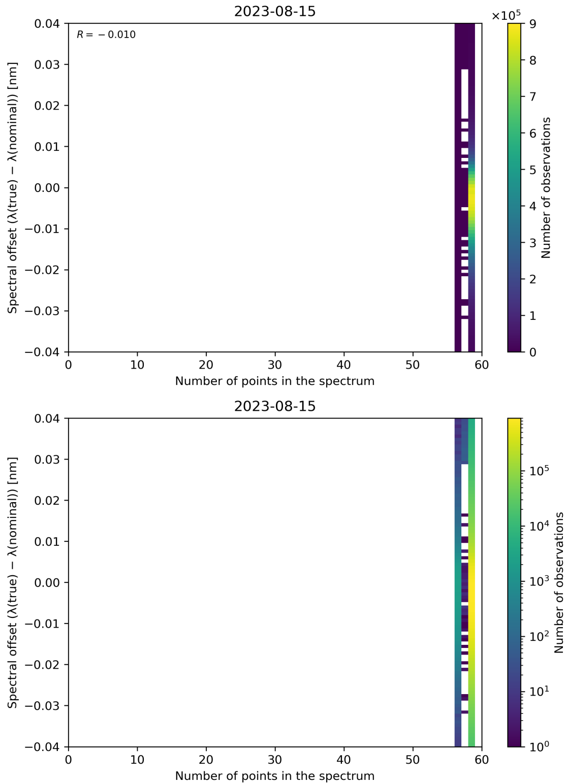
Figure 110: Scatter density plot of “Number of points in the spectrum” against “Spectral offset ( \lambda(\text{true}) - \lambda(\text{nominal}) )” for 2023-08-14 to 2023-08-16.
