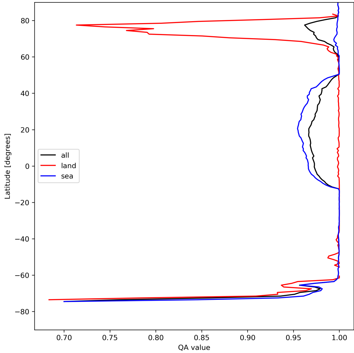
Figure 12: Zonal average of “QA value” for 2023-08-14 to 2023-08-16.
