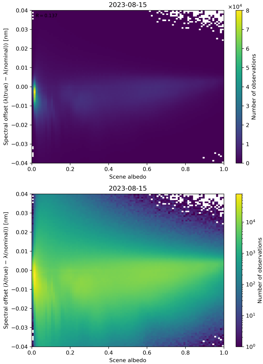
Figure 117: Scatter density plot of “Scene albedo” against “Spectral offset ( \lambda(\text{true}) - \lambda(\text{nominal}) )” for 2023-08-14 to 2023-08-16.
