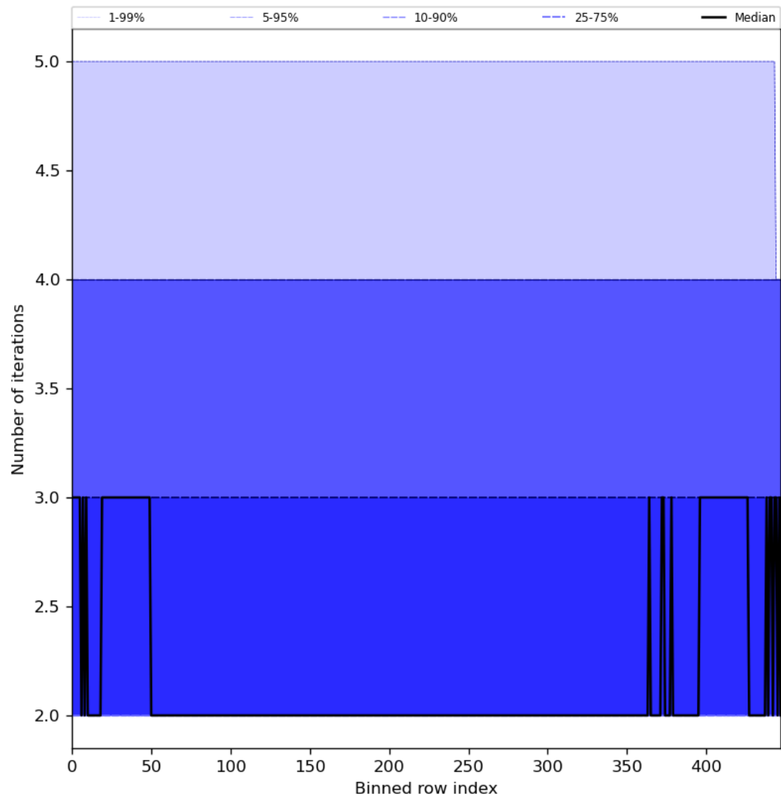
Figure 56: Along track statistics of “Number of iterations” for 2023-08-14 to 2023-08-16
