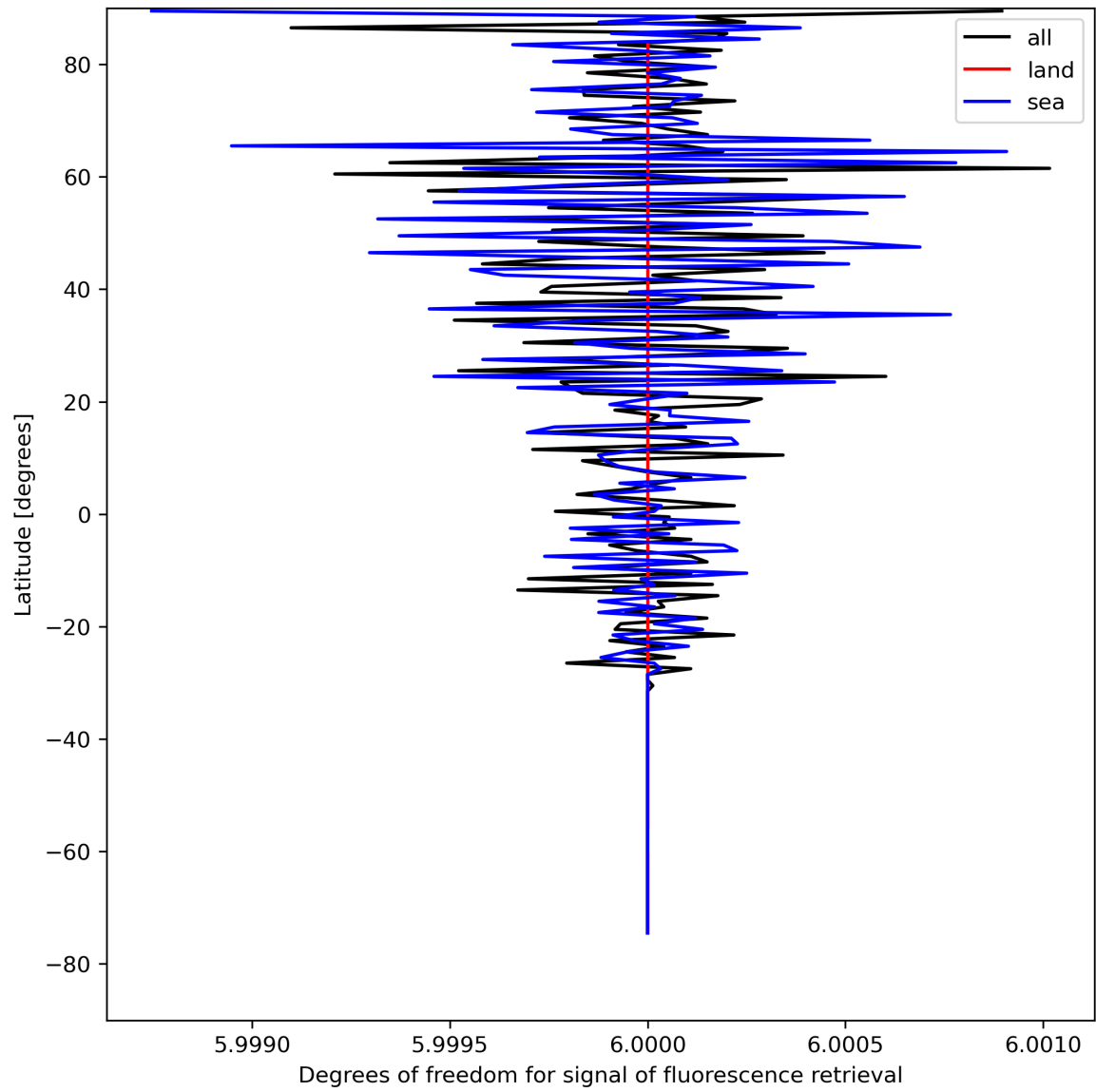
Figure 26: Zonal average of “Degrees of freedom for signal of fluorescence retrieval” for 2023-08-15 to 2023-08-17.
