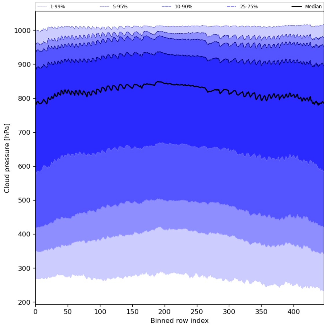
Figure 47: Along track statistics of “Cloud pressure” for 2023-08-15 to 2023-08-17
