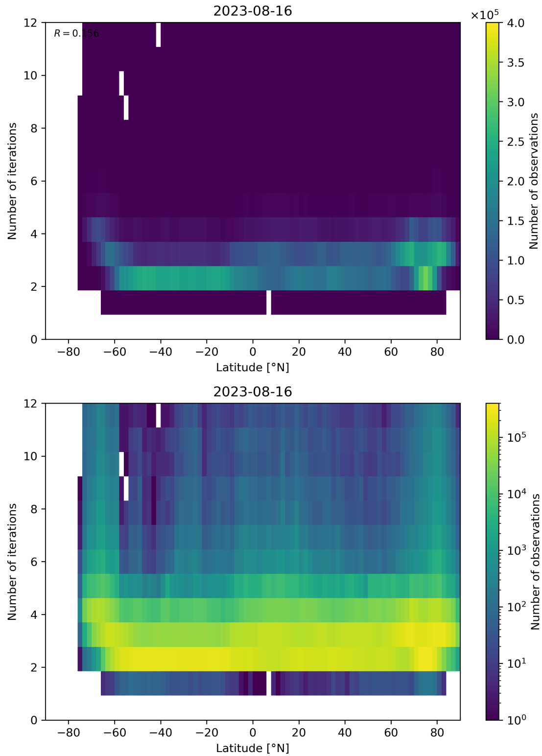
Figure 102: Scatter density plot of “Latitude” against “Number of iterations” for 2023-08-15 to 2023-08-17.
