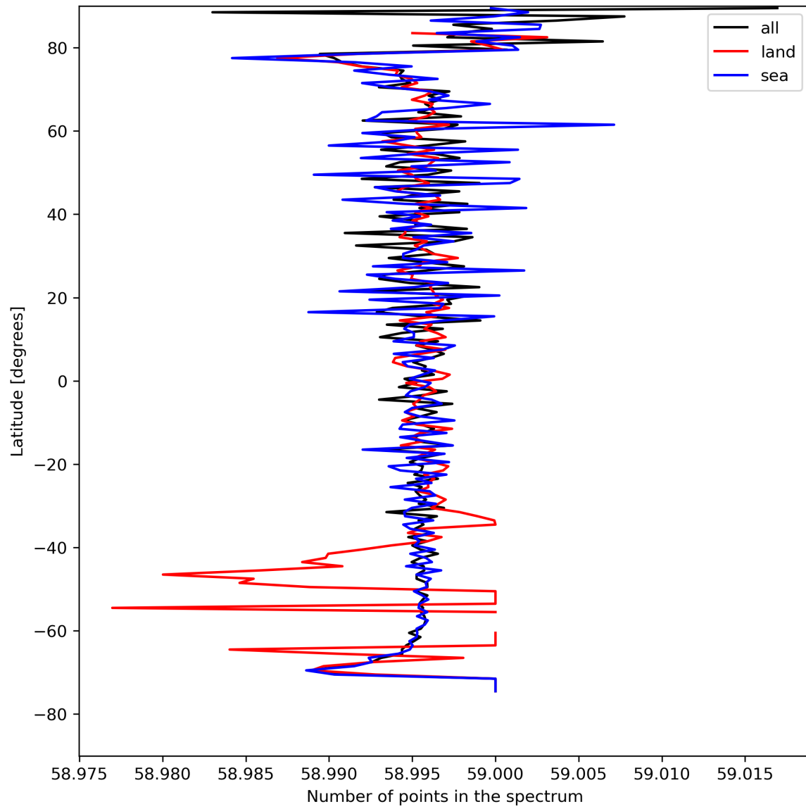
Figure 27: Zonal average of “Number of points in the spectrum” for 2023-08-15 to 2023-08-17.
