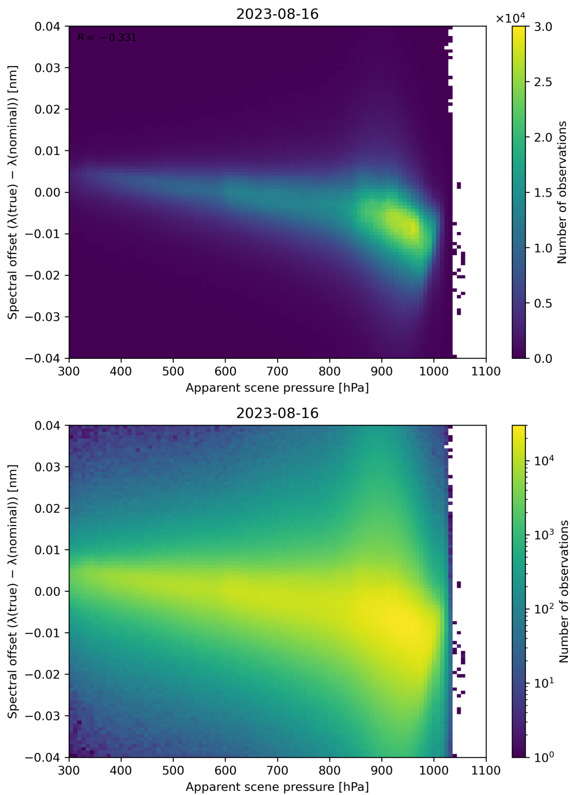
Figure 68: Scatter density plot of “Apparent scene pressure” against “Spectral offset ( \lambda(\text{true}) - \lambda(\text{nominal}) )” for 2023-08-15 to 2023-08-17.
