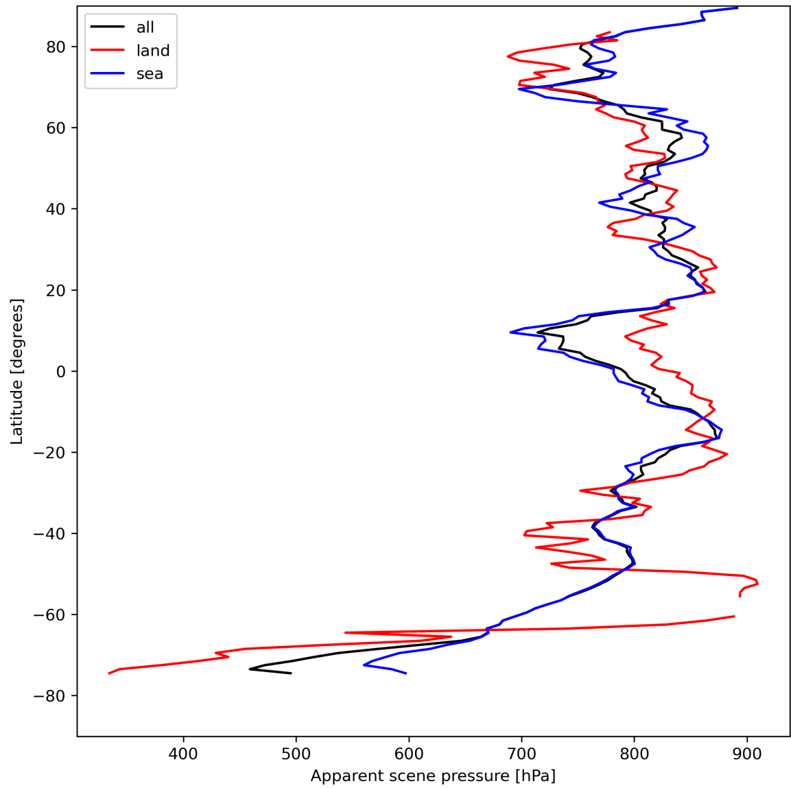
Figure 19: Zonal average of “Apparent scene pressure” for 2023-08-15 to 2023-08-17.
