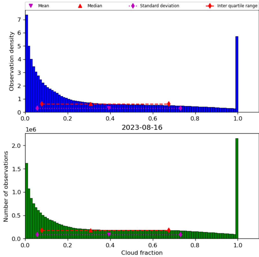
Figure 32: Histogram of “Cloud fraction” for 2023-08-15 to 2023-08-17
