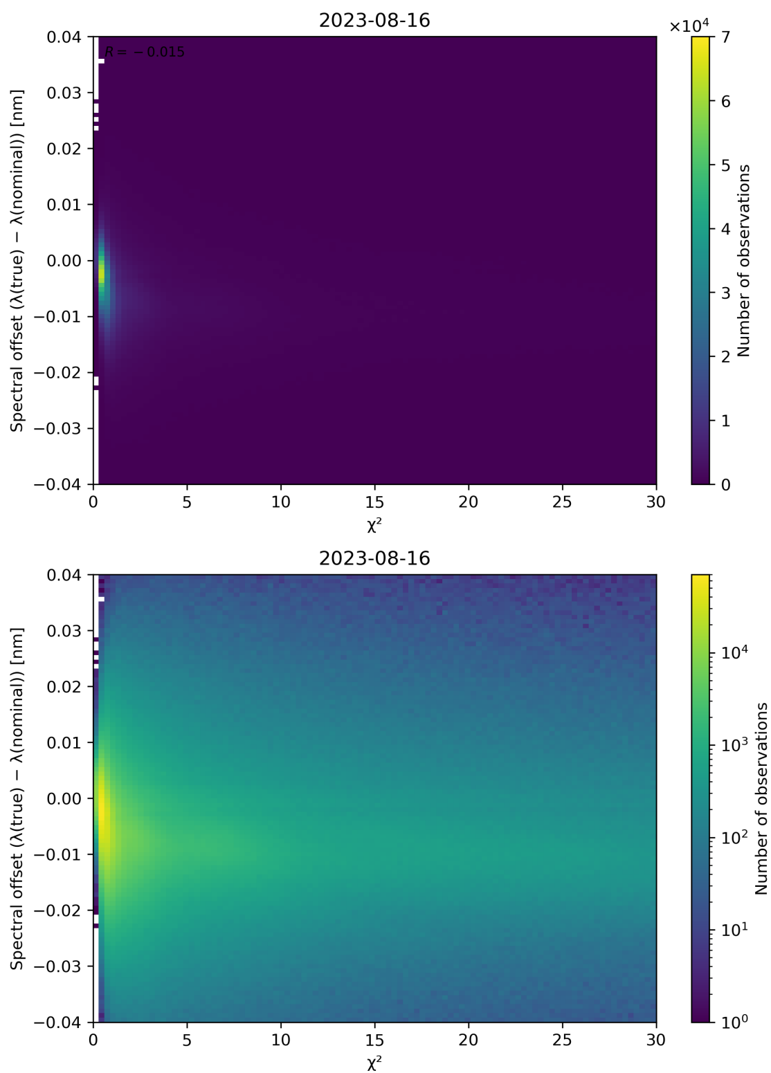
Figure 75: Scatter density plot of “ \chi^2 ” against “Spectral offset ( \lambda(\text{true}) - \lambda(\text{nominal}) )” for 2023-08-15 to 2023-08-17.
