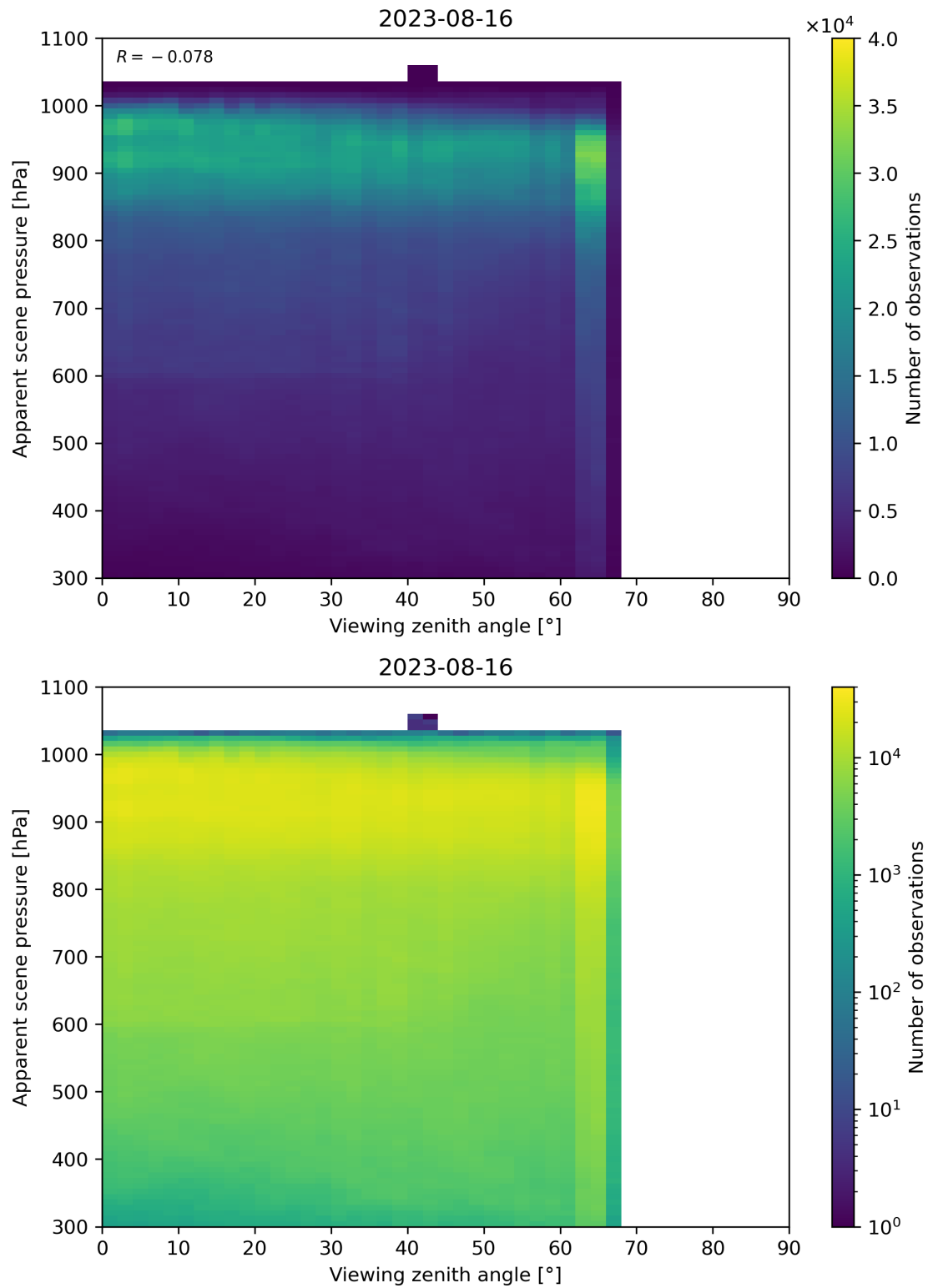
Figure 129: Scatter density plot of “Viewing zenith angle” against “Apparent scene pressure” for 2023-08-15 to 2023-08-17.
