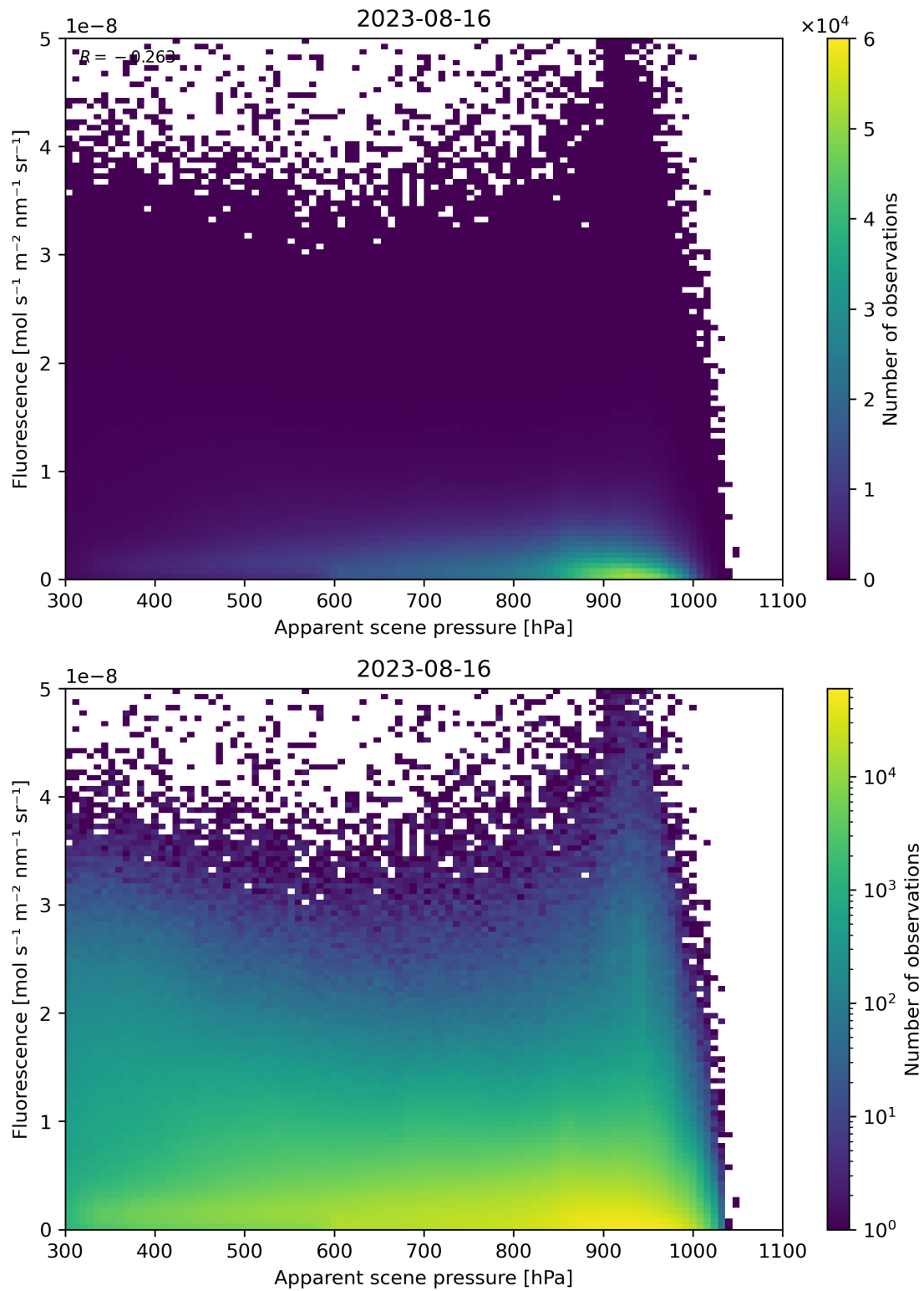
Figure 65: Scatter density plot of “Apparent scene pressure” against “Fluorescence” for 2023-08-15 to 2023-08-17.
