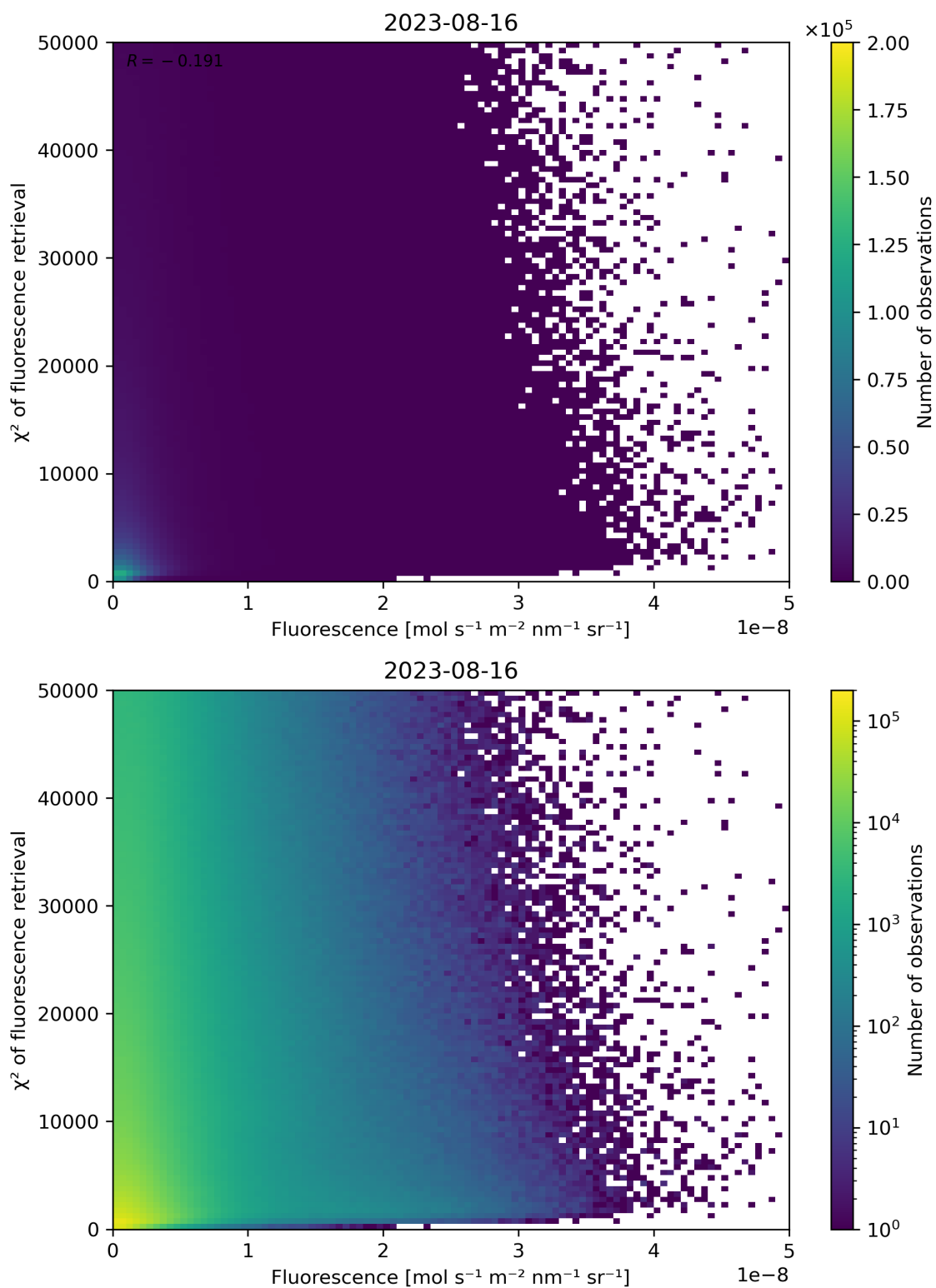
Figure 93: Scatter density plot of “Fluorescence” against “ \chi^2 of fluorescence retrieval” for 2023-08-15 to 2023-08-17.
