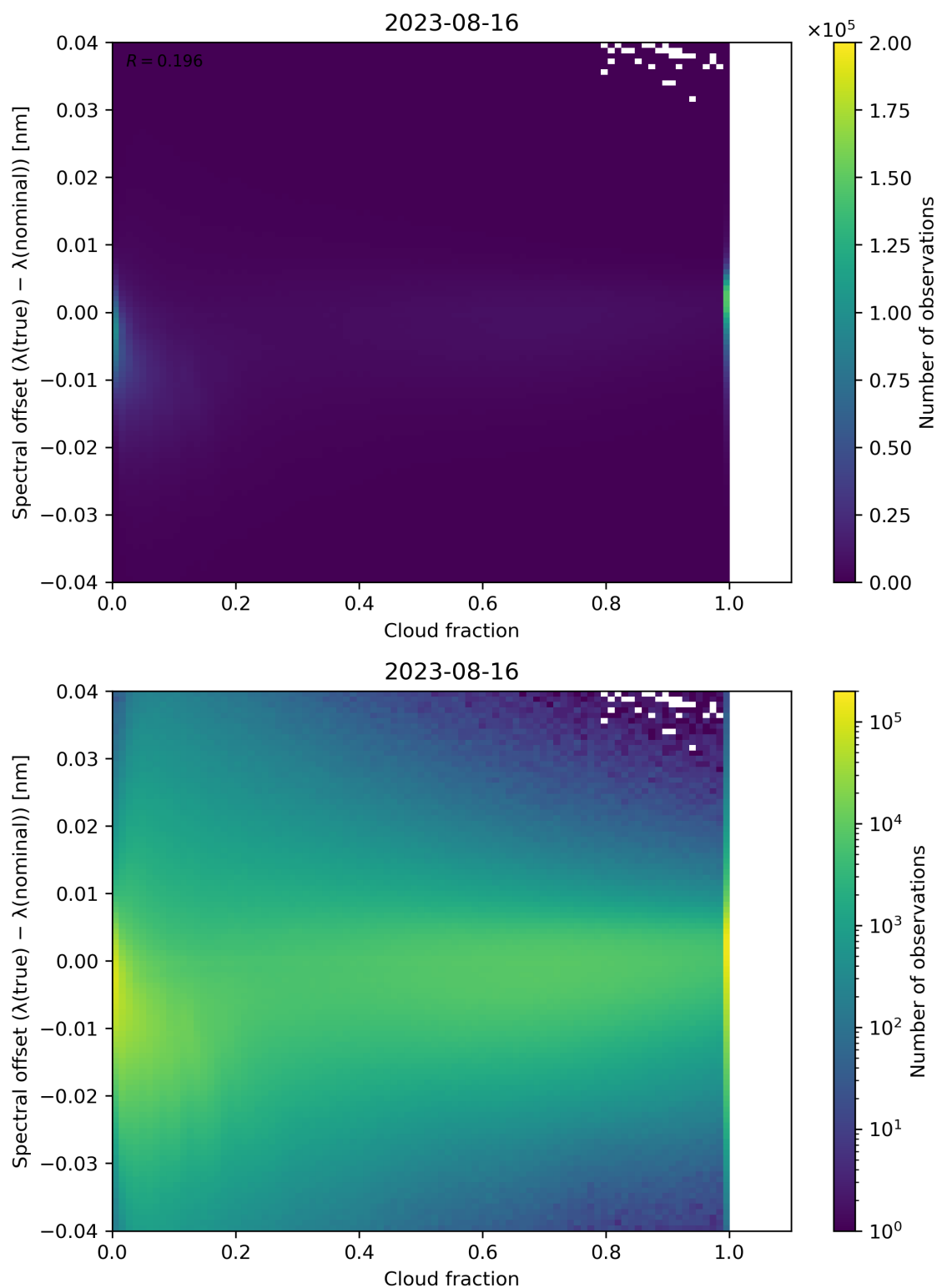
Figure 83: Scatter density plot of “Cloud fraction” against “Spectral offset ( \lambda(\text{true}) - \lambda(\text{nominal}) )” for 2023-08-15 to 2023-08-17.
