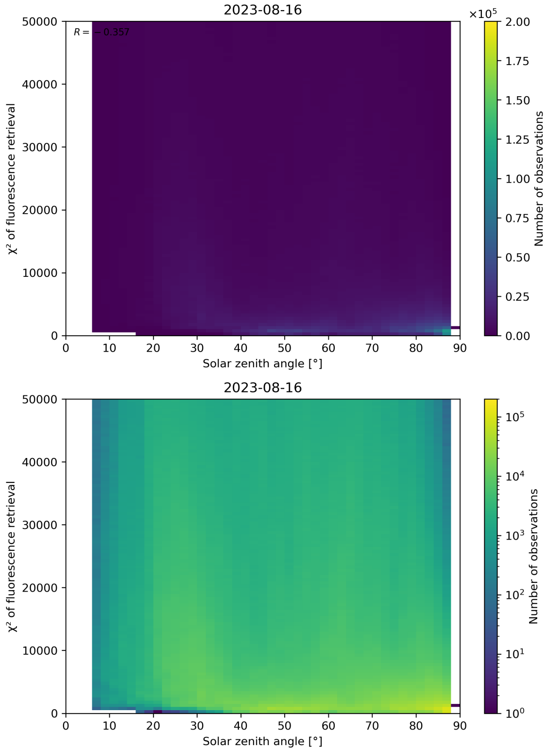
Figure 120: Scatter density plot of “Solar zenith angle” against “ \chi^2 of fluorescence retrieval” for 2023-08-15 to 2023-08-17.
