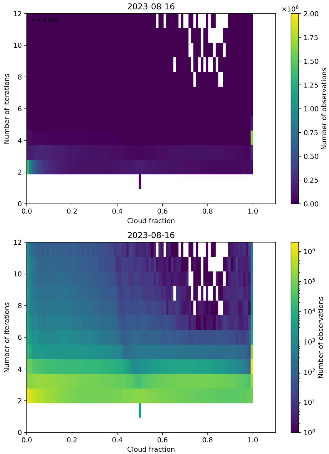
Figure 80: Scatter density plot of “Cloud fraction” against “Number of iterations” for 2023-08-15 to 2023-08-17.
