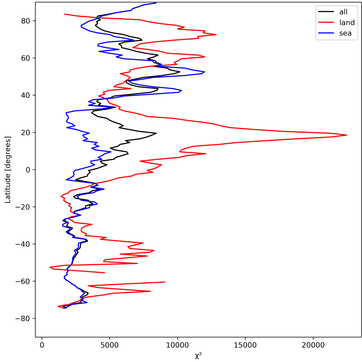
Figure 21: Zonal average of “ \chi^2 ” for 2023-08-15 to 2023-08-17.
