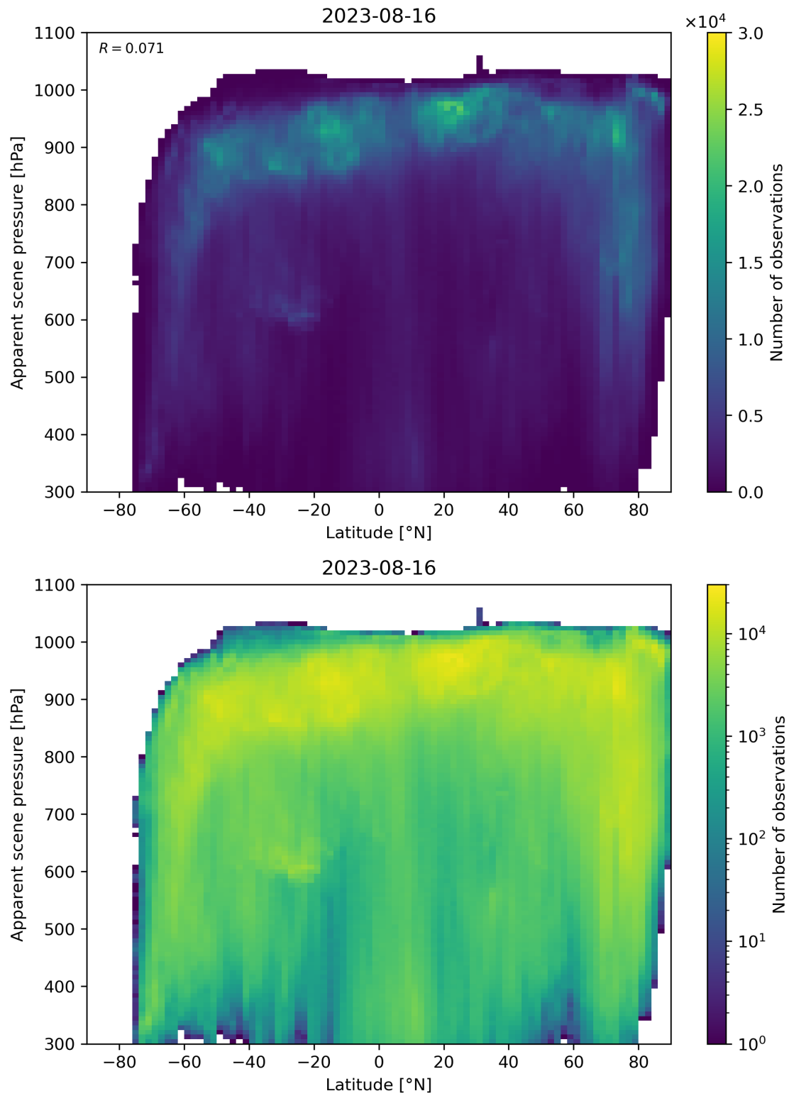
Figure 96: Scatter density plot of “Latitude” against “Apparent scene pressure” for 2023-08-15 to 2023-08-17.
