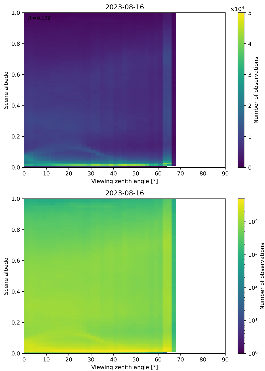
Figure 138: Scatter density plot of “Viewing zenith angle” against “Scene albedo” for 2023-08-15 to 2023-08-17.
