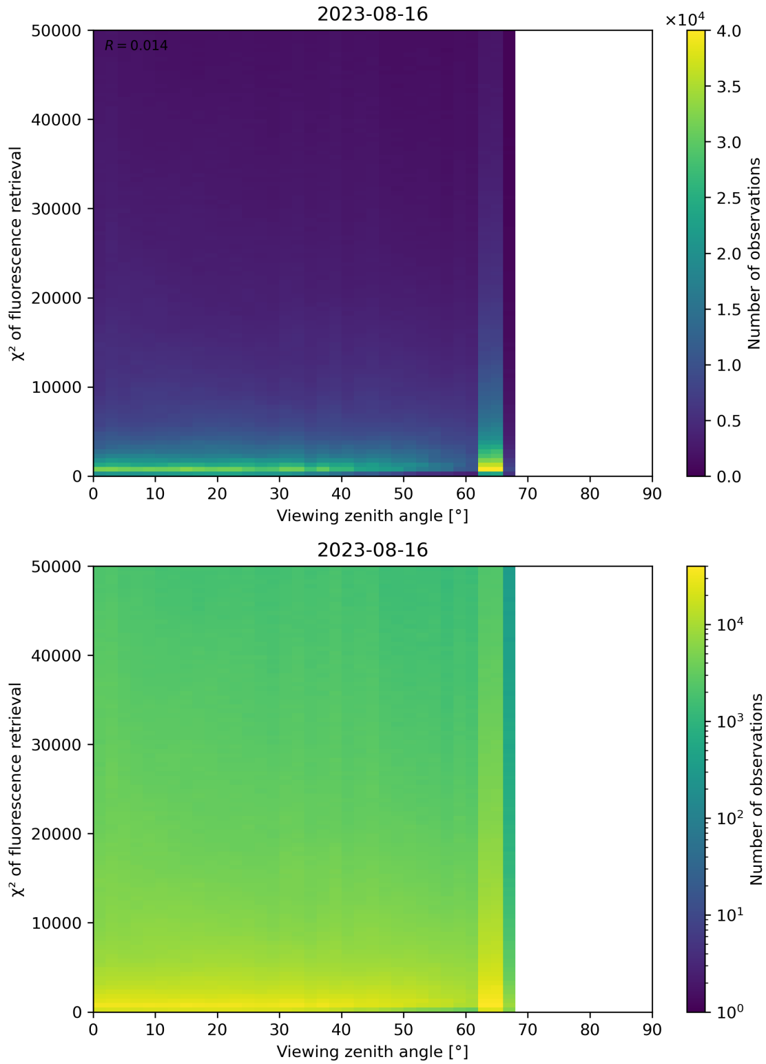
Figure 131: Scatter density plot of “Viewing zenith angle” against “ \chi^2 of fluorescence retrieval” for 2023-08-15 to 2023-08-17.
