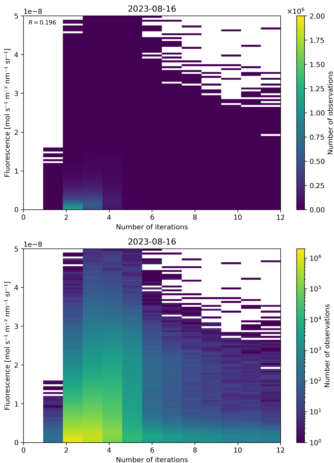
Figure 107: Scatter density plot of “Number of iterations” against “Fluorescence” for 2023-08-15 to 2023-08-17.
