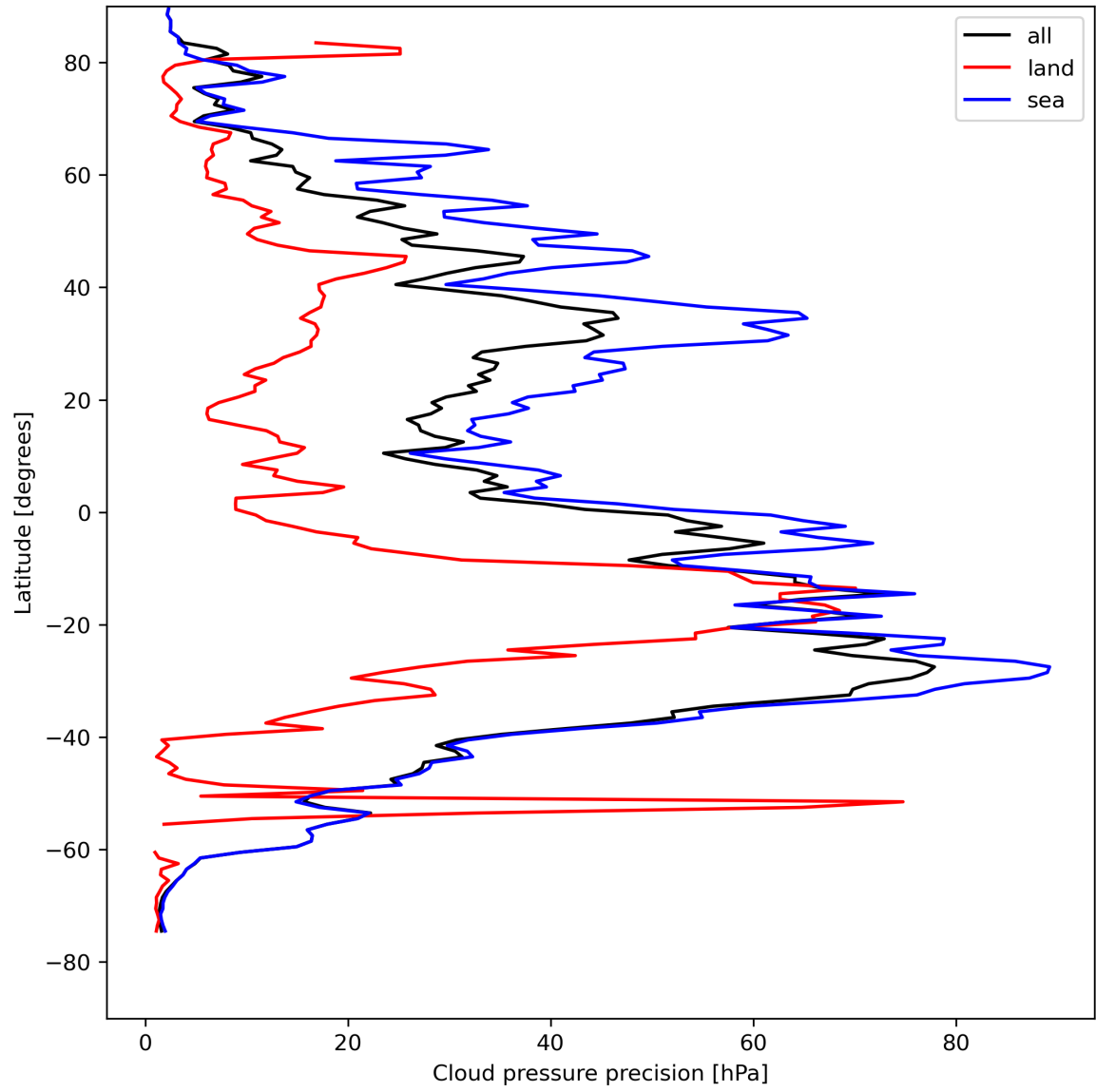
Figure 14: Zonal average of “Cloud pressure precision” for 2023-08-15 to 2023-08-17.
