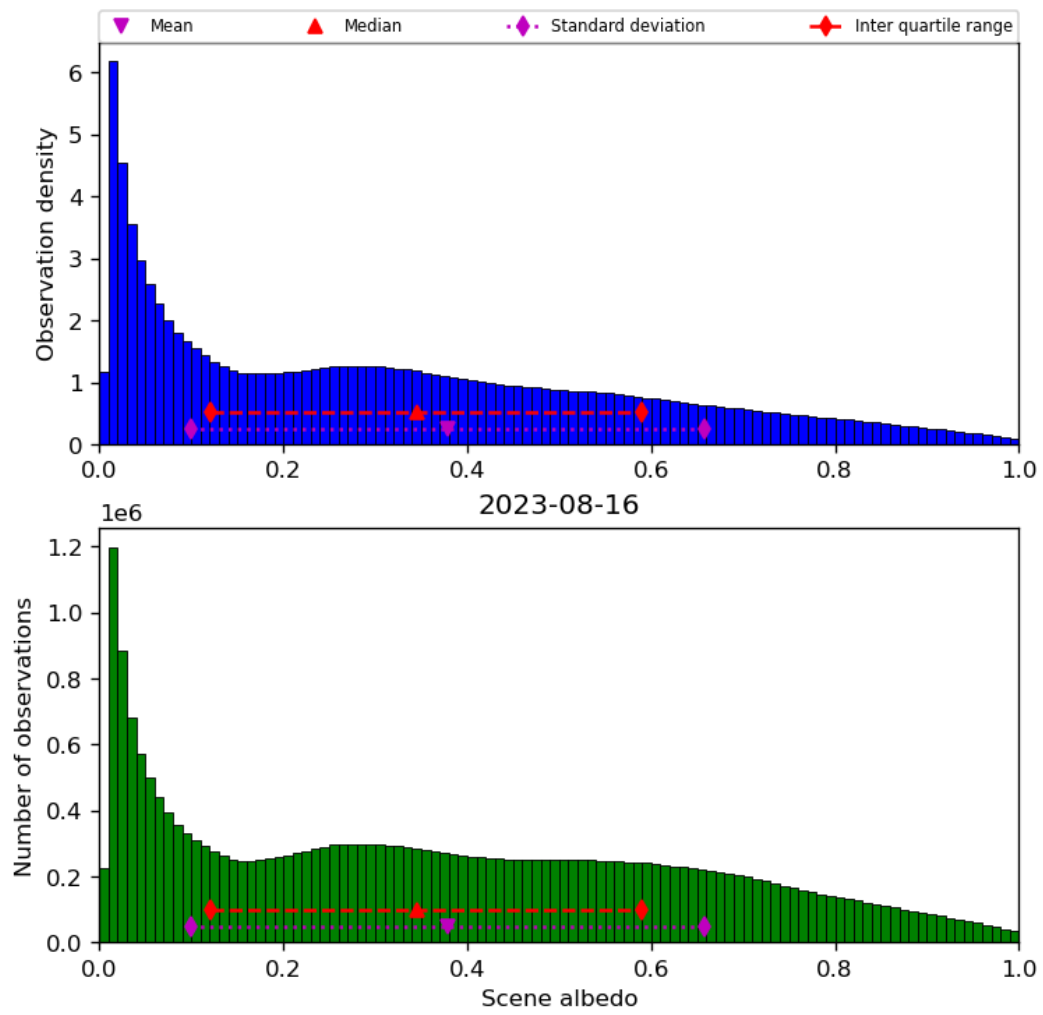
Figure 34: Histogram of “Scene albedo” for 2023-08-15 to 2023-08-17
