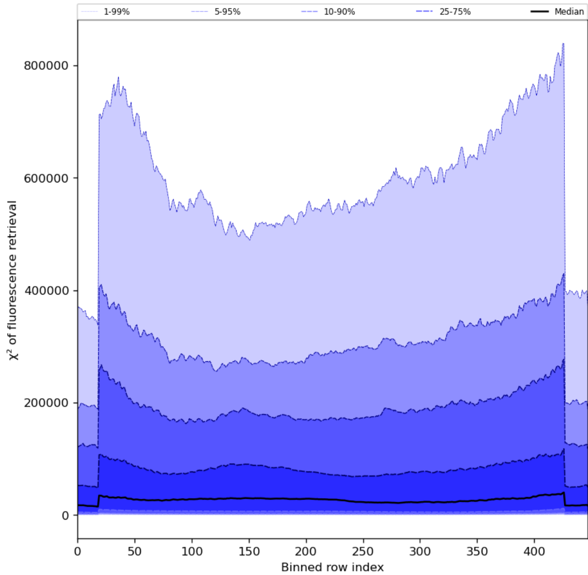
Figure 59: Along track statistics of “ \chi^2 of fluorescence retrieval” for 2023-08-15 to 2023-08-17
