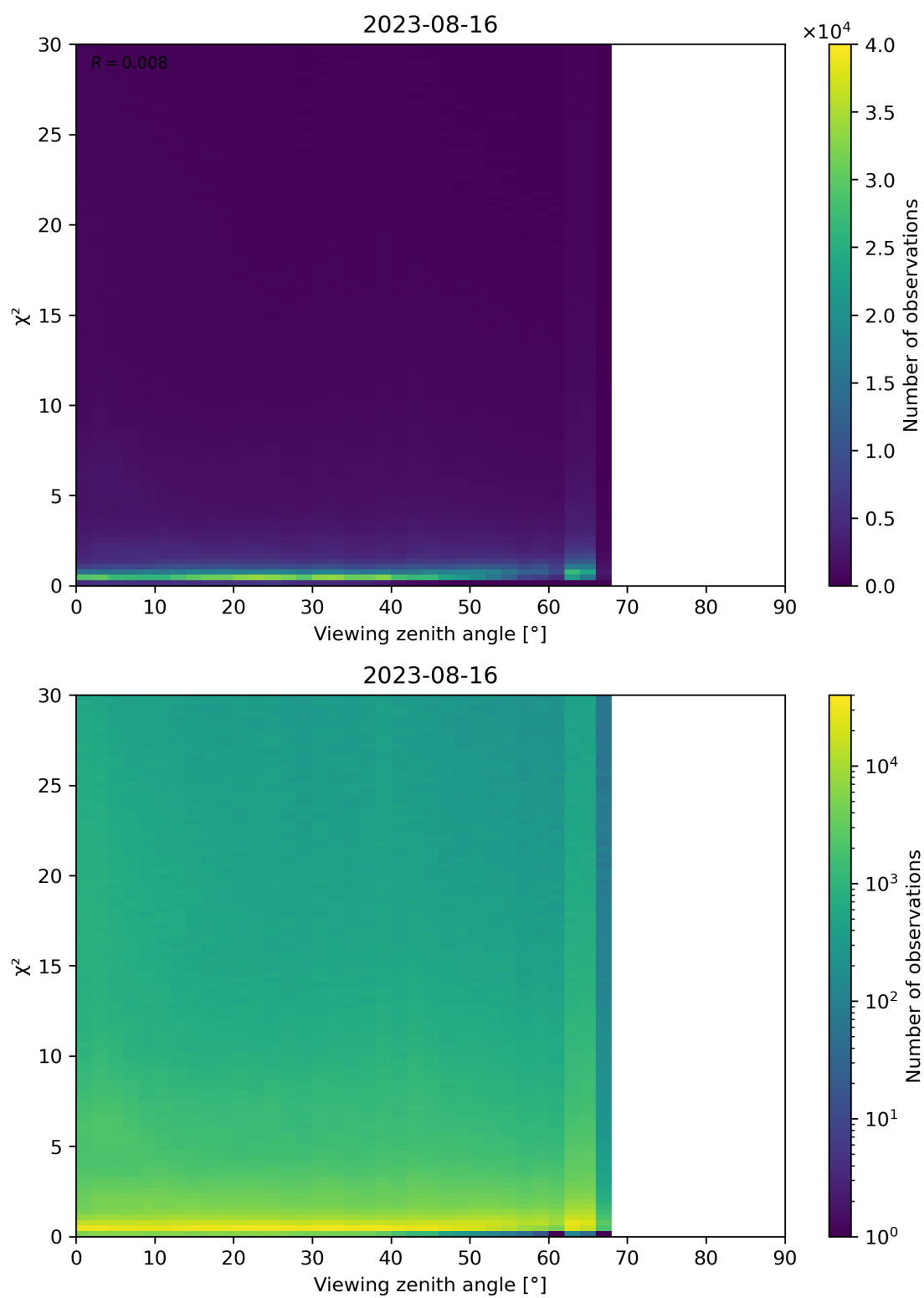
Figure 130: Scatter density plot of “Viewing zenith angle” against “ \chi^2 ” for 2023-08-15 to 2023-08-17.
