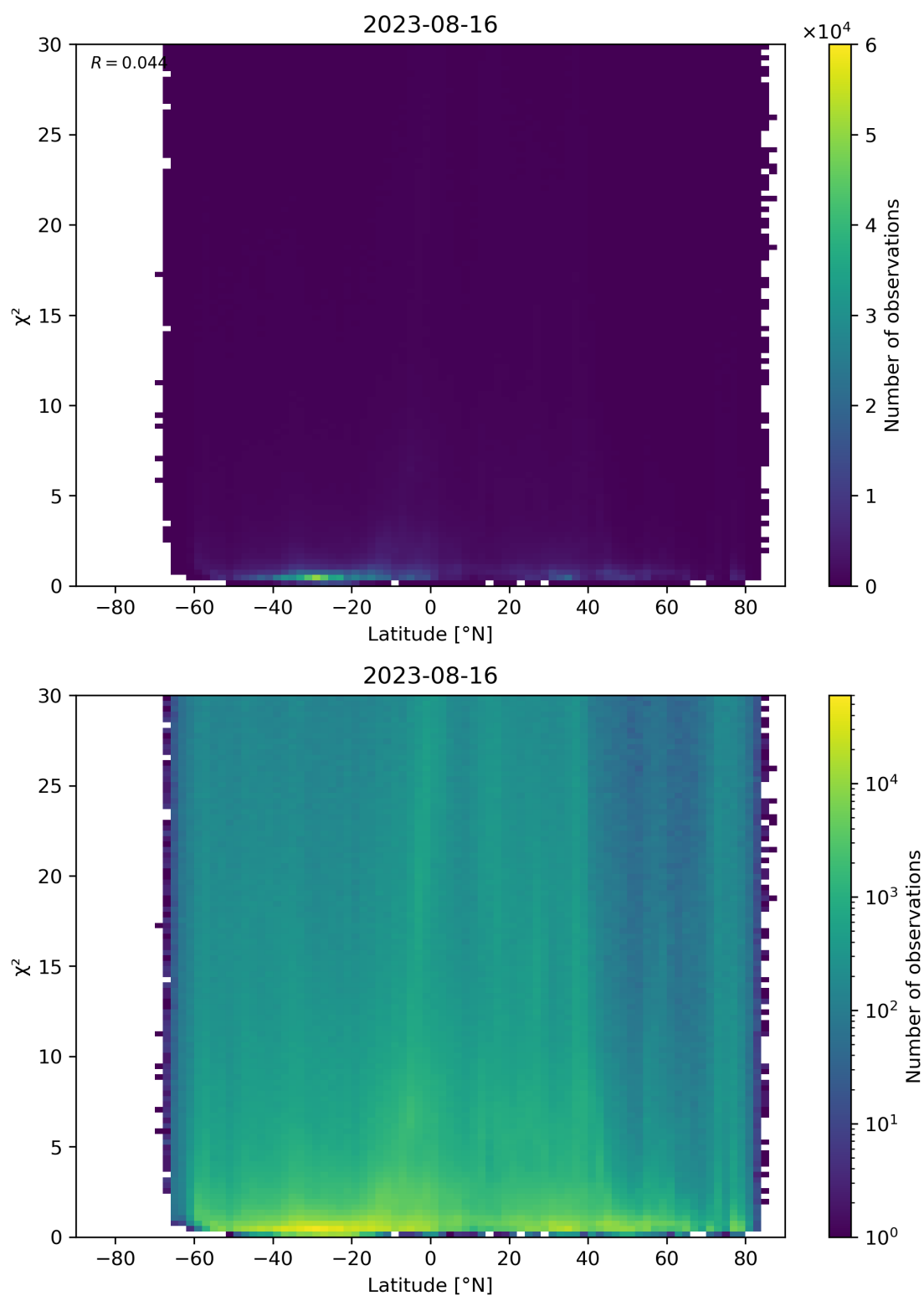
Figure 97: Scatter density plot of “Latitude” against “ \chi^2 ” for 2023-08-15 to 2023-08-17.
