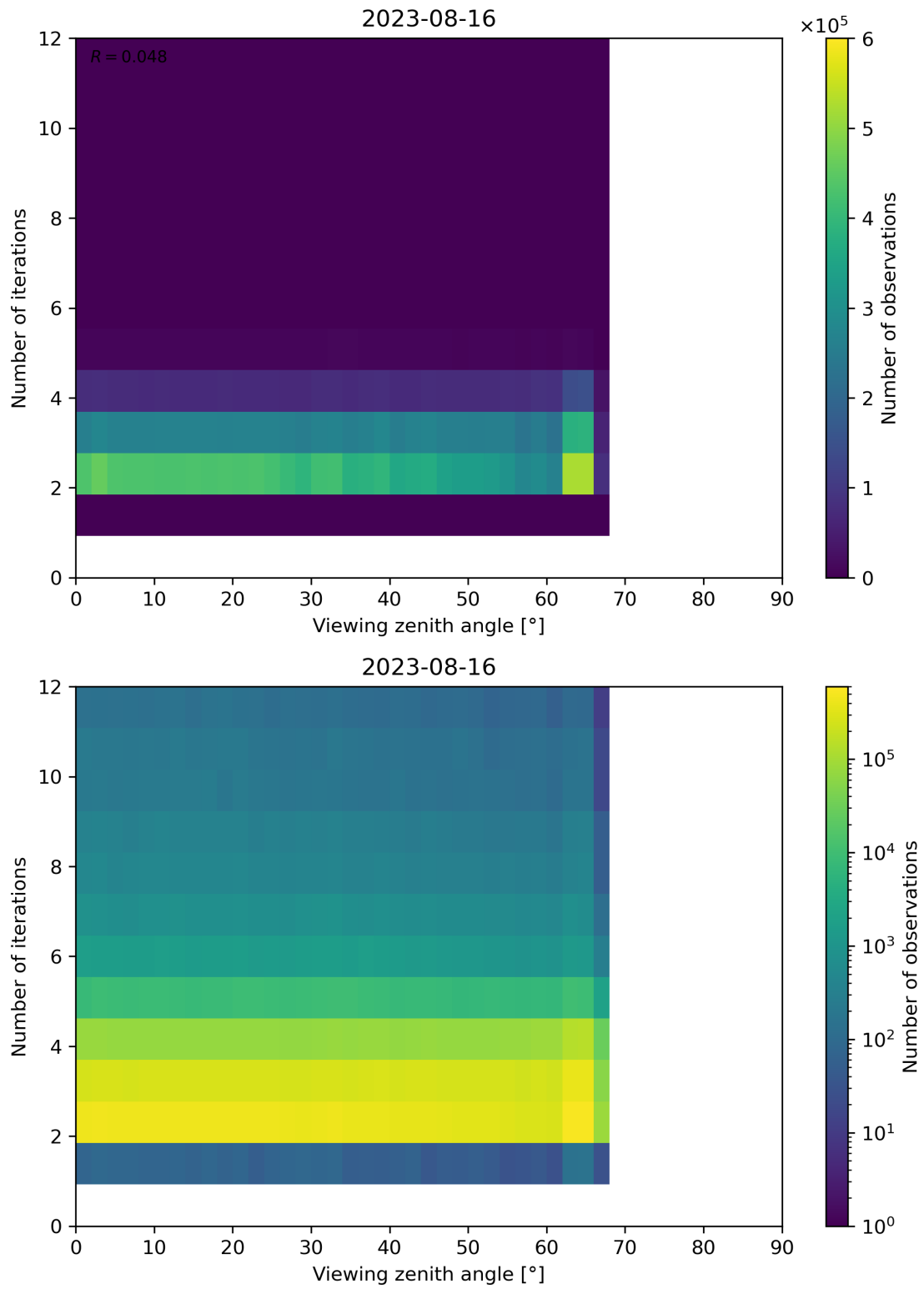
Figure 136: Scatter density plot of “Viewing zenith angle” against “Number of iterations” for 2023-08-15 to 2023-08-17.
