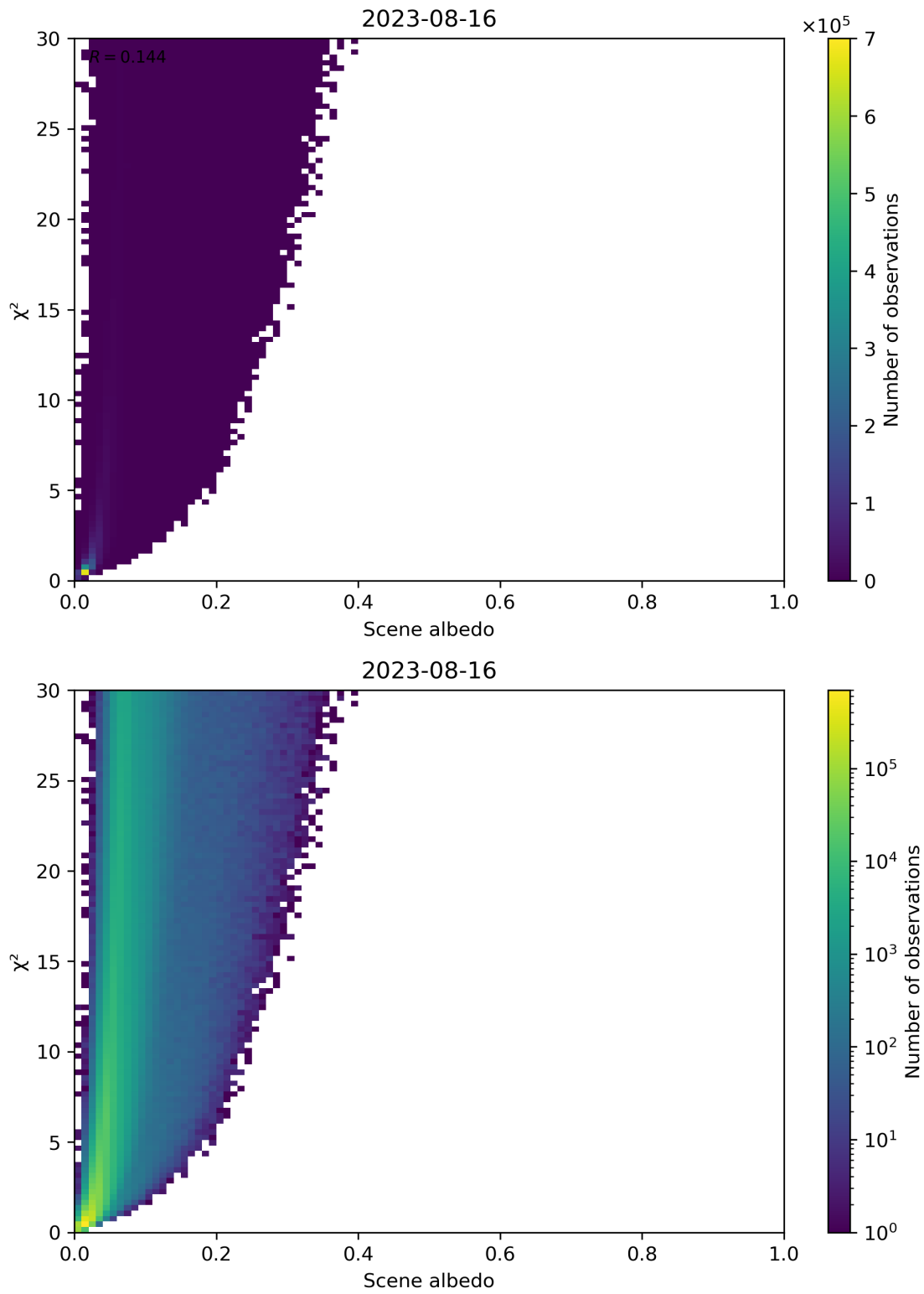
Figure 112: Scatter density plot of “Scene albedo” against “ \chi^2 ” for 2023-08-15 to 2023-08-17.
