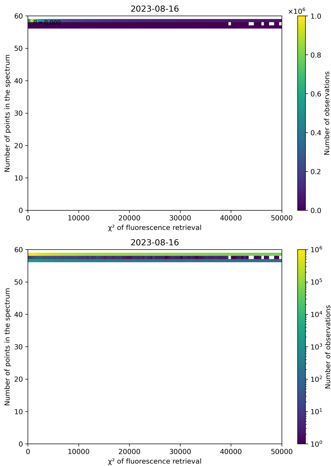
Figure 71: Scatter density plot of “ \chi^2 of fluorescence retrieval” against “Number of points in the spectrum” for 2023-08-15 to 2023-08-17.
