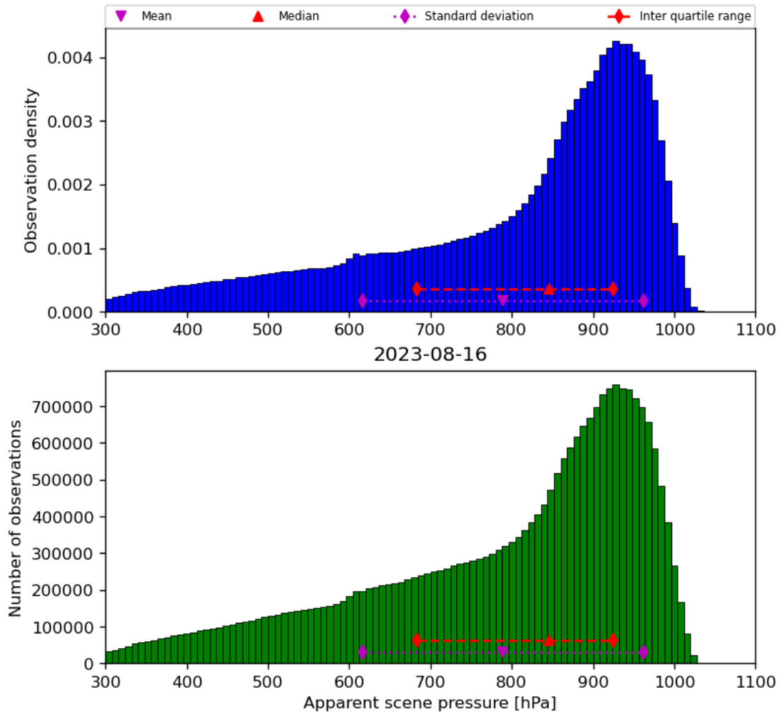
Figure 36: Histogram of “Apparent scene pressure” for 2023-08-15 to 2023-08-17
