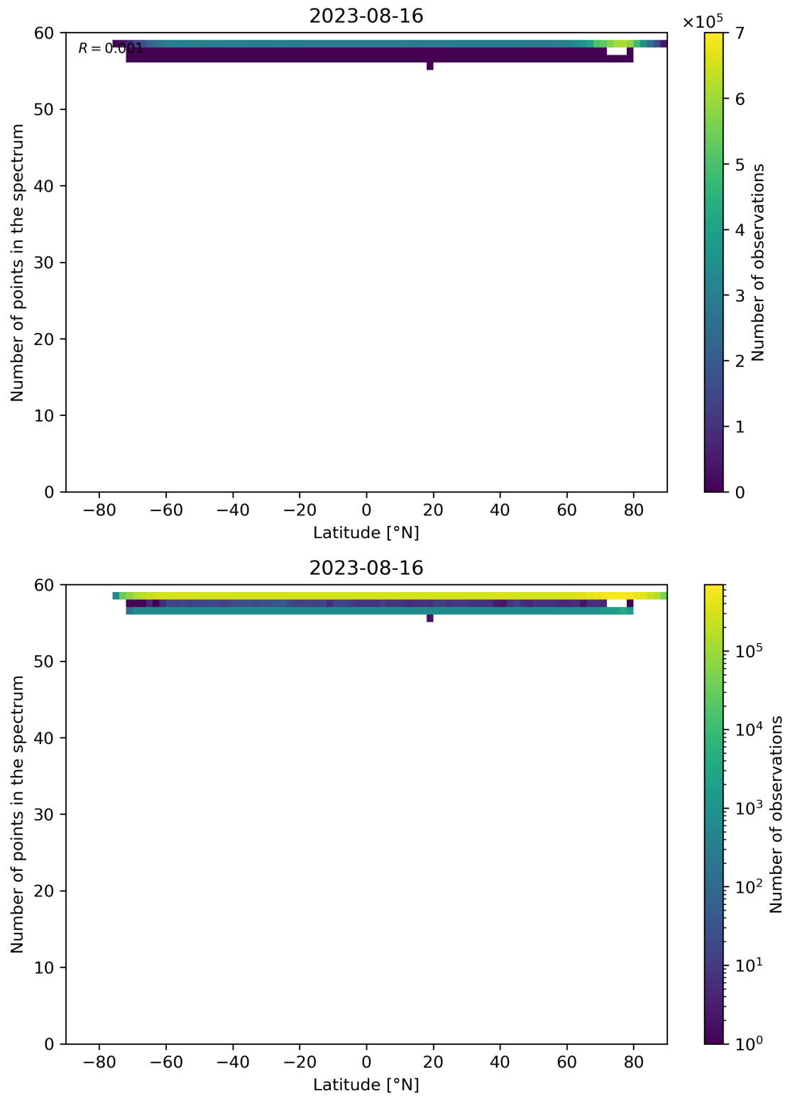
Figure 103: Scatter density plot of “Latitude” against “Number of points in the spectrum” for 2023-08-15 to 2023-08-17.
