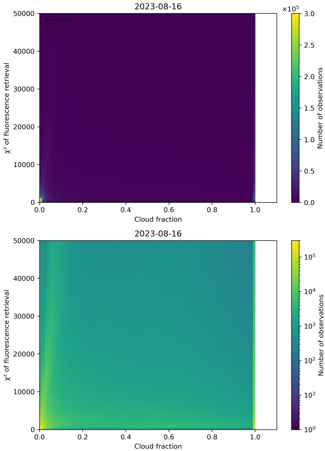
Figure 78: Scatter density plot of “Cloud fraction” against “ \chi^2 of fluorescence retrieval” for 2023-08-15 to 2023-08-17.
