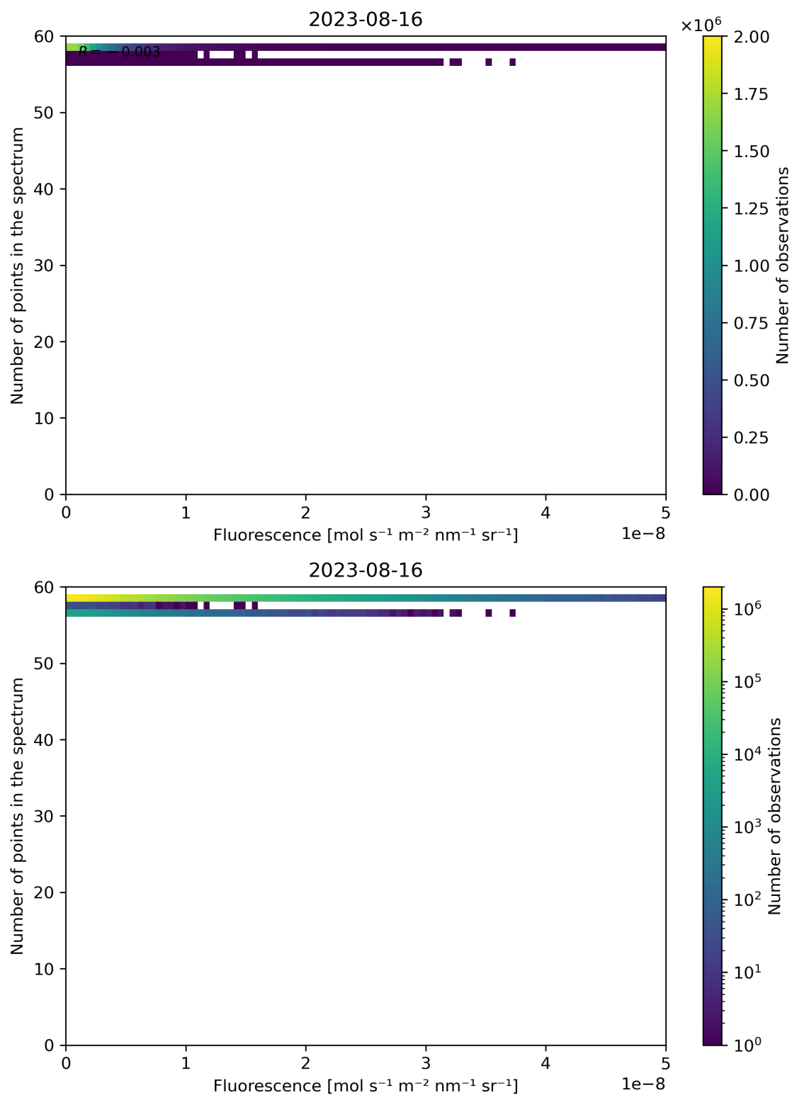
Figure 94: Scatter density plot of “Fluorescence” against “Number of points in the spectrum” for 2023-08-15 to 2023-08-17.
