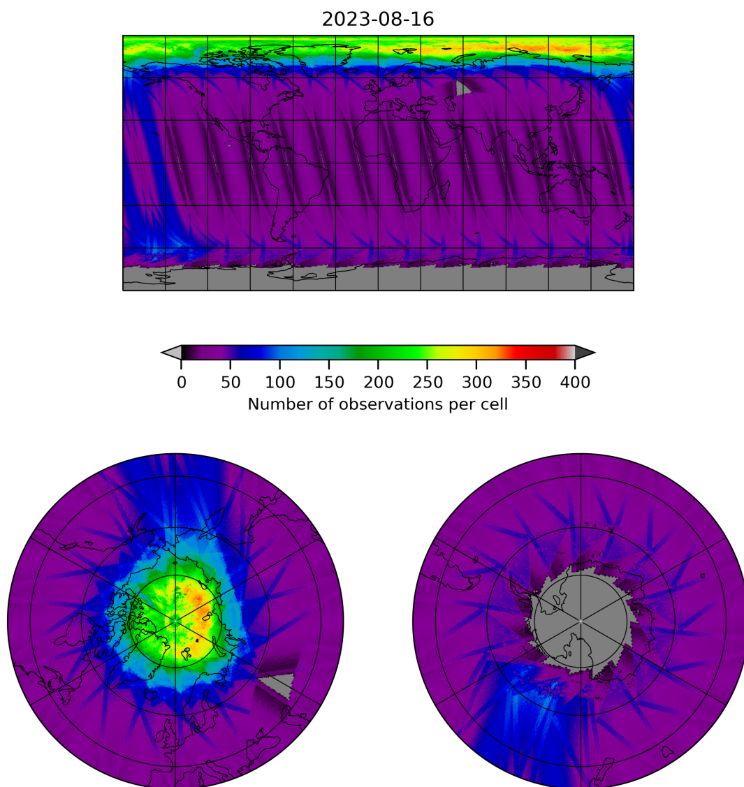
Figure 11: Map of the number of observations for 2023-08-15 to 2023-08-17
