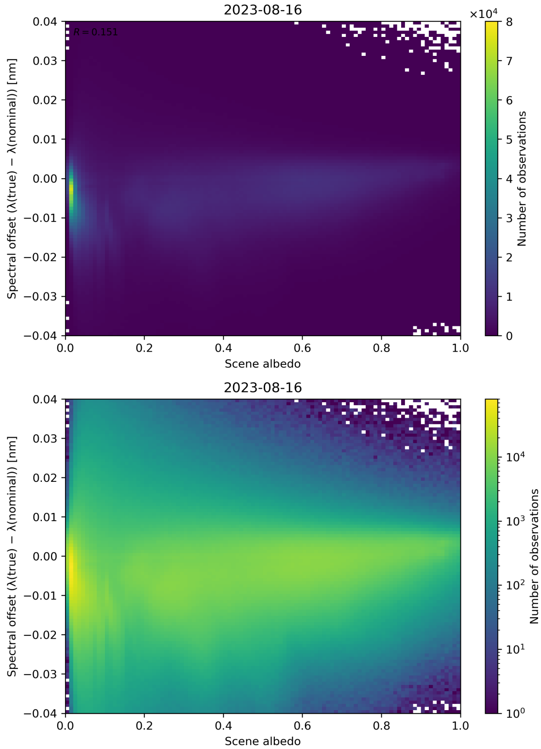
Figure 117: Scatter density plot of “Scene albedo” against “Spectral offset ( \lambda(\text{true}) - \lambda(\text{nominal}) )” for 2023-08-15 to 2023-08-17.
