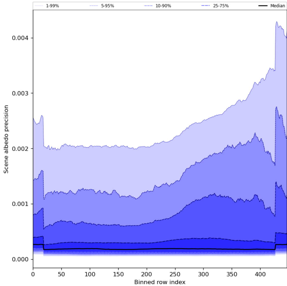
Figure 52: Along track statistics of “Scene albedo precision” for 2023-08-15 to 2023-08-17
