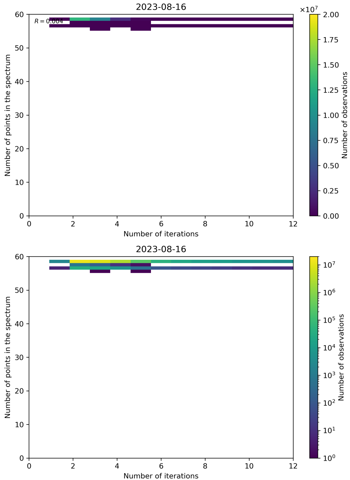
Figure 108: Scatter density plot of “Number of iterations” against “Number of points in the spectrum” for 2023-08-15 to 2023-08-17.
