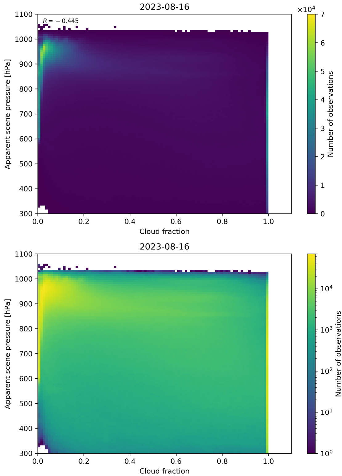
Figure 76: Scatter density plot of “Cloud fraction” against “Apparent scene pressure” for 2023-08-15 to 2023-08-17.
