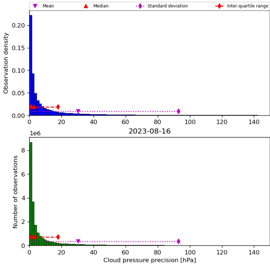
Figure 31: Histogram of “Cloud pressure precision” for 2023-08-15 to 2023-08-17
