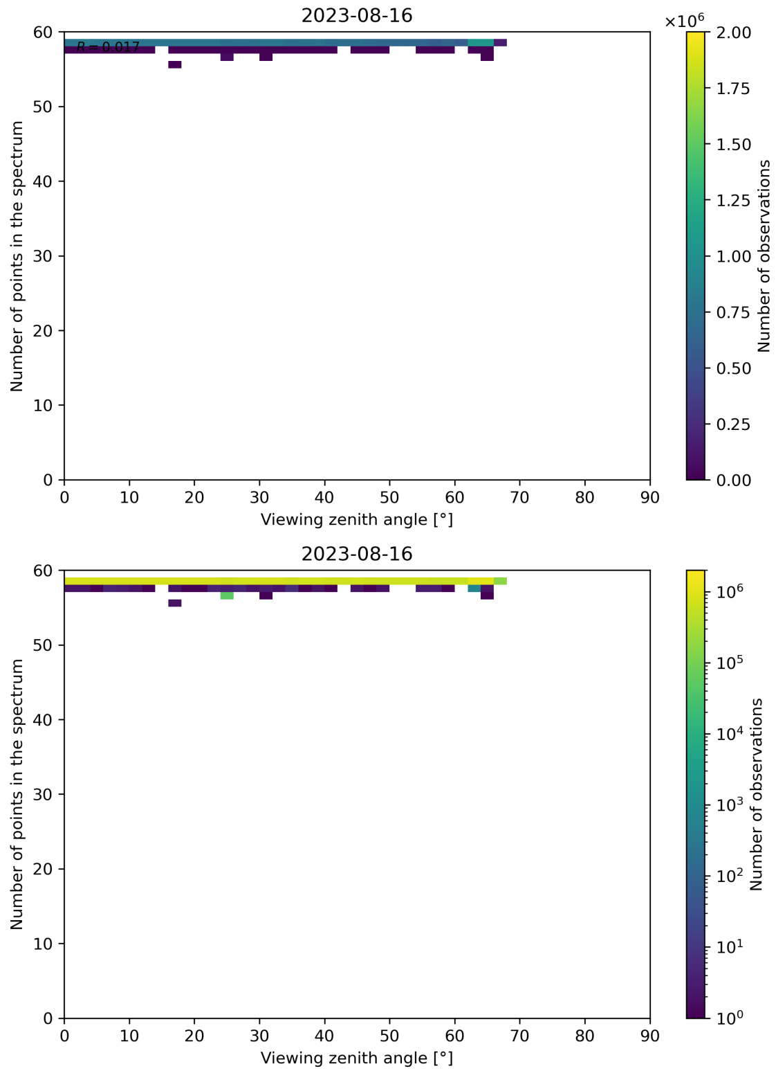
Figure 137: Scatter density plot of “Viewing zenith angle” against “Number of points in the spectrum” for 2023-08-15 to 2023-08-17.
