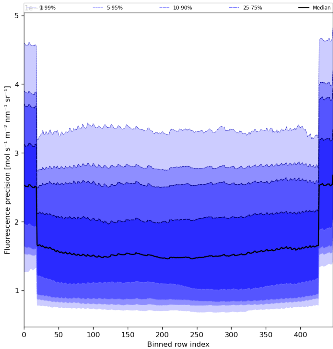
Figure 58: Along track statistics of “Fluorescence precision” for 2023-08-15 to 2023-08-17
