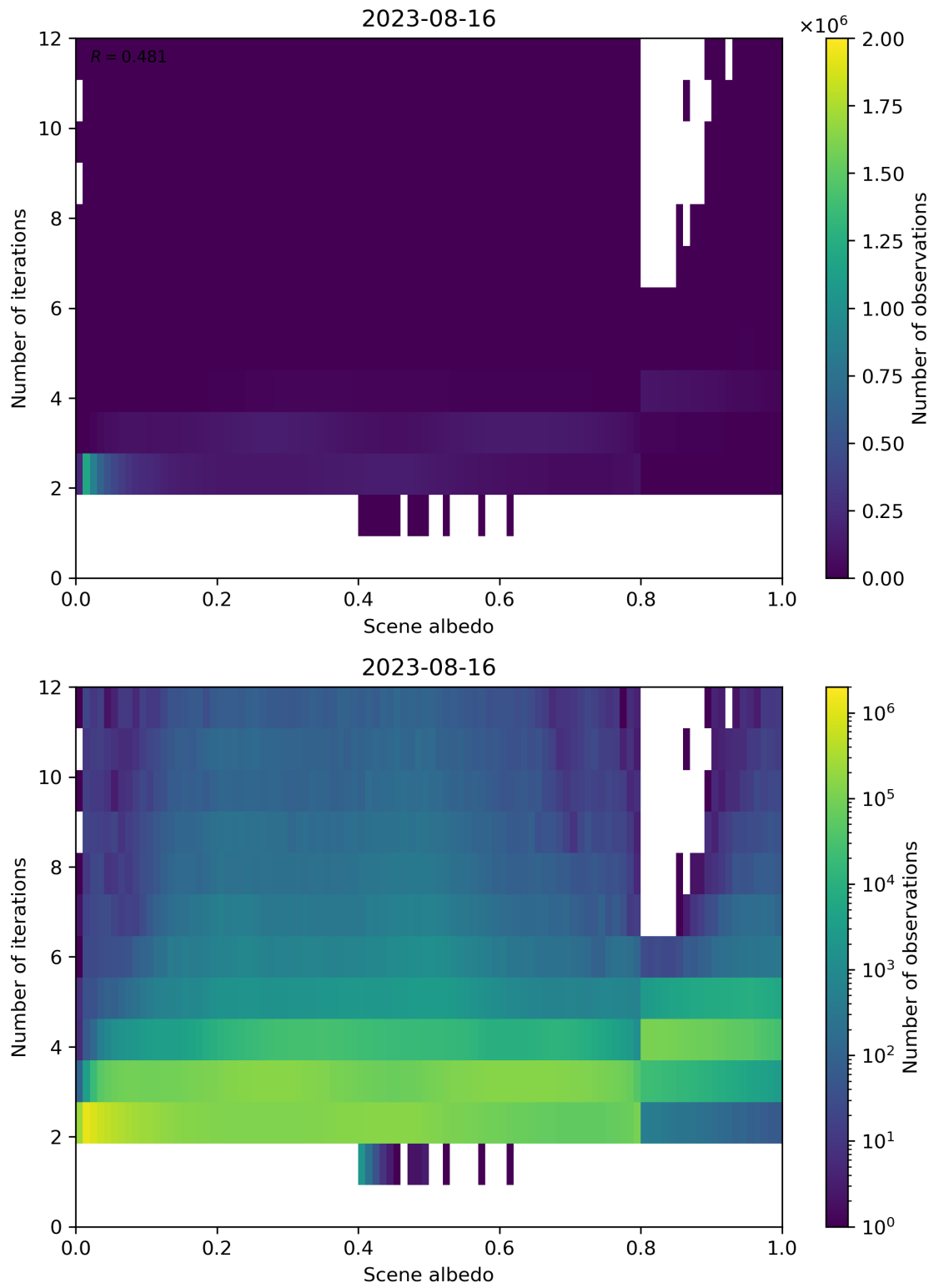
Figure 115: Scatter density plot of “Scene albedo” against “Number of iterations” for 2023-08-15 to 2023-08-17.
