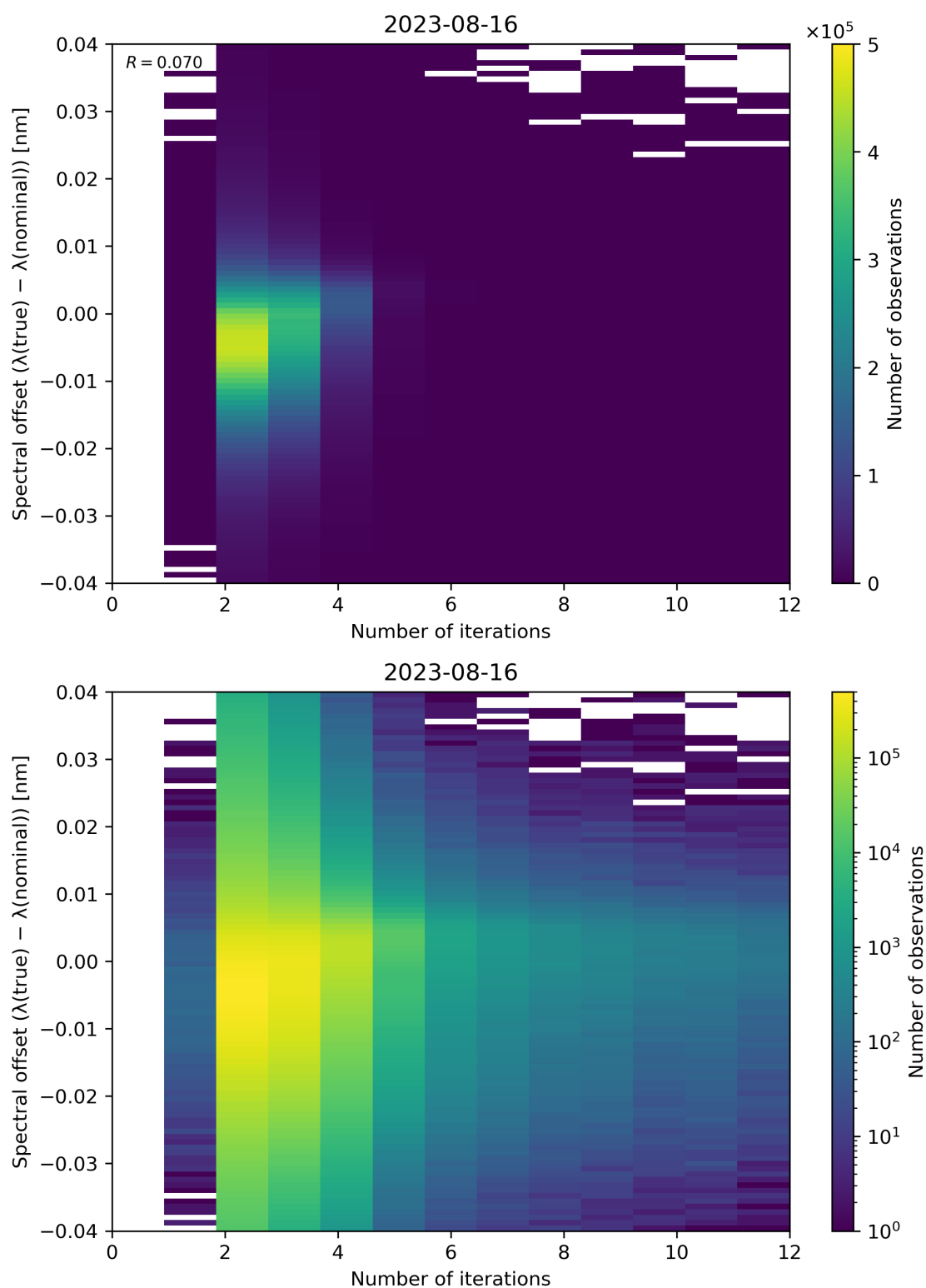
Figure 109: Scatter density plot of “Number of iterations” against “Spectral offset ( \lambda(\text{true}) - \lambda(\text{nominal}) )” for 2023-08-15 to 2023-08-17.
