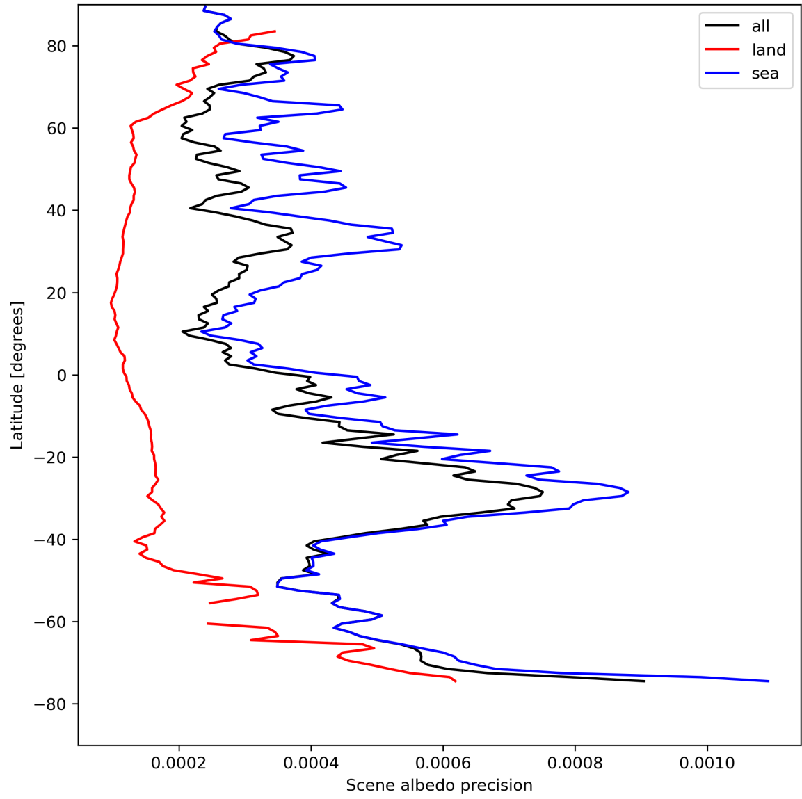
Figure 18: Zonal average of “Scene albedo precision” for 2023-08-15 to 2023-08-17.
