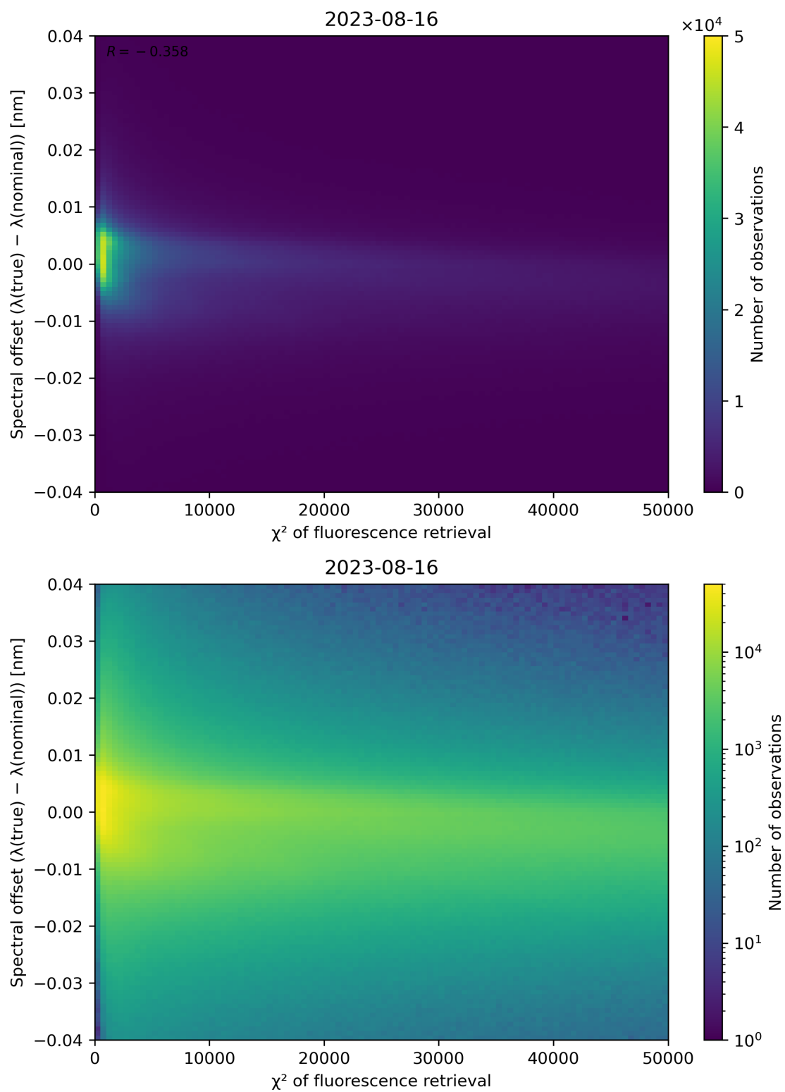
Figure 72: Scatter density plot of “ \chi^2 of fluorescence retrieval” against “Spectral offset ( \lambda(\text{true}) - \lambda(\text{nominal}) )” for 2023-08-15 to 2023-08-17.
