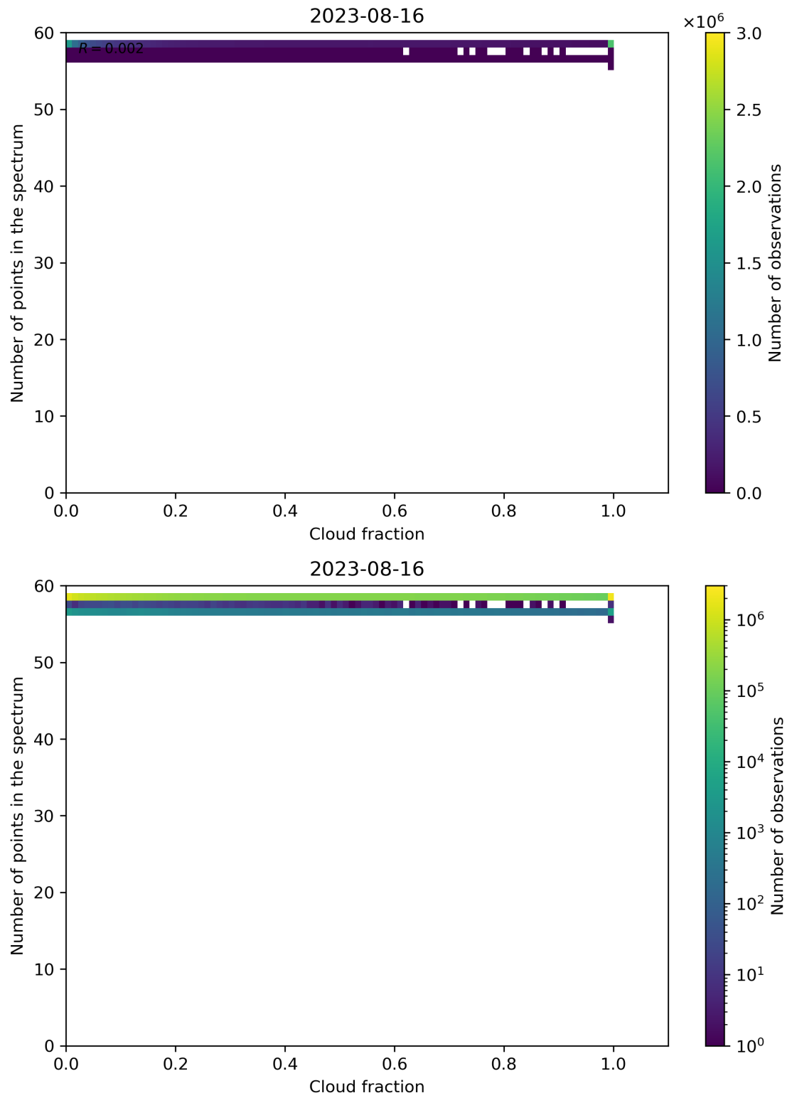
Figure 81: Scatter density plot of “Cloud fraction” against “Number of points in the spectrum” for 2023-08-15 to 2023-08-17.
