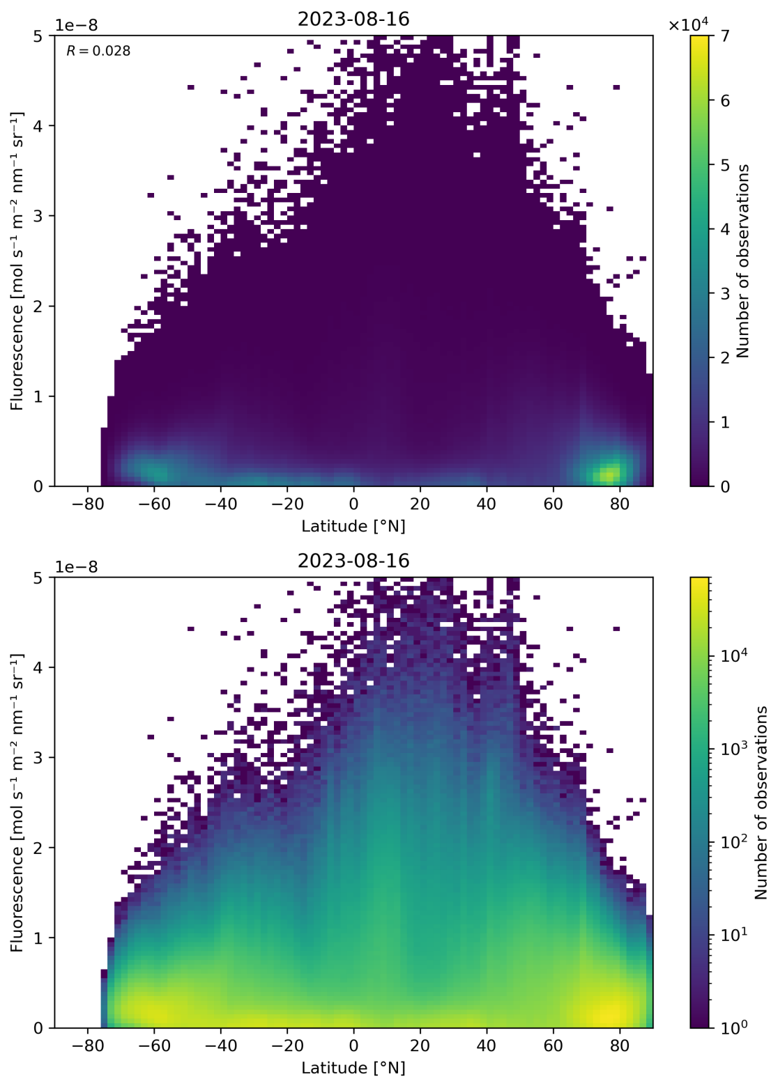
Figure 101: Scatter density plot of “Latitude” against “Fluorescence” for 2023-08-15 to 2023-08-17.
