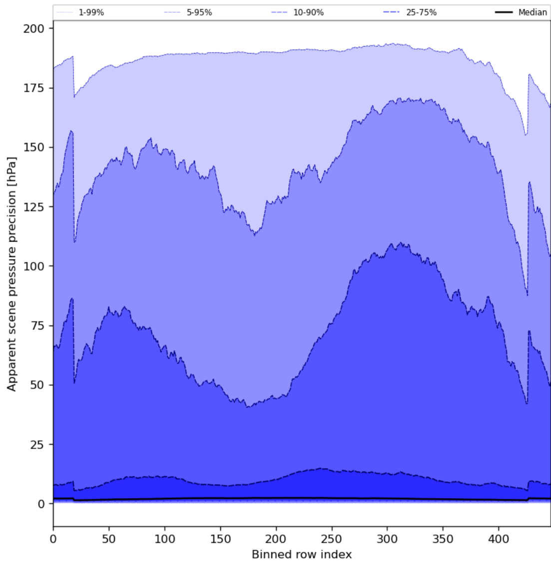
Figure 54: Along track statistics of “Apparent scene pressure precision” for 2023-08-15 to 2023-08-17
