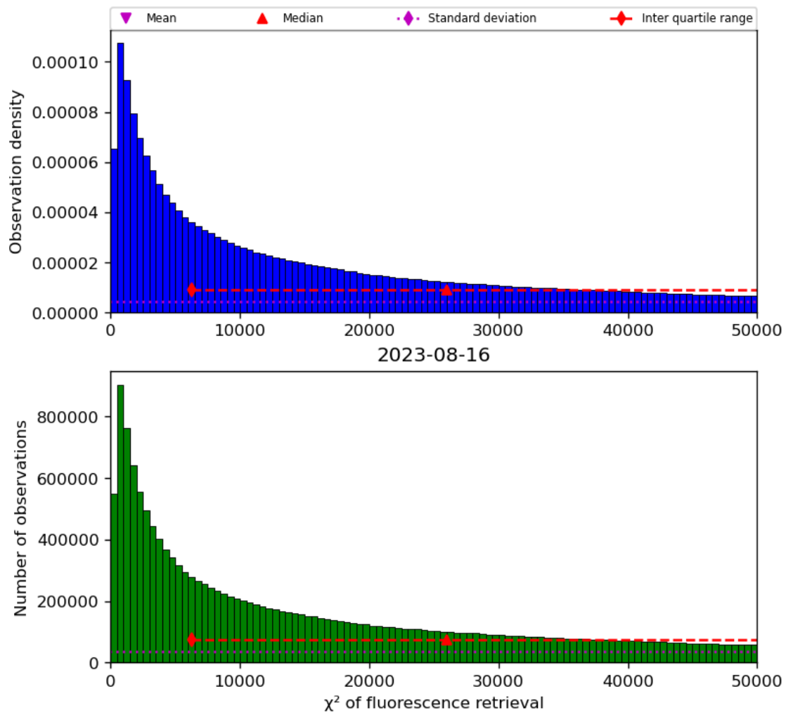
Figure 42: Histogram of “ \chi^2 of fluorescence retrieval” for 2023-08-15 to 2023-08-17
