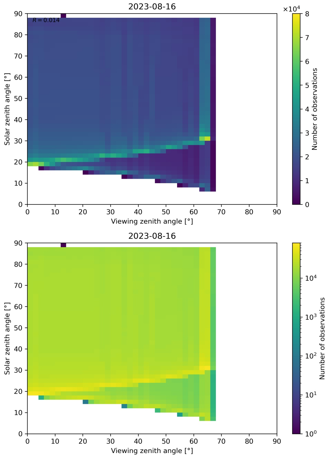
Figure 139: Scatter density plot of “Viewing zenith angle” against “Solar zenith angle” for 2023-08-15 to 2023-08-17.
