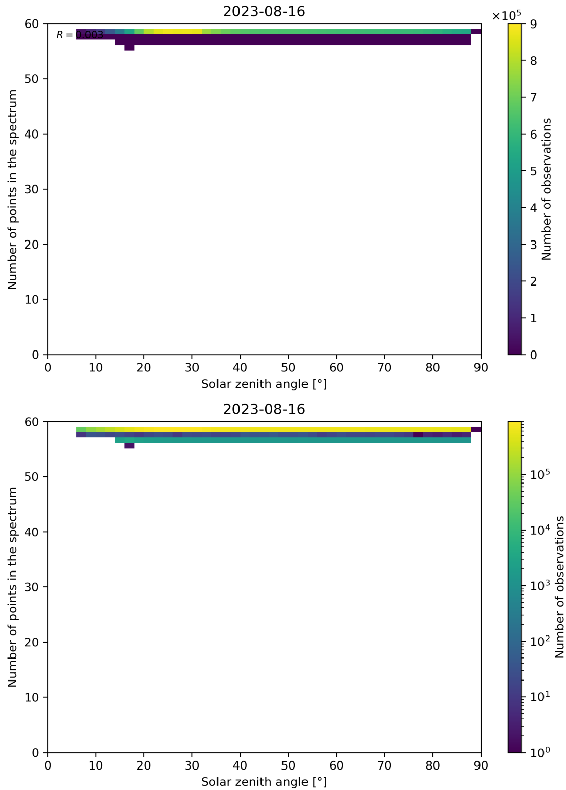
Figure 126: Scatter density plot of “Solar zenith angle” against “Number of points in the spectrum” for 2023-08-15 to 2023-08-17.
