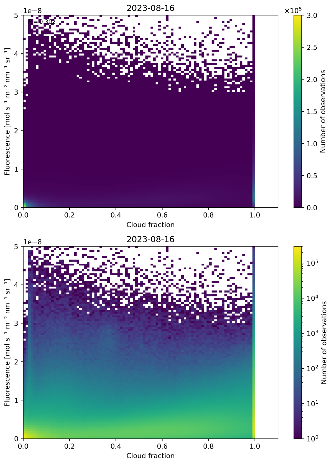
Figure 79: Scatter density plot of “Cloud fraction” against “Fluorescence” for 2023-08-15 to 2023-08-17.
