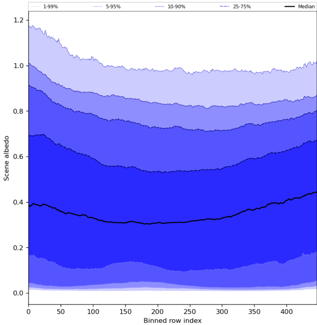
Figure 51: Along track statistics of “Scene albedo” for 2023-08-15 to 2023-08-17
