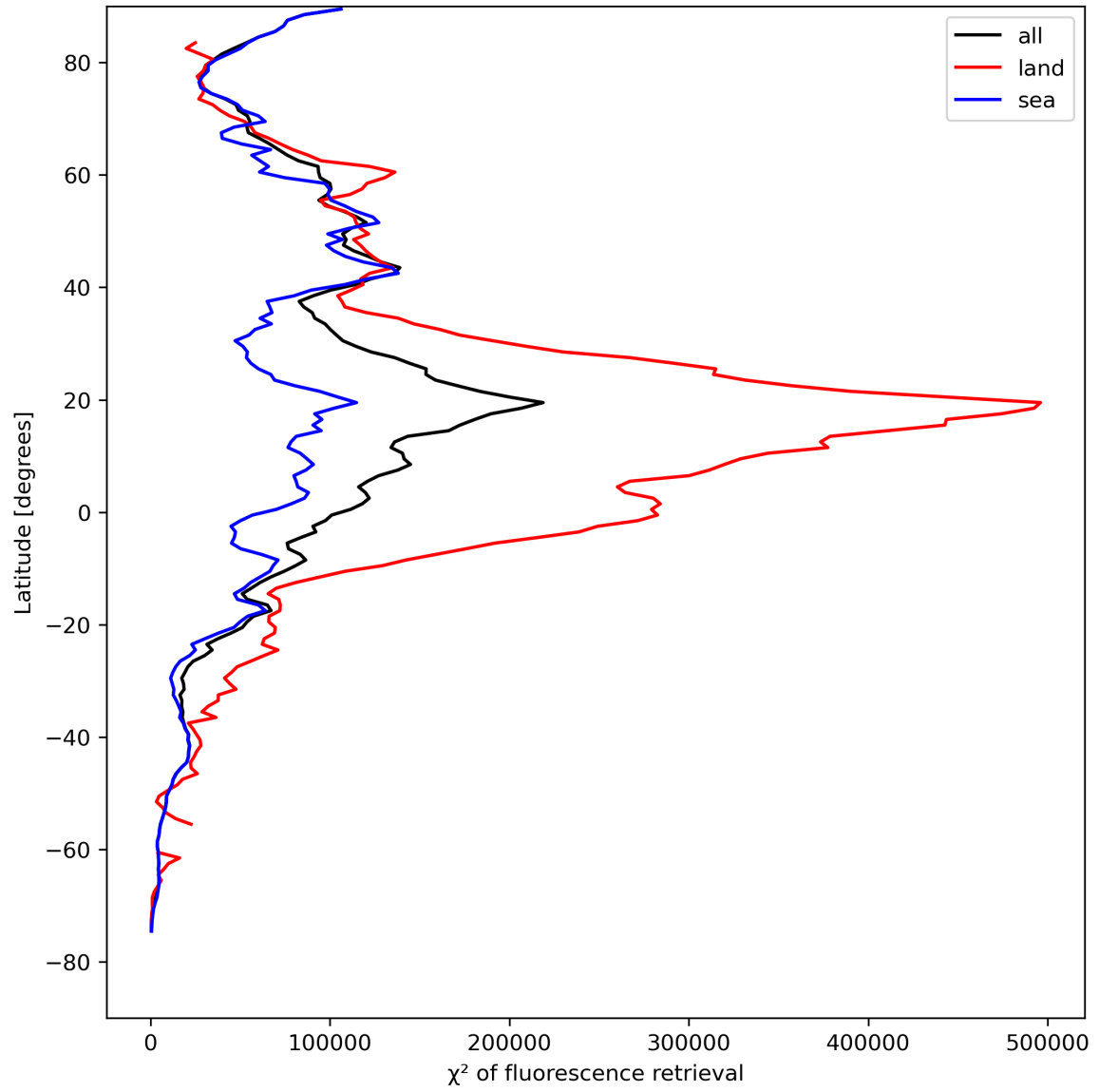
Figure 25: Zonal average of “ \chi^2 of fluorescence retrieval” for 2023-08-15 to 2023-08-17.
