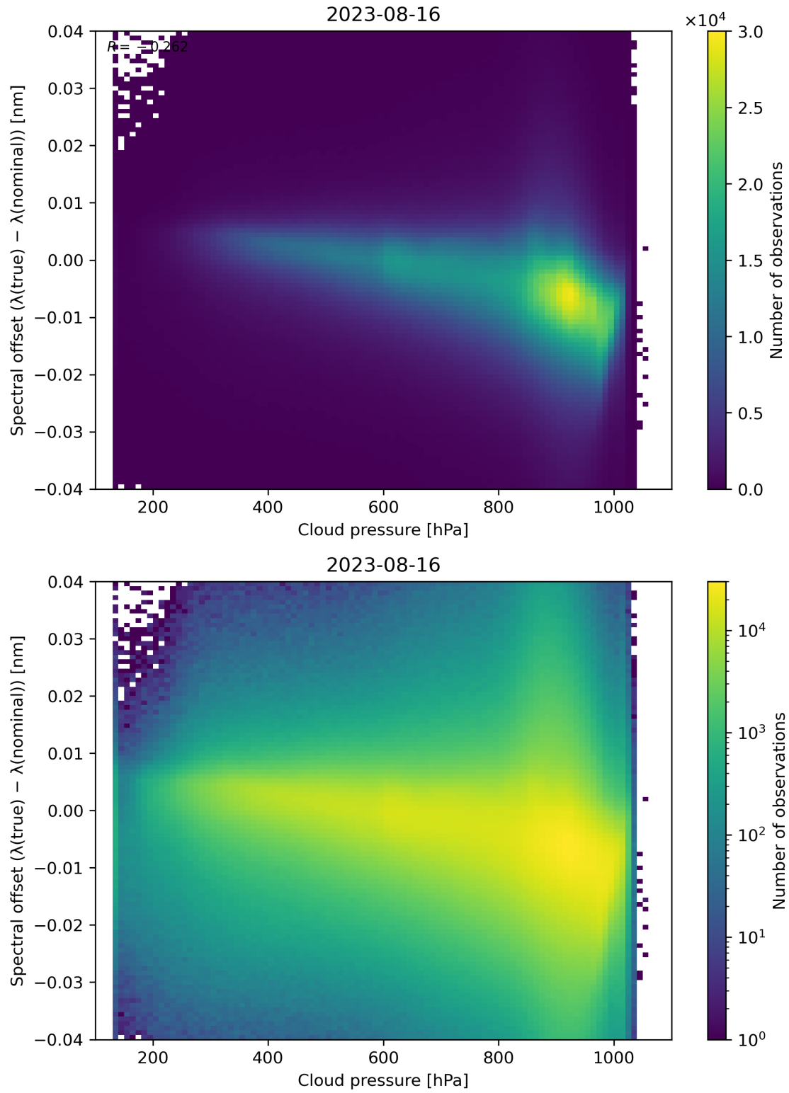
Figure 92: Scatter density plot of “Cloud pressure” against “Spectral offset ( \lambda(\text{true}) - \lambda(\text{nominal}) )” for 2023-08-15 to 2023-08-17.
