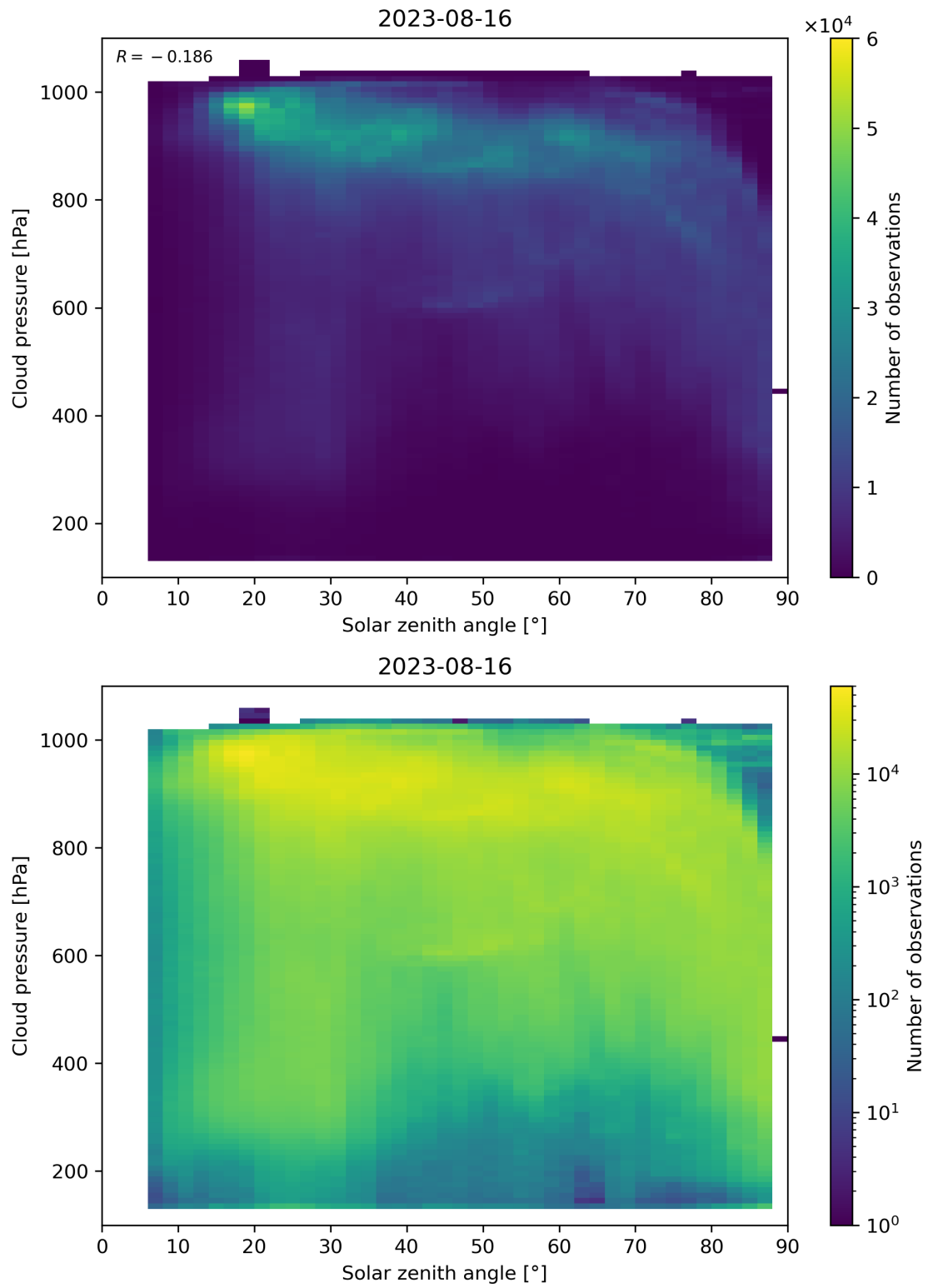
Figure 122: Scatter density plot of “Solar zenith angle” against “Cloud pressure” for 2023-08-15 to 2023-08-17.
