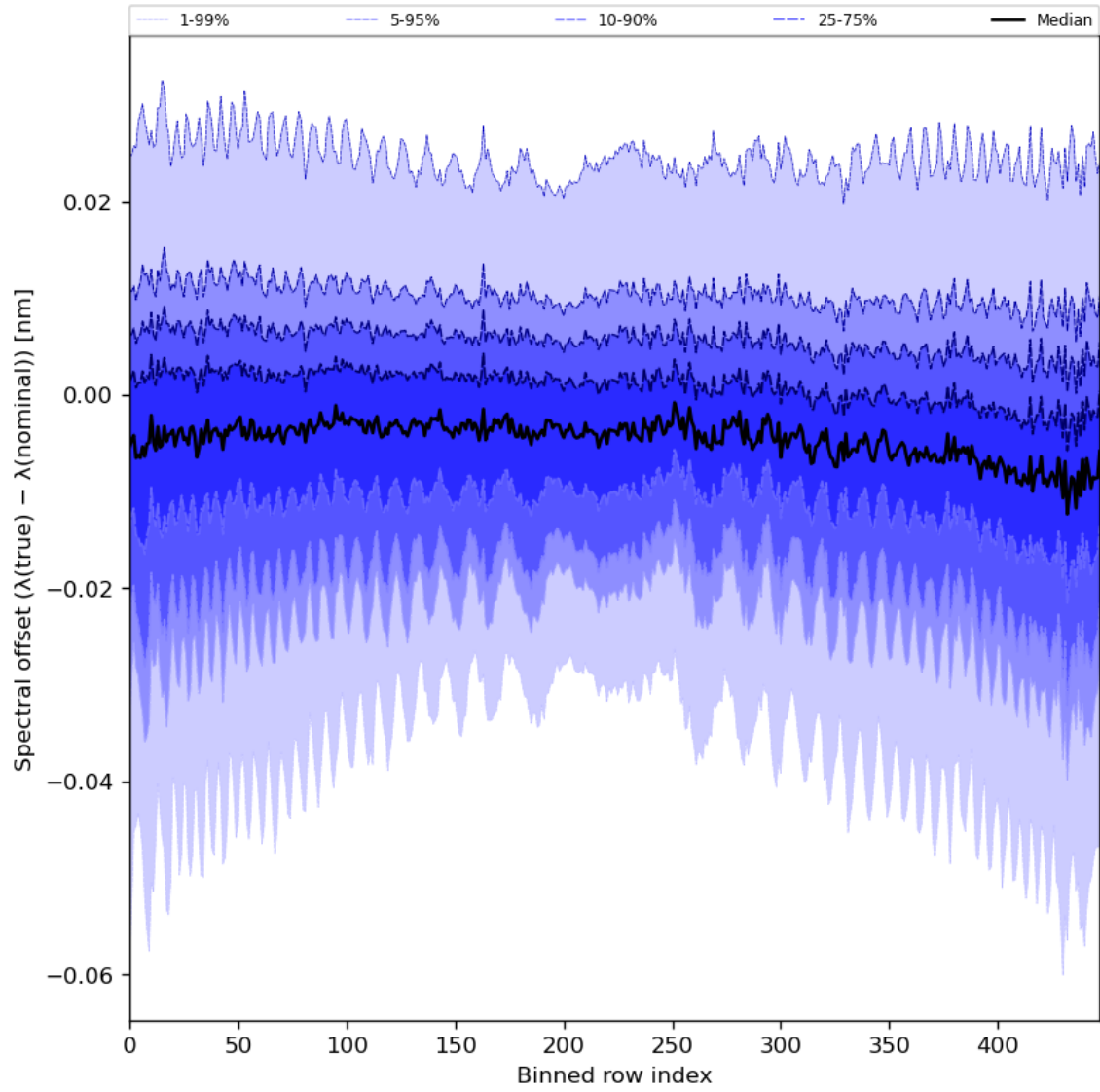
Figure 62: Along track statistics of “Spectral offset ( \lambda(\text{true}) - \lambda(\text{nominal}) )” for 2023-08-15 to 2023-08-17
