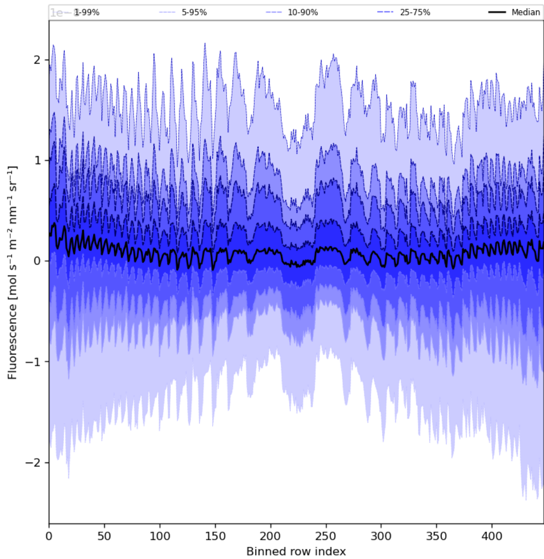
Figure 57: Along track statistics of “Fluorescence” for 2023-08-15 to 2023-08-17
