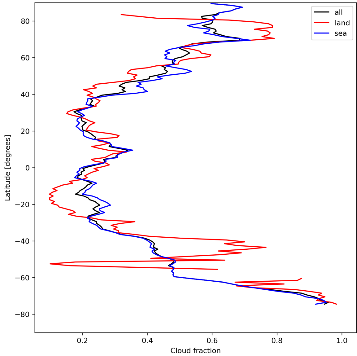
Figure 15: Zonal average of “Cloud fraction” for 2023-08-15 to 2023-08-17.
