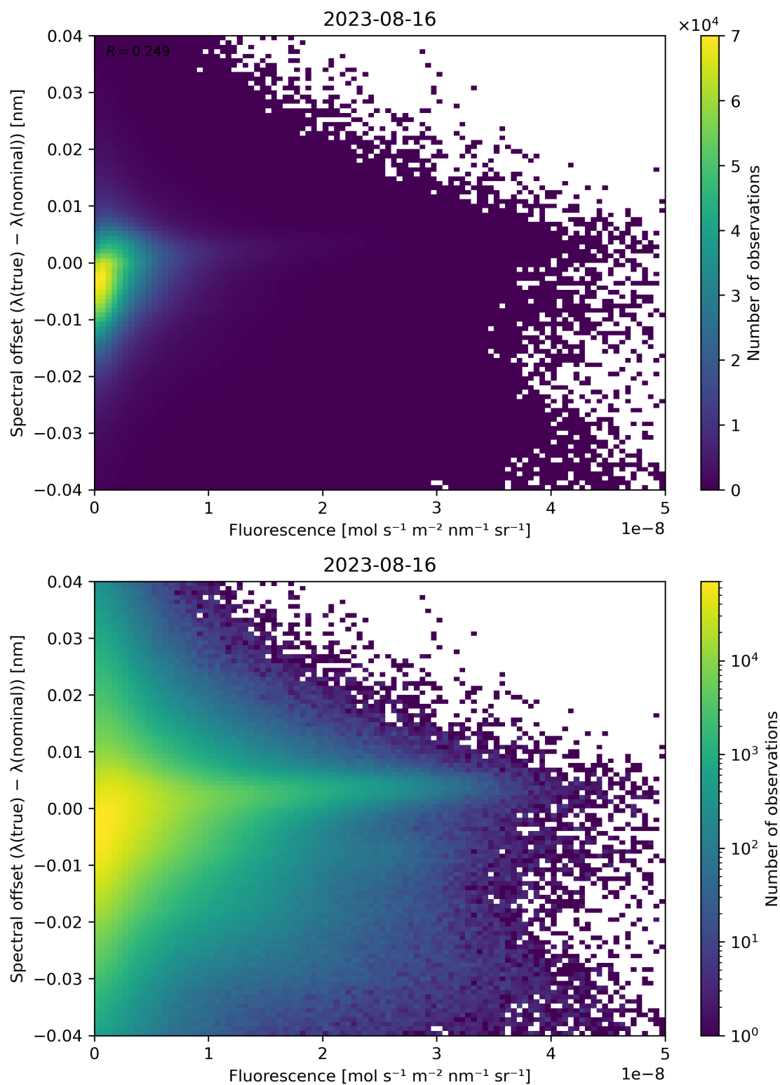
Figure 95: Scatter density plot of “Fluorescence” against “Spectral offset ( \lambda(\text{true}) - \lambda(\text{nominal}) )” for 2023-08-15 to 2023-08-17.
