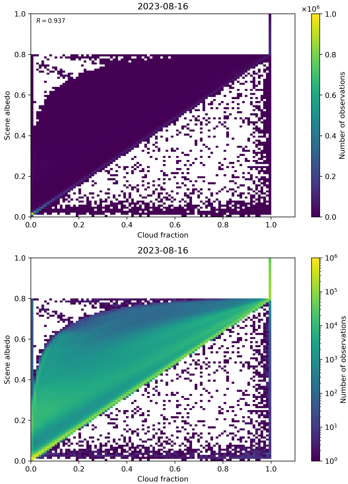
Figure 82: Scatter density plot of “Cloud fraction” against “Scene albedo” for 2023-08-15 to 2023-08-17.
