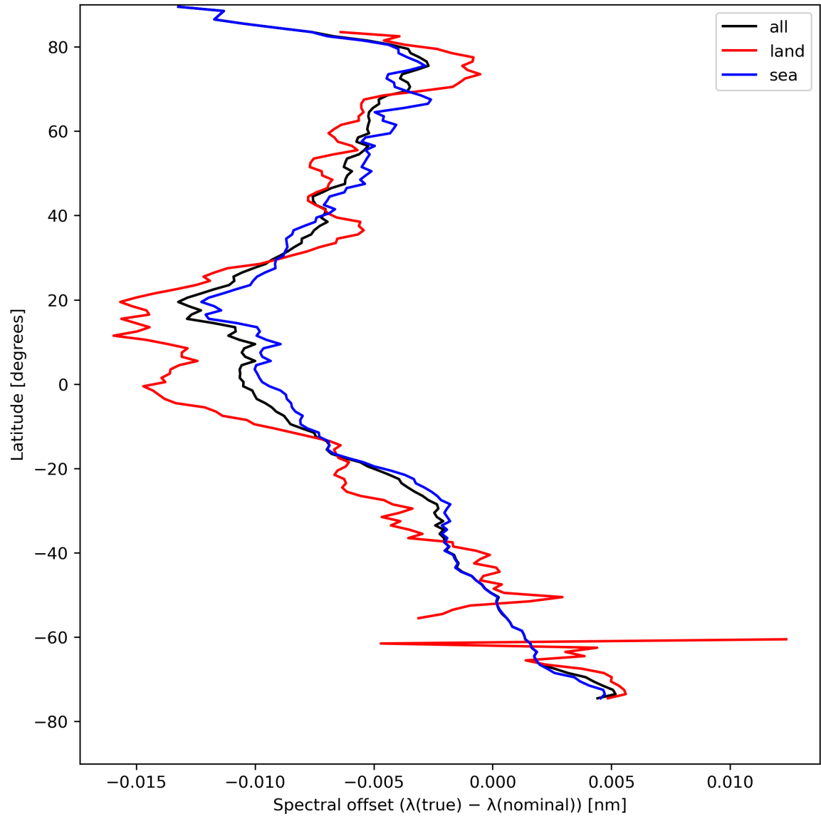
Figure 28: Zonal average of “Spectral offset ( \lambda(\text{true}) - \lambda(\text{nominal}) )” for 2023-08-15 to 2023-08-17.
