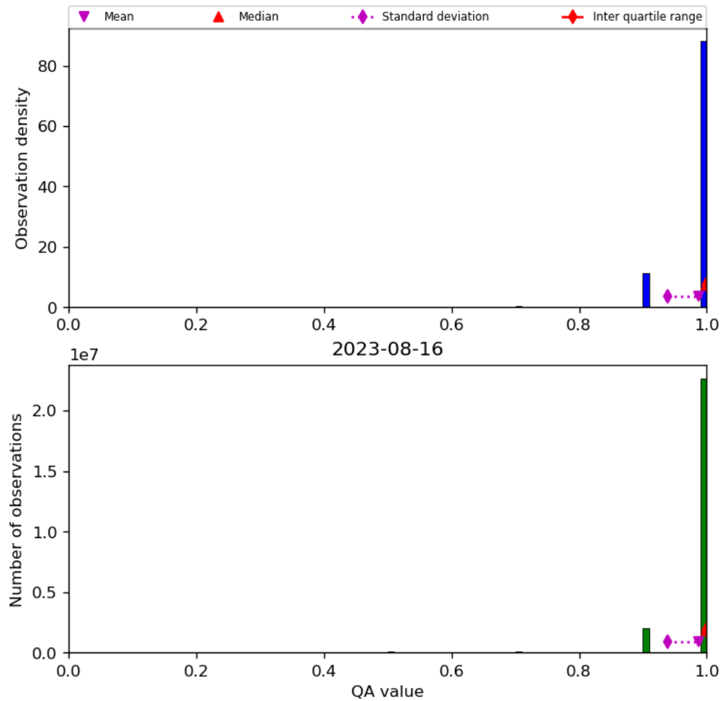
Figure 29: Histogram of “QA value” for 2023-08-15 to 2023-08-17
