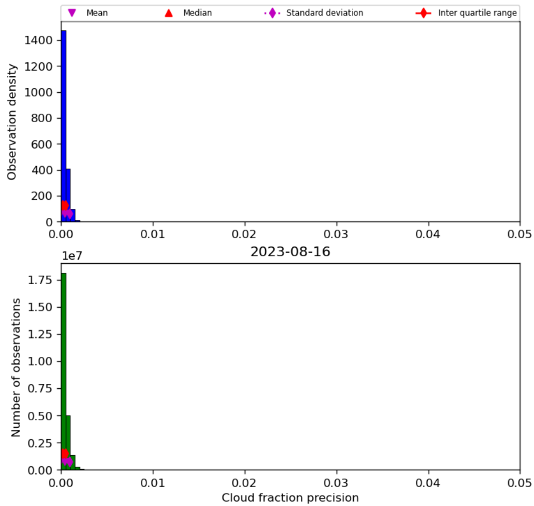
Figure 33: Histogram of “Cloud fraction precision” for 2023-08-15 to 2023-08-17
