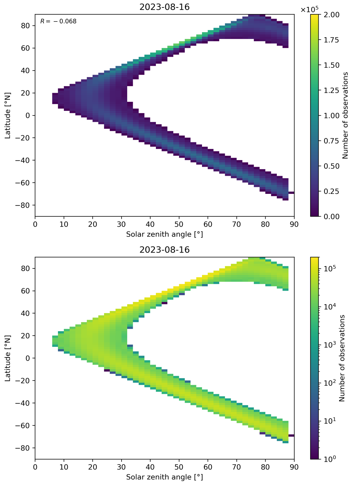
Figure 124: Scatter density plot of “Solar zenith angle” against “Latitude” for 2023-08-15 to 2023-08-17.
