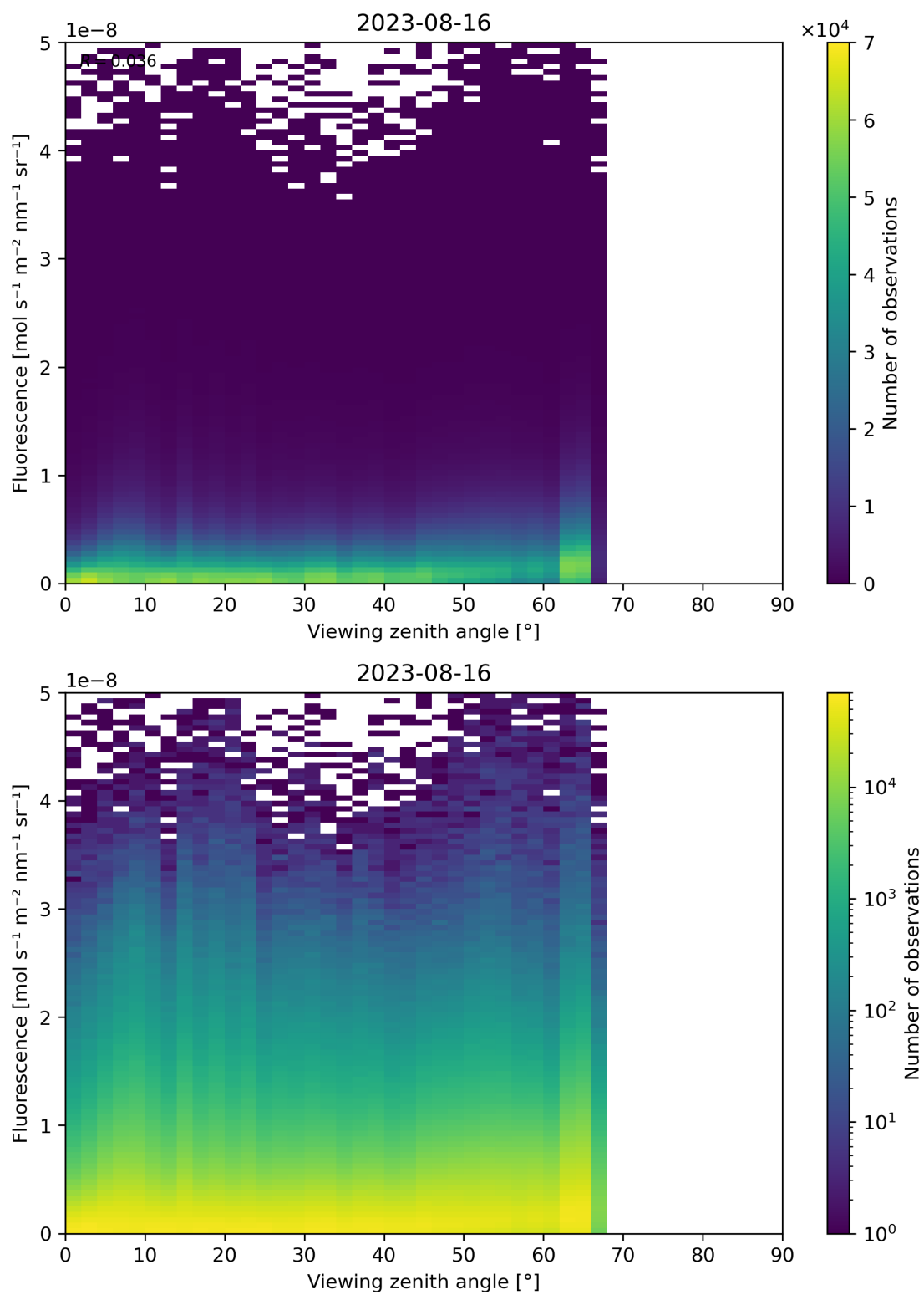
Figure 134: Scatter density plot of “Viewing zenith angle” against “Fluorescence” for 2023-08-15 to 2023-08-17.
