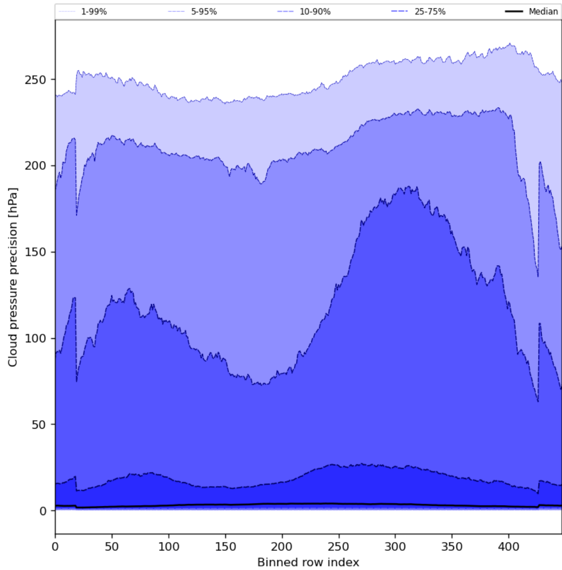
Figure 48: Along track statistics of “Cloud pressure precision” for 2023-08-15 to 2023-08-17
