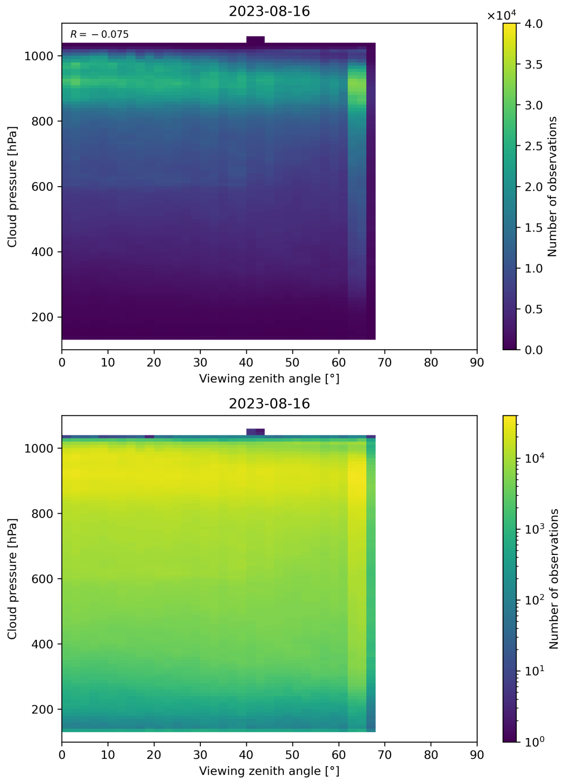
Figure 133: Scatter density plot of “Viewing zenith angle” against “Cloud pressure” for 2023-08-15 to 2023-08-17.
