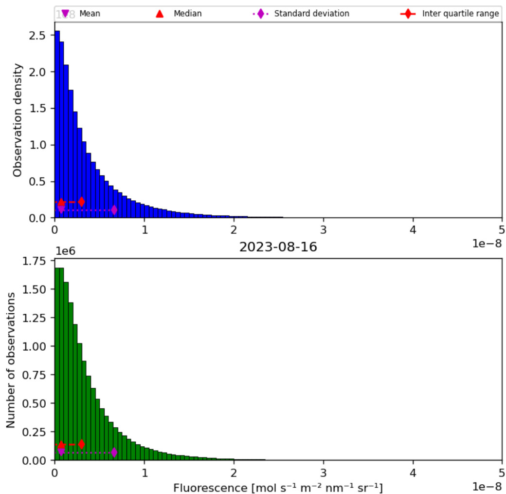
Figure 40: Histogram of “Fluorescence” for 2023-08-15 to 2023-08-17
