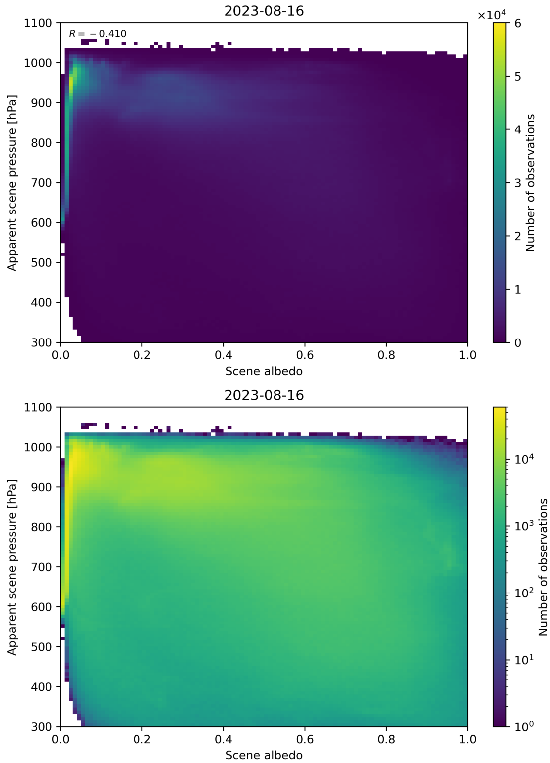
Figure 111: Scatter density plot of “Scene albedo” against “Apparent scene pressure” for 2023-08-15 to 2023-08-17.
