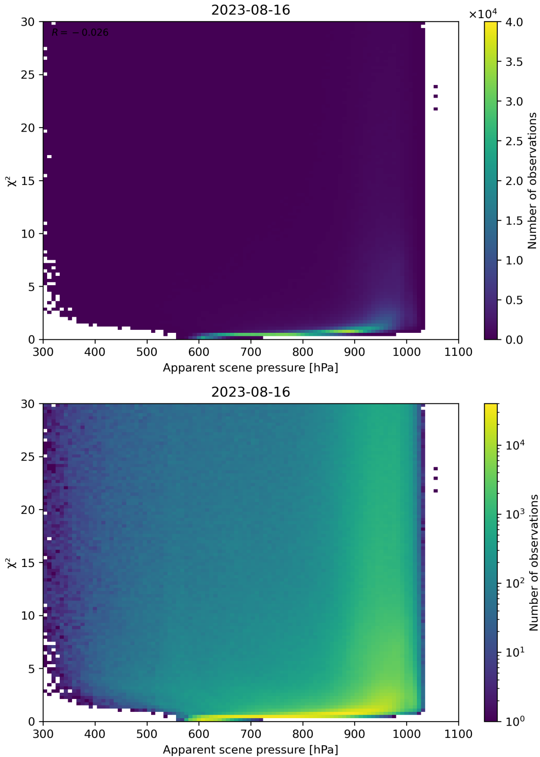
Figure 63: Scatter density plot of “Apparent scene pressure” against “ \chi^2 ” for 2023-08-15 to 2023-08-17.
