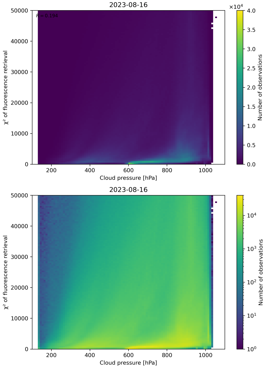
Figure 86: Scatter density plot of “Cloud pressure” against “ \chi^2 of fluorescence retrieval” for 2023-08-15 to 2023-08-17.
