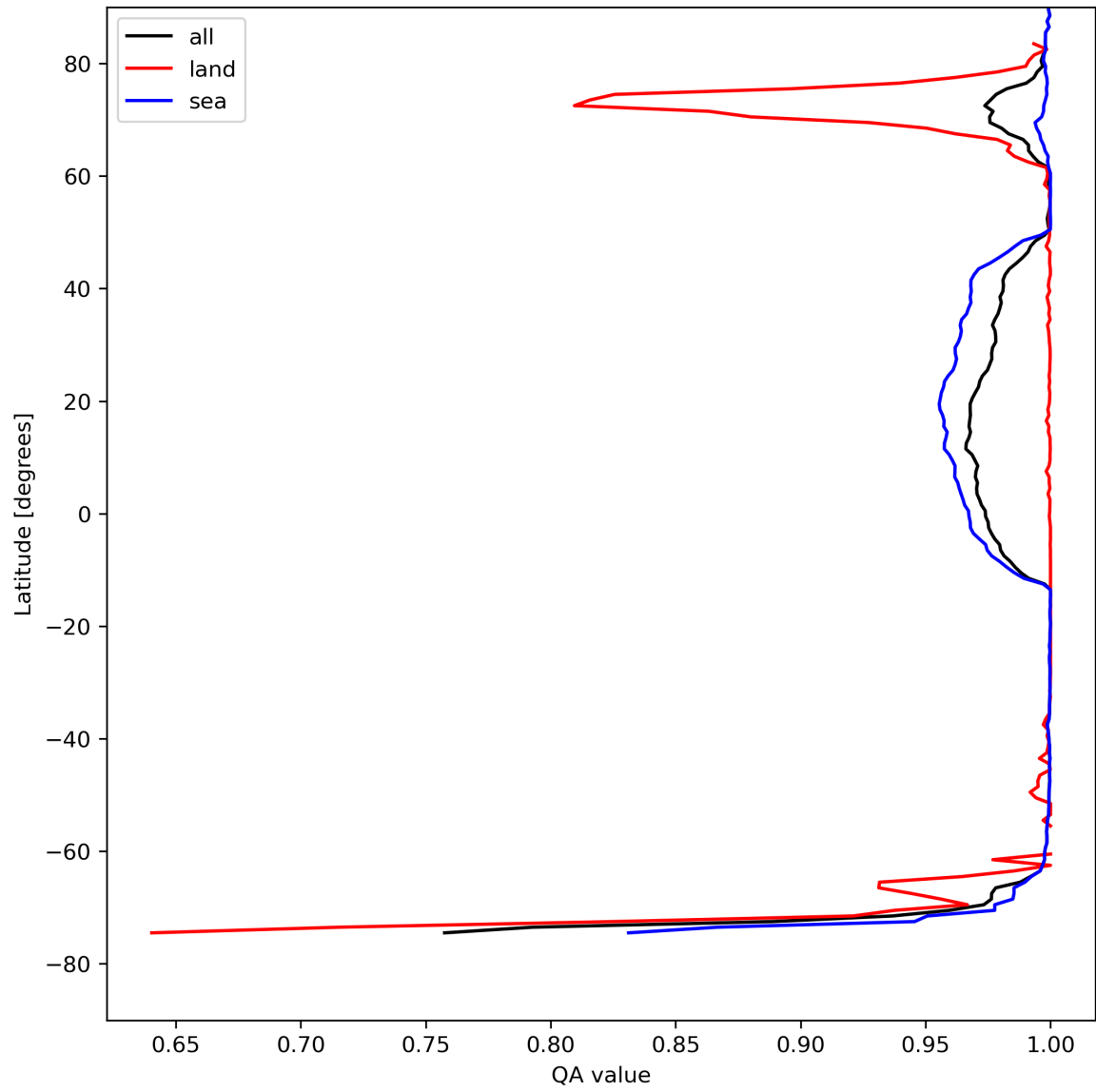
Figure 12: Zonal average of “QA value” for 2023-08-15 to 2023-08-17.
