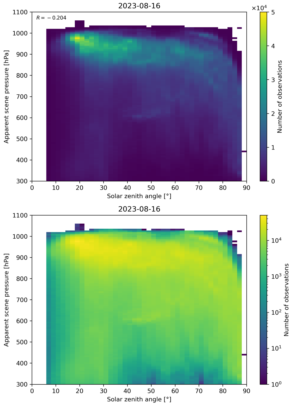
Figure 118: Scatter density plot of “Solar zenith angle” against “Apparent scene pressure” for 2023-08-15 to 2023-08-17.
