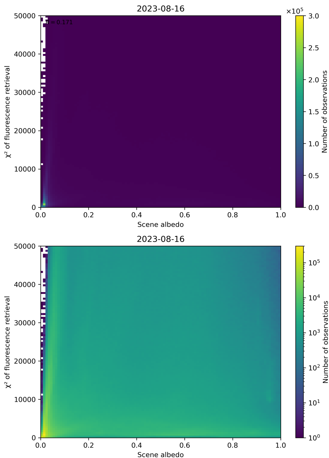
Figure 113: Scatter density plot of “Scene albedo” against “ \chi^2 of fluorescence retrieval” for 2023-08-15 to 2023-08-17.
