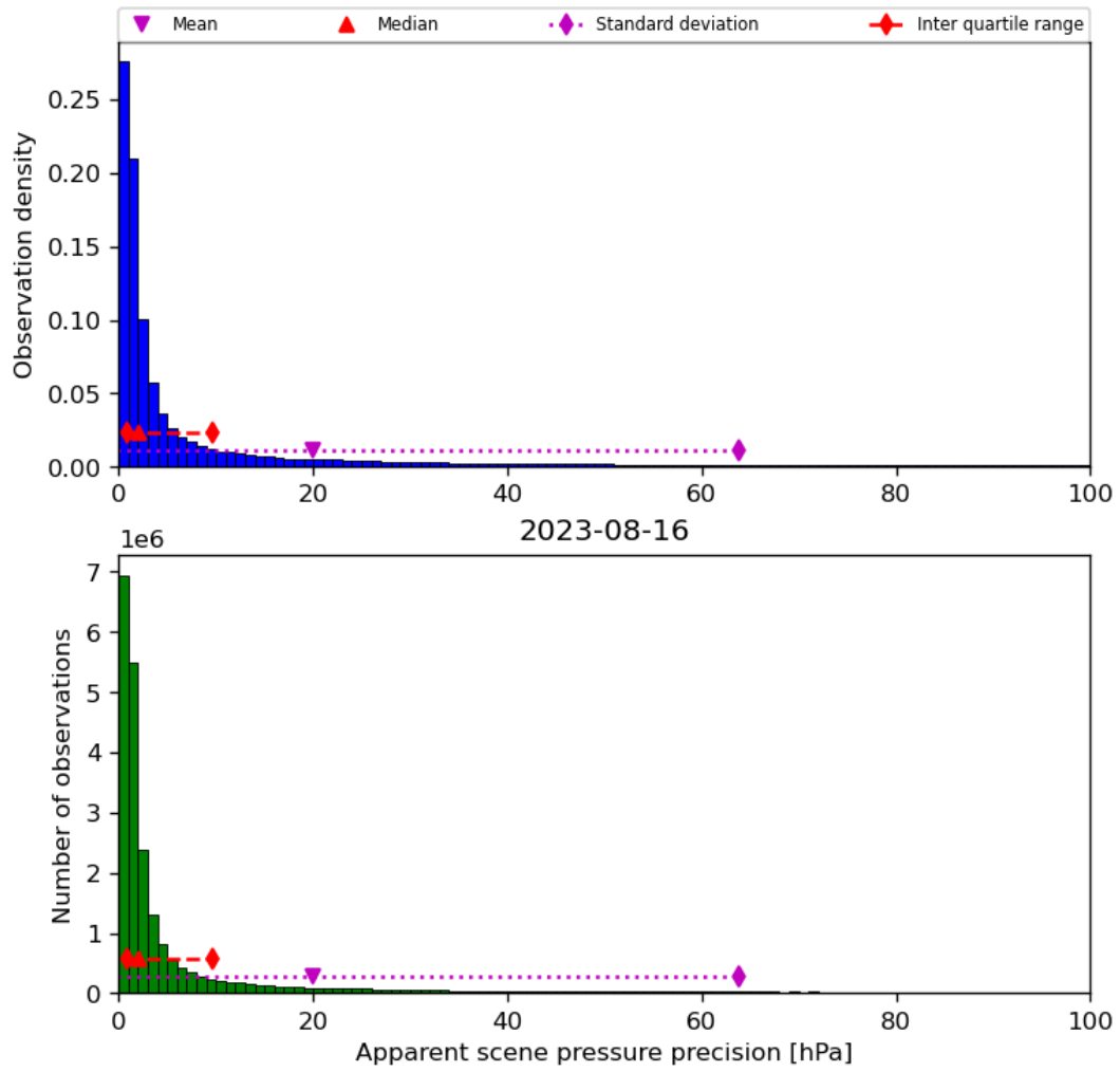
Figure 37: Histogram of “Apparent scene pressure precision” for 2023-08-15 to 2023-08-17
