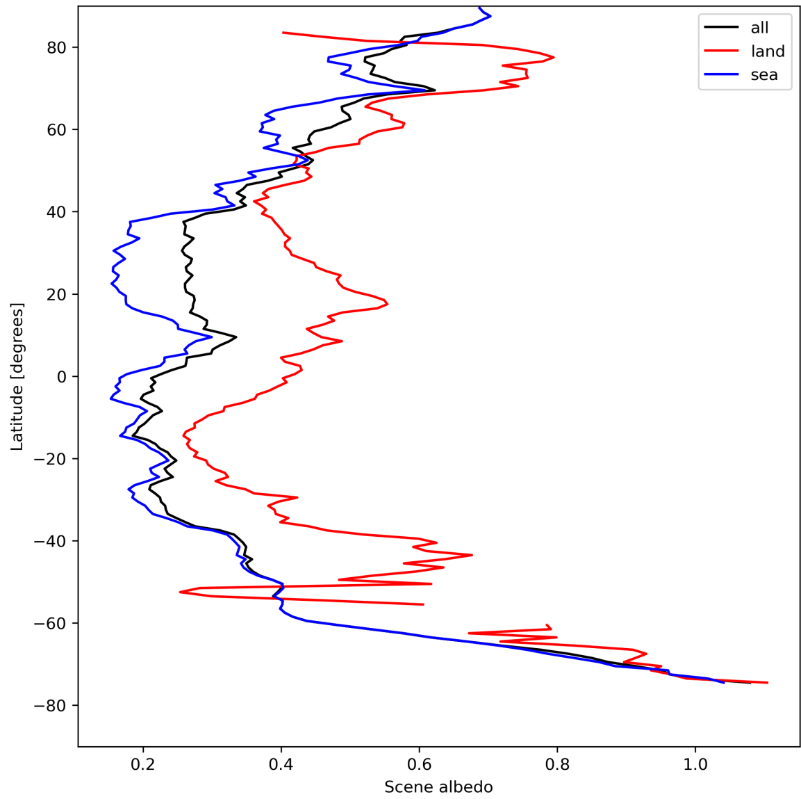
Figure 17: Zonal average of “Scene albedo” for 2023-08-15 to 2023-08-17.
