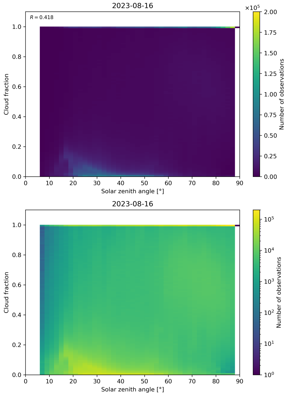
Figure 121: Scatter density plot of “Solar zenith angle” against “Cloud fraction” for 2023-08-15 to 2023-08-17.
