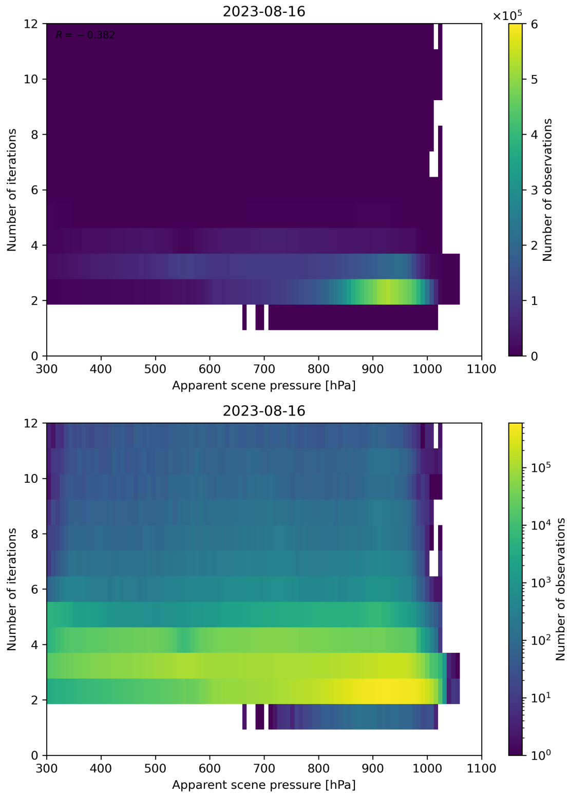
Figure 66: Scatter density plot of “Apparent scene pressure” against “Number of iterations” for 2023-08-15 to 2023-08-17.
