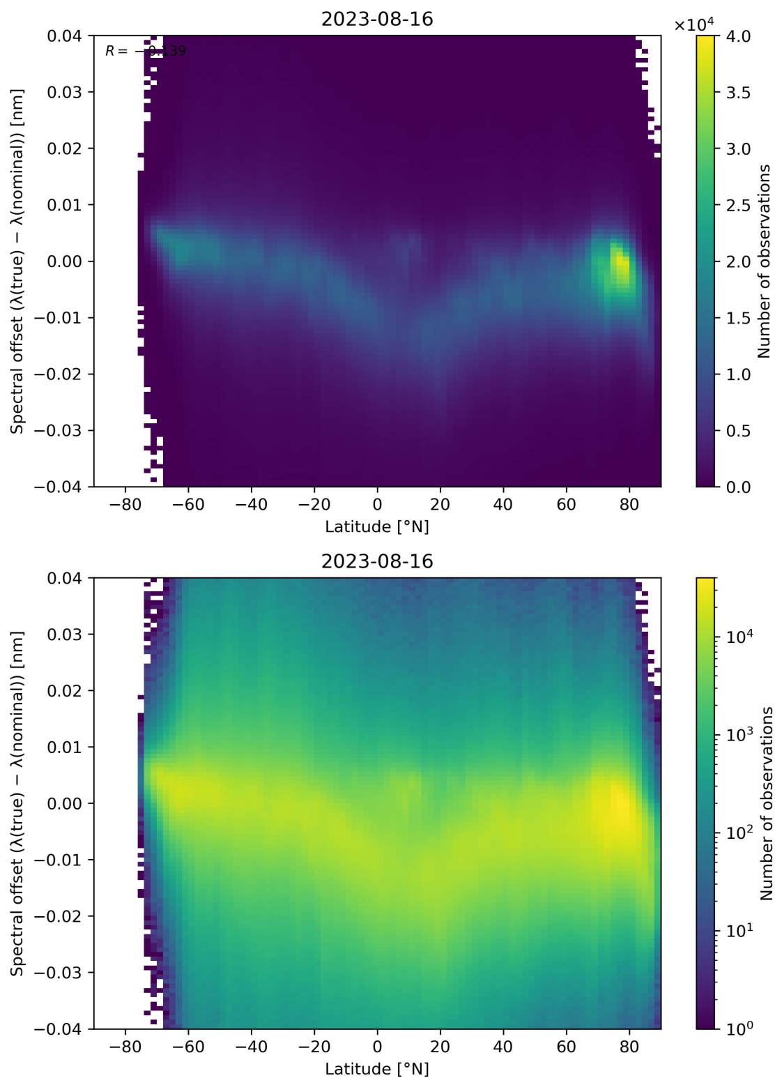
Figure 105: Scatter density plot of “Latitude” against “Spectral offset ( \lambda(\text{true}) - \lambda(\text{nominal}) )” for 2023-08-15 to 2023-08-17.
