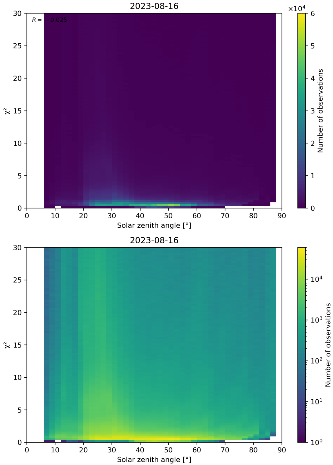
Figure 119: Scatter density plot of “Solar zenith angle” against “ \chi^2 ” for 2023-08-15 to 2023-08-17.
