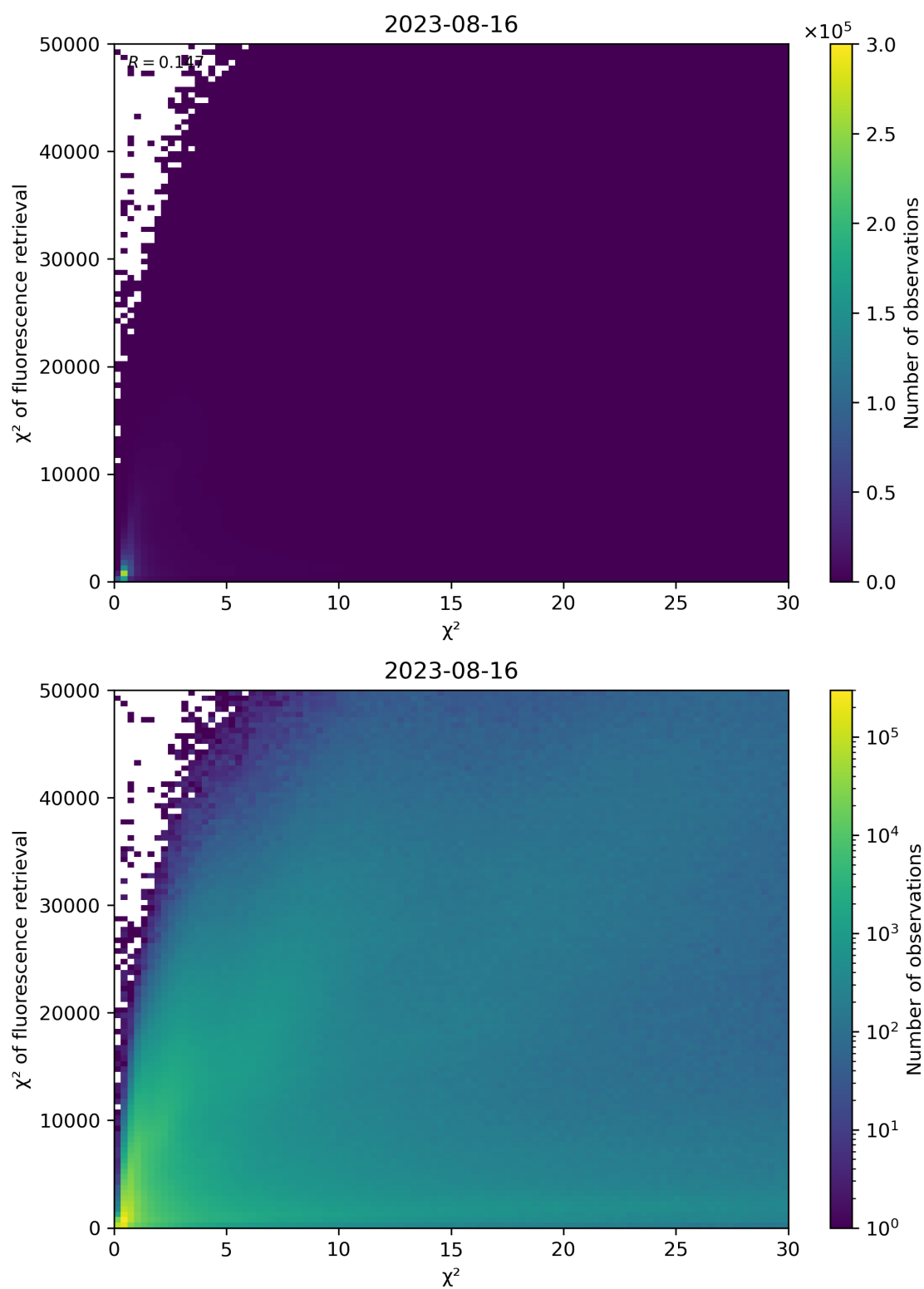
Figure 69: Scatter density plot of “ \chi^2 ” against “ \chi^2 of fluorescence retrieval” for 2023-08-15 to 2023-08-17.
