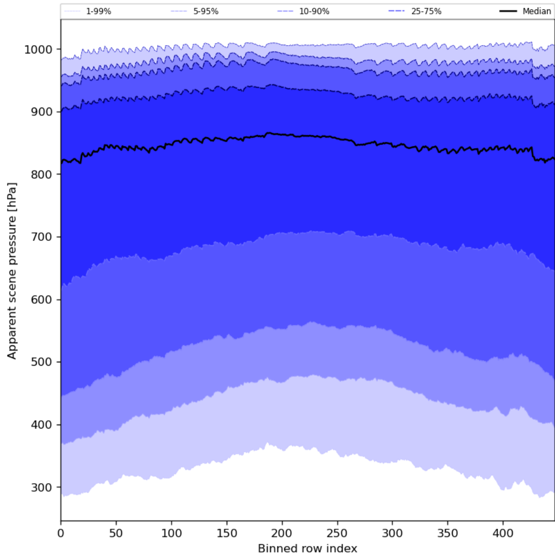
Figure 53: Along track statistics of “Apparent scene pressure” for 2023-08-15 to 2023-08-17
