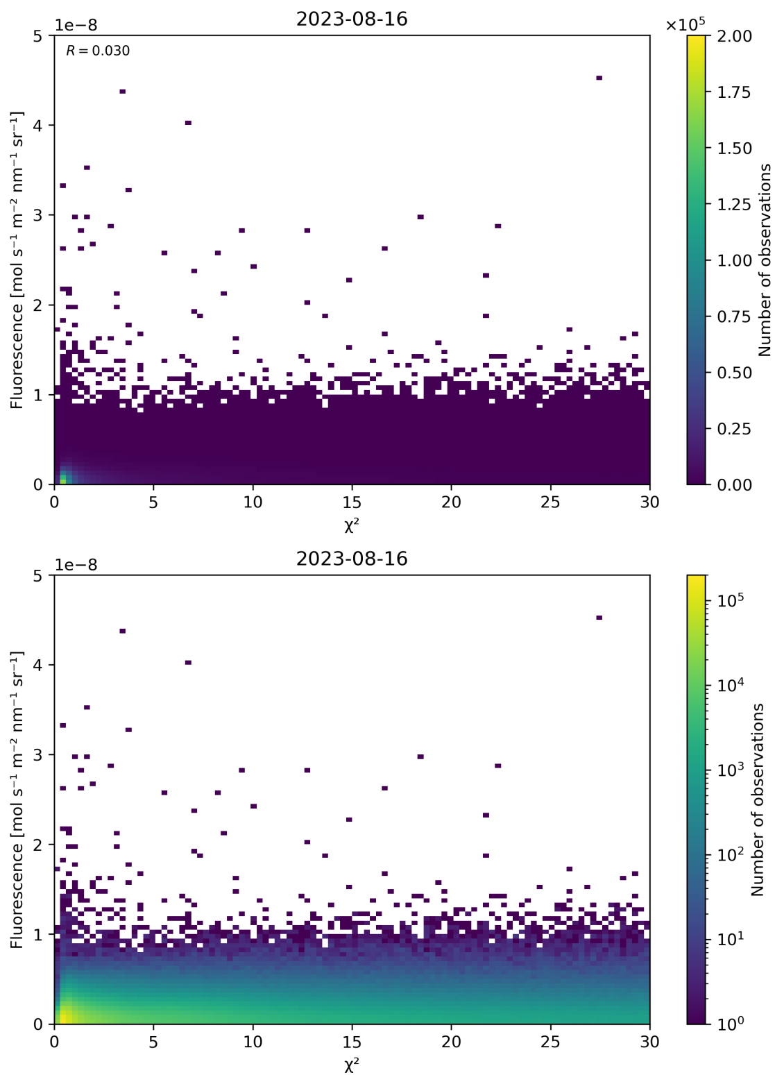
Figure 70: Scatter density plot of “ \chi^2 ” against “Fluorescence” for 2023-08-15 to 2023-08-17.
