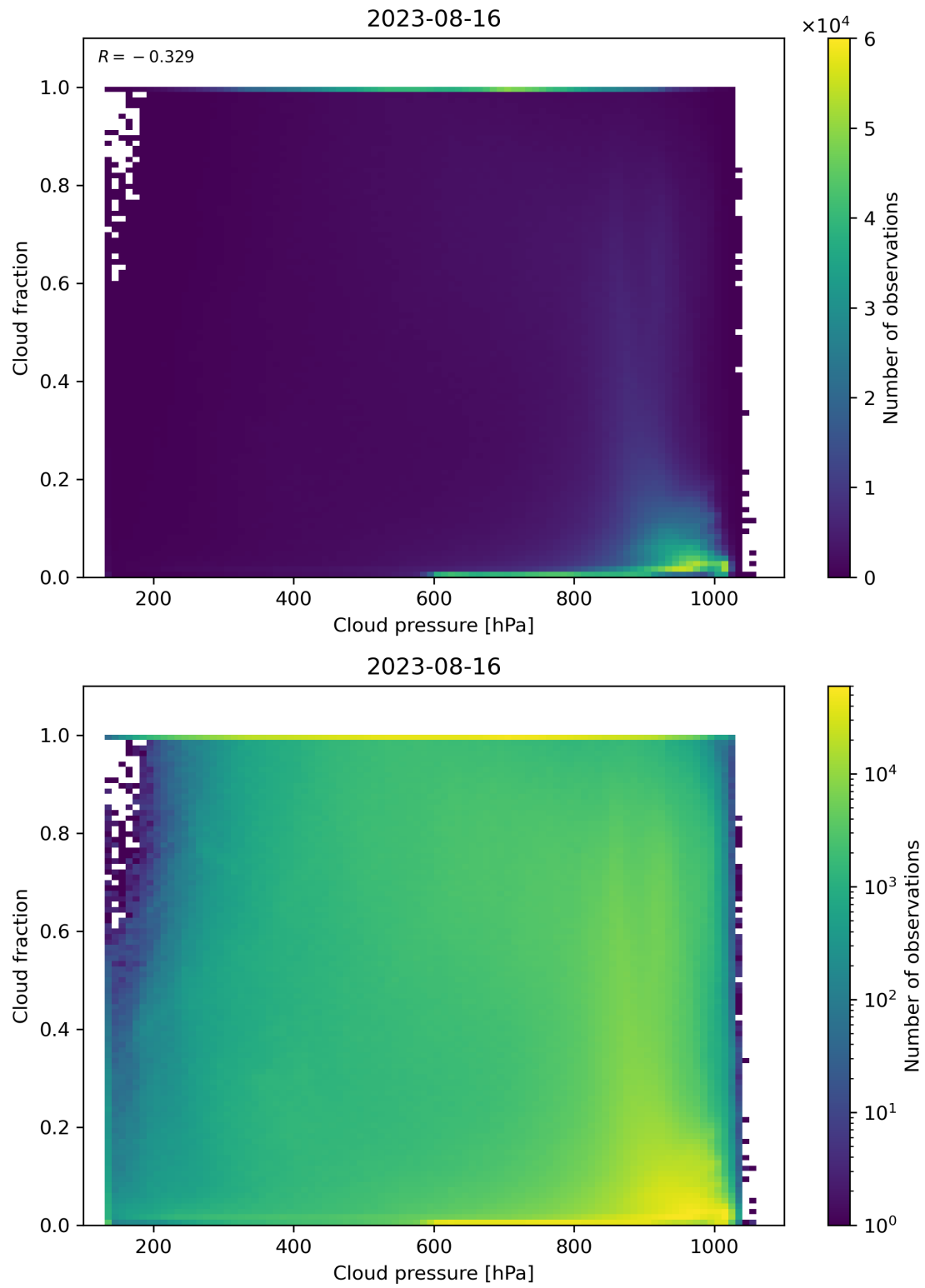
Figure 87: Scatter density plot of “Cloud pressure” against “Cloud fraction” for 2023-08-15 to 2023-08-17.
