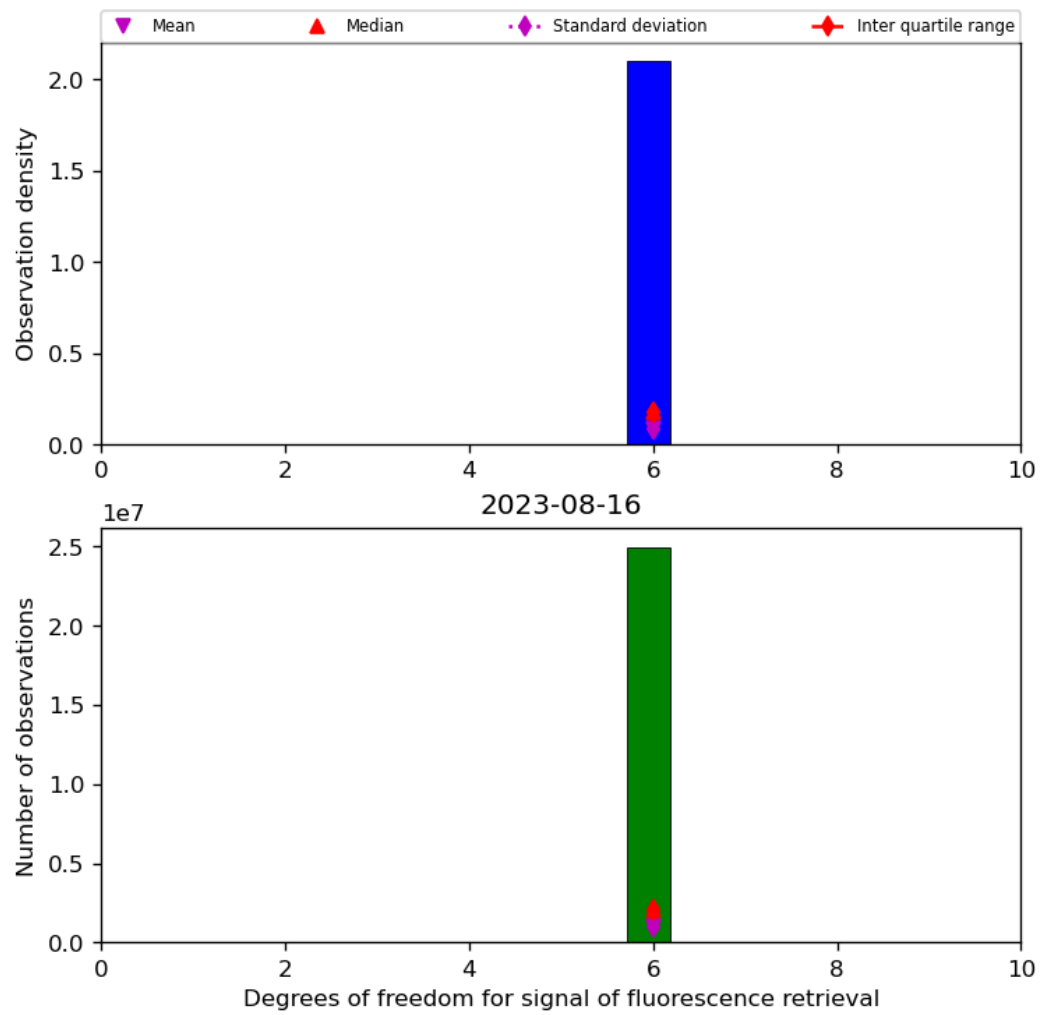
Figure 43: Histogram of “Degrees of freedom for signal of fluorescence retrieval” for 2023-08-15 to 2023-08-17
