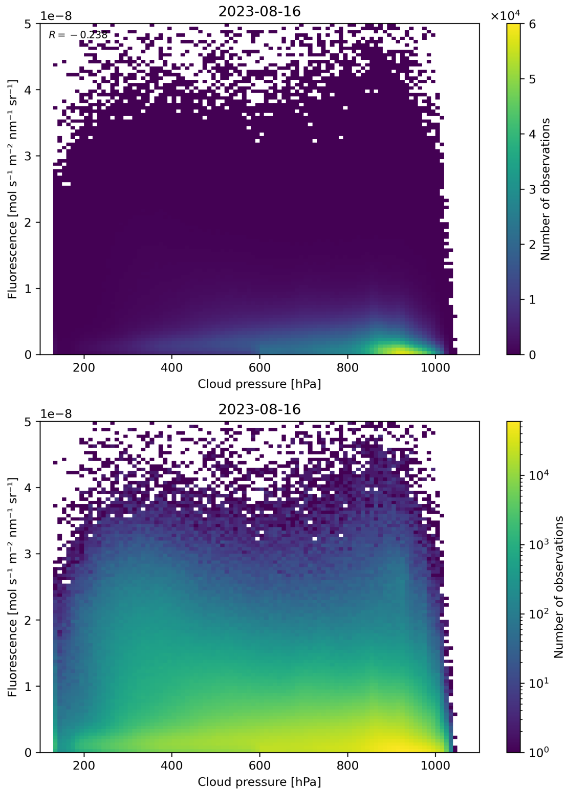
Figure 88: Scatter density plot of “Cloud pressure” against “Fluorescence” for 2023-08-15 to 2023-08-17.
