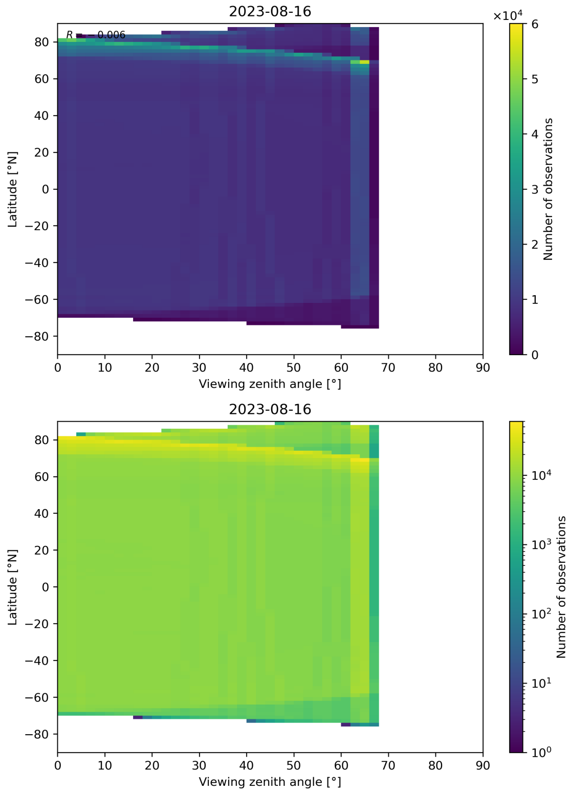
Figure 135: Scatter density plot of “Viewing zenith angle” against “Latitude” for 2023-08-15 to 2023-08-17.
