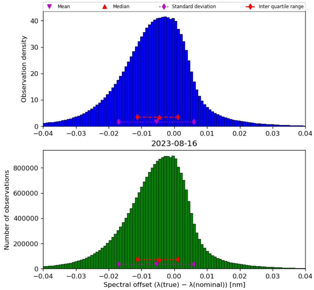
Figure 45: Histogram of “Spectral offset ( \lambda(\text{true}) - \lambda(\text{nominal}) )” for 2023-08-15 to 2023-08-17
