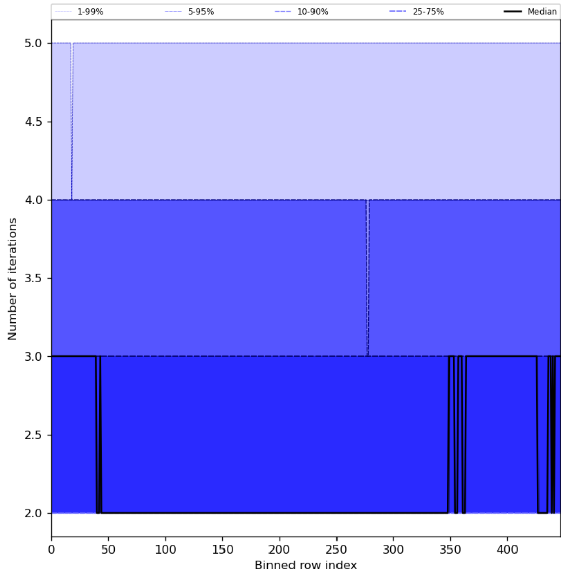
Figure 56: Along track statistics of “Number of iterations” for 2023-08-15 to 2023-08-17
