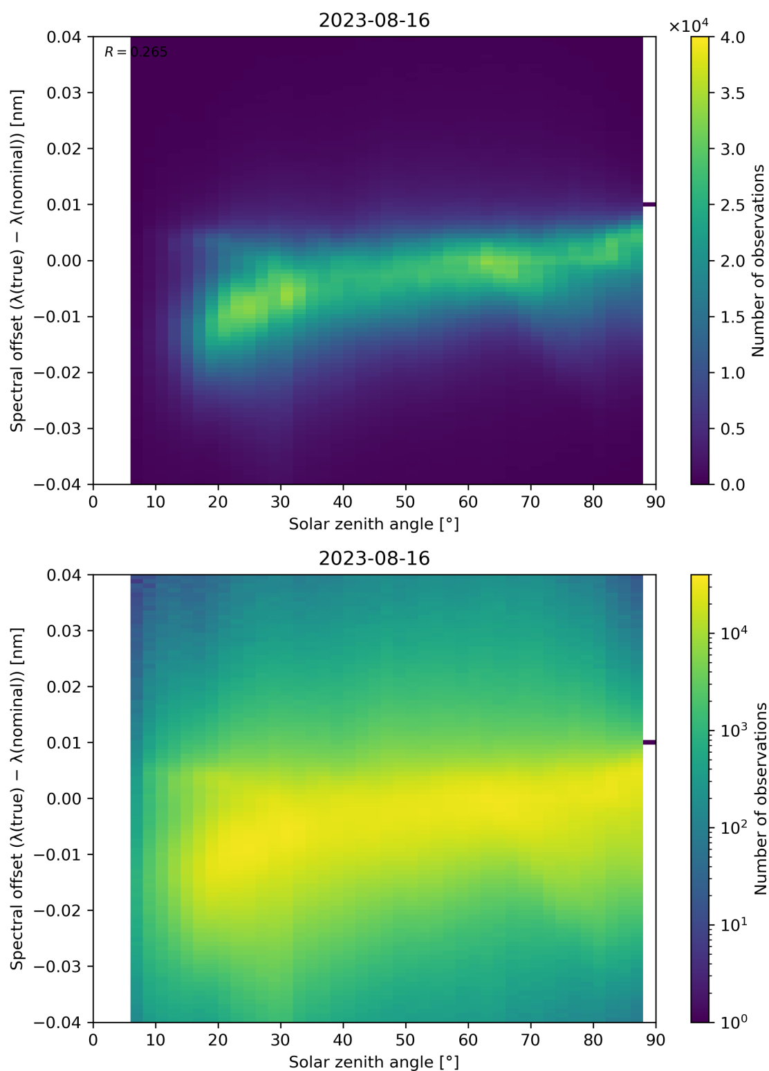
Figure 128: Scatter density plot of “Solar zenith angle” against “Spectral offset ( \lambda(\text{true}) - \lambda(\text{nominal}) )” for 2023-08-15 to 2023-08-17.
