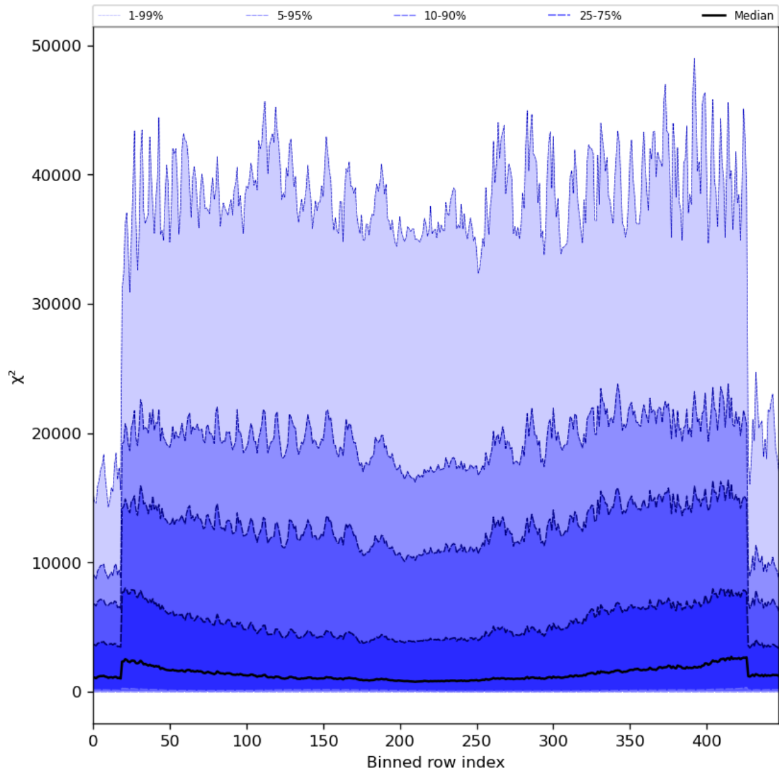
Figure 55: Along track statistics of “ \chi^2 ” for 2023-08-15 to 2023-08-17
