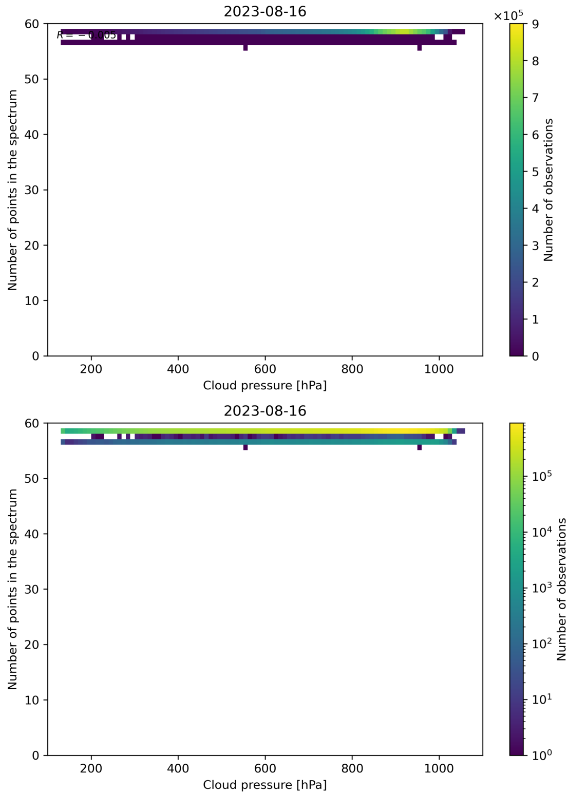
Figure 90: Scatter density plot of “Cloud pressure” against “Number of points in the spectrum” for 2023-08-15 to 2023-08-17.
