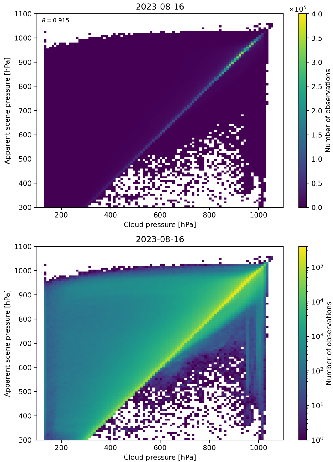
Figure 84: Scatter density plot of “Cloud pressure” against “Apparent scene pressure” for 2023-08-15 to 2023-08-17.
