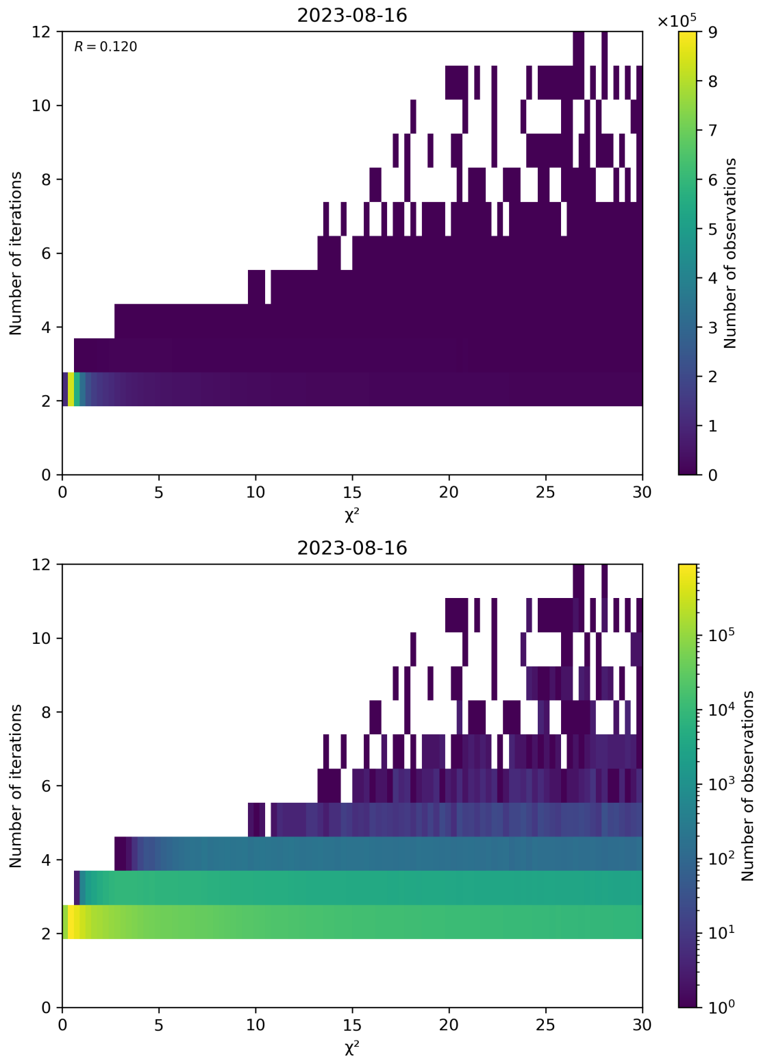
Figure 73: Scatter density plot of “ \chi^2 ” against “Number of iterations” for 2023-08-15 to 2023-08-17.
