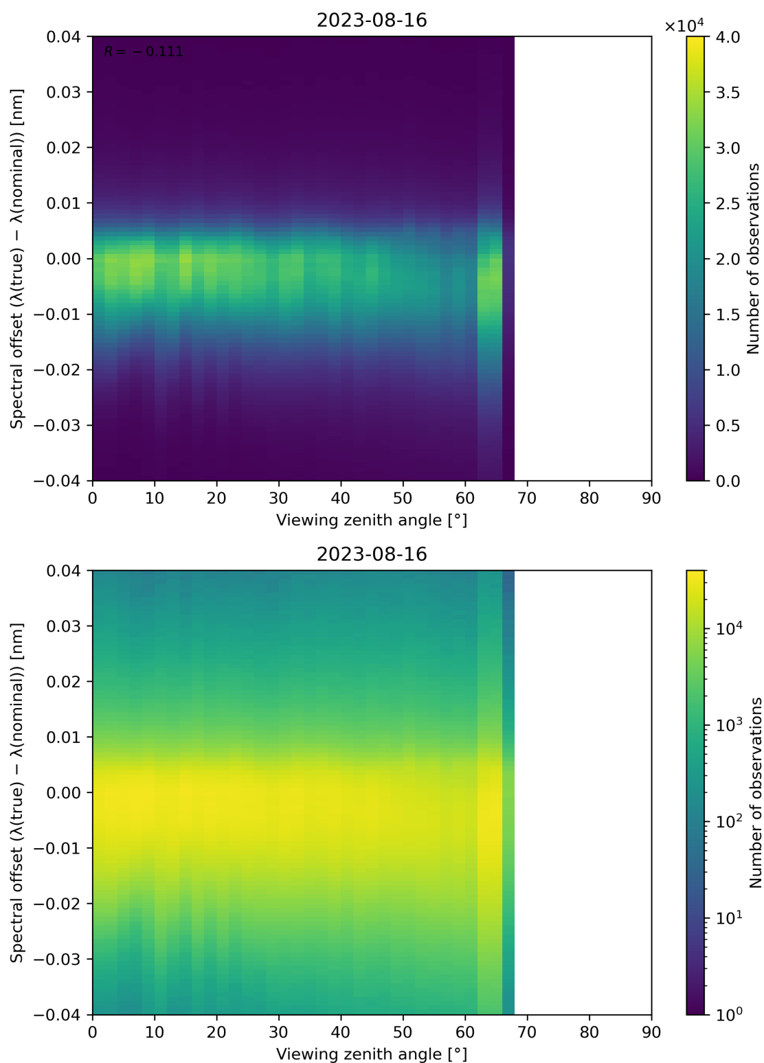
Figure 140: Scatter density plot of “Viewing zenith angle” against “Spectral offset ( \lambda(\text{true}) - \lambda(\text{nominal}) )” for 2023-08-15 to 2023-08-17.
