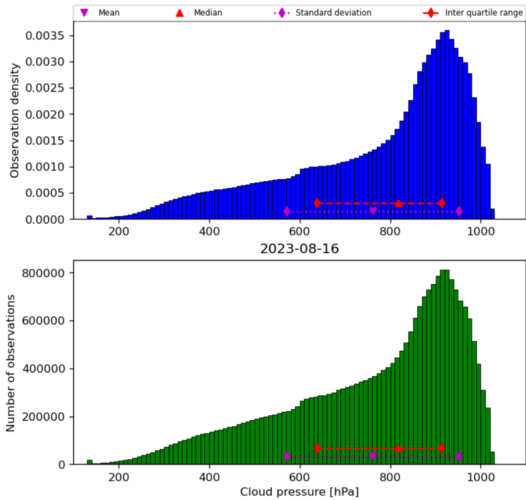
Figure 30: Histogram of “Cloud pressure” for 2023-08-15 to 2023-08-17
