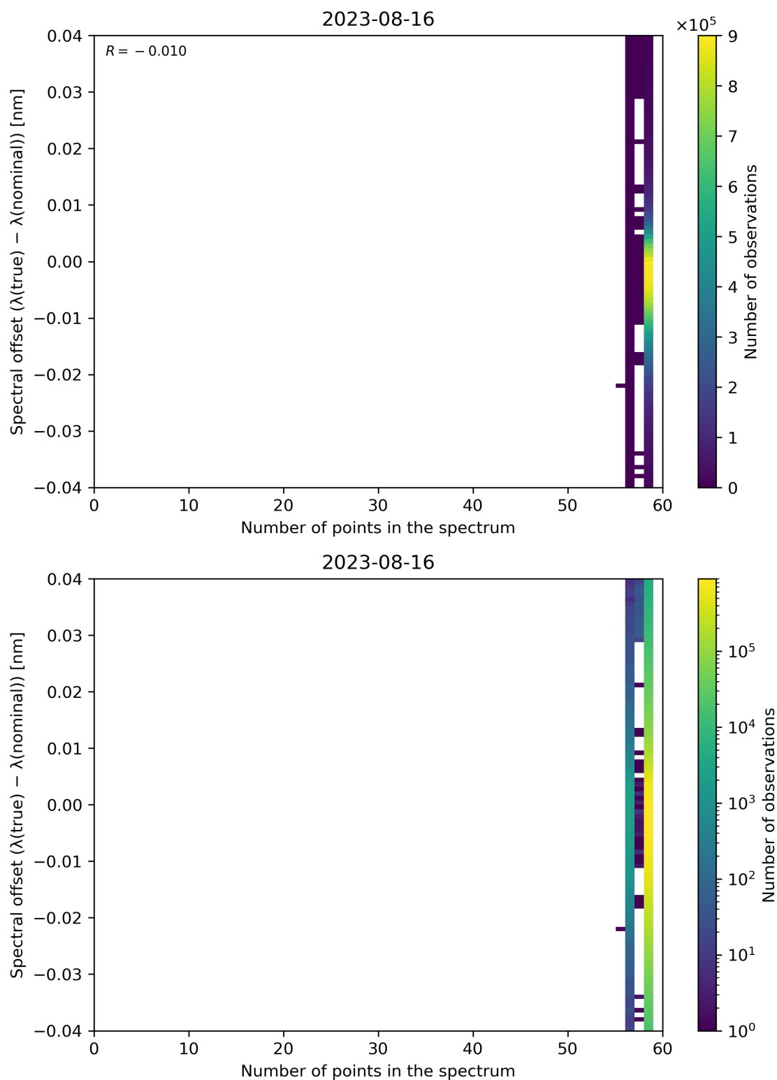
Figure 110: Scatter density plot of “Number of points in the spectrum” against “Spectral offset ( \lambda(\text{true}) - \lambda(\text{nominal}) )” for 2023-08-15 to 2023-08-17.
