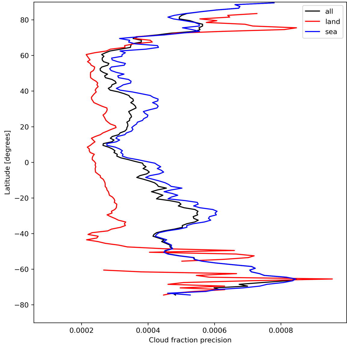
Figure 16: Zonal average of “Cloud fraction precision” for 2023-08-15 to 2023-08-17.
