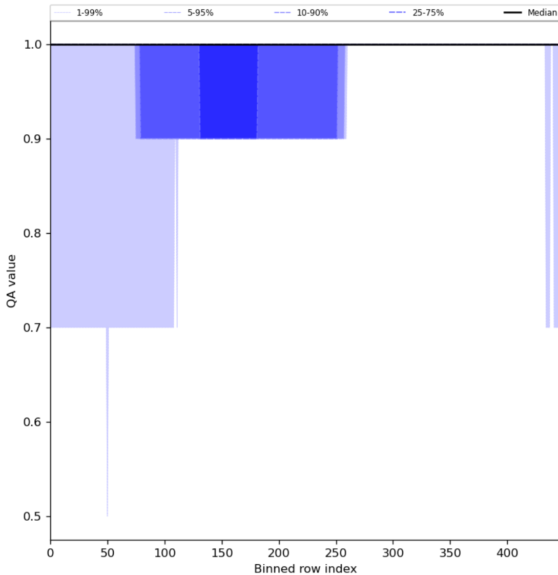
Figure 46: Along track statistics of “QA value” for 2023-08-15 to 2023-08-17
