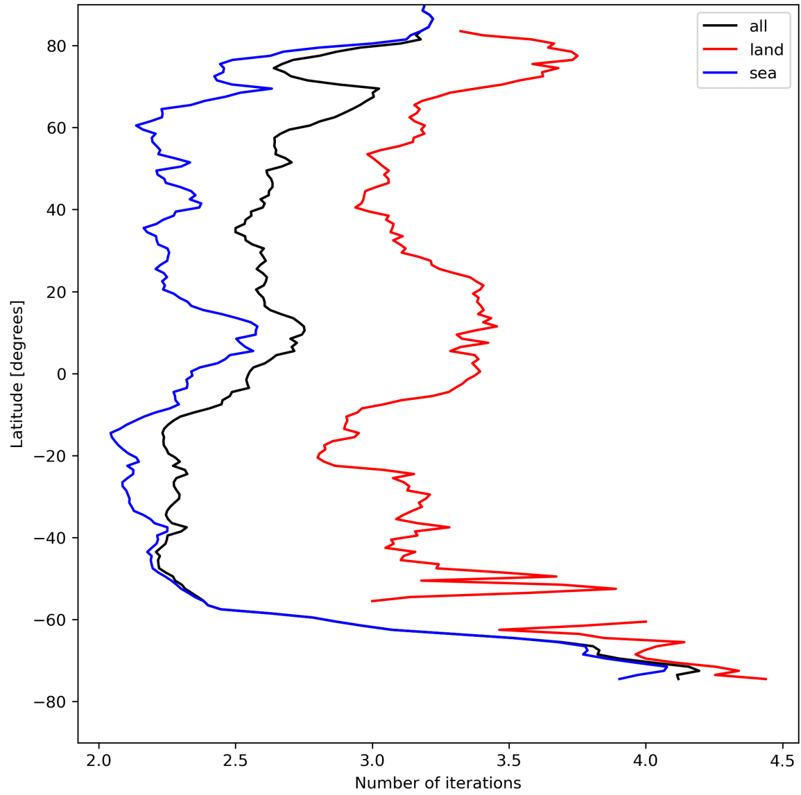
Figure 22: Zonal average of “Number of iterations” for 2023-08-15 to 2023-08-17.
