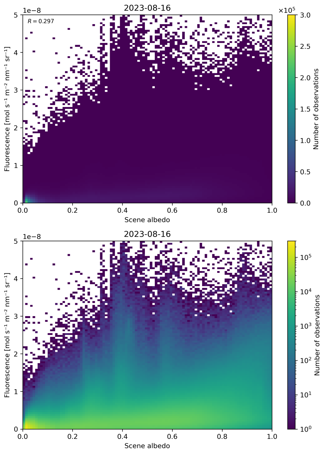
Figure 114: Scatter density plot of “Scene albedo” against “Fluorescence” for 2023-08-15 to 2023-08-17.
