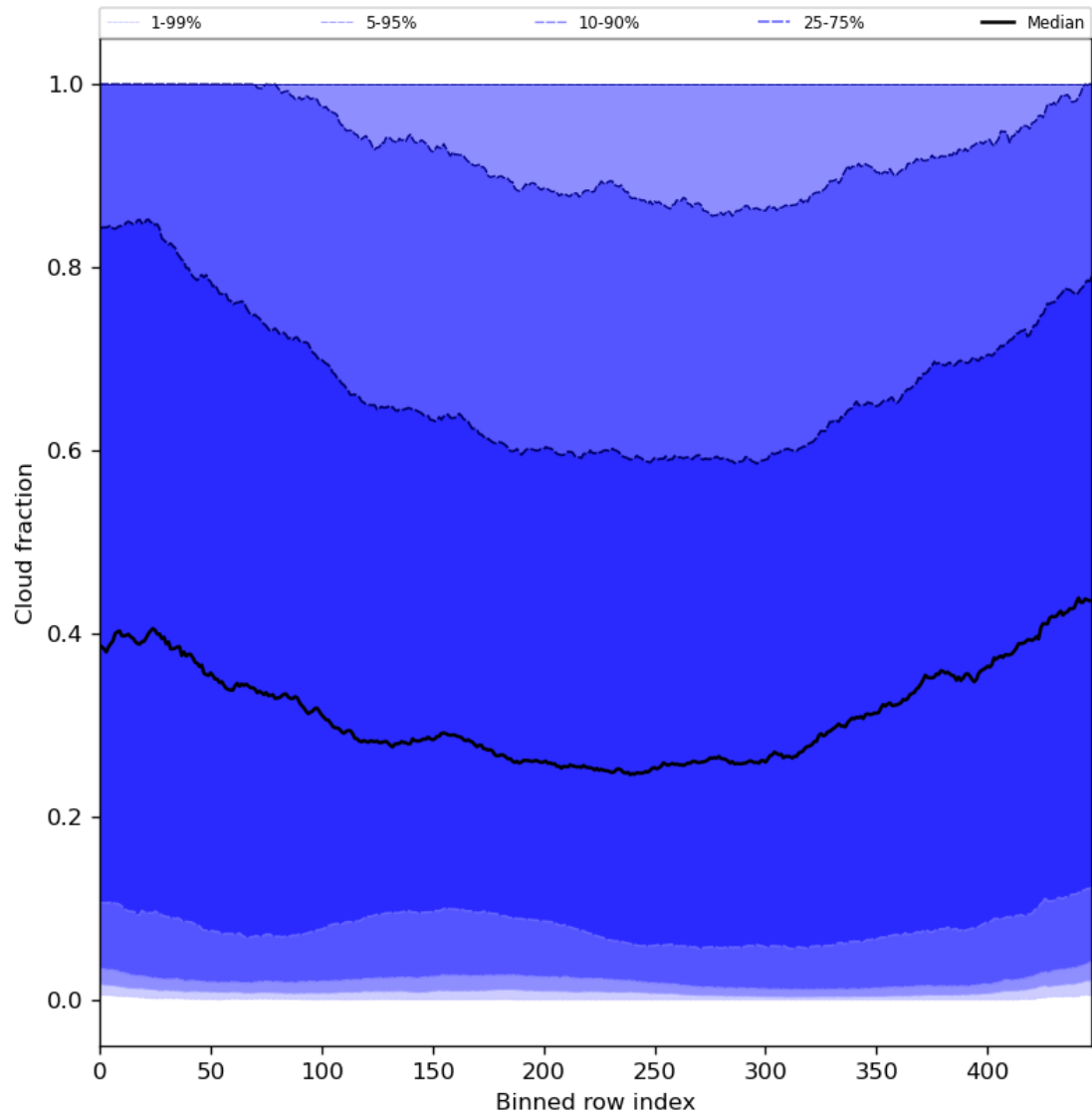
Figure 49: Along track statistics of “Cloud fraction” for 2023-08-15 to 2023-08-17
