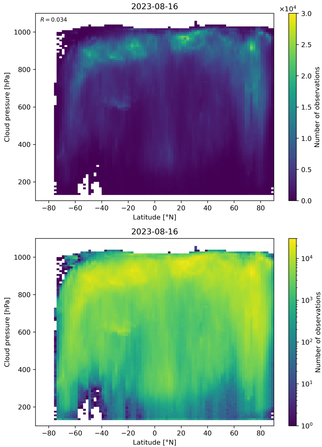
Figure 100: Scatter density plot of “Latitude” against “Cloud pressure” for 2023-08-15 to 2023-08-17.
