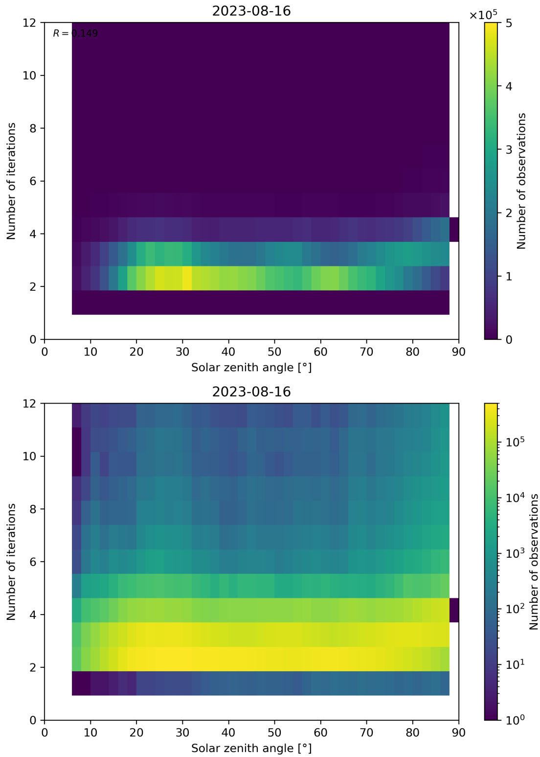
Figure 125: Scatter density plot of “Solar zenith angle” against “Number of iterations” for 2023-08-15 to 2023-08-17.
