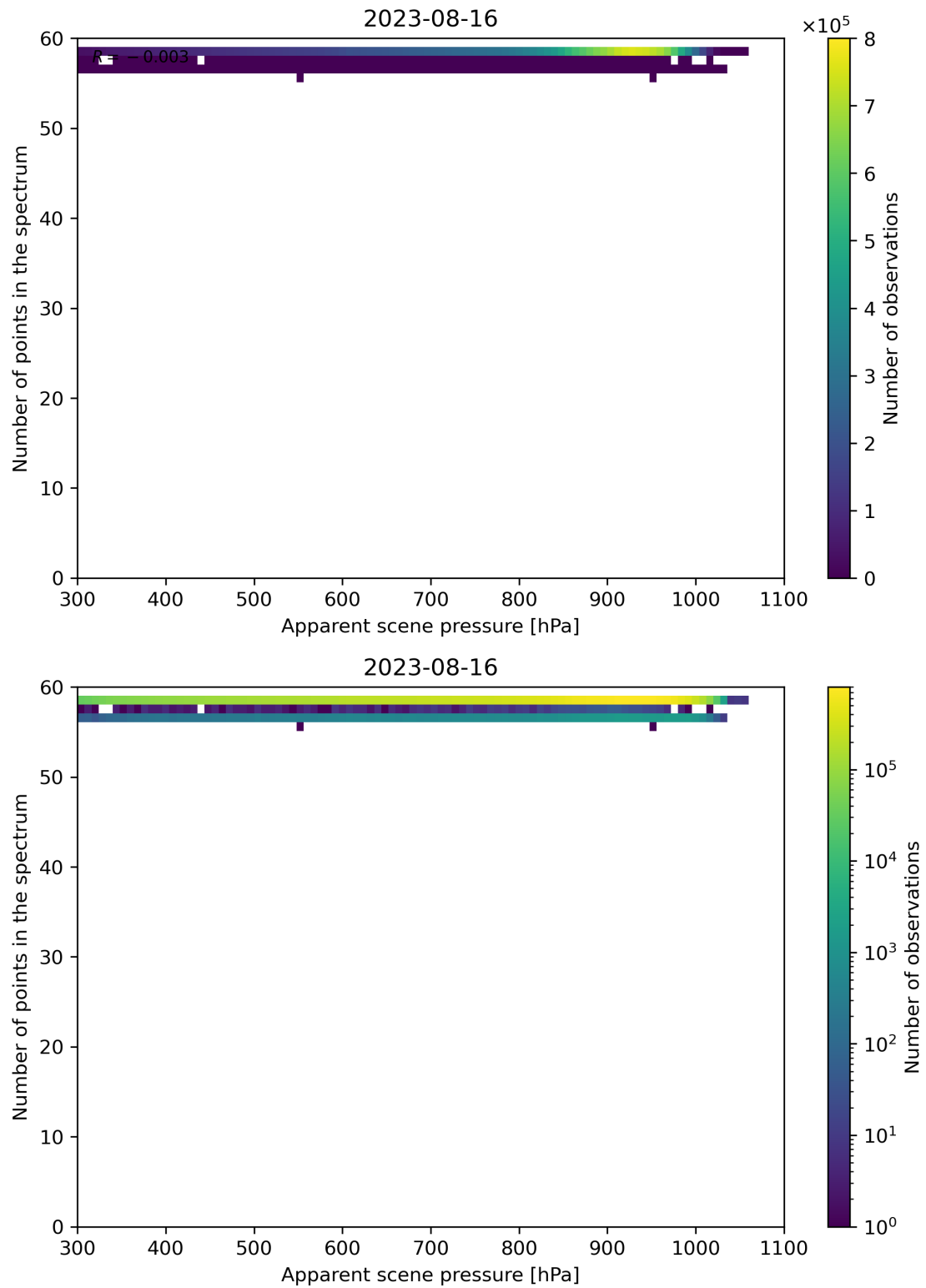
Figure 67: Scatter density plot of “Apparent scene pressure” against “Number of points in the spectrum” for 2023-08-15 to 2023-08-17.
