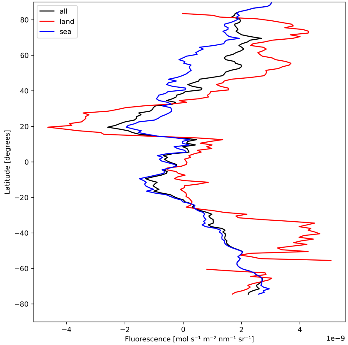
Figure 23: Zonal average of “Fluorescence” for 2023-08-15 to 2023-08-17.
