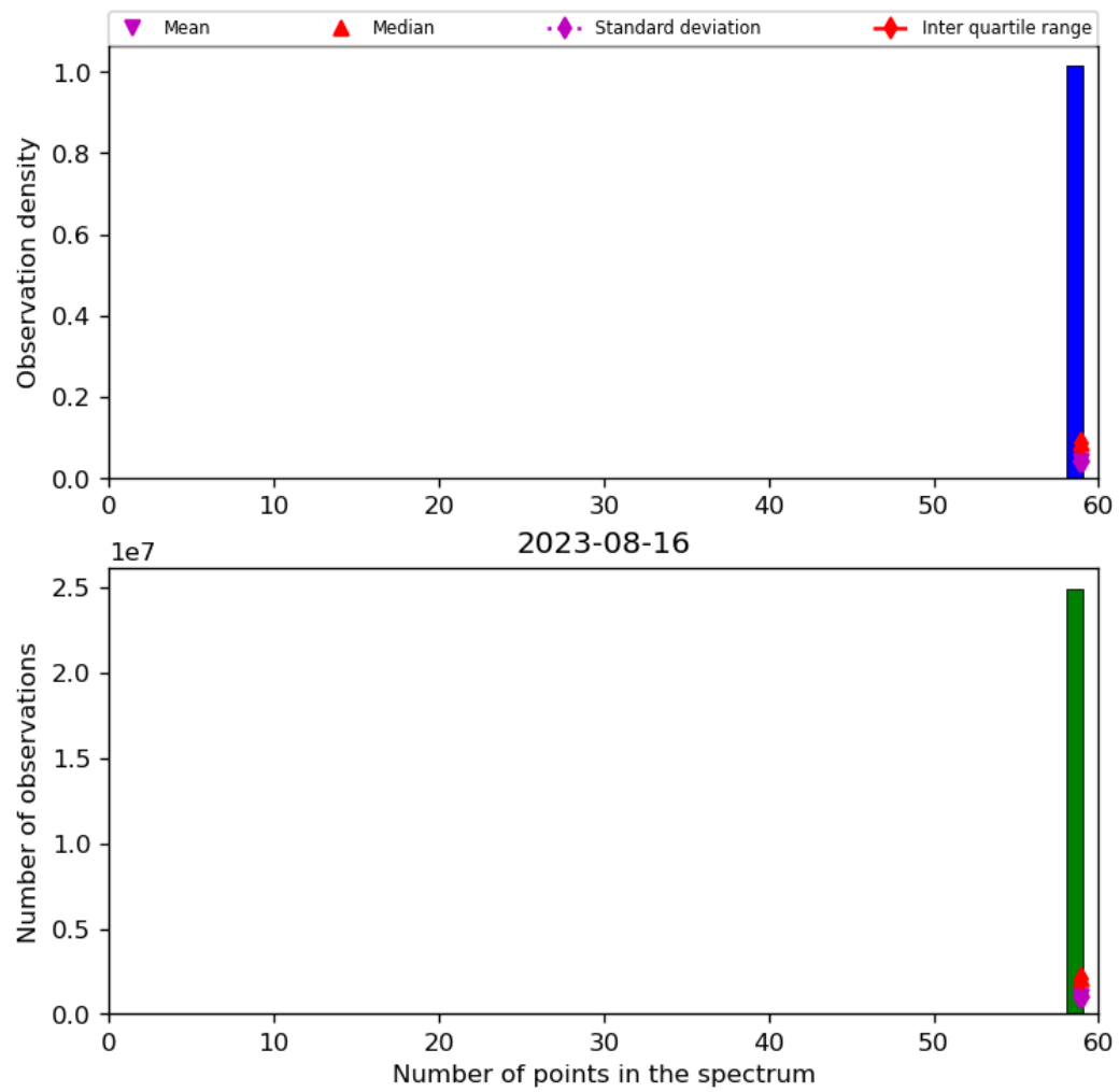
Figure 44: Histogram of “Number of points in the spectrum” for 2023-08-15 to 2023-08-17
