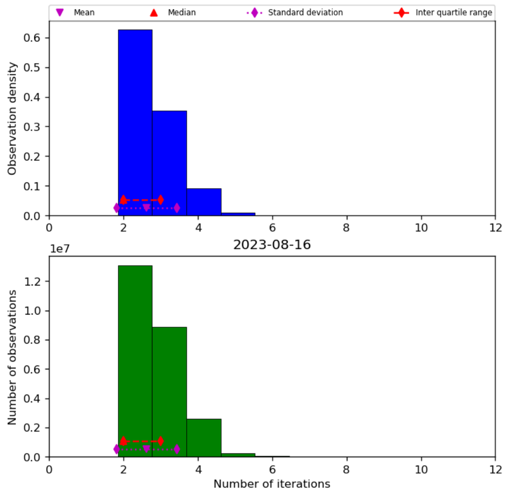
Figure 39: Histogram of “Number of iterations” for 2023-08-15 to 2023-08-17
