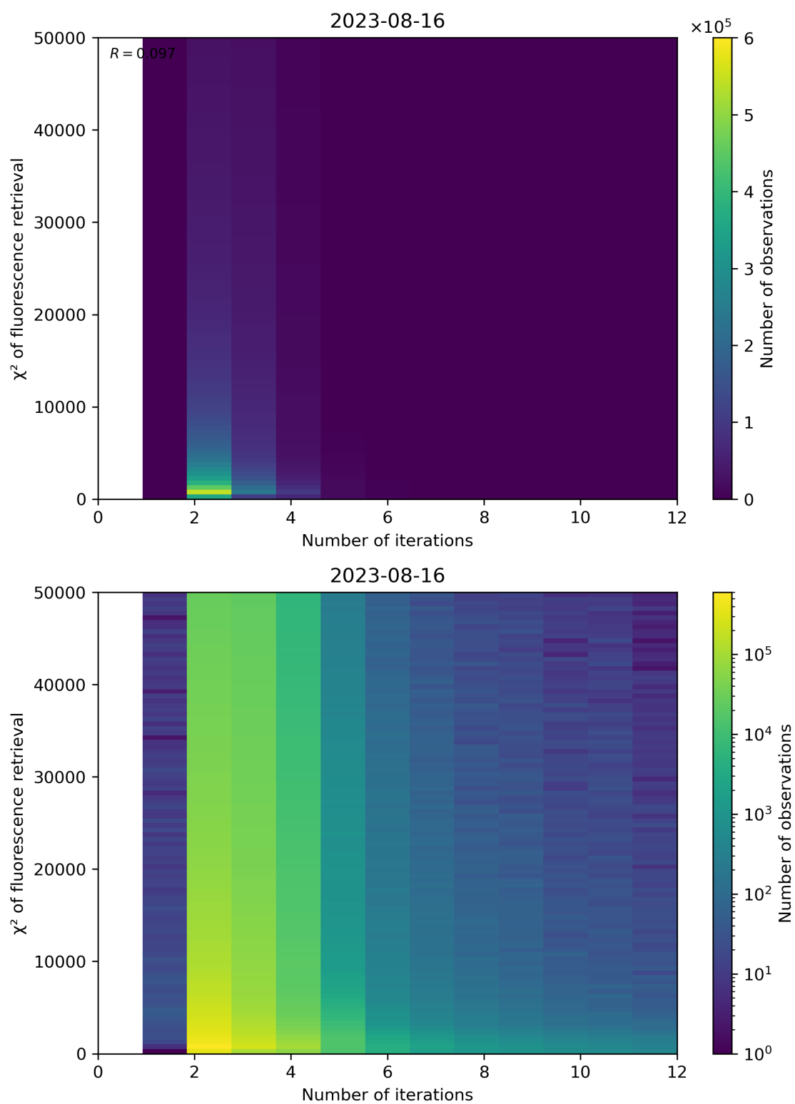
Figure 106: Scatter density plot of “Number of iterations” against “ \chi^2 of fluorescence retrieval” for 2023-08-15 to 2023-08-17.
