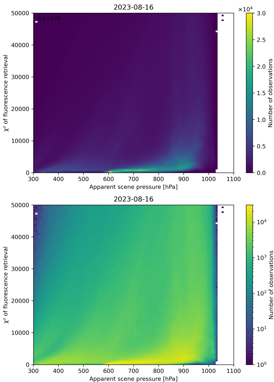
Figure 64: Scatter density plot of “Apparent scene pressure” against “ \chi^2 of fluorescence retrieval” for 2023-08-15 to 2023-08-17.
