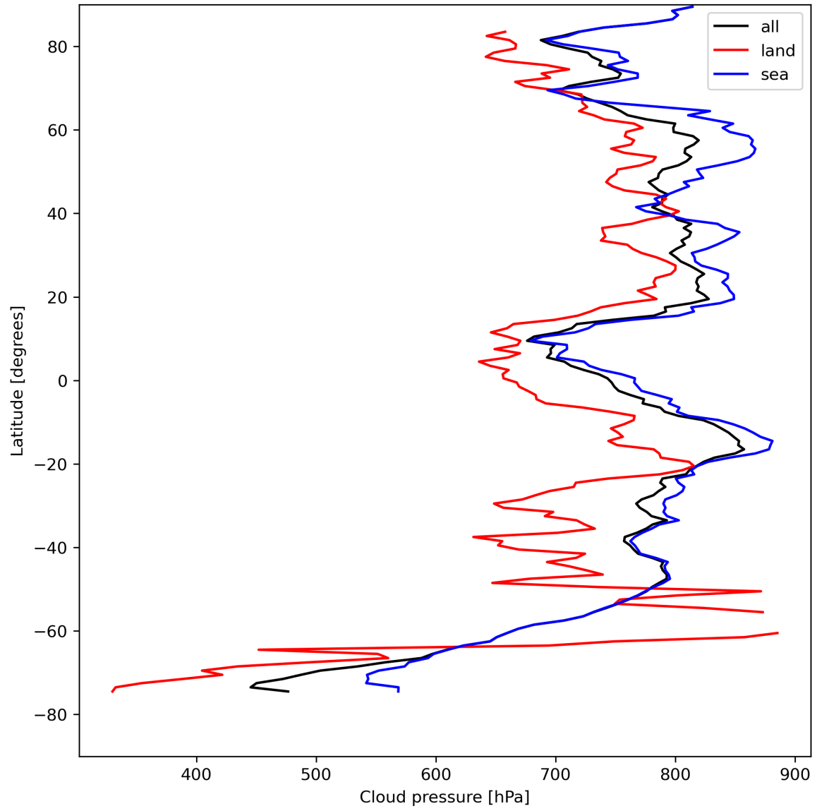
Figure 13: Zonal average of “Cloud pressure” for 2023-08-15 to 2023-08-17.
