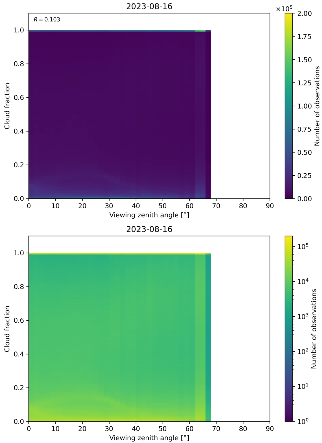
Figure 132: Scatter density plot of “Viewing zenith angle” against “Cloud fraction” for 2023-08-15 to 2023-08-17.
