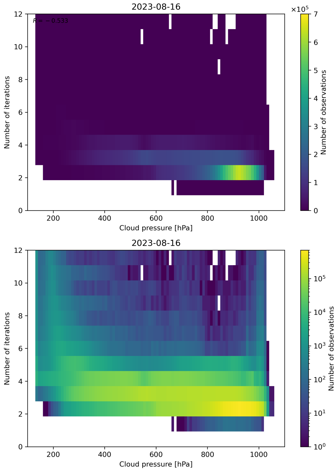
Figure 89: Scatter density plot of “Cloud pressure” against “Number of iterations” for 2023-08-15 to 2023-08-17.
