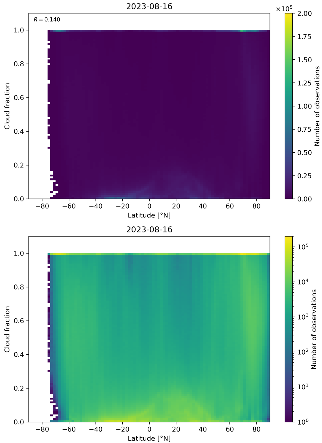
Figure 99: Scatter density plot of “Latitude” against “Cloud fraction” for 2023-08-15 to 2023-08-17.
