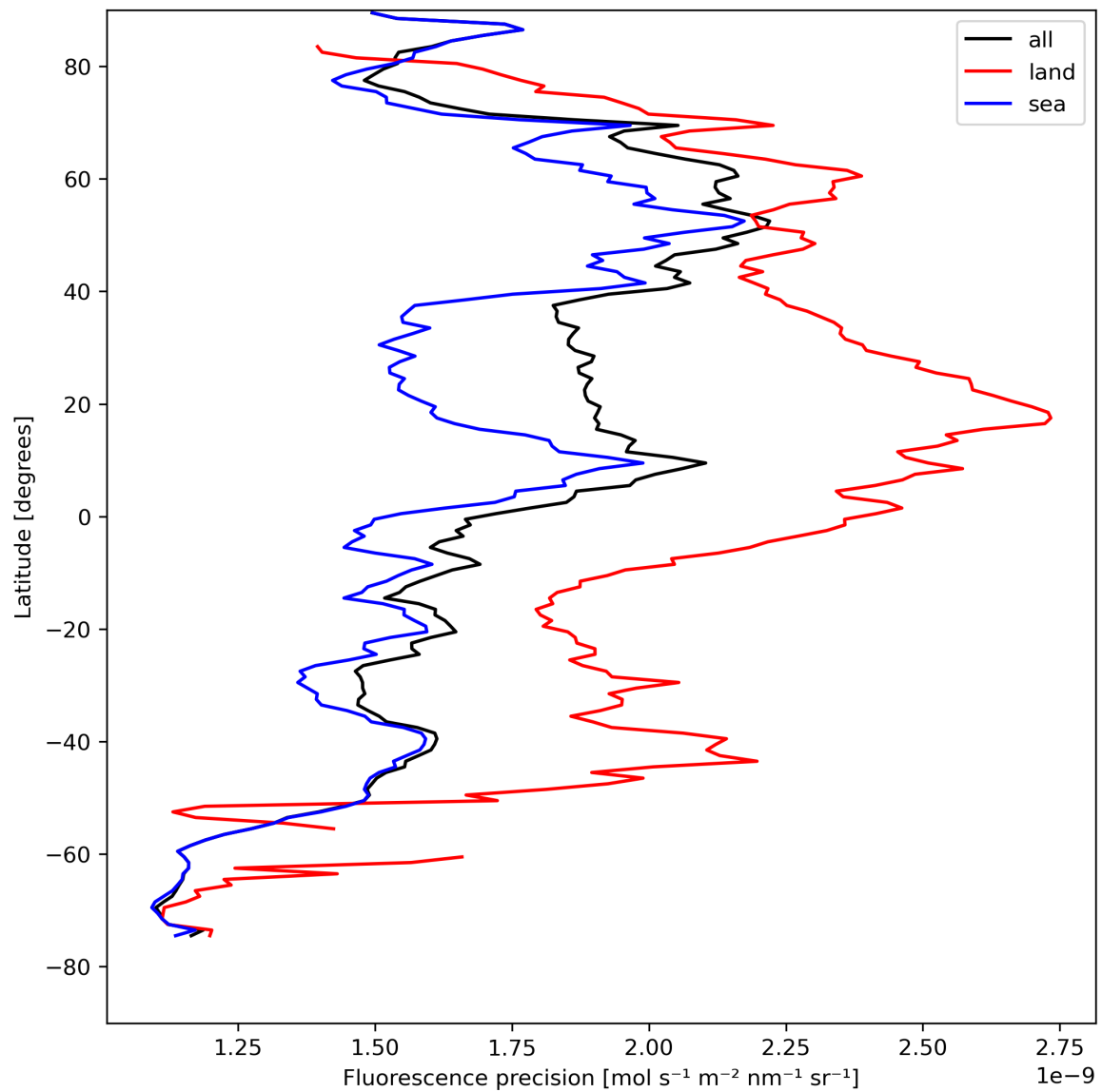
Figure 24: Zonal average of “Fluorescence precision” for 2023-08-15 to 2023-08-17.
