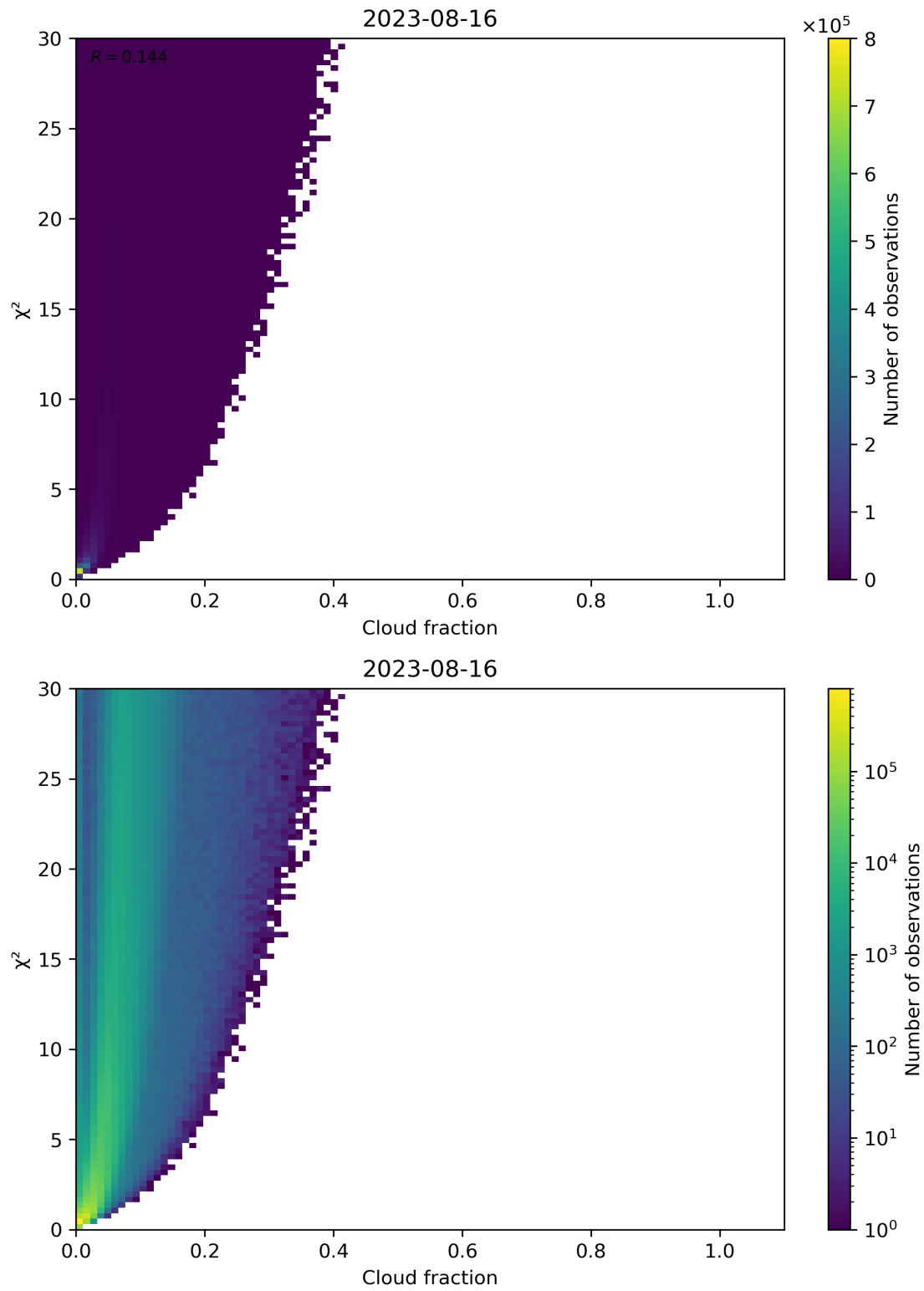
Figure 77: Scatter density plot of “Cloud fraction” against “ \chi^2 ” for 2023-08-15 to 2023-08-17.
