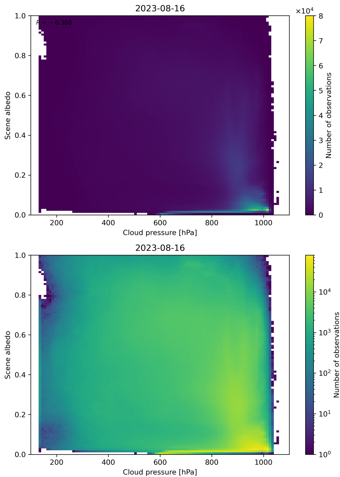
Figure 91: Scatter density plot of “Cloud pressure” against “Scene albedo” for 2023-08-15 to 2023-08-17.
