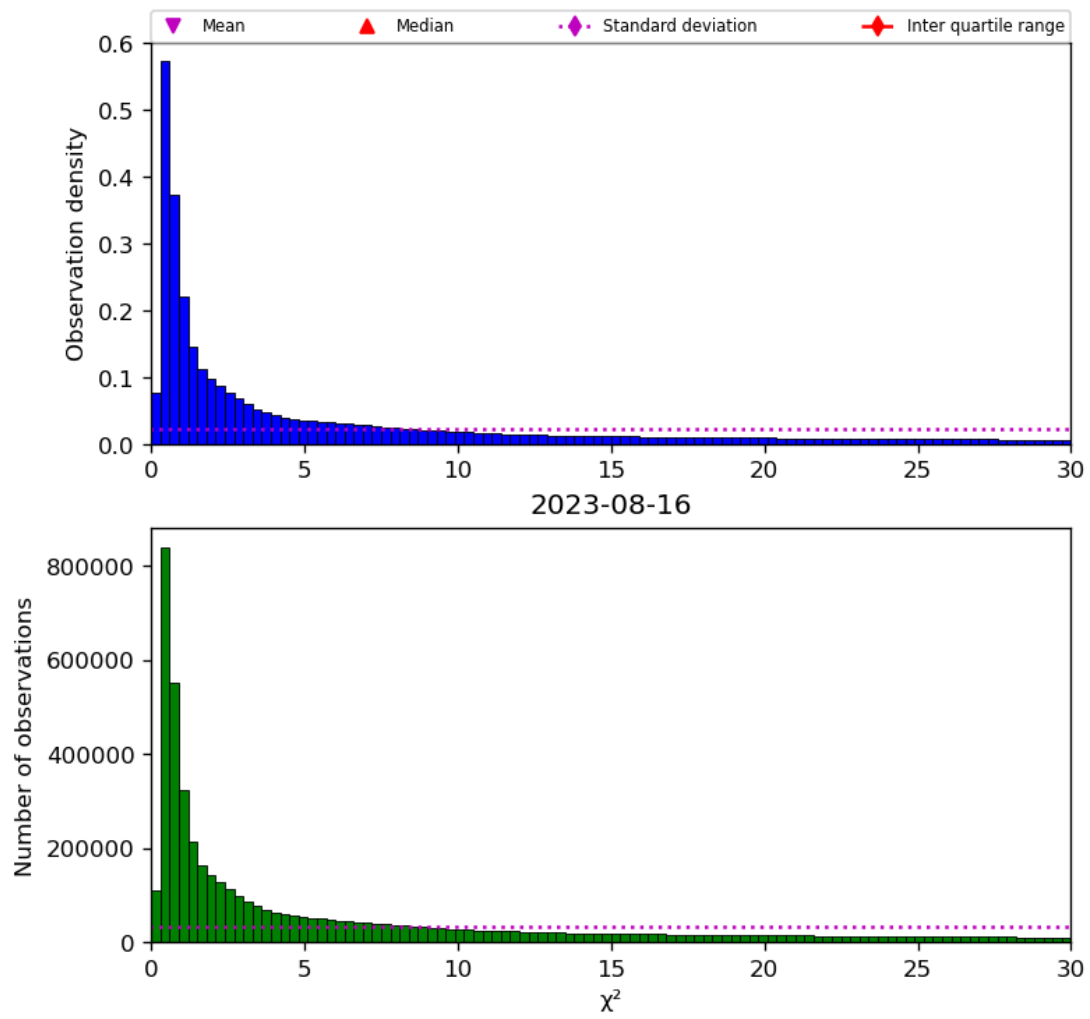
Figure 38: Histogram of “ \chi^2 ” for 2023-08-15 to 2023-08-17
