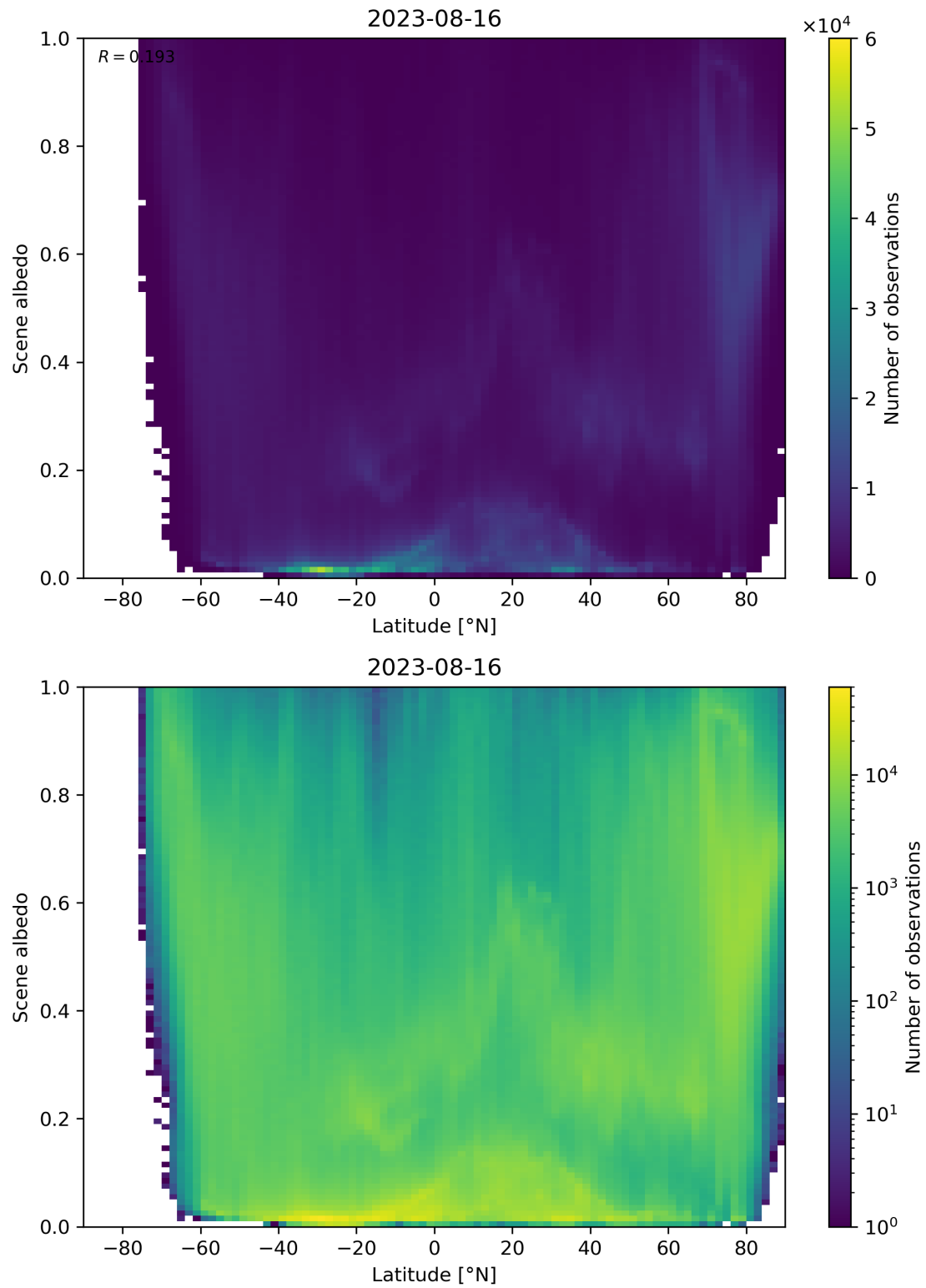
Figure 104: Scatter density plot of “Latitude” against “Scene albedo” for 2023-08-15 to 2023-08-17.
