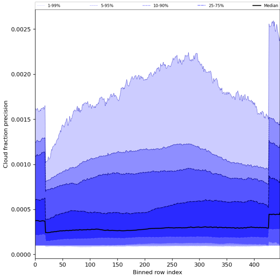
Figure 50: Along track statistics of “Cloud fraction precision” for 2023-08-15 to 2023-08-17
