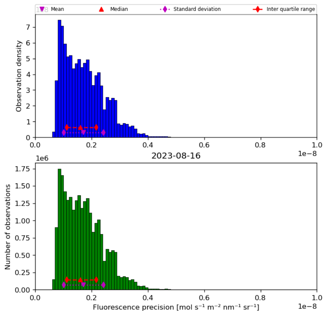
Figure 41: Histogram of “Fluorescence precision” for 2023-08-15 to 2023-08-17
