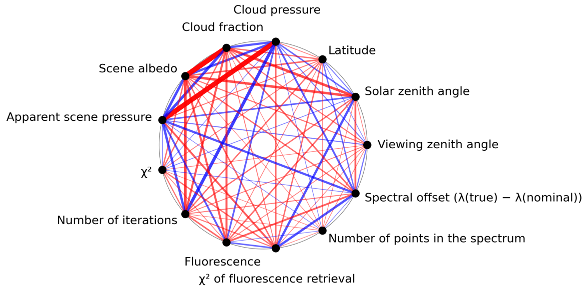
Figure 1: Map of correlation graph for 2023-08-15 to 2023-08-17.
