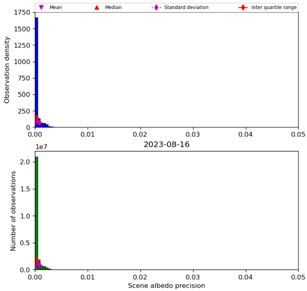
Figure 35: Histogram of “Scene albedo precision” for 2023-08-15 to 2023-08-17
