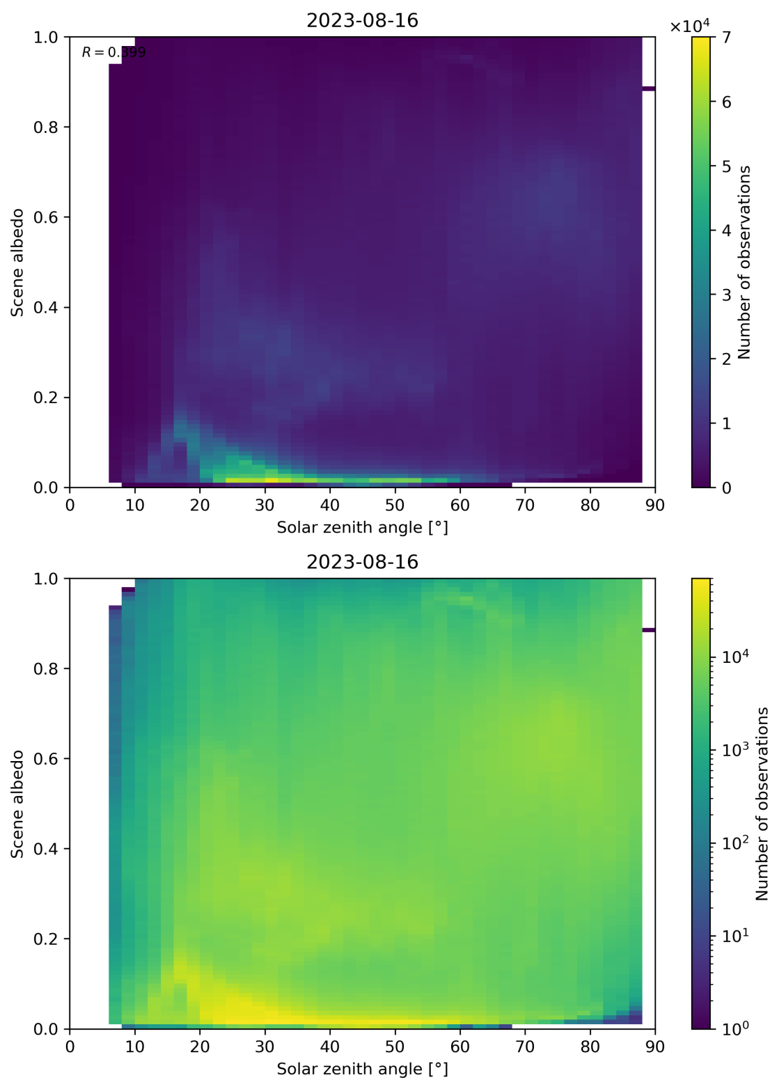
Figure 127: Scatter density plot of “Solar zenith angle” against “Scene albedo” for 2023-08-15 to 2023-08-17.
