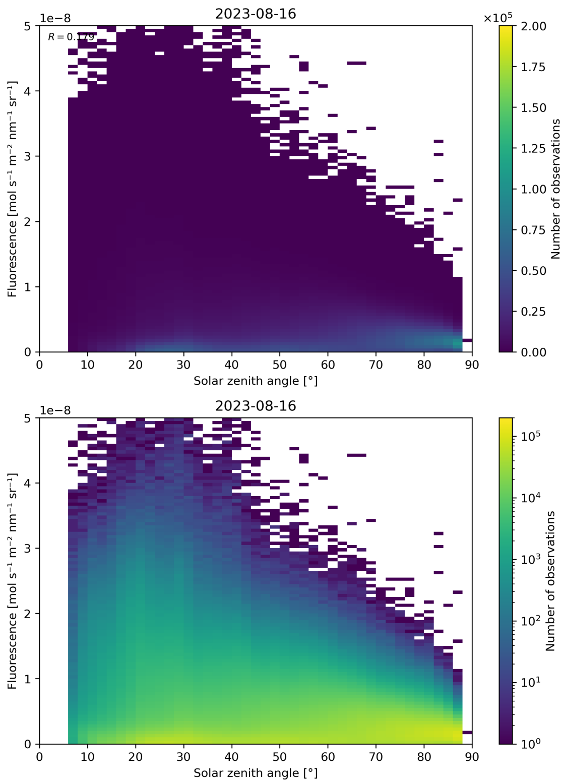
Figure 123: Scatter density plot of “Solar zenith angle” against “Fluorescence” for 2023-08-15 to 2023-08-17.
