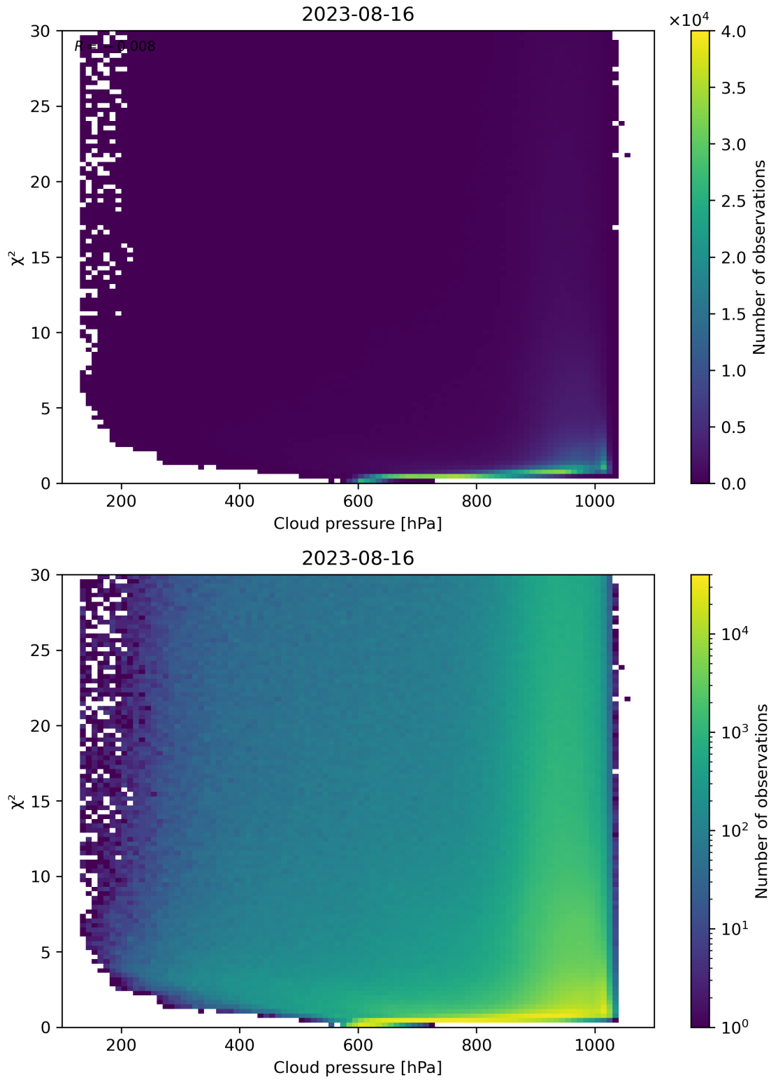
Figure 85: Scatter density plot of “Cloud pressure” against “ \chi^2 ” for 2023-08-15 to 2023-08-17.
