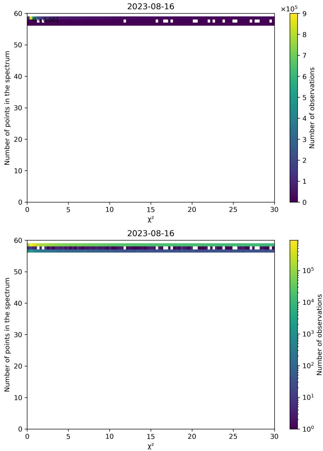
Figure 74: Scatter density plot of “ \chi^2 ” against “Number of points in the spectrum” for 2023-08-15 to 2023-08-17.
