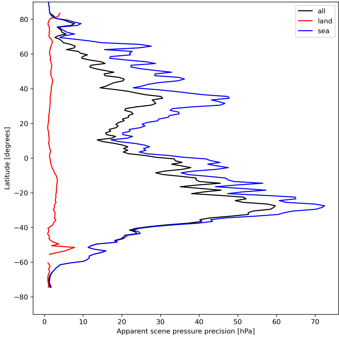
Figure 20: Zonal average of “Apparent scene pressure precision” for 2023-08-15 to 2023-08-17.
