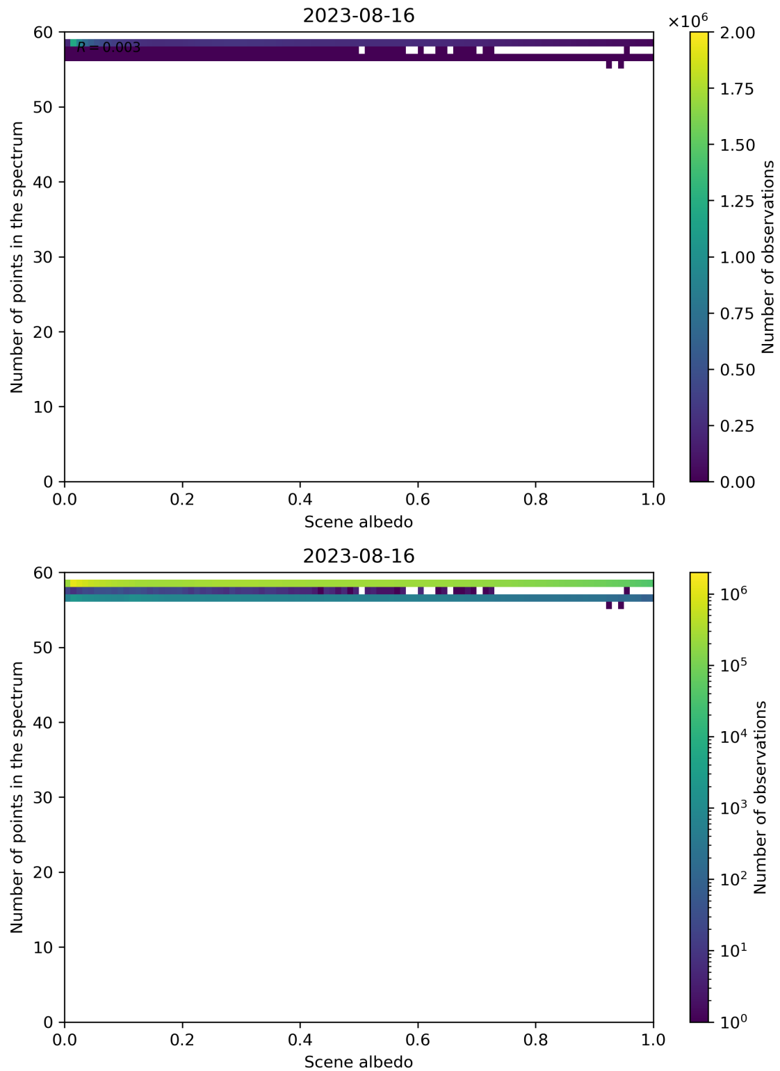
Figure 116: Scatter density plot of “Scene albedo” against “Number of points in the spectrum” for 2023-08-15 to 2023-08-17.
