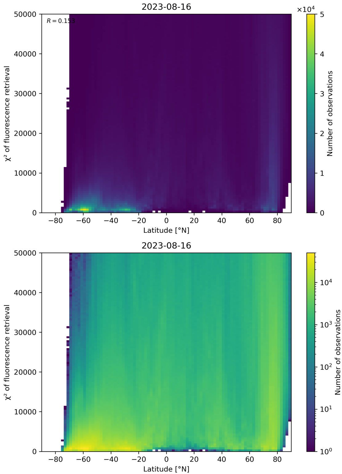
Figure 98: Scatter density plot of “Latitude” against “ \chi^2 of fluorescence retrieval” for 2023-08-15 to 2023-08-17.
