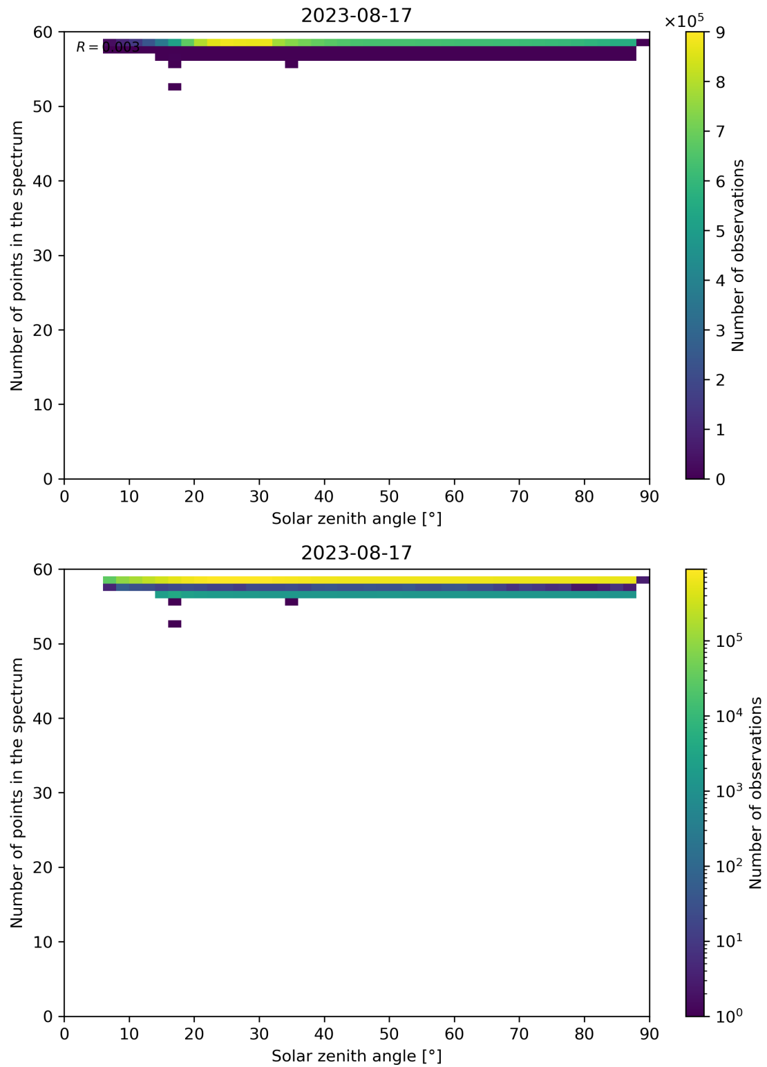
Figure 126: Scatter density plot of “Solar zenith angle” against “Number of points in the spectrum” for 2023-08-16 to 2023-08-18.
