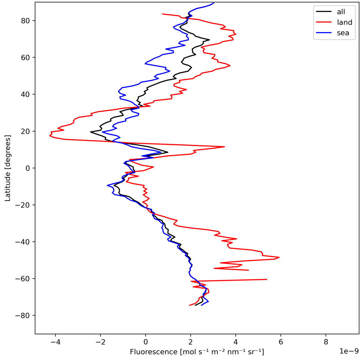
Figure 23: Zonal average of “Fluorescence” for 2023-08-16 to 2023-08-18.
