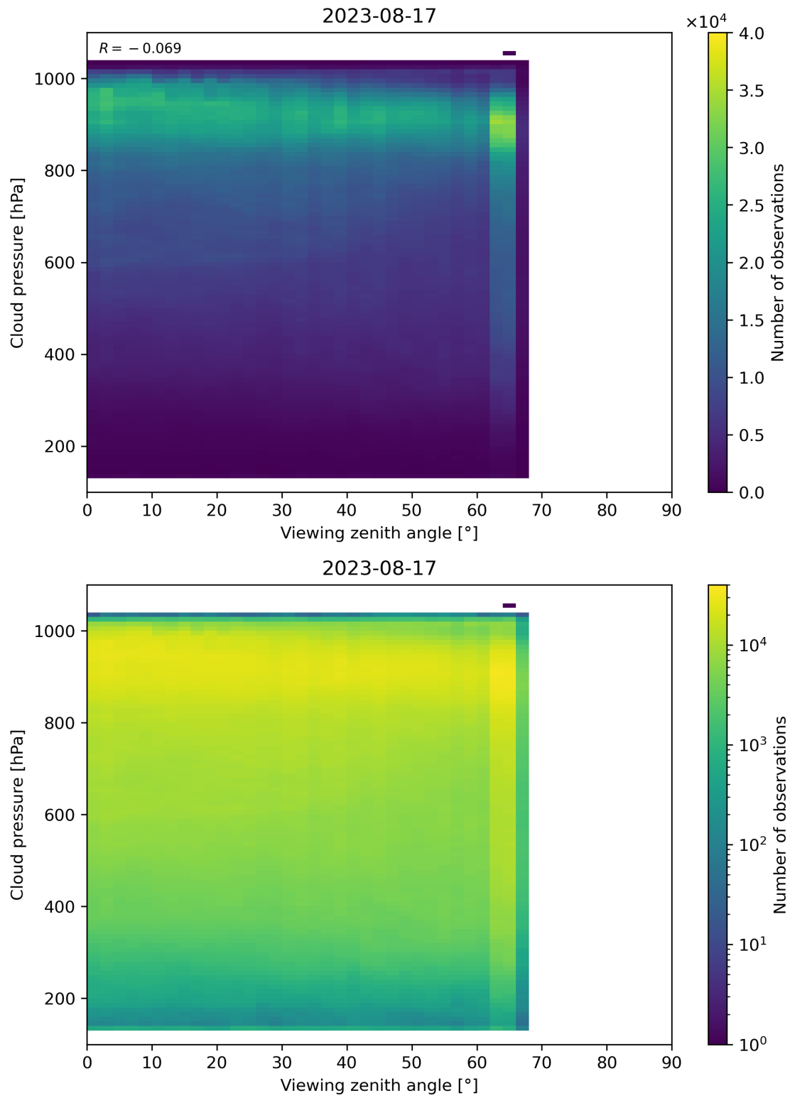
Figure 133: Scatter density plot of “Viewing zenith angle” against “Cloud pressure” for 2023-08-16 to 2023-08-18.
