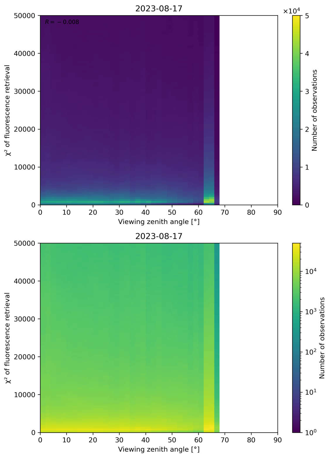
Figure 131: Scatter density plot of “Viewing zenith angle” against “ \chi^2 of fluorescence retrieval” for 2023-08-16 to 2023-08-18.
