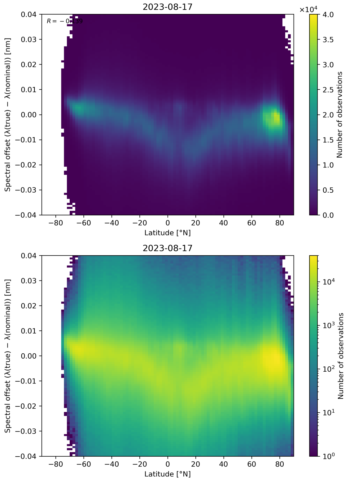
Figure 105: Scatter density plot of “Latitude” against “Spectral offset ( \lambda(\text{true}) - \lambda(\text{nominal}) )” for 2023-08-16 to 2023-08-18.
