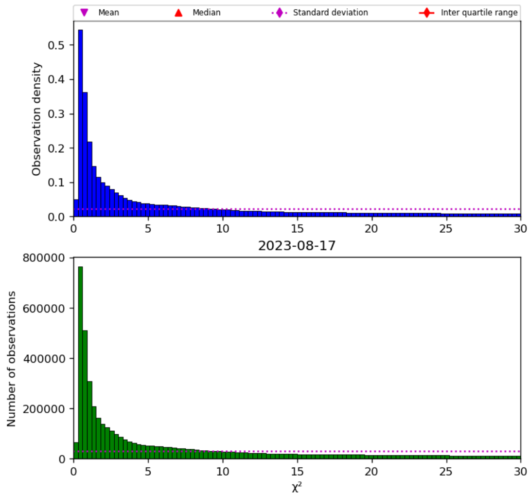
Figure 38: Histogram of “ \chi^2 ” for 2023-08-16 to 2023-08-18
