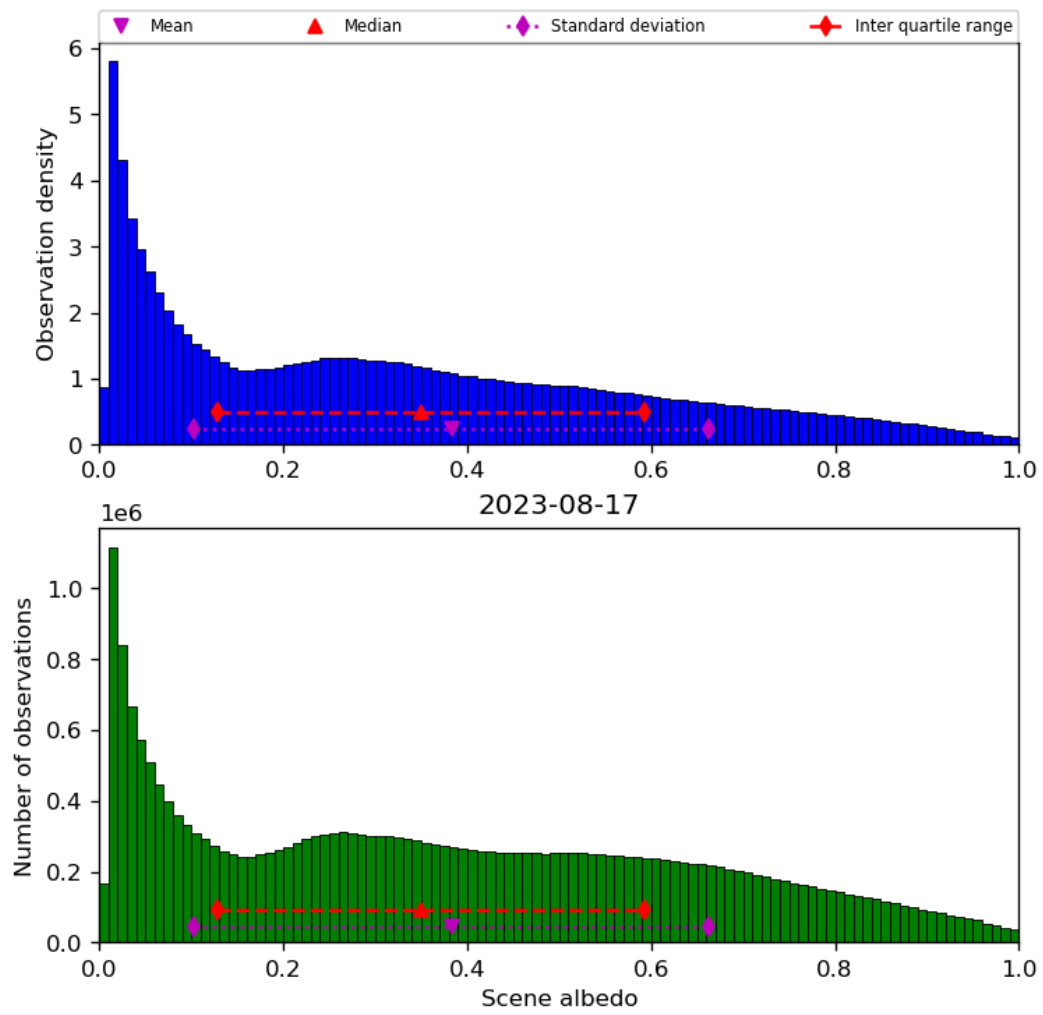
Figure 34: Histogram of “Scene albedo” for 2023-08-16 to 2023-08-18
