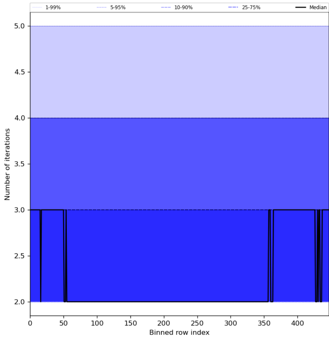
Figure 56: Along track statistics of “Number of iterations” for 2023-08-16 to 2023-08-18
