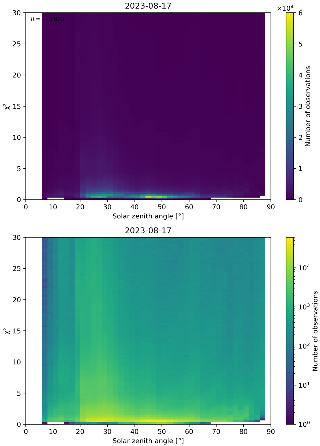
Figure 119: Scatter density plot of “Solar zenith angle” against “ \chi^2 ” for 2023-08-16 to 2023-08-18.
