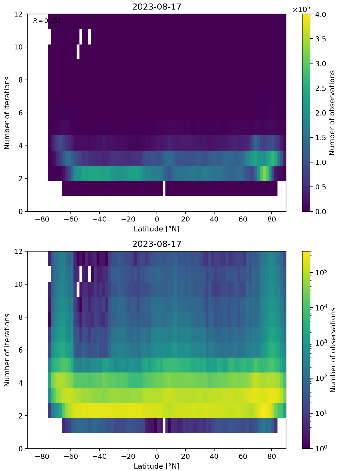
Figure 102: Scatter density plot of “Latitude” against “Number of iterations” for 2023-08-16 to 2023-08-18.
