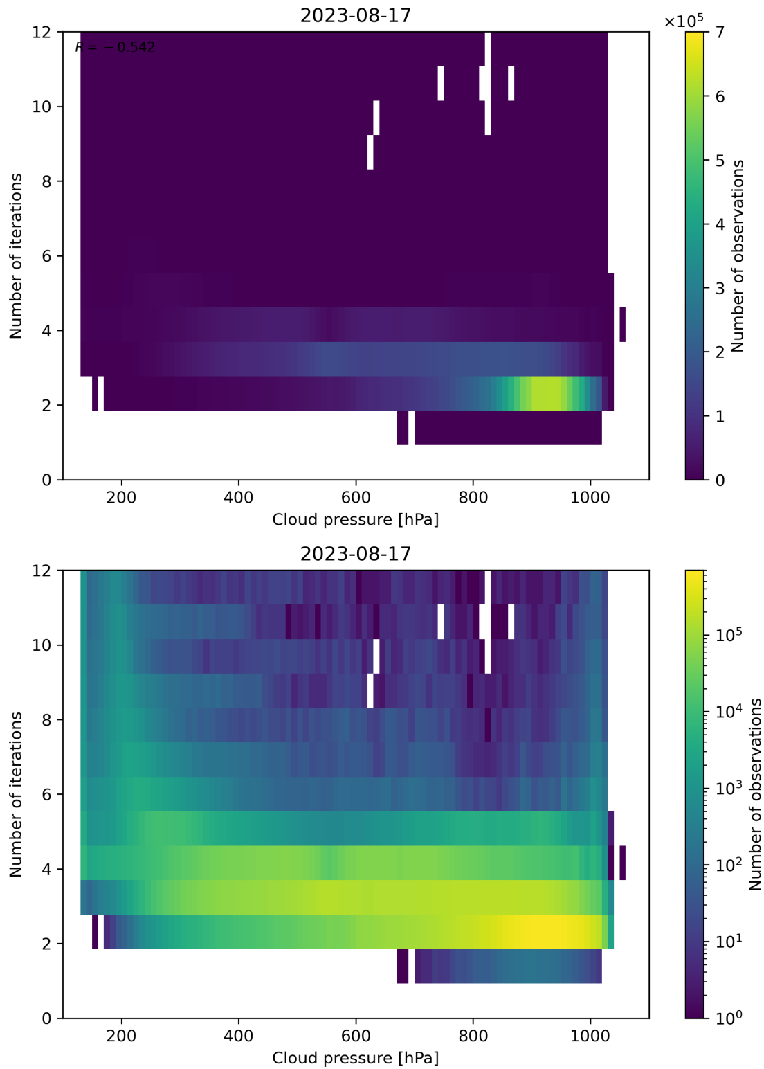
Figure 89: Scatter density plot of “Cloud pressure” against “Number of iterations” for 2023-08-16 to 2023-08-18.
