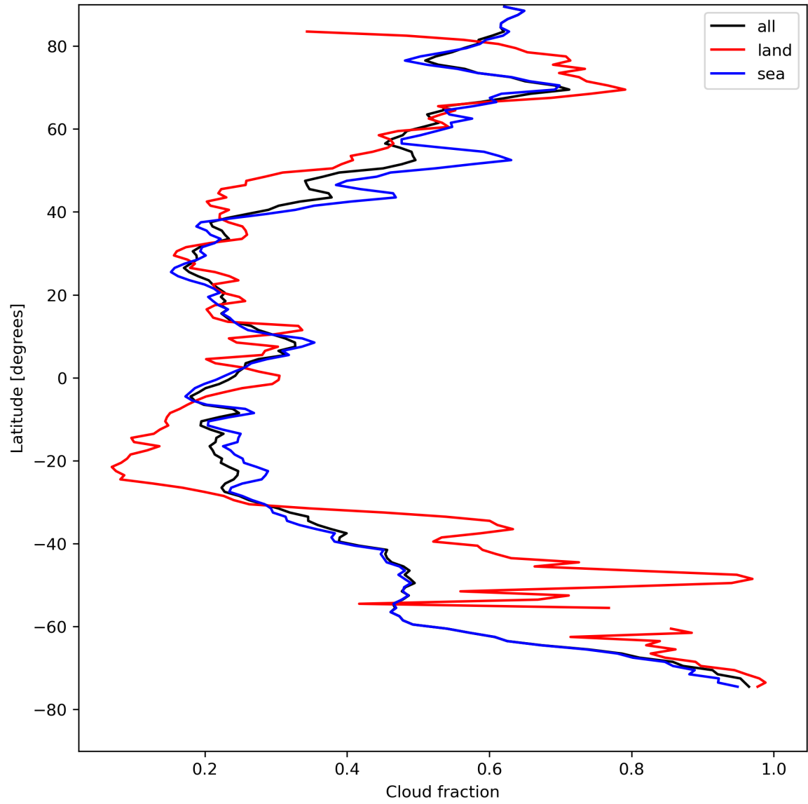
Figure 15: Zonal average of “Cloud fraction” for 2023-08-16 to 2023-08-18.
