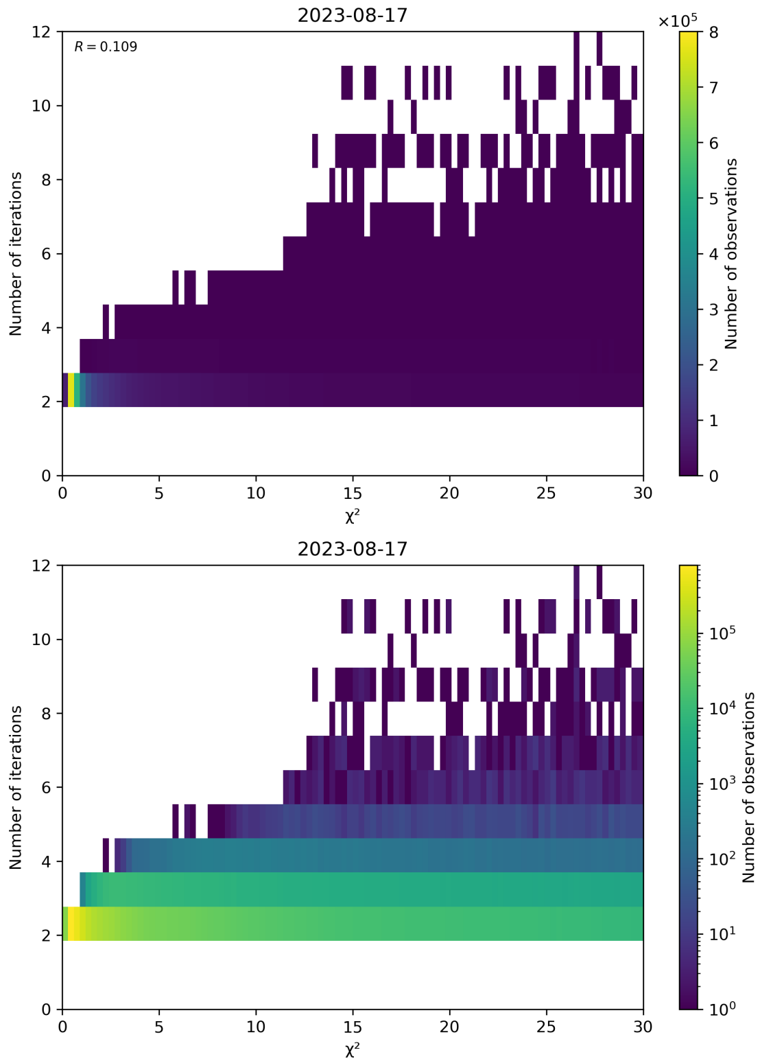
Figure 73: Scatter density plot of “ \chi^2 ” against “Number of iterations” for 2023-08-16 to 2023-08-18.
