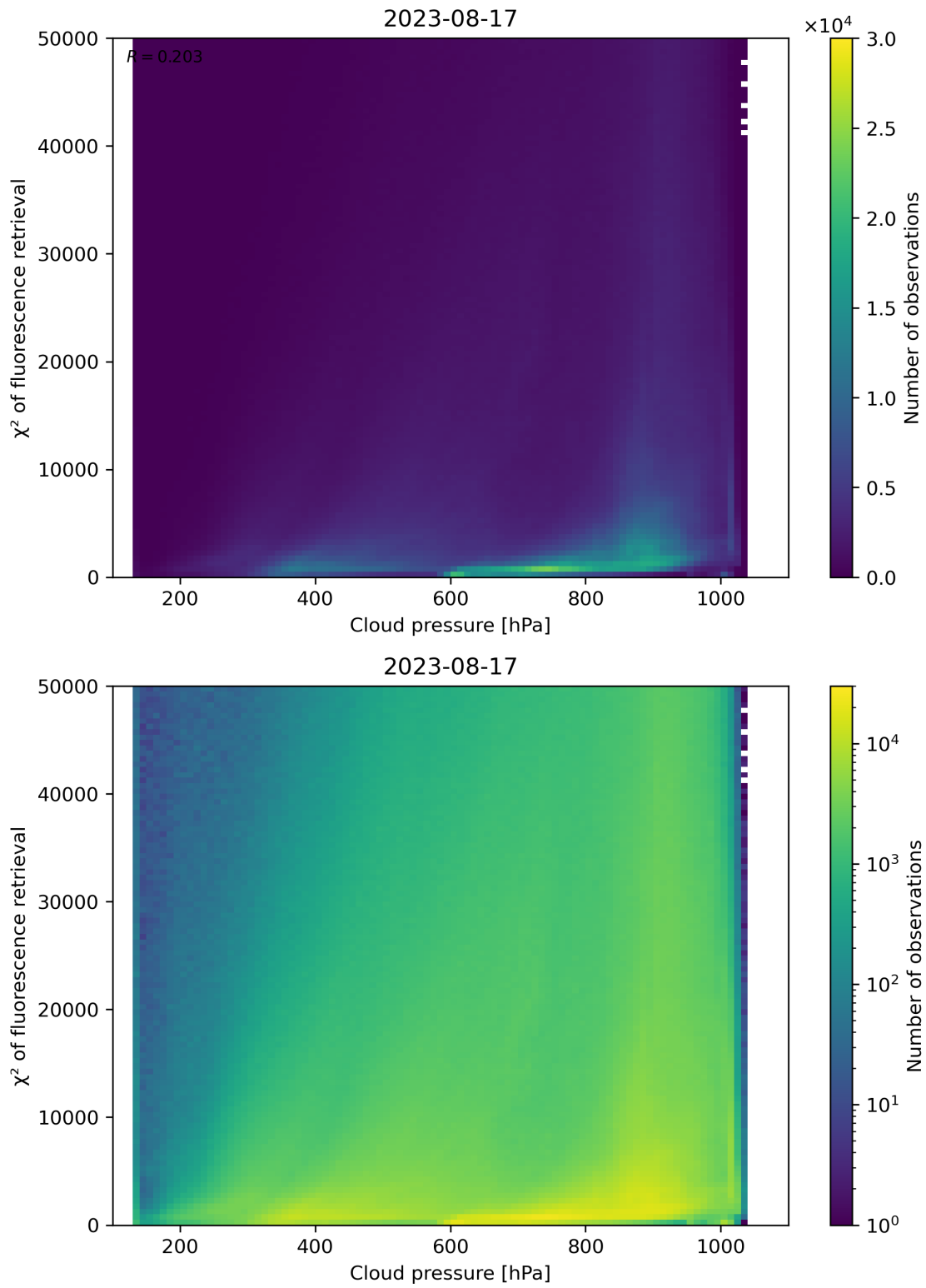
Figure 86: Scatter density plot of “Cloud pressure” against “ \chi^2 of fluorescence retrieval” for 2023-08-16 to 2023-08-18.
