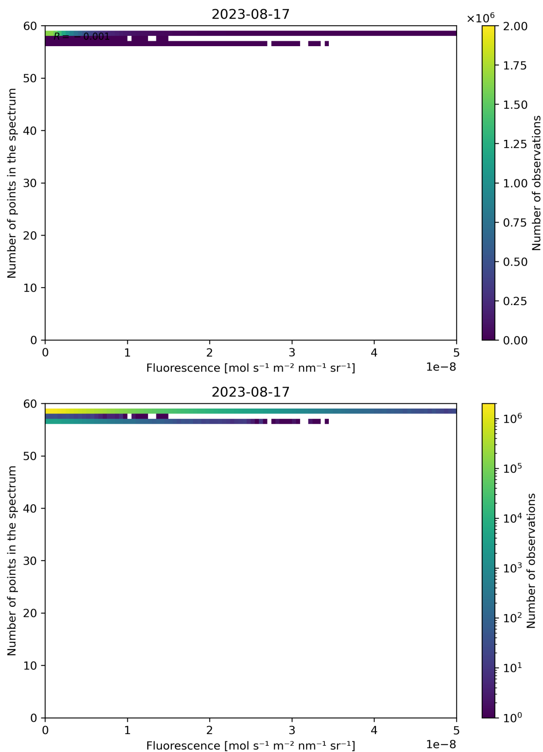
Figure 94: Scatter density plot of “Fluorescence” against “Number of points in the spectrum” for 2023-08-16 to 2023-08-18.
