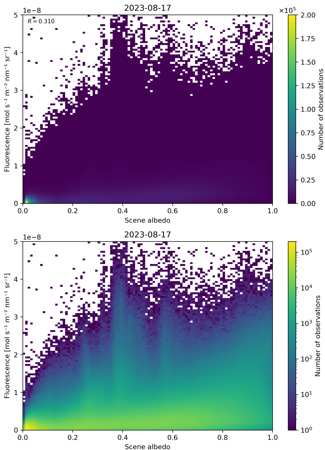
Figure 114: Scatter density plot of “Scene albedo” against “Fluorescence” for 2023-08-16 to 2023-08-18.
