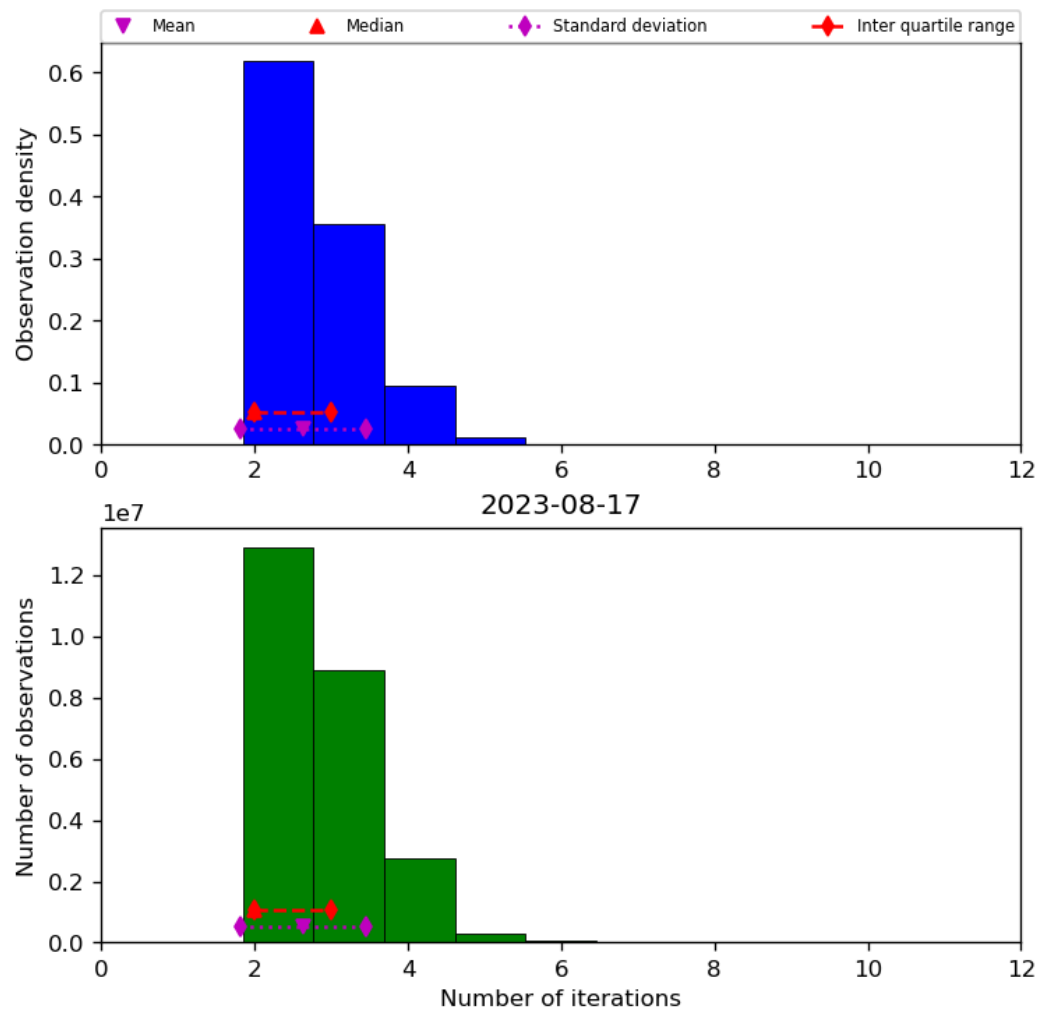
Figure 39: Histogram of “Number of iterations” for 2023-08-16 to 2023-08-18
