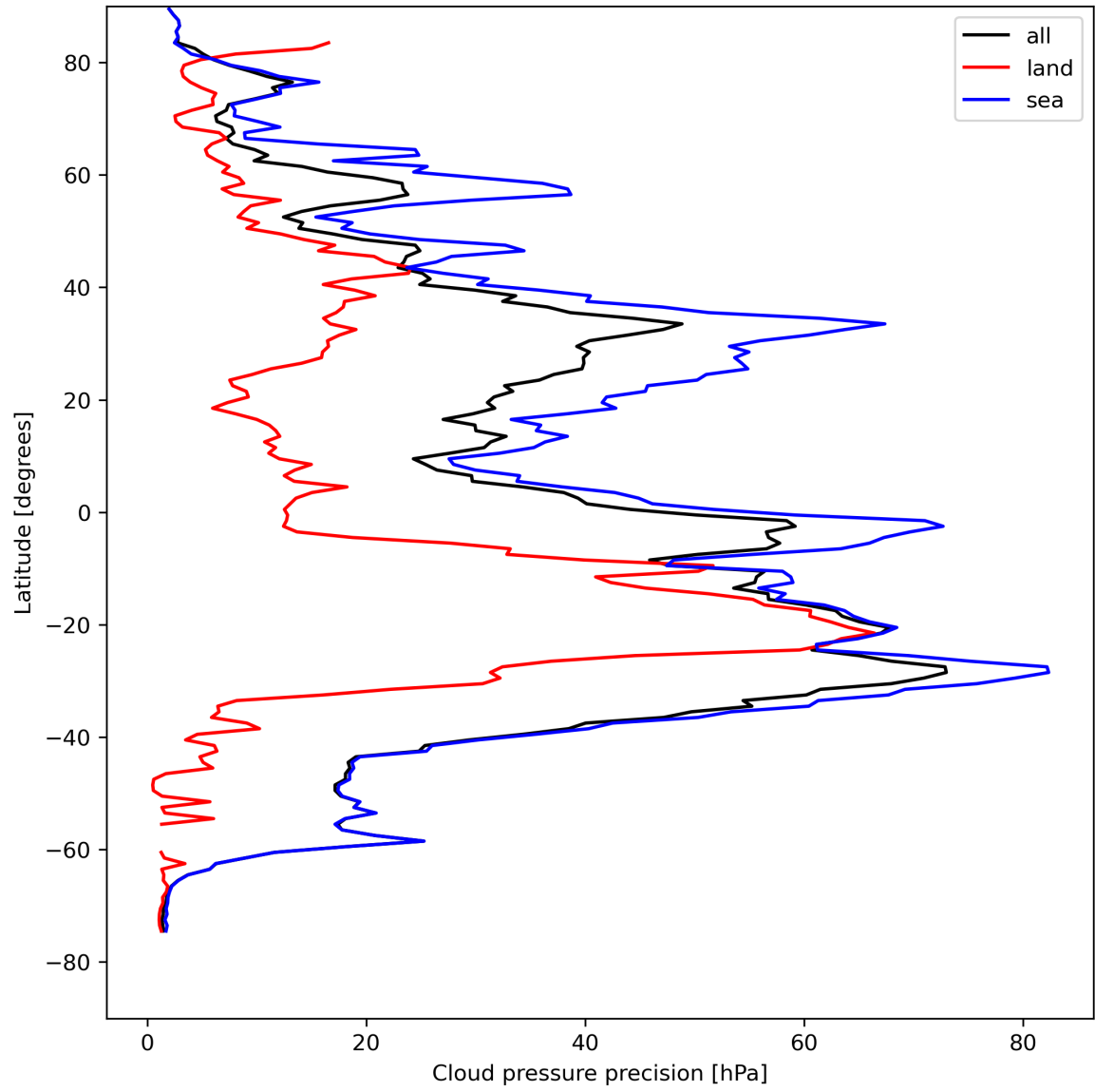
Figure 14: Zonal average of “Cloud pressure precision” for 2023-08-16 to 2023-08-18.
