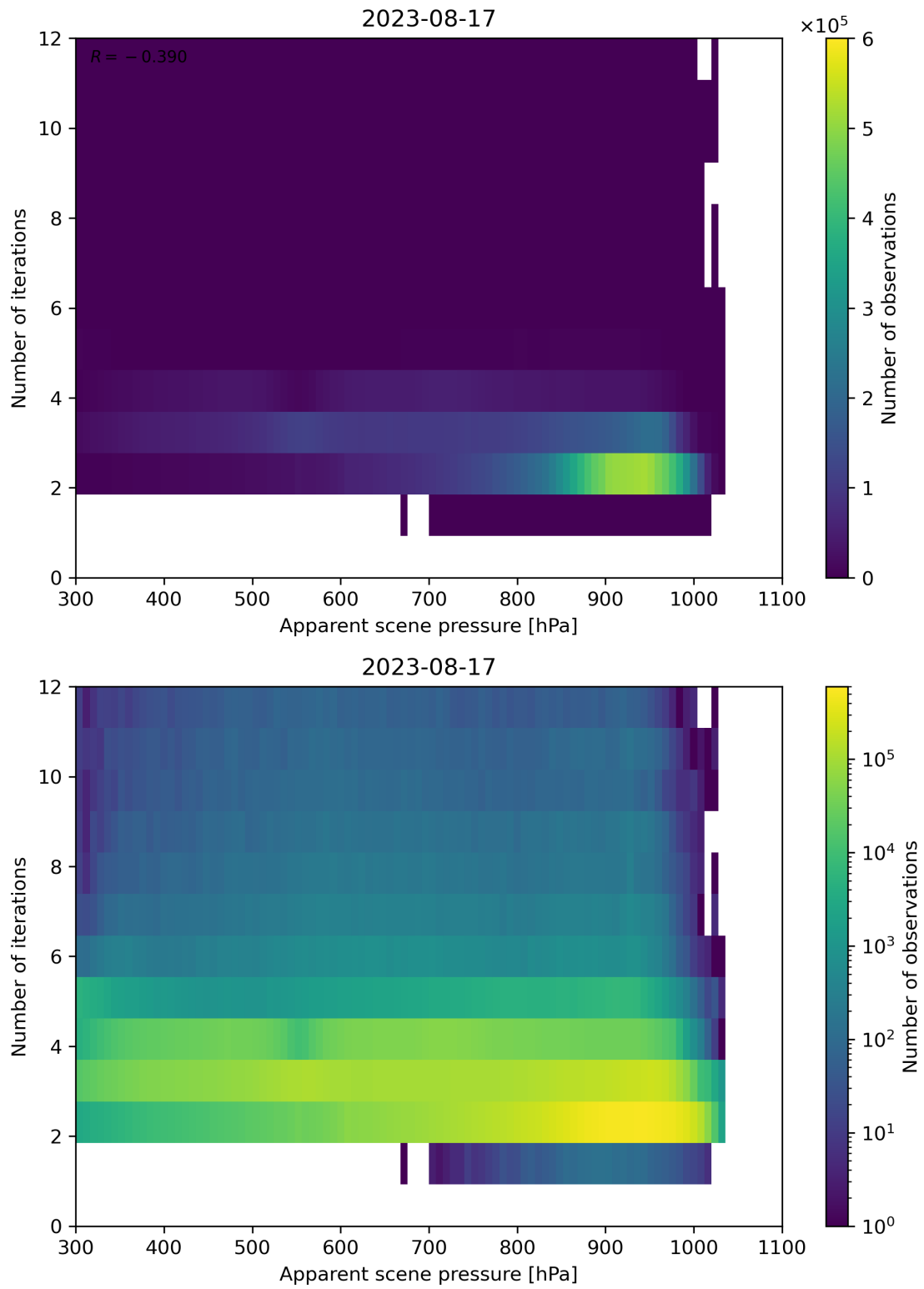
Figure 66: Scatter density plot of “Apparent scene pressure” against “Number of iterations” for 2023-08-16 to 2023-08-18.
