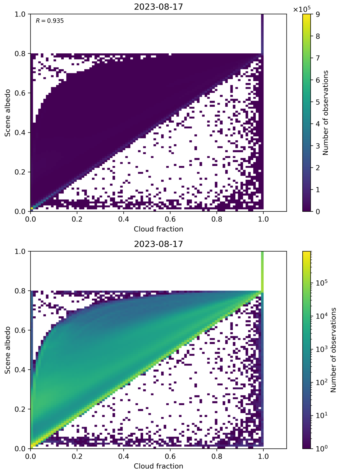
Figure 82: Scatter density plot of “Cloud fraction” against “Scene albedo” for 2023-08-16 to 2023-08-18.
