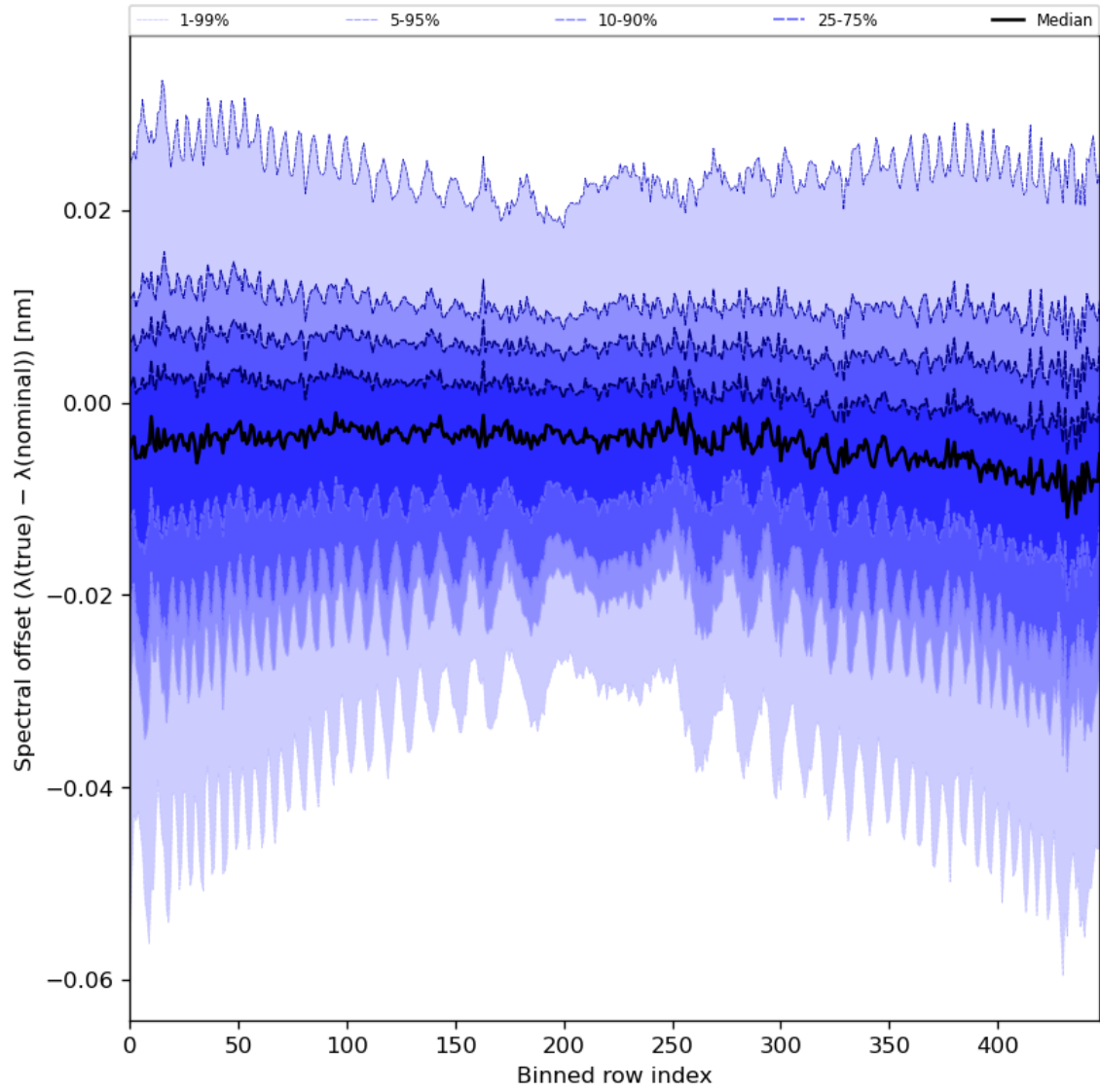
Figure 62: Along track statistics of “Spectral offset ( \lambda(\text{true}) - \lambda(\text{nominal}) )” for 2023-08-16 to 2023-08-18
