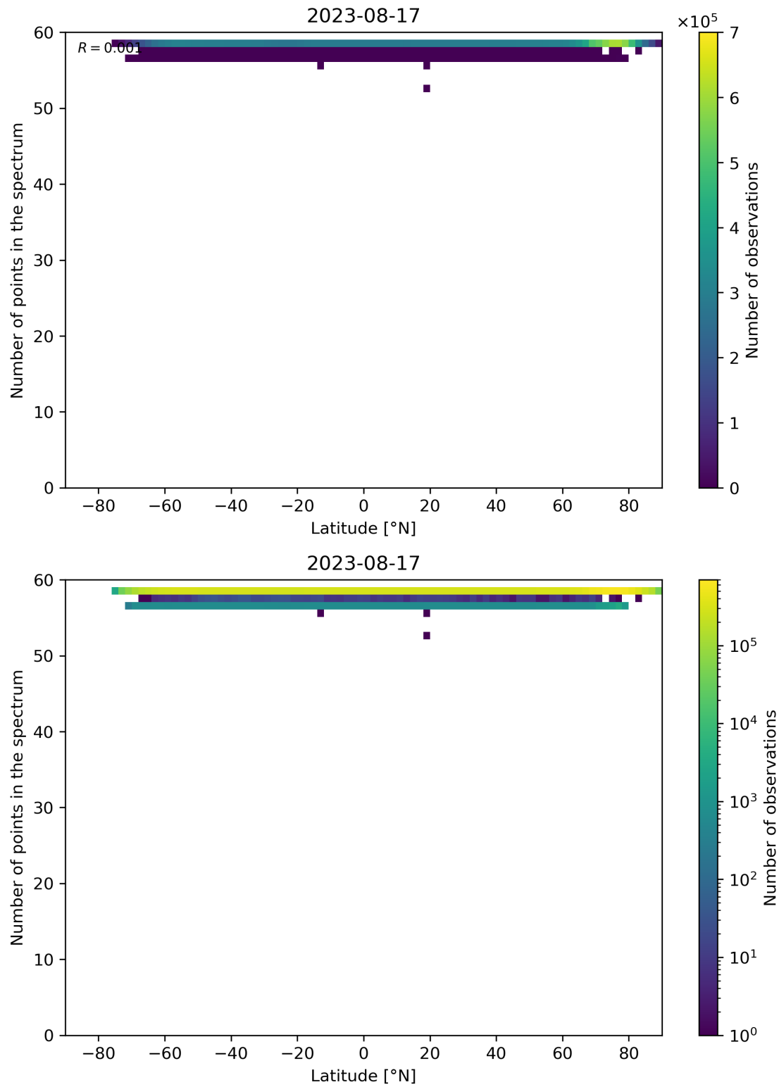
Figure 103: Scatter density plot of “Latitude” against “Number of points in the spectrum” for 2023-08-16 to 2023-08-18.
