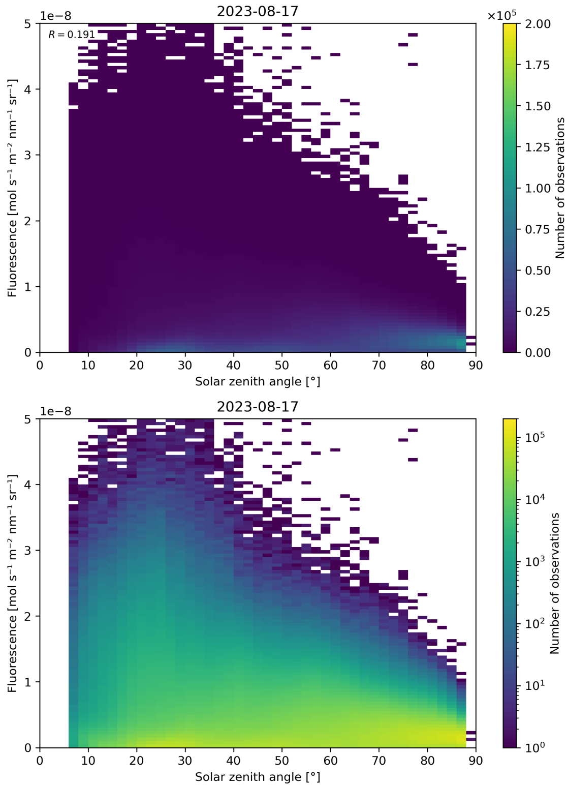
Figure 123: Scatter density plot of “Solar zenith angle” against “Fluorescence” for 2023-08-16 to 2023-08-18.
