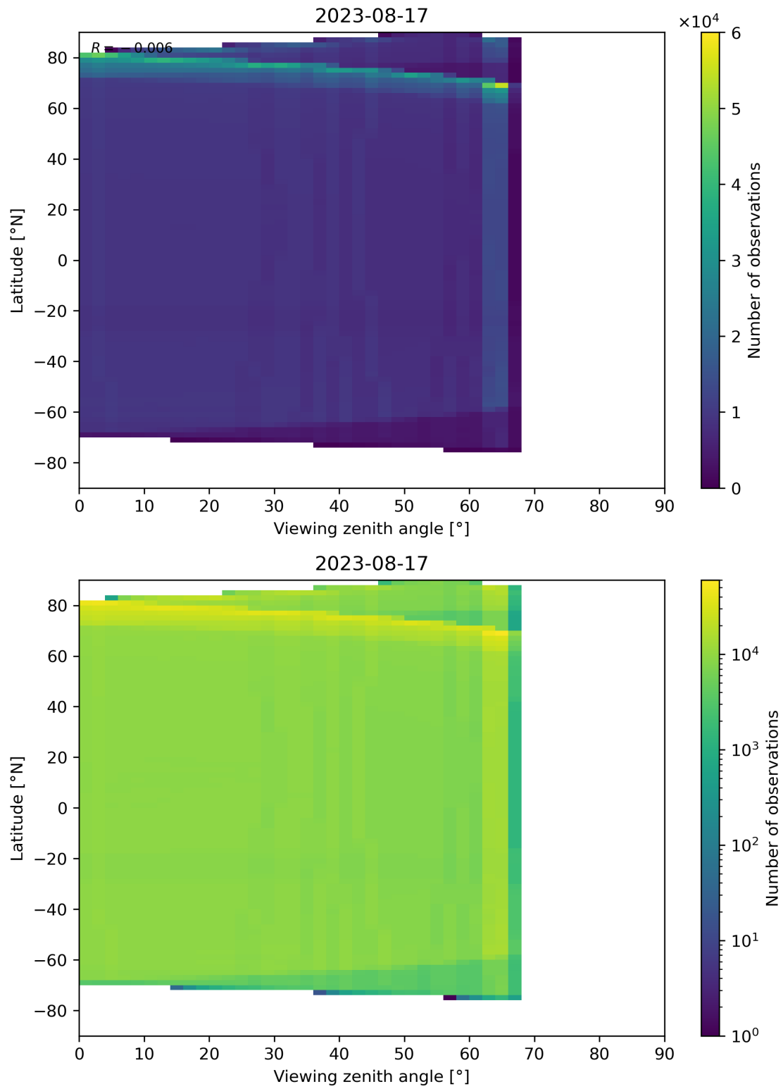
Figure 135: Scatter density plot of “Viewing zenith angle” against “Latitude” for 2023-08-16 to 2023-08-18.
