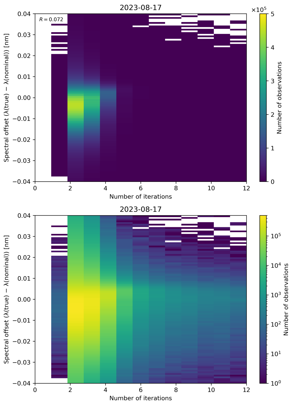
Figure 109: Scatter density plot of “Number of iterations” against “Spectral offset ( \lambda(\text{true}) - \lambda(\text{nominal}) )” for 2023-08-16 to 2023-08-18.
