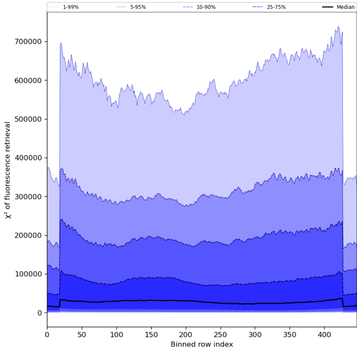
Figure 59: Along track statistics of “ \chi^2 of fluorescence retrieval” for 2023-08-16 to 2023-08-18
