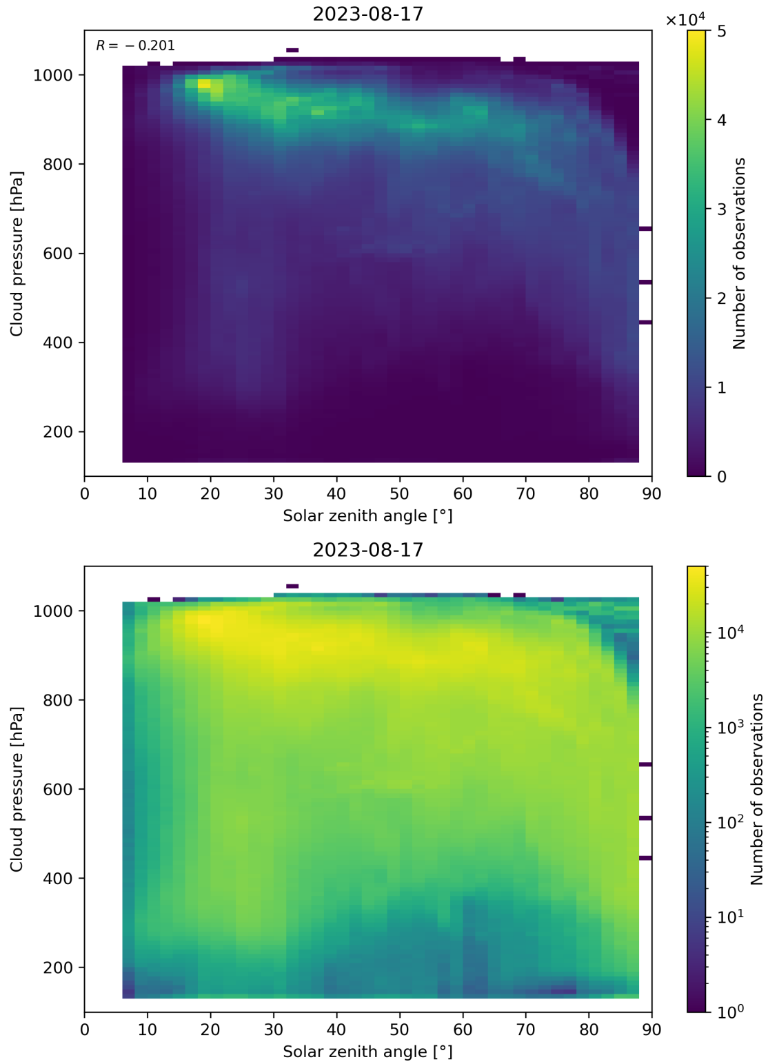
Figure 122: Scatter density plot of “Solar zenith angle” against “Cloud pressure” for 2023-08-16 to 2023-08-18.
