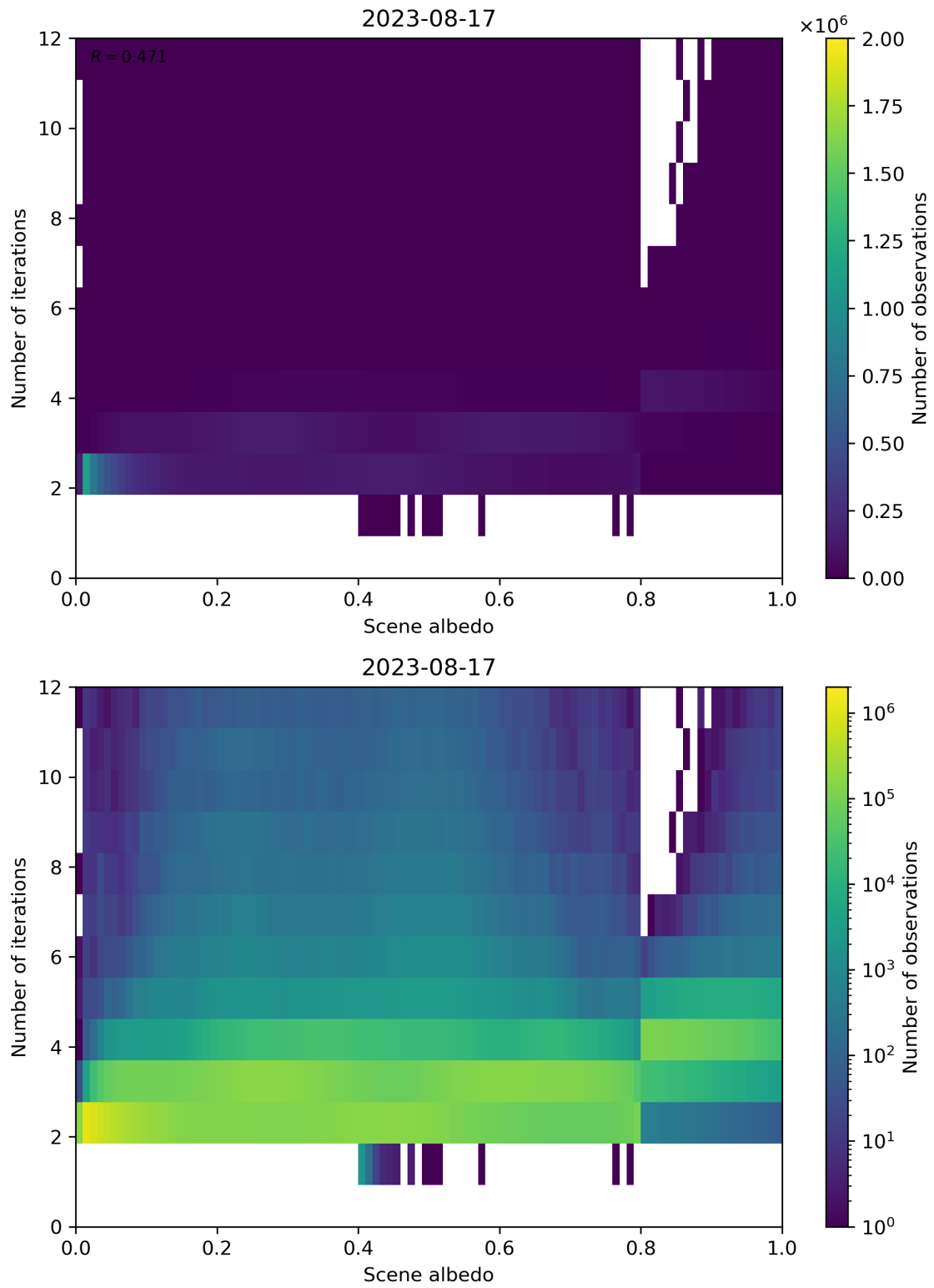
Figure 115: Scatter density plot of “Scene albedo” against “Number of iterations” for 2023-08-16 to 2023-08-18.
