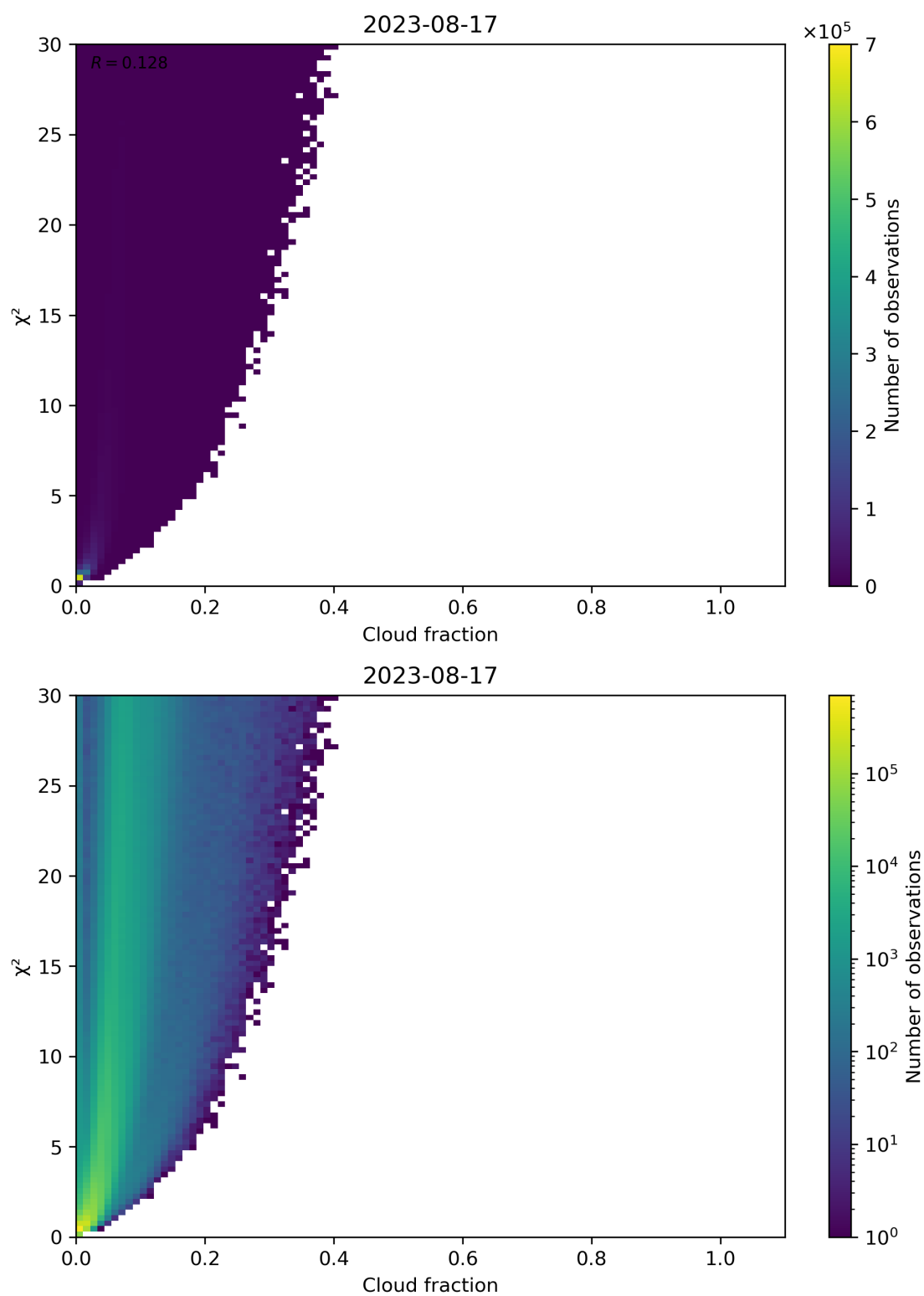
Figure 77: Scatter density plot of “Cloud fraction” against “ \chi^2 ” for 2023-08-16 to 2023-08-18.
