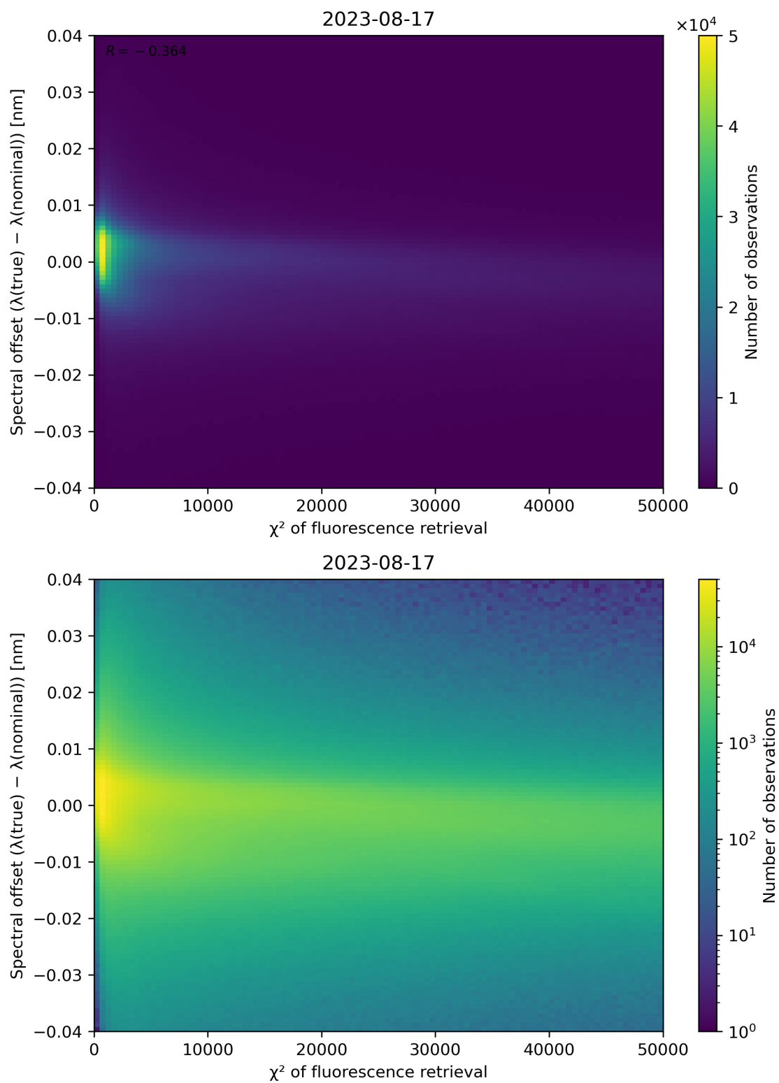
Figure 72: Scatter density plot of “ \chi^2 of fluorescence retrieval” against “Spectral offset ( \lambda(\text{true}) - \lambda(\text{nominal}) )” for 2023-08-16 to 2023-08-18.
