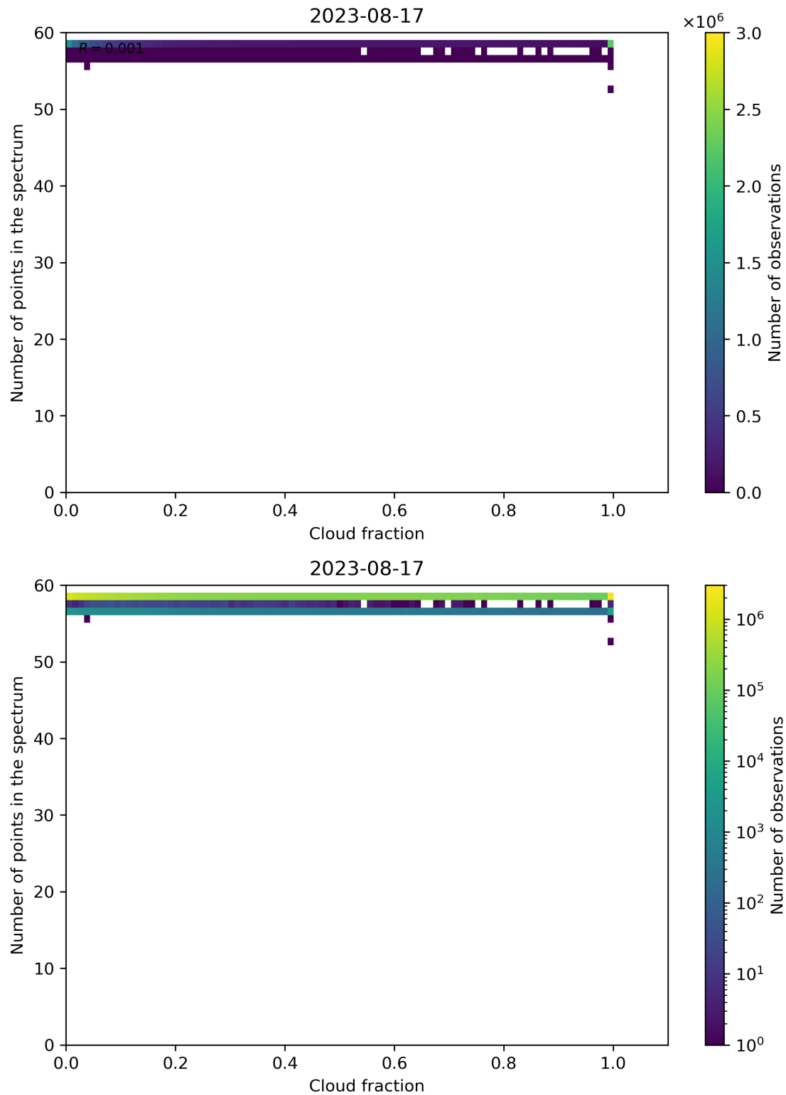
Figure 81: Scatter density plot of “Cloud fraction” against “Number of points in the spectrum” for 2023-08-16 to 2023-08-18.
