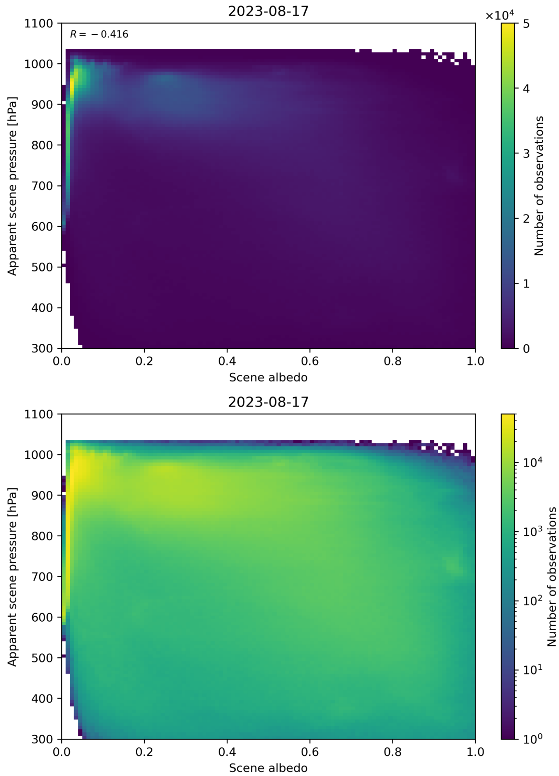
Figure 111: Scatter density plot of “Scene albedo” against “Apparent scene pressure” for 2023-08-16 to 2023-08-18.
