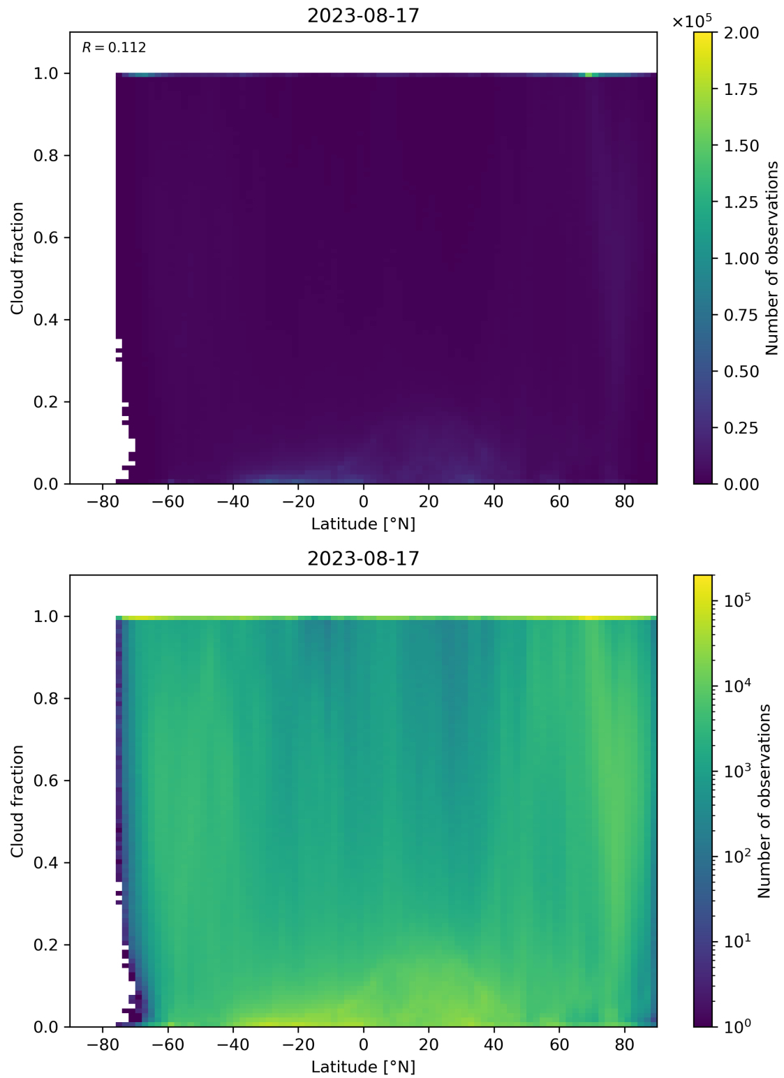
Figure 99: Scatter density plot of “Latitude” against “Cloud fraction” for 2023-08-16 to 2023-08-18.
