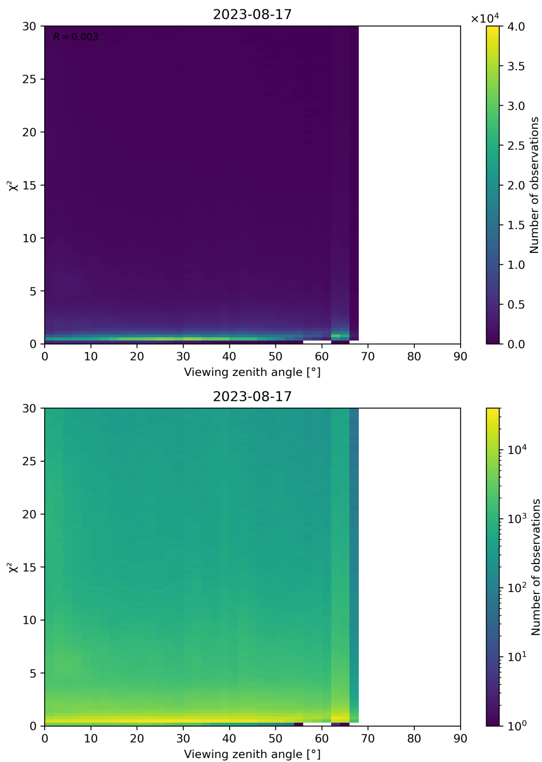
Figure 130: Scatter density plot of “Viewing zenith angle” against “ \chi^2 ” for 2023-08-16 to 2023-08-18.
