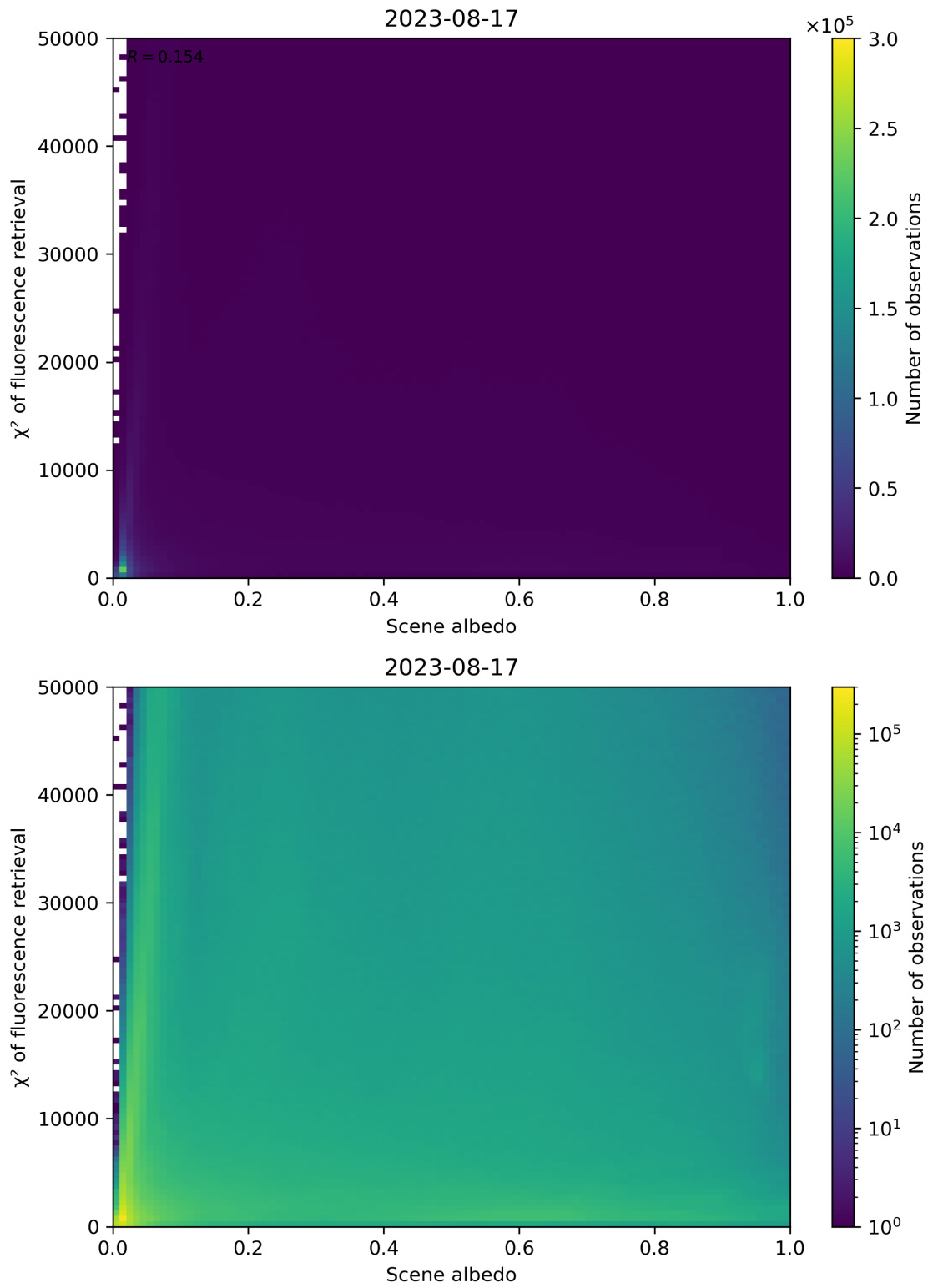
Figure 113: Scatter density plot of “Scene albedo” against “ \chi^2 of fluorescence retrieval” for 2023-08-16 to 2023-08-18.
