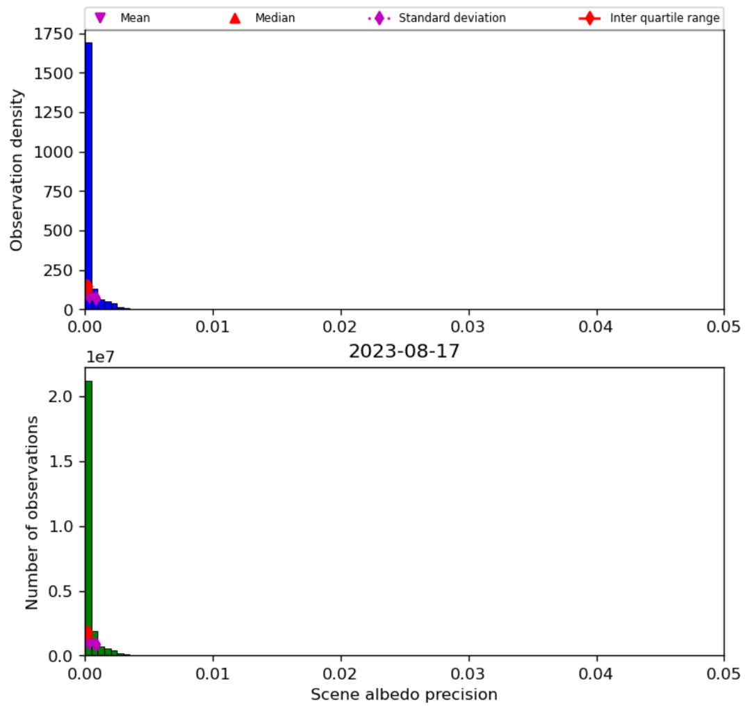
Figure 35: Histogram of “Scene albedo precision” for 2023-08-16 to 2023-08-18
