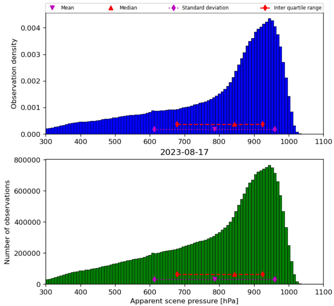
Figure 36: Histogram of “Apparent scene pressure” for 2023-08-16 to 2023-08-18
