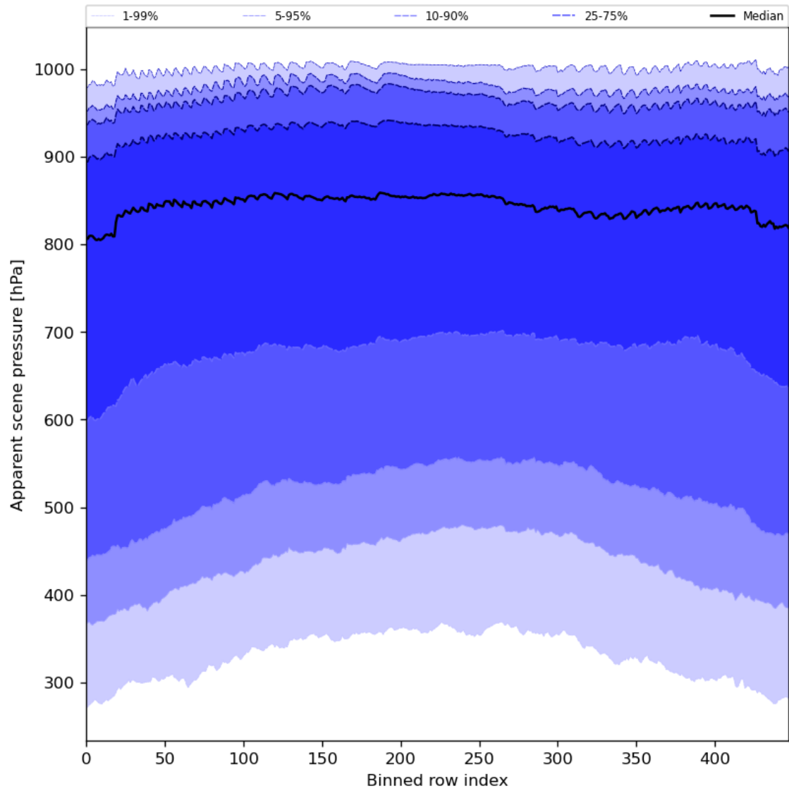
Figure 53: Along track statistics of “Apparent scene pressure” for 2023-08-16 to 2023-08-18
