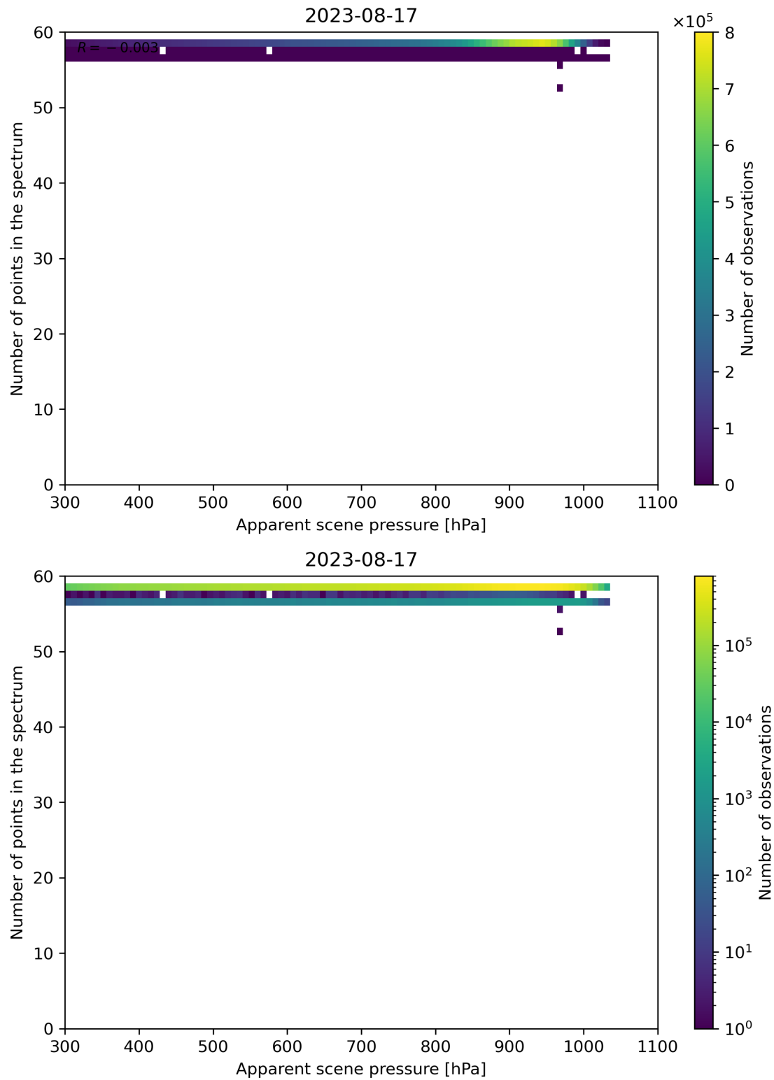
Figure 67: Scatter density plot of “Apparent scene pressure” against “Number of points in the spectrum” for 2023-08-16 to 2023-08-18.
