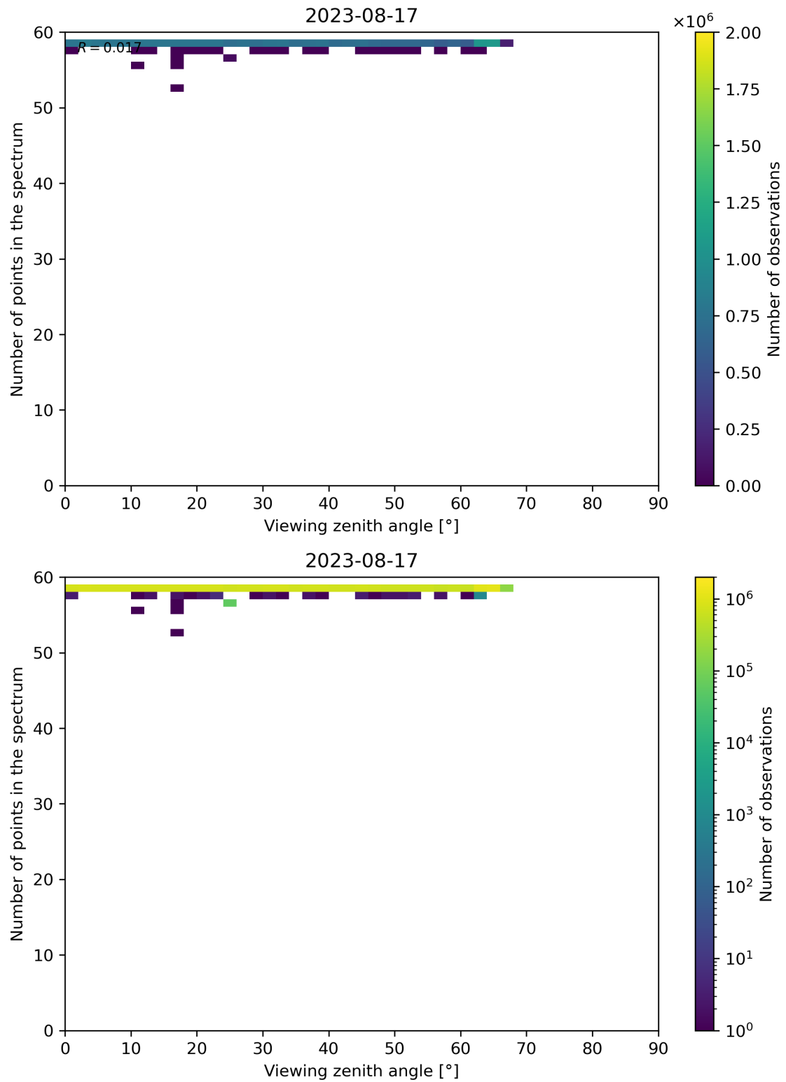
Figure 137: Scatter density plot of “Viewing zenith angle” against “Number of points in the spectrum” for 2023-08-16 to 2023-08-18.
