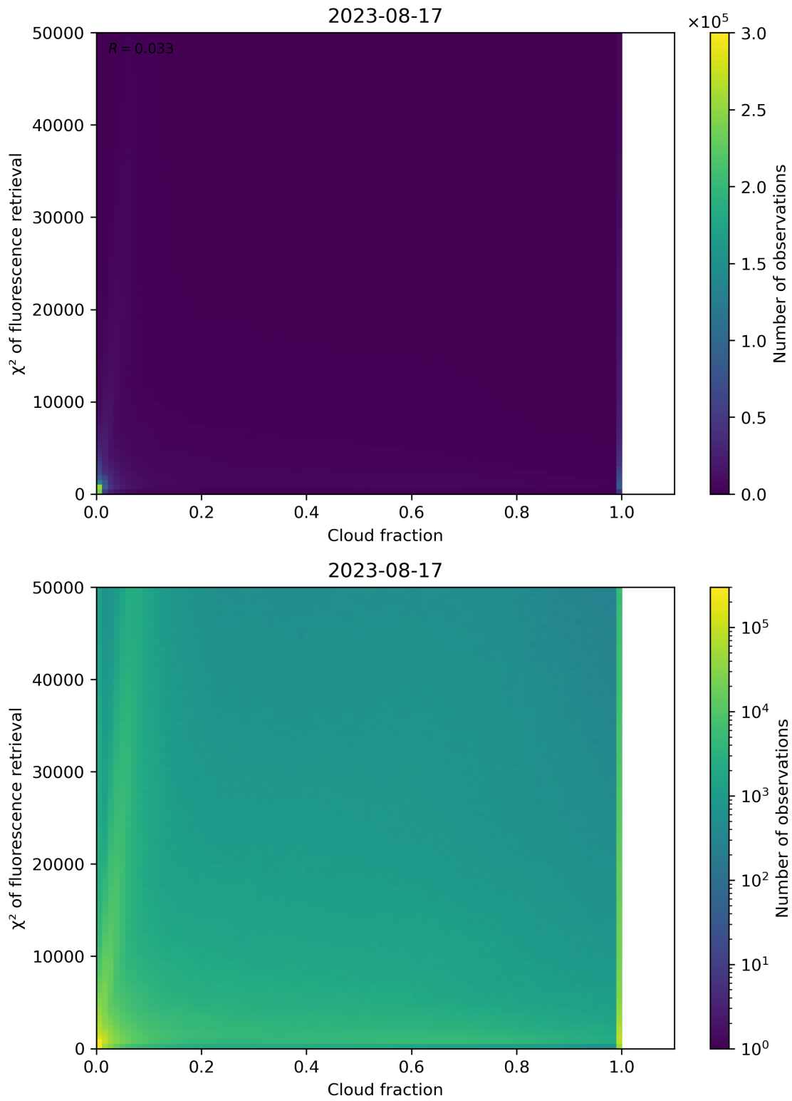
Figure 78: Scatter density plot of “Cloud fraction” against “ \chi^2 of fluorescence retrieval” for 2023-08-16 to 2023-08-18.
