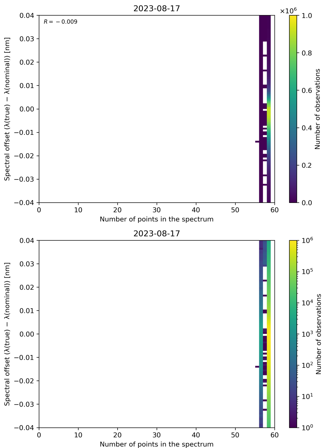
Figure 110: Scatter density plot of “Number of points in the spectrum” against “Spectral offset ( \lambda(\text{true}) - \lambda(\text{nominal}) )” for 2023-08-16 to 2023-08-18.
