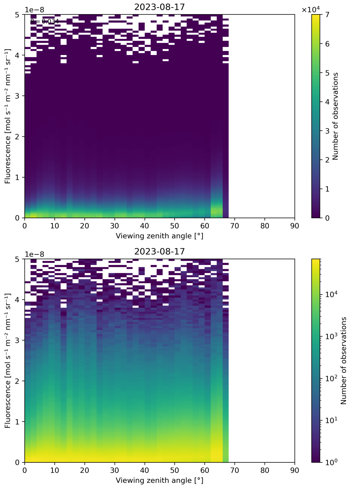
Figure 134: Scatter density plot of “Viewing zenith angle” against “Fluorescence” for 2023-08-16 to 2023-08-18.
