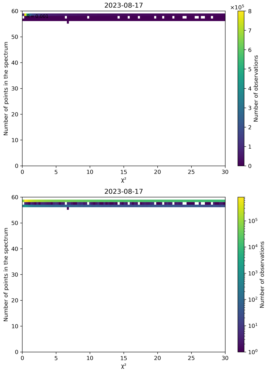
Figure 74: Scatter density plot of “ \chi^2 ” against “Number of points in the spectrum” for 2023-08-16 to 2023-08-18.
