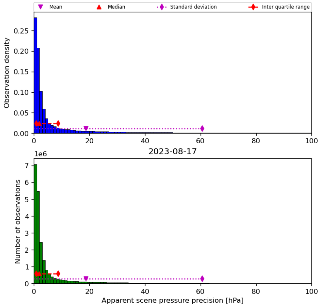
Figure 37: Histogram of “Apparent scene pressure precision” for 2023-08-16 to 2023-08-18
