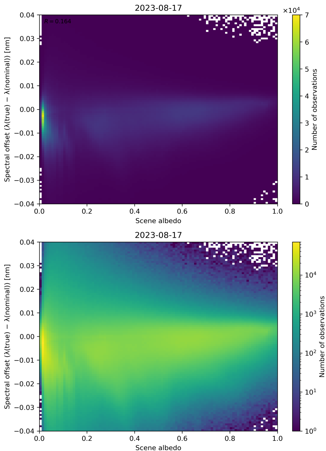
Figure 117: Scatter density plot of “Scene albedo” against “Spectral offset ( \lambda(\text{true}) - \lambda(\text{nominal}) )” for 2023-08-16 to 2023-08-18.
