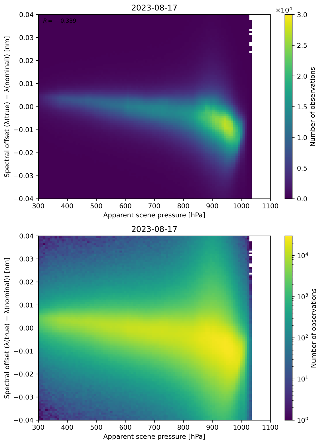
Figure 68: Scatter density plot of “Apparent scene pressure” against “Spectral offset ( \lambda(\text{true}) - \lambda(\text{nominal}) )” for 2023-08-16 to 2023-08-18.
