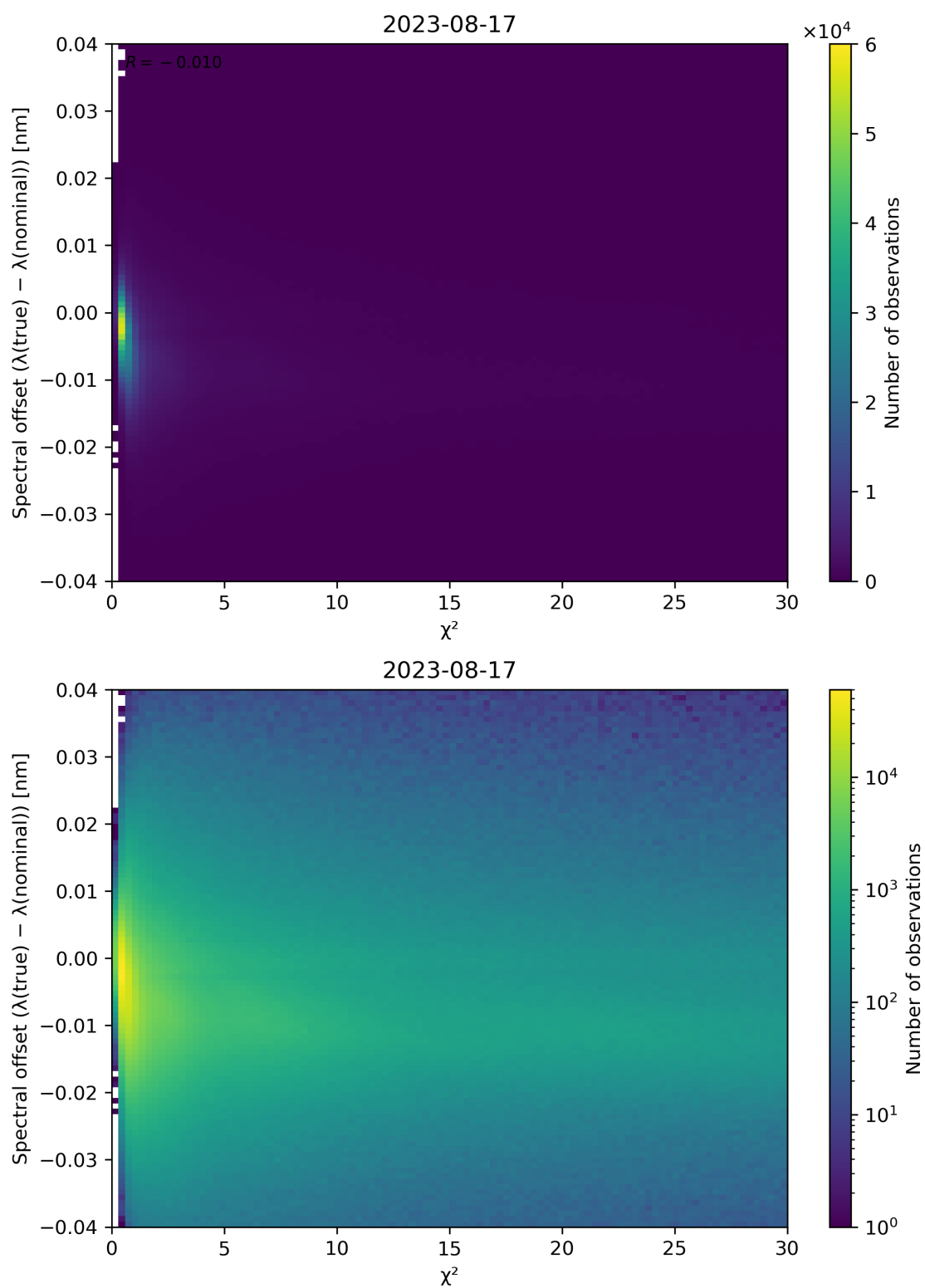
Figure 75: Scatter density plot of “ \chi^2 ” against “Spectral offset ( \lambda(\text{true}) - \lambda(\text{nominal}) )” for 2023-08-16 to 2023-08-18.
