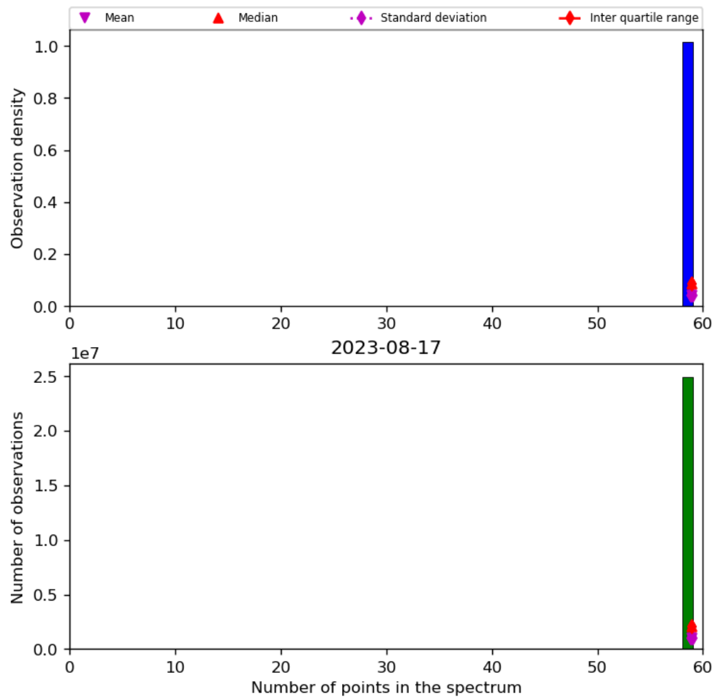
Figure 44: Histogram of “Number of points in the spectrum” for 2023-08-16 to 2023-08-18
