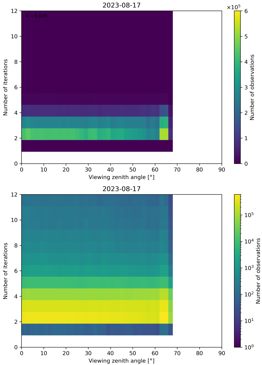
Figure 136: Scatter density plot of “Viewing zenith angle” against “Number of iterations” for 2023-08-16 to 2023-08-18.
