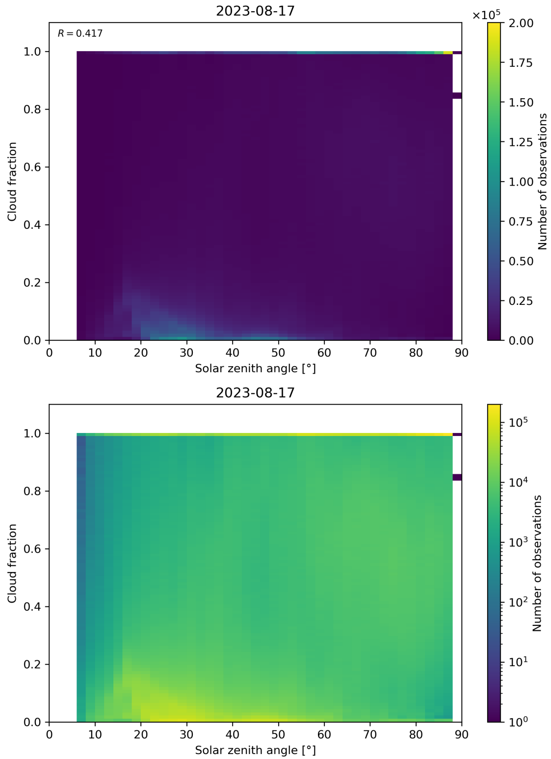
Figure 121: Scatter density plot of “Solar zenith angle” against “Cloud fraction” for 2023-08-16 to 2023-08-18.
