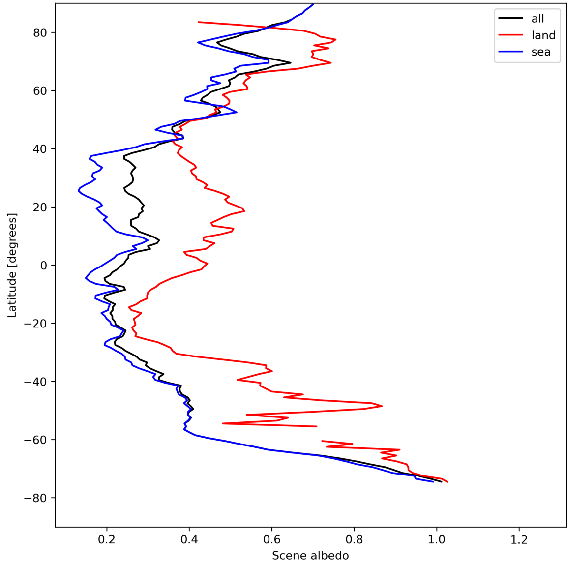
Figure 17: Zonal average of “Scene albedo” for 2023-08-16 to 2023-08-18.
