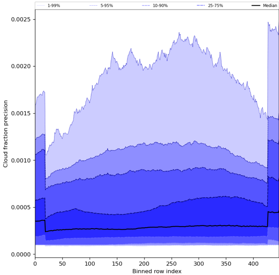
Figure 50: Along track statistics of “Cloud fraction precision” for 2023-08-16 to 2023-08-18
