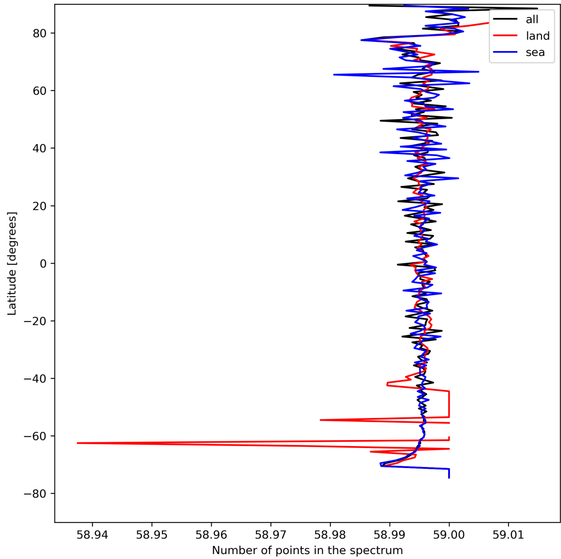
Figure 27: Zonal average of “Number of points in the spectrum” for 2023-08-16 to 2023-08-18.
