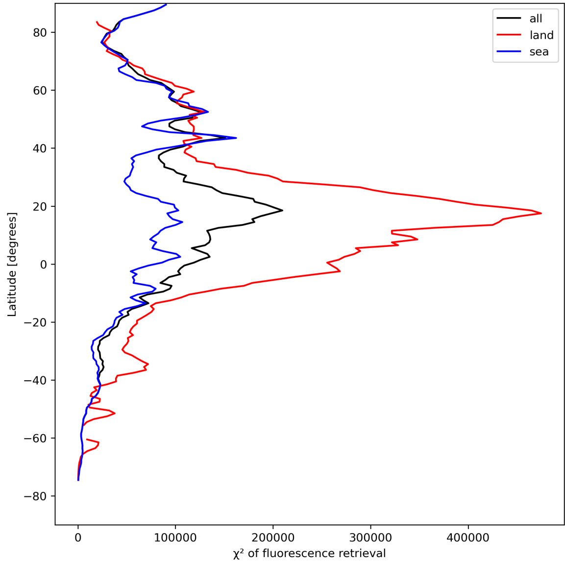
Figure 25: Zonal average of “ \chi^2 of fluorescence retrieval” for 2023-08-16 to 2023-08-18.
