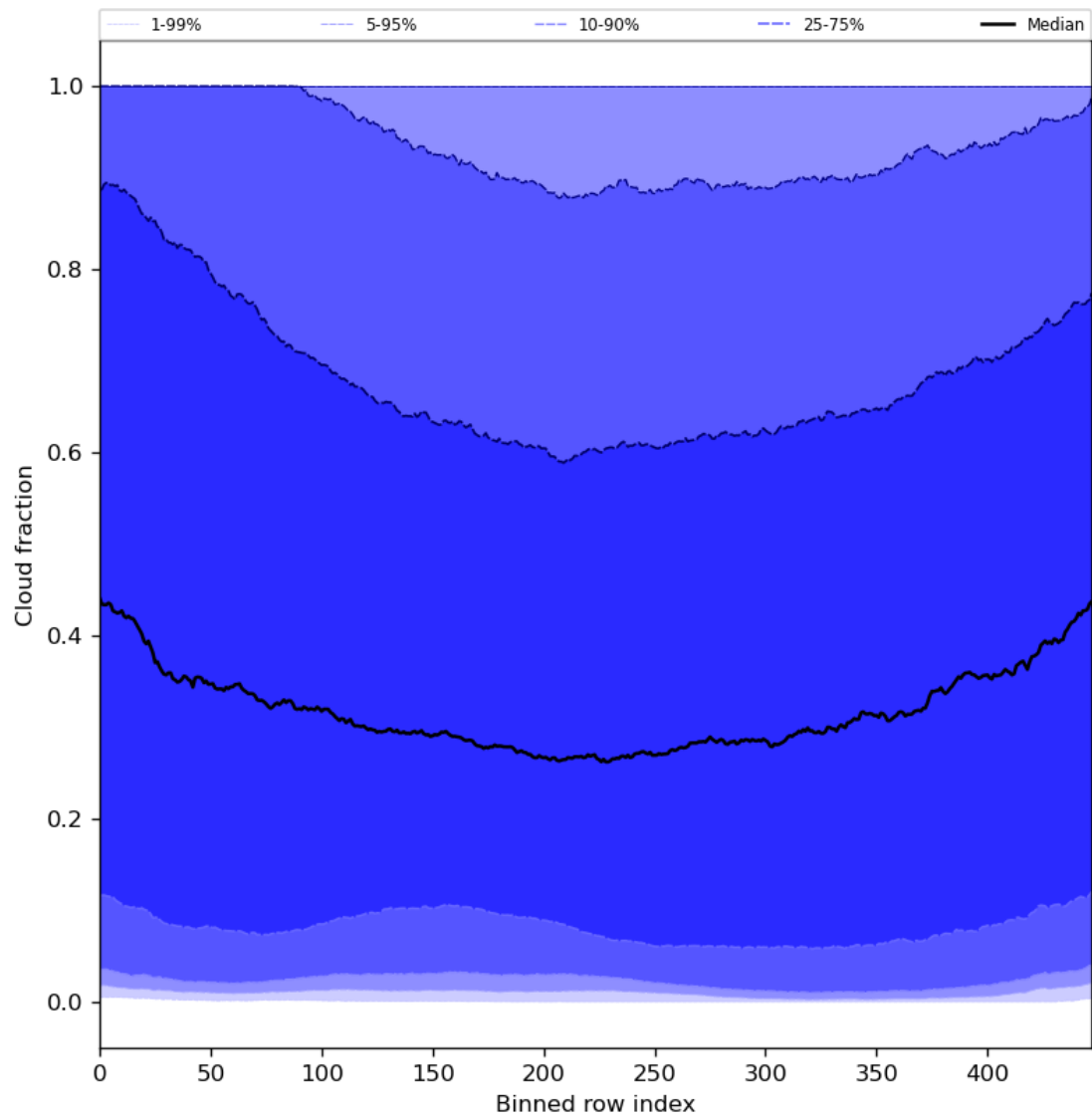
Figure 49: Along track statistics of “Cloud fraction” for 2023-08-16 to 2023-08-18
