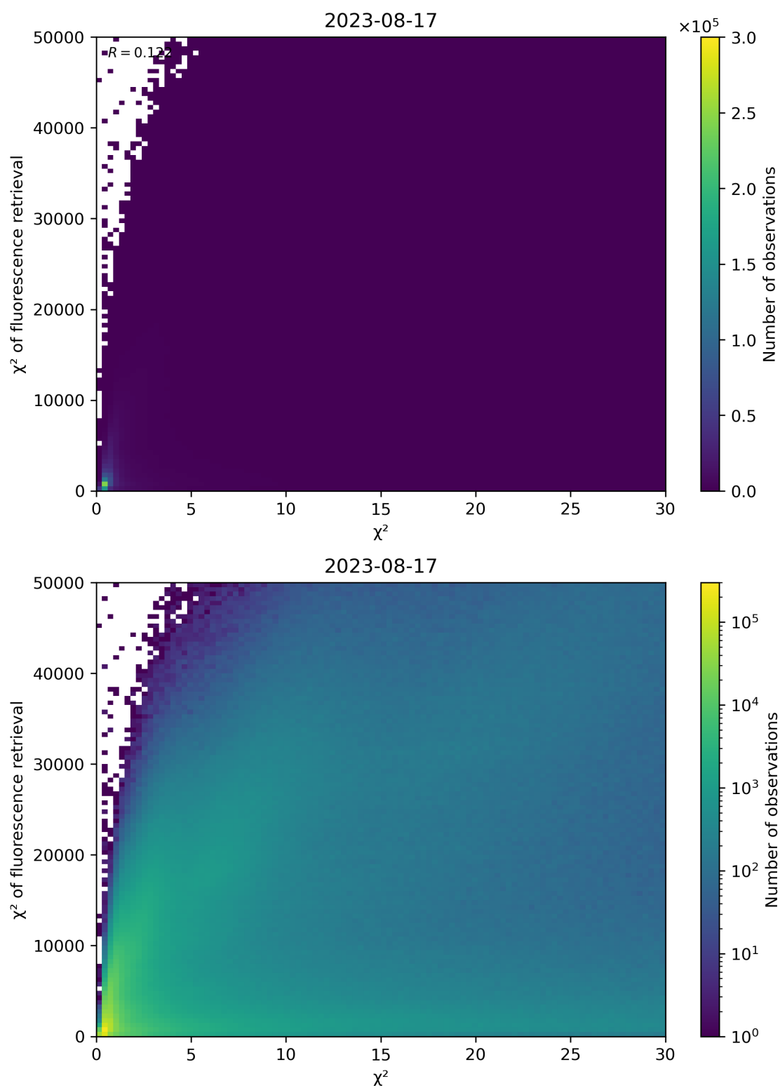
Figure 69: Scatter density plot of “ \chi^2 ” against “ \chi^2 of fluorescence retrieval” for 2023-08-16 to 2023-08-18.
