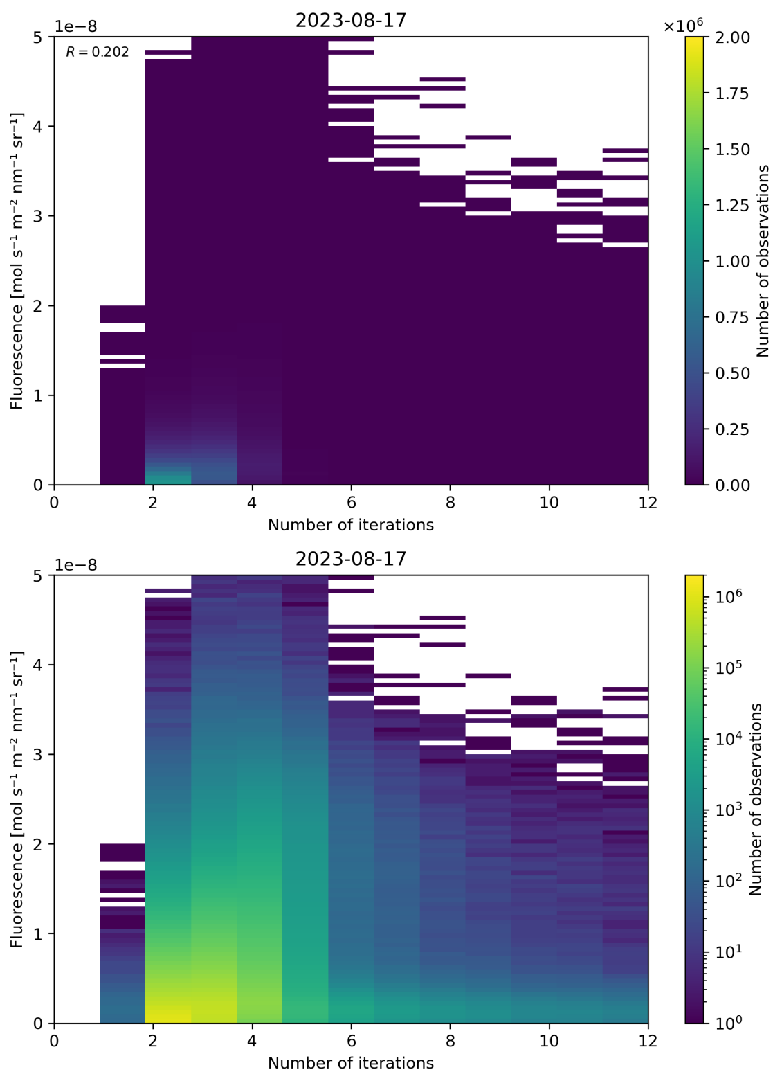
Figure 107: Scatter density plot of “Number of iterations” against “Fluorescence” for 2023-08-16 to 2023-08-18.
