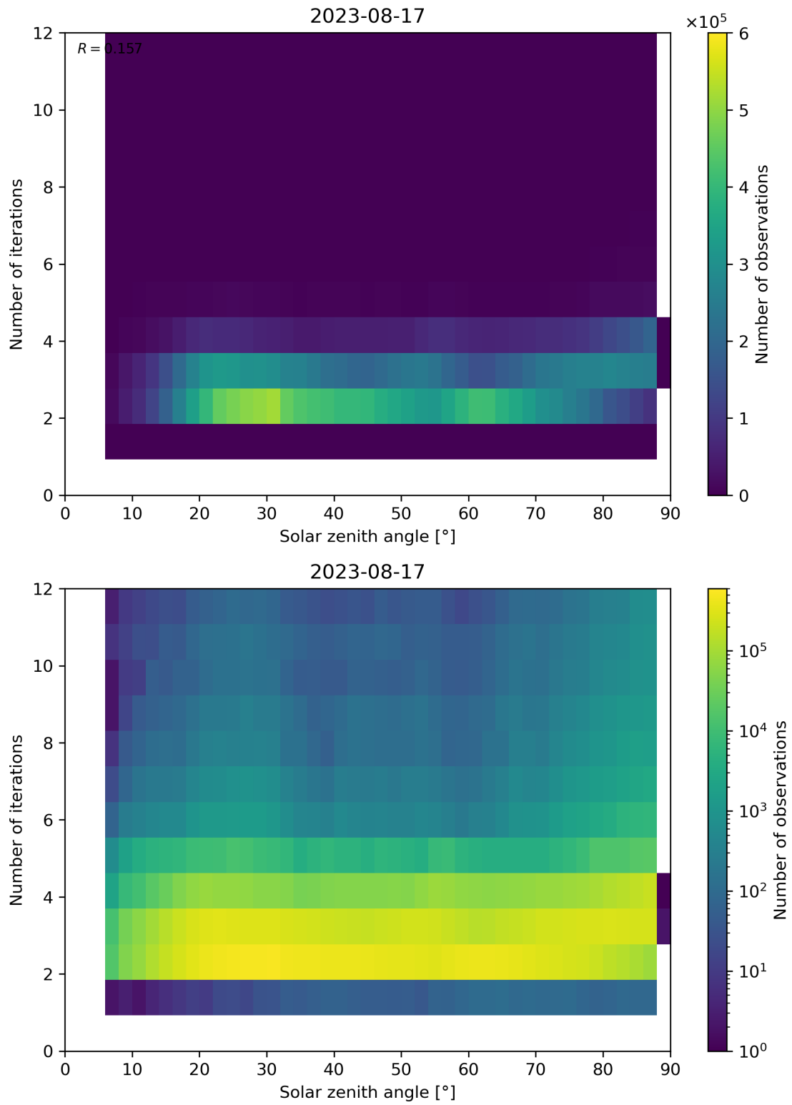
Figure 125: Scatter density plot of “Solar zenith angle” against “Number of iterations” for 2023-08-16 to 2023-08-18.
