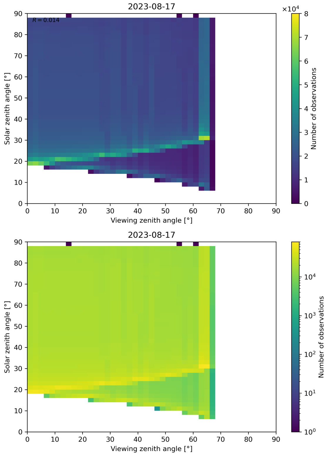
Figure 139: Scatter density plot of “Viewing zenith angle” against “Solar zenith angle” for 2023-08-16 to 2023-08-18.
