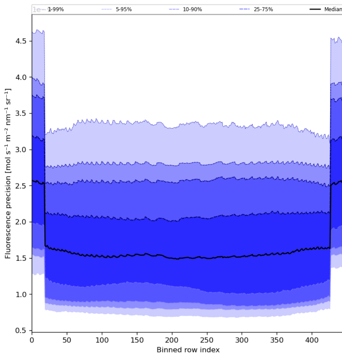
Figure 58: Along track statistics of “Fluorescence precision” for 2023-08-16 to 2023-08-18
