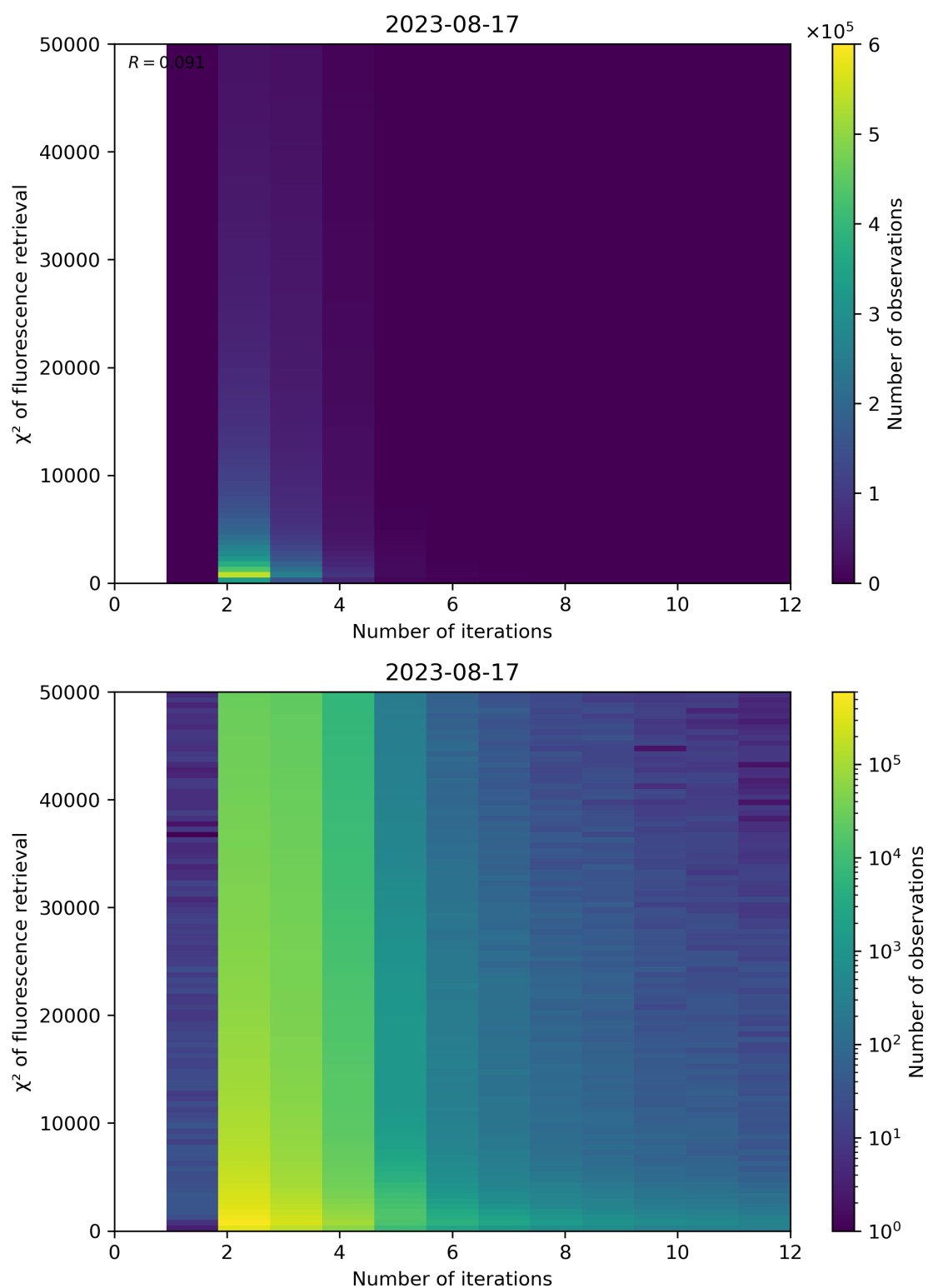
Figure 106: Scatter density plot of “Number of iterations” against “ \chi^2 of fluorescence retrieval” for 2023-08-16 to 2023-08-18.
