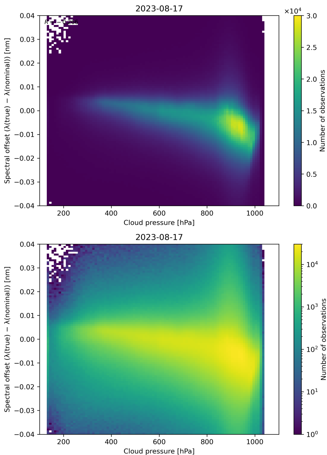
Figure 92: Scatter density plot of “Cloud pressure” against “Spectral offset ( \lambda(\text{true}) - \lambda(\text{nominal}) )” for 2023-08-16 to 2023-08-18.
