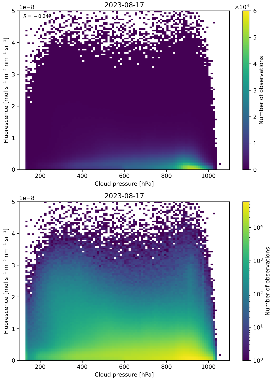
Figure 88: Scatter density plot of “Cloud pressure” against “Fluorescence” for 2023-08-16 to 2023-08-18.
