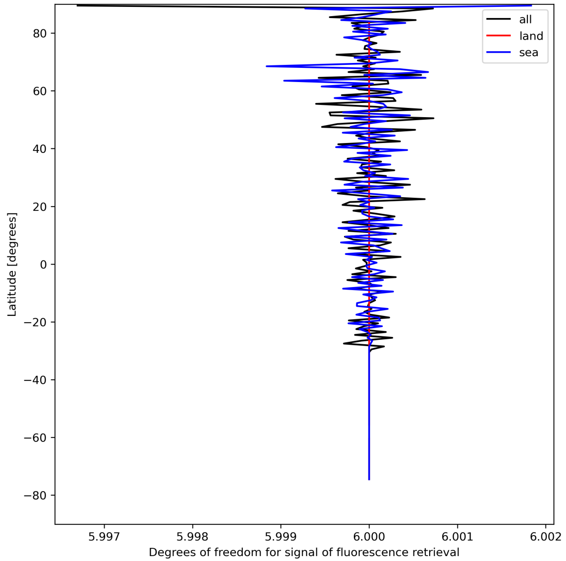
Figure 26: Zonal average of “Degrees of freedom for signal of fluorescence retrieval” for 2023-08-16 to 2023-08-18.
