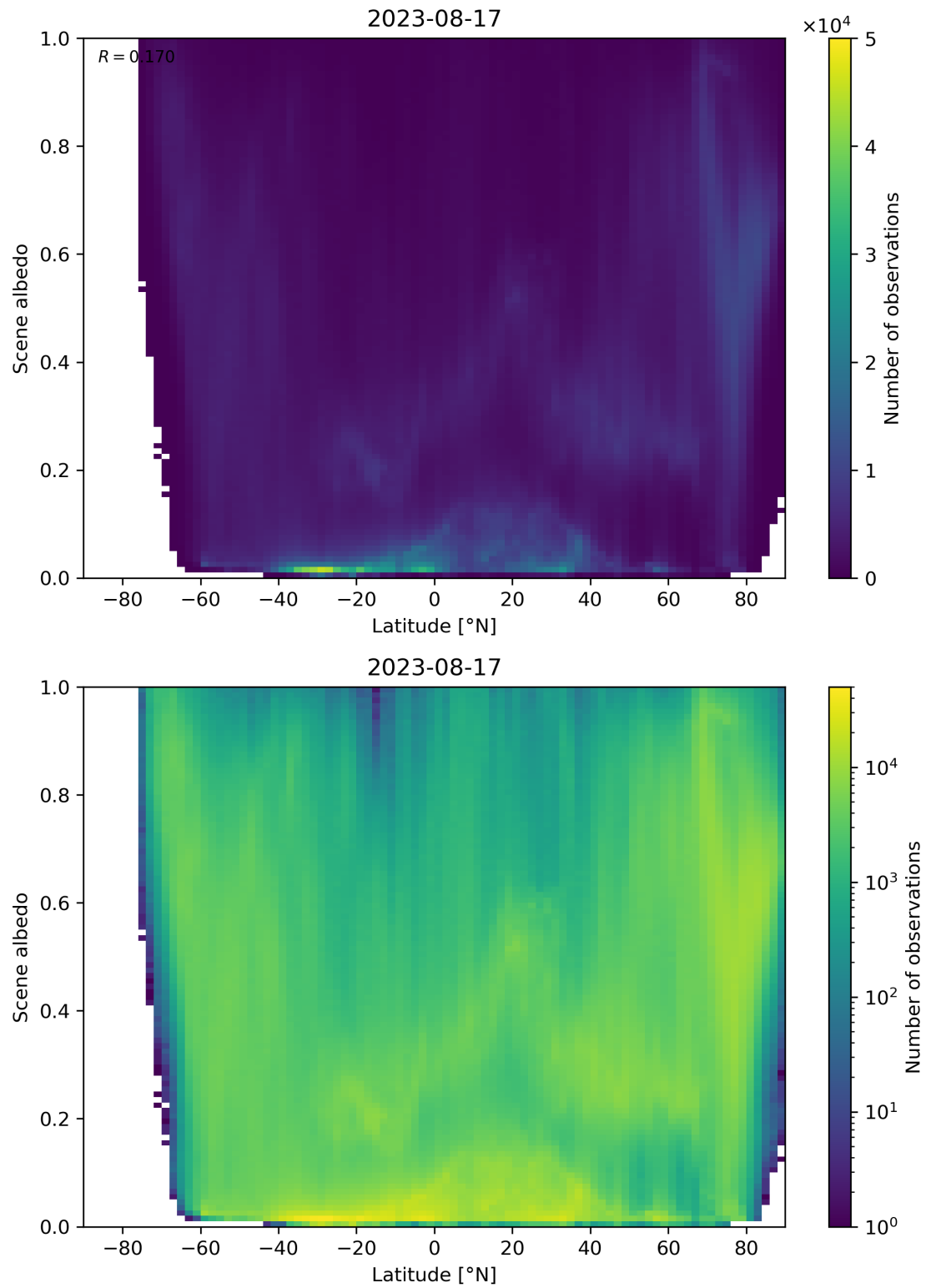
Figure 104: Scatter density plot of “Latitude” against “Scene albedo” for 2023-08-16 to 2023-08-18.
