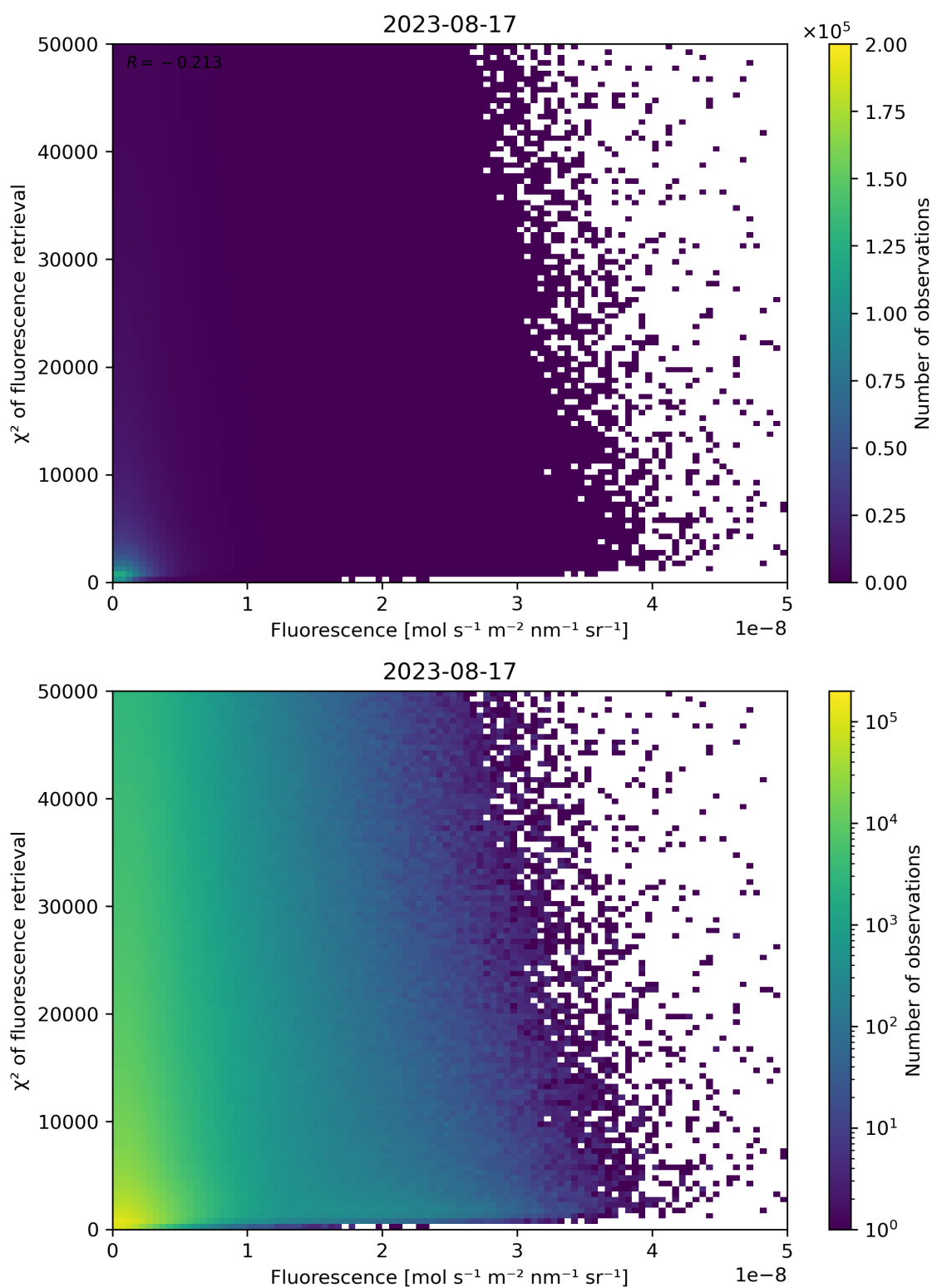
Figure 93: Scatter density plot of “Fluorescence” against “ \chi^2 of fluorescence retrieval” for 2023-08-16 to 2023-08-18.
