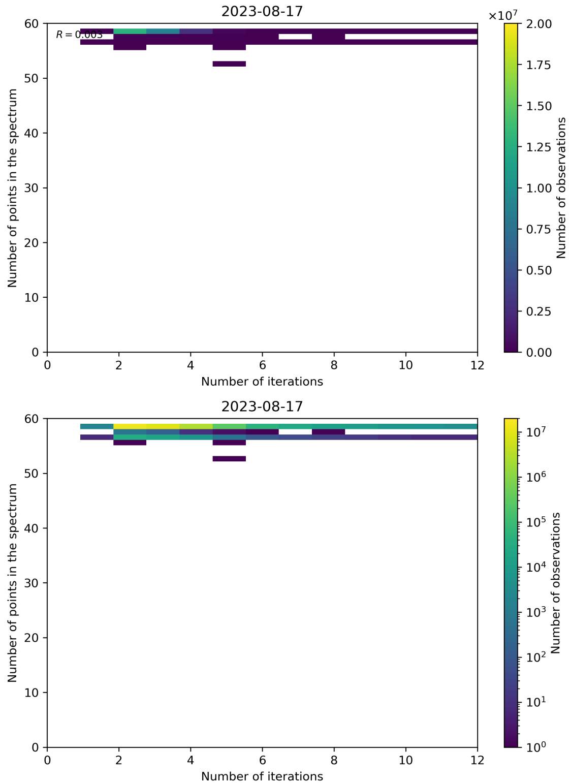
Figure 108: Scatter density plot of “Number of iterations” against “Number of points in the spectrum” for 2023-08-16 to 2023-08-18.
