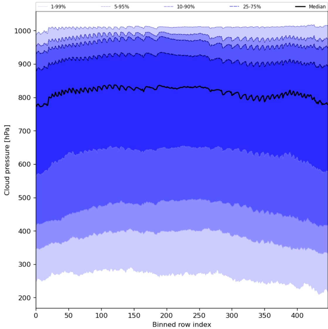
Figure 47: Along track statistics of “Cloud pressure” for 2023-08-16 to 2023-08-18
