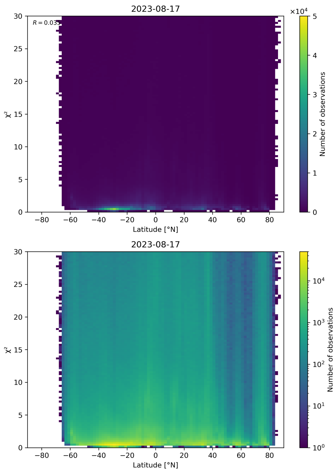
Figure 97: Scatter density plot of “Latitude” against “ \chi^2 ” for 2023-08-16 to 2023-08-18.
