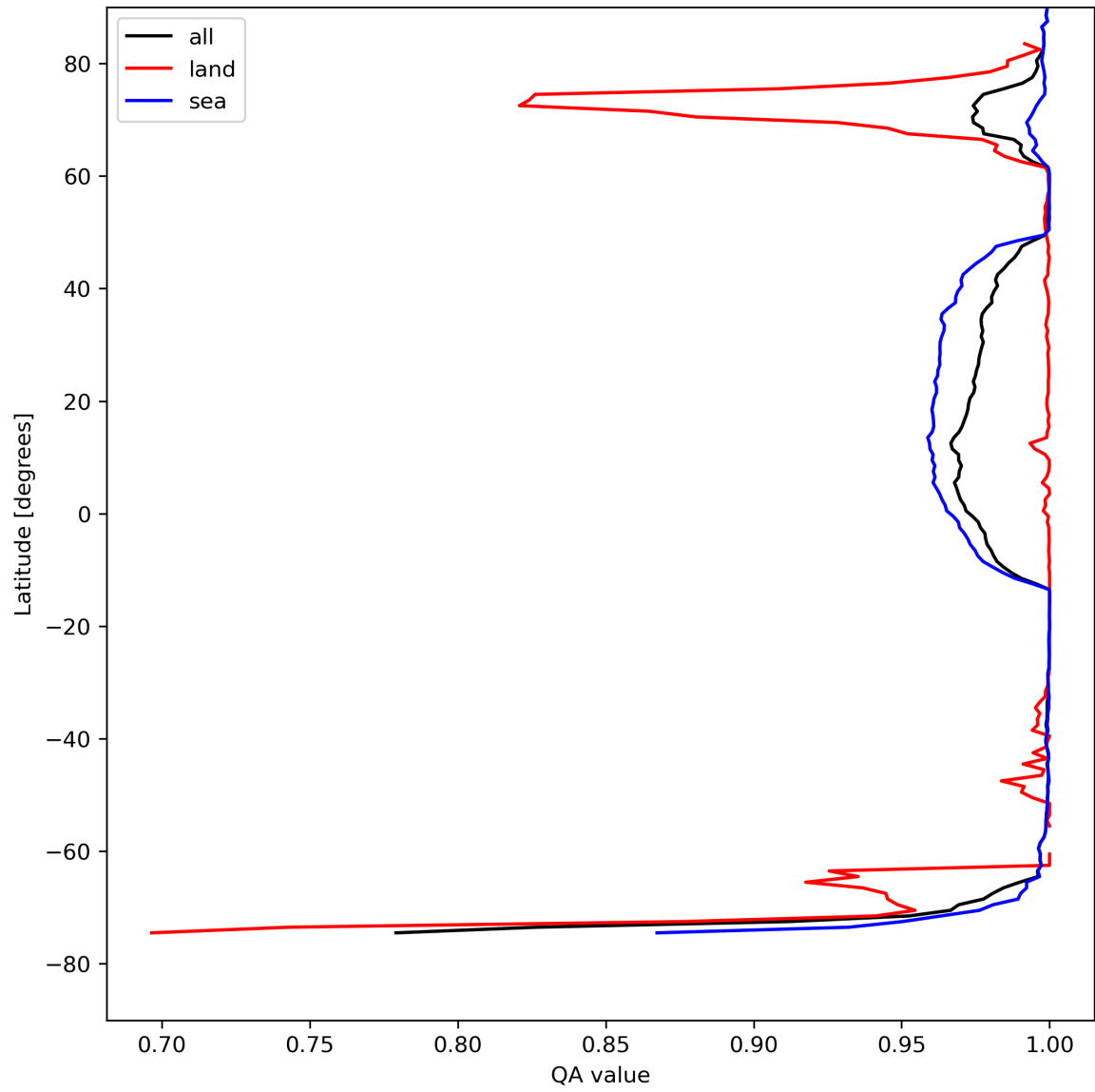
Figure 12: Zonal average of “QA value” for 2023-08-16 to 2023-08-18.
