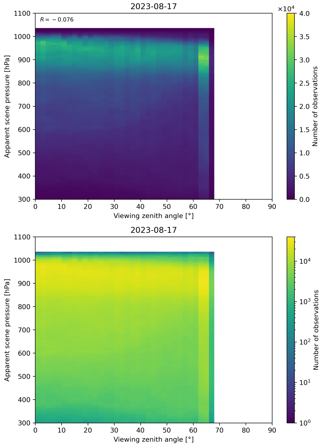
Figure 129: Scatter density plot of “Viewing zenith angle” against “Apparent scene pressure” for 2023-08-16 to 2023-08-18.
