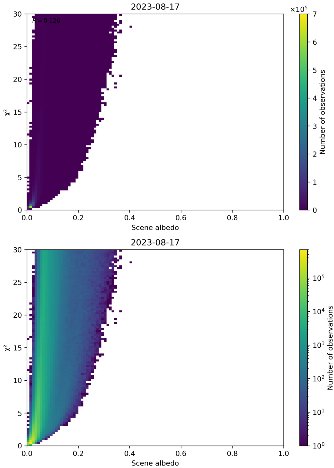
Figure 112: Scatter density plot of “Scene albedo” against “ \chi^2 ” for 2023-08-16 to 2023-08-18.
