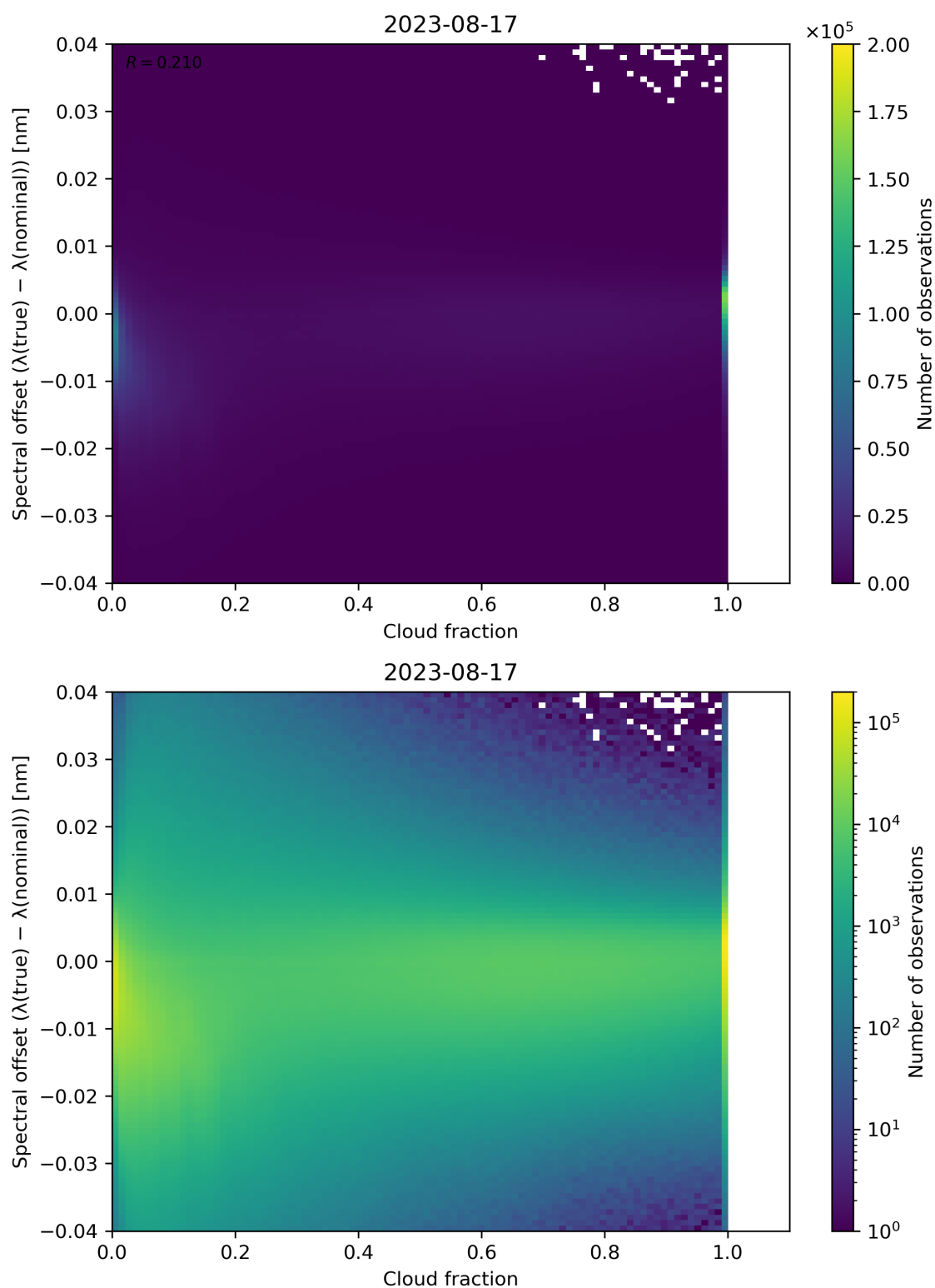
Figure 83: Scatter density plot of “Cloud fraction” against “Spectral offset ( \lambda(\text{true}) - \lambda(\text{nominal}) )” for 2023-08-16 to 2023-08-18.
