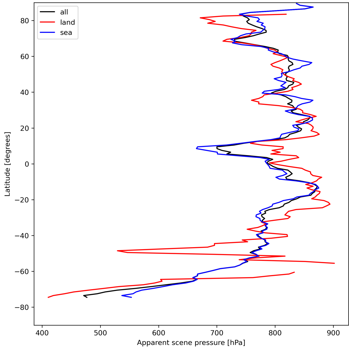
Figure 19: Zonal average of “Apparent scene pressure” for 2023-08-16 to 2023-08-18.
