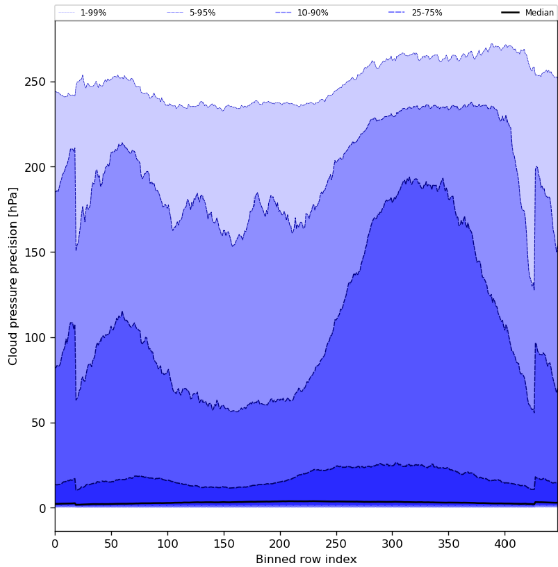
Figure 48: Along track statistics of “Cloud pressure precision” for 2023-08-16 to 2023-08-18
