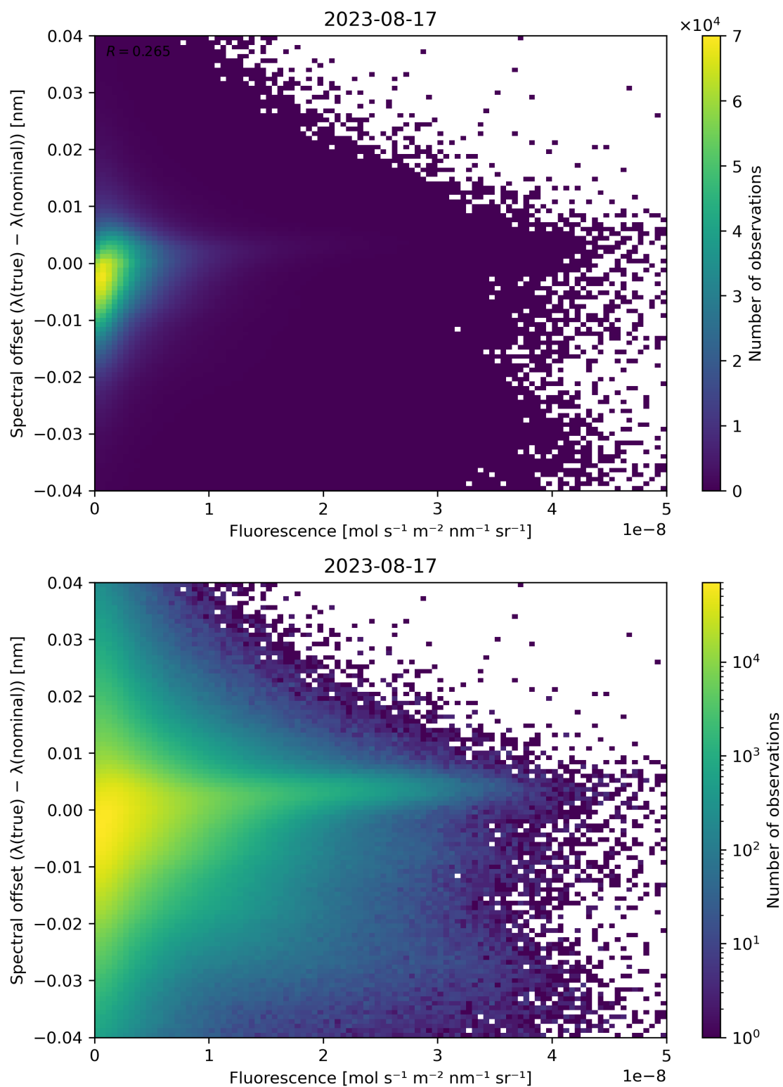
Figure 95: Scatter density plot of “Fluorescence” against “Spectral offset ( \lambda(\text{true}) - \lambda(\text{nominal}) )” for 2023-08-16 to 2023-08-18.
