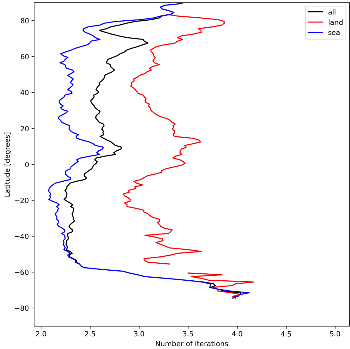
Figure 22: Zonal average of “Number of iterations” for 2023-08-16 to 2023-08-18.
