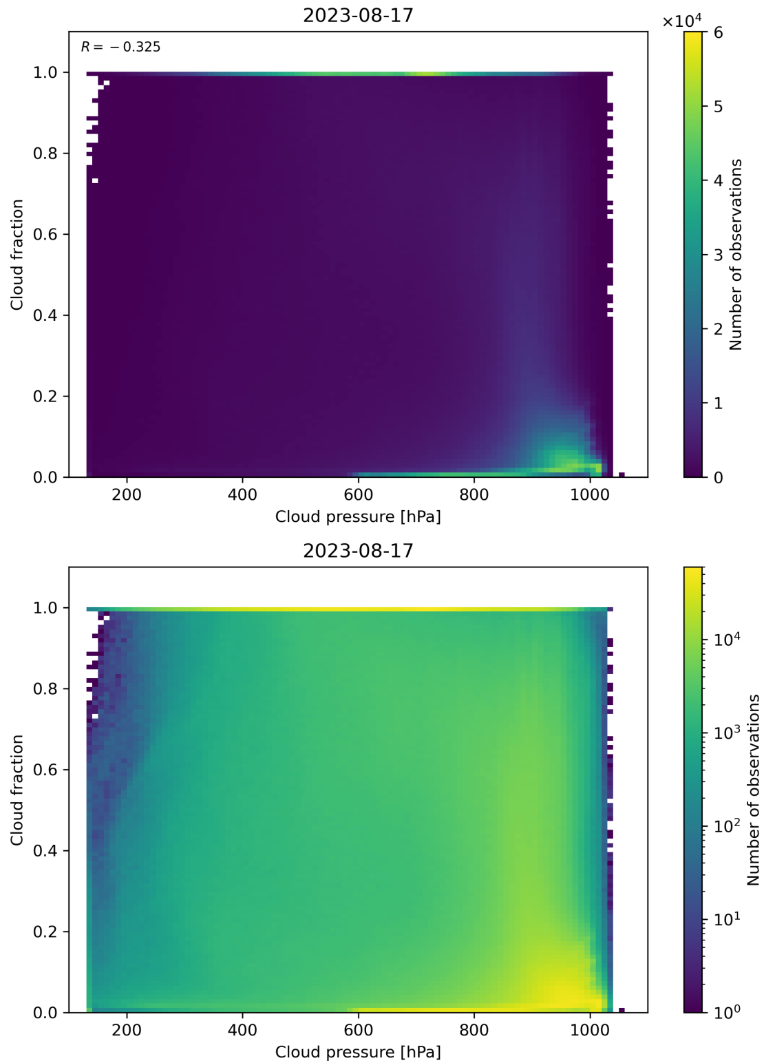
Figure 87: Scatter density plot of “Cloud pressure” against “Cloud fraction” for 2023-08-16 to 2023-08-18.
