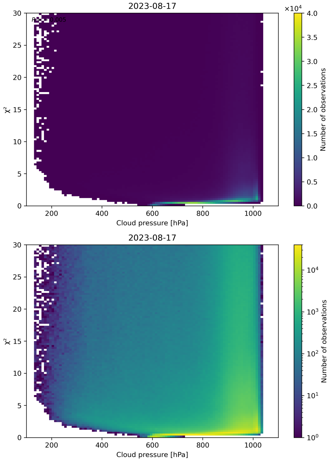
Figure 85: Scatter density plot of “Cloud pressure” against “ \chi^2 ” for 2023-08-16 to 2023-08-18.
