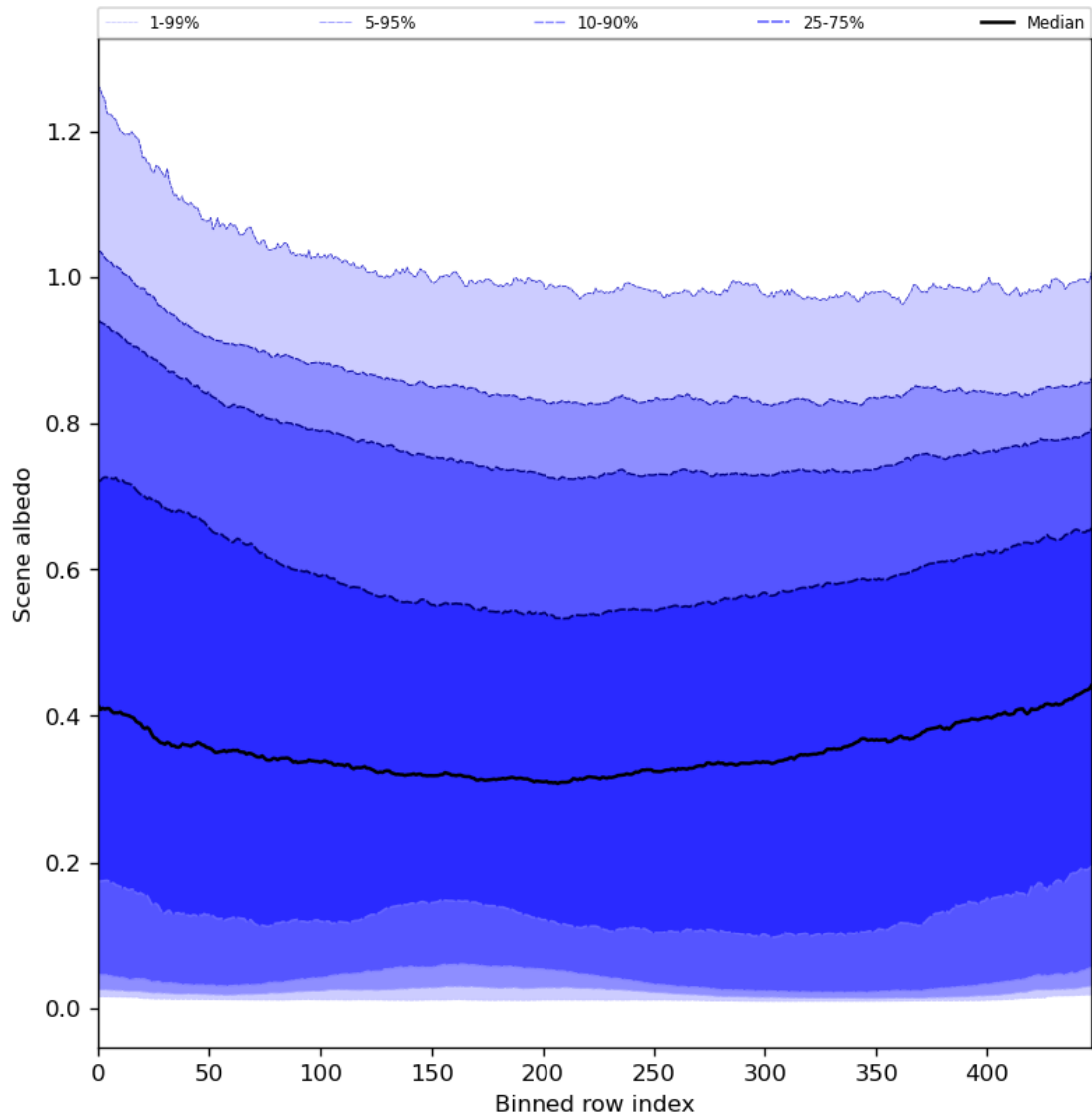
Figure 51: Along track statistics of “Scene albedo” for 2023-08-16 to 2023-08-18
