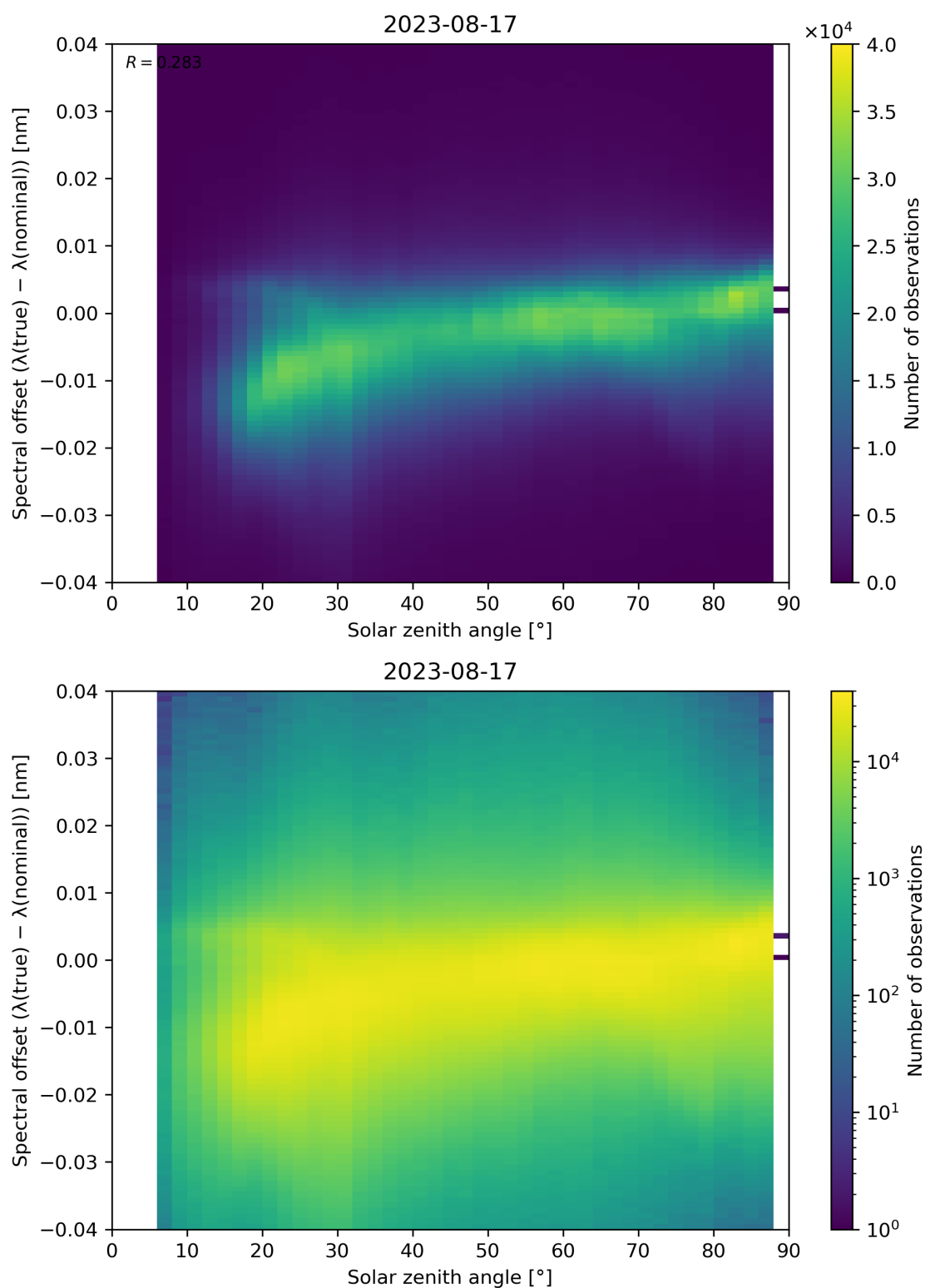
Figure 128: Scatter density plot of “Solar zenith angle” against “Spectral offset ( \lambda(\text{true}) - \lambda(\text{nominal}) )” for 2023-08-16 to 2023-08-18.
