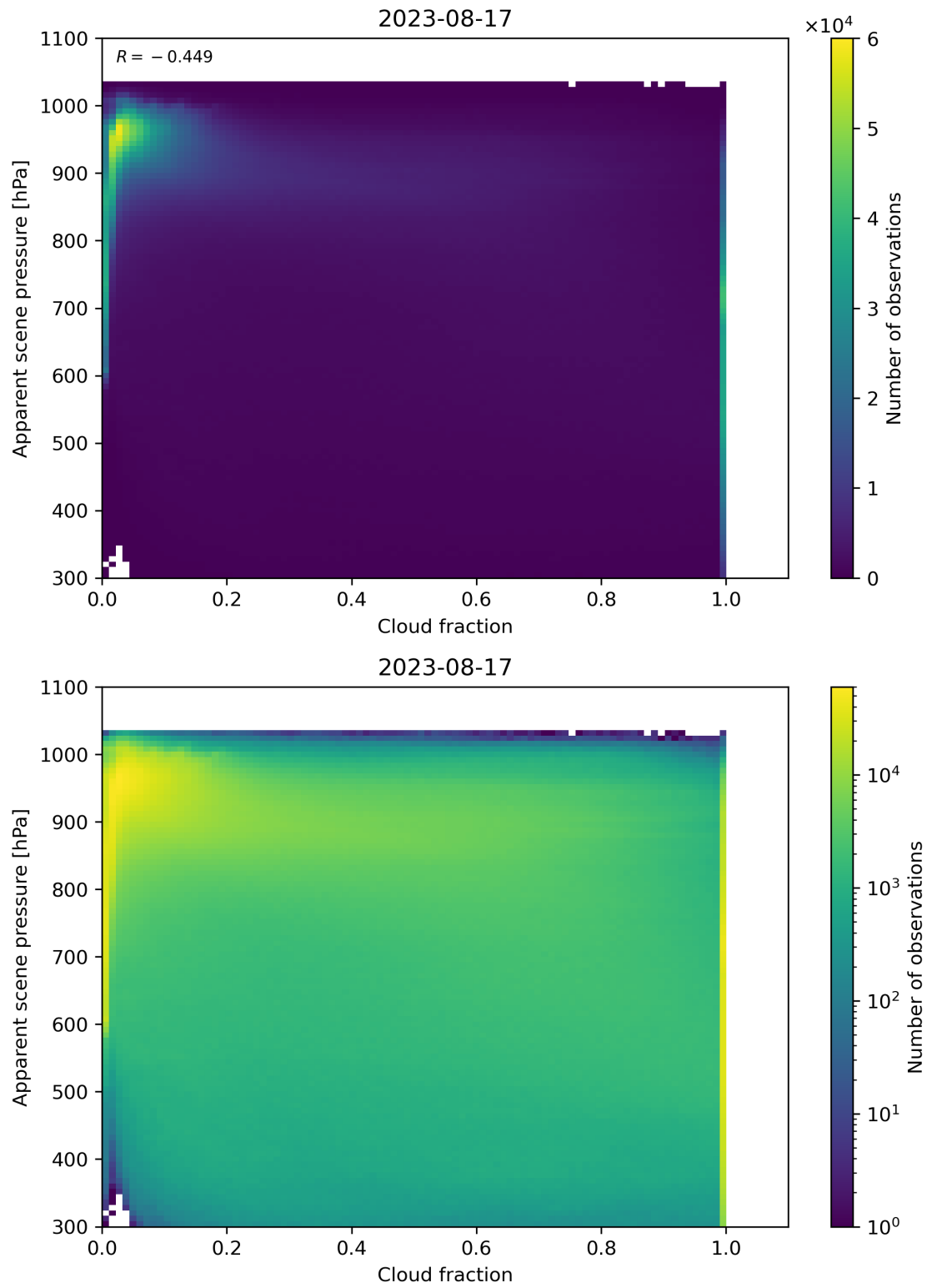
Figure 76: Scatter density plot of “Cloud fraction” against “Apparent scene pressure” for 2023-08-16 to 2023-08-18.
