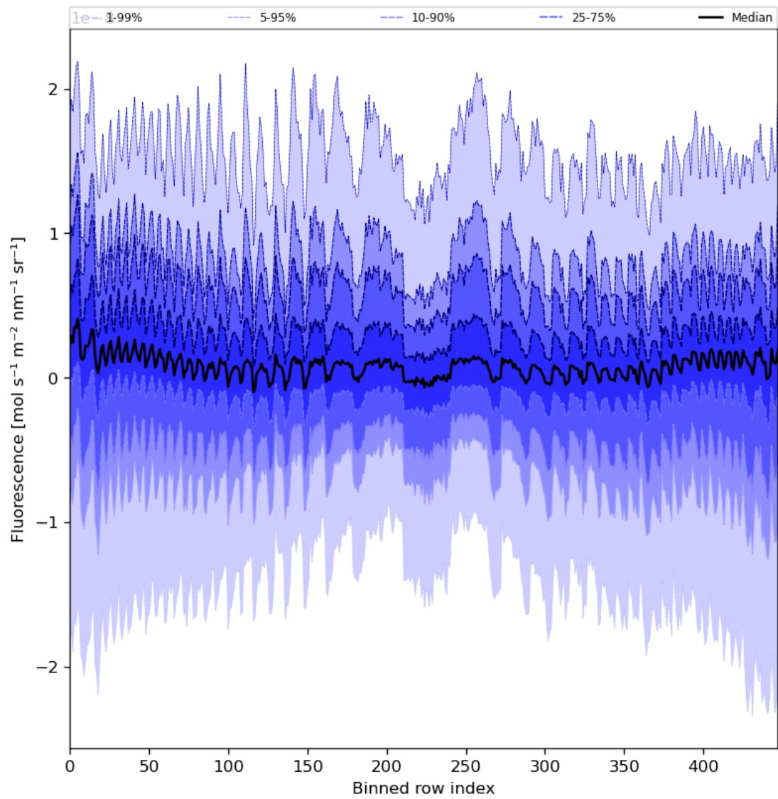
Figure 57: Along track statistics of “Fluorescence” for 2023-08-16 to 2023-08-18
