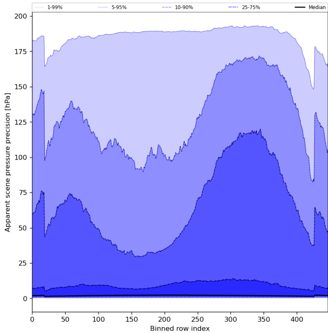
Figure 54: Along track statistics of “Apparent scene pressure precision” for 2023-08-16 to 2023-08-18
