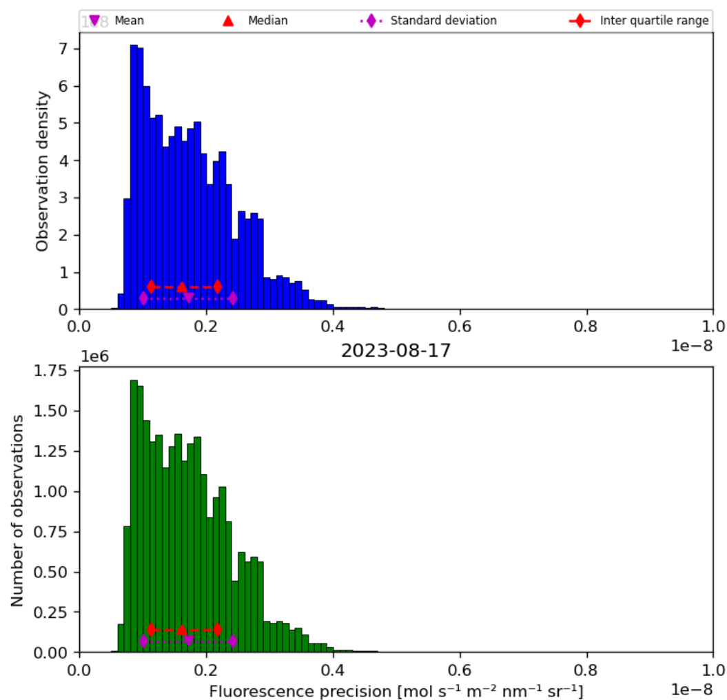
Figure 41: Histogram of “Fluorescence precision” for 2023-08-16 to 2023-08-18
