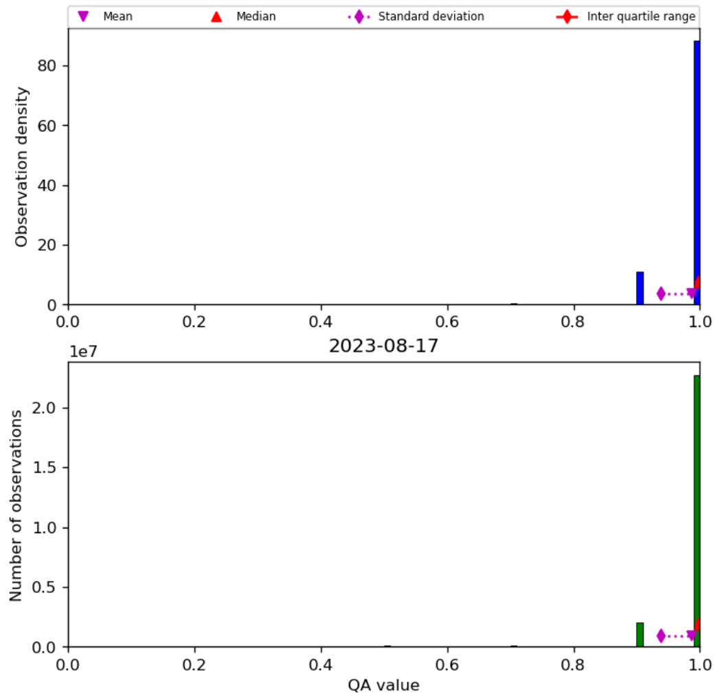
Figure 29: Histogram of “QA value” for 2023-08-16 to 2023-08-18
