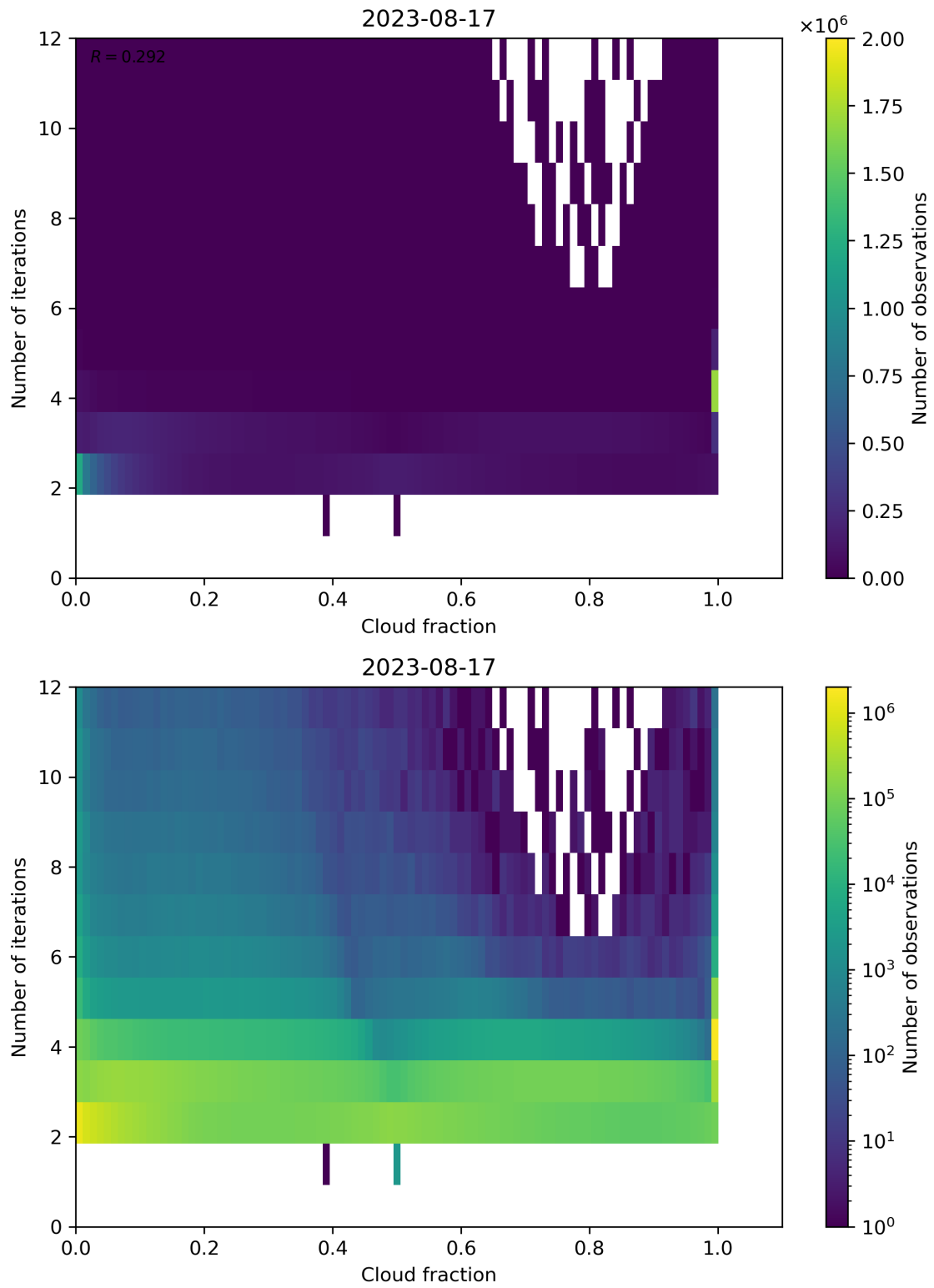
Figure 80: Scatter density plot of “Cloud fraction” against “Number of iterations” for 2023-08-16 to 2023-08-18.
