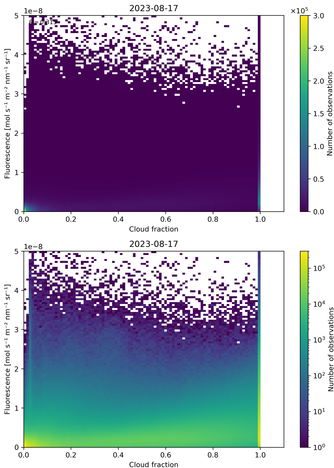
Figure 79: Scatter density plot of “Cloud fraction” against “Fluorescence” for 2023-08-16 to 2023-08-18.
