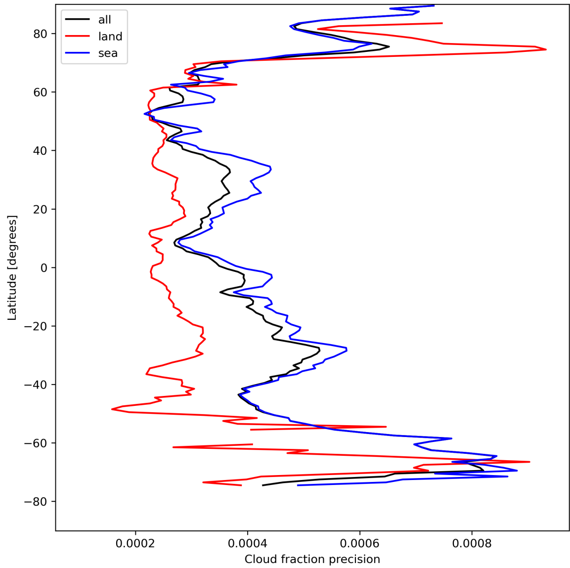
Figure 16: Zonal average of “Cloud fraction precision” for 2023-08-16 to 2023-08-18.
