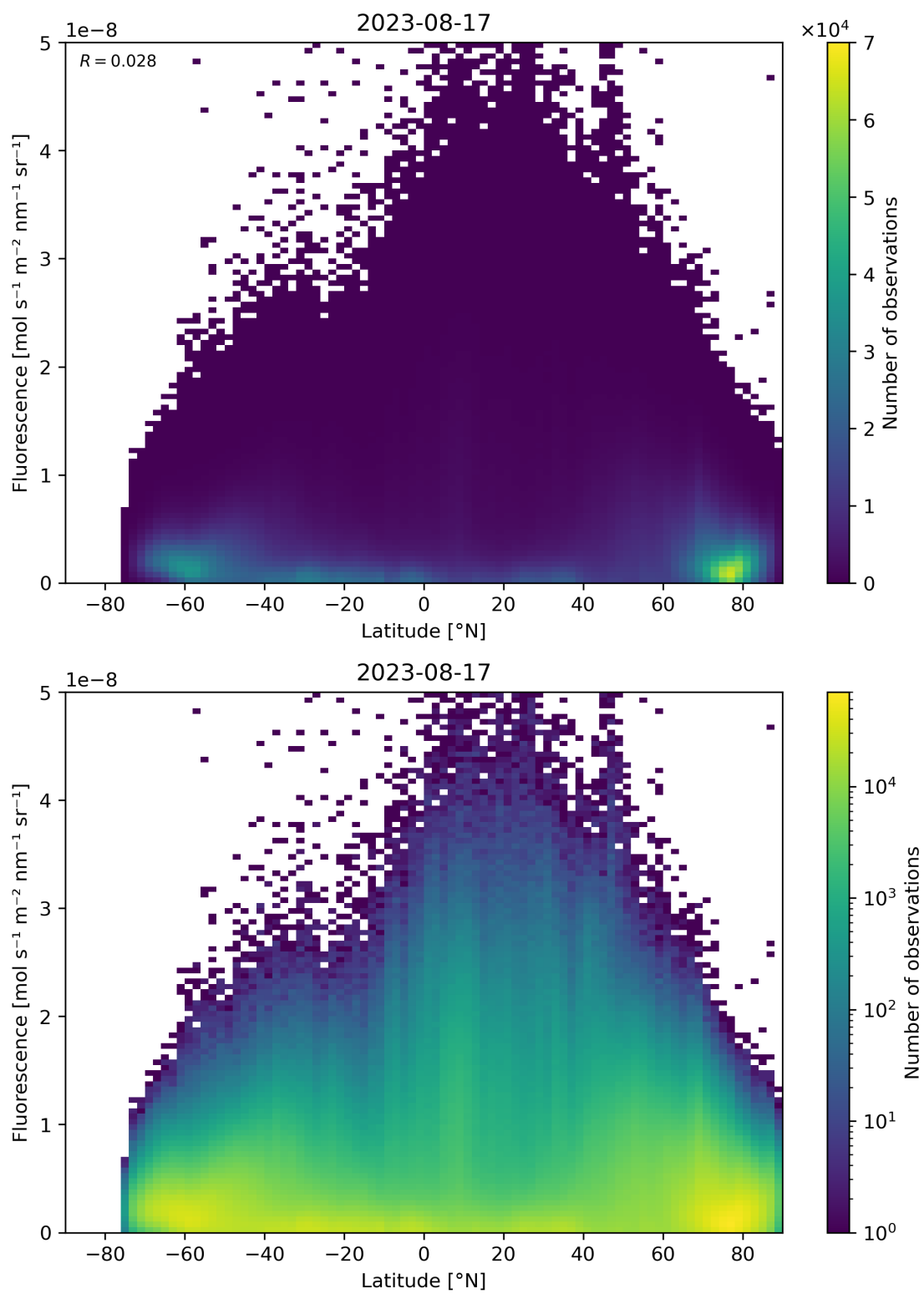
Figure 101: Scatter density plot of “Latitude” against “Fluorescence” for 2023-08-16 to 2023-08-18.
