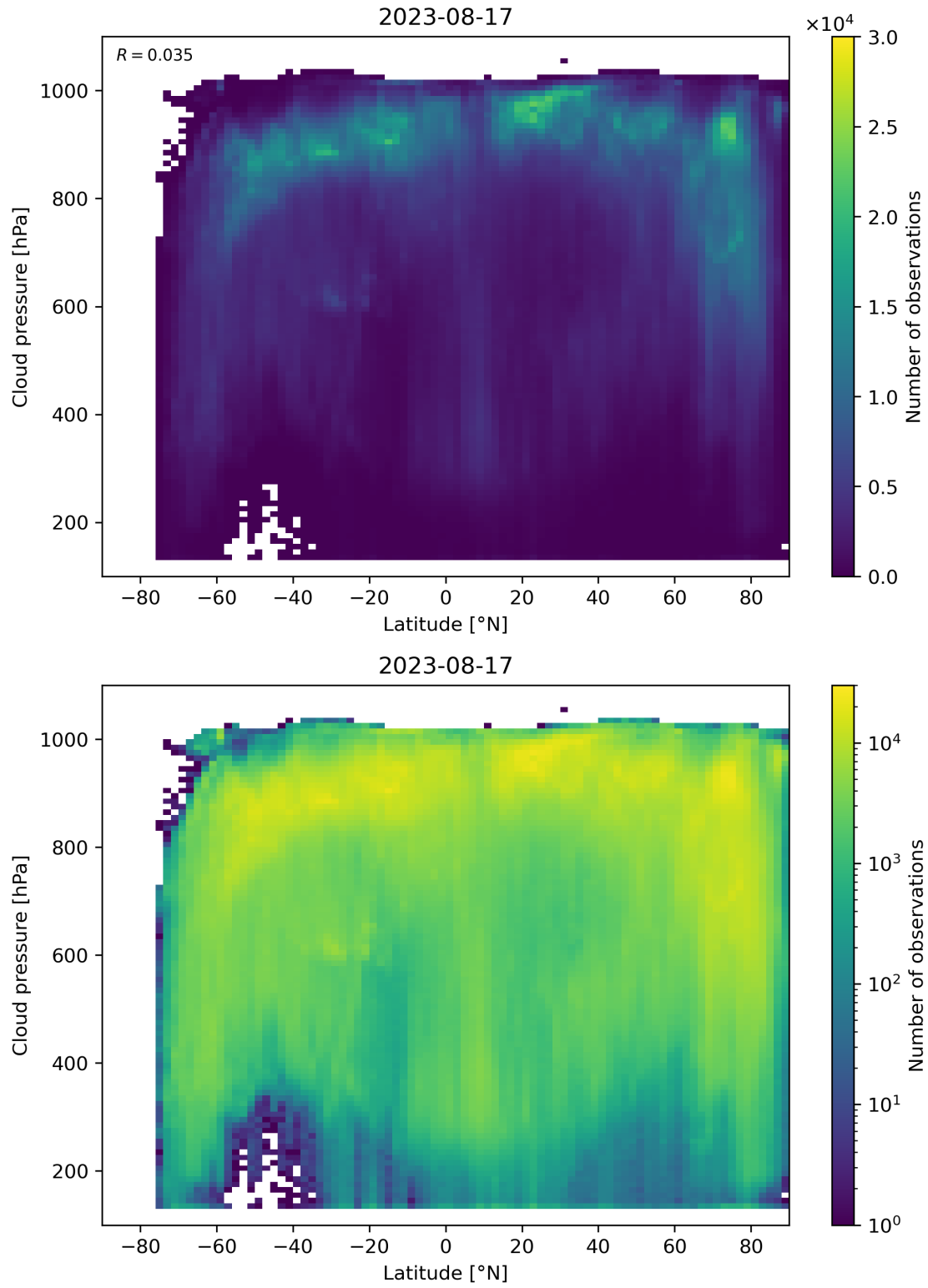
Figure 100: Scatter density plot of “Latitude” against “Cloud pressure” for 2023-08-16 to 2023-08-18.
