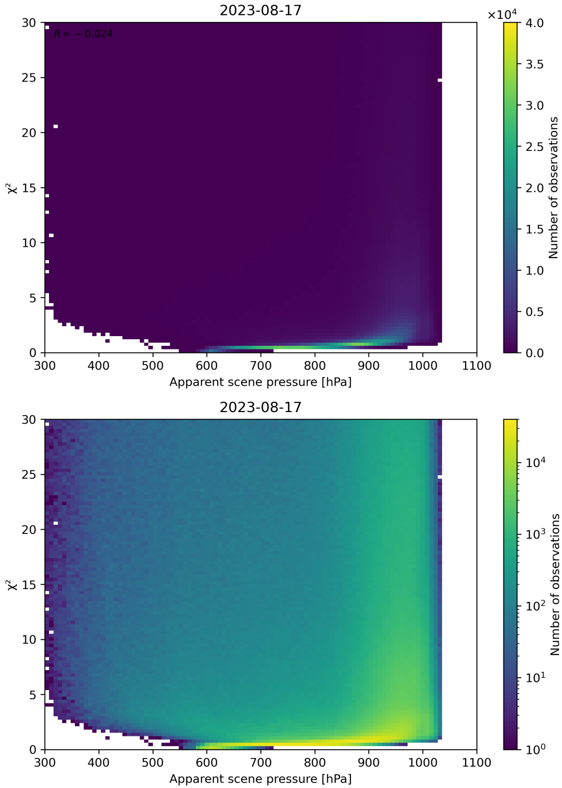
Figure 63: Scatter density plot of “Apparent scene pressure” against “ \chi^2 ” for 2023-08-16 to 2023-08-18.
