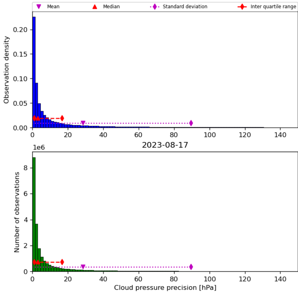
Figure 31: Histogram of “Cloud pressure precision” for 2023-08-16 to 2023-08-18
