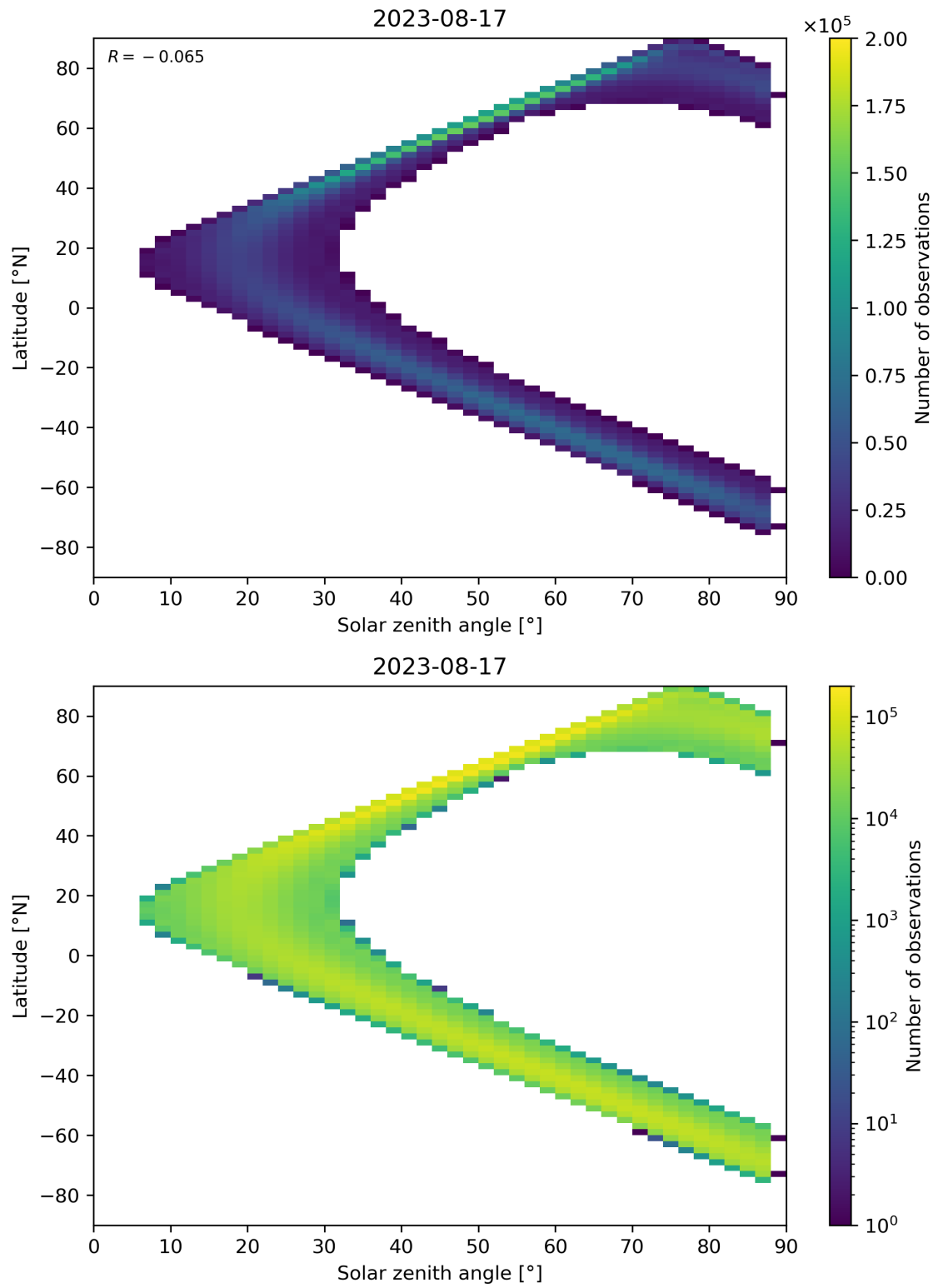
Figure 124: Scatter density plot of “Solar zenith angle” against “Latitude” for 2023-08-16 to 2023-08-18.
