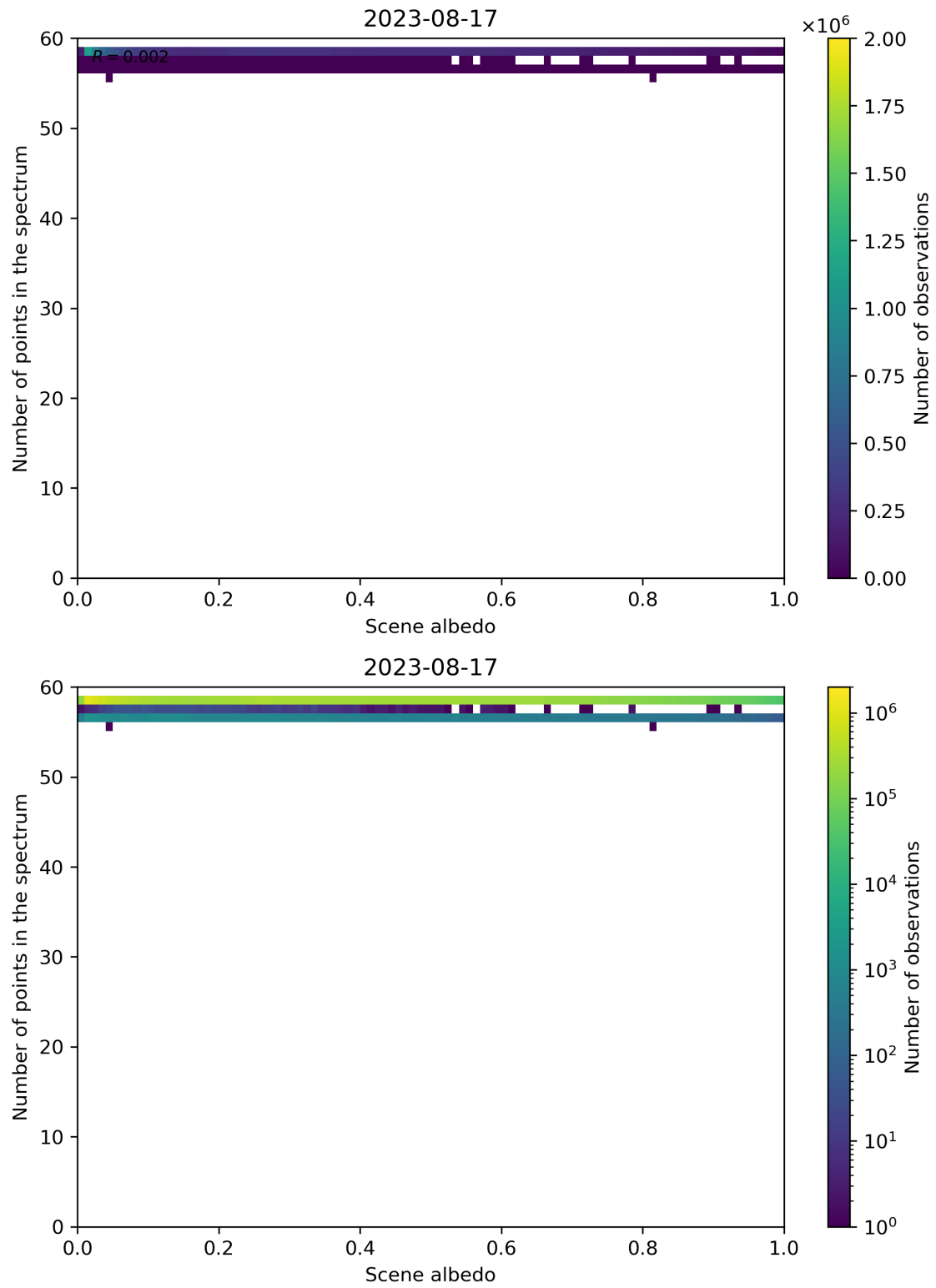
Figure 116: Scatter density plot of “Scene albedo” against “Number of points in the spectrum” for 2023-08-16 to 2023-08-18.
