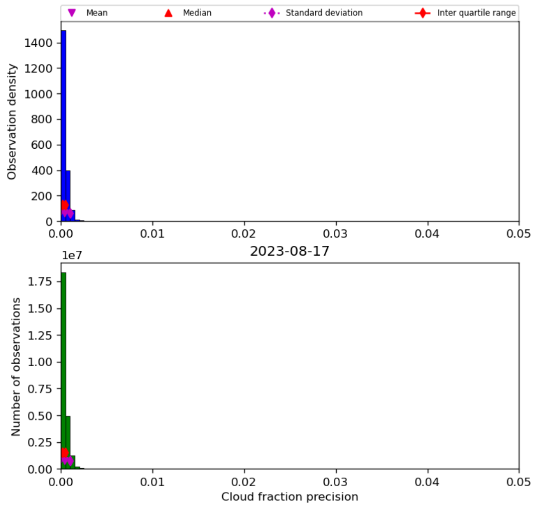
Figure 33: Histogram of “Cloud fraction precision” for 2023-08-16 to 2023-08-18
