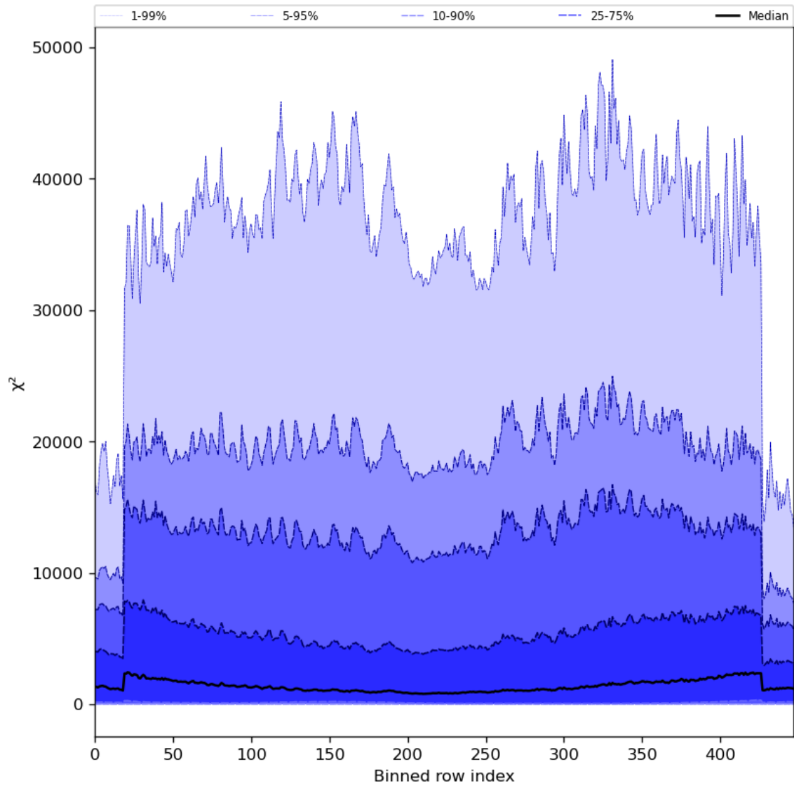
Figure 55: Along track statistics of “ \chi^2 ” for 2023-08-16 to 2023-08-18
