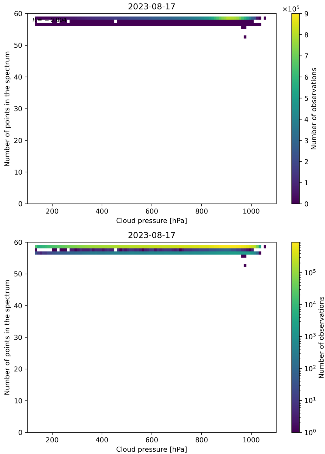
Figure 90: Scatter density plot of “Cloud pressure” against “Number of points in the spectrum” for 2023-08-16 to 2023-08-18.
