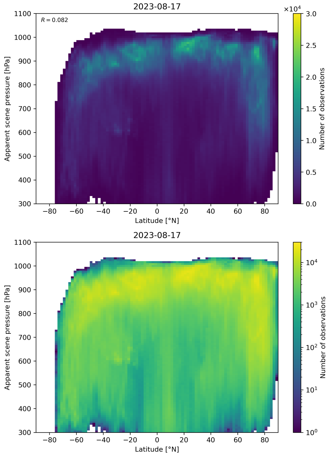
Figure 96: Scatter density plot of “Latitude” against “Apparent scene pressure” for 2023-08-16 to 2023-08-18.
