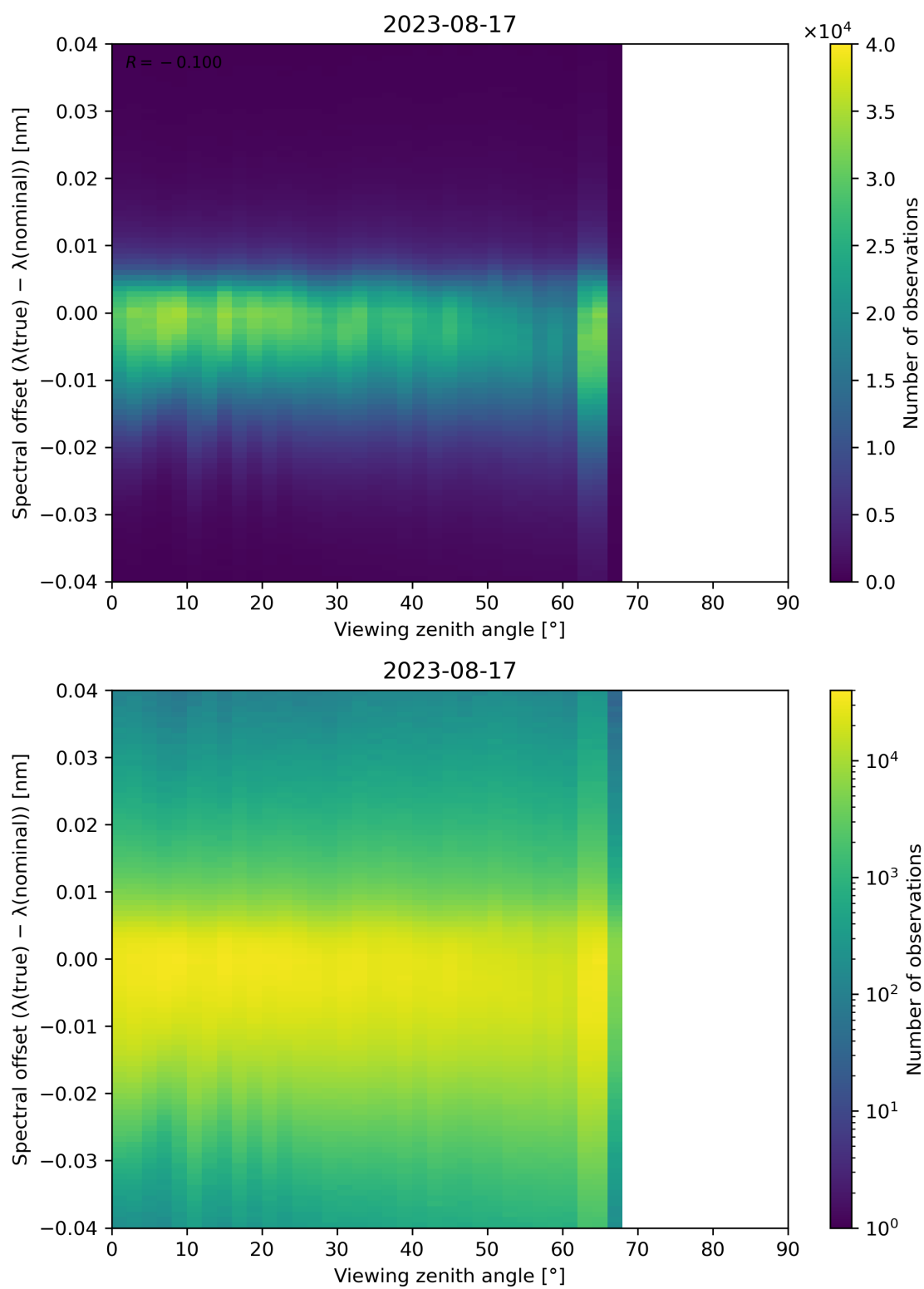
Figure 140: Scatter density plot of “Viewing zenith angle” against “Spectral offset ( \lambda(\text{true}) - \lambda(\text{nominal}) )” for 2023-08-16 to 2023-08-18.
