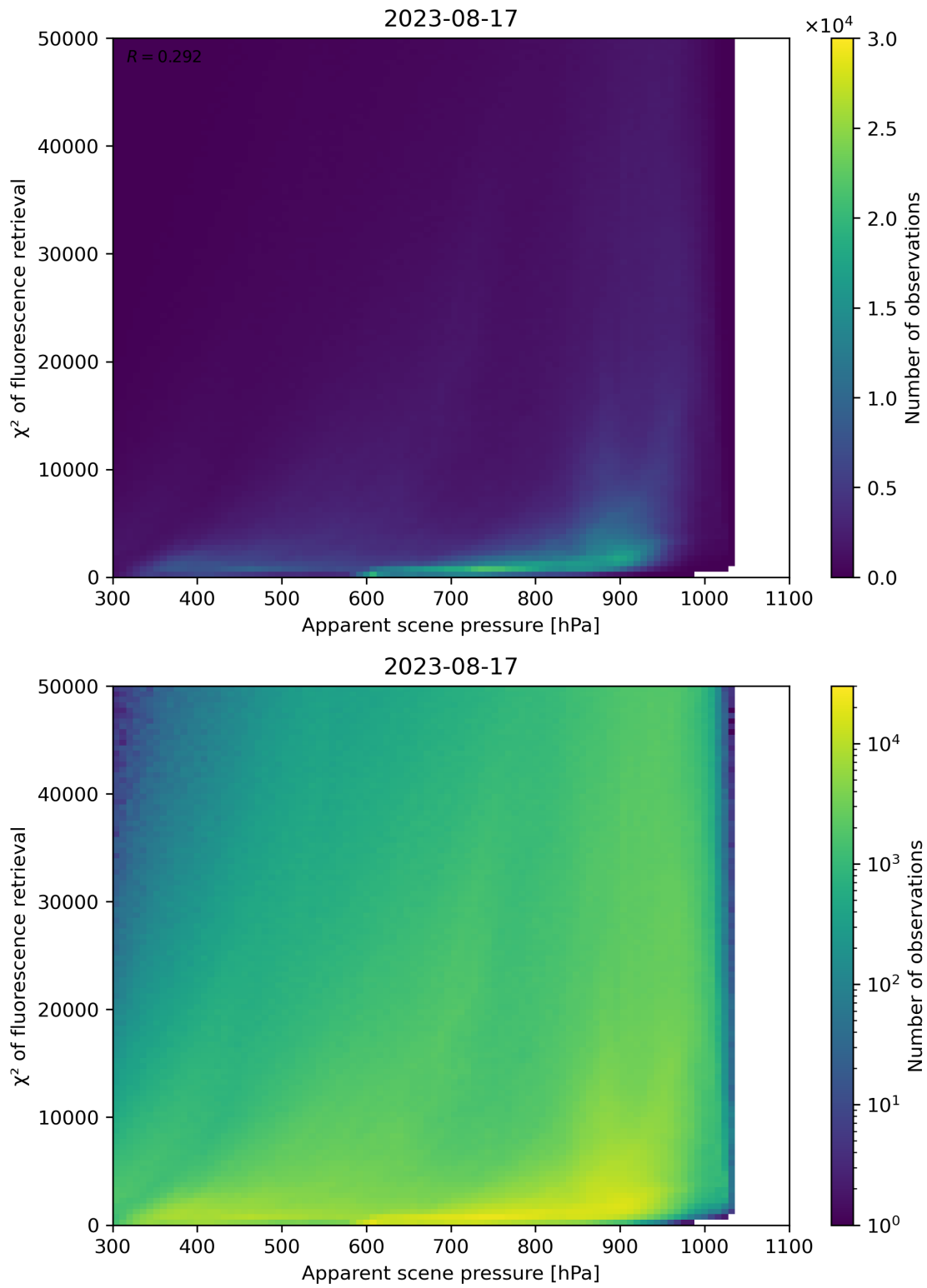
Figure 64: Scatter density plot of “Apparent scene pressure” against “ \chi^2 of fluorescence retrieval” for 2023-08-16 to 2023-08-18.
