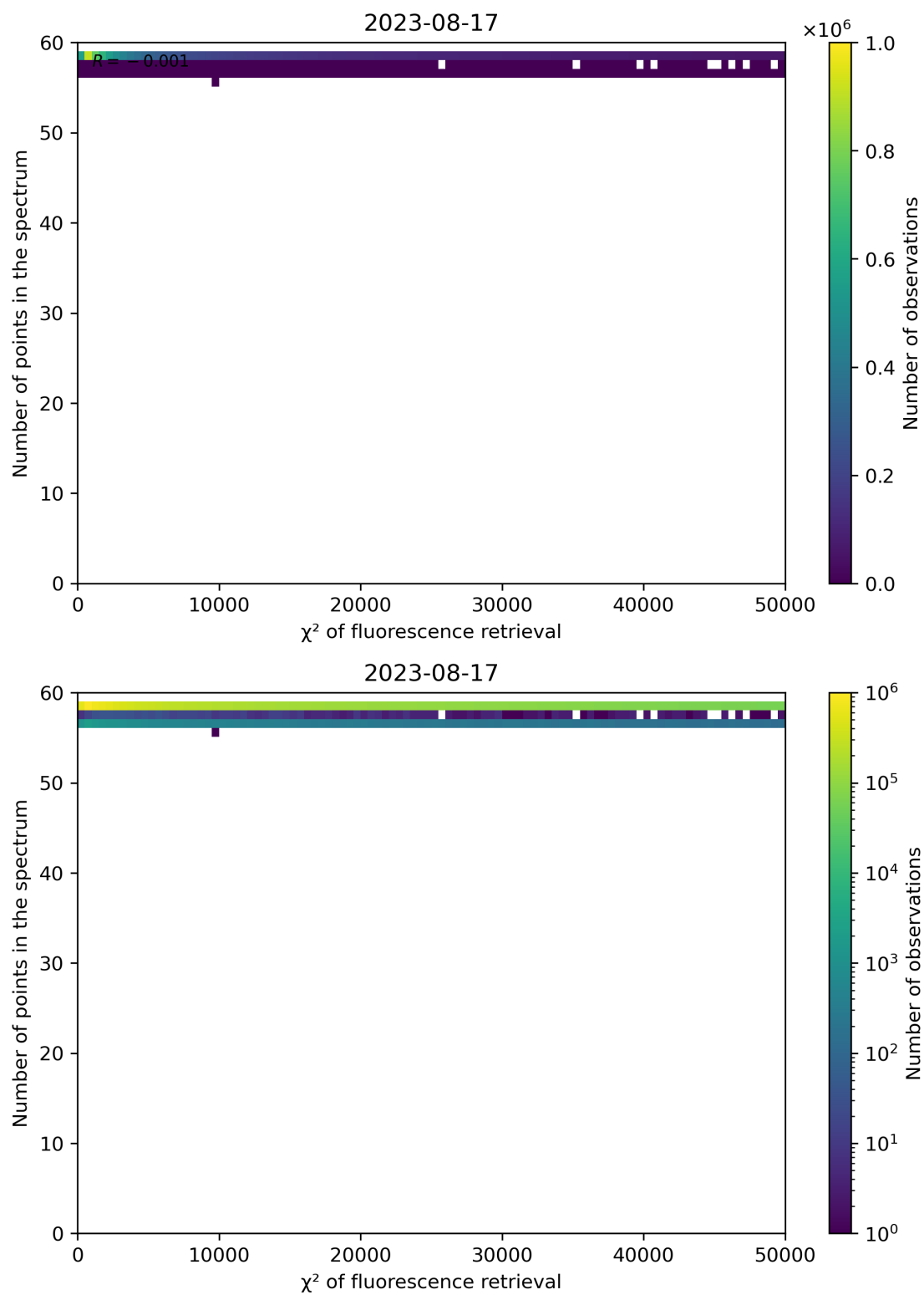
Figure 71: Scatter density plot of “ \chi^2 of fluorescence retrieval” against “Number of points in the spectrum” for 2023-08-16 to 2023-08-18.
