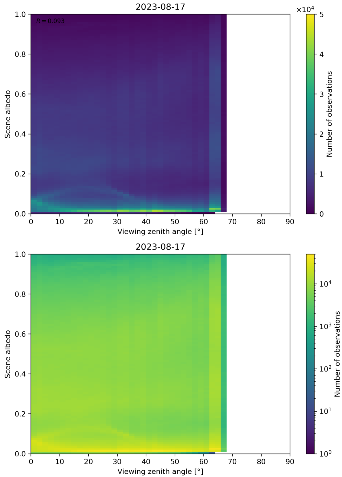
Figure 138: Scatter density plot of “Viewing zenith angle” against “Scene albedo” for 2023-08-16 to 2023-08-18.
