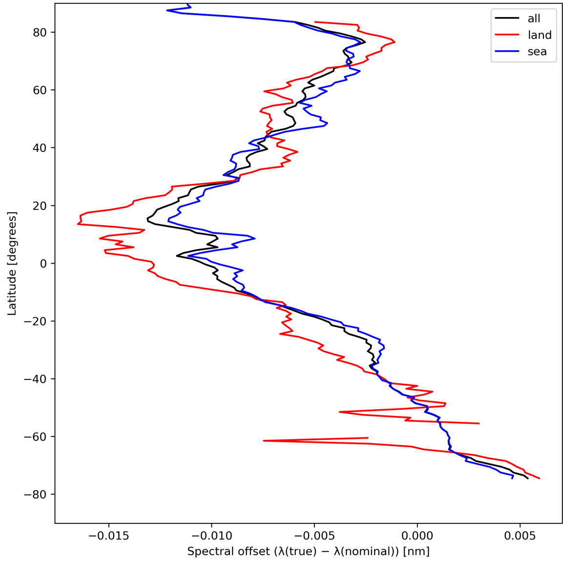
Figure 28: Zonal average of “Spectral offset ( \lambda(\text{true}) - \lambda(\text{nominal}) )” for 2023-08-16 to 2023-08-18.
