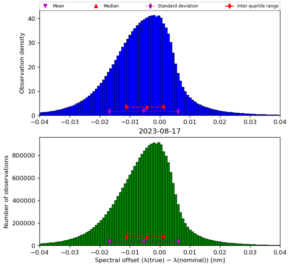
Figure 45: Histogram of “Spectral offset ( \lambda(\text{true}) - \lambda(\text{nominal}) )” for 2023-08-16 to 2023-08-18
