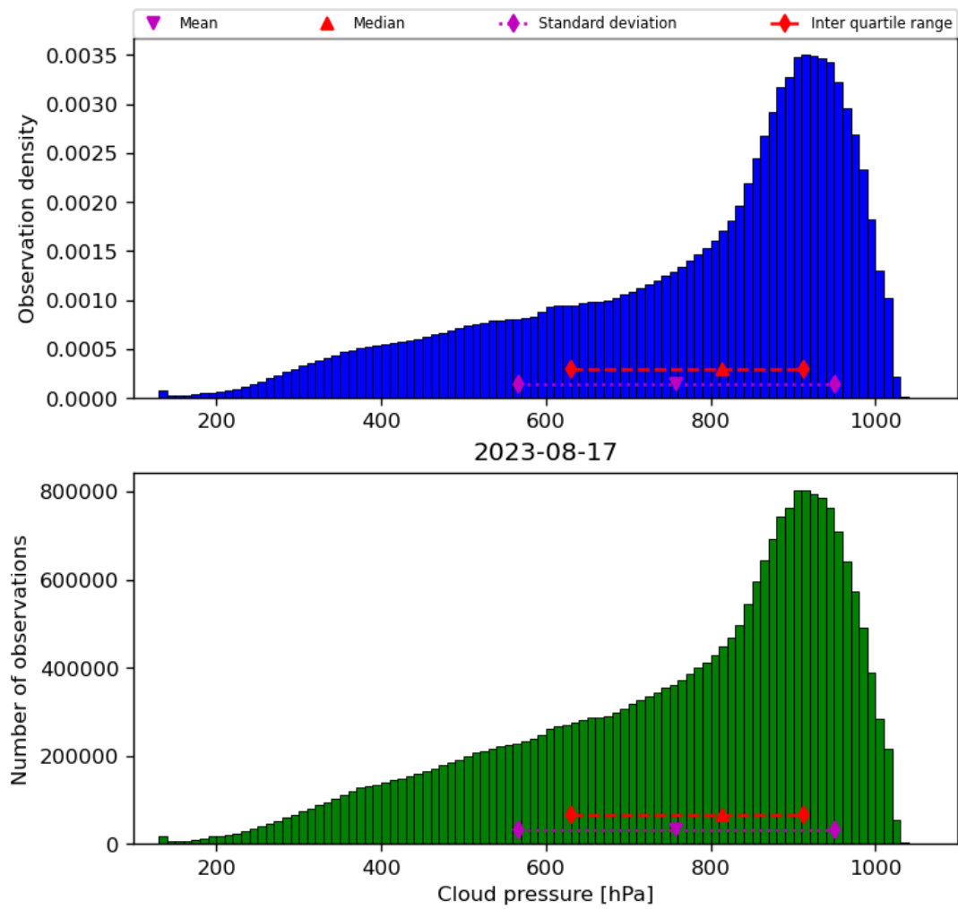
Figure 30: Histogram of “Cloud pressure” for 2023-08-16 to 2023-08-18
