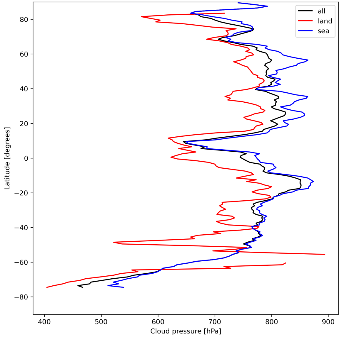
Figure 13: Zonal average of “Cloud pressure” for 2023-08-16 to 2023-08-18.
