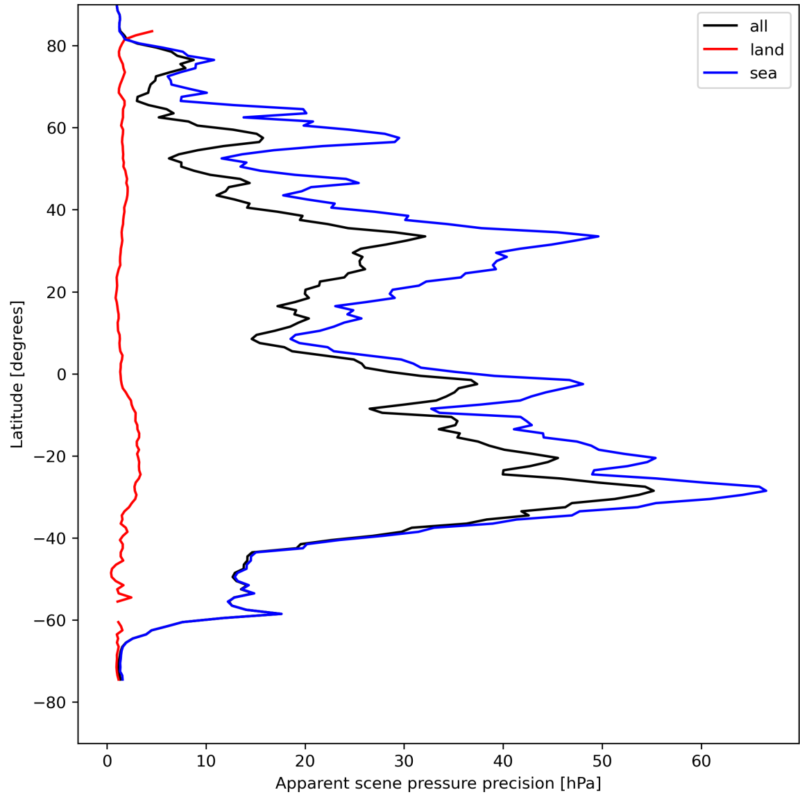
Figure 20: Zonal average of “Apparent scene pressure precision” for 2023-08-16 to 2023-08-18.
