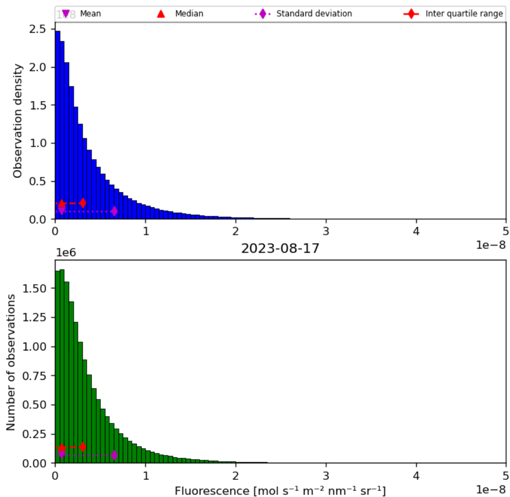
Figure 40: Histogram of “Fluorescence” for 2023-08-16 to 2023-08-18
