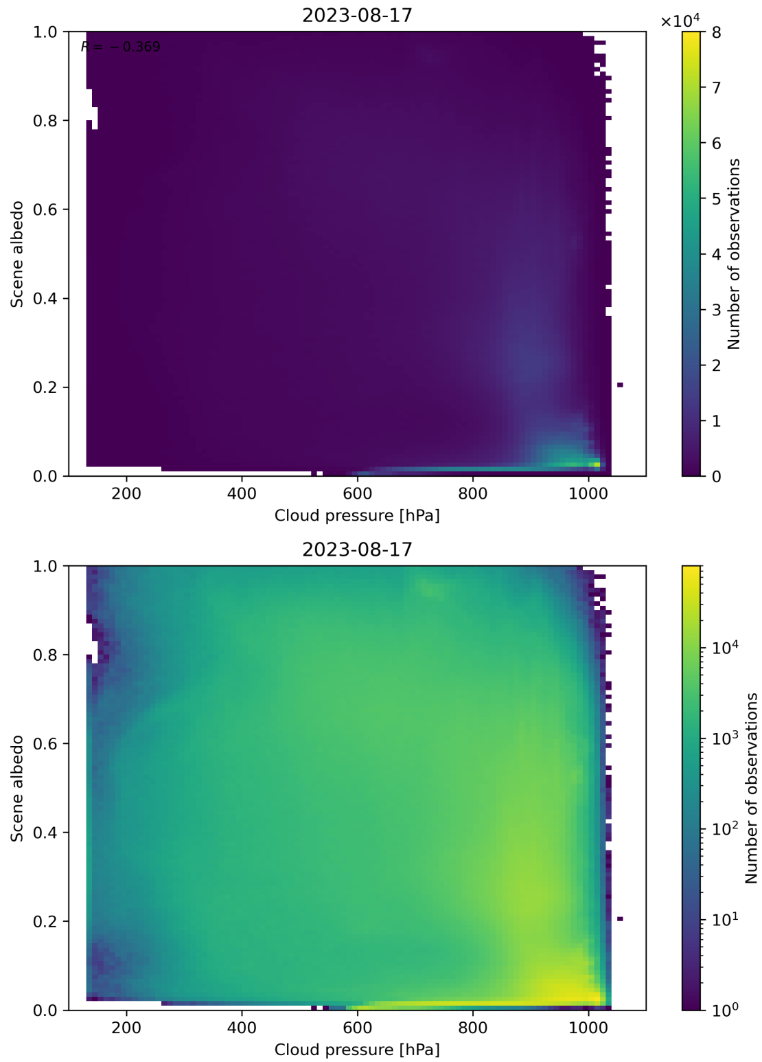
Figure 91: Scatter density plot of “Cloud pressure” against “Scene albedo” for 2023-08-16 to 2023-08-18.
