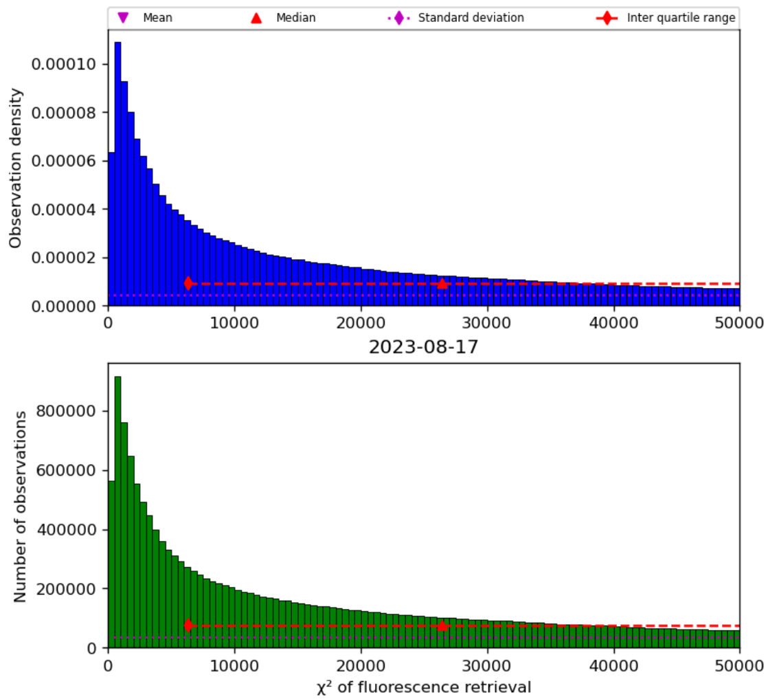
Figure 42: Histogram of “ \chi^2 of fluorescence retrieval” for 2023-08-16 to 2023-08-18
