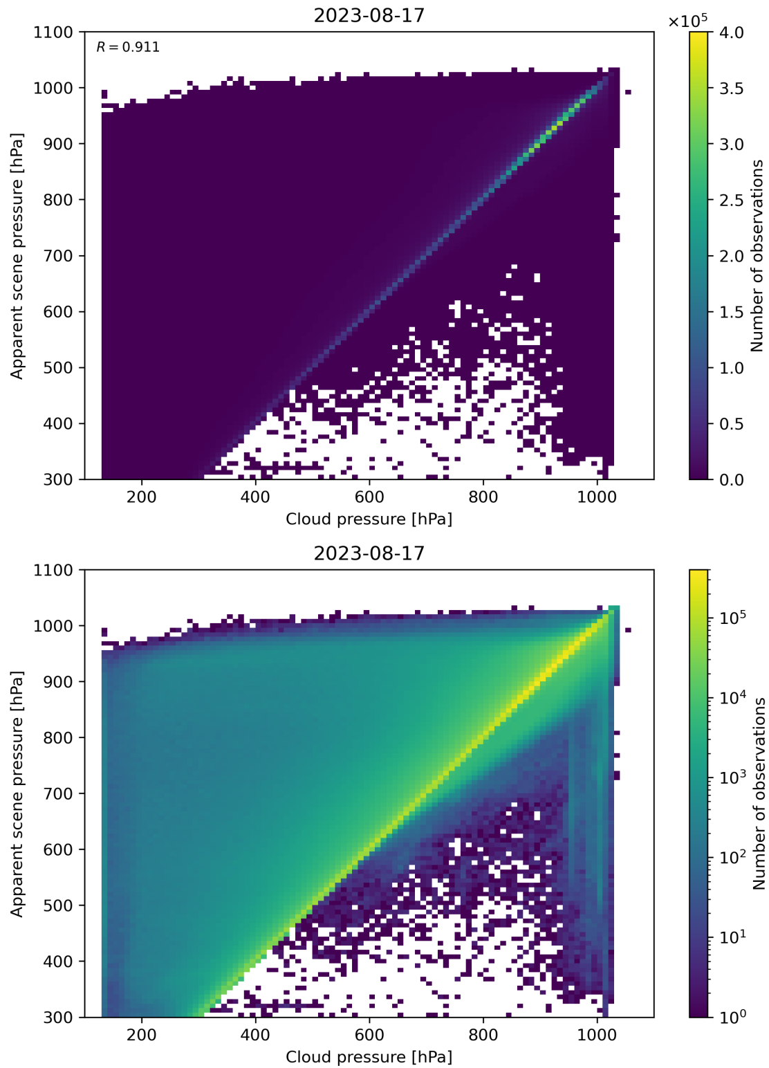
Figure 84: Scatter density plot of “Cloud pressure” against “Apparent scene pressure” for 2023-08-16 to 2023-08-18.
