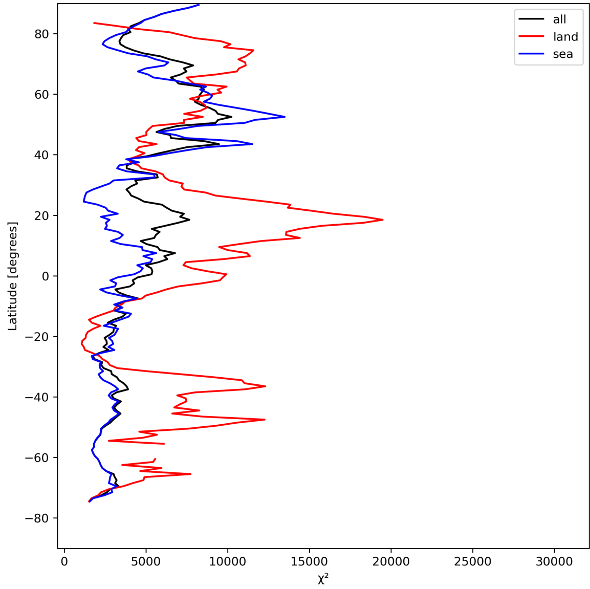
Figure 21: Zonal average of “ \chi^2 ” for 2023-08-16 to 2023-08-18.
