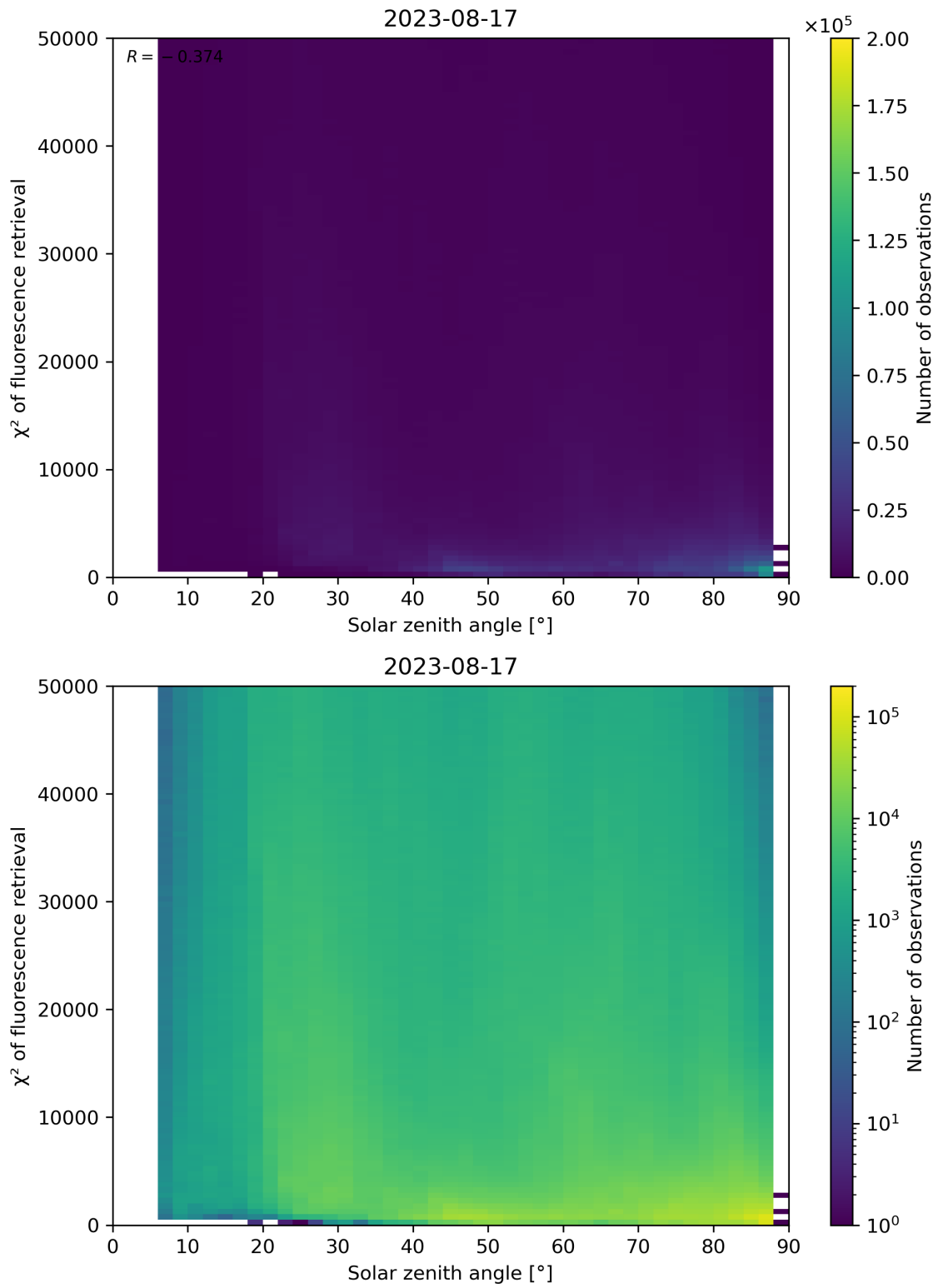
Figure 120: Scatter density plot of “Solar zenith angle” against “ \chi^2 of fluorescence retrieval” for 2023-08-16 to 2023-08-18.
