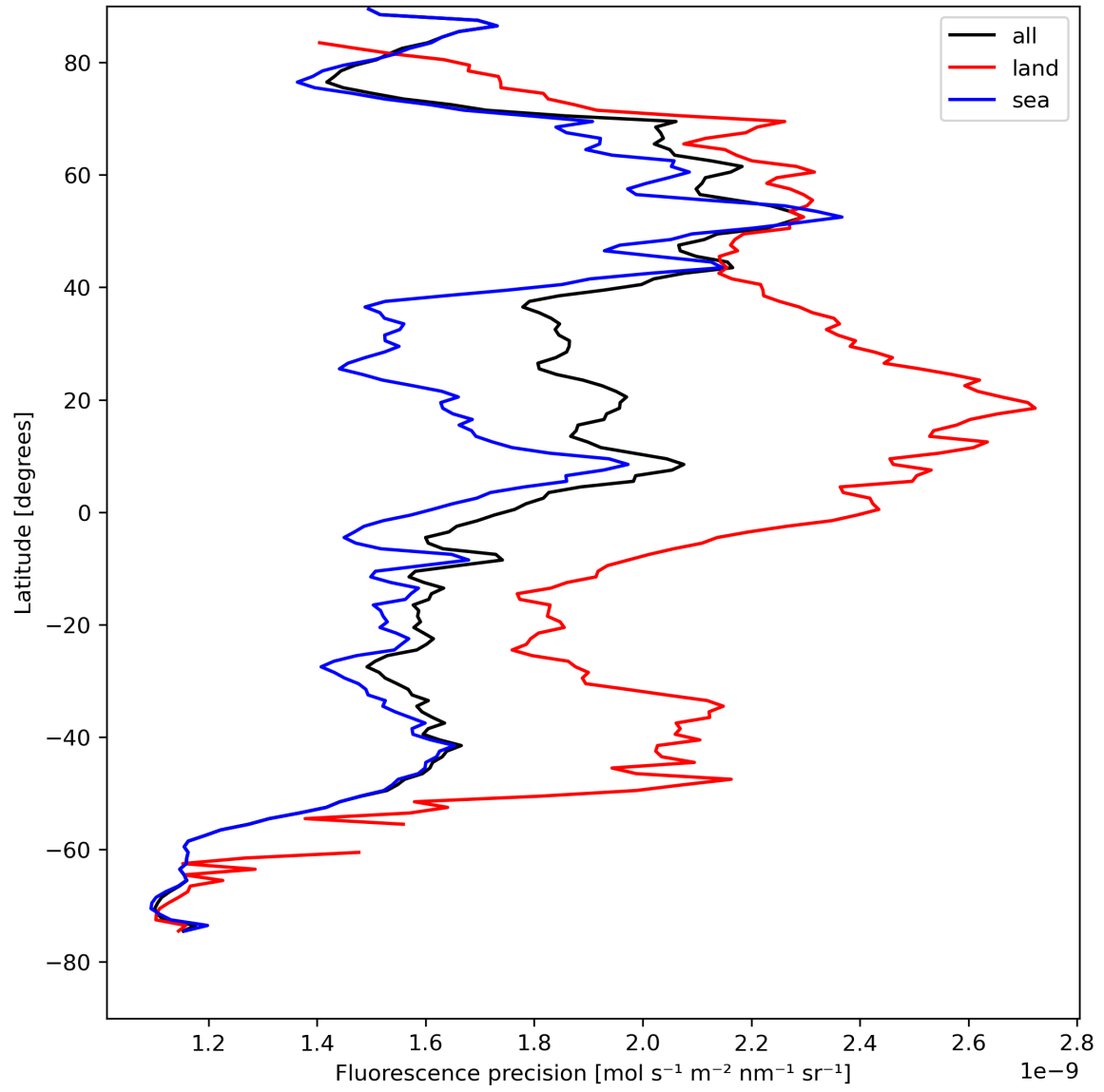
Figure 24: Zonal average of “Fluorescence precision” for 2023-08-16 to 2023-08-18.
