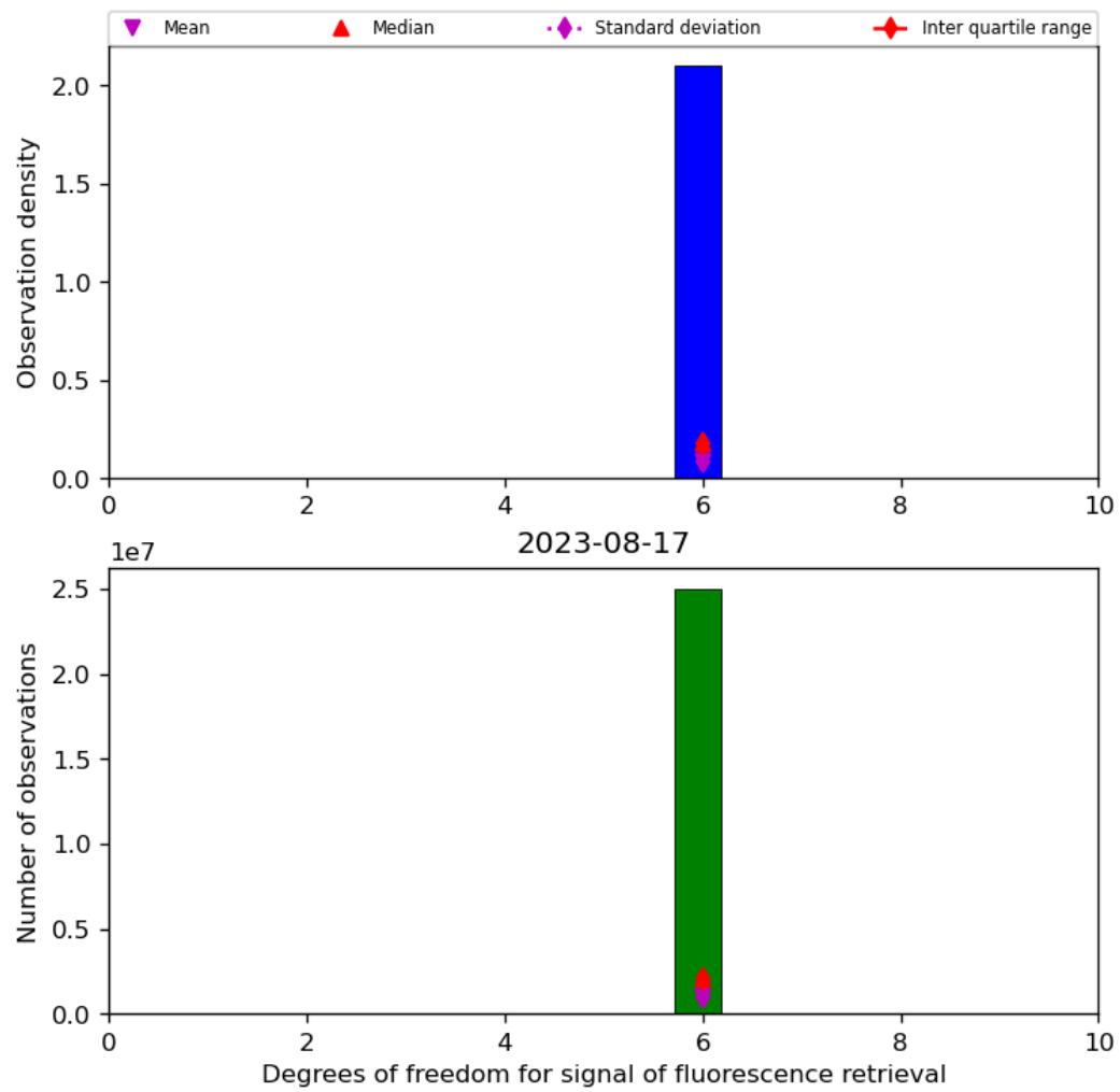
Figure 43: Histogram of “Degrees of freedom for signal of fluorescence retrieval” for 2023-08-16 to 2023-08-18
