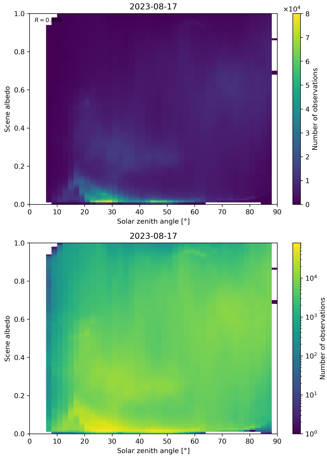
Figure 127: Scatter density plot of “Solar zenith angle” against “Scene albedo” for 2023-08-16 to 2023-08-18.
