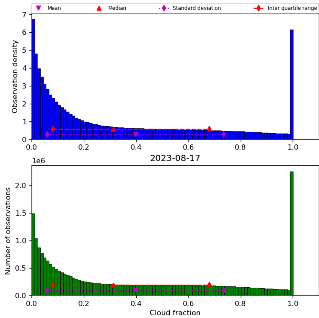
Figure 32: Histogram of “Cloud fraction” for 2023-08-16 to 2023-08-18
