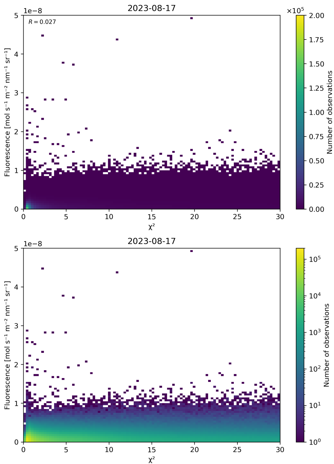
Figure 70: Scatter density plot of “ \chi^2 ” against “Fluorescence” for 2023-08-16 to 2023-08-18.
