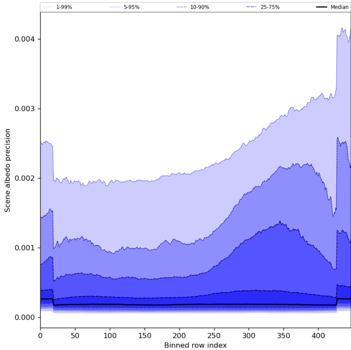
Figure 52: Along track statistics of “Scene albedo precision” for 2023-08-16 to 2023-08-18
