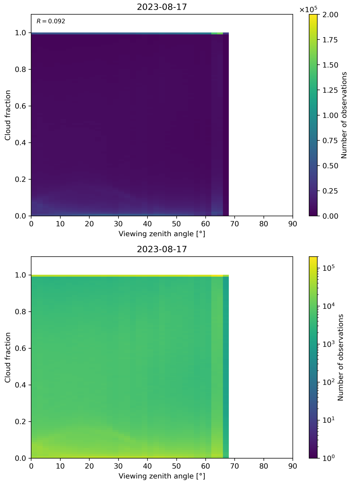
Figure 132: Scatter density plot of “Viewing zenith angle” against “Cloud fraction” for 2023-08-16 to 2023-08-18.
