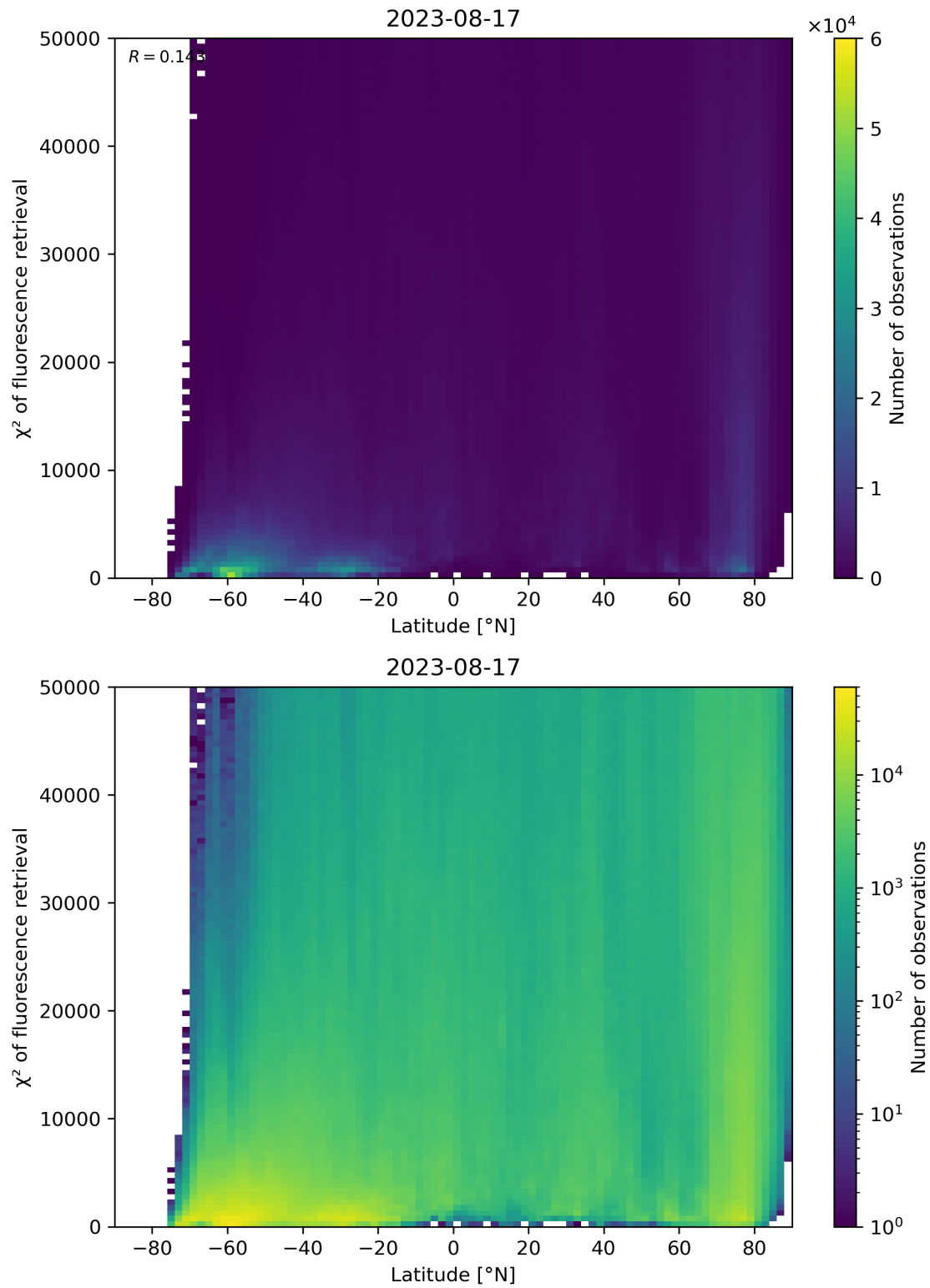
Figure 98: Scatter density plot of “Latitude” against “ \chi^2 of fluorescence retrieval” for 2023-08-16 to 2023-08-18.
