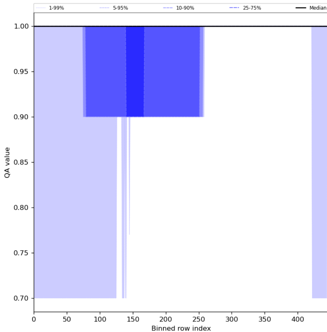
Figure 46: Along track statistics of “QA value” for 2023-08-16 to 2023-08-18
