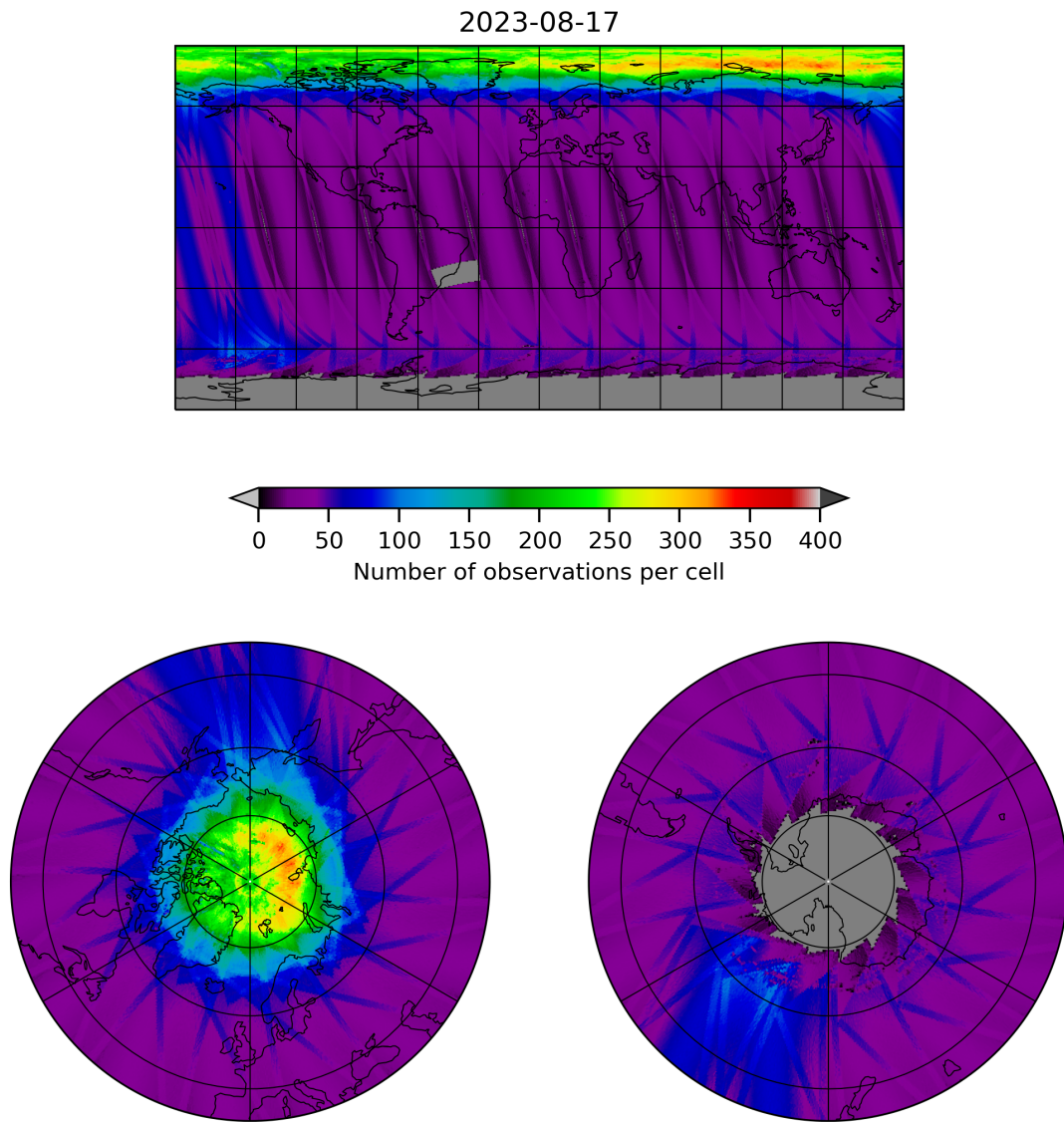
Figure 11: Map of the number of observations for 2023-08-16 to 2023-08-18
