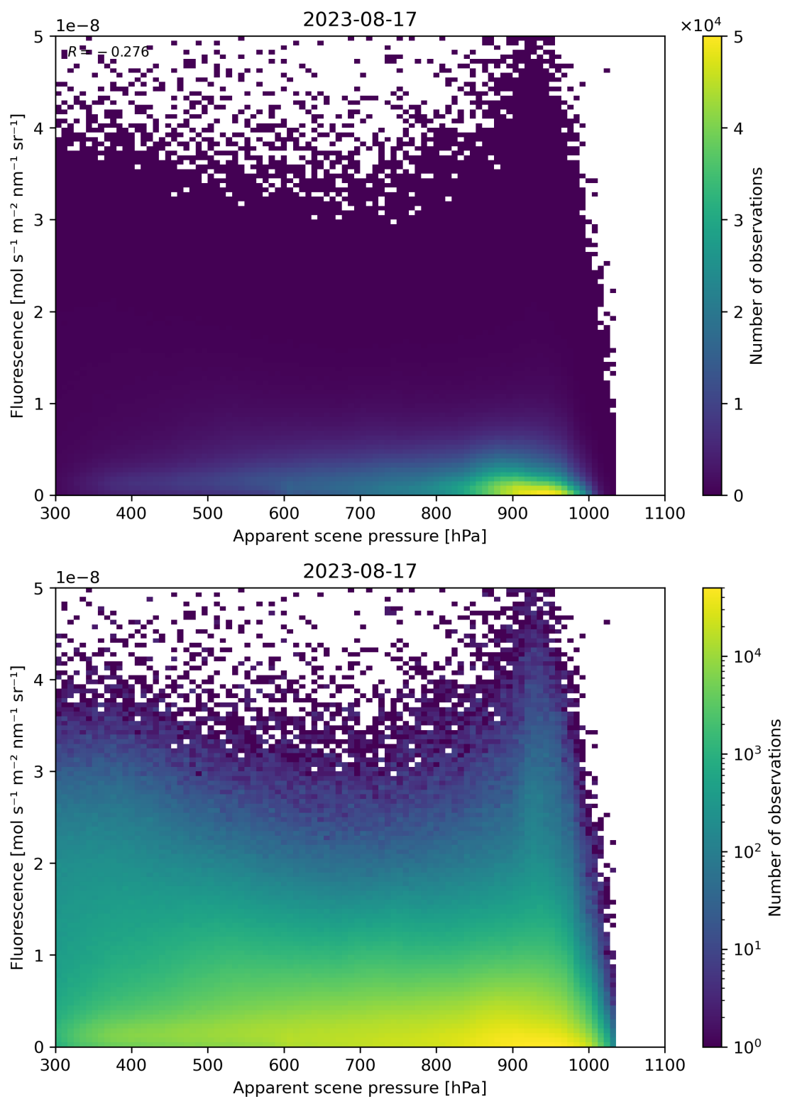
Figure 65: Scatter density plot of “Apparent scene pressure” against “Fluorescence” for 2023-08-16 to 2023-08-18.
