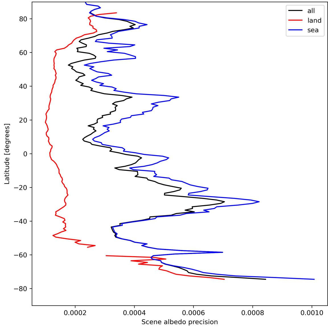
Figure 18: Zonal average of “Scene albedo precision” for 2023-08-16 to 2023-08-18.
