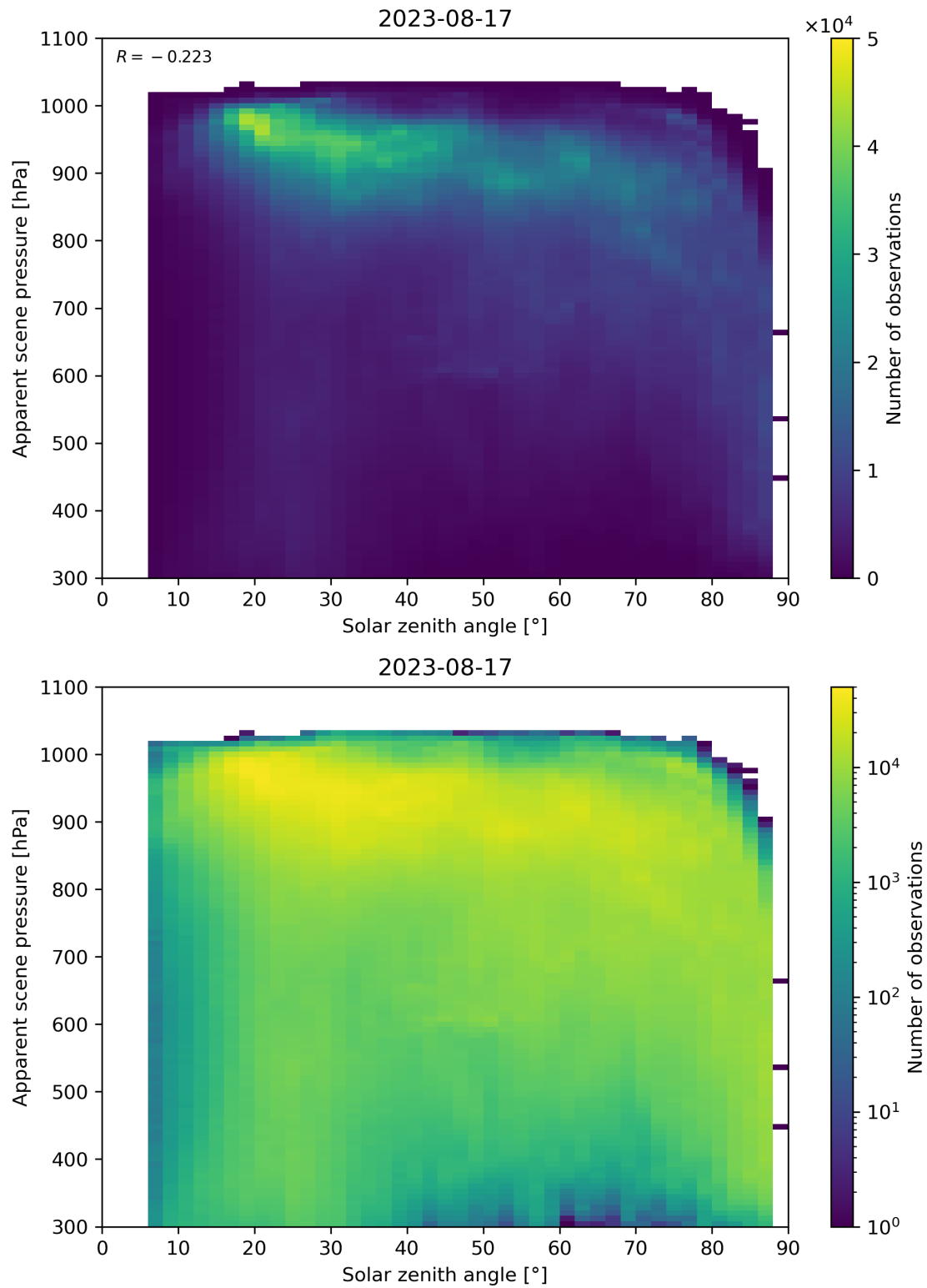
Figure 118: Scatter density plot of “Solar zenith angle” against “Apparent scene pressure” for 2023-08-16 to 2023-08-18.
