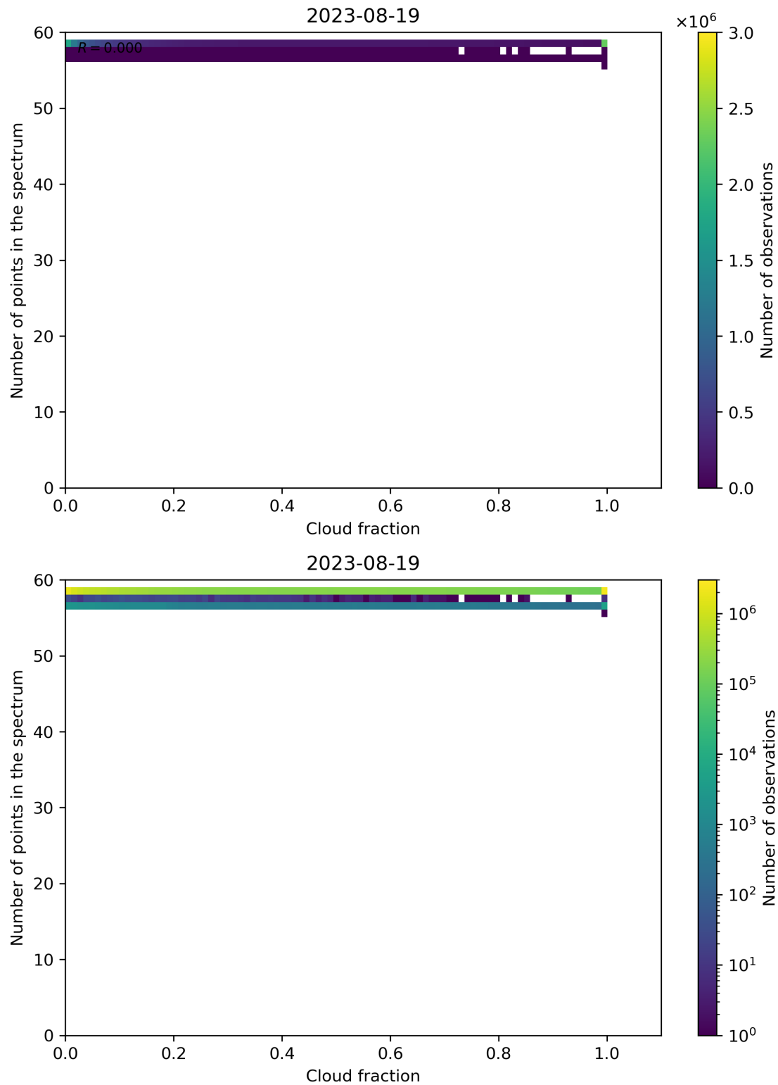
Figure 81: Scatter density plot of “Cloud fraction” against “Number of points in the spectrum” for 2023-08-18 to 2023-08-20.
