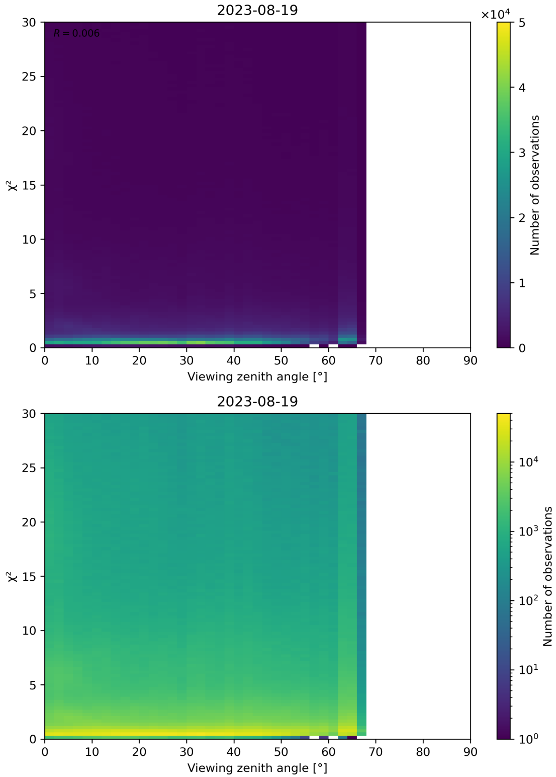
Figure 130: Scatter density plot of “Viewing zenith angle” against “ \chi^2 ” for 2023-08-18 to 2023-08-20.
