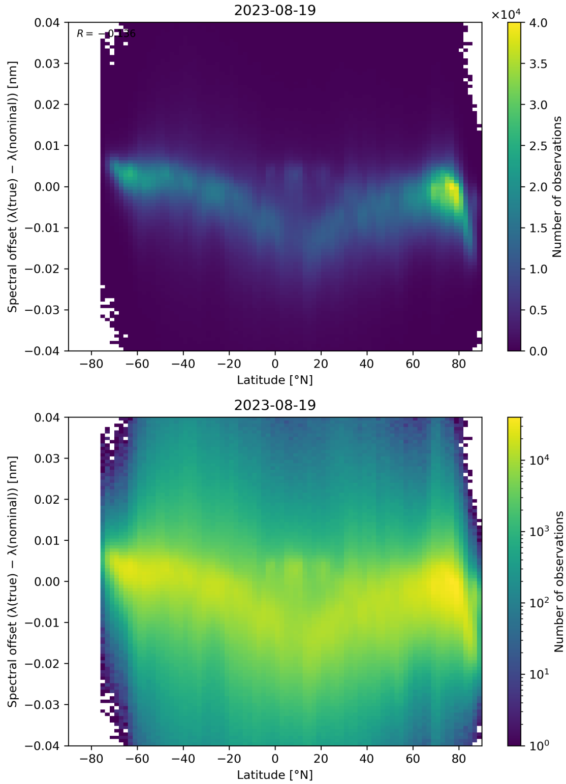
Figure 105: Scatter density plot of “Latitude” against “Spectral offset ( \lambda(\text{true}) - \lambda(\text{nominal}) )” for 2023-08-18 to 2023-08-20.
