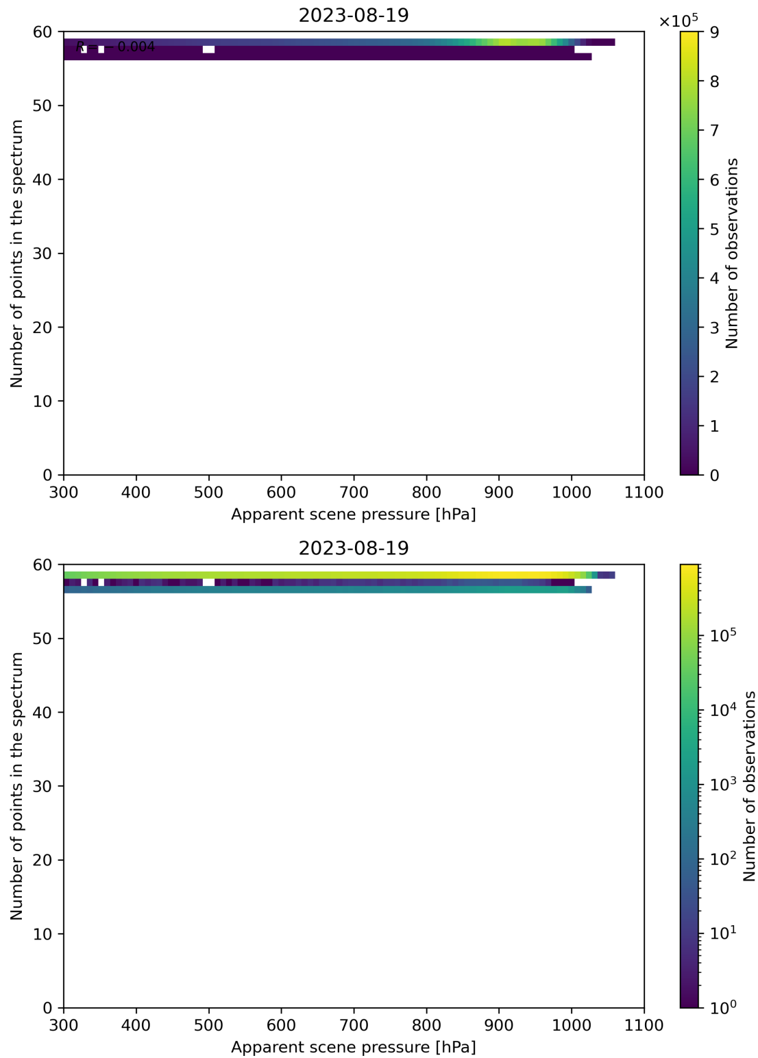
Figure 67: Scatter density plot of “Apparent scene pressure” against “Number of points in the spectrum” for 2023-08-18 to 2023-08-20.
