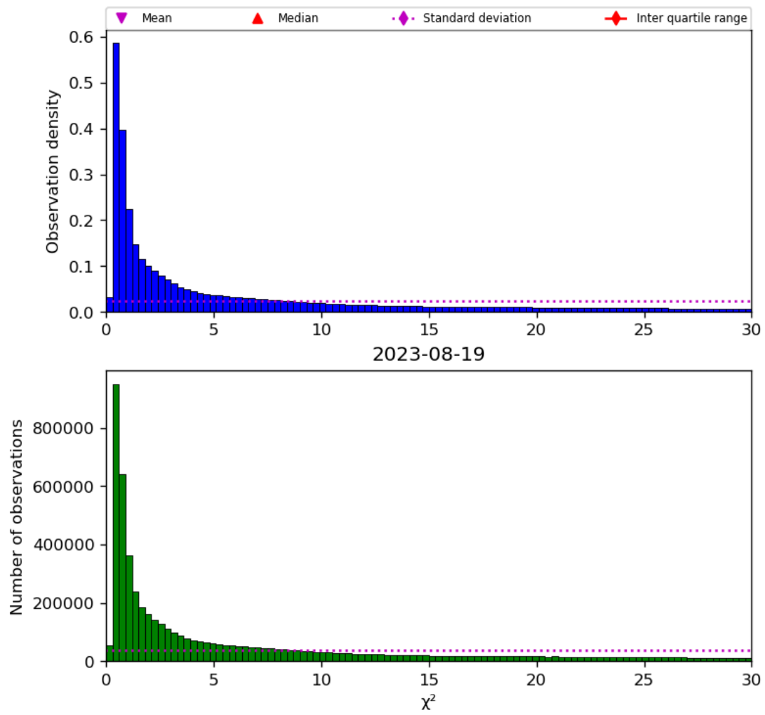
Figure 38: Histogram of “ \chi^2 ” for 2023-08-18 to 2023-08-20
