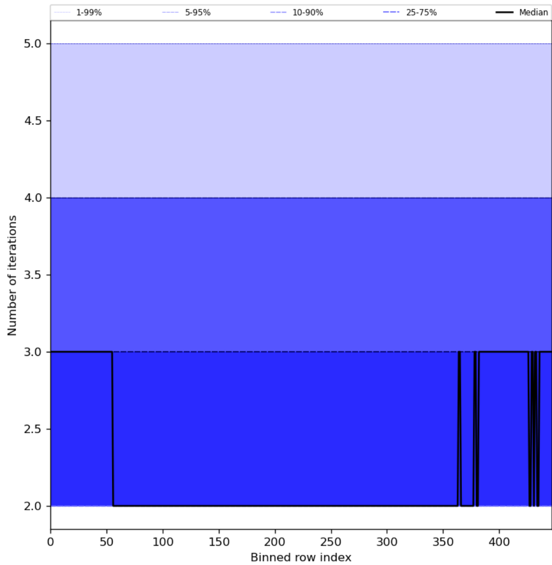
Figure 56: Along track statistics of “Number of iterations” for 2023-08-18 to 2023-08-20
