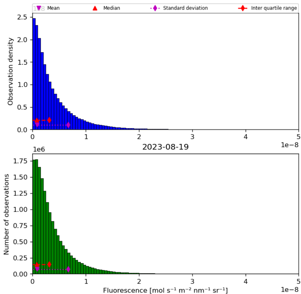
Figure 40: Histogram of “Fluorescence” for 2023-08-18 to 2023-08-20
