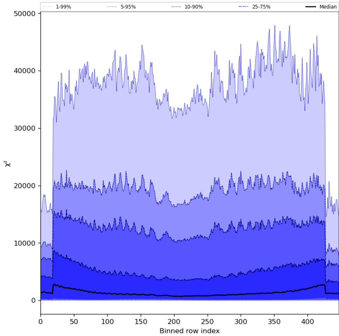
Figure 55: Along track statistics of “ \chi^2 ” for 2023-08-18 to 2023-08-20
