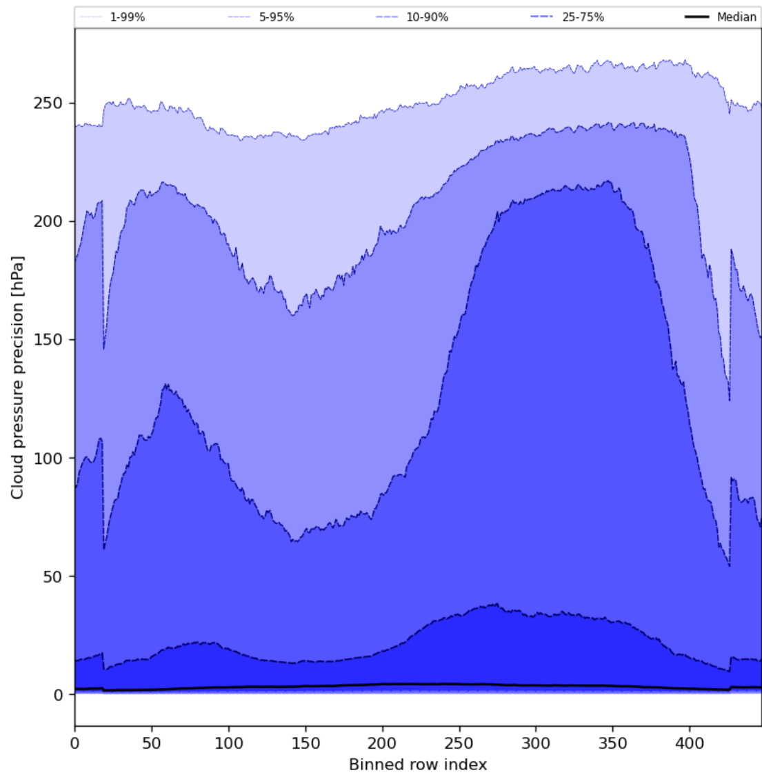
Figure 48: Along track statistics of “Cloud pressure precision” for 2023-08-18 to 2023-08-20
