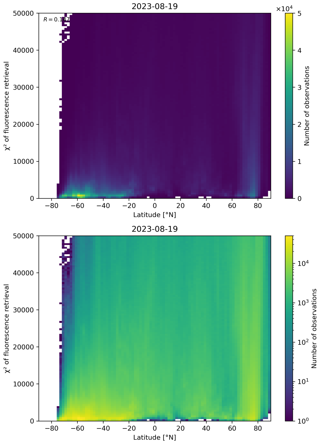
Figure 98: Scatter density plot of “Latitude” against “ \chi^2 of fluorescence retrieval” for 2023-08-18 to 2023-08-20.
