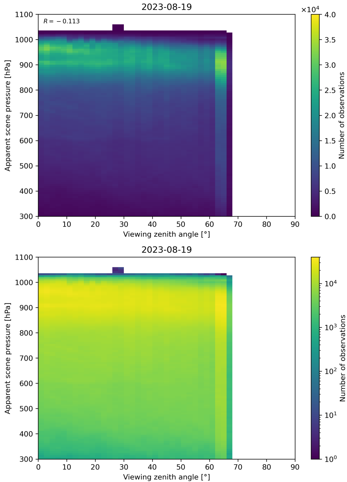
Figure 129: Scatter density plot of “Viewing zenith angle” against “Apparent scene pressure” for 2023-08-18 to 2023-08-20.
