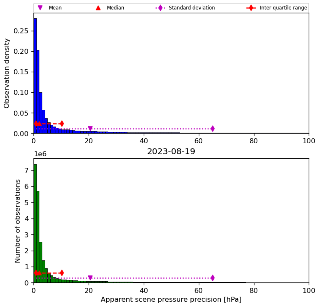
Figure 37: Histogram of “Apparent scene pressure precision” for 2023-08-18 to 2023-08-20
