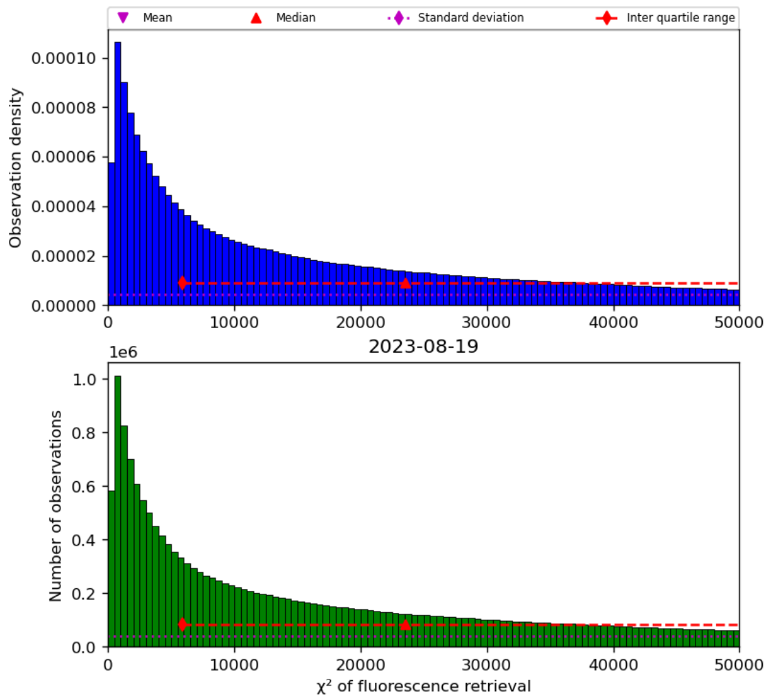
Figure 42: Histogram of “ \chi^2 of fluorescence retrieval” for 2023-08-18 to 2023-08-20
