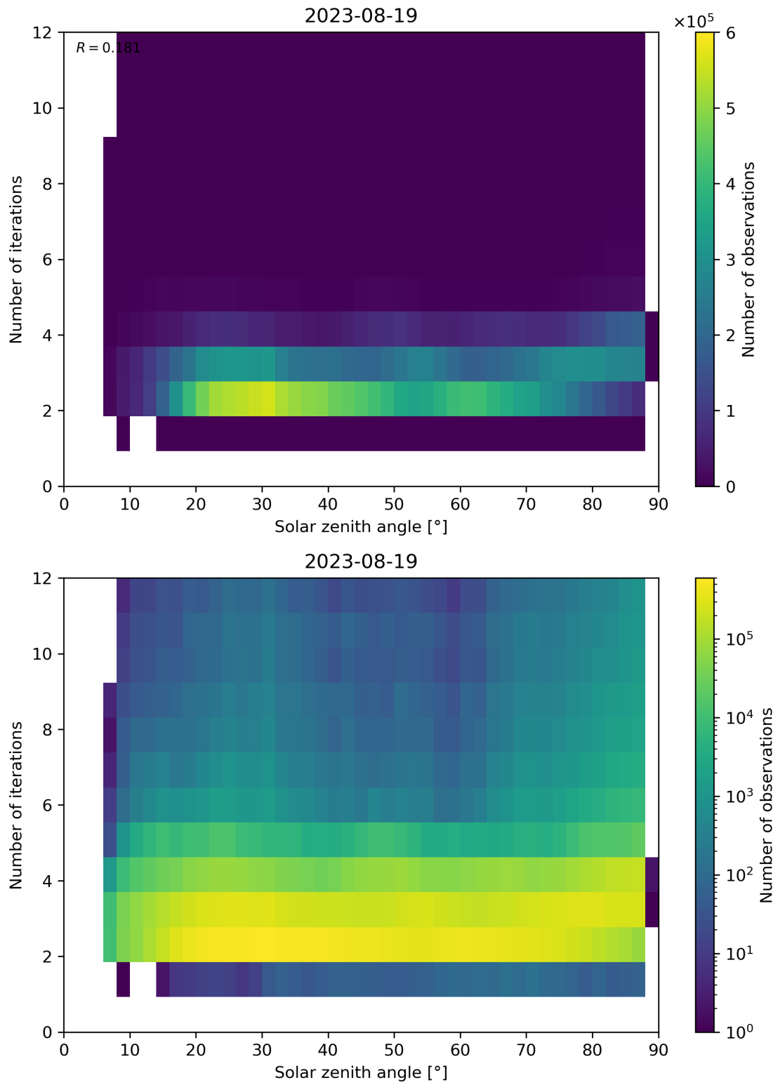
Figure 125: Scatter density plot of “Solar zenith angle” against “Number of iterations” for 2023-08-18 to 2023-08-20.
