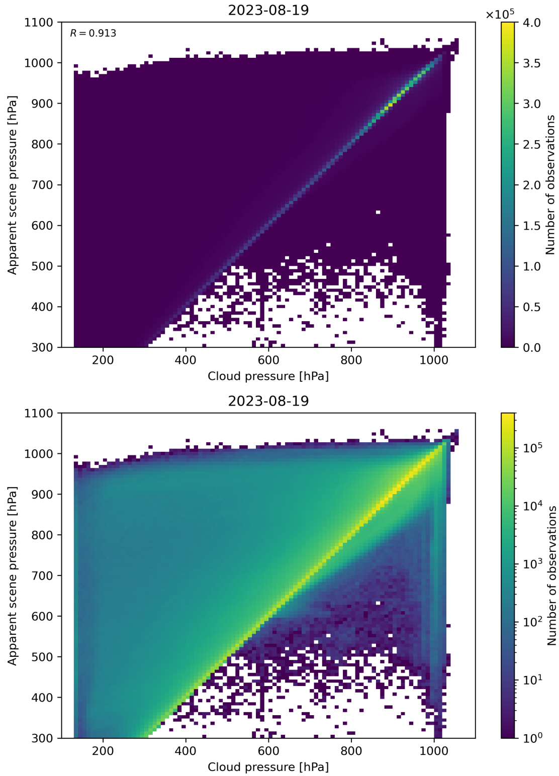
Figure 84: Scatter density plot of “Cloud pressure” against “Apparent scene pressure” for 2023-08-18 to 2023-08-20.
