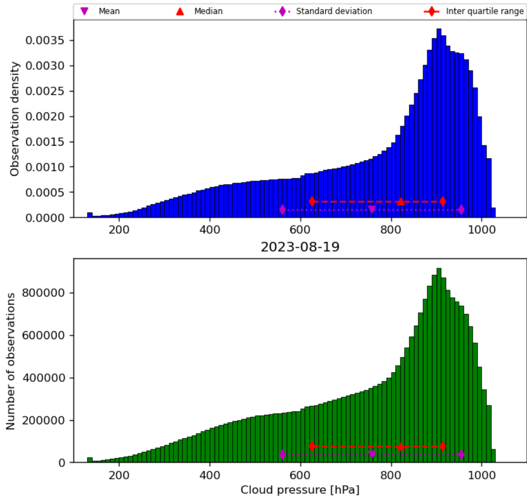
Figure 30: Histogram of “Cloud pressure” for 2023-08-18 to 2023-08-20
