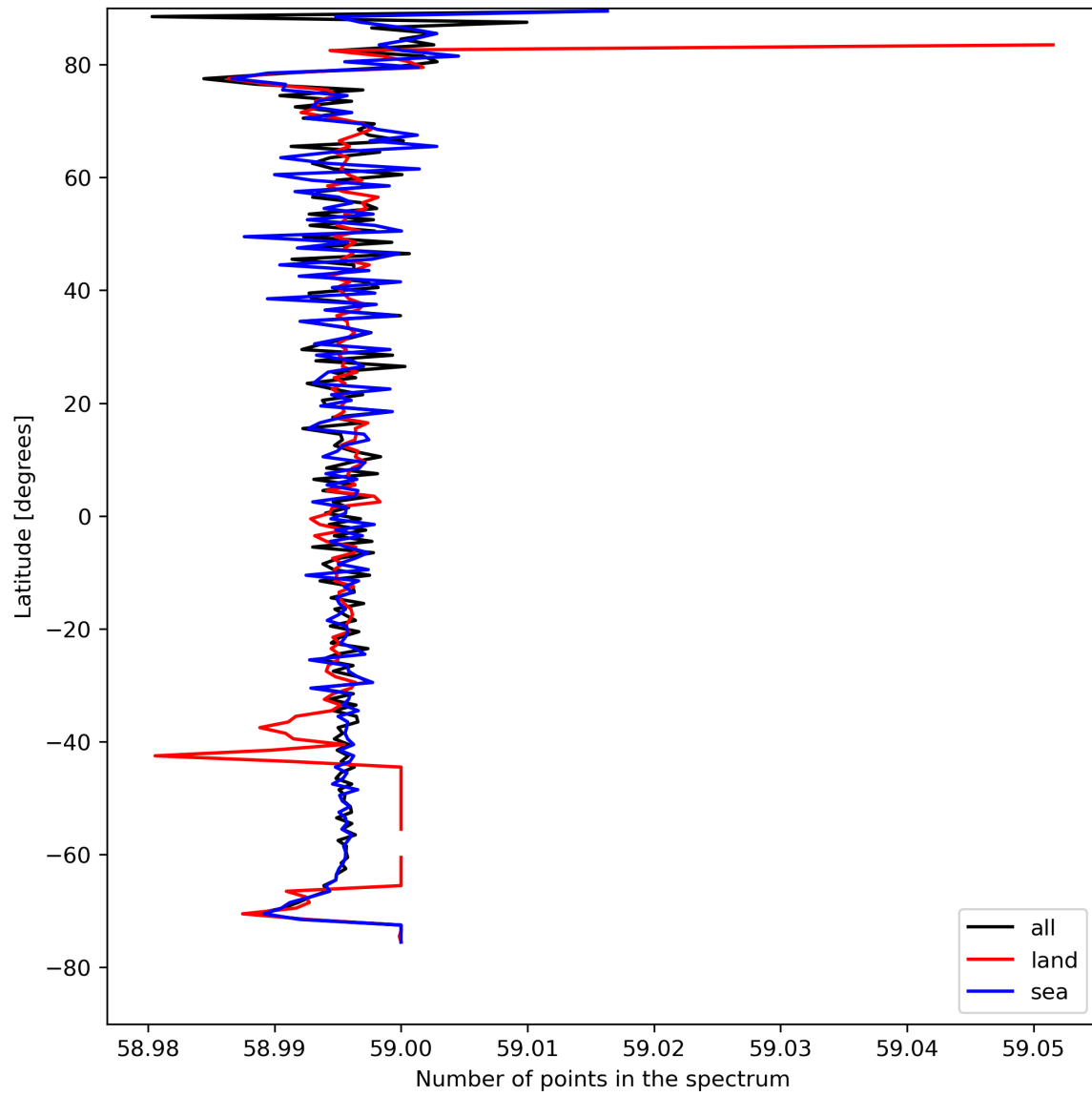
Figure 27: Zonal average of “Number of points in the spectrum” for 2023-08-18 to 2023-08-20.
