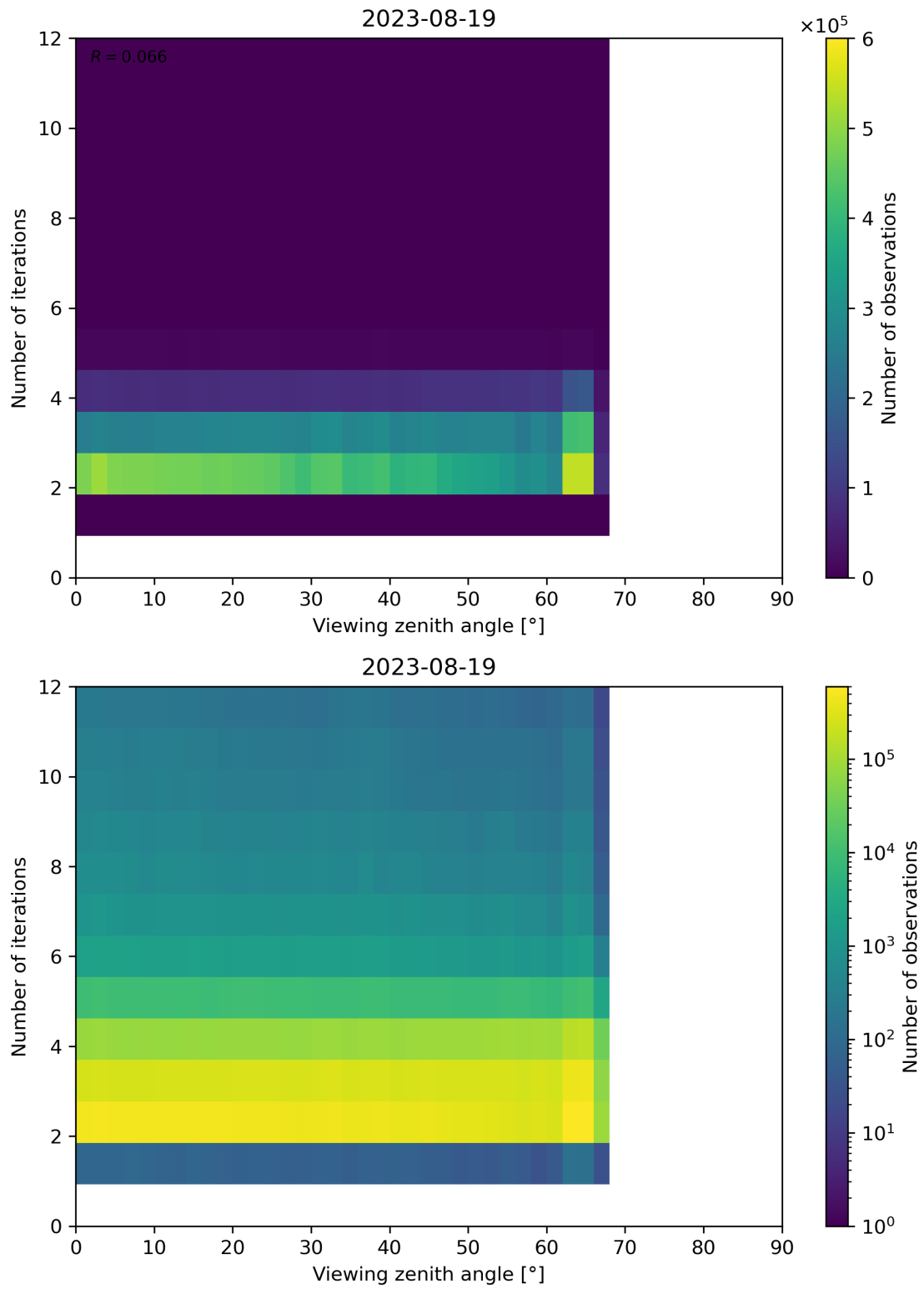
Figure 136: Scatter density plot of “Viewing zenith angle” against “Number of iterations” for 2023-08-18 to 2023-08-20.
