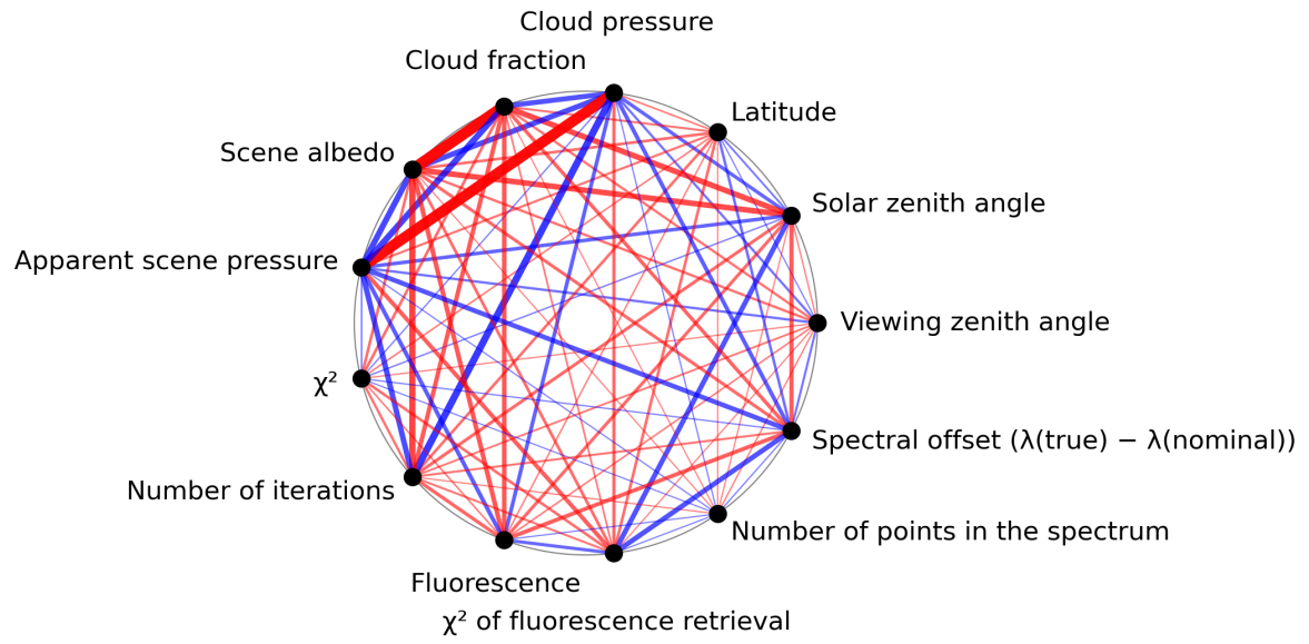
Figure 1: Map of correlation graph for 2023-08-18 to 2023-08-20.
