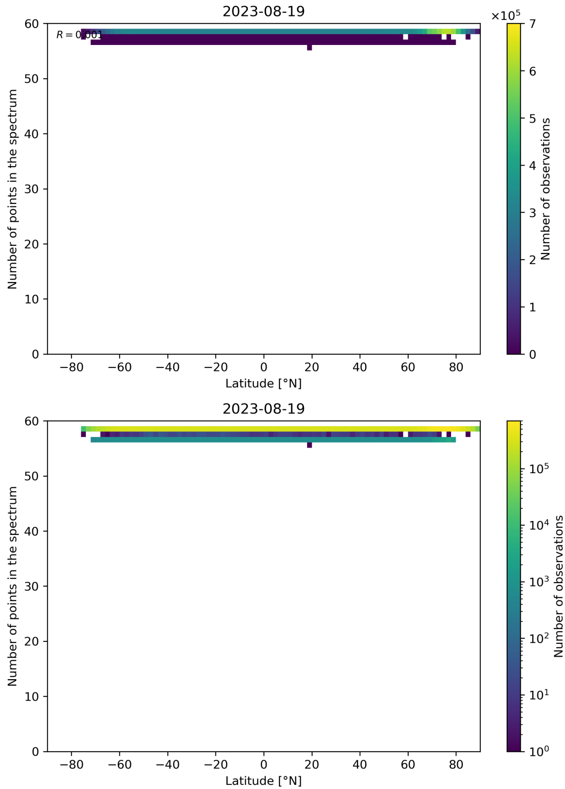
Figure 103: Scatter density plot of “Latitude” against “Number of points in the spectrum” for 2023-08-18 to 2023-08-20.
