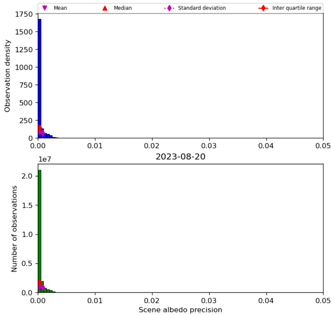
Figure 35: Histogram of “Scene albedo precision” for 2023-08-20 to 2023-08-21
