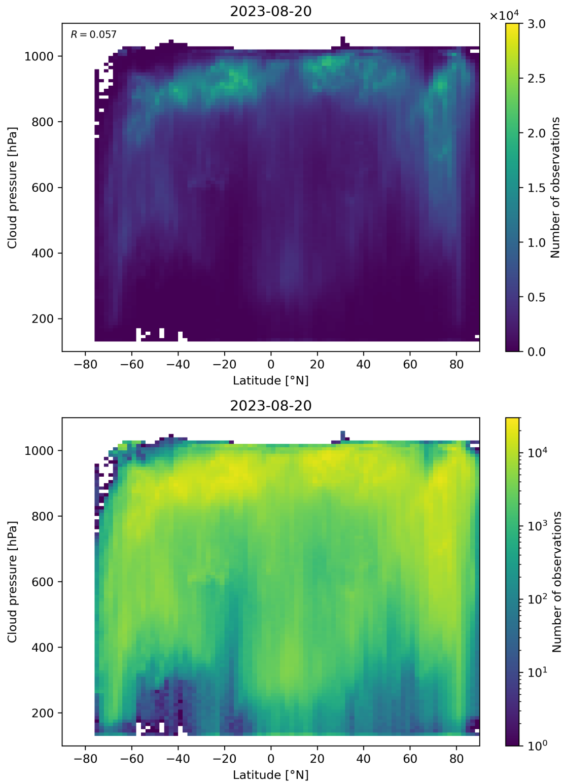
Figure 100: Scatter density plot of “Latitude” against “Cloud pressure” for 2023-08-20 to 2023-08-21.
