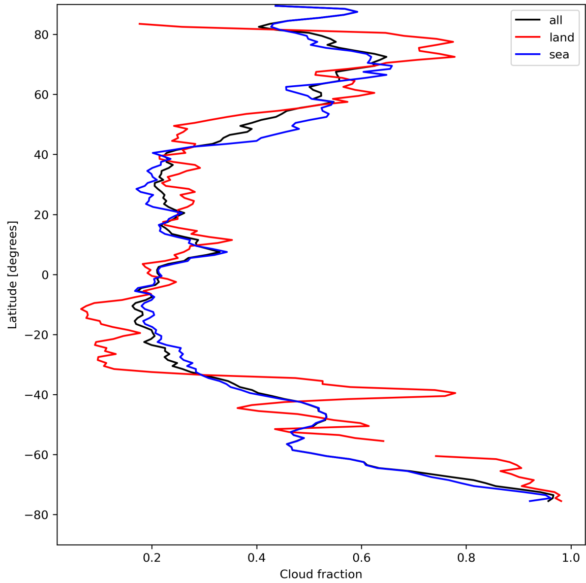
Figure 15: Zonal average of “Cloud fraction” for 2023-08-20 to 2023-08-21.
