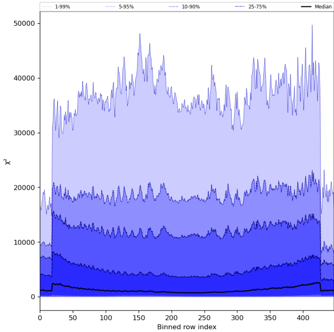
Figure 55: Along track statistics of “ \chi^2 ” for 2023-08-20 to 2023-08-21
