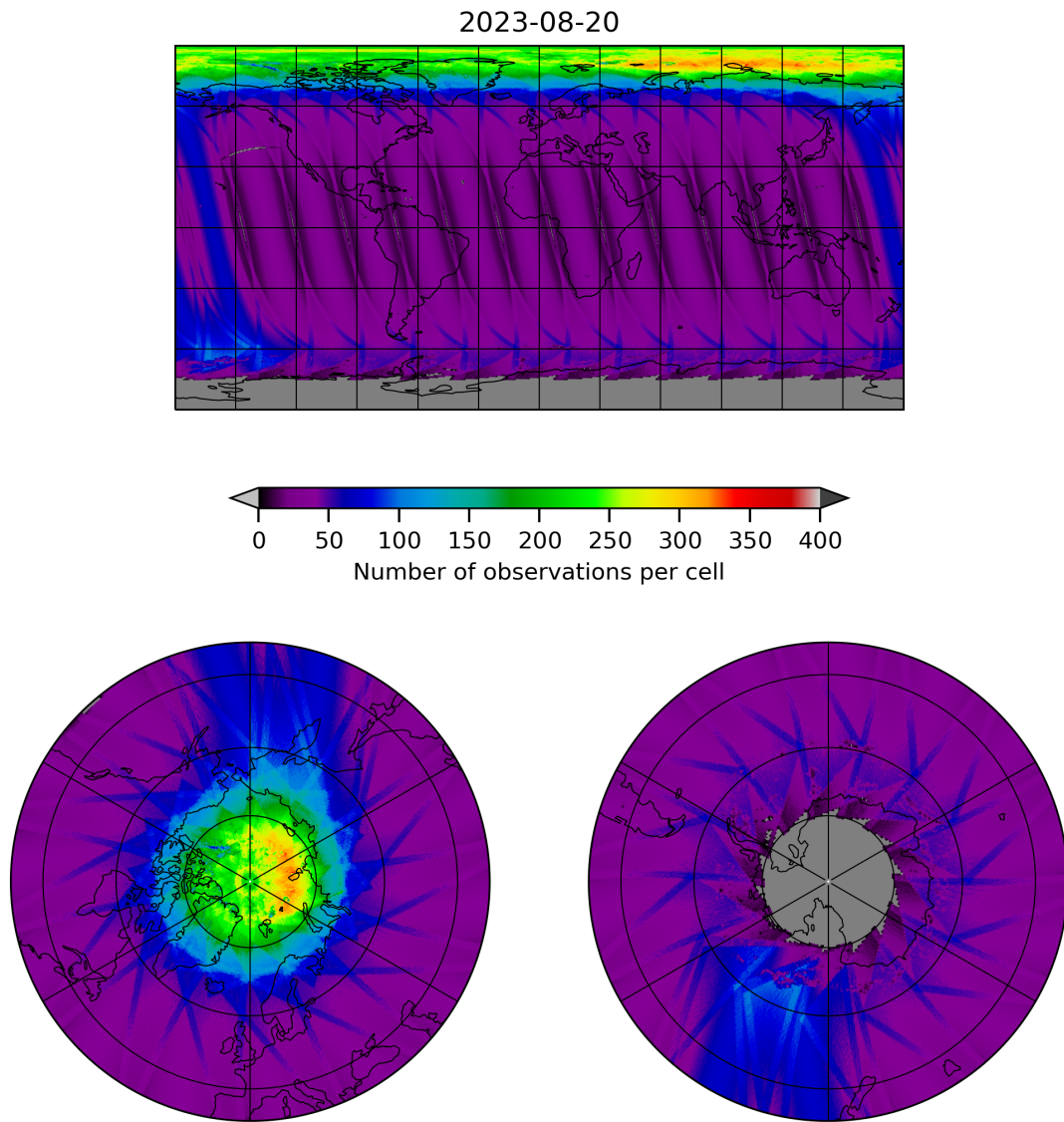
Figure 11: Map of the number of observations for 2023-08-20 to 2023-08-21
