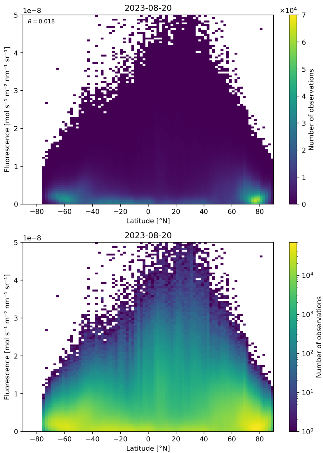
Figure 101: Scatter density plot of “Latitude” against “Fluorescence” for 2023-08-20 to 2023-08-21.
