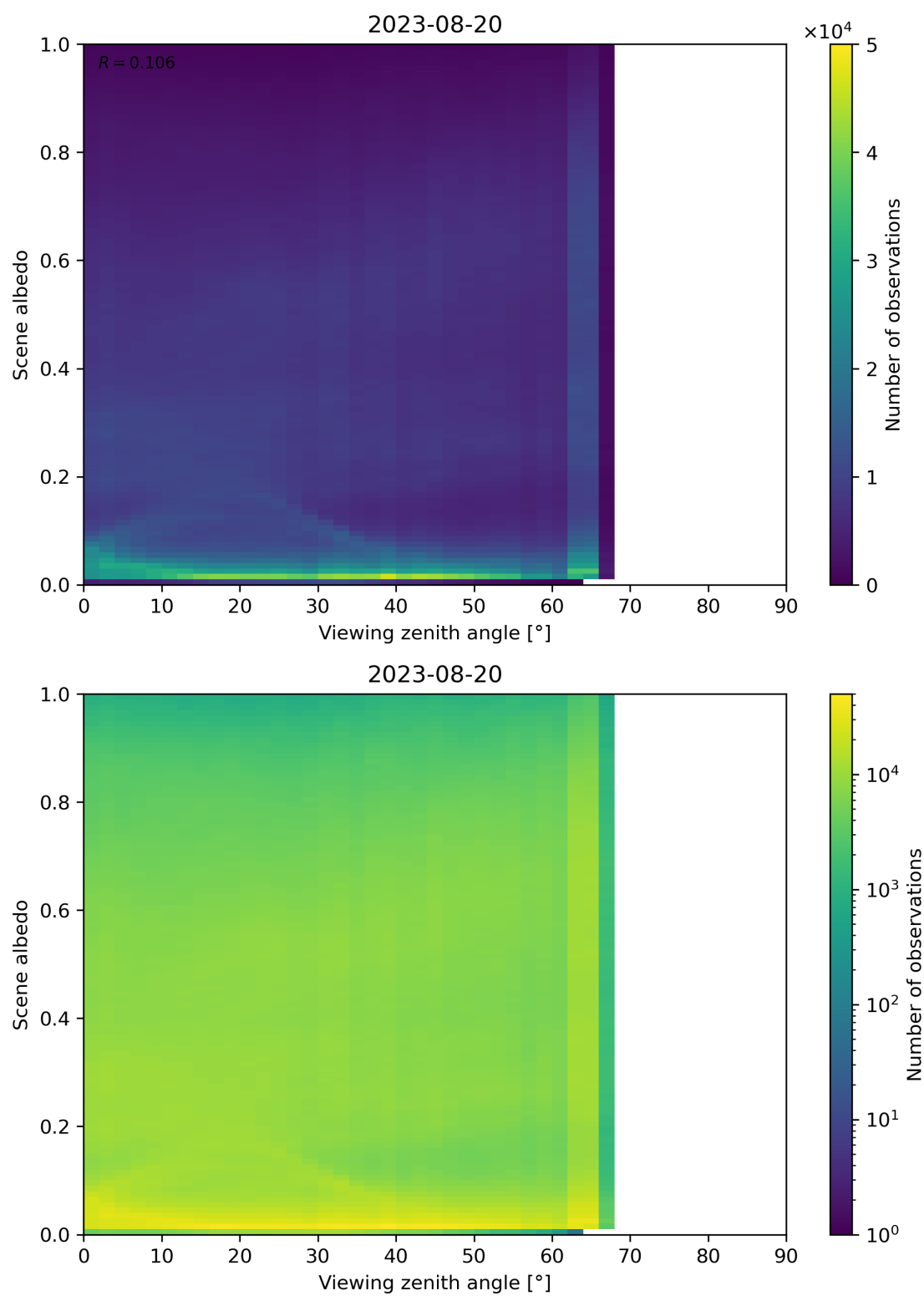
Figure 138: Scatter density plot of “Viewing zenith angle” against “Scene albedo” for 2023-08-20 to 2023-08-21.
