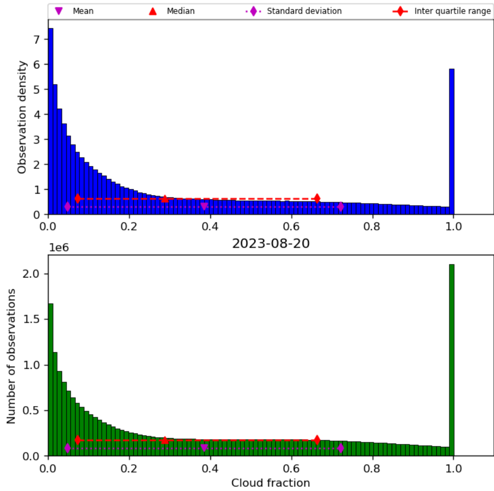
Figure 32: Histogram of “Cloud fraction” for 2023-08-20 to 2023-08-21
