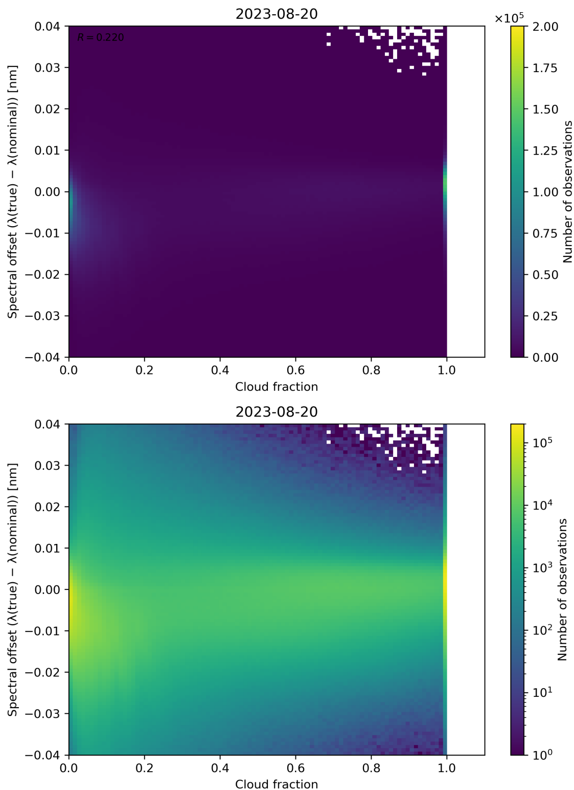
Figure 83: Scatter density plot of “Cloud fraction” against “Spectral offset ( \lambda(\text{true}) - \lambda(\text{nominal}) )” for 2023-08-20 to 2023-08-21.
