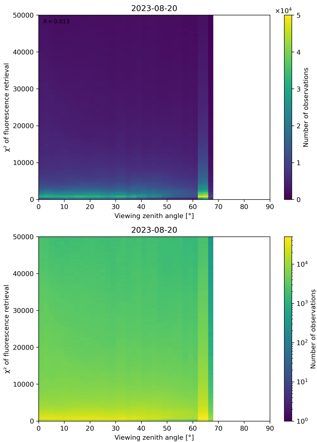
Figure 131: Scatter density plot of “Viewing zenith angle” against “ \chi^2 of fluorescence retrieval” for 2023-08-20 to 2023-08-21.
