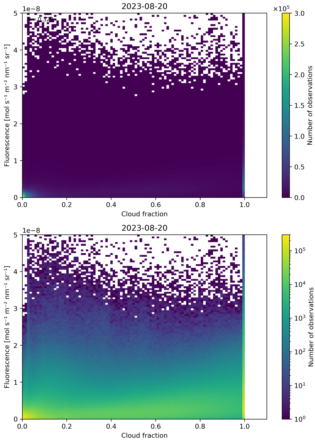
Figure 79: Scatter density plot of “Cloud fraction” against “Fluorescence” for 2023-08-20 to 2023-08-21.
