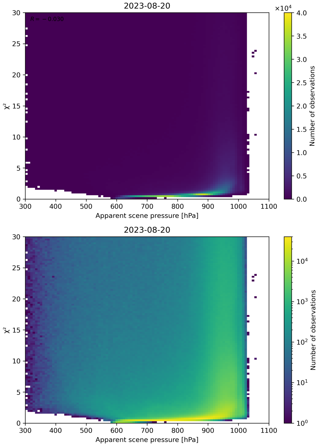
Figure 63: Scatter density plot of “Apparent scene pressure” against “ \chi^2 ” for 2023-08-20 to 2023-08-21.
