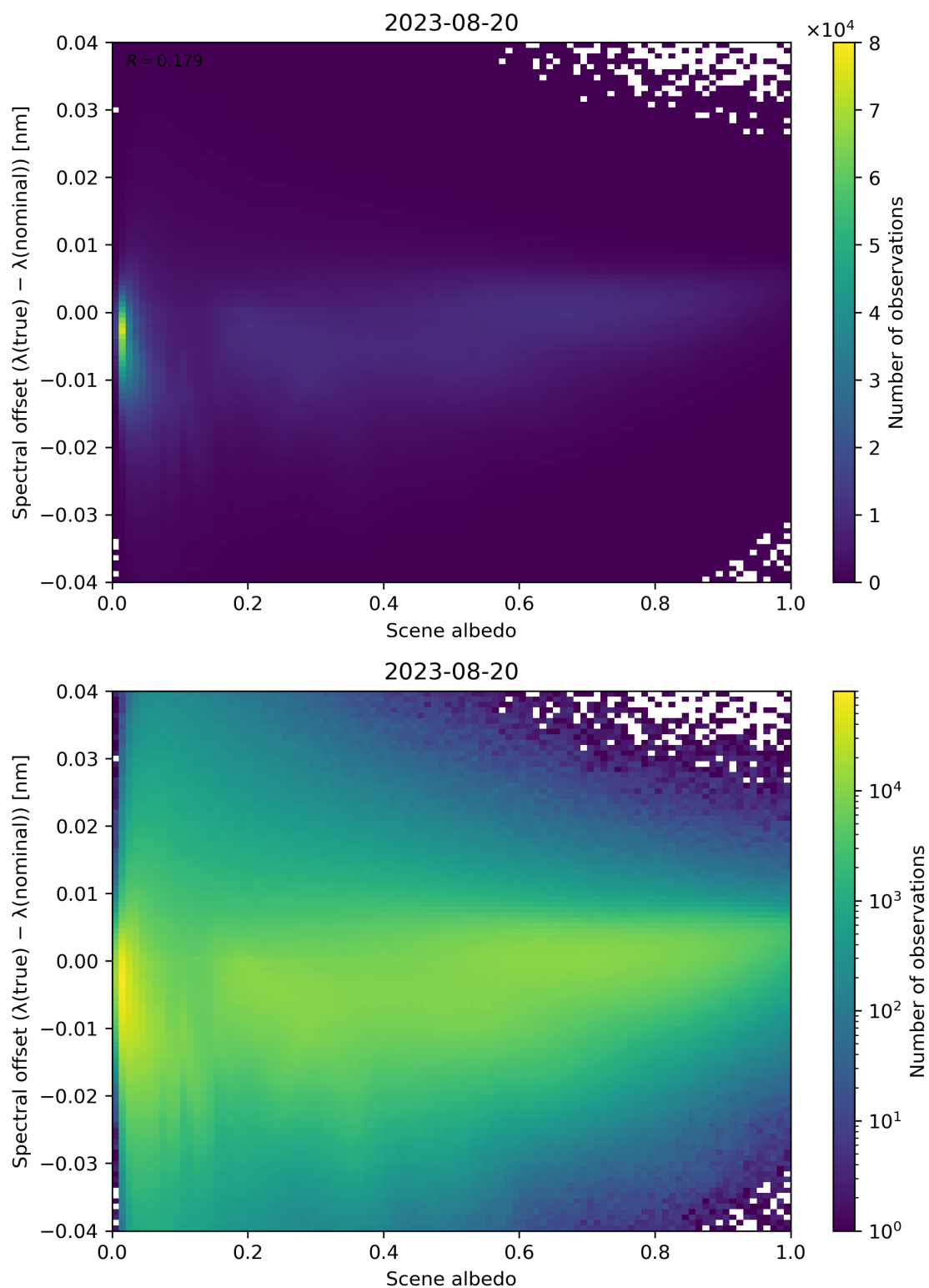
Figure 117: Scatter density plot of “Scene albedo” against “Spectral offset ( \lambda(\text{true}) - \lambda(\text{nominal}) )” for 2023-08-20 to 2023-08-21.
