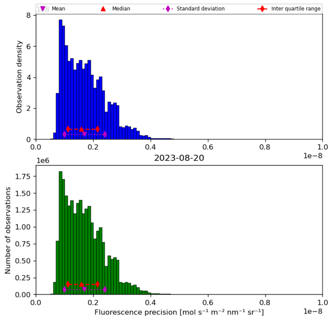
Figure 41: Histogram of “Fluorescence precision” for 2023-08-20 to 2023-08-21
