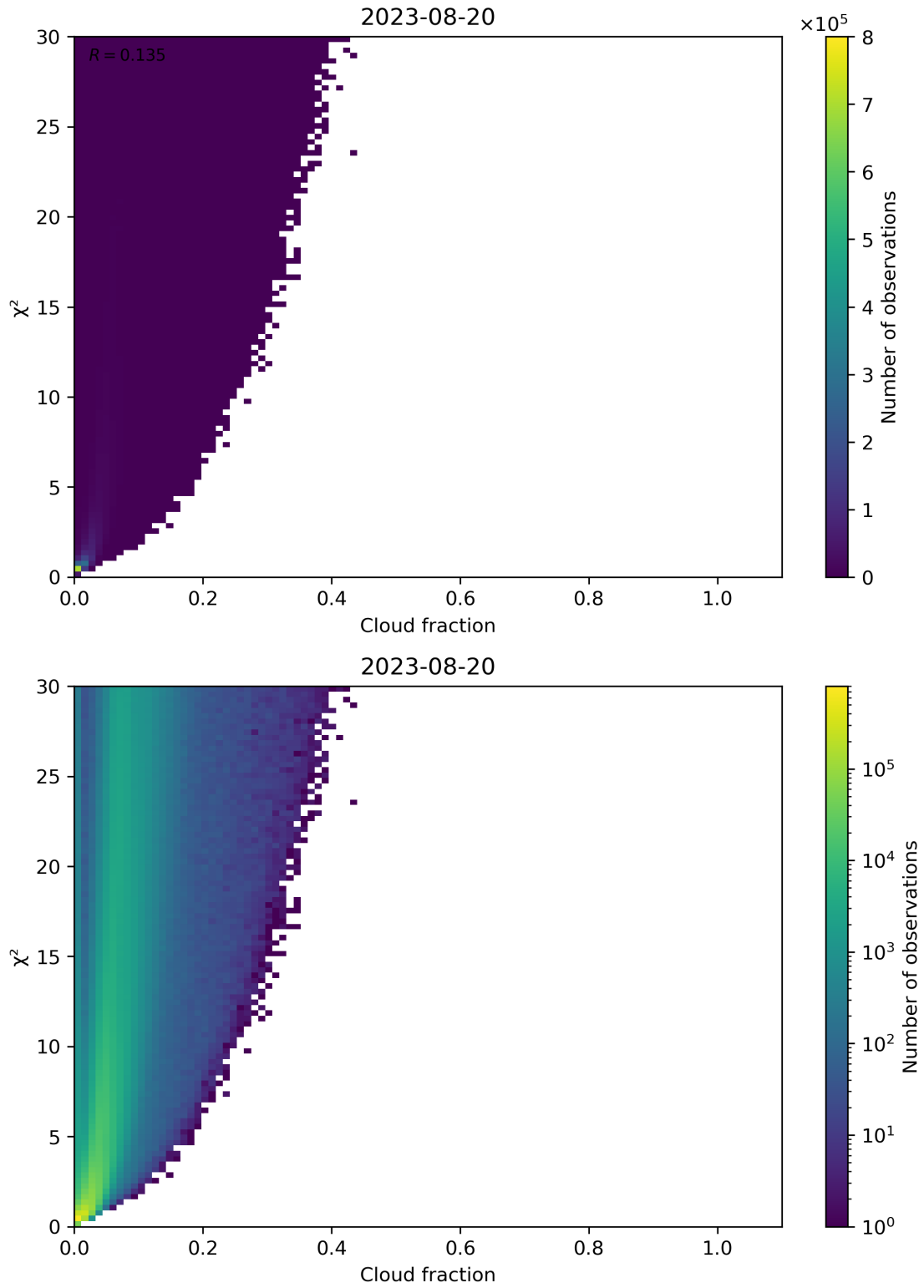
Figure 77: Scatter density plot of “Cloud fraction” against “ \chi^2 ” for 2023-08-20 to 2023-08-21.
