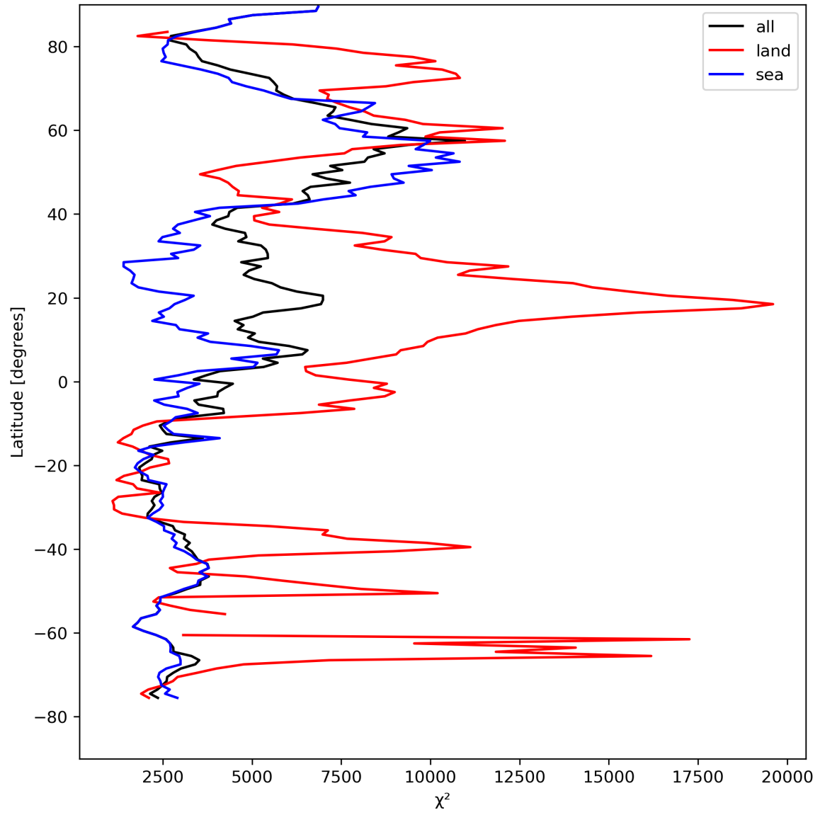
Figure 21: Zonal average of “ \chi^2 ” for 2023-08-20 to 2023-08-21.
