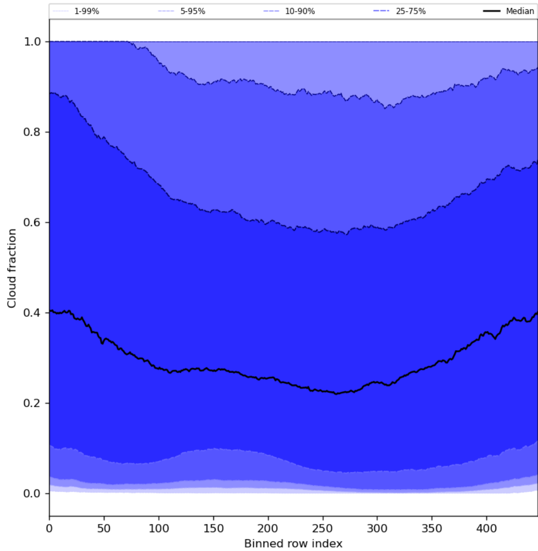
Figure 49: Along track statistics of “Cloud fraction” for 2023-08-20 to 2023-08-21
