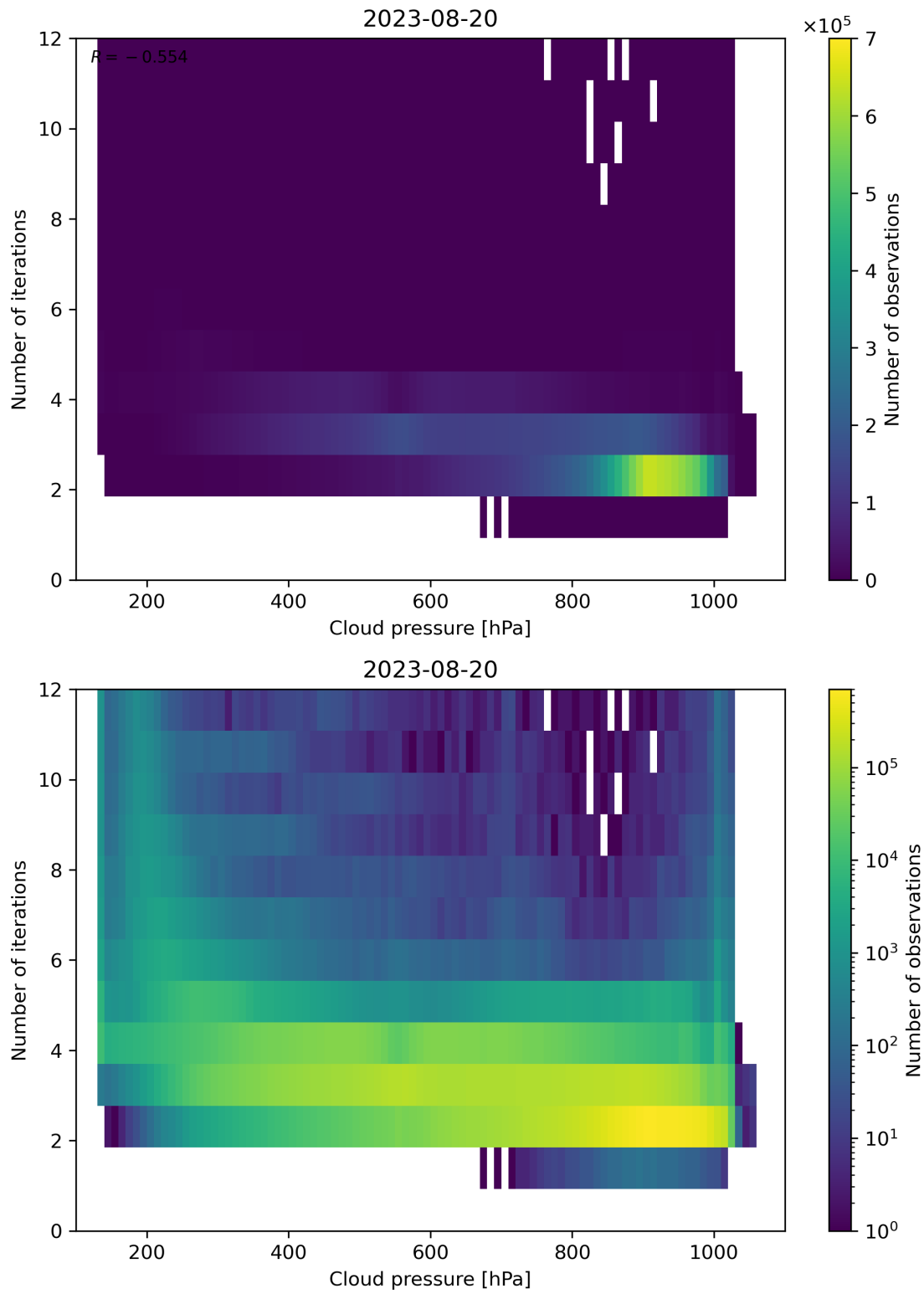
Figure 89: Scatter density plot of “Cloud pressure” against “Number of iterations” for 2023-08-20 to 2023-08-21.
