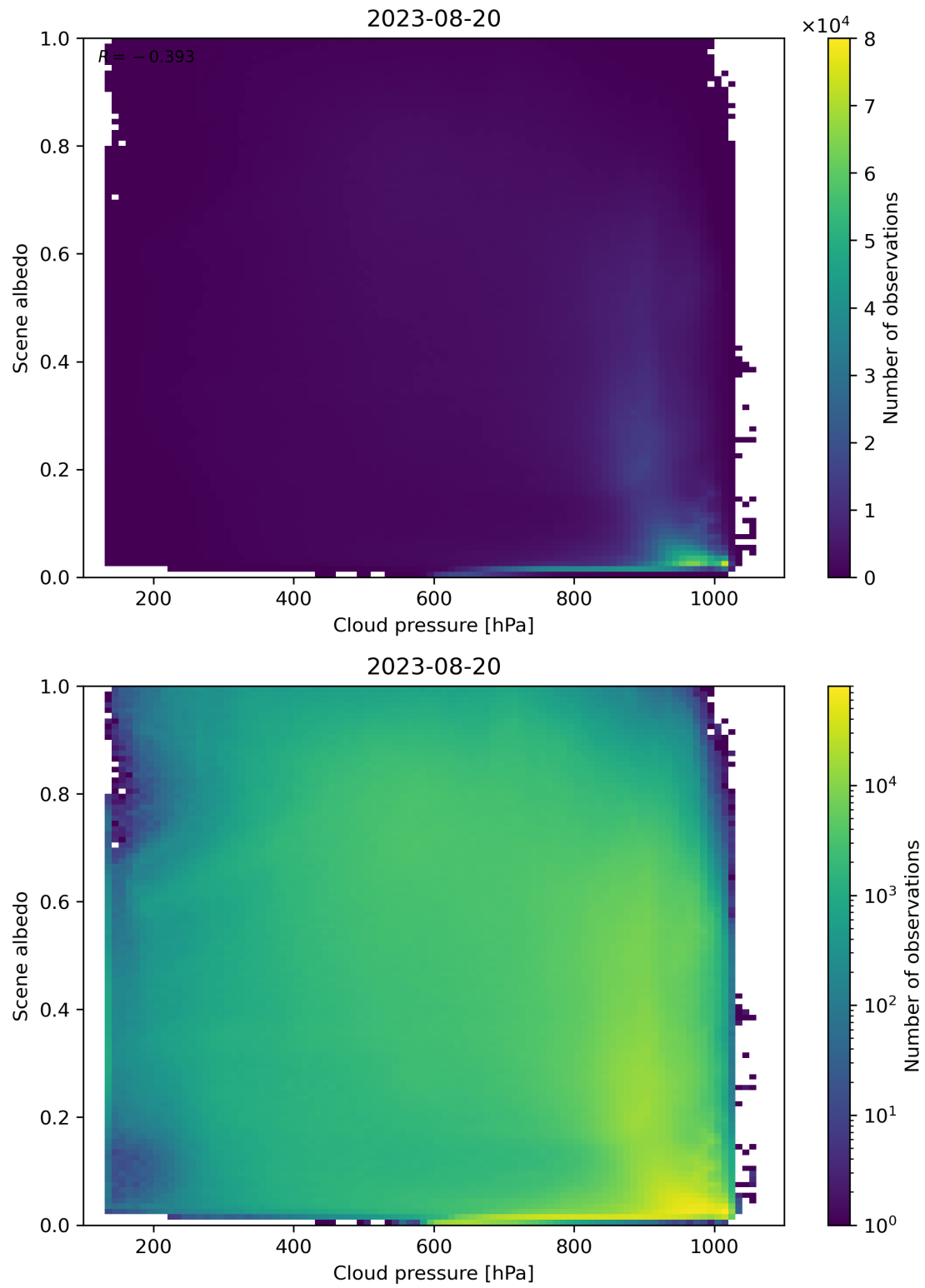
Figure 91: Scatter density plot of “Cloud pressure” against “Scene albedo” for 2023-08-20 to 2023-08-21.
