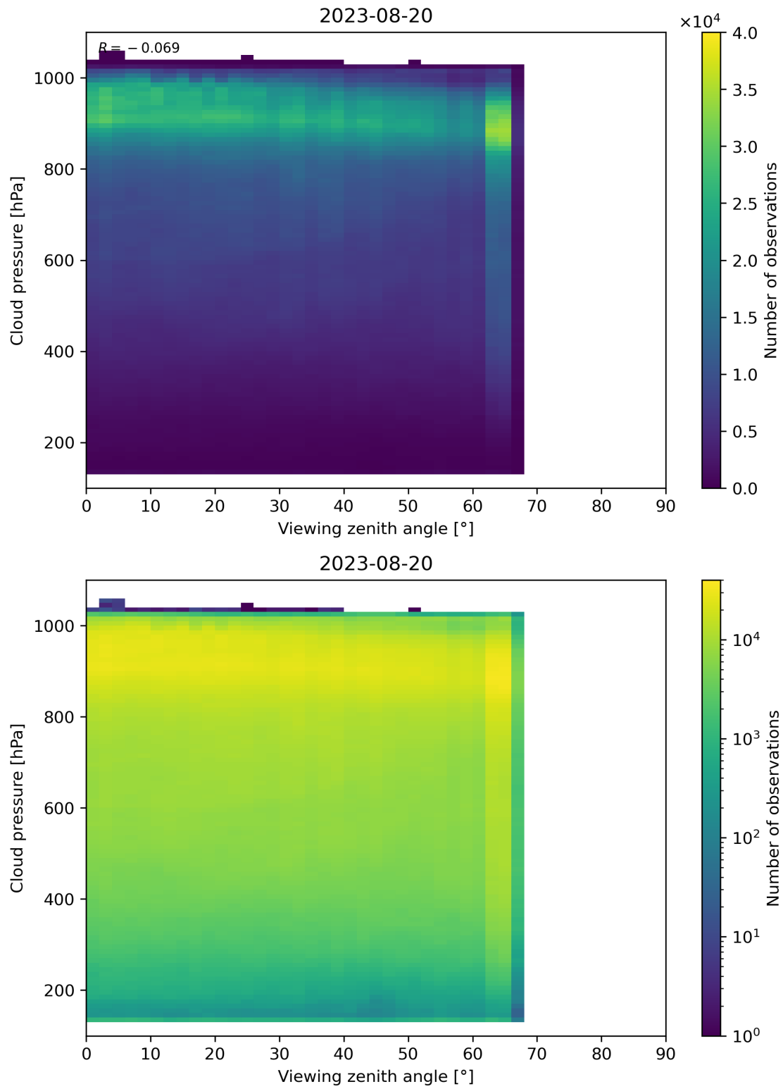
Figure 133: Scatter density plot of “Viewing zenith angle” against “Cloud pressure” for 2023-08-20 to 2023-08-21.
