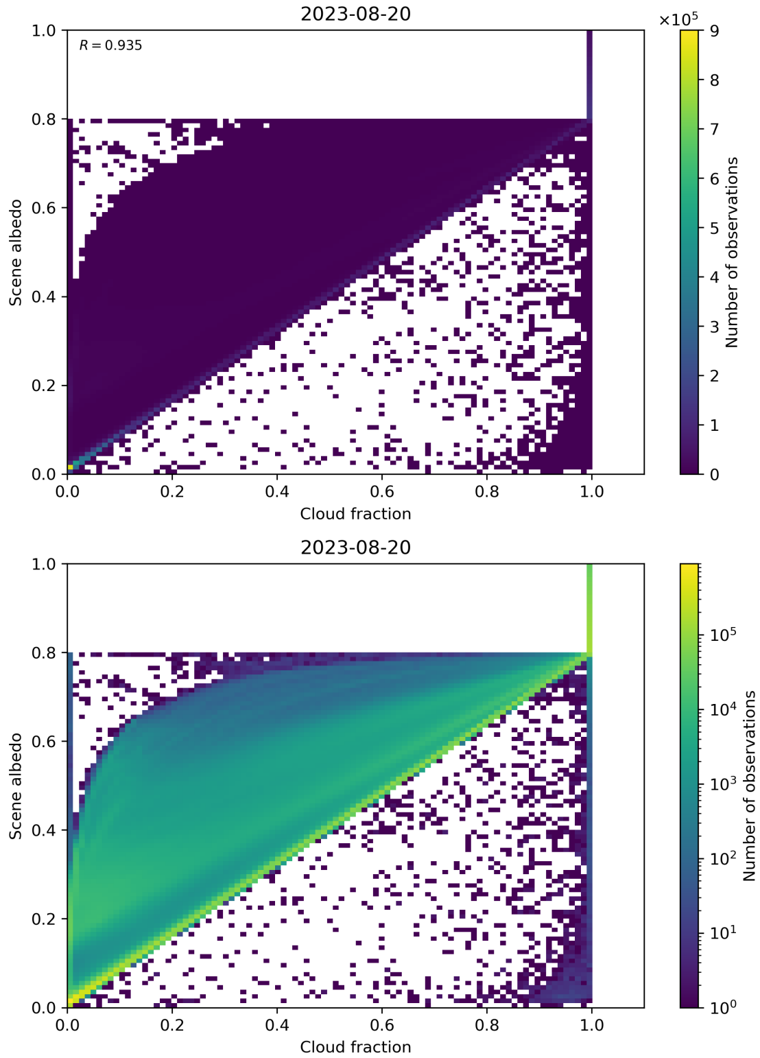
Figure 82: Scatter density plot of “Cloud fraction” against “Scene albedo” for 2023-08-20 to 2023-08-21.
