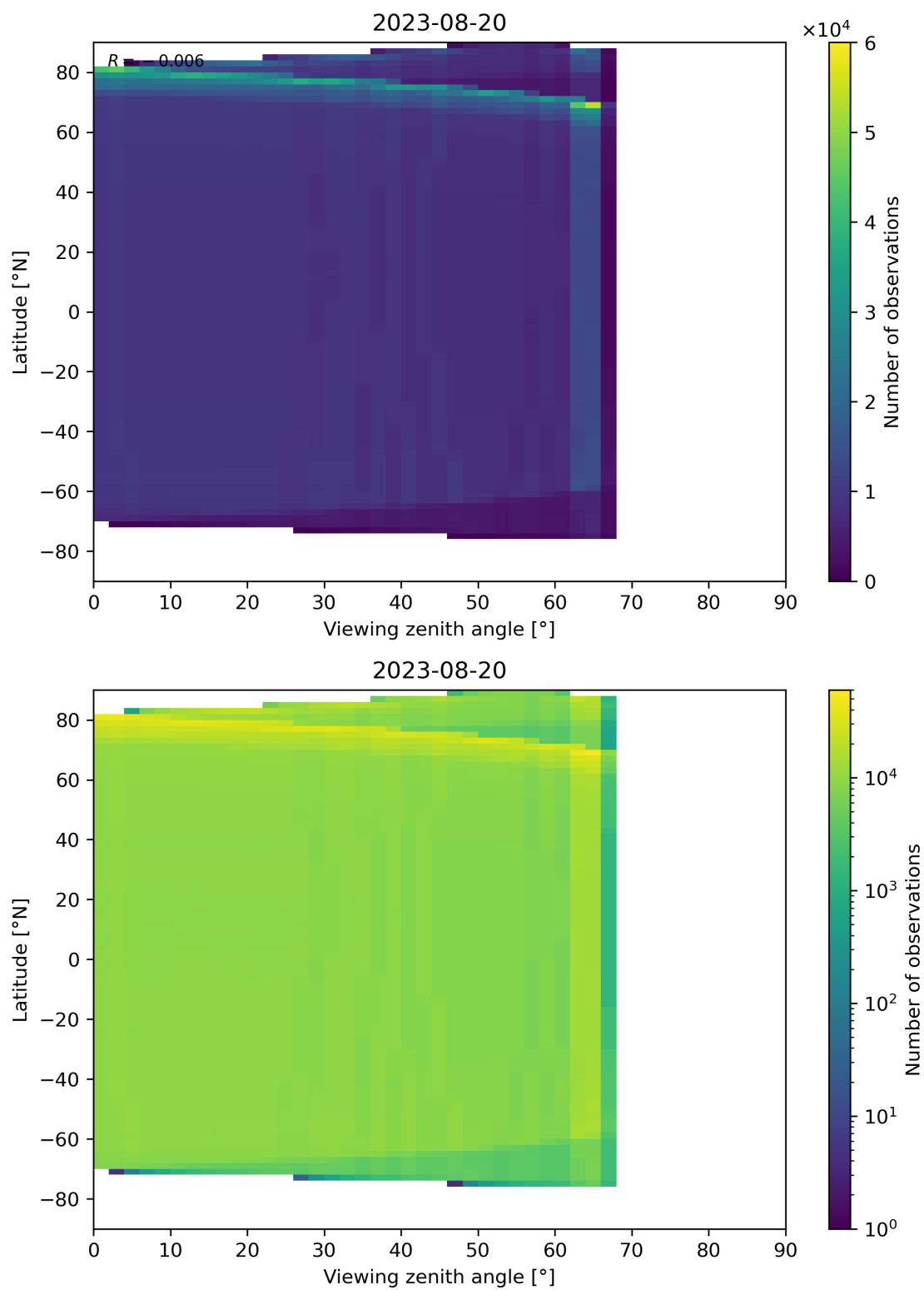
Figure 135: Scatter density plot of “Viewing zenith angle” against “Latitude” for 2023-08-20 to 2023-08-21.
