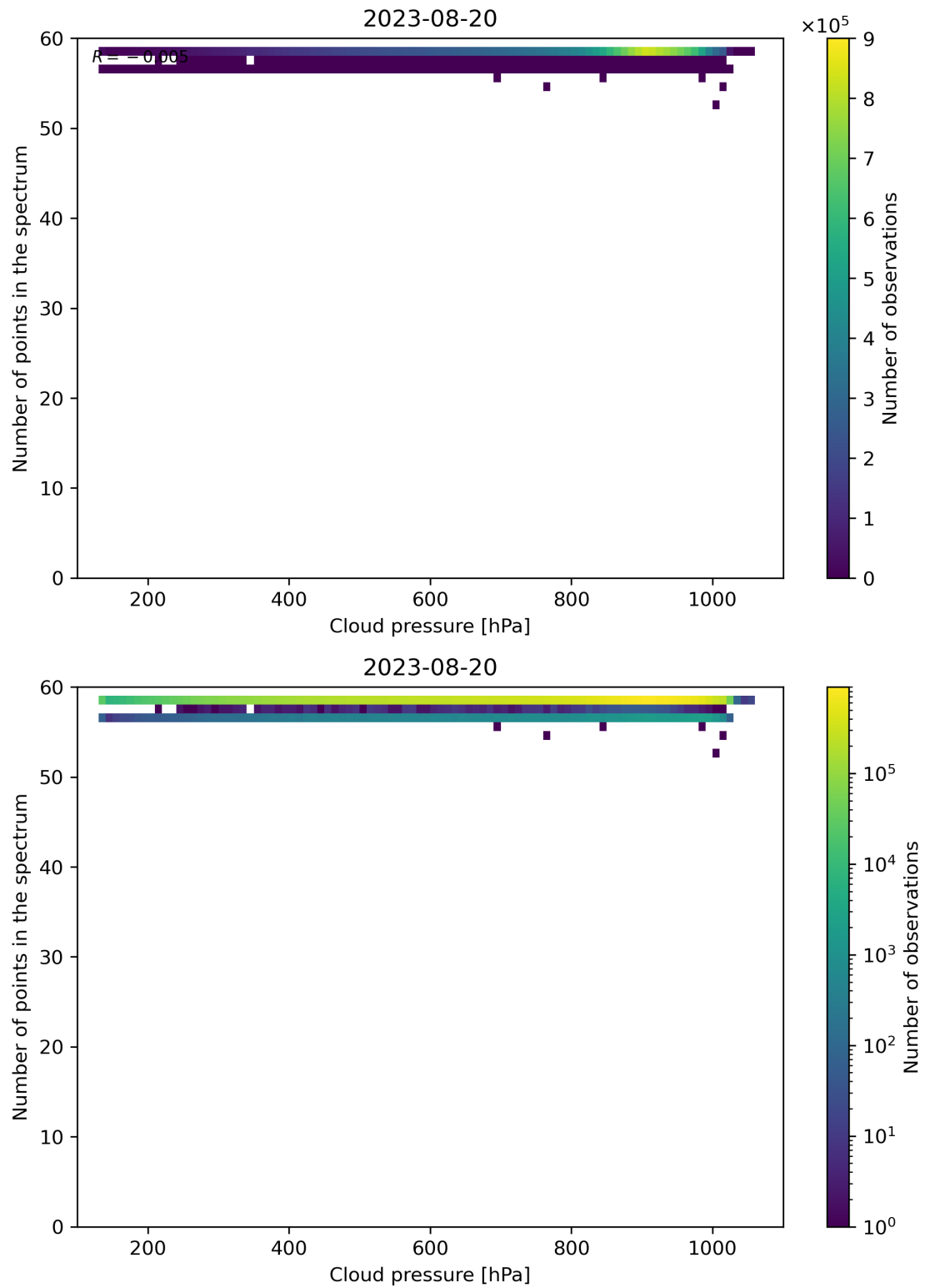
Figure 90: Scatter density plot of “Cloud pressure” against “Number of points in the spectrum” for 2023-08-20 to 2023-08-21.
