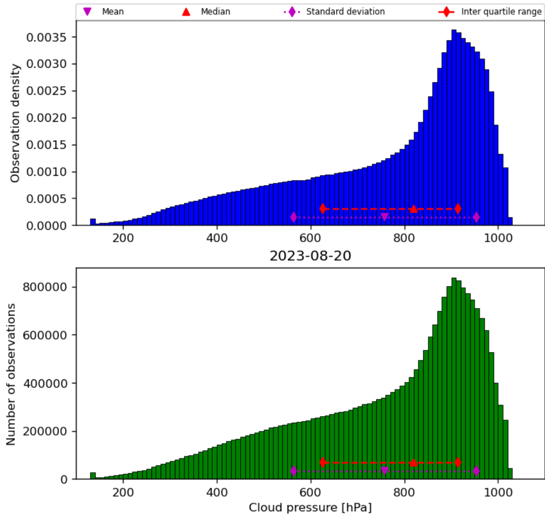
Figure 30: Histogram of “Cloud pressure” for 2023-08-20 to 2023-08-21
