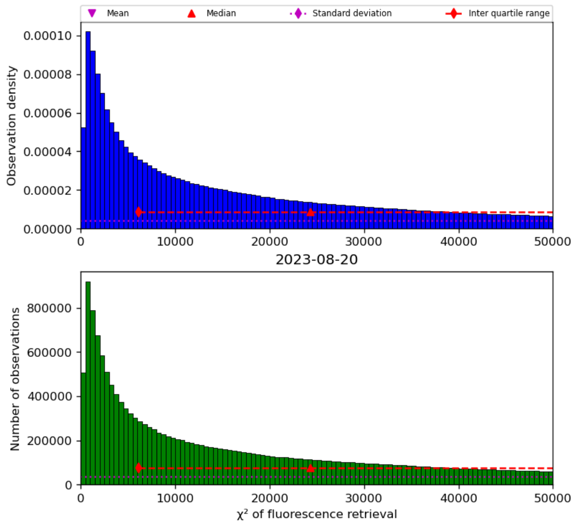
Figure 42: Histogram of “ \chi^2 of fluorescence retrieval” for 2023-08-20 to 2023-08-21
