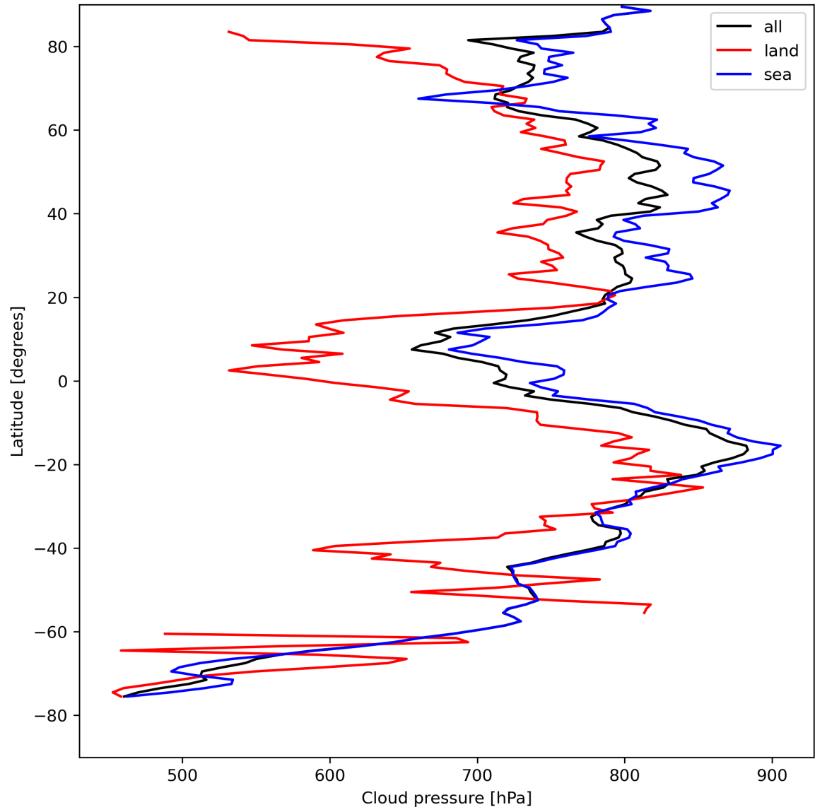
Figure 13: Zonal average of “Cloud pressure” for 2023-08-20 to 2023-08-21.
