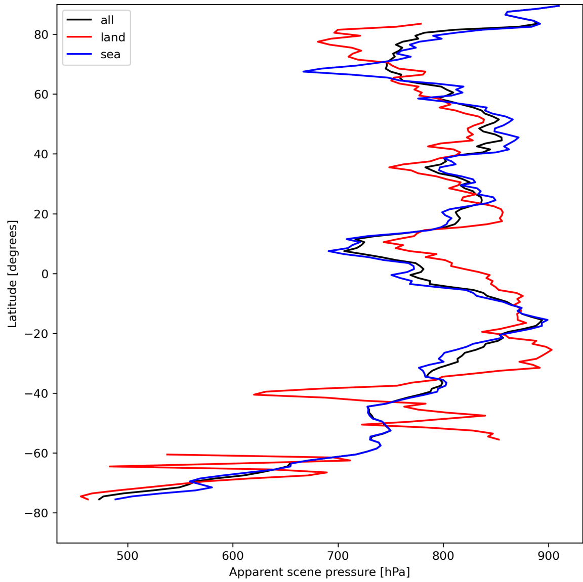
Figure 19: Zonal average of “Apparent scene pressure” for 2023-08-20 to 2023-08-21.
