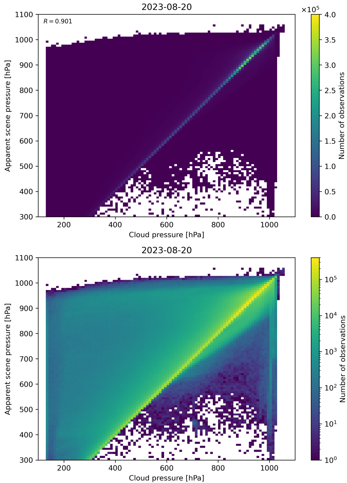
Figure 84: Scatter density plot of “Cloud pressure” against “Apparent scene pressure” for 2023-08-20 to 2023-08-21.
