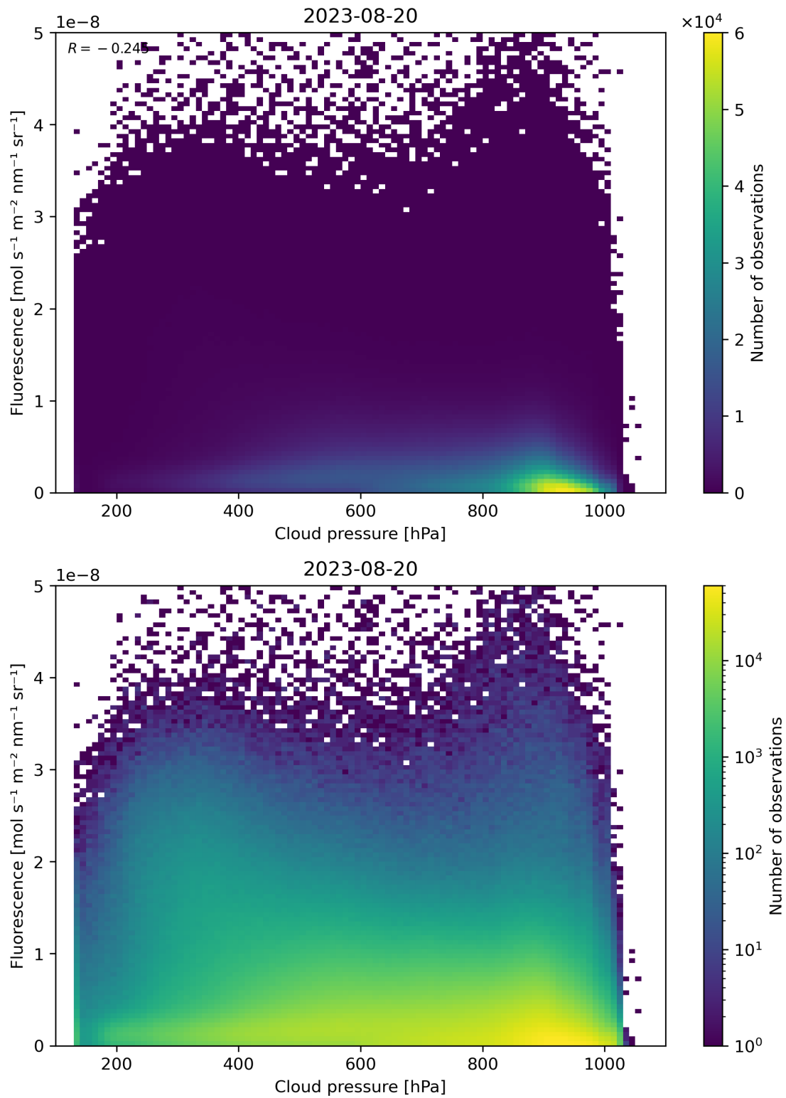
Figure 88: Scatter density plot of “Cloud pressure” against “Fluorescence” for 2023-08-20 to 2023-08-21.
