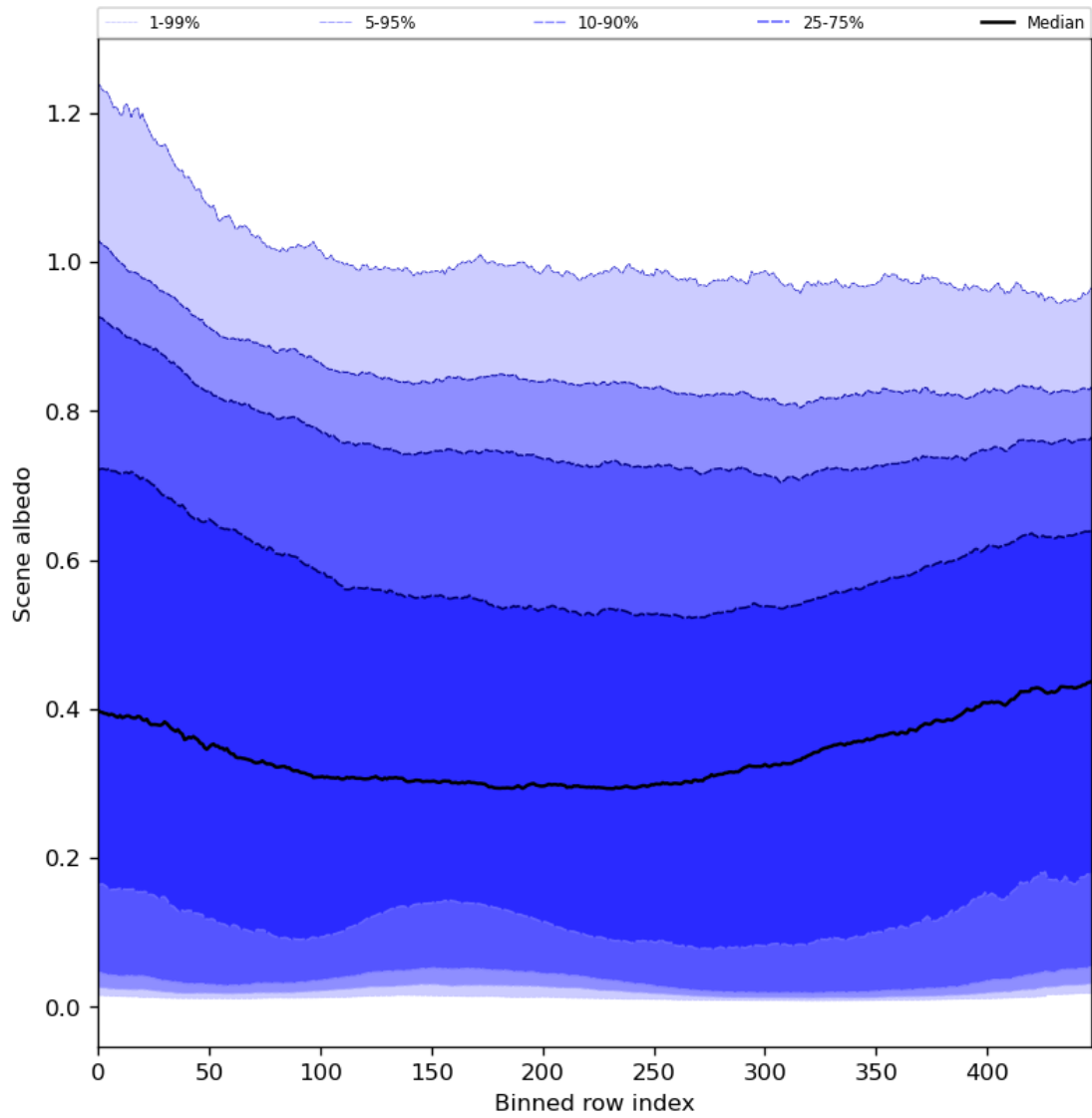
Figure 51: Along track statistics of “Scene albedo” for 2023-08-20 to 2023-08-21
