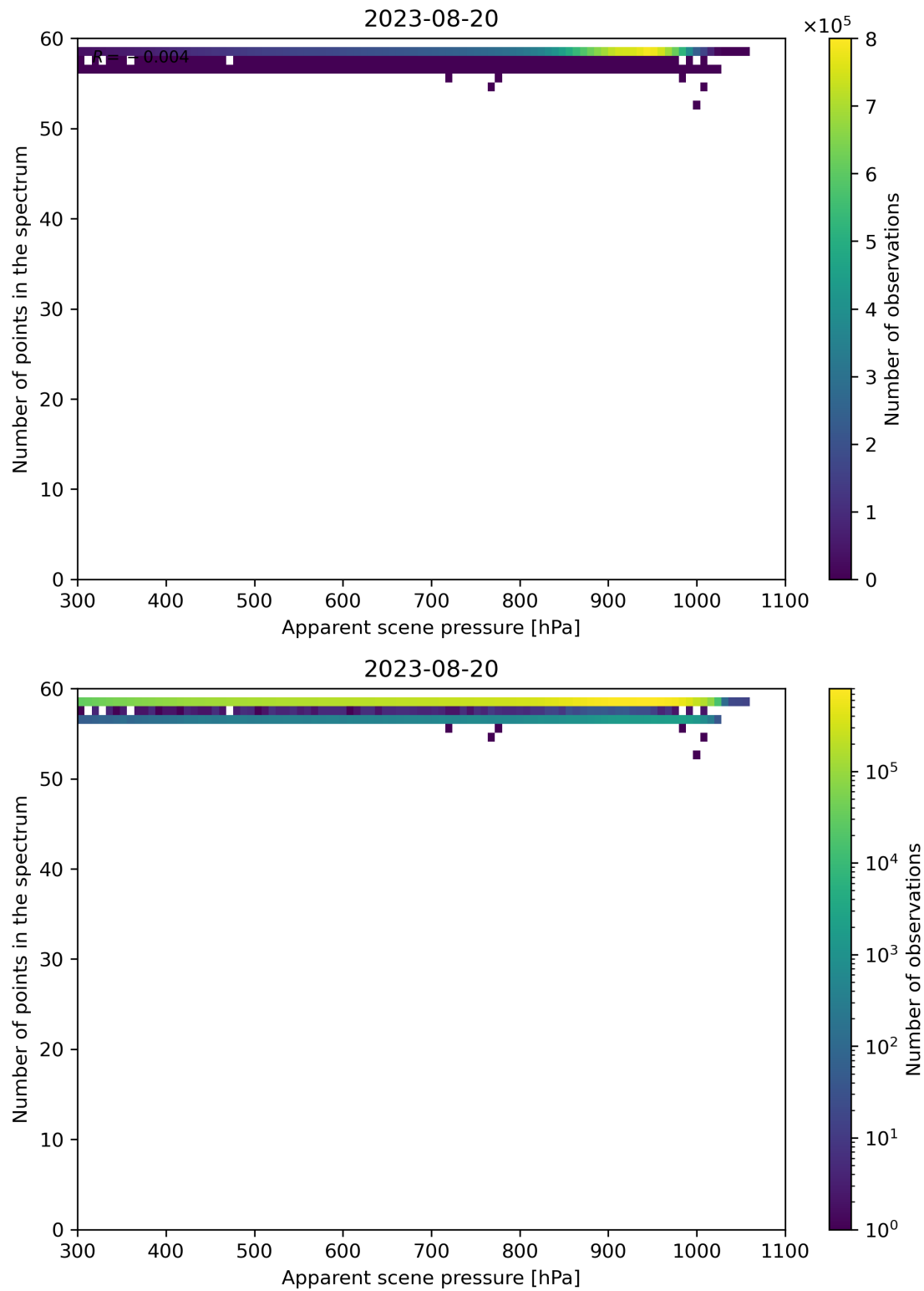
Figure 67: Scatter density plot of “Apparent scene pressure” against “Number of points in the spectrum” for 2023-08-20 to 2023-08-21.
