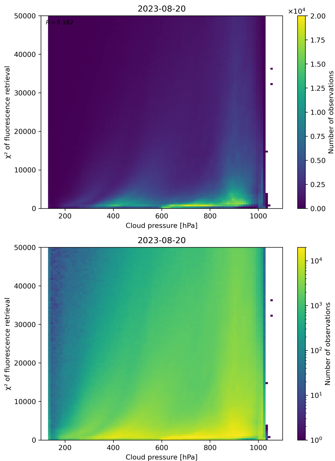
Figure 86: Scatter density plot of “Cloud pressure” against “ \chi^2 of fluorescence retrieval” for 2023-08-20 to 2023-08-21.
