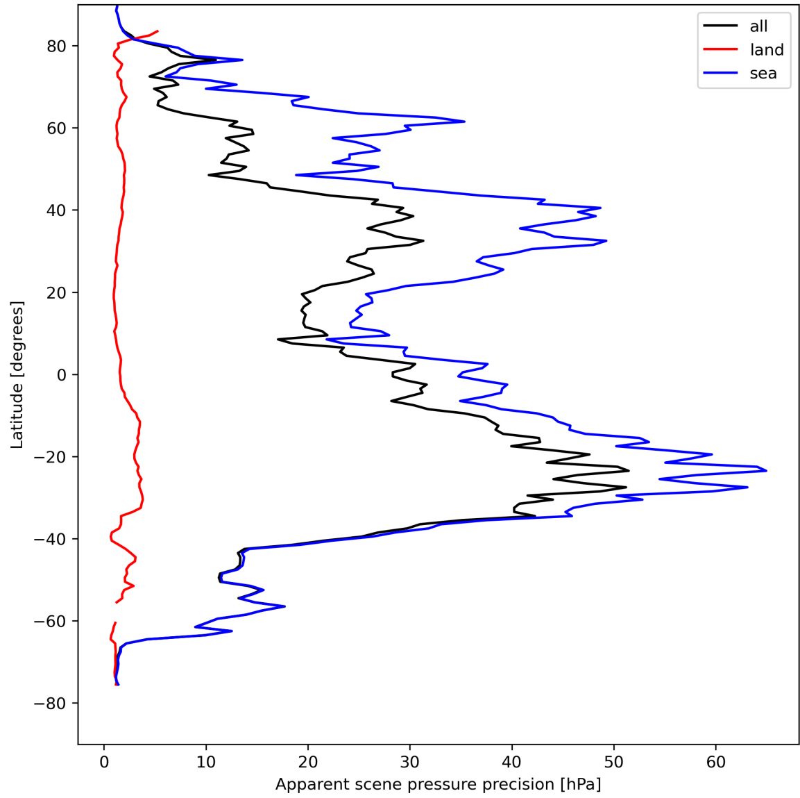
Figure 20: Zonal average of “Apparent scene pressure precision” for 2023-08-20 to 2023-08-21.
