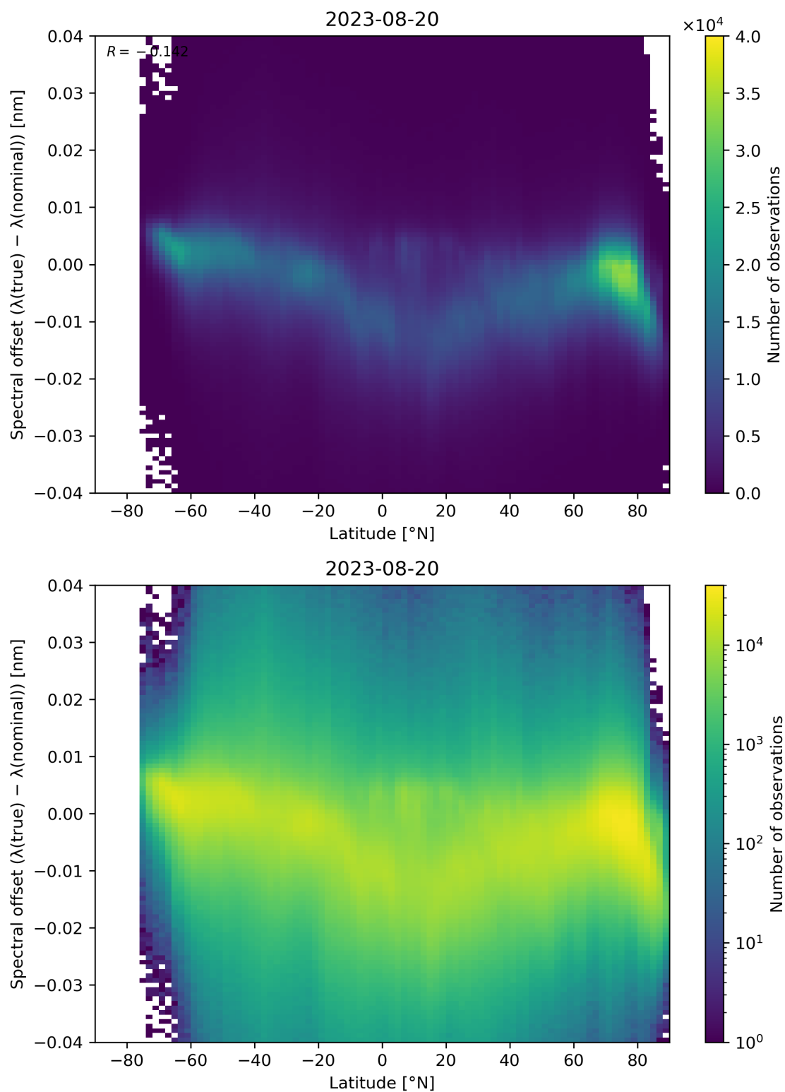
Figure 105: Scatter density plot of “Latitude” against “Spectral offset ( \lambda(\text{true}) - \lambda(\text{nominal}) )” for 2023-08-20 to 2023-08-21.
