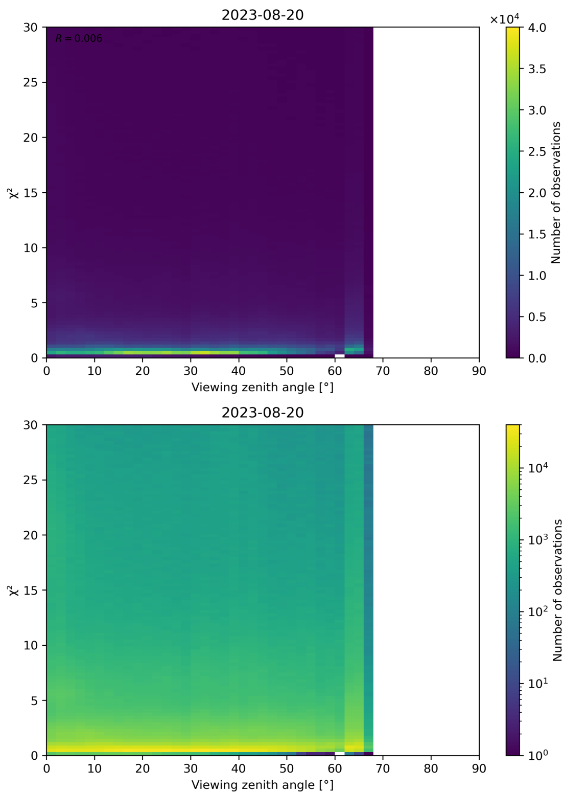
Figure 130: Scatter density plot of “Viewing zenith angle” against “ \chi^2 ” for 2023-08-20 to 2023-08-21.
