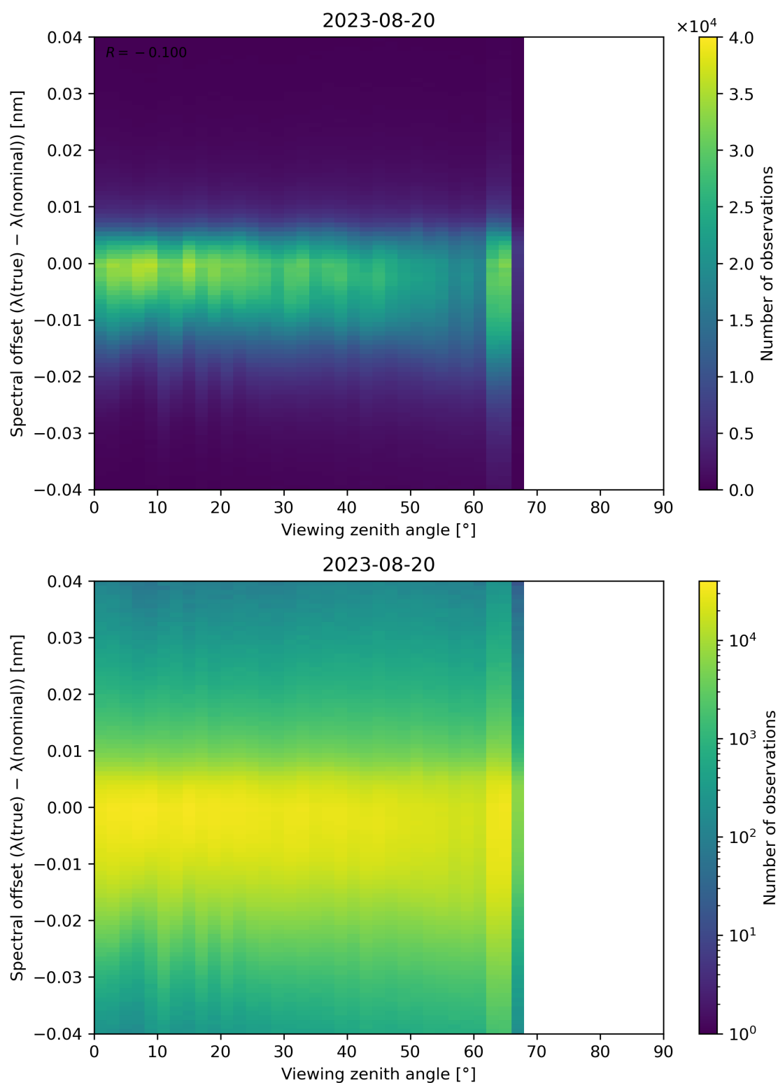
Figure 140: Scatter density plot of “Viewing zenith angle” against “Spectral offset ( \lambda(\text{true}) - \lambda(\text{nominal}) )” for 2023-08-20 to 2023-08-21.
