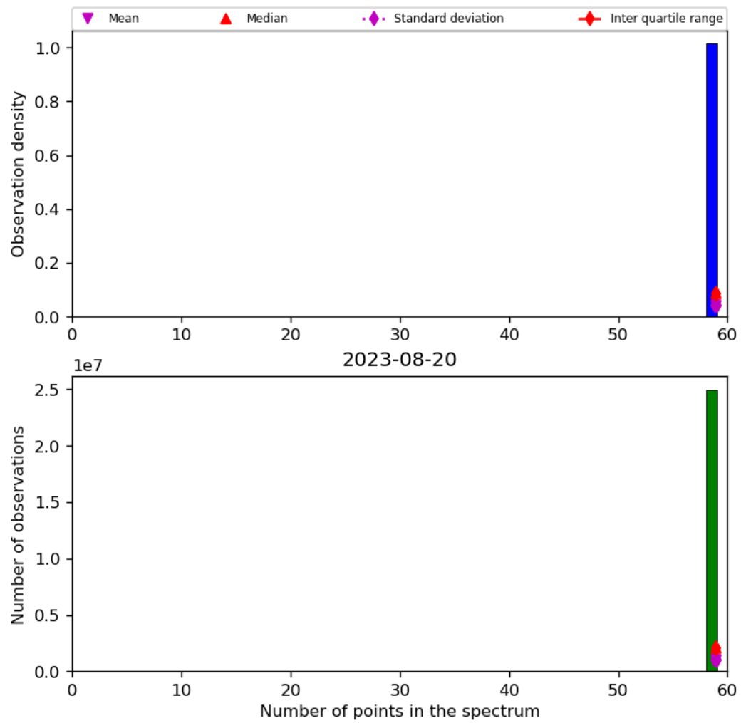
Figure 44: Histogram of “Number of points in the spectrum” for 2023-08-20 to 2023-08-21
