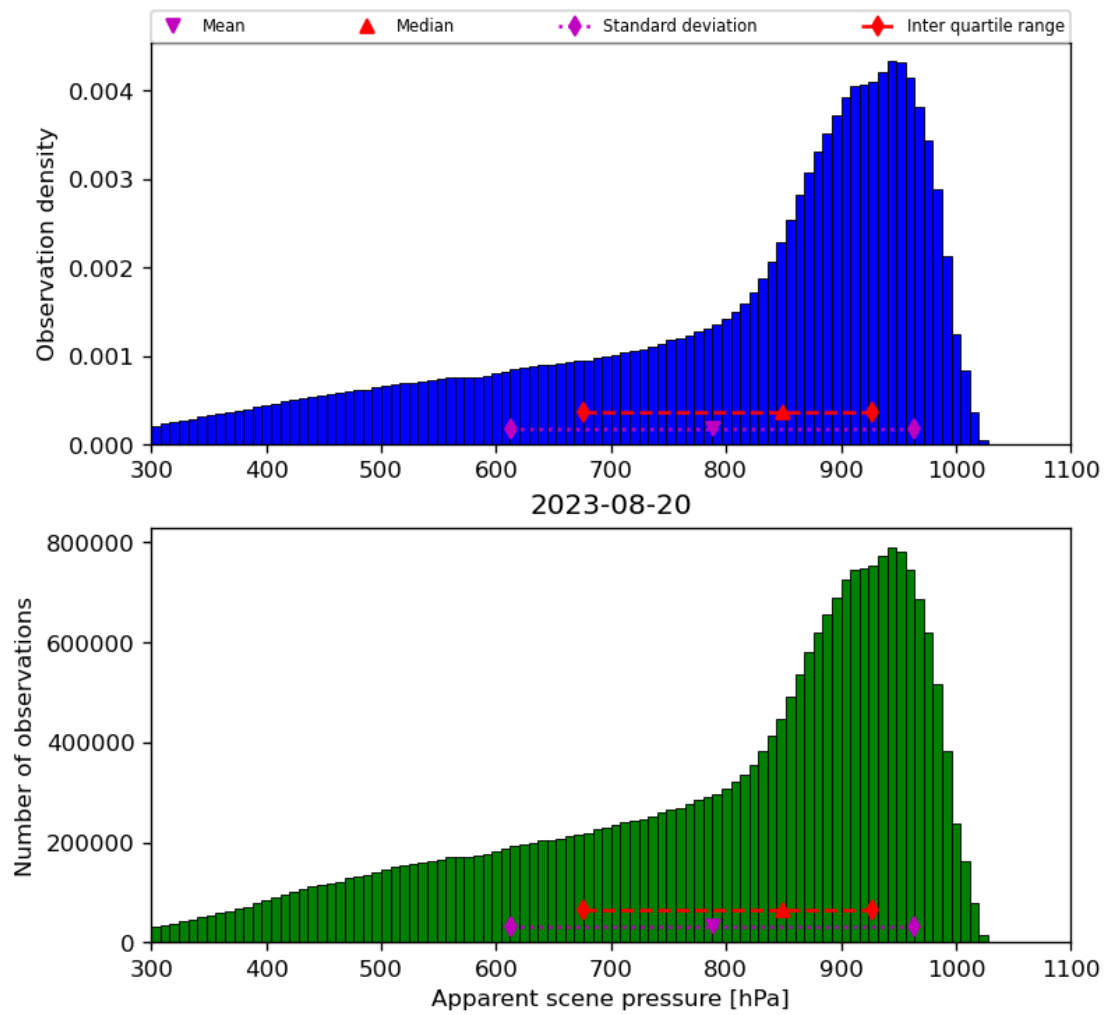
Figure 36: Histogram of “Apparent scene pressure” for 2023-08-20 to 2023-08-21
