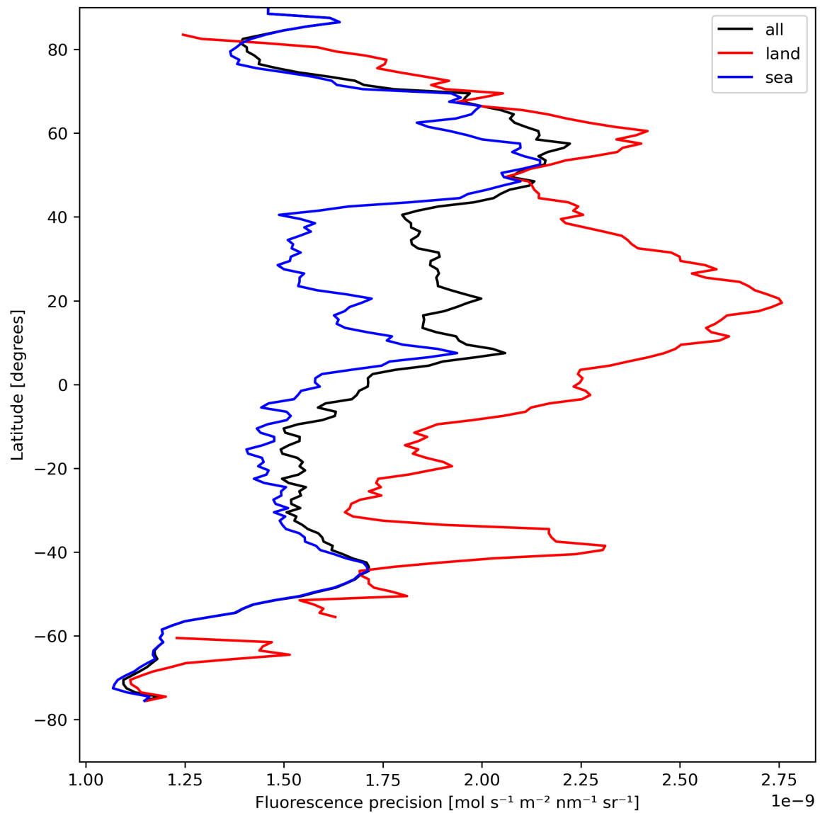
Figure 24: Zonal average of “Fluorescence precision” for 2023-08-20 to 2023-08-21.
