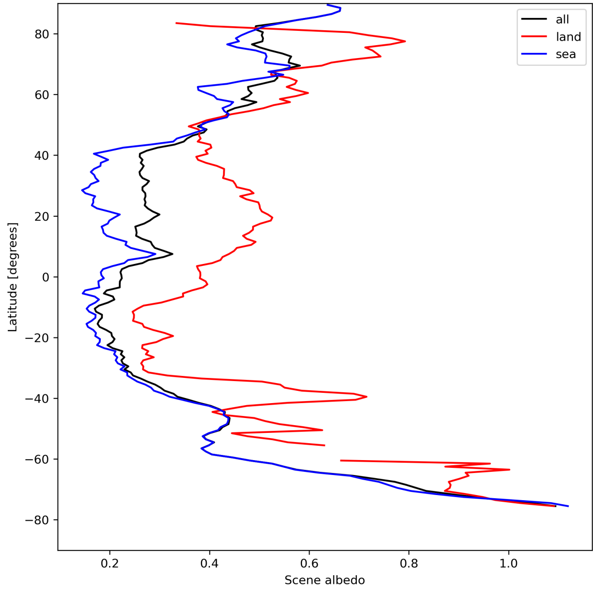
Figure 17: Zonal average of “Scene albedo” for 2023-08-20 to 2023-08-21.
