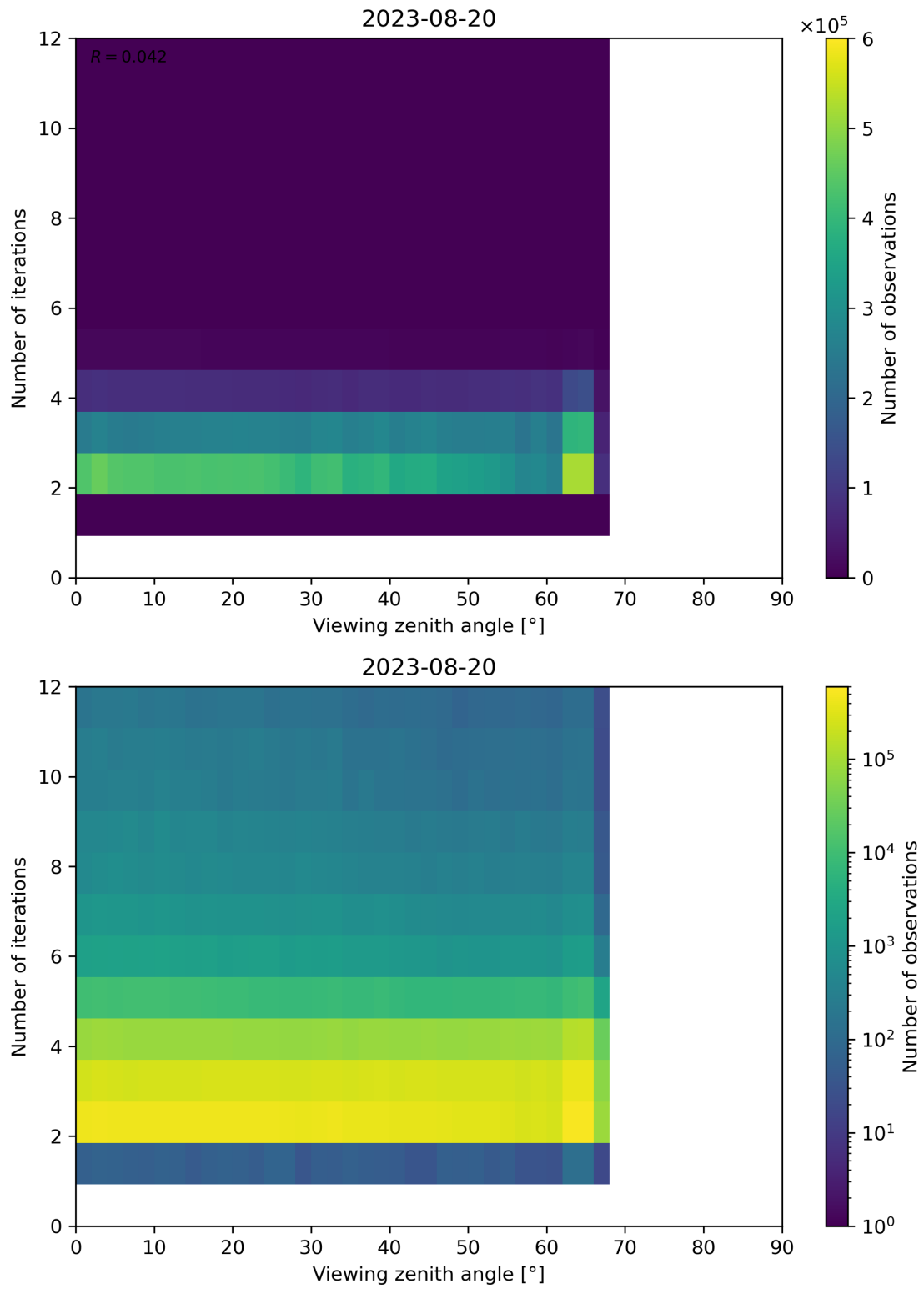
Figure 136: Scatter density plot of “Viewing zenith angle” against “Number of iterations” for 2023-08-20 to 2023-08-21.
