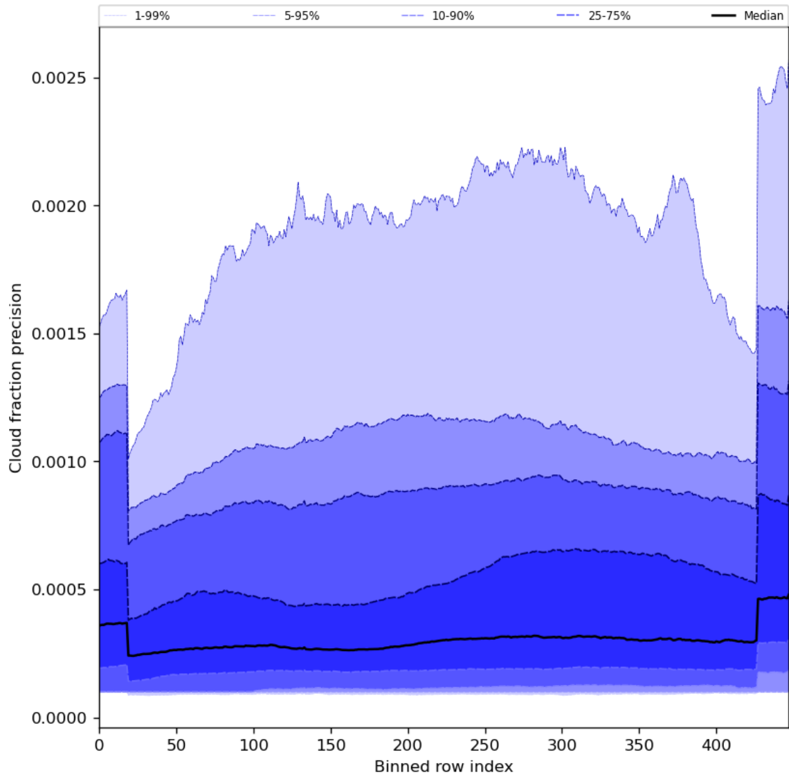
Figure 50: Along track statistics of “Cloud fraction precision” for 2023-08-20 to 2023-08-21
