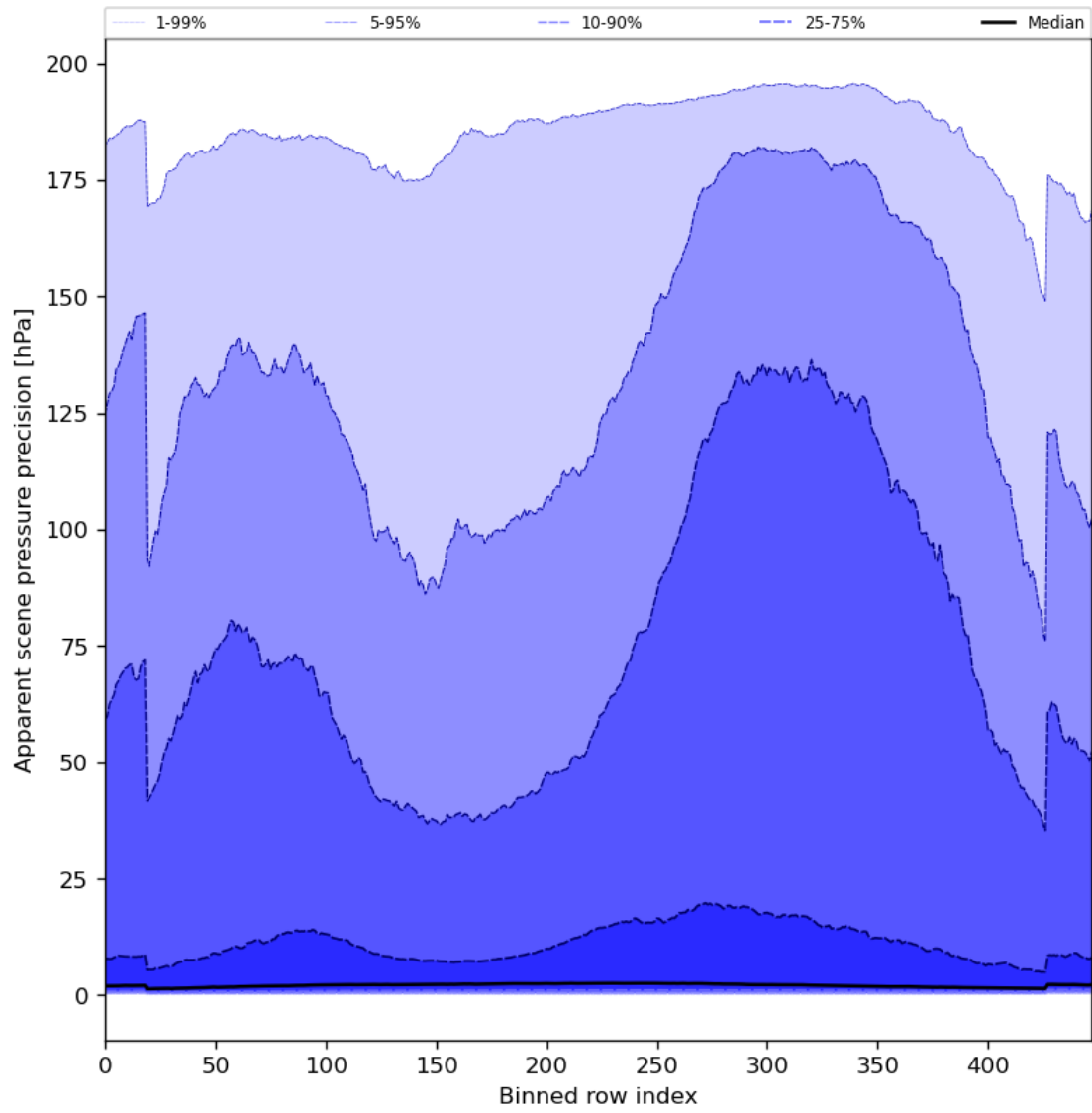
Figure 54: Along track statistics of “Apparent scene pressure precision” for 2023-08-20 to 2023-08-21
