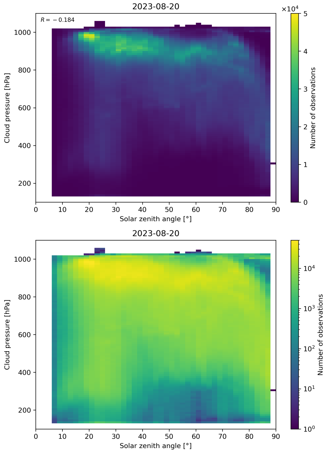
Figure 122: Scatter density plot of “Solar zenith angle” against “Cloud pressure” for 2023-08-20 to 2023-08-21.
