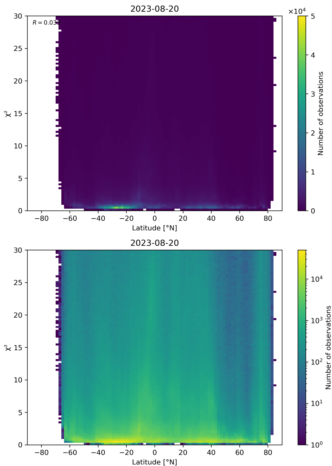
Figure 97: Scatter density plot of “Latitude” against “ \chi^2 ” for 2023-08-20 to 2023-08-21.
