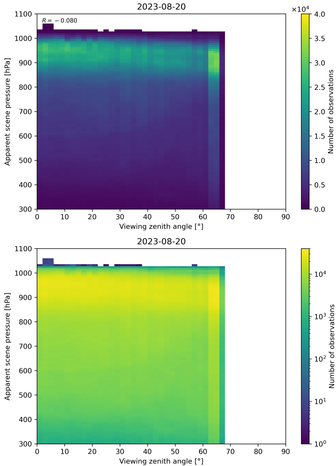
Figure 129: Scatter density plot of “Viewing zenith angle” against “Apparent scene pressure” for 2023-08-20 to 2023-08-21.
