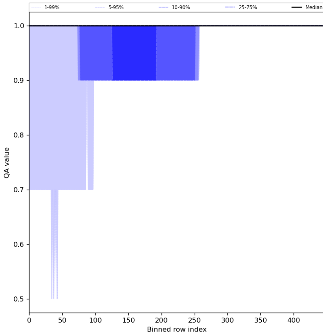
Figure 46: Along track statistics of "QA value" for 2023-08-20 to 2023-08-21
