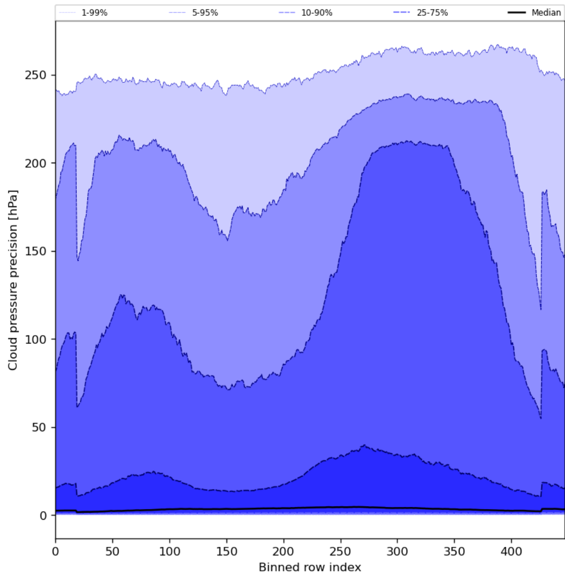
Figure 48: Along track statistics of “Cloud pressure precision” for 2023-08-20 to 2023-08-21
