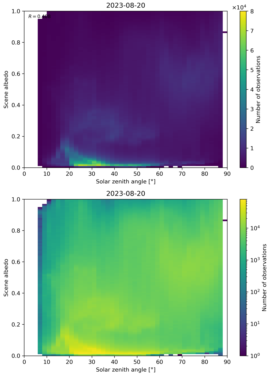
Figure 127: Scatter density plot of “Solar zenith angle” against “Scene albedo” for 2023-08-20 to 2023-08-21.
