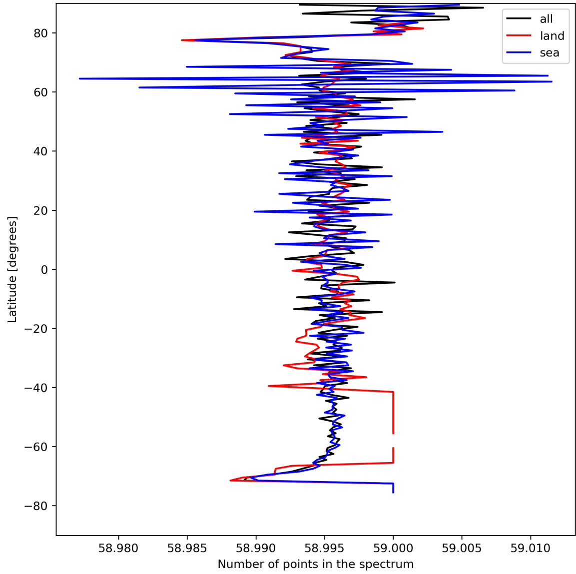
Figure 27: Zonal average of “Number of points in the spectrum” for 2023-08-20 to 2023-08-21.
