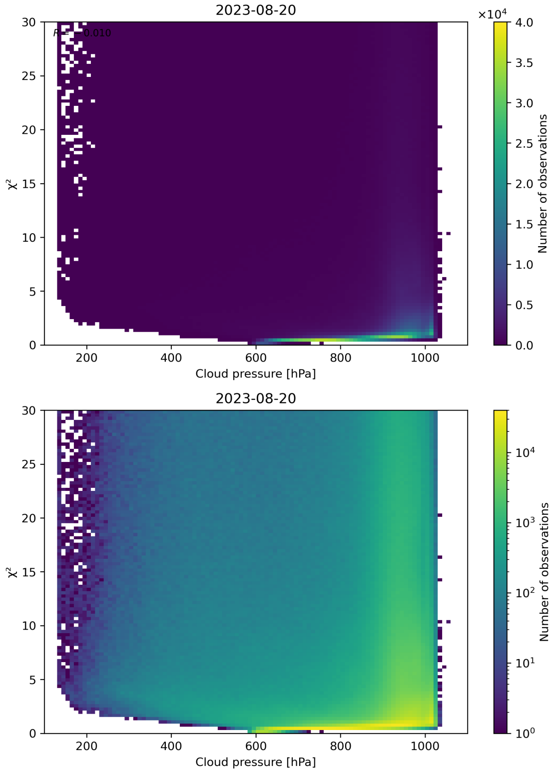
Figure 85: Scatter density plot of “Cloud pressure” against “ \chi^2 ” for 2023-08-20 to 2023-08-21.
