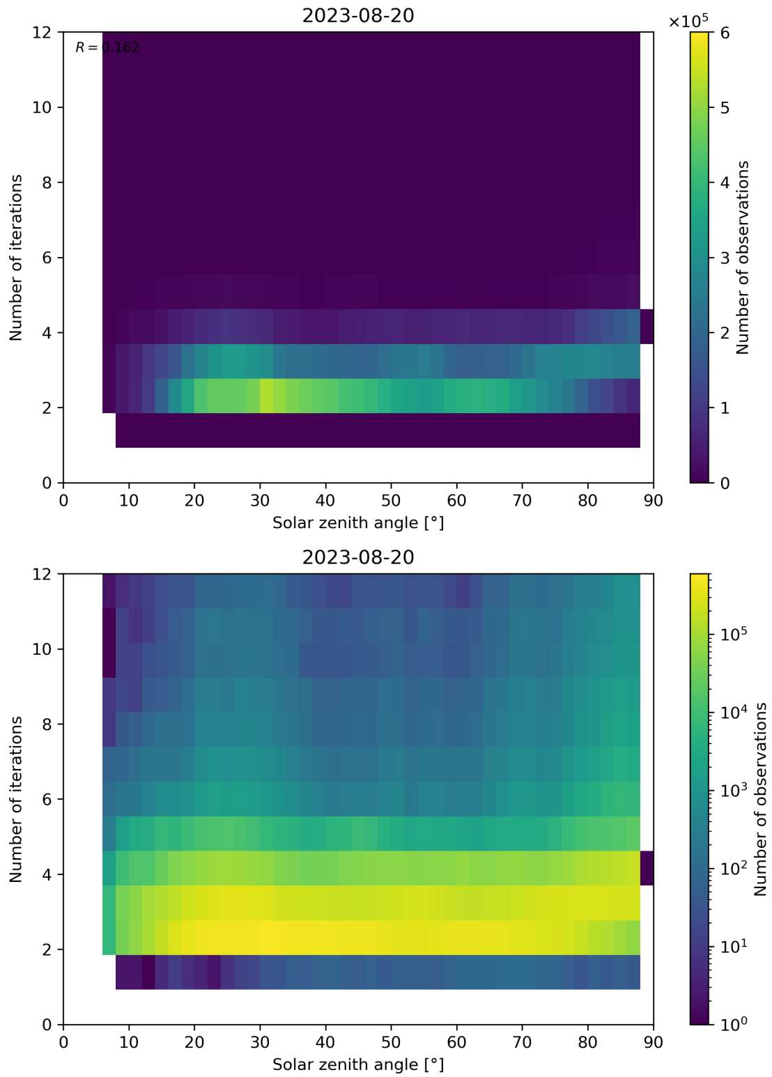
Figure 125: Scatter density plot of “Solar zenith angle” against “Number of iterations” for 2023-08-20 to 2023-08-21.
