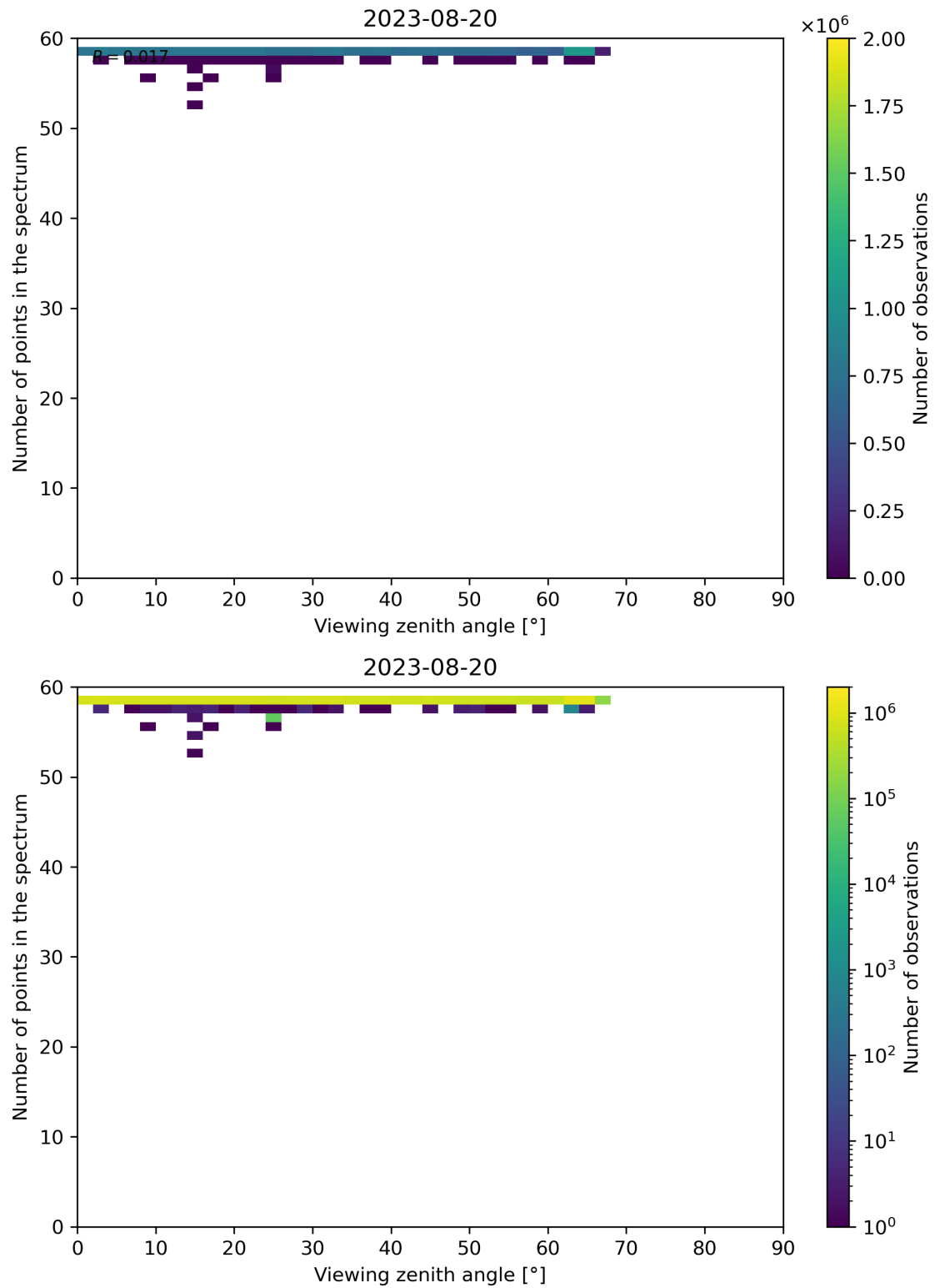
Figure 137: Scatter density plot of “Viewing zenith angle” against “Number of points in the spectrum” for 2023-08-20 to 2023-08-21.
