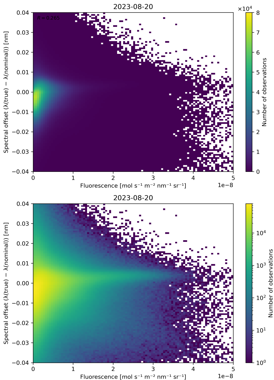
Figure 95: Scatter density plot of “Fluorescence” against “Spectral offset ( \lambda(\text{true}) - \lambda(\text{nominal}) )” for 2023-08-20 to 2023-08-21.
