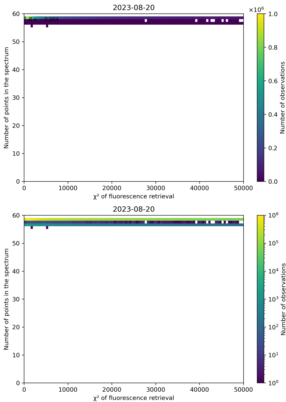
Figure 71: Scatter density plot of “ \chi^2 of fluorescence retrieval” against “Number of points in the spectrum” for 2023-08-20 to 2023-08-21.
