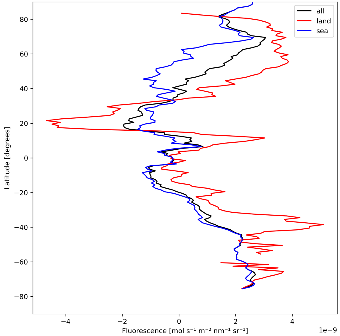
Figure 23: Zonal average of “Fluorescence” for 2023-08-20 to 2023-08-21.
