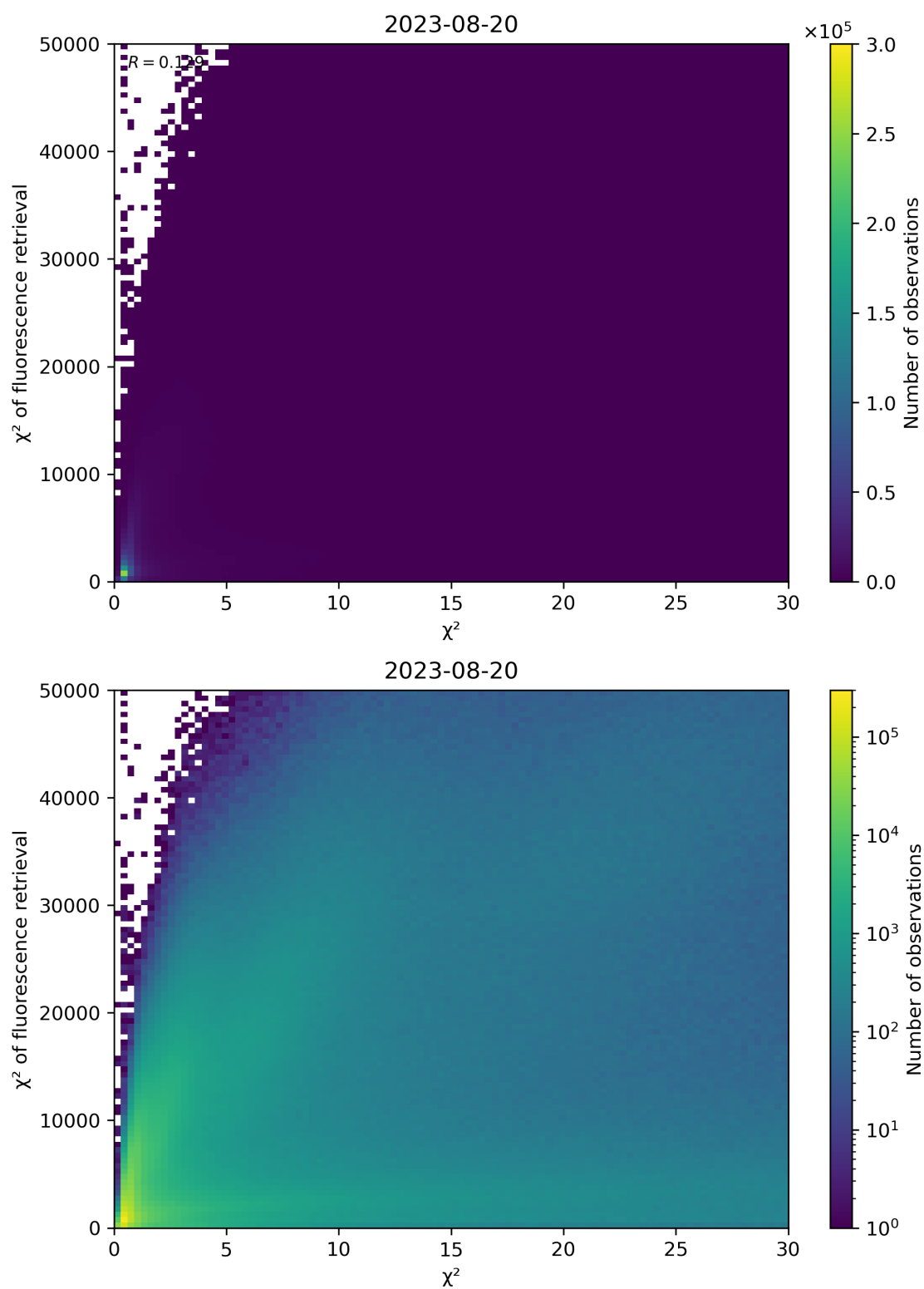
Figure 69: Scatter density plot of “ \chi^2 ” against “ \chi^2 of fluorescence retrieval” for 2023-08-20 to 2023-08-21.
