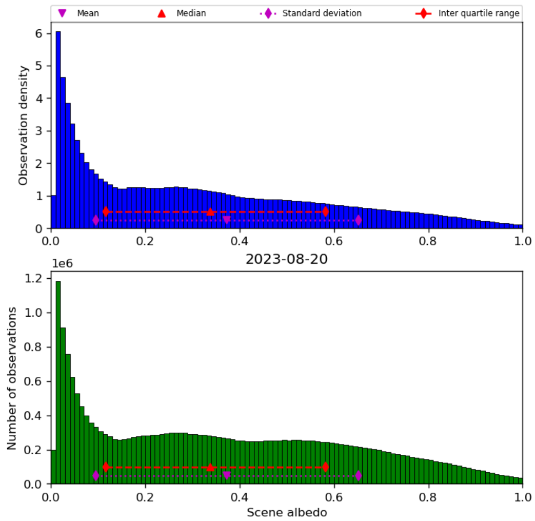
Figure 34: Histogram of “Scene albedo” for 2023-08-20 to 2023-08-21
