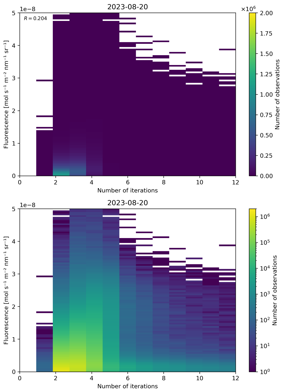
Figure 107: Scatter density plot of “Number of iterations” against “Fluorescence” for 2023-08-20 to 2023-08-21.
