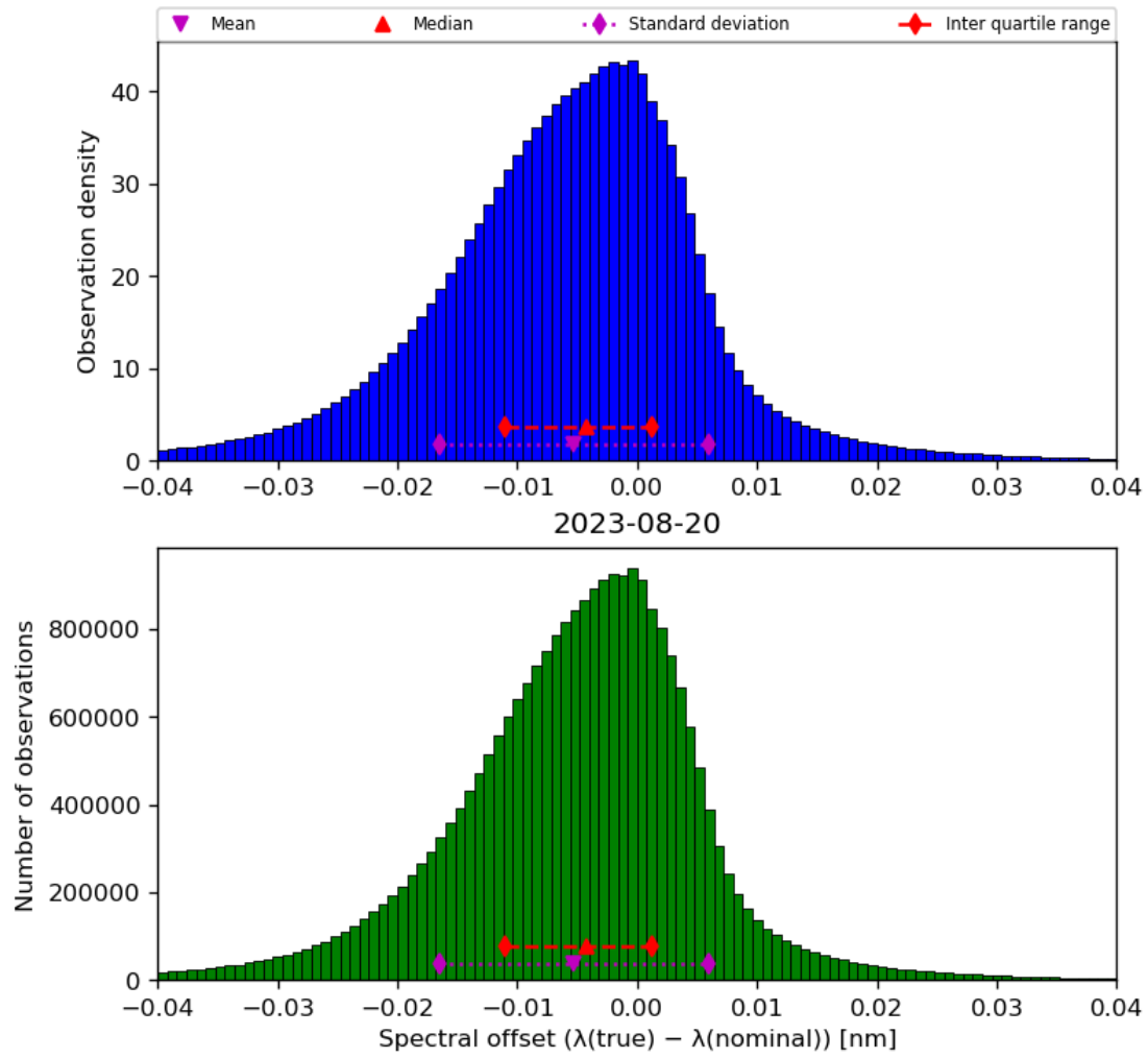
Figure 45: Histogram of “Spectral offset ( \lambda(\text{true}) - \lambda(\text{nominal}) )” for 2023-08-20 to 2023-08-21
