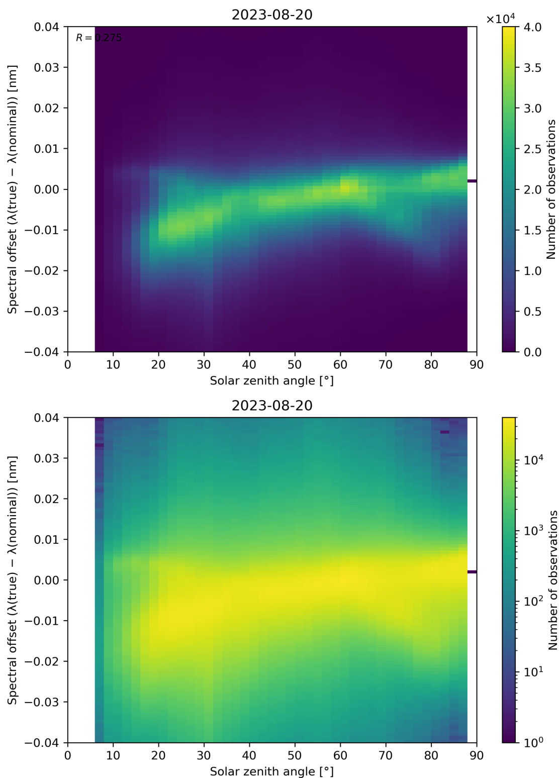
Figure 128: Scatter density plot of “Solar zenith angle” against “Spectral offset ( \lambda(\text{true}) - \lambda(\text{nominal}) )” for 2023-08-20 to 2023-08-21.
