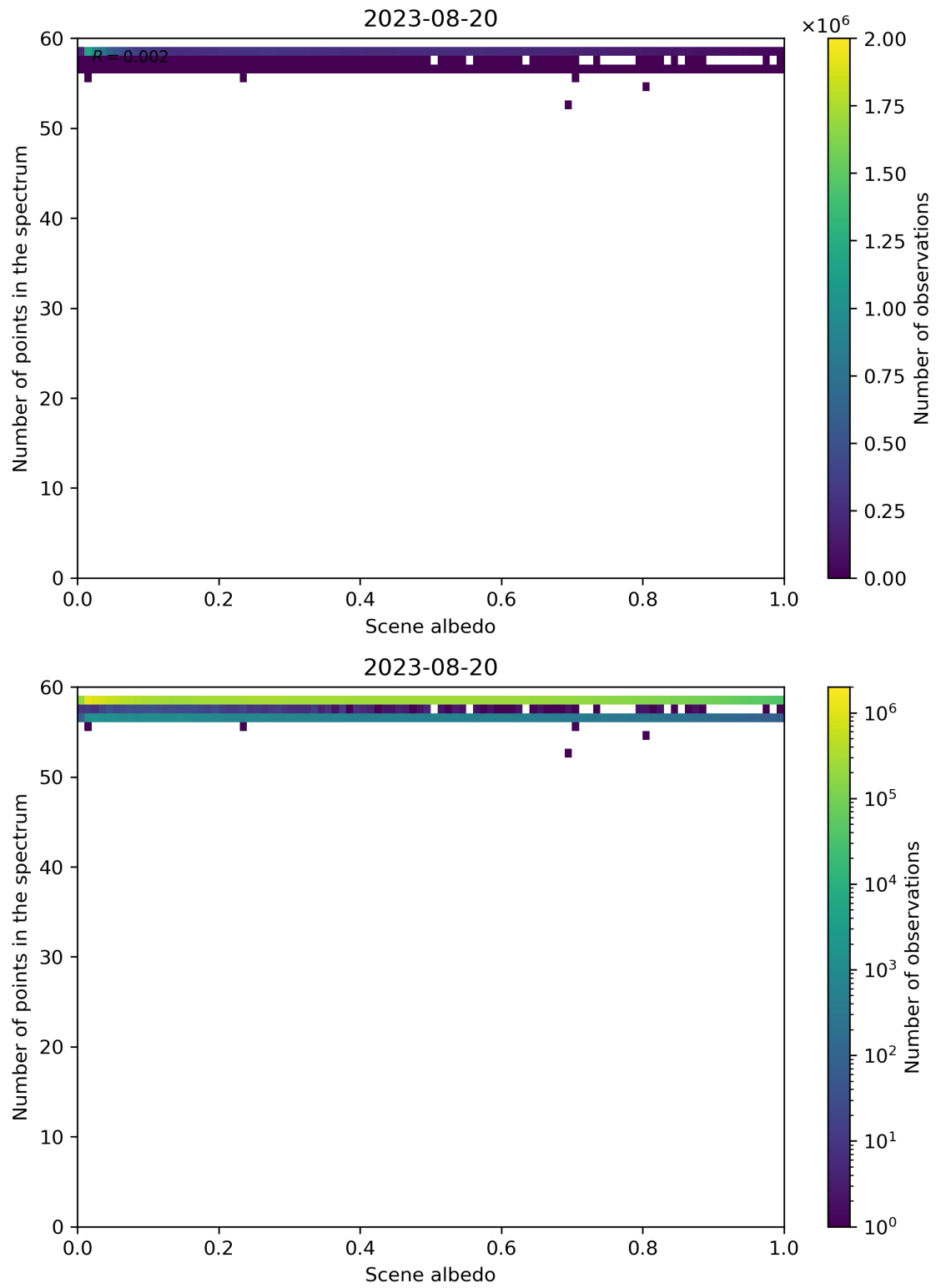
Figure 116: Scatter density plot of “Scene albedo” against “Number of points in the spectrum” for 2023-08-20 to 2023-08-21.
