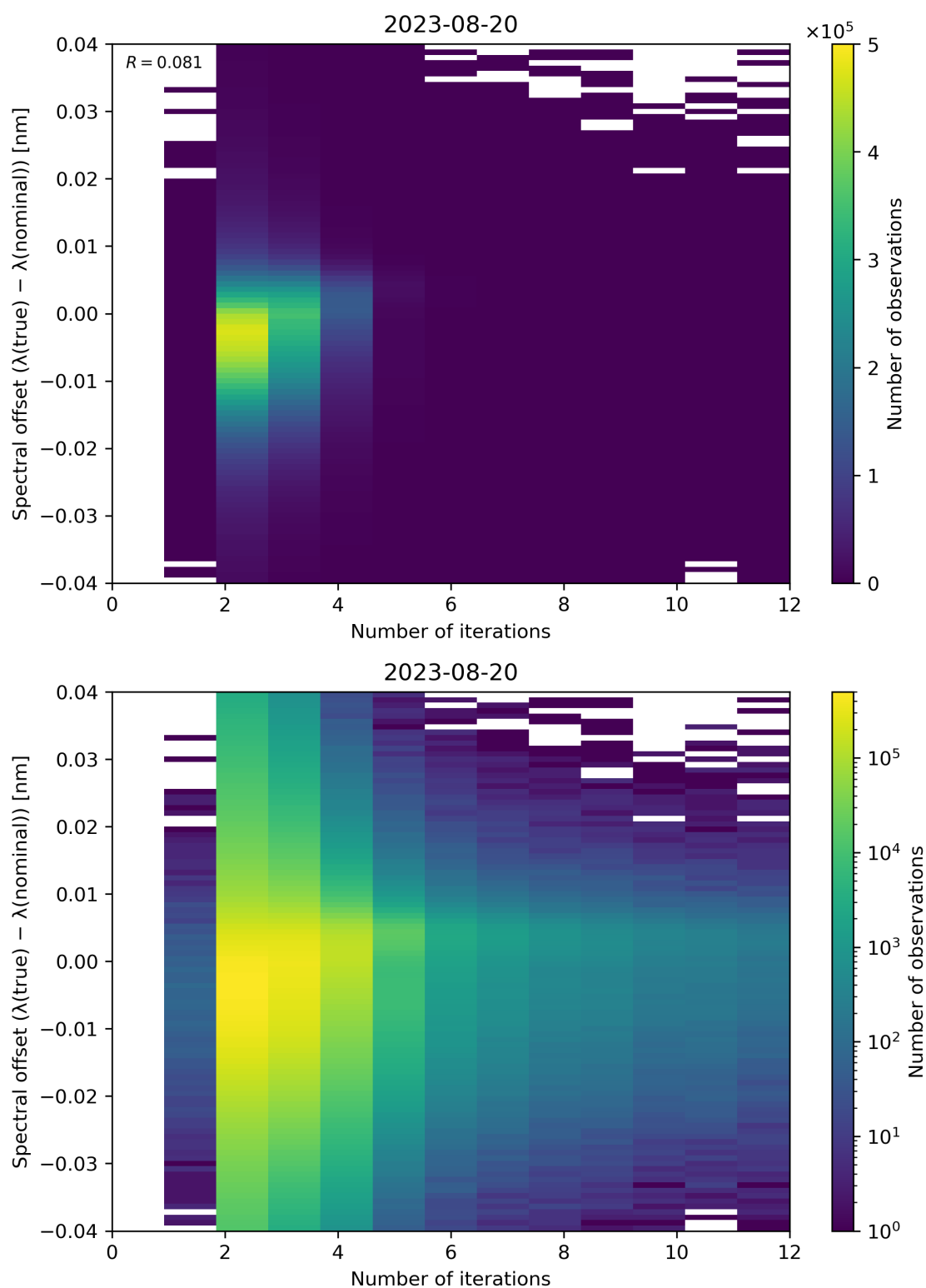
Figure 109: Scatter density plot of “Number of iterations” against “Spectral offset ( \lambda(\text{true}) - \lambda(\text{nominal}) )” for 2023-08-20 to 2023-08-21.
