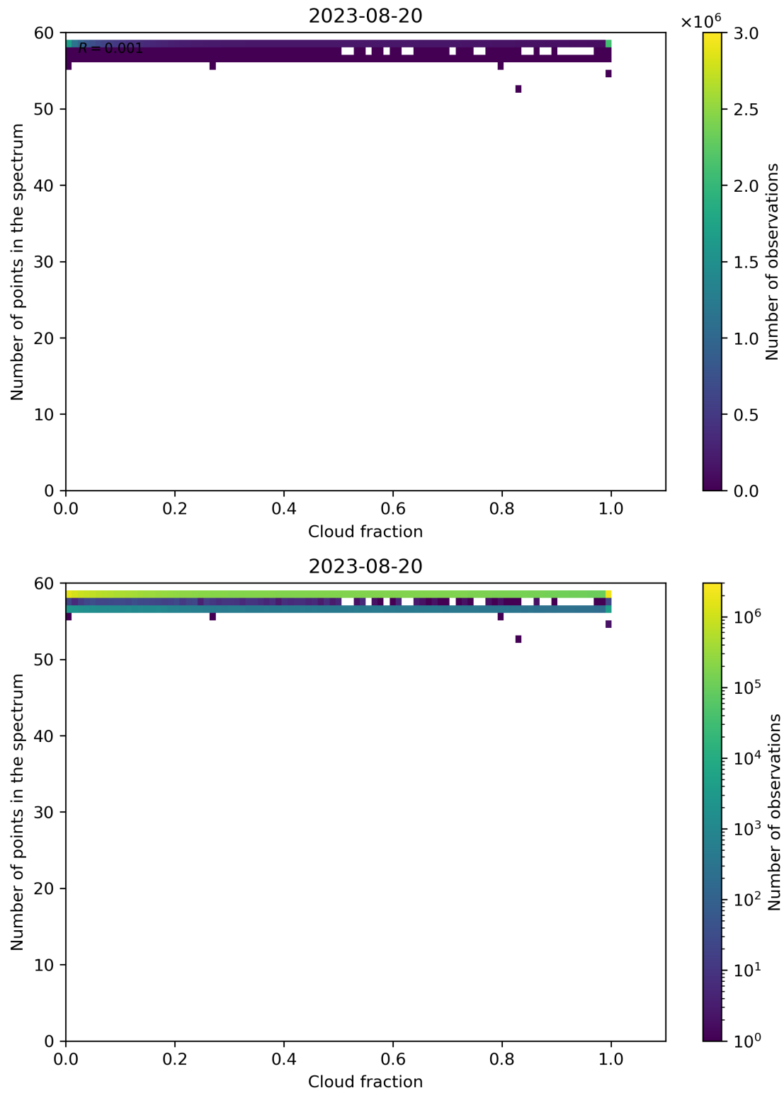
Figure 81: Scatter density plot of “Cloud fraction” against “Number of points in the spectrum” for 2023-08-20 to 2023-08-21.
