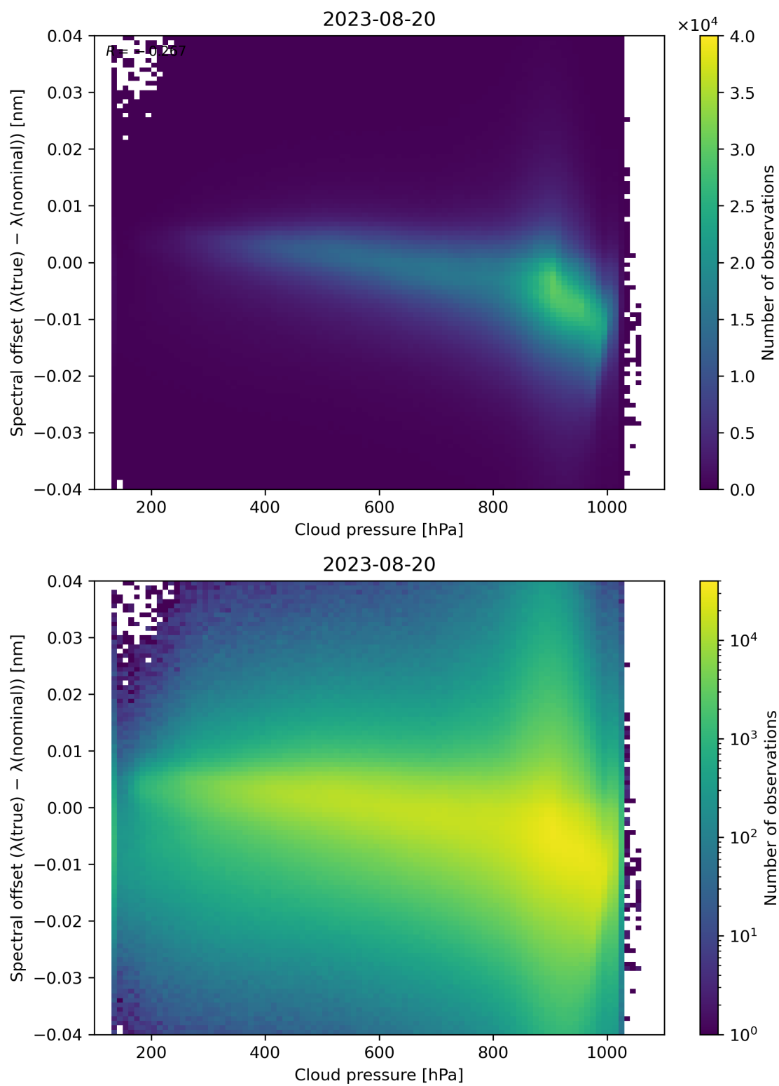
Figure 92: Scatter density plot of “Cloud pressure” against “Spectral offset ( \lambda(\text{true}) - \lambda(\text{nominal}) )” for 2023-08-20 to 2023-08-21.
