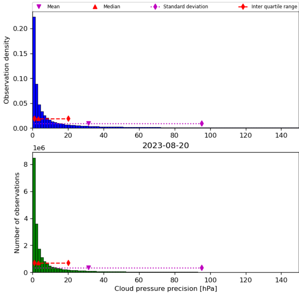
Figure 31: Histogram of “Cloud pressure precision” for 2023-08-20 to 2023-08-21
