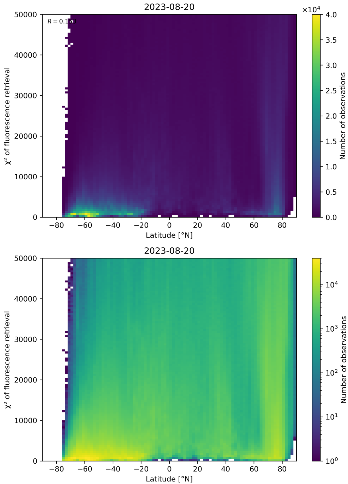
Figure 98: Scatter density plot of “Latitude” against “ \chi^2 of fluorescence retrieval” for 2023-08-20 to 2023-08-21.
