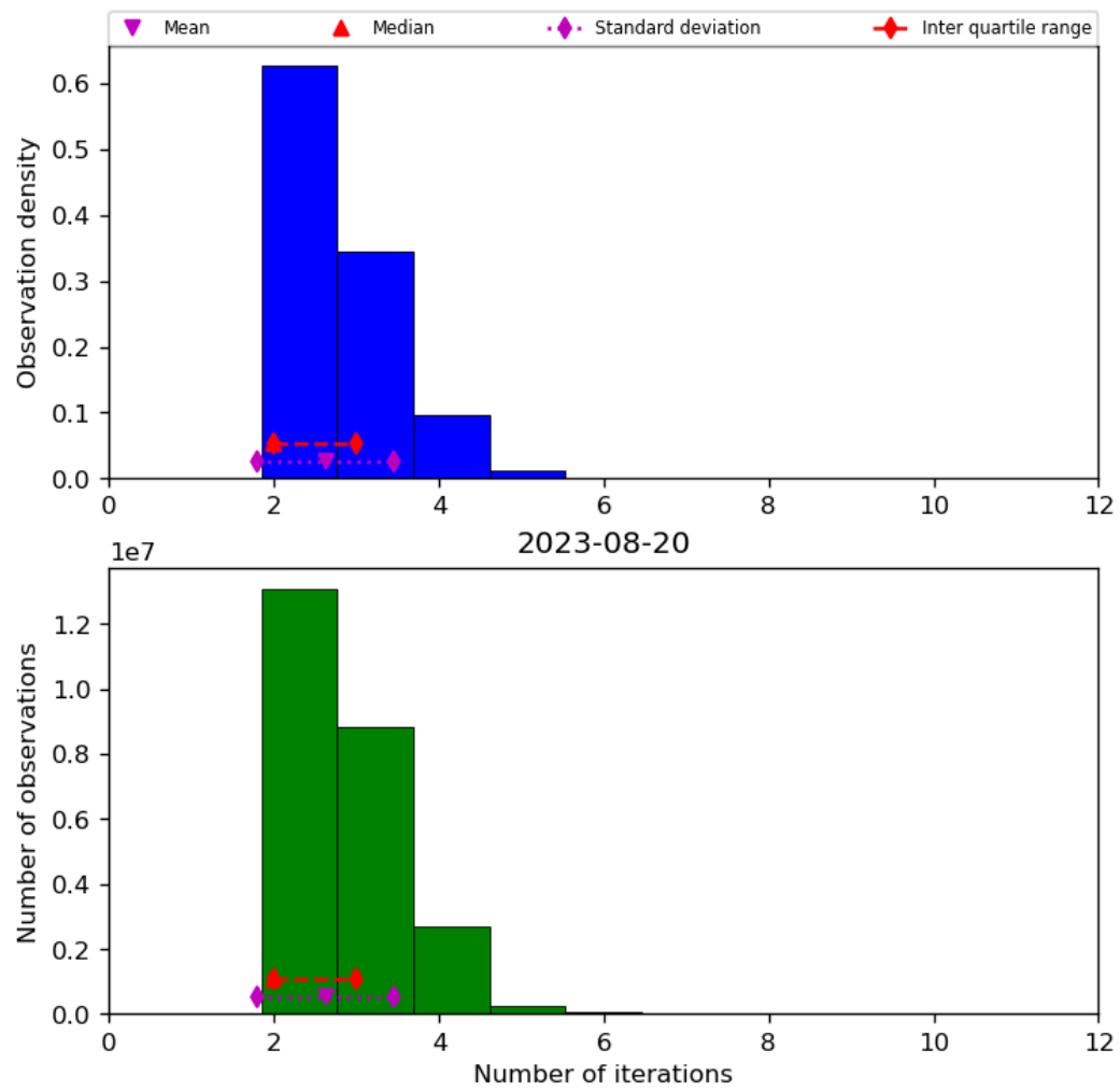
Figure 39: Histogram of “Number of iterations” for 2023-08-20 to 2023-08-21
