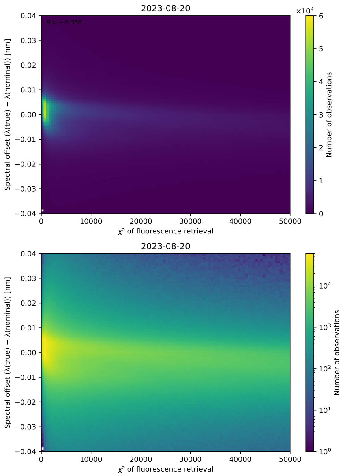
Figure 72: Scatter density plot of " \chi^2 of fluorescence retrieval" against "Spectral offset ( \lambda(\text{true}) - \lambda(\text{nominal})) " for 2023-08-20 to 2023-08-21.
