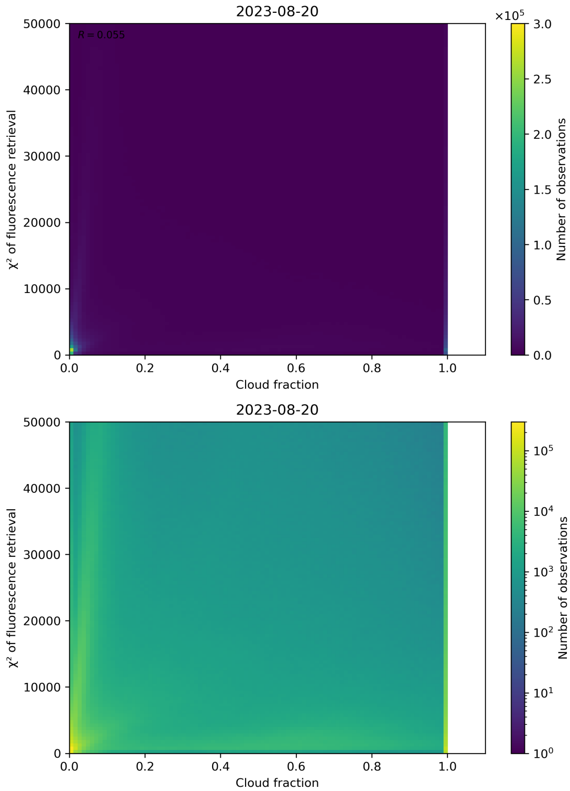
Figure 78: Scatter density plot of “Cloud fraction” against “ \chi^2 of fluorescence retrieval” for 2023-08-20 to 2023-08-21.
