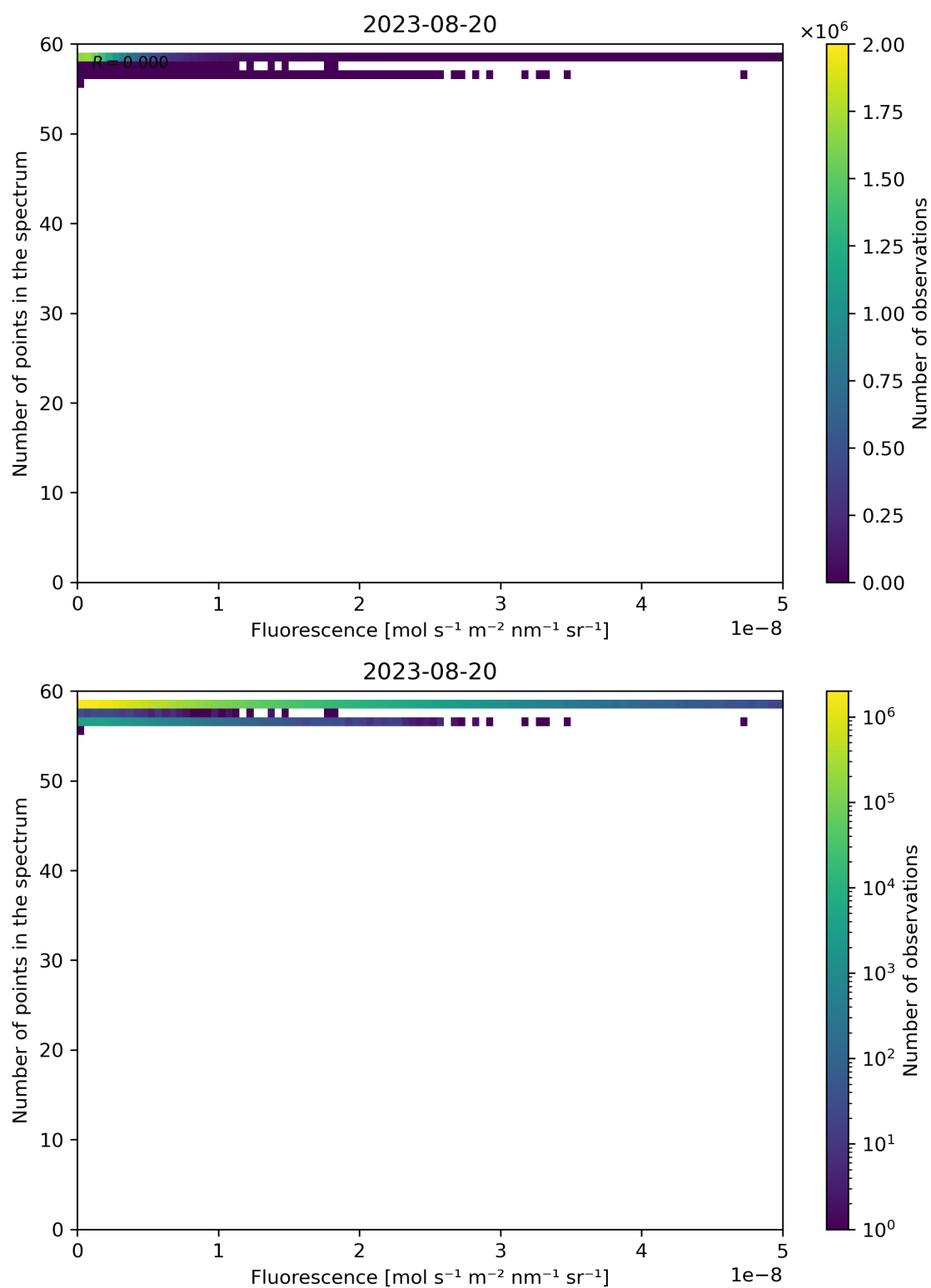
Figure 94: Scatter density plot of “Fluorescence” against “Number of points in the spectrum” for 2023-08-20 to 2023-08-21.
