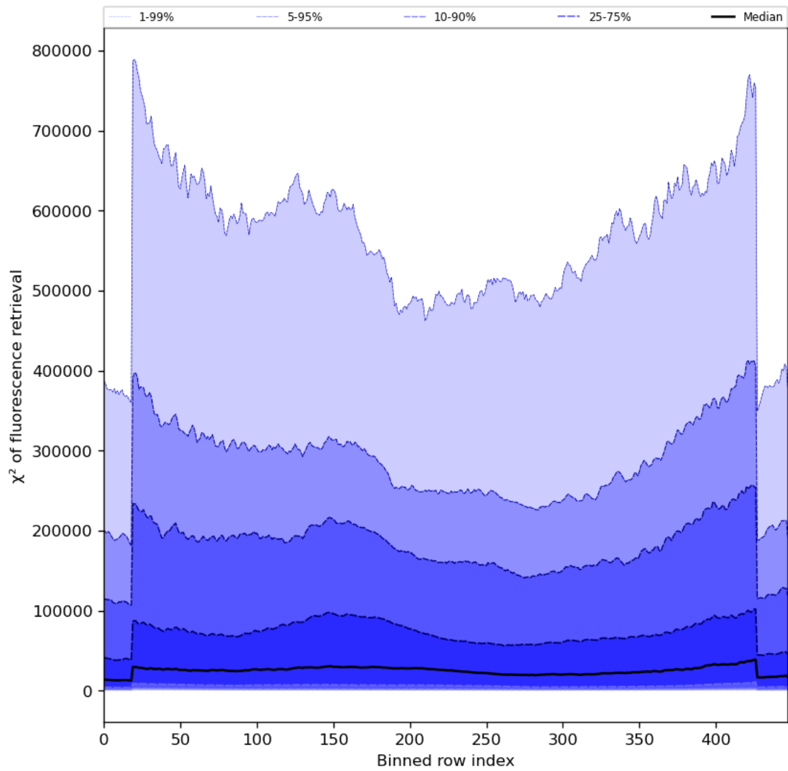
Figure 59: Along track statistics of “ \chi^2 of fluorescence retrieval” for 2023-08-20 to 2023-08-21
