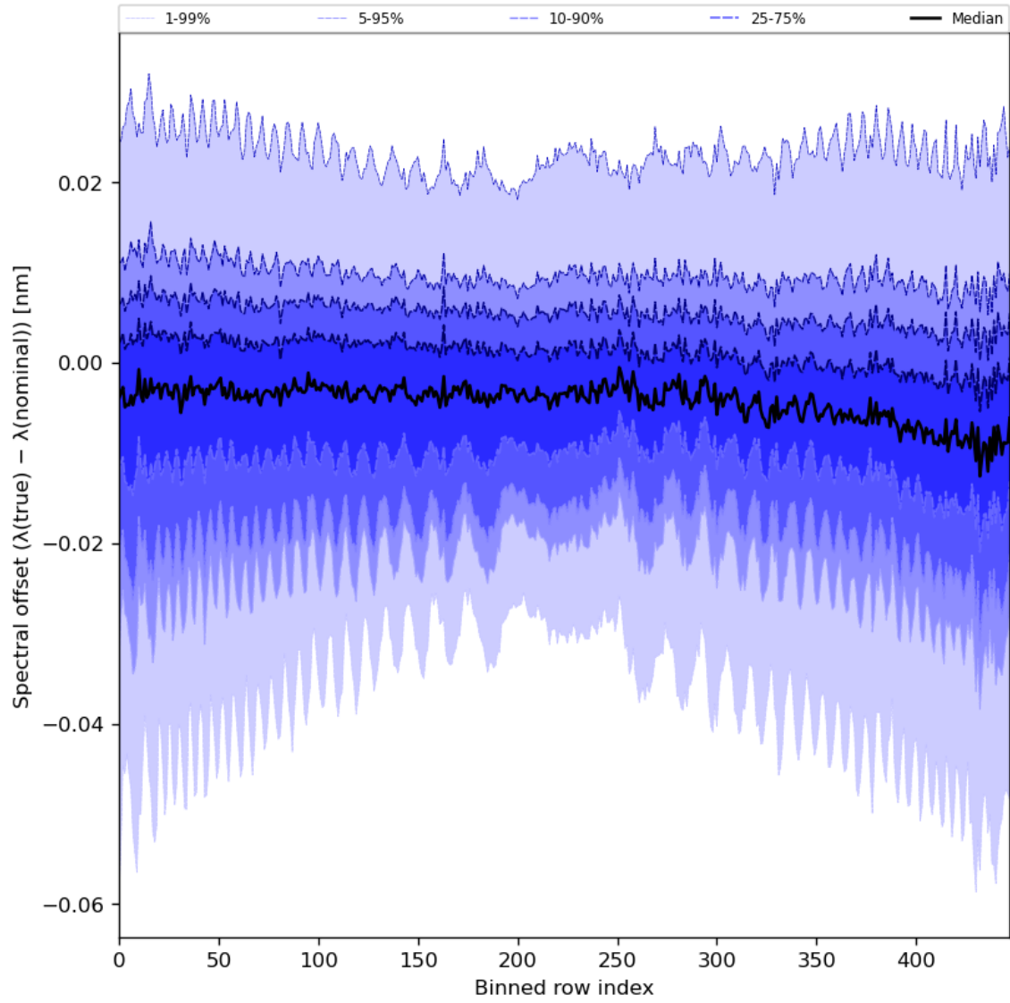
Figure 62: Along track statistics of “Spectral offset ( \lambda(\text{true}) - \lambda(\text{nominal}) )” for 2023-08-20 to 2023-08-21
