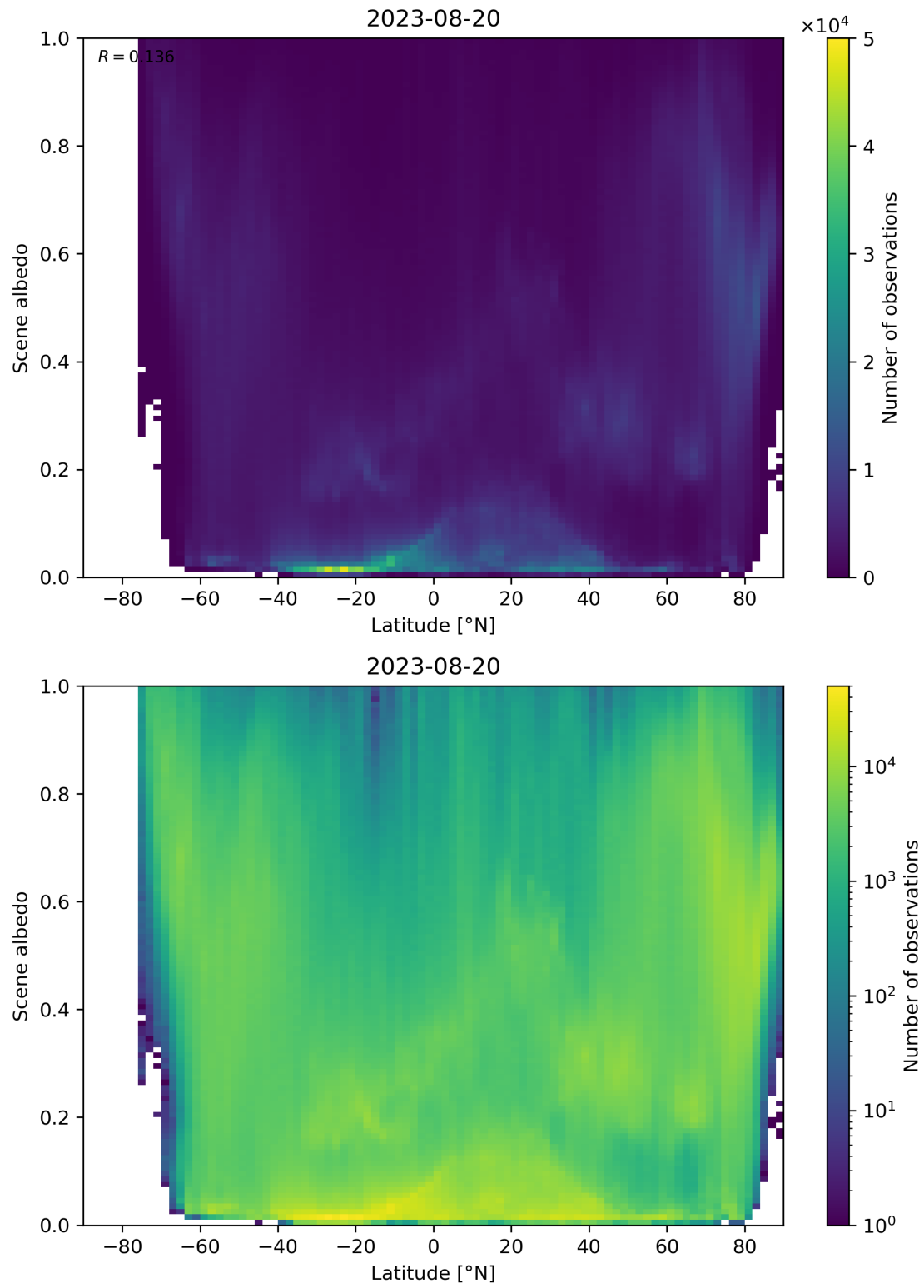
Figure 104: Scatter density plot of “Latitude” against “Scene albedo” for 2023-08-20 to 2023-08-21.
