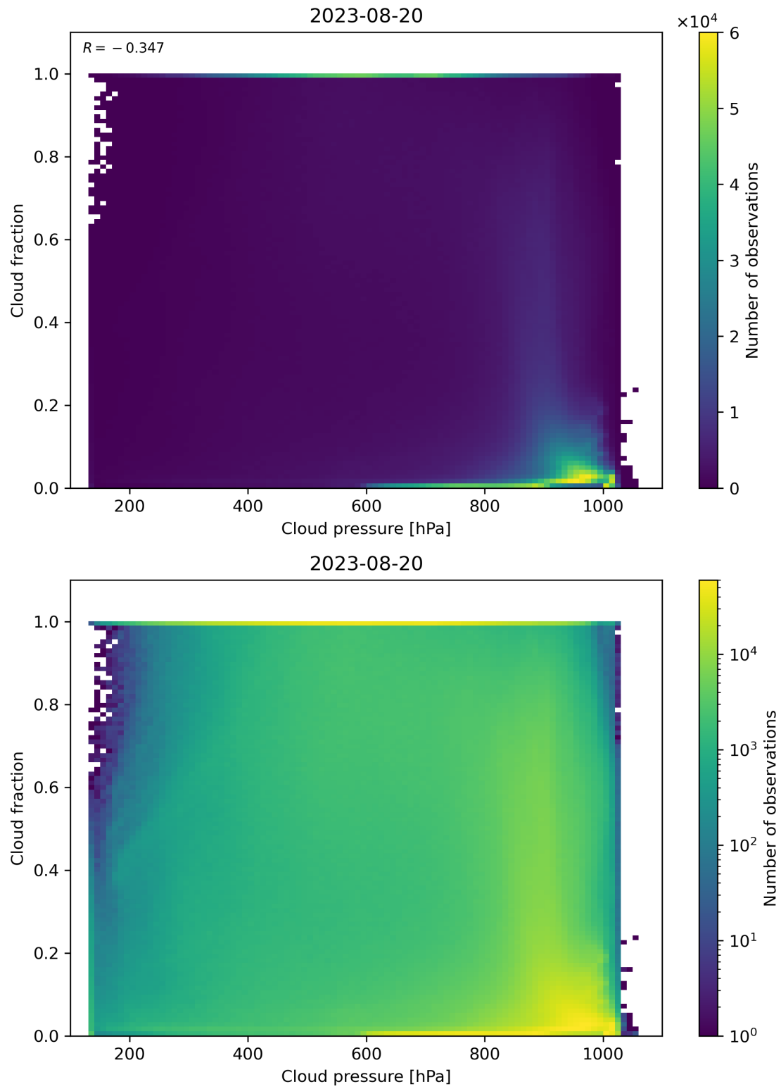
Figure 87: Scatter density plot of “Cloud pressure” against “Cloud fraction” for 2023-08-20 to 2023-08-21.
