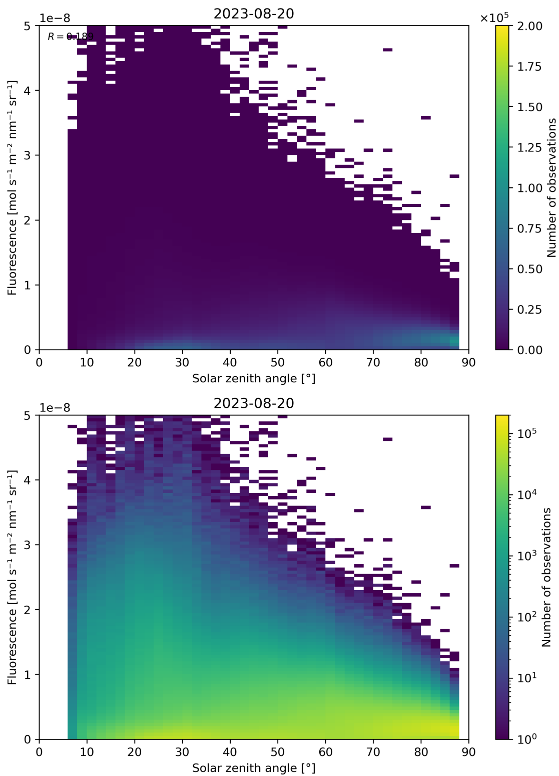
Figure 123: Scatter density plot of “Solar zenith angle” against “Fluorescence” for 2023-08-20 to 2023-08-21.
