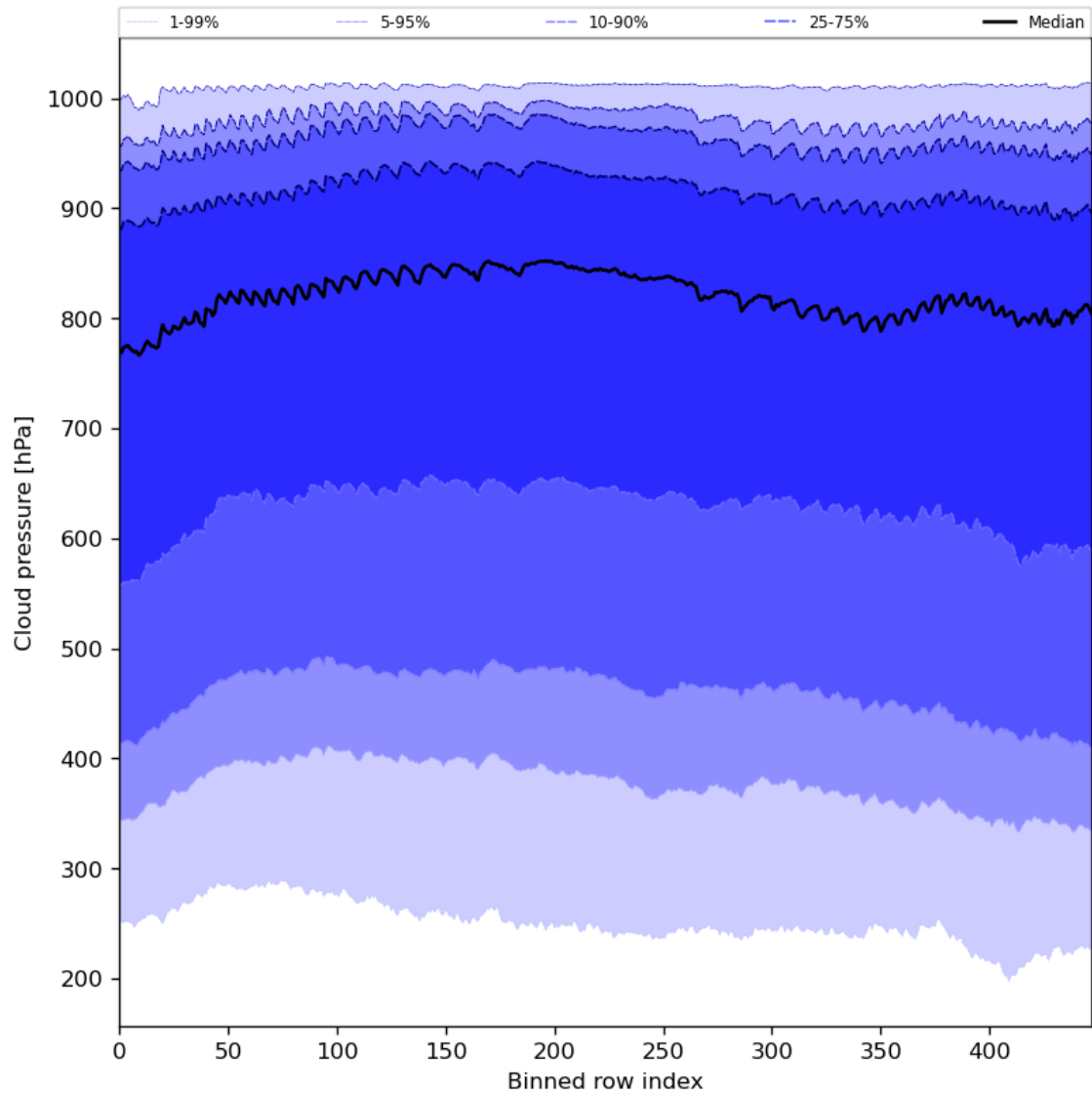
Figure 47: Along track statistics of “Cloud pressure” for 2023-08-20 to 2023-08-21
