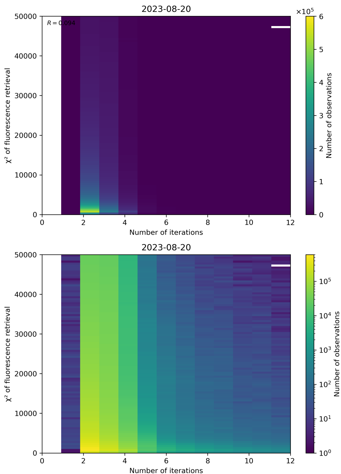
Figure 106: Scatter density plot of “Number of iterations” against “ \chi^2 of fluorescence retrieval” for 2023-08-20 to 2023-08-21.
