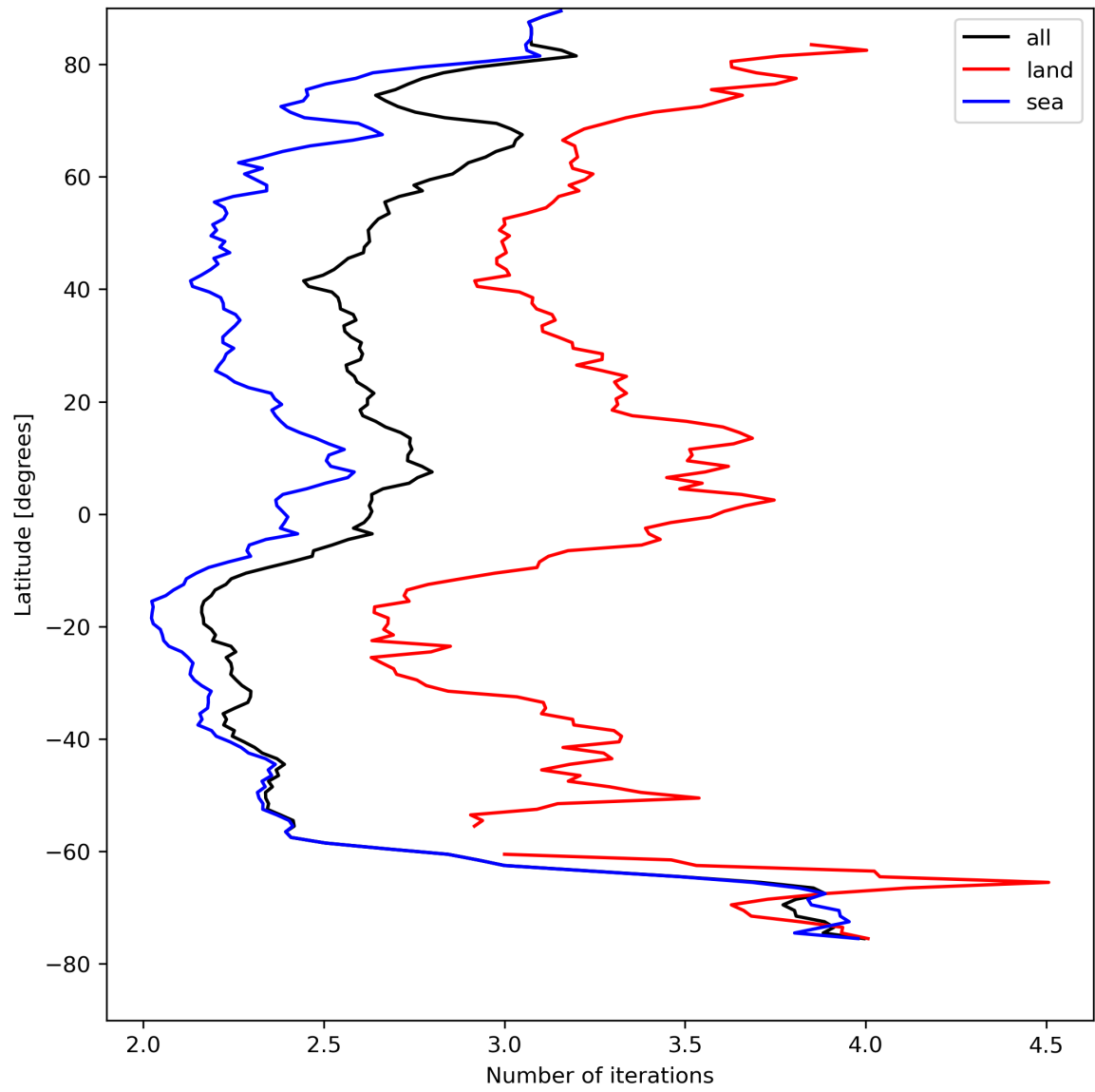
Figure 22: Zonal average of “Number of iterations” for 2023-08-20 to 2023-08-21.
