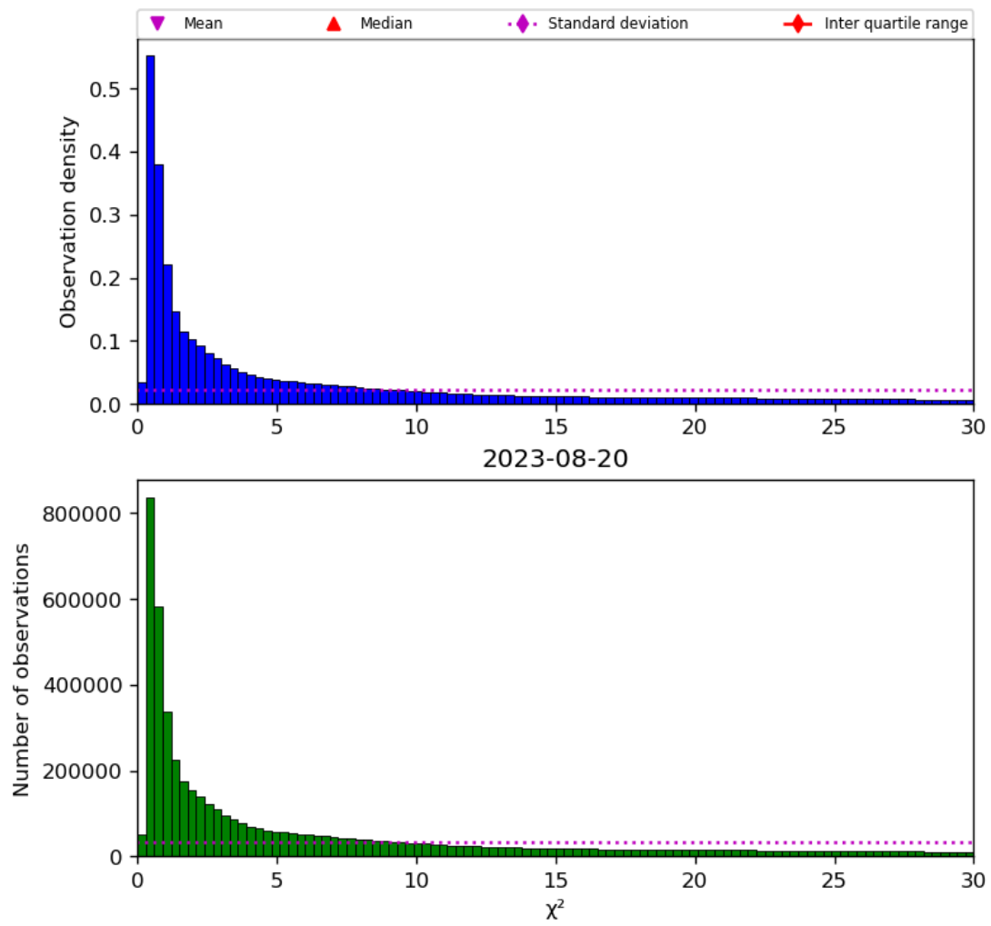
Figure 38: Histogram of “ \chi^2 ” for 2023-08-20 to 2023-08-21
