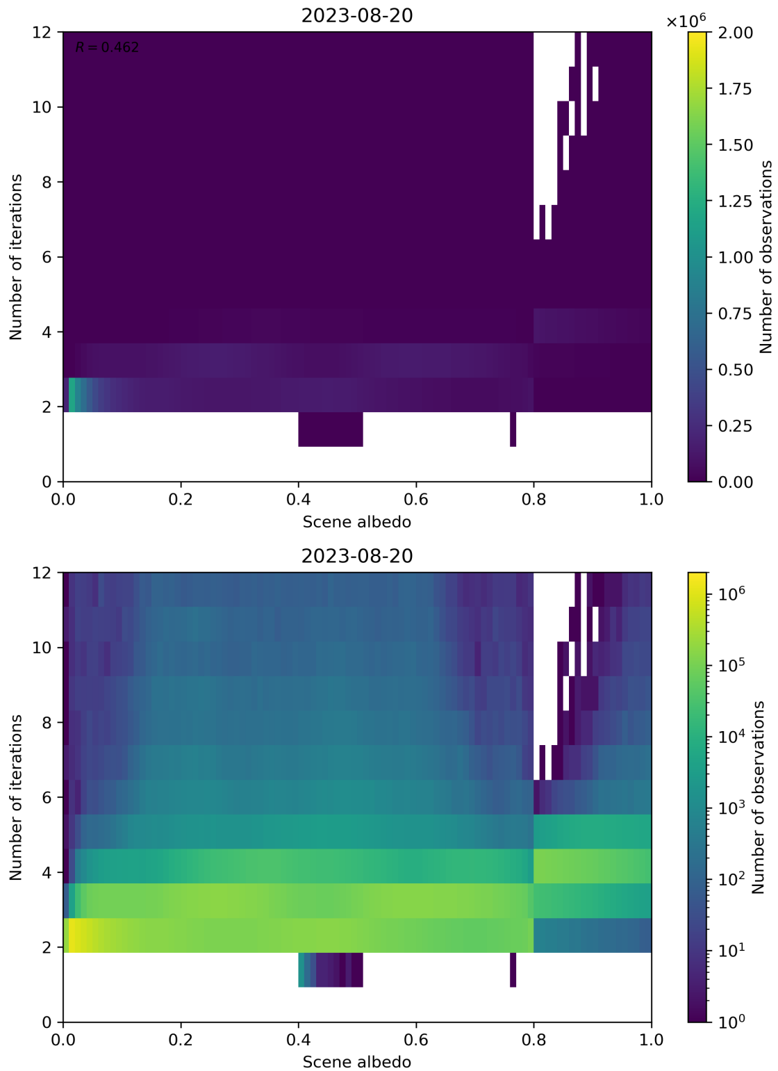
Figure 115: Scatter density plot of “Scene albedo” against “Number of iterations” for 2023-08-20 to 2023-08-21.
