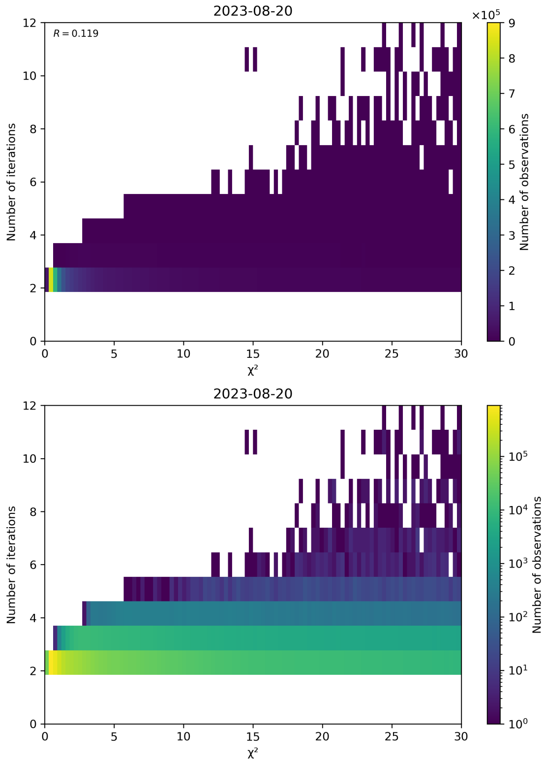
Figure 73: Scatter density plot of “ \chi^2 ” against “Number of iterations” for 2023-08-20 to 2023-08-21.
