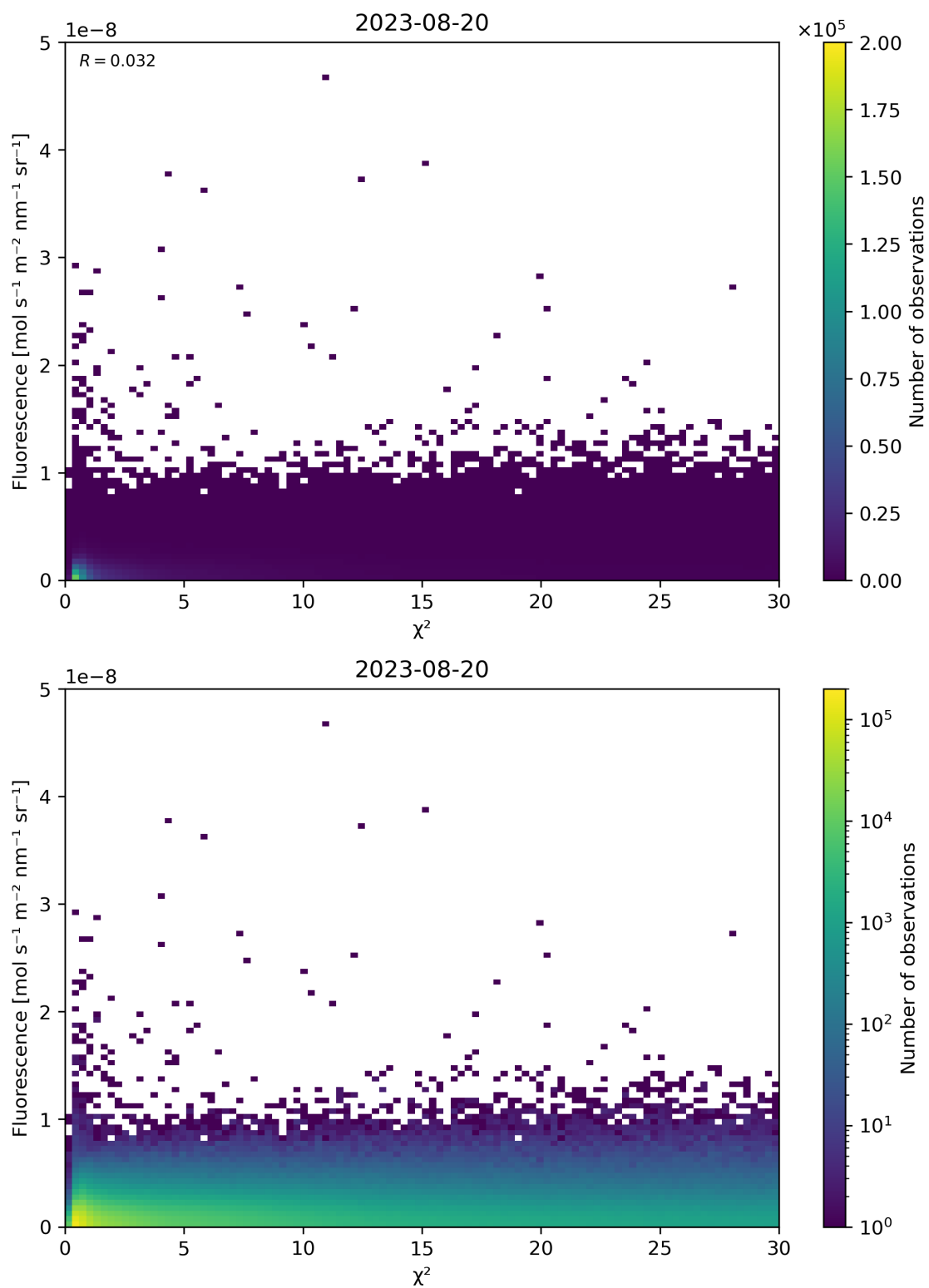
Figure 70: Scatter density plot of “ \chi^2 ” against “Fluorescence” for 2023-08-20 to 2023-08-21.
