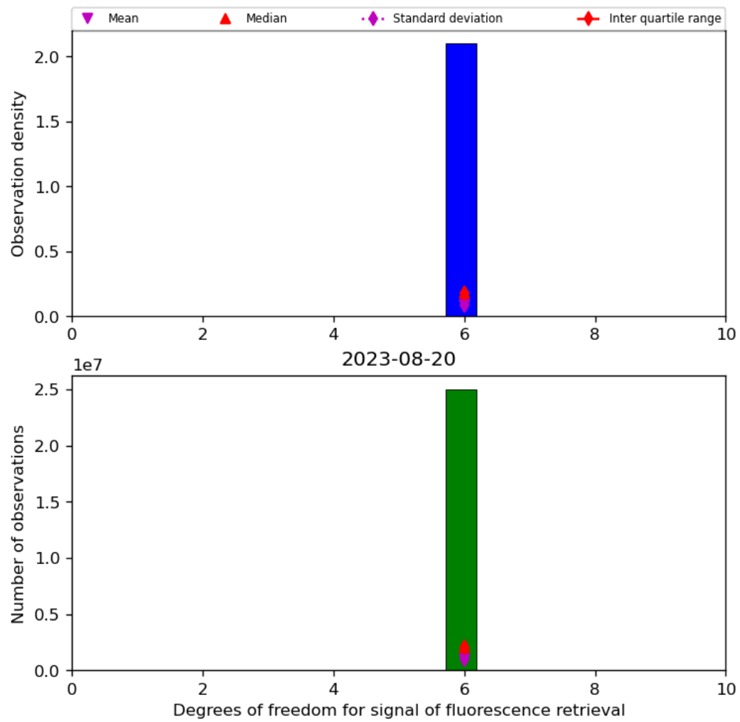
Figure 43: Histogram of “Degrees of freedom for signal of fluorescence retrieval” for 2023-08-20 to 2023-08-21
