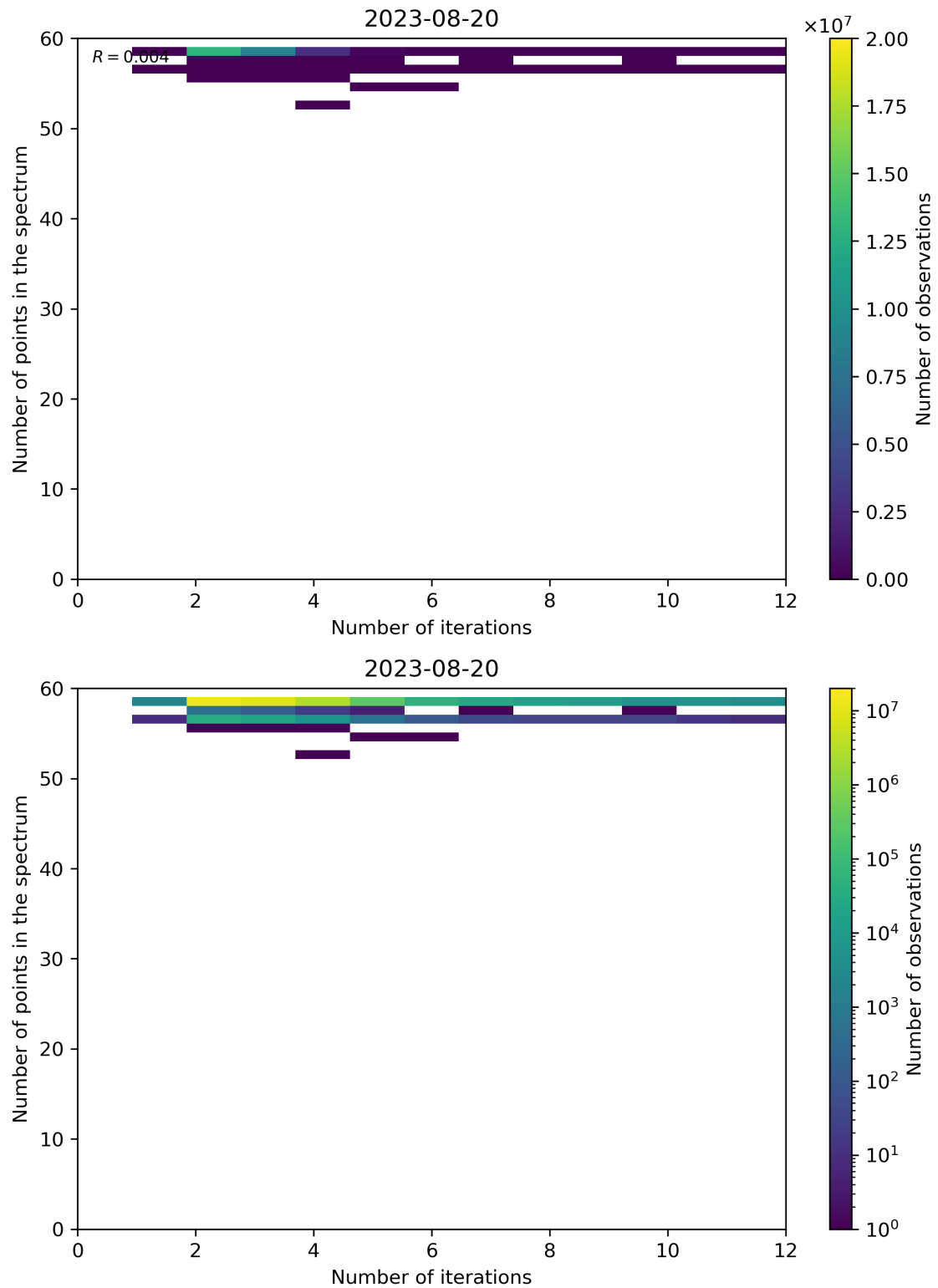
Figure 108: Scatter density plot of “Number of iterations” against “Number of points in the spectrum” for 2023-08-20 to 2023-08-21.
