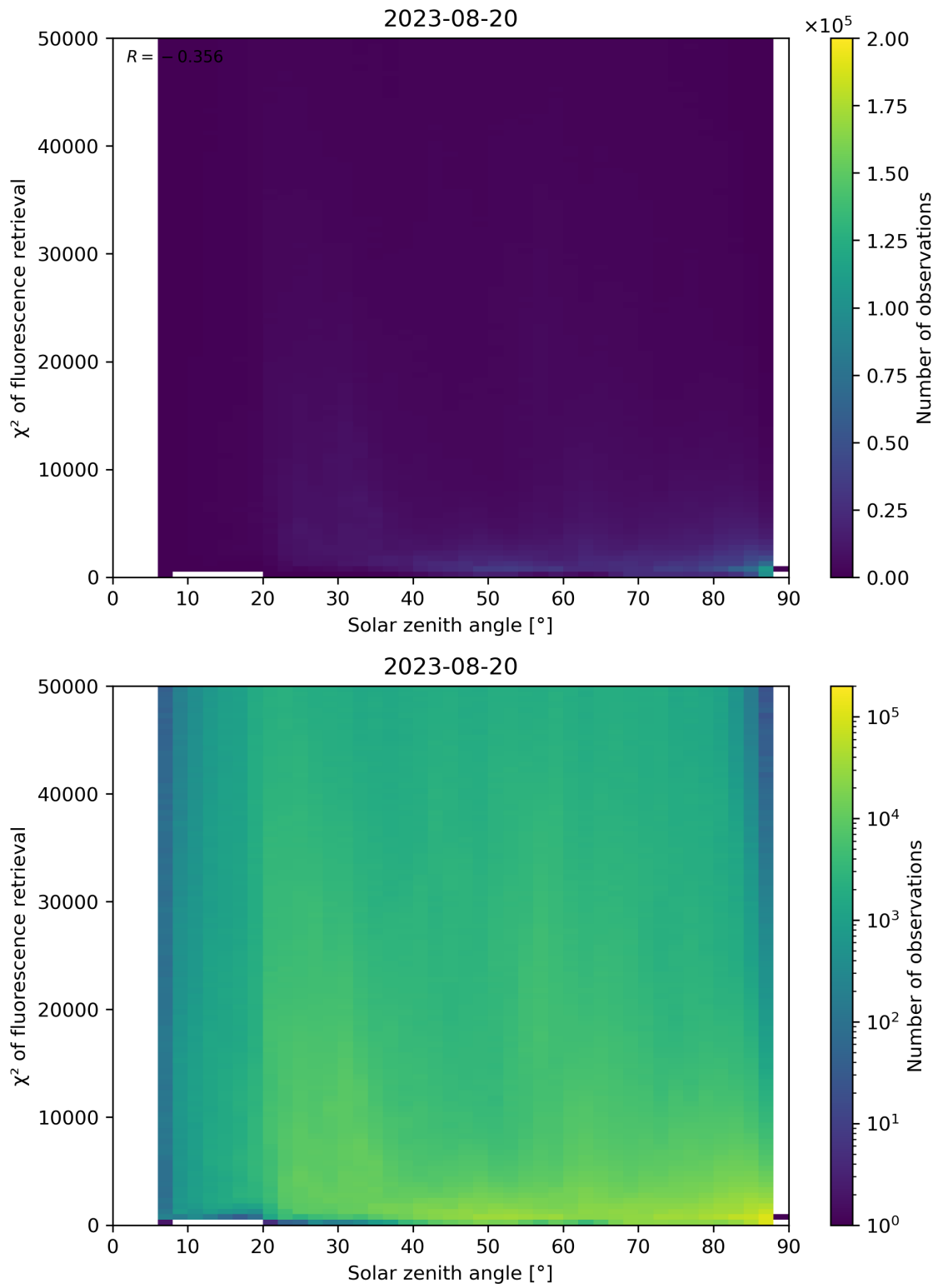
Figure 120: Scatter density plot of “Solar zenith angle” against “ \chi^2 of fluorescence retrieval” for 2023-08-20 to 2023-08-21.
