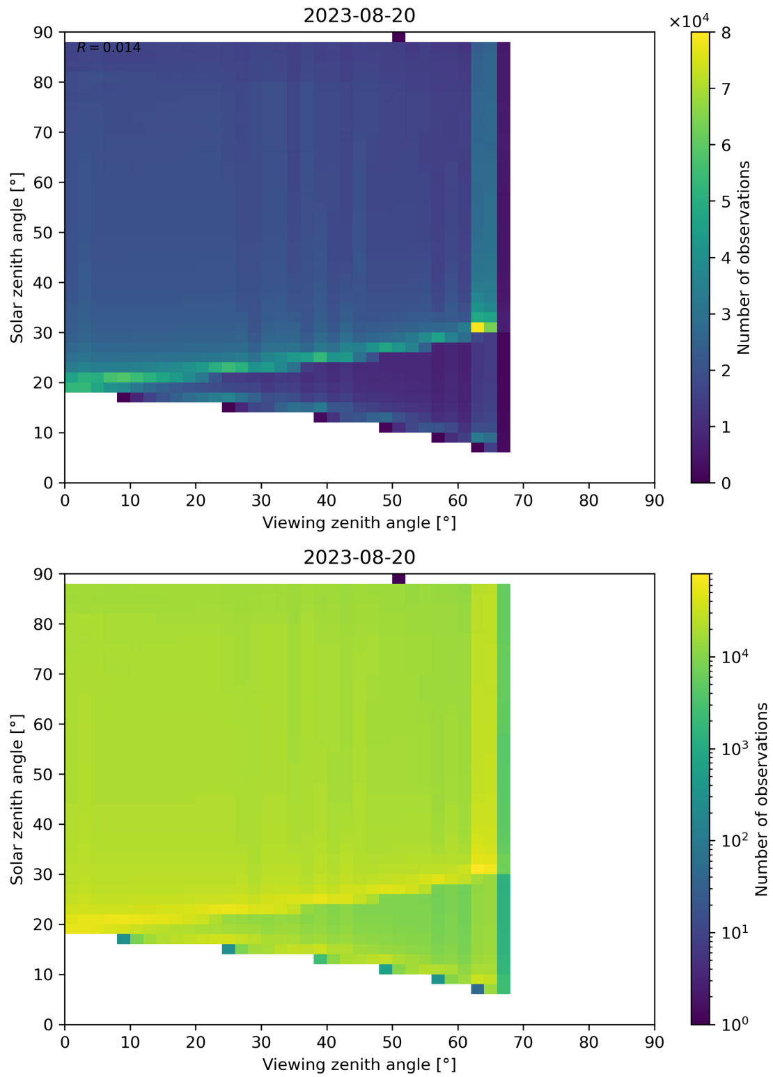
Figure 139: Scatter density plot of “Viewing zenith angle” against “Solar zenith angle” for 2023-08-20 to 2023-08-21.
