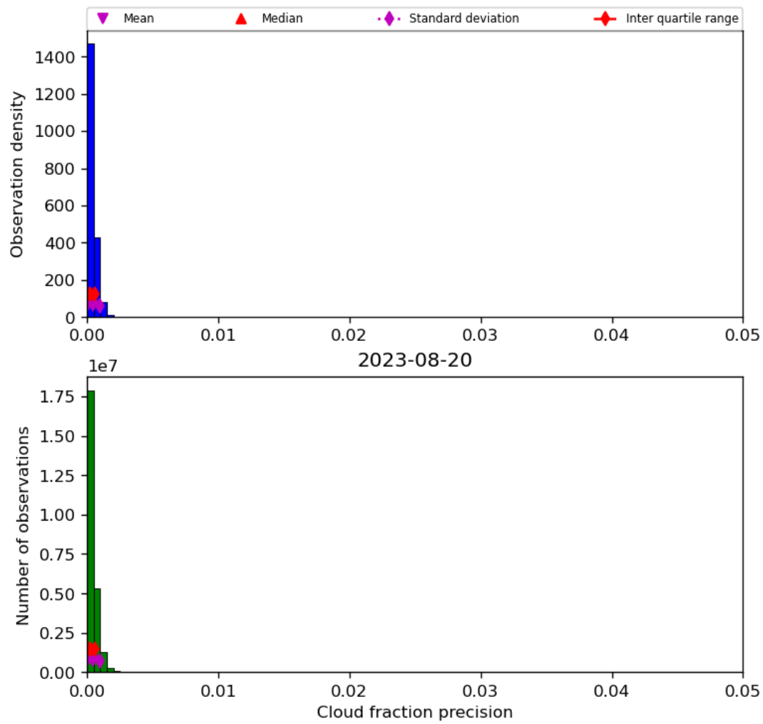
Figure 33: Histogram of “Cloud fraction precision” for 2023-08-20 to 2023-08-21
