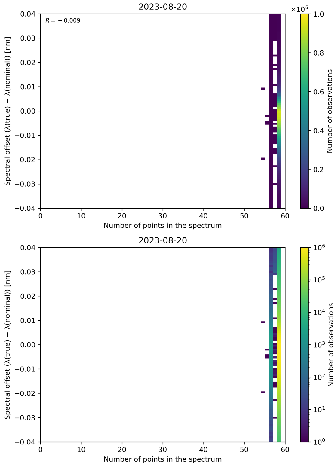
Figure 110: Scatter density plot of “Number of points in the spectrum” against “Spectral offset ( \lambda(\text{true}) - \lambda(\text{nominal}) )” for 2023-08-20 to 2023-08-21.
