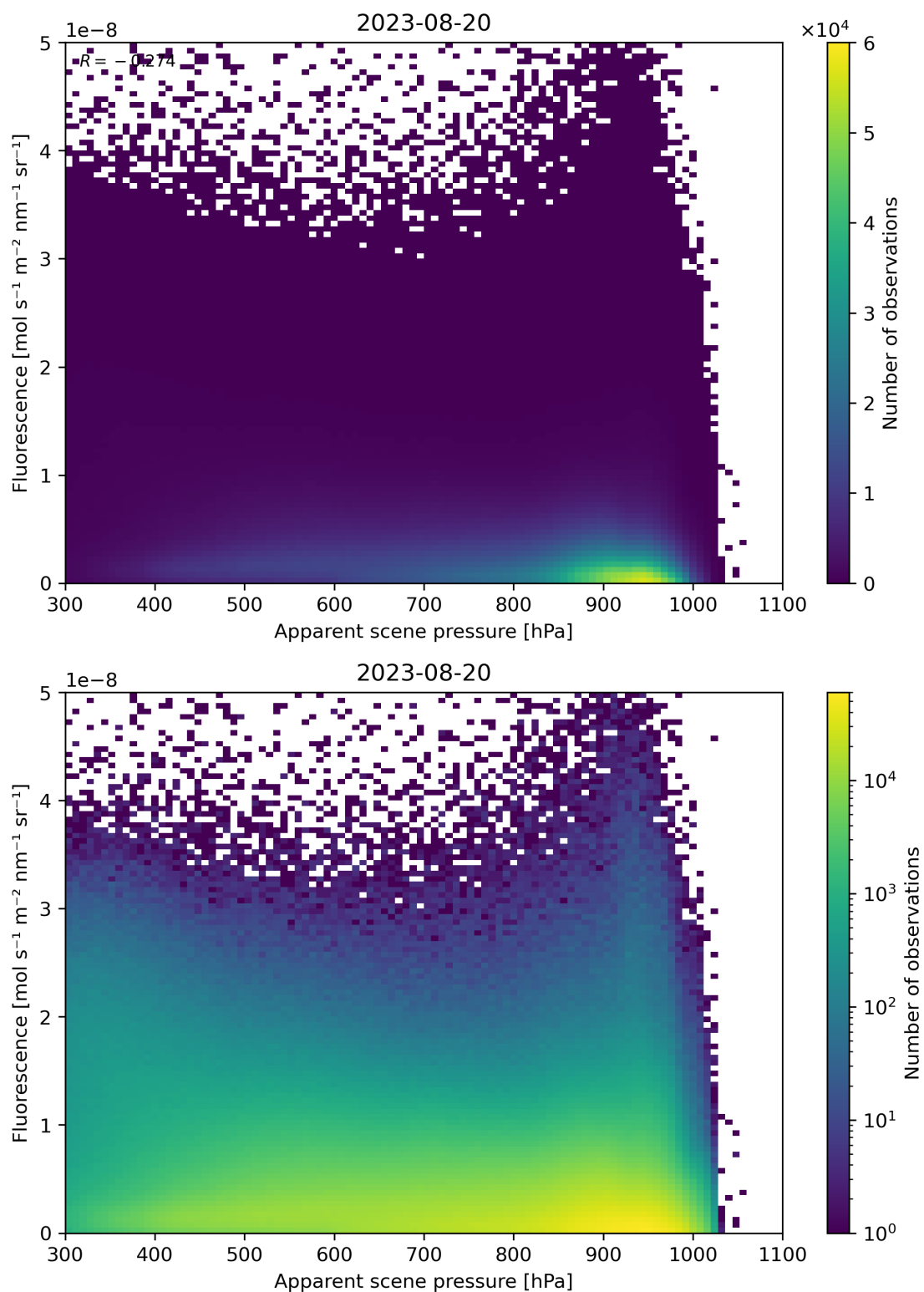
Figure 65: Scatter density plot of “Apparent scene pressure” against “Fluorescence” for 2023-08-20 to 2023-08-21.
