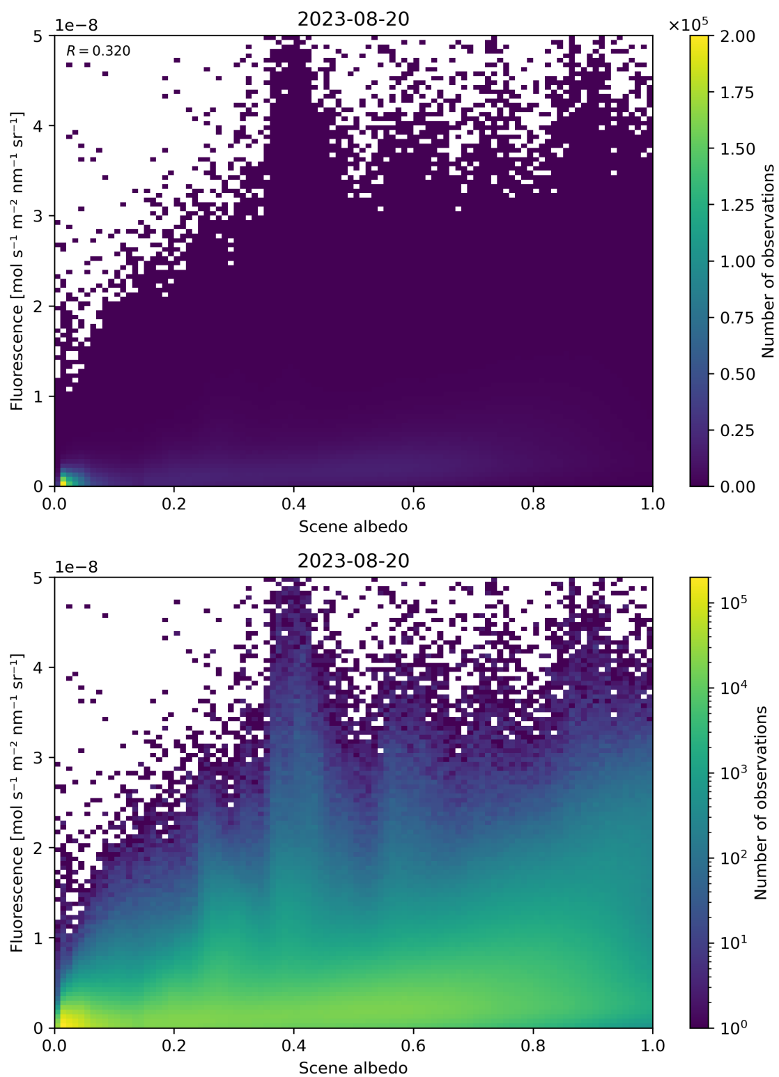
Figure 114: Scatter density plot of “Scene albedo” against “Fluorescence” for 2023-08-20 to 2023-08-21.
