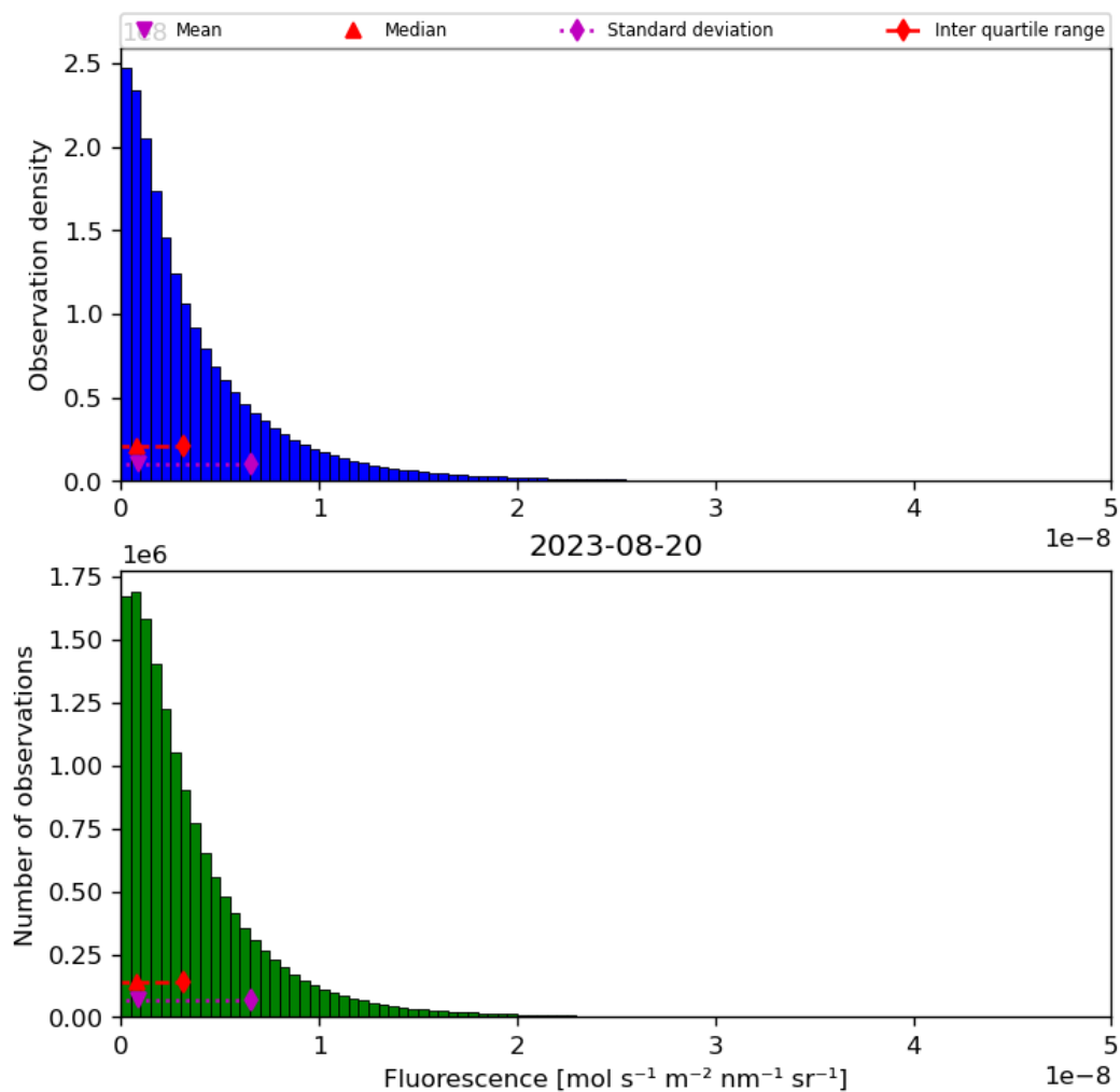
Figure 40: Histogram of “Fluorescence” for 2023-08-20 to 2023-08-21
