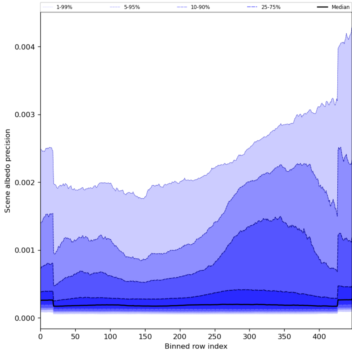
Figure 52: Along track statistics of “Scene albedo precision” for 2023-08-20 to 2023-08-21
