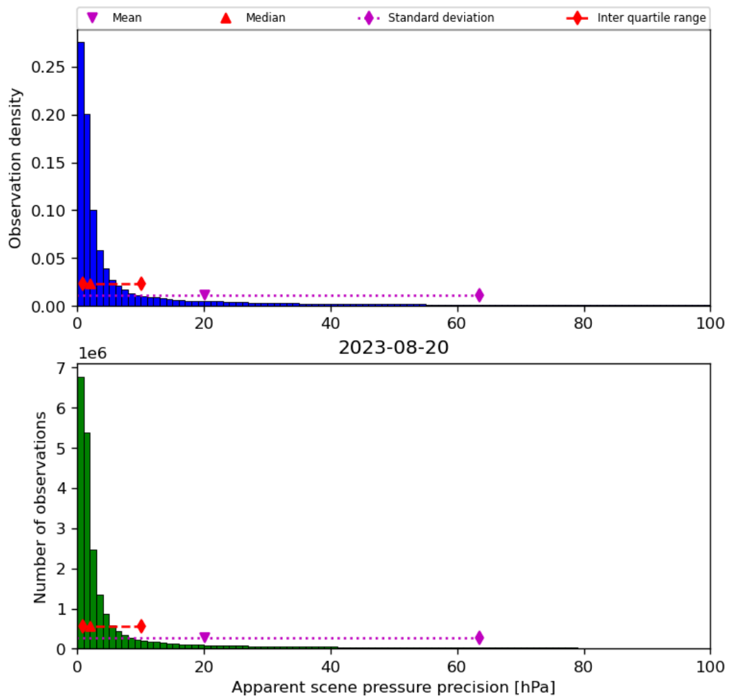
Figure 37: Histogram of “Apparent scene pressure precision” for 2023-08-20 to 2023-08-21
