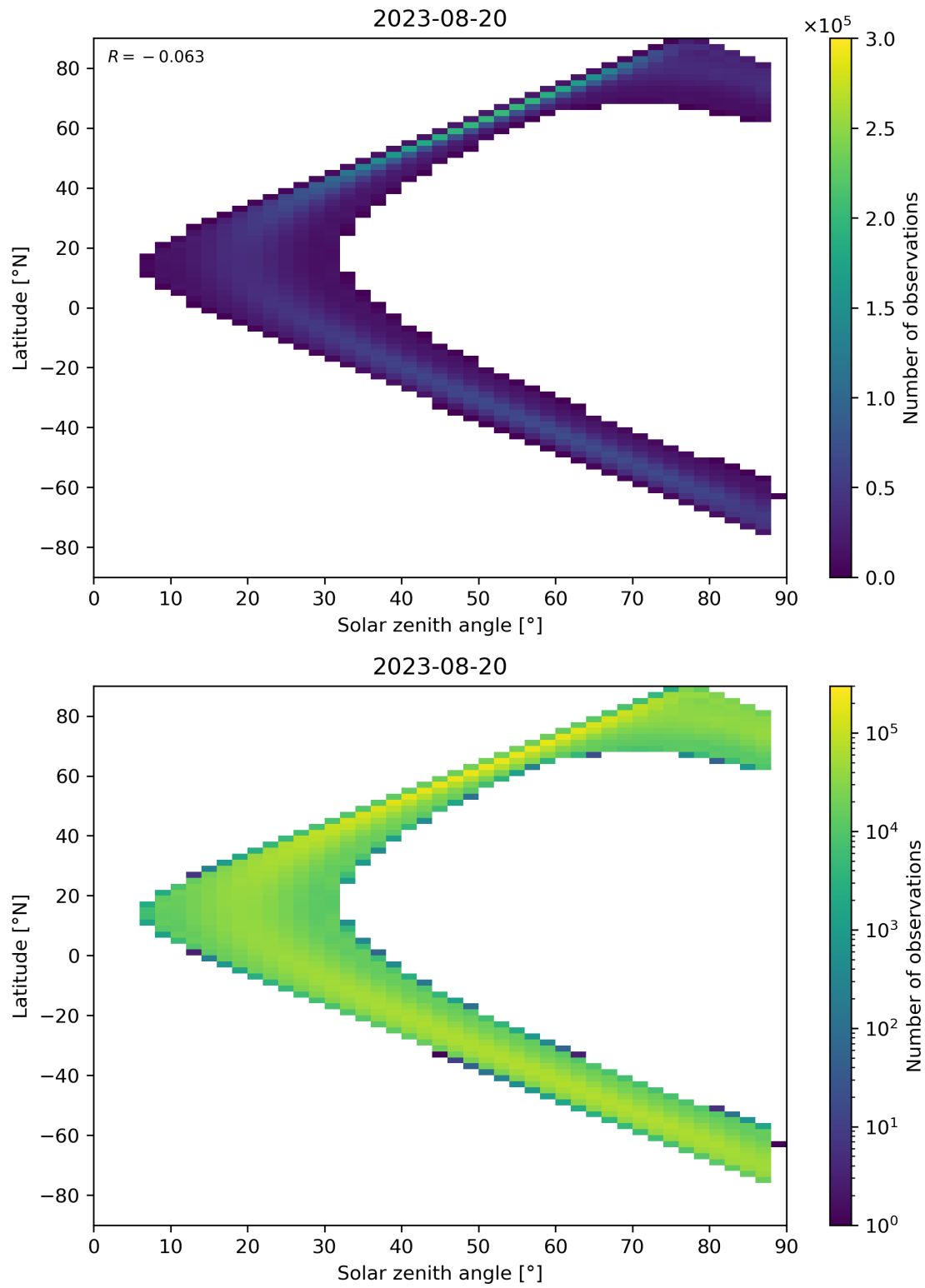
Figure 124: Scatter density plot of “Solar zenith angle” against “Latitude” for 2023-08-20 to 2023-08-21.
