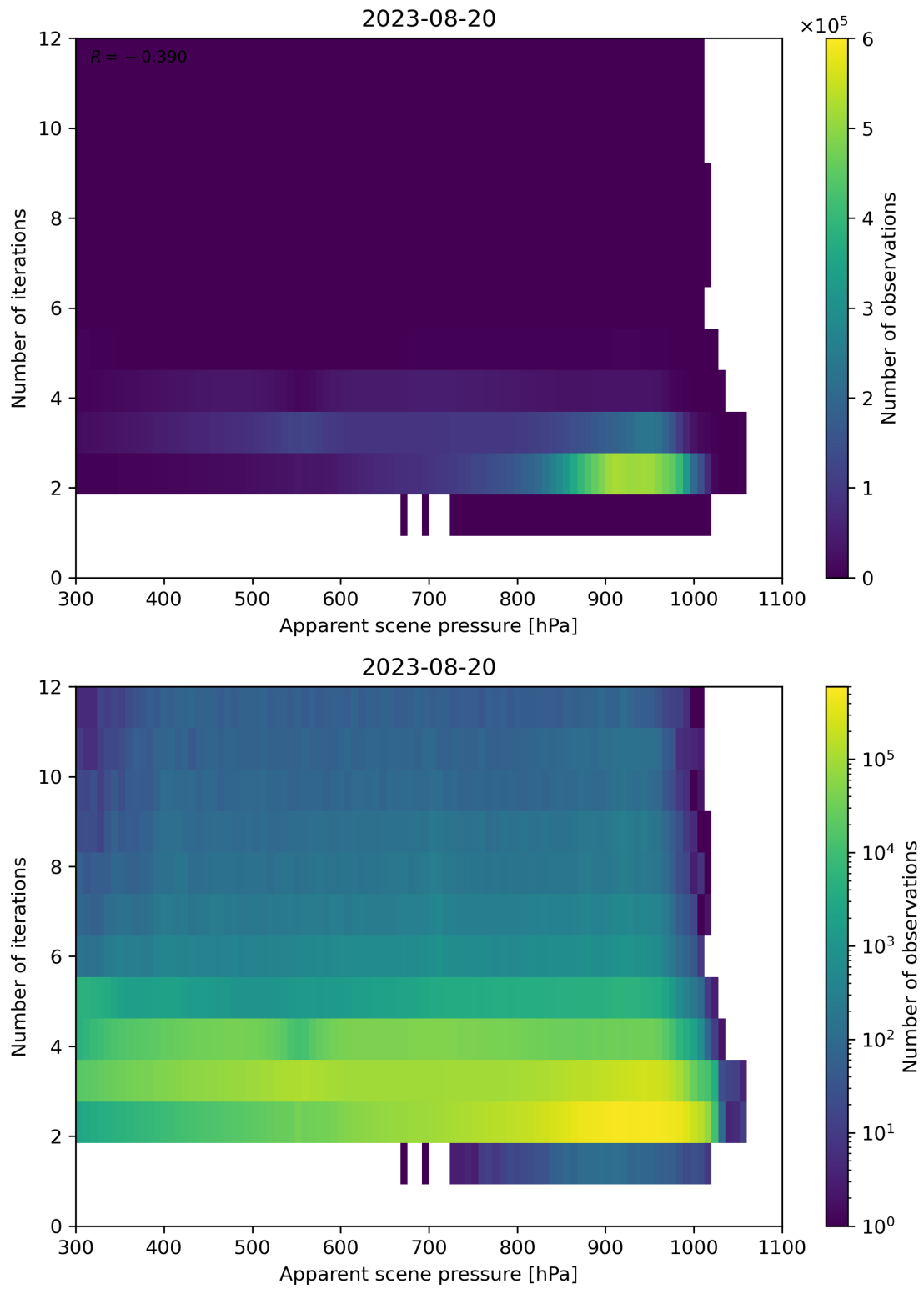
Figure 66: Scatter density plot of “Apparent scene pressure” against “Number of iterations” for 2023-08-20 to 2023-08-21.
