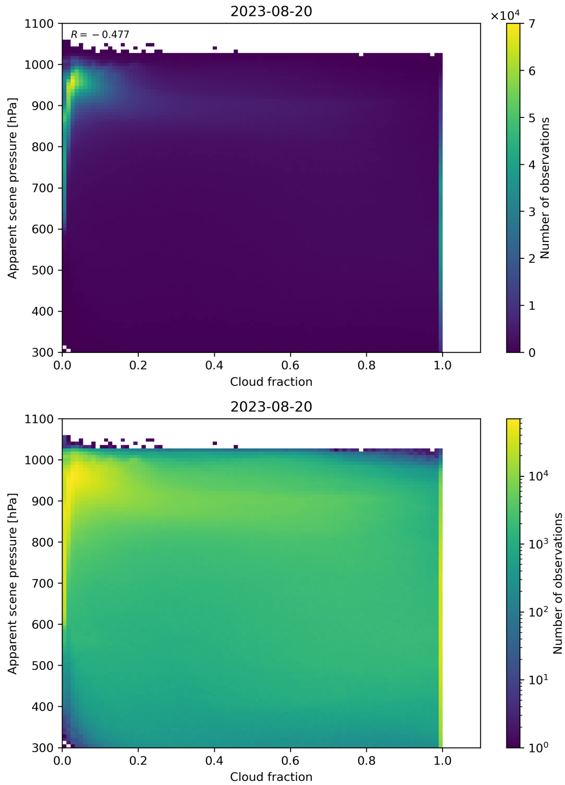
Figure 76: Scatter density plot of “Cloud fraction” against “Apparent scene pressure” for 2023-08-20 to 2023-08-21.
