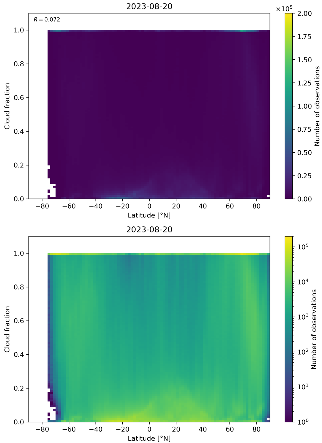
Figure 99: Scatter density plot of “Latitude” against “Cloud fraction” for 2023-08-20 to 2023-08-21.
