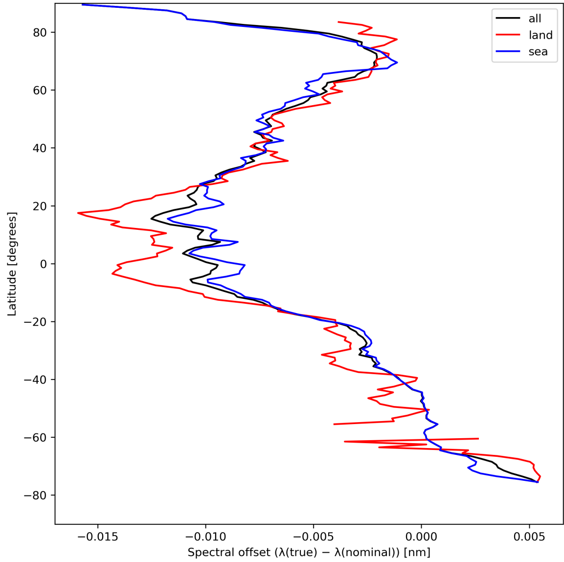
Figure 28: Zonal average of “Spectral offset ( \lambda(\text{true}) - \lambda(\text{nominal}) )” for 2023-08-20 to 2023-08-21.
