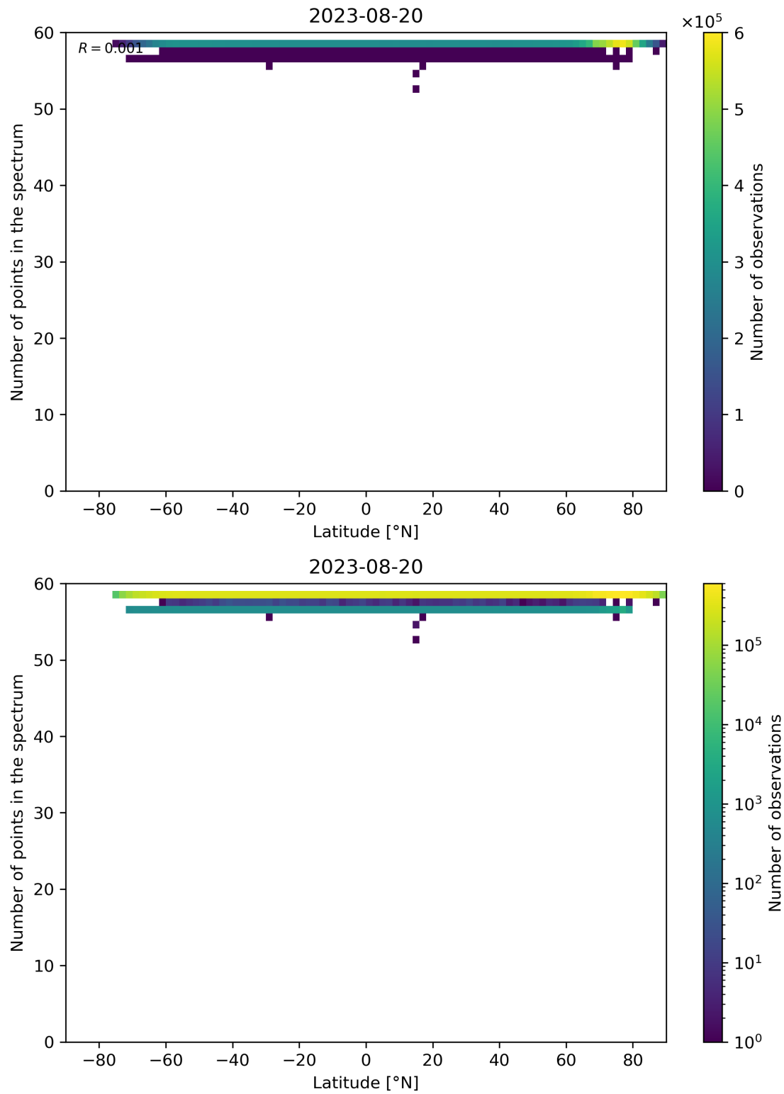
Figure 103: Scatter density plot of “Latitude” against “Number of points in the spectrum” for 2023-08-20 to 2023-08-21.
