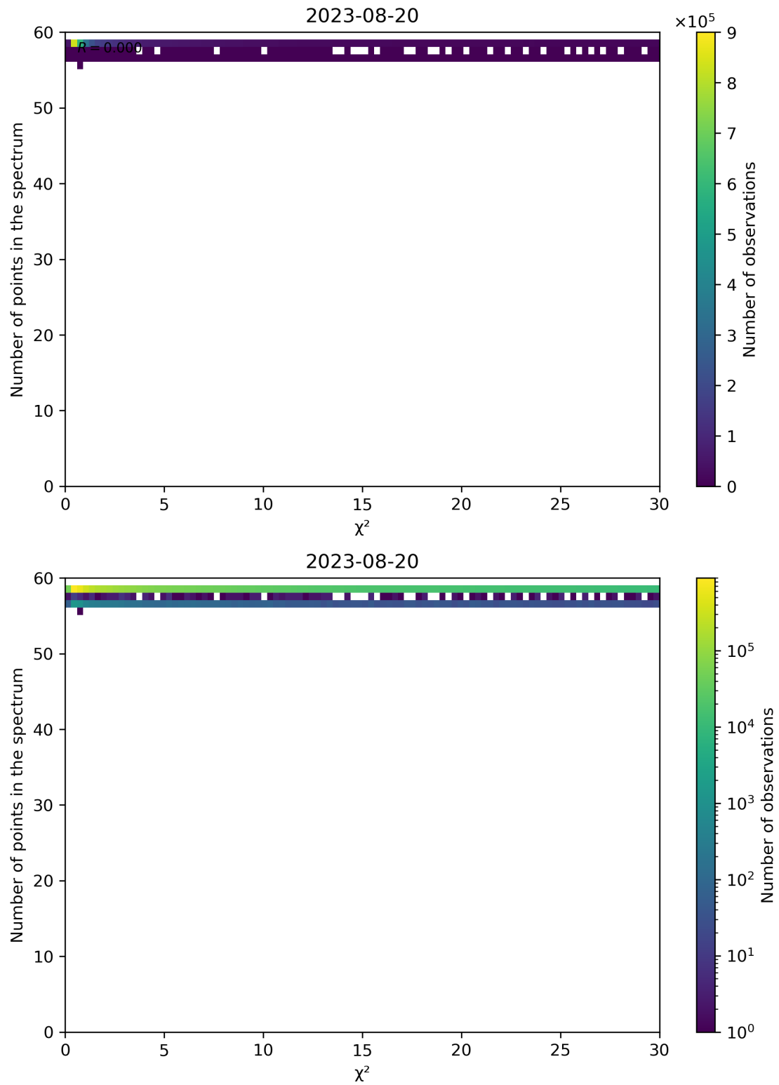
Figure 74: Scatter density plot of " \chi^2 " against "Number of points in the spectrum" for 2023-08-20 to 2023-08-21.
