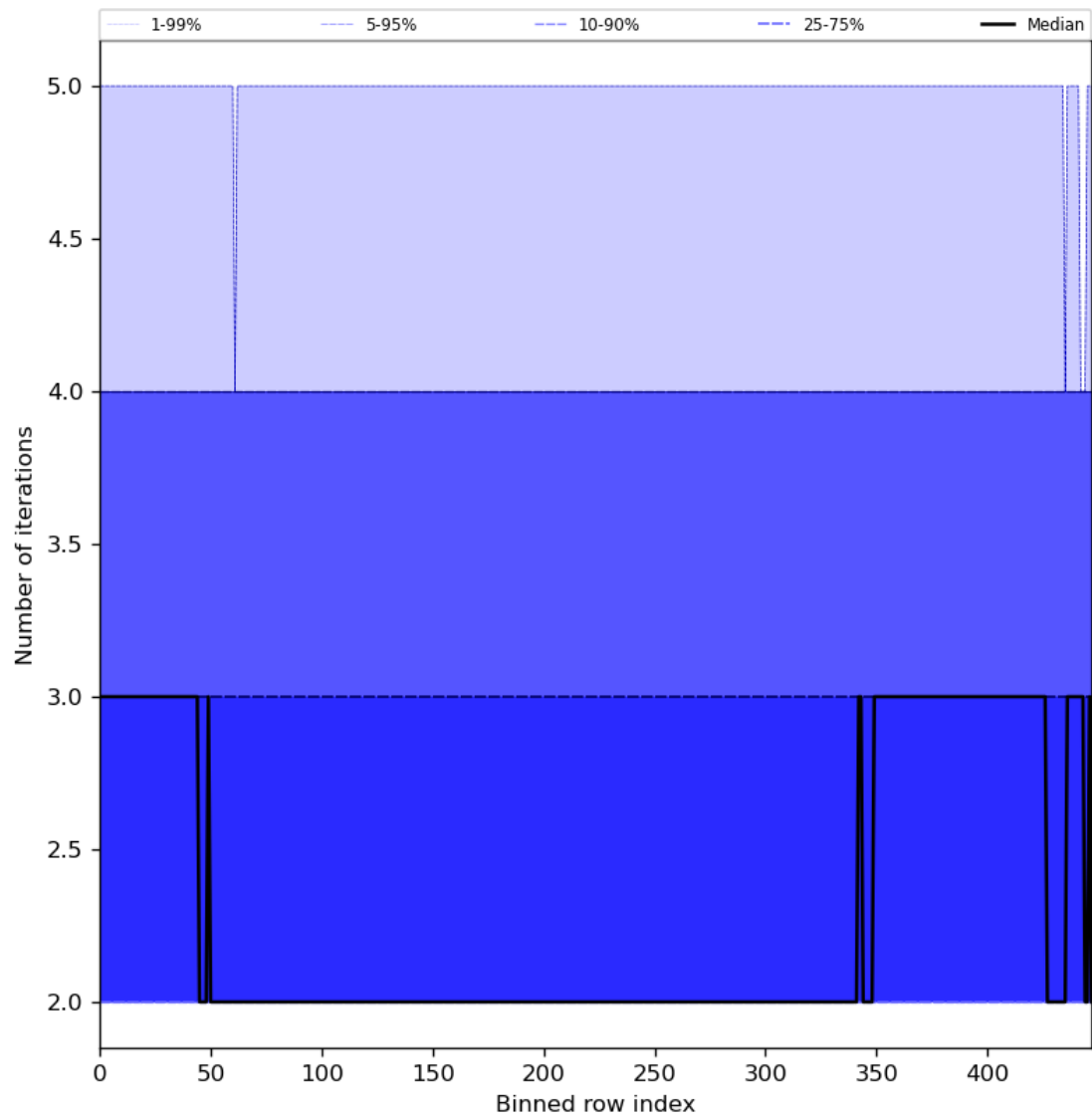
Figure 56: Along track statistics of “Number of iterations” for 2023-08-20 to 2023-08-21
