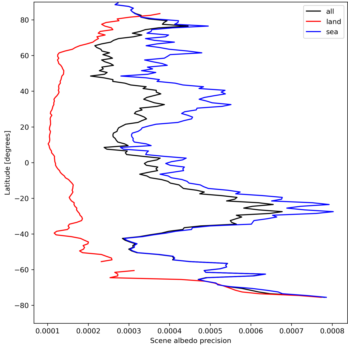
Figure 18: Zonal average of “Scene albedo precision” for 2023-08-20 to 2023-08-21.
