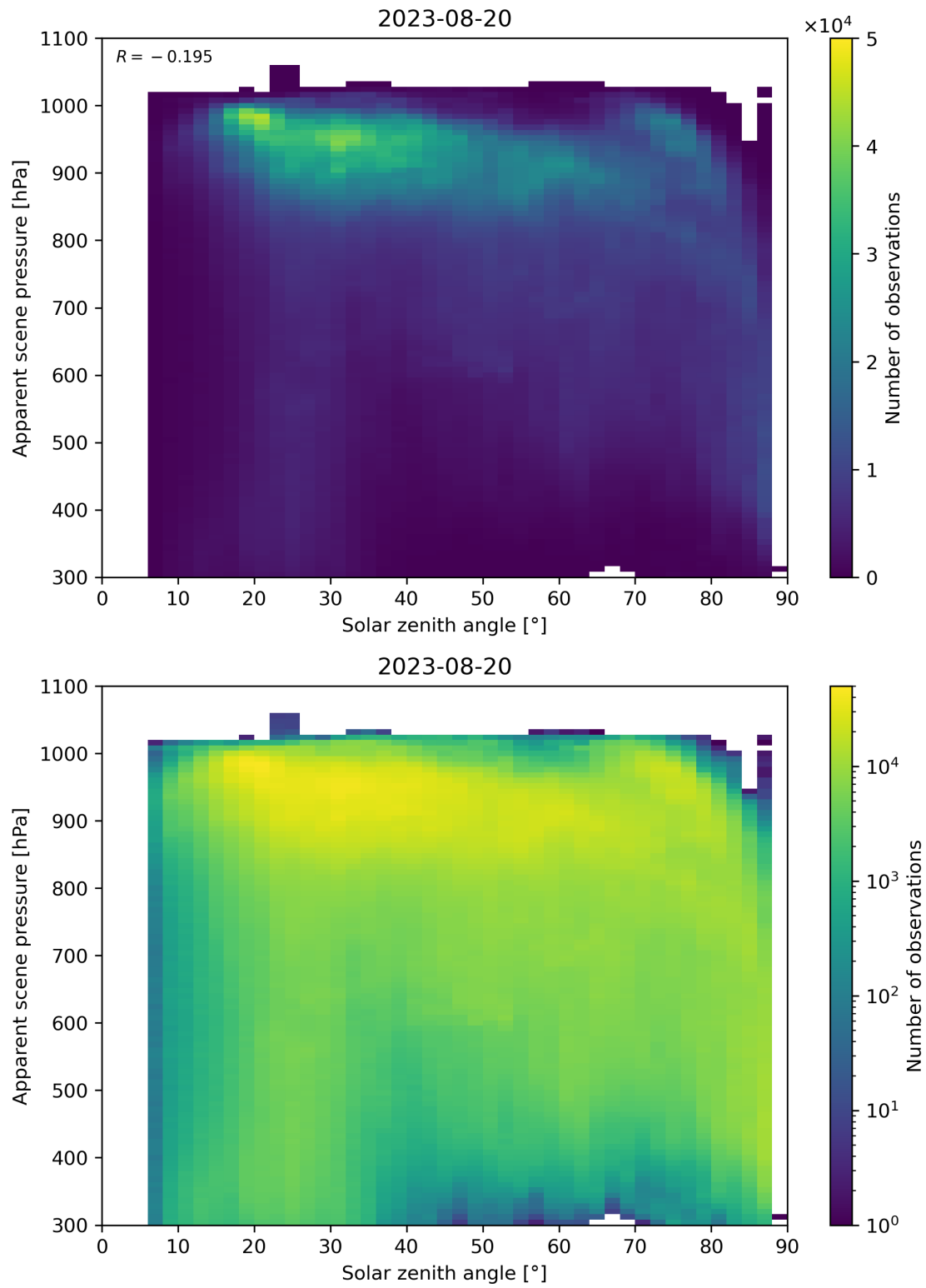
Figure 118: Scatter density plot of “Solar zenith angle” against “Apparent scene pressure” for 2023-08-20 to 2023-08-21.
