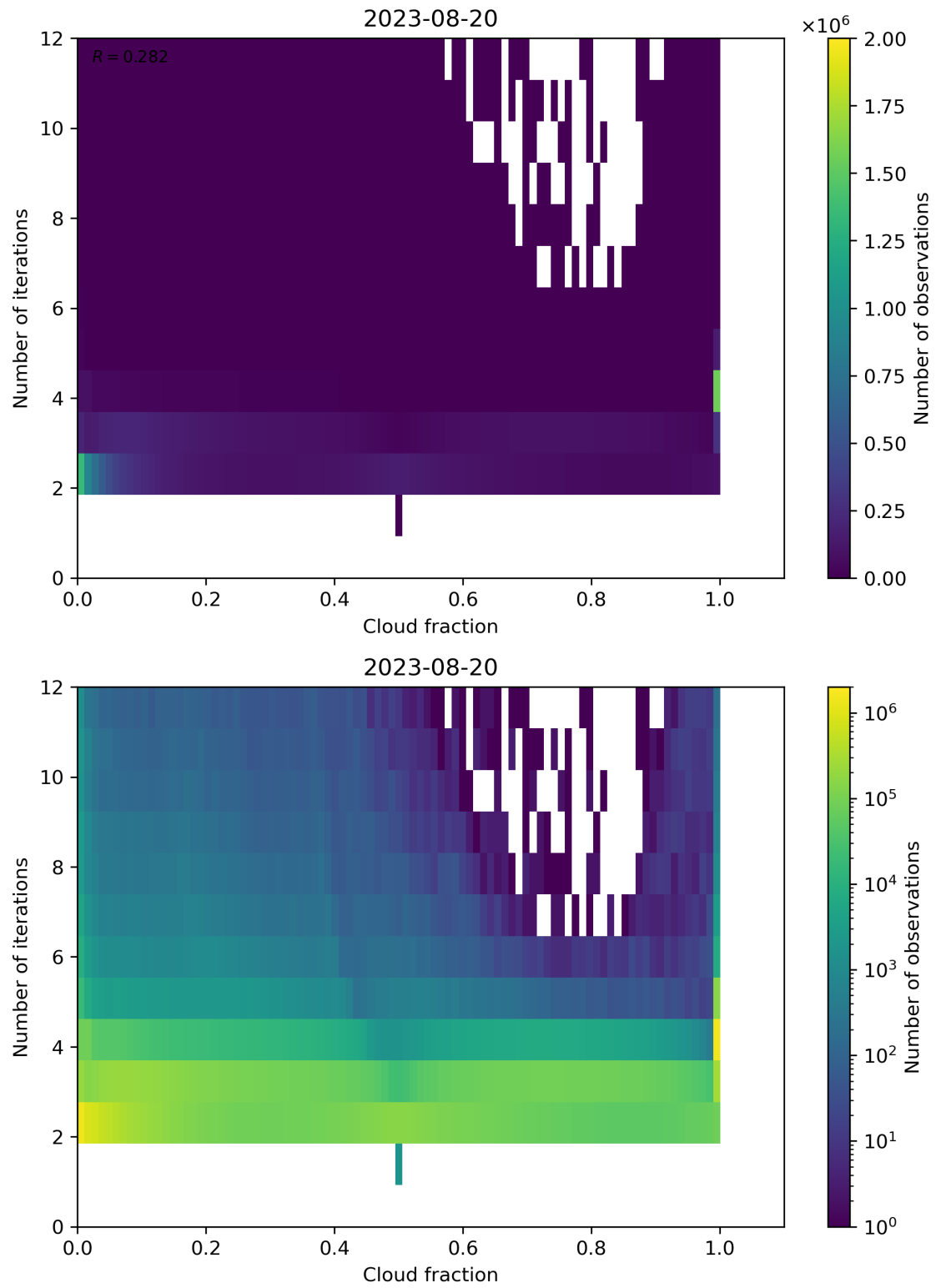
Figure 80: Scatter density plot of “Cloud fraction” against “Number of iterations” for 2023-08-20 to 2023-08-21.
