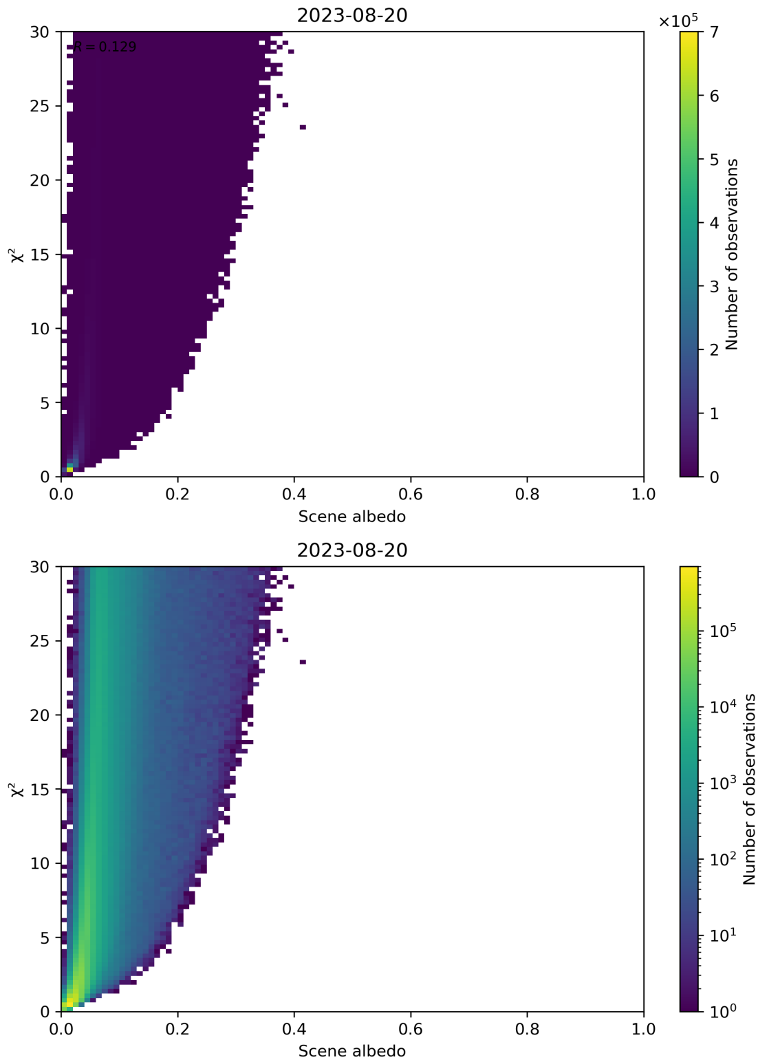
Figure 112: Scatter density plot of “Scene albedo” against “ \chi^2 ” for 2023-08-20 to 2023-08-21.
