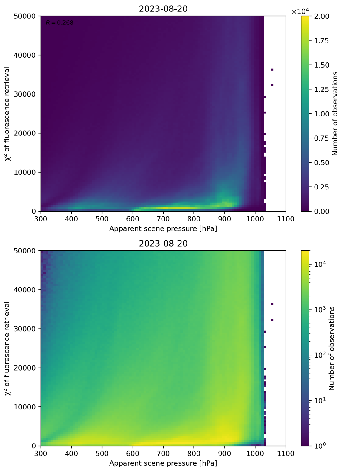
Figure 64: Scatter density plot of “Apparent scene pressure” against “ \chi^2 of fluorescence retrieval” for 2023-08-20 to 2023-08-21.
