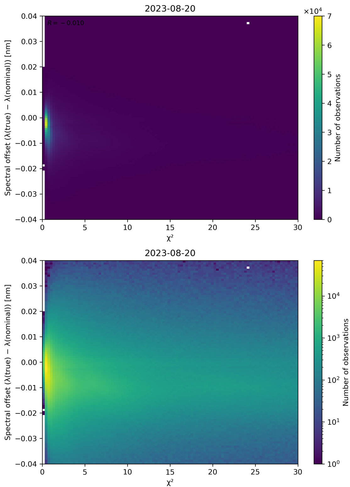
Figure 75: Scatter density plot of “ \chi^2 ” against “Spectral offset ( \lambda(\text{true}) - \lambda(\text{nominal}) )” for 2023-08-20 to 2023-08-21.
