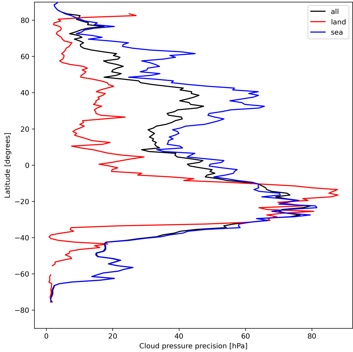
Figure 14: Zonal average of “Cloud pressure precision” for 2023-08-20 to 2023-08-21.
