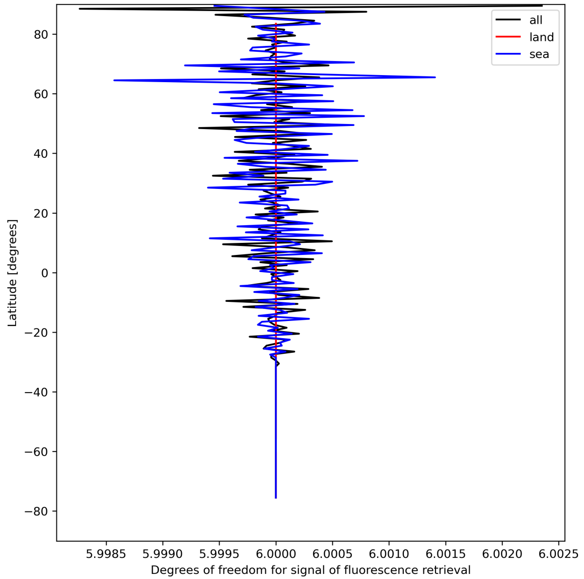
Figure 26: Zonal average of “Degrees of freedom for signal of fluorescence retrieval” for 2023-08-20 to 2023-08-21.
