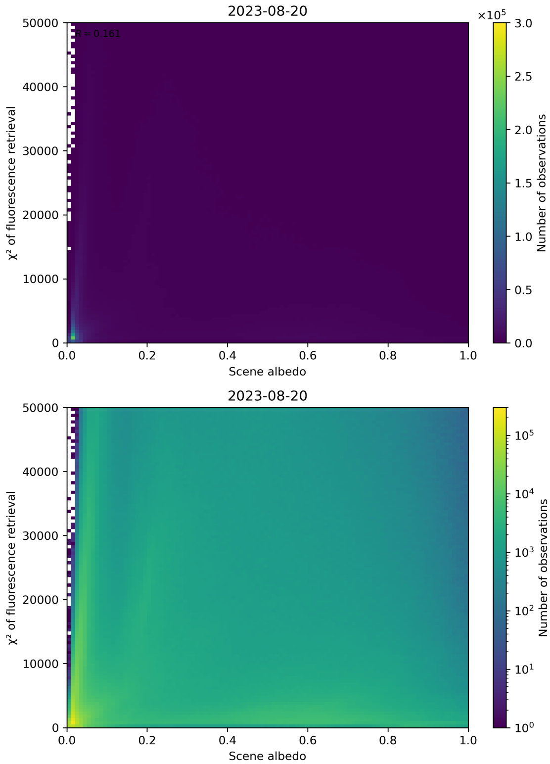
Figure 113: Scatter density plot of “Scene albedo” against “ \chi^2 of fluorescence retrieval” for 2023-08-20 to 2023-08-21.
