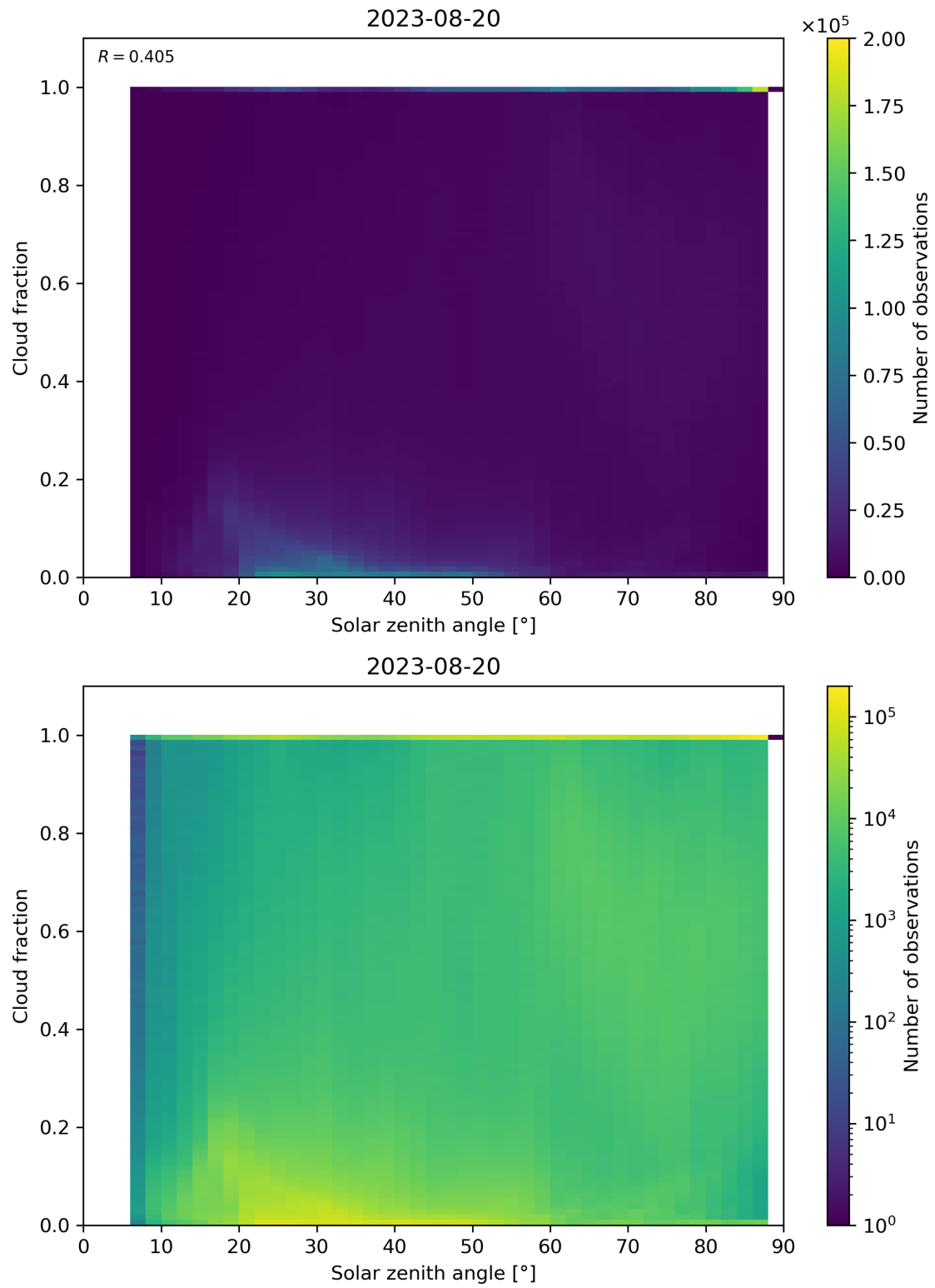
Figure 121: Scatter density plot of “Solar zenith angle” against “Cloud fraction” for 2023-08-20 to 2023-08-21.
