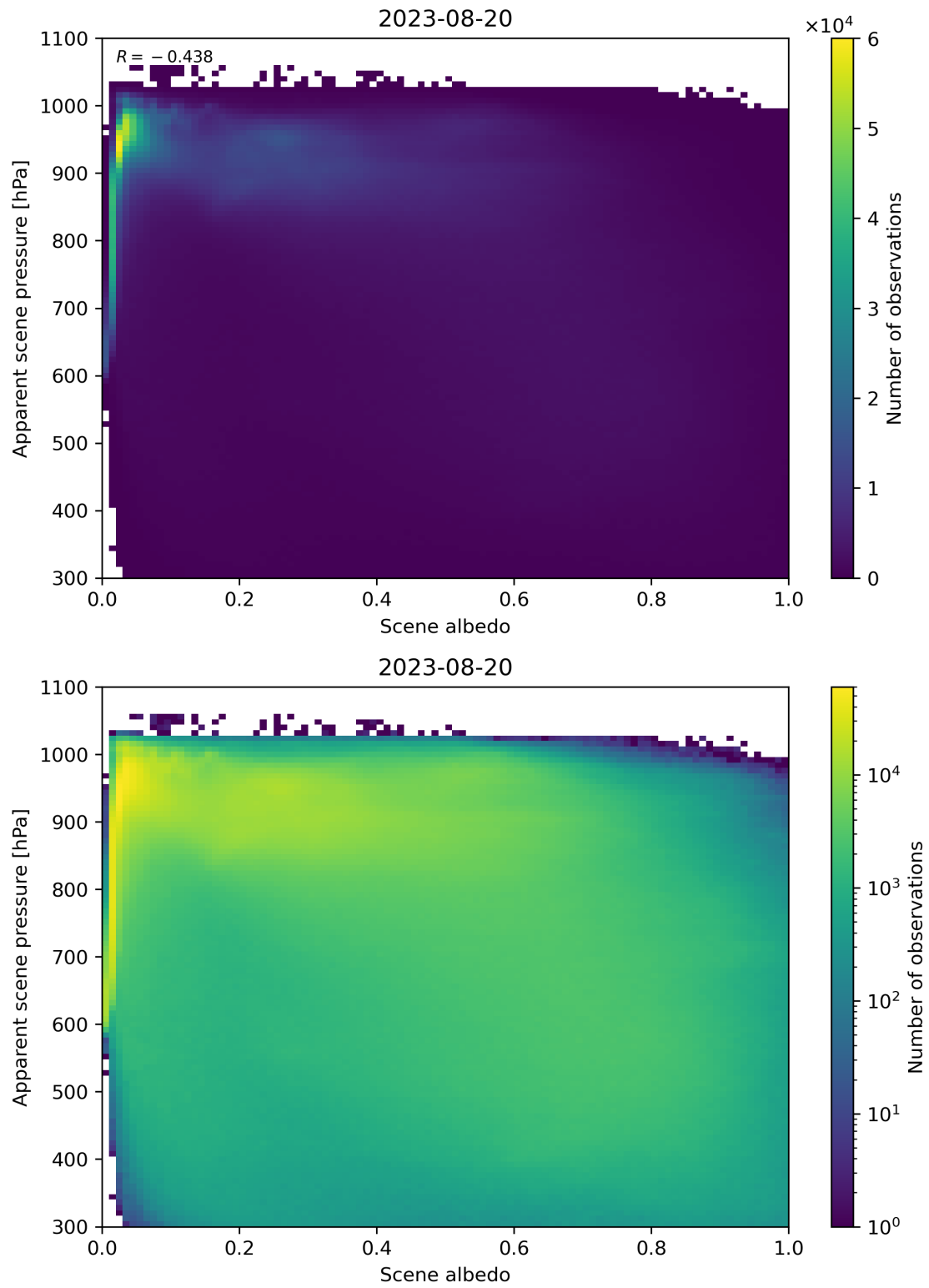
Figure 111: Scatter density plot of “Scene albedo” against “Apparent scene pressure” for 2023-08-20 to 2023-08-21.
