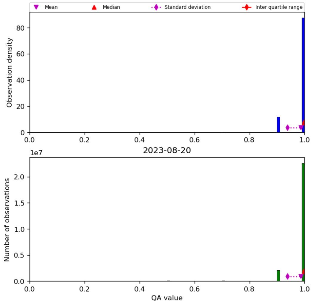
Figure 29: Histogram of “QA value” for 2023-08-20 to 2023-08-21
