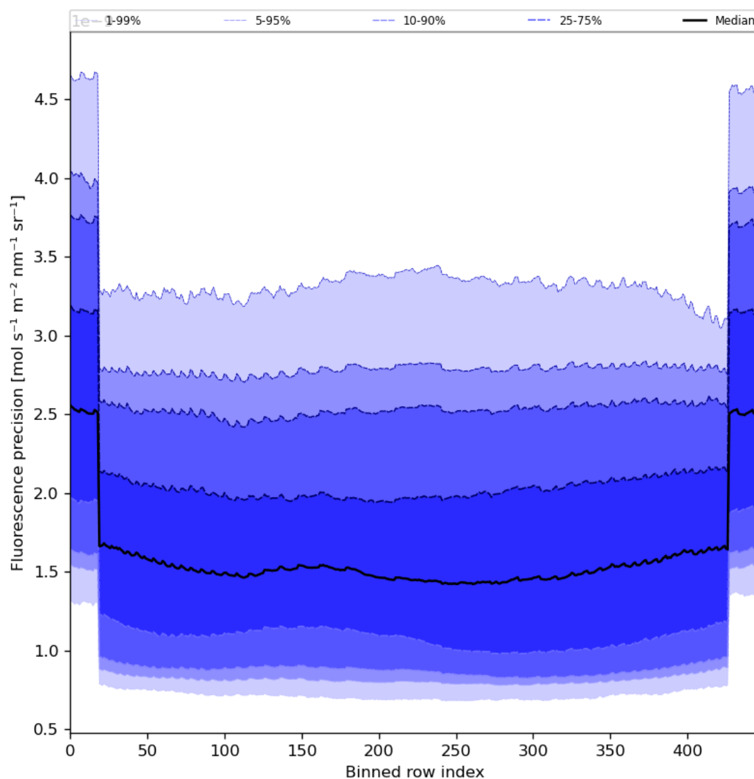
Figure 58: Along track statistics of “Fluorescence precision” for 2023-08-20 to 2023-08-21
