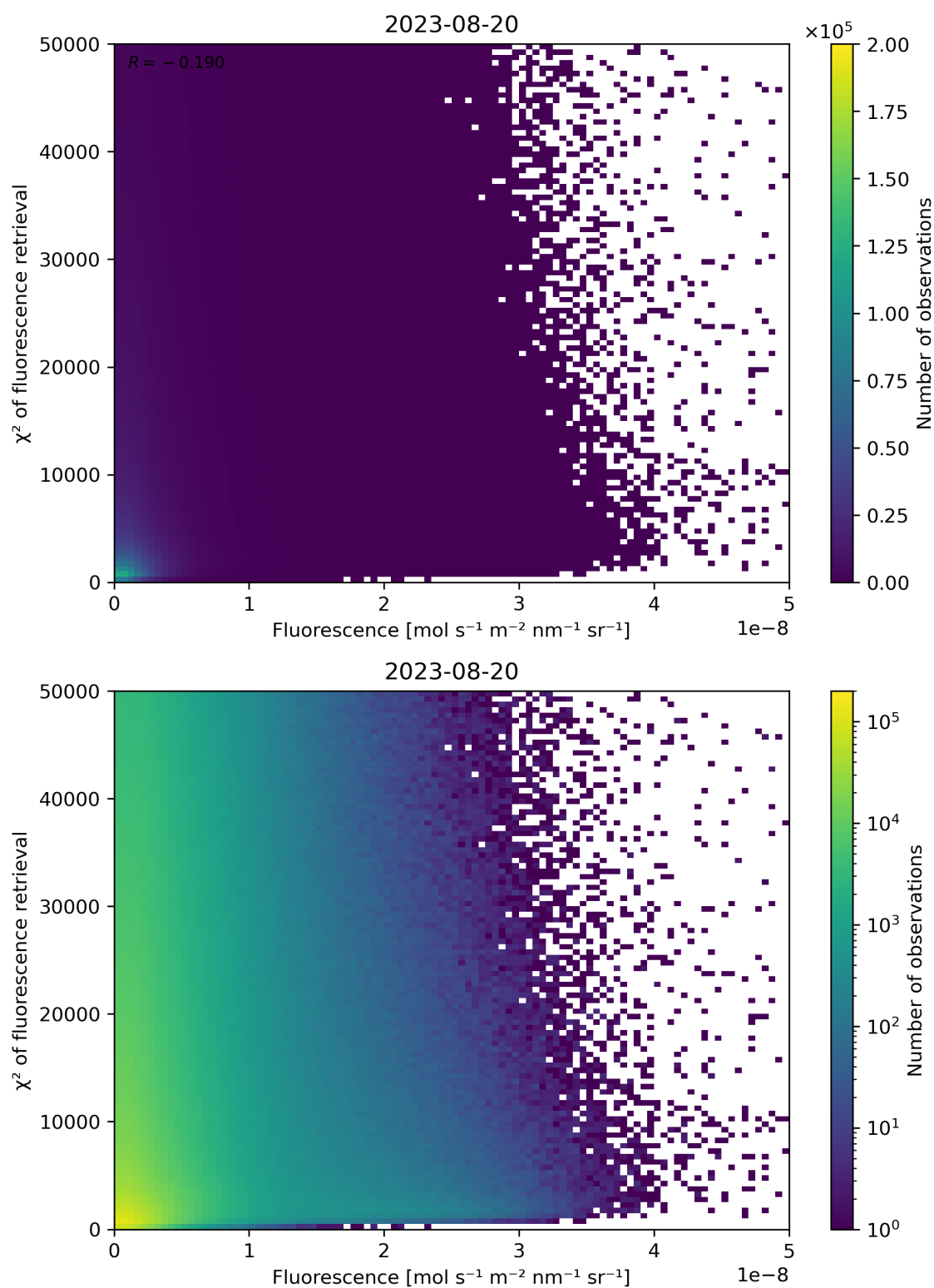
Figure 93: Scatter density plot of “Fluorescence” against “ \chi^2 of fluorescence retrieval” for 2023-08-20 to 2023-08-21.
