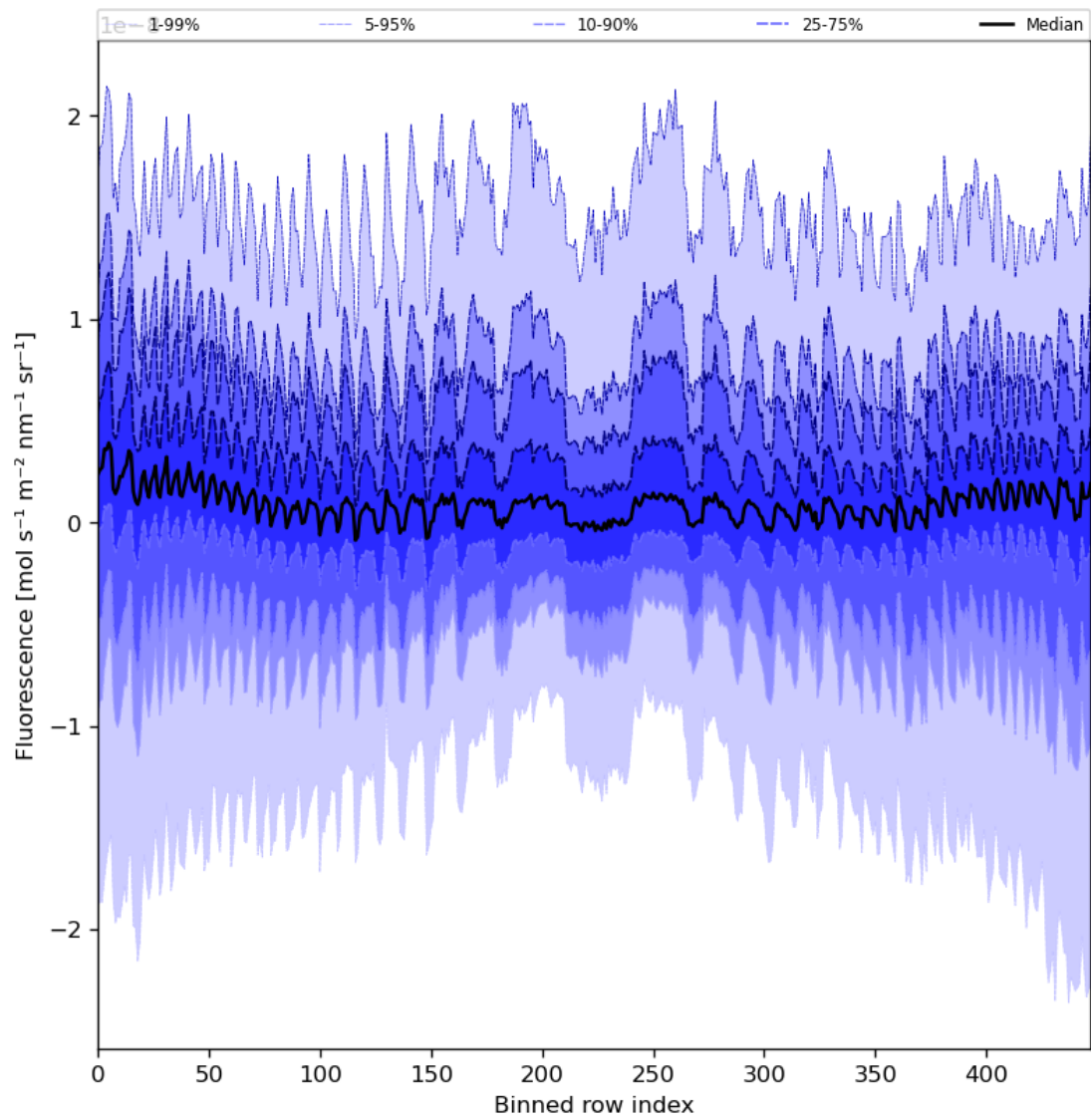
Figure 57: Along track statistics of “Fluorescence” for 2023-08-20 to 2023-08-21
