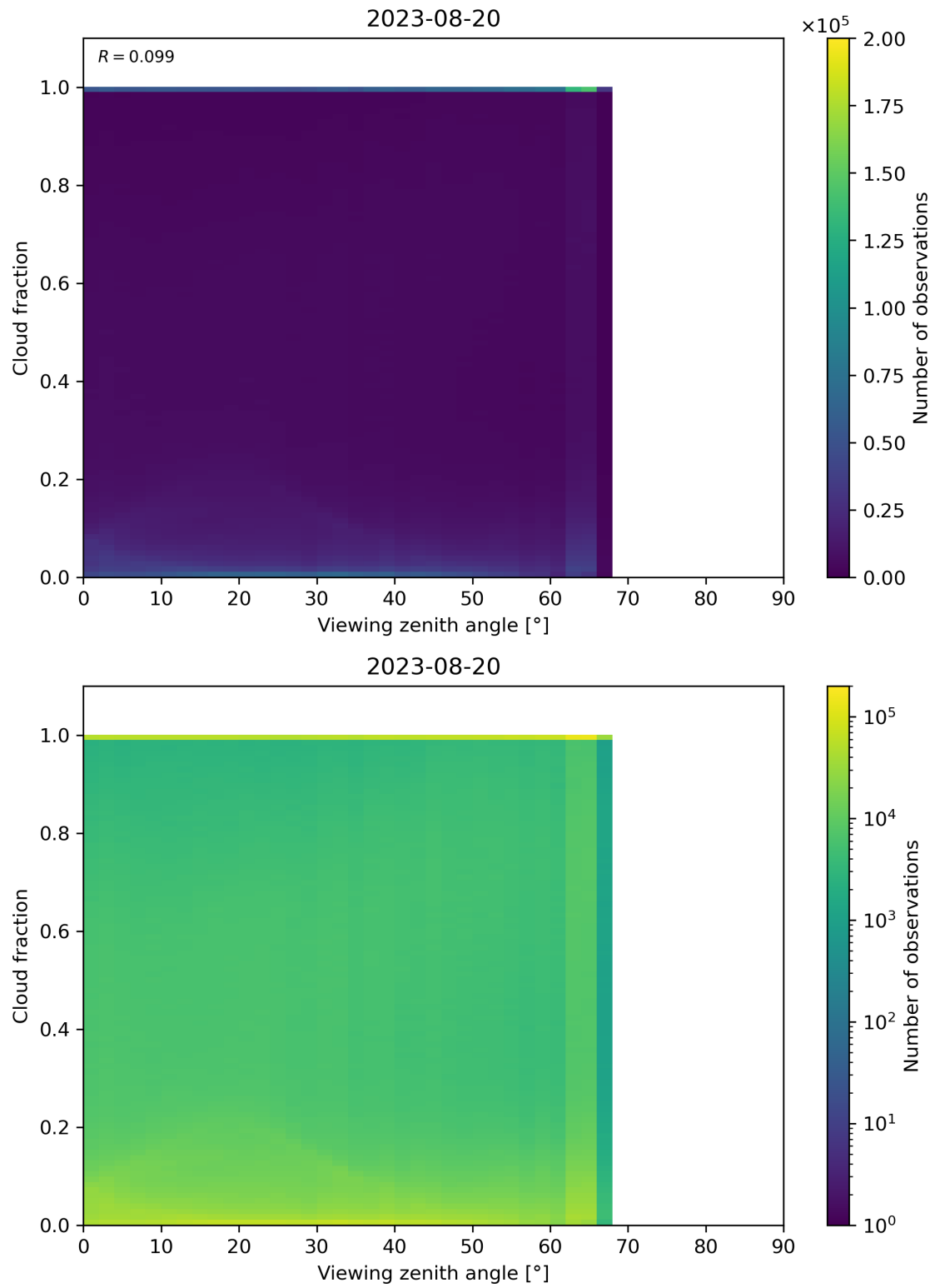
Figure 132: Scatter density plot of “Viewing zenith angle” against “Cloud fraction” for 2023-08-20 to 2023-08-21.
