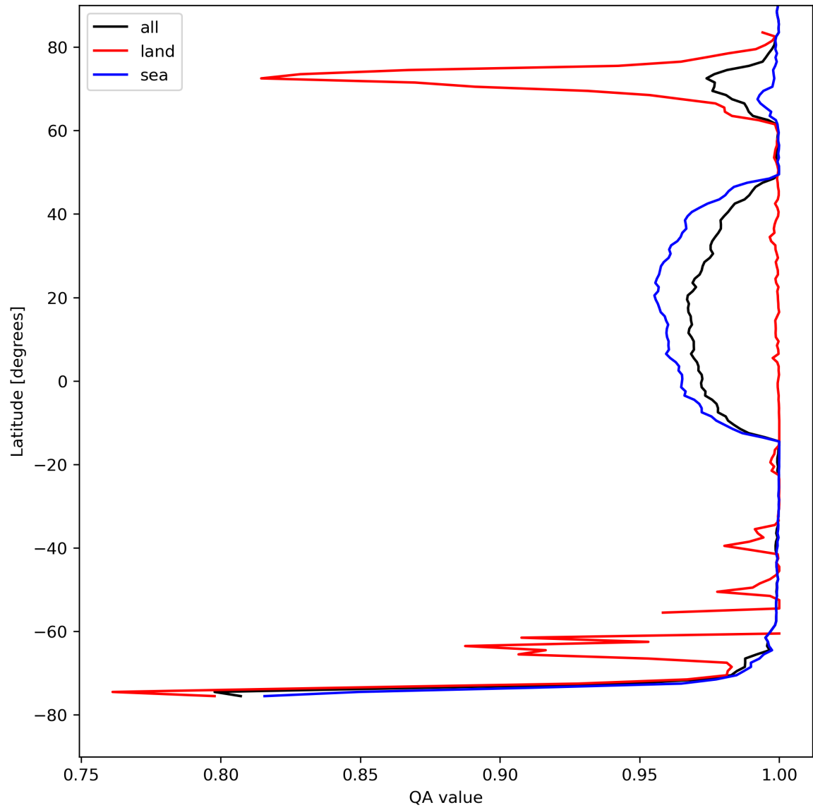
Figure 12: Zonal average of “QA value” for 2023-08-20 to 2023-08-21.
