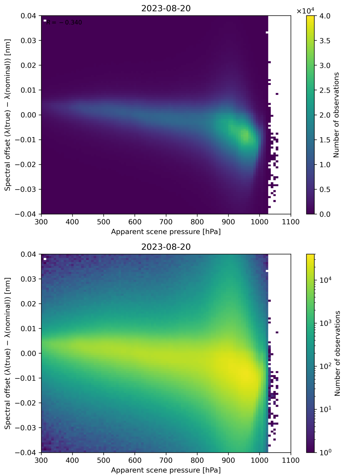
Figure 68: Scatter density plot of “Apparent scene pressure” against “Spectral offset ( \lambda(\text{true}) - \lambda(\text{nominal}) )” for 2023-08-20 to 2023-08-21.
