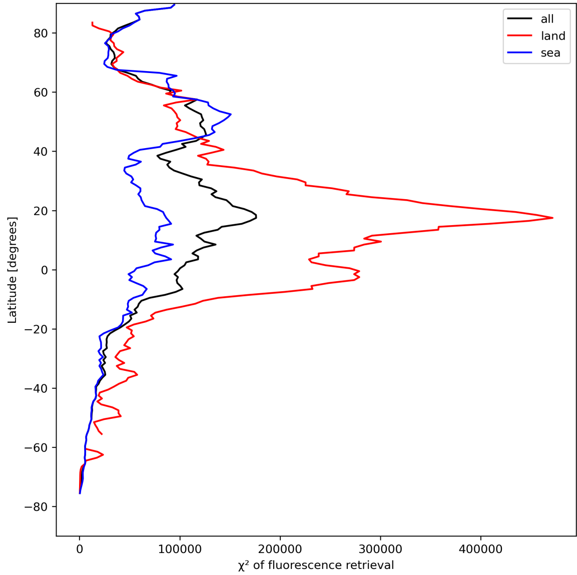
Figure 25: Zonal average of “ \chi^2 of fluorescence retrieval” for 2023-08-20 to 2023-08-21.
