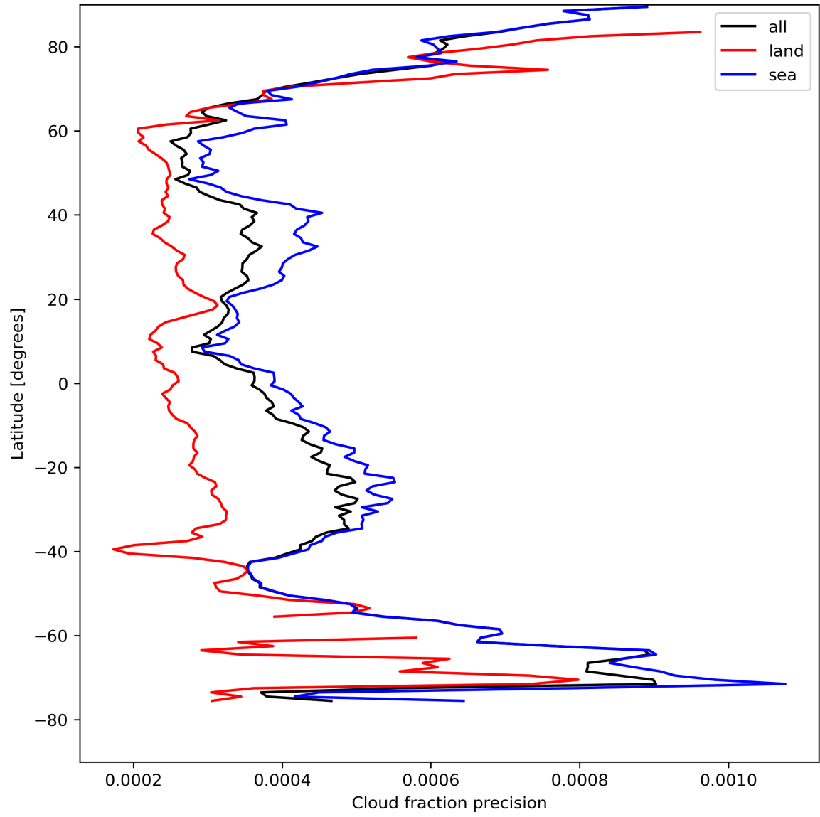
Figure 16: Zonal average of “Cloud fraction precision” for 2023-08-20 to 2023-08-21.
