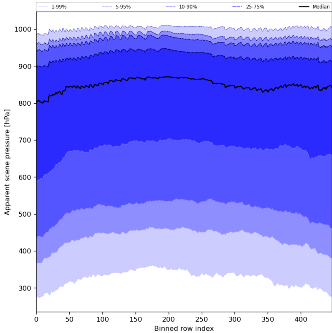
Figure 53: Along track statistics of “Apparent scene pressure” for 2023-08-20 to 2023-08-21
