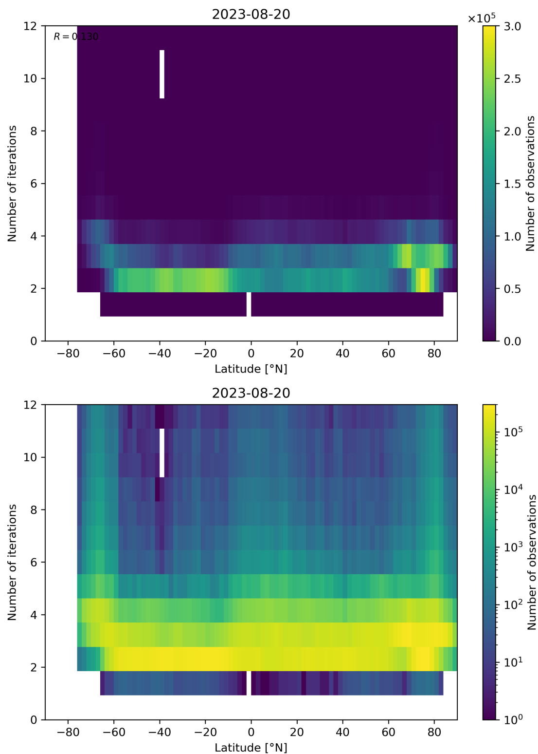
Figure 102: Scatter density plot of “Latitude” against “Number of iterations” for 2023-08-20 to 2023-08-21.
