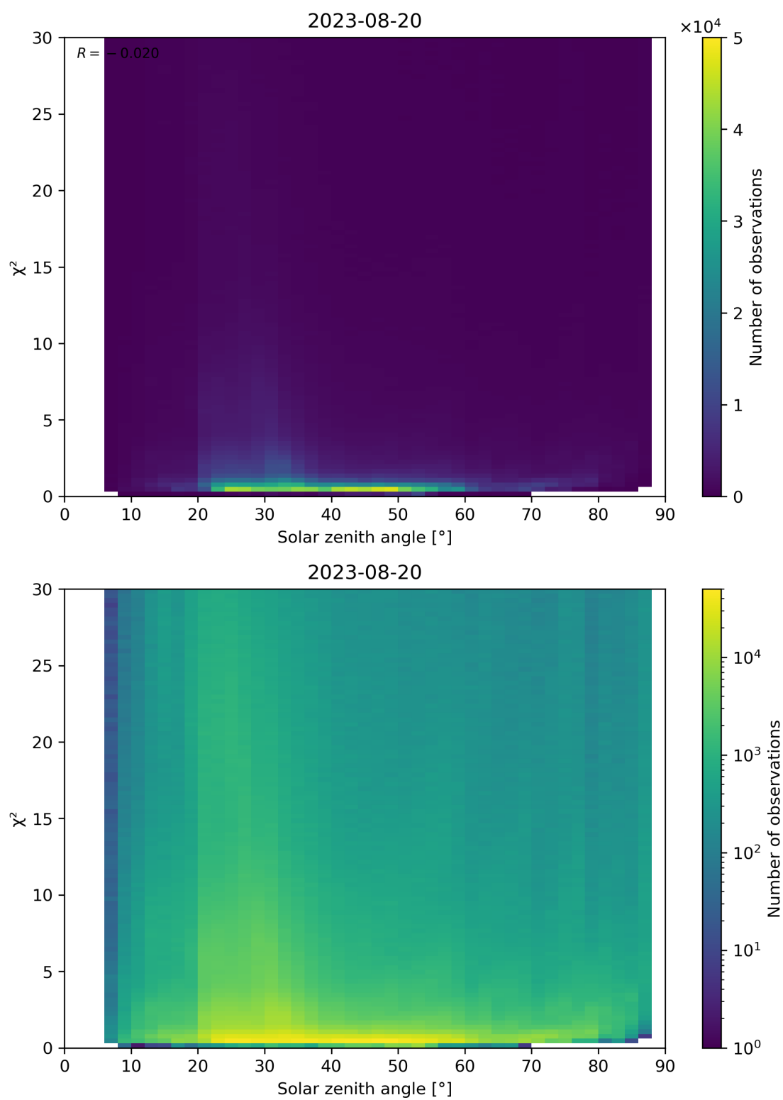
Figure 119: Scatter density plot of “Solar zenith angle” against “ \chi^2 ” for 2023-08-20 to 2023-08-21.
