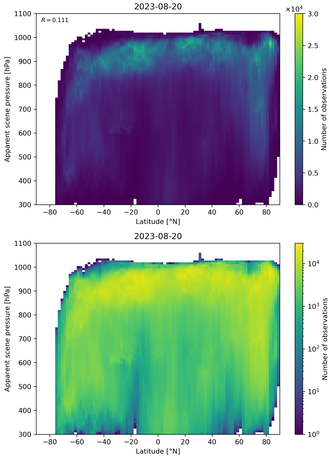
Figure 96: Scatter density plot of “Latitude” against “Apparent scene pressure” for 2023-08-20 to 2023-08-21.
