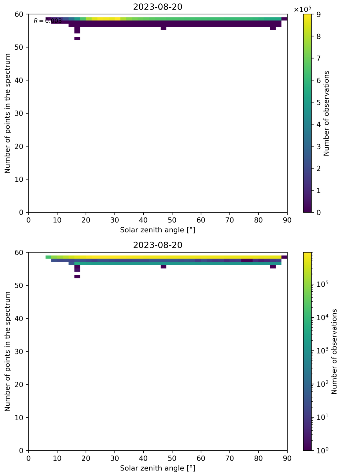
Figure 126: Scatter density plot of “Solar zenith angle” against “Number of points in the spectrum” for 2023-08-20 to 2023-08-21.
