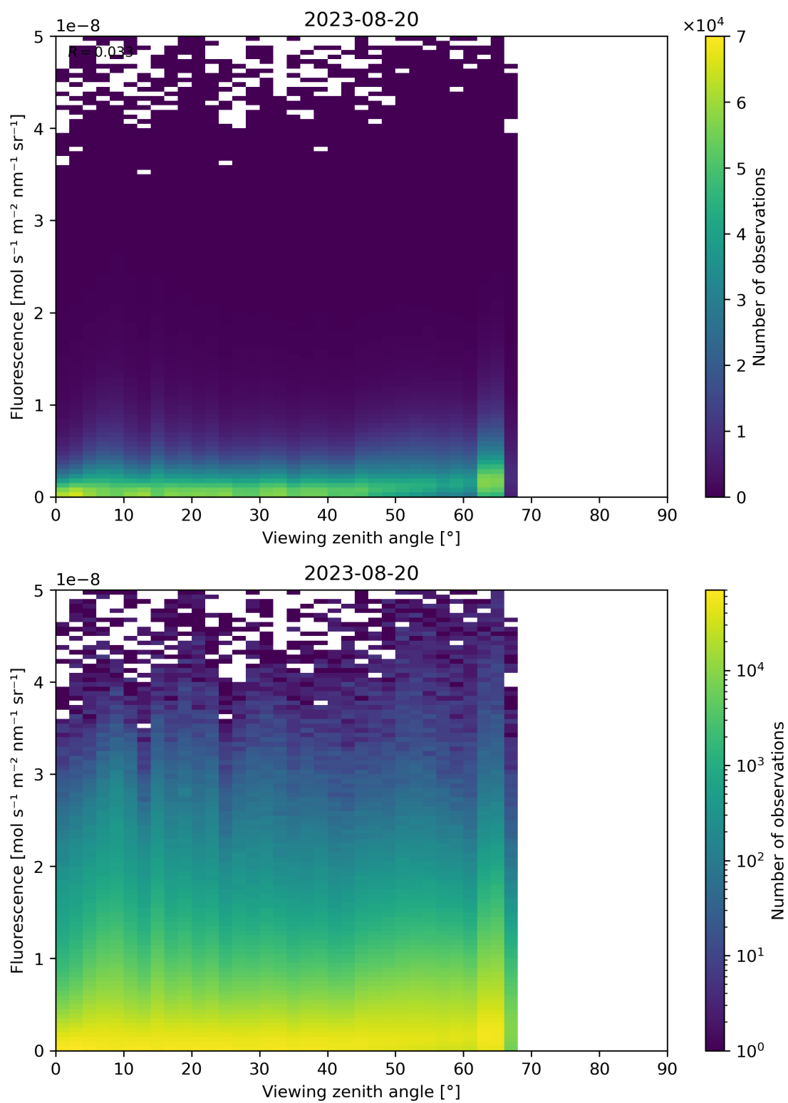
Figure 134: Scatter density plot of “Viewing zenith angle” against “Fluorescence” for 2023-08-20 to 2023-08-21.
