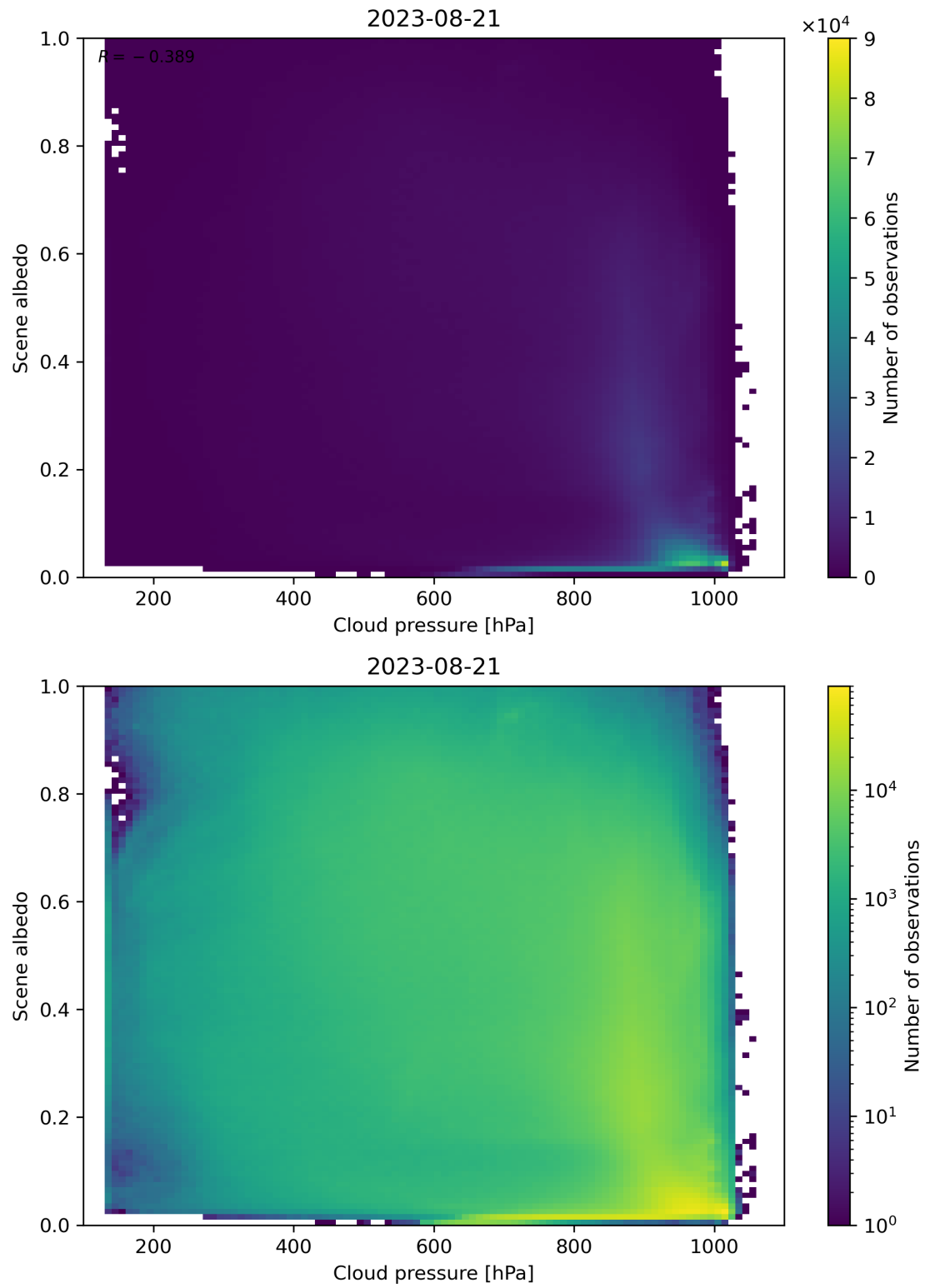
Figure 91: Scatter density plot of “Cloud pressure” against “Scene albedo” for 2023-08-20 to 2023-08-22.
