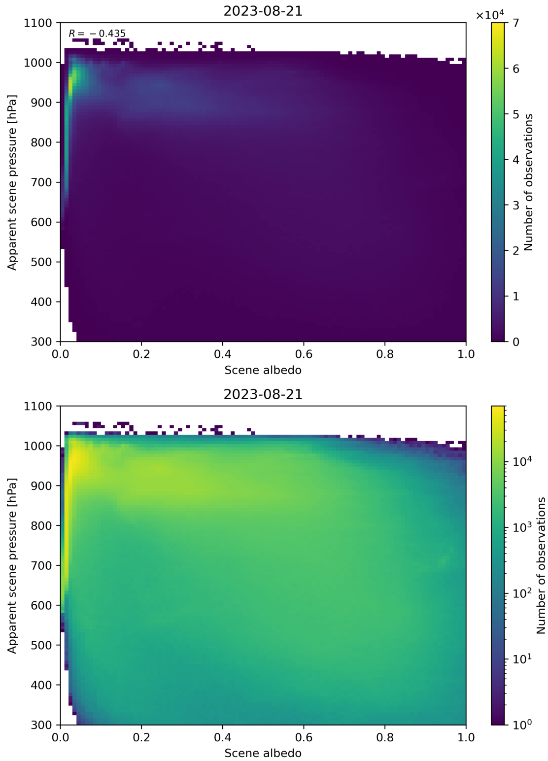
Figure 111: Scatter density plot of “Scene albedo” against “Apparent scene pressure” for 2023-08-20 to 2023-08-22.
