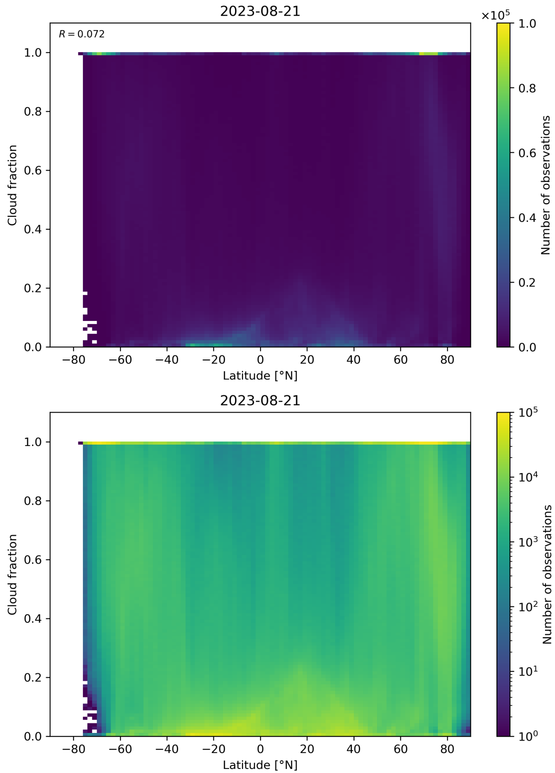
Figure 99: Scatter density plot of “Latitude” against “Cloud fraction” for 2023-08-20 to 2023-08-22.
