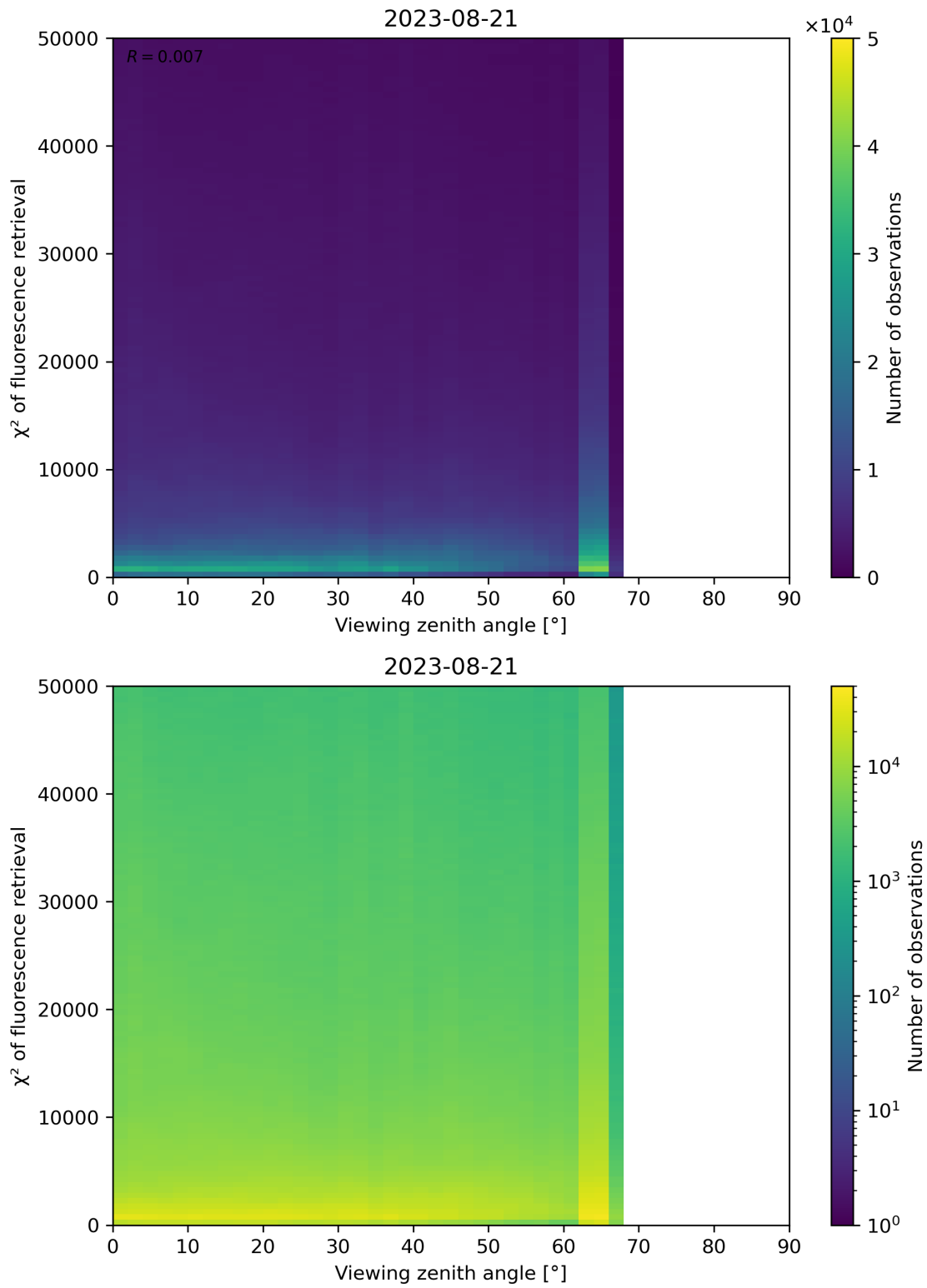
Figure 131: Scatter density plot of “Viewing zenith angle” against “ \chi^2 of fluorescence retrieval” for 2023-08-20 to 2023-08-22.
