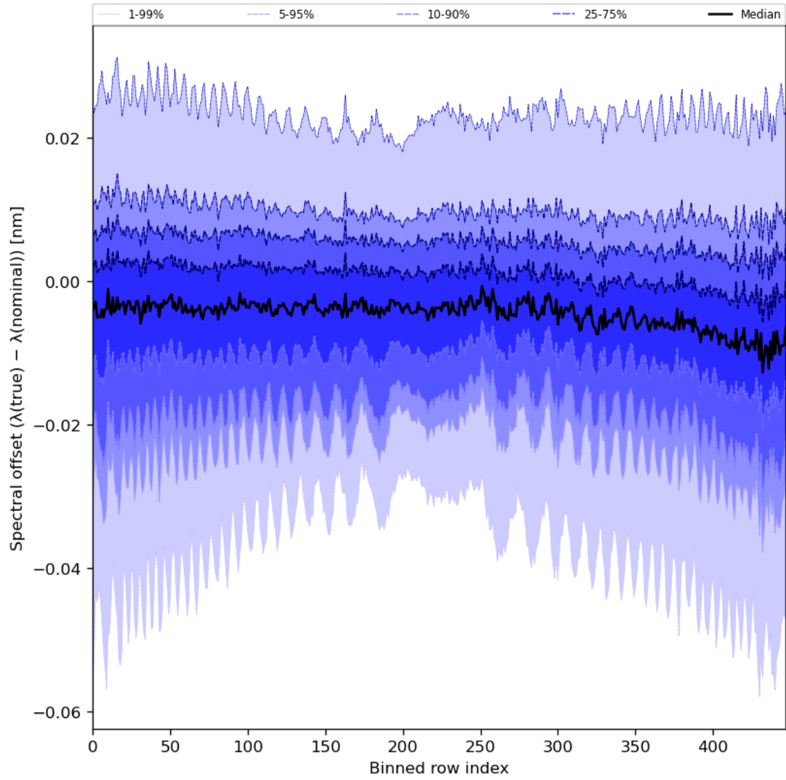
Figure 62: Along track statistics of “Spectral offset ( \lambda(\text{true}) - \lambda(\text{nominal}) )” for 2023-08-20 to 2023-08-22
