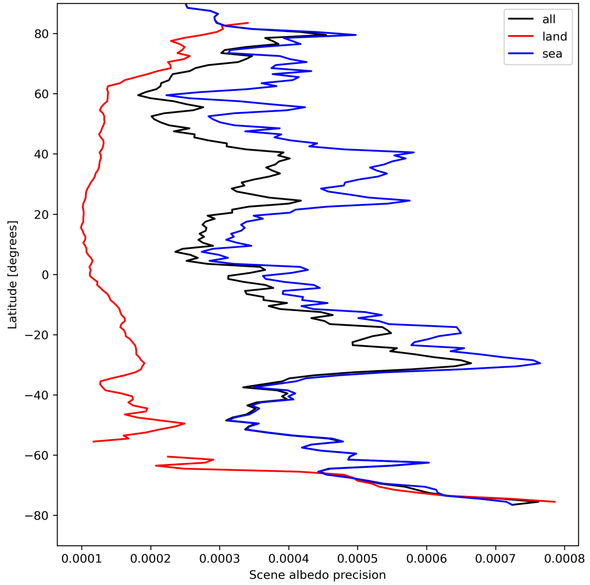
Figure 18: Zonal average of “Scene albedo precision” for 2023-08-20 to 2023-08-22.
