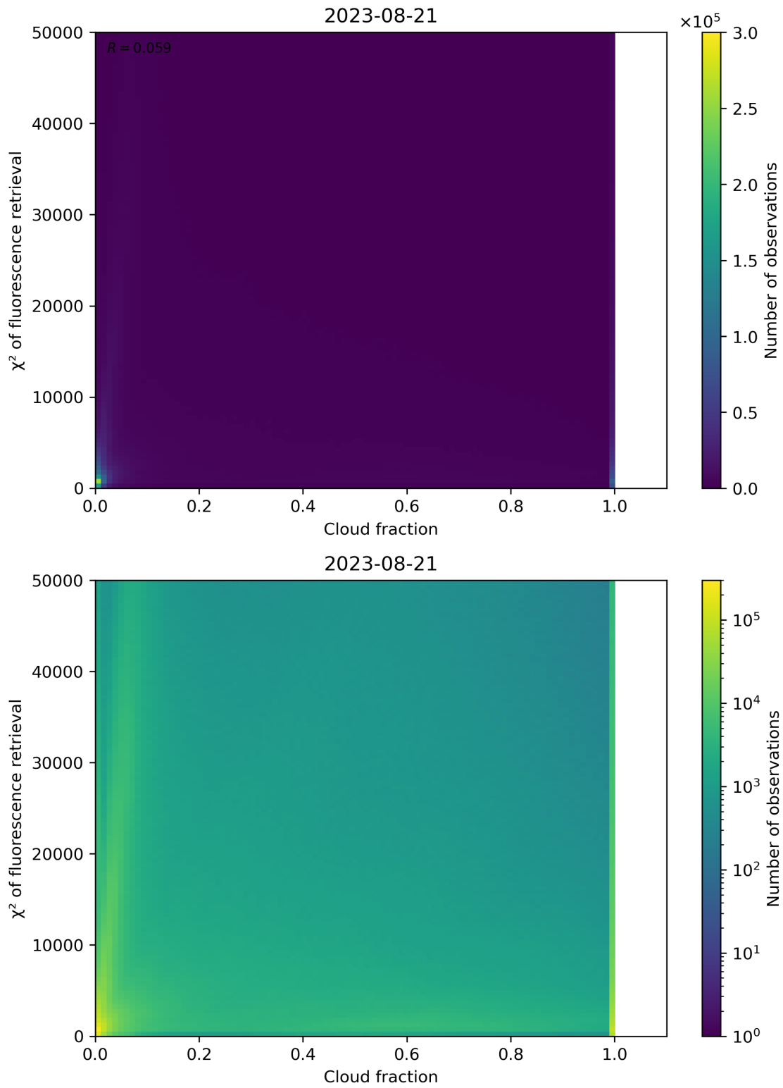
Figure 78: Scatter density plot of “Cloud fraction” against “ \chi^2 of fluorescence retrieval” for 2023-08-20 to 2023-08-22.
