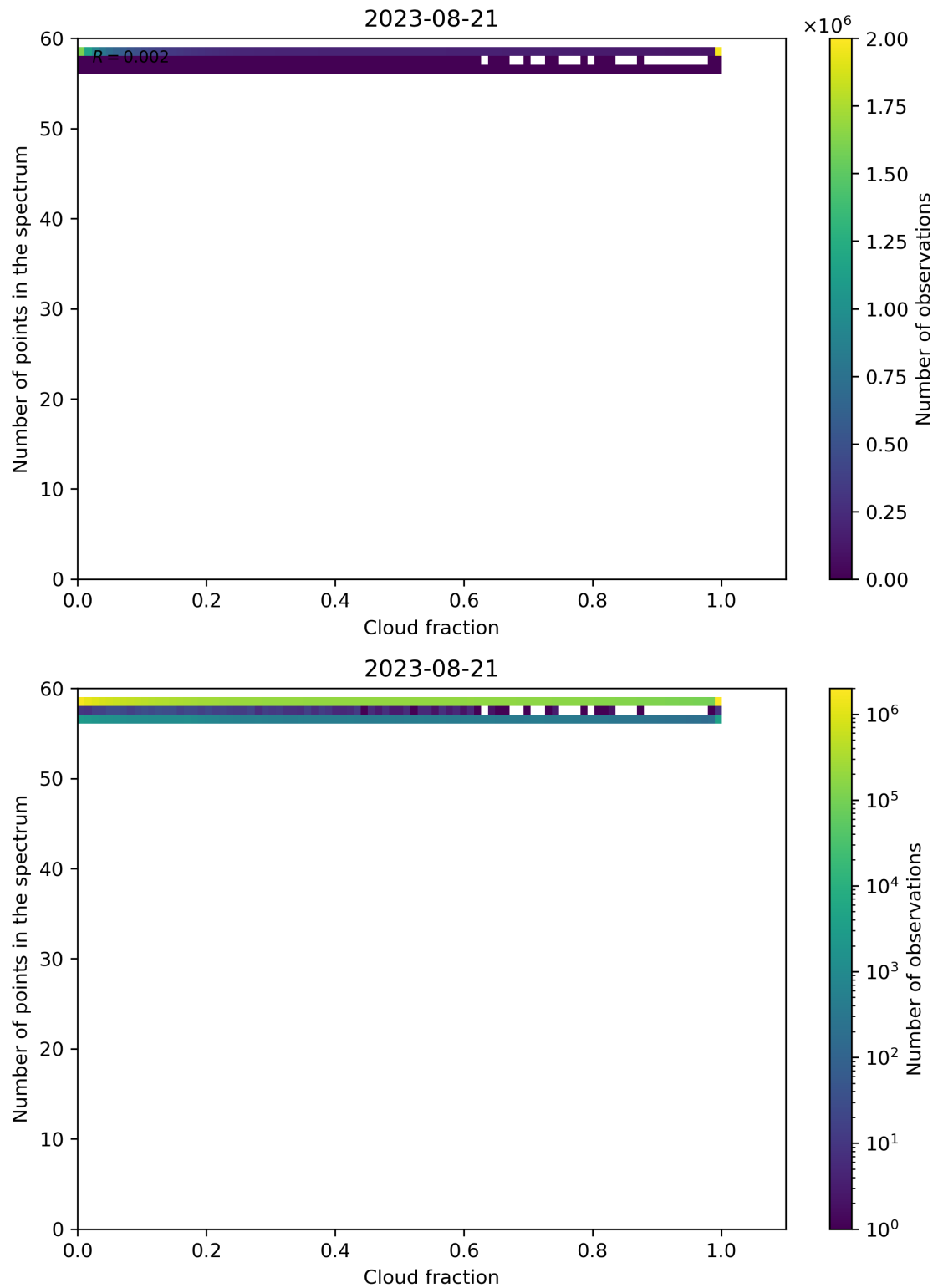
Figure 81: Scatter density plot of “Cloud fraction” against “Number of points in the spectrum” for 2023-08-20 to 2023-08-22.
