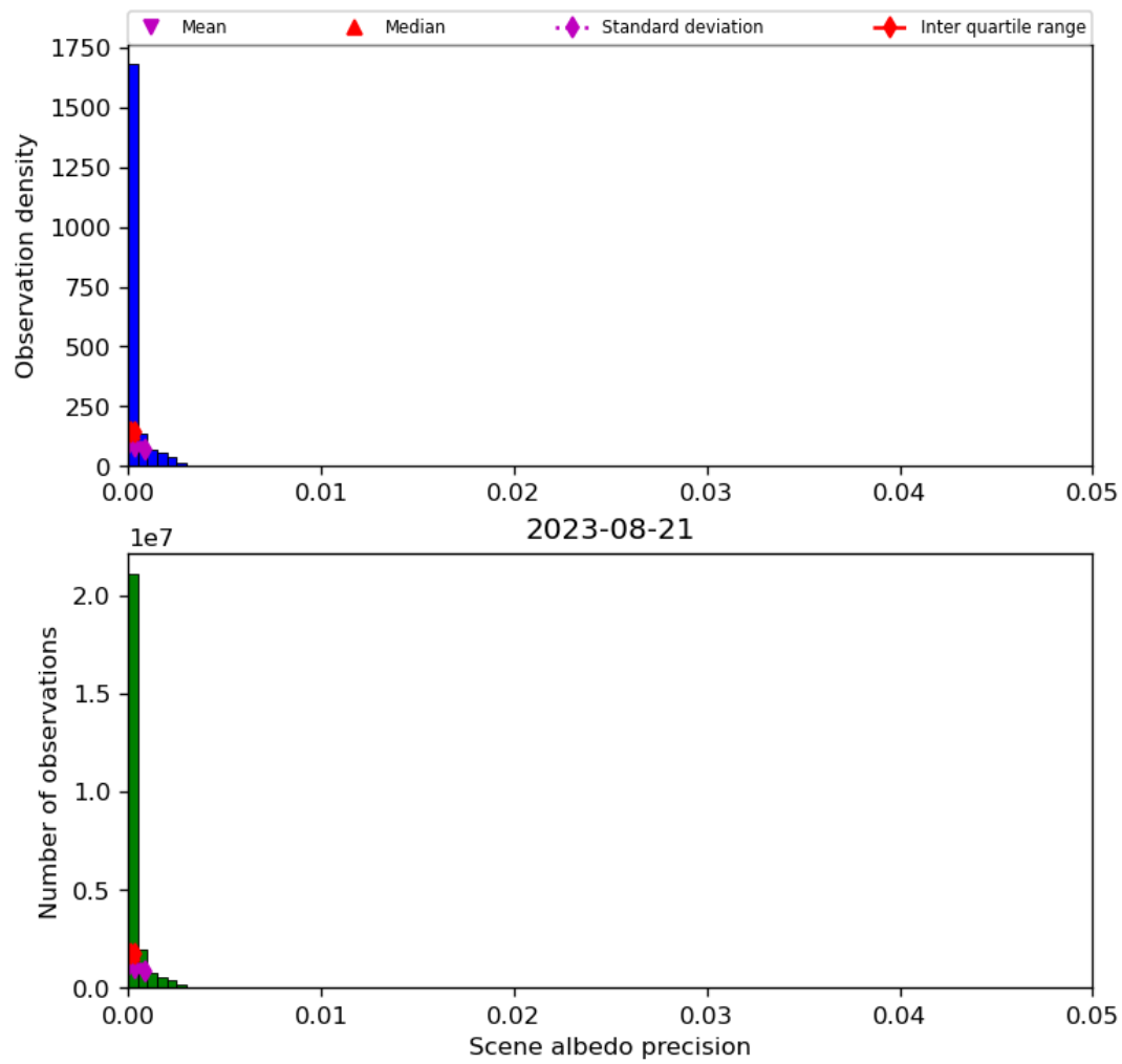
Figure 35: Histogram of “Scene albedo precision” for 2023-08-20 to 2023-08-22
