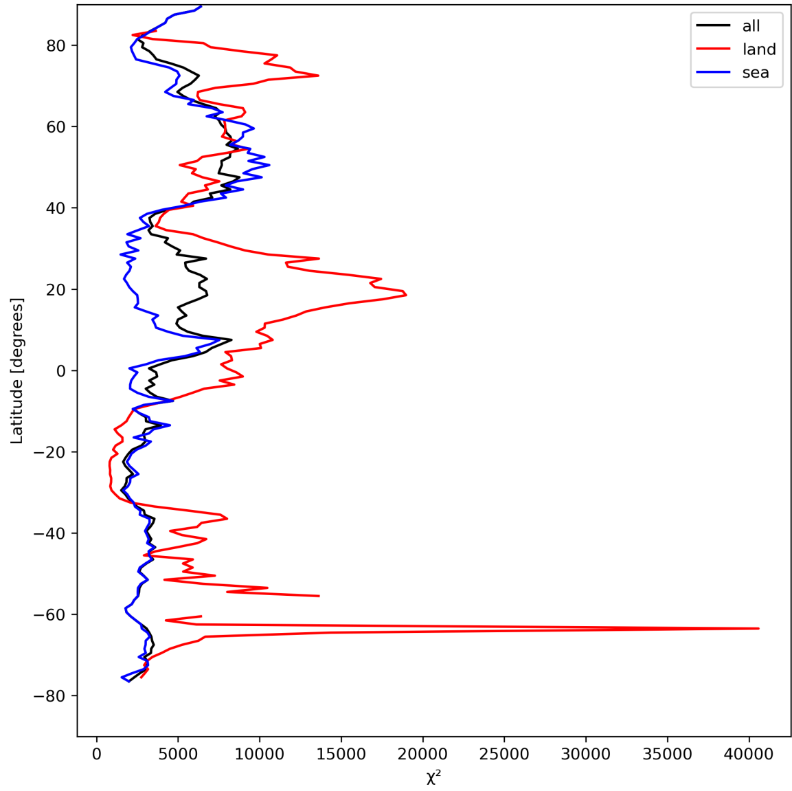
Figure 21: Zonal average of “ \chi^2 ” for 2023-08-20 to 2023-08-22.
