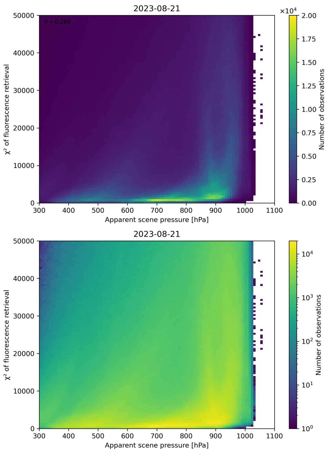
Figure 64: Scatter density plot of “Apparent scene pressure” against “ \chi^2 of fluorescence retrieval” for 2023-08-20 to 2023-08-22.
