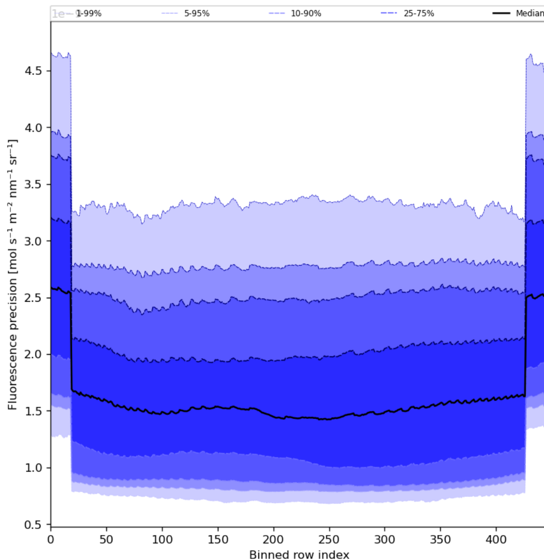
Figure 58: Along track statistics of “Fluorescence precision” for 2023-08-20 to 2023-08-22
