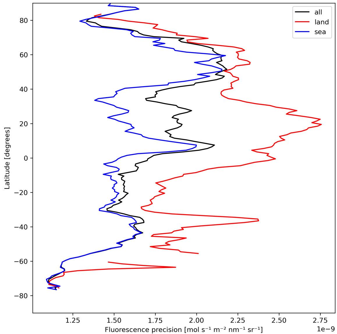
Figure 24: Zonal average of “Fluorescence precision” for 2023-08-20 to 2023-08-22.
