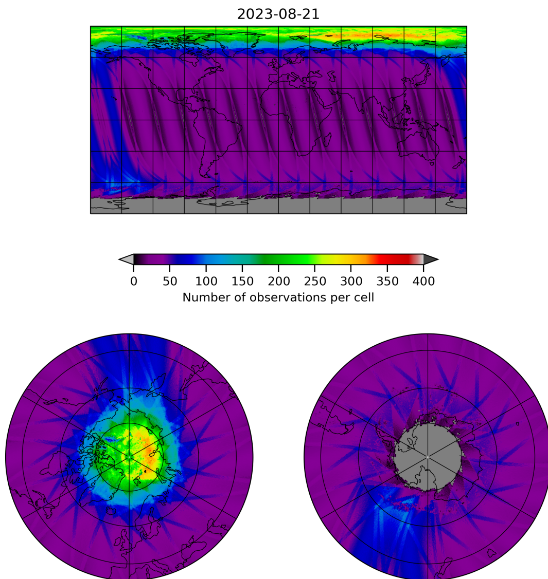
Figure 11: Map of the number of observations for 2023-08-20 to 2023-08-22
