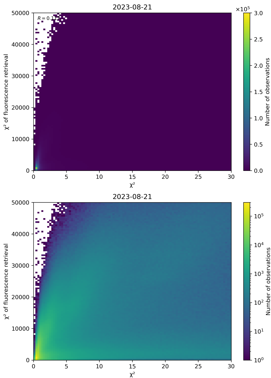
Figure 69: Scatter density plot of “ \chi^2 ” against “ \chi^2 of fluorescence retrieval” for 2023-08-20 to 2023-08-22.
