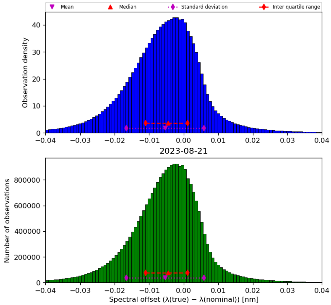
Figure 45: Histogram of “Spectral offset ( \lambda(\text{true}) - \lambda(\text{nominal}) )” for 2023-08-20 to 2023-08-22
