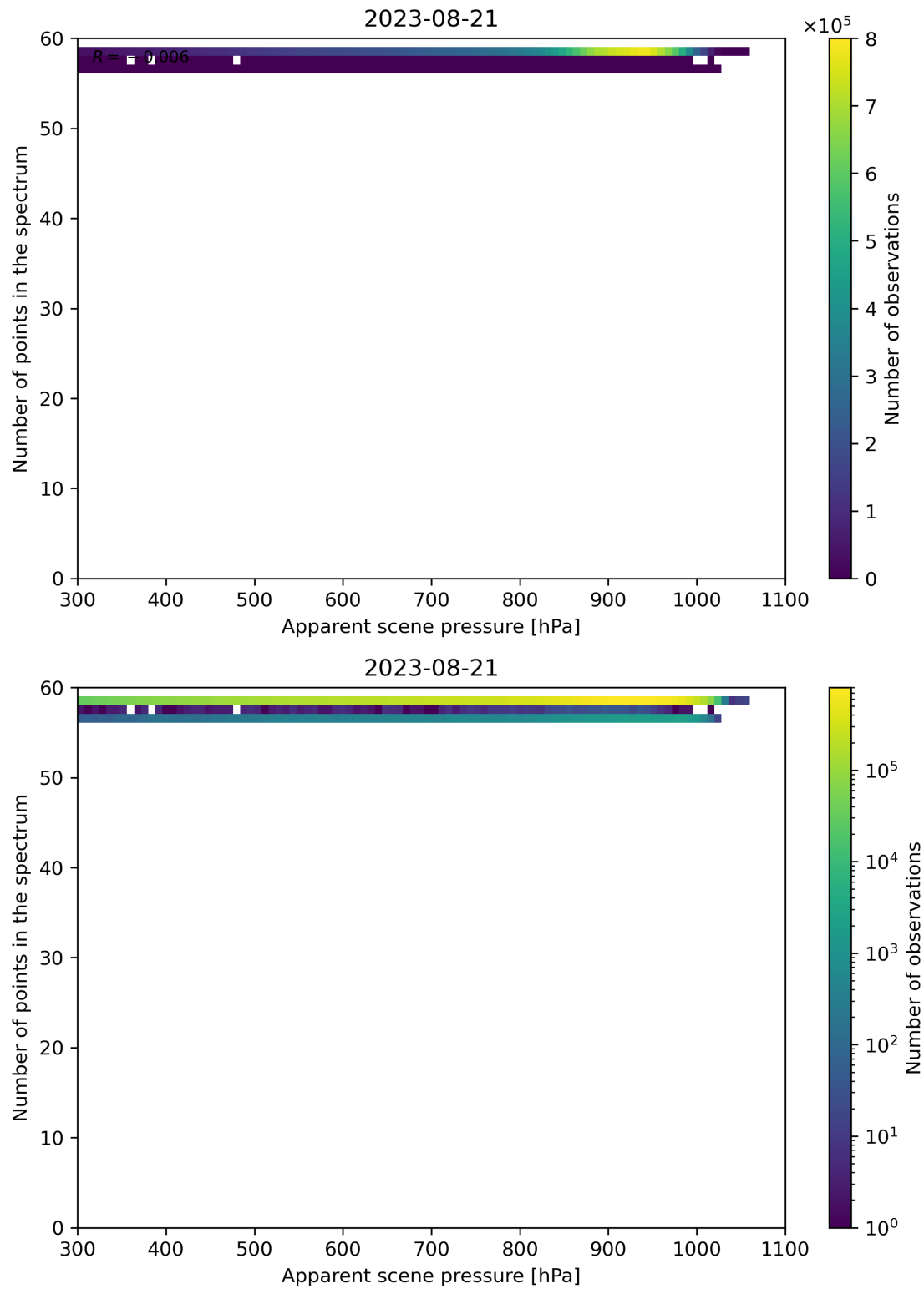
Figure 67: Scatter density plot of “Apparent scene pressure” against “Number of points in the spectrum” for 2023-08-20 to 2023-08-22.
