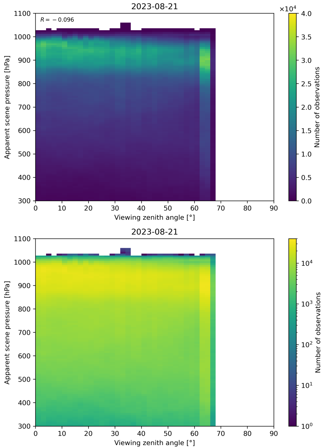
Figure 129: Scatter density plot of “Viewing zenith angle” against “Apparent scene pressure” for 2023-08-20 to 2023-08-22.
