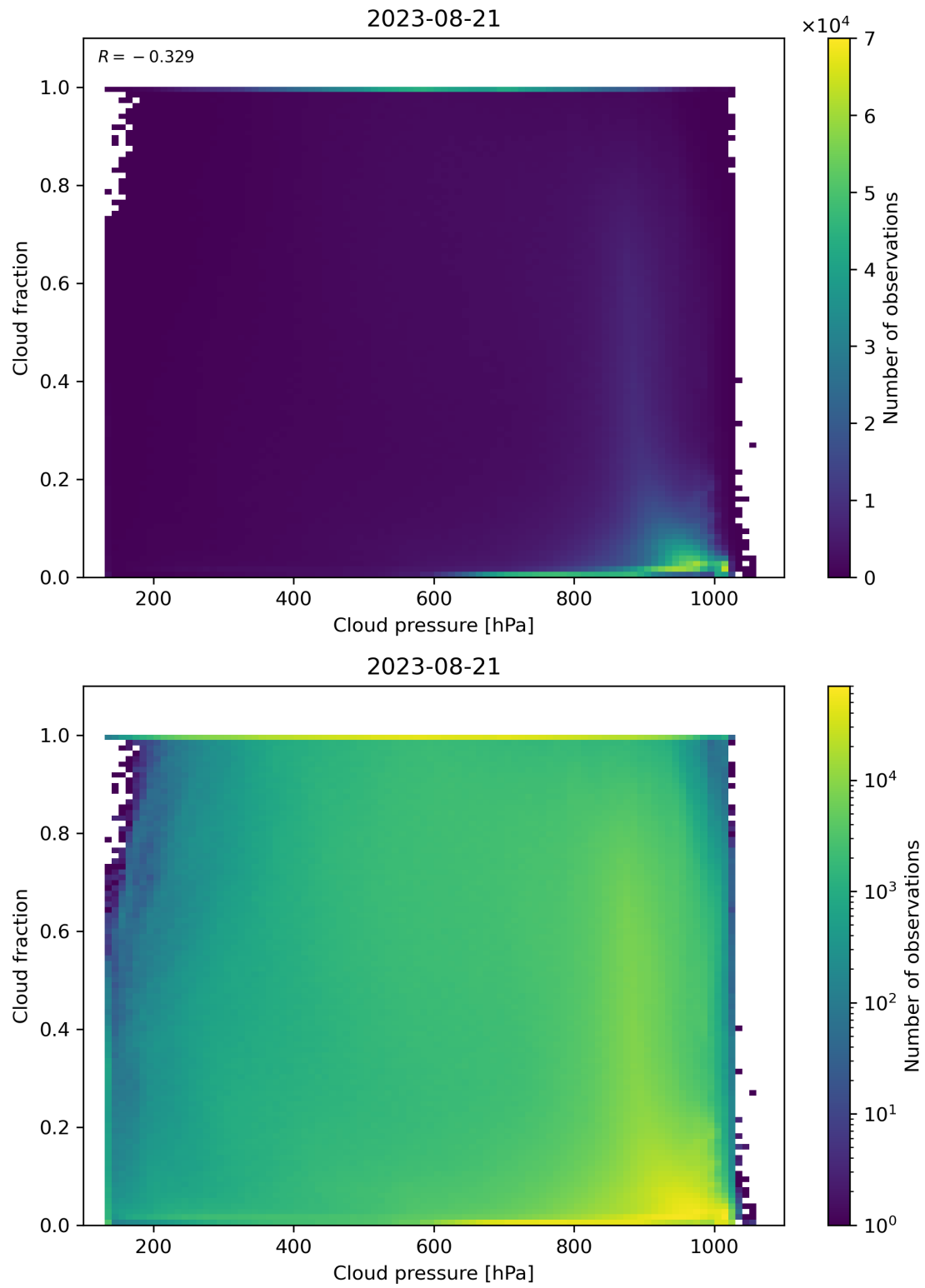
Figure 87: Scatter density plot of “Cloud pressure” against “Cloud fraction” for 2023-08-20 to 2023-08-22.
