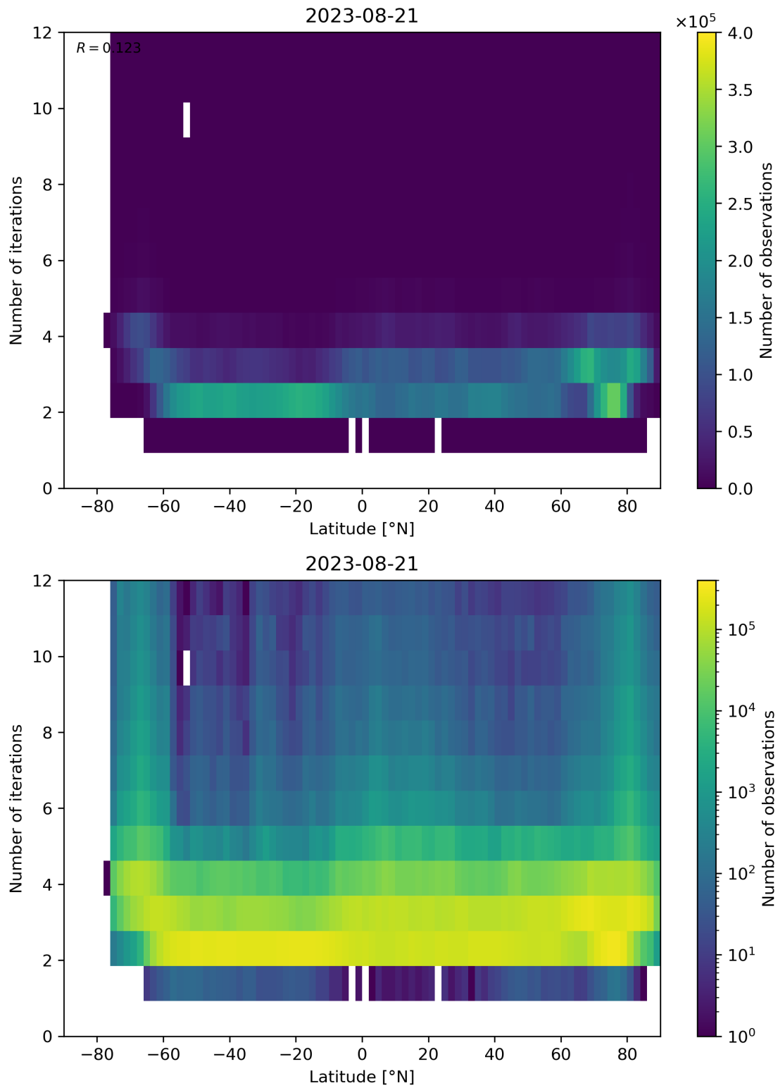
Figure 102: Scatter density plot of “Latitude” against “Number of iterations” for 2023-08-20 to 2023-08-22.
