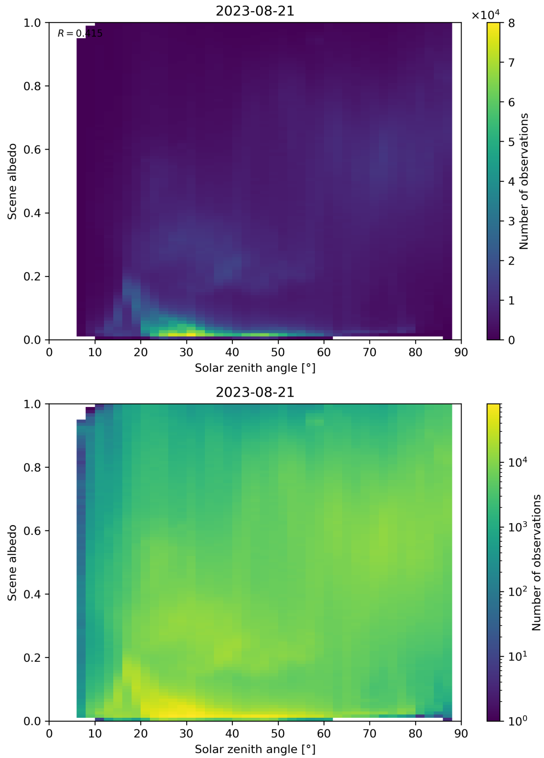
Figure 127: Scatter density plot of “Solar zenith angle” against “Scene albedo” for 2023-08-20 to 2023-08-22.
