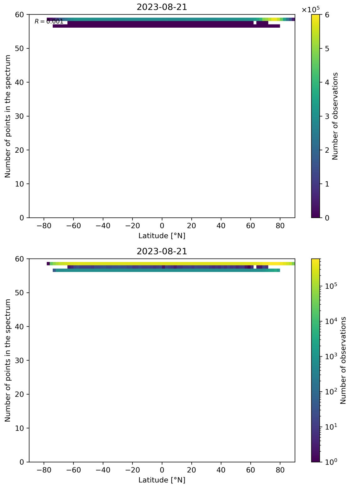
Figure 103: Scatter density plot of “Latitude” against “Number of points in the spectrum” for 2023-08-20 to 2023-08-22.
