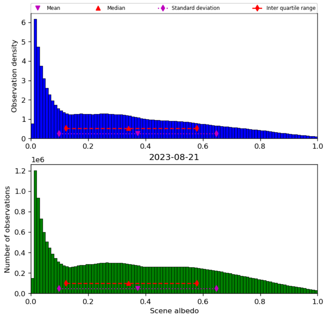
Figure 34: Histogram of “Scene albedo” for 2023-08-20 to 2023-08-22
