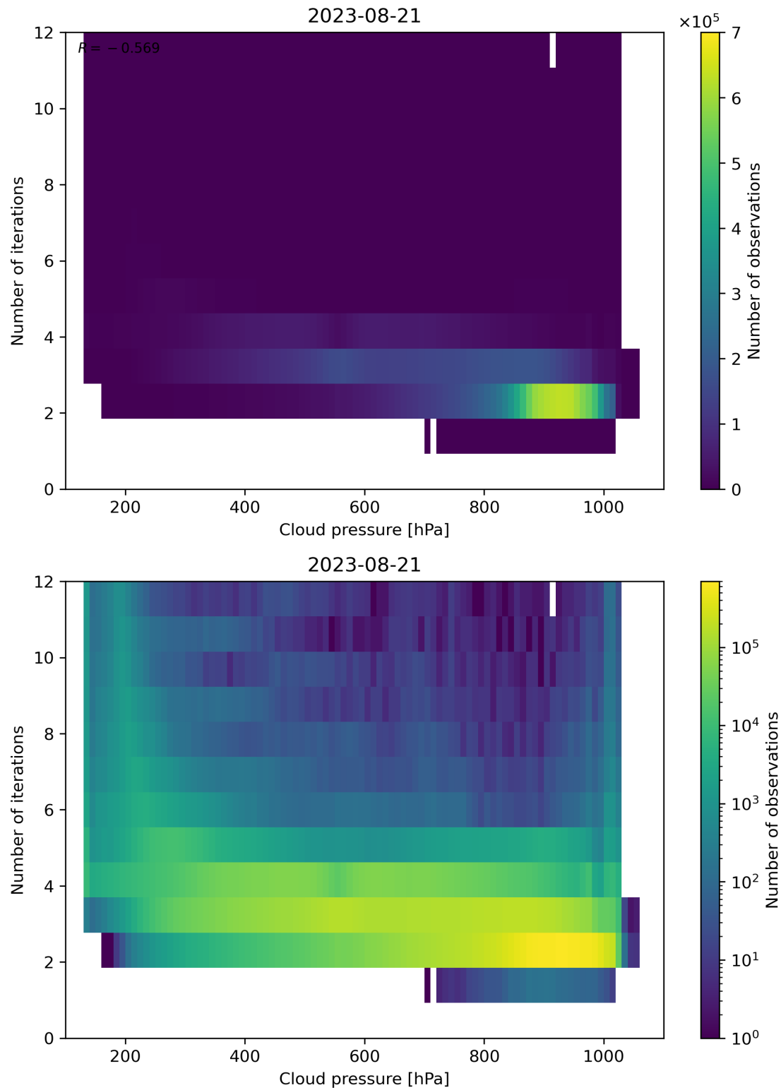
Figure 89: Scatter density plot of “Cloud pressure” against “Number of iterations” for 2023-08-20 to 2023-08-22.
