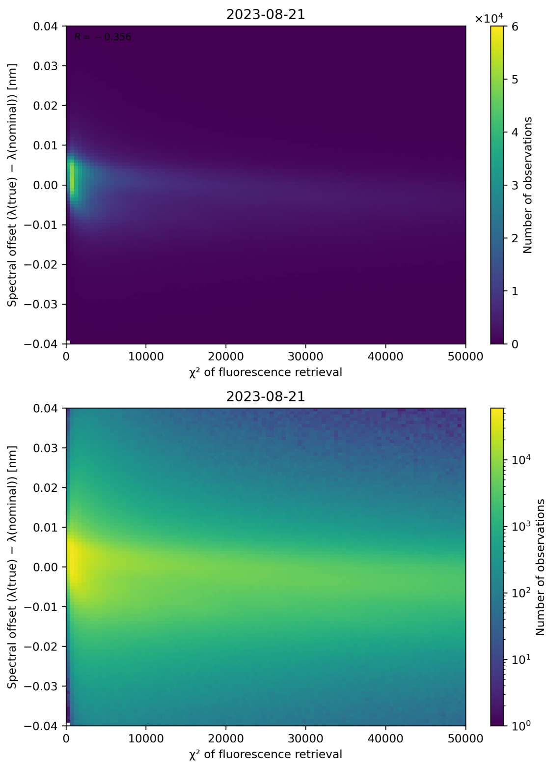
Figure 72: Scatter density plot of " \chi^2 of fluorescence retrieval" against "Spectral offset ( \lambda(\text{true}) - \lambda(\text{nominal}) )" for 2023-08-20 to 2023-08-22.
