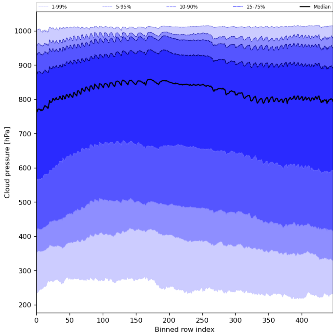
Figure 47: Along track statistics of “Cloud pressure” for 2023-08-20 to 2023-08-22
