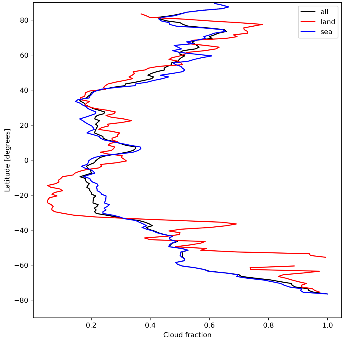
Figure 15: Zonal average of “Cloud fraction” for 2023-08-20 to 2023-08-22.
