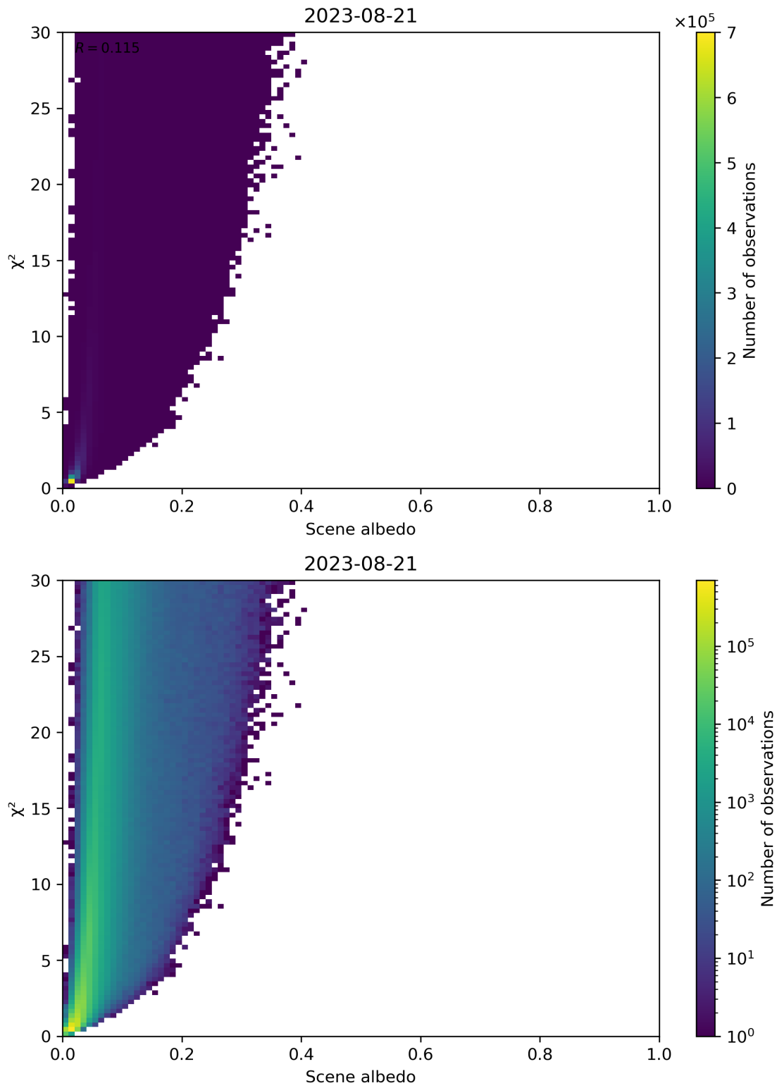
Figure 112: Scatter density plot of “Scene albedo” against “ \chi^2 ” for 2023-08-20 to 2023-08-22.
