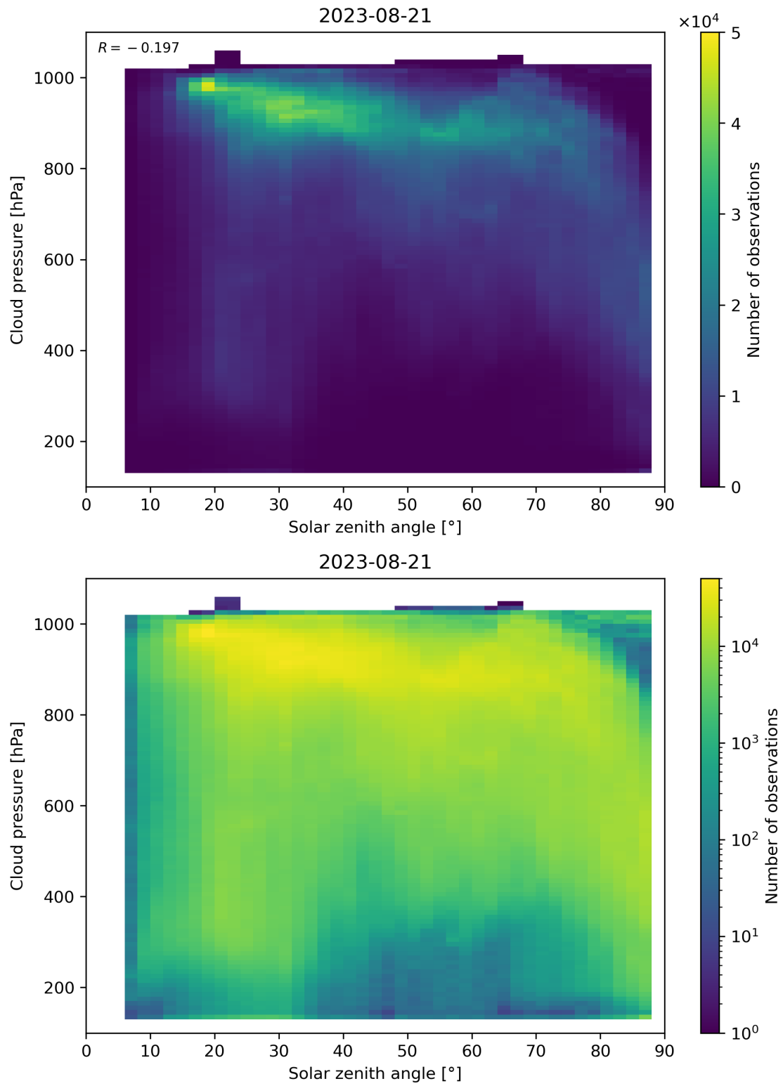
Figure 122: Scatter density plot of “Solar zenith angle” against “Cloud pressure” for 2023-08-20 to 2023-08-22.
