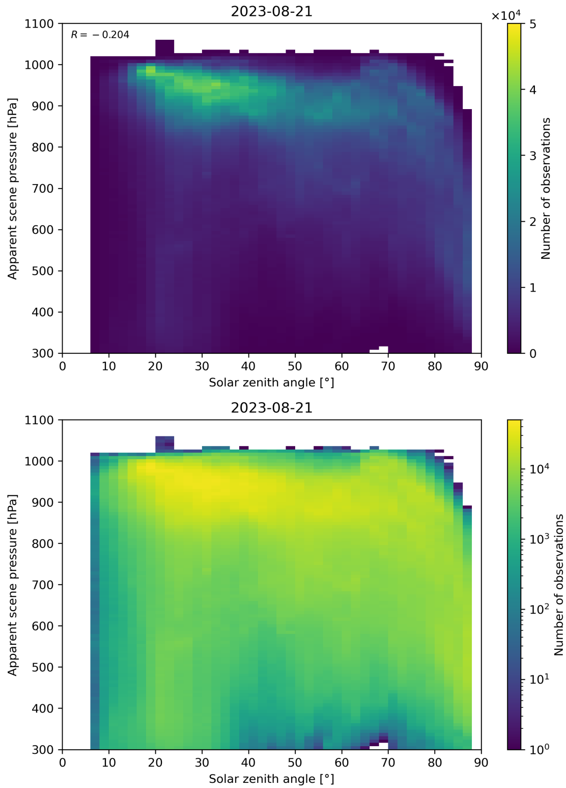
Figure 118: Scatter density plot of “Solar zenith angle” against “Apparent scene pressure” for 2023-08-20 to 2023-08-22.
