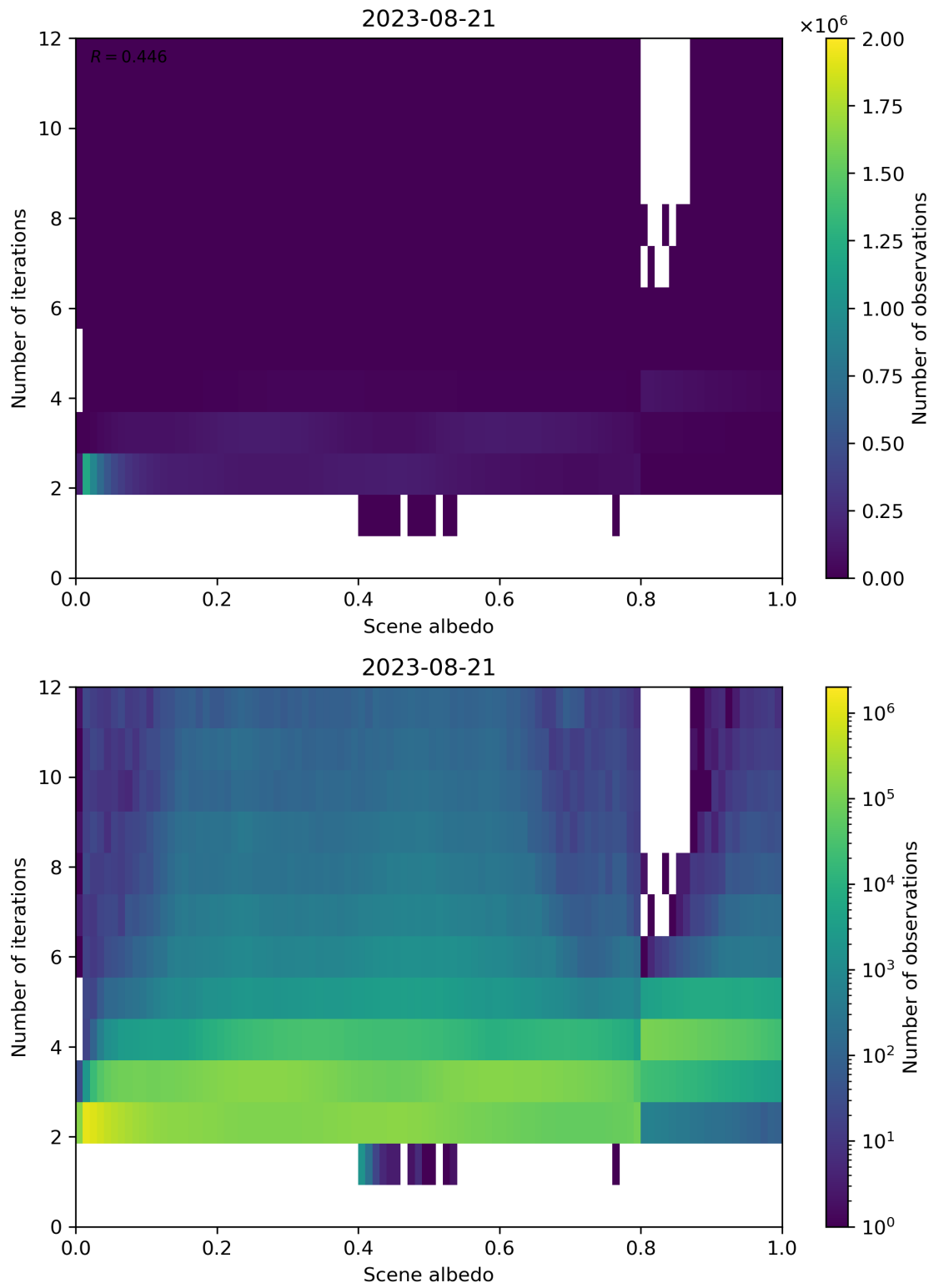
Figure 115: Scatter density plot of “Scene albedo” against “Number of iterations” for 2023-08-20 to 2023-08-22.
