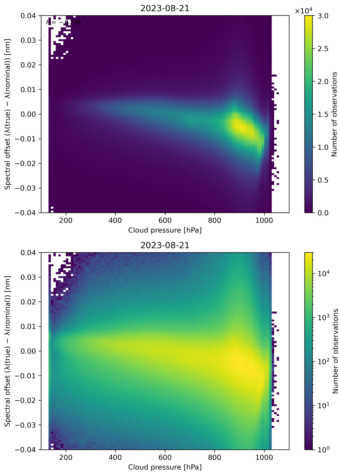
Figure 92: Scatter density plot of “Cloud pressure” against “Spectral offset ( \lambda(\text{true}) - \lambda(\text{nominal}) )” for 2023-08-20 to 2023-08-22.
