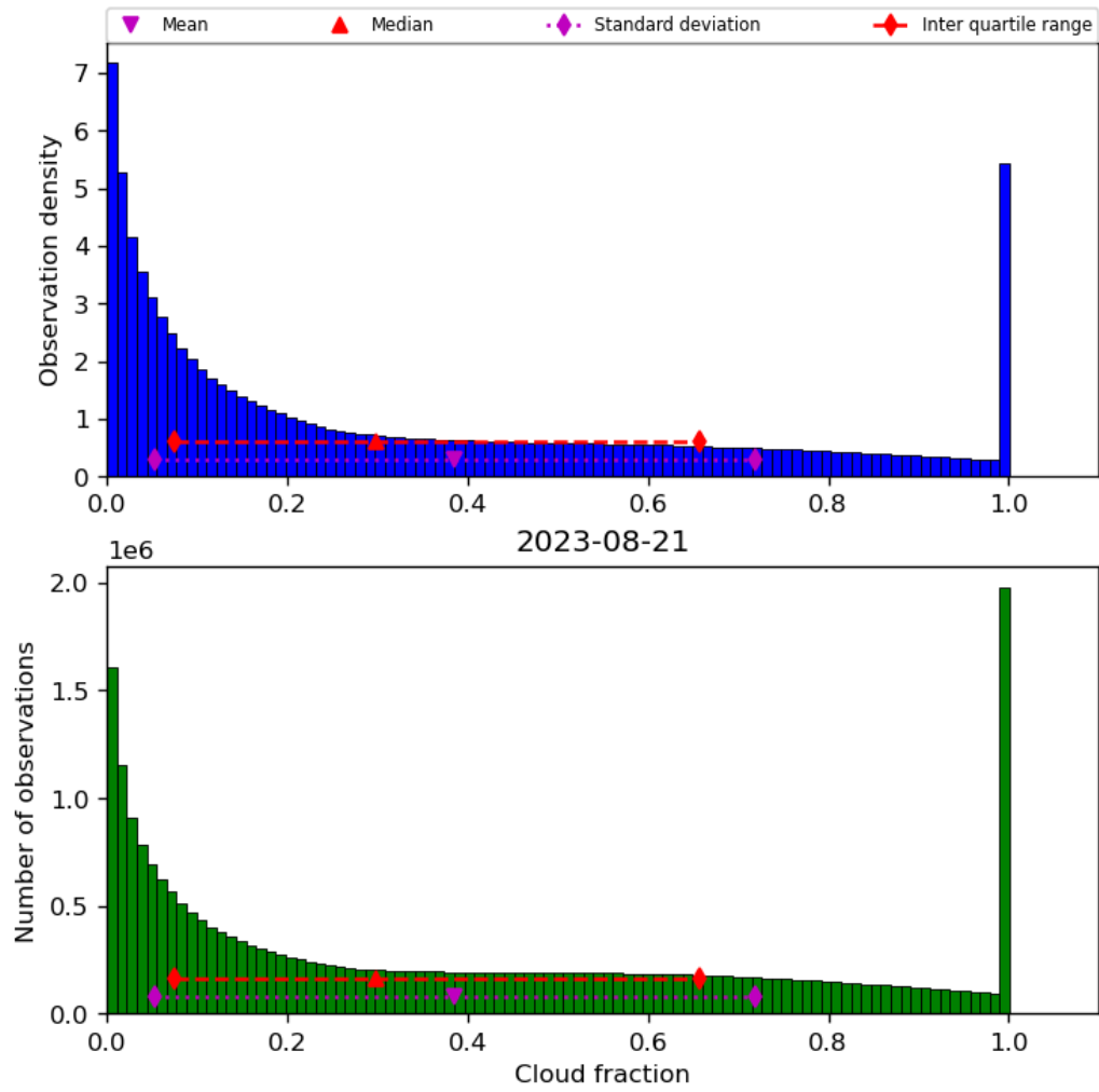
Figure 32: Histogram of “Cloud fraction” for 2023-08-20 to 2023-08-22
