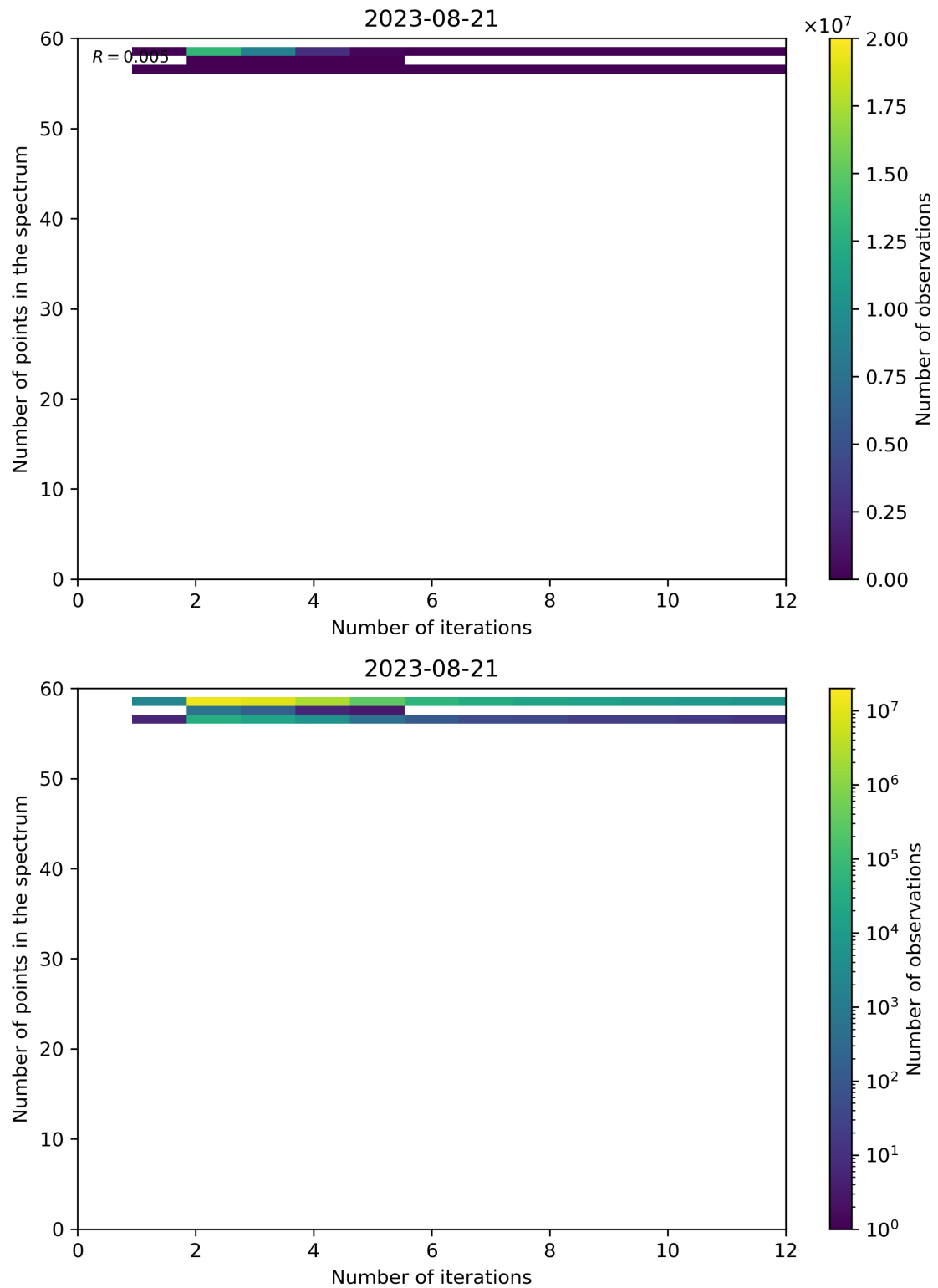
Figure 108: Scatter density plot of “Number of iterations” against “Number of points in the spectrum” for 2023-08-20 to 2023-08-22.
