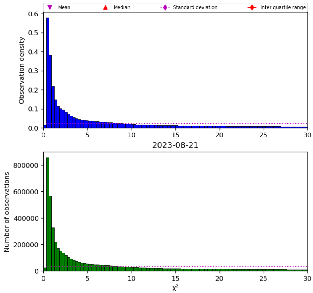
Figure 38: Histogram of “ \chi^2 ” for 2023-08-20 to 2023-08-22
