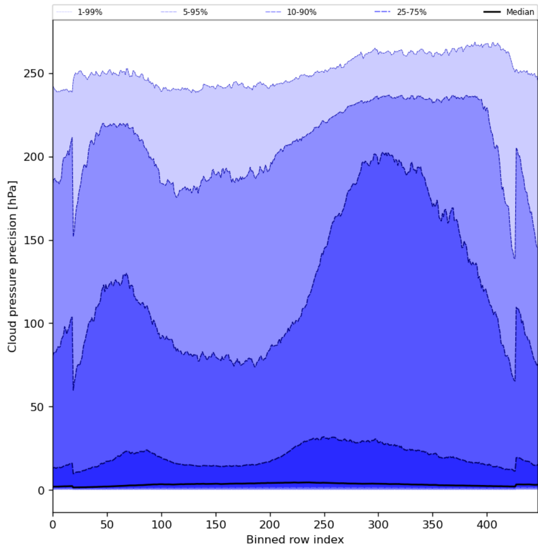
Figure 48: Along track statistics of “Cloud pressure precision” for 2023-08-20 to 2023-08-22
