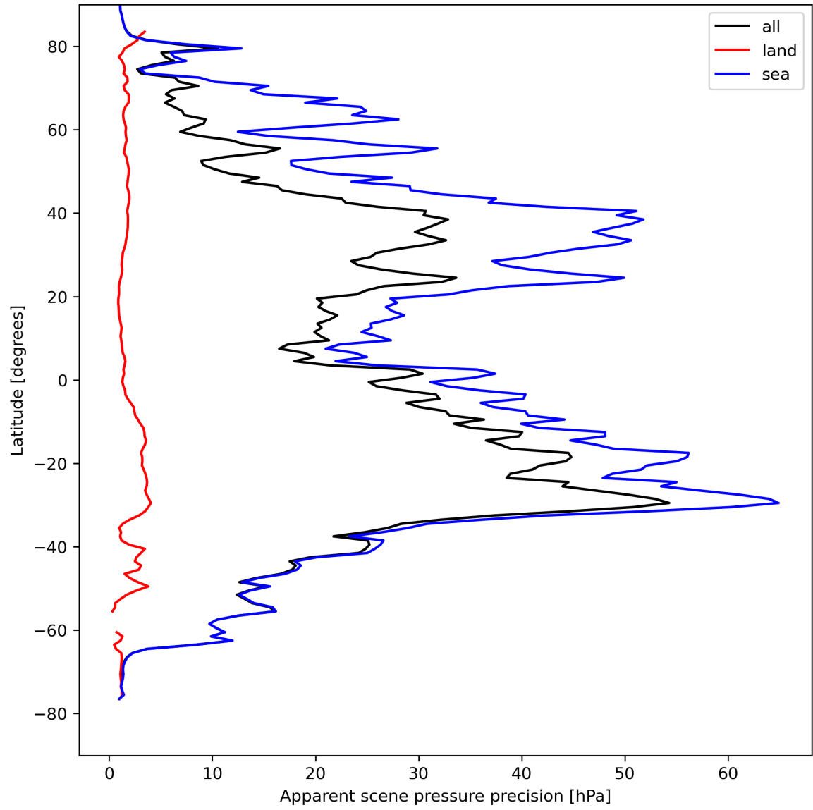
Figure 20: Zonal average of “Apparent scene pressure precision” for 2023-08-20 to 2023-08-22.
