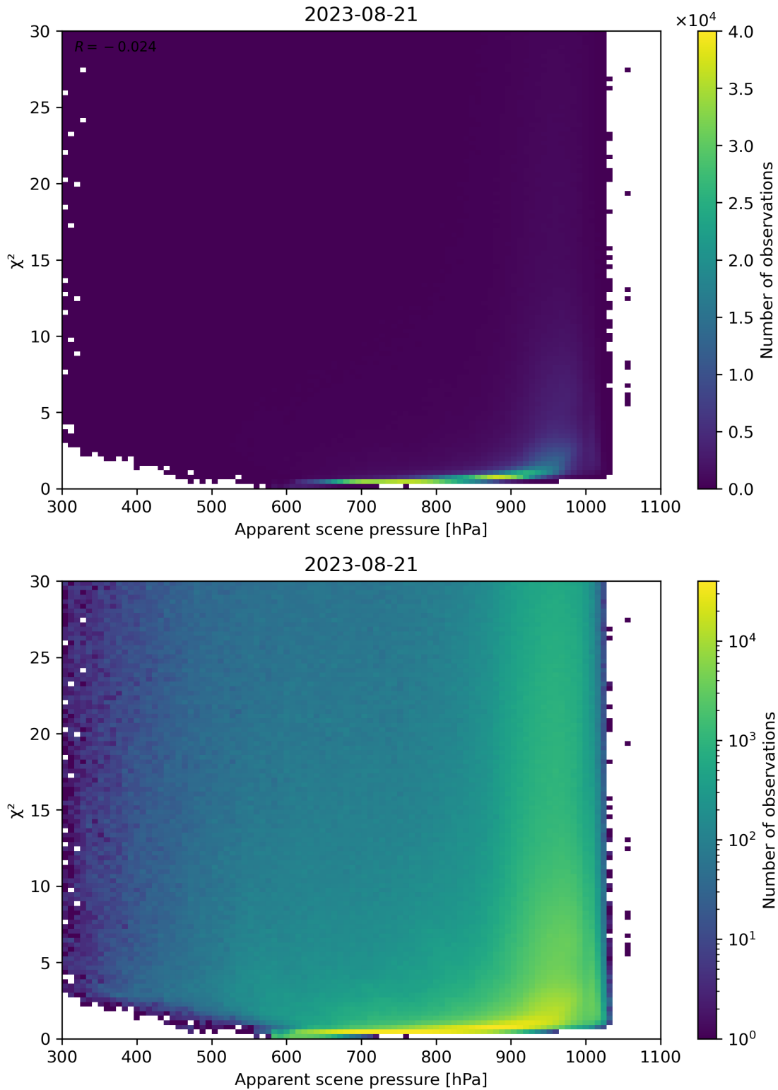
Figure 63: Scatter density plot of “Apparent scene pressure” against “ \chi^2 ” for 2023-08-20 to 2023-08-22.
