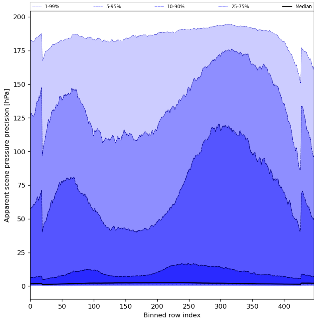
Figure 54: Along track statistics of “Apparent scene pressure precision” for 2023-08-20 to 2023-08-22
