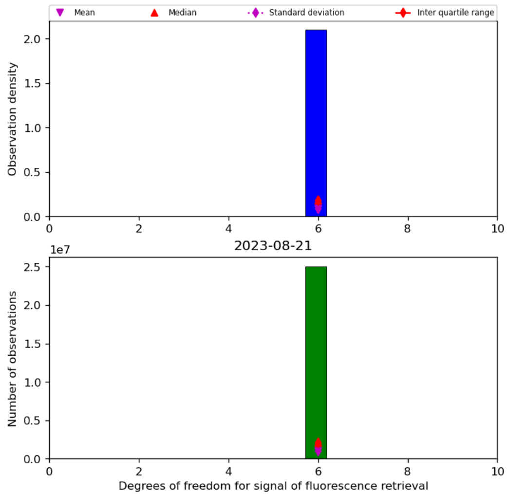
Figure 43: Histogram of “Degrees of freedom for signal of fluorescence retrieval” for 2023-08-20 to 2023-08-22
