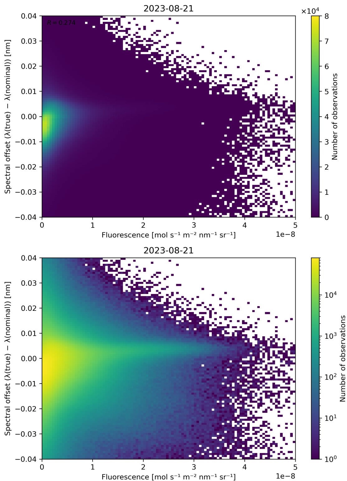
Figure 95: Scatter density plot of “Fluorescence” against “Spectral offset ( \lambda(\text{true}) - \lambda(\text{nominal}) )” for 2023-08-20 to 2023-08-22.
