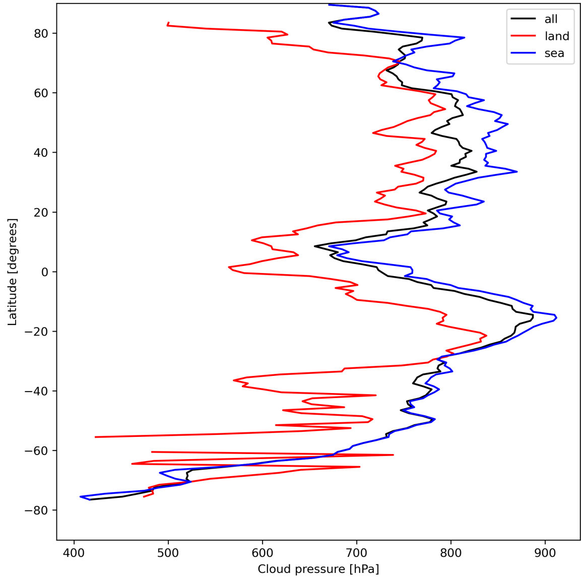
Figure 13: Zonal average of “Cloud pressure” for 2023-08-20 to 2023-08-22.
