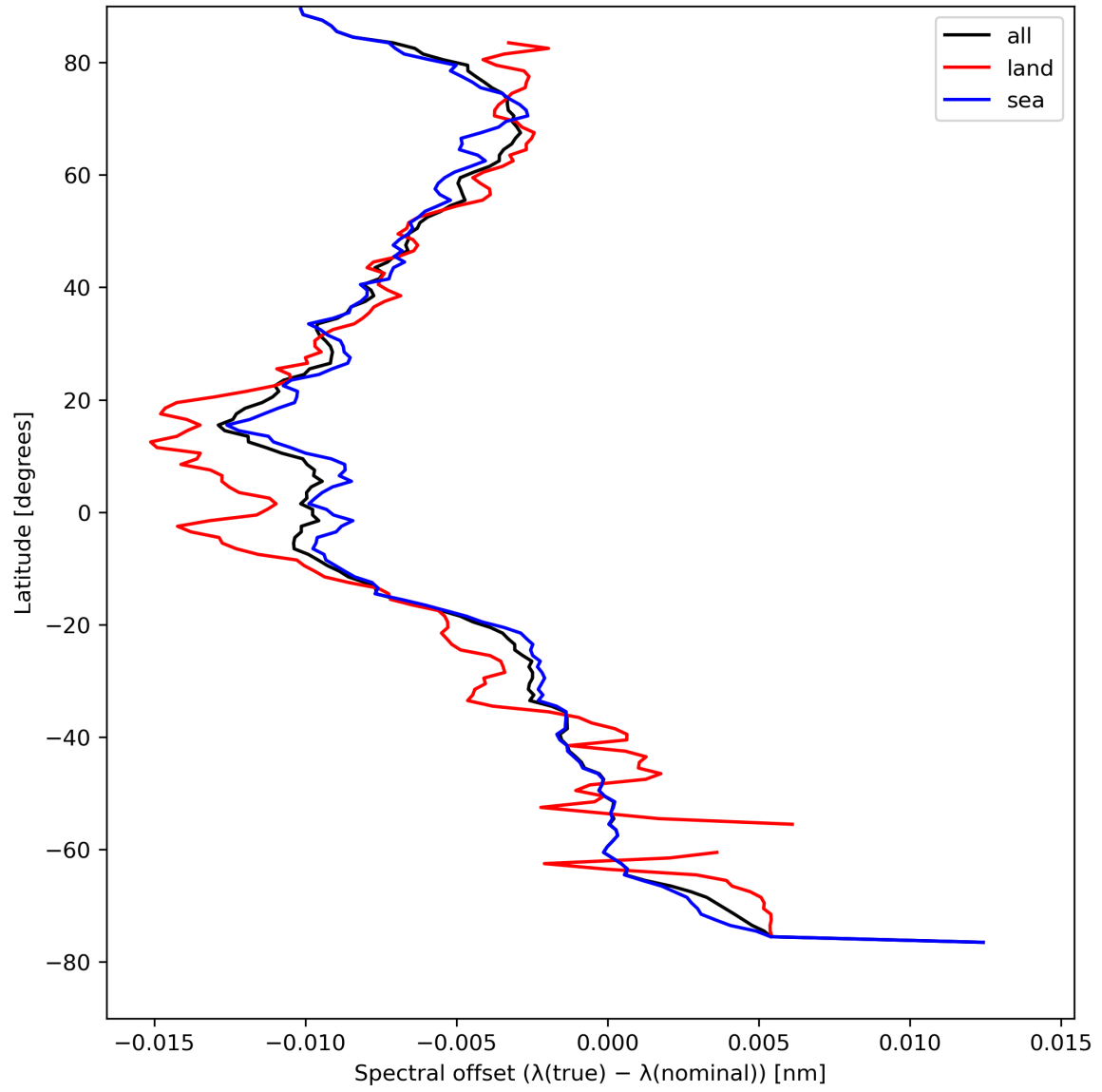
Figure 28: Zonal average of “Spectral offset ( \lambda(\text{true}) - \lambda(\text{nominal}) )” for 2023-08-20 to 2023-08-22.
