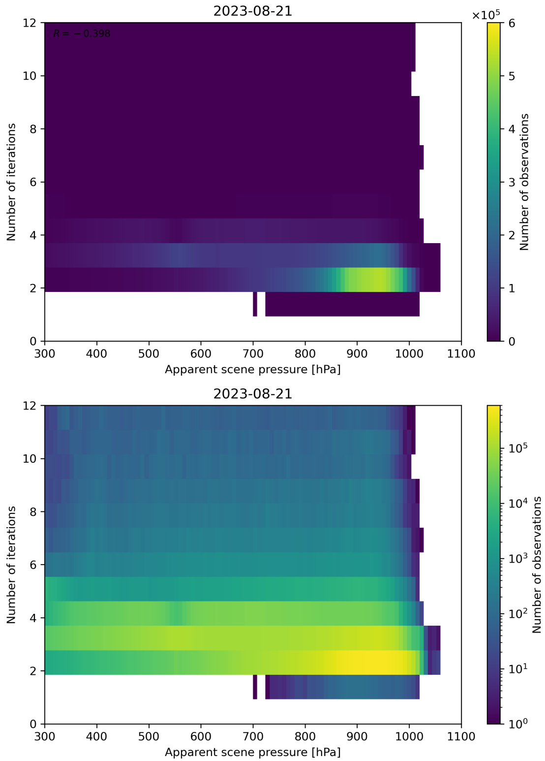
Figure 66: Scatter density plot of “Apparent scene pressure” against “Number of iterations” for 2023-08-20 to 2023-08-22.
