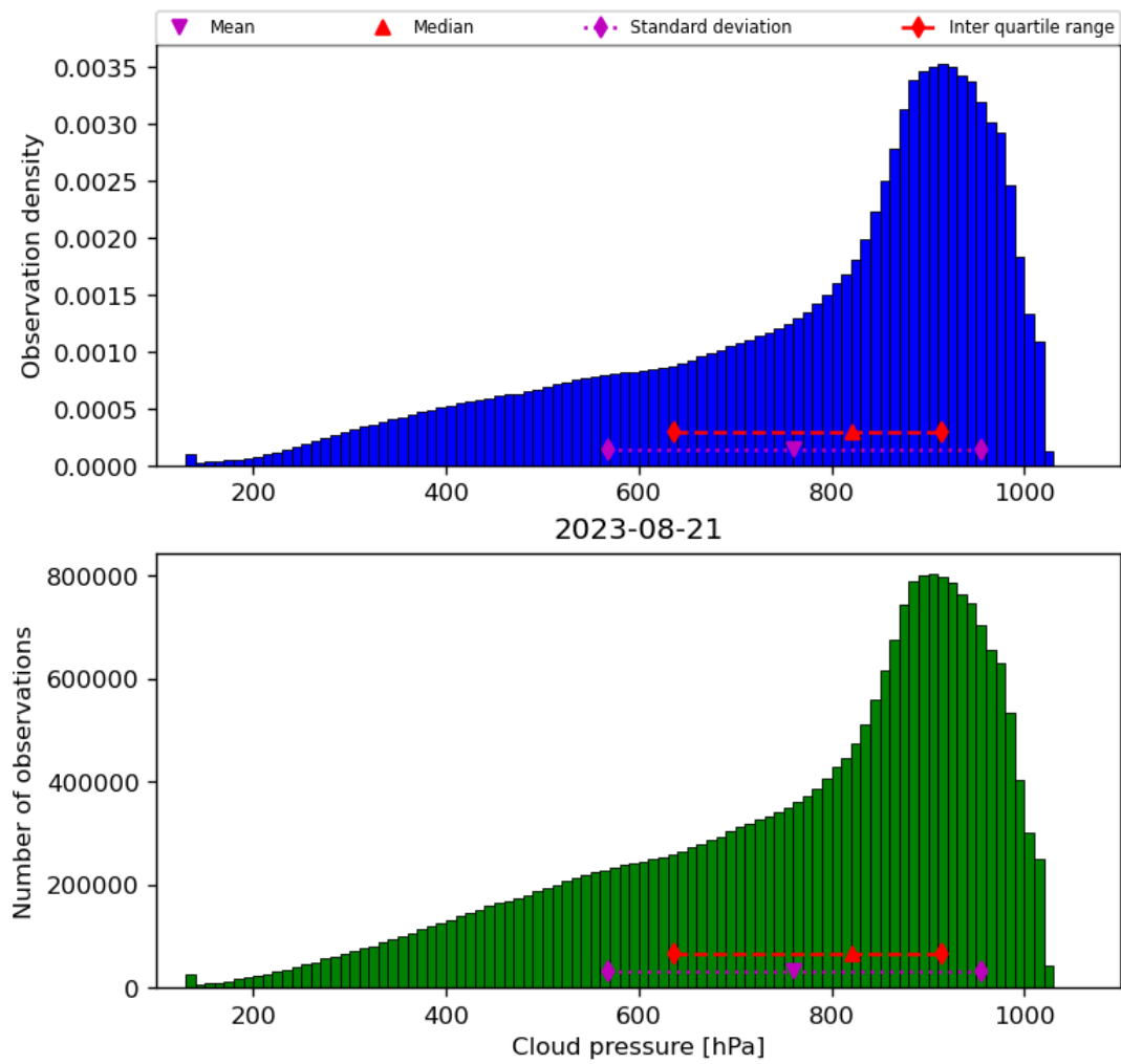
Figure 30: Histogram of “Cloud pressure” for 2023-08-20 to 2023-08-22
