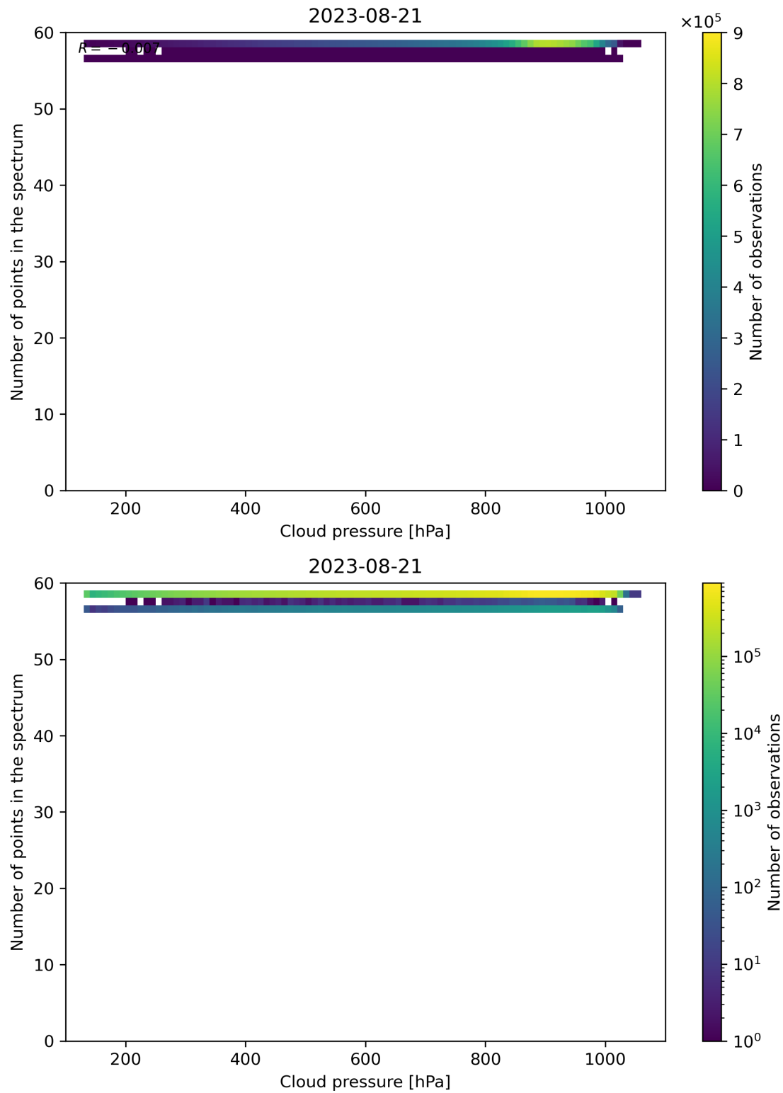
Figure 90: Scatter density plot of “Cloud pressure” against “Number of points in the spectrum” for 2023-08-20 to 2023-08-22.
