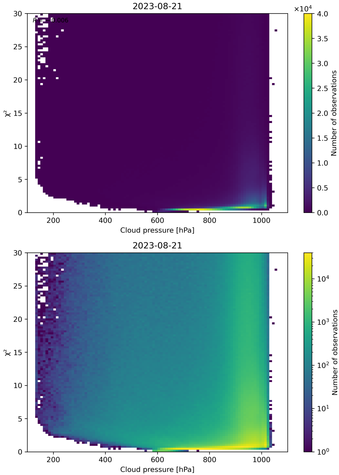
Figure 85: Scatter density plot of “Cloud pressure” against “ \chi^2 ” for 2023-08-20 to 2023-08-22.
