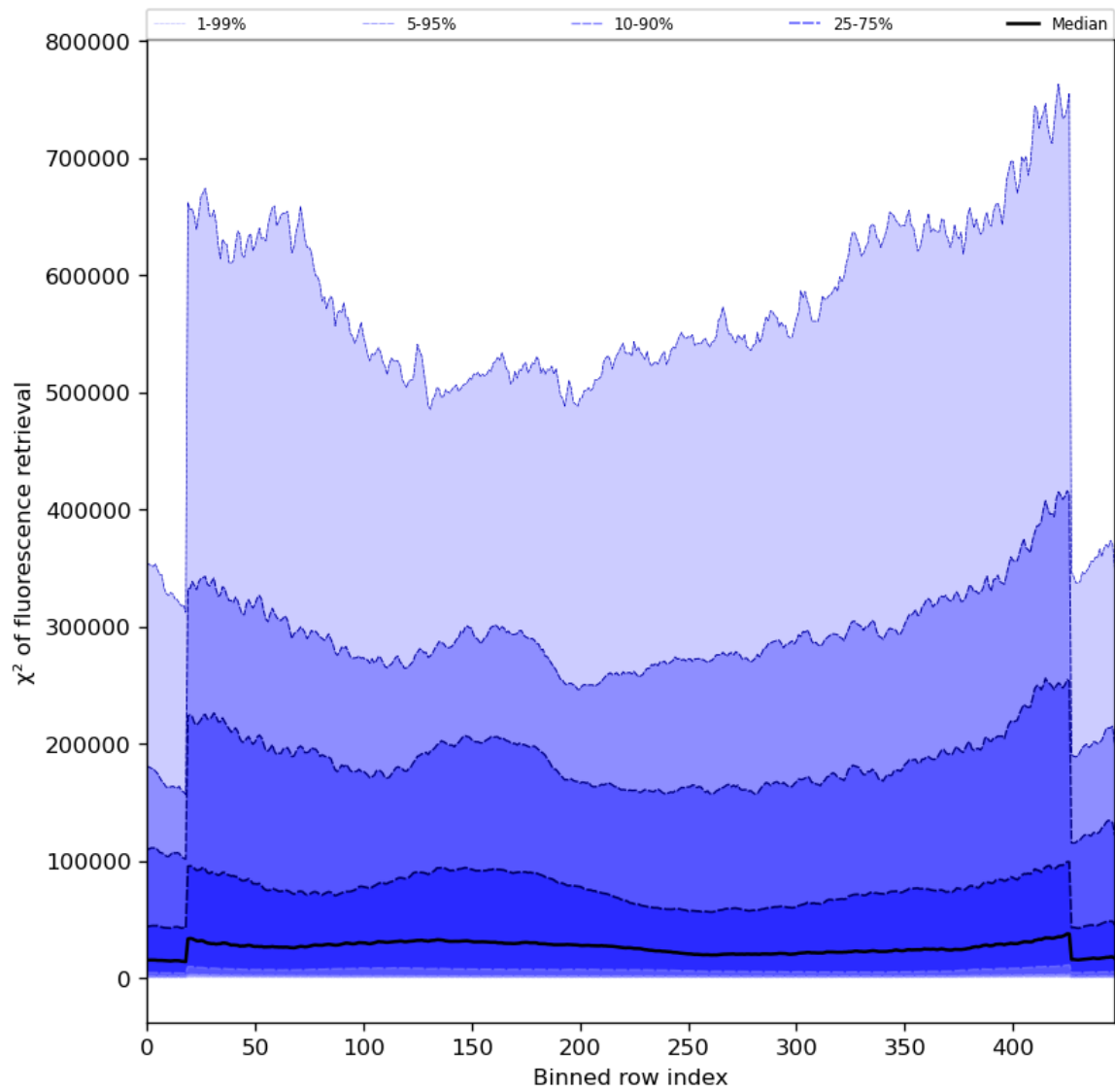
Figure 59: Along track statistics of “ \chi^2 of fluorescence retrieval” for 2023-08-20 to 2023-08-22
