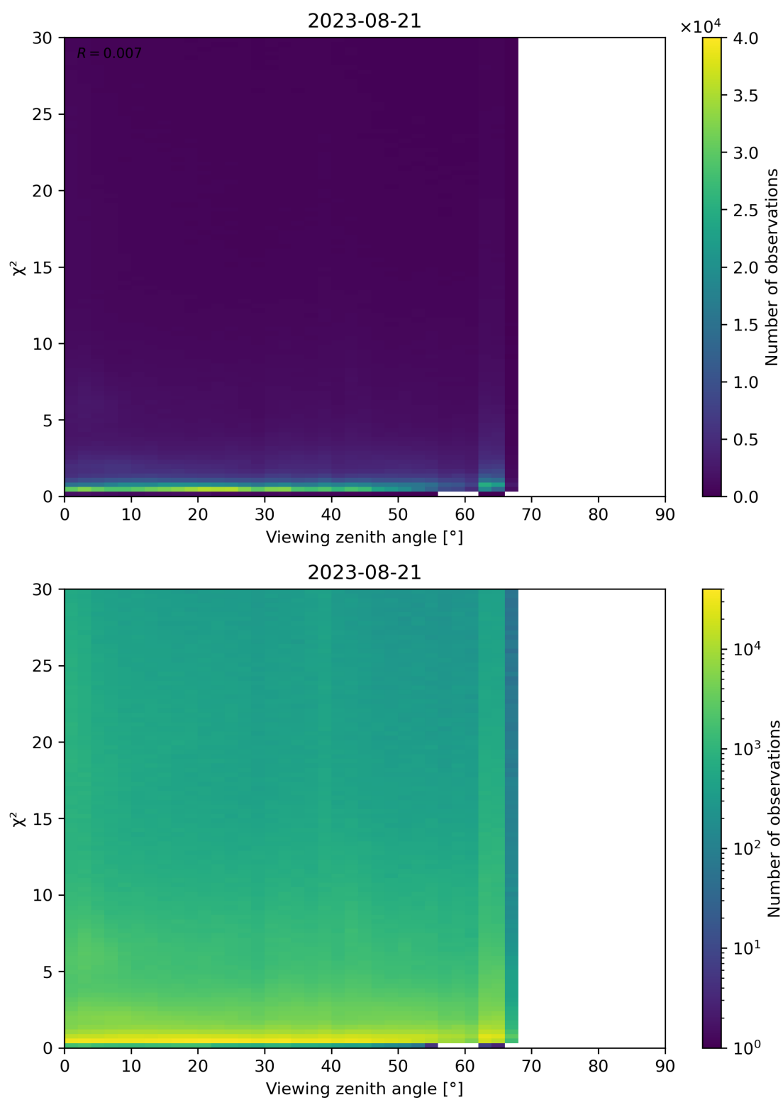
Figure 130: Scatter density plot of “Viewing zenith angle” against “ \chi^2 ” for 2023-08-20 to 2023-08-22.
