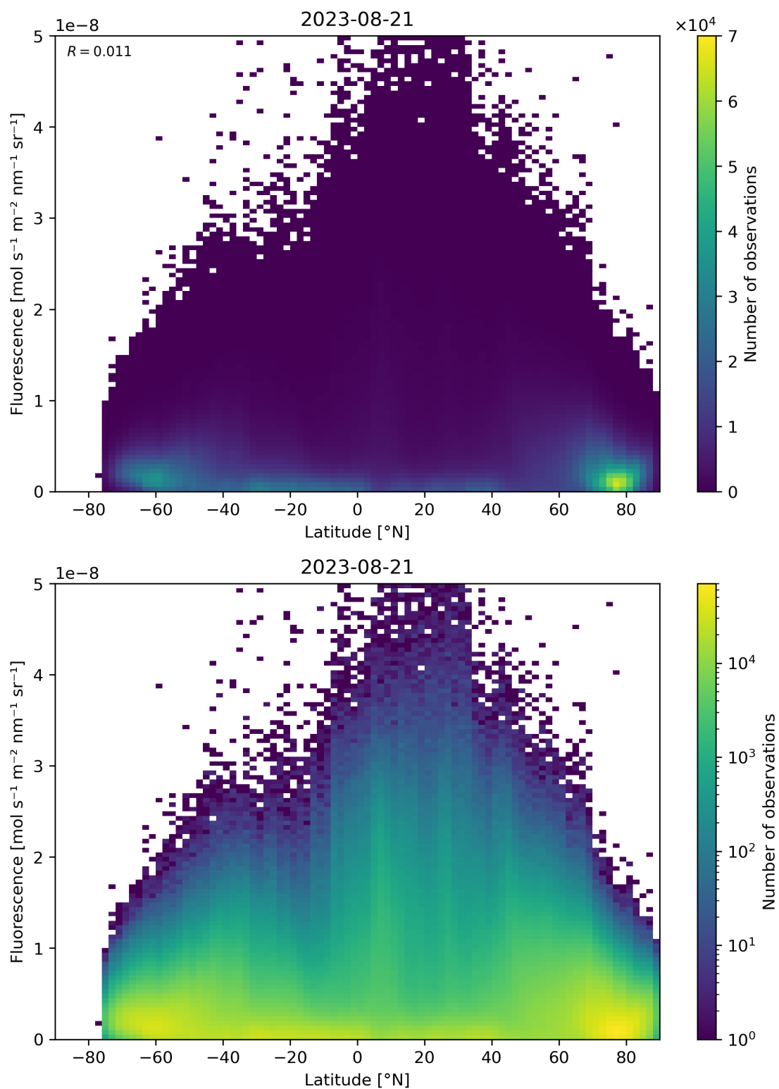
Figure 101: Scatter density plot of “Latitude” against “Fluorescence” for 2023-08-20 to 2023-08-22.
