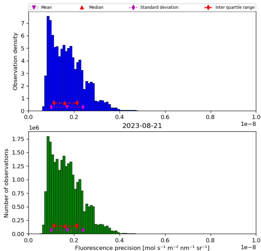
Figure 41: Histogram of “Fluorescence precision” for 2023-08-20 to 2023-08-22
