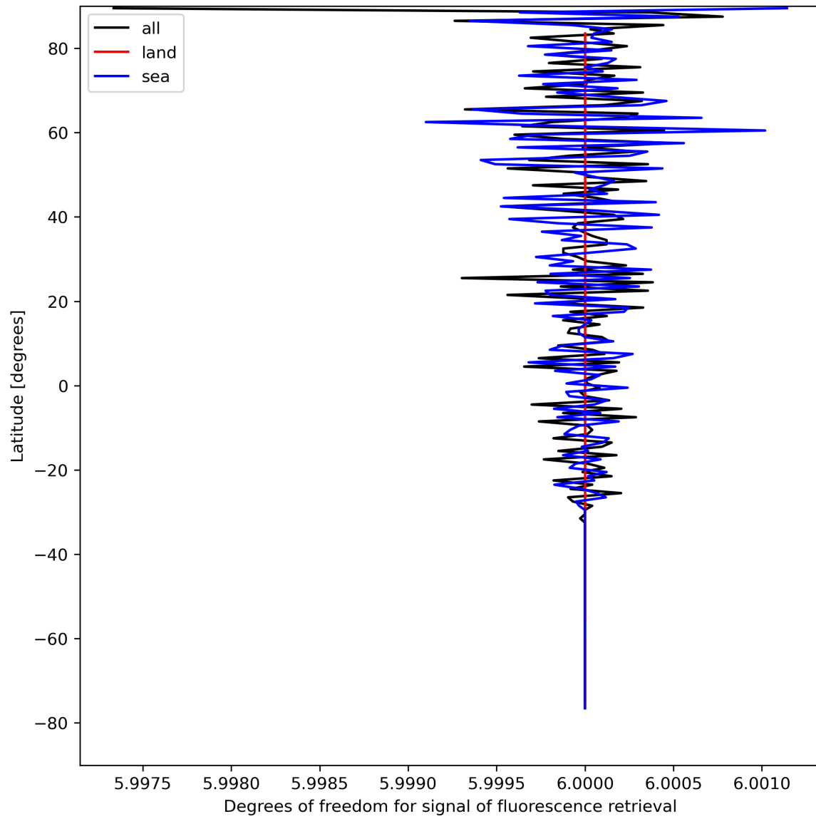
Figure 26: Zonal average of “Degrees of freedom for signal of fluorescence retrieval” for 2023-08-20 to 2023-08-22.
