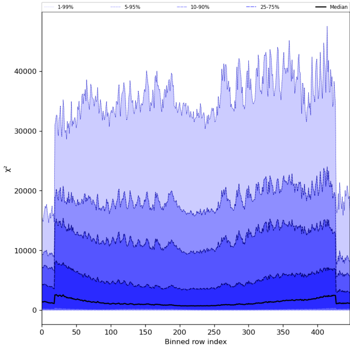
Figure 55: Along track statistics of “ \chi^2 ” for 2023-08-20 to 2023-08-22
