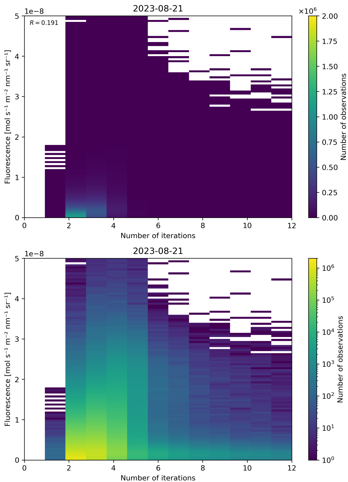
Figure 107: Scatter density plot of “Number of iterations” against “Fluorescence” for 2023-08-20 to 2023-08-22.
