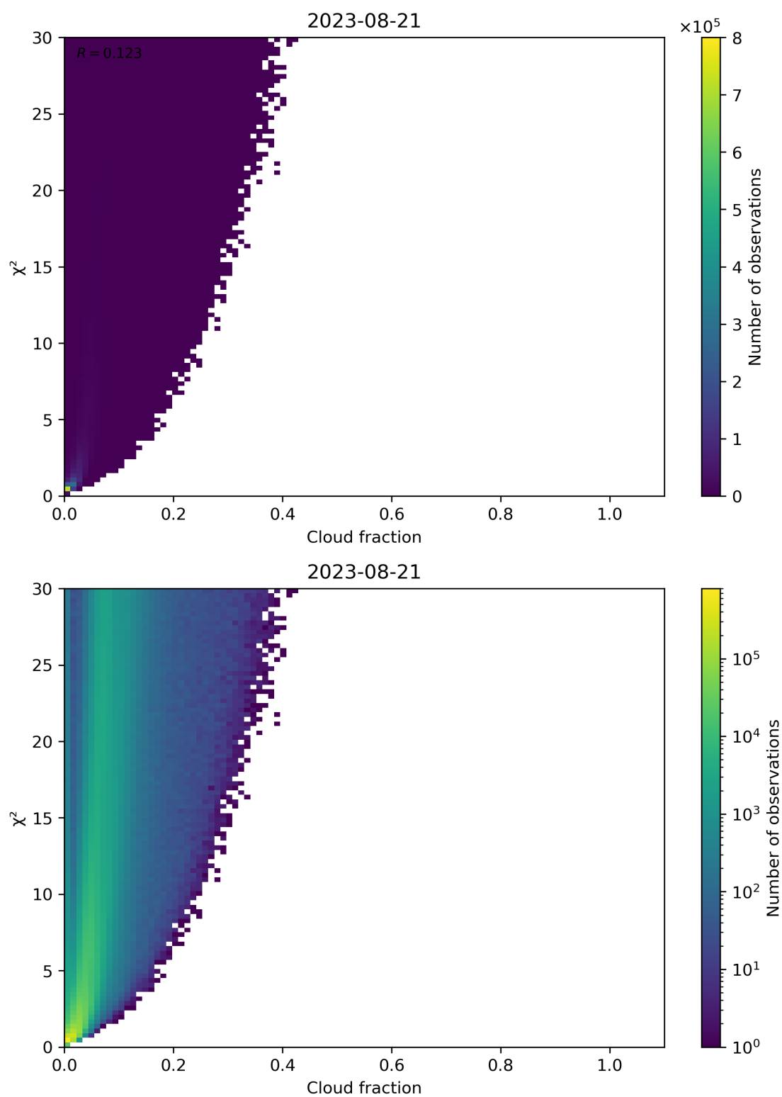
Figure 77: Scatter density plot of “Cloud fraction” against “ \chi^2 ” for 2023-08-20 to 2023-08-22.
