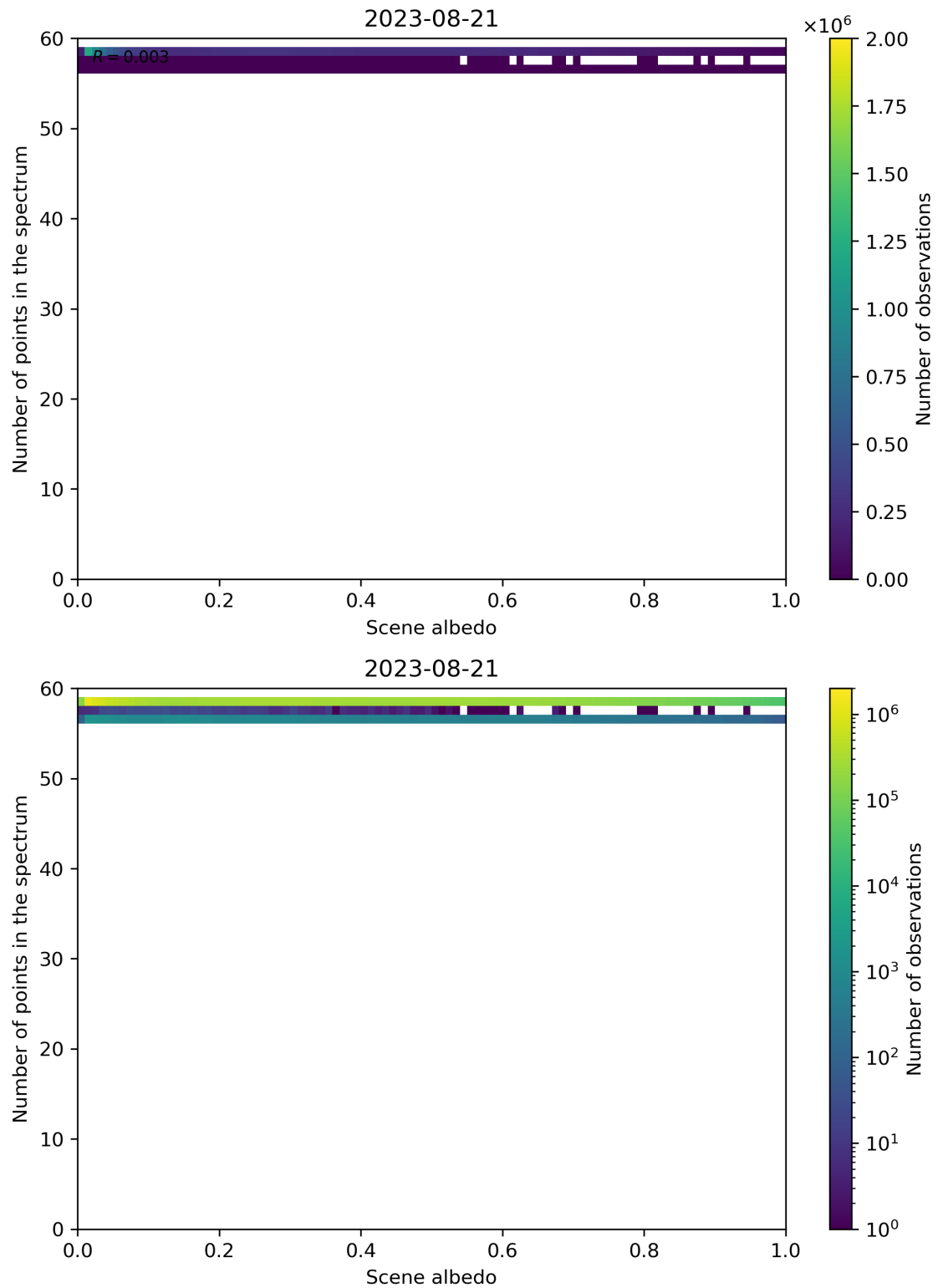
Figure 116: Scatter density plot of “Scene albedo” against “Number of points in the spectrum” for 2023-08-20 to 2023-08-22.
