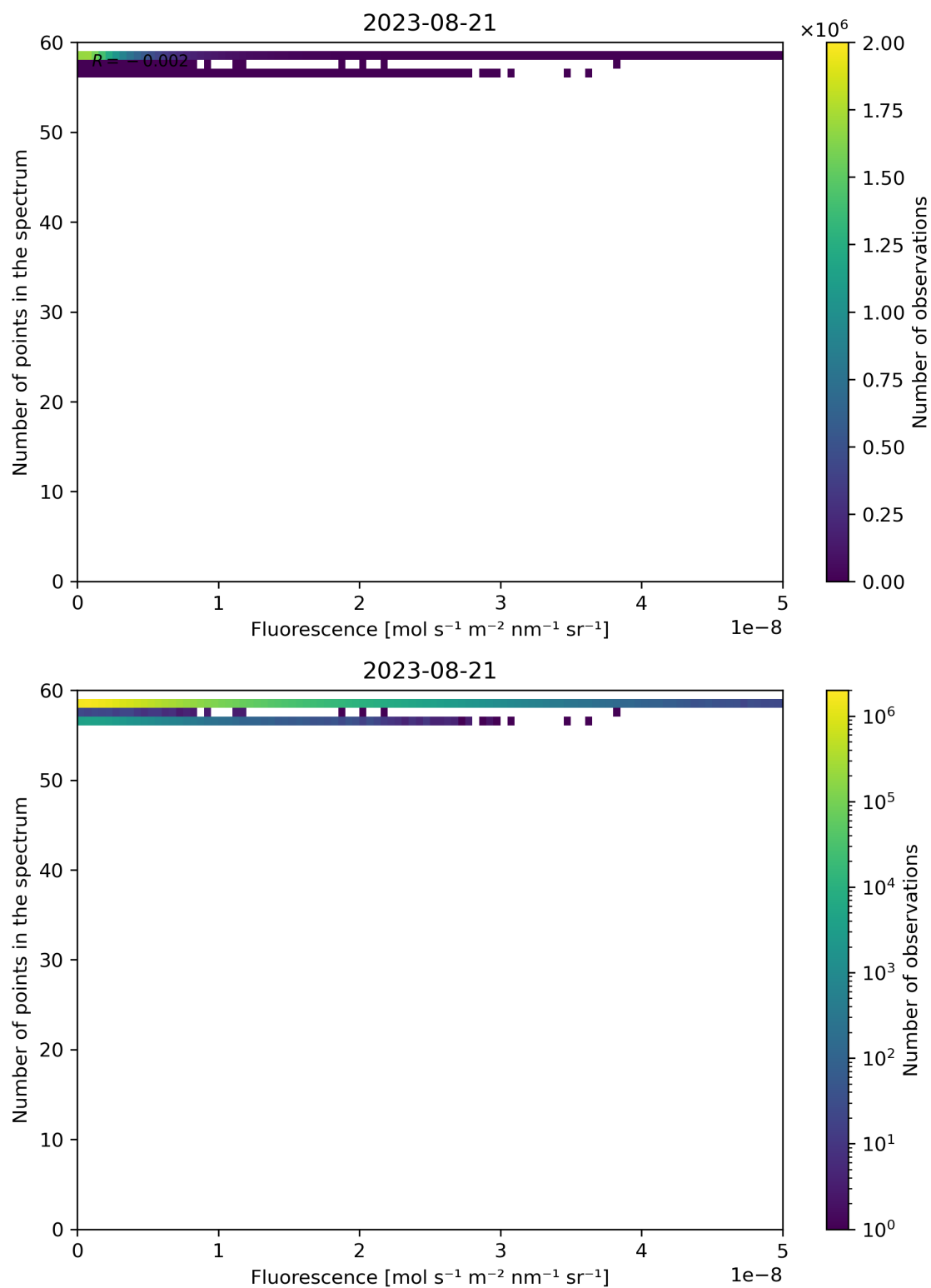
Figure 94: Scatter density plot of “Fluorescence” against “Number of points in the spectrum” for 2023-08-20 to 2023-08-22.
