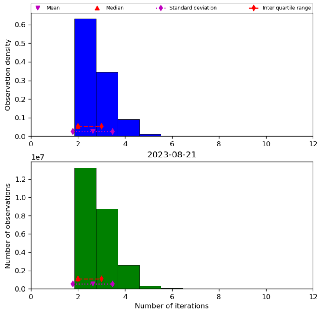
Figure 39: Histogram of “Number of iterations” for 2023-08-20 to 2023-08-22
