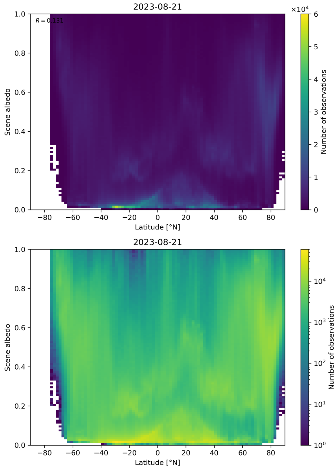
Figure 104: Scatter density plot of “Latitude” against “Scene albedo” for 2023-08-20 to 2023-08-22.
