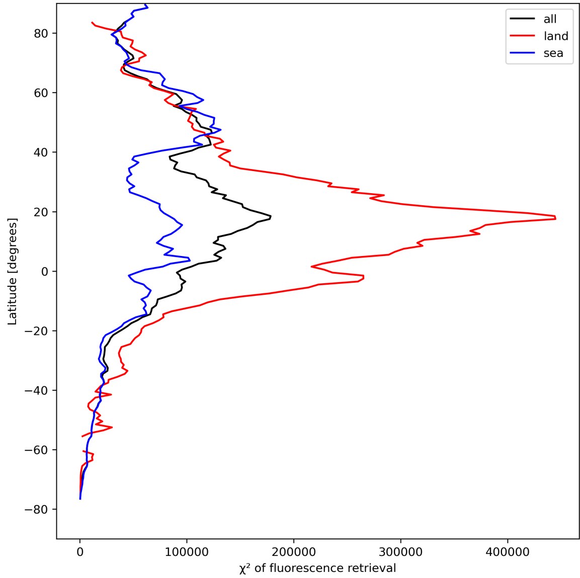
Figure 25: Zonal average of “ \chi^2 of fluorescence retrieval” for 2023-08-20 to 2023-08-22.
