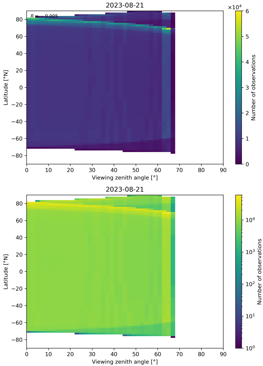
Figure 135: Scatter density plot of “Viewing zenith angle” against “Latitude” for 2023-08-20 to 2023-08-22.
