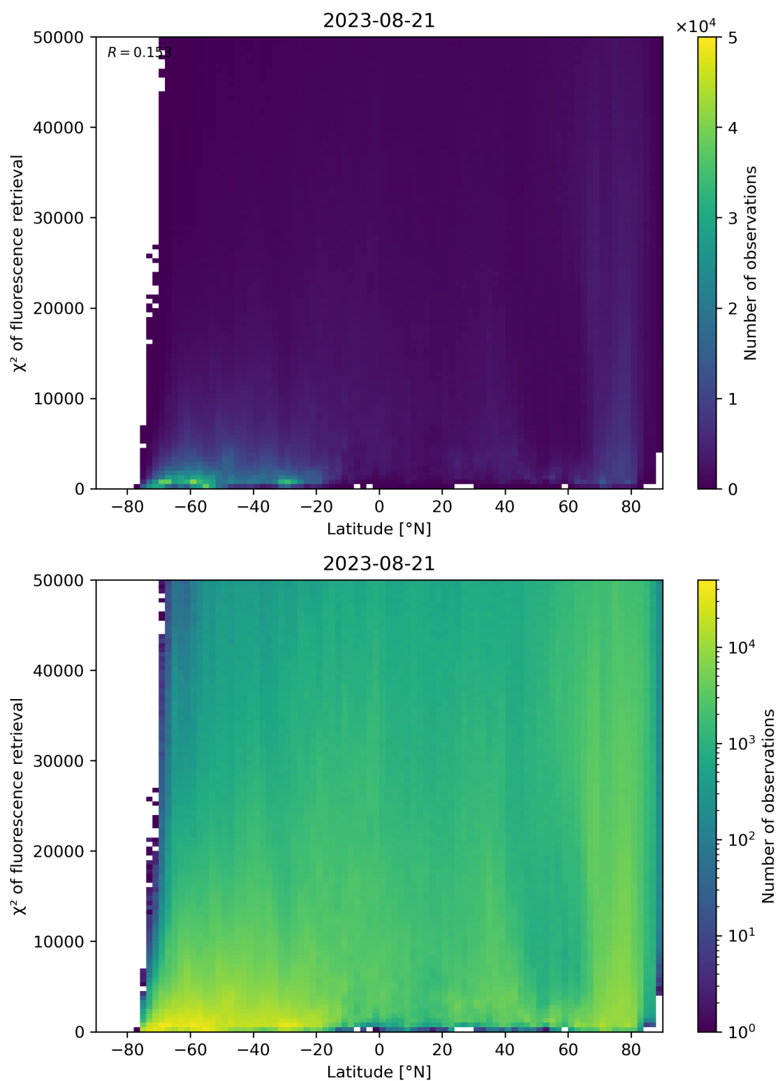
Figure 98: Scatter density plot of “Latitude” against “ \chi^2 of fluorescence retrieval” for 2023-08-20 to 2023-08-22.
