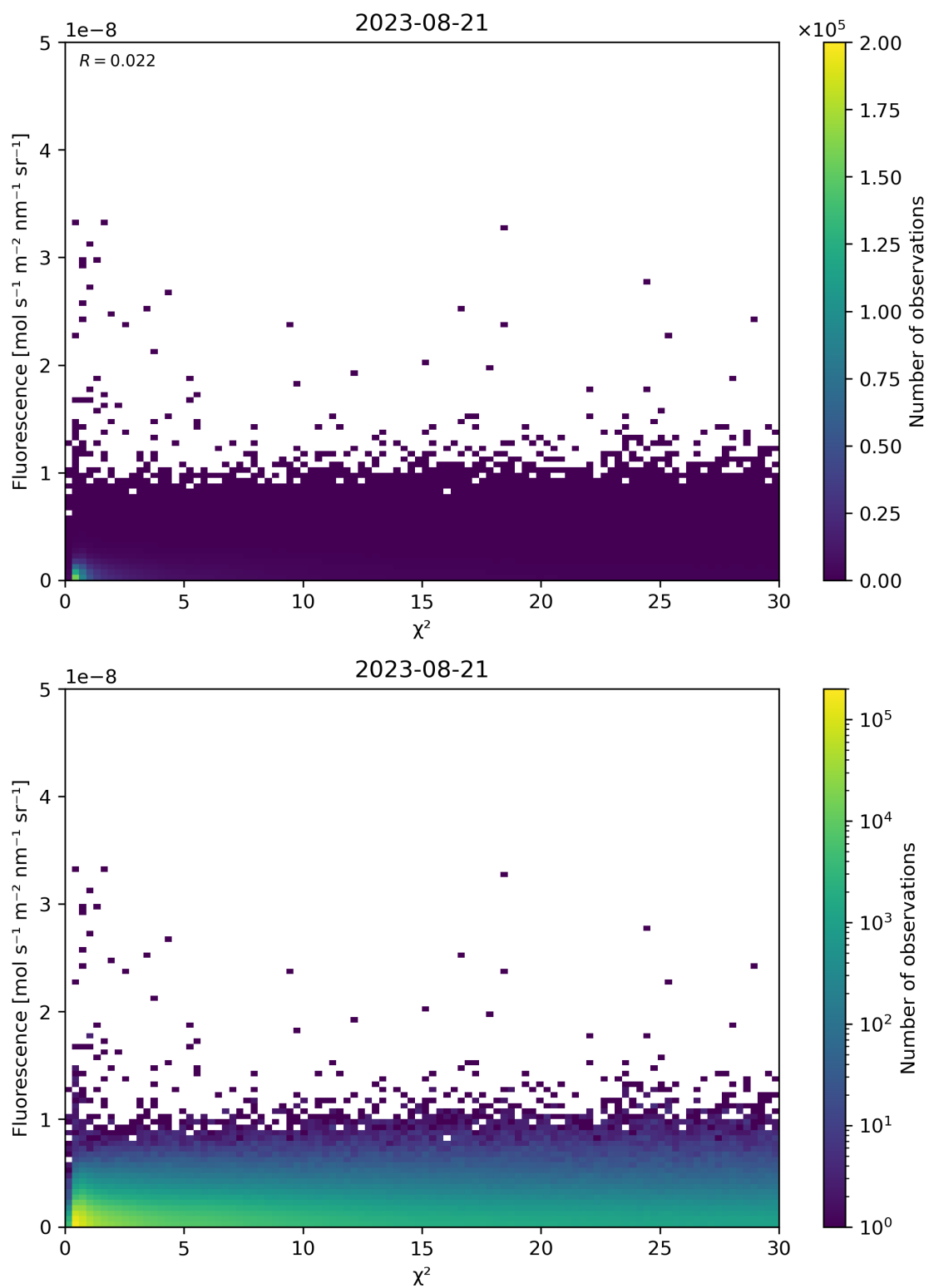
Figure 70: Scatter density plot of “ \chi^2 ” against “Fluorescence” for 2023-08-20 to 2023-08-22.
