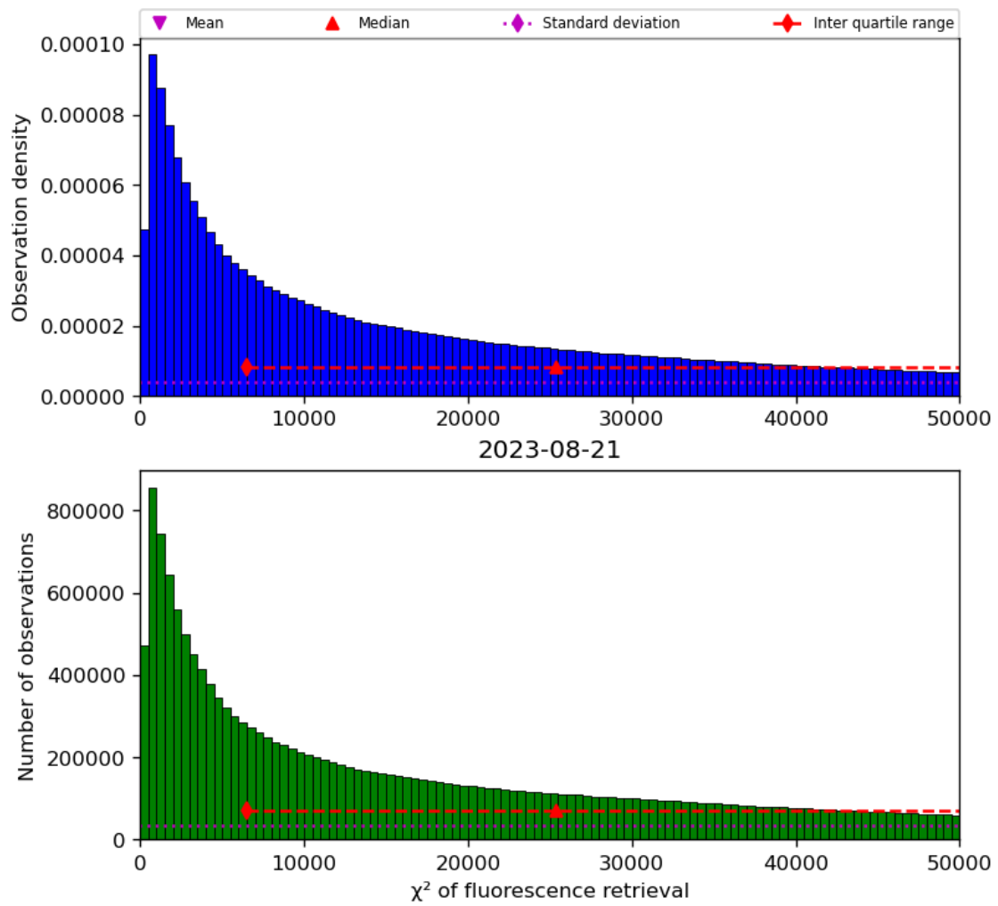
Figure 42: Histogram of “ \chi^2 of fluorescence retrieval” for 2023-08-20 to 2023-08-22
