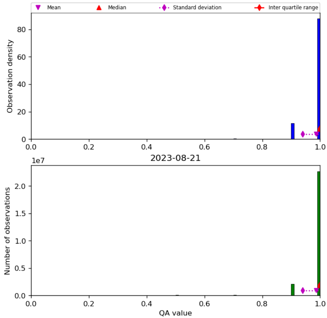
Figure 29: Histogram of “QA value” for 2023-08-20 to 2023-08-22
