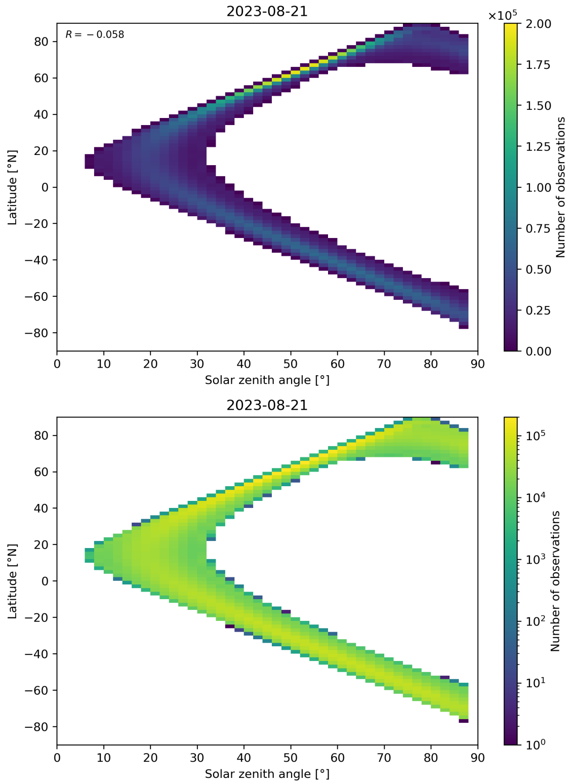
Figure 124: Scatter density plot of “Solar zenith angle” against “Latitude” for 2023-08-20 to 2023-08-22.
