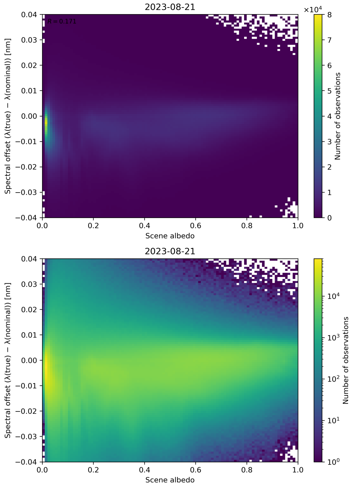
Figure 117: Scatter density plot of “Scene albedo” against “Spectral offset ( \lambda(\text{true}) - \lambda(\text{nominal}) )” for 2023-08-20 to 2023-08-22.
