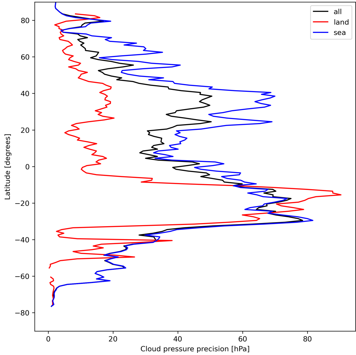
Figure 14: Zonal average of “Cloud pressure precision” for 2023-08-20 to 2023-08-22.
