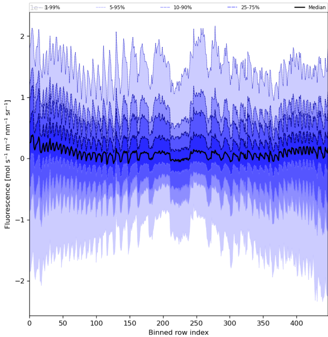
Figure 57: Along track statistics of “Fluorescence” for 2023-08-20 to 2023-08-22
