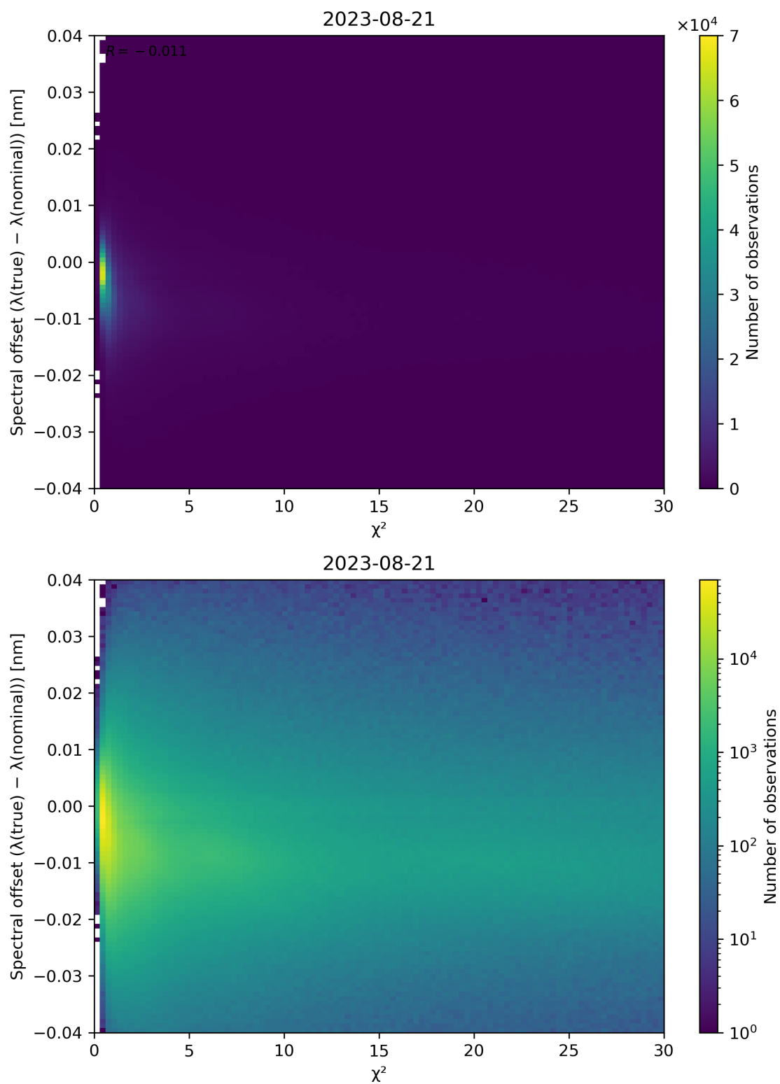
Figure 75: Scatter density plot of " \chi^2 " against "Spectral offset ( \lambda(\text{true}) - \lambda(\text{nominal}) )" for 2023-08-20 to 2023-08-22.
