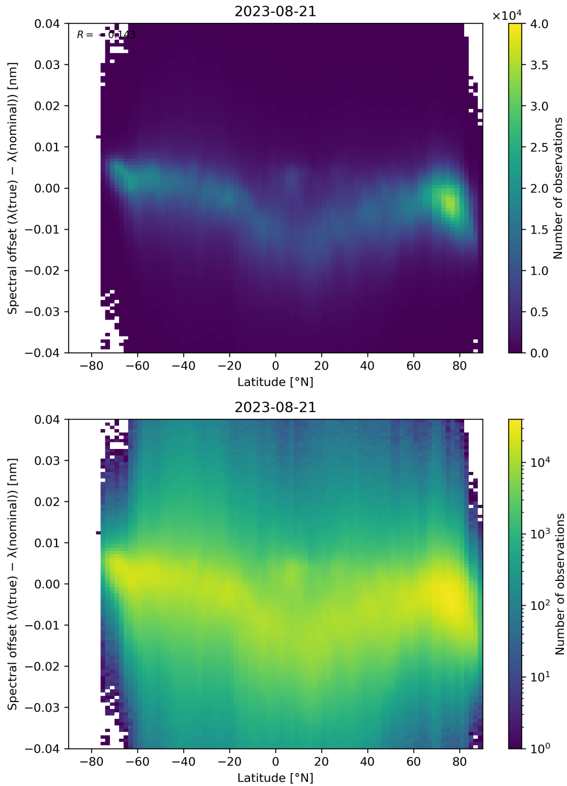
Figure 105: Scatter density plot of “Latitude” against “Spectral offset ( \lambda(\text{true}) - \lambda(\text{nominal}) )” for 2023-08-20 to 2023-08-22.
