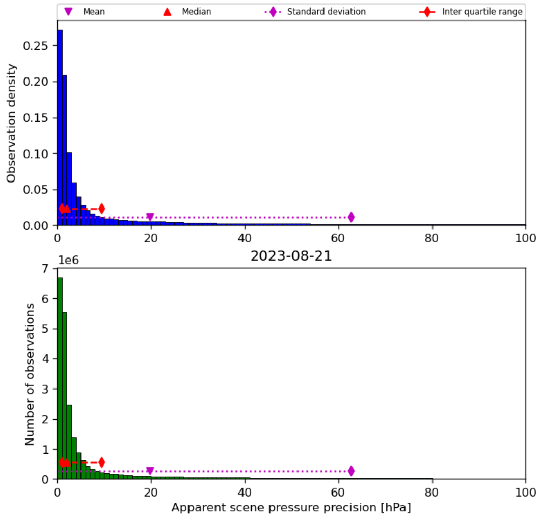
Figure 37: Histogram of “Apparent scene pressure precision” for 2023-08-20 to 2023-08-22
