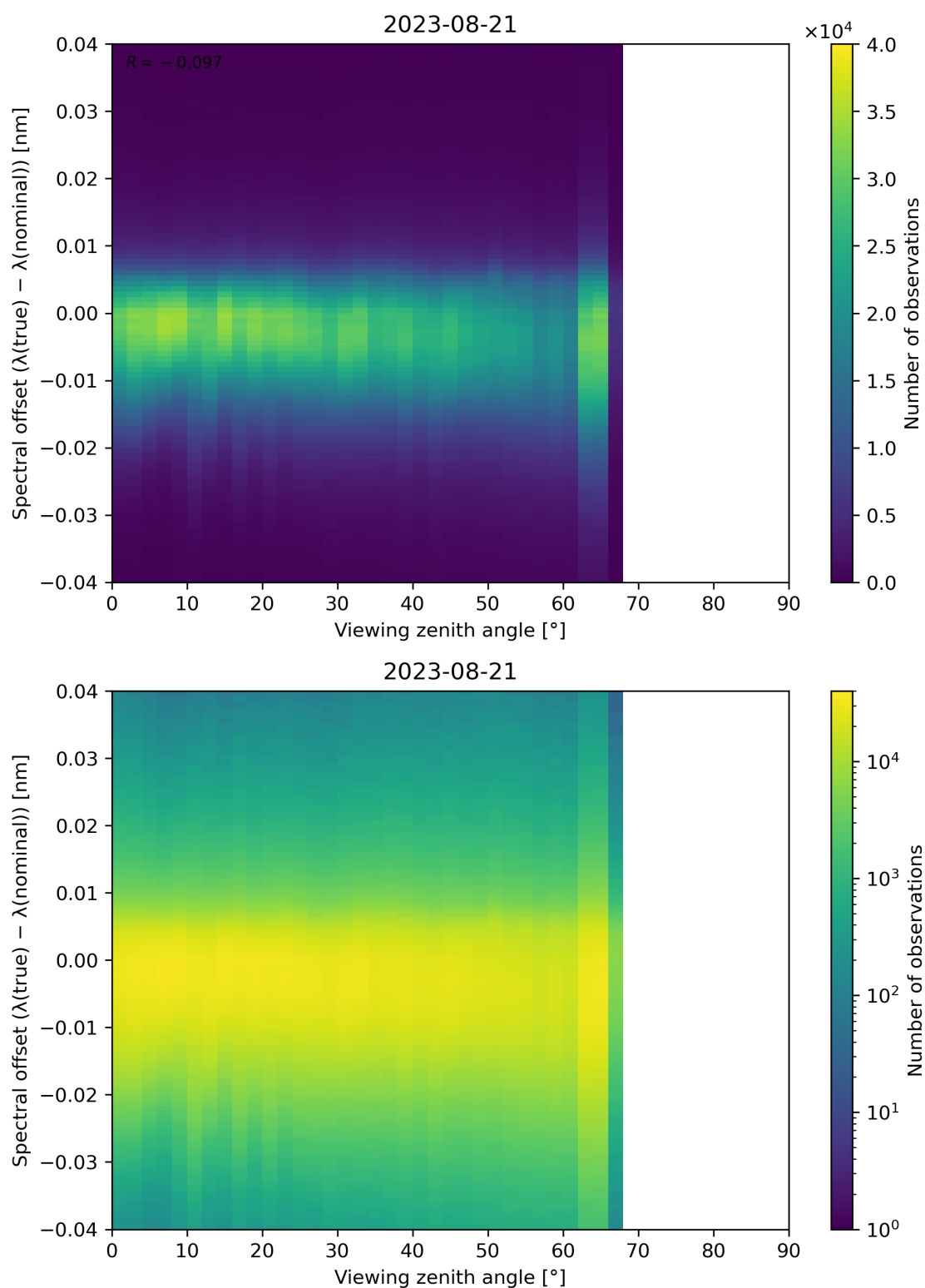
Figure 140: Scatter density plot of “Viewing zenith angle” against “Spectral offset ( \lambda(\text{true}) - \lambda(\text{nominal}) )” for 2023-08-20 to 2023-08-22.
