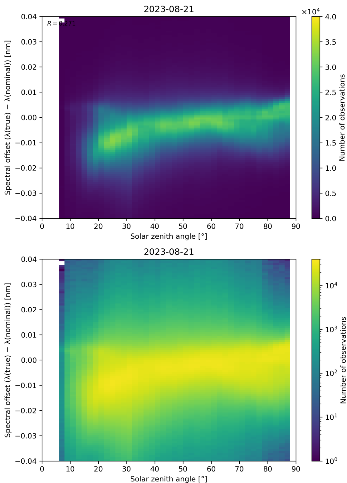
Figure 128: Scatter density plot of “Solar zenith angle” against “Spectral offset ( \lambda(\text{true}) - \lambda(\text{nominal}) )” for 2023-08-20 to 2023-08-22.
