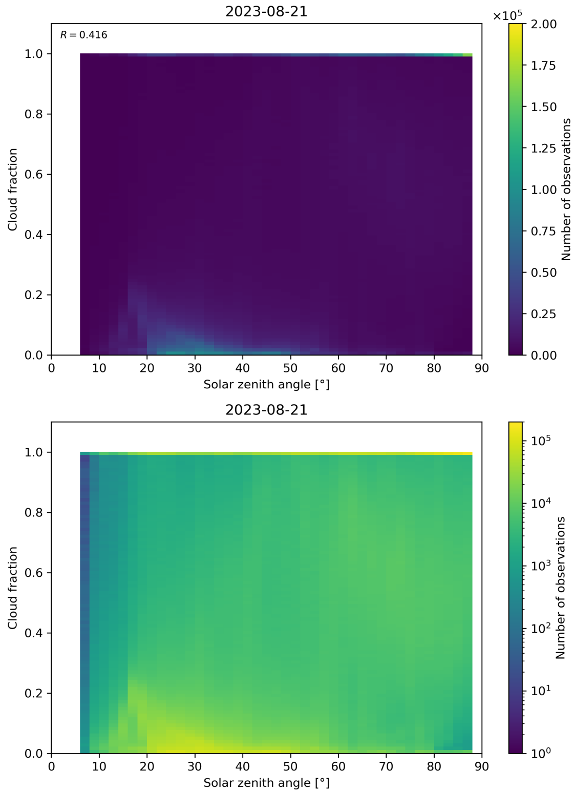
Figure 121: Scatter density plot of “Solar zenith angle” against “Cloud fraction” for 2023-08-20 to 2023-08-22.
