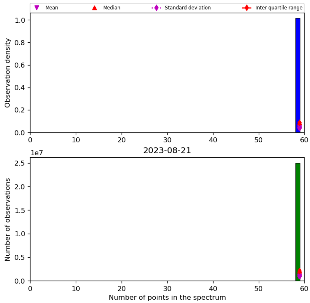
Figure 44: Histogram of “Number of points in the spectrum” for 2023-08-20 to 2023-08-22
