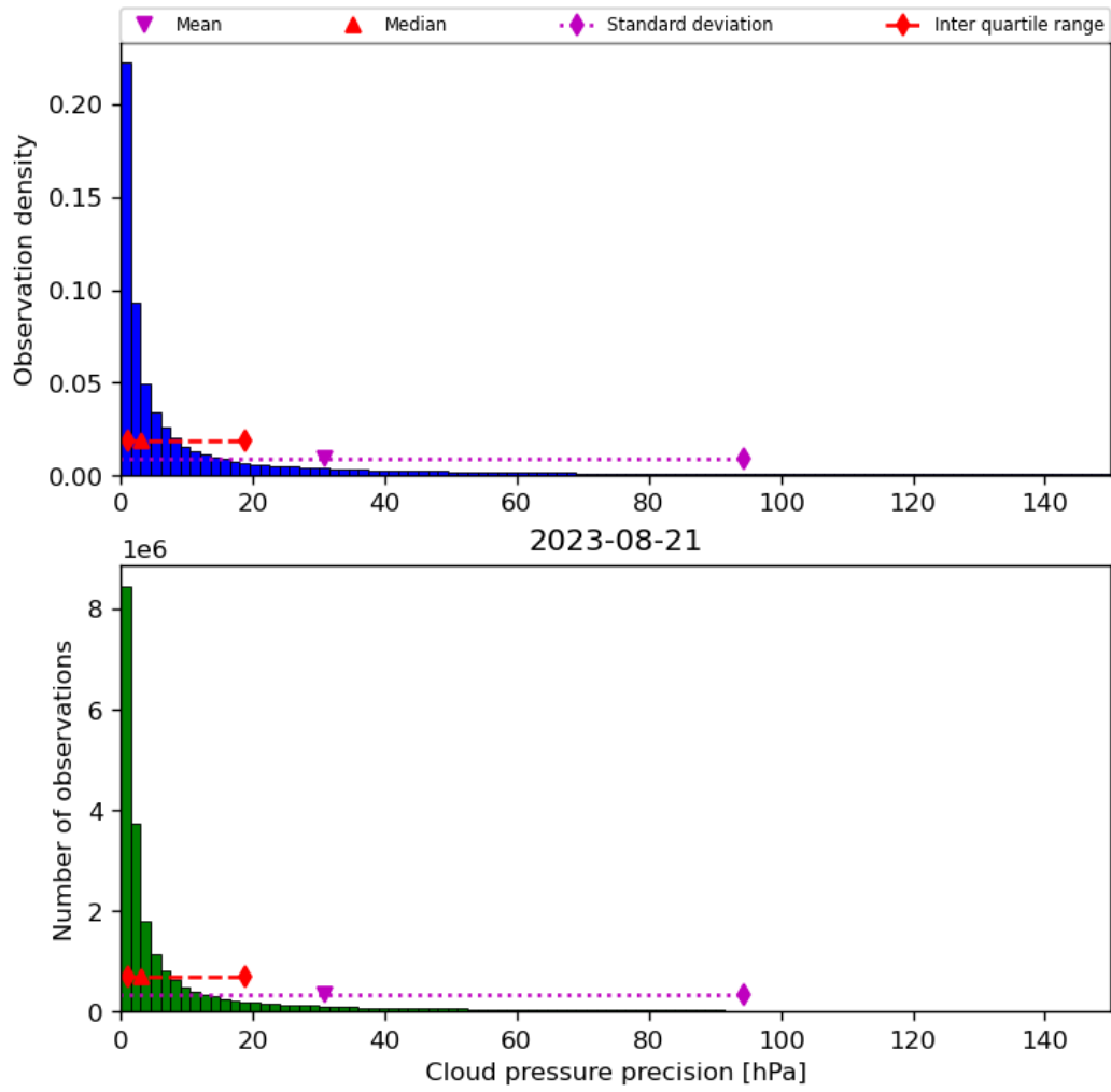
Figure 31: Histogram of “Cloud pressure precision” for 2023-08-20 to 2023-08-22
