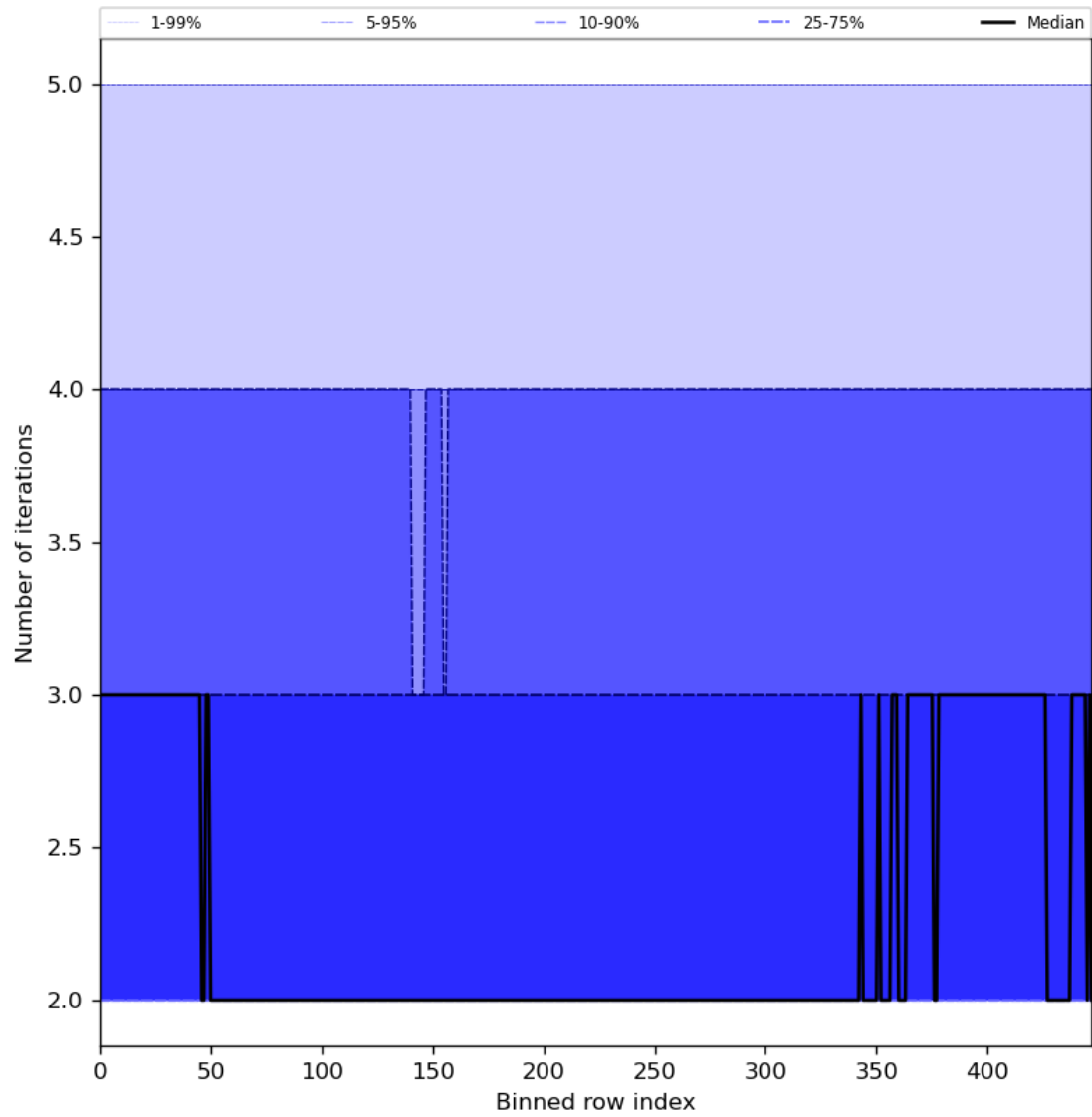
Figure 56: Along track statistics of “Number of iterations” for 2023-08-20 to 2023-08-22
