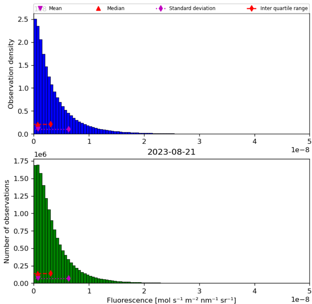
Figure 40: Histogram of “Fluorescence” for 2023-08-20 to 2023-08-22
