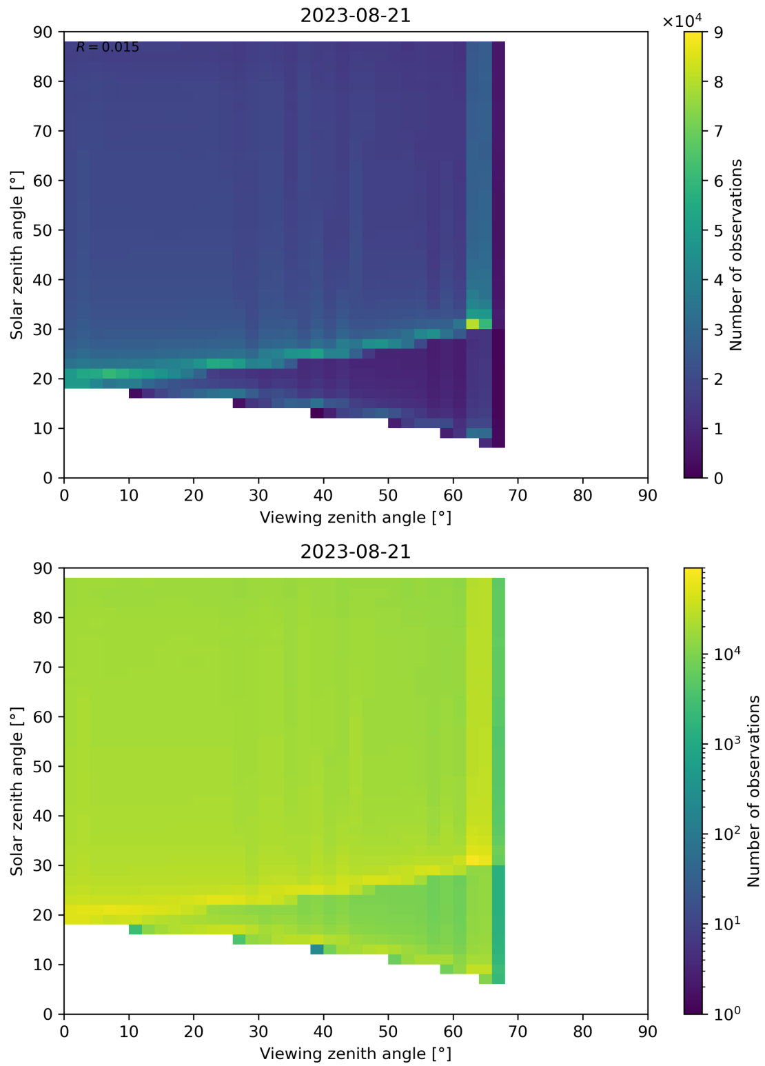
Figure 139: Scatter density plot of “Viewing zenith angle” against “Solar zenith angle” for 2023-08-20 to 2023-08-22.
