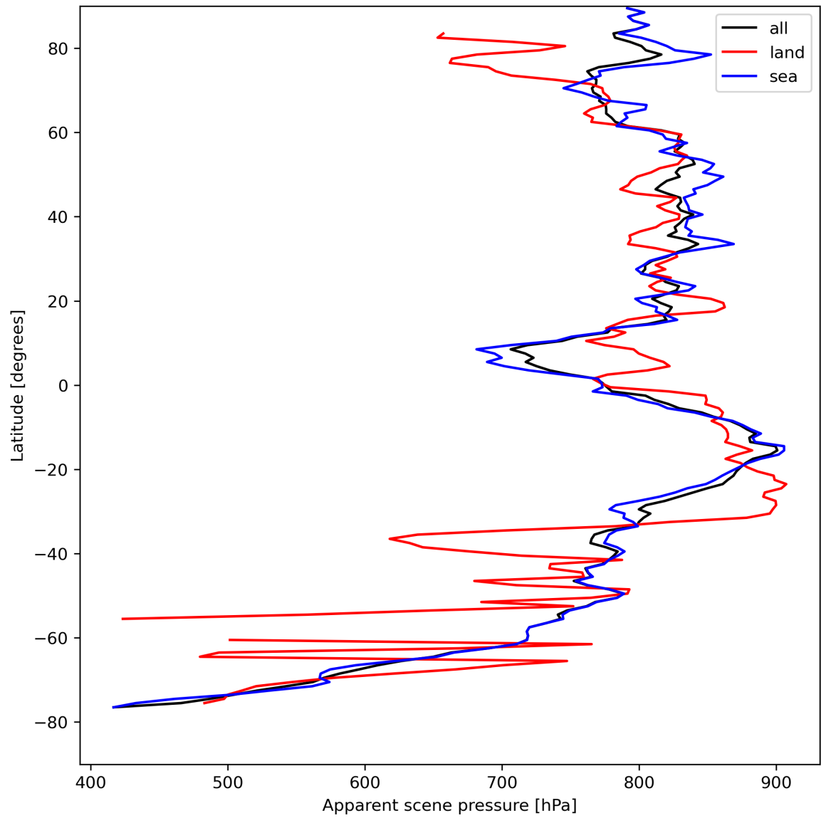
Figure 19: Zonal average of “Apparent scene pressure” for 2023-08-20 to 2023-08-22.
