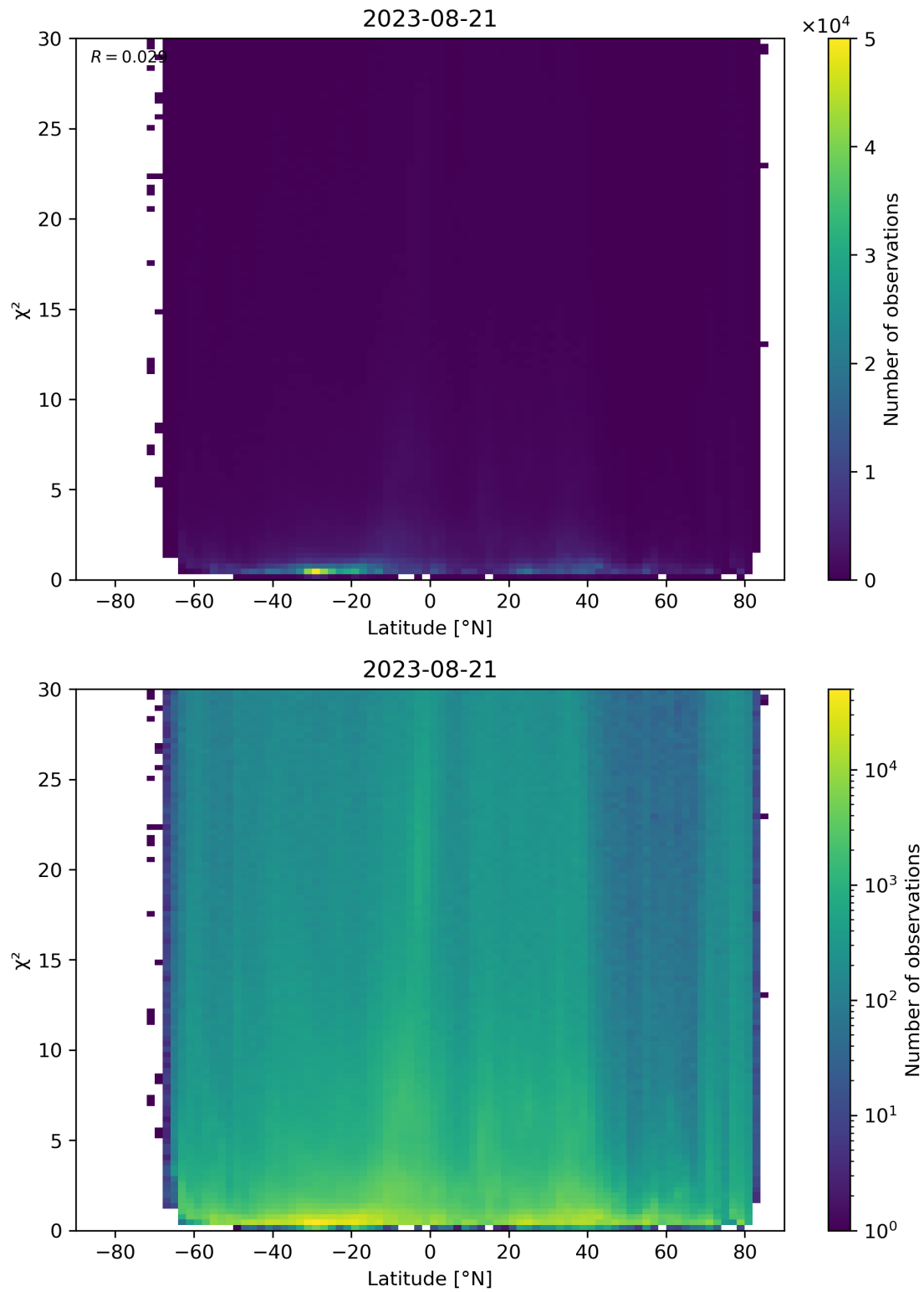
Figure 97: Scatter density plot of “Latitude” against “ \chi^2 ” for 2023-08-20 to 2023-08-22.
