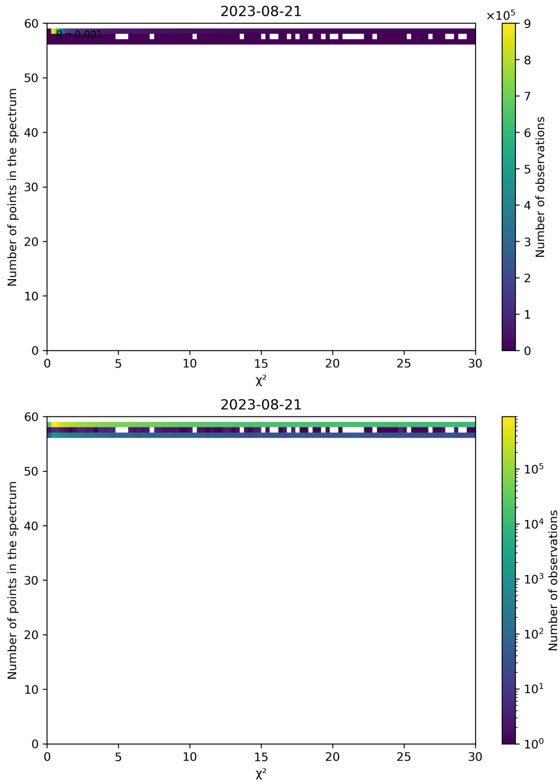
Figure 74: Scatter density plot of " \chi^2 " against "Number of points in the spectrum" for 2023-08-20 to 2023-08-22.
