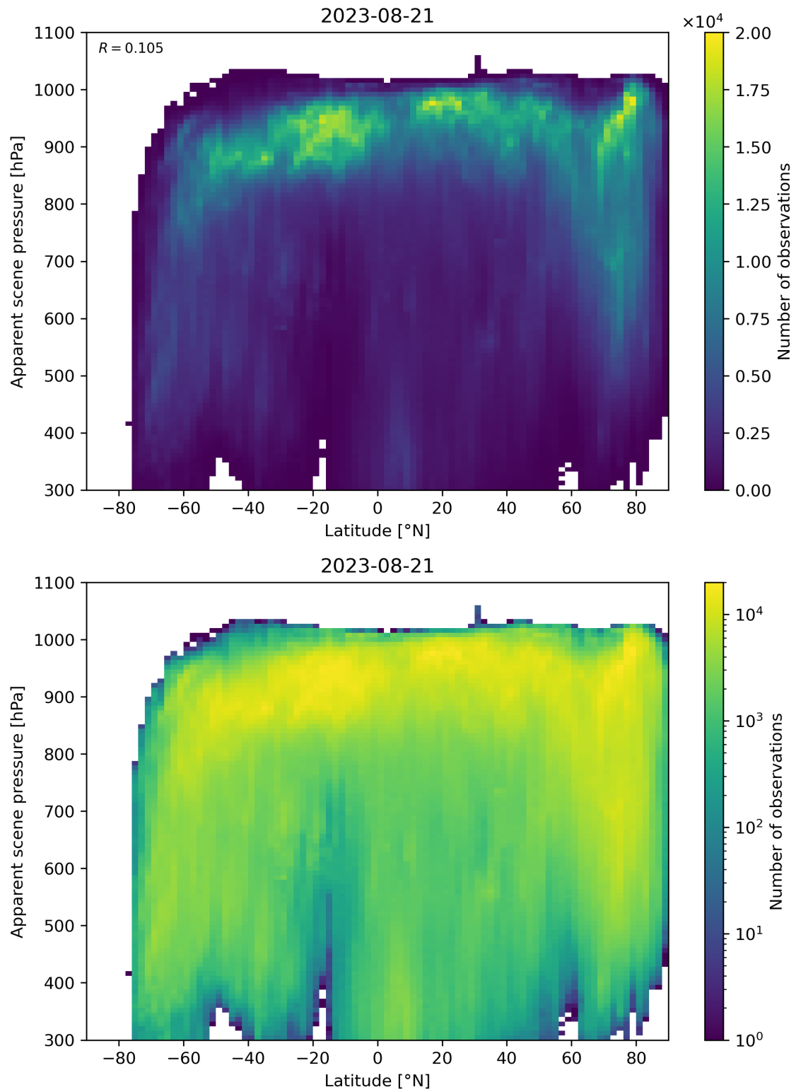
Figure 96: Scatter density plot of “Latitude” against “Apparent scene pressure” for 2023-08-20 to 2023-08-22.
