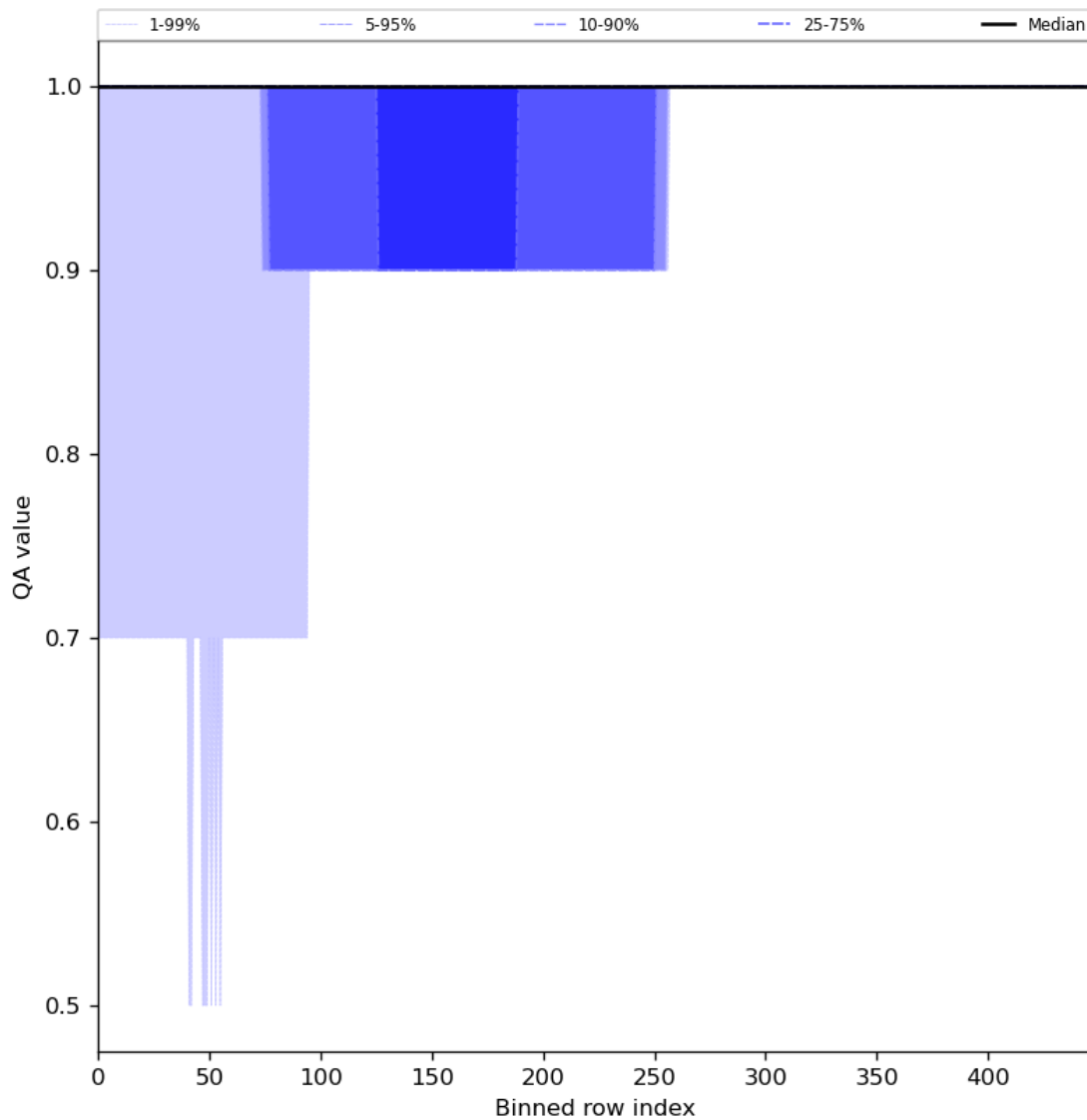
Figure 46: Along track statistics of "QA value" for 2023-08-20 to 2023-08-22
