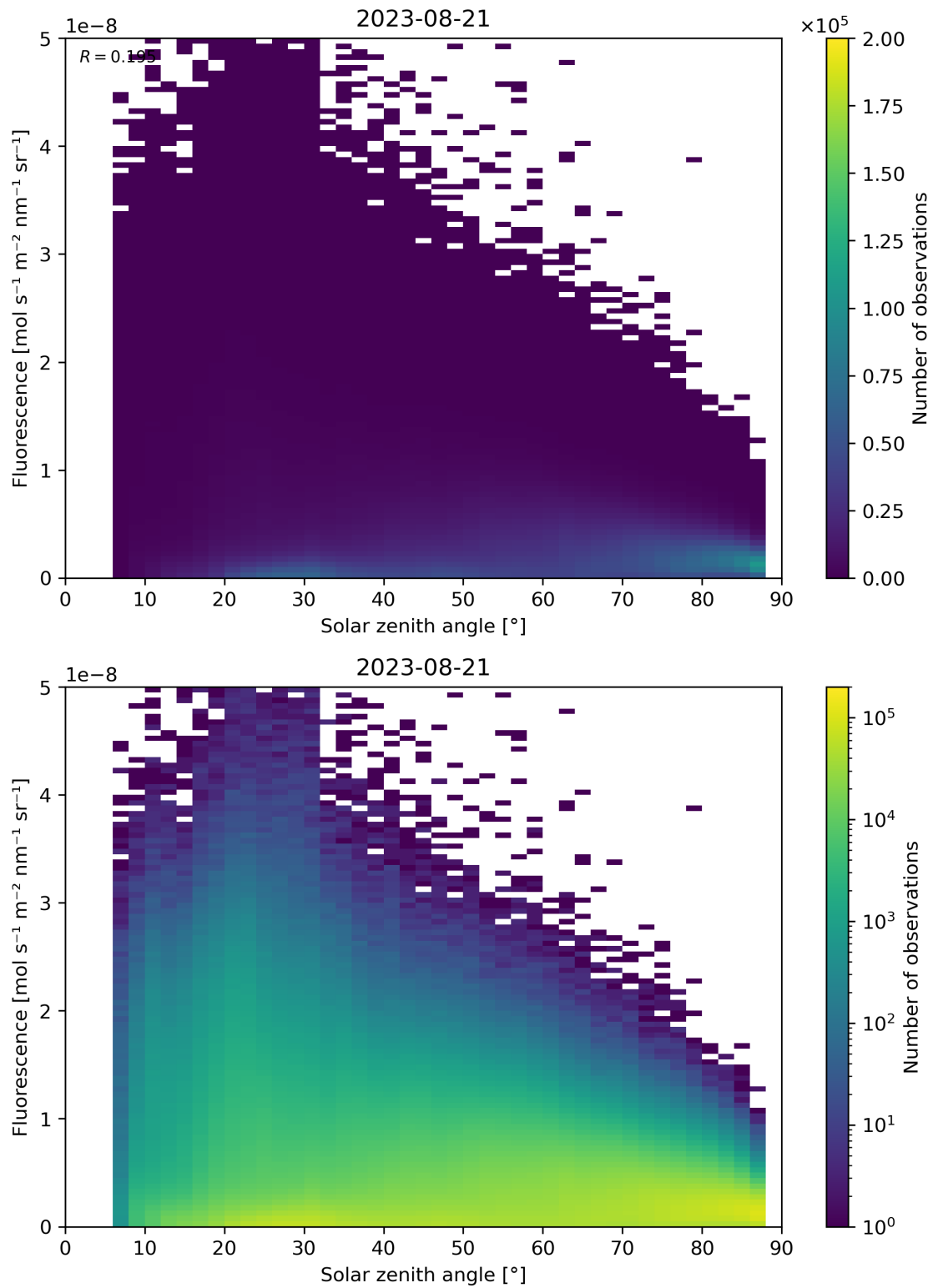
Figure 123: Scatter density plot of “Solar zenith angle” against “Fluorescence” for 2023-08-20 to 2023-08-22.
