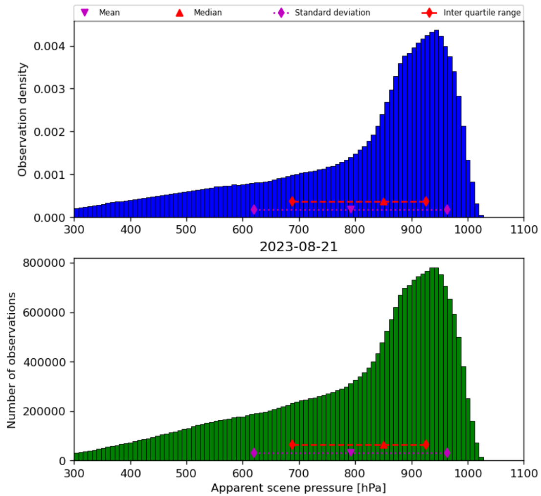
Figure 36: Histogram of “Apparent scene pressure” for 2023-08-20 to 2023-08-22
