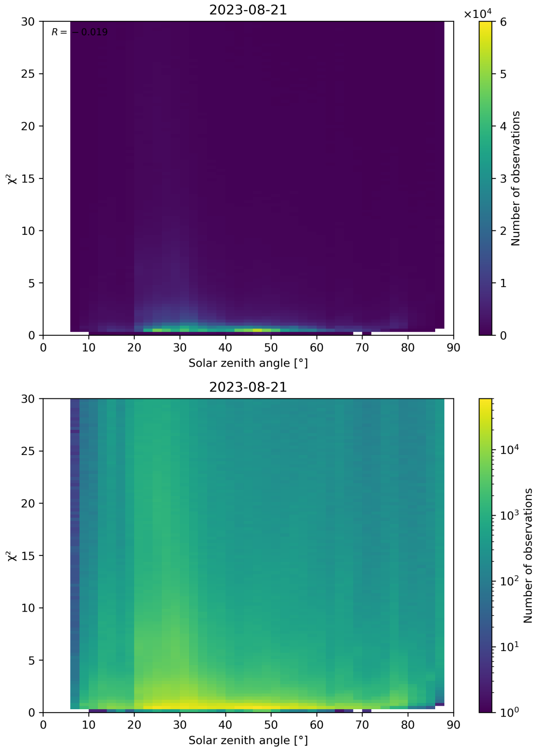
Figure 119: Scatter density plot of “Solar zenith angle” against “ \chi^2 ” for 2023-08-20 to 2023-08-22.
