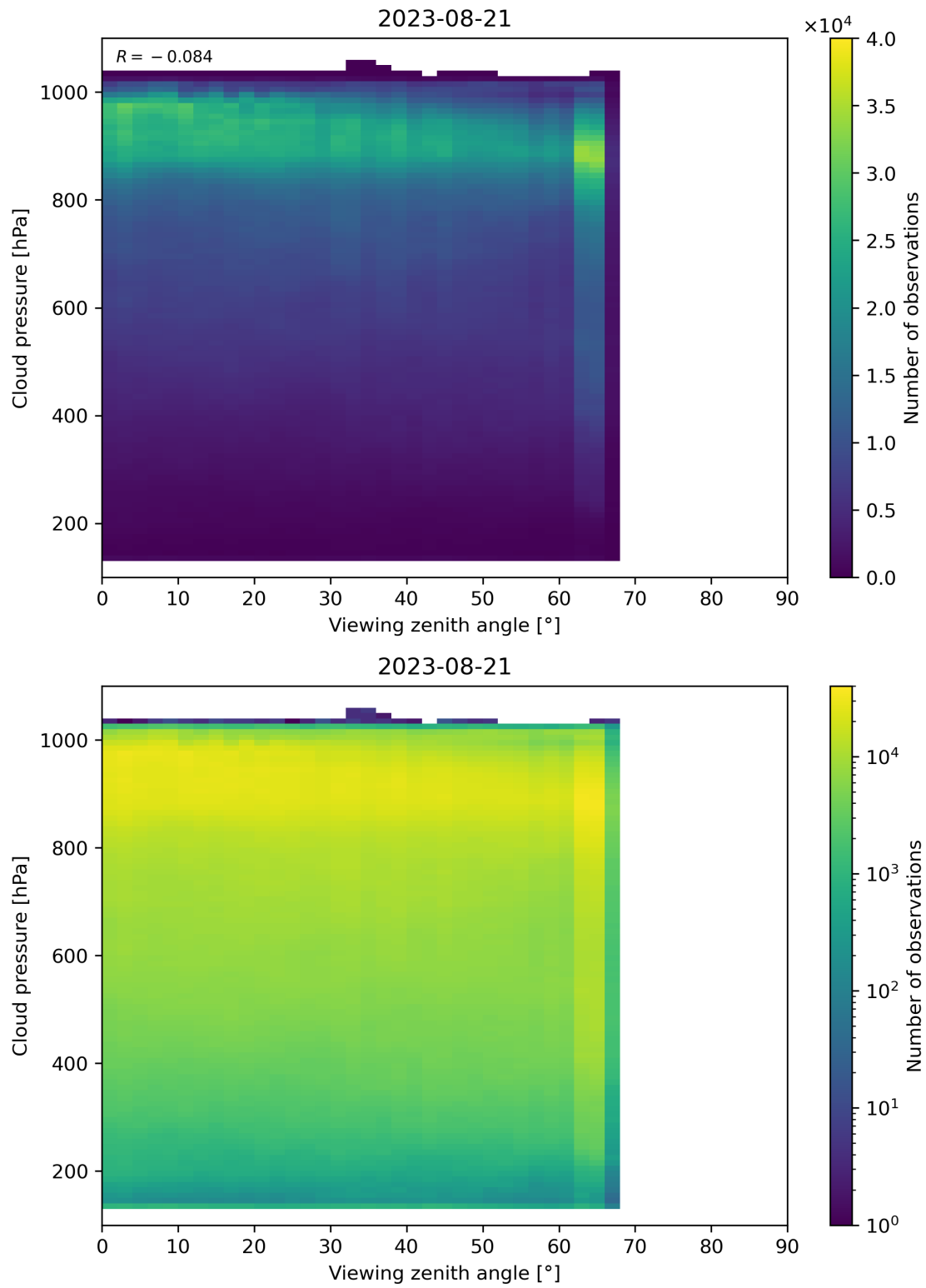
Figure 133: Scatter density plot of “Viewing zenith angle” against “Cloud pressure” for 2023-08-20 to 2023-08-22.
