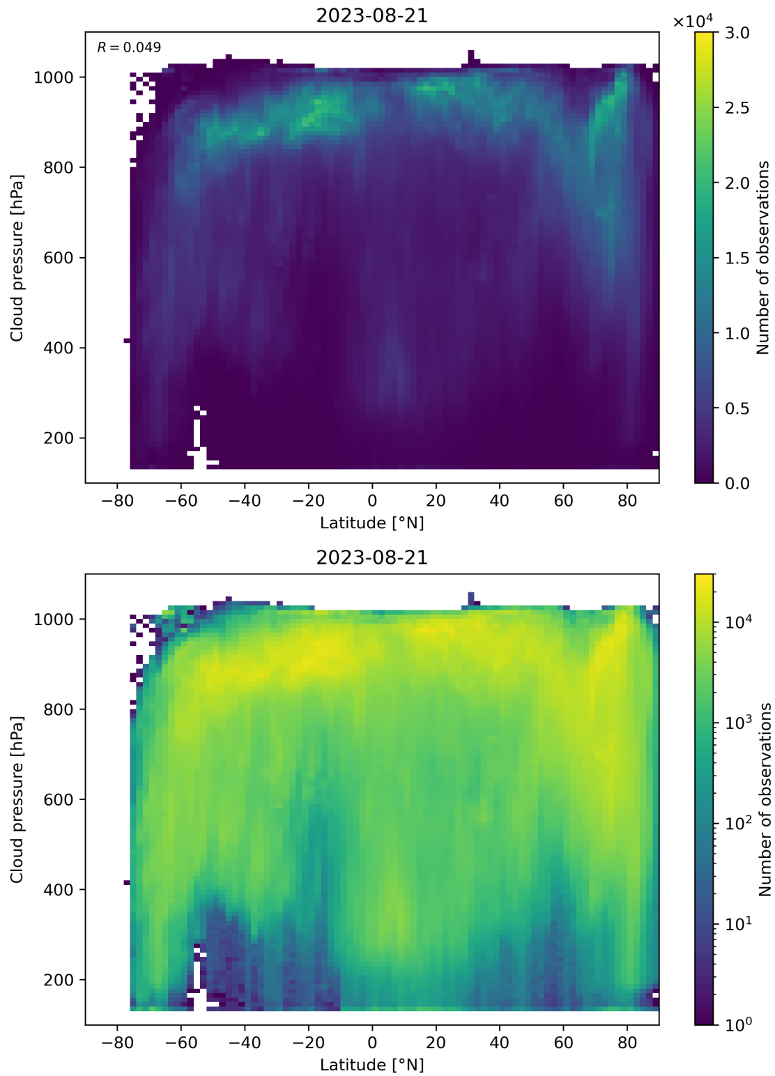
Figure 100: Scatter density plot of “Latitude” against “Cloud pressure” for 2023-08-20 to 2023-08-22.
