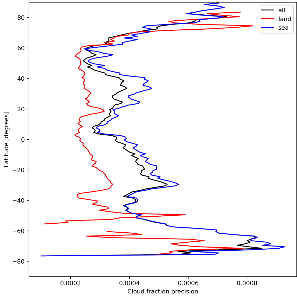
Figure 16: Zonal average of “Cloud fraction precision” for 2023-08-20 to 2023-08-22.
