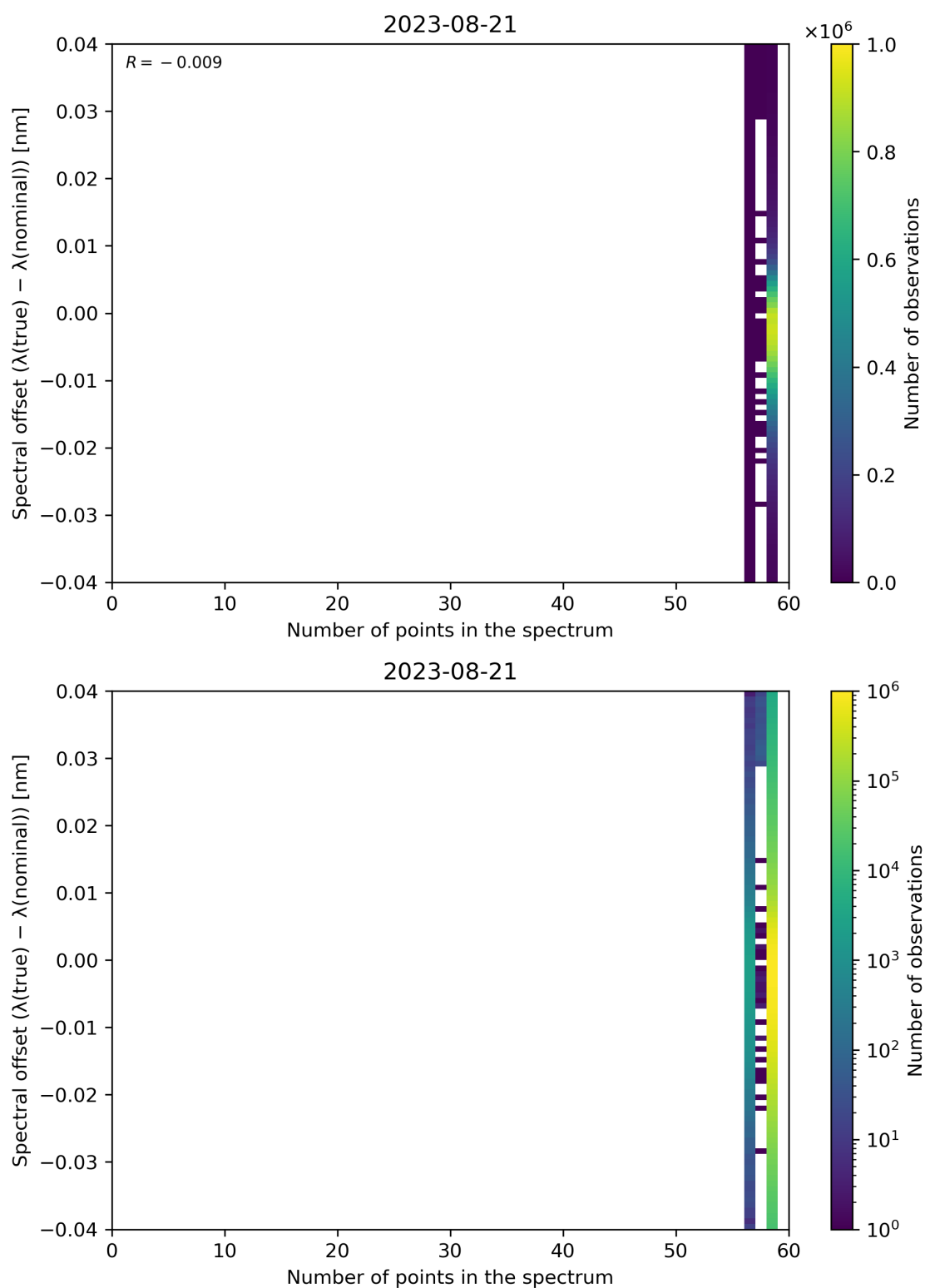
Figure 110: Scatter density plot of “Number of points in the spectrum” against “Spectral offset ( \lambda(\text{true}) - \lambda(\text{nominal}) )” for 2023-08-20 to 2023-08-22.
