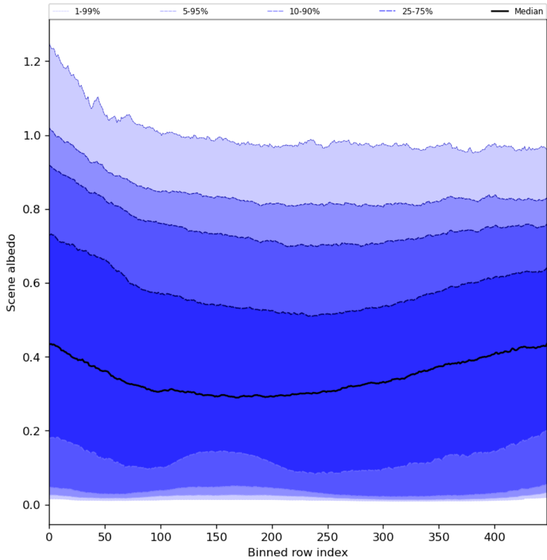
Figure 51: Along track statistics of “Scene albedo” for 2023-08-20 to 2023-08-22
