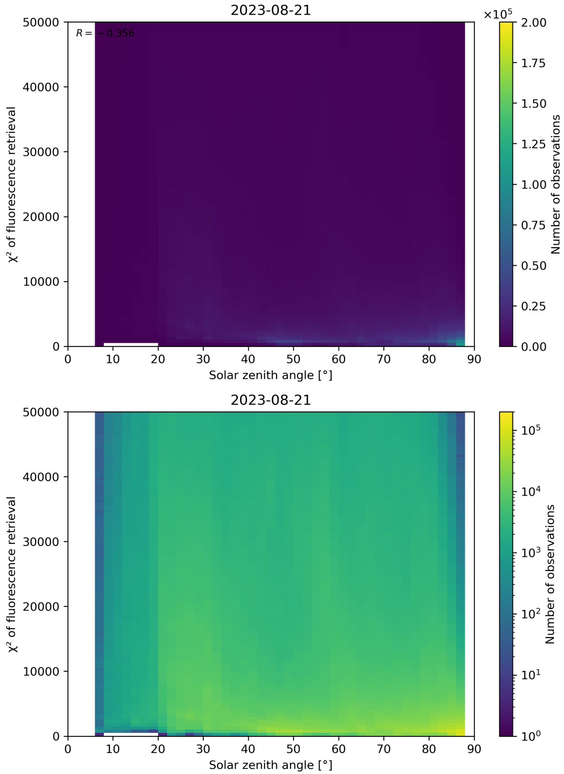
Figure 120: Scatter density plot of “Solar zenith angle” against “ \chi^2 of fluorescence retrieval” for 2023-08-20 to 2023-08-22.
