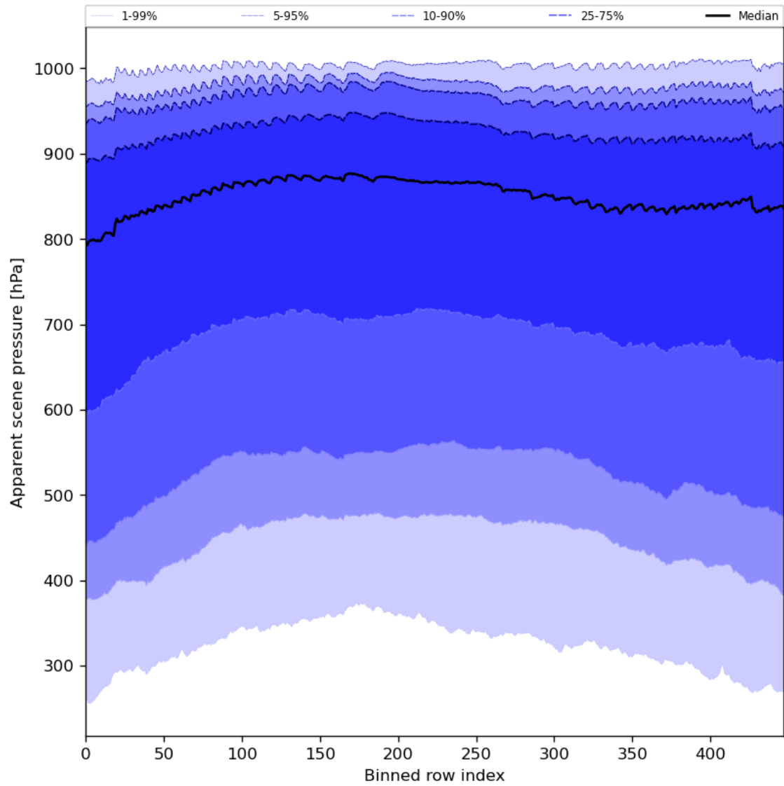
Figure 53: Along track statistics of “Apparent scene pressure” for 2023-08-20 to 2023-08-22
