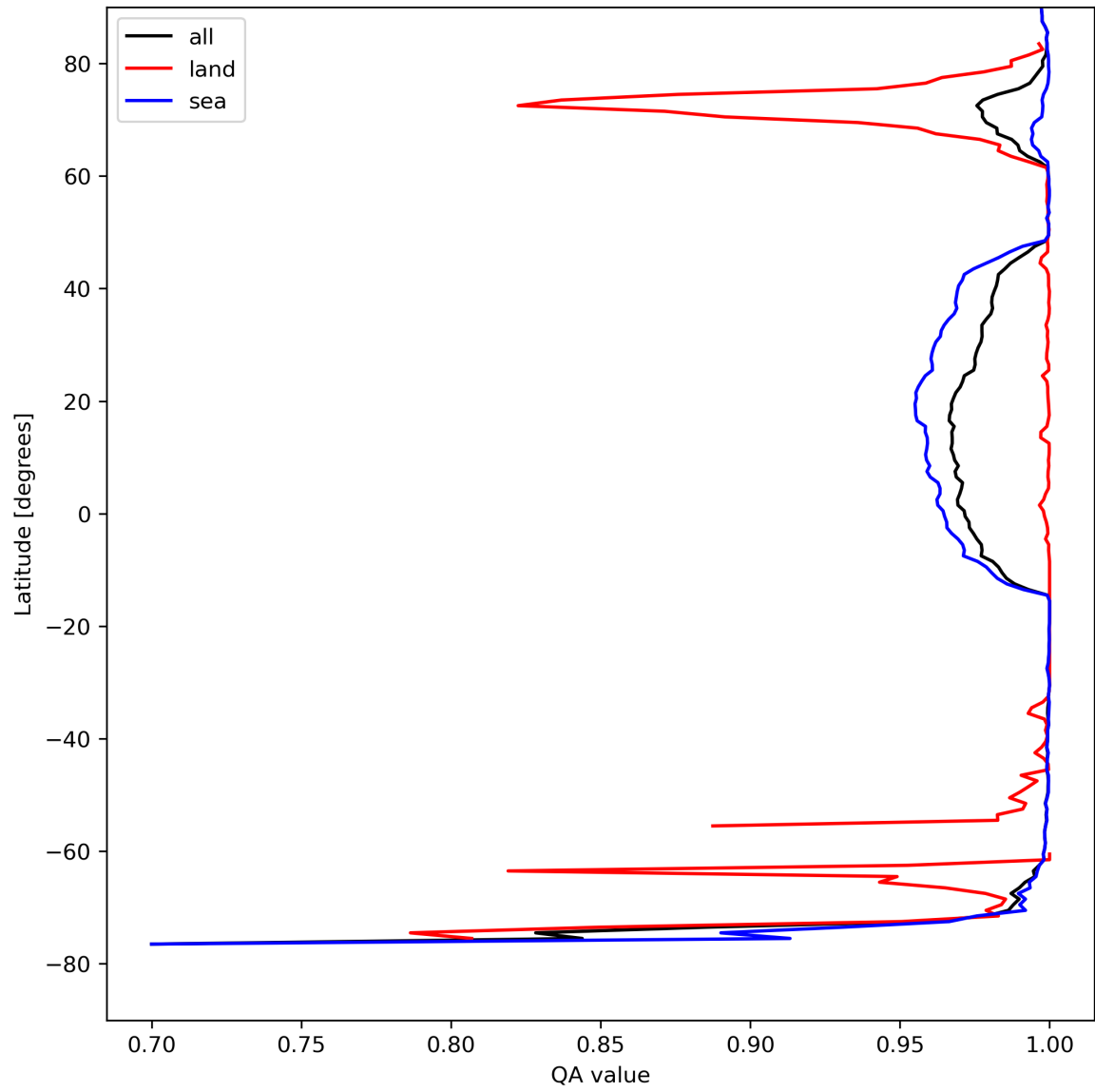
Figure 12: Zonal average of "QA value" for 2023-08-20 to 2023-08-22.
