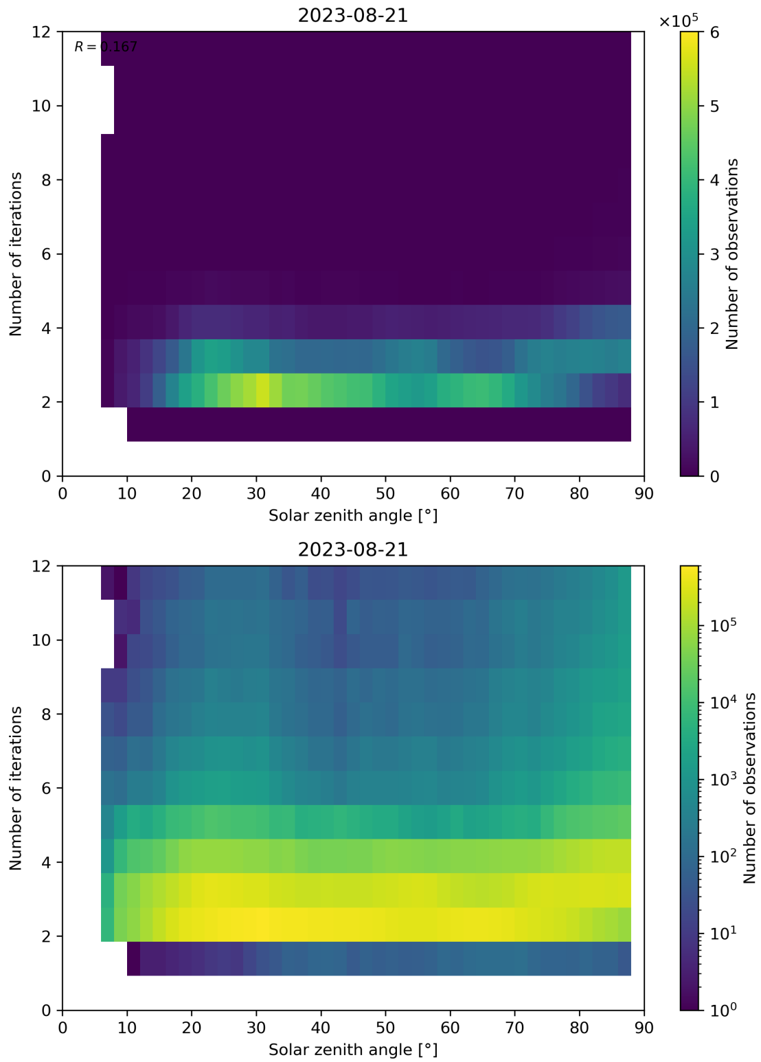
Figure 125: Scatter density plot of “Solar zenith angle” against “Number of iterations” for 2023-08-20 to 2023-08-22.
