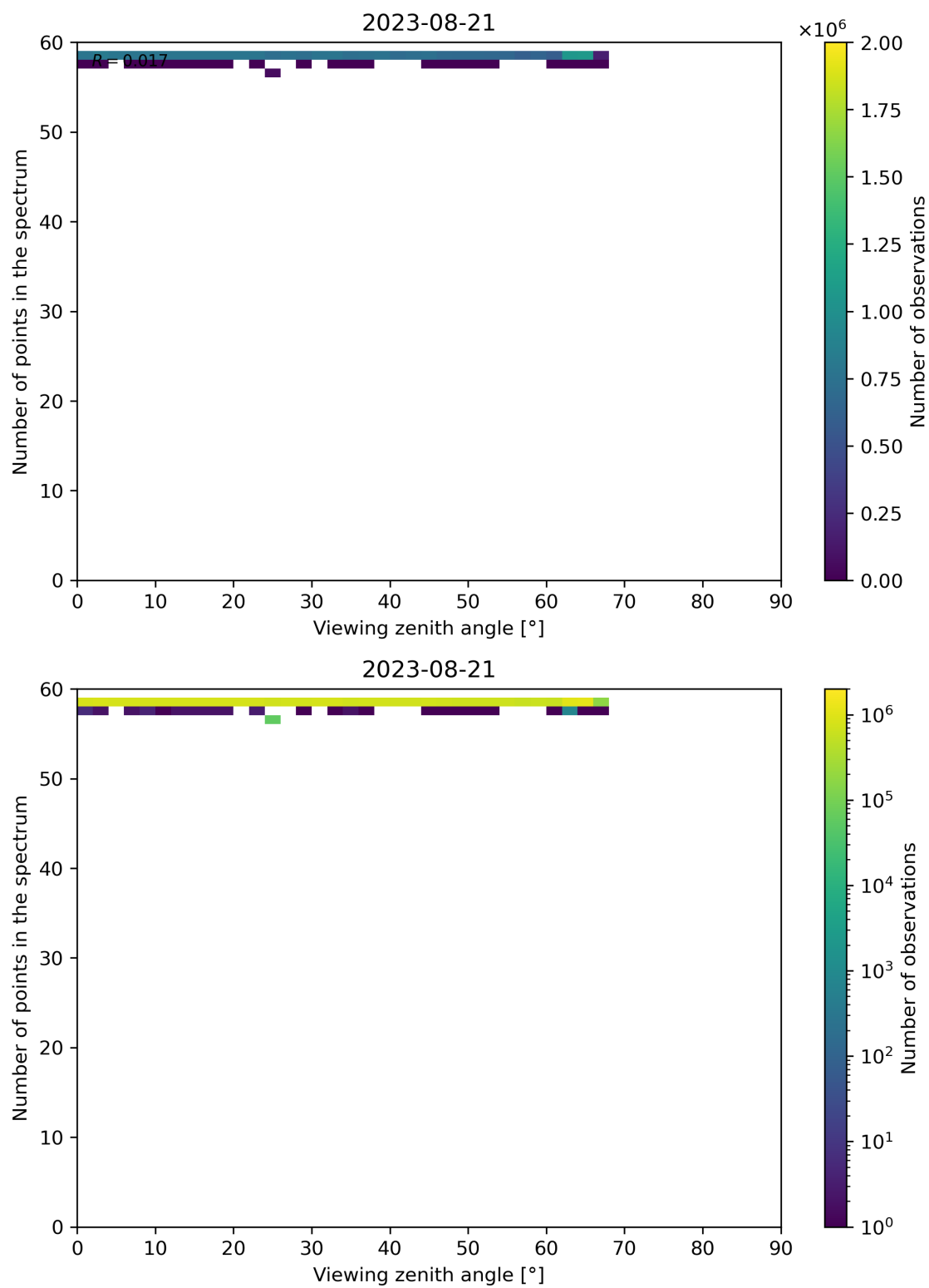
Figure 137: Scatter density plot of “Viewing zenith angle” against “Number of points in the spectrum” for 2023-08-20 to 2023-08-22.
