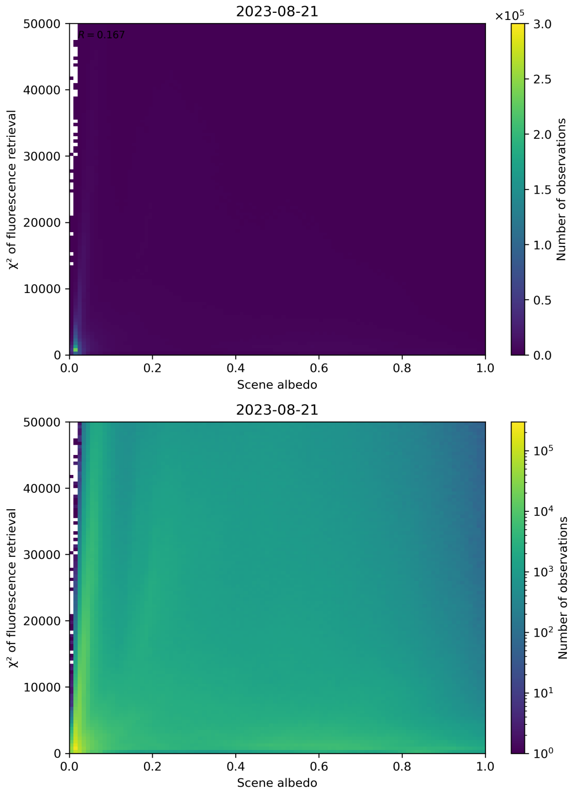
Figure 113: Scatter density plot of “Scene albedo” against “ \chi^2 of fluorescence retrieval” for 2023-08-20 to 2023-08-22.
