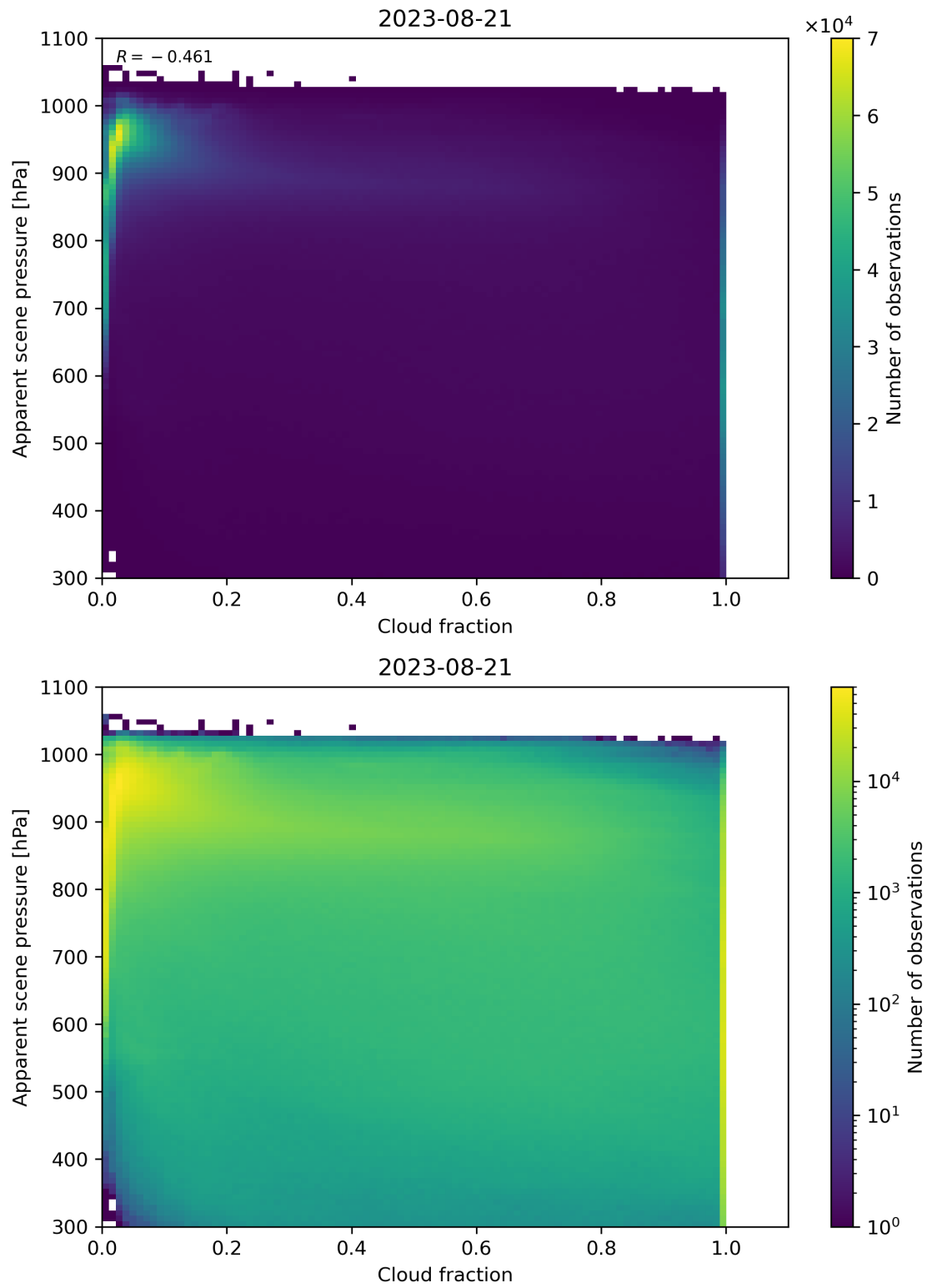
Figure 76: Scatter density plot of “Cloud fraction” against “Apparent scene pressure” for 2023-08-20 to 2023-08-22.
