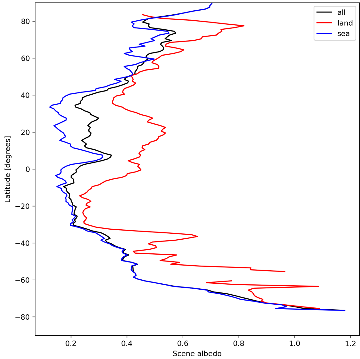
Figure 17: Zonal average of “Scene albedo” for 2023-08-20 to 2023-08-22.
