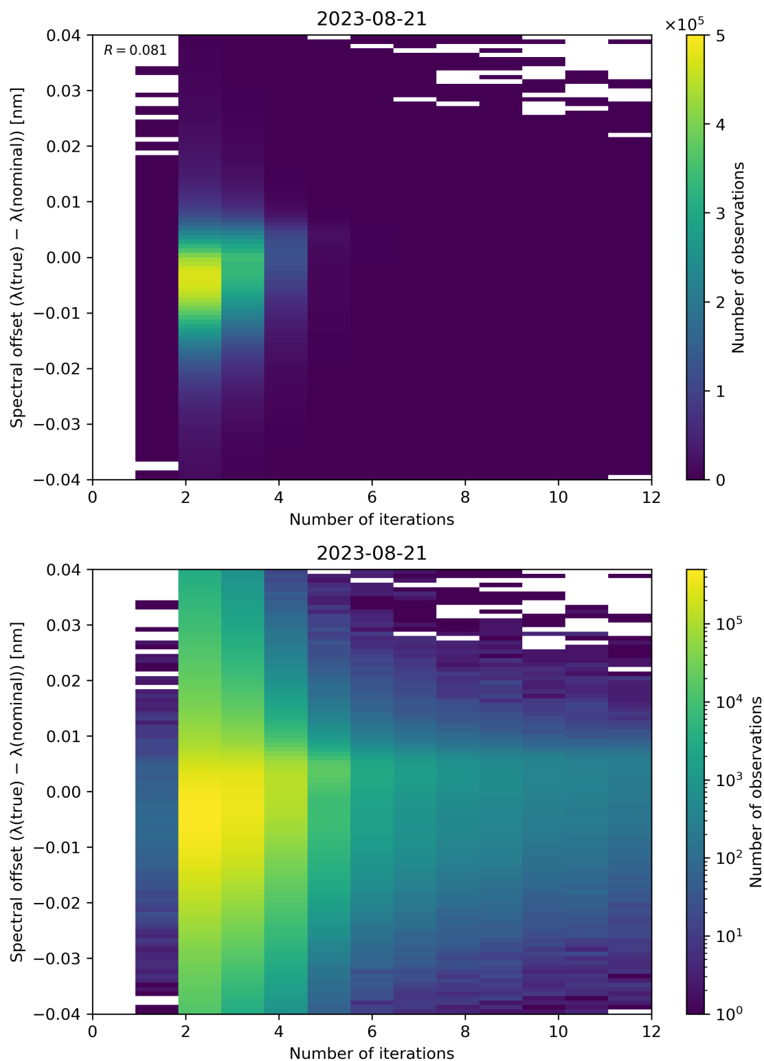
Figure 109: Scatter density plot of “Number of iterations” against “Spectral offset ( \lambda(\text{true}) - \lambda(\text{nominal}) )” for 2023-08-20 to 2023-08-22.
