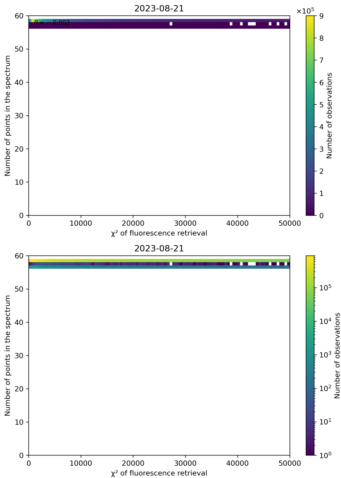
Figure 71: Scatter density plot of " \chi^2 of fluorescence retrieval" against "Number of points in the spectrum" for 2023-08-20 to 2023-08-22.
