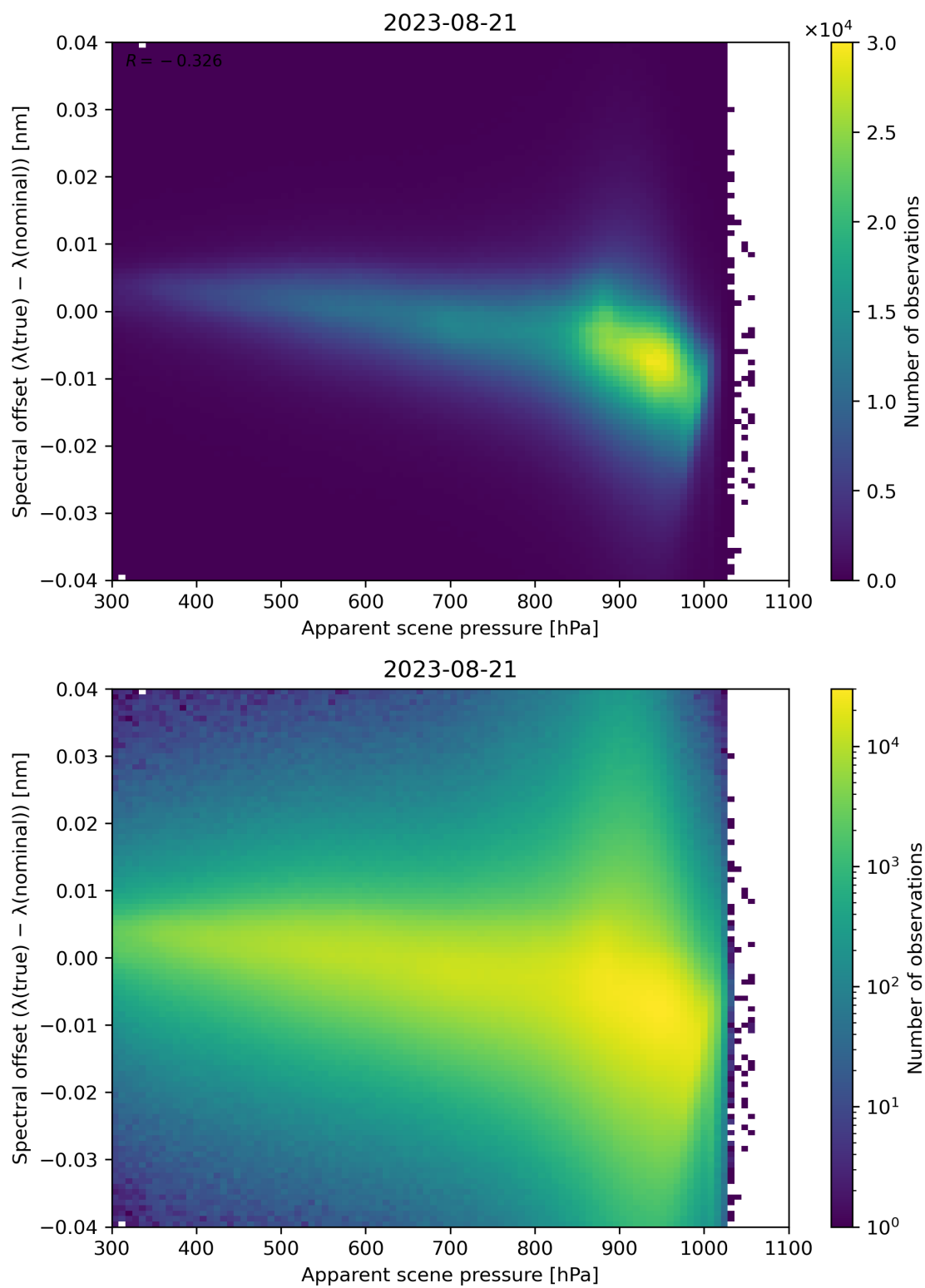
Figure 68: Scatter density plot of “Apparent scene pressure” against “Spectral offset ( \lambda(\text{true}) - \lambda(\text{nominal}) )” for 2023-08-20 to 2023-08-22.
