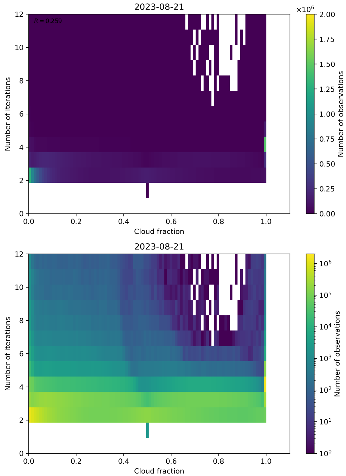
Figure 80: Scatter density plot of “Cloud fraction” against “Number of iterations” for 2023-08-20 to 2023-08-22.
