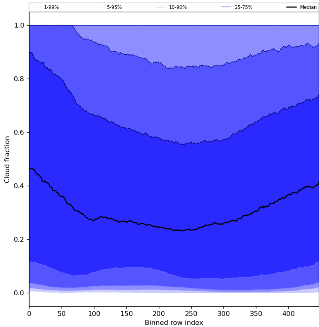
Figure 49: Along track statistics of “Cloud fraction” for 2023-08-20 to 2023-08-22
