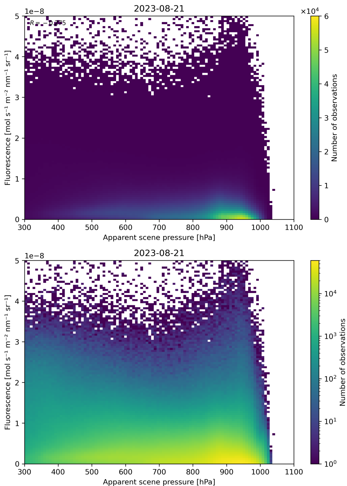
Figure 65: Scatter density plot of “Apparent scene pressure” against “Fluorescence” for 2023-08-20 to 2023-08-22.
