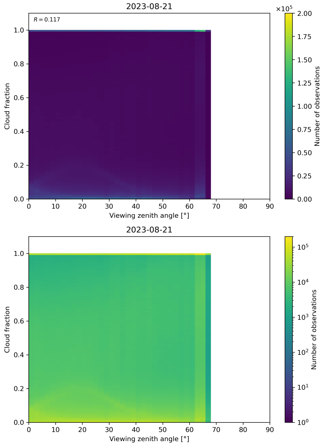
Figure 132: Scatter density plot of “Viewing zenith angle” against “Cloud fraction” for 2023-08-20 to 2023-08-22.
