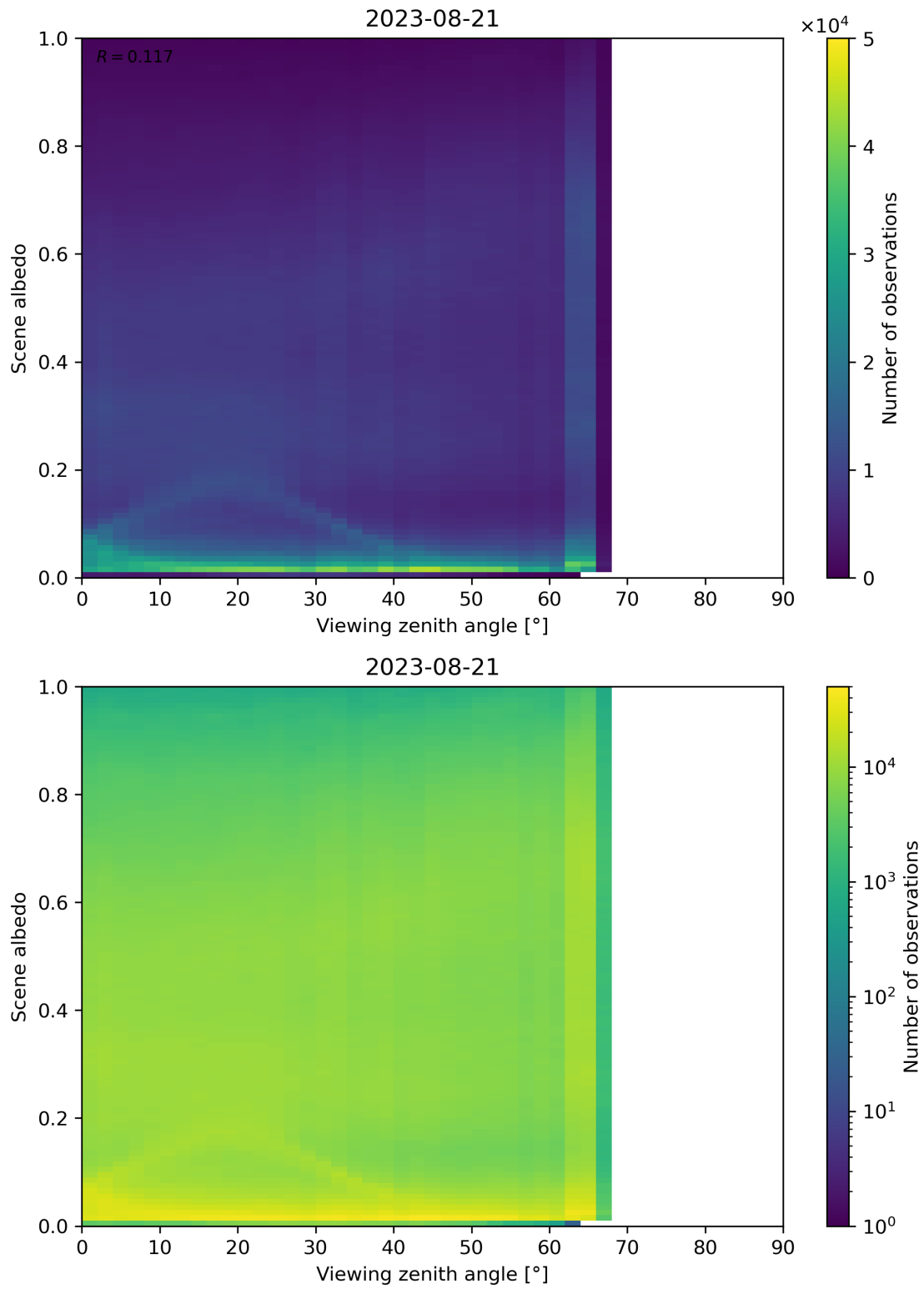
Figure 138: Scatter density plot of “Viewing zenith angle” against “Scene albedo” for 2023-08-20 to 2023-08-22.
