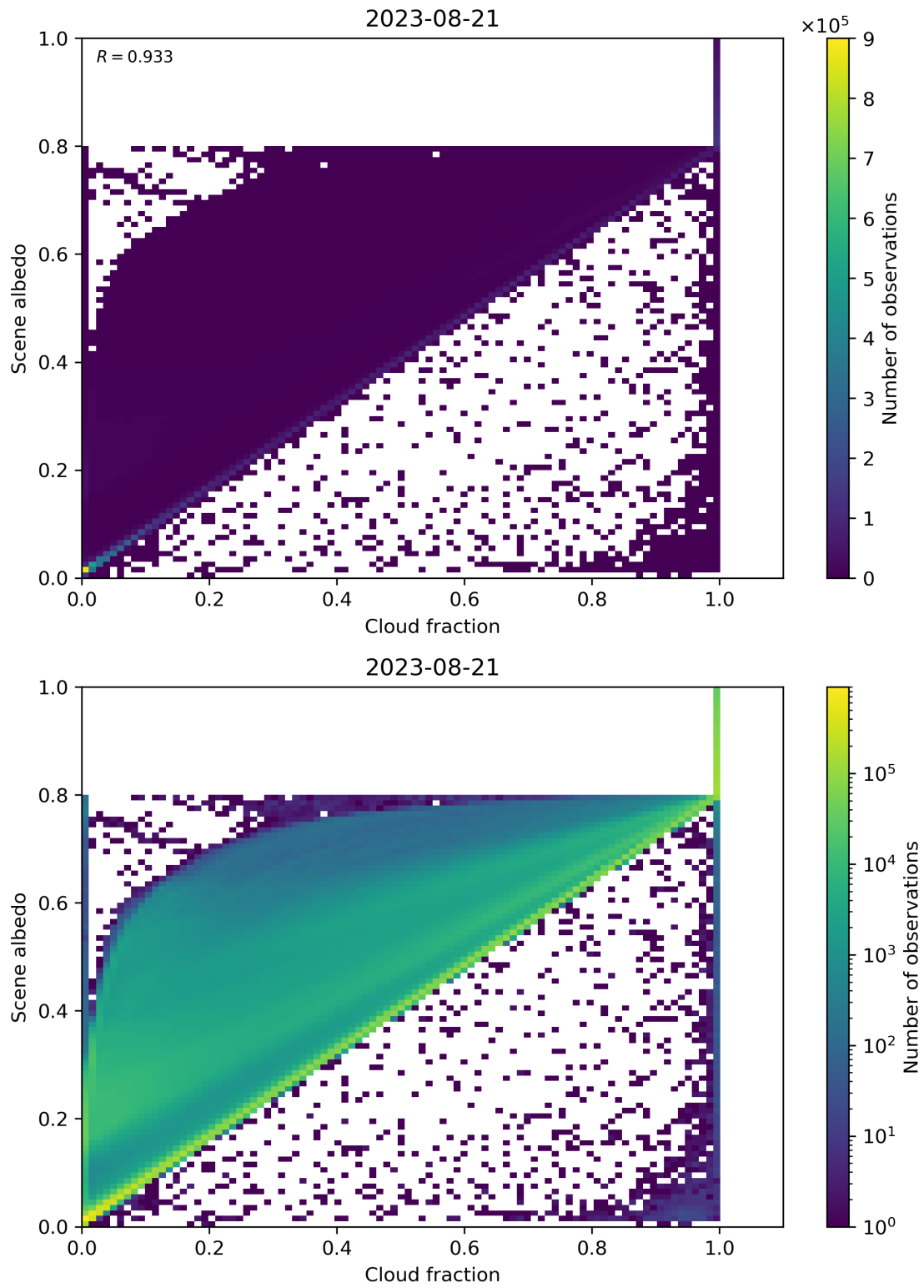
Figure 82: Scatter density plot of “Cloud fraction” against “Scene albedo” for 2023-08-20 to 2023-08-22.
