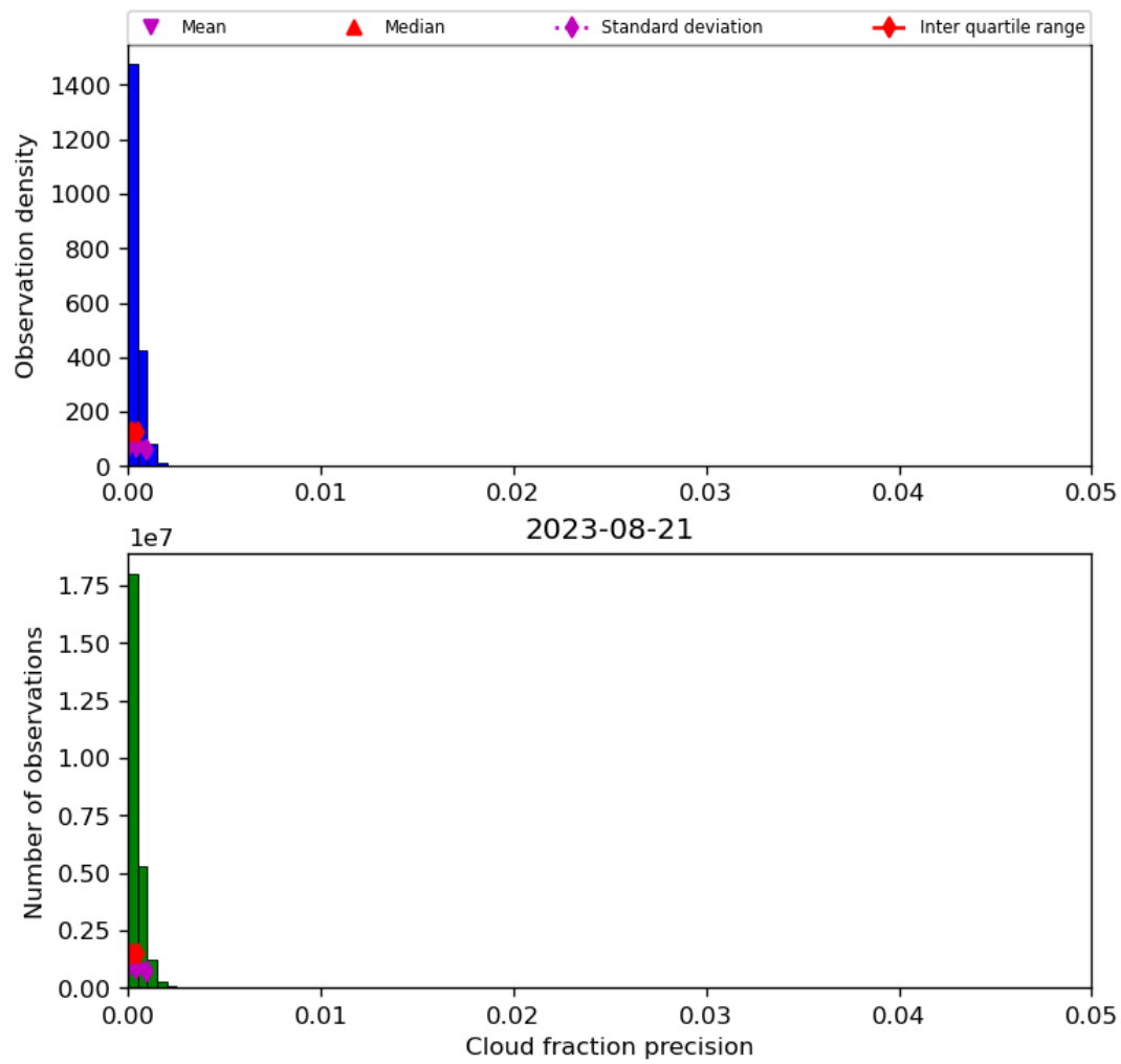
Figure 33: Histogram of "Cloud fraction precision" for 2023-08-20 to 2023-08-22
