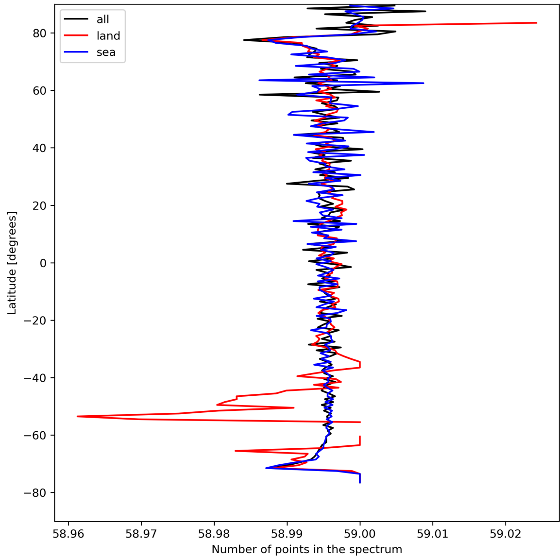
Figure 27: Zonal average of “Number of points in the spectrum” for 2023-08-20 to 2023-08-22.
