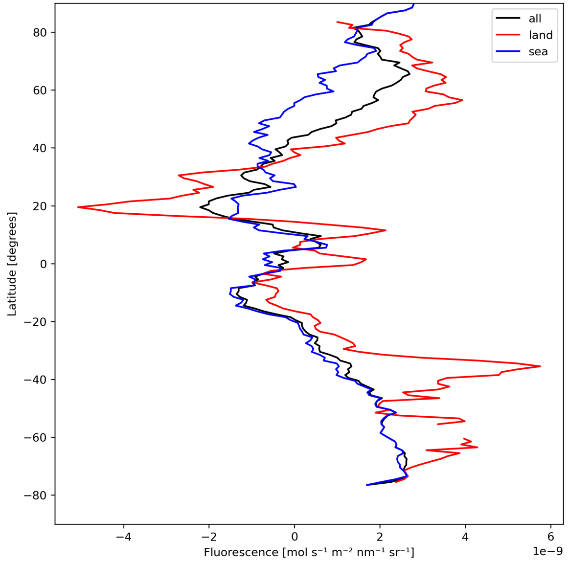
Figure 23: Zonal average of “Fluorescence” for 2023-08-20 to 2023-08-22.
