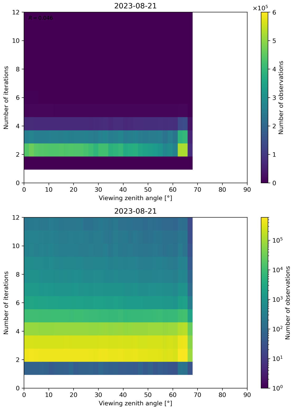
Figure 136: Scatter density plot of “Viewing zenith angle” against “Number of iterations” for 2023-08-20 to 2023-08-22.
