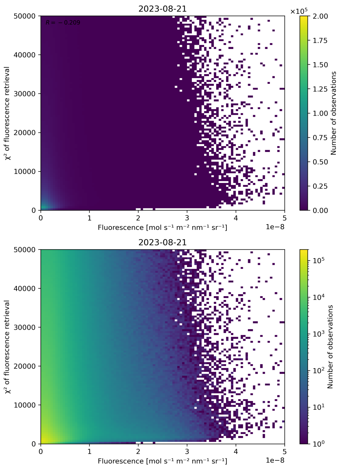
Figure 93: Scatter density plot of “Fluorescence” against “ \chi^2 of fluorescence retrieval” for 2023-08-20 to 2023-08-22.
