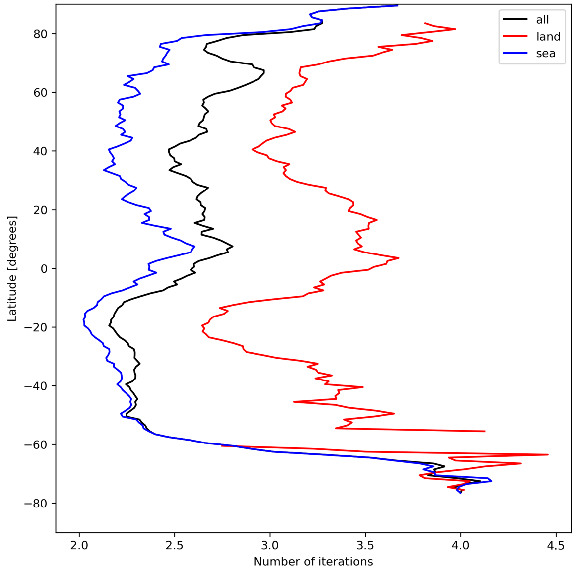
Figure 22: Zonal average of “Number of iterations” for 2023-08-20 to 2023-08-22.
