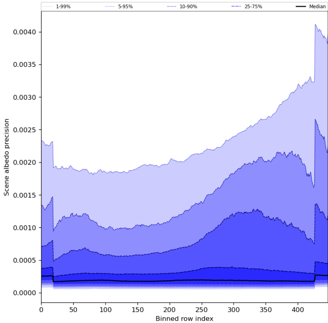
Figure 52: Along track statistics of “Scene albedo precision” for 2023-08-20 to 2023-08-22
