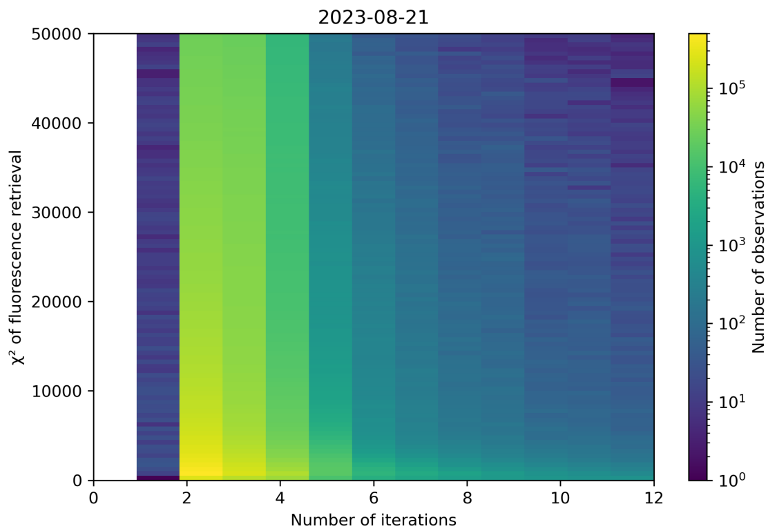
Figure 106: Scatter density plot of “Number of iterations” against “ \chi^2 of fluorescence retrieval” for 2023-08-20 to 2023-08-22.
