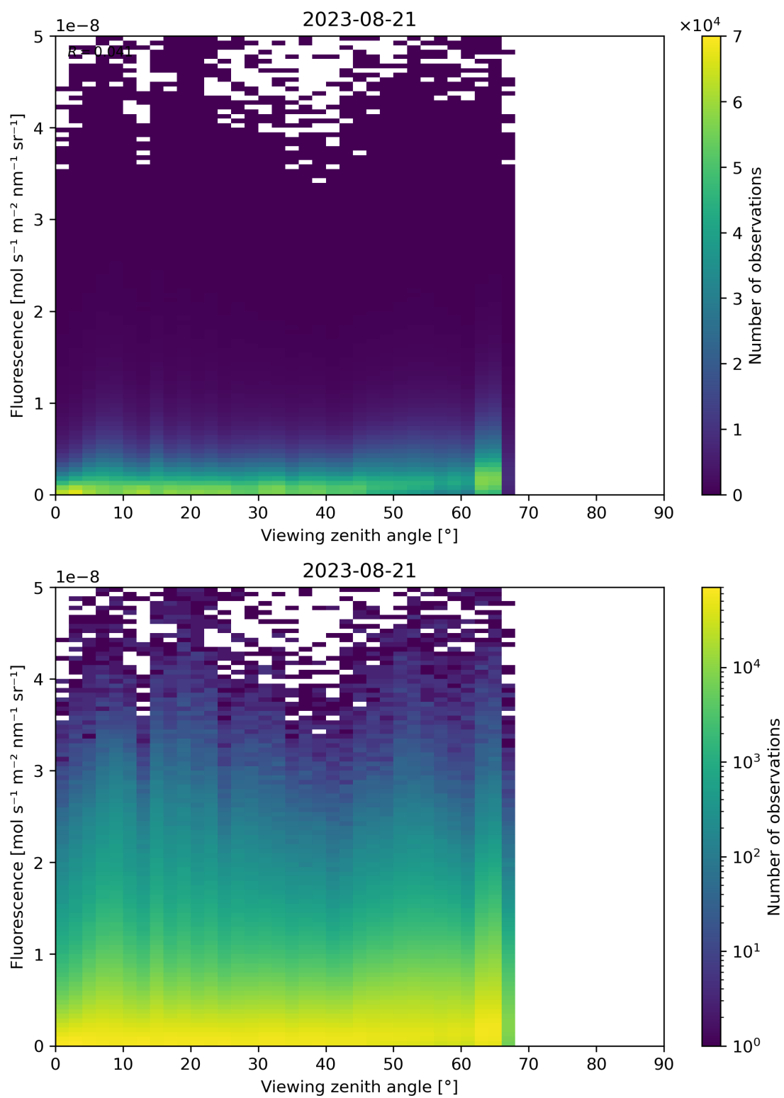
Figure 134: Scatter density plot of “Viewing zenith angle” against “Fluorescence” for 2023-08-20 to 2023-08-22.
