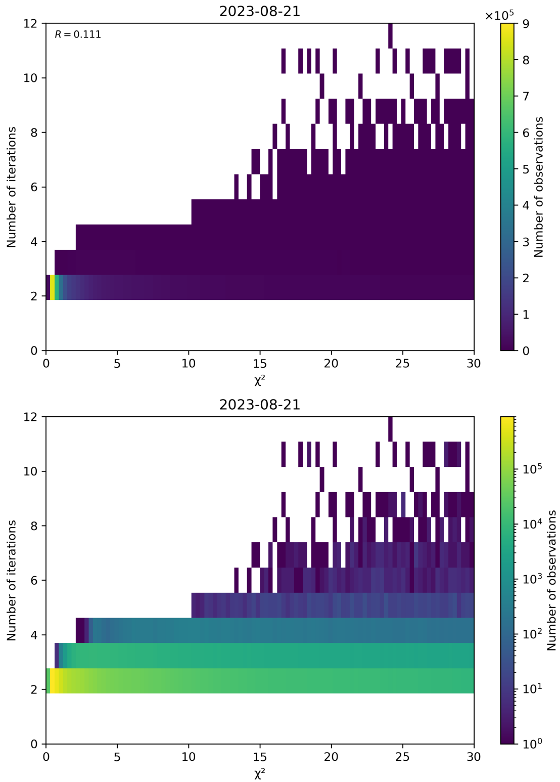
Figure 73: Scatter density plot of “ \chi^2 ” against “Number of iterations” for 2023-08-20 to 2023-08-22.
