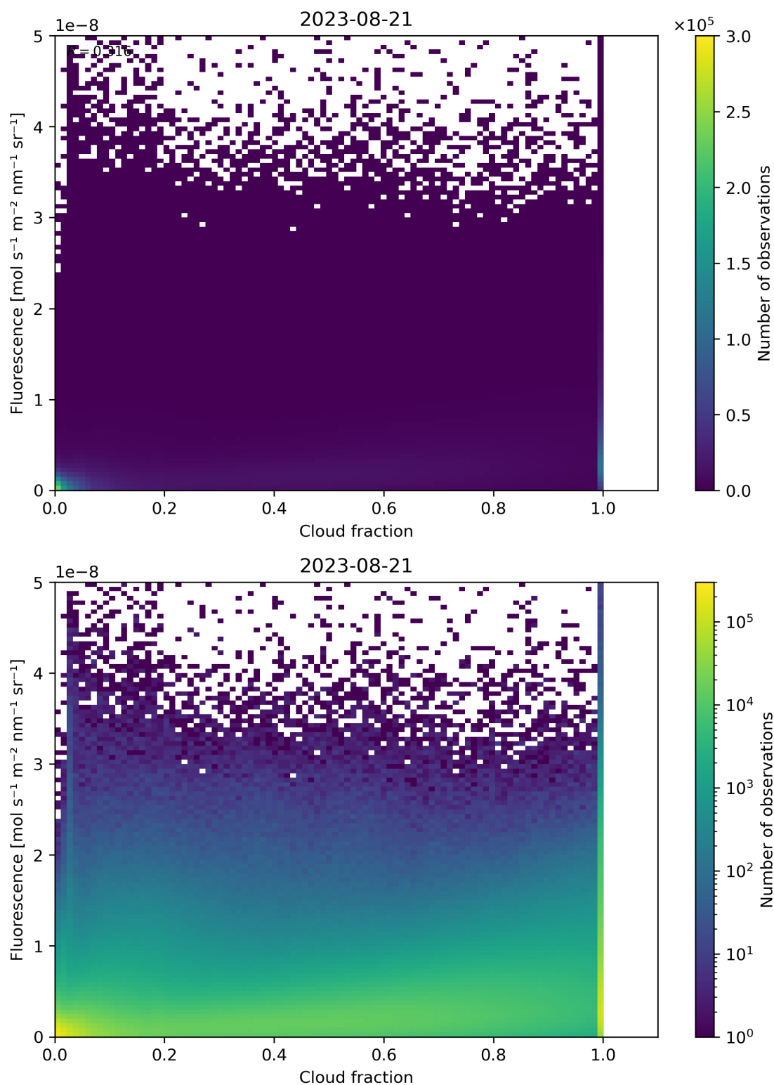
Figure 79: Scatter density plot of “Cloud fraction” against “Fluorescence” for 2023-08-20 to 2023-08-22.
