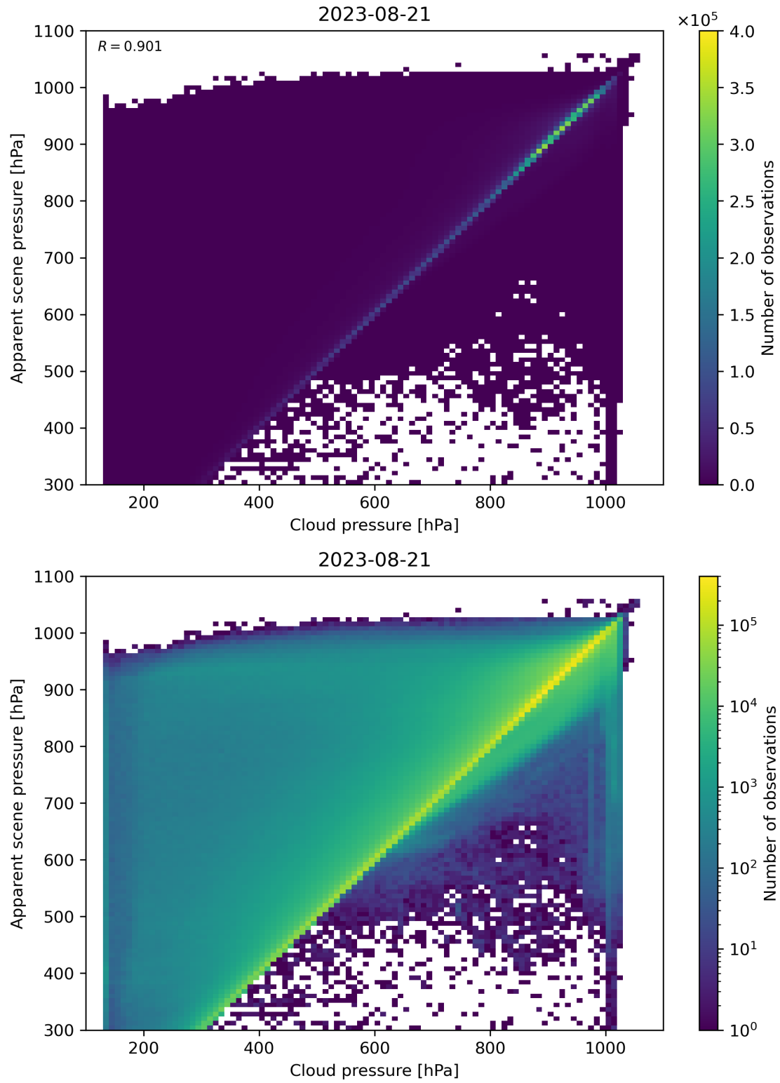
Figure 84: Scatter density plot of “Cloud pressure” against “Apparent scene pressure” for 2023-08-20 to 2023-08-22.
