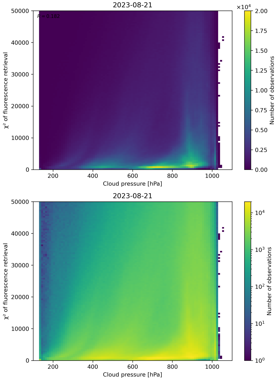
Figure 86: Scatter density plot of “Cloud pressure” against “ \chi^2 of fluorescence retrieval” for 2023-08-20 to 2023-08-22.
