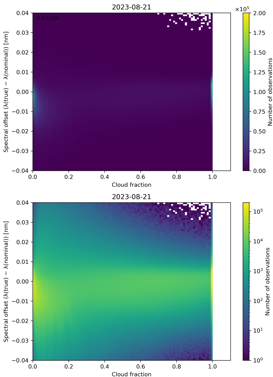
Figure 83: Scatter density plot of “Cloud fraction” against “Spectral offset ( \lambda(\text{true}) - \lambda(\text{nominal}) )” for 2023-08-20 to 2023-08-22.
