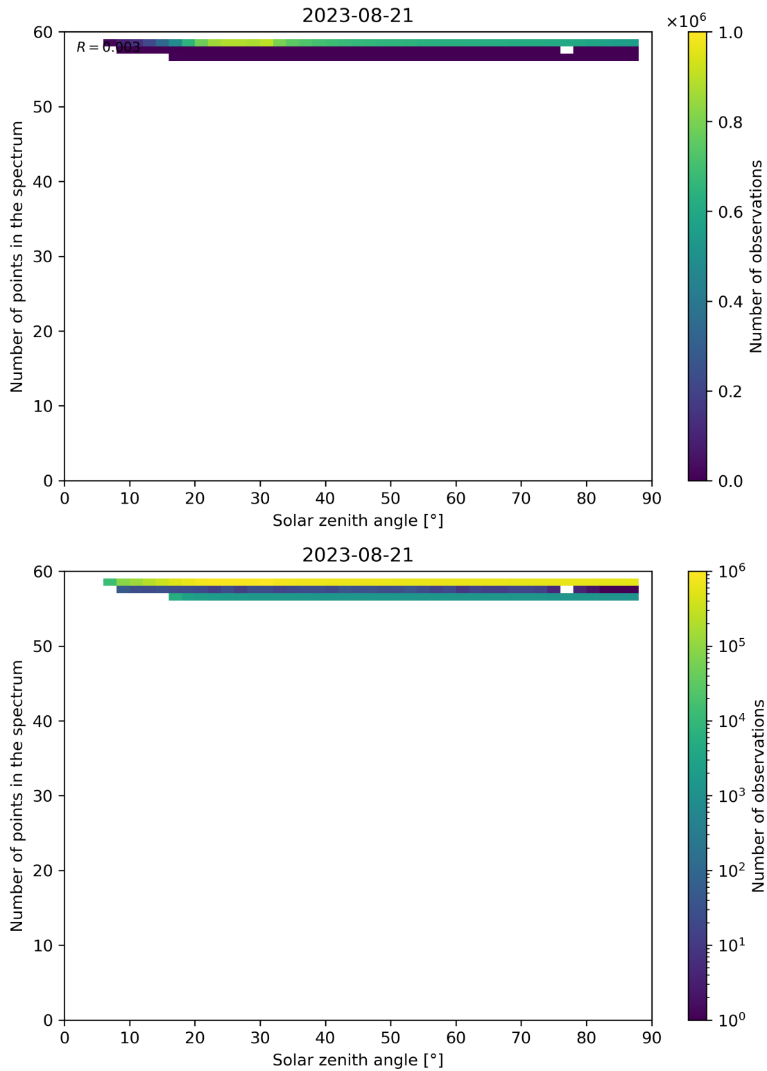
Figure 126: Scatter density plot of “Solar zenith angle” against “Number of points in the spectrum” for 2023-08-20 to 2023-08-22.
