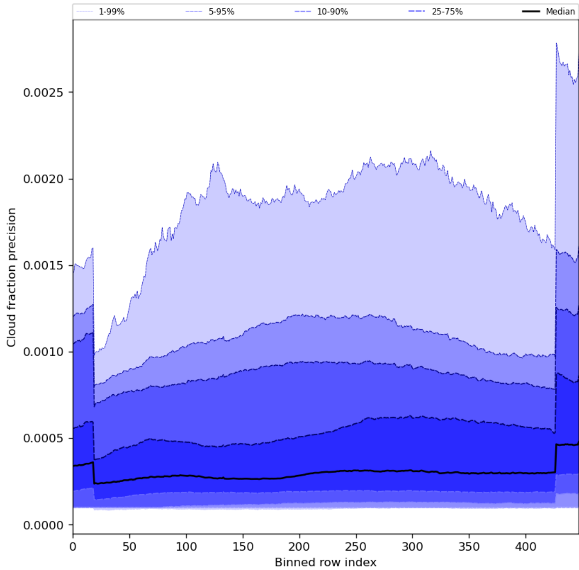
Figure 50: Along track statistics of “Cloud fraction precision” for 2023-08-20 to 2023-08-22
