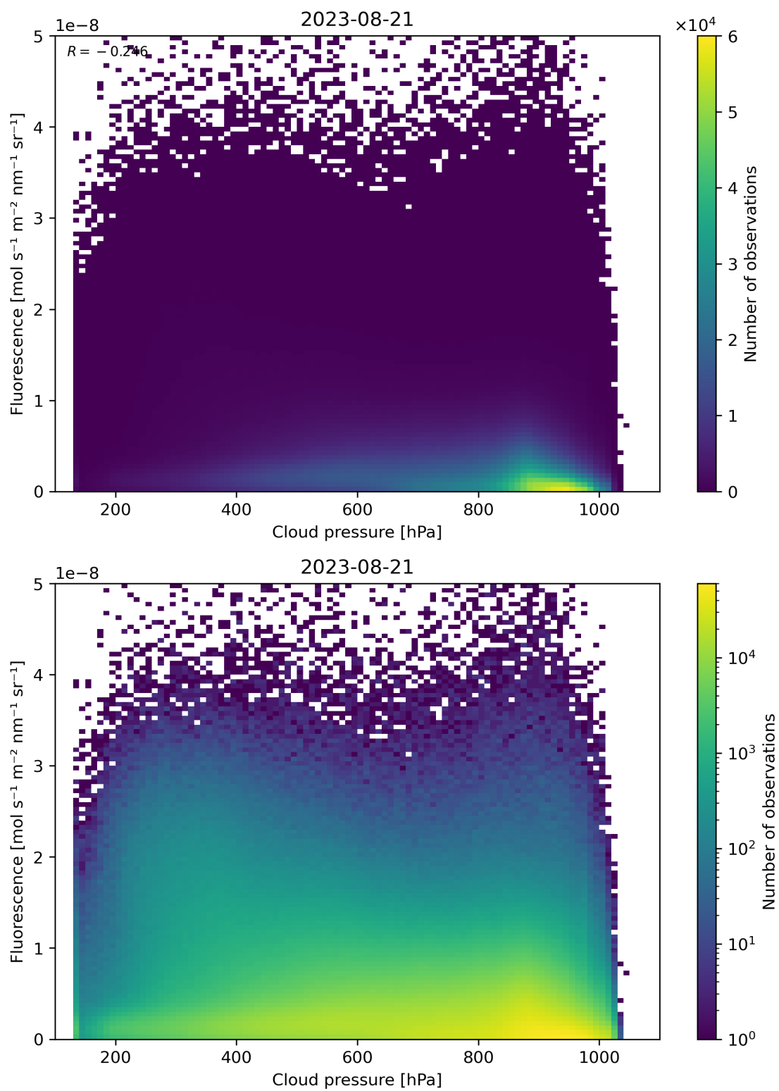
Figure 88: Scatter density plot of “Cloud pressure” against “Fluorescence” for 2023-08-20 to 2023-08-22.
