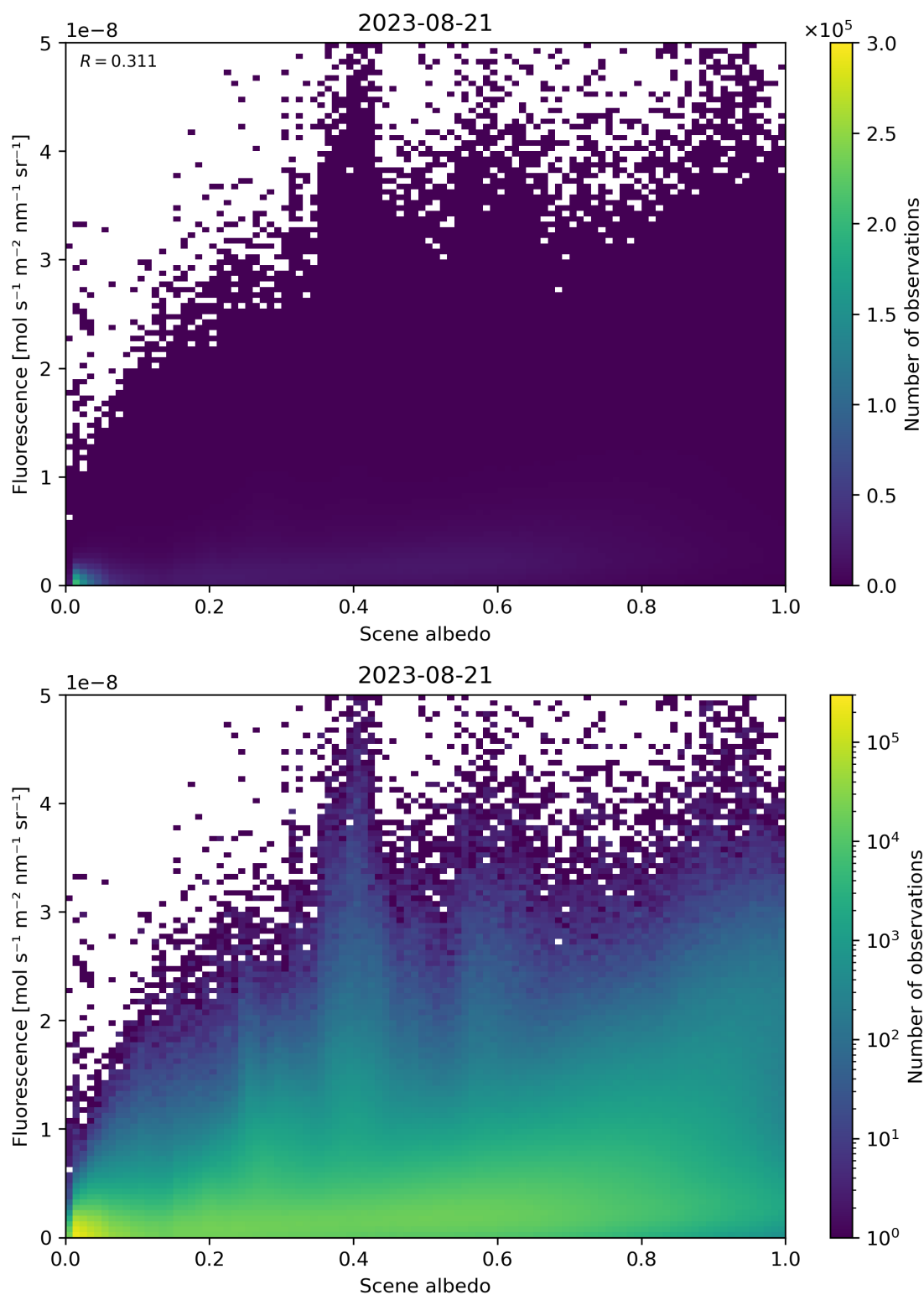
Figure 114: Scatter density plot of “Scene albedo” against “Fluorescence” for 2023-08-20 to 2023-08-22.
