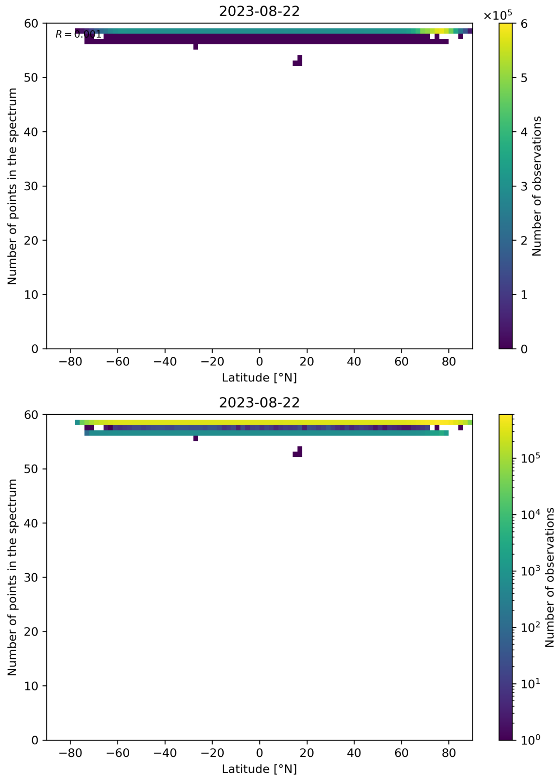
Figure 103: Scatter density plot of “Latitude” against “Number of points in the spectrum” for 2023-08-21 to 2023-08-23.
