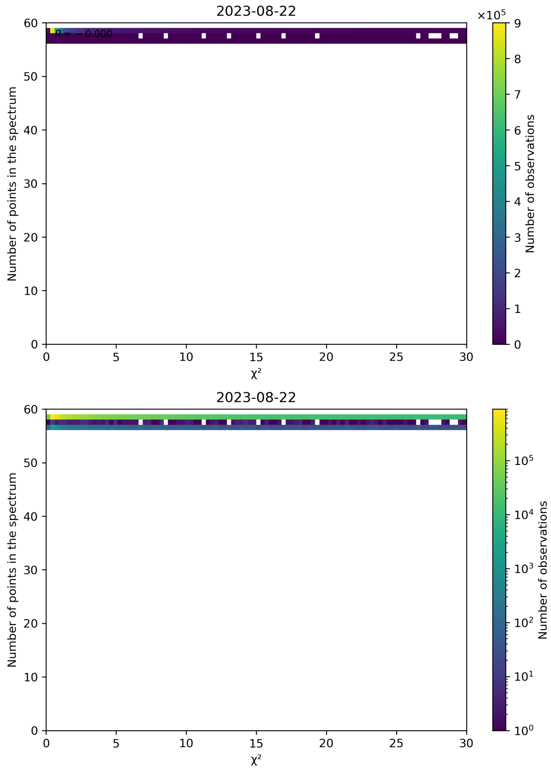
Figure 74: Scatter density plot of " \chi^2 " against "Number of points in the spectrum" for 2023-08-21 to 2023-08-23.
