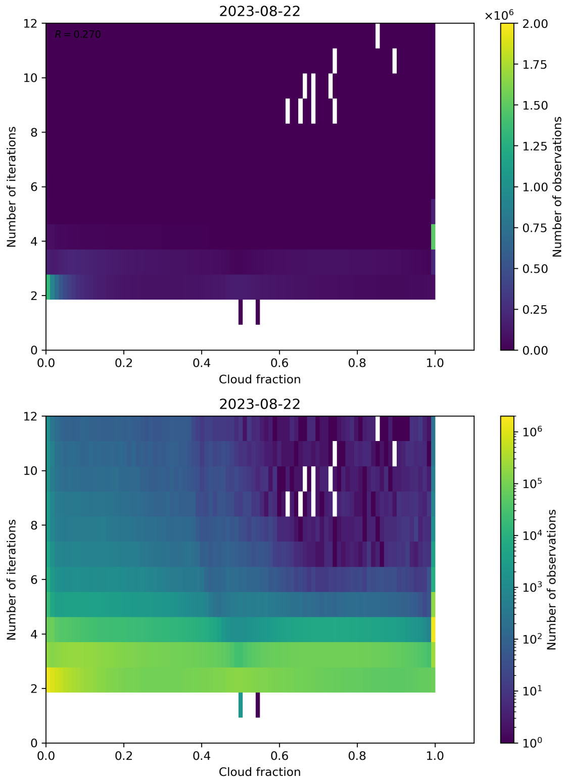
Figure 80: Scatter density plot of “Cloud fraction” against “Number of iterations” for 2023-08-21 to 2023-08-23.
