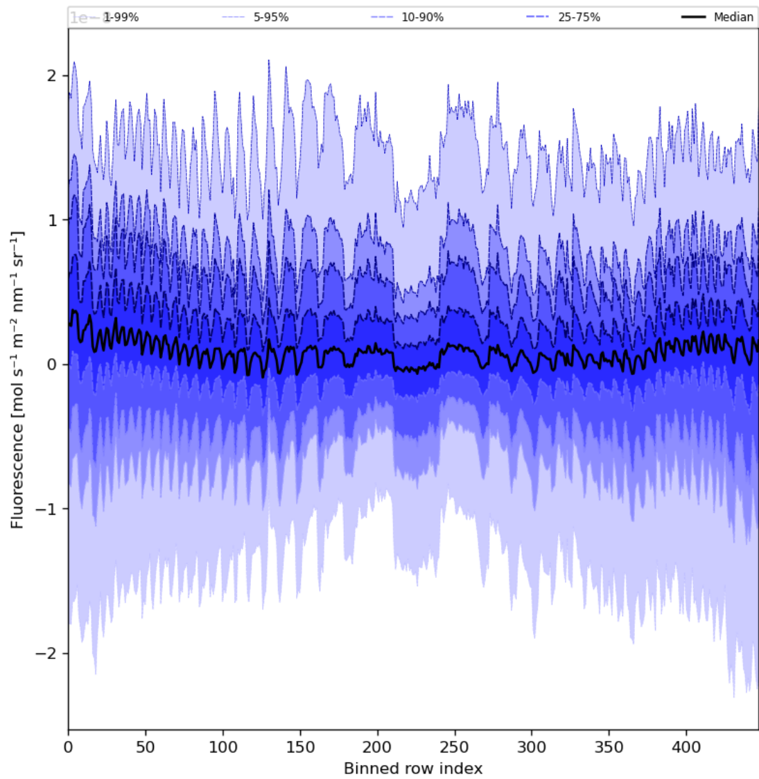
Figure 57: Along track statistics of “Fluorescence” for 2023-08-21 to 2023-08-23
