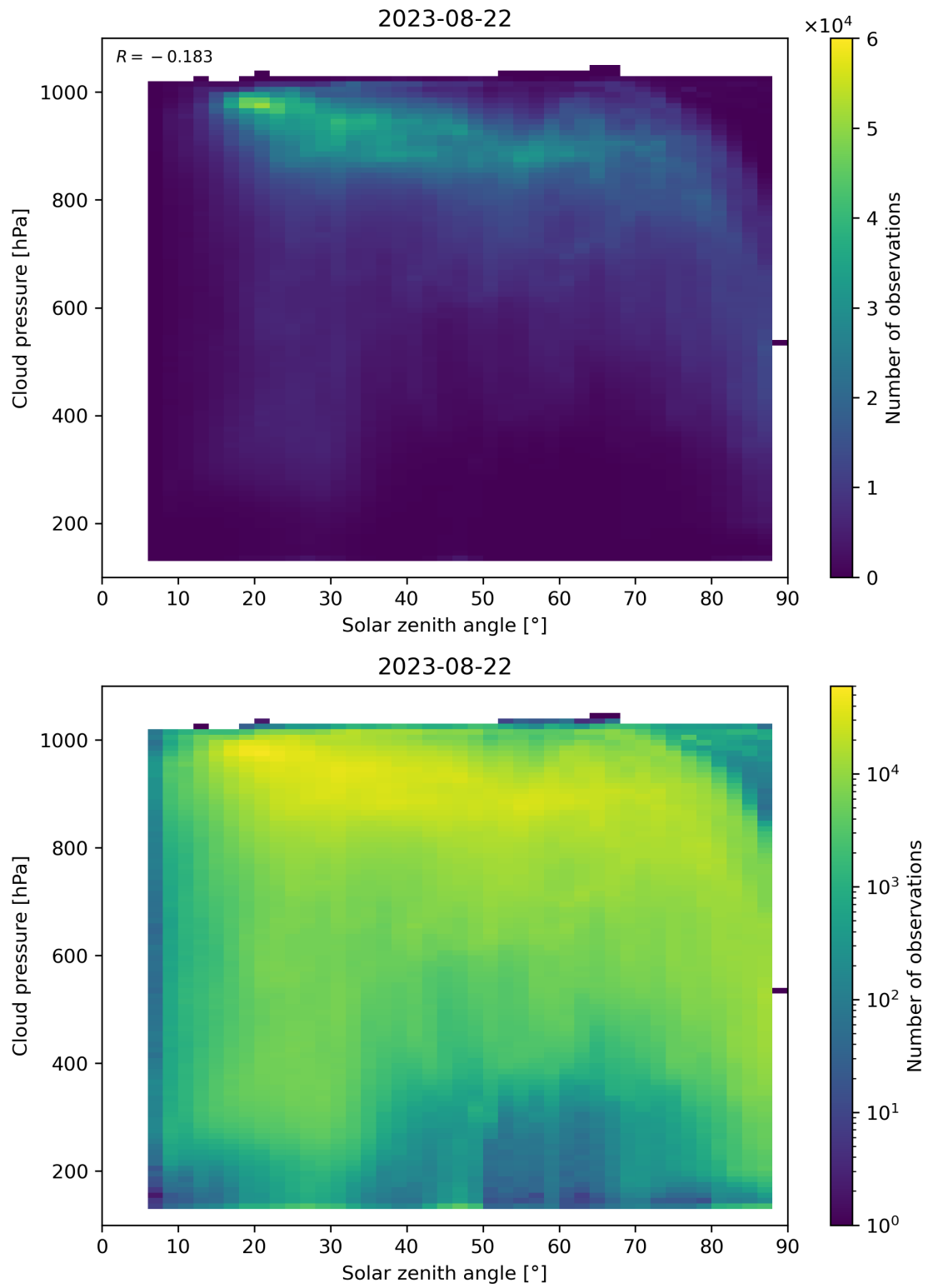
Figure 122: Scatter density plot of “Solar zenith angle” against “Cloud pressure” for 2023-08-21 to 2023-08-23.
