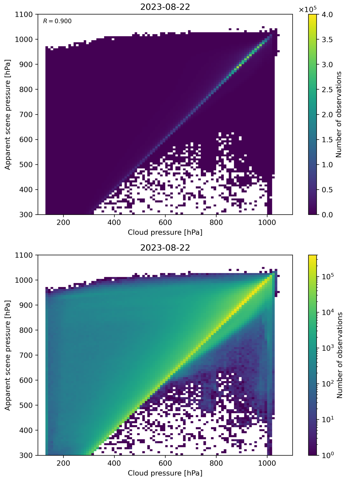
Figure 84: Scatter density plot of “Cloud pressure” against “Apparent scene pressure” for 2023-08-21 to 2023-08-23.
