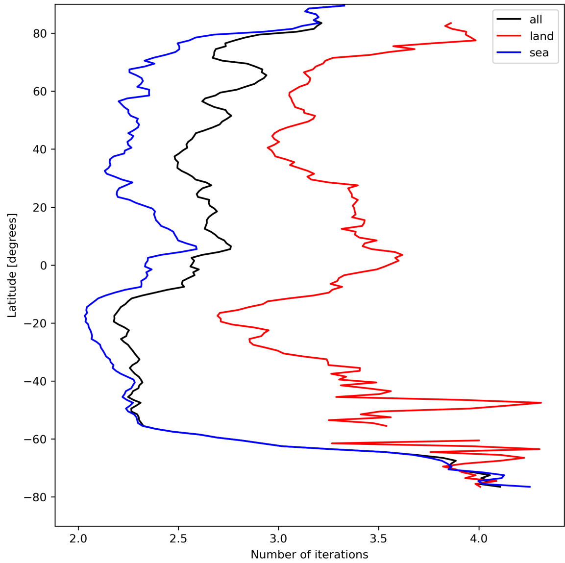
Figure 22: Zonal average of “Number of iterations” for 2023-08-21 to 2023-08-23.
