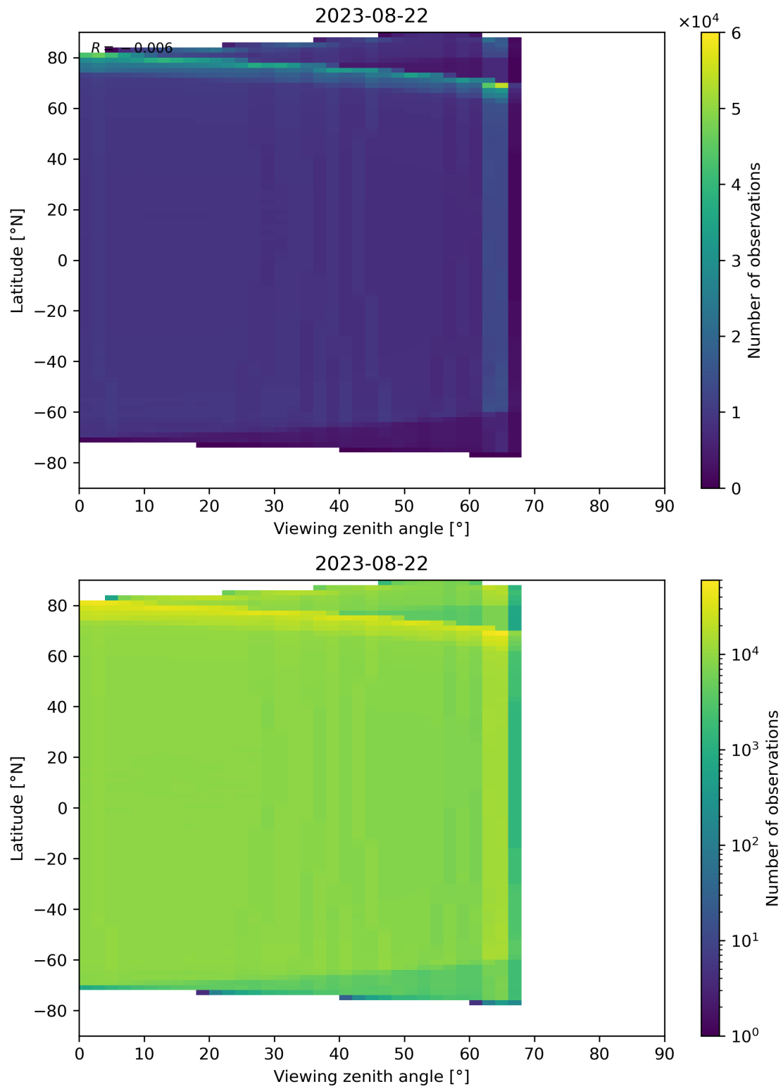
Figure 135: Scatter density plot of “Viewing zenith angle” against “Latitude” for 2023-08-21 to 2023-08-23.
