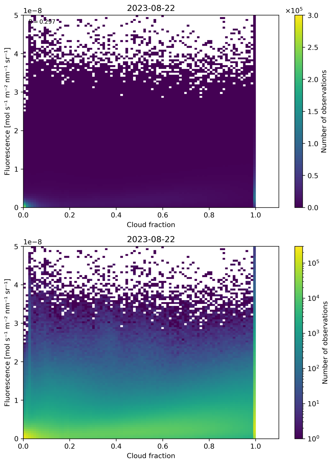
Figure 79: Scatter density plot of “Cloud fraction” against “Fluorescence” for 2023-08-21 to 2023-08-23.
