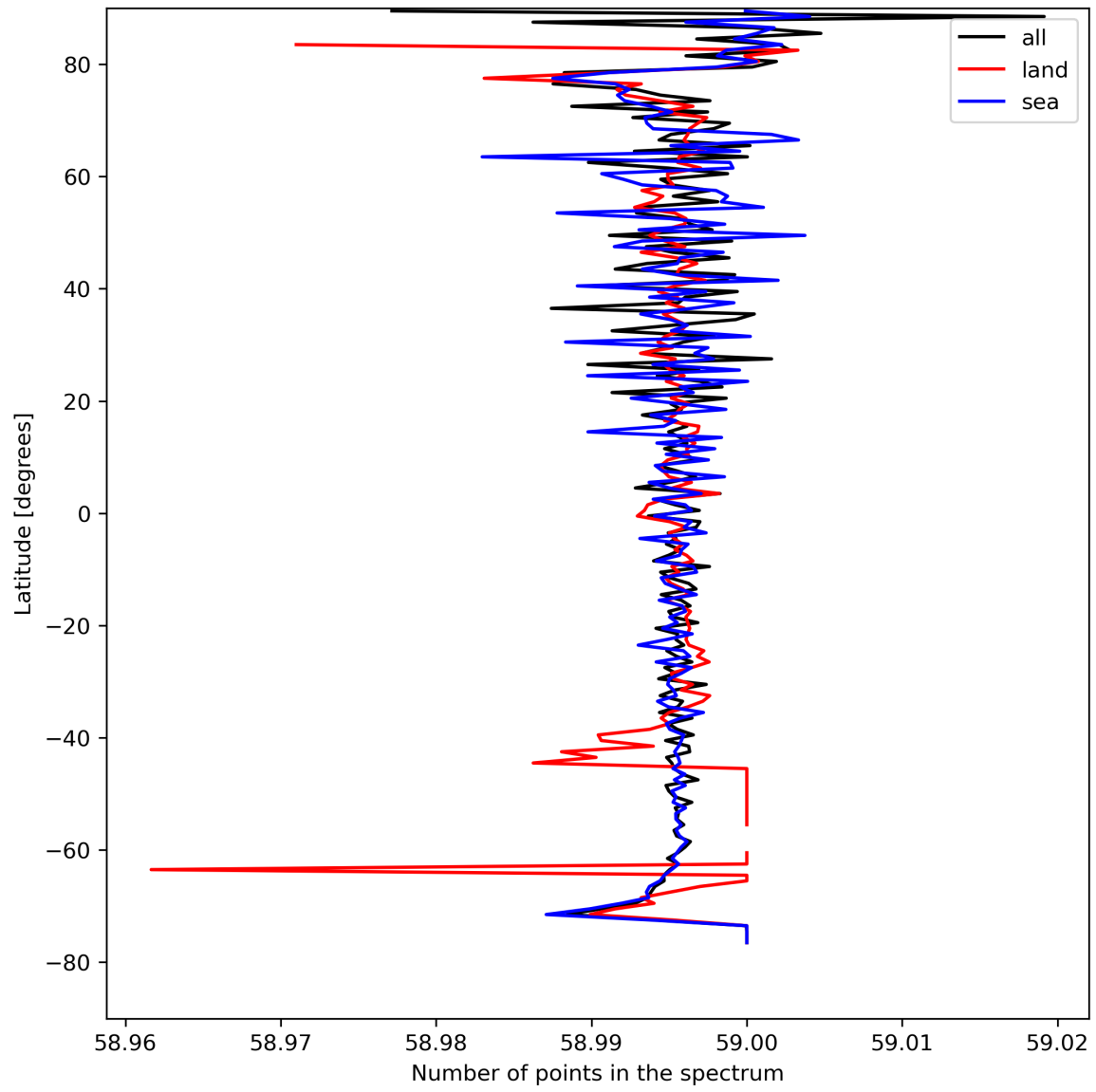
Figure 27: Zonal average of “Number of points in the spectrum” for 2023-08-21 to 2023-08-23.
