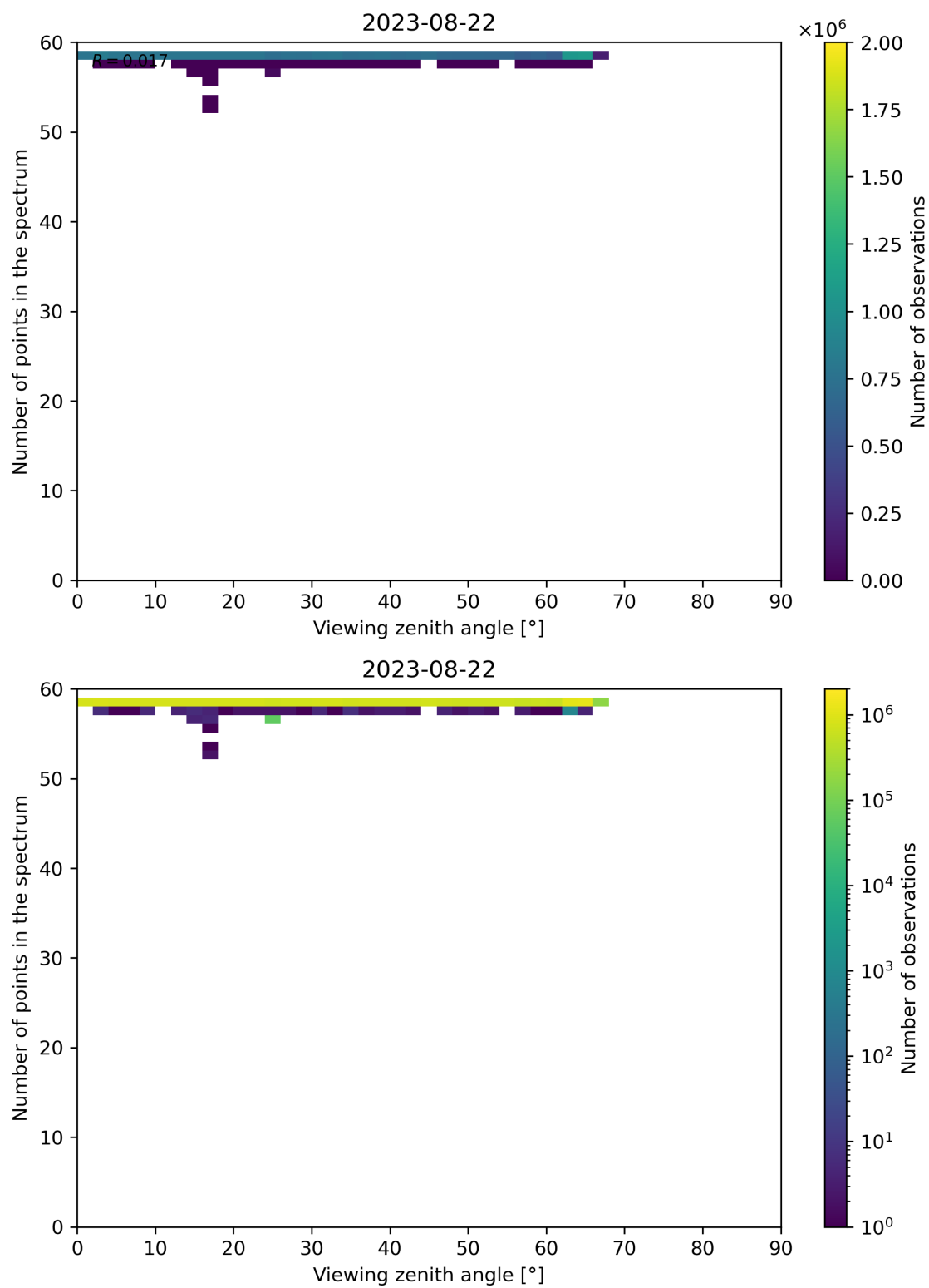
Figure 137: Scatter density plot of “Viewing zenith angle” against “Number of points in the spectrum” for 2023-08-21 to 2023-08-23.
