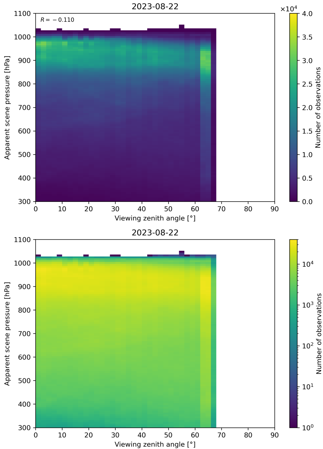
Figure 129: Scatter density plot of “Viewing zenith angle” against “Apparent scene pressure” for 2023-08-21 to 2023-08-23.
