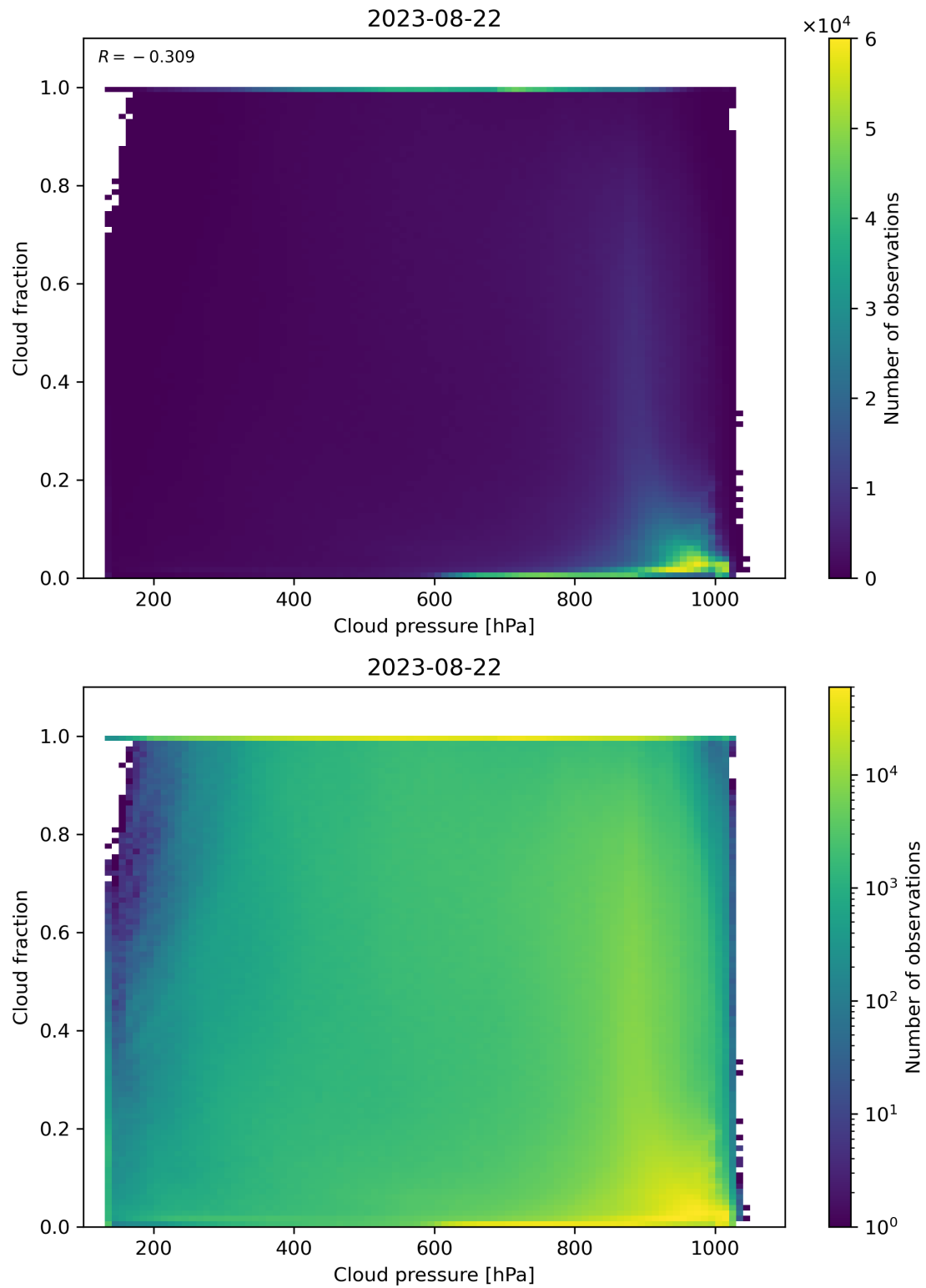
Figure 87: Scatter density plot of “Cloud pressure” against “Cloud fraction” for 2023-08-21 to 2023-08-23.
