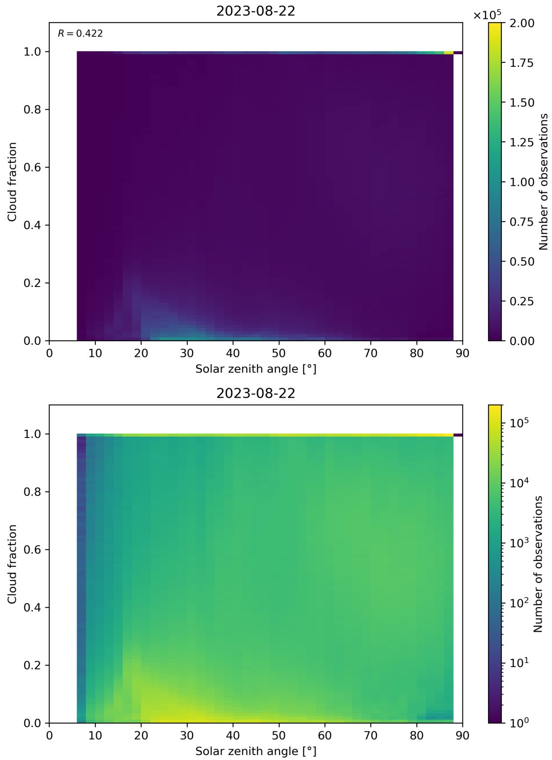
Figure 121: Scatter density plot of “Solar zenith angle” against “Cloud fraction” for 2023-08-21 to 2023-08-23.
