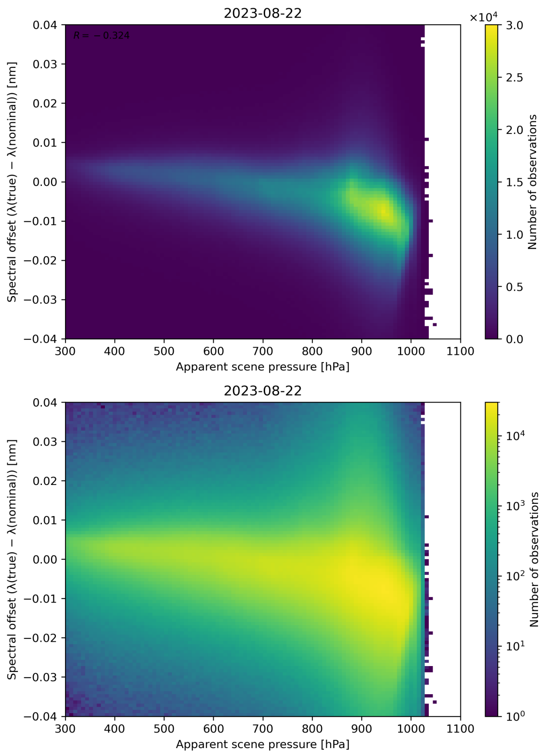
Figure 68: Scatter density plot of “Apparent scene pressure” against “Spectral offset ( \lambda(\text{true}) - \lambda(\text{nominal}) )” for 2023-08-21 to 2023-08-23.
