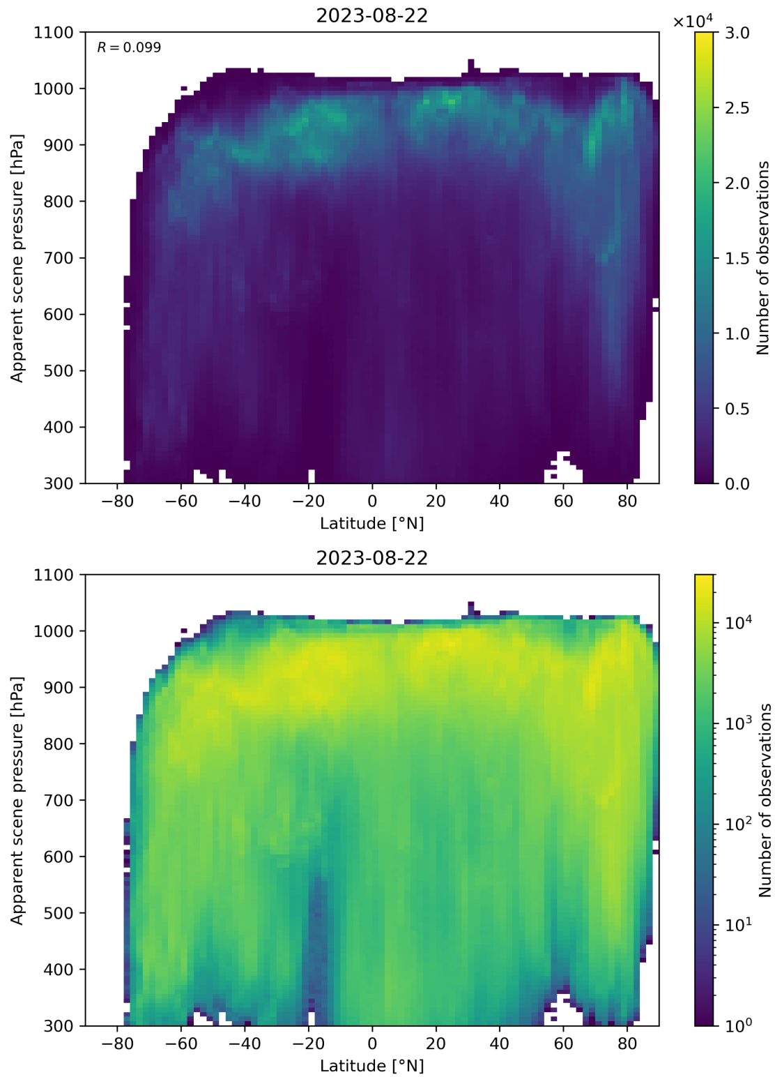
Figure 96: Scatter density plot of “Latitude” against “Apparent scene pressure” for 2023-08-21 to 2023-08-23.
