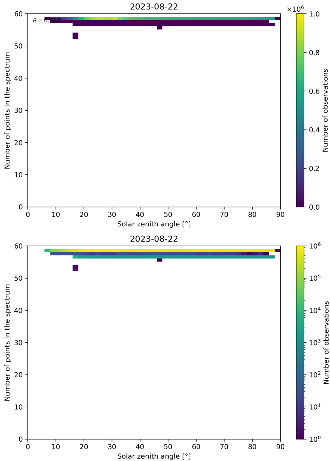
Figure 126: Scatter density plot of “Solar zenith angle” against “Number of points in the spectrum” for 2023-08-21 to 2023-08-23.
