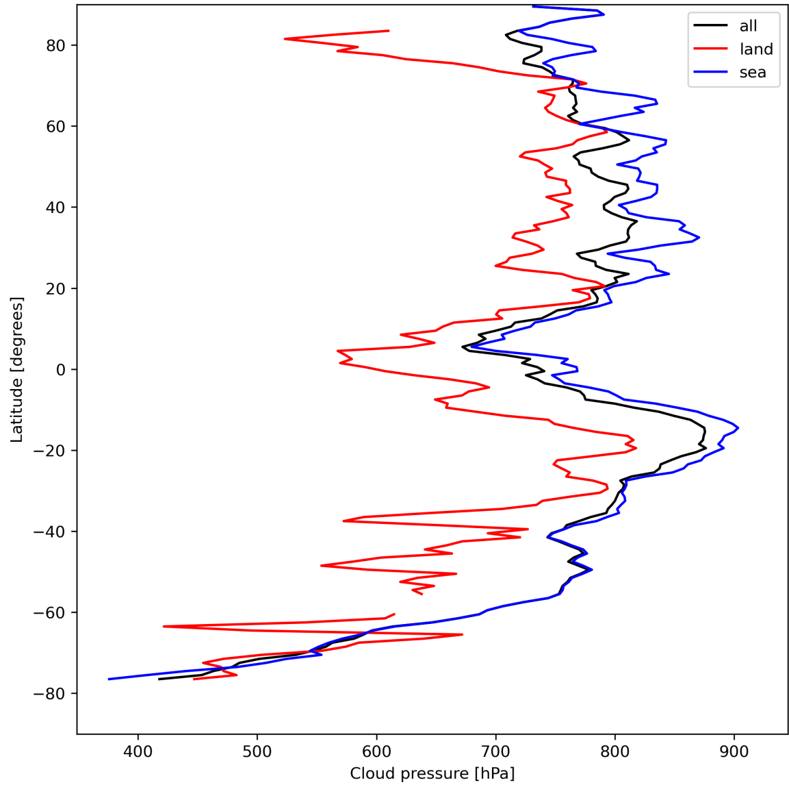
Figure 13: Zonal average of “Cloud pressure” for 2023-08-21 to 2023-08-23.
