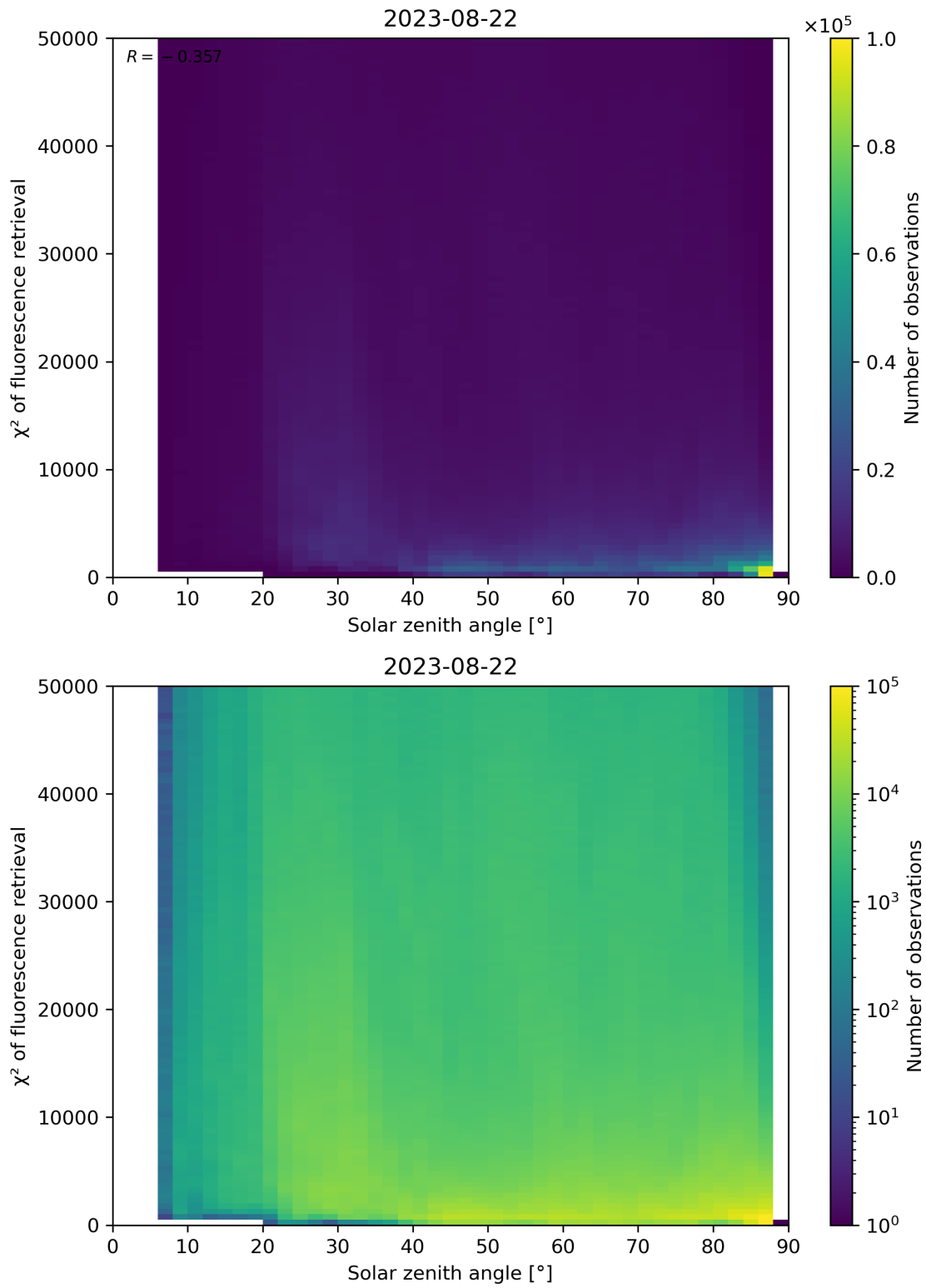
Figure 120: Scatter density plot of “Solar zenith angle” against “ \chi^2 of fluorescence retrieval” for 2023-08-21 to 2023-08-23.
