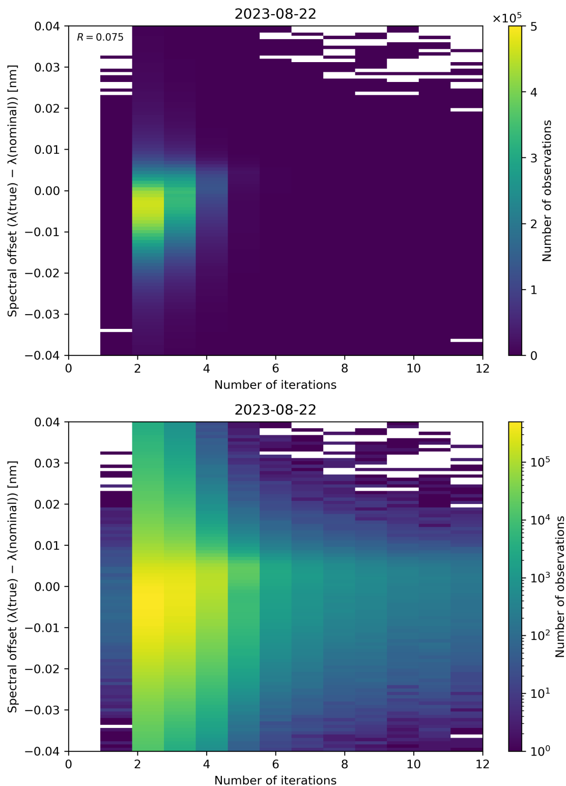
Figure 109: Scatter density plot of “Number of iterations” against “Spectral offset ( \lambda(\text{true}) - \lambda(\text{nominal}) )” for 2023-08-21 to 2023-08-23.
