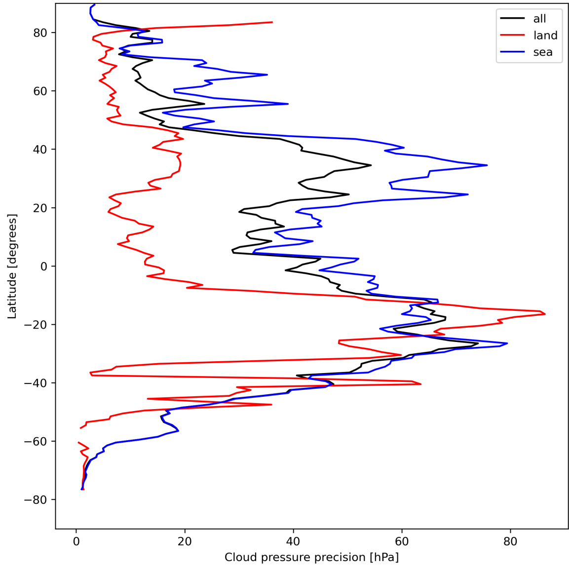
Figure 14: Zonal average of “Cloud pressure precision” for 2023-08-21 to 2023-08-23.
