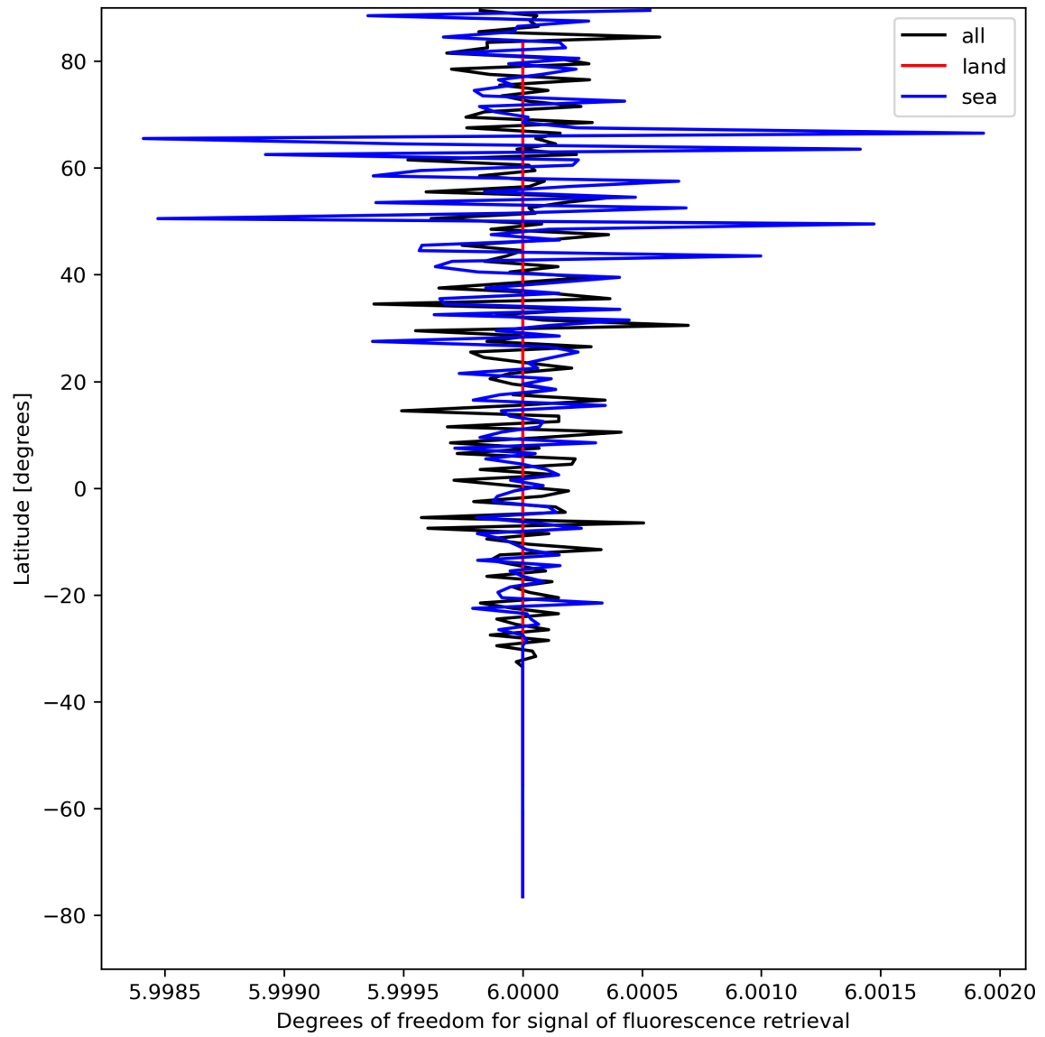
Figure 26: Zonal average of “Degrees of freedom for signal of fluorescence retrieval” for 2023-08-21 to 2023-08-23.
