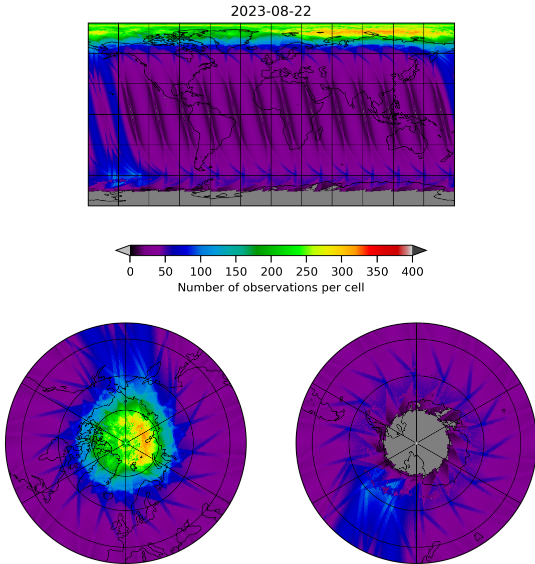
Figure 11: Map of the number of observations for 2023-08-21 to 2023-08-23
