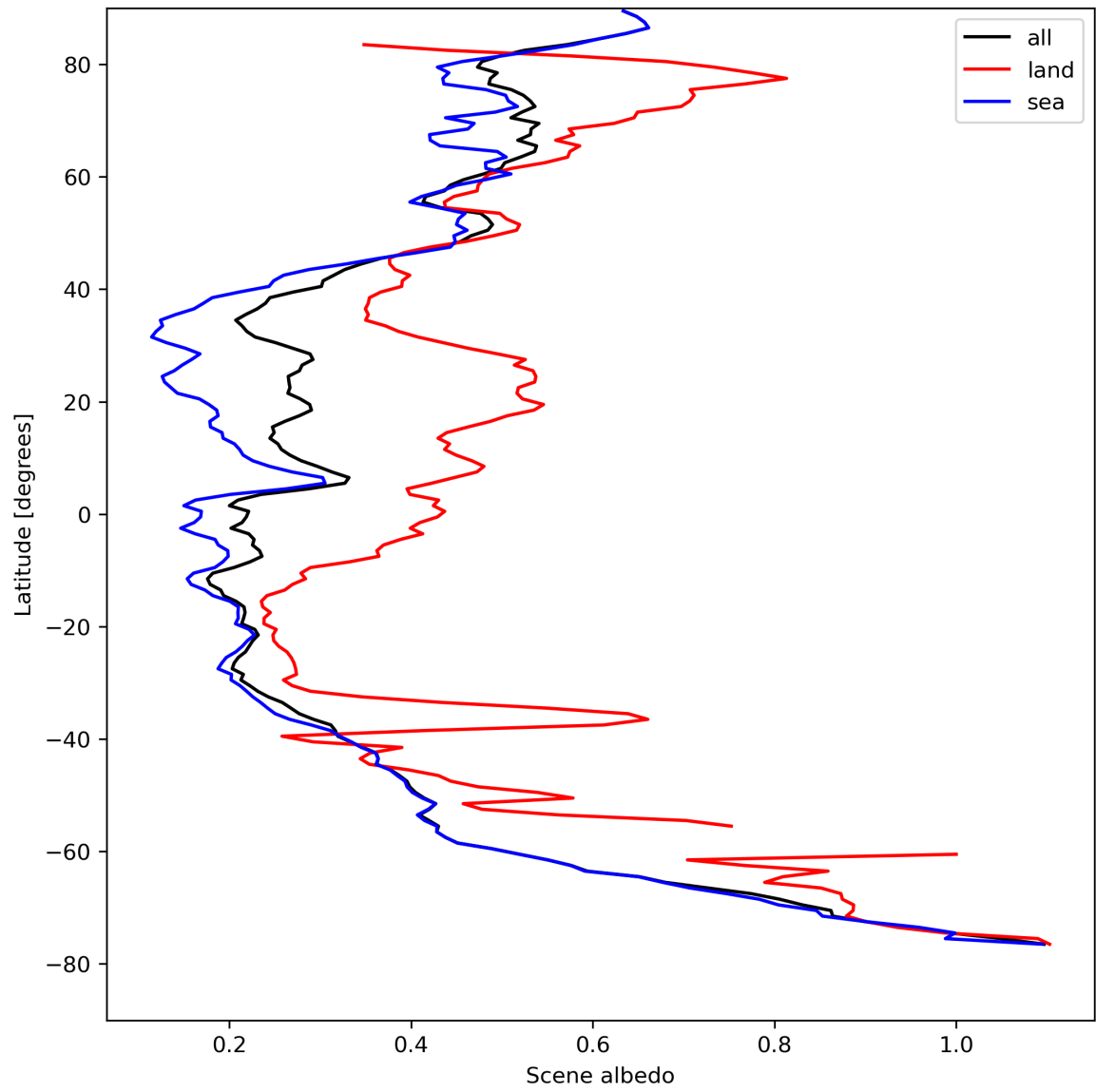
Figure 17: Zonal average of “Scene albedo” for 2023-08-21 to 2023-08-23.
