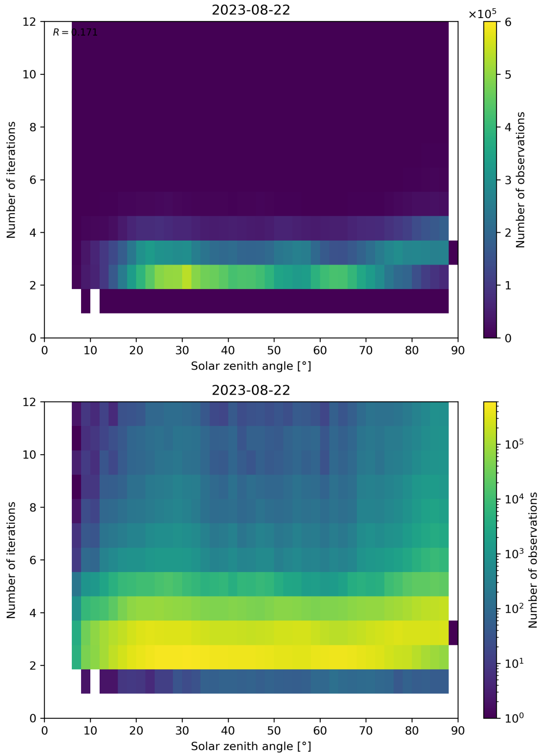
Figure 125: Scatter density plot of “Solar zenith angle” against “Number of iterations” for 2023-08-21 to 2023-08-23.
