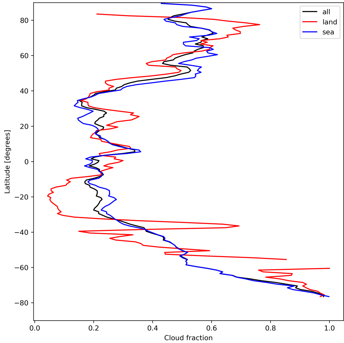
Figure 15: Zonal average of “Cloud fraction” for 2023-08-21 to 2023-08-23.
