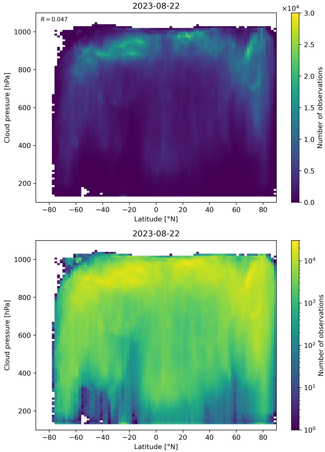
Figure 100: Scatter density plot of “Latitude” against “Cloud pressure” for 2023-08-21 to 2023-08-23.
