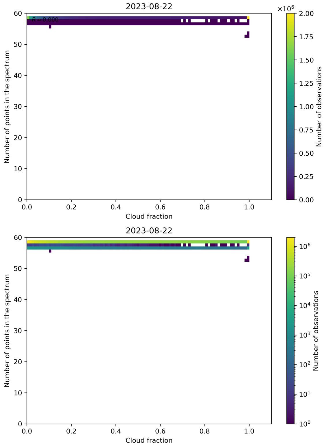
Figure 81: Scatter density plot of “Cloud fraction” against “Number of points in the spectrum” for 2023-08-21 to 2023-08-23.
