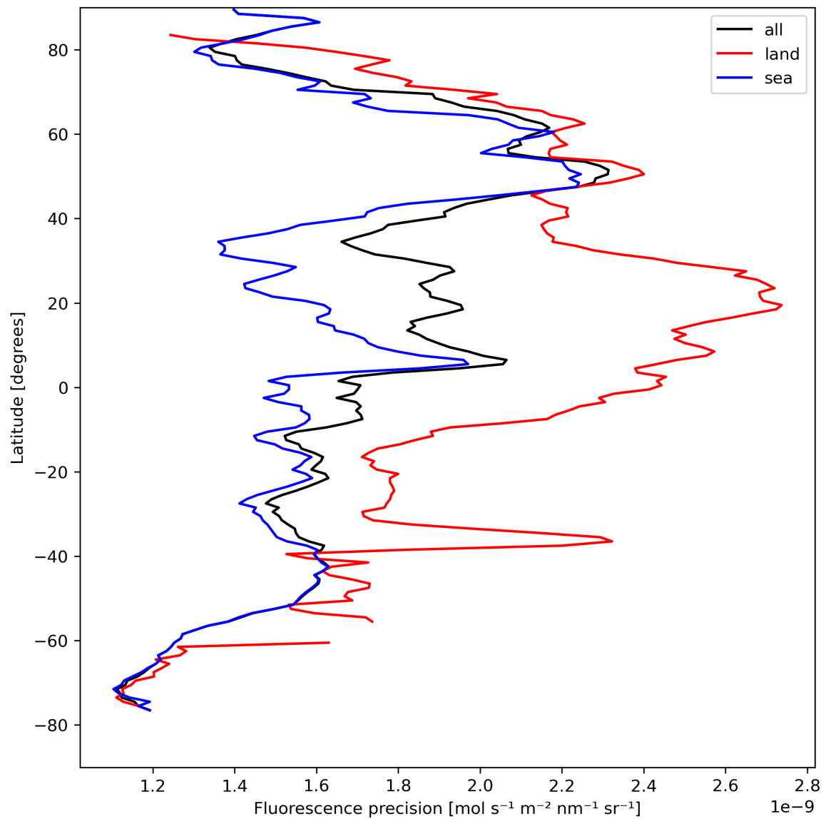
Figure 24: Zonal average of “Fluorescence precision” for 2023-08-21 to 2023-08-23.
