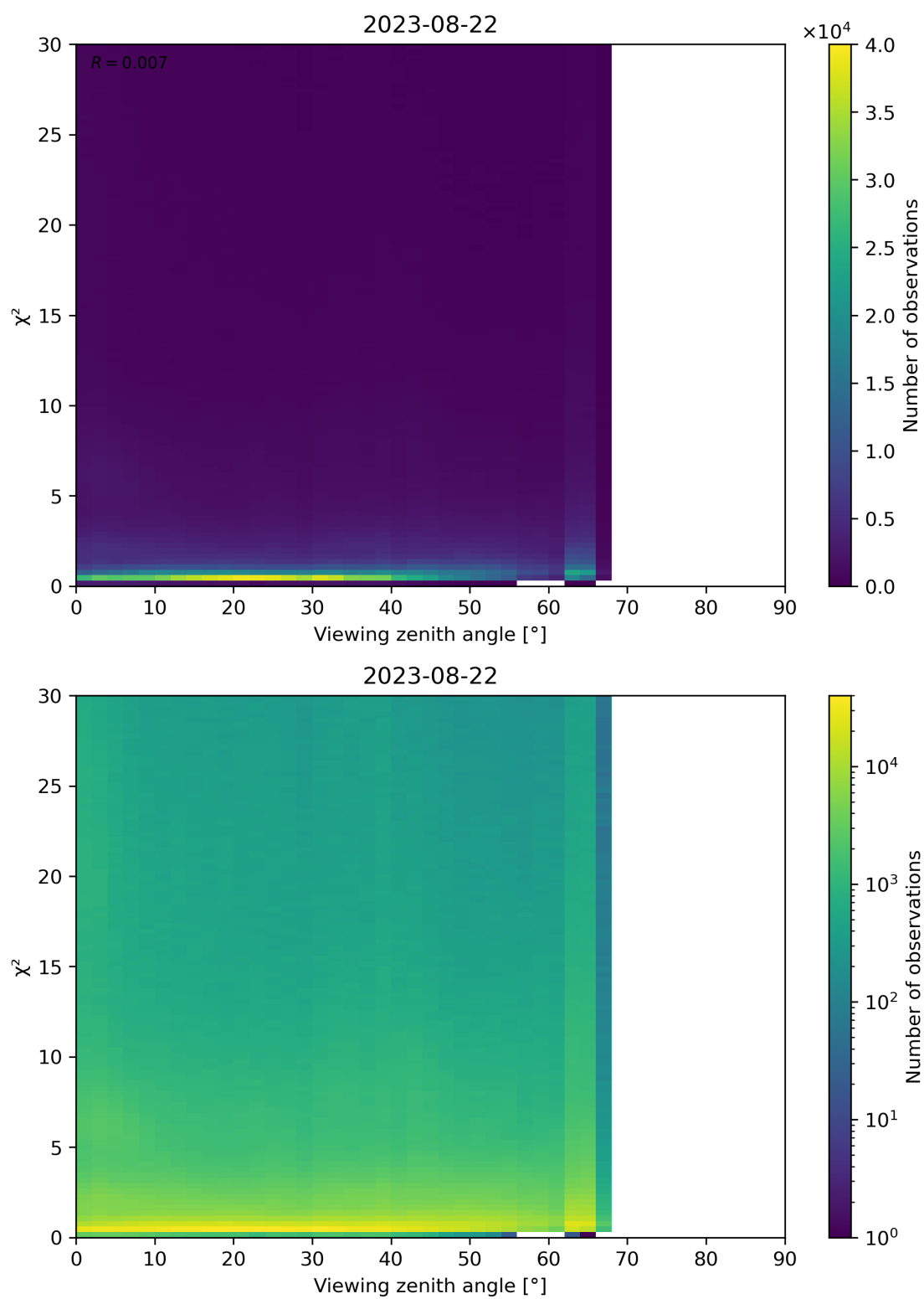
Figure 130: Scatter density plot of “Viewing zenith angle” against “ \chi^2 ” for 2023-08-21 to 2023-08-23.
