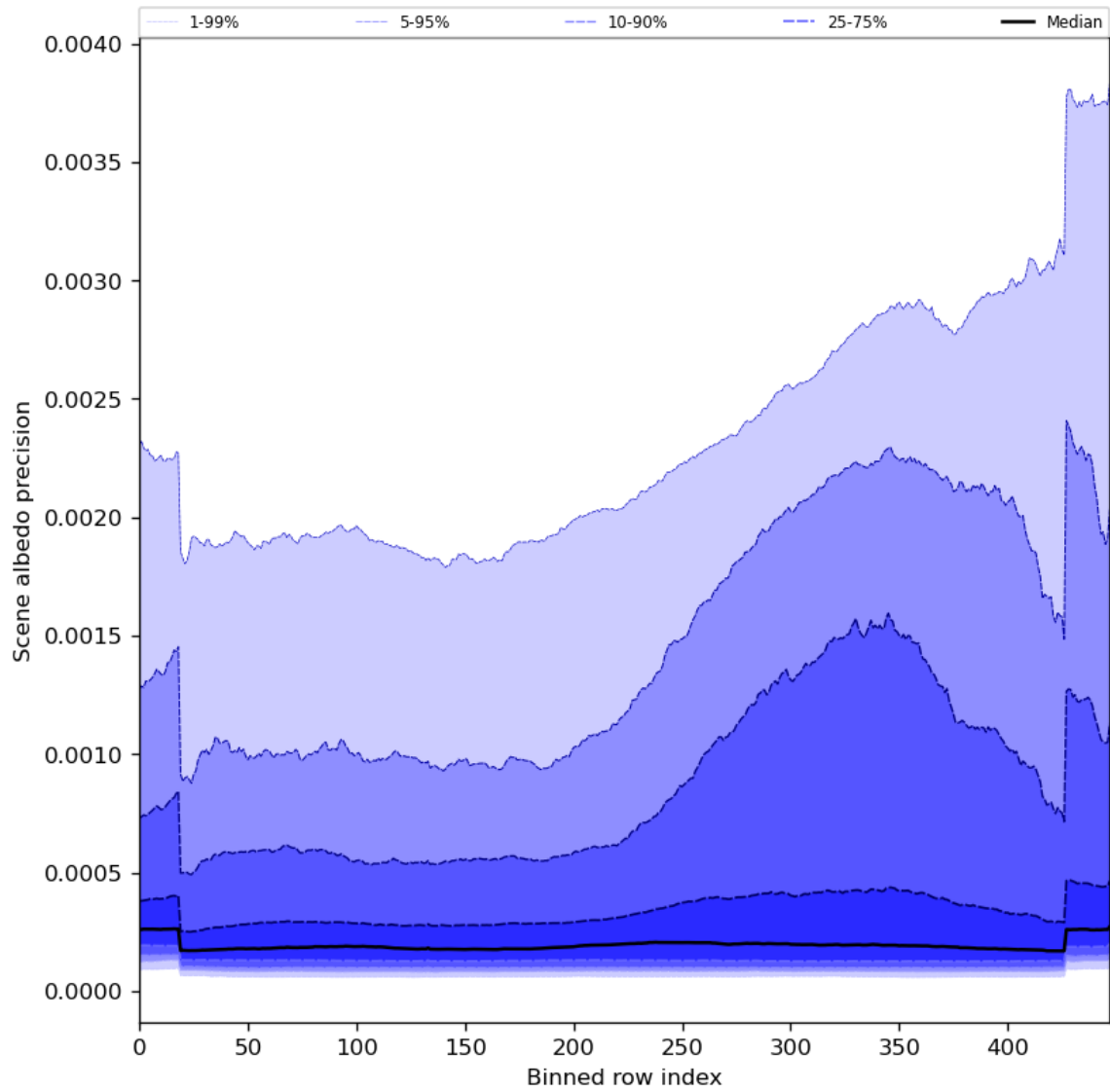
Figure 52: Along track statistics of “Scene albedo precision” for 2023-08-21 to 2023-08-23
