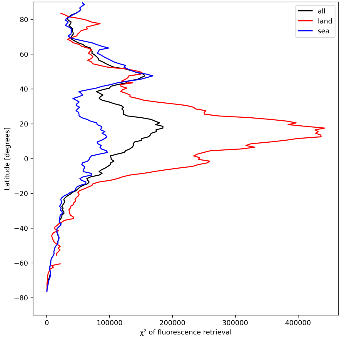
Figure 25: Zonal average of “ \chi^2 of fluorescence retrieval” for 2023-08-21 to 2023-08-23.
