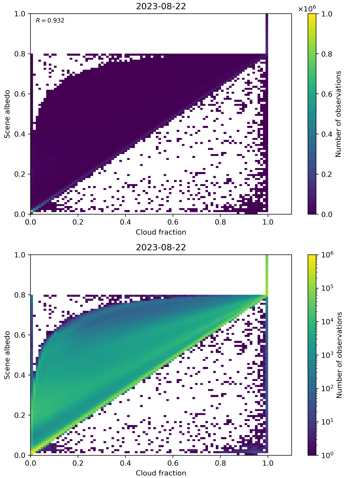
Figure 82: Scatter density plot of “Cloud fraction” against “Scene albedo” for 2023-08-21 to 2023-08-23.
