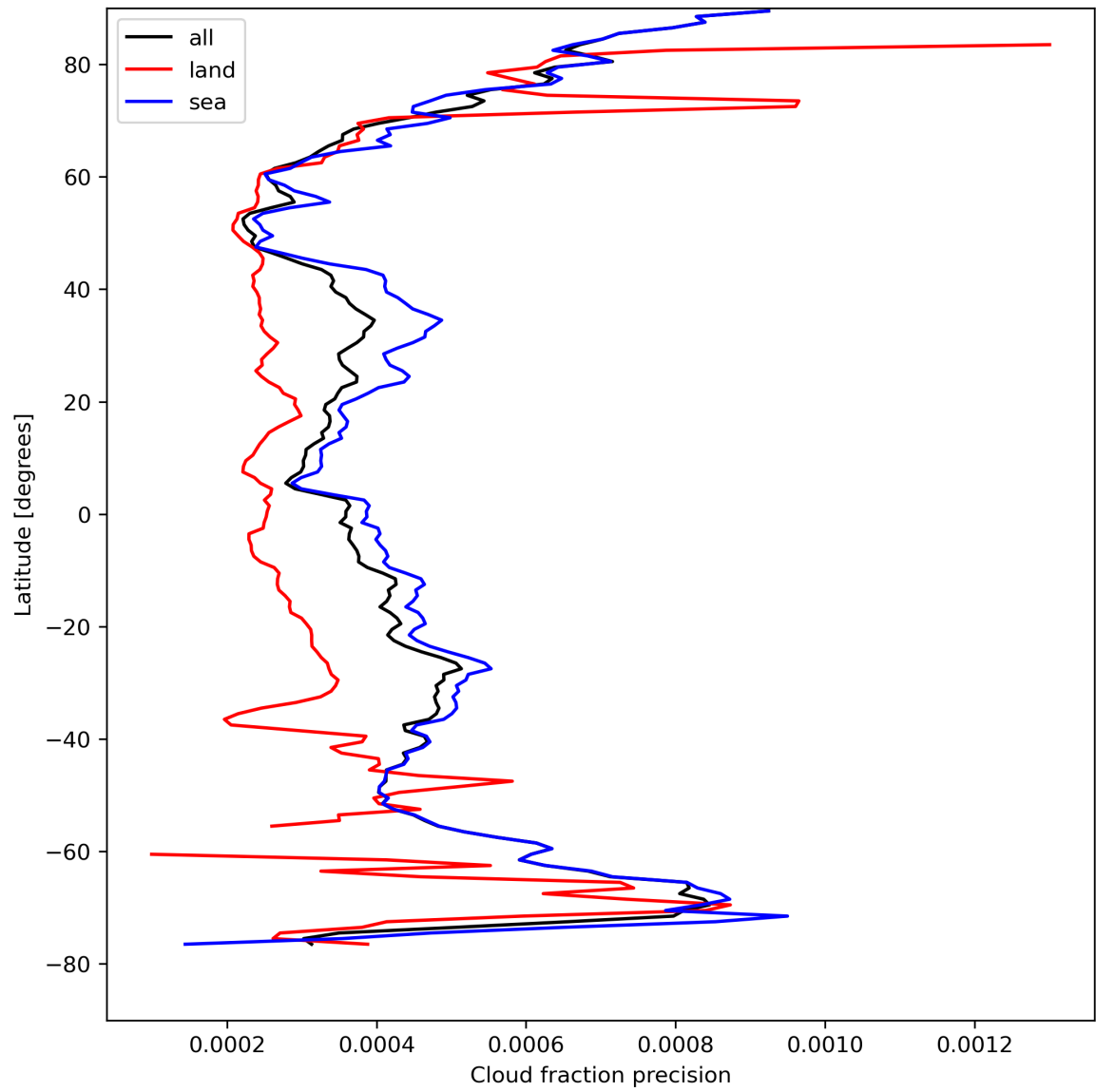
Figure 16: Zonal average of “Cloud fraction precision” for 2023-08-21 to 2023-08-23.
