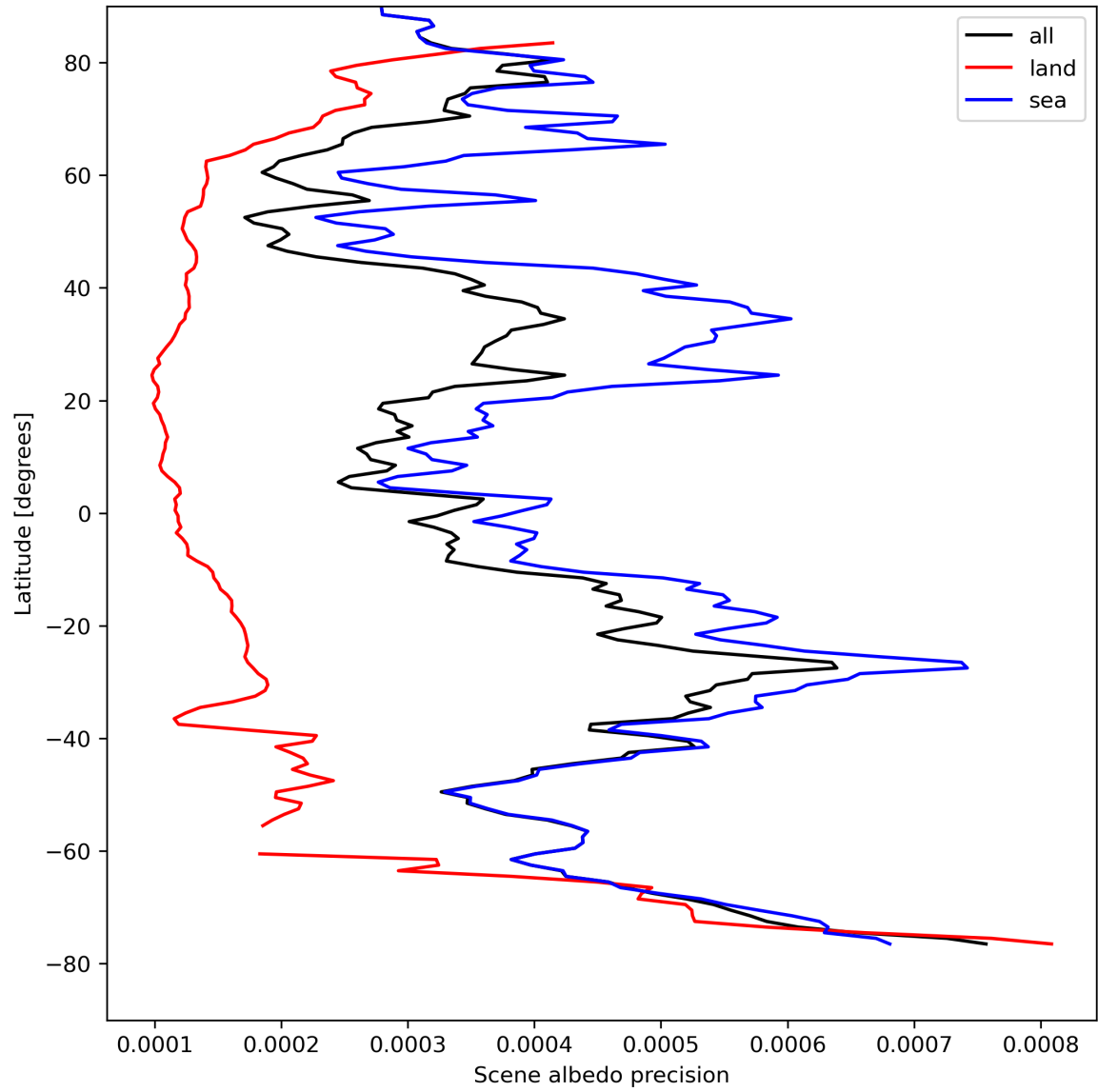
Figure 18: Zonal average of “Scene albedo precision” for 2023-08-21 to 2023-08-23.
