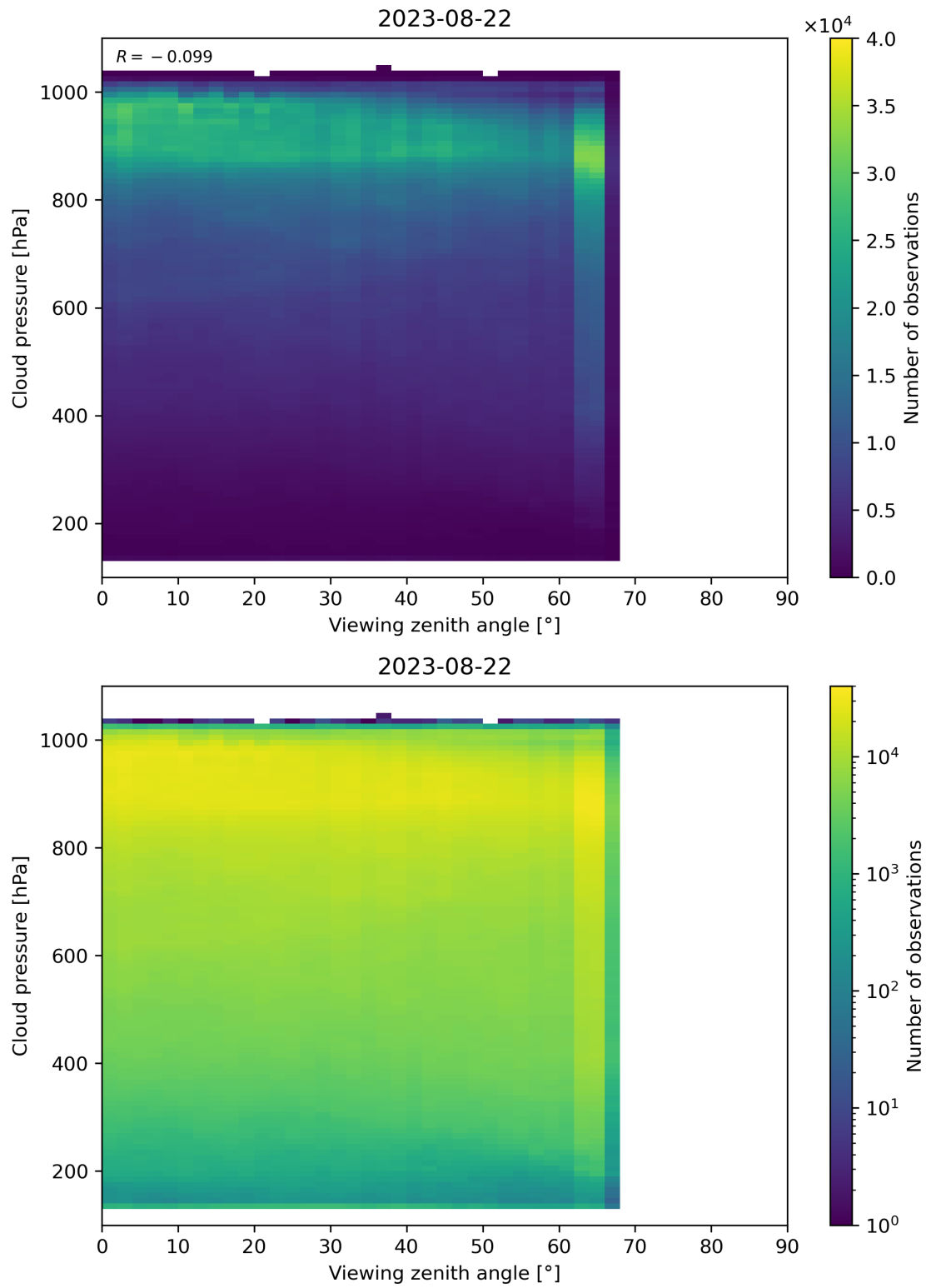
Figure 133: Scatter density plot of “Viewing zenith angle” against “Cloud pressure” for 2023-08-21 to 2023-08-23.
