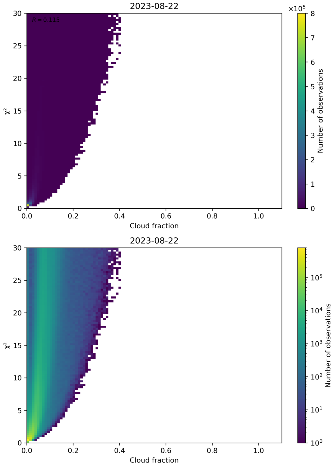
Figure 77: Scatter density plot of “Cloud fraction” against “ \chi^2 ” for 2023-08-21 to 2023-08-23.
