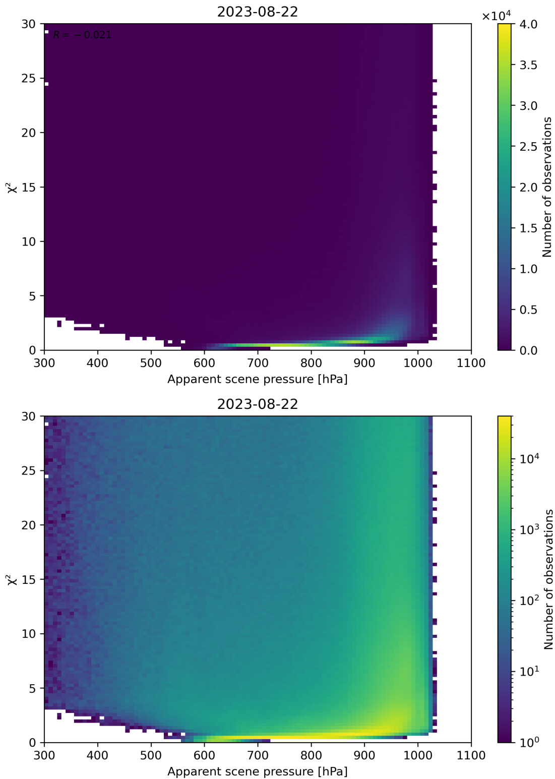
Figure 63: Scatter density plot of “Apparent scene pressure” against “ \chi^2 ” for 2023-08-21 to 2023-08-23.
