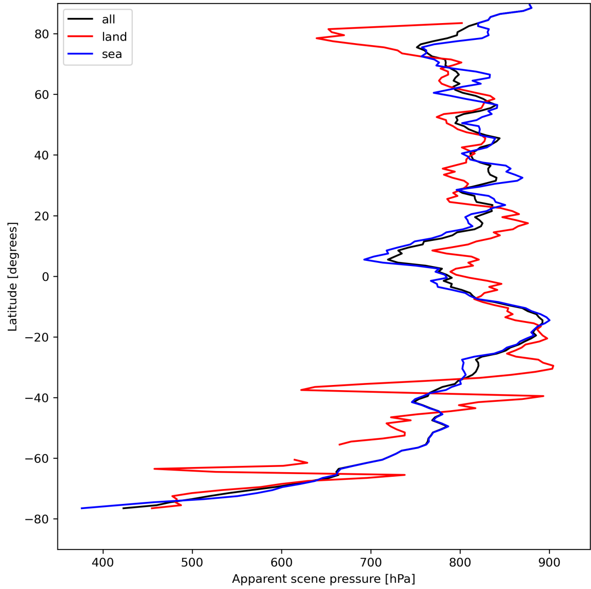
Figure 19: Zonal average of “Apparent scene pressure” for 2023-08-21 to 2023-08-23.
