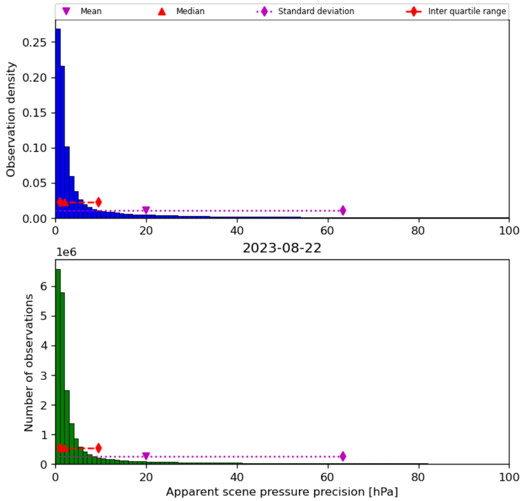
Figure 37: Histogram of “Apparent scene pressure precision” for 2023-08-21 to 2023-08-23
