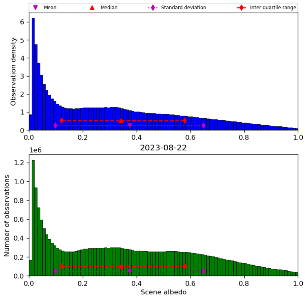
Figure 34: Histogram of “Scene albedo” for 2023-08-21 to 2023-08-23
