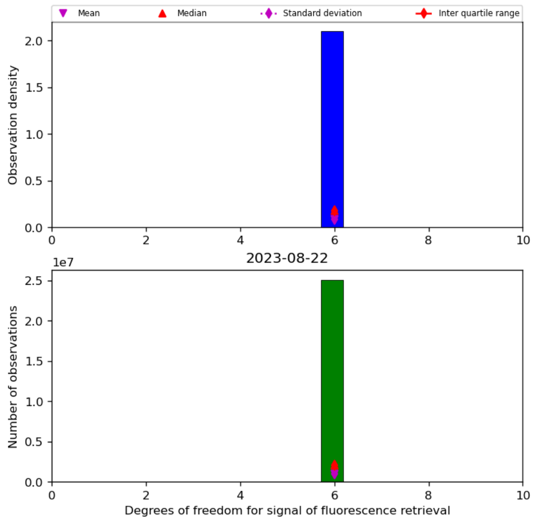
Figure 43: Histogram of “Degrees of freedom for signal of fluorescence retrieval” for 2023-08-21 to 2023-08-23
