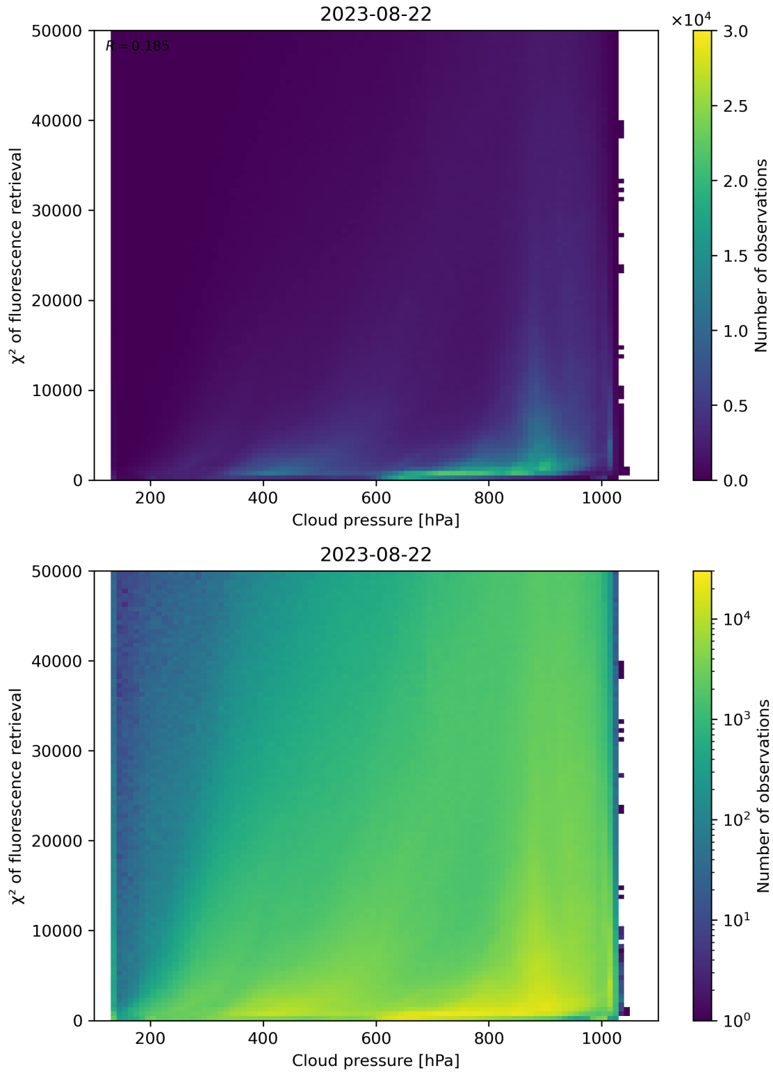
Figure 86: Scatter density plot of “Cloud pressure” against “ \chi^2 of fluorescence retrieval” for 2023-08-21 to 2023-08-23.
