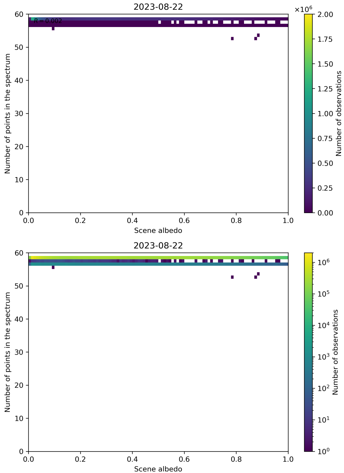
Figure 116: Scatter density plot of “Scene albedo” against “Number of points in the spectrum” for 2023-08-21 to 2023-08-23.
