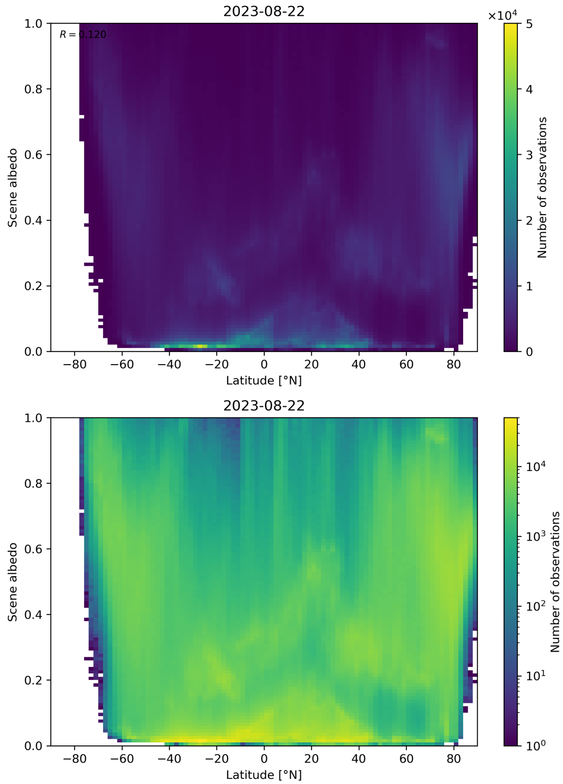
Figure 104: Scatter density plot of “Latitude” against “Scene albedo” for 2023-08-21 to 2023-08-23.
