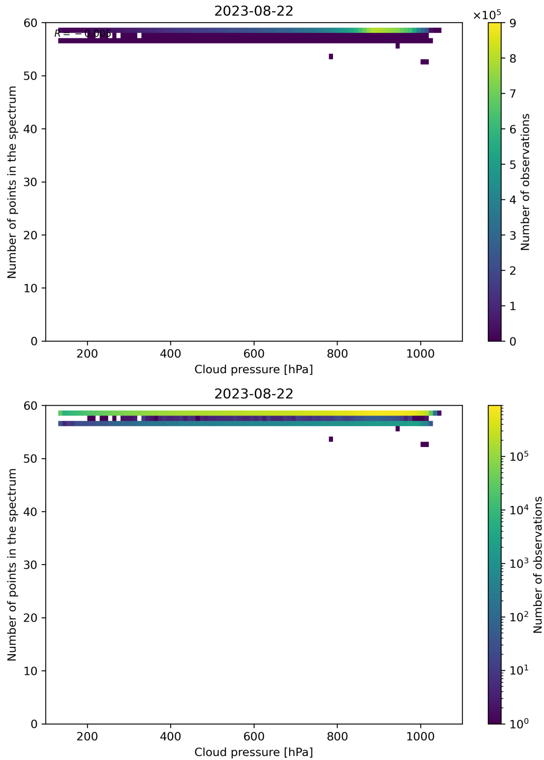
Figure 90: Scatter density plot of “Cloud pressure” against “Number of points in the spectrum” for 2023-08-21 to 2023-08-23.
