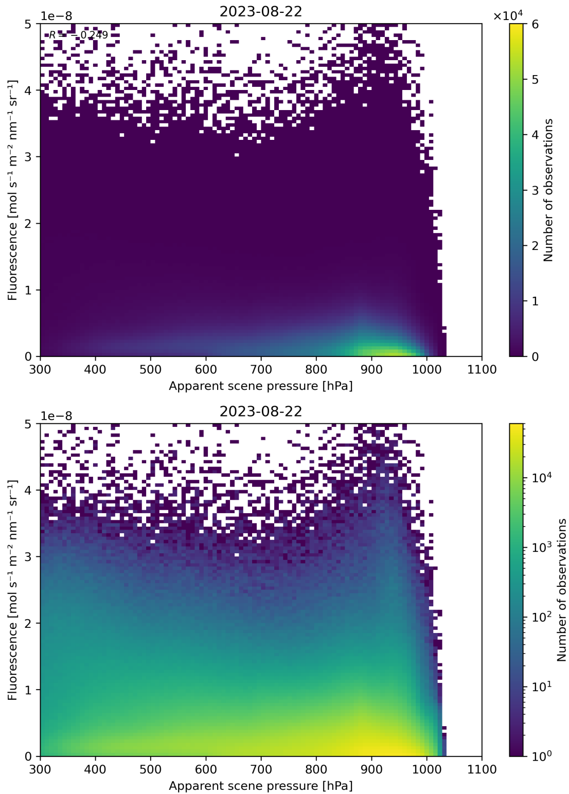
Figure 65: Scatter density plot of “Apparent scene pressure” against “Fluorescence” for 2023-08-21 to 2023-08-23.
