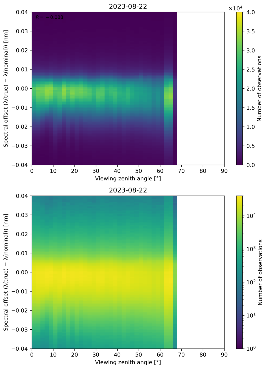
Figure 140: Scatter density plot of “Viewing zenith angle” against “Spectral offset ( \lambda(\text{true}) - \lambda(\text{nominal}) )” for 2023-08-21 to 2023-08-23.
