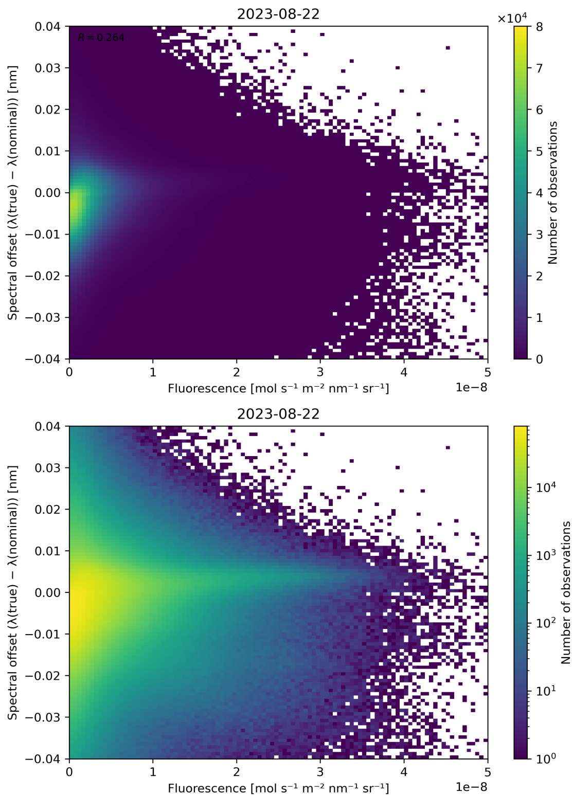
Figure 95: Scatter density plot of “Fluorescence” against “Spectral offset ( \lambda(\text{true}) - \lambda(\text{nominal}) )” for 2023-08-21 to 2023-08-23.
