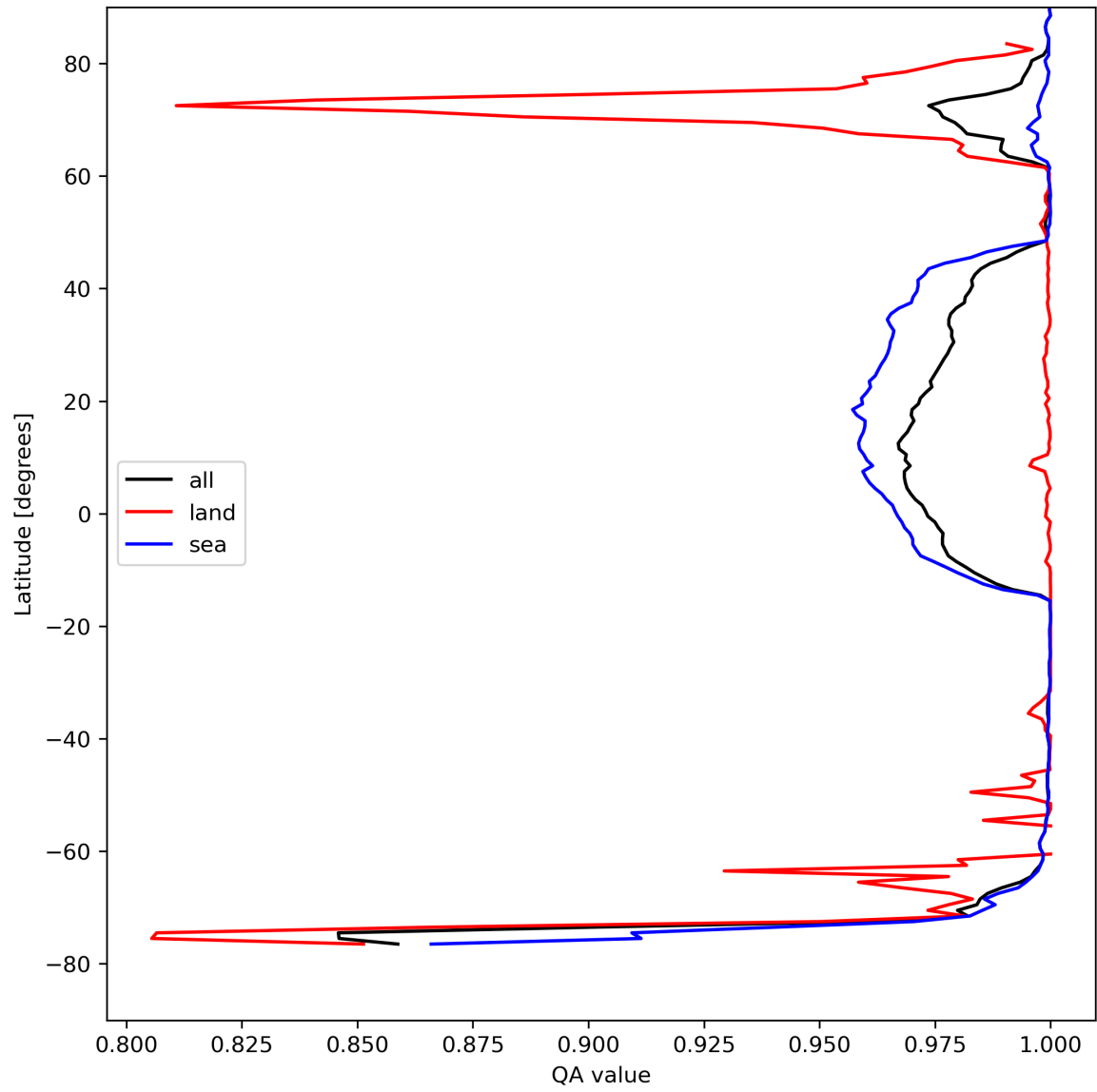
Figure 12: Zonal average of “QA value” for 2023-08-21 to 2023-08-23.
