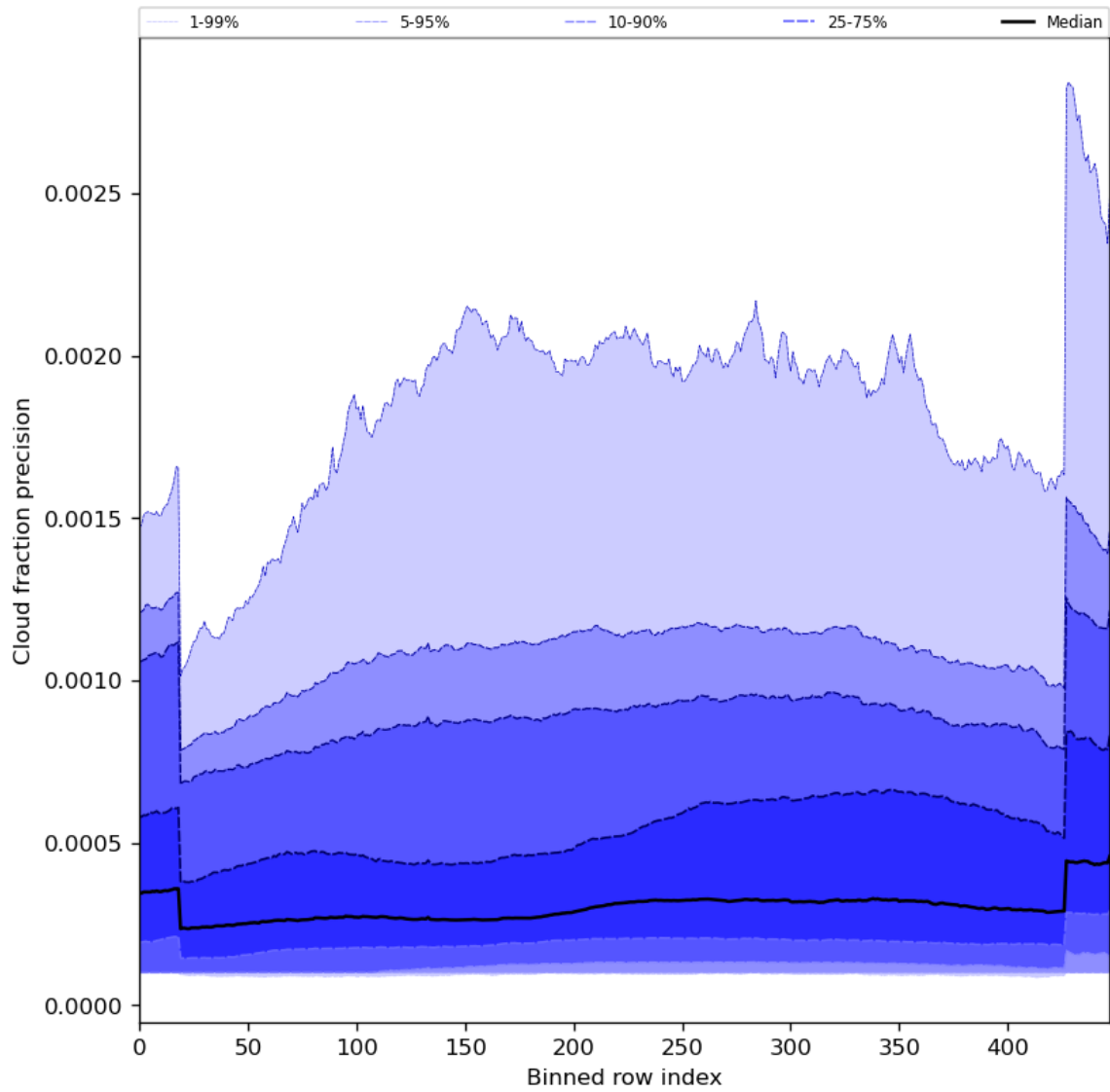
Figure 50: Along track statistics of “Cloud fraction precision” for 2023-08-21 to 2023-08-23
