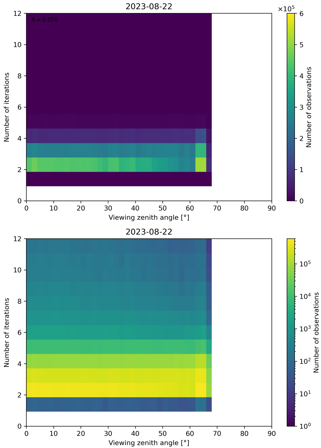
Figure 136: Scatter density plot of “Viewing zenith angle” against “Number of iterations” for 2023-08-21 to 2023-08-23.
