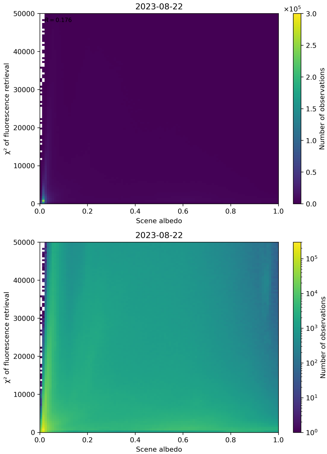
Figure 113: Scatter density plot of “Scene albedo” against “ \chi^2 of fluorescence retrieval” for 2023-08-21 to 2023-08-23.
