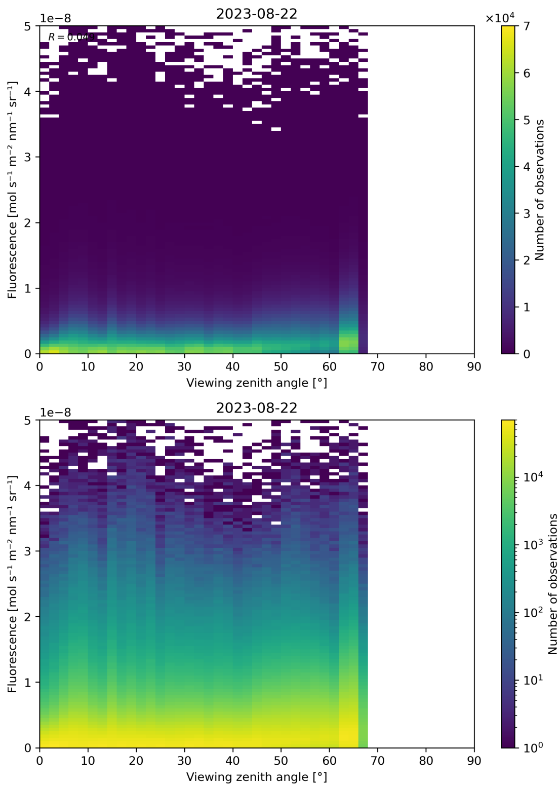
Figure 134: Scatter density plot of “Viewing zenith angle” against “Fluorescence” for 2023-08-21 to 2023-08-23.
