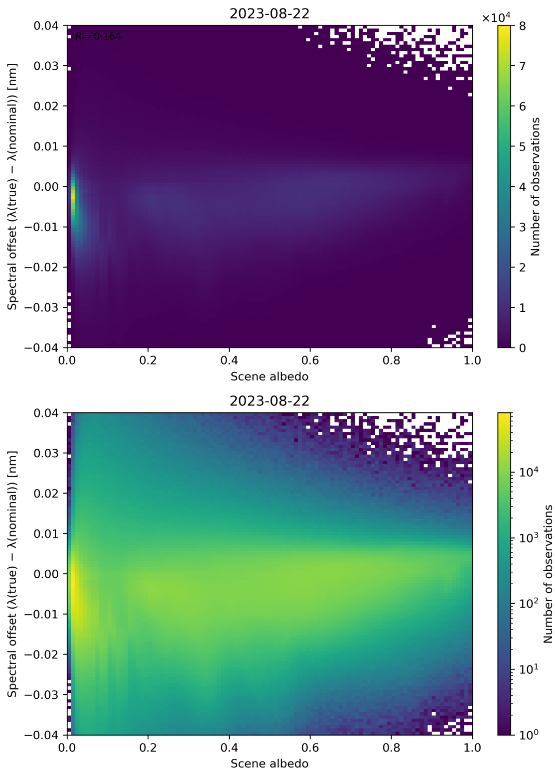
Figure 117: Scatter density plot of “Scene albedo” against “Spectral offset ( \lambda(\text{true}) - \lambda(\text{nominal}) )” for 2023-08-21 to 2023-08-23.
