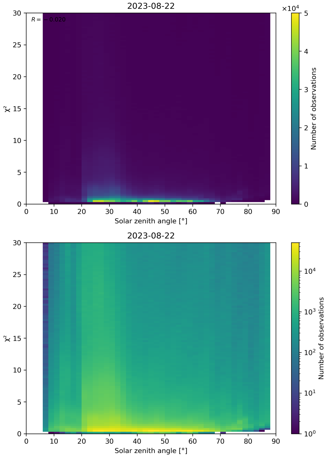
Figure 119: Scatter density plot of “Solar zenith angle” against “ \chi^2 ” for 2023-08-21 to 2023-08-23.
