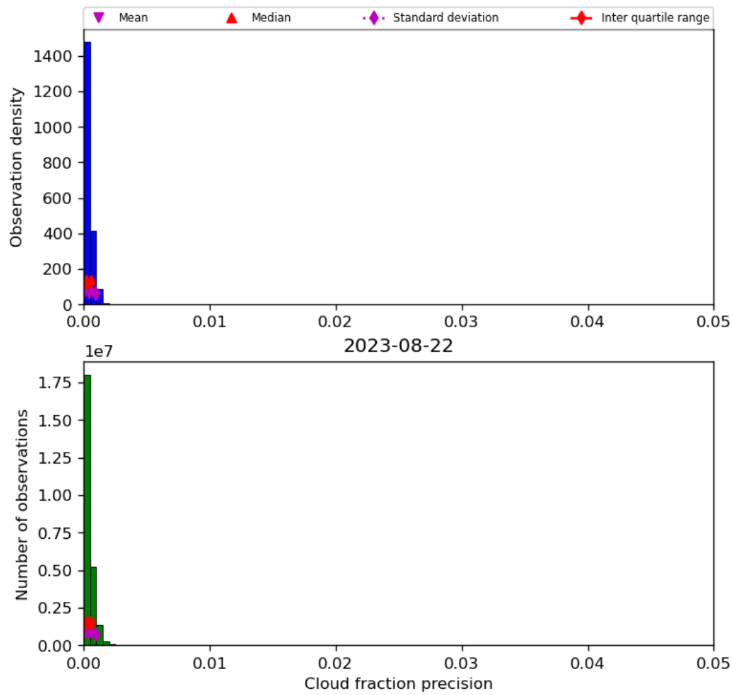
Figure 33: Histogram of “Cloud fraction precision” for 2023-08-21 to 2023-08-23
