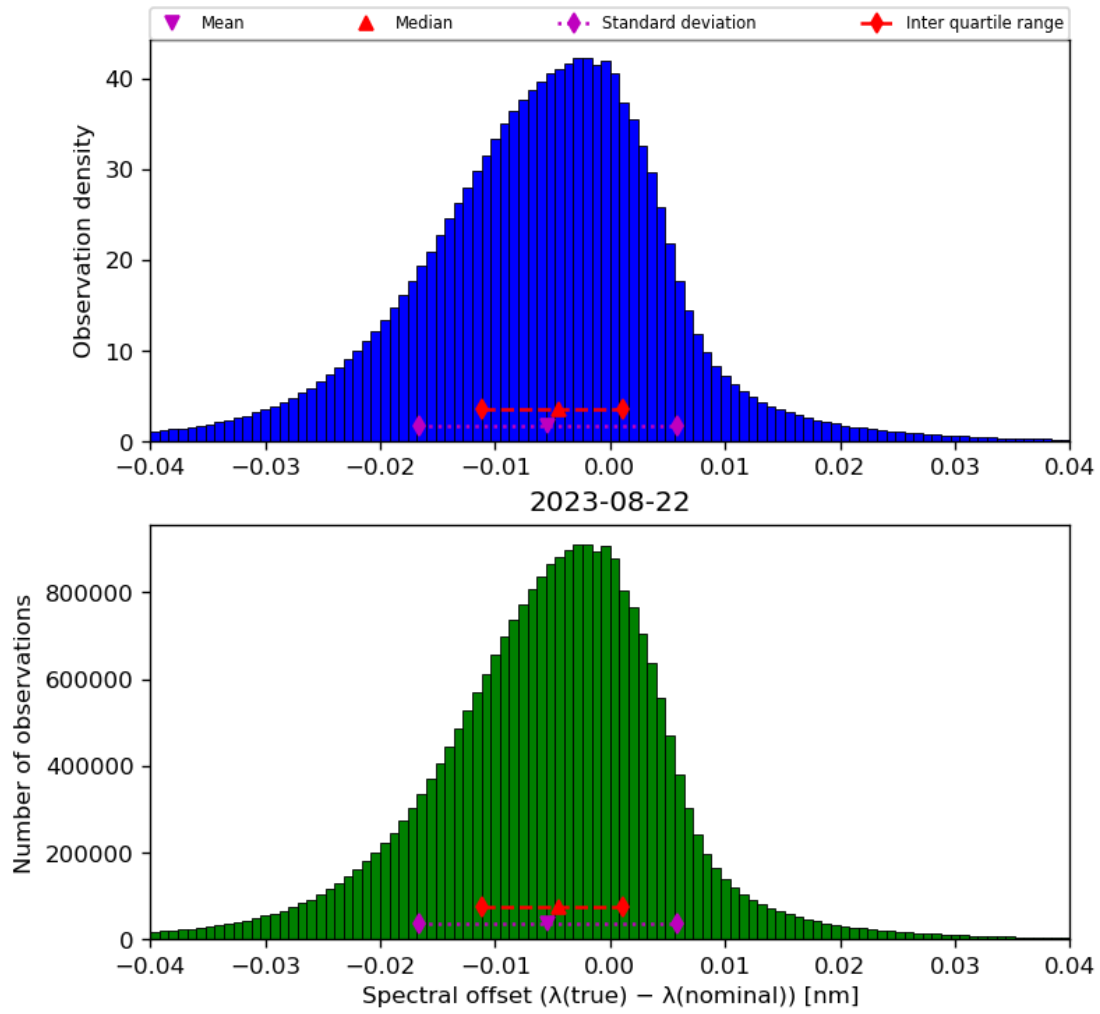
Figure 45: Histogram of “Spectral offset ( \lambda(\text{true}) - \lambda(\text{nominal}) )” for 2023-08-21 to 2023-08-23
