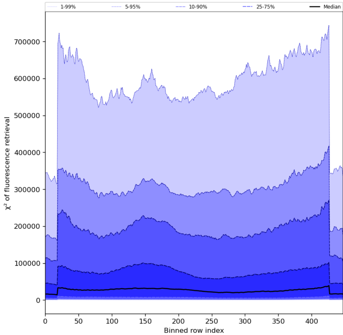
Figure 59: Along track statistics of “ \chi^2 of fluorescence retrieval” for 2023-08-21 to 2023-08-23
