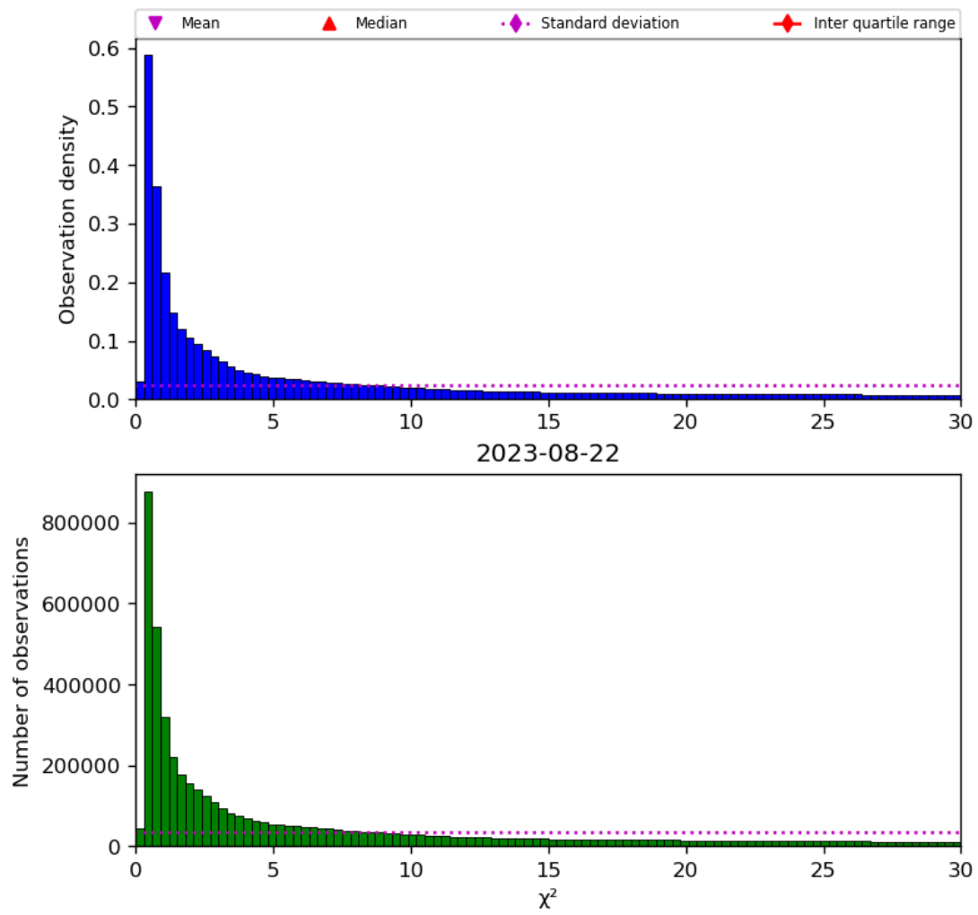
Figure 38: Histogram of “ \chi^2 ” for 2023-08-21 to 2023-08-23
