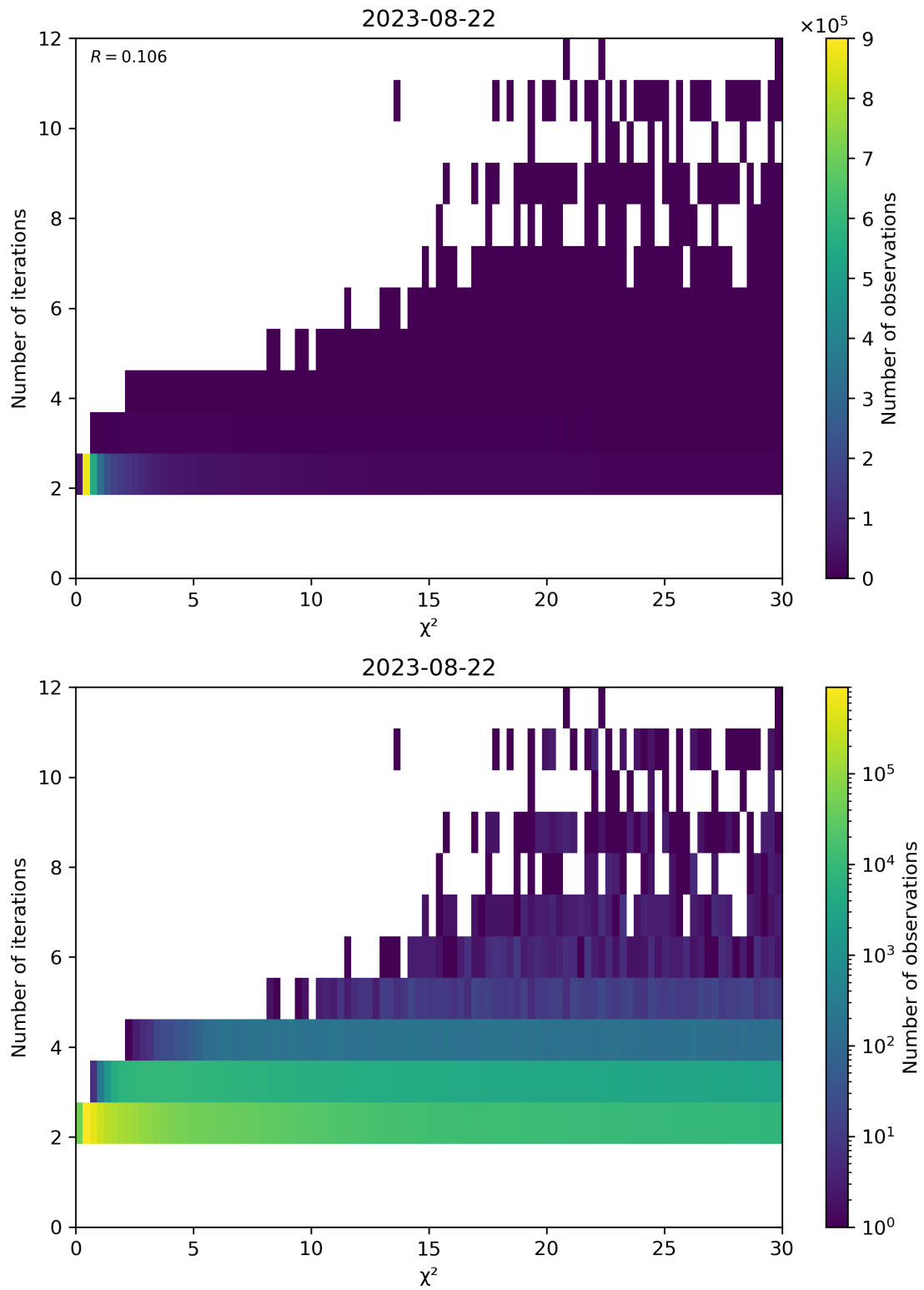
Figure 73: Scatter density plot of “ \chi^2 ” against “Number of iterations” for 2023-08-21 to 2023-08-23.
