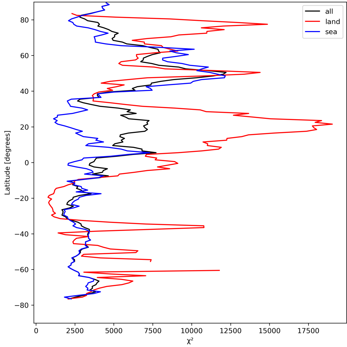
Figure 21: Zonal average of “ \chi^2 ” for 2023-08-21 to 2023-08-23.
