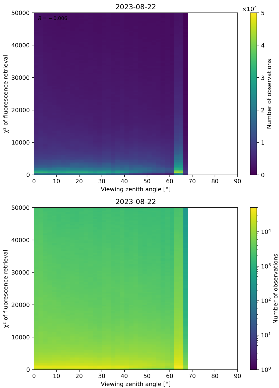
Figure 131: Scatter density plot of “Viewing zenith angle” against “ \chi^2 of fluorescence retrieval” for 2023-08-21 to 2023-08-23.
