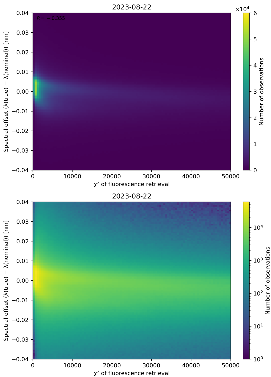
Figure 72: Scatter density plot of " \chi^2 of fluorescence retrieval" against "Spectral offset ( \lambda(\text{true}) - \lambda(\text{nominal})) " for 2023-08-21 to 2023-08-23.
