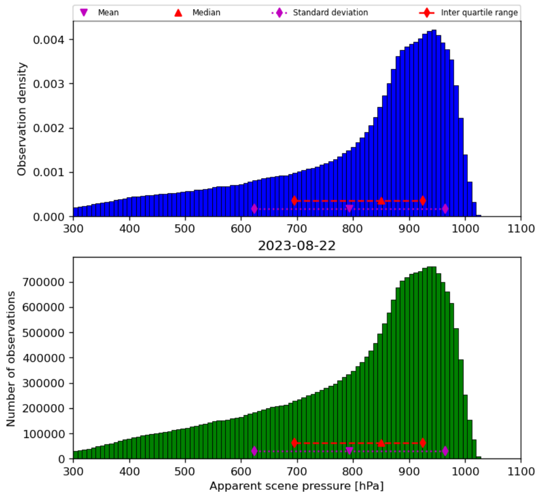
Figure 36: Histogram of “Apparent scene pressure” for 2023-08-21 to 2023-08-23
