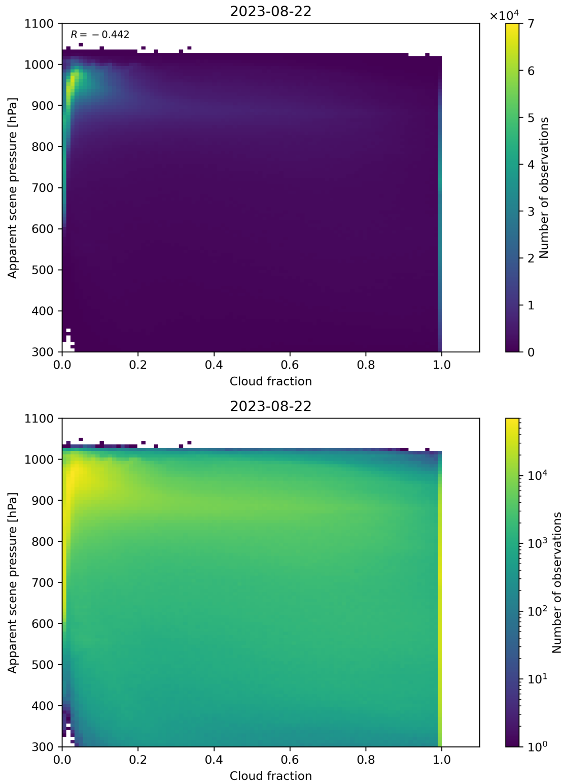
Figure 76: Scatter density plot of “Cloud fraction” against “Apparent scene pressure” for 2023-08-21 to 2023-08-23.
