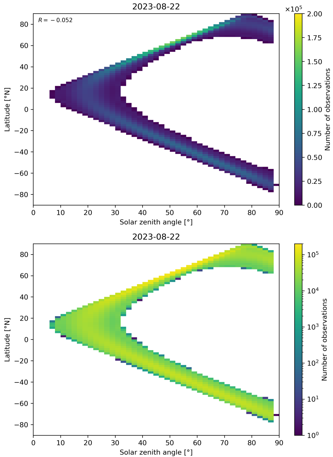
Figure 124: Scatter density plot of “Solar zenith angle” against “Latitude” for 2023-08-21 to 2023-08-23.
