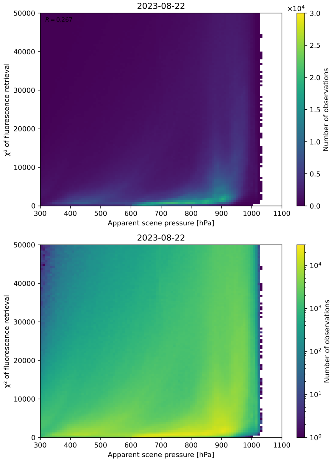
Figure 64: Scatter density plot of “Apparent scene pressure” against “ \chi^2 of fluorescence retrieval” for 2023-08-21 to 2023-08-23.
