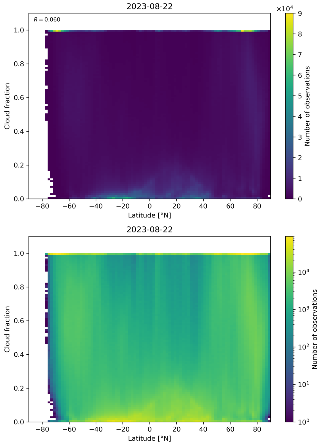
Figure 99: Scatter density plot of “Latitude” against “Cloud fraction” for 2023-08-21 to 2023-08-23.
