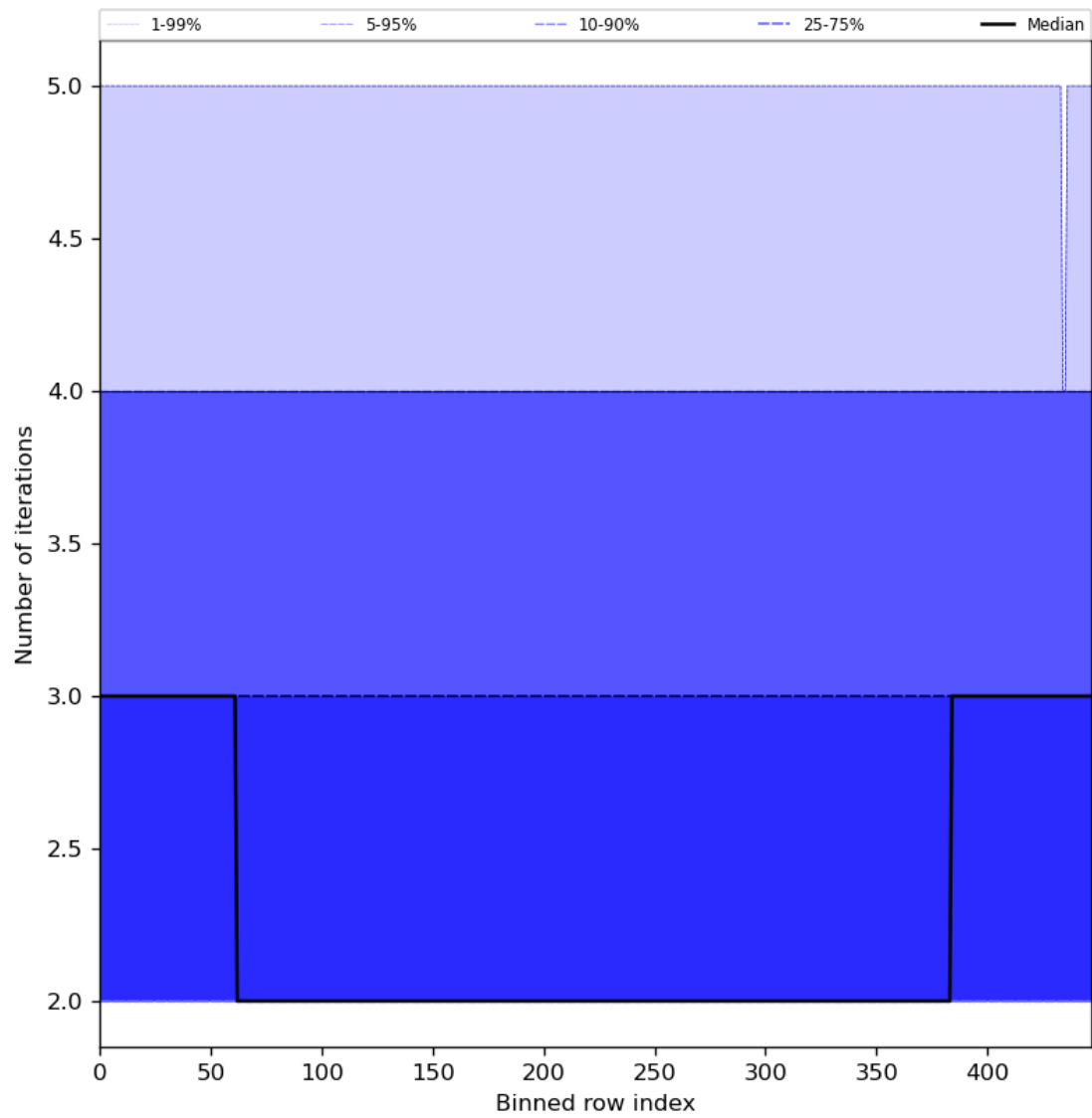
Figure 56: Along track statistics of “Number of iterations” for 2023-08-21 to 2023-08-23
