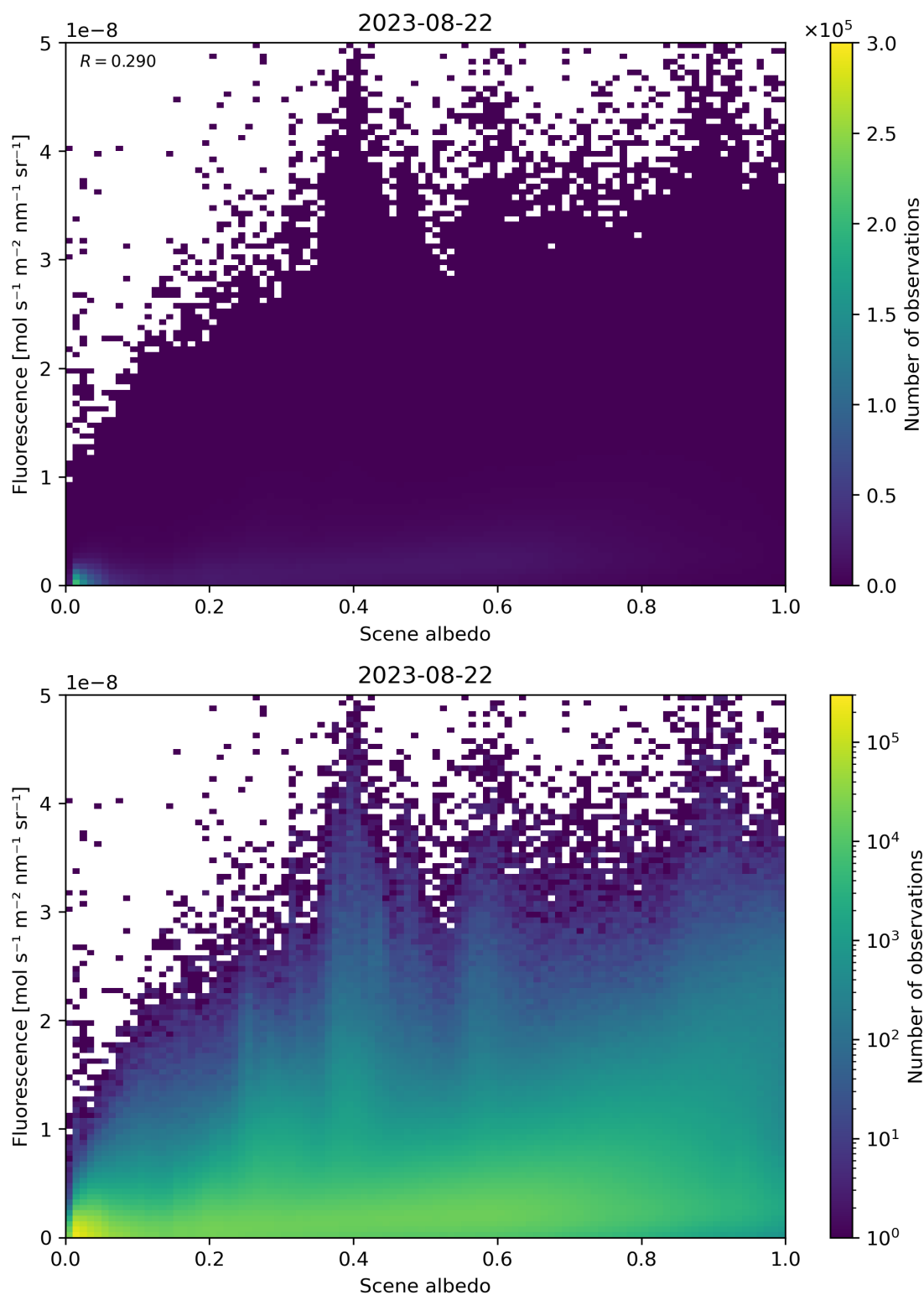
Figure 114: Scatter density plot of “Scene albedo” against “Fluorescence” for 2023-08-21 to 2023-08-23.
