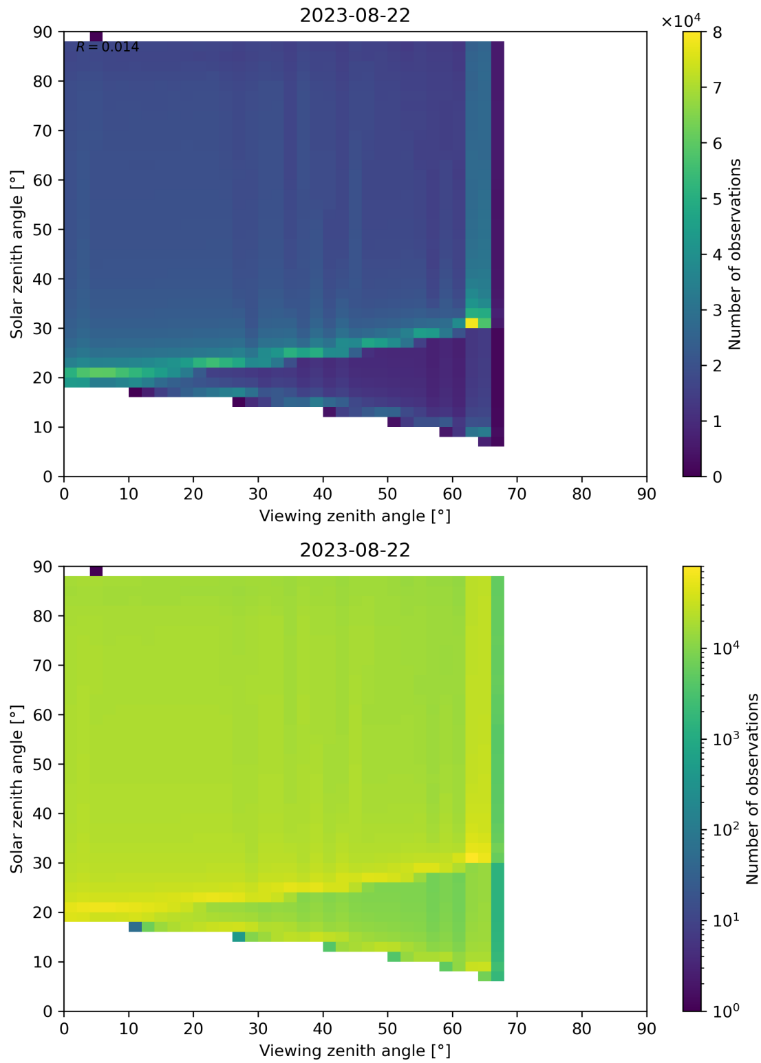
Figure 139: Scatter density plot of “Viewing zenith angle” against “Solar zenith angle” for 2023-08-21 to 2023-08-23.
