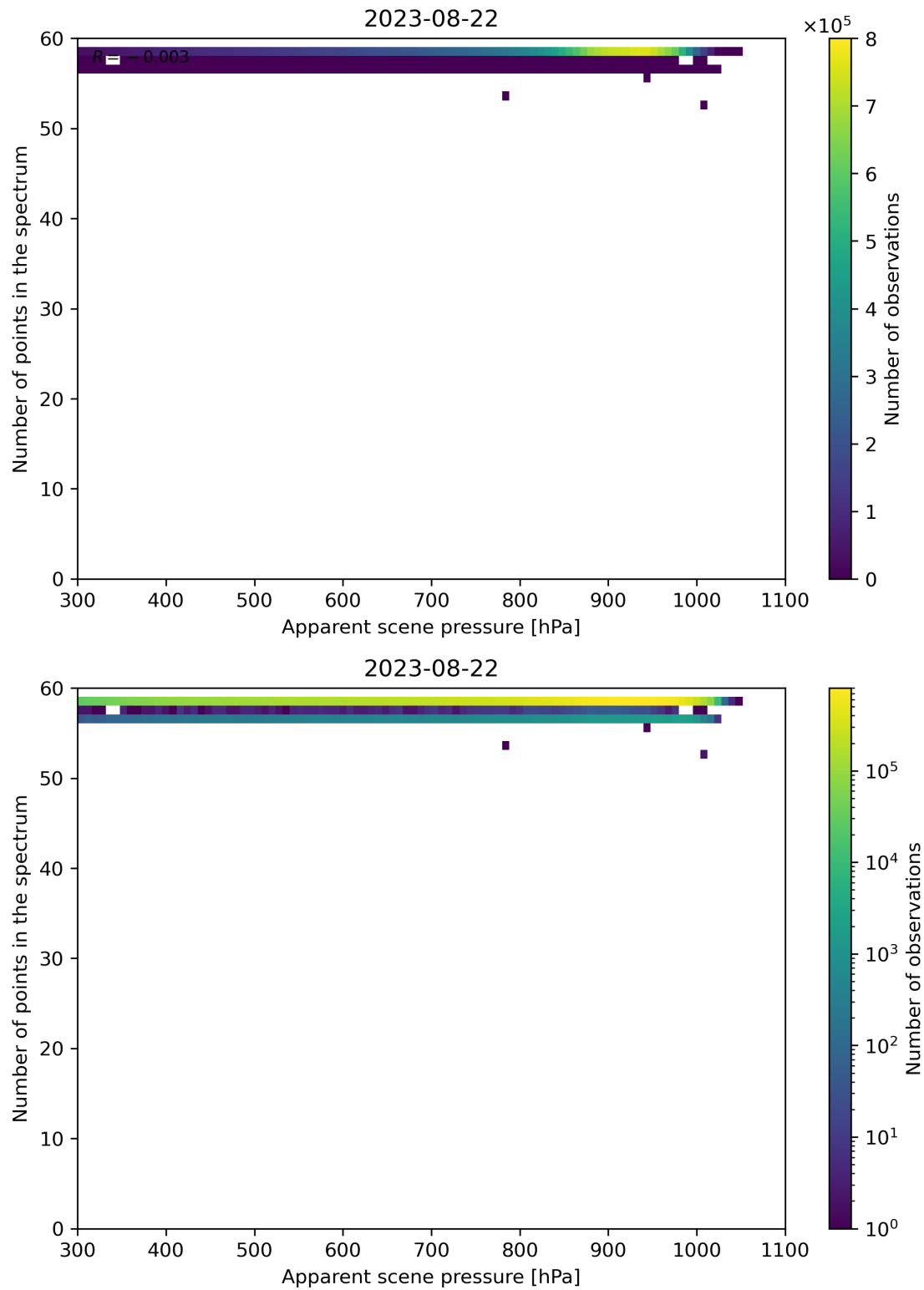
Figure 67: Scatter density plot of “Apparent scene pressure” against “Number of points in the spectrum” for 2023-08-21 to 2023-08-23.
