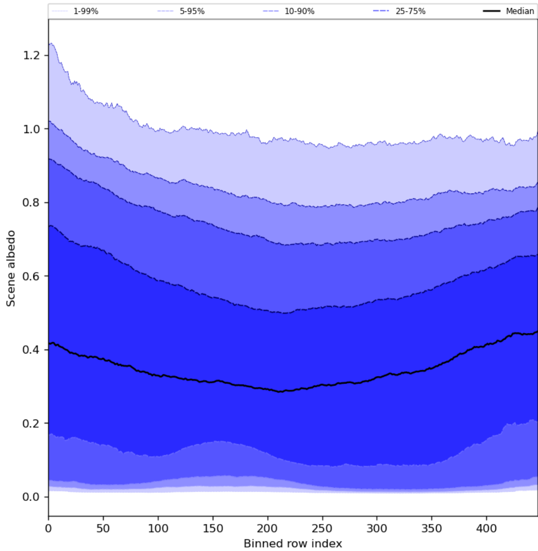
Figure 51: Along track statistics of “Scene albedo” for 2023-08-21 to 2023-08-23
