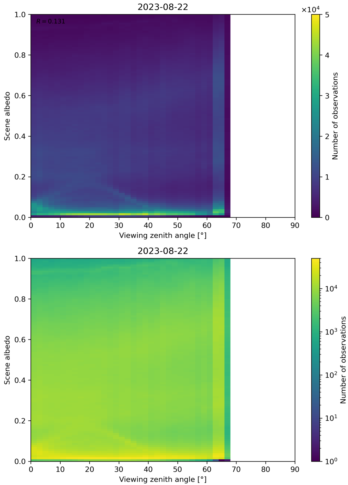
Figure 138: Scatter density plot of “Viewing zenith angle” against “Scene albedo” for 2023-08-21 to 2023-08-23.
