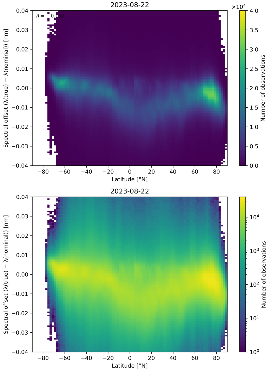
Figure 105: Scatter density plot of “Latitude” against “Spectral offset ( \lambda(\text{true}) - \lambda(\text{nominal}) )” for 2023-08-21 to 2023-08-23.
