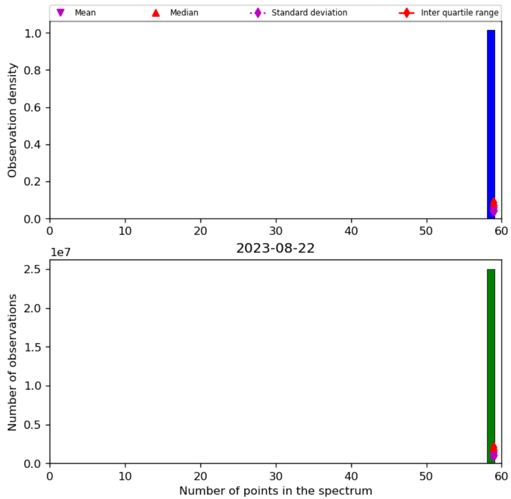
Figure 44: Histogram of “Number of points in the spectrum” for 2023-08-21 to 2023-08-23
