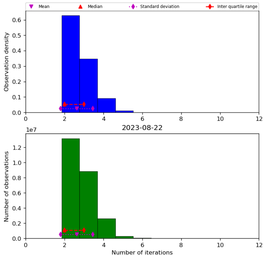
Figure 39: Histogram of “Number of iterations” for 2023-08-21 to 2023-08-23
