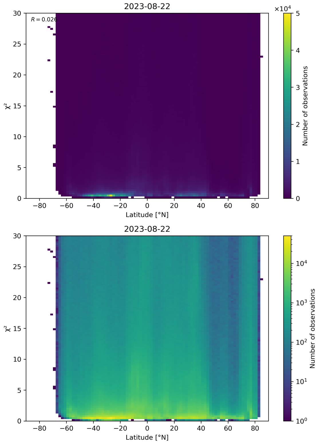
Figure 97: Scatter density plot of “Latitude” against “ \chi^2 ” for 2023-08-21 to 2023-08-23.
