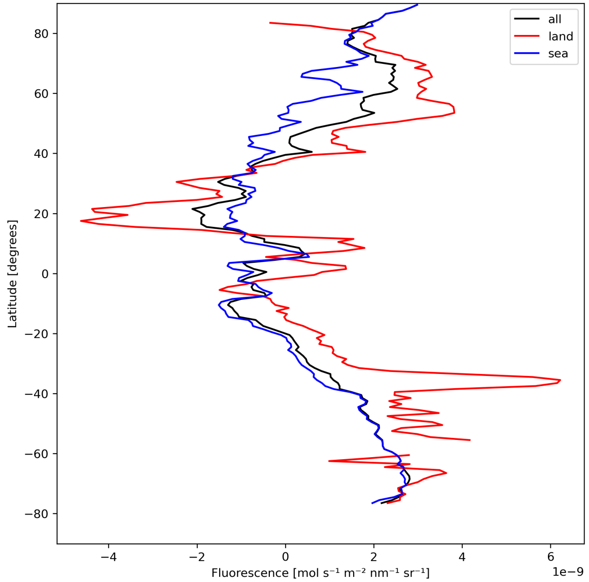
Figure 23: Zonal average of “Fluorescence” for 2023-08-21 to 2023-08-23.
