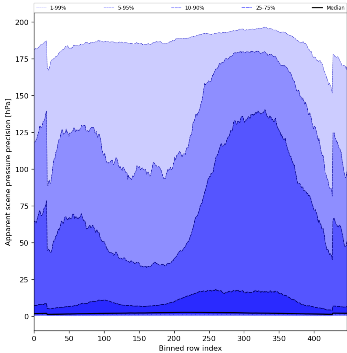
Figure 54: Along track statistics of “Apparent scene pressure precision” for 2023-08-21 to 2023-08-23
