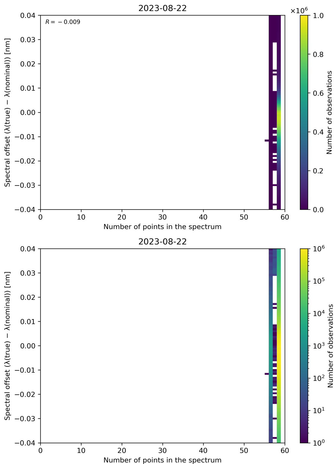
Figure 110: Scatter density plot of “Number of points in the spectrum” against “Spectral offset ( \lambda(\text{true}) - \lambda(\text{nominal}) )” for 2023-08-21 to 2023-08-23.
