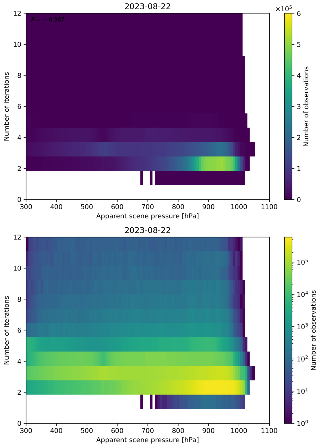
Figure 66: Scatter density plot of “Apparent scene pressure” against “Number of iterations” for 2023-08-21 to 2023-08-23.
