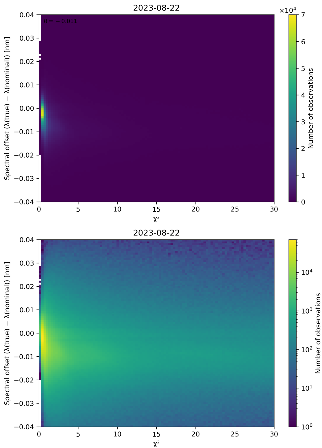
Figure 75: Scatter density plot of “ \chi^2 ” against “Spectral offset ( \lambda(\text{true}) - \lambda(\text{nominal}) )” for 2023-08-21 to 2023-08-23.
