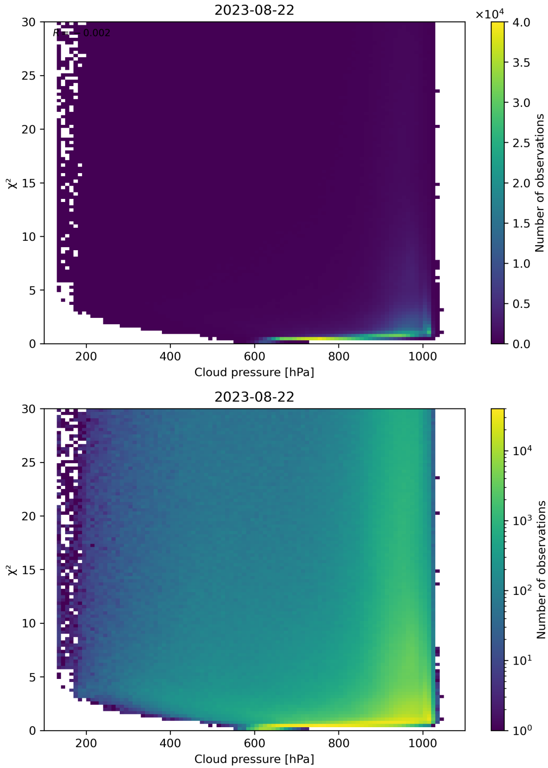
Figure 85: Scatter density plot of “Cloud pressure” against “ \chi^2 ” for 2023-08-21 to 2023-08-23.
