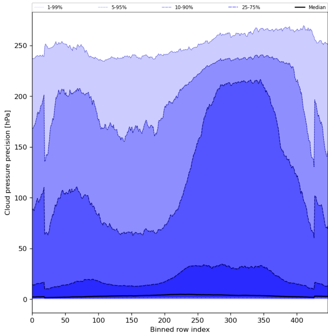
Figure 48: Along track statistics of “Cloud pressure precision” for 2023-08-21 to 2023-08-23
