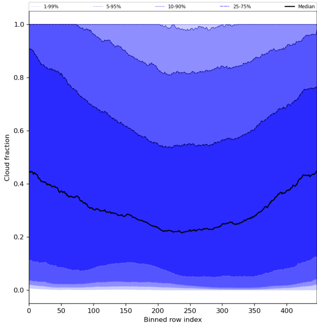
Figure 49: Along track statistics of “Cloud fraction” for 2023-08-21 to 2023-08-23
