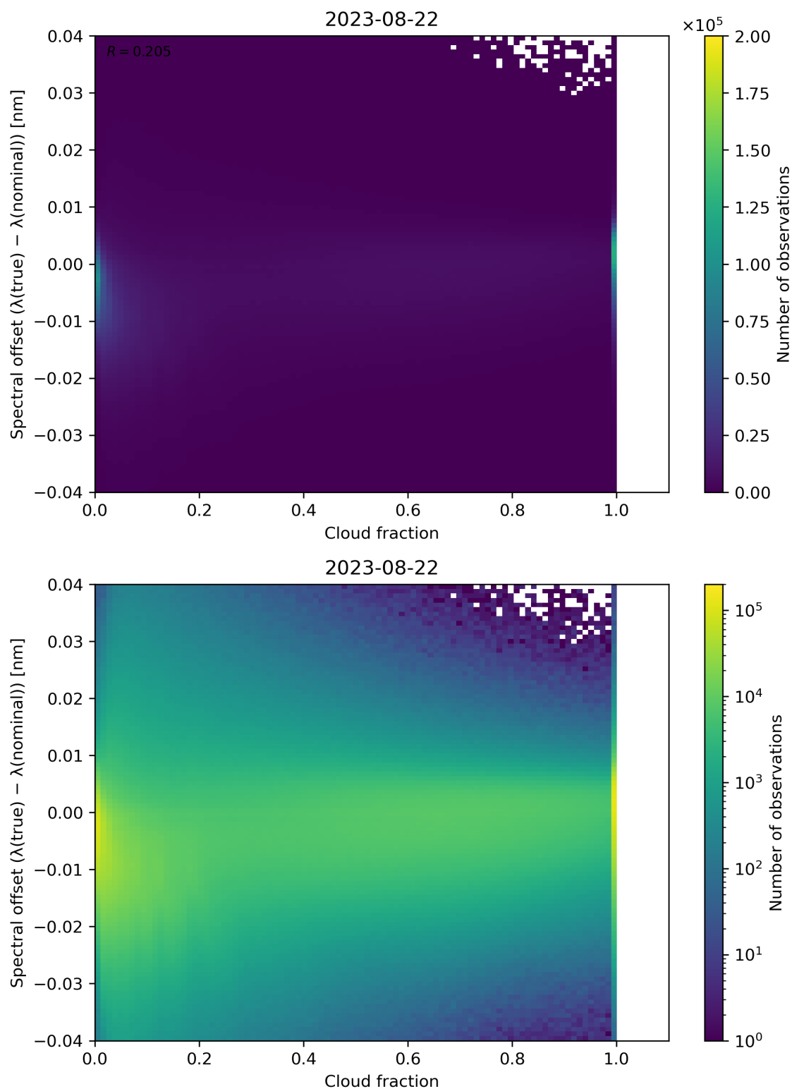
Figure 83: Scatter density plot of “Cloud fraction” against “Spectral offset ( \lambda(\text{true}) - \lambda(\text{nominal}) )” for 2023-08-21 to 2023-08-23.
