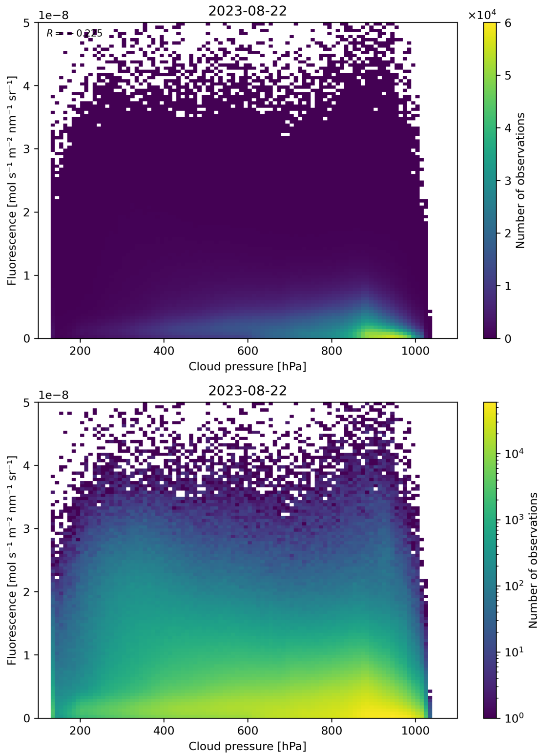
Figure 88: Scatter density plot of “Cloud pressure” against “Fluorescence” for 2023-08-21 to 2023-08-23.
