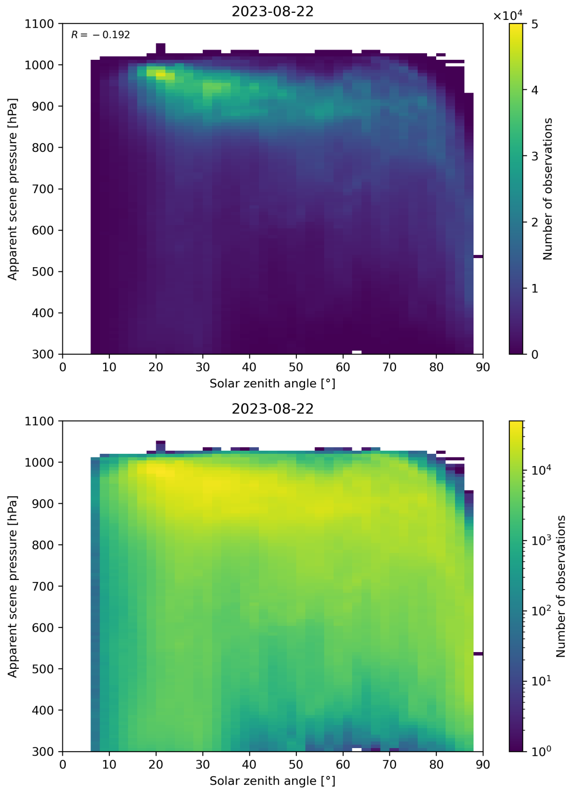
Figure 118: Scatter density plot of “Solar zenith angle” against “Apparent scene pressure” for 2023-08-21 to 2023-08-23.
