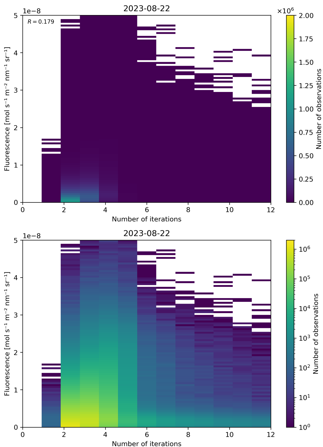
Figure 107: Scatter density plot of “Number of iterations” against “Fluorescence” for 2023-08-21 to 2023-08-23.
