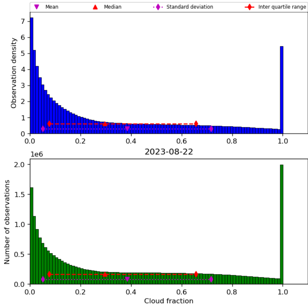
Figure 32: Histogram of “Cloud fraction” for 2023-08-21 to 2023-08-23
