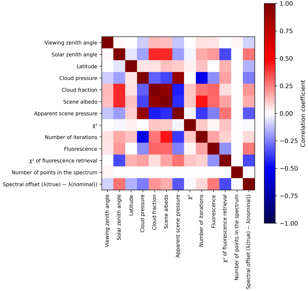
Figure 2: Map of correlation matrix for 2023-08-21 to 2023-08-23.
