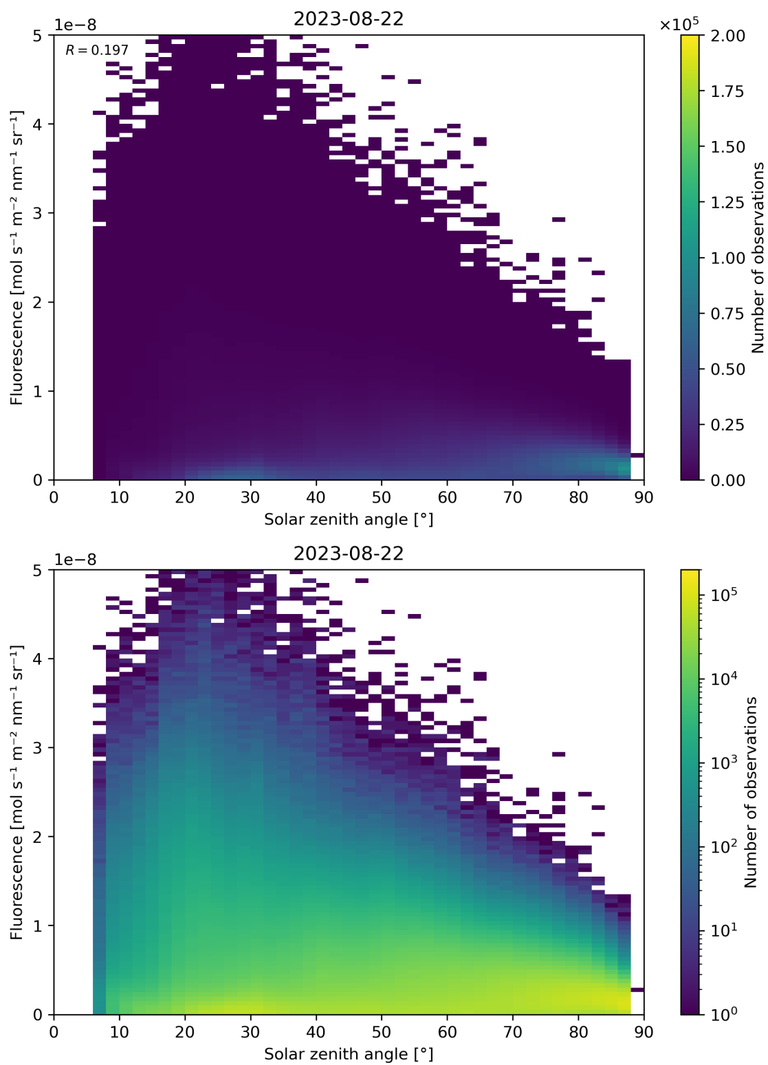
Figure 123: Scatter density plot of “Solar zenith angle” against “Fluorescence” for 2023-08-21 to 2023-08-23.
