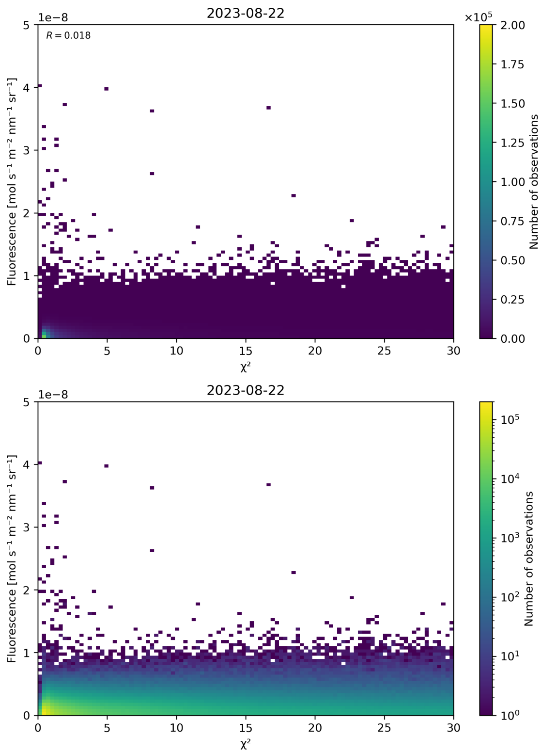
Figure 70: Scatter density plot of “ \chi^2 ” against “Fluorescence” for 2023-08-21 to 2023-08-23.
