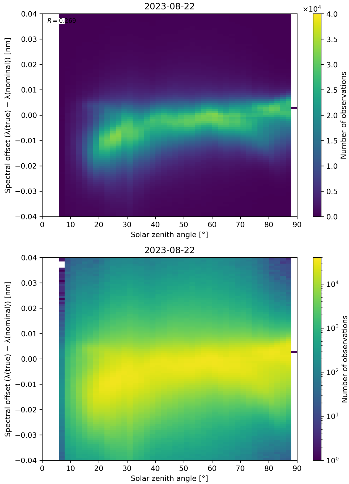
Figure 128: Scatter density plot of “Solar zenith angle” against “Spectral offset ( \lambda(\text{true}) - \lambda(\text{nominal}) )” for 2023-08-21 to 2023-08-23.
