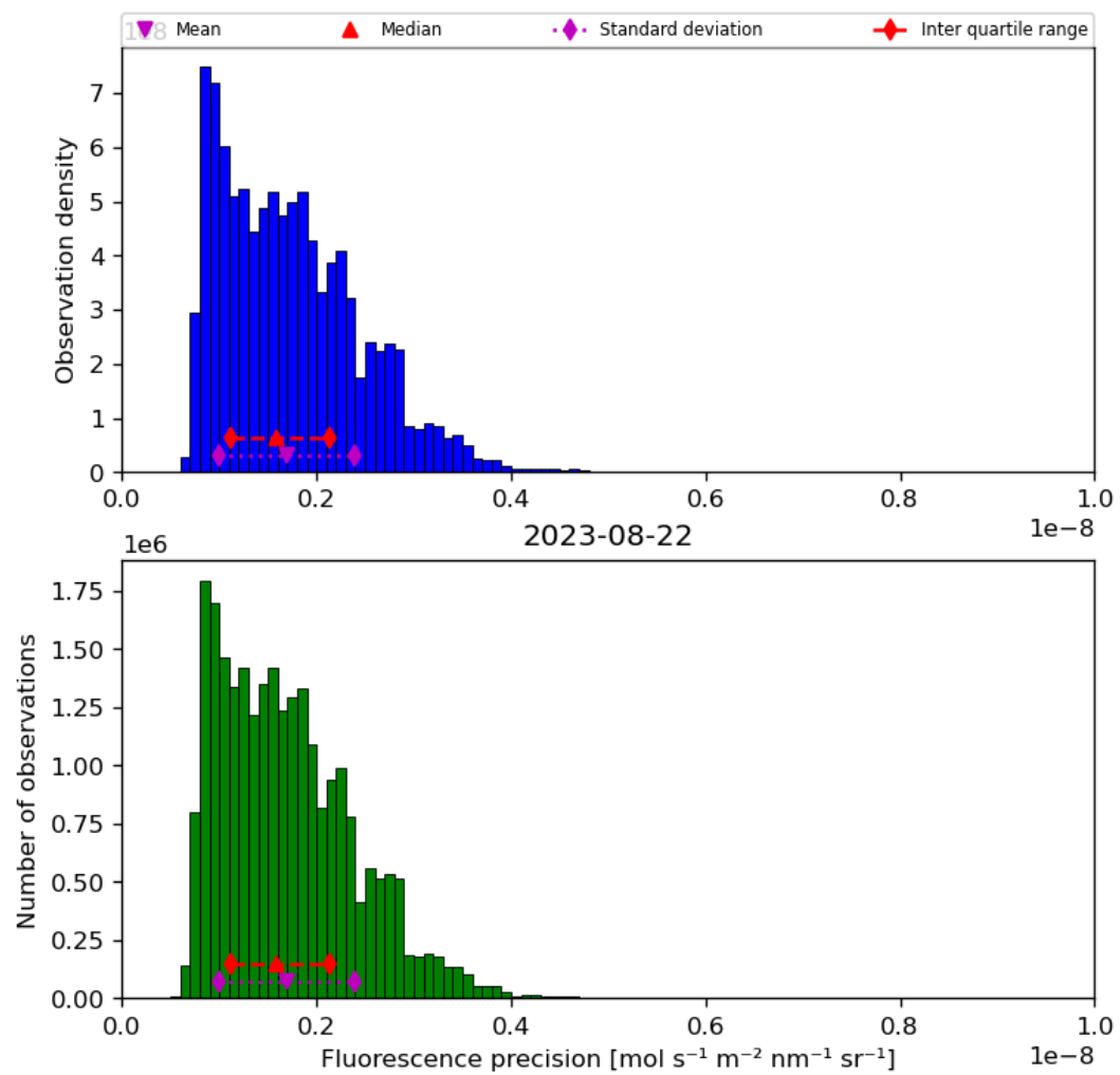
Figure 41: Histogram of “Fluorescence precision” for 2023-08-21 to 2023-08-23
