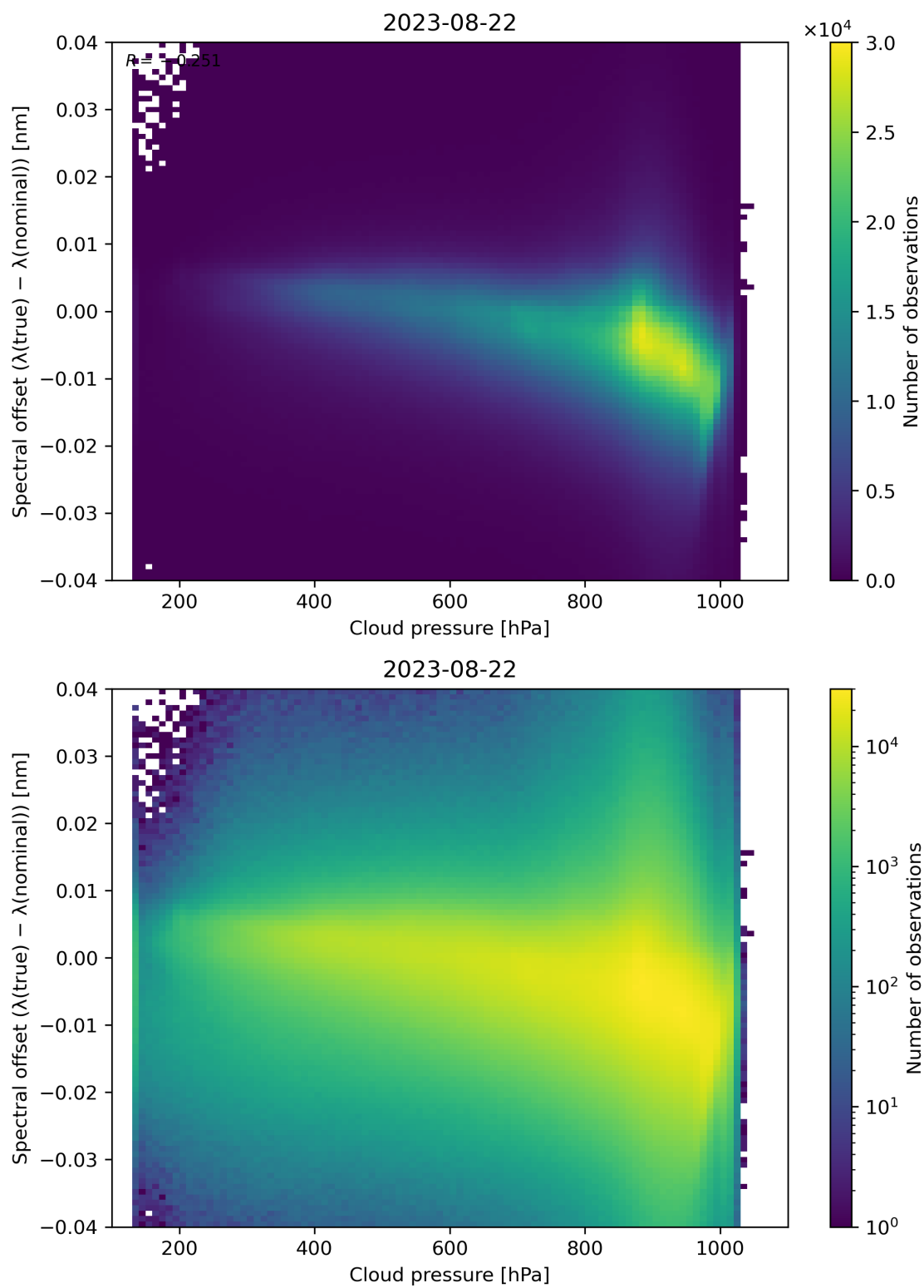
Figure 92: Scatter density plot of “Cloud pressure” against “Spectral offset ( \lambda(\text{true}) - \lambda(\text{nominal}) )” for 2023-08-21 to 2023-08-23.
