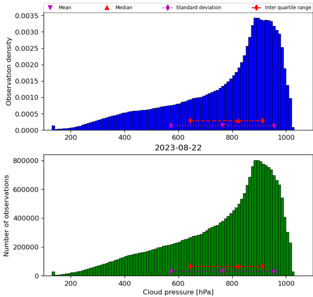
Figure 30: Histogram of “Cloud pressure” for 2023-08-21 to 2023-08-23
