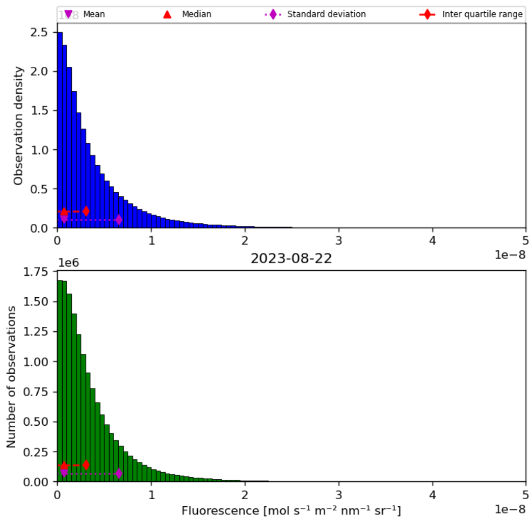
Figure 40: Histogram of “Fluorescence” for 2023-08-21 to 2023-08-23
