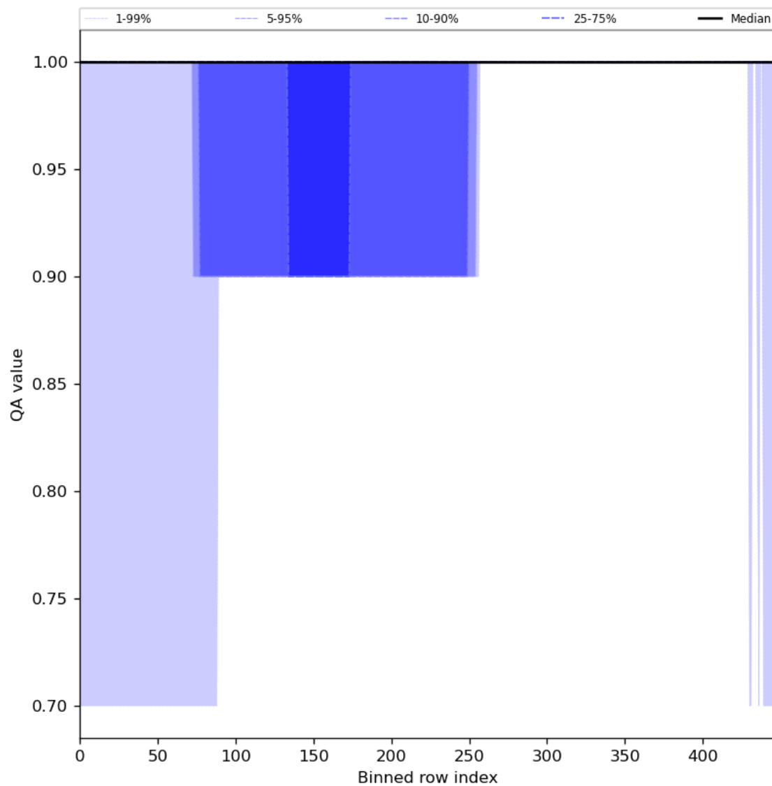
Figure 46: Along track statistics of “QA value” for 2023-08-21 to 2023-08-23
