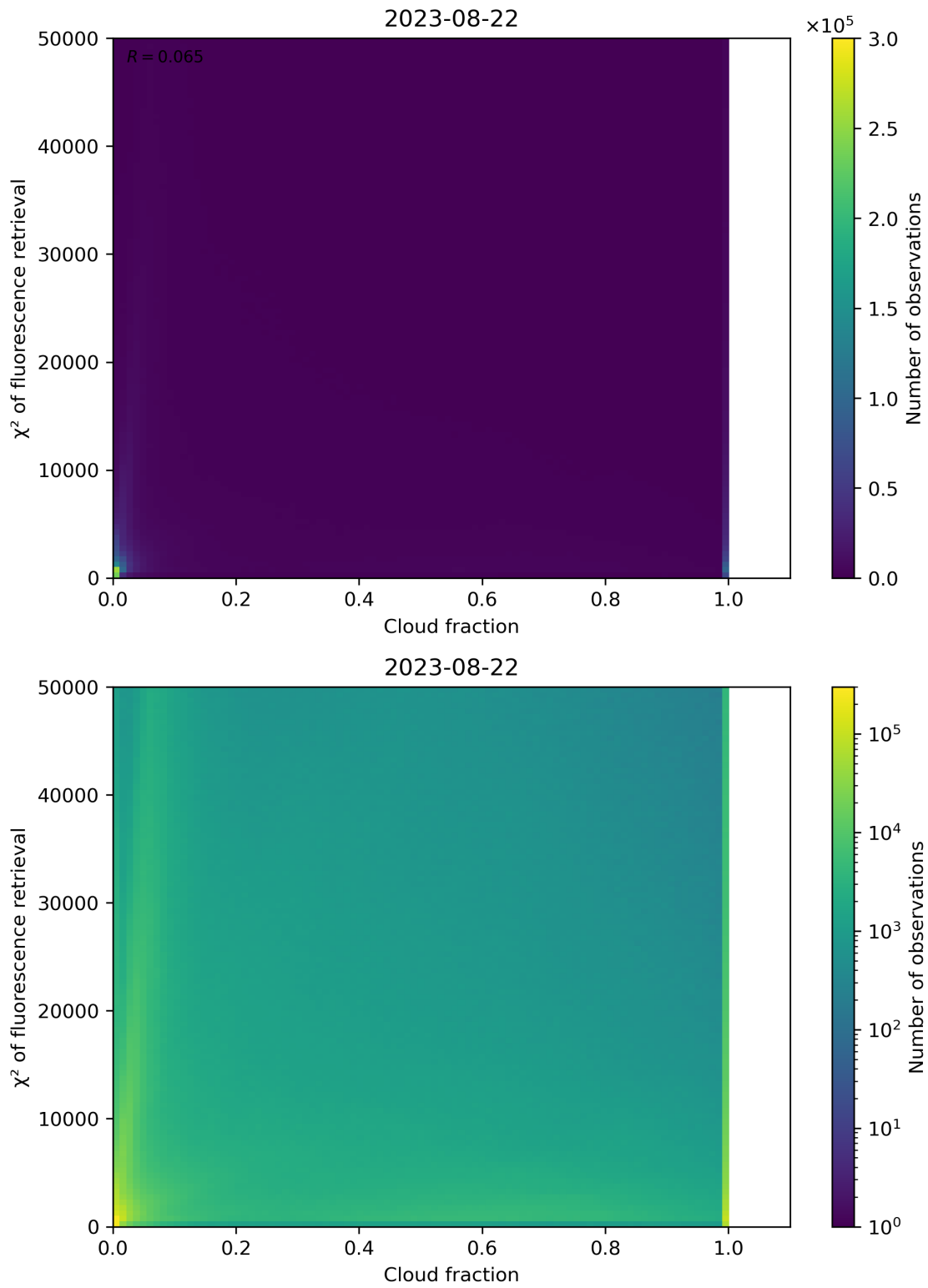
Figure 78: Scatter density plot of “Cloud fraction” against “ \chi^2 of fluorescence retrieval” for 2023-08-21 to 2023-08-23.
