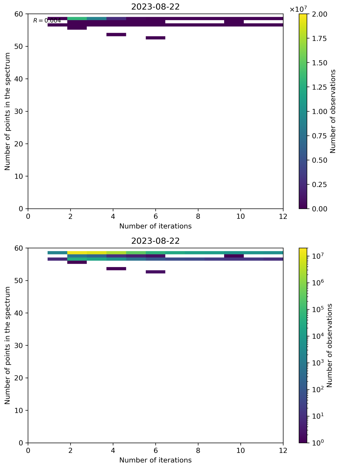
Figure 108: Scatter density plot of “Number of iterations” against “Number of points in the spectrum” for 2023-08-21 to 2023-08-23.
