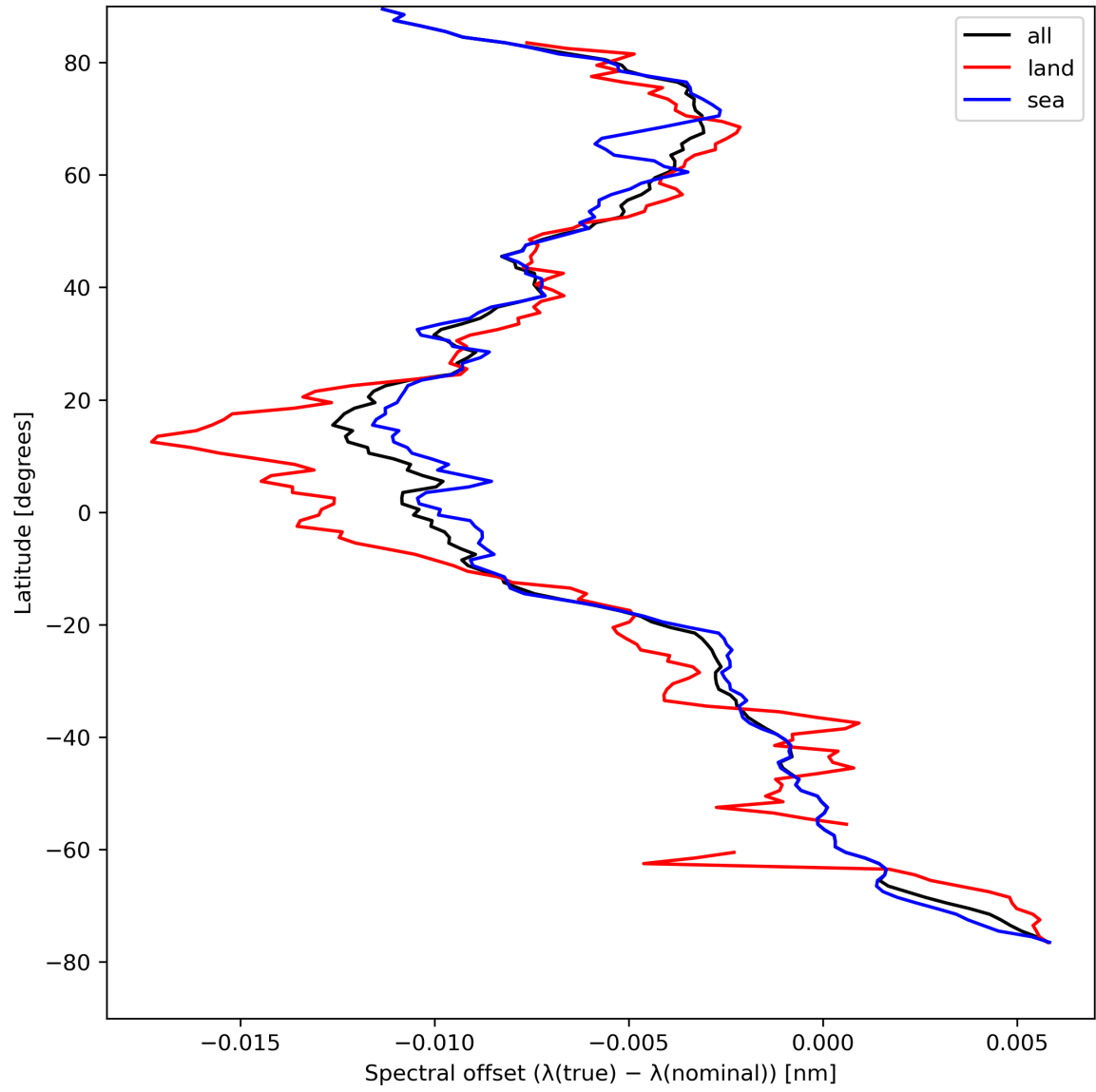
Figure 28: Zonal average of “Spectral offset ( \lambda(\text{true}) - \lambda(\text{nominal}) )” for 2023-08-21 to 2023-08-23.
