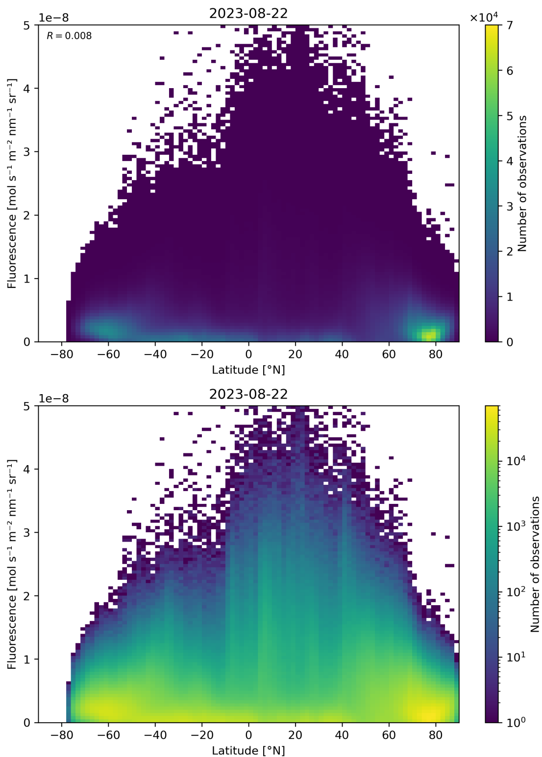
Figure 101: Scatter density plot of “Latitude” against “Fluorescence” for 2023-08-21 to 2023-08-23.
