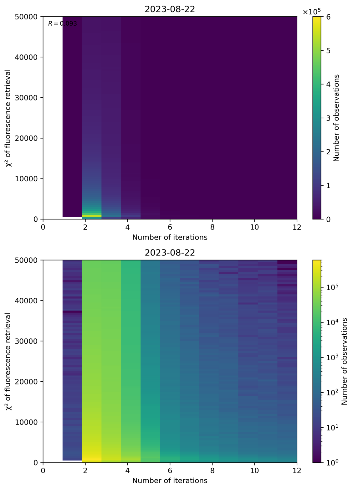
Figure 106: Scatter density plot of “Number of iterations” against “ \chi^2 of fluorescence retrieval” for 2023-08-21 to 2023-08-23.
