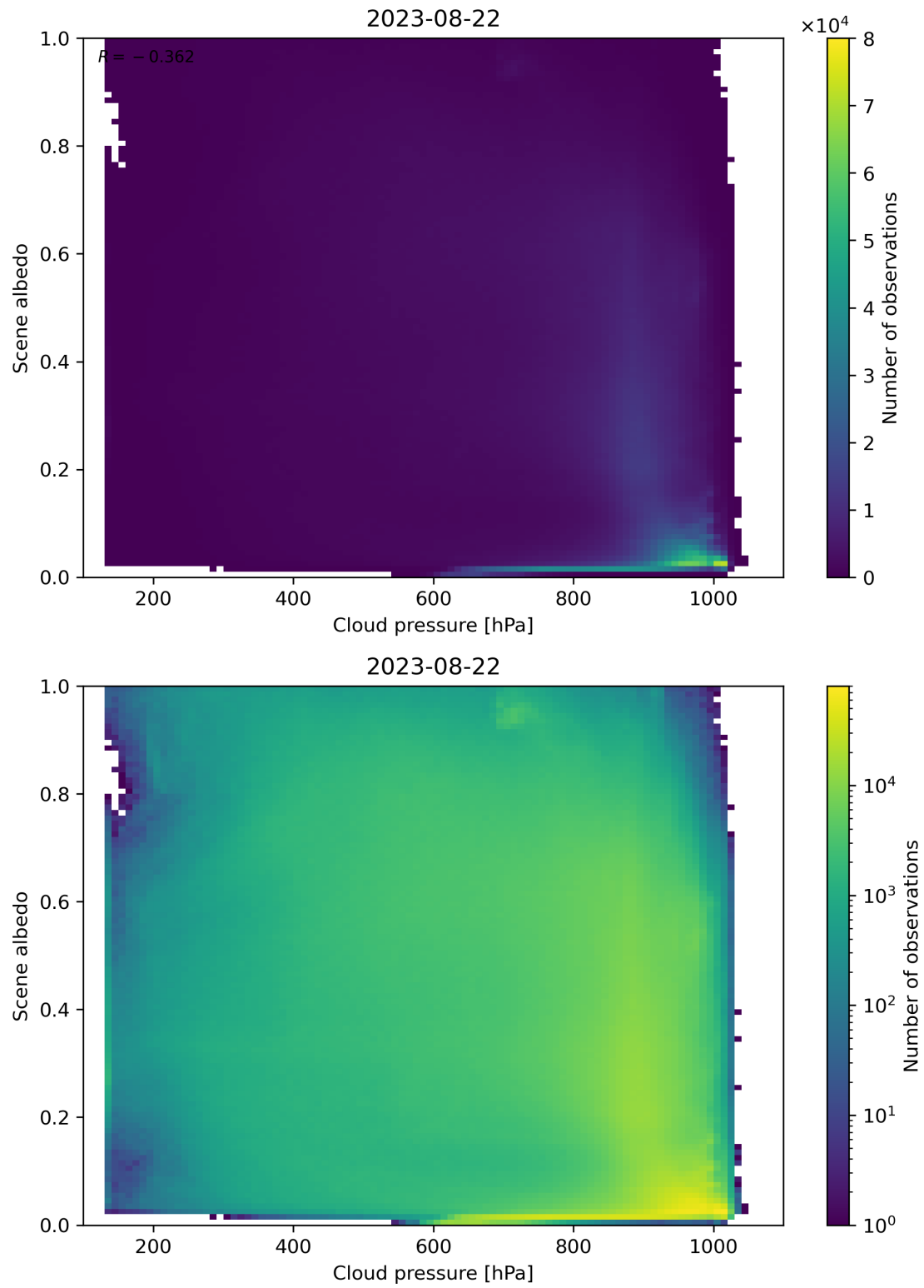
Figure 91: Scatter density plot of “Cloud pressure” against “Scene albedo” for 2023-08-21 to 2023-08-23.
