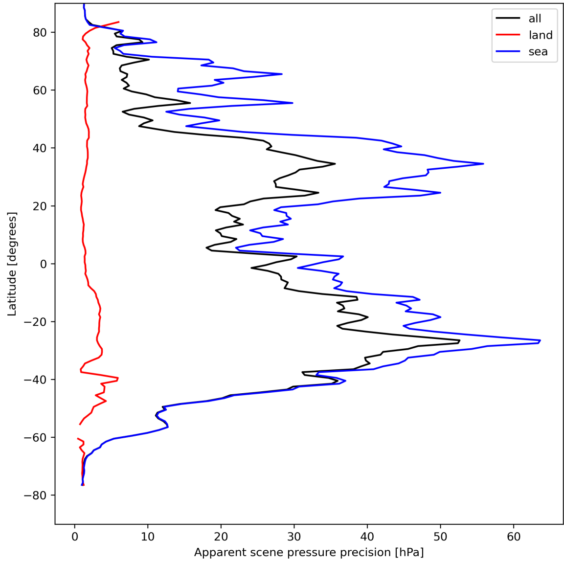
Figure 20: Zonal average of “Apparent scene pressure precision” for 2023-08-21 to 2023-08-23.
