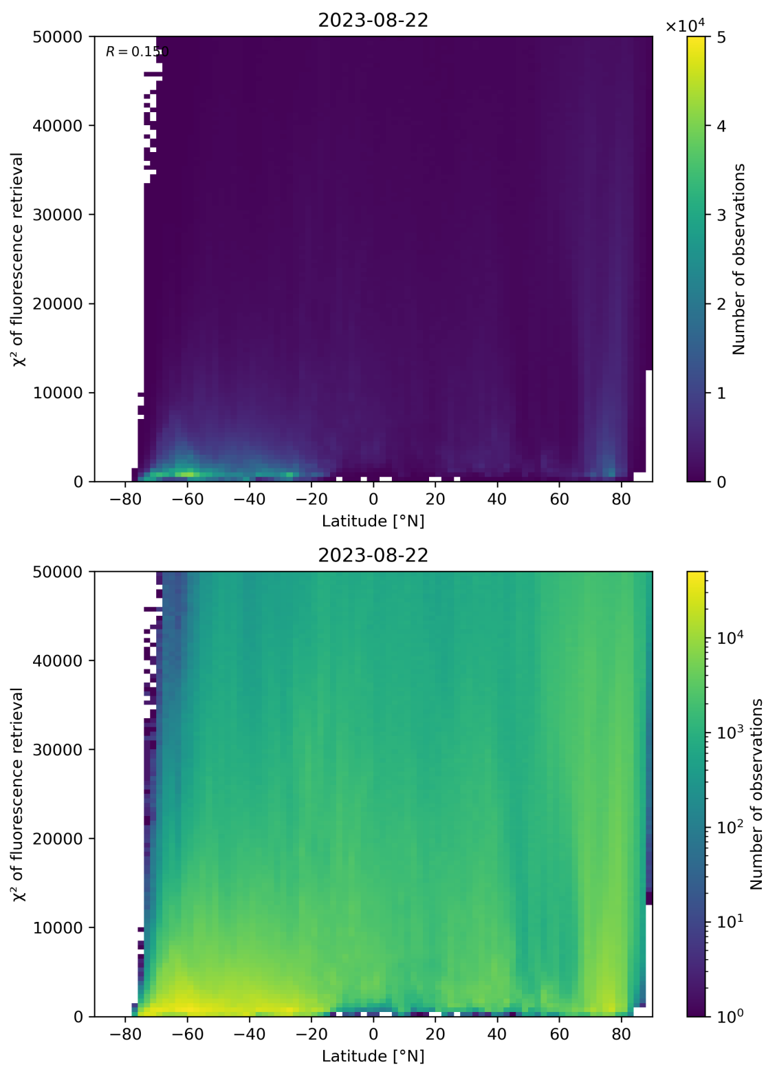
Figure 98: Scatter density plot of “Latitude” against “ \chi^2 of fluorescence retrieval” for 2023-08-21 to 2023-08-23.
