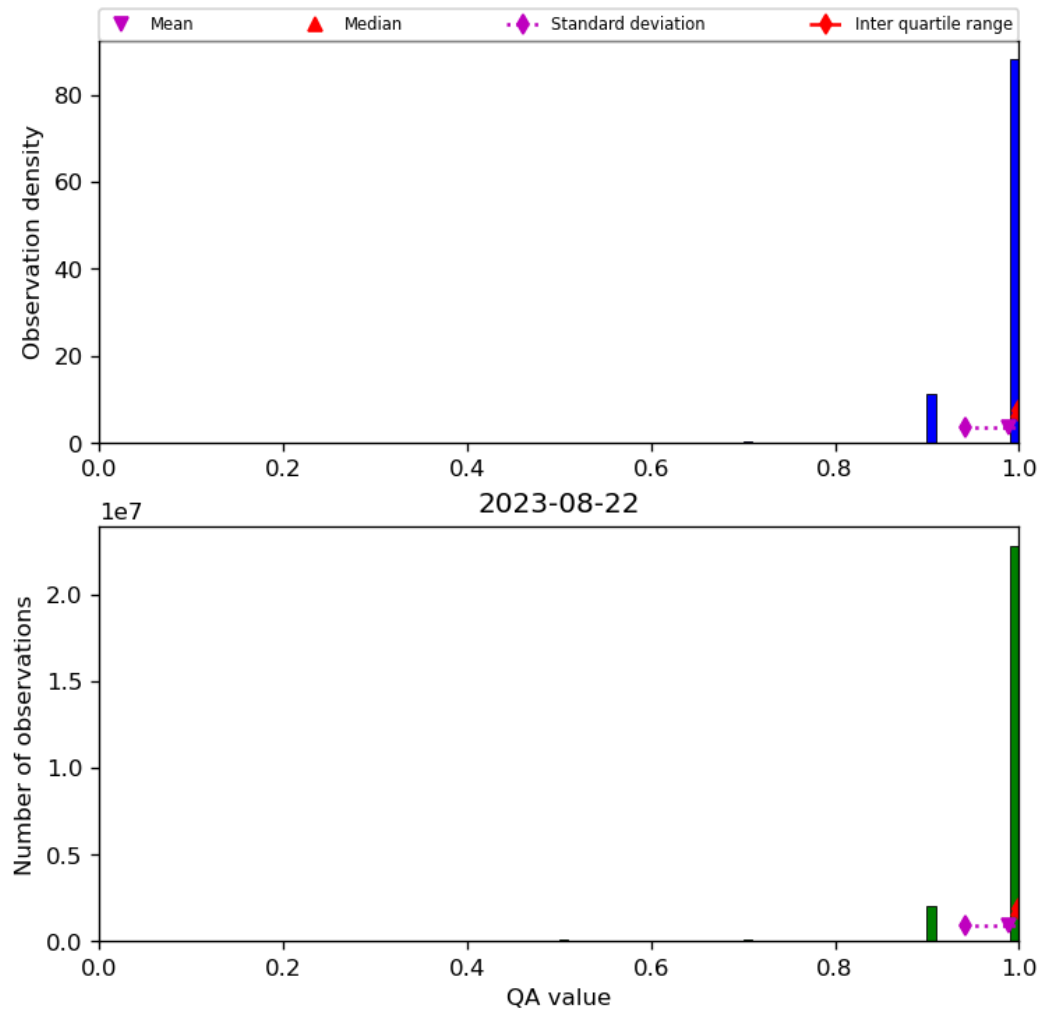
Figure 29: Histogram of “QA value” for 2023-08-21 to 2023-08-23
