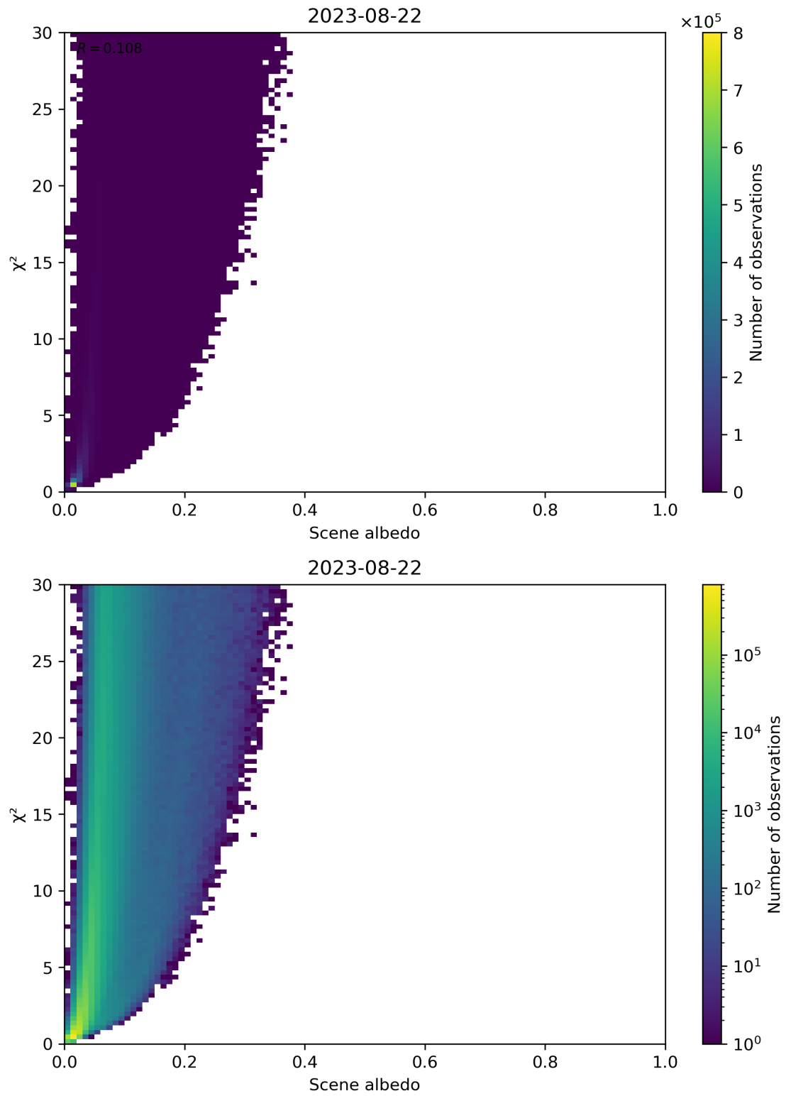
Figure 112: Scatter density plot of “Scene albedo” against “ \chi^2 ” for 2023-08-21 to 2023-08-23.
