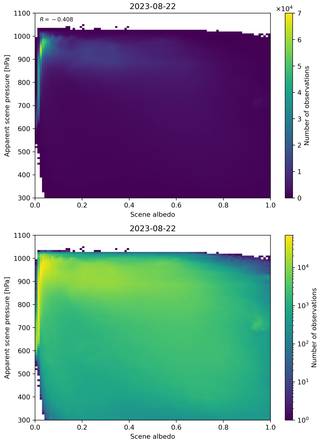
Figure 111: Scatter density plot of “Scene albedo” against “Apparent scene pressure” for 2023-08-21 to 2023-08-23.
