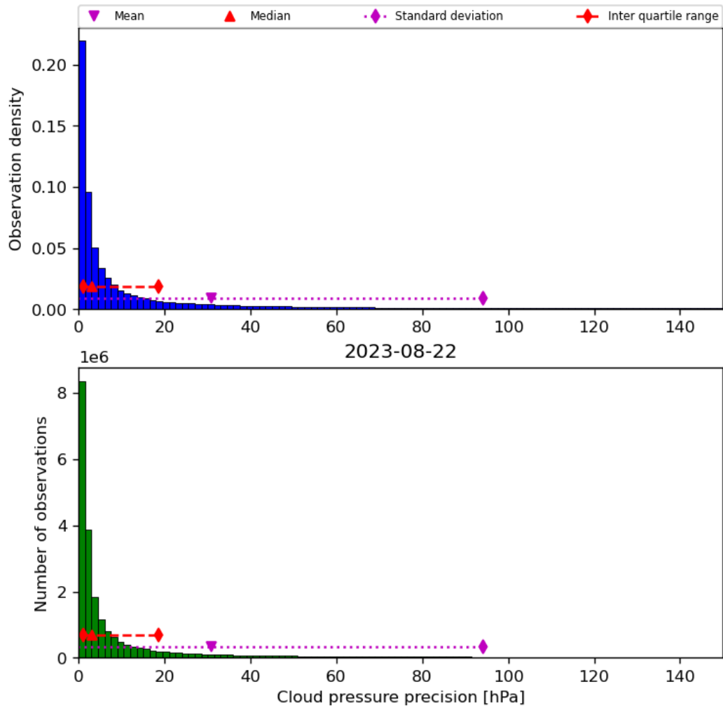
Figure 31: Histogram of “Cloud pressure precision” for 2023-08-21 to 2023-08-23
