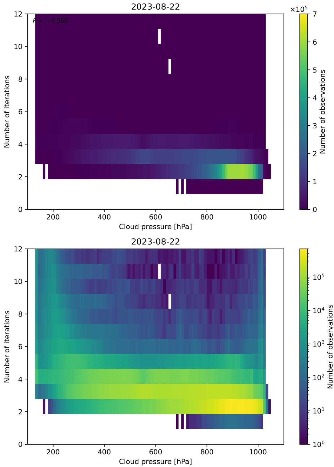
Figure 89: Scatter density plot of “Cloud pressure” against “Number of iterations” for 2023-08-21 to 2023-08-23.
