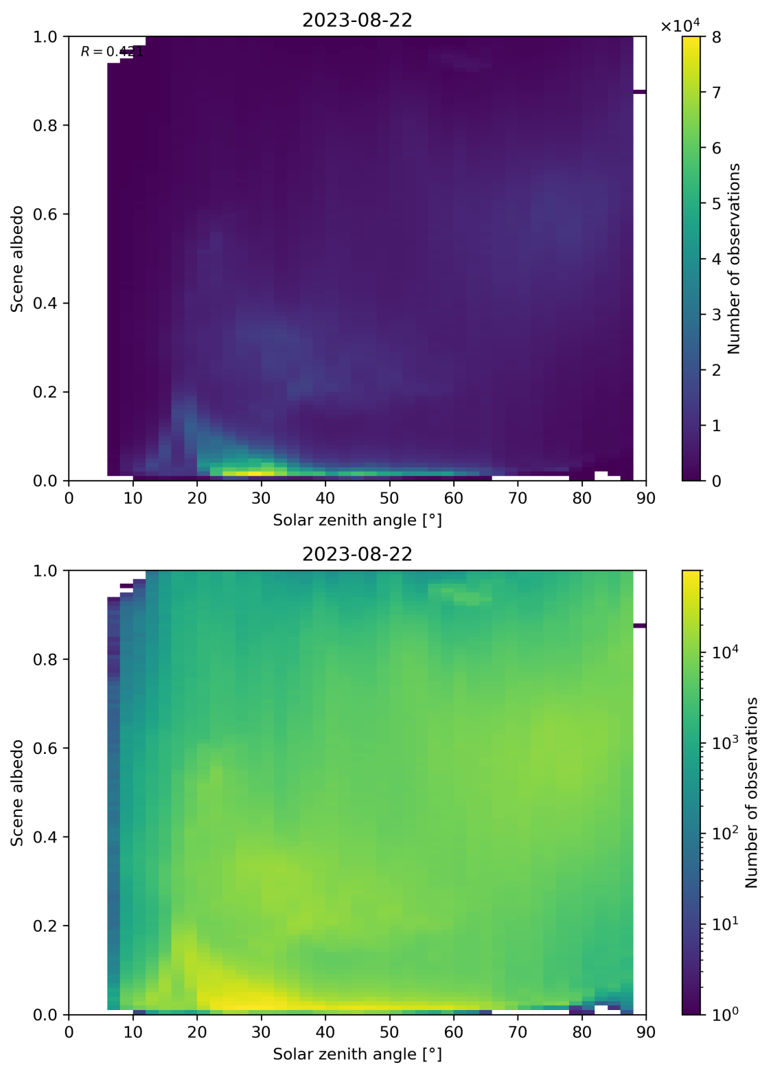
Figure 127: Scatter density plot of “Solar zenith angle” against “Scene albedo” for 2023-08-21 to 2023-08-23.
