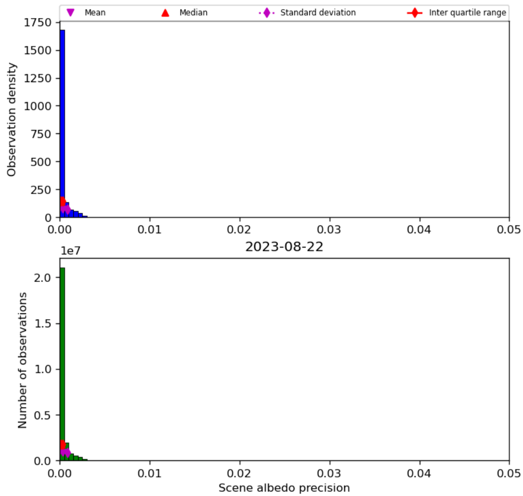
Figure 35: Histogram of “Scene albedo precision” for 2023-08-21 to 2023-08-23
