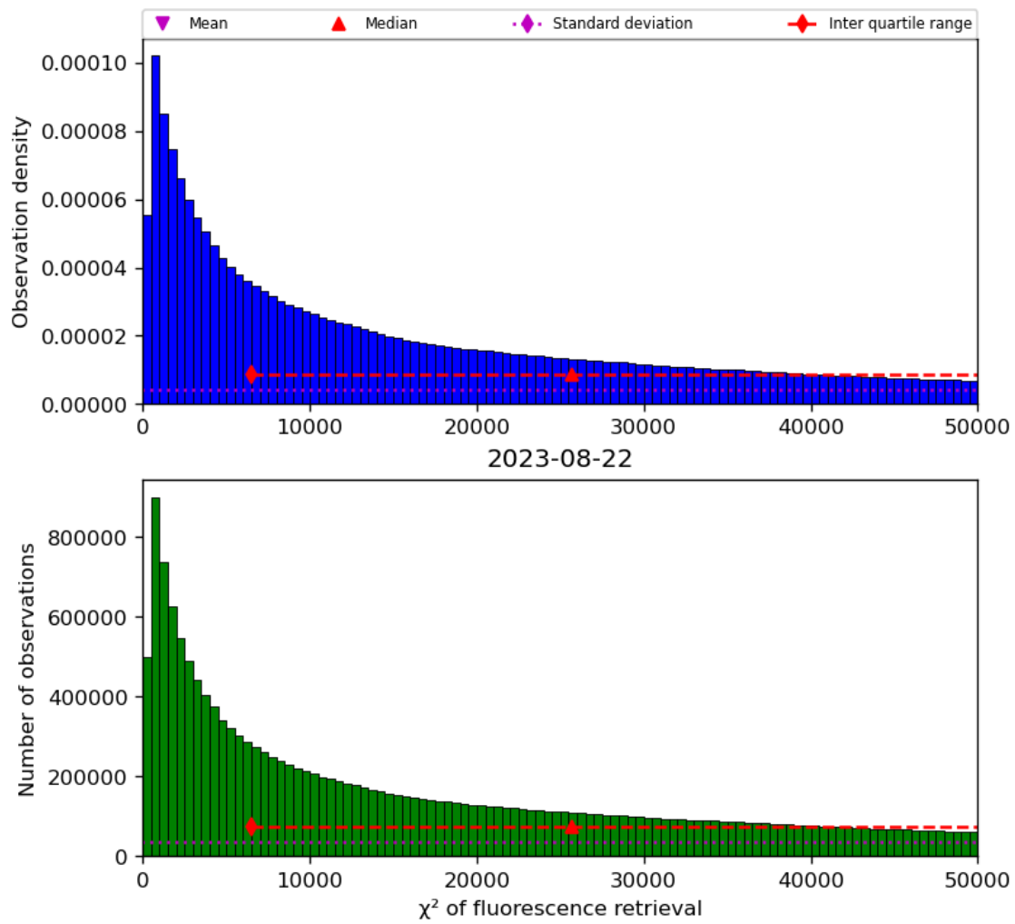
Figure 42: Histogram of “ \chi^2 of fluorescence retrieval” for 2023-08-21 to 2023-08-23
