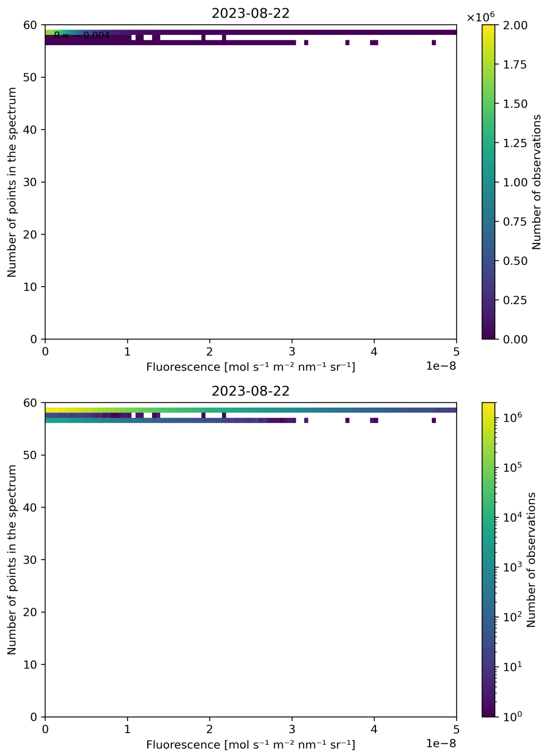
Figure 94: Scatter density plot of “Fluorescence” against “Number of points in the spectrum” for 2023-08-21 to 2023-08-23.
