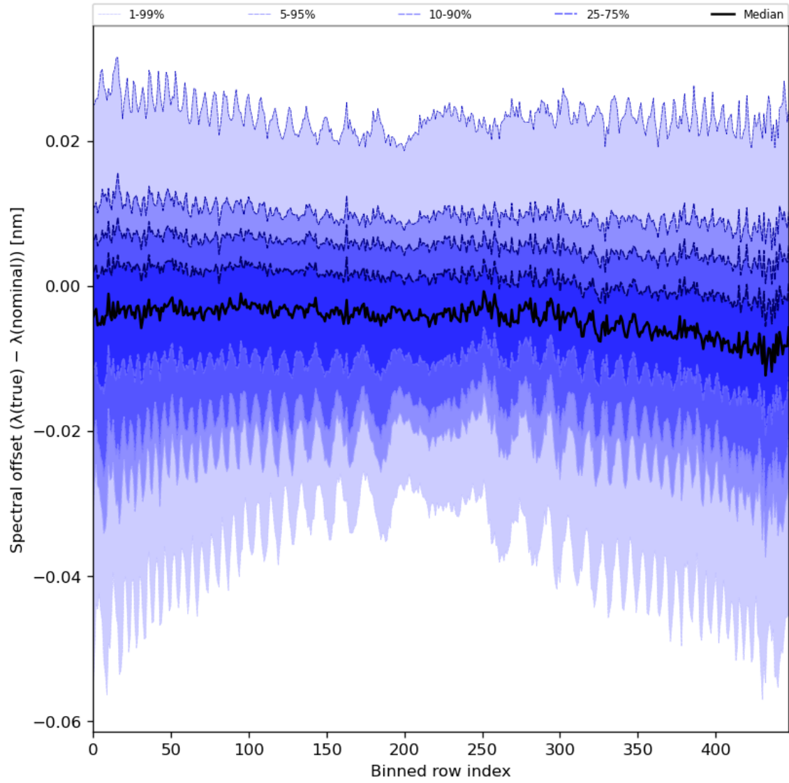
Figure 62: Along track statistics of “Spectral offset ( \lambda(\text{true}) - \lambda(\text{nominal}) )” for 2023-08-21 to 2023-08-23
