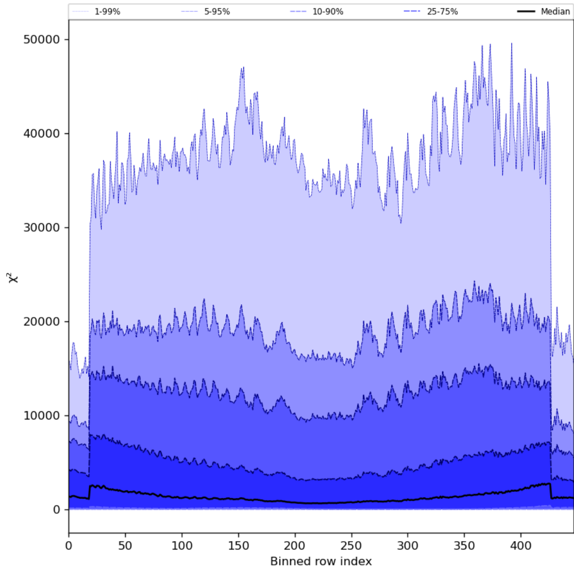
Figure 55: Along track statistics of “ \chi^2 ” for 2023-08-21 to 2023-08-23
