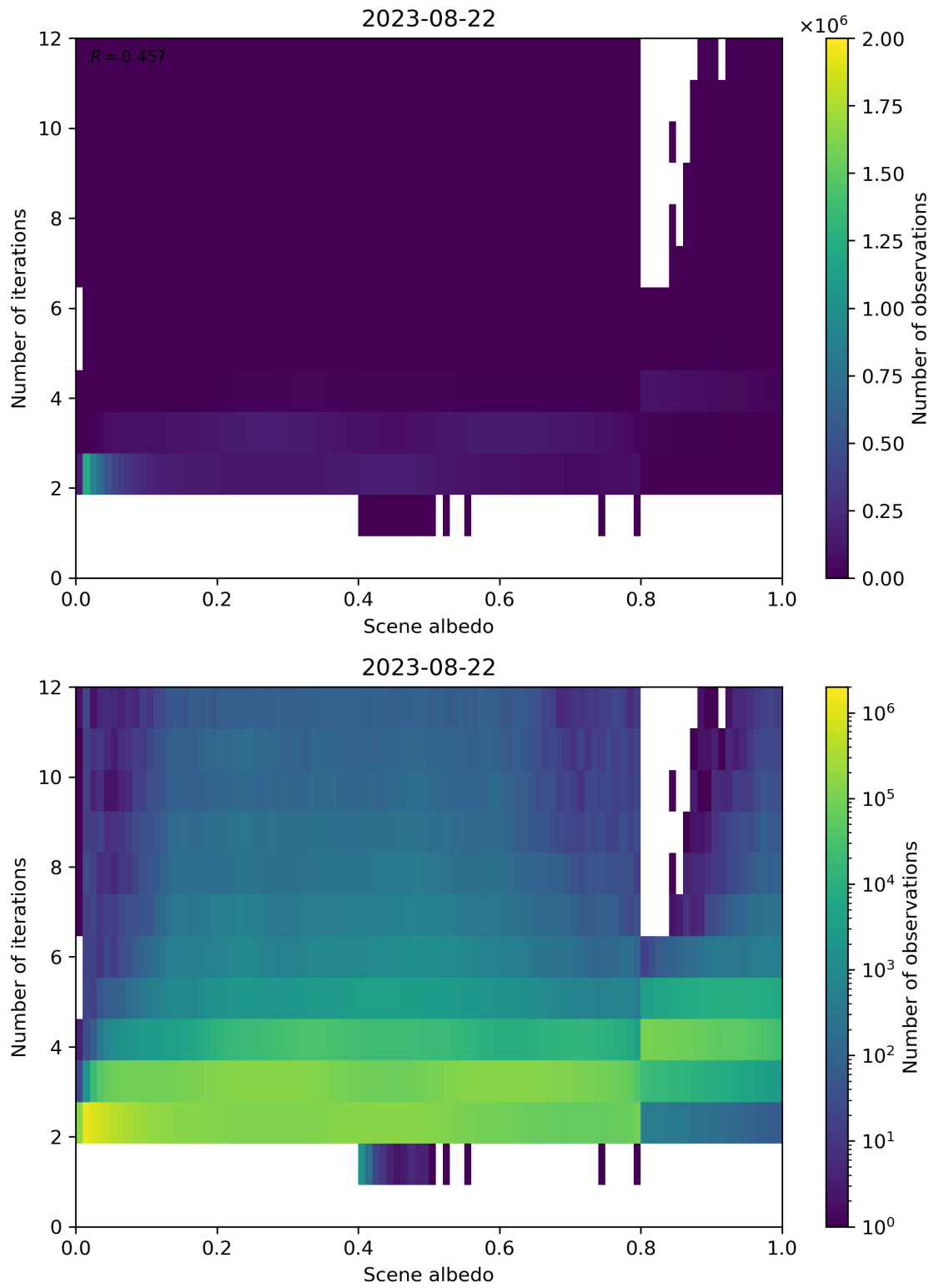
Figure 115: Scatter density plot of “Scene albedo” against “Number of iterations” for 2023-08-21 to 2023-08-23.
