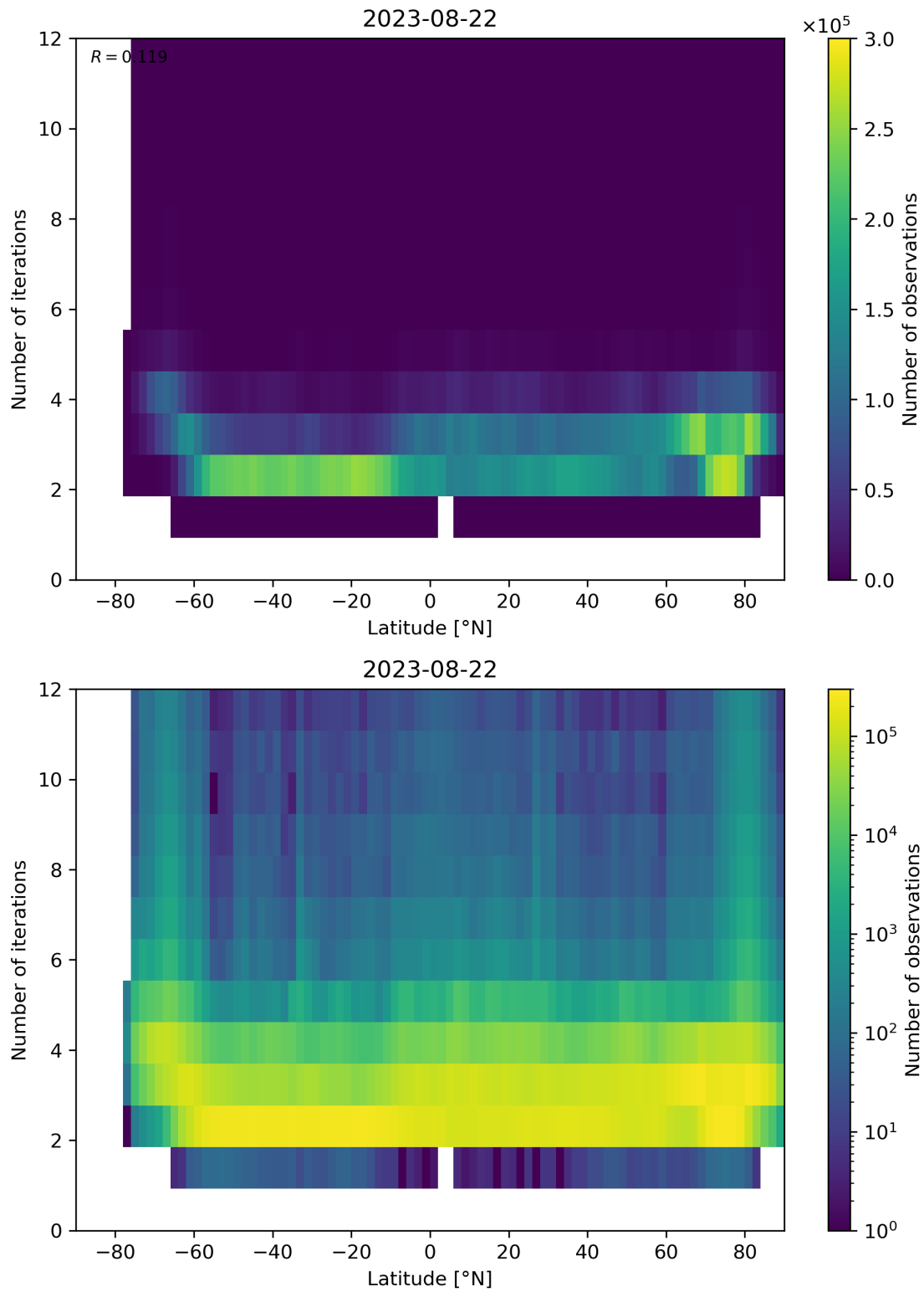
Figure 102: Scatter density plot of “Latitude” against “Number of iterations” for 2023-08-21 to 2023-08-23.
