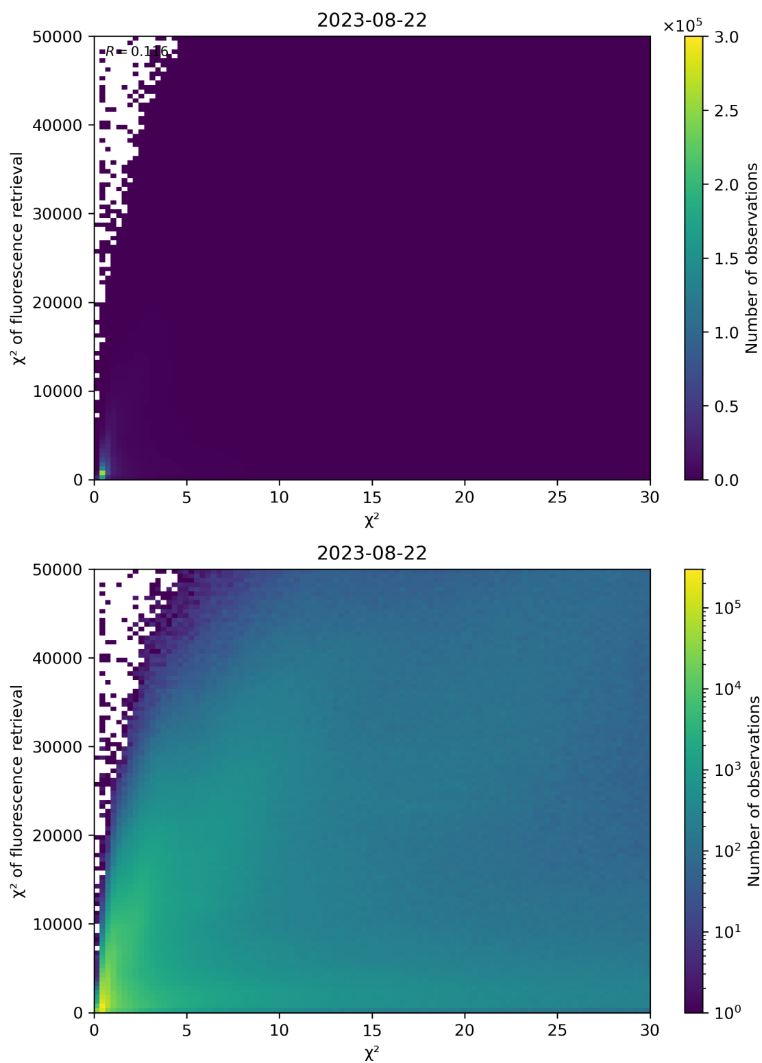
Figure 69: Scatter density plot of “ \chi^2 ” against “ \chi^2 of fluorescence retrieval” for 2023-08-21 to 2023-08-23.
