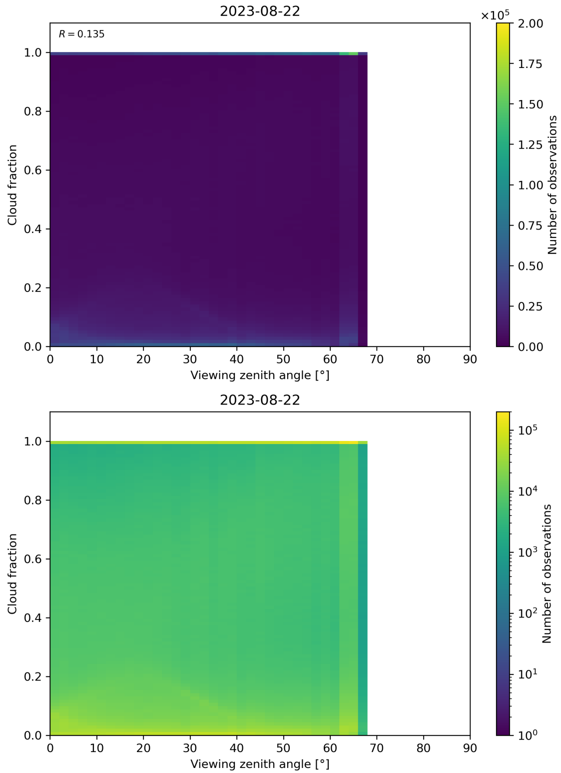
Figure 132: Scatter density plot of “Viewing zenith angle” against “Cloud fraction” for 2023-08-21 to 2023-08-23.
