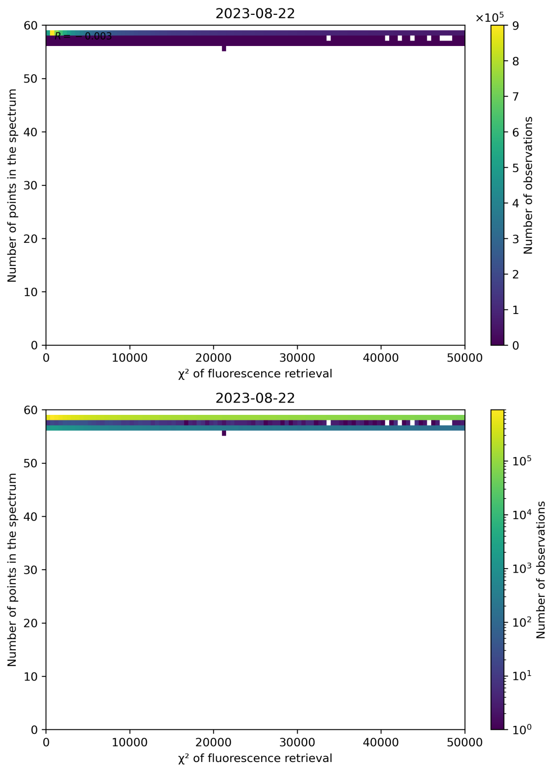
Figure 71: Scatter density plot of " \chi^2 of fluorescence retrieval" against "Number of points in the spectrum" for 2023-08-21 to 2023-08-23.
