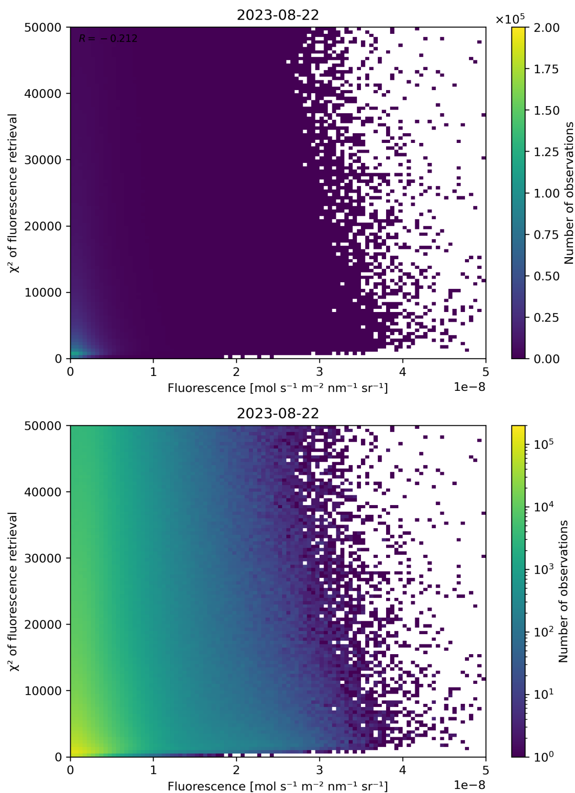
Figure 93: Scatter density plot of “Fluorescence” against “ \chi^2 of fluorescence retrieval” for 2023-08-21 to 2023-08-23.
