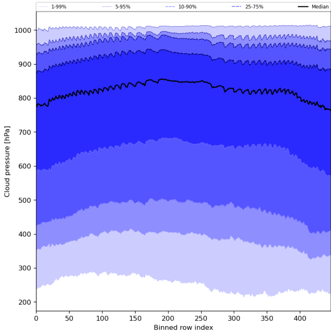
Figure 47: Along track statistics of “Cloud pressure” for 2023-08-21 to 2023-08-23
