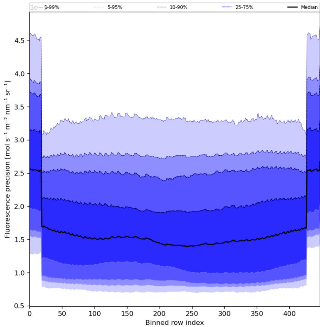
Figure 58: Along track statistics of “Fluorescence precision” for 2023-08-21 to 2023-08-23
