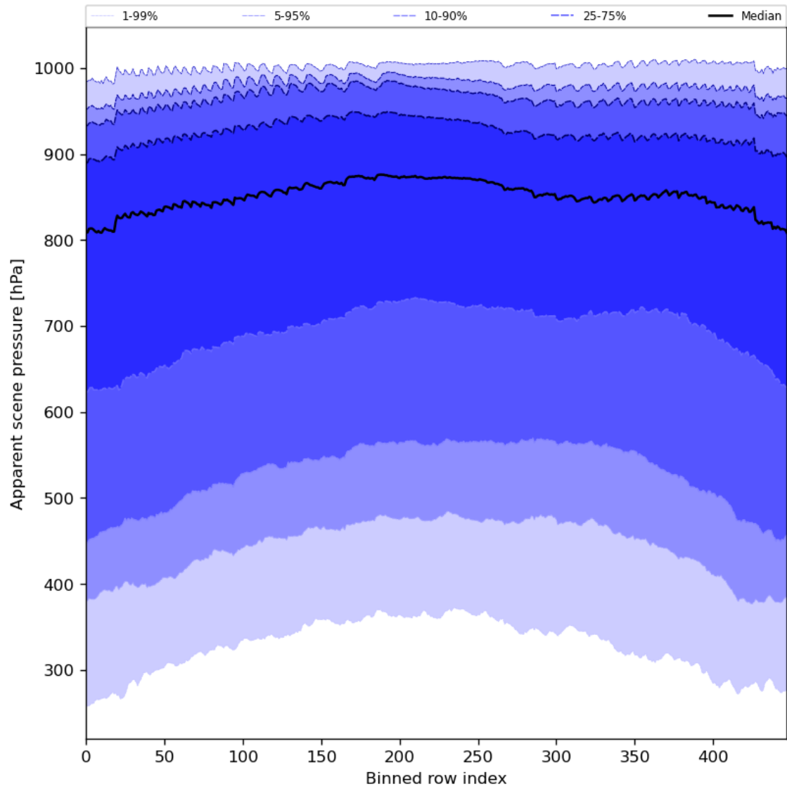
Figure 53: Along track statistics of “Apparent scene pressure” for 2023-08-21 to 2023-08-23
