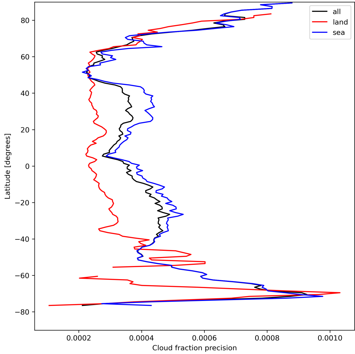
Figure 16: Zonal average of “Cloud fraction precision” for 2023-08-22 to 2023-08-24.
