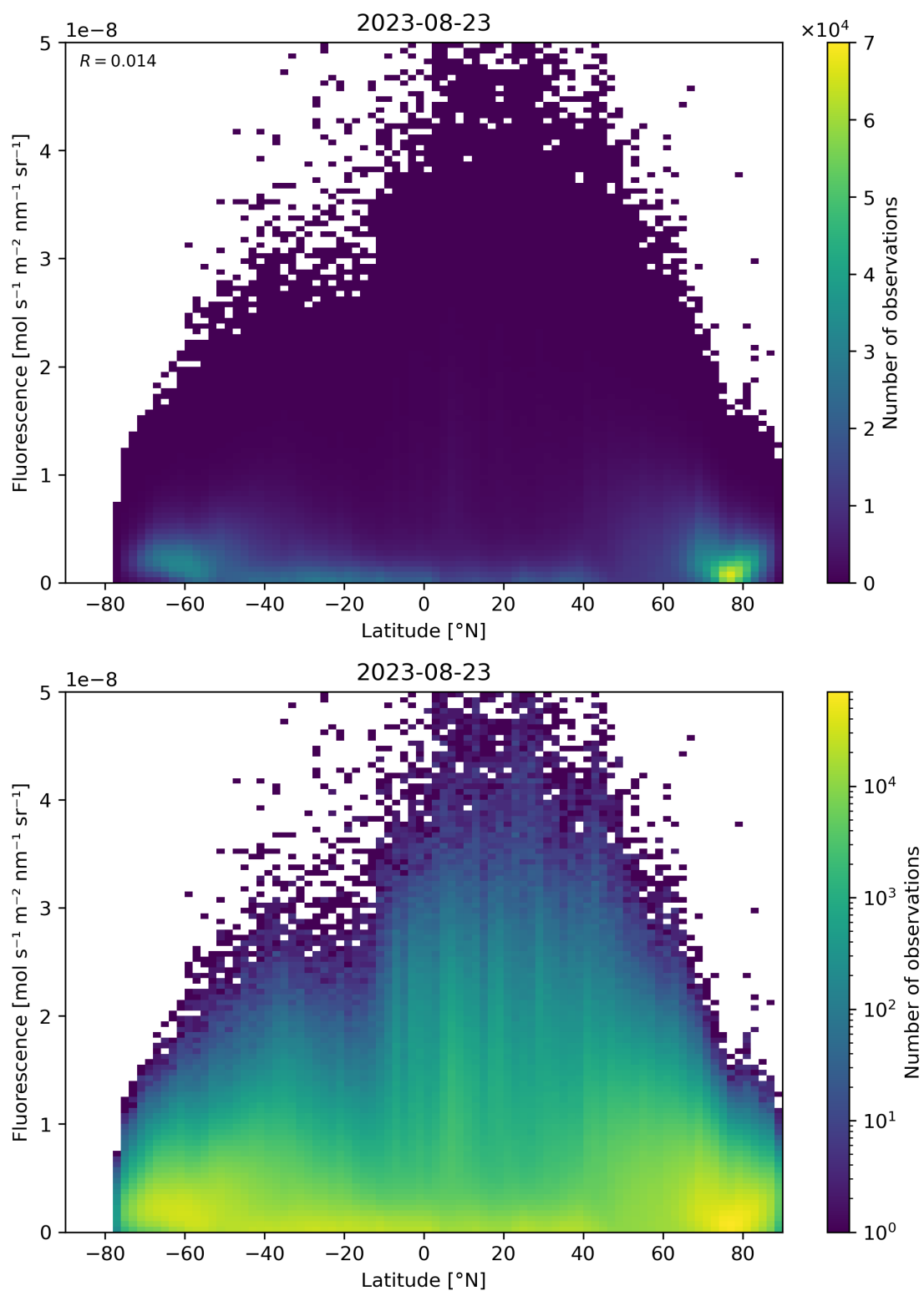
Figure 101: Scatter density plot of “Latitude” against “Fluorescence” for 2023-08-22 to 2023-08-24.
