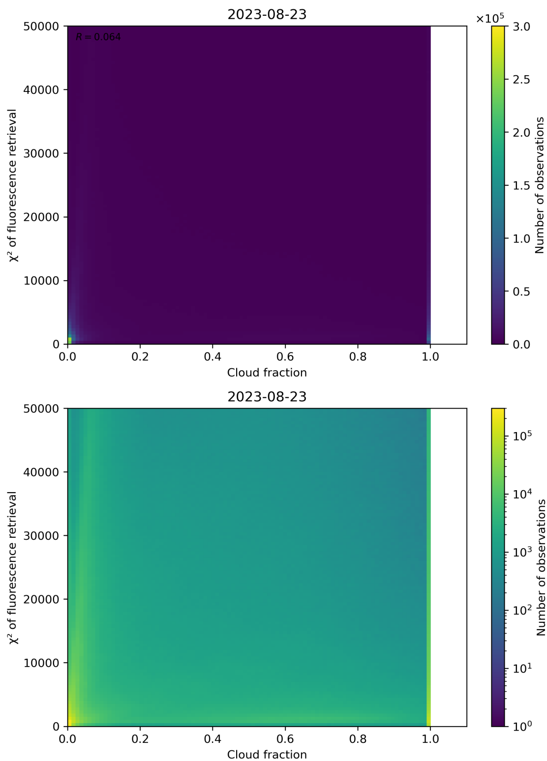
Figure 78: Scatter density plot of “Cloud fraction” against “ \chi^2 of fluorescence retrieval” for 2023-08-22 to 2023-08-24.
