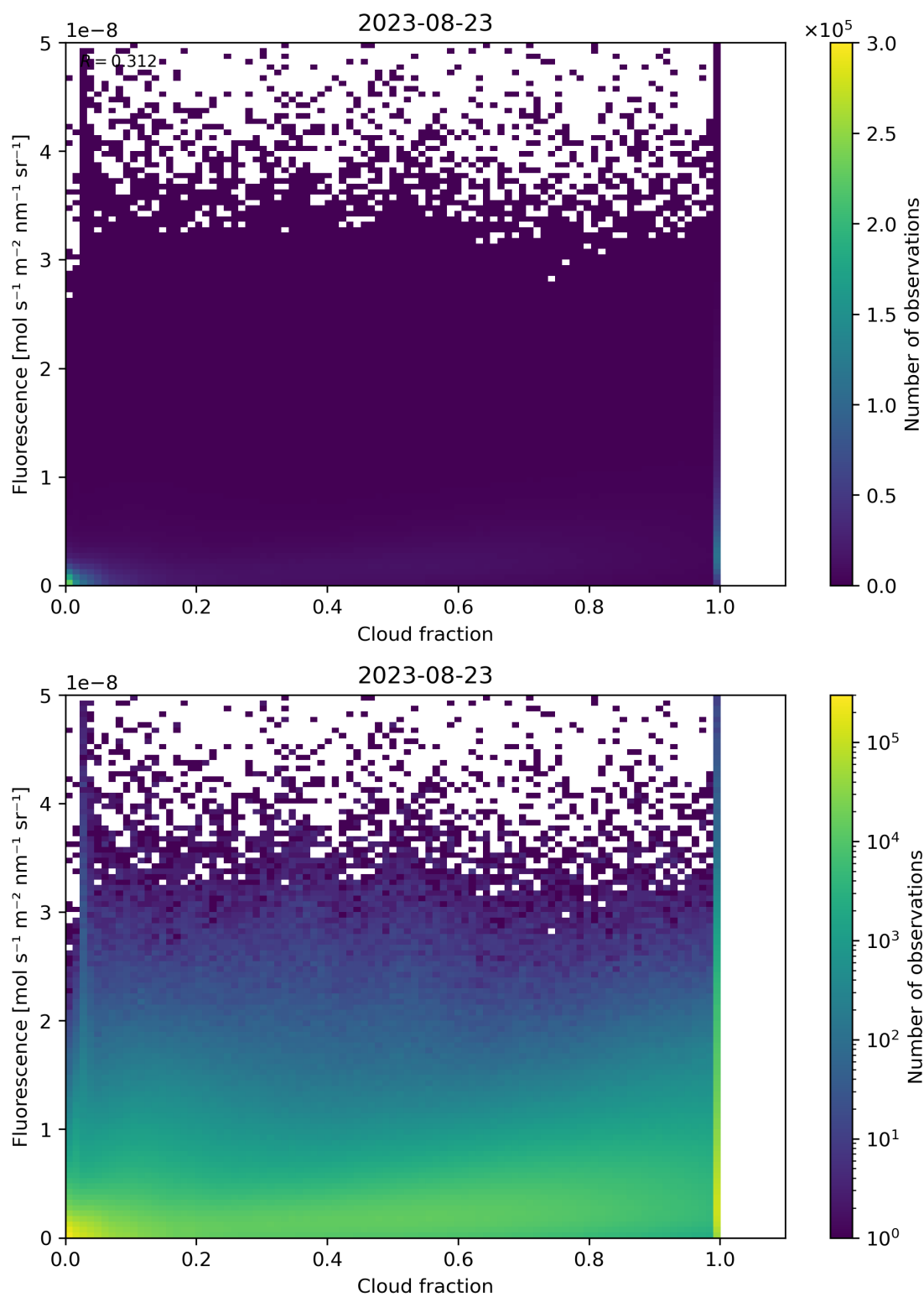
Figure 79: Scatter density plot of “Cloud fraction” against “Fluorescence” for 2023-08-22 to 2023-08-24.
