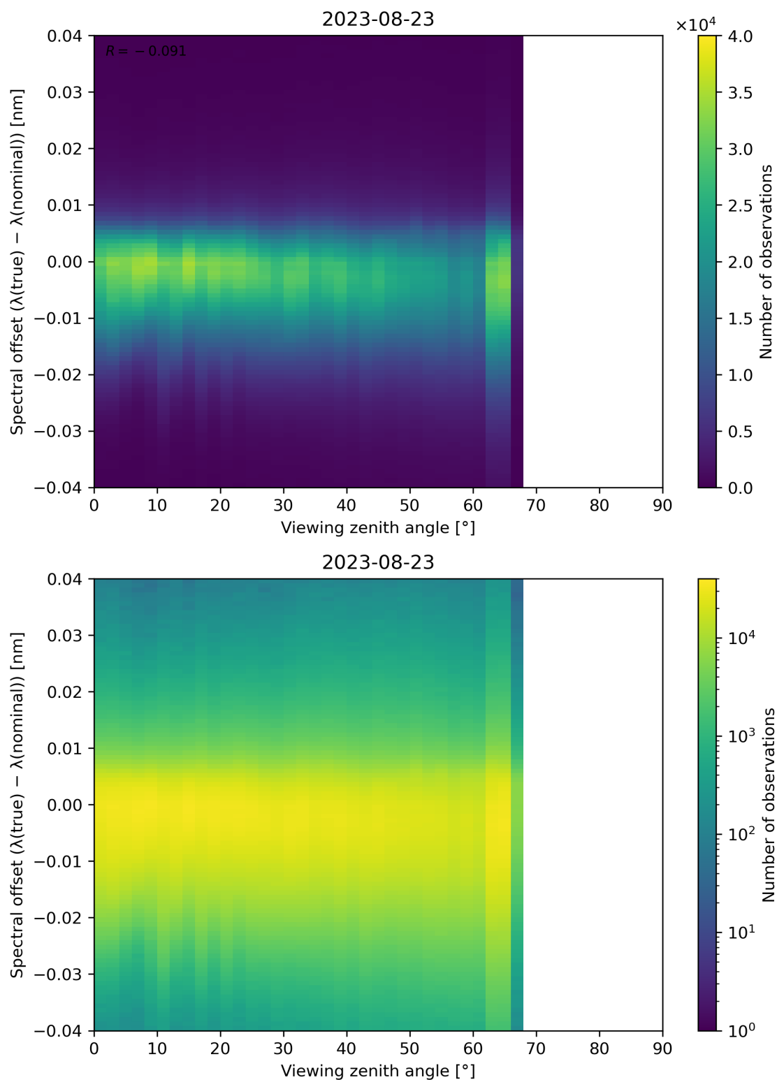
Figure 140: Scatter density plot of “Viewing zenith angle” against “Spectral offset ( \lambda(\text{true}) - \lambda(\text{nominal}) )” for 2023-08-22 to 2023-08-24.
