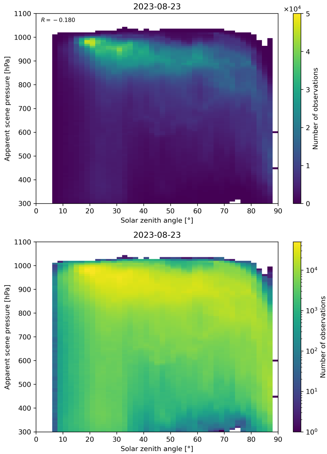
Figure 118: Scatter density plot of “Solar zenith angle” against “Apparent scene pressure” for 2023-08-22 to 2023-08-24.
