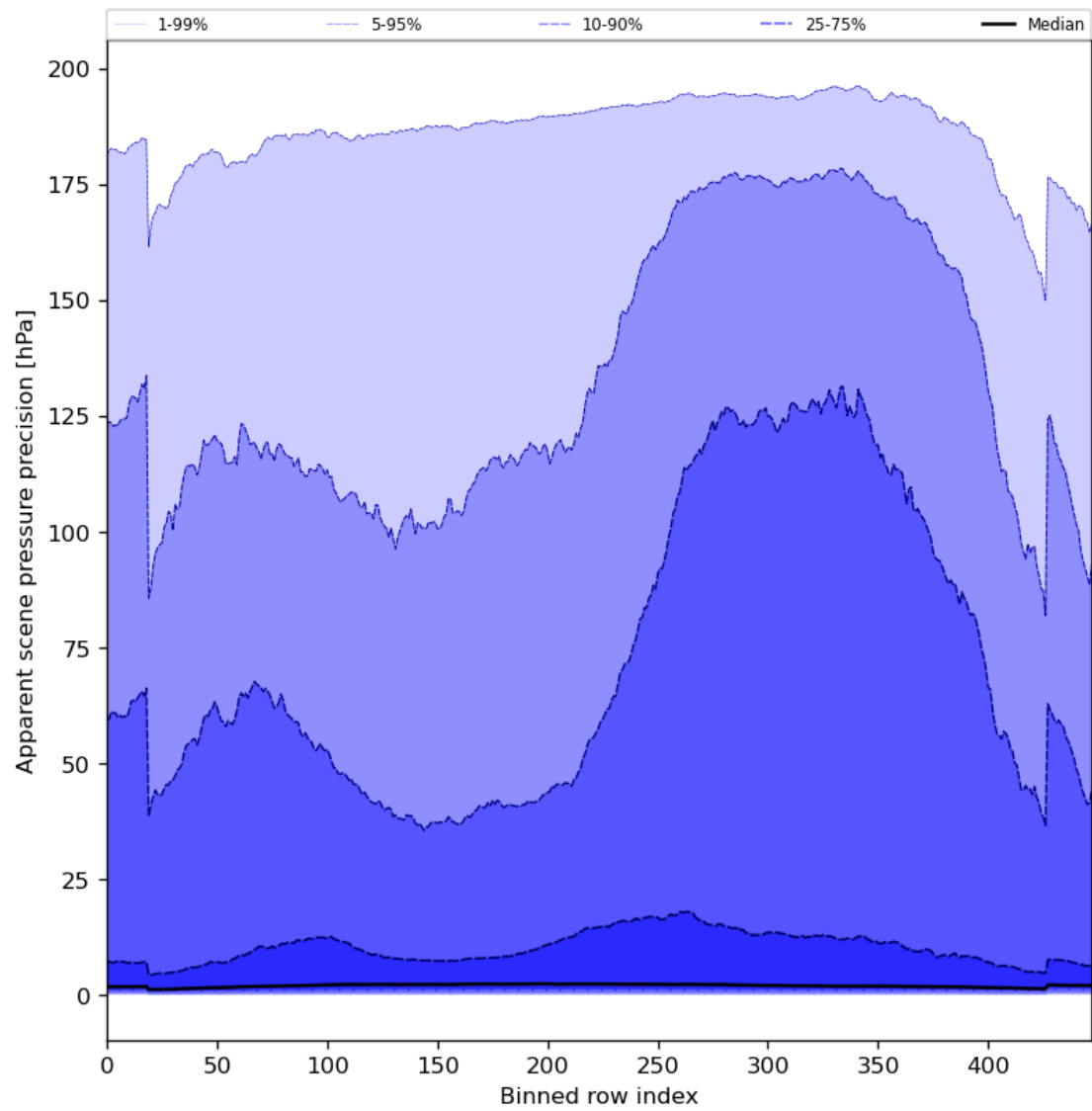
Figure 54: Along track statistics of “Apparent scene pressure precision” for 2023-08-22 to 2023-08-24
