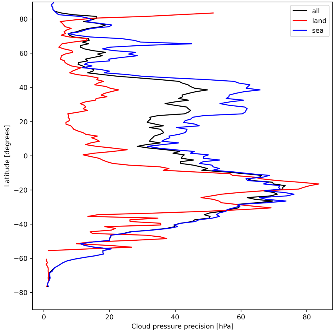
Figure 14: Zonal average of “Cloud pressure precision” for 2023-08-22 to 2023-08-24.
