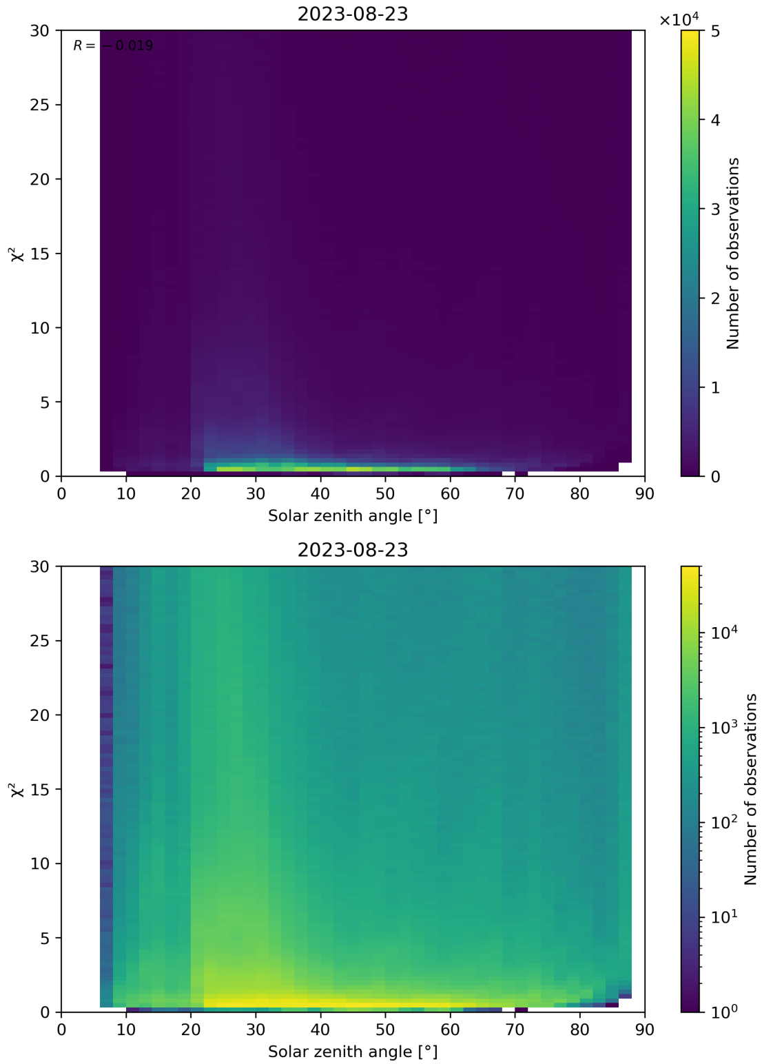
Figure 119: Scatter density plot of “Solar zenith angle” against “ \chi^2 ” for 2023-08-22 to 2023-08-24.
