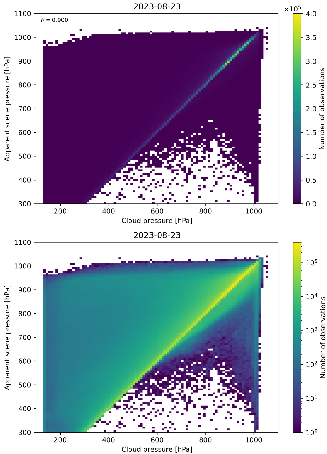
Figure 84: Scatter density plot of “Cloud pressure” against “Apparent scene pressure” for 2023-08-22 to 2023-08-24.
