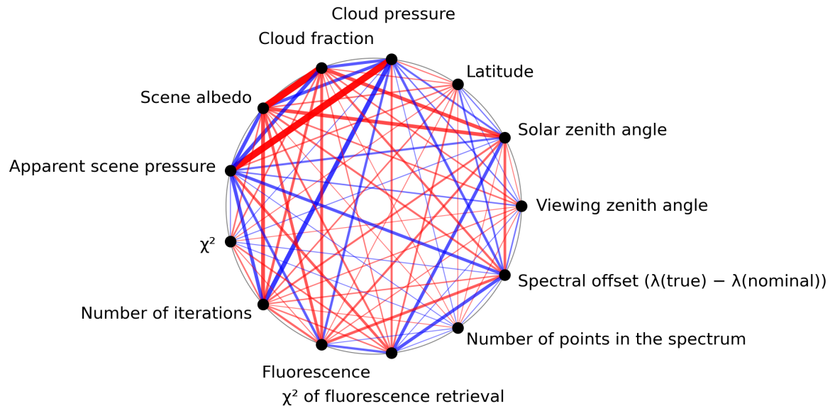
Figure 1: Map of correlation graph for 2023-08-22 to 2023-08-24.
