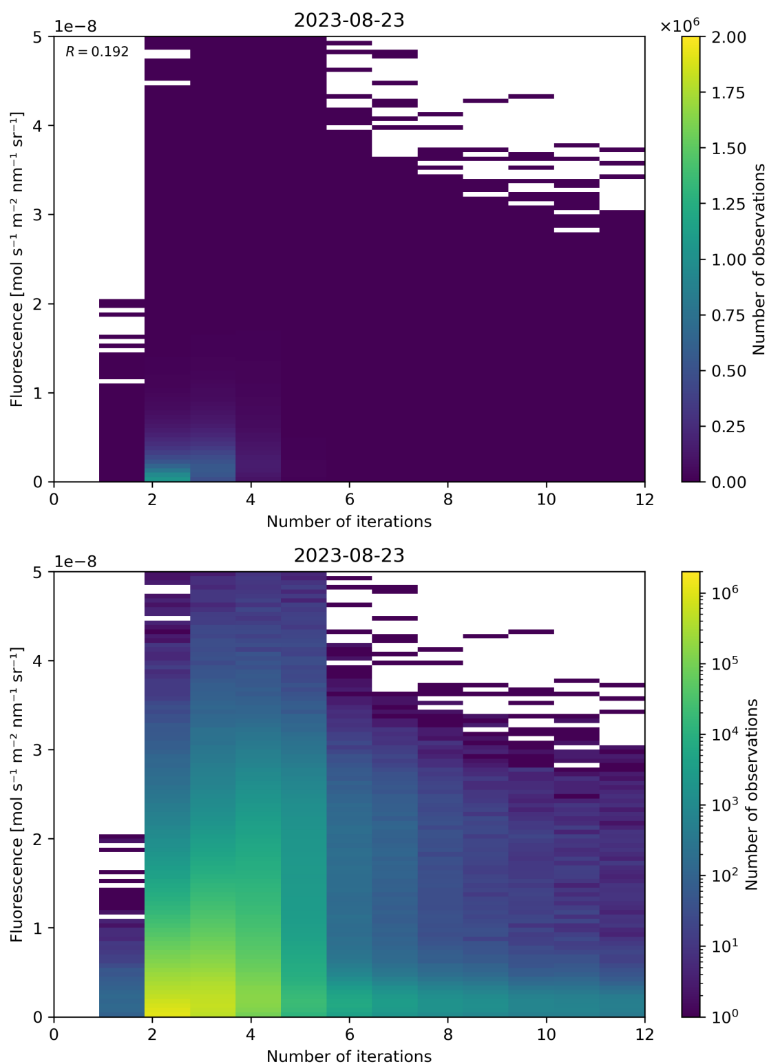
Figure 107: Scatter density plot of “Number of iterations” against “Fluorescence” for 2023-08-22 to 2023-08-24.
