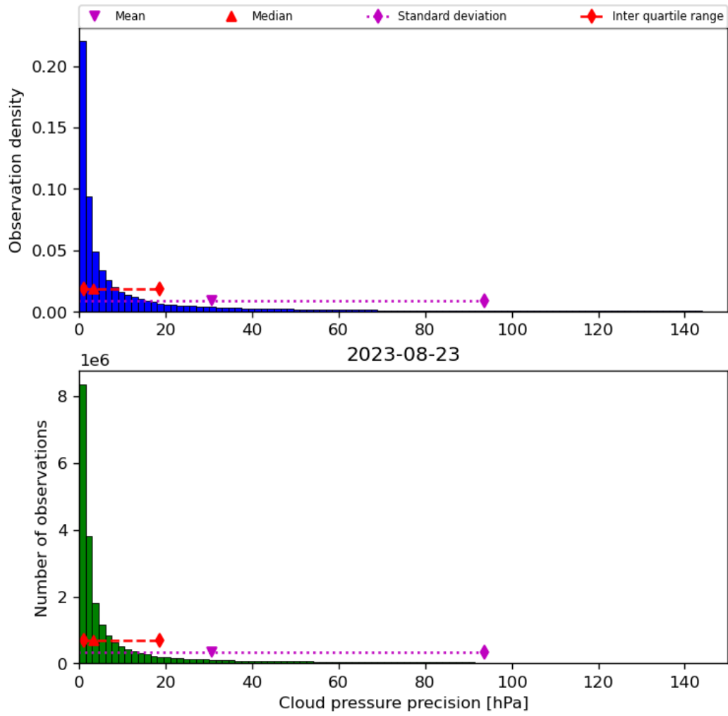
Figure 31: Histogram of “Cloud pressure precision” for 2023-08-22 to 2023-08-24
