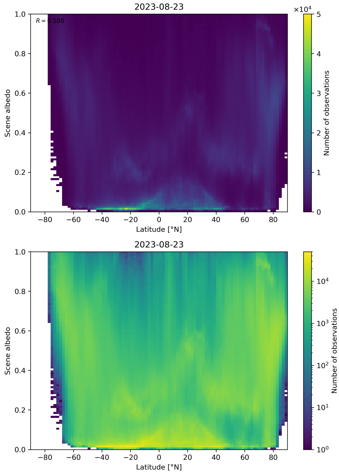
Figure 104: Scatter density plot of “Latitude” against “Scene albedo” for 2023-08-22 to 2023-08-24.
