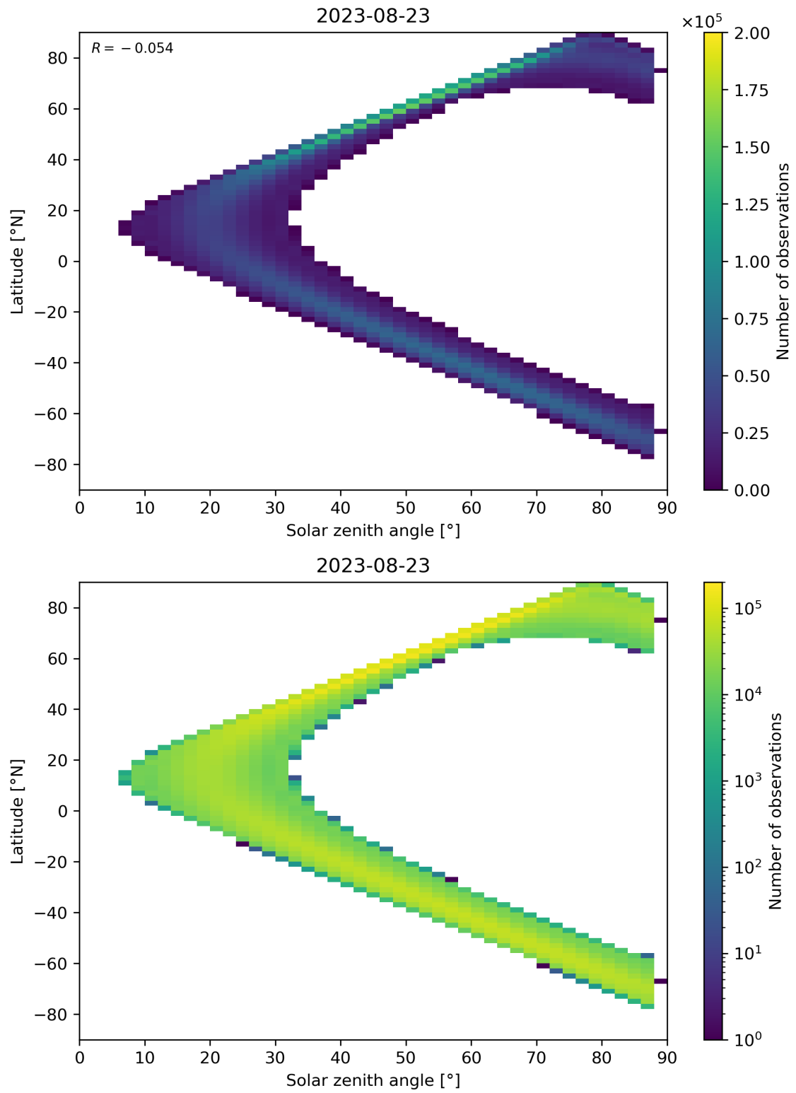
Figure 124: Scatter density plot of “Solar zenith angle” against “Latitude” for 2023-08-22 to 2023-08-24.
