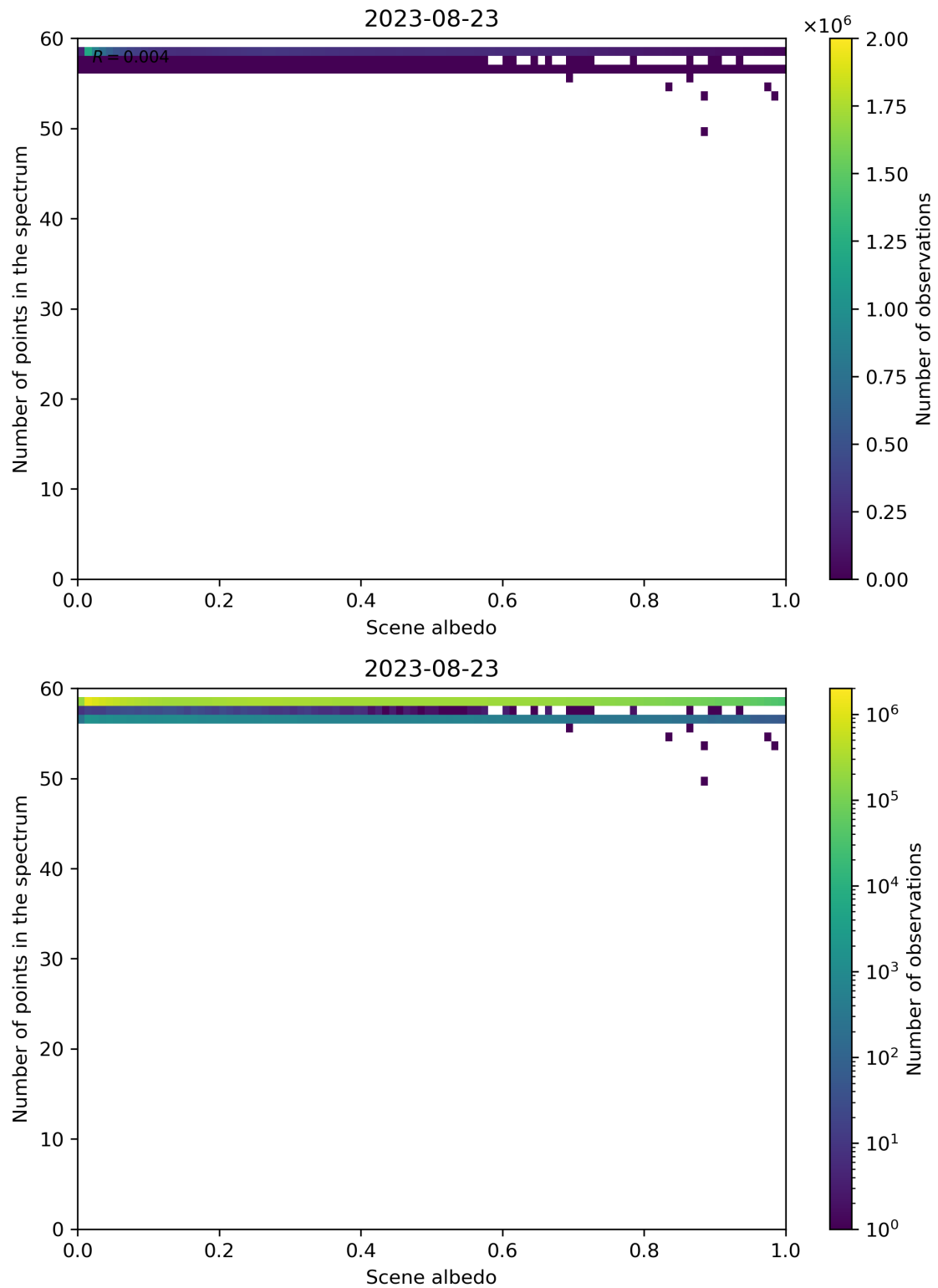
Figure 116: Scatter density plot of “Scene albedo” against “Number of points in the spectrum” for 2023-08-22 to 2023-08-24.
