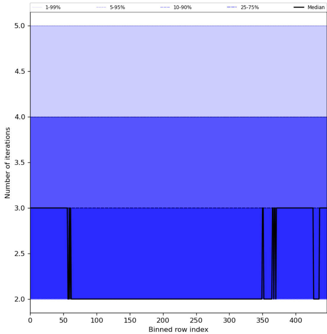
Figure 56: Along track statistics of “Number of iterations” for 2023-08-22 to 2023-08-24
