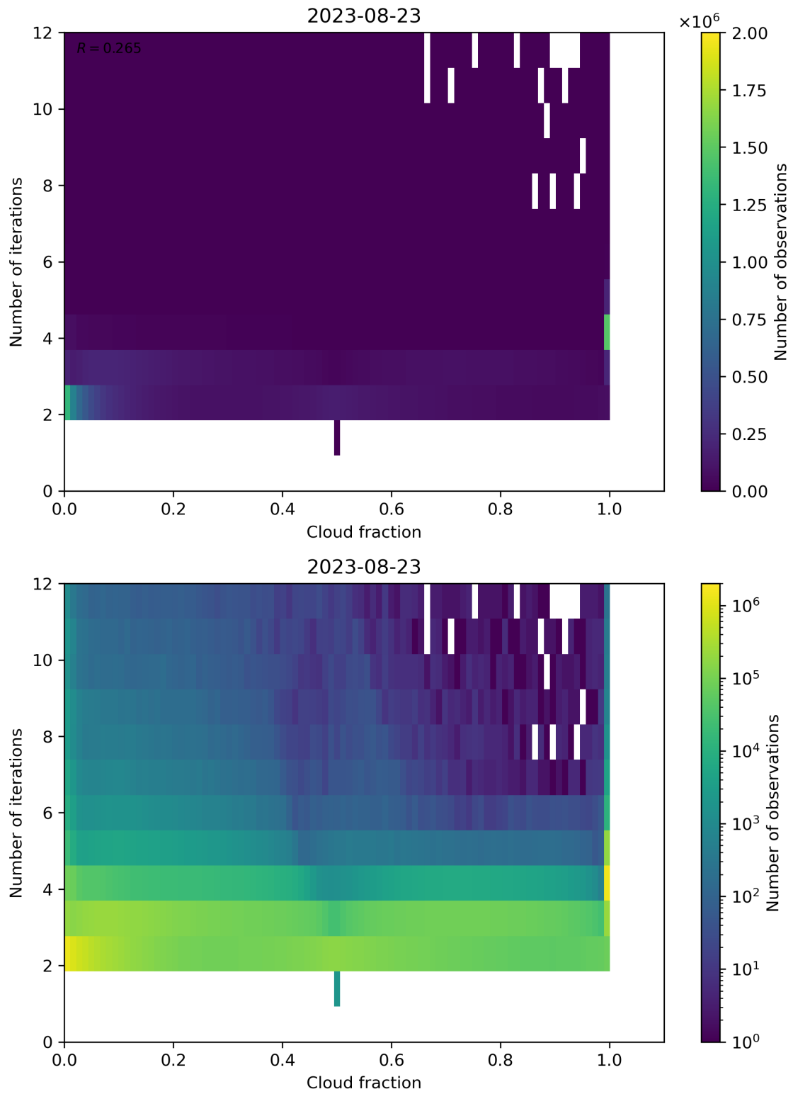
Figure 80: Scatter density plot of “Cloud fraction” against “Number of iterations” for 2023-08-22 to 2023-08-24.
