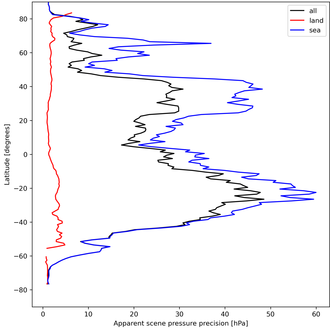
Figure 20: Zonal average of “Apparent scene pressure precision” for 2023-08-22 to 2023-08-24.
