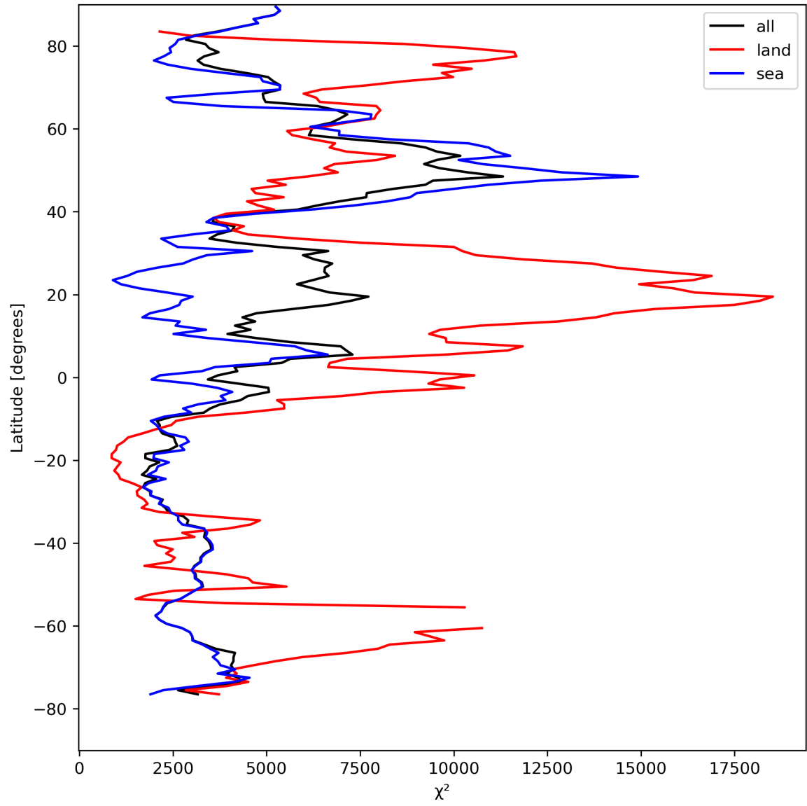
Figure 21: Zonal average of “ \chi^2 ” for 2023-08-22 to 2023-08-24.
