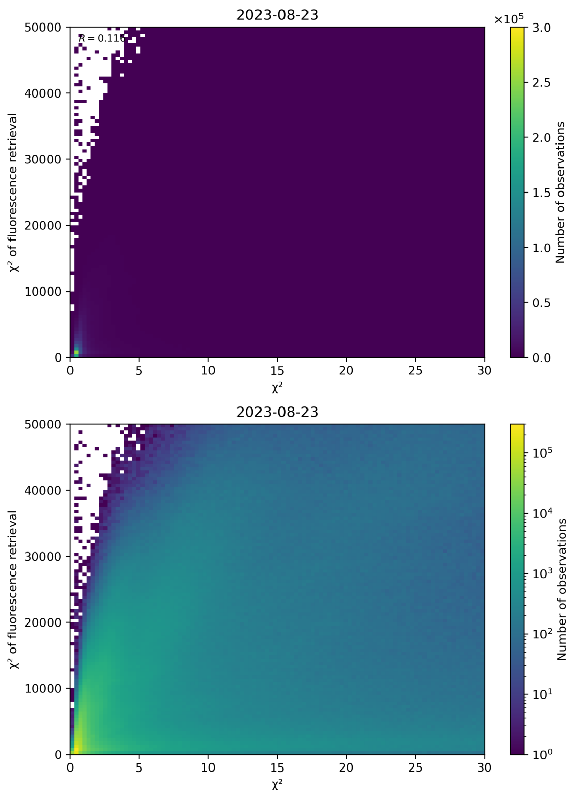
Figure 69: Scatter density plot of “ \chi^2 ” against “ \chi^2 of fluorescence retrieval” for 2023-08-22 to 2023-08-24.
