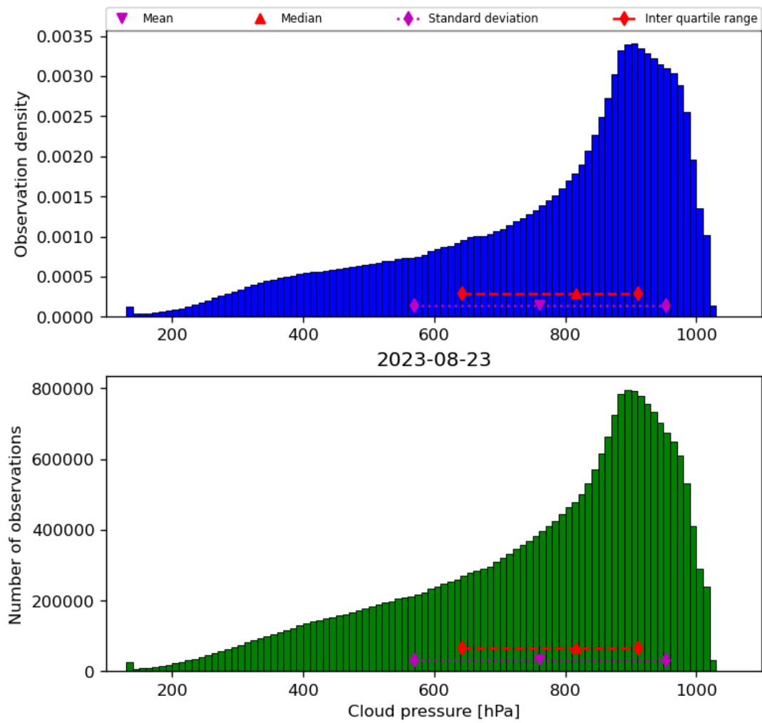
Figure 30: Histogram of “Cloud pressure” for 2023-08-22 to 2023-08-24
