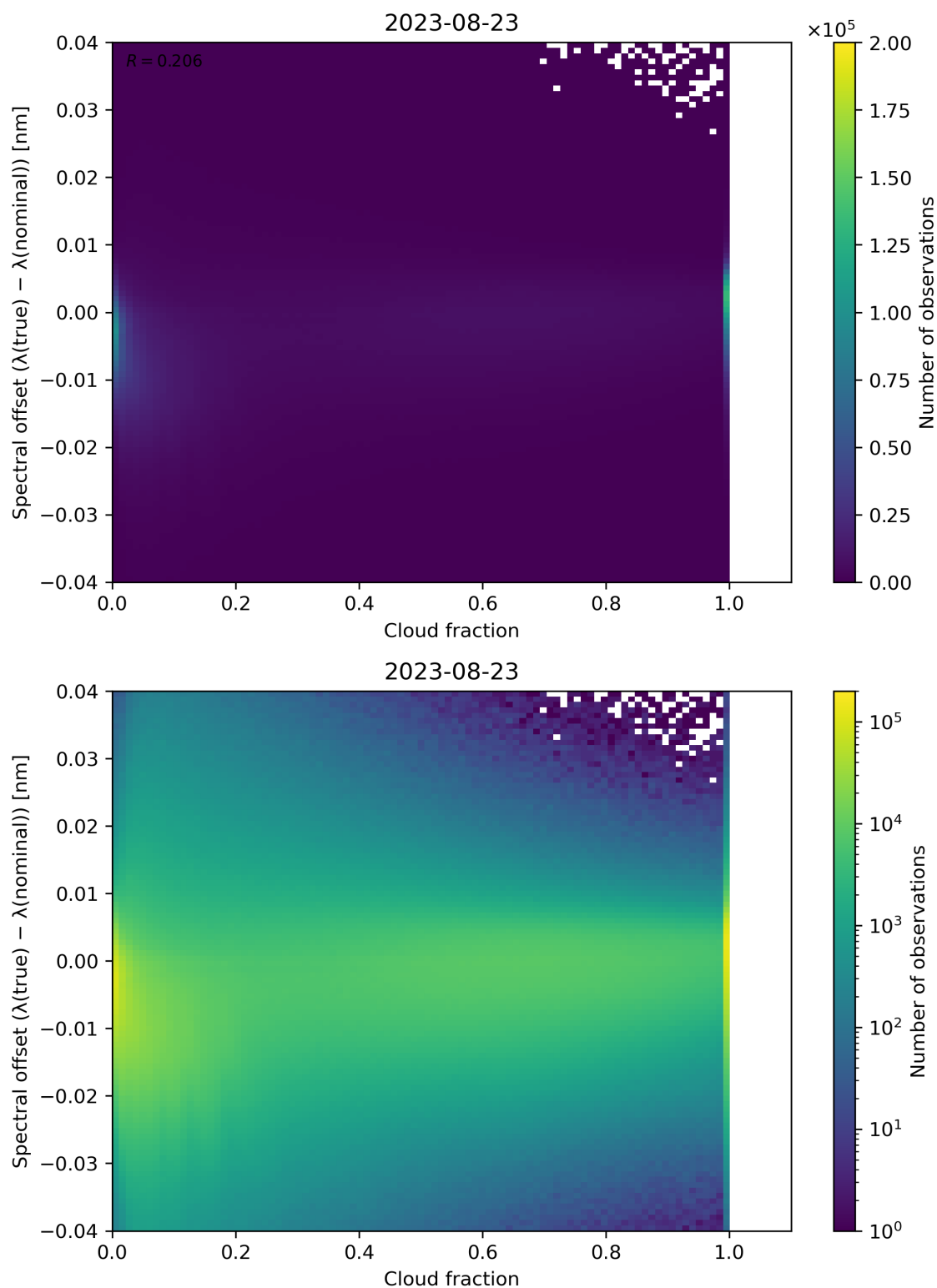
Figure 83: Scatter density plot of “Cloud fraction” against “Spectral offset ( \lambda(\text{true}) - \lambda(\text{nominal}) )” for 2023-08-22 to 2023-08-24.
