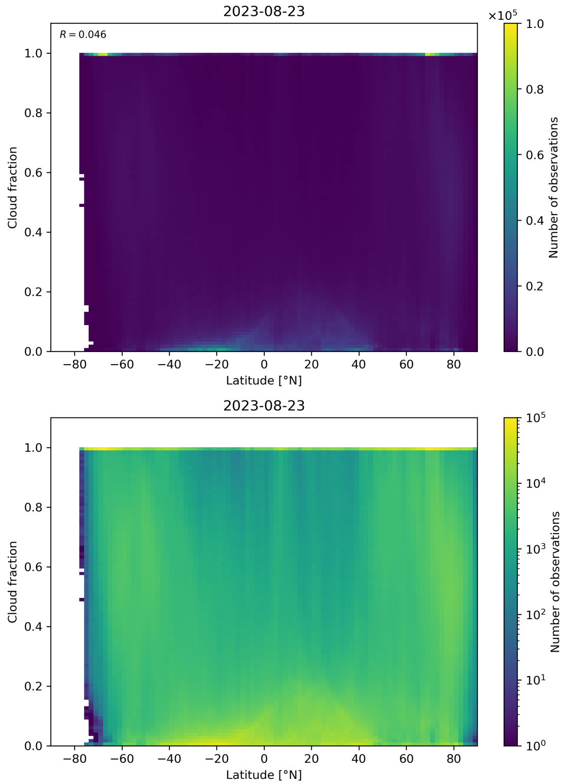
Figure 99: Scatter density plot of “Latitude” against “Cloud fraction” for 2023-08-22 to 2023-08-24.
