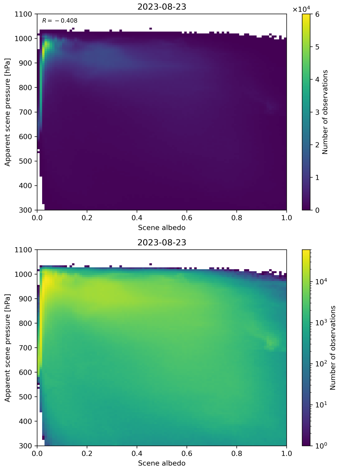
Figure 111: Scatter density plot of “Scene albedo” against “Apparent scene pressure” for 2023-08-22 to 2023-08-24.
