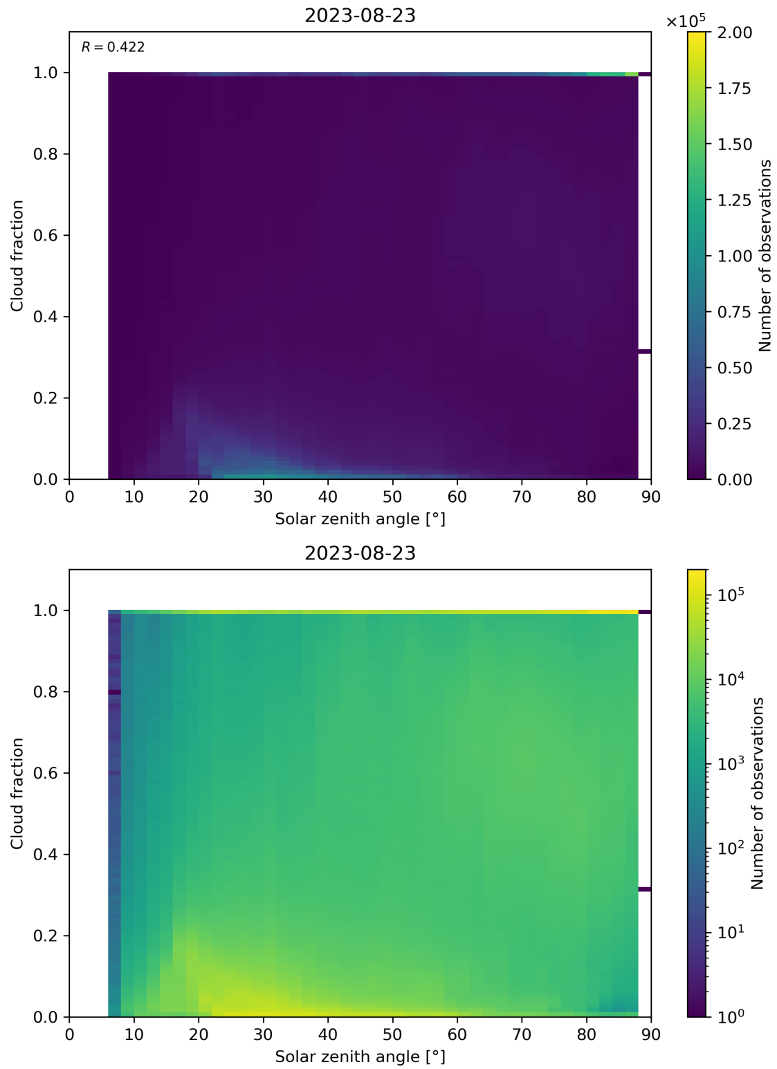
Figure 121: Scatter density plot of “Solar zenith angle” against “Cloud fraction” for 2023-08-22 to 2023-08-24.
