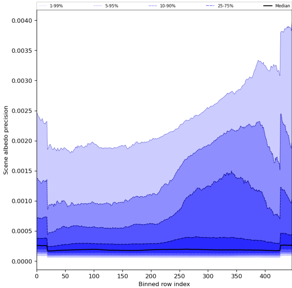
Figure 52: Along track statistics of “Scene albedo precision” for 2023-08-22 to 2023-08-24
