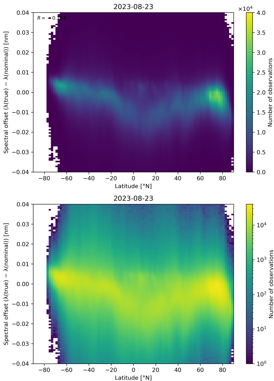
Figure 105: Scatter density plot of “Latitude” against “Spectral offset ( \lambda(\text{true}) - \lambda(\text{nominal}) )” for 2023-08-22 to 2023-08-24.
