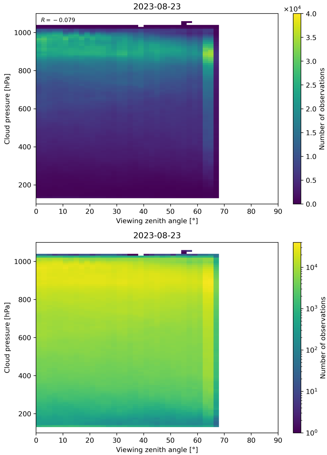
Figure 133: Scatter density plot of “Viewing zenith angle” against “Cloud pressure” for 2023-08-22 to 2023-08-24.
