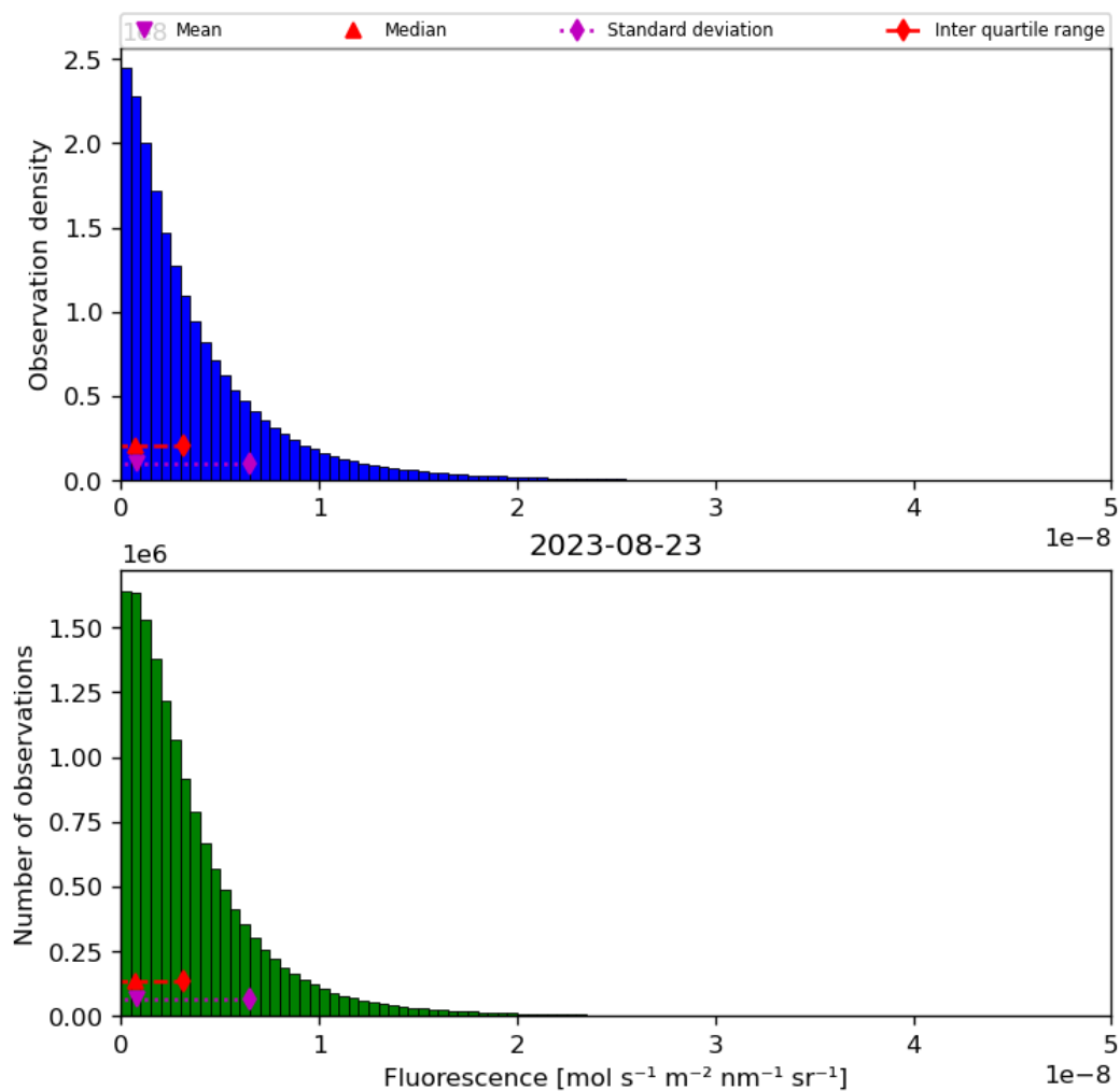
Figure 40: Histogram of “Fluorescence” for 2023-08-22 to 2023-08-24
