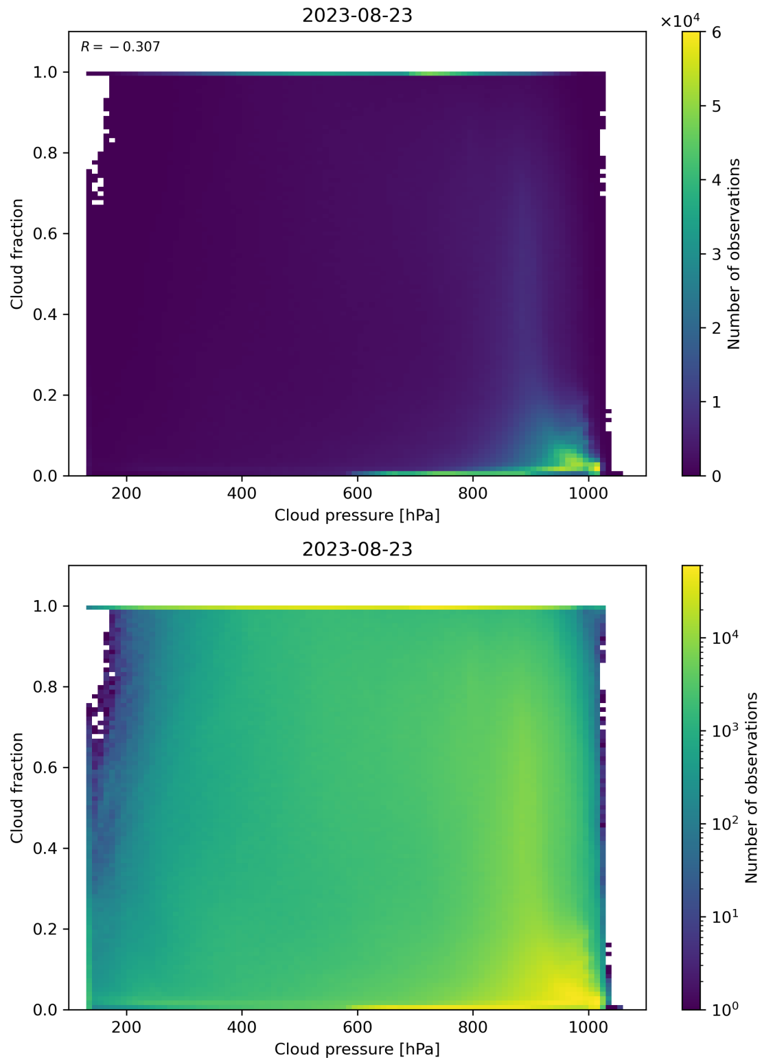
Figure 87: Scatter density plot of “Cloud pressure” against “Cloud fraction” for 2023-08-22 to 2023-08-24.
