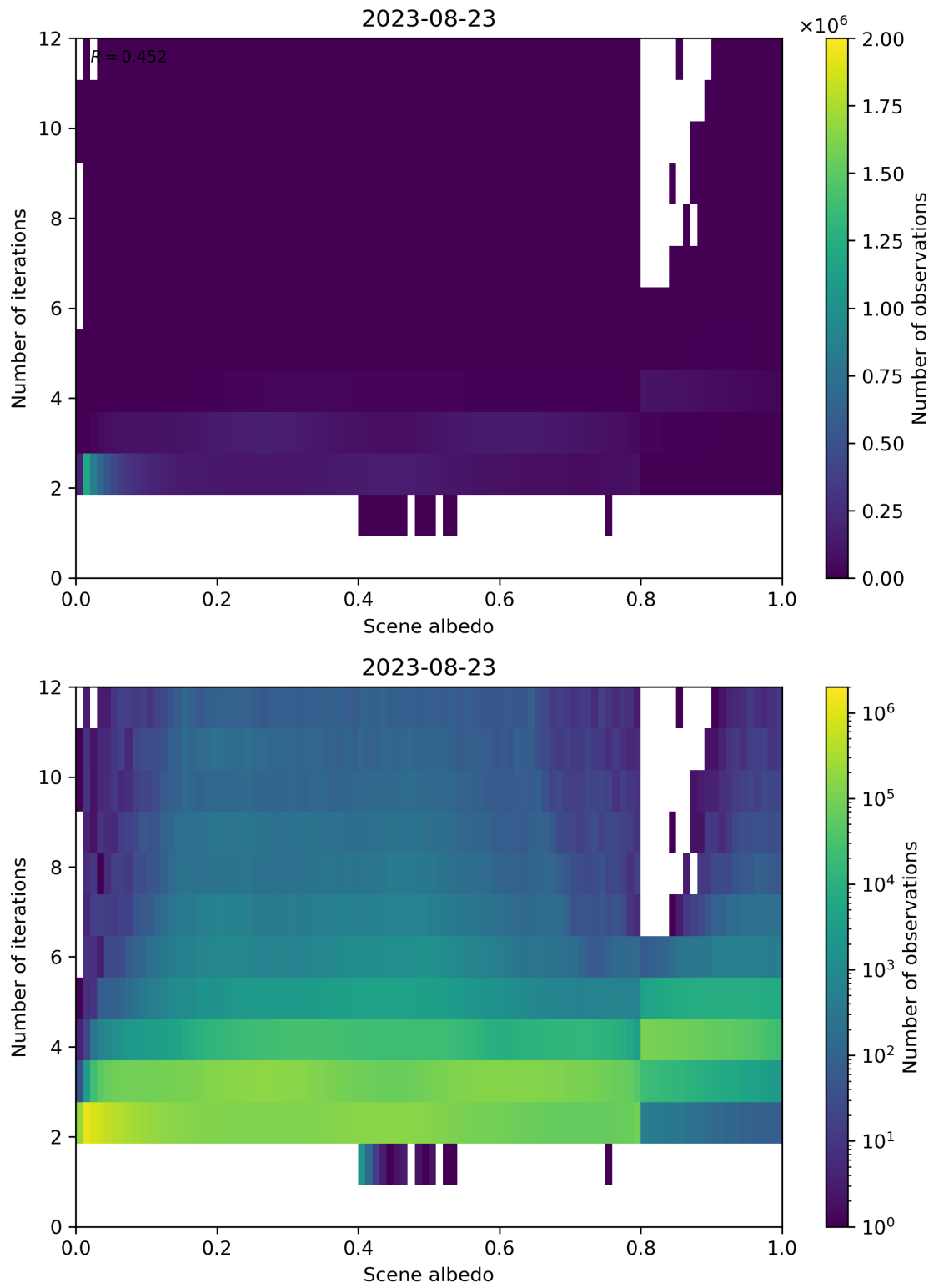
Figure 115: Scatter density plot of “Scene albedo” against “Number of iterations” for 2023-08-22 to 2023-08-24.
