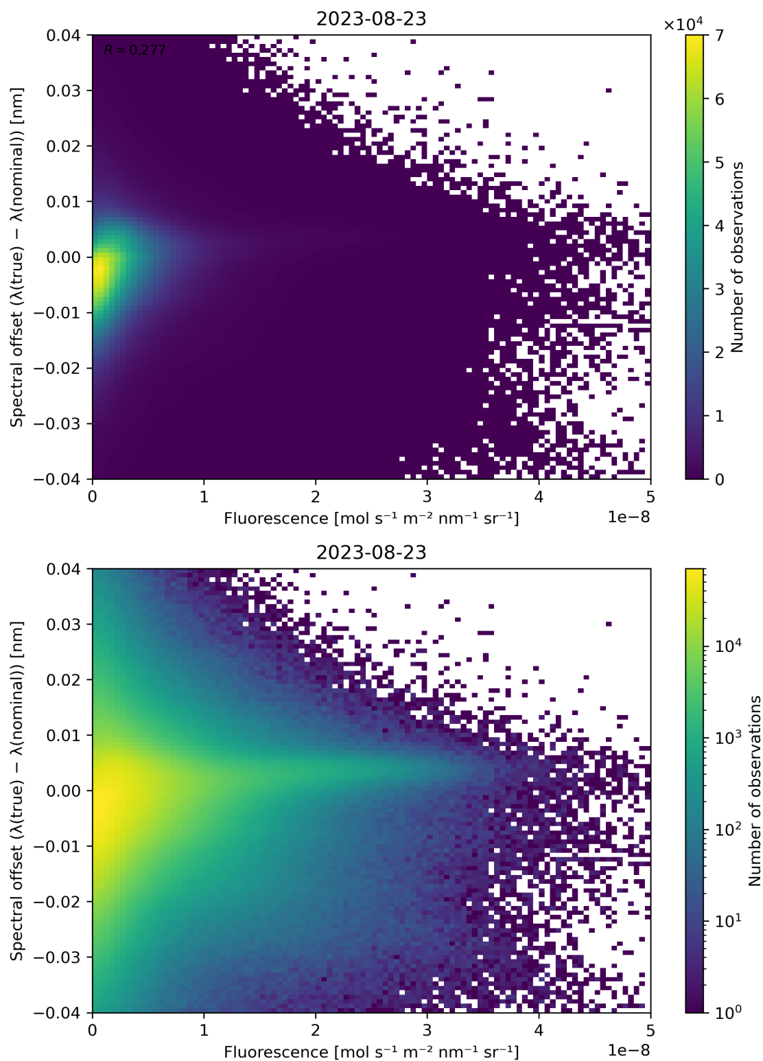
Figure 95: Scatter density plot of “Fluorescence” against “Spectral offset ( \lambda(\text{true}) - \lambda(\text{nominal}) )” for 2023-08-22 to 2023-08-24.
