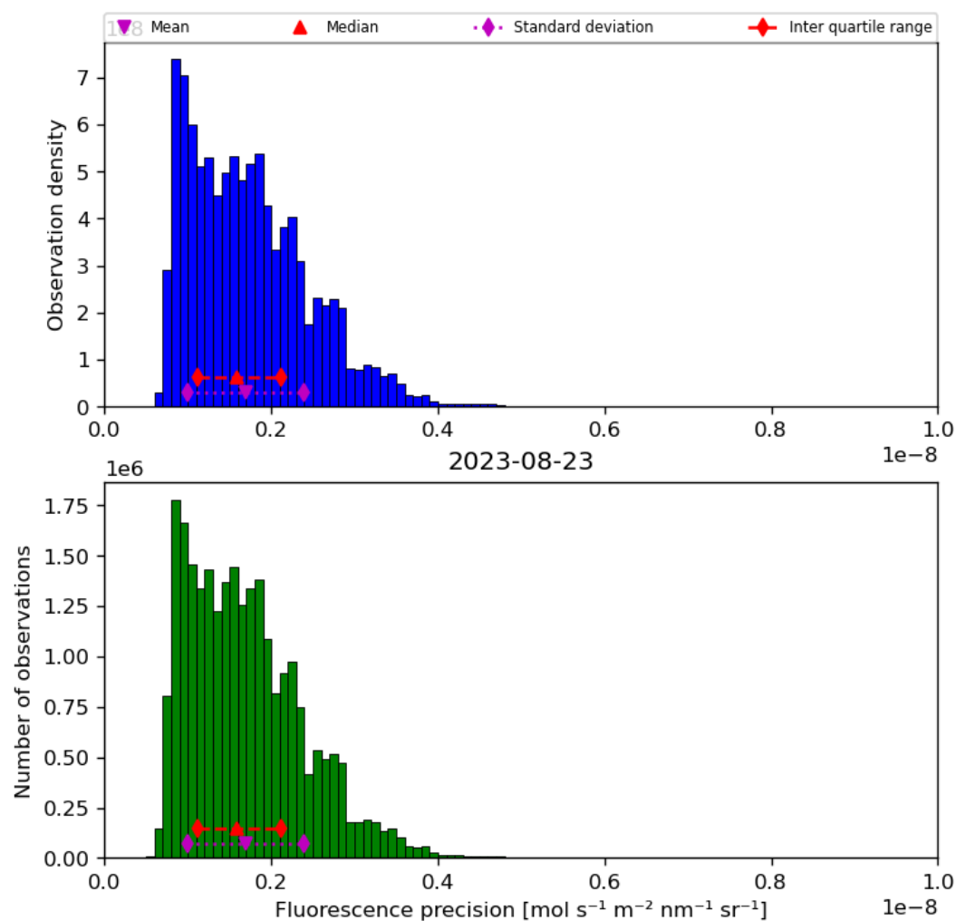
Figure 41: Histogram of “Fluorescence precision” for 2023-08-22 to 2023-08-24
