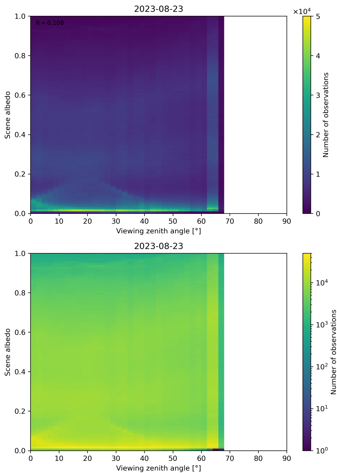
Figure 138: Scatter density plot of “Viewing zenith angle” against “Scene albedo” for 2023-08-22 to 2023-08-24.
