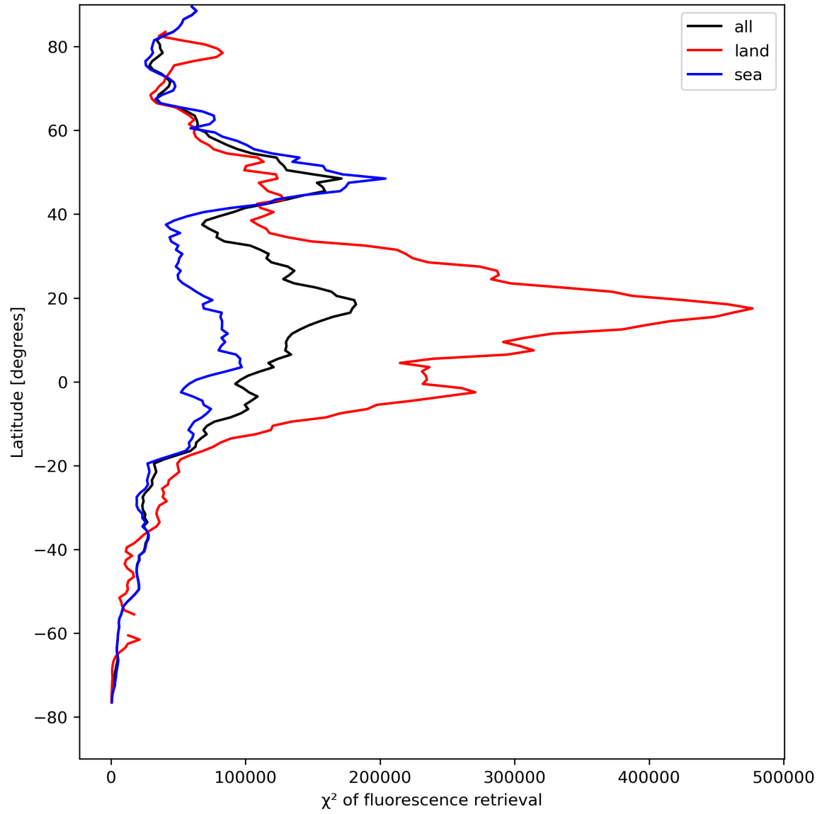
Figure 25: Zonal average of “ \chi^2 of fluorescence retrieval” for 2023-08-22 to 2023-08-24.
