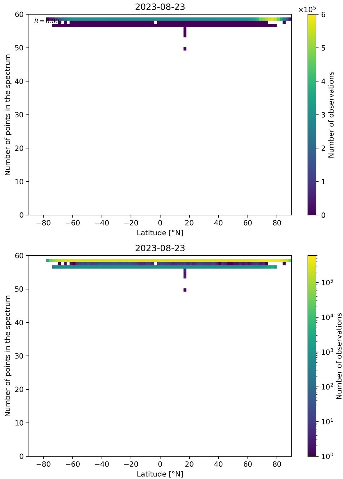
Figure 103: Scatter density plot of “Latitude” against “Number of points in the spectrum” for 2023-08-22 to 2023-08-24.
