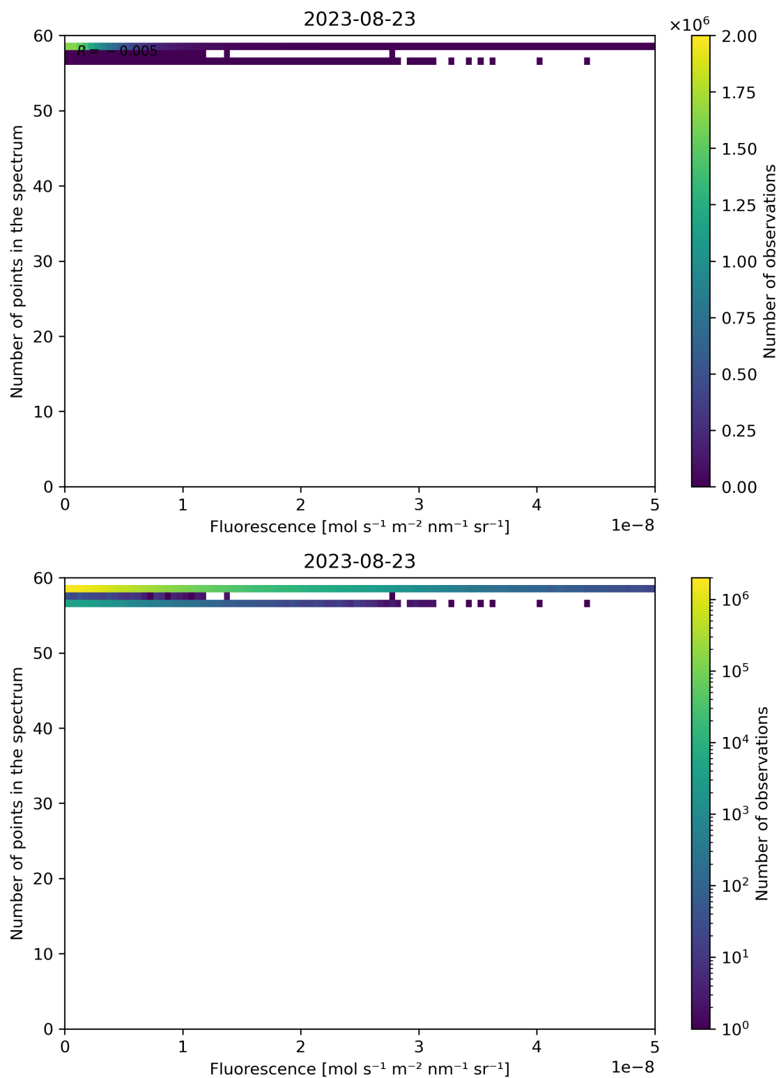
Figure 94: Scatter density plot of “Fluorescence” against “Number of points in the spectrum” for 2023-08-22 to 2023-08-24.
