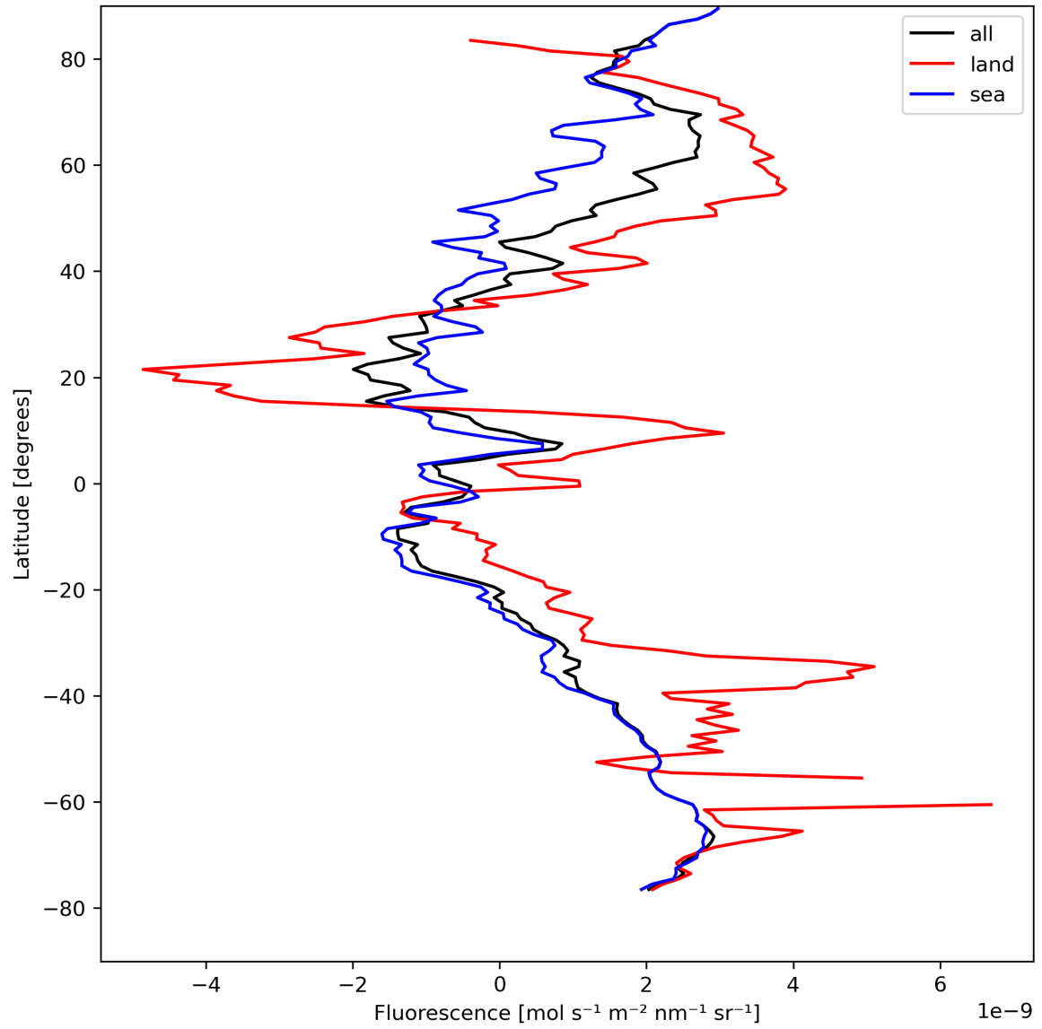
Figure 23: Zonal average of “Fluorescence” for 2023-08-22 to 2023-08-24.
