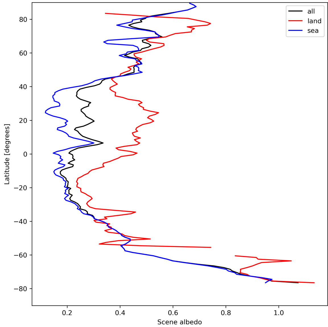
Figure 17: Zonal average of “Scene albedo” for 2023-08-22 to 2023-08-24.
