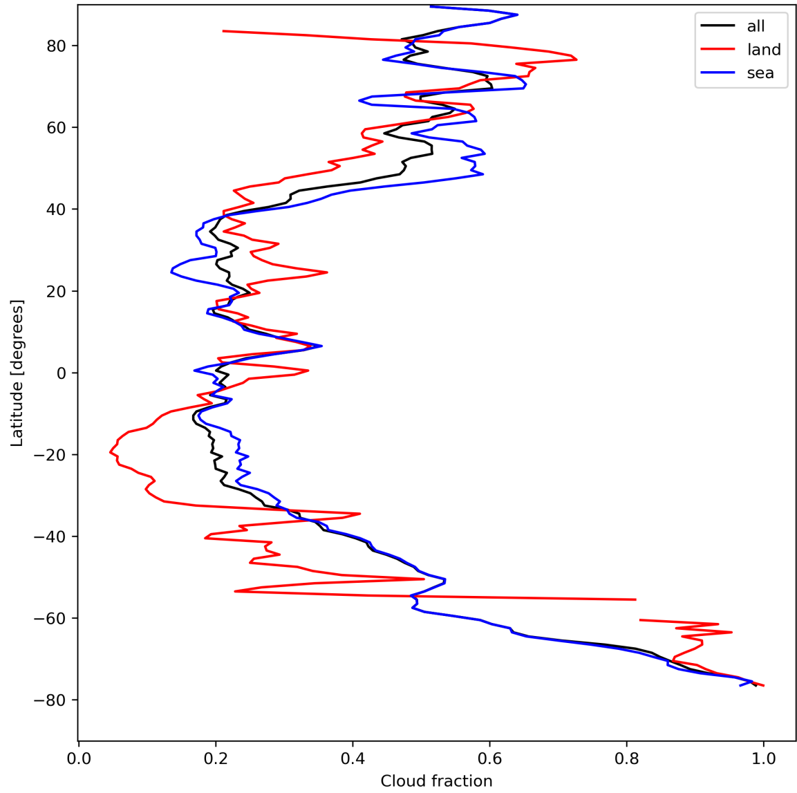
Figure 15: Zonal average of “Cloud fraction” for 2023-08-22 to 2023-08-24.
