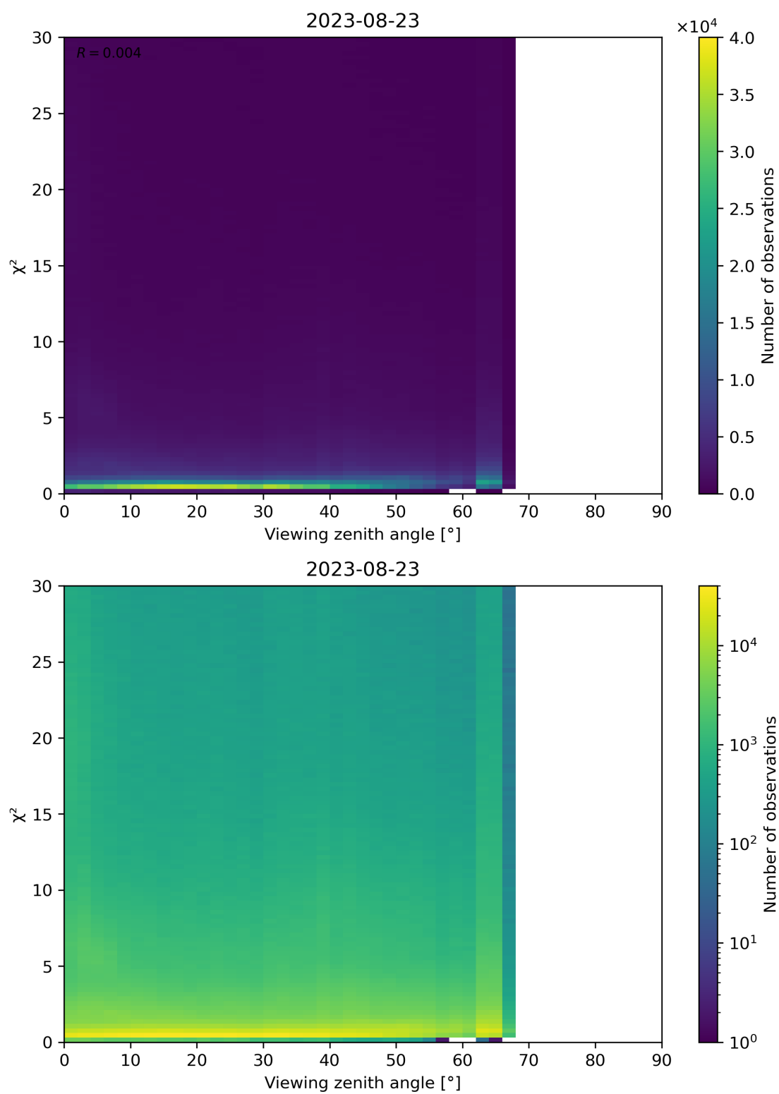
Figure 130: Scatter density plot of “Viewing zenith angle” against “ \chi^2 ” for 2023-08-22 to 2023-08-24.
