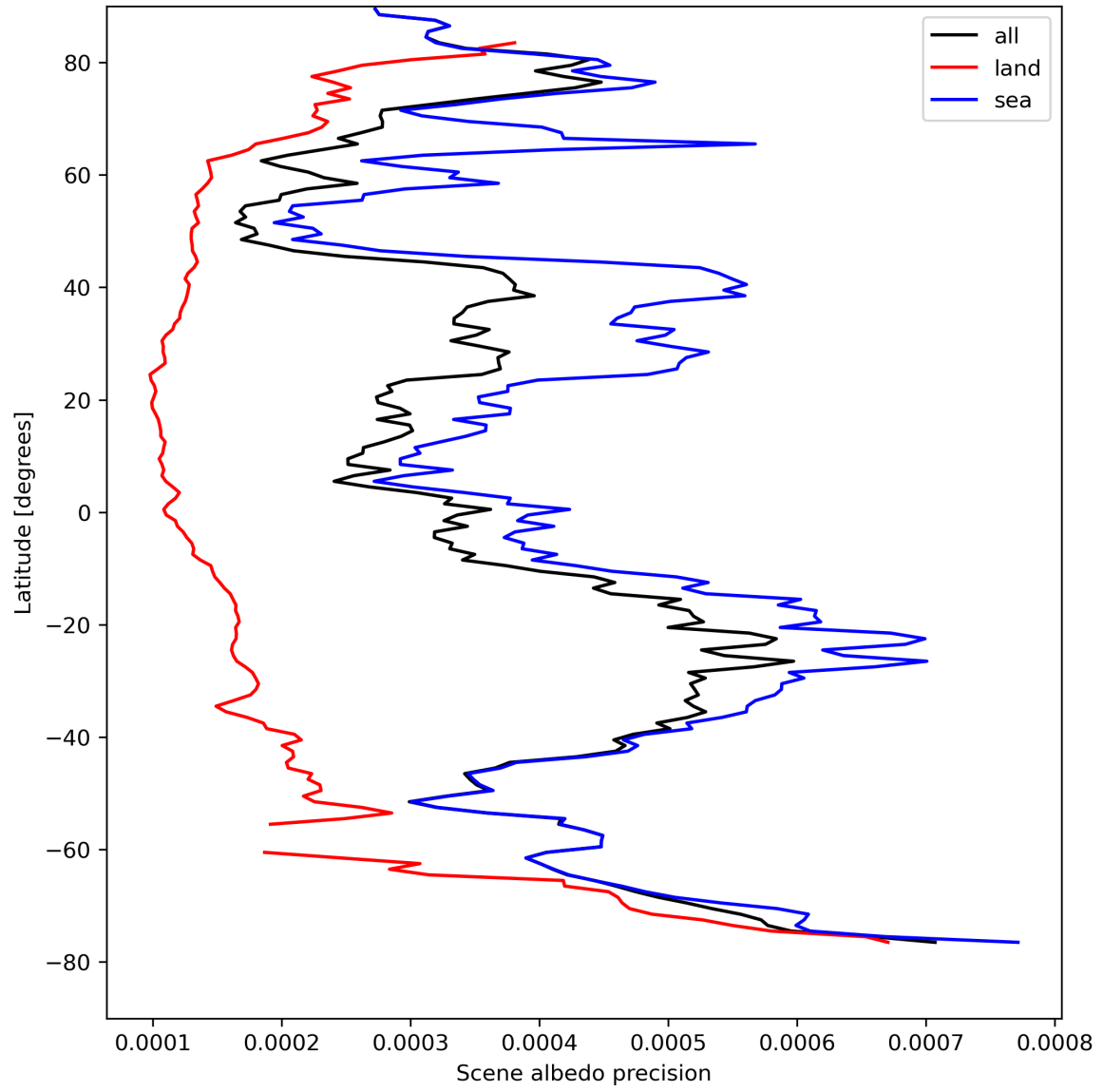
Figure 18: Zonal average of “Scene albedo precision” for 2023-08-22 to 2023-08-24.
