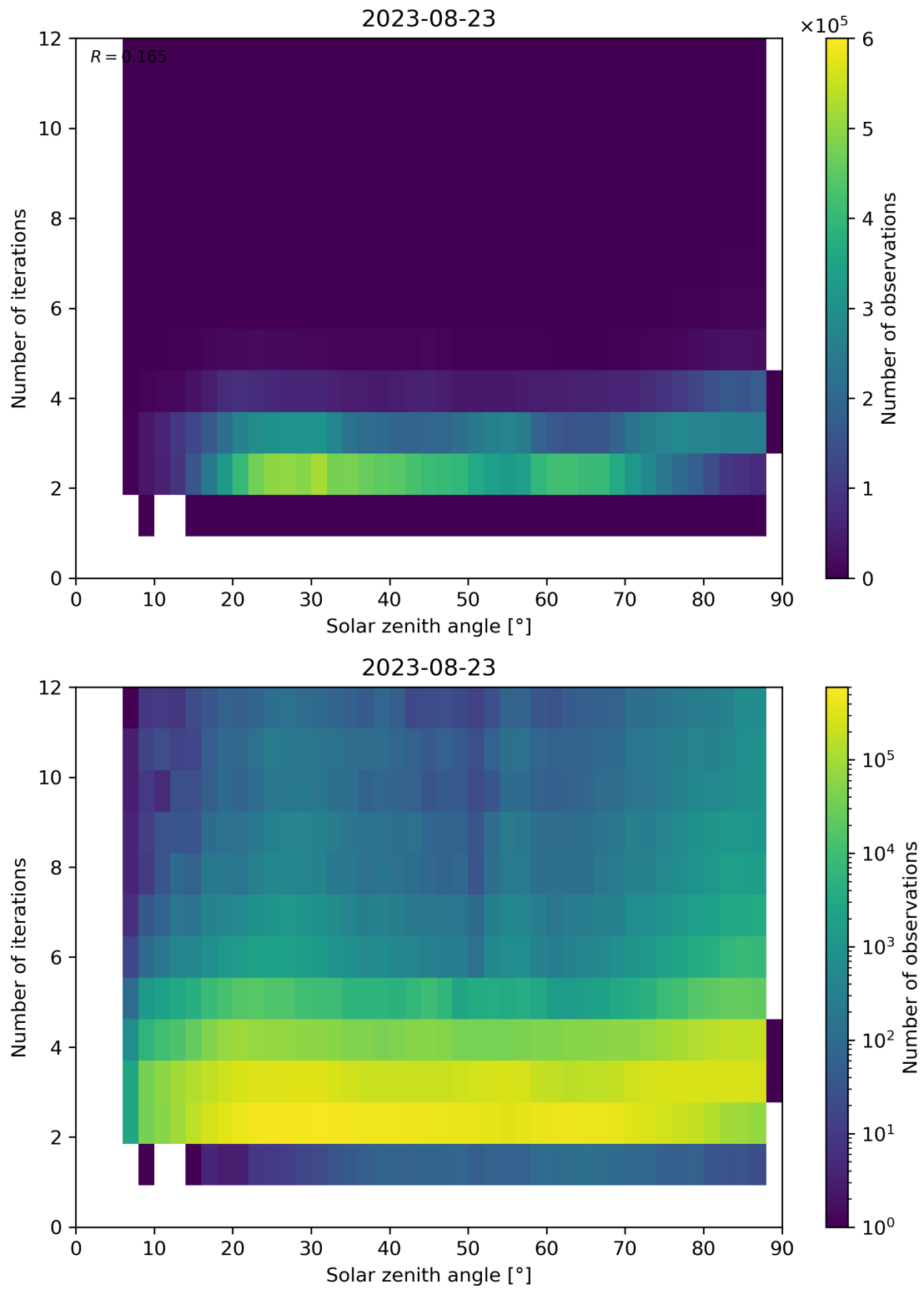
Figure 125: Scatter density plot of “Solar zenith angle” against “Number of iterations” for 2023-08-22 to 2023-08-24.
