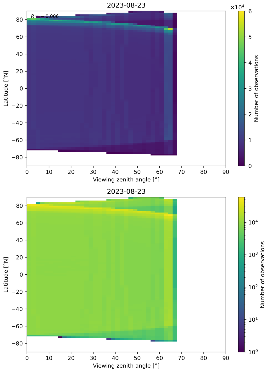
Figure 135: Scatter density plot of “Viewing zenith angle” against “Latitude” for 2023-08-22 to 2023-08-24.
