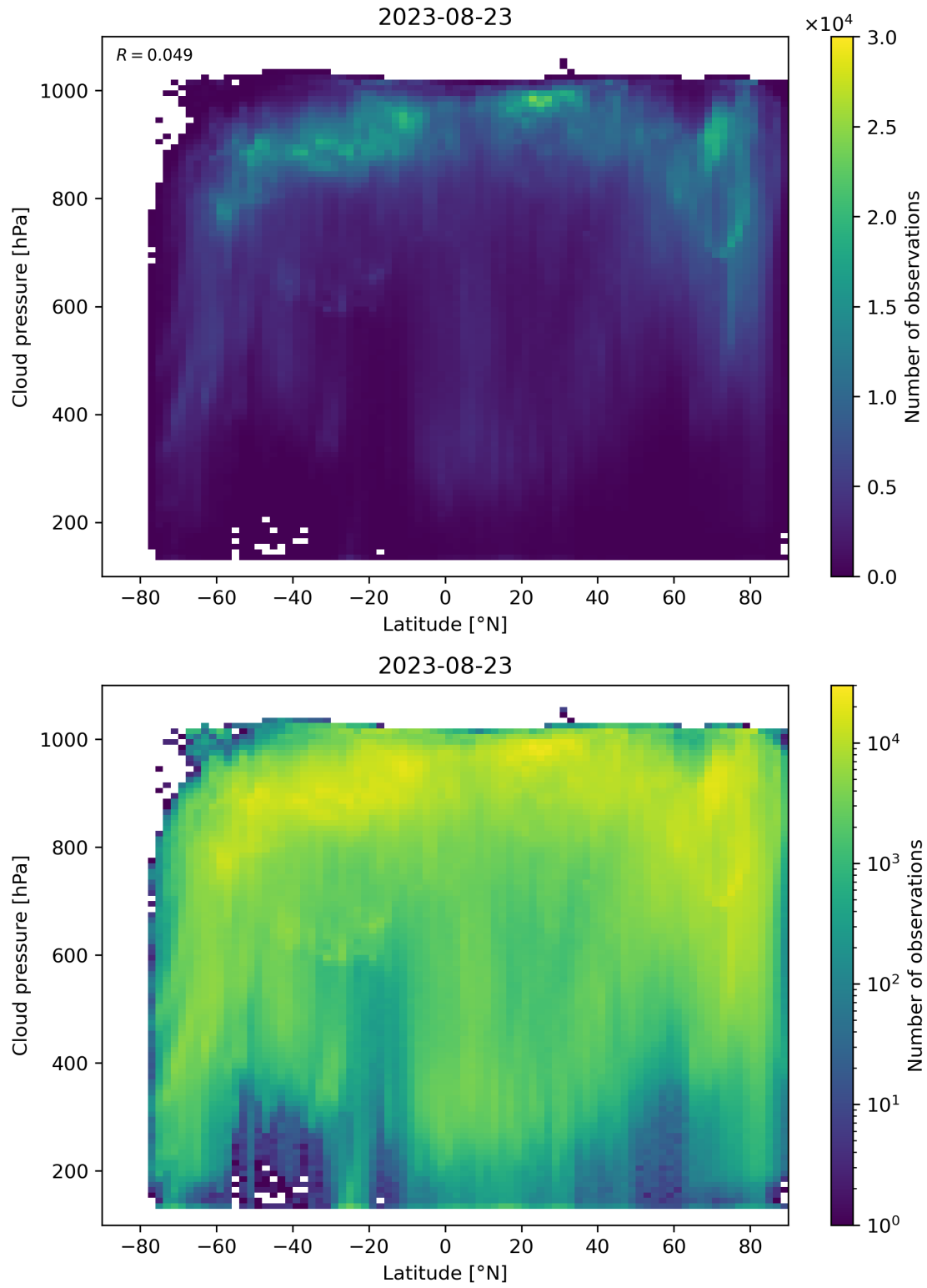
Figure 100: Scatter density plot of “Latitude” against “Cloud pressure” for 2023-08-22 to 2023-08-24.
