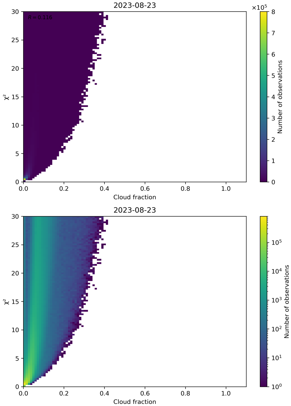
Figure 77: Scatter density plot of “Cloud fraction” against “ \chi^2 ” for 2023-08-22 to 2023-08-24.
