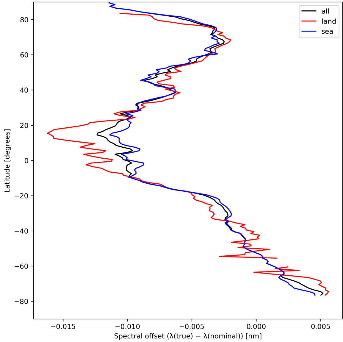
Figure 28: Zonal average of “Spectral offset ( \lambda(\text{true}) - \lambda(\text{nominal}) )” for 2023-08-22 to 2023-08-24.
