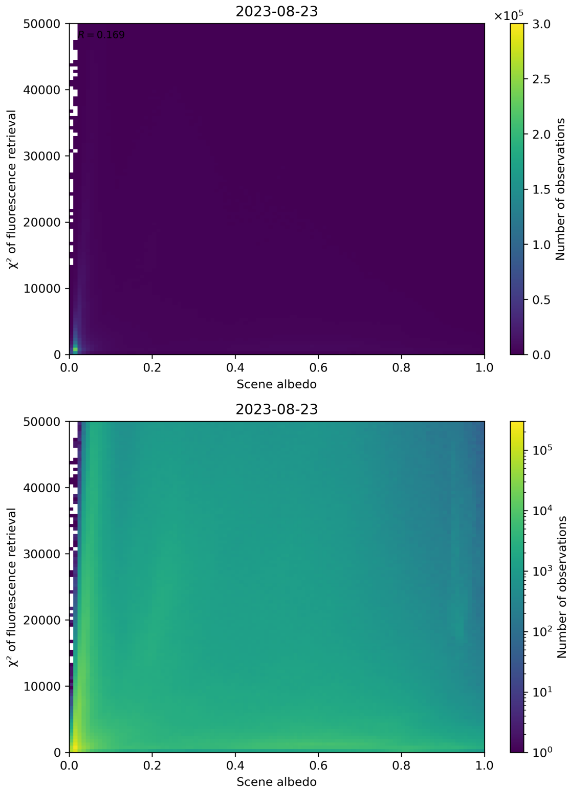
Figure 113: Scatter density plot of “Scene albedo” against “ \chi^2 of fluorescence retrieval” for 2023-08-22 to 2023-08-24.
