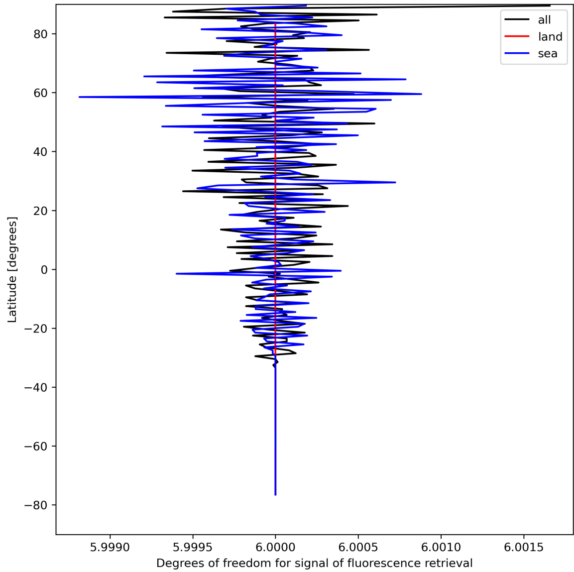
Figure 26: Zonal average of “Degrees of freedom for signal of fluorescence retrieval” for 2023-08-22 to 2023-08-24.
