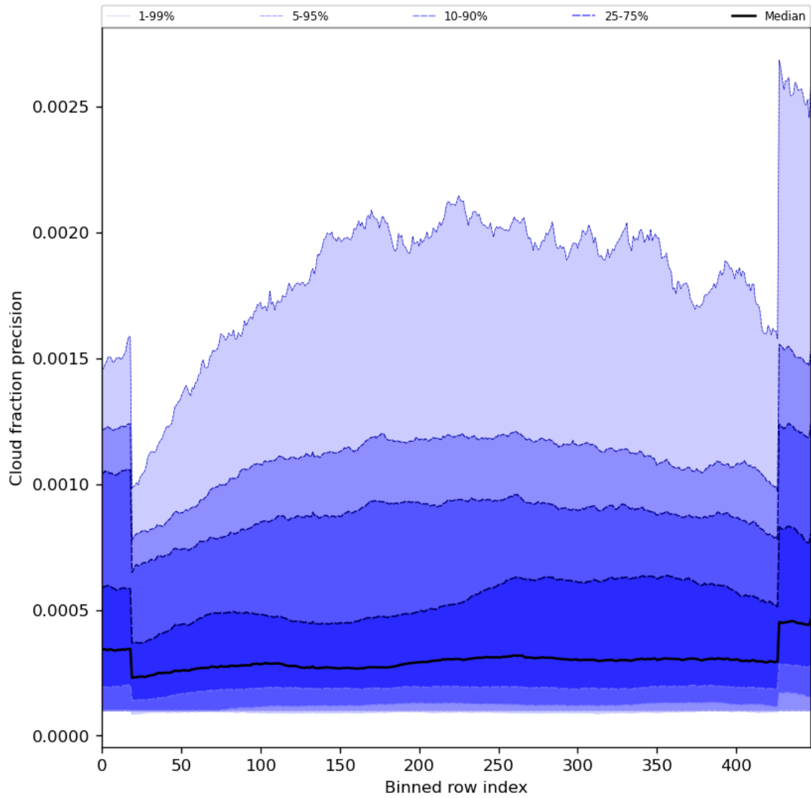
Figure 50: Along track statistics of “Cloud fraction precision” for 2023-08-22 to 2023-08-24
