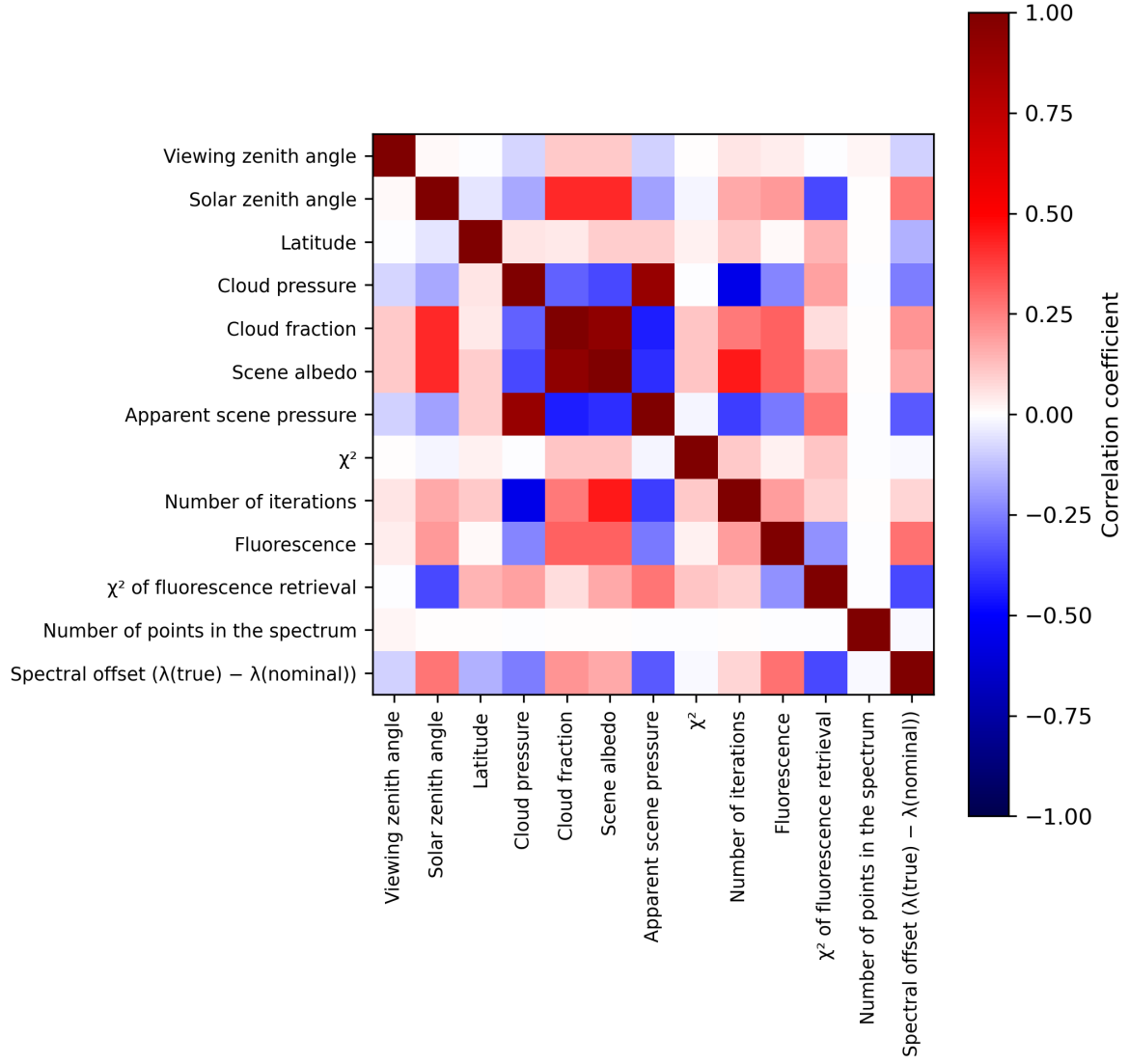
Figure 2: Map of correlation matrix for 2023-08-22 to 2023-08-24.
