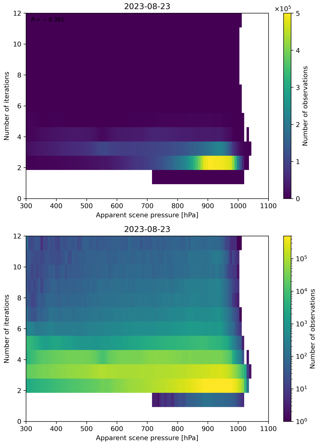
Figure 66: Scatter density plot of “Apparent scene pressure” against “Number of iterations” for 2023-08-22 to 2023-08-24.
