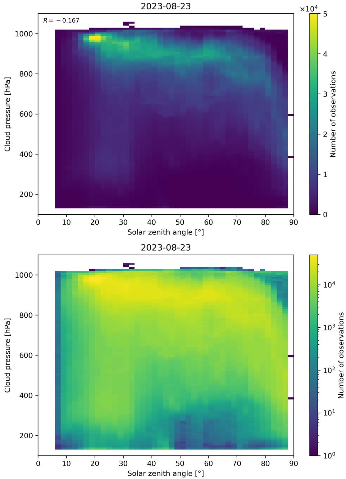
Figure 122: Scatter density plot of “Solar zenith angle” against “Cloud pressure” for 2023-08-22 to 2023-08-24.
