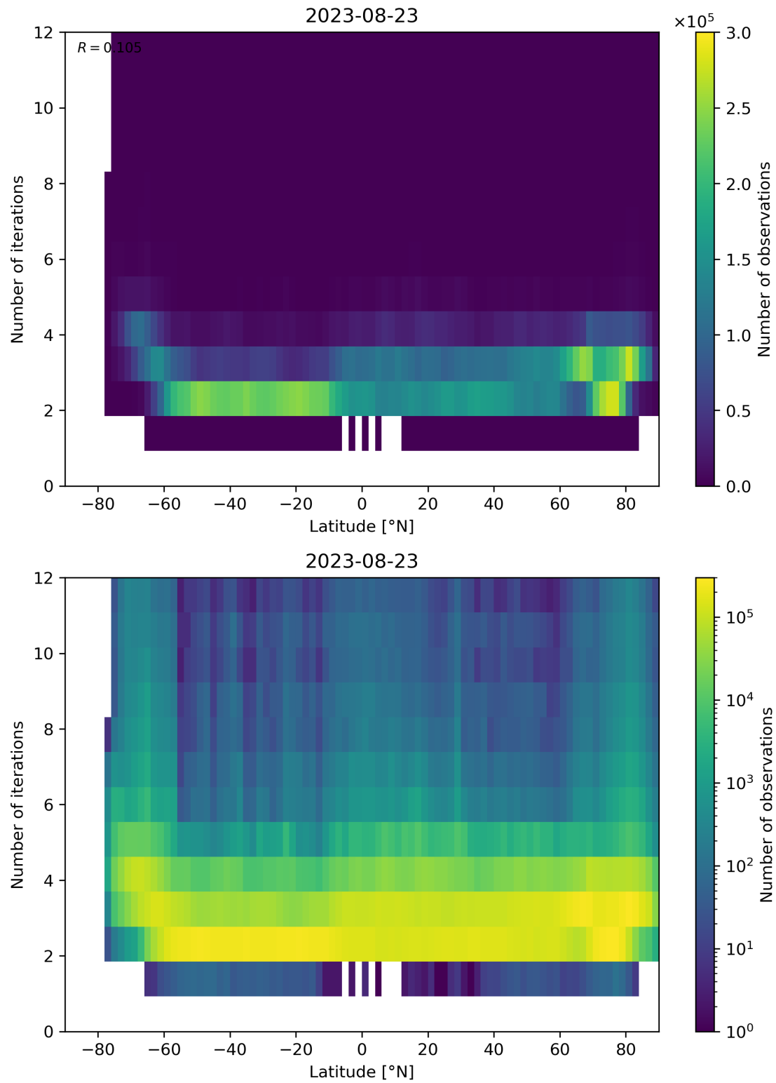
Figure 102: Scatter density plot of “Latitude” against “Number of iterations” for 2023-08-22 to 2023-08-24.
