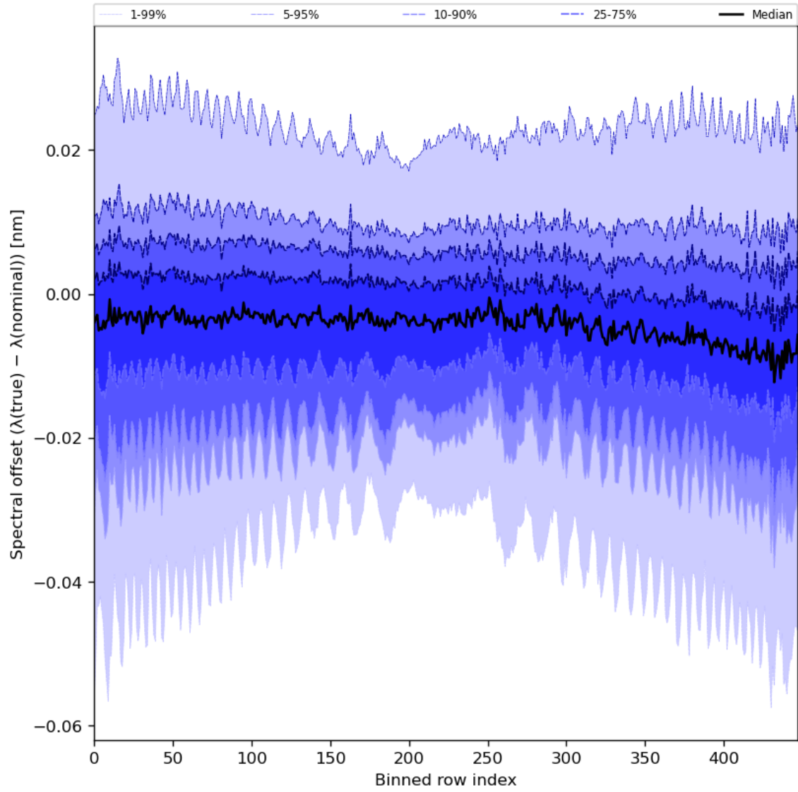
Figure 62: Along track statistics of “Spectral offset ( \lambda(\text{true}) - \lambda(\text{nominal}) )” for 2023-08-22 to 2023-08-24
