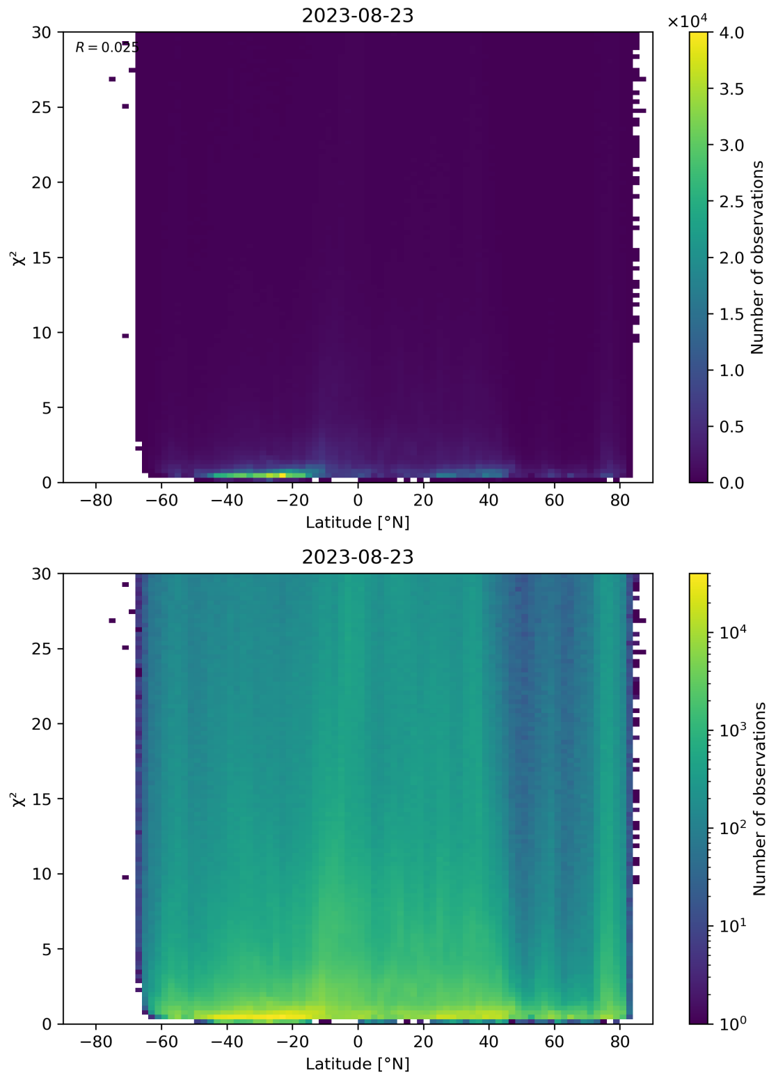
Figure 97: Scatter density plot of “Latitude” against “ \chi^2 ” for 2023-08-22 to 2023-08-24.
