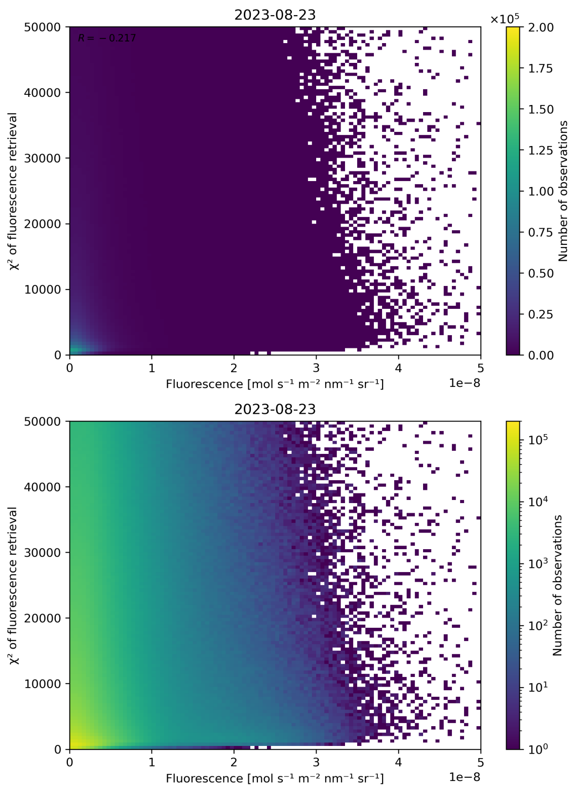
Figure 93: Scatter density plot of “Fluorescence” against “ \chi^2 of fluorescence retrieval” for 2023-08-22 to 2023-08-24.
