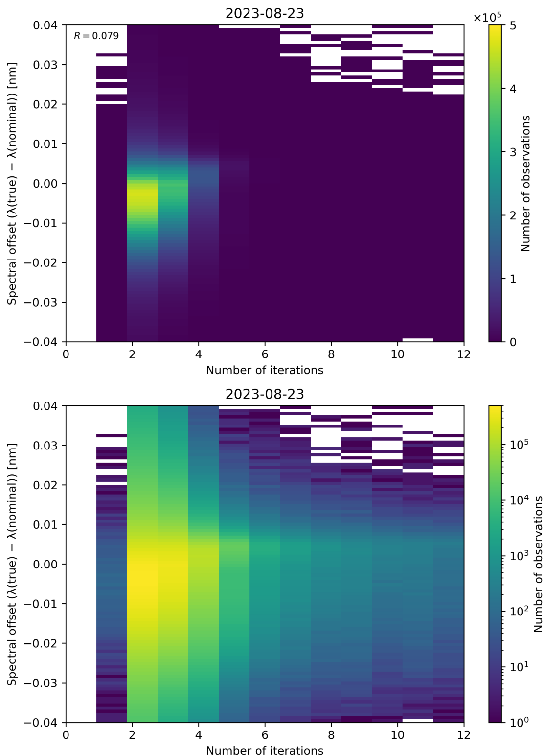
Figure 109: Scatter density plot of “Number of iterations” against “Spectral offset ( \lambda(\text{true}) - \lambda(\text{nominal}) )” for 2023-08-22 to 2023-08-24.
