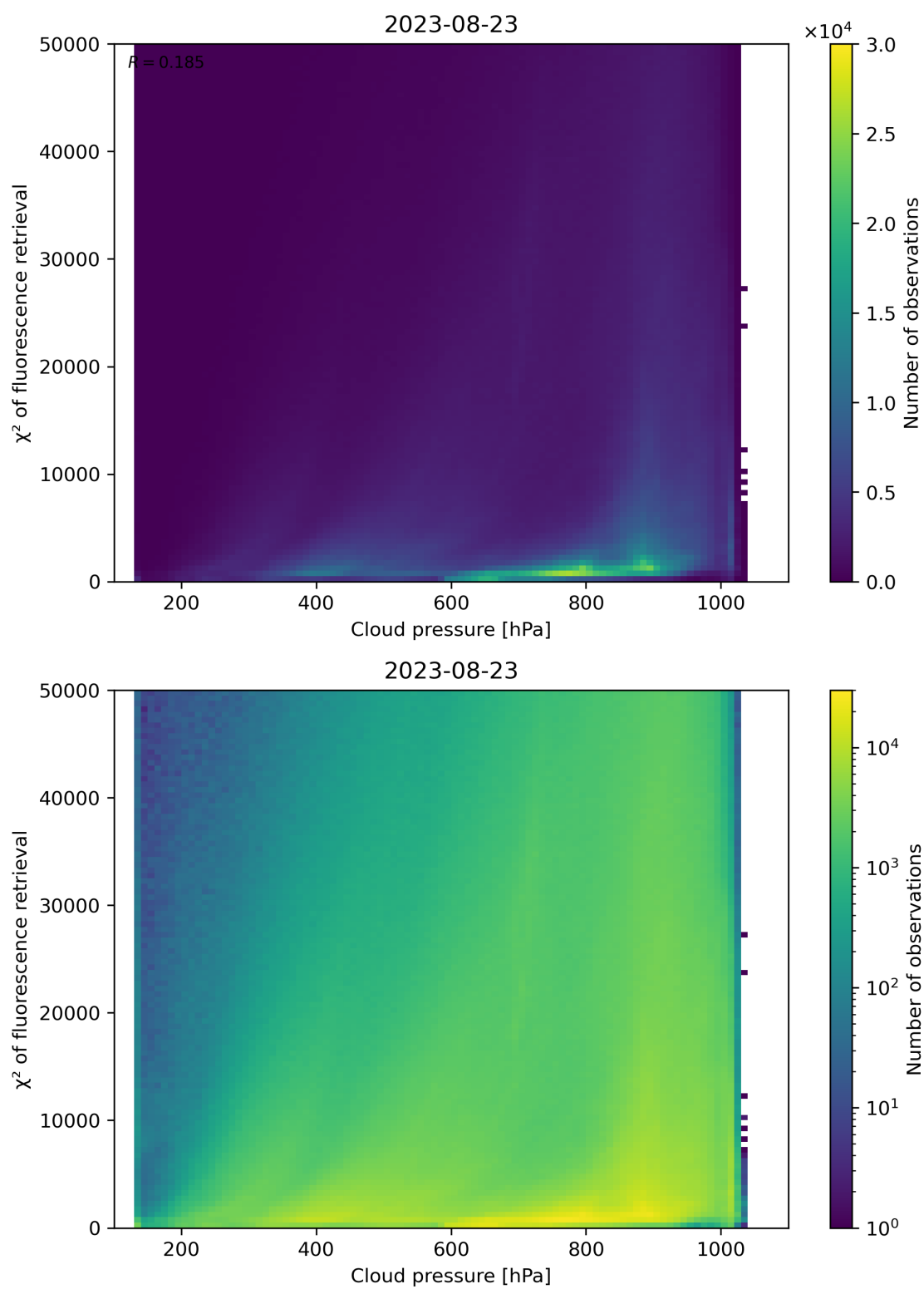
Figure 86: Scatter density plot of “Cloud pressure” against “ \chi^2 of fluorescence retrieval” for 2023-08-22 to 2023-08-24.
