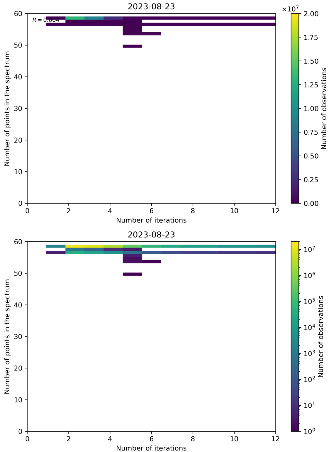
Figure 108: Scatter density plot of “Number of iterations” against “Number of points in the spectrum” for 2023-08-22 to 2023-08-24.
