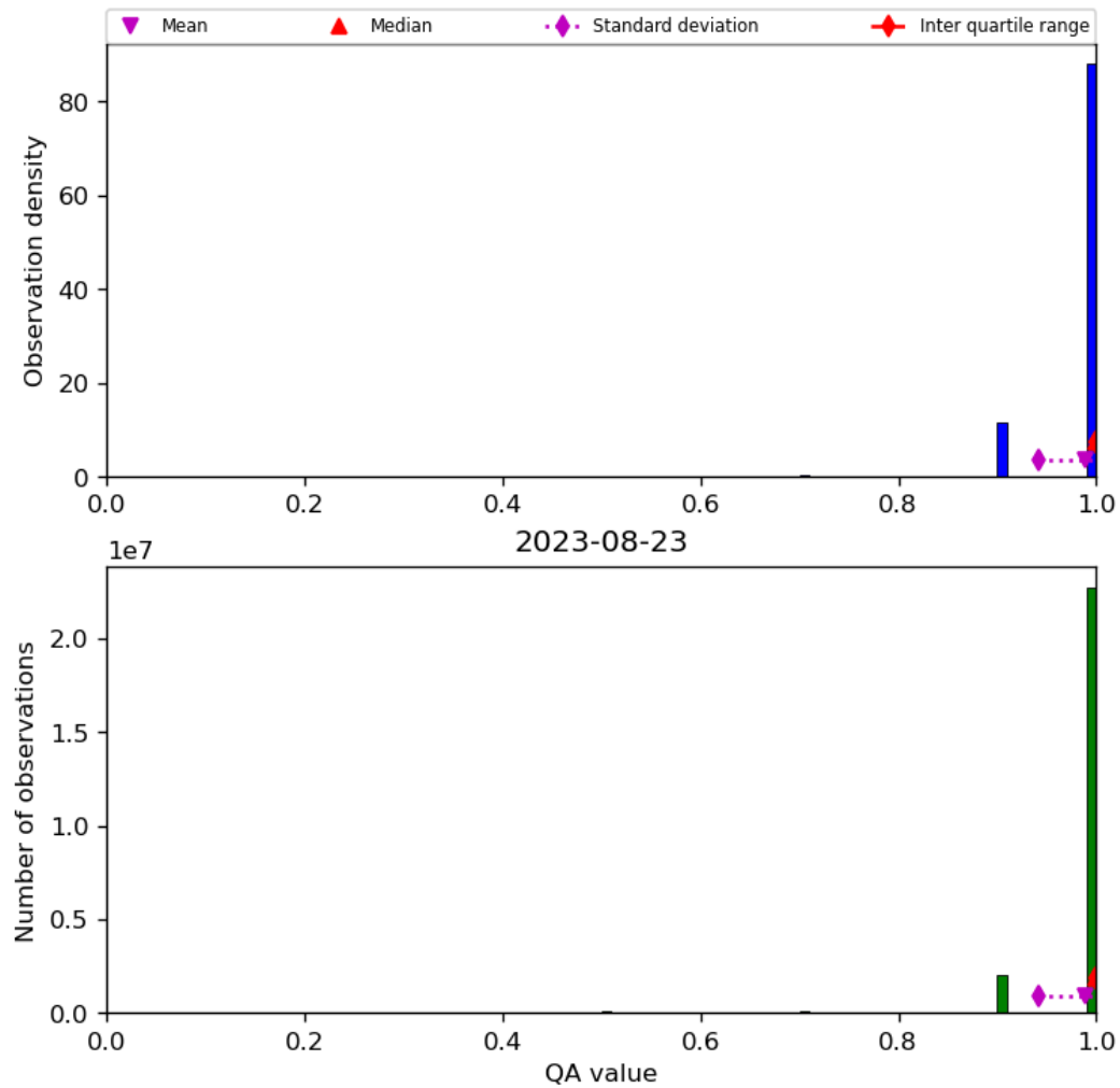
Figure 29: Histogram of “QA value” for 2023-08-22 to 2023-08-24
