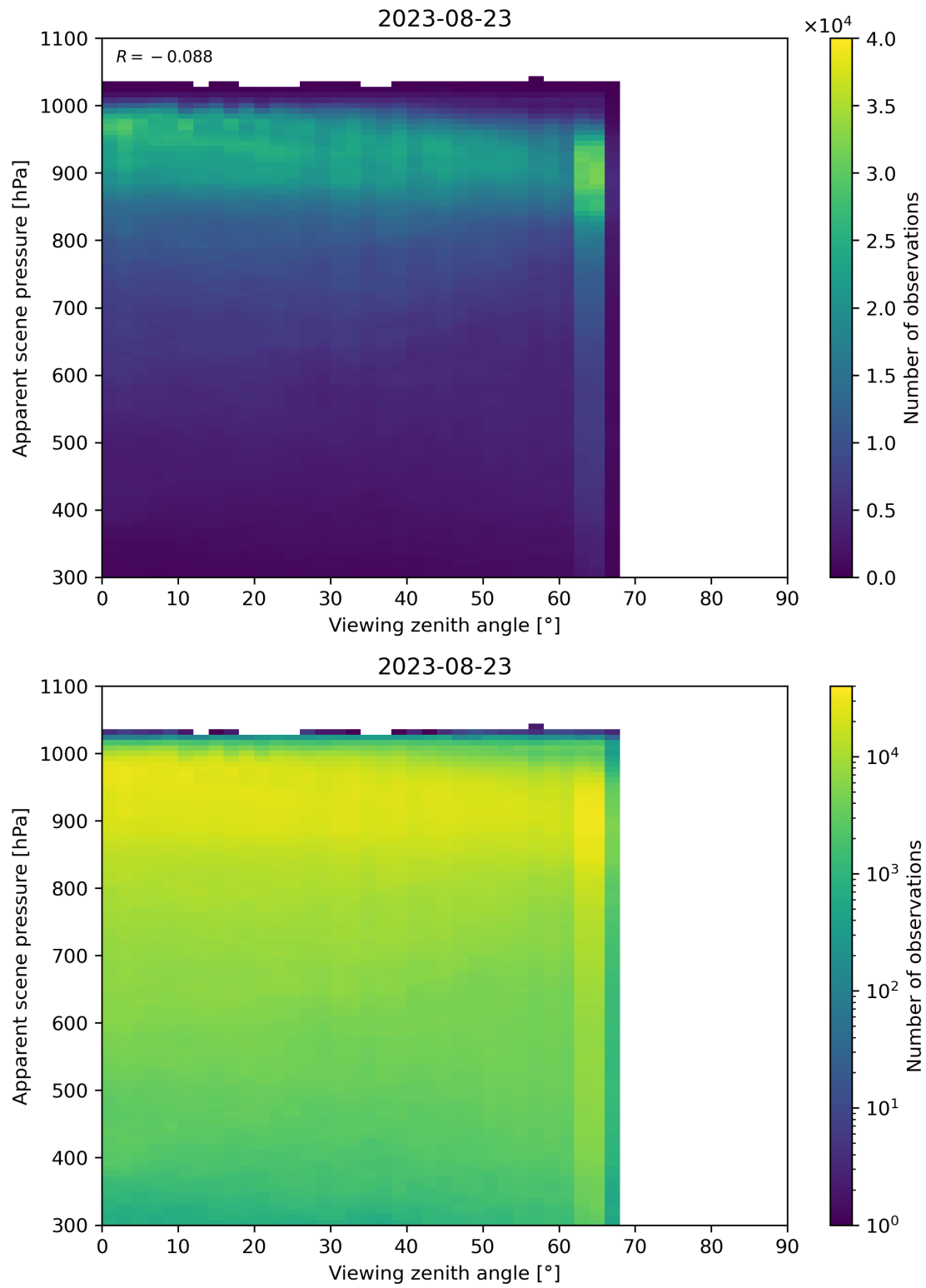
Figure 129: Scatter density plot of “Viewing zenith angle” against “Apparent scene pressure” for 2023-08-22 to 2023-08-24.
