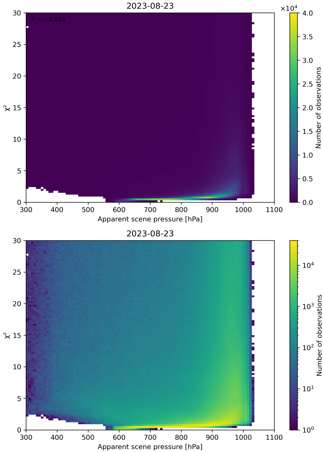
Figure 63: Scatter density plot of “Apparent scene pressure” against “ \chi^2 ” for 2023-08-22 to 2023-08-24.
