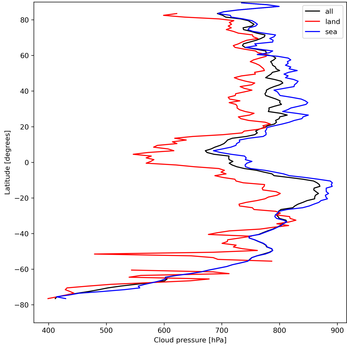
Figure 13: Zonal average of “Cloud pressure” for 2023-08-22 to 2023-08-24.
