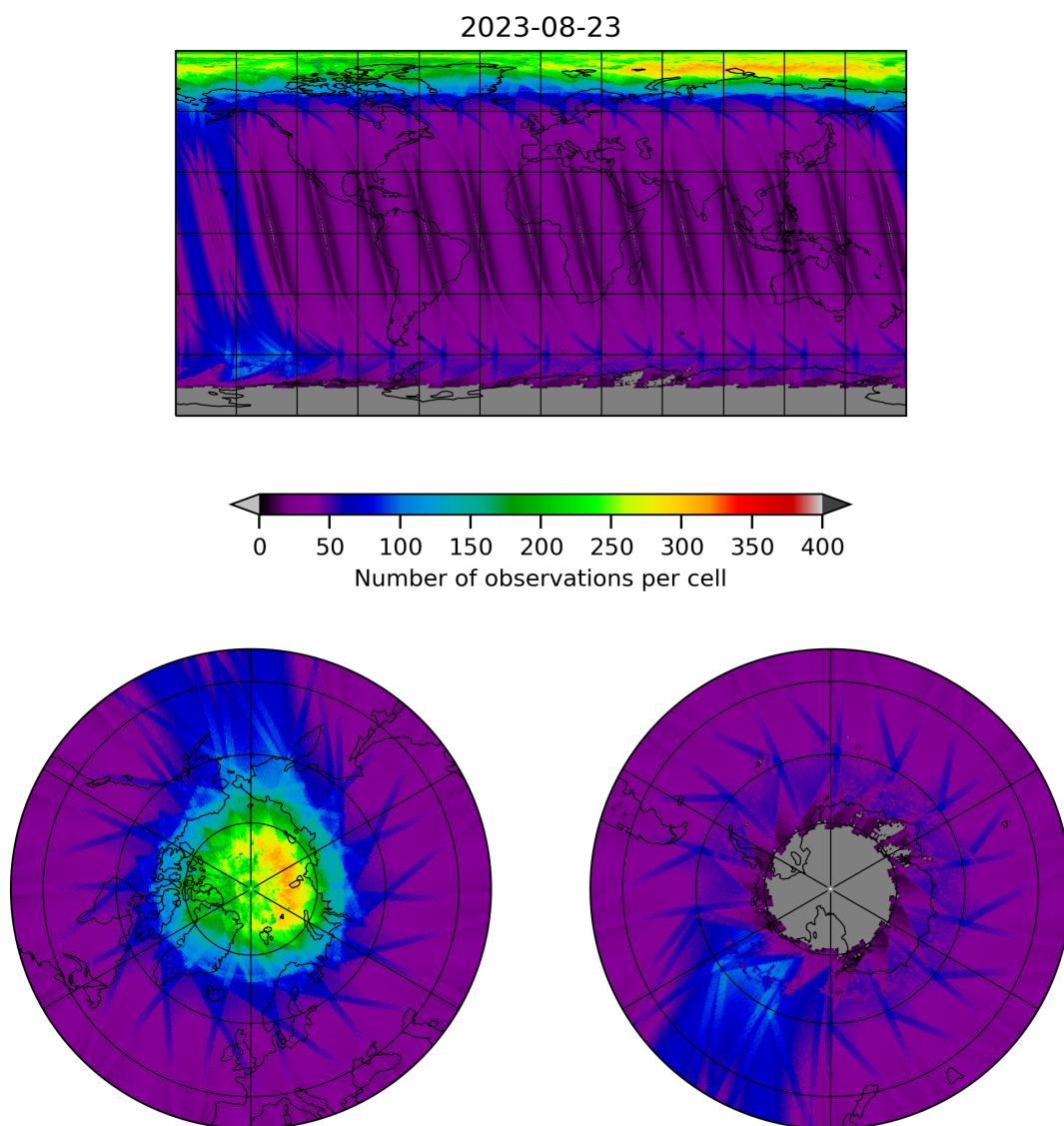
Figure 11: Map of the number of observations for 2023-08-22 to 2023-08-24
