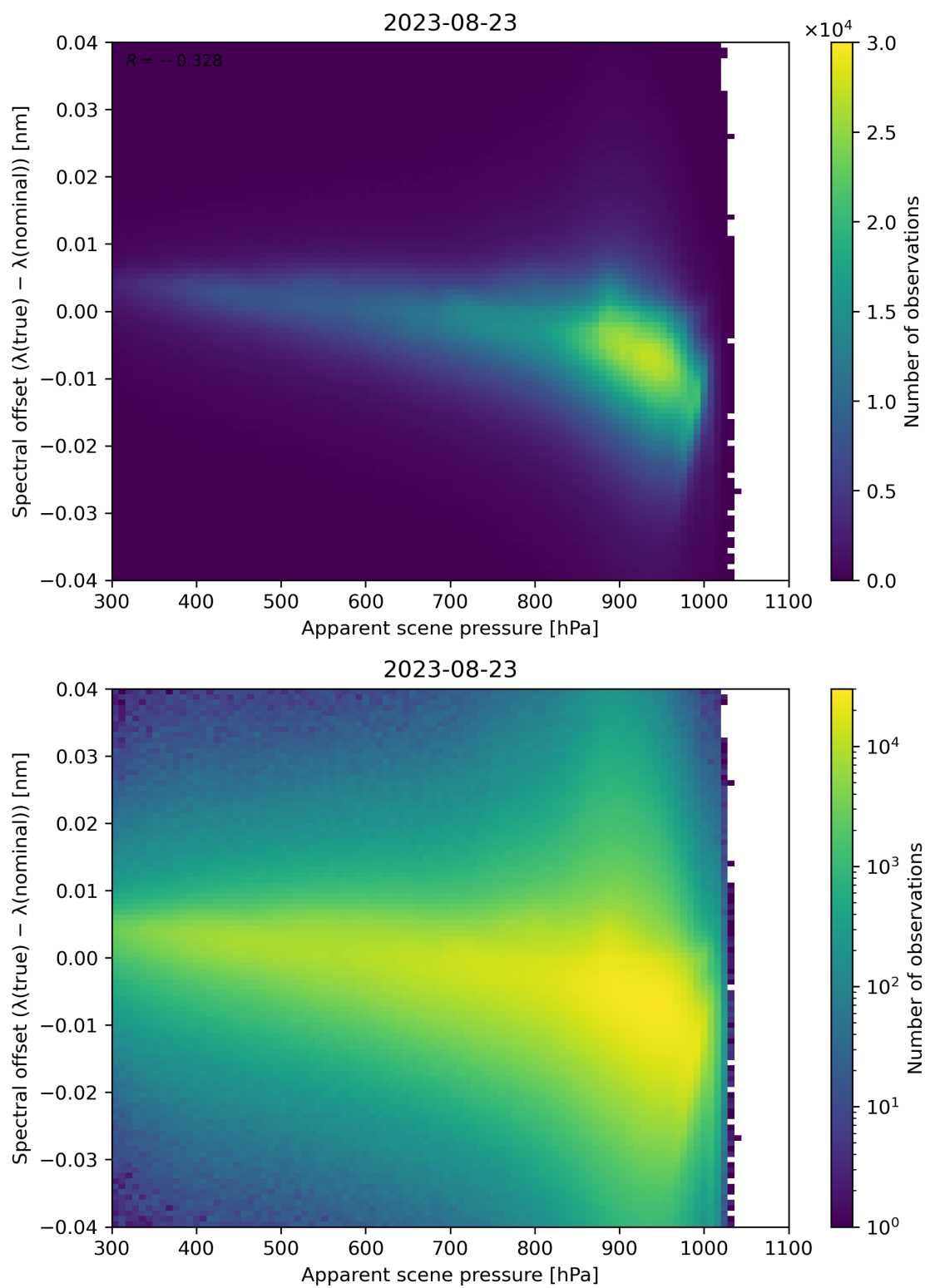
Figure 68: Scatter density plot of “Apparent scene pressure” against “Spectral offset ( \lambda(\text{true}) - \lambda(\text{nominal}) )” for 2023-08-22 to 2023-08-24.
