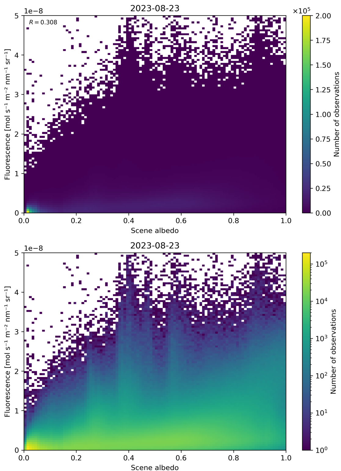
Figure 114: Scatter density plot of “Scene albedo” against “Fluorescence” for 2023-08-22 to 2023-08-24.
