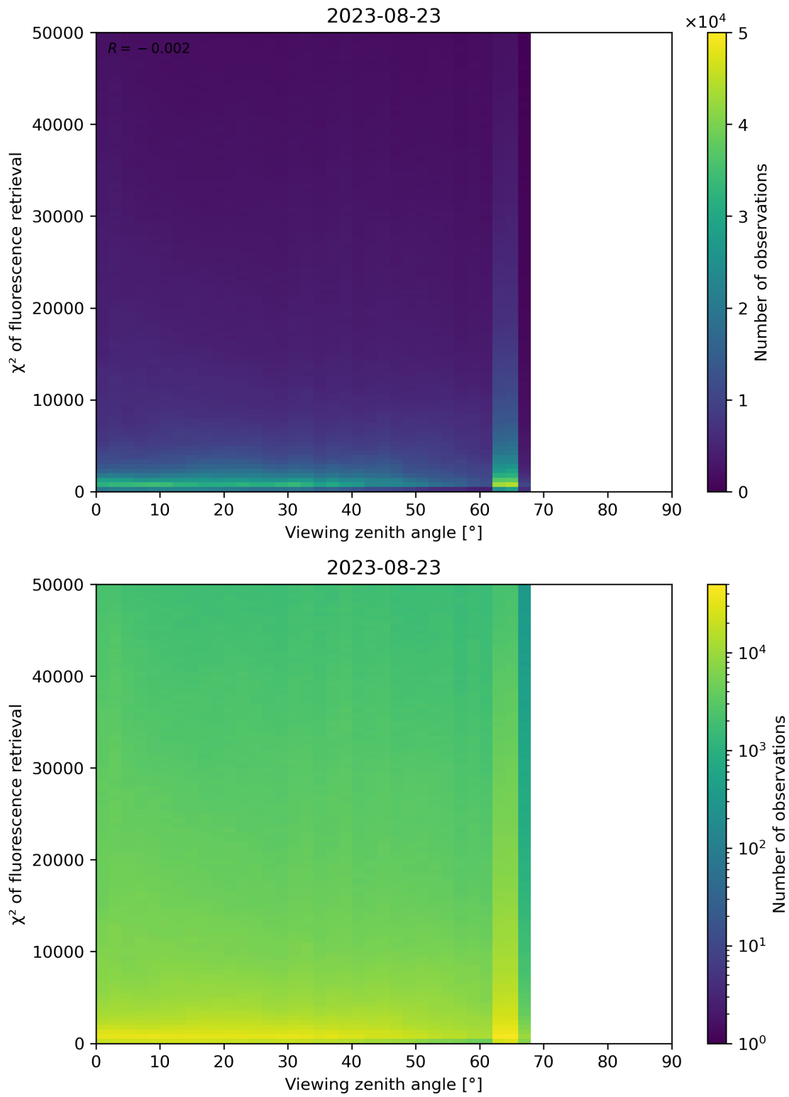
Figure 131: Scatter density plot of “Viewing zenith angle” against “ \chi^2 of fluorescence retrieval” for 2023-08-22 to 2023-08-24.
