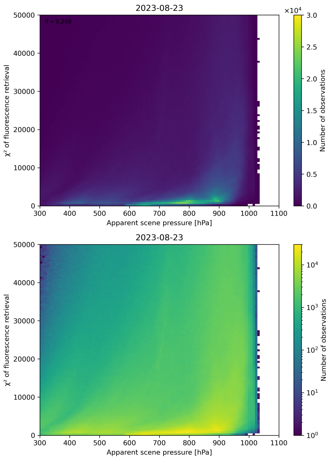
Figure 64: Scatter density plot of “Apparent scene pressure” against “ \chi^2 of fluorescence retrieval” for 2023-08-22 to 2023-08-24.
