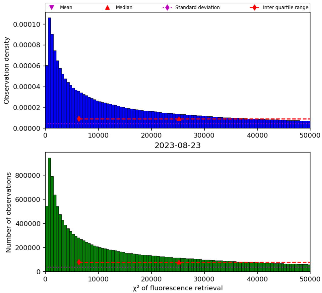
Figure 42: Histogram of “ \chi^2 of fluorescence retrieval” for 2023-08-22 to 2023-08-24
