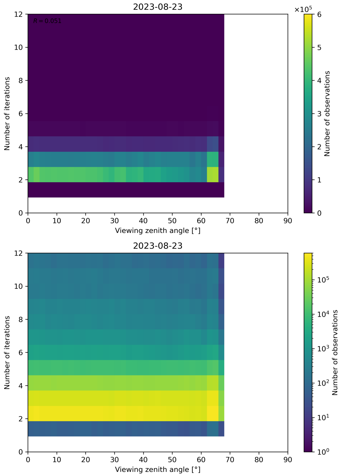
Figure 136: Scatter density plot of “Viewing zenith angle” against “Number of iterations” for 2023-08-22 to 2023-08-24.
