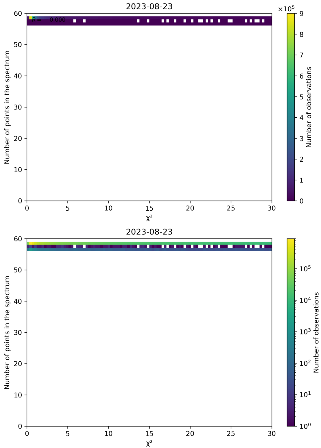
Figure 74: Scatter density plot of " \chi^2 " against "Number of points in the spectrum" for 2023-08-22 to 2023-08-24.
