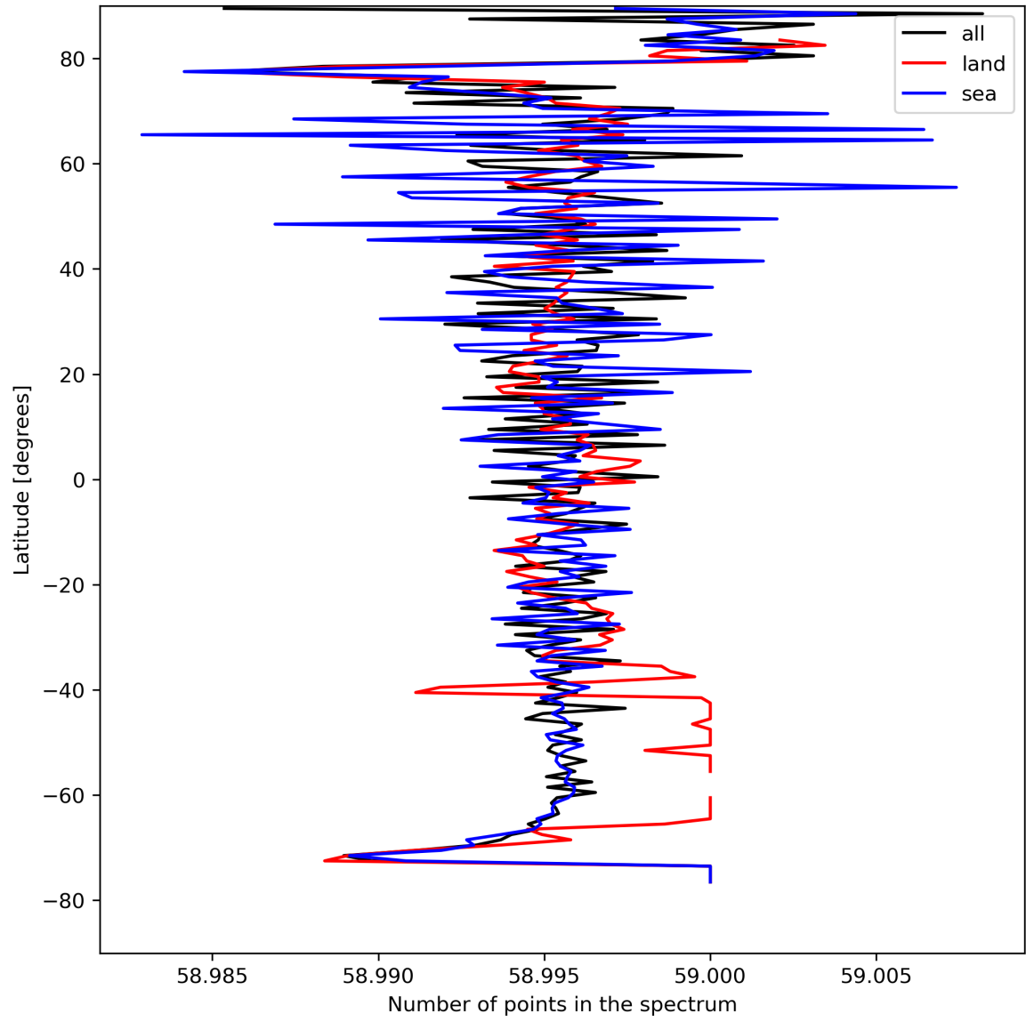
Figure 27: Zonal average of “Number of points in the spectrum” for 2023-08-22 to 2023-08-24.
