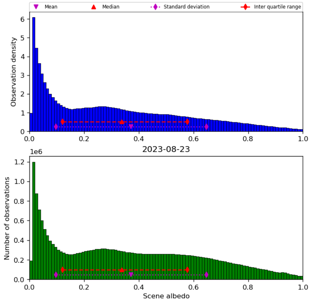
Figure 34: Histogram of “Scene albedo” for 2023-08-22 to 2023-08-24
