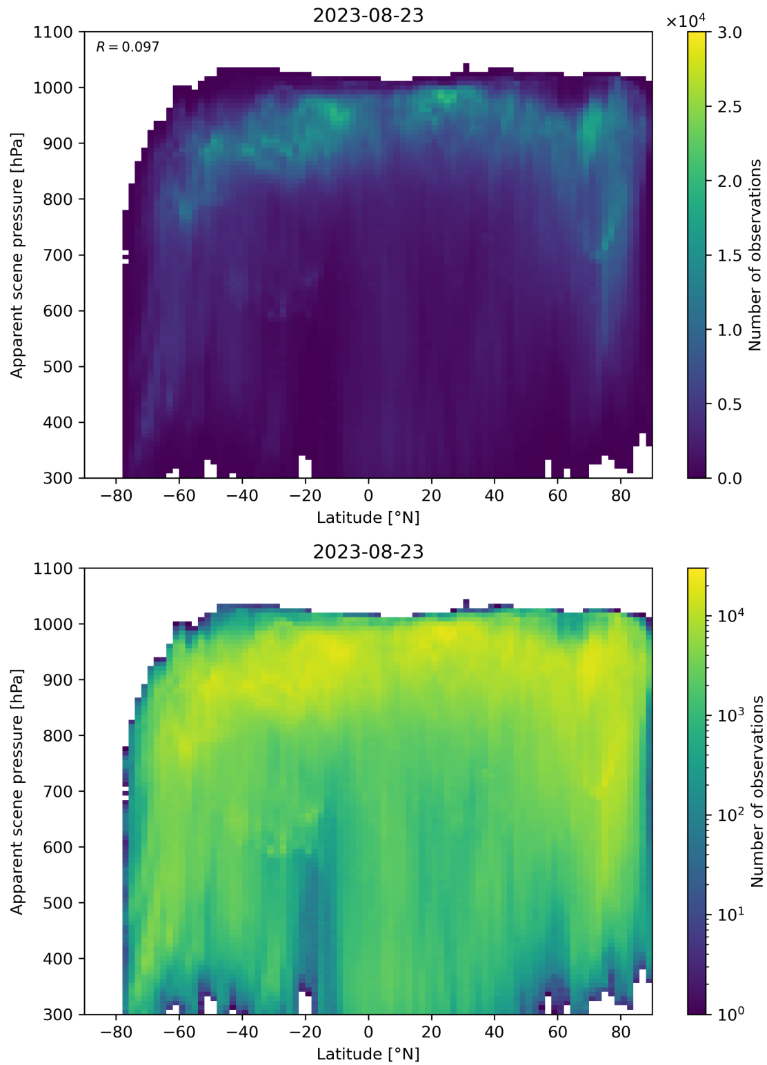
Figure 96: Scatter density plot of “Latitude” against “Apparent scene pressure” for 2023-08-22 to 2023-08-24.
