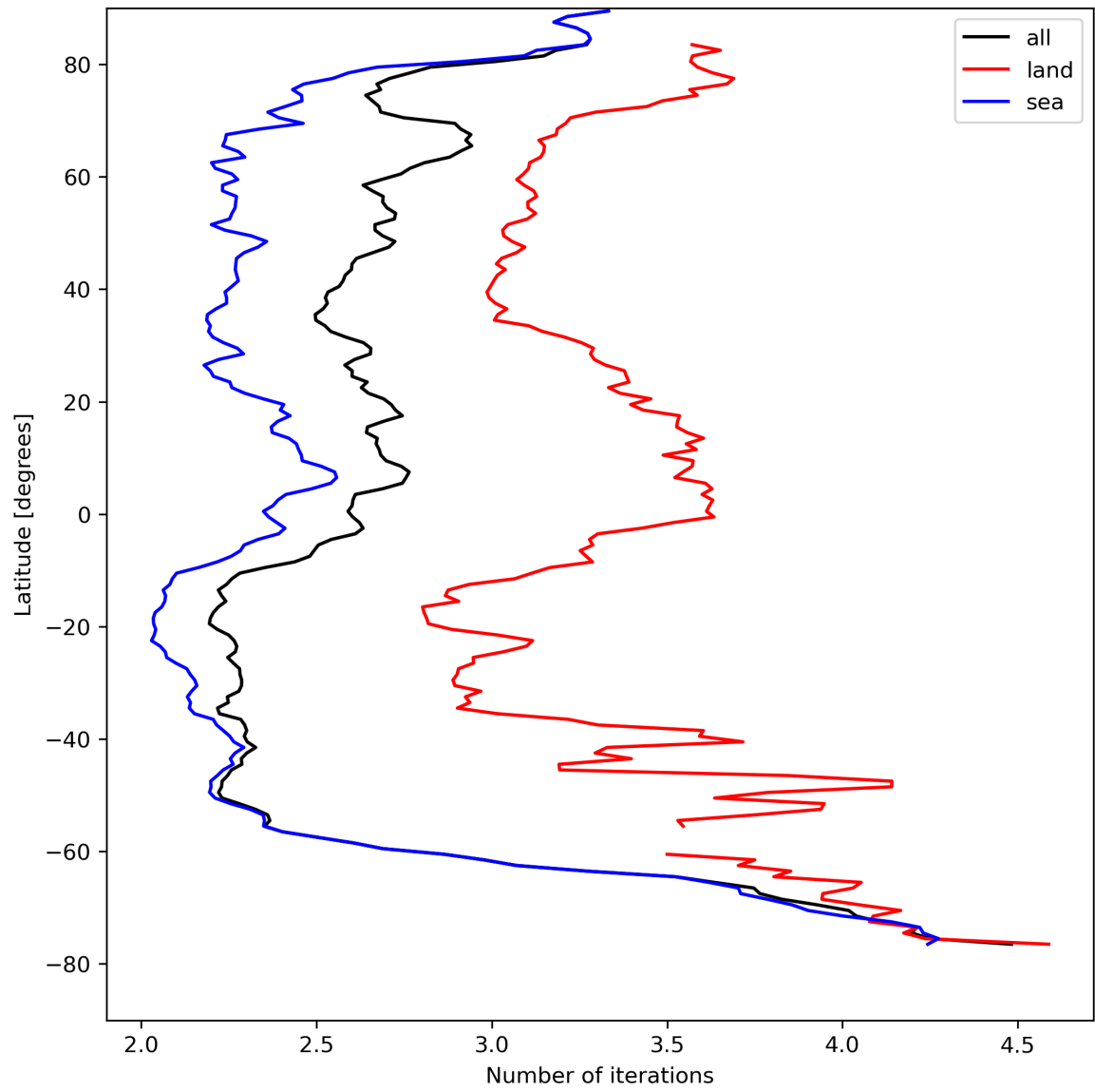
Figure 22: Zonal average of “Number of iterations” for 2023-08-22 to 2023-08-24.
