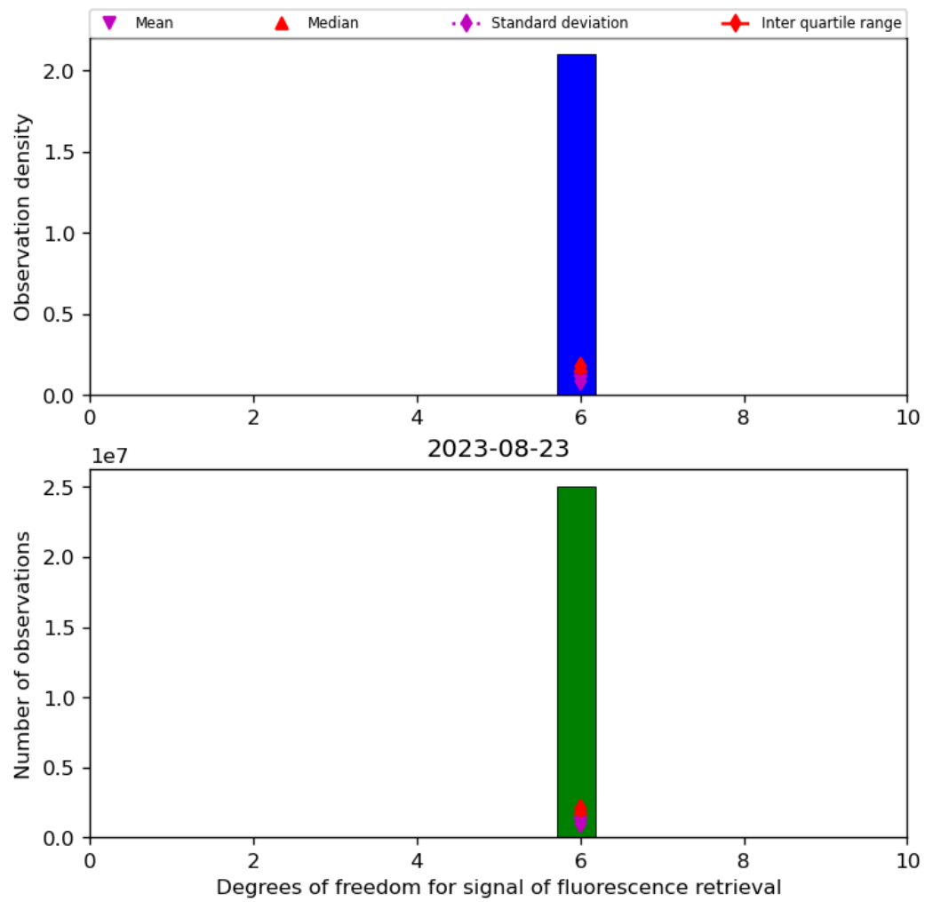
Figure 43: Histogram of “Degrees of freedom for signal of fluorescence retrieval” for 2023-08-22 to 2023-08-24
