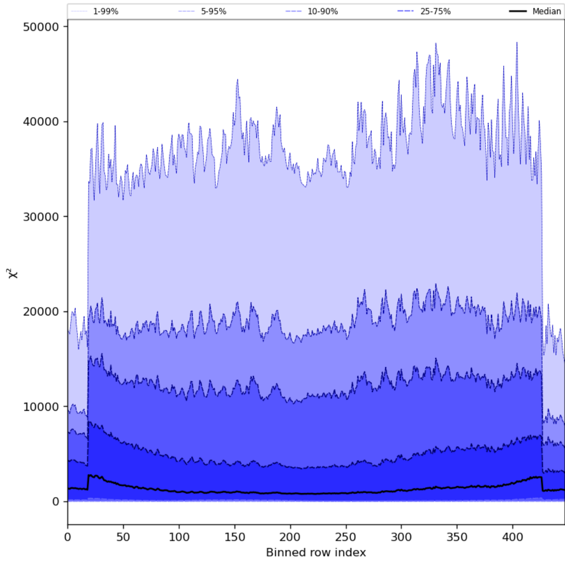
Figure 55: Along track statistics of “ \chi^2 ” for 2023-08-22 to 2023-08-24
