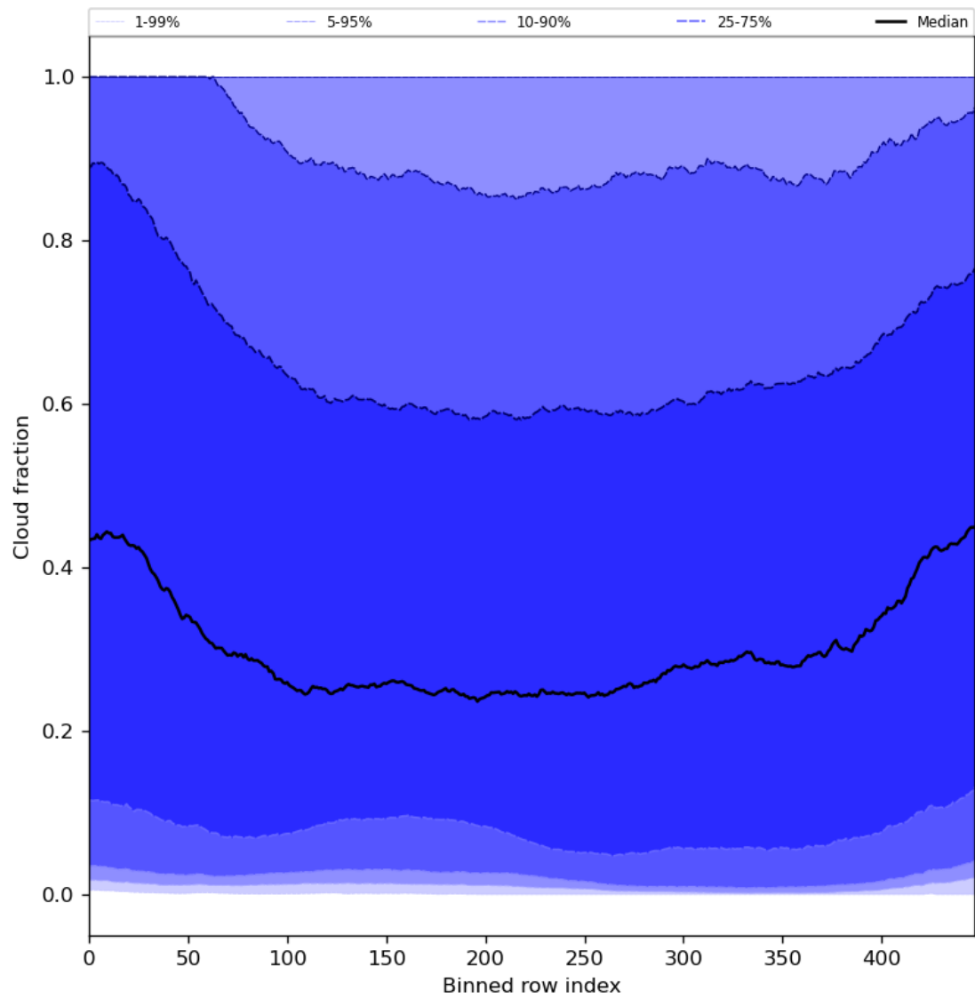
Figure 49: Along track statistics of “Cloud fraction” for 2023-08-22 to 2023-08-24
