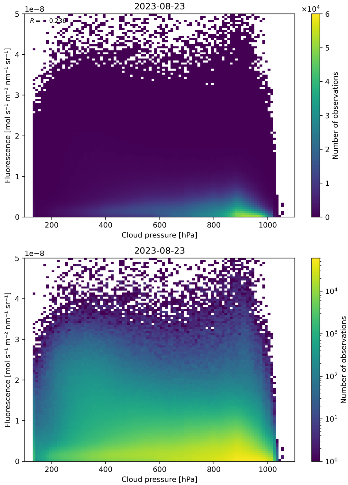
Figure 88: Scatter density plot of “Cloud pressure” against “Fluorescence” for 2023-08-22 to 2023-08-24.
