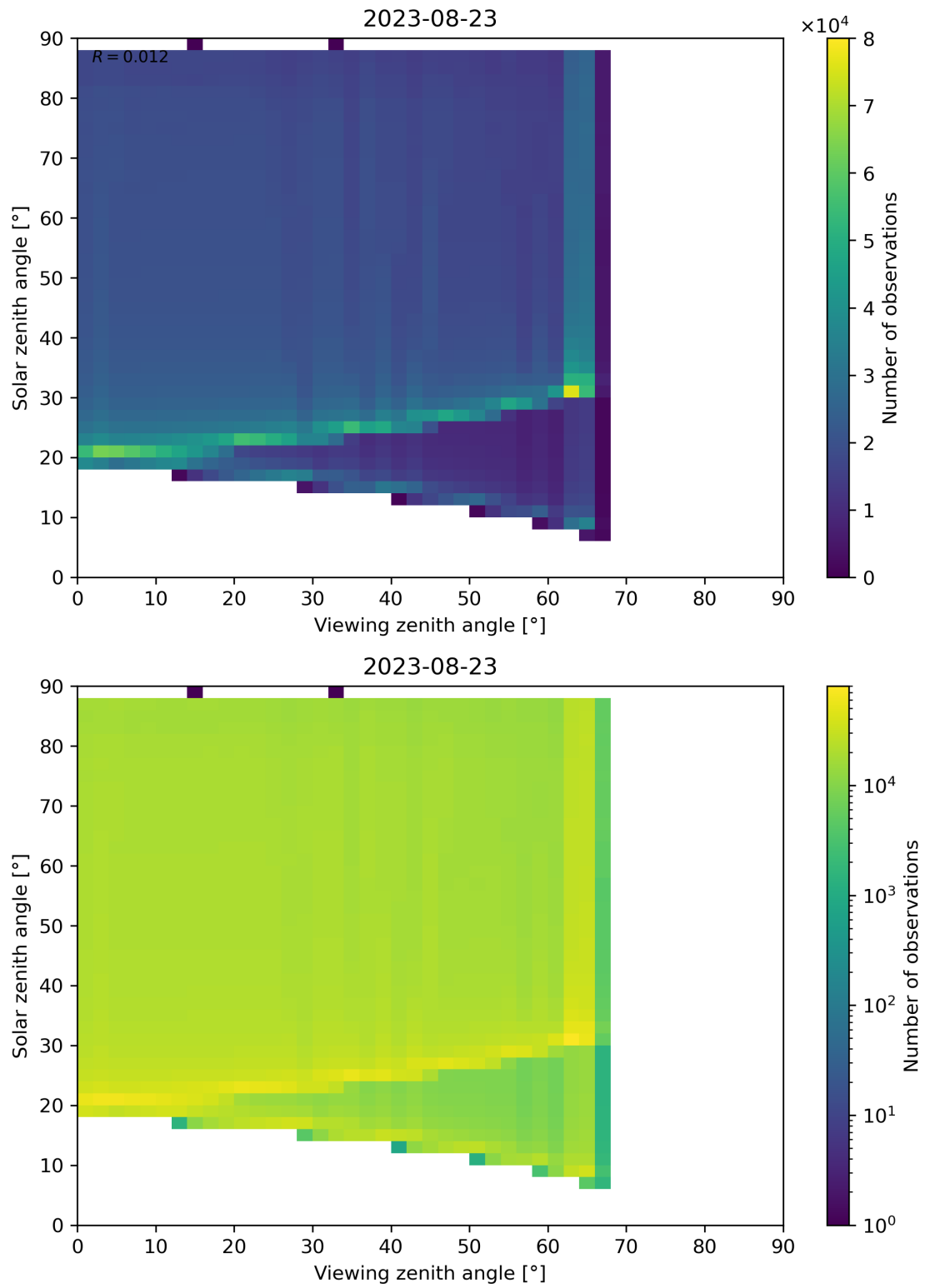
Figure 139: Scatter density plot of “Viewing zenith angle” against “Solar zenith angle” for 2023-08-22 to 2023-08-24.
