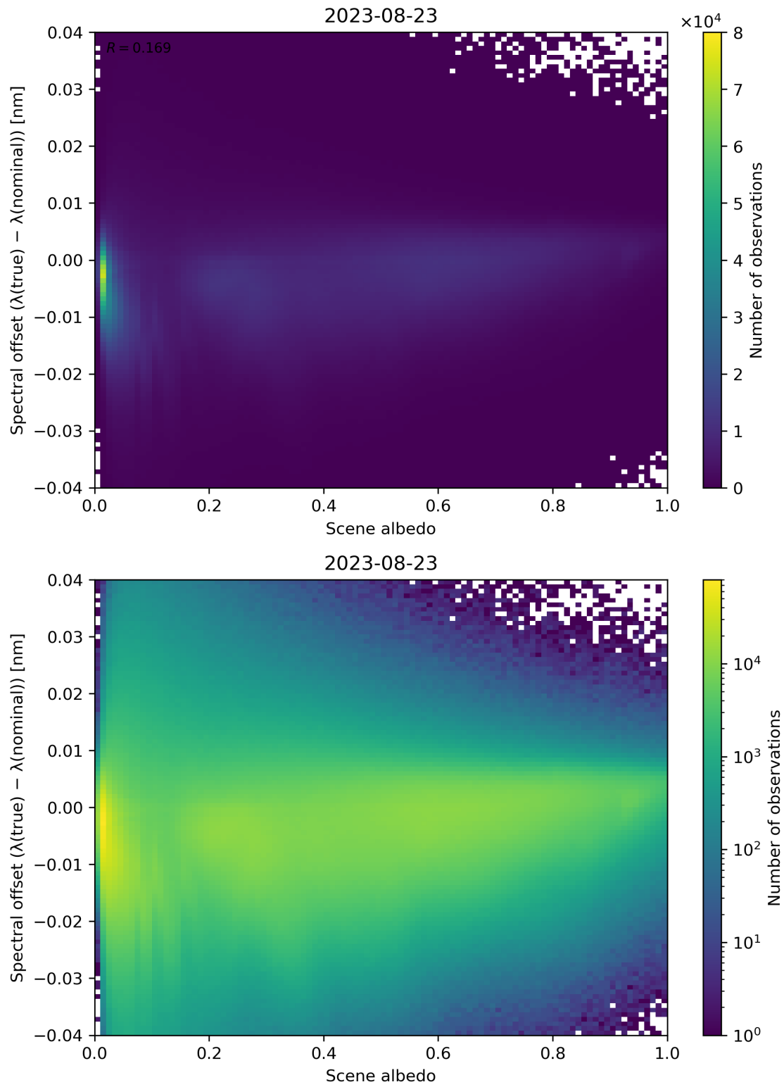
Figure 117: Scatter density plot of “Scene albedo” against “Spectral offset ( \lambda(\text{true}) - \lambda(\text{nominal}) )” for 2023-08-22 to 2023-08-24.
