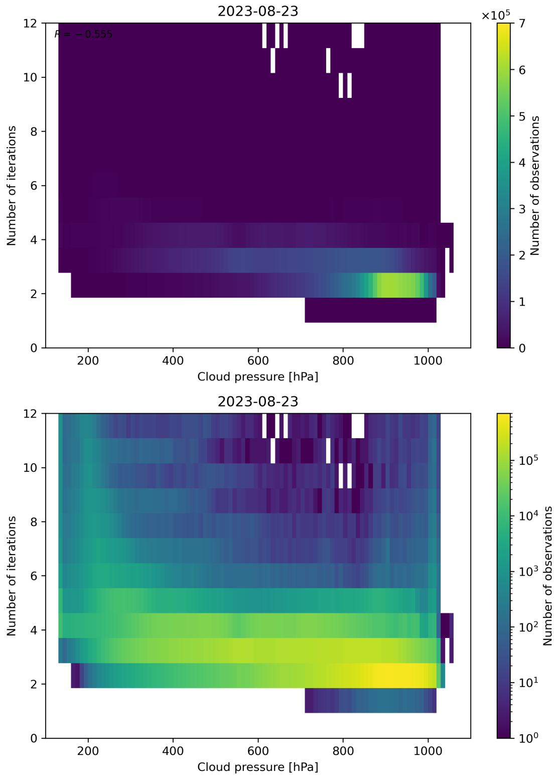
Figure 89: Scatter density plot of “Cloud pressure” against “Number of iterations” for 2023-08-22 to 2023-08-24.
