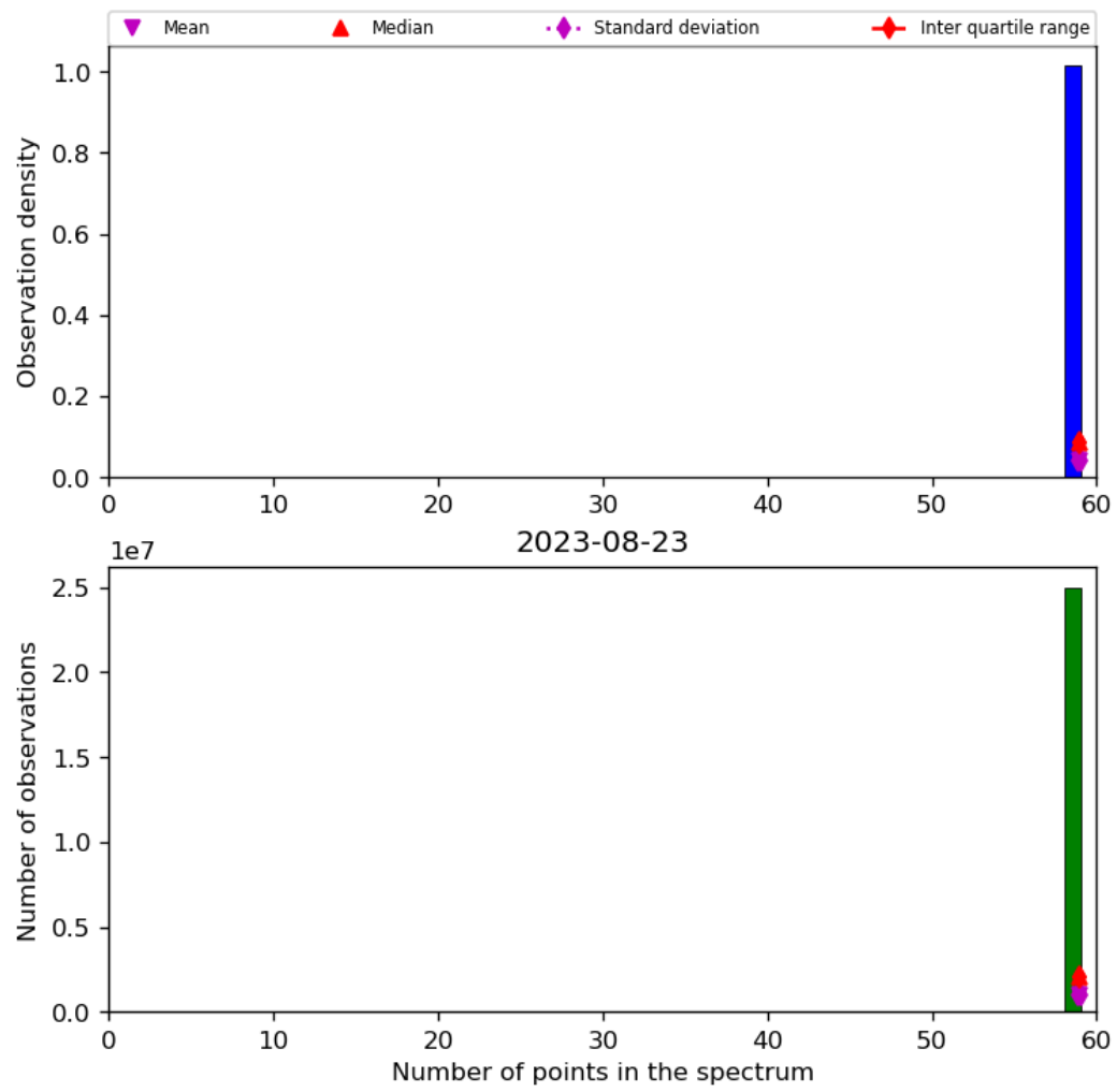
Figure 44: Histogram of “Number of points in the spectrum” for 2023-08-22 to 2023-08-24
