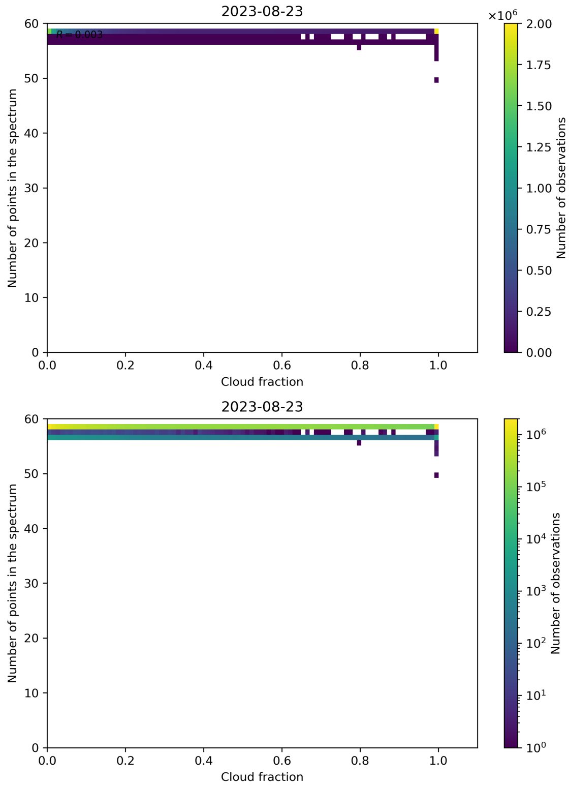
Figure 81: Scatter density plot of “Cloud fraction” against “Number of points in the spectrum” for 2023-08-22 to 2023-08-24.
