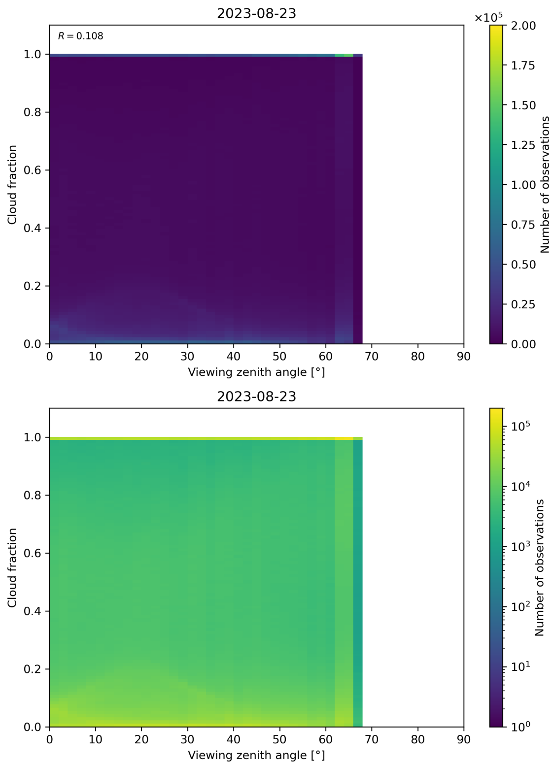
Figure 132: Scatter density plot of “Viewing zenith angle” against “Cloud fraction” for 2023-08-22 to 2023-08-24.
