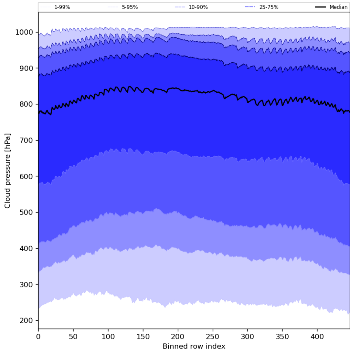
Figure 47: Along track statistics of “Cloud pressure” for 2023-08-22 to 2023-08-24
