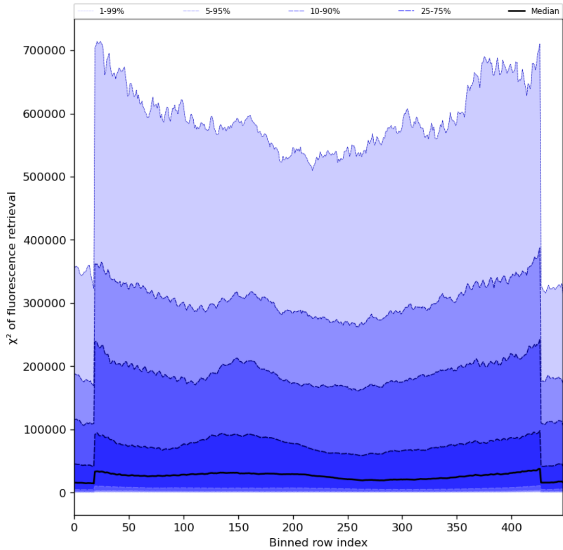
Figure 59: Along track statistics of “ \chi^2 of fluorescence retrieval” for 2023-08-22 to 2023-08-24
