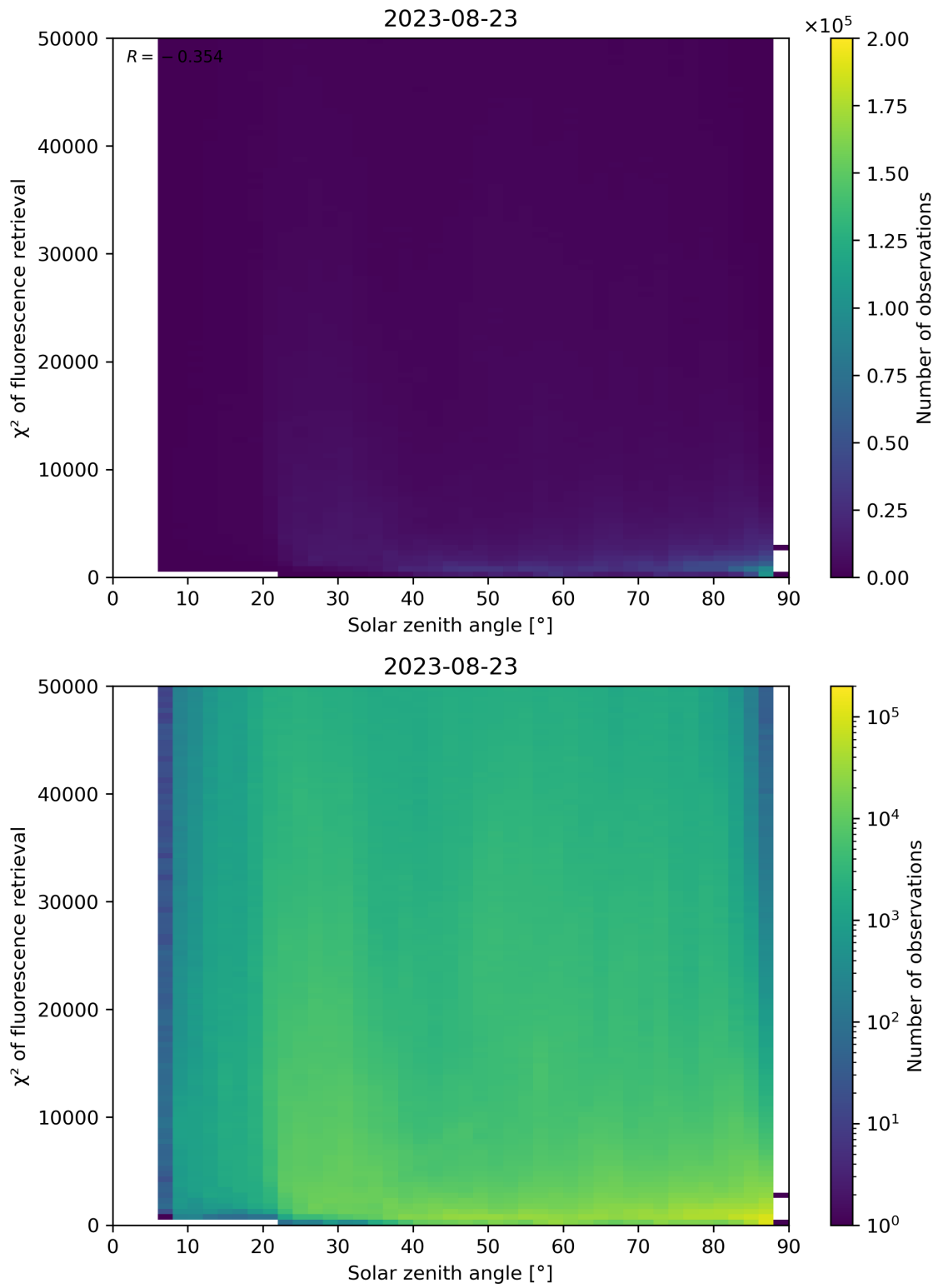
Figure 120: Scatter density plot of “Solar zenith angle” against “ \chi^2 of fluorescence retrieval” for 2023-08-22 to 2023-08-24.
