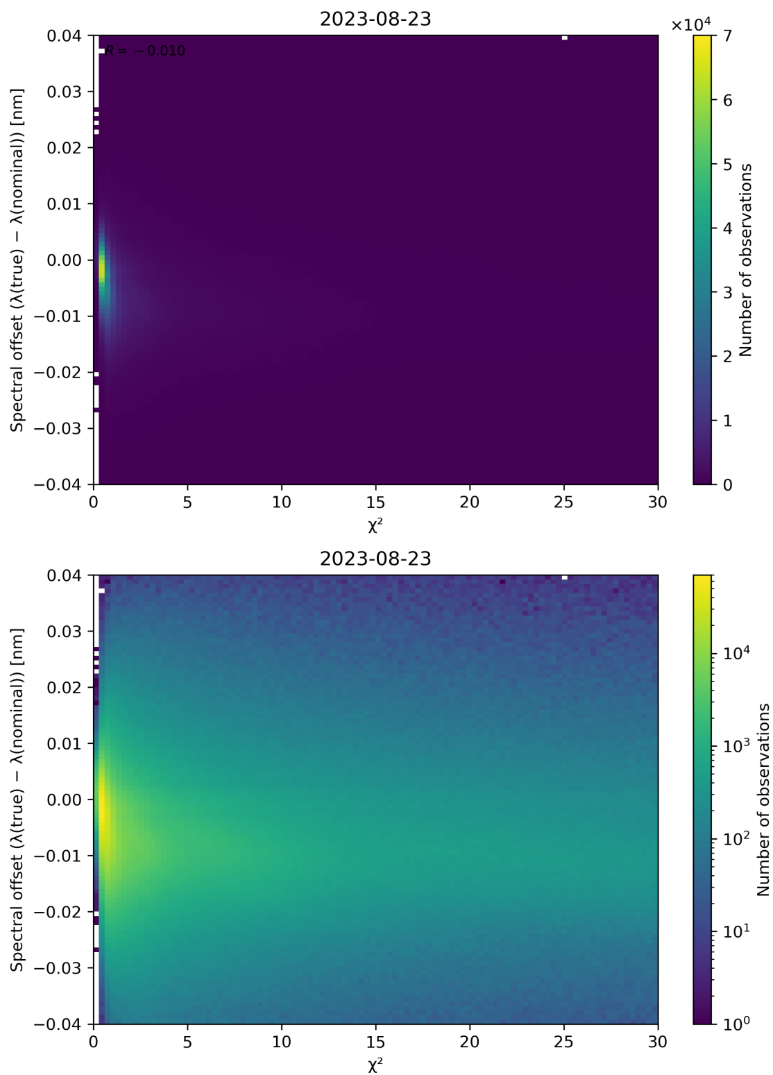
Figure 75: Scatter density plot of “ \chi^2 ” against “Spectral offset ( \lambda(\text{true}) - \lambda(\text{nominal}) )” for 2023-08-22 to 2023-08-24.
