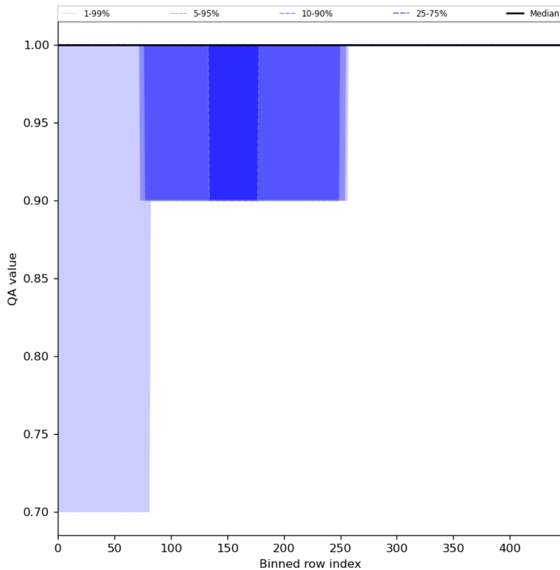
Figure 46: Along track statistics of “QA value” for 2023-08-22 to 2023-08-24
