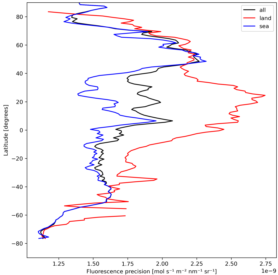
Figure 24: Zonal average of “Fluorescence precision” for 2023-08-22 to 2023-08-24.
