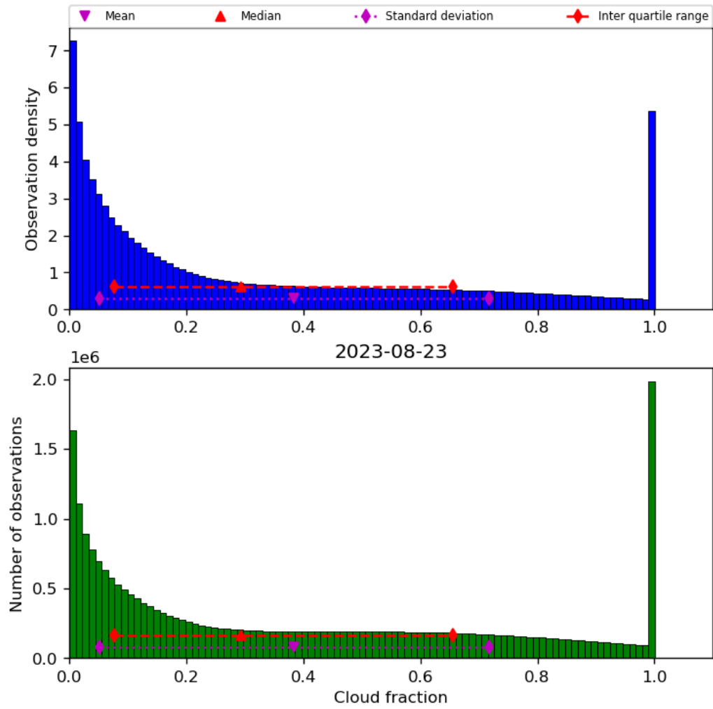
Figure 32: Histogram of “Cloud fraction” for 2023-08-22 to 2023-08-24
