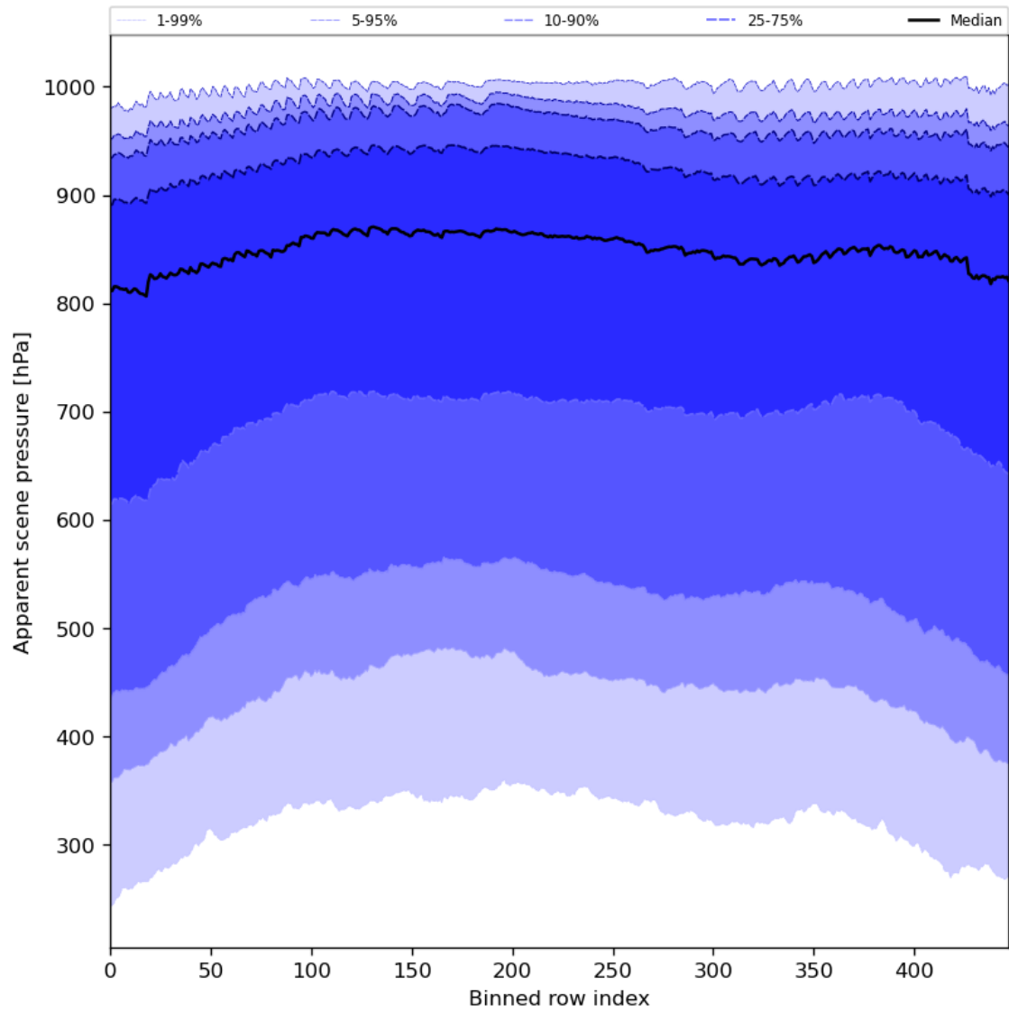
Figure 53: Along track statistics of “Apparent scene pressure” for 2023-08-22 to 2023-08-24
