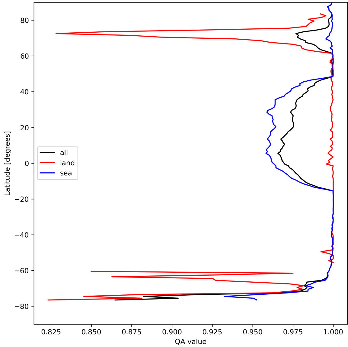
Figure 12: Zonal average of "QA value" for 2023-08-22 to 2023-08-24.
