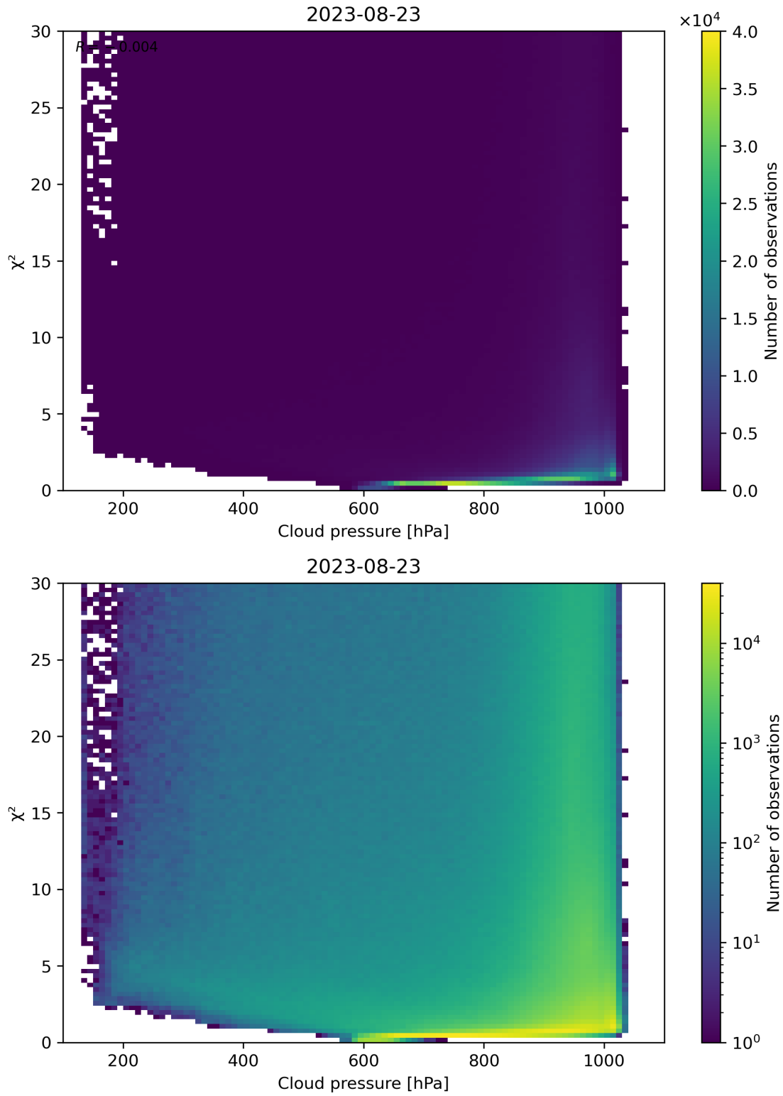
Figure 85: Scatter density plot of “Cloud pressure” against “ \chi^2 ” for 2023-08-22 to 2023-08-24.
