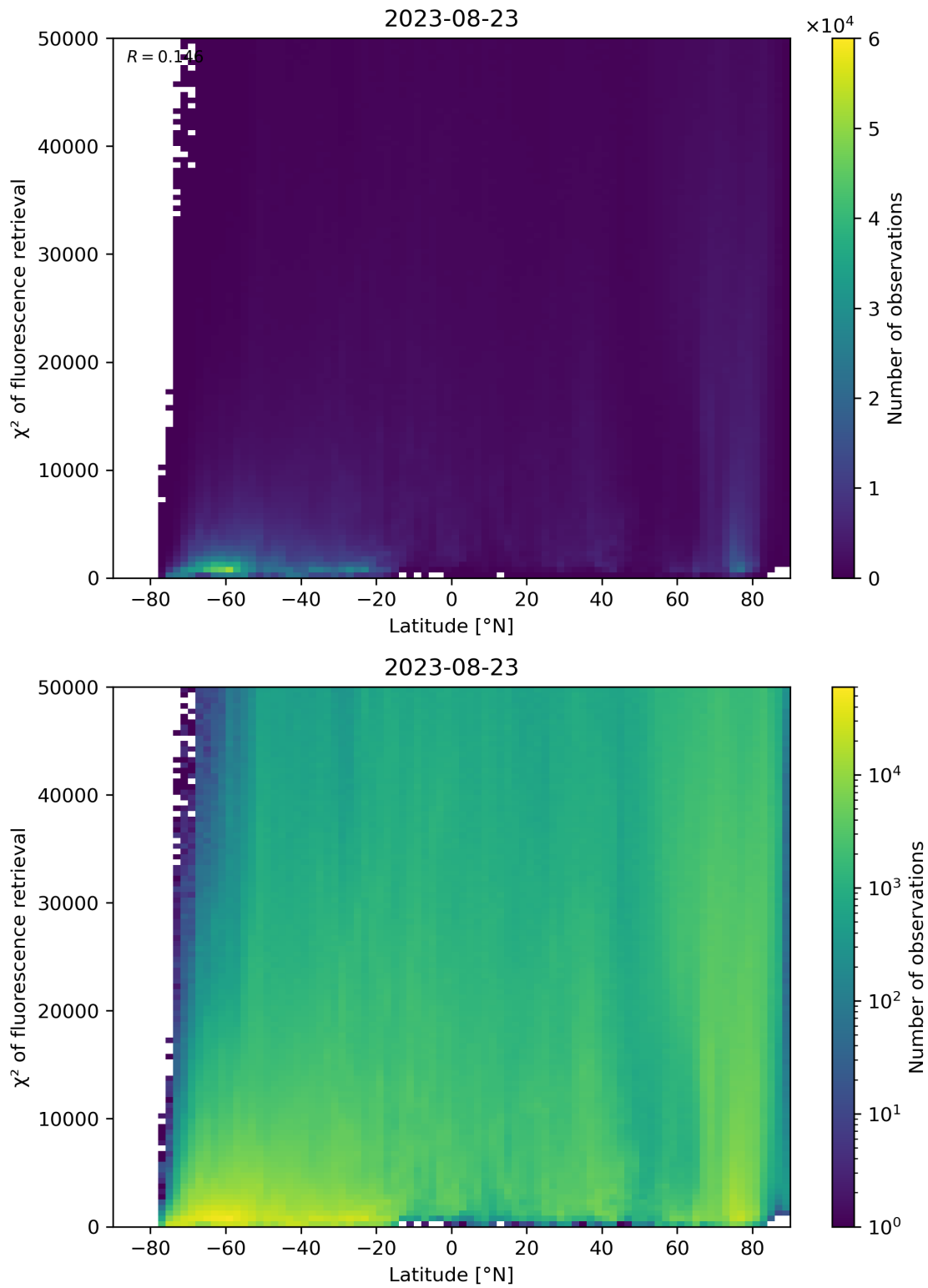
Figure 98: Scatter density plot of “Latitude” against “ \chi^2 of fluorescence retrieval” for 2023-08-22 to 2023-08-24.
