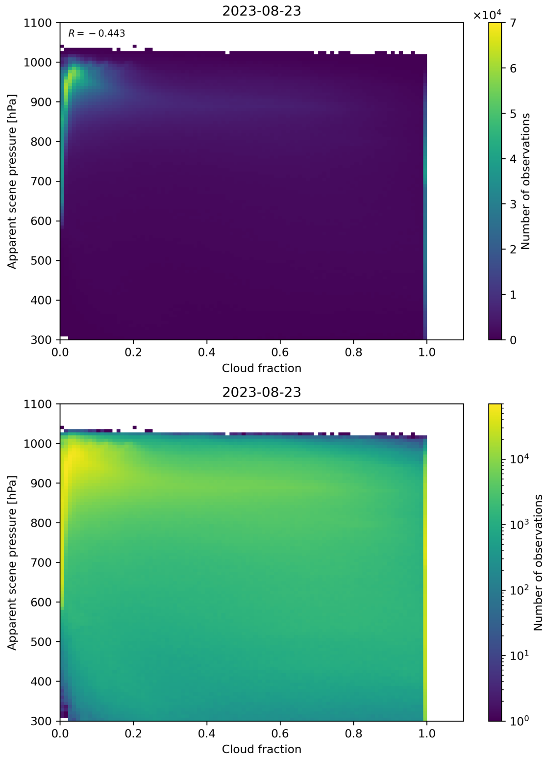
Figure 76: Scatter density plot of “Cloud fraction” against “Apparent scene pressure” for 2023-08-22 to 2023-08-24.
