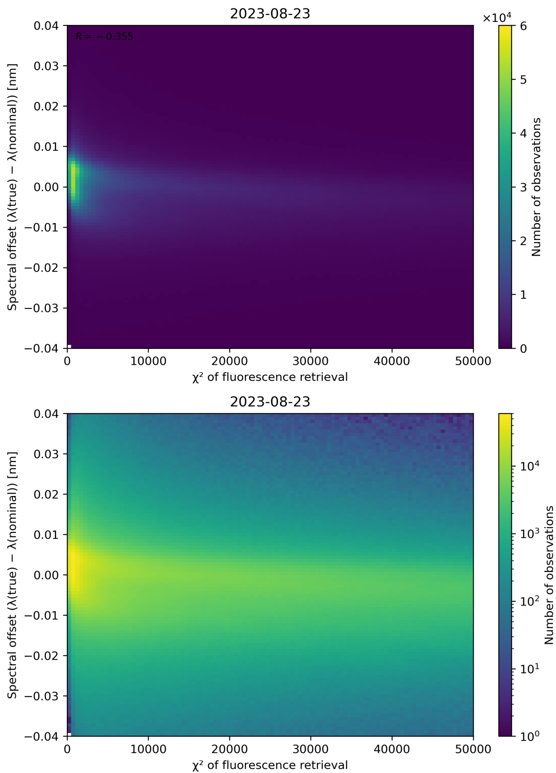
Figure 72: Scatter density plot of " \chi^2 of fluorescence retrieval" against "Spectral offset ( \lambda(\text{true}) - \lambda(\text{nominal}) )" for 2023-08-22 to 2023-08-24.
