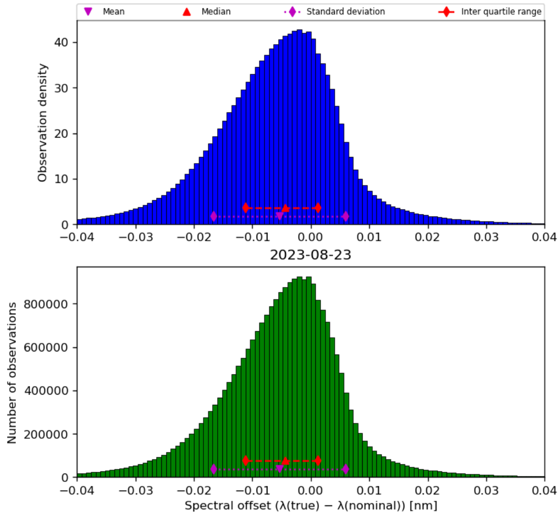
Figure 45: Histogram of “Spectral offset ( \lambda(\text{true}) - \lambda(\text{nominal}) )” for 2023-08-22 to 2023-08-24
