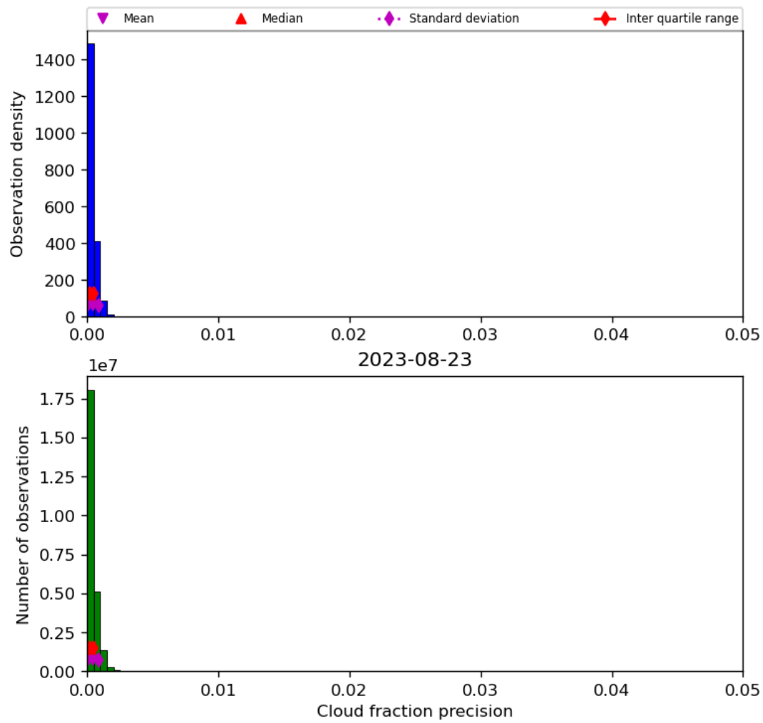
Figure 33: Histogram of “Cloud fraction precision” for 2023-08-22 to 2023-08-24
