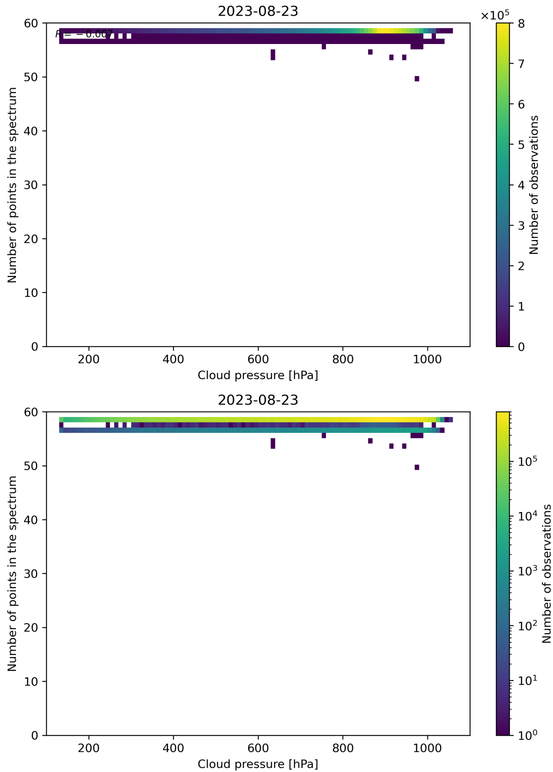
Figure 90: Scatter density plot of “Cloud pressure” against “Number of points in the spectrum” for 2023-08-22 to 2023-08-24.
