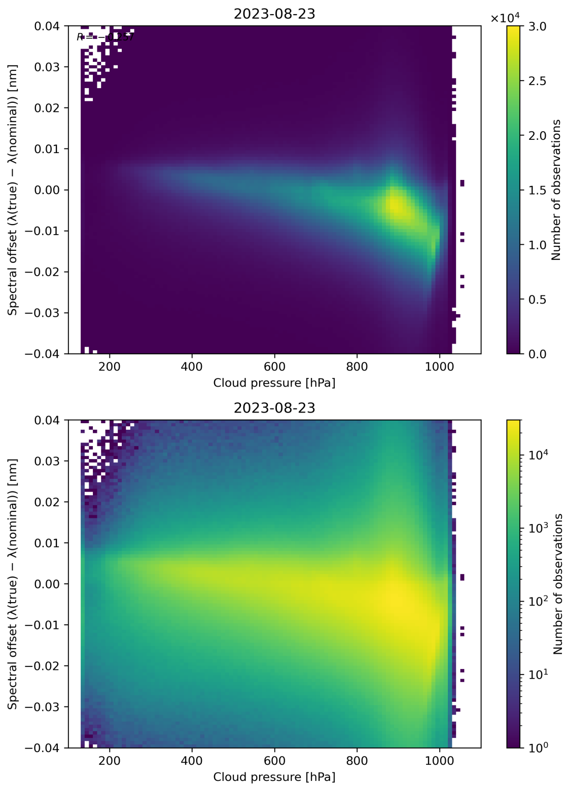
Figure 92: Scatter density plot of “Cloud pressure” against “Spectral offset ( \lambda(\text{true}) - \lambda(\text{nominal}) )” for 2023-08-22 to 2023-08-24.
