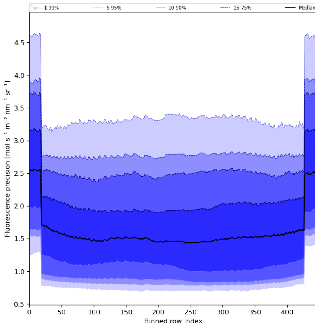
Figure 58: Along track statistics of “Fluorescence precision” for 2023-08-22 to 2023-08-24
