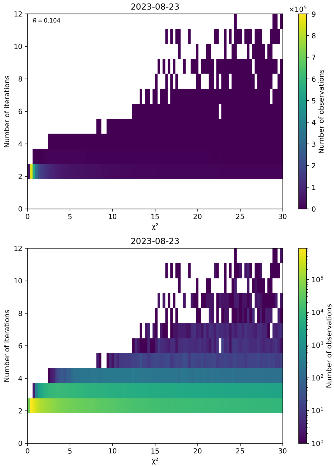
Figure 73: Scatter density plot of “ \chi^2 ” against “Number of iterations” for 2023-08-22 to 2023-08-24.
