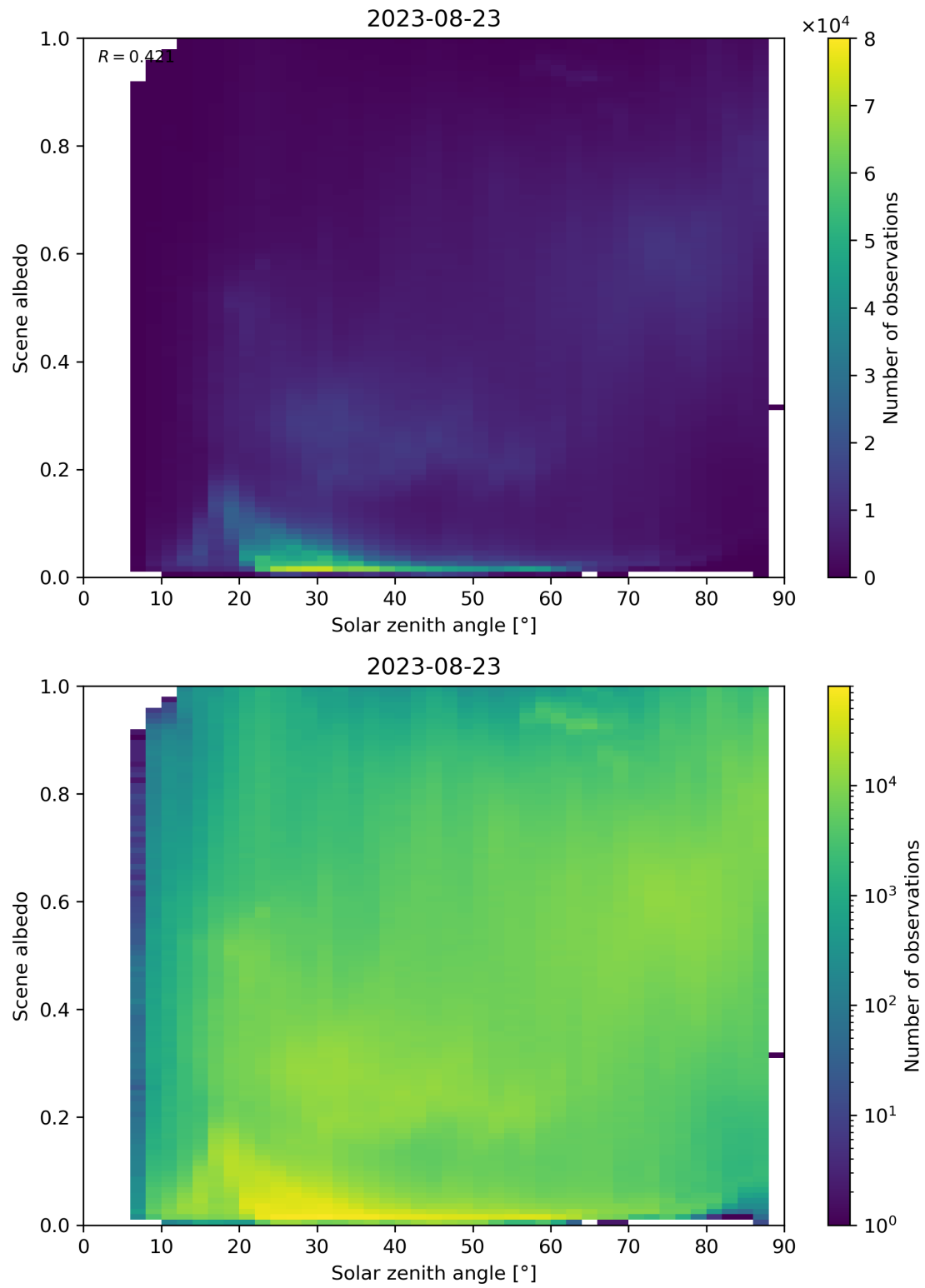
Figure 127: Scatter density plot of “Solar zenith angle” against “Scene albedo” for 2023-08-22 to 2023-08-24.
