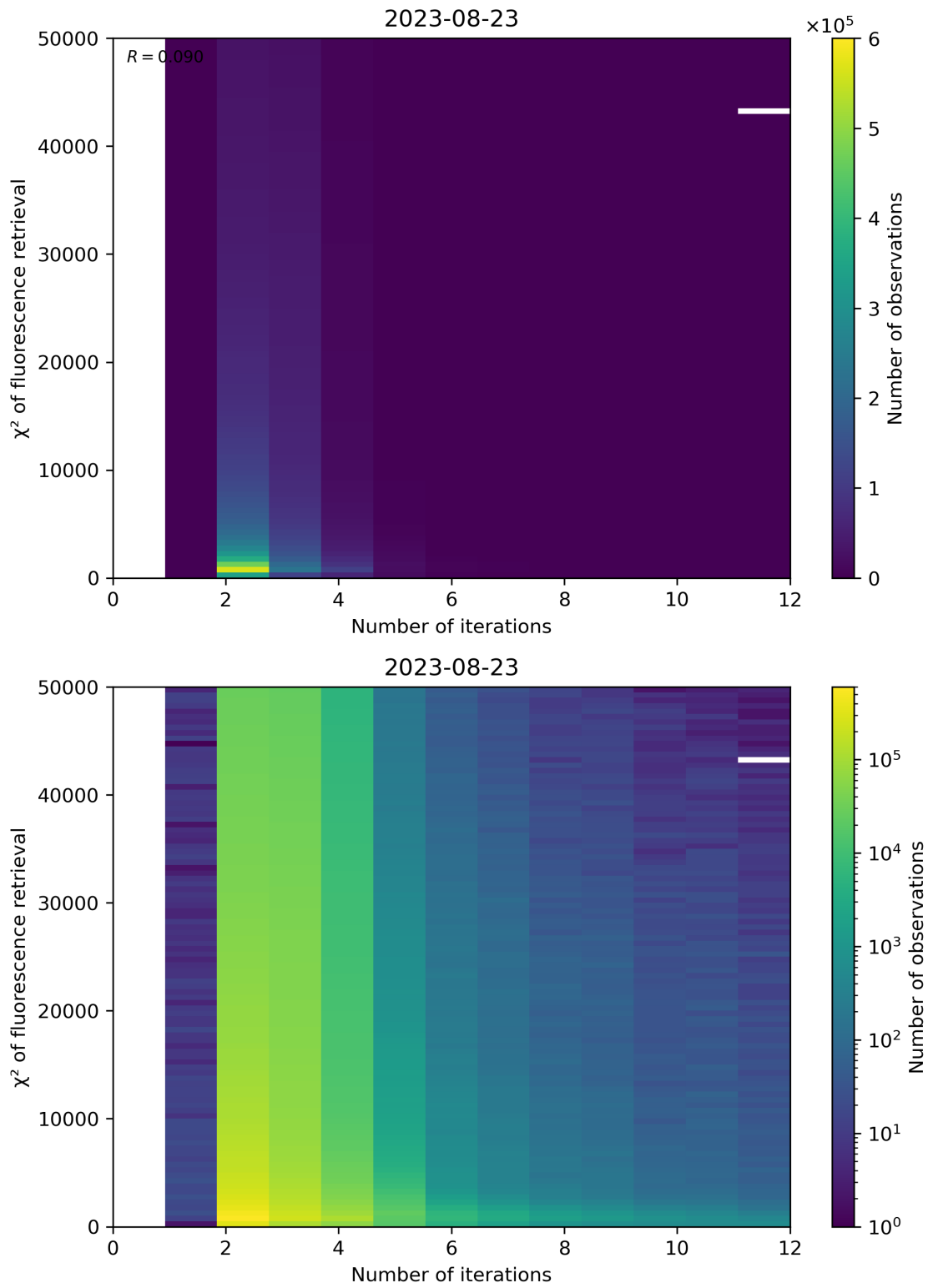
Figure 106: Scatter density plot of “Number of iterations” against “ \chi^2 of fluorescence retrieval” for 2023-08-22 to 2023-08-24.
