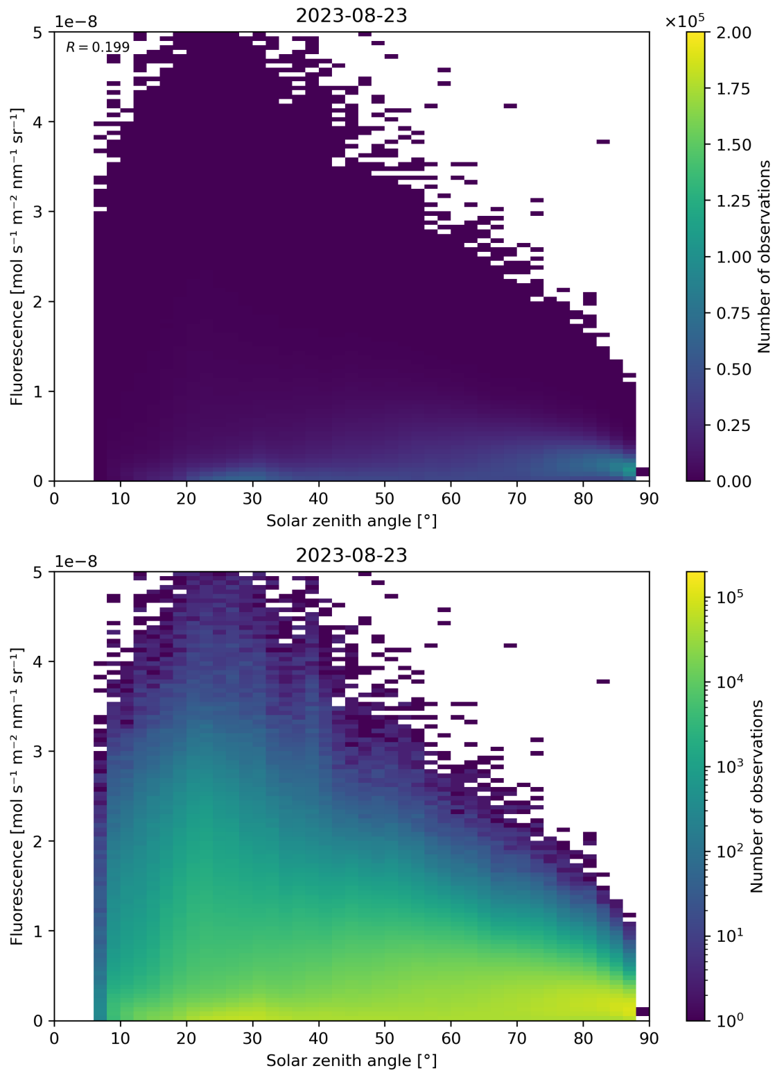
Figure 123: Scatter density plot of “Solar zenith angle” against “Fluorescence” for 2023-08-22 to 2023-08-24.
