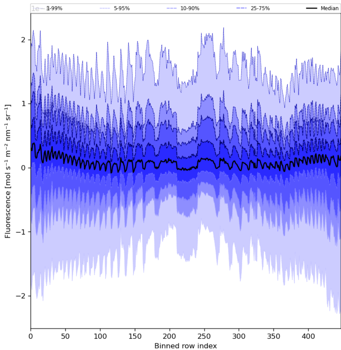
Figure 57: Along track statistics of “Fluorescence” for 2023-08-22 to 2023-08-24
