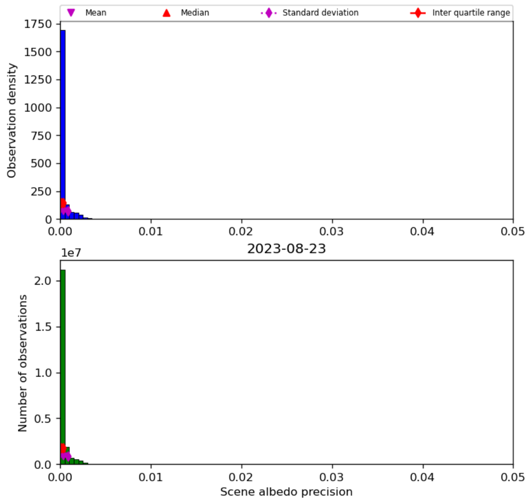
Figure 35: Histogram of “Scene albedo precision” for 2023-08-22 to 2023-08-24
