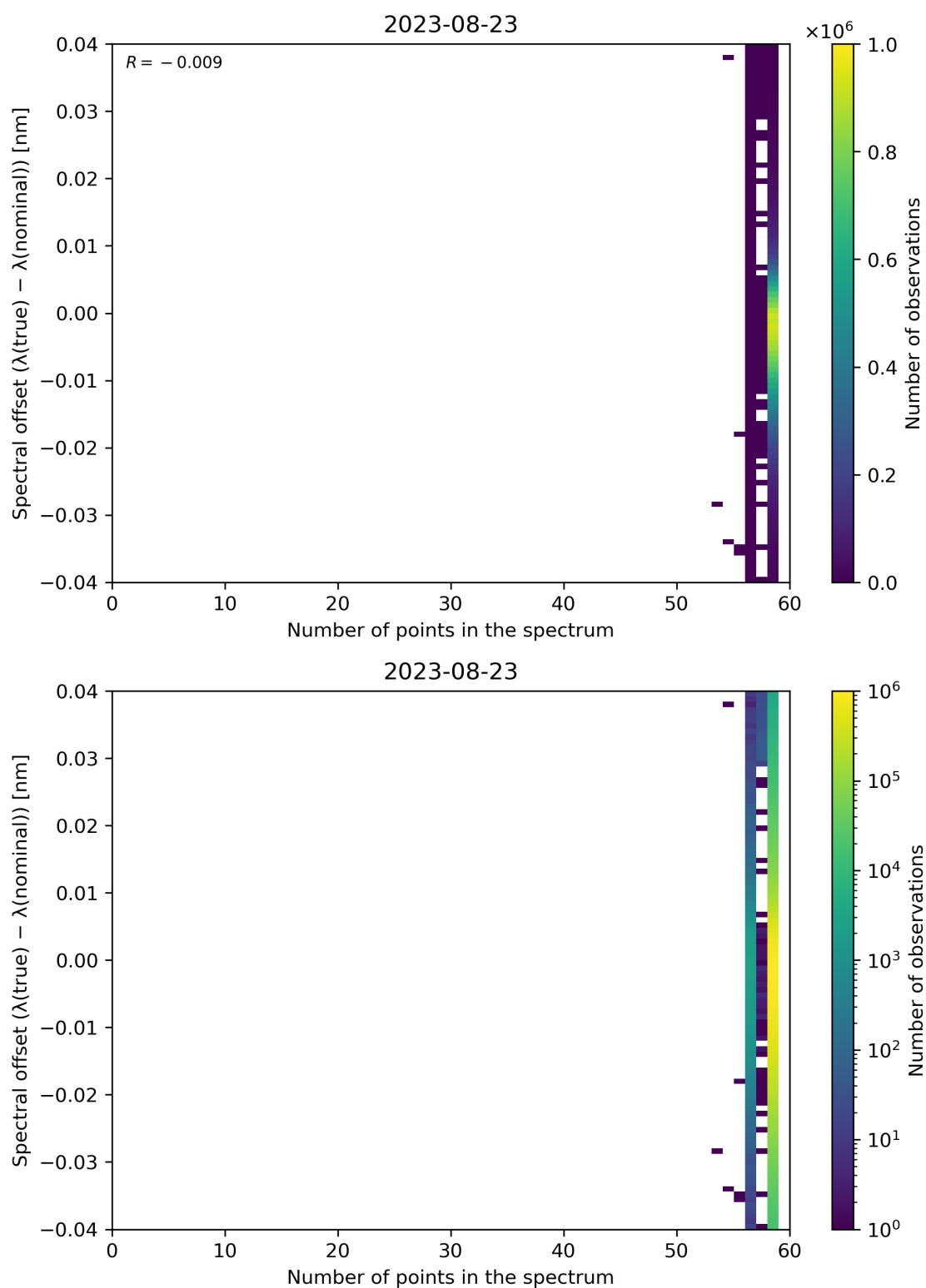
Figure 110: Scatter density plot of “Number of points in the spectrum” against “Spectral offset ( \lambda(\text{true}) - \lambda(\text{nominal}) )” for 2023-08-22 to 2023-08-24.
