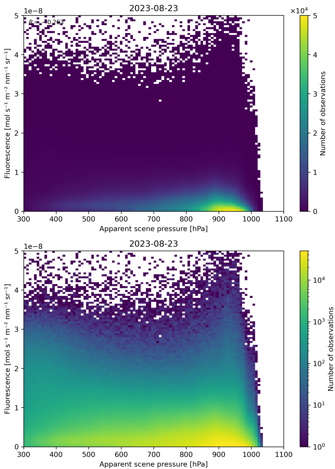
Figure 65: Scatter density plot of “Apparent scene pressure” against “Fluorescence” for 2023-08-22 to 2023-08-24.
