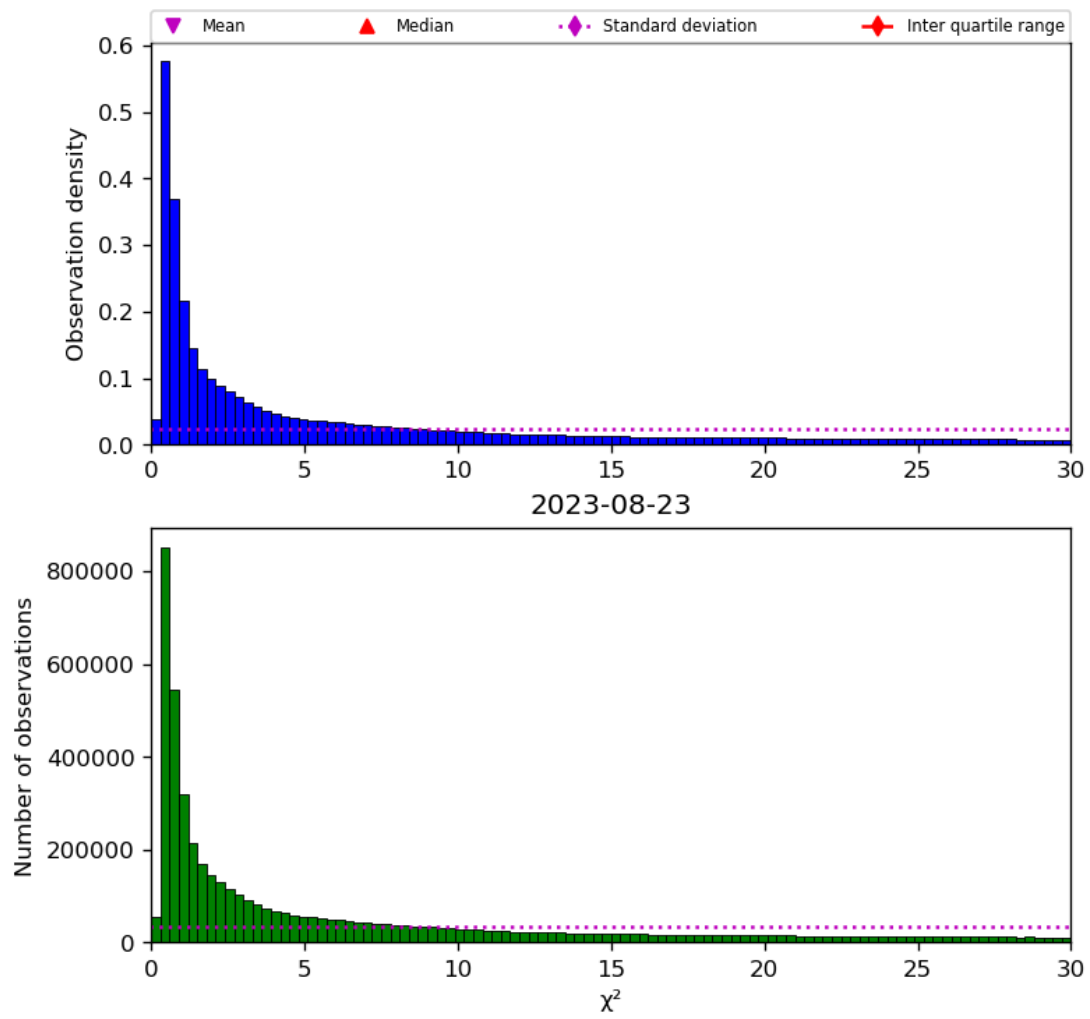
Figure 38: Histogram of “ \chi^2 ” for 2023-08-22 to 2023-08-24
