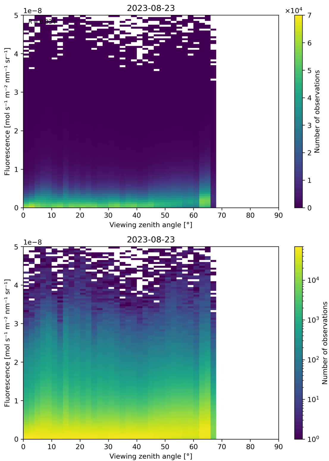
Figure 134: Scatter density plot of “Viewing zenith angle” against “Fluorescence” for 2023-08-22 to 2023-08-24.
