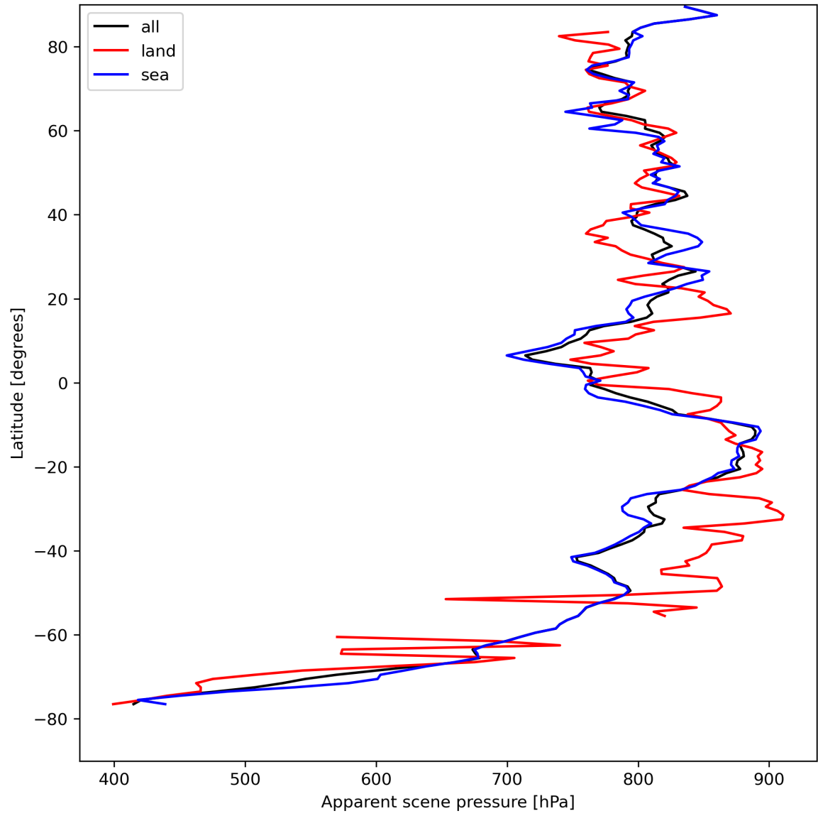
Figure 19: Zonal average of “Apparent scene pressure” for 2023-08-22 to 2023-08-24.
