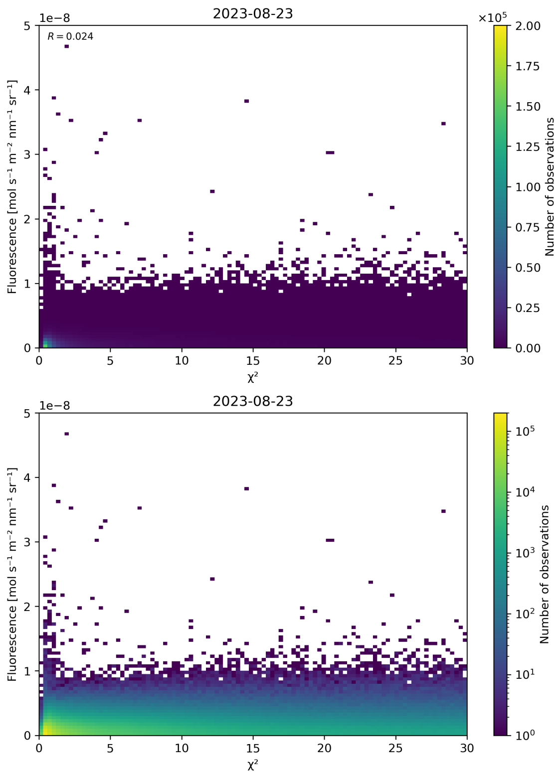
Figure 70: Scatter density plot of “ \chi^2 ” against “Fluorescence” for 2023-08-22 to 2023-08-24.
