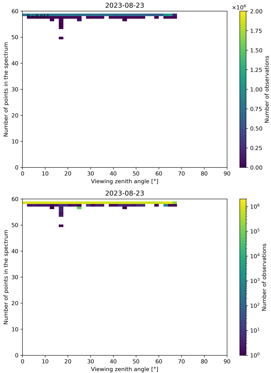
Figure 137: Scatter density plot of “Viewing zenith angle” against “Number of points in the spectrum” for 2023-08-22 to 2023-08-24.
