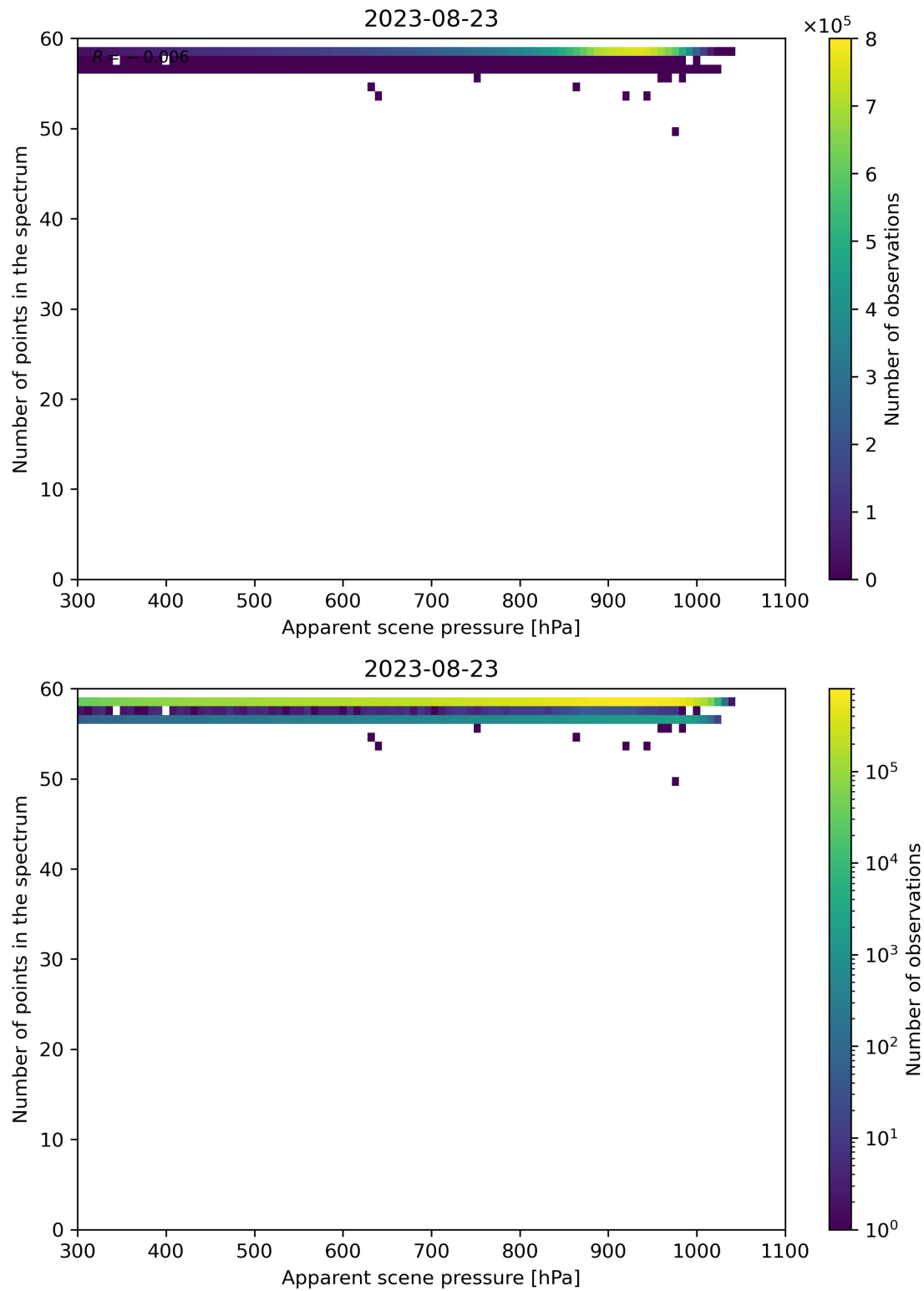
Figure 67: Scatter density plot of “Apparent scene pressure” against “Number of points in the spectrum” for 2023-08-22 to 2023-08-24.
