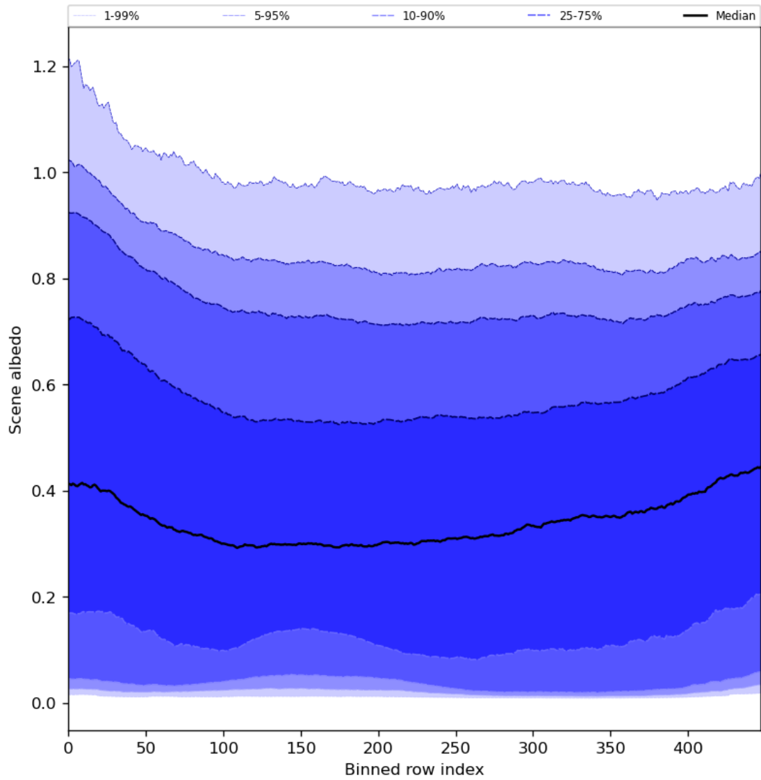
Figure 51: Along track statistics of “Scene albedo” for 2023-08-22 to 2023-08-24
