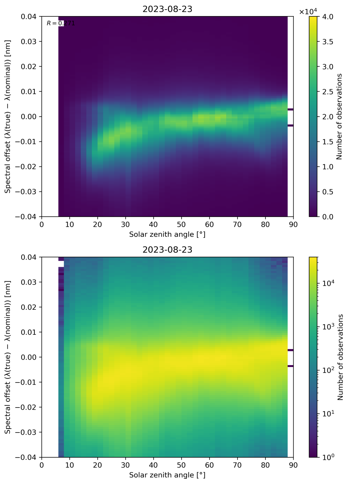
Figure 128: Scatter density plot of “Solar zenith angle” against “Spectral offset ( \lambda(\text{true}) - \lambda(\text{nominal}) )” for 2023-08-22 to 2023-08-24.
