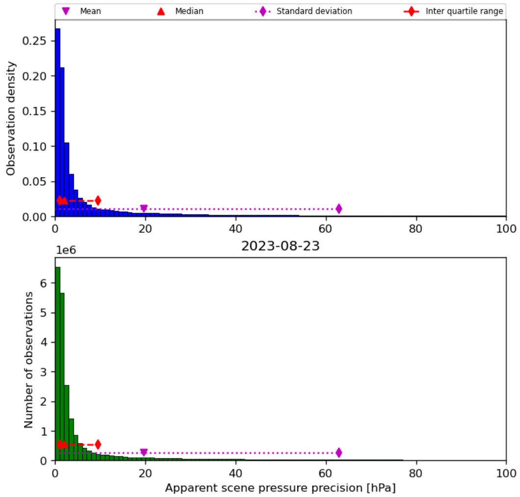
Figure 37: Histogram of “Apparent scene pressure precision” for 2023-08-22 to 2023-08-24
