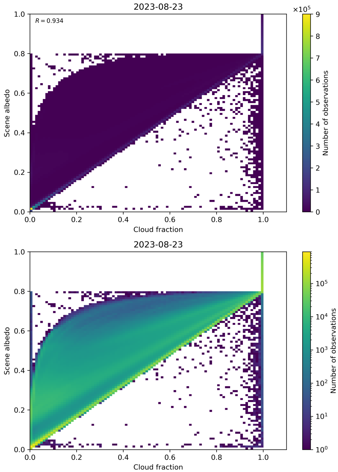
Figure 82: Scatter density plot of “Cloud fraction” against “Scene albedo” for 2023-08-22 to 2023-08-24.
