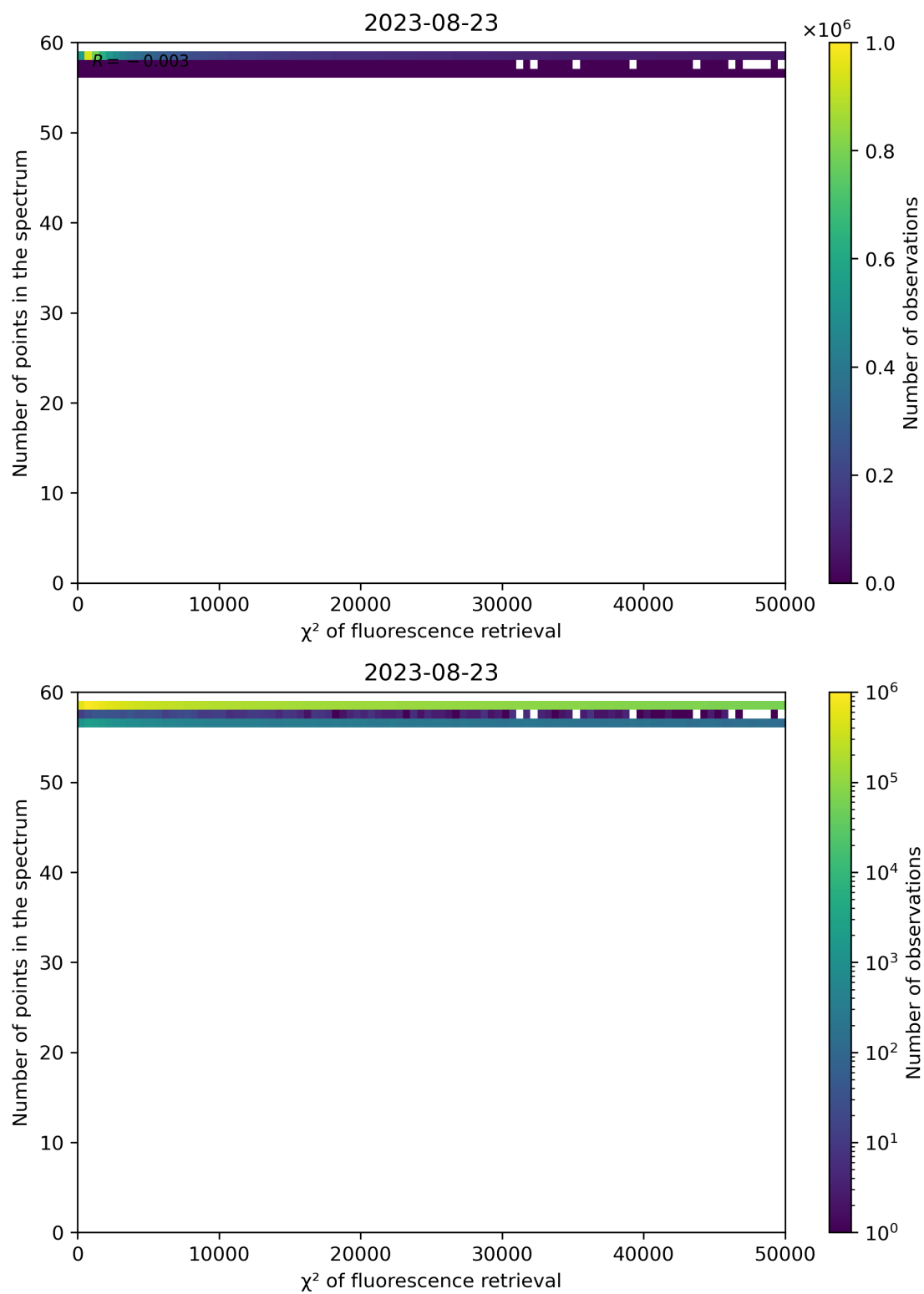
Figure 71: Scatter density plot of " \chi^2 of fluorescence retrieval" against "Number of points in the spectrum" for 2023-08-22 to 2023-08-24.
