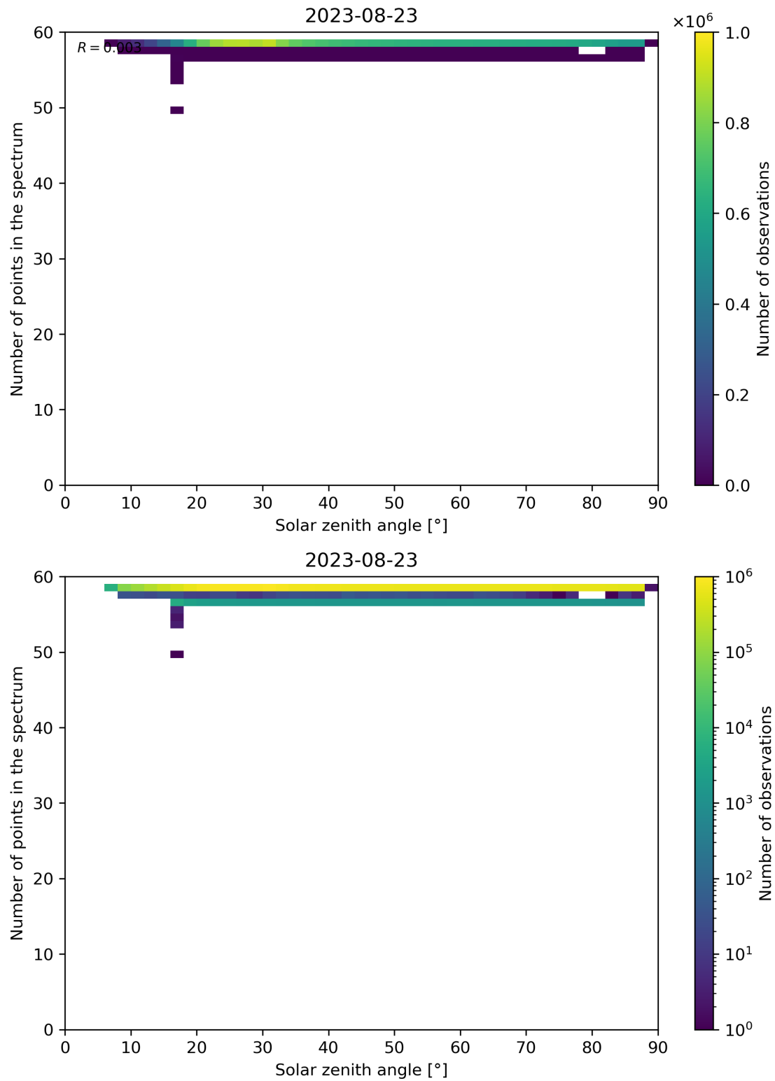
Figure 126: Scatter density plot of “Solar zenith angle” against “Number of points in the spectrum” for 2023-08-22 to 2023-08-24.
