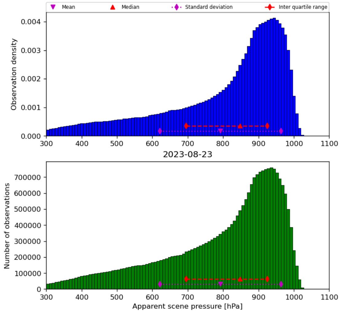
Figure 36: Histogram of “Apparent scene pressure” for 2023-08-22 to 2023-08-24
