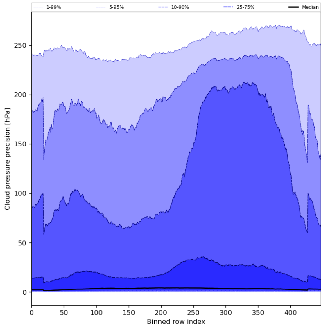
Figure 48: Along track statistics of “Cloud pressure precision” for 2023-08-22 to 2023-08-24
