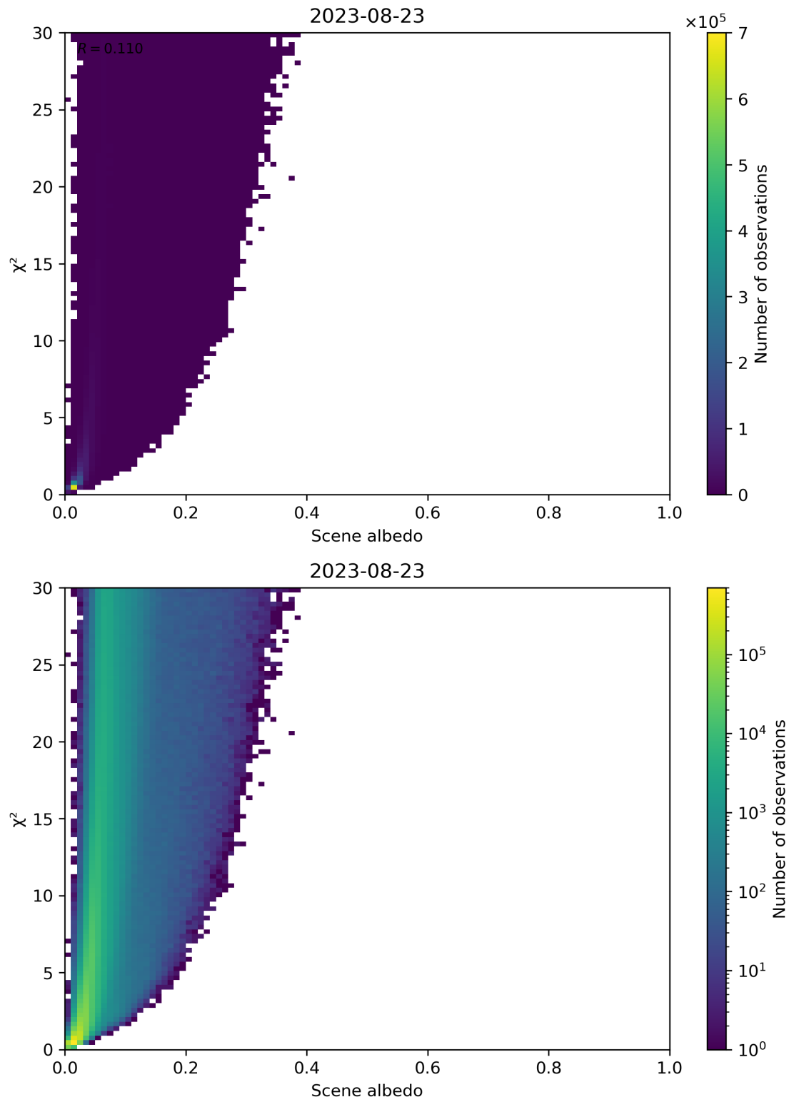
Figure 112: Scatter density plot of “Scene albedo” against “ \chi^2 ” for 2023-08-22 to 2023-08-24.
