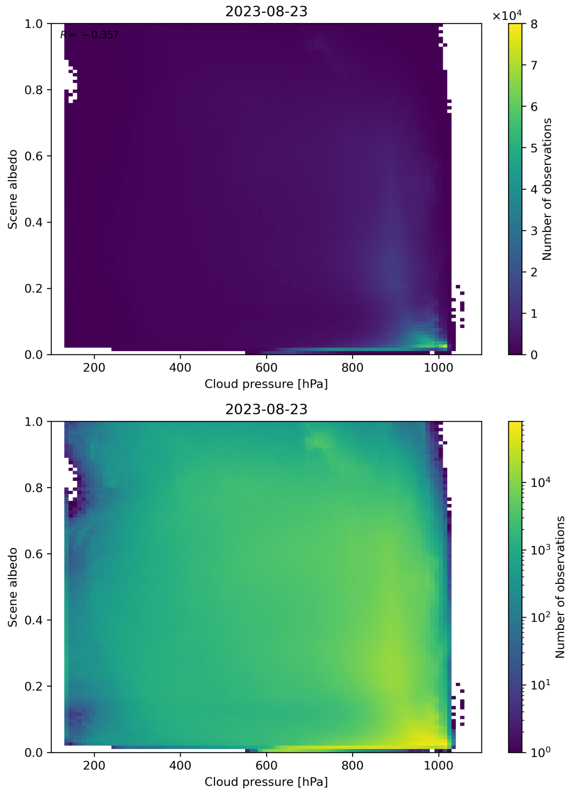
Figure 91: Scatter density plot of “Cloud pressure” against “Scene albedo” for 2023-08-22 to 2023-08-24.
