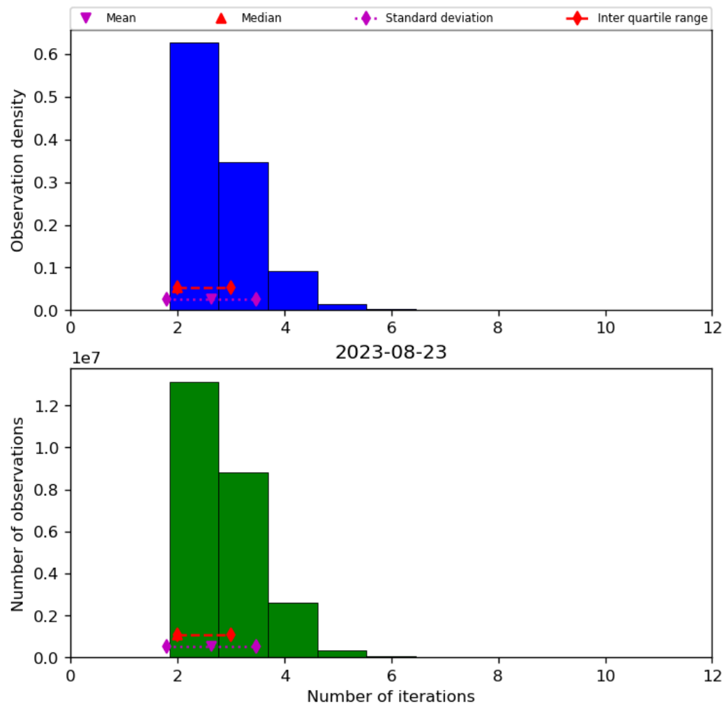
Figure 39: Histogram of “Number of iterations” for 2023-08-22 to 2023-08-24
