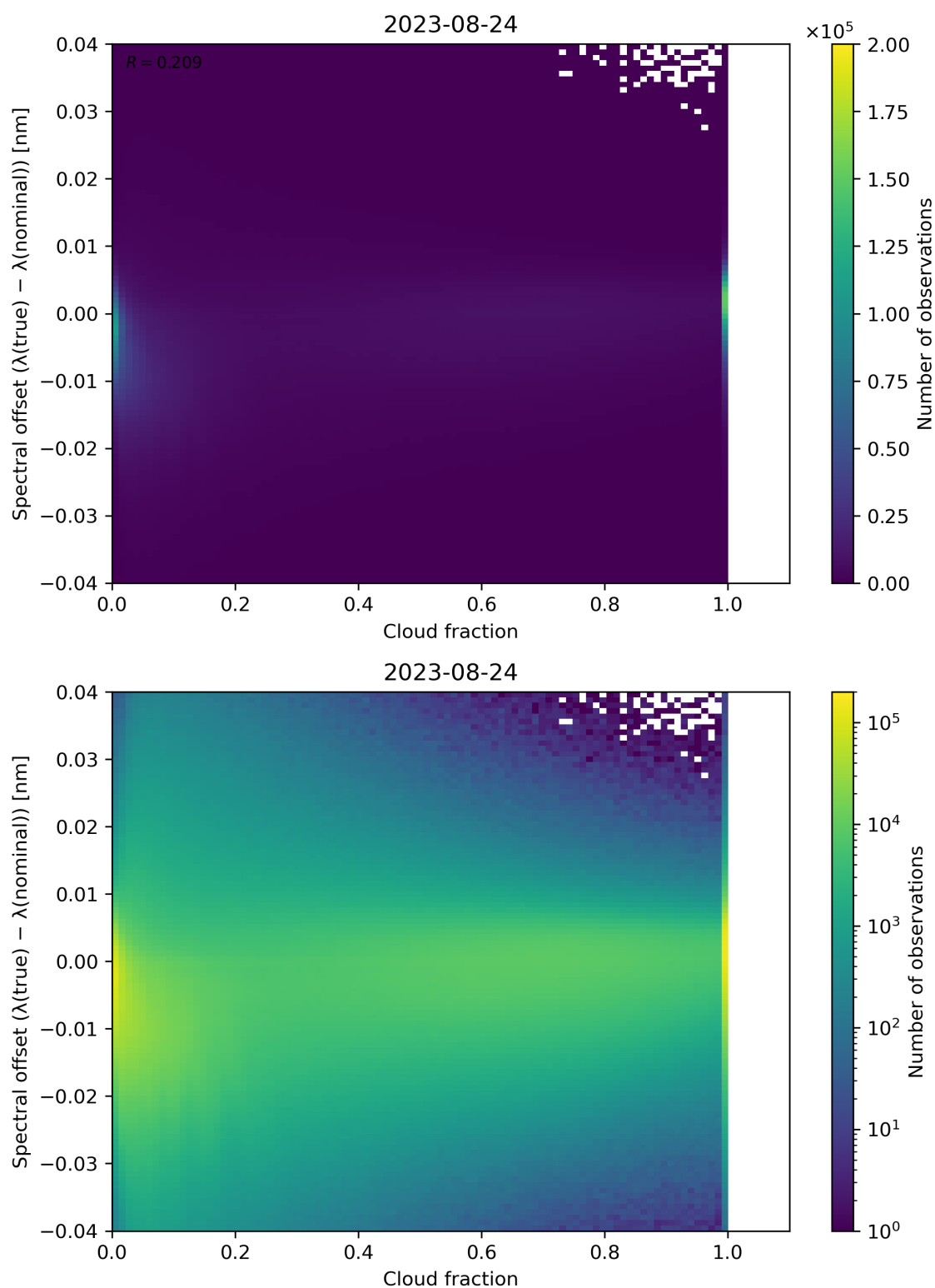
Figure 83: Scatter density plot of “Cloud fraction” against “Spectral offset ( \lambda(\text{true}) - \lambda(\text{nominal}) )” for 2023-08-23 to 2023-08-25.
