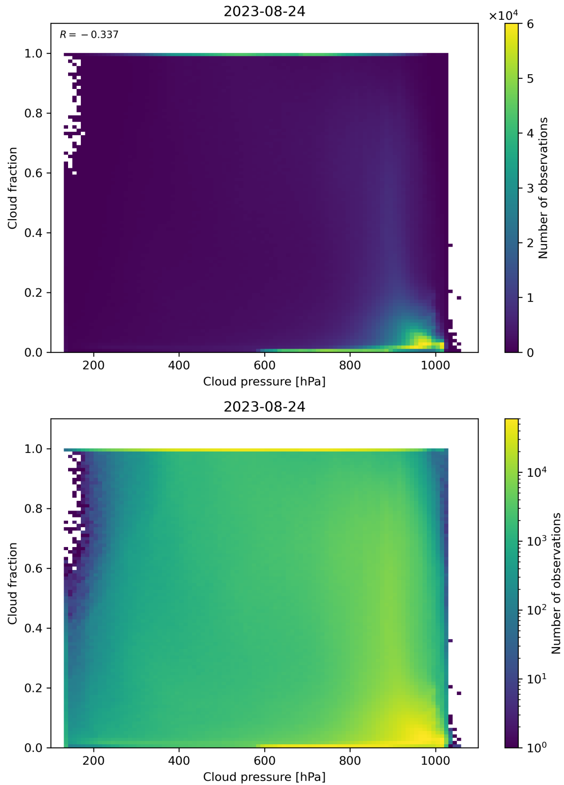
Figure 87: Scatter density plot of “Cloud pressure” against “Cloud fraction” for 2023-08-23 to 2023-08-25.
