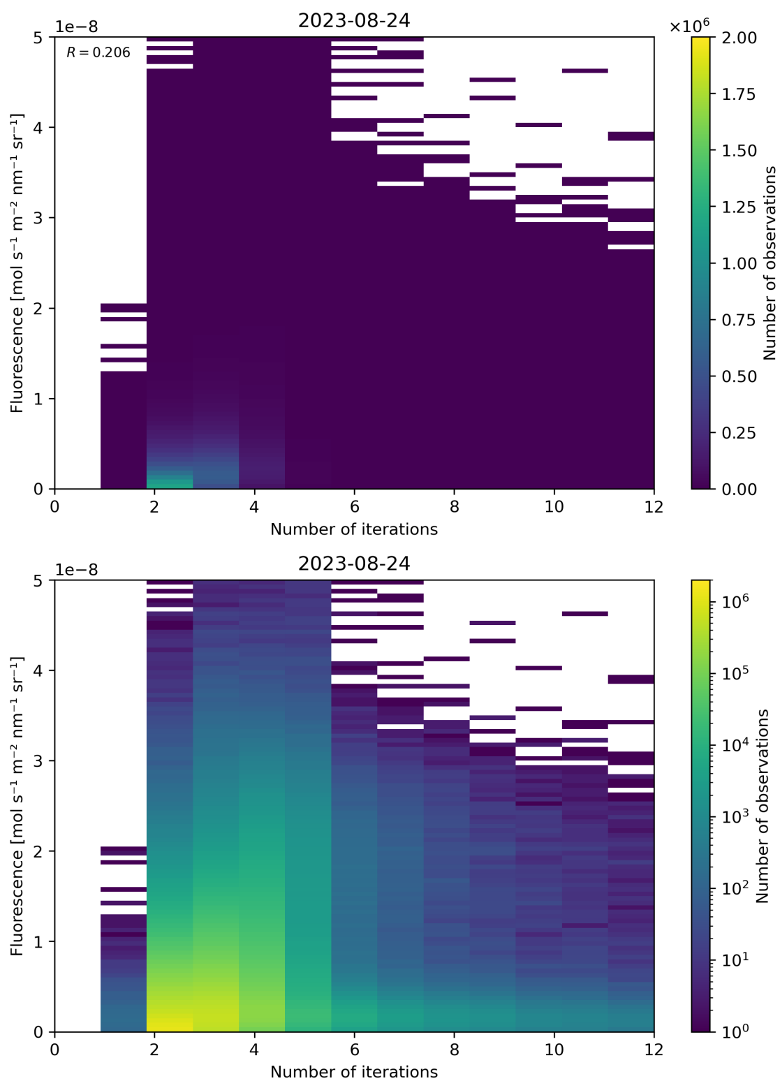
Figure 107: Scatter density plot of “Number of iterations” against “Fluorescence” for 2023-08-23 to 2023-08-25.
