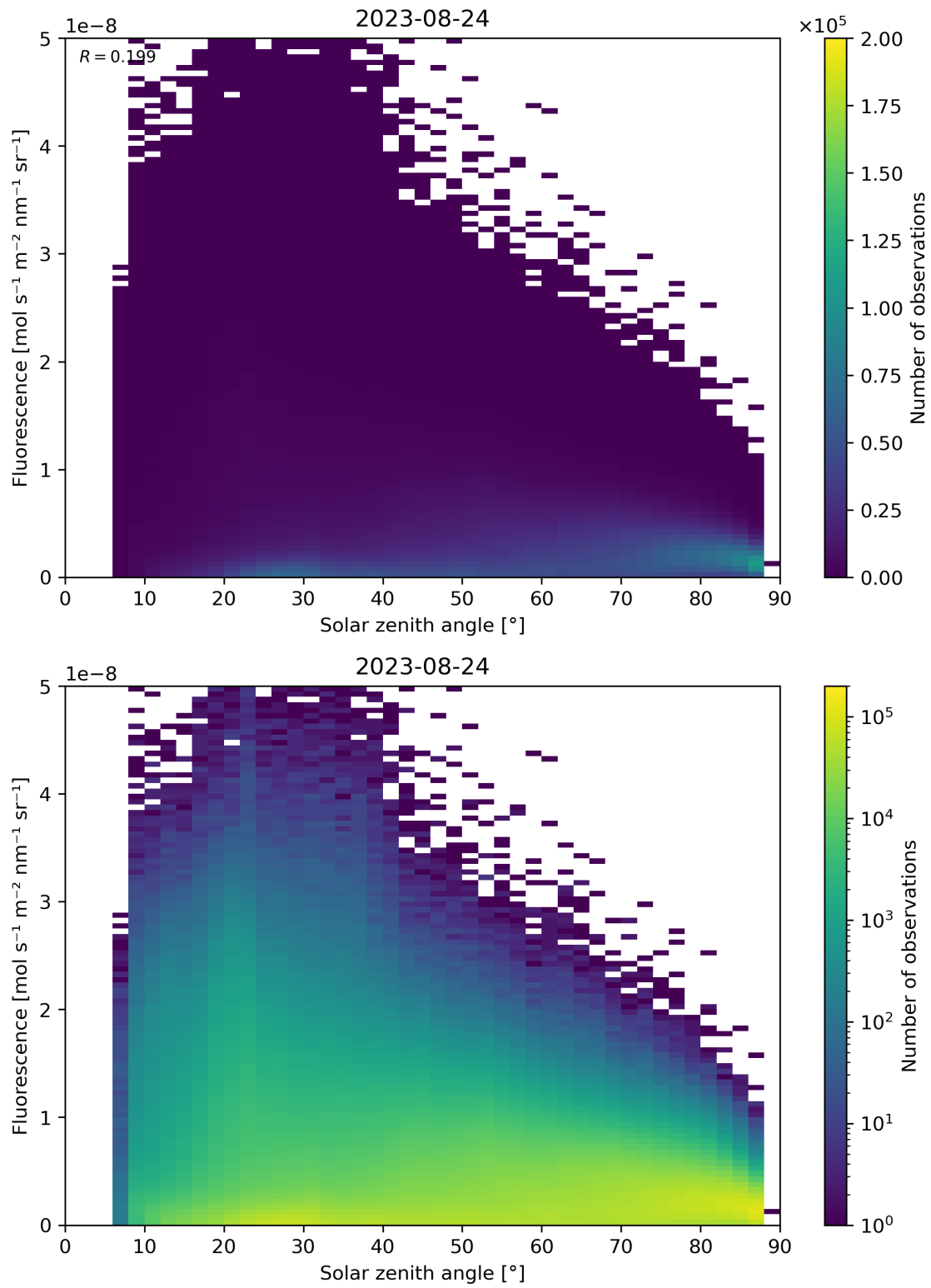
Figure 123: Scatter density plot of “Solar zenith angle” against “Fluorescence” for 2023-08-23 to 2023-08-25.
