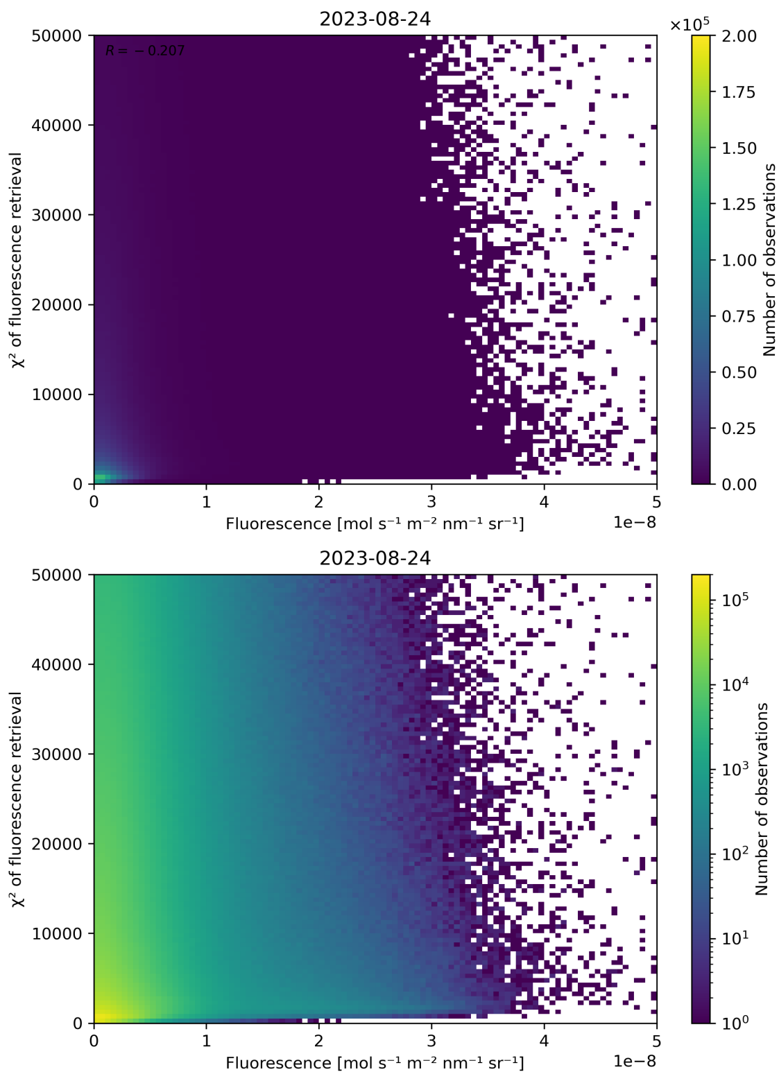
Figure 93: Scatter density plot of “Fluorescence” against “ \chi^2 of fluorescence retrieval” for 2023-08-23 to 2023-08-25.
