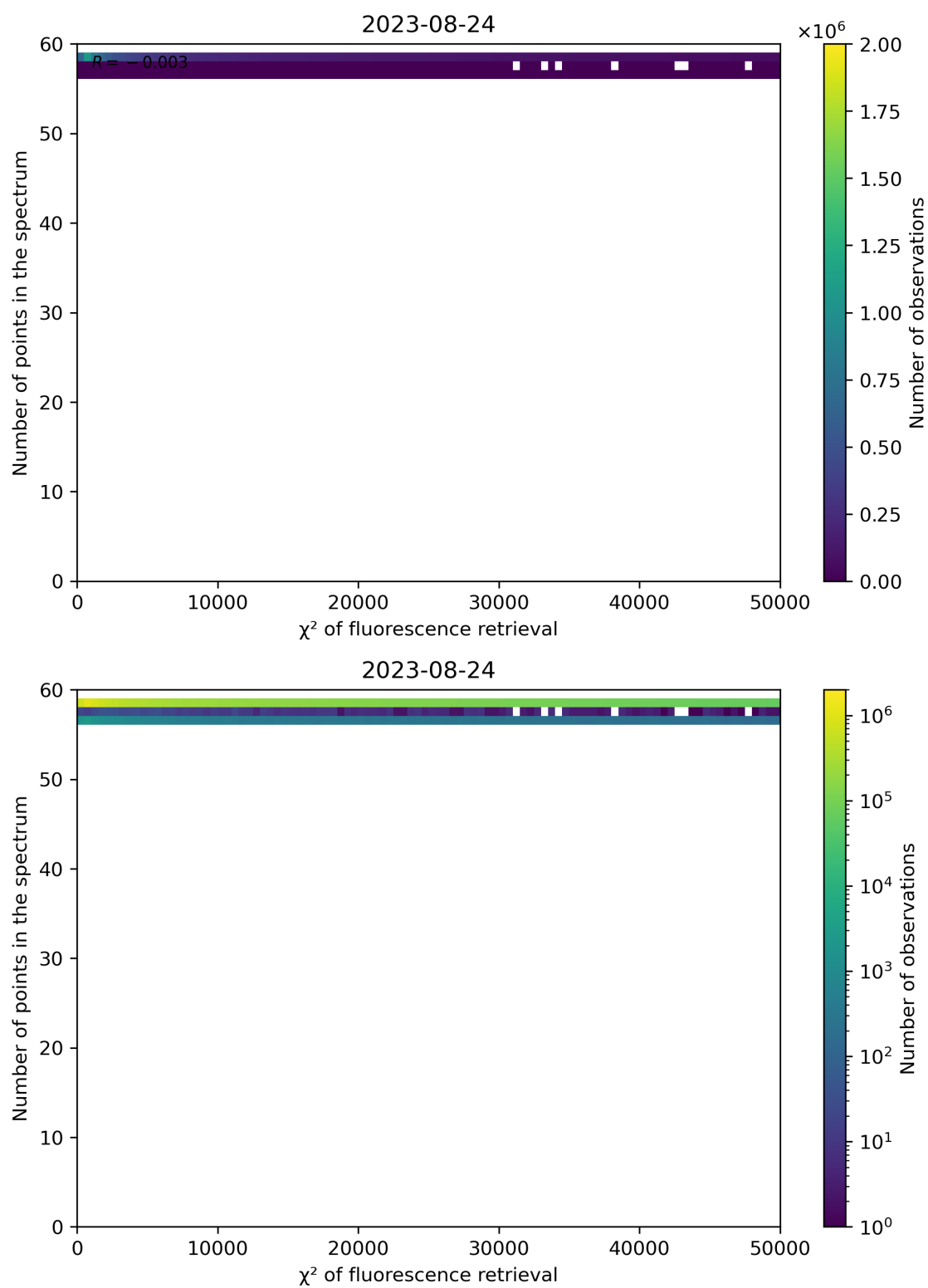
Figure 71: Scatter density plot of " \chi^2 of fluorescence retrieval" against "Number of points in the spectrum" for 2023-08-23 to 2023-08-25.
