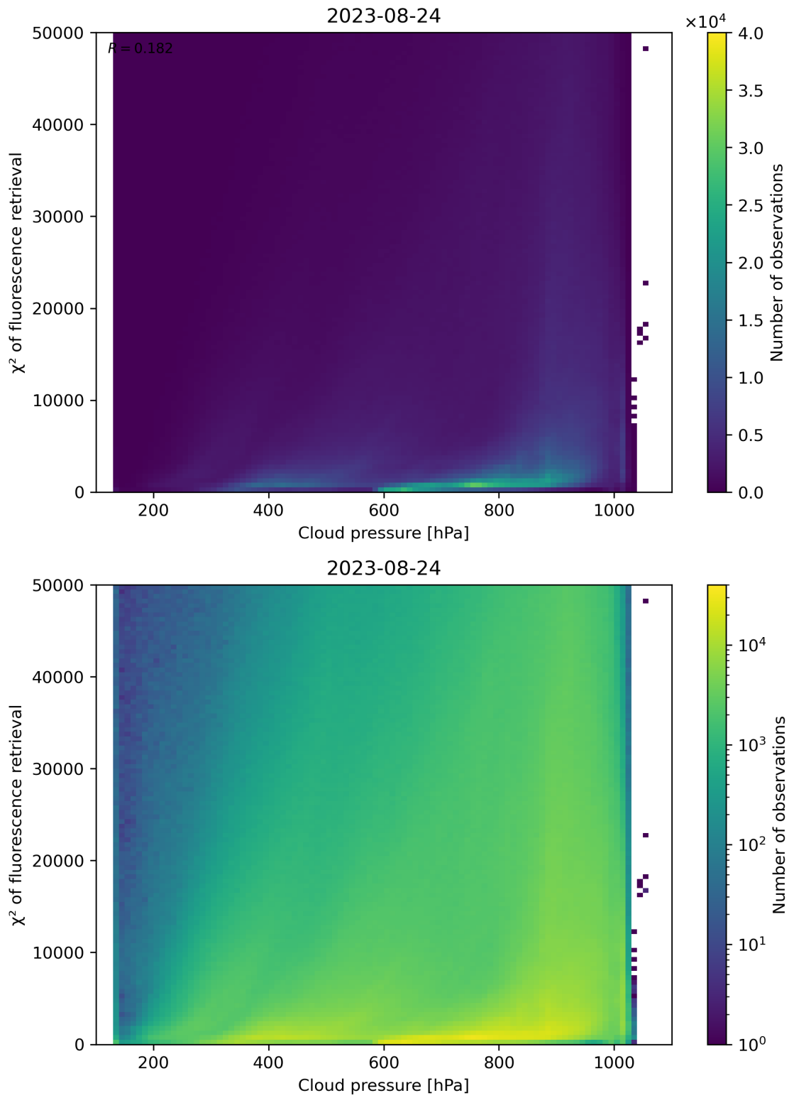
Figure 86: Scatter density plot of “Cloud pressure” against “ \chi^2 of fluorescence retrieval” for 2023-08-23 to 2023-08-25.
