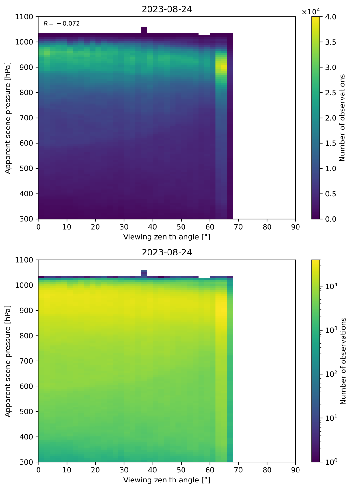
Figure 129: Scatter density plot of “Viewing zenith angle” against “Apparent scene pressure” for 2023-08-23 to 2023-08-25.
