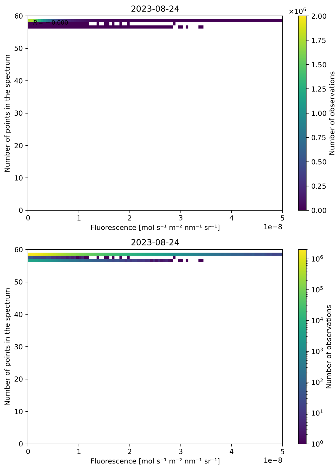
Figure 94: Scatter density plot of “Fluorescence” against “Number of points in the spectrum” for 2023-08-23 to 2023-08-25.
