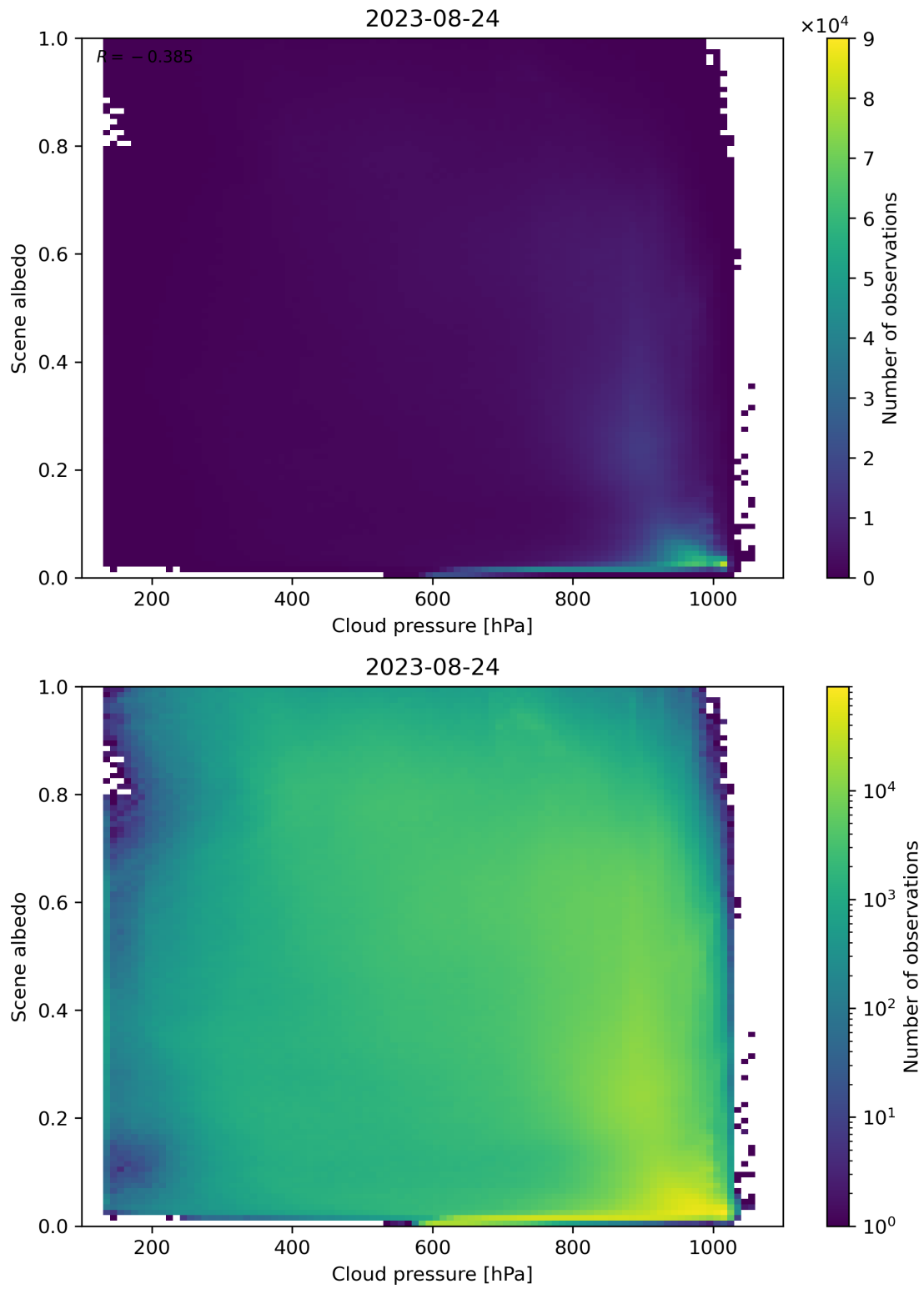
Figure 91: Scatter density plot of “Cloud pressure” against “Scene albedo” for 2023-08-23 to 2023-08-25.
