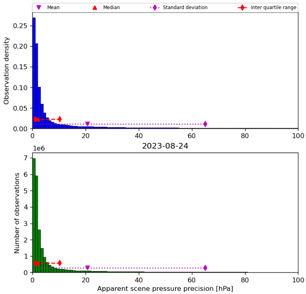
Figure 37: Histogram of “Apparent scene pressure precision” for 2023-08-23 to 2023-08-25
