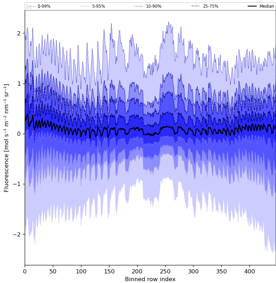
Figure 57: Along track statistics of “Fluorescence” for 2023-08-23 to 2023-08-25
