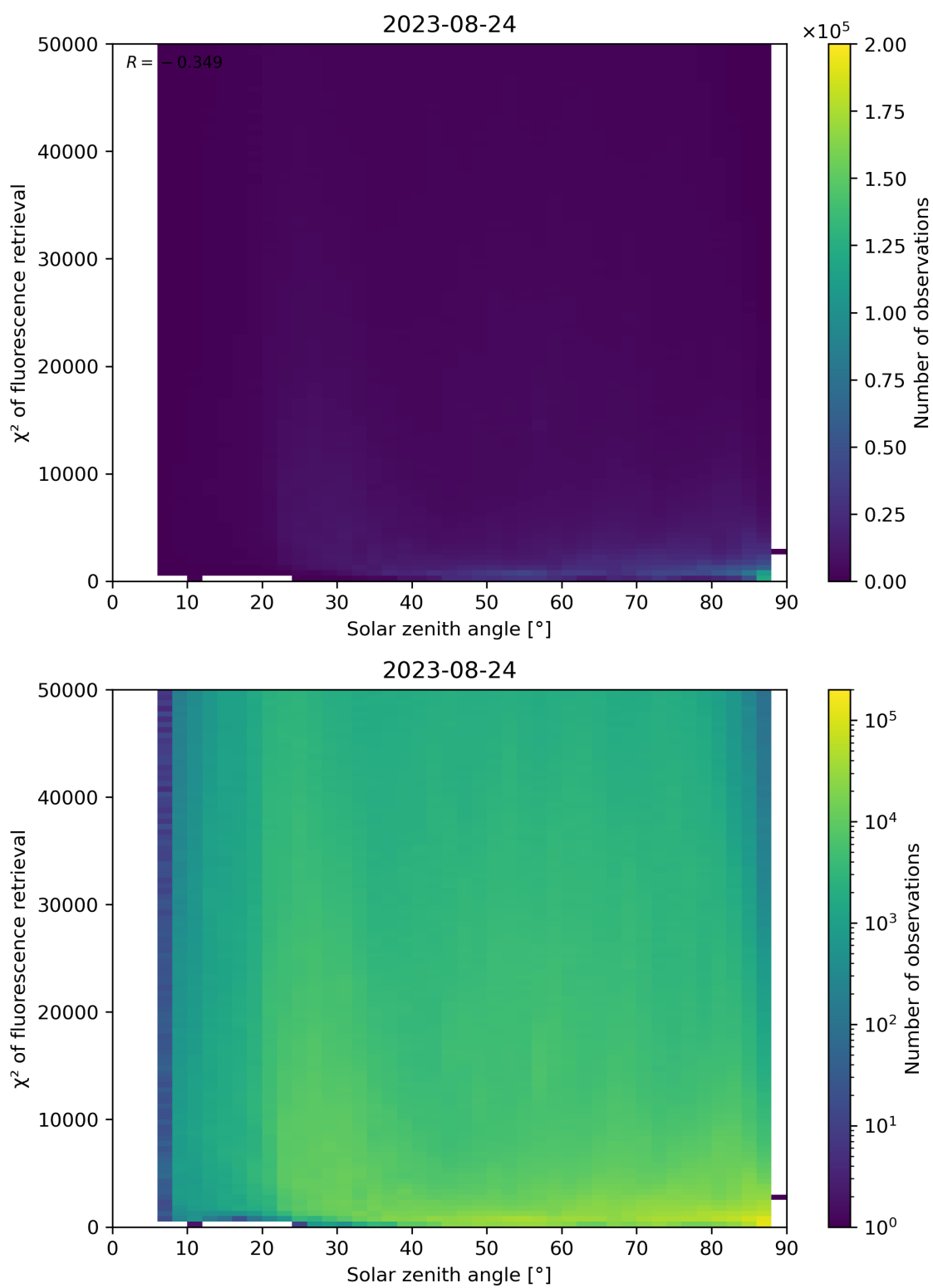
Figure 120: Scatter density plot of “Solar zenith angle” against “ \chi^2 of fluorescence retrieval” for 2023-08-23 to 2023-08-25.
