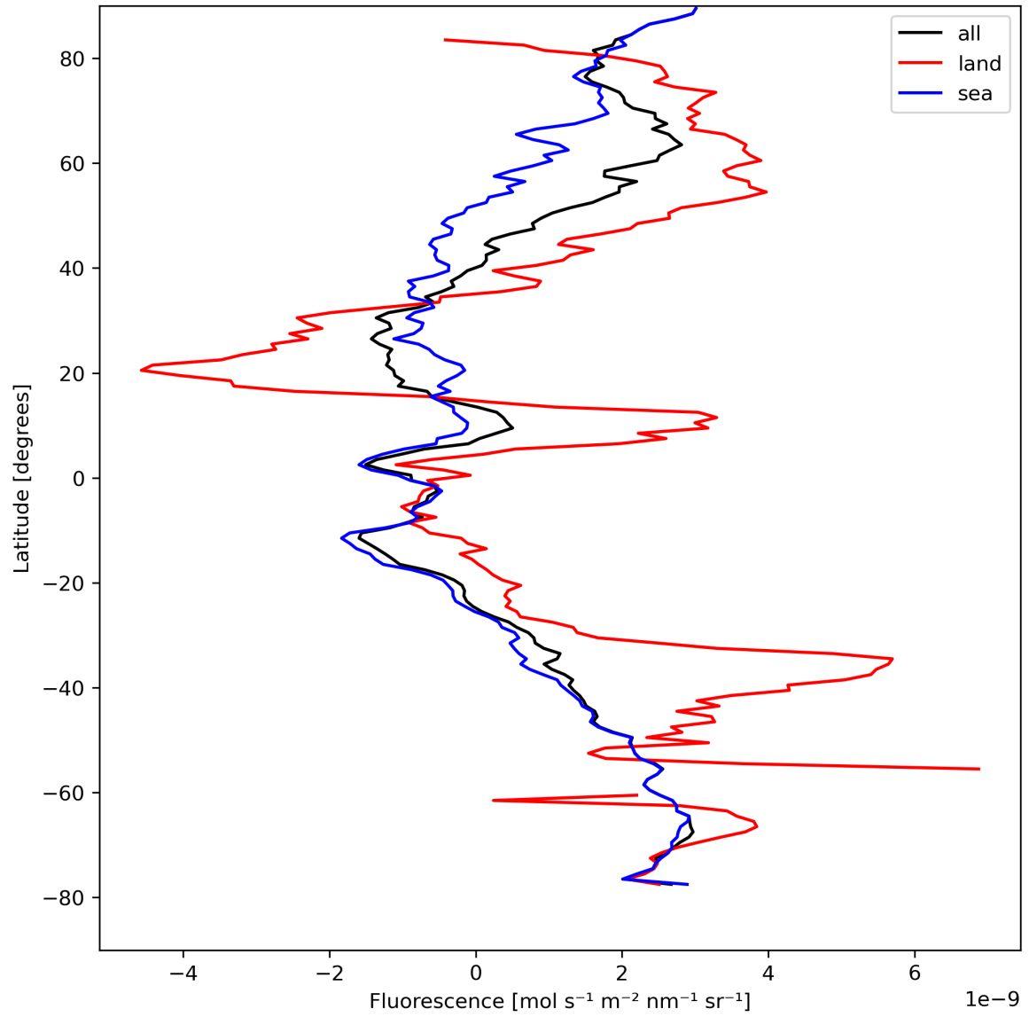
Figure 23: Zonal average of “Fluorescence” for 2023-08-23 to 2023-08-25.
