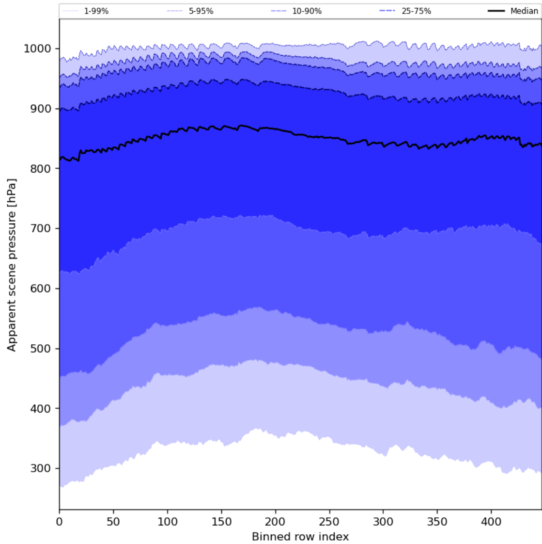
Figure 53: Along track statistics of “Apparent scene pressure” for 2023-08-23 to 2023-08-25
