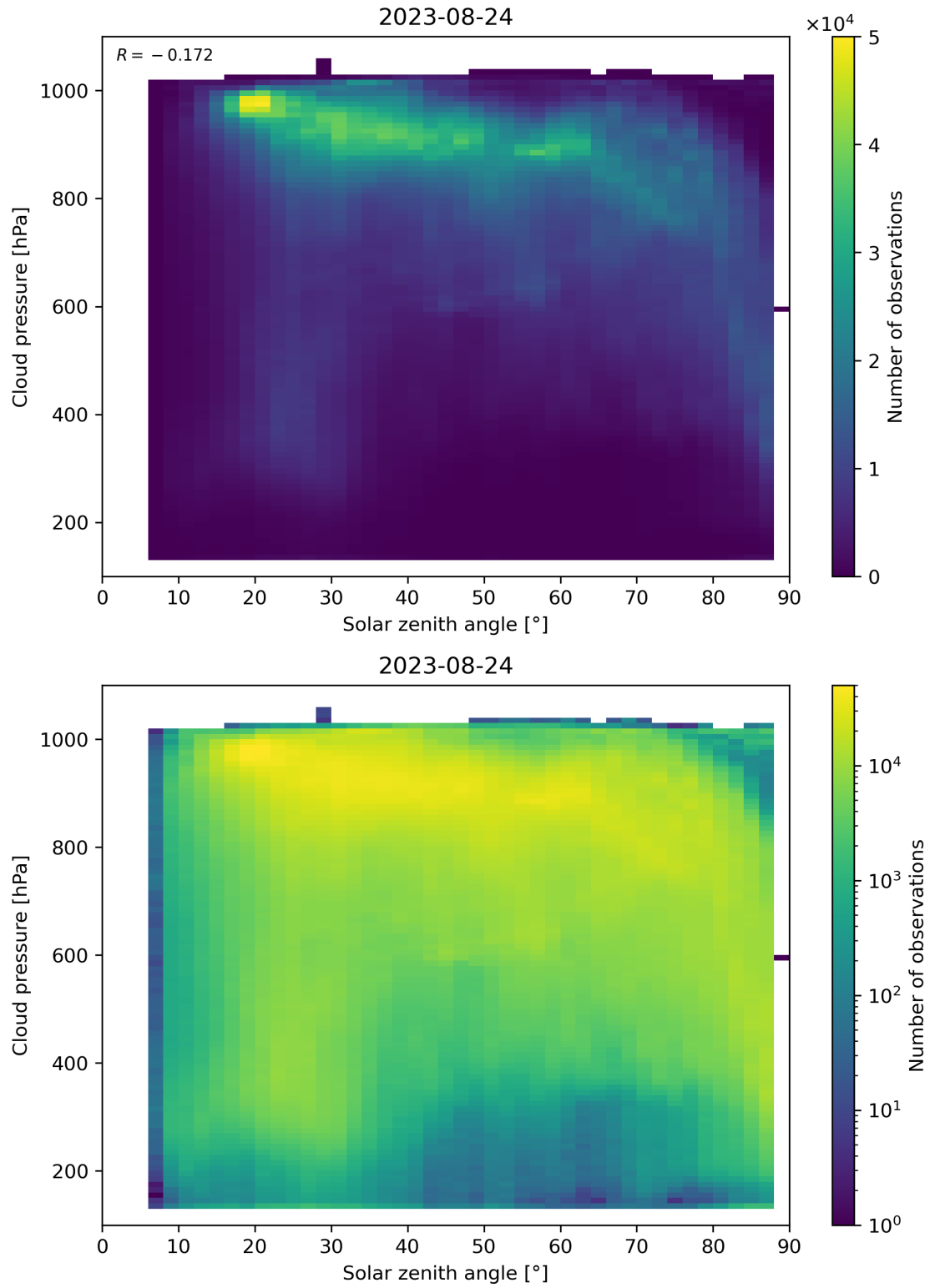
Figure 122: Scatter density plot of “Solar zenith angle” against “Cloud pressure” for 2023-08-23 to 2023-08-25.
