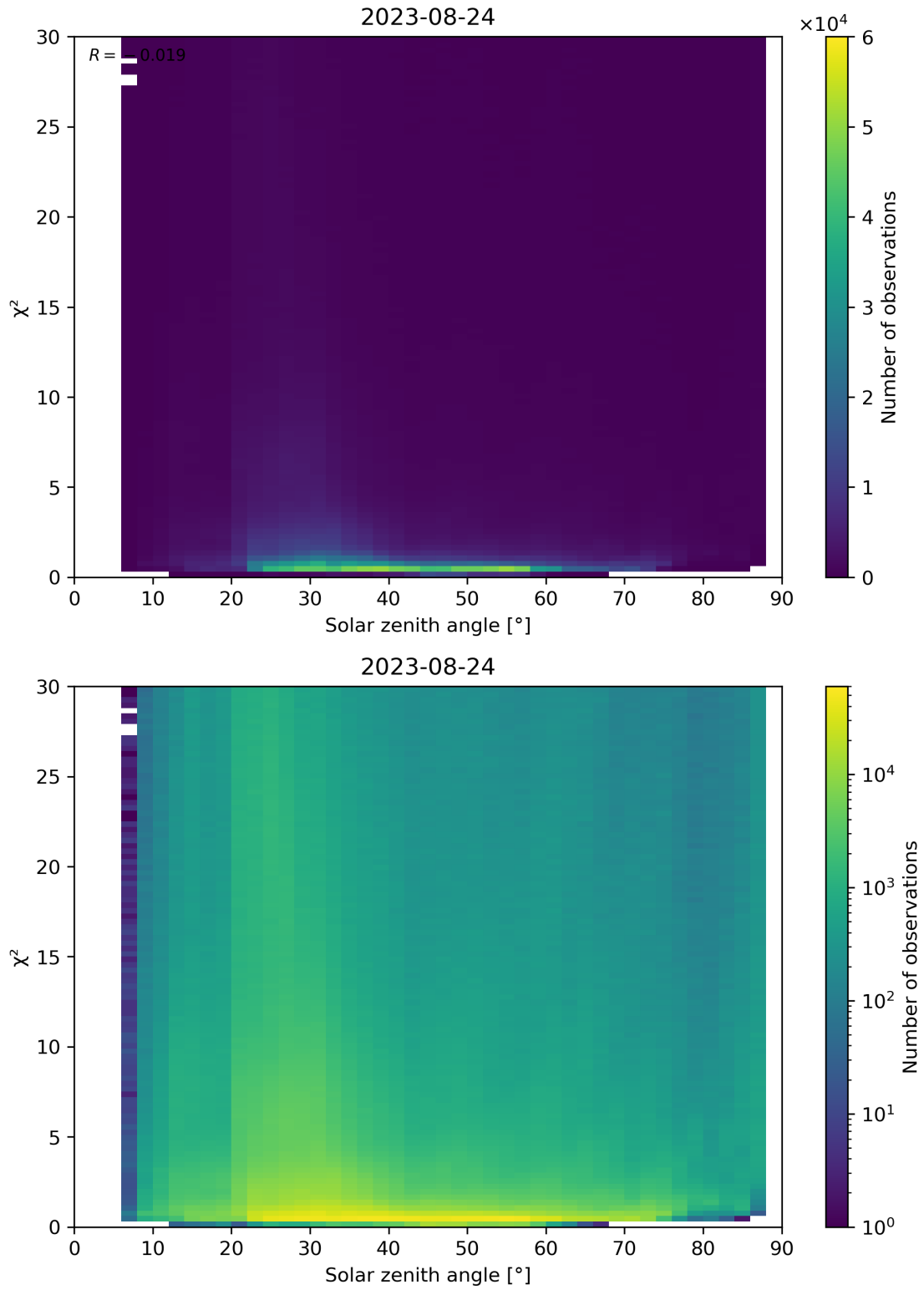
Figure 119: Scatter density plot of “Solar zenith angle” against “ \chi^2 ” for 2023-08-23 to 2023-08-25.
