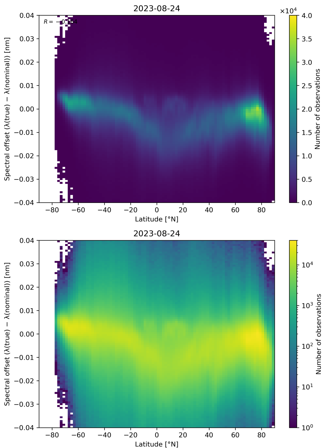
Figure 105: Scatter density plot of “Latitude” against “Spectral offset ( \lambda(\text{true}) - \lambda(\text{nominal}) )” for 2023-08-23 to 2023-08-25.
