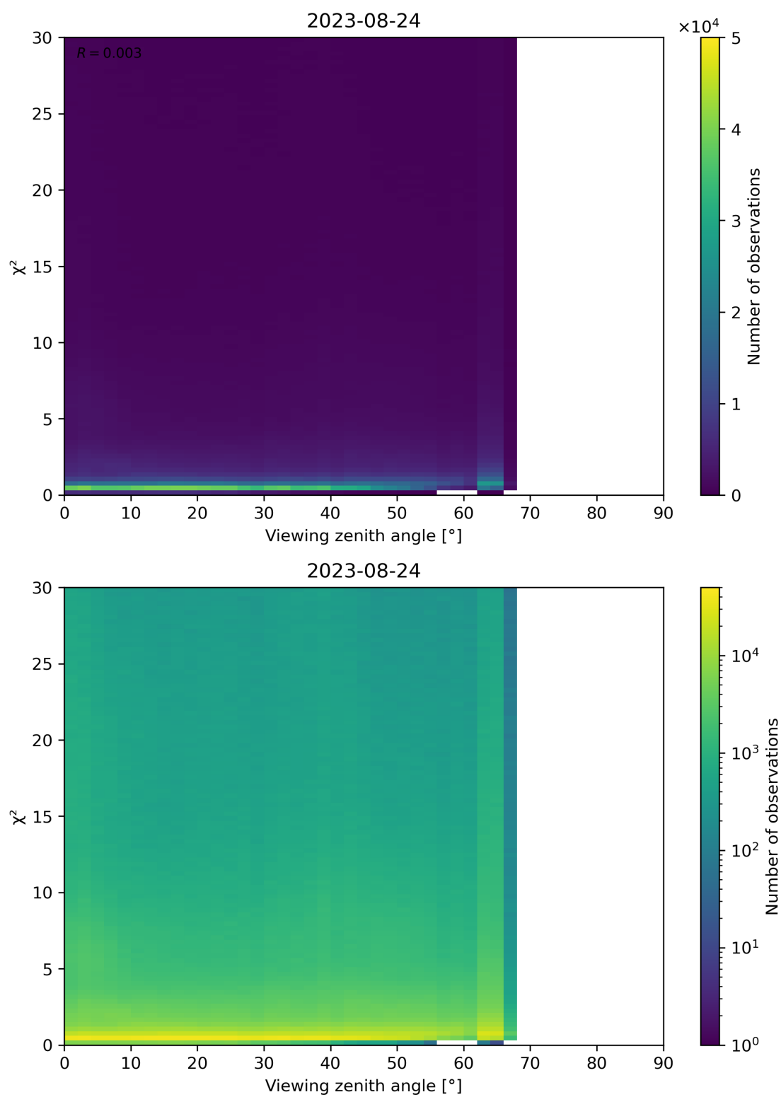
Figure 130: Scatter density plot of “Viewing zenith angle” against “ \chi^2 ” for 2023-08-23 to 2023-08-25.
