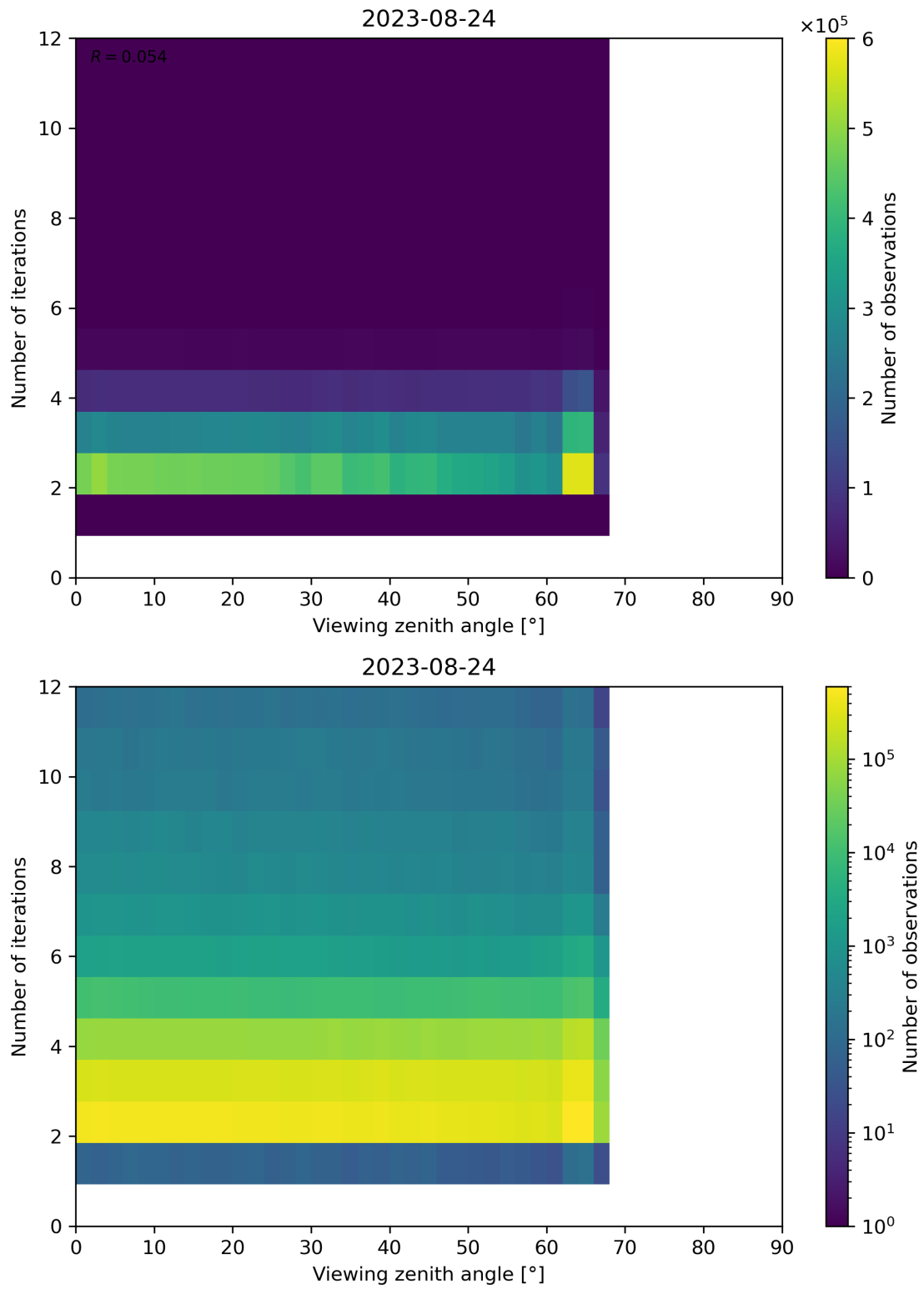
Figure 136: Scatter density plot of “Viewing zenith angle” against “Number of iterations” for 2023-08-23 to 2023-08-25.
