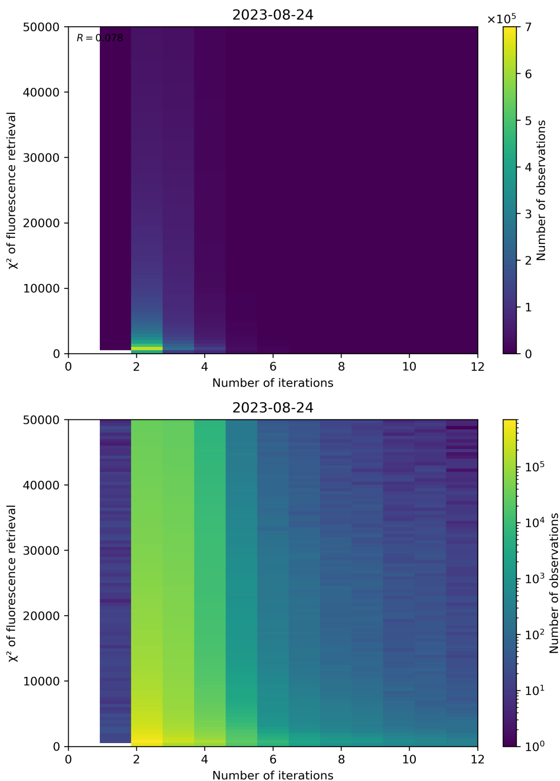
Figure 106: Scatter density plot of “Number of iterations” against “ \chi^2 of fluorescence retrieval” for 2023-08-23 to 2023-08-25.
