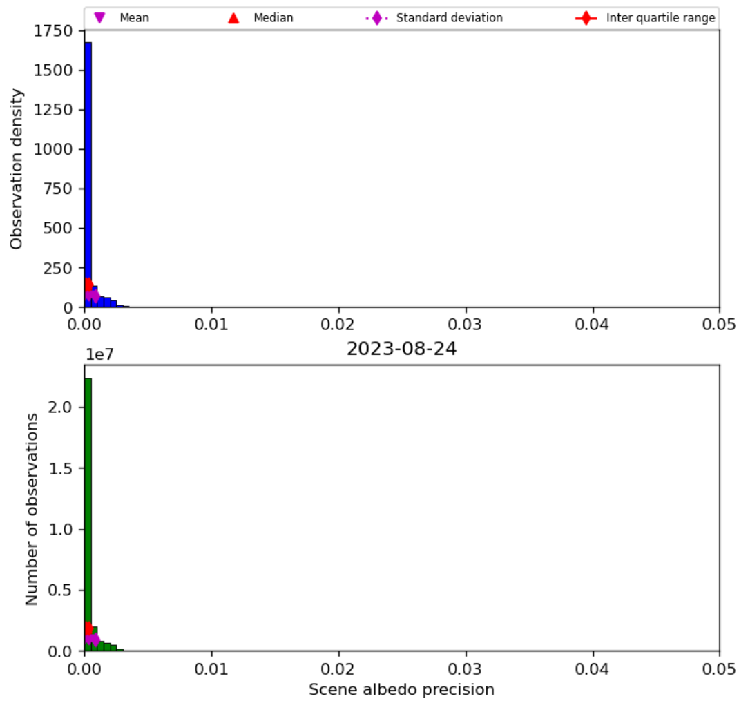
Figure 35: Histogram of “Scene albedo precision” for 2023-08-23 to 2023-08-25
