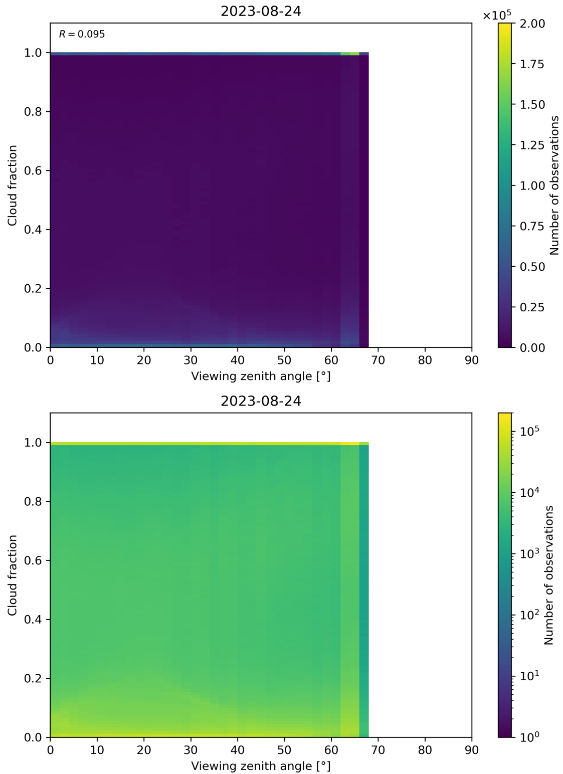
Figure 132: Scatter density plot of “Viewing zenith angle” against “Cloud fraction” for 2023-08-23 to 2023-08-25.
