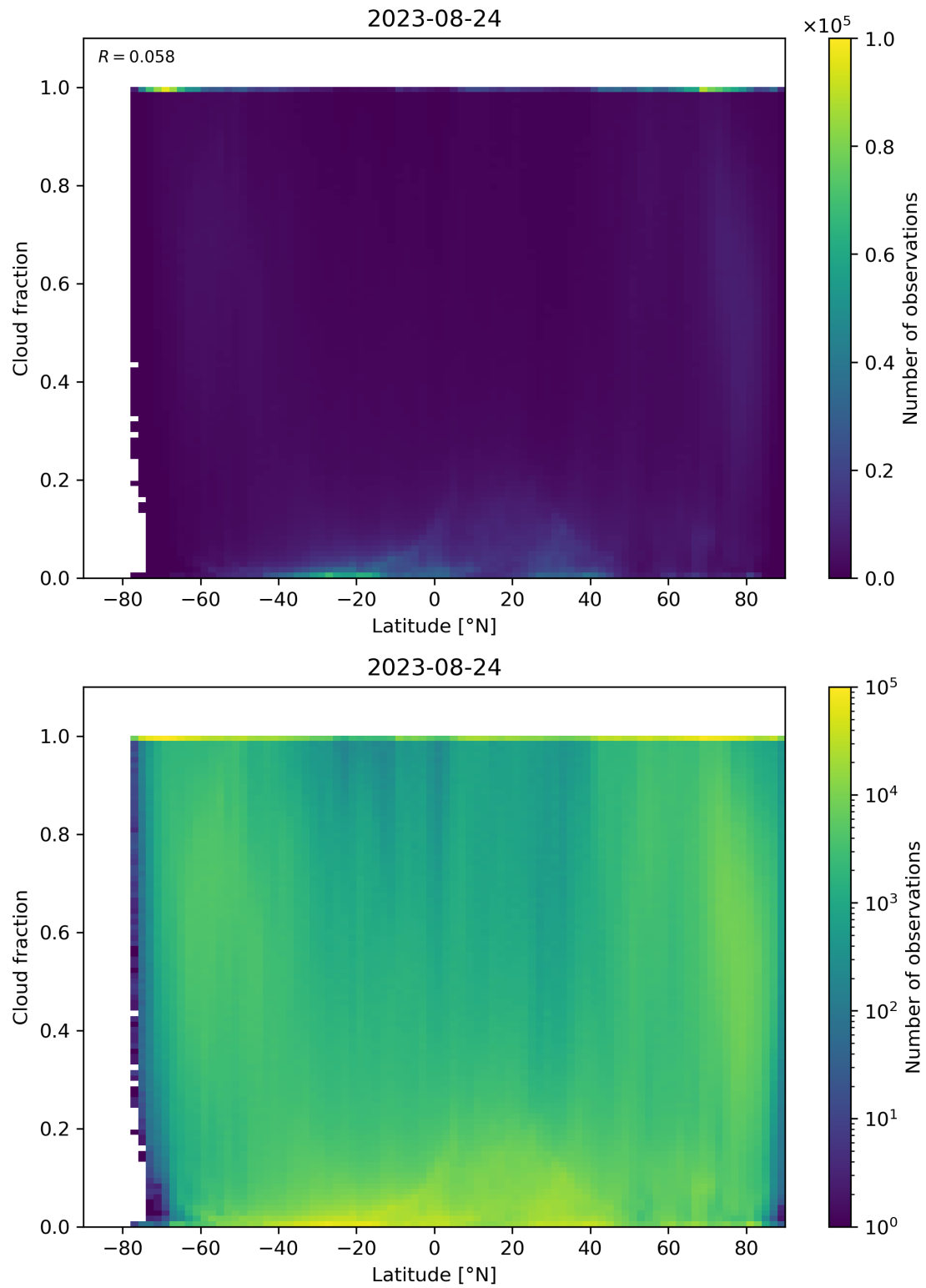
Figure 99: Scatter density plot of “Latitude” against “Cloud fraction” for 2023-08-23 to 2023-08-25.
