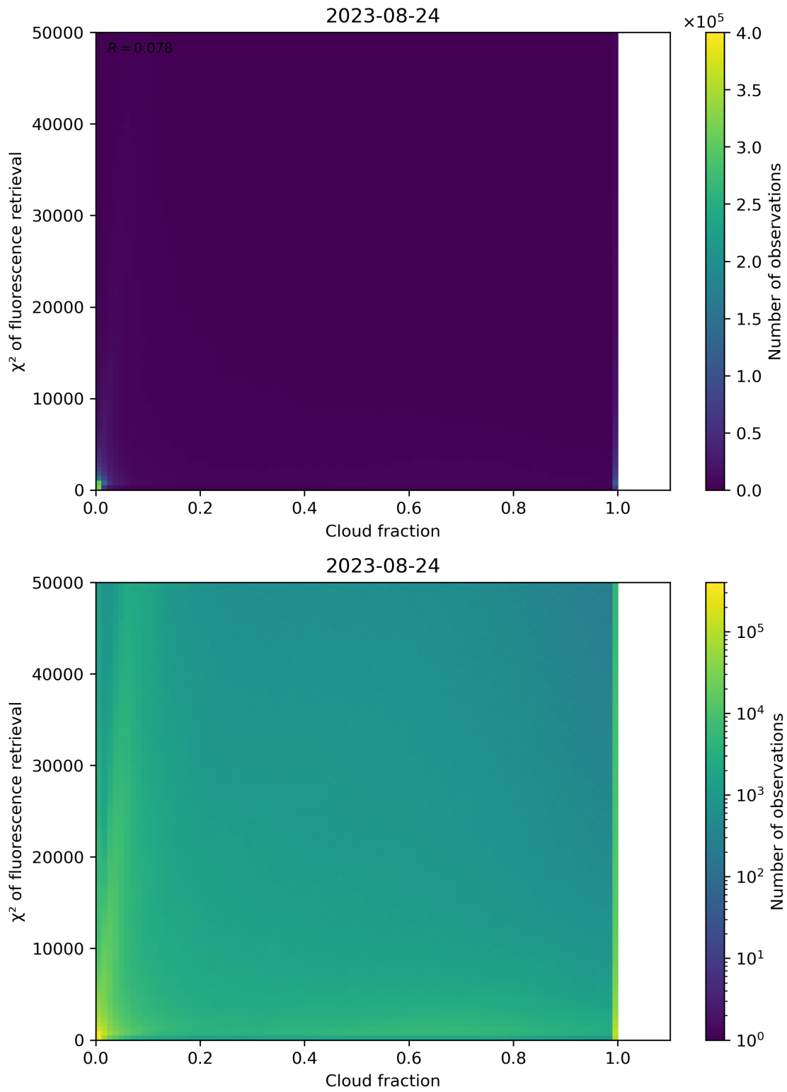
Figure 78: Scatter density plot of “Cloud fraction” against “ \chi^2 of fluorescence retrieval” for 2023-08-23 to 2023-08-25.
