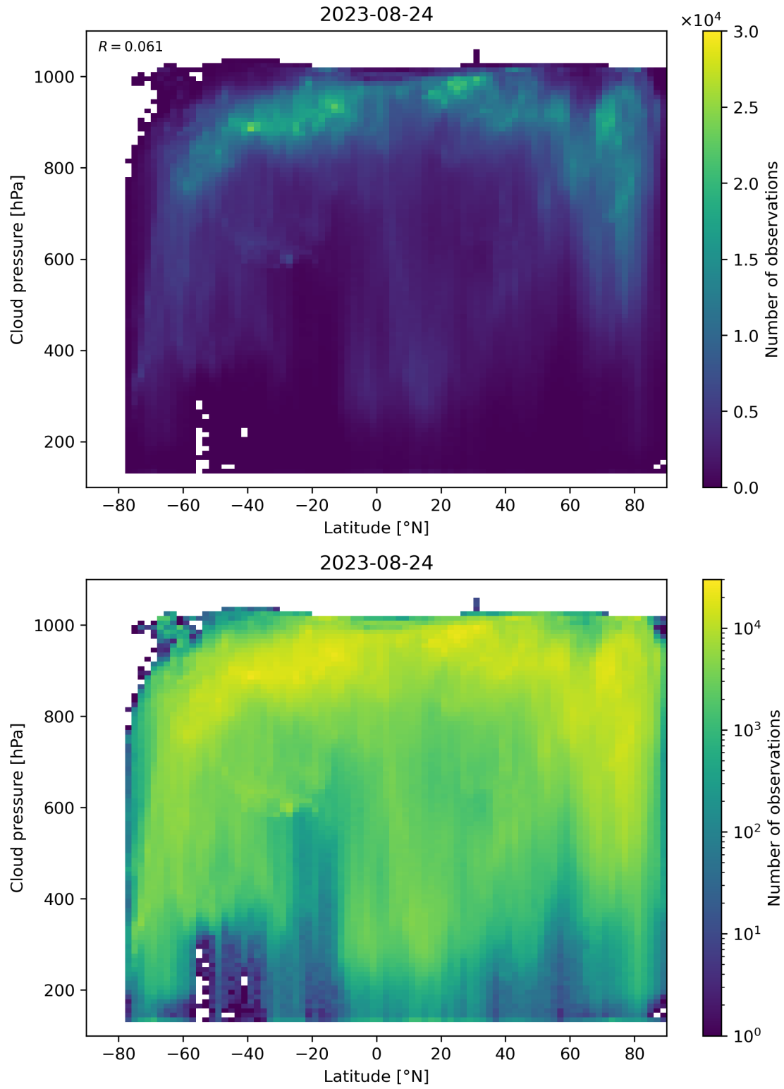
Figure 100: Scatter density plot of “Latitude” against “Cloud pressure” for 2023-08-23 to 2023-08-25.
