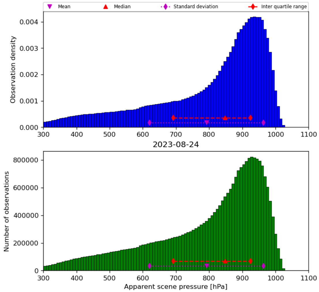
Figure 36: Histogram of “Apparent scene pressure” for 2023-08-23 to 2023-08-25
