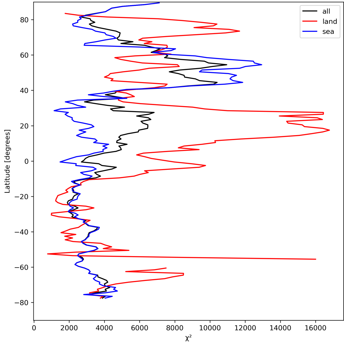
Figure 21: Zonal average of “ \chi^2 ” for 2023-08-23 to 2023-08-25.
