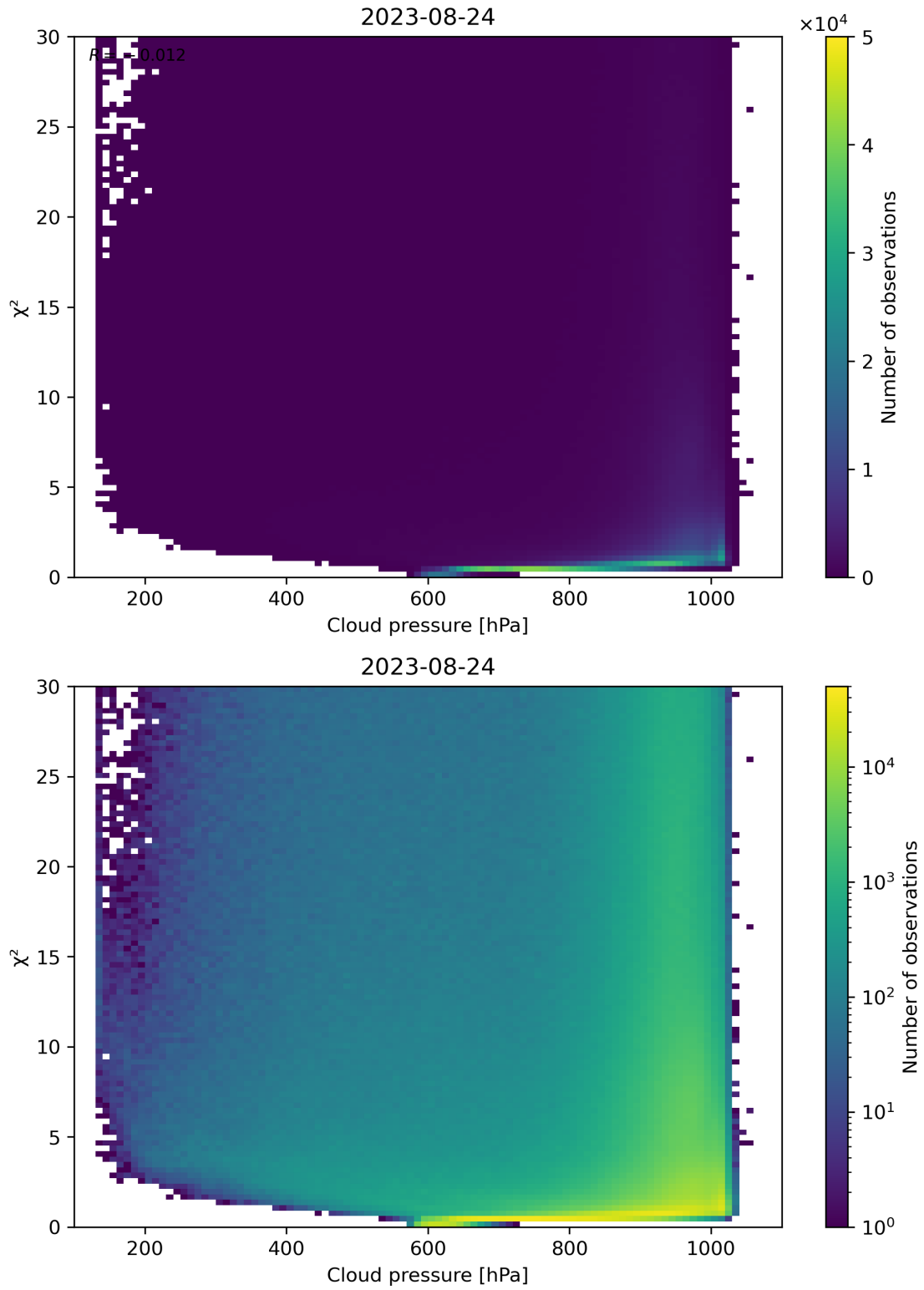
Figure 85: Scatter density plot of “Cloud pressure” against “ \chi^2 ” for 2023-08-23 to 2023-08-25.
