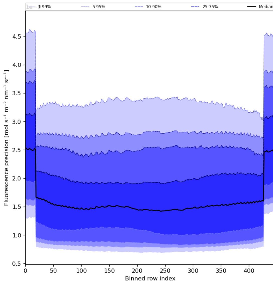
Figure 58: Along track statistics of “Fluorescence precision” for 2023-08-23 to 2023-08-25
