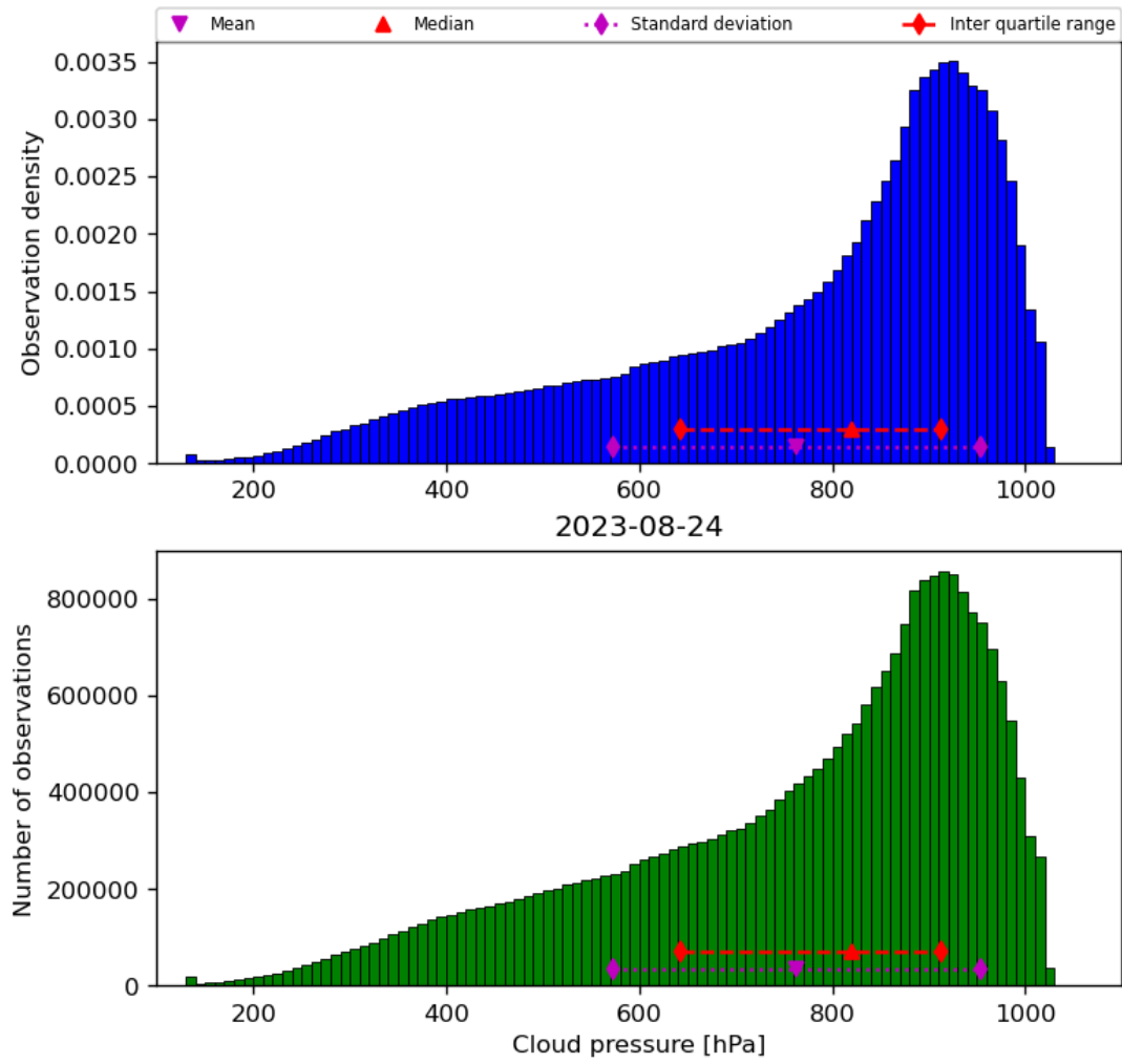
Figure 30: Histogram of “Cloud pressure” for 2023-08-23 to 2023-08-25
