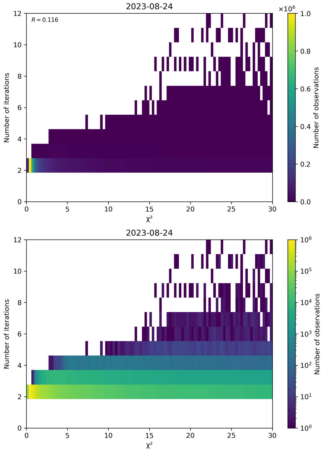
Figure 73: Scatter density plot of “ \chi^2 ” against “Number of iterations” for 2023-08-23 to 2023-08-25.
