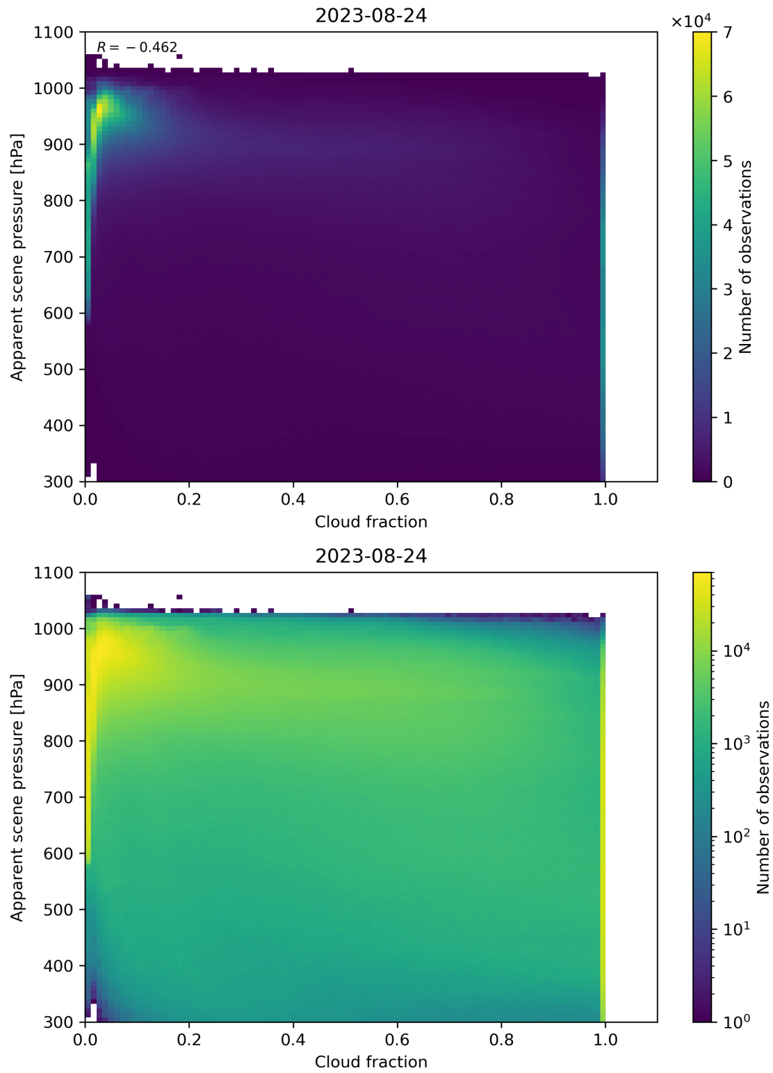
Figure 76: Scatter density plot of “Cloud fraction” against “Apparent scene pressure” for 2023-08-23 to 2023-08-25.
