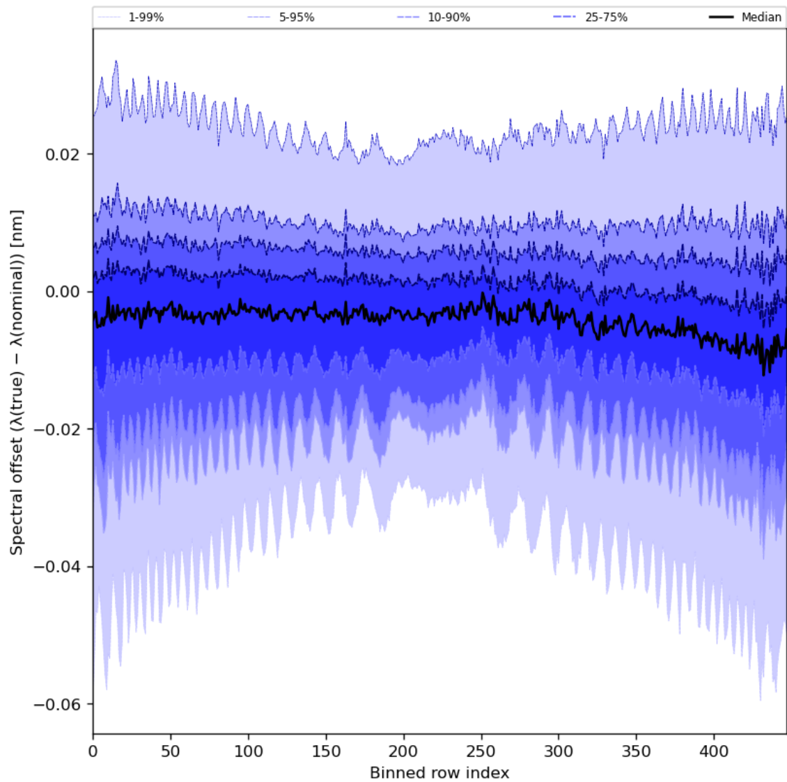
Figure 62: Along track statistics of “Spectral offset ( \lambda(\text{true}) - \lambda(\text{nominal}) )” for 2023-08-23 to 2023-08-25
