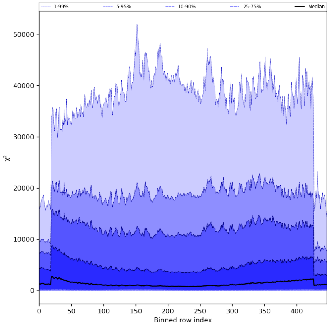
Figure 55: Along track statistics of “ \chi^2 ” for 2023-08-23 to 2023-08-25
