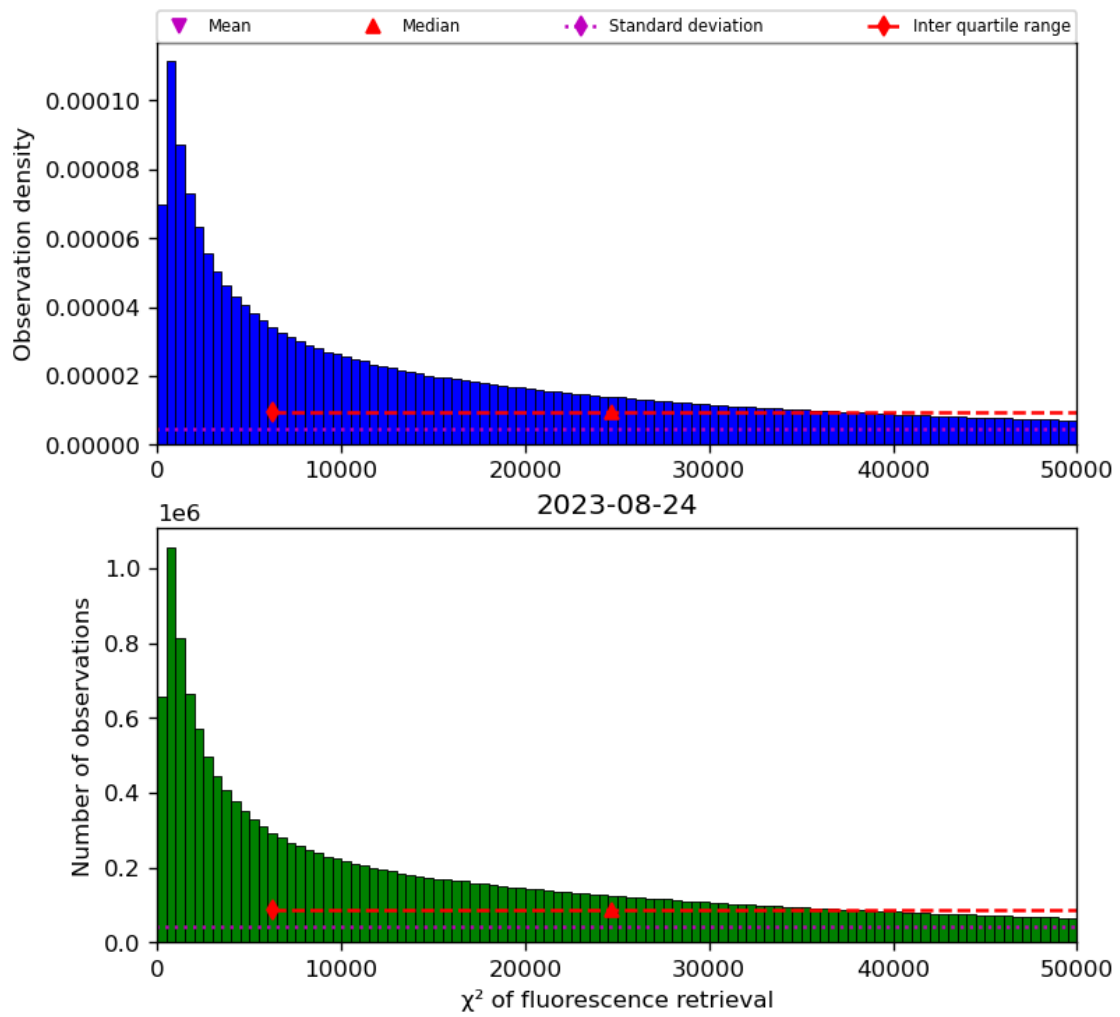
Figure 42: Histogram of “ \chi^2 of fluorescence retrieval” for 2023-08-23 to 2023-08-25
