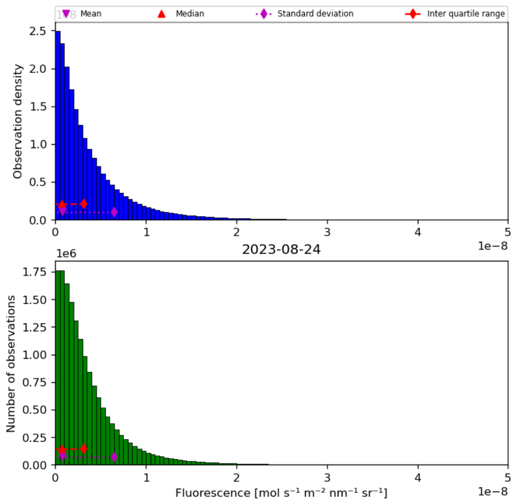
Figure 40: Histogram of “Fluorescence” for 2023-08-23 to 2023-08-25
