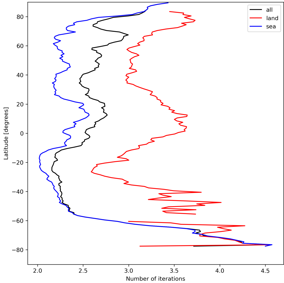
Figure 22: Zonal average of “Number of iterations” for 2023-08-23 to 2023-08-25.
