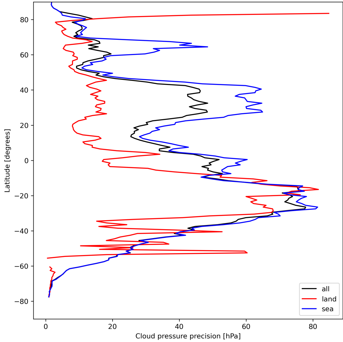
Figure 14: Zonal average of “Cloud pressure precision” for 2023-08-23 to 2023-08-25.
