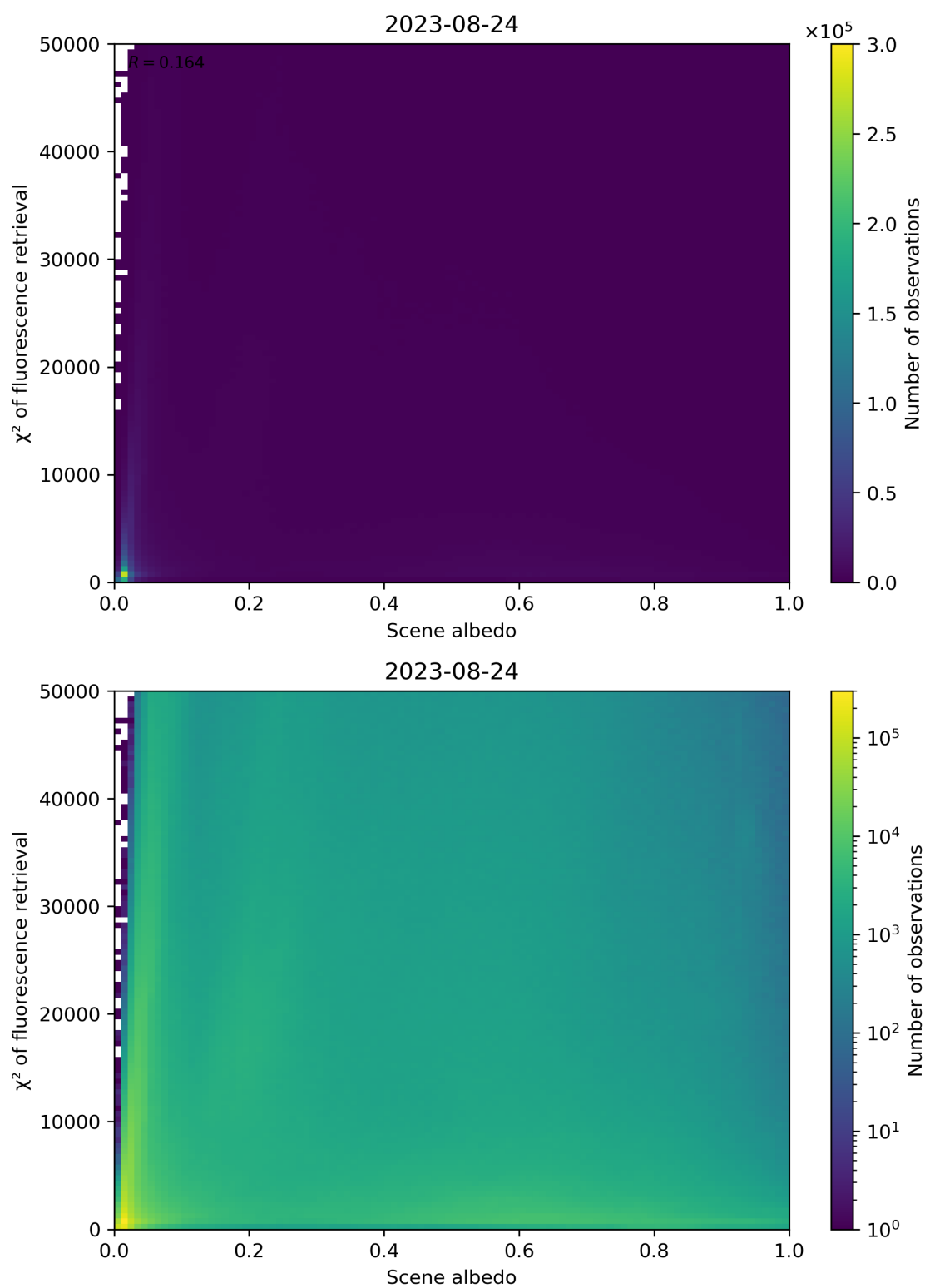
Figure 113: Scatter density plot of “Scene albedo” against “ \chi^2 of fluorescence retrieval” for 2023-08-23 to 2023-08-25.
