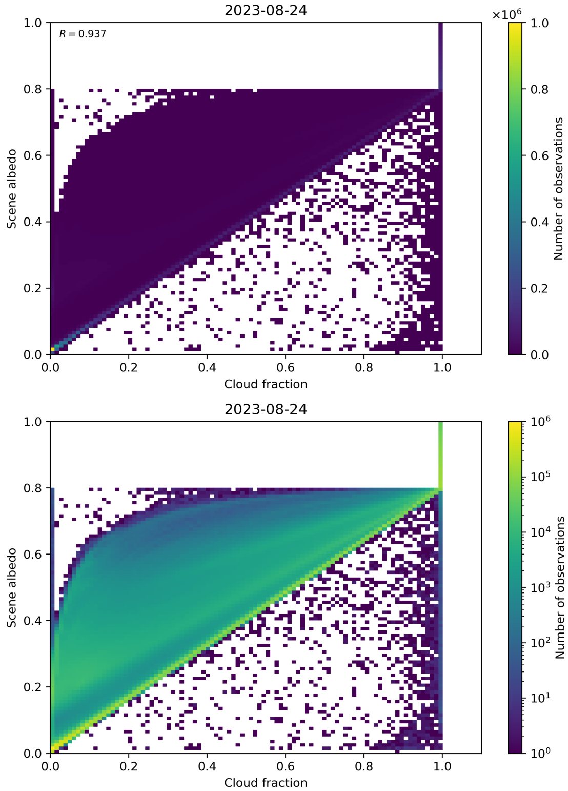
Figure 82: Scatter density plot of “Cloud fraction” against “Scene albedo” for 2023-08-23 to 2023-08-25.
