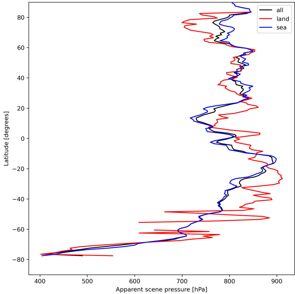
Figure 19: Zonal average of “Apparent scene pressure” for 2023-08-23 to 2023-08-25.
