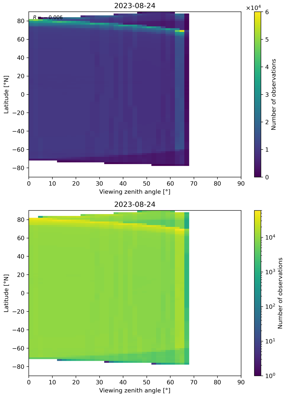
Figure 135: Scatter density plot of “Viewing zenith angle” against “Latitude” for 2023-08-23 to 2023-08-25.
