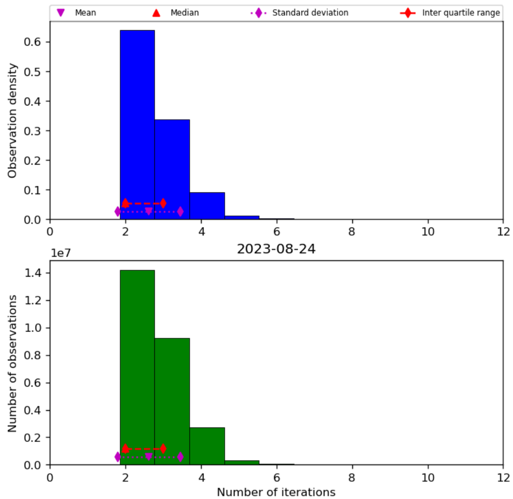
Figure 39: Histogram of “Number of iterations” for 2023-08-23 to 2023-08-25
