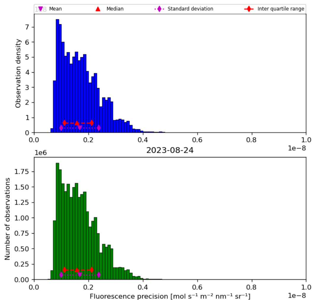
Figure 41: Histogram of “Fluorescence precision” for 2023-08-23 to 2023-08-25
