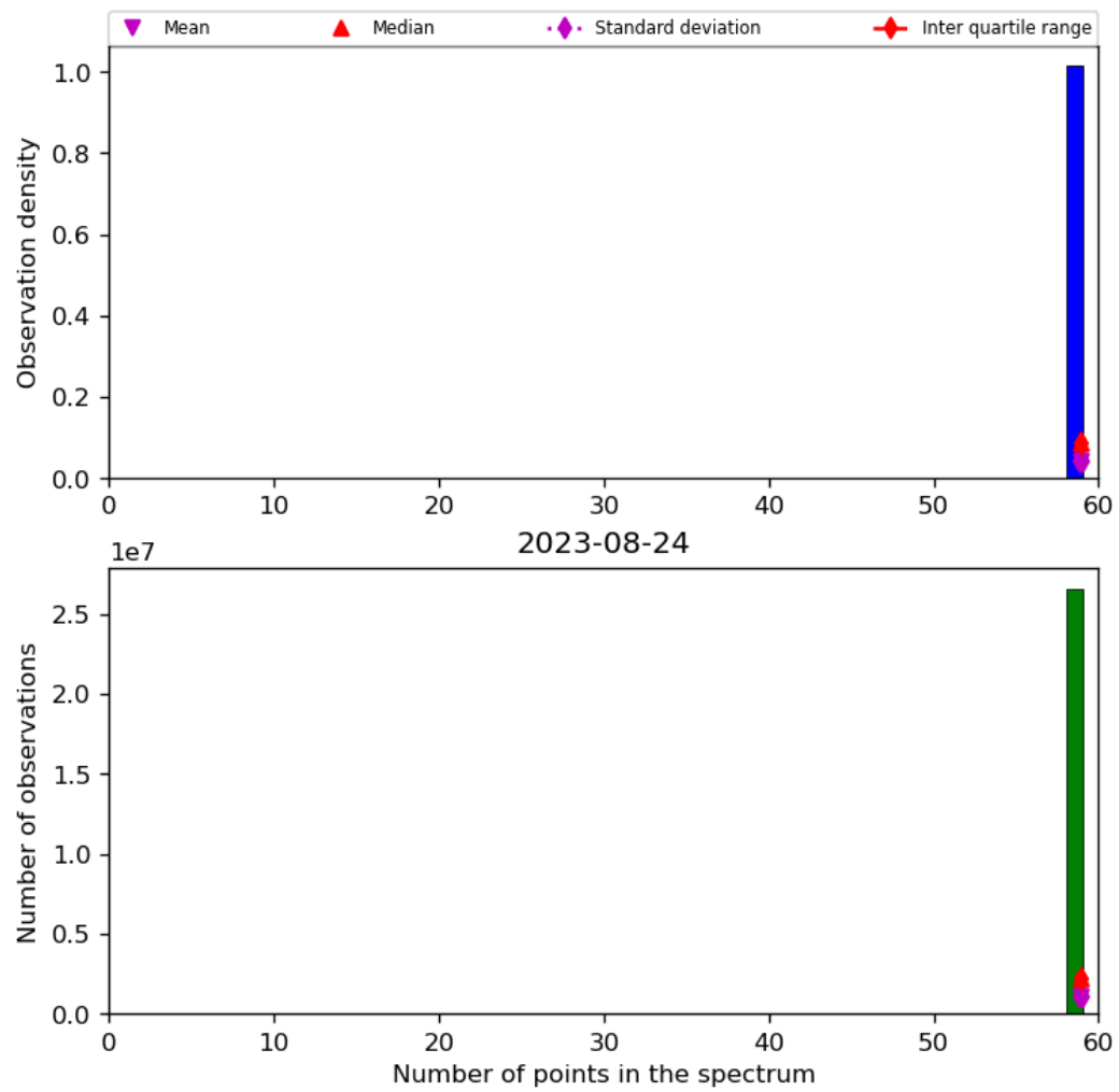
Figure 44: Histogram of “Number of points in the spectrum” for 2023-08-23 to 2023-08-25
