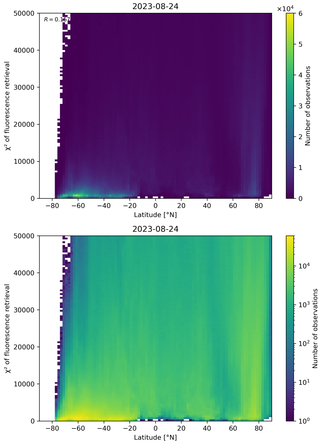
Figure 98: Scatter density plot of “Latitude” against “ \chi^2 of fluorescence retrieval” for 2023-08-23 to 2023-08-25.
