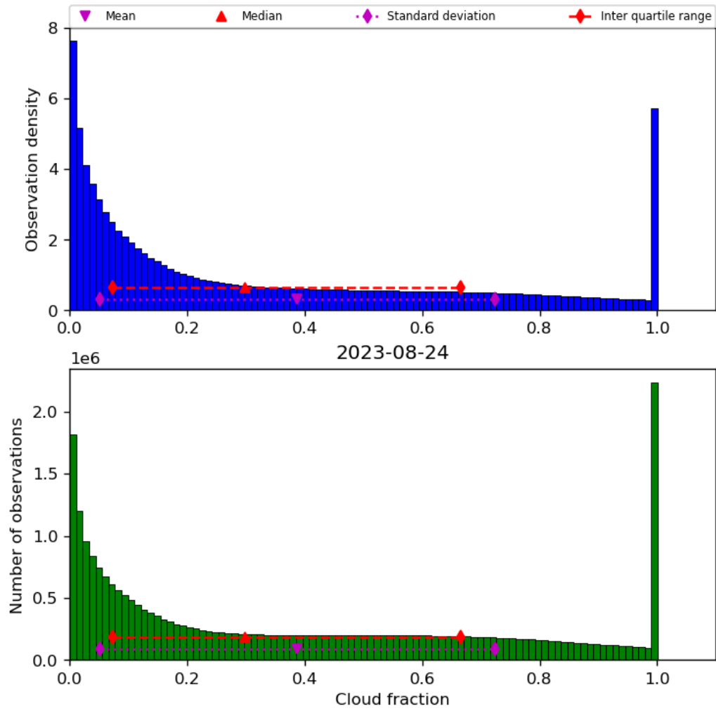
Figure 32: Histogram of “Cloud fraction” for 2023-08-23 to 2023-08-25
