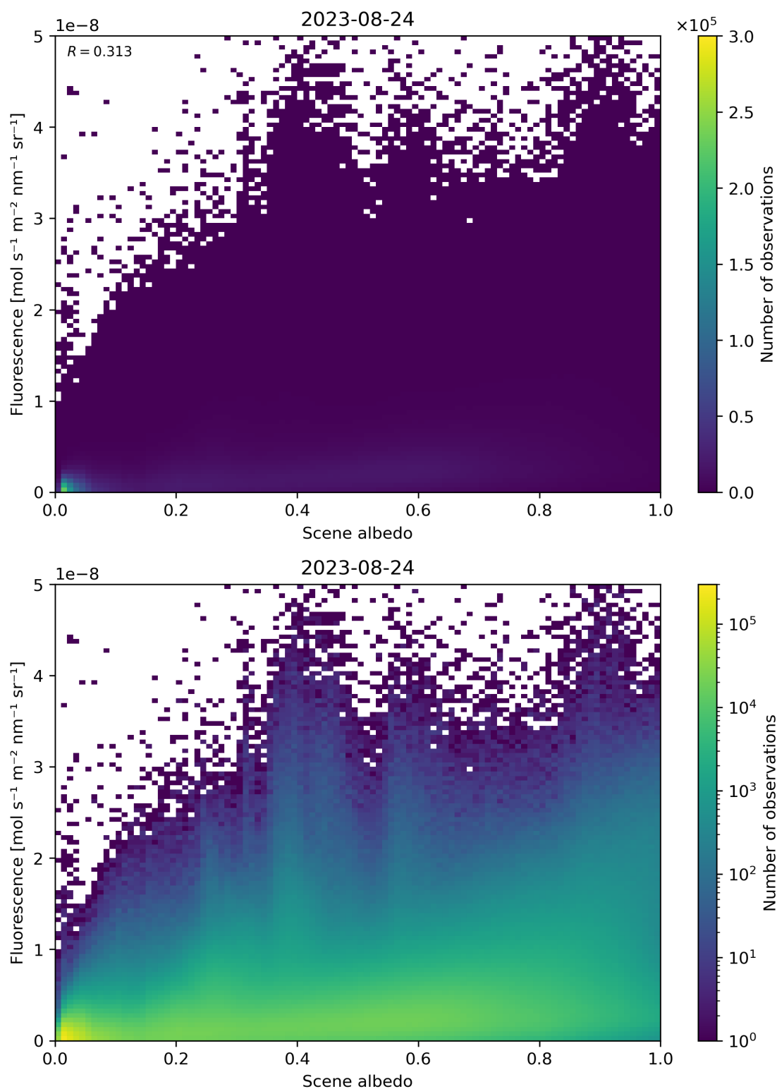
Figure 114: Scatter density plot of “Scene albedo” against “Fluorescence” for 2023-08-23 to 2023-08-25.
