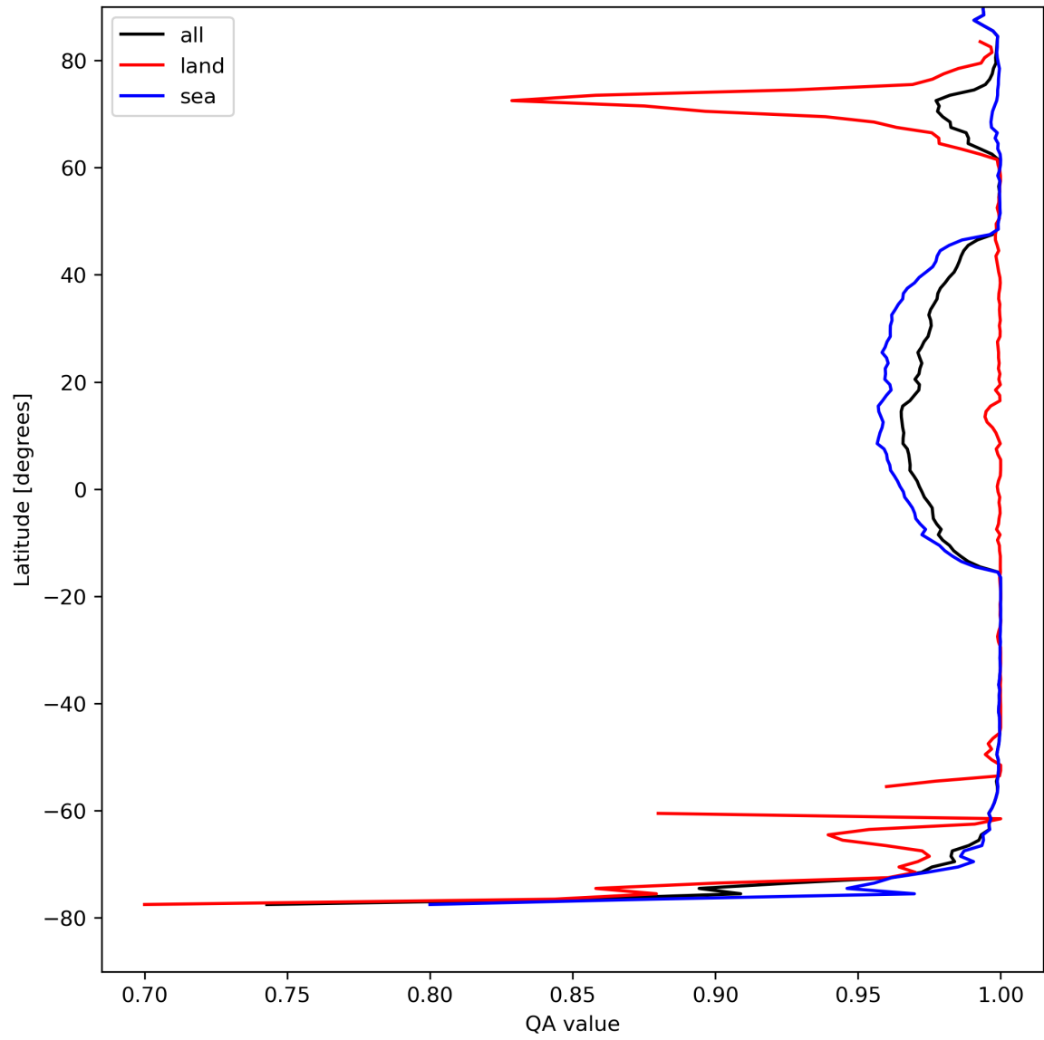
Figure 12: Zonal average of "QA value" for 2023-08-23 to 2023-08-25.
