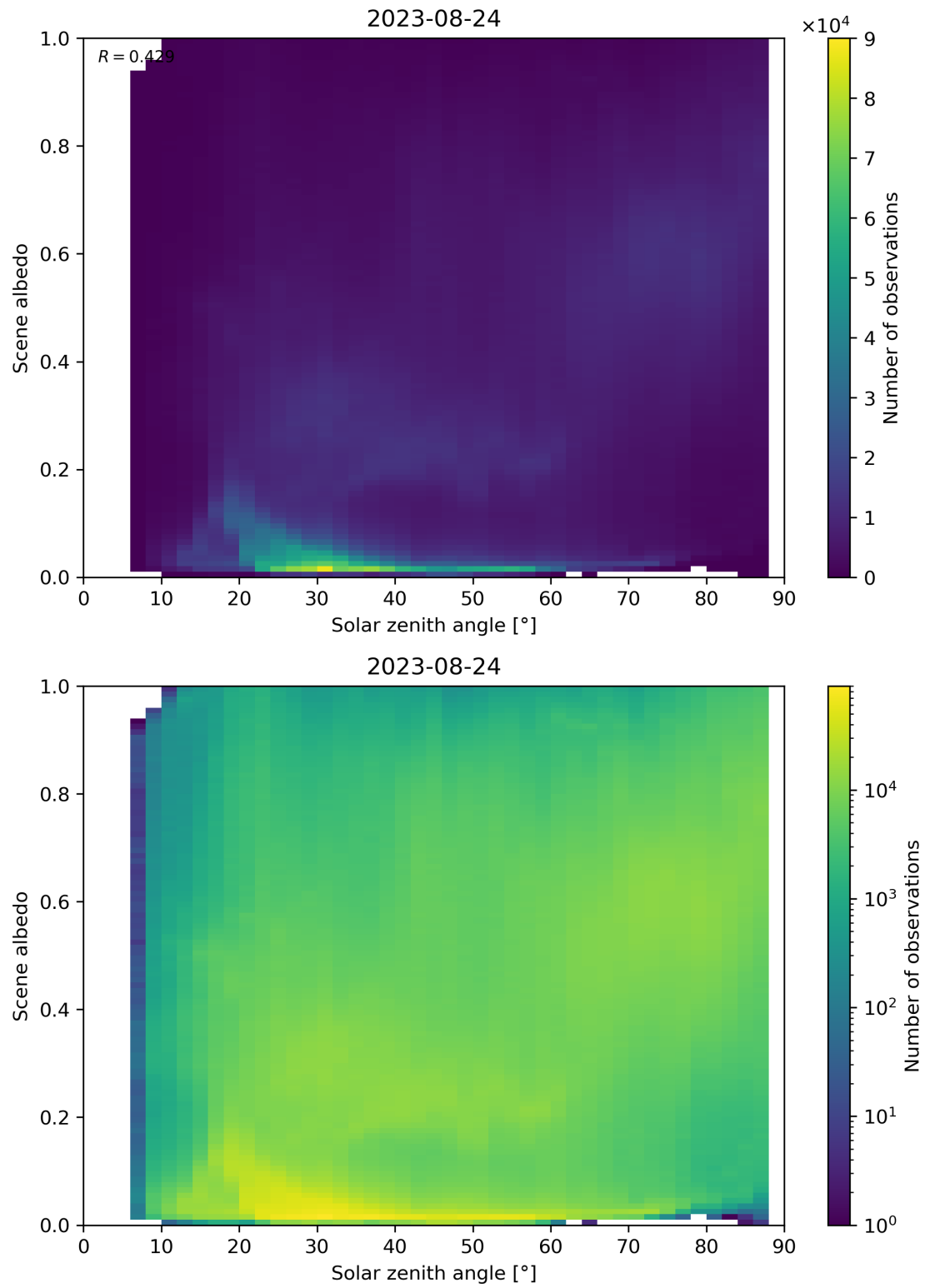
Figure 127: Scatter density plot of “Solar zenith angle” against “Scene albedo” for 2023-08-23 to 2023-08-25.
