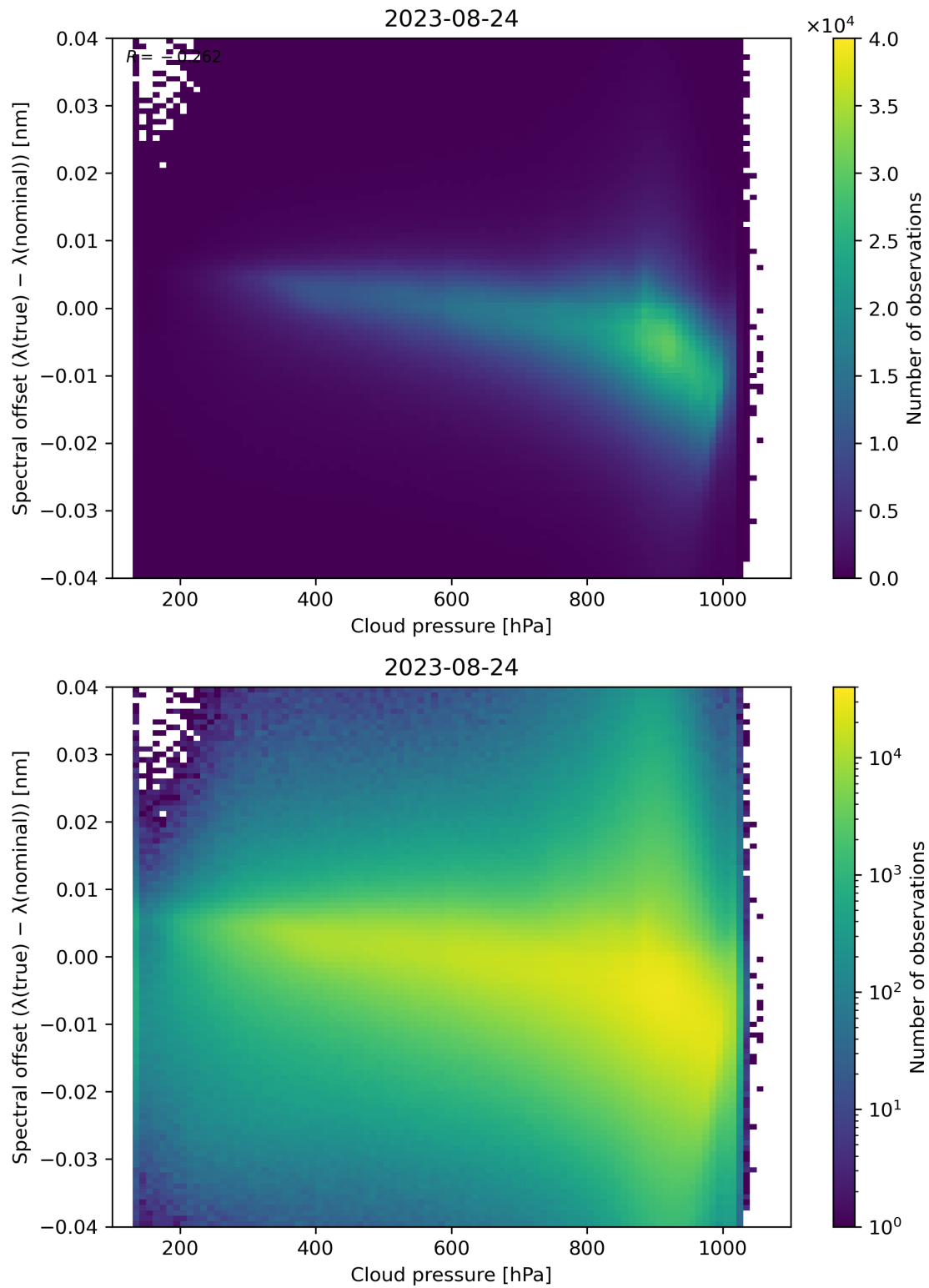
Figure 92: Scatter density plot of “Cloud pressure” against “Spectral offset ( \lambda(\text{true}) - \lambda(\text{nominal}) )” for 2023-08-23 to 2023-08-25.
