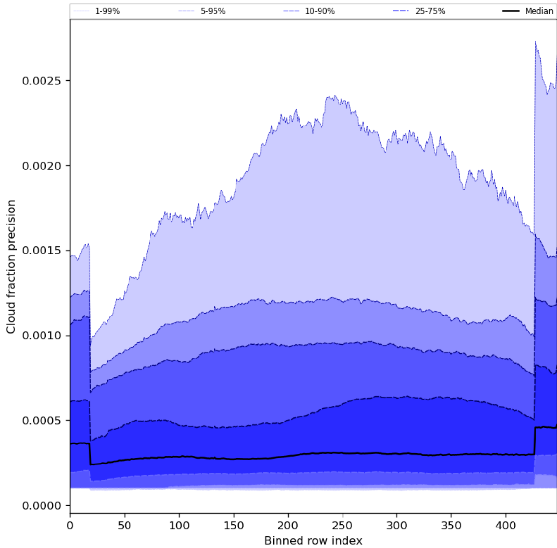
Figure 50: Along track statistics of “Cloud fraction precision” for 2023-08-23 to 2023-08-25
