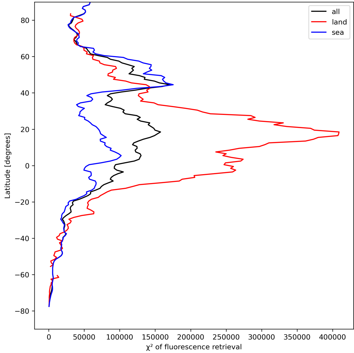
Figure 25: Zonal average of “ \chi^2 of fluorescence retrieval” for 2023-08-23 to 2023-08-25.
