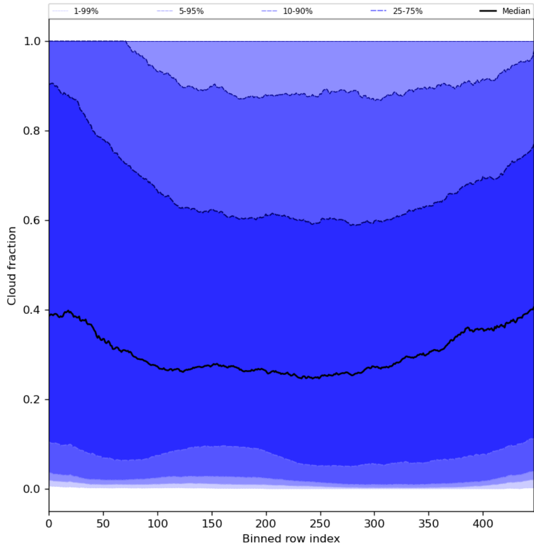
Figure 49: Along track statistics of “Cloud fraction” for 2023-08-23 to 2023-08-25
