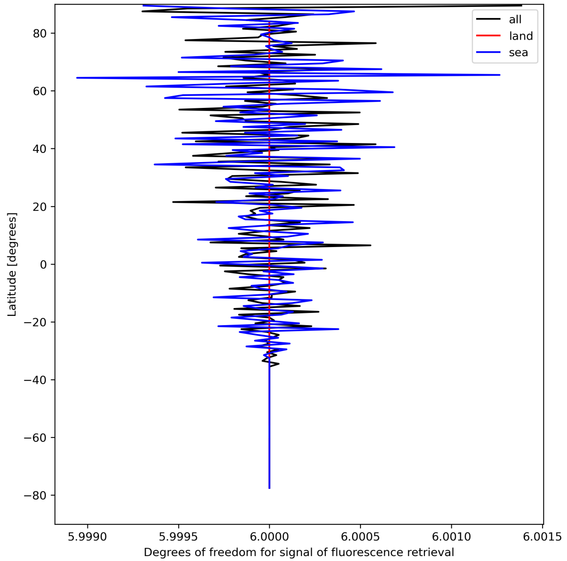
Figure 26: Zonal average of “Degrees of freedom for signal of fluorescence retrieval” for 2023-08-23 to 2023-08-25.
