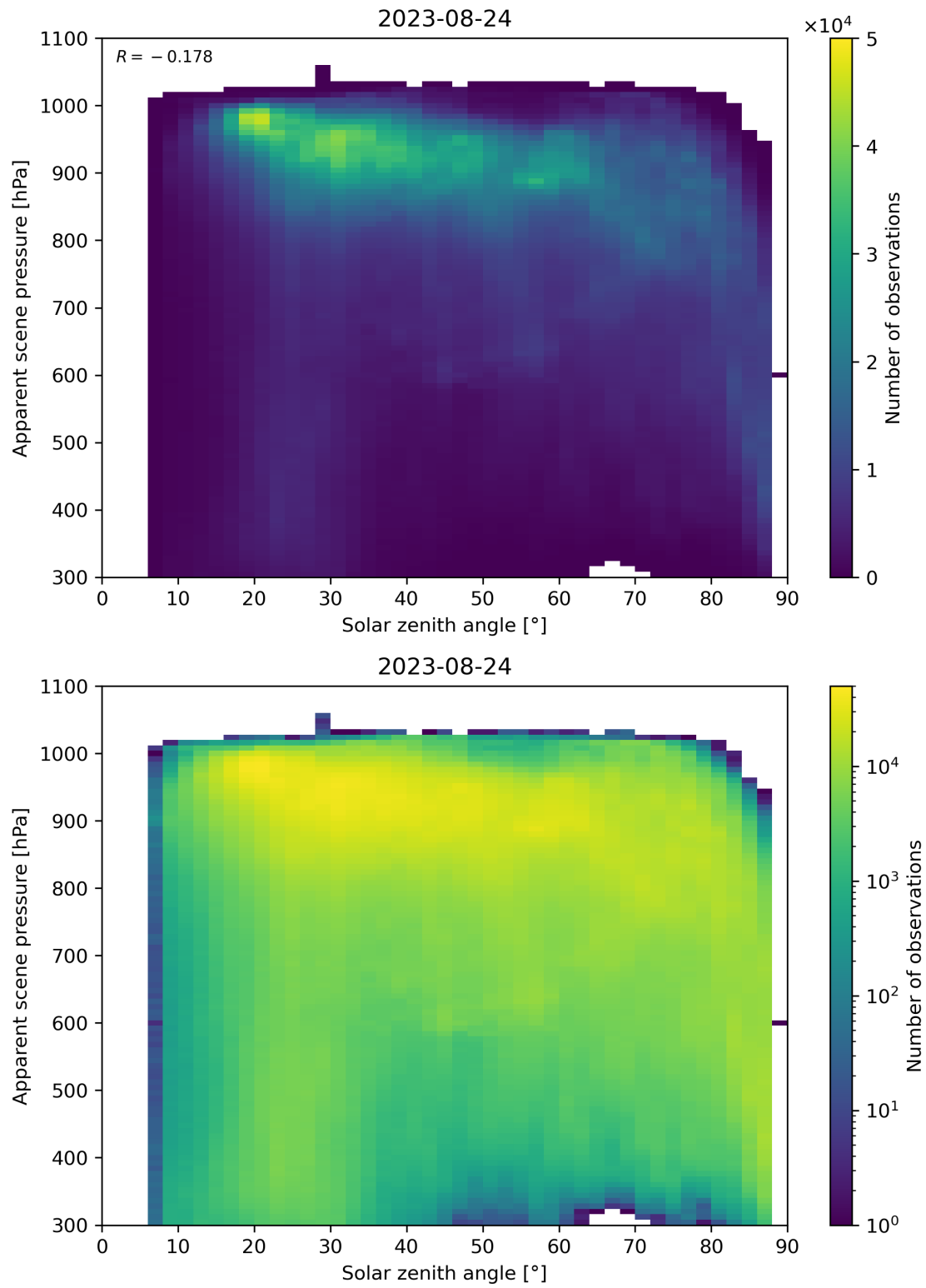
Figure 118: Scatter density plot of “Solar zenith angle” against “Apparent scene pressure” for 2023-08-23 to 2023-08-25.
