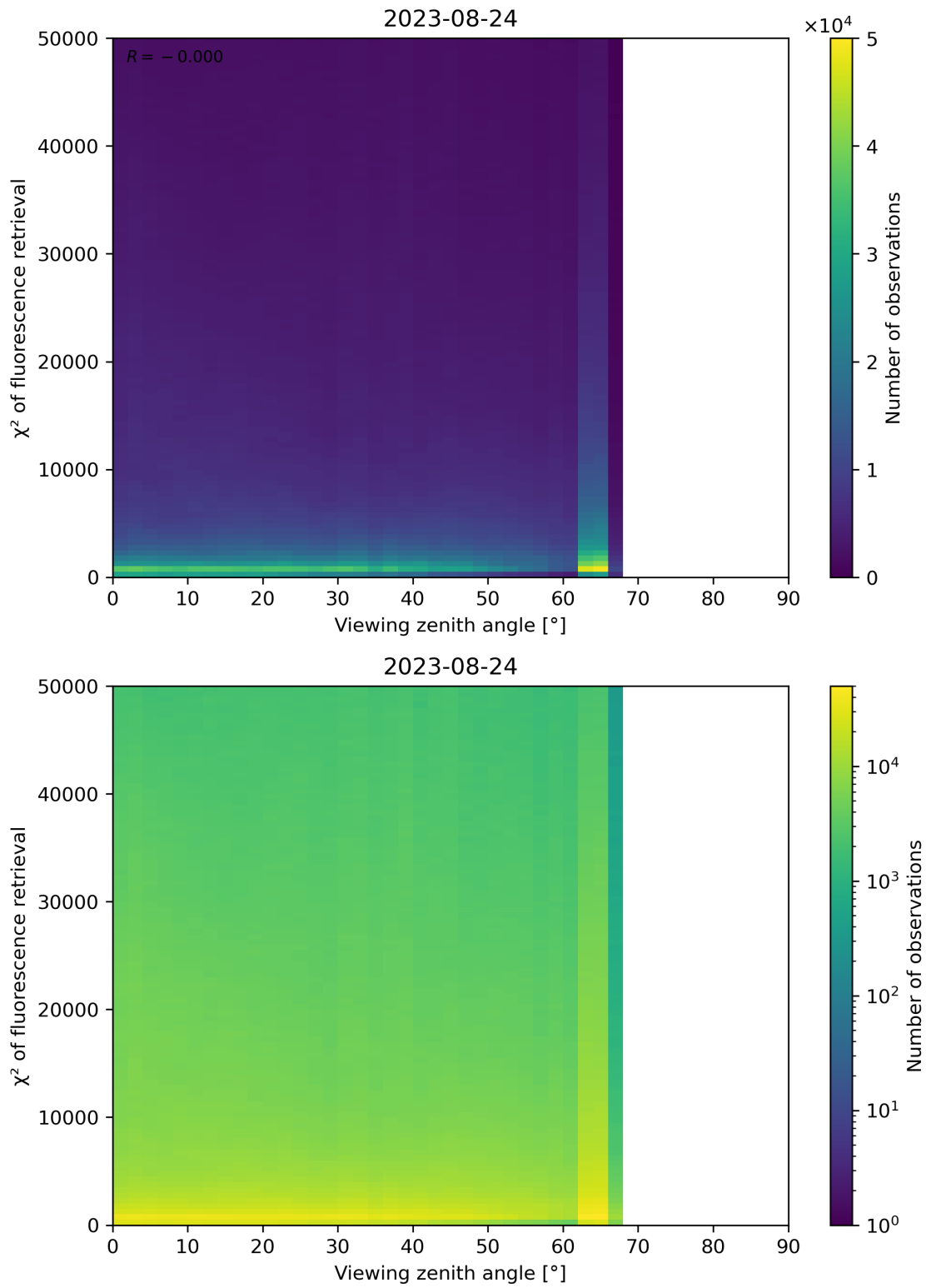
Figure 131: Scatter density plot of “Viewing zenith angle” against “ \chi^2 of fluorescence retrieval” for 2023-08-23 to 2023-08-25.
