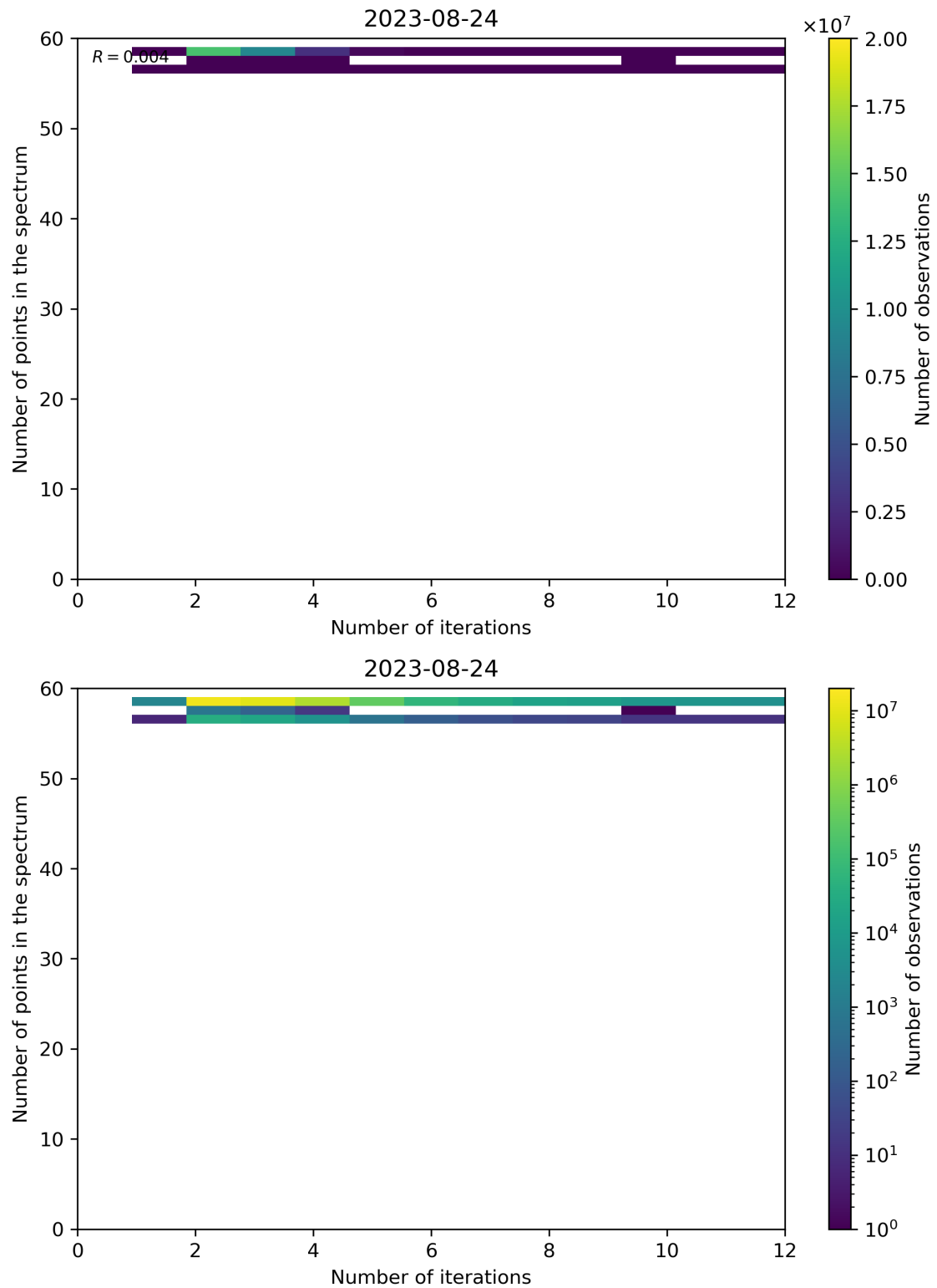
Figure 108: Scatter density plot of “Number of iterations” against “Number of points in the spectrum” for 2023-08-23 to 2023-08-25.
