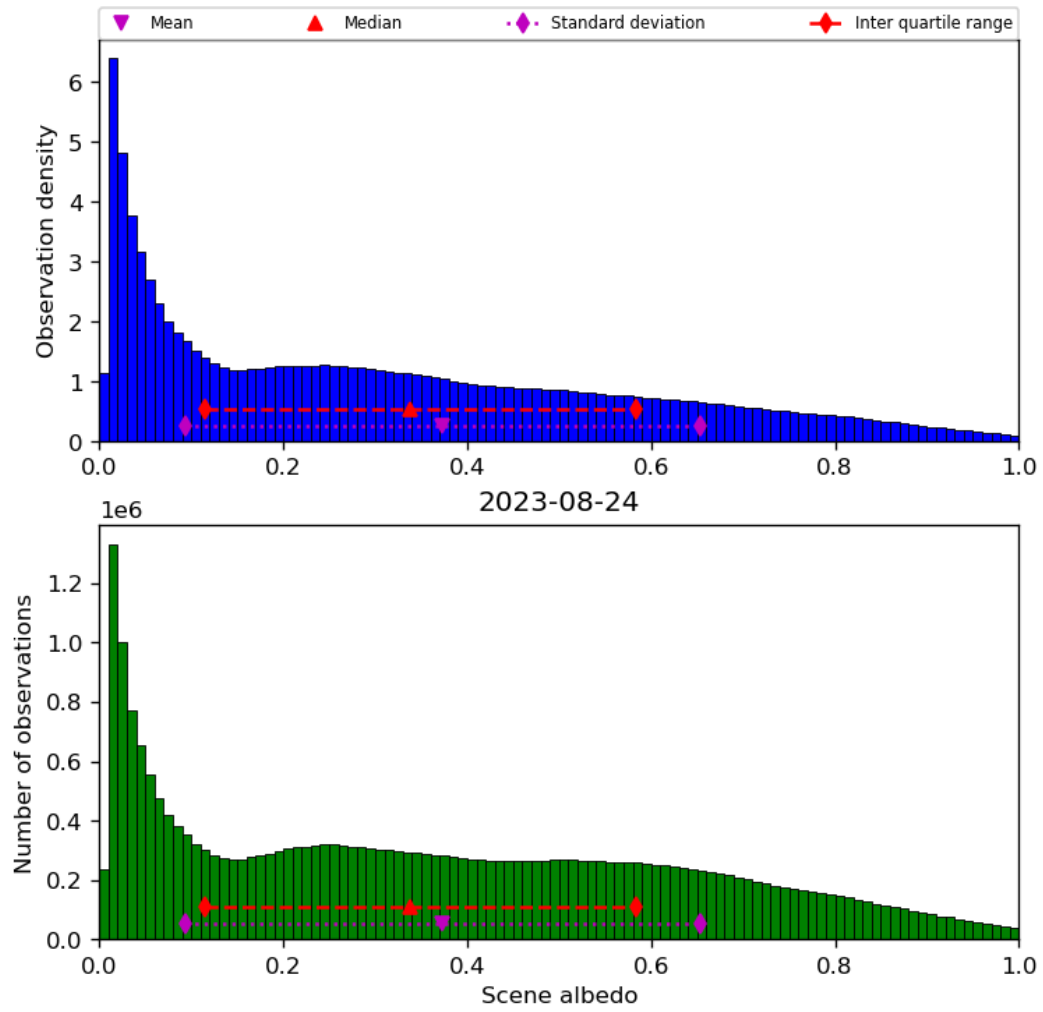
Figure 34: Histogram of “Scene albedo” for 2023-08-23 to 2023-08-25
