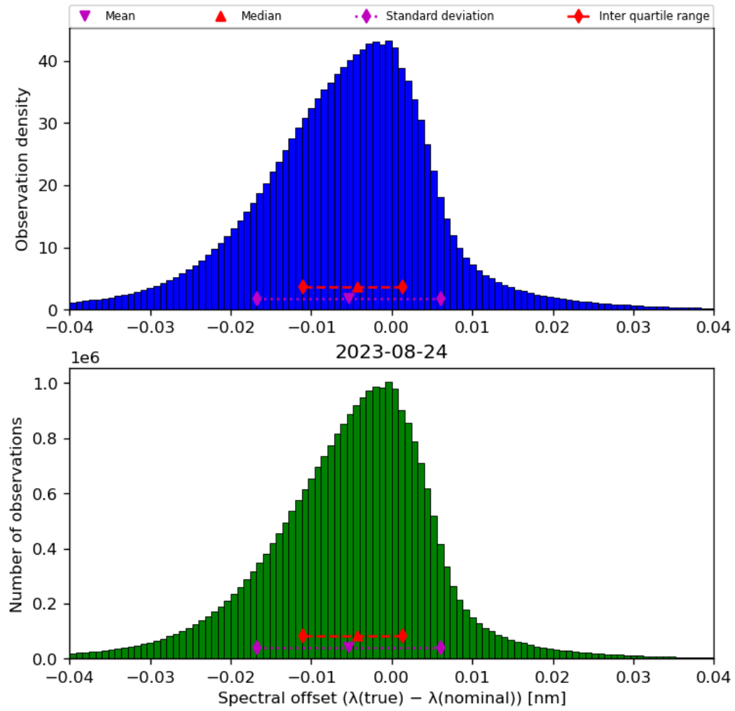
Figure 45: Histogram of “Spectral offset ( \lambda(\text{true}) - \lambda(\text{nominal}) )” for 2023-08-23 to 2023-08-25
