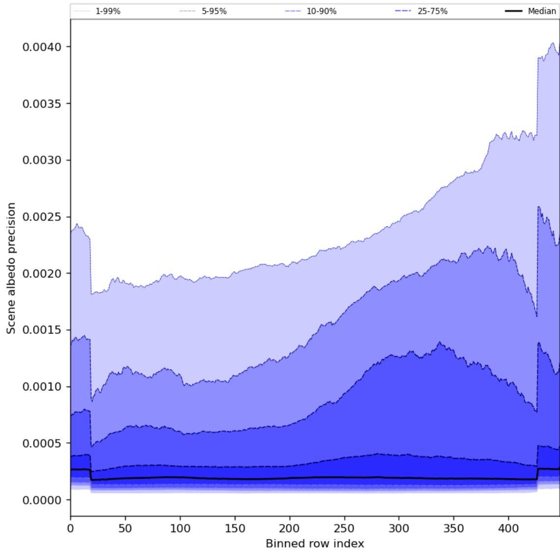
Figure 52: Along track statistics of “Scene albedo precision” for 2023-08-23 to 2023-08-25
