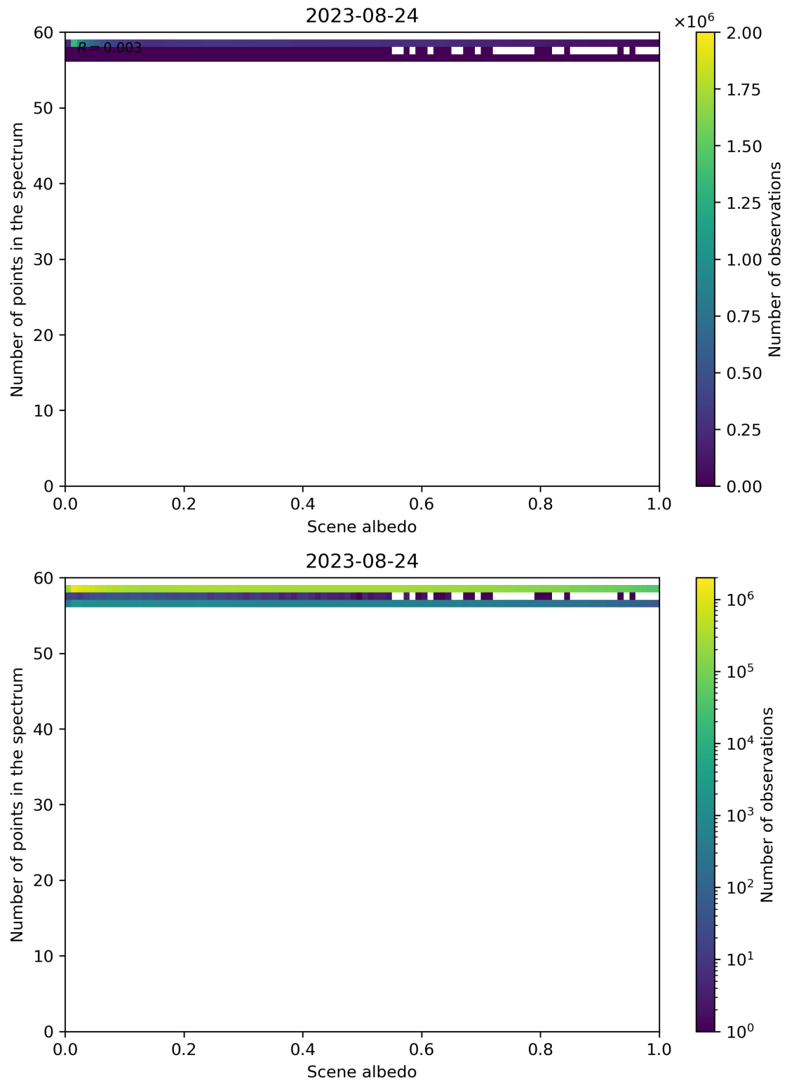
Figure 116: Scatter density plot of “Scene albedo” against “Number of points in the spectrum” for 2023-08-23 to 2023-08-25.
