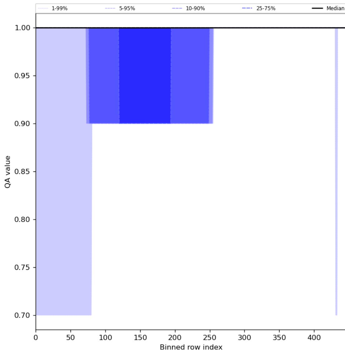
Figure 46: Along track statistics of “QA value” for 2023-08-23 to 2023-08-25
