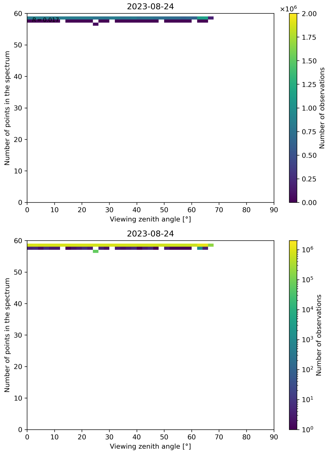
Figure 137: Scatter density plot of “Viewing zenith angle” against “Number of points in the spectrum” for 2023-08-23 to 2023-08-25.
