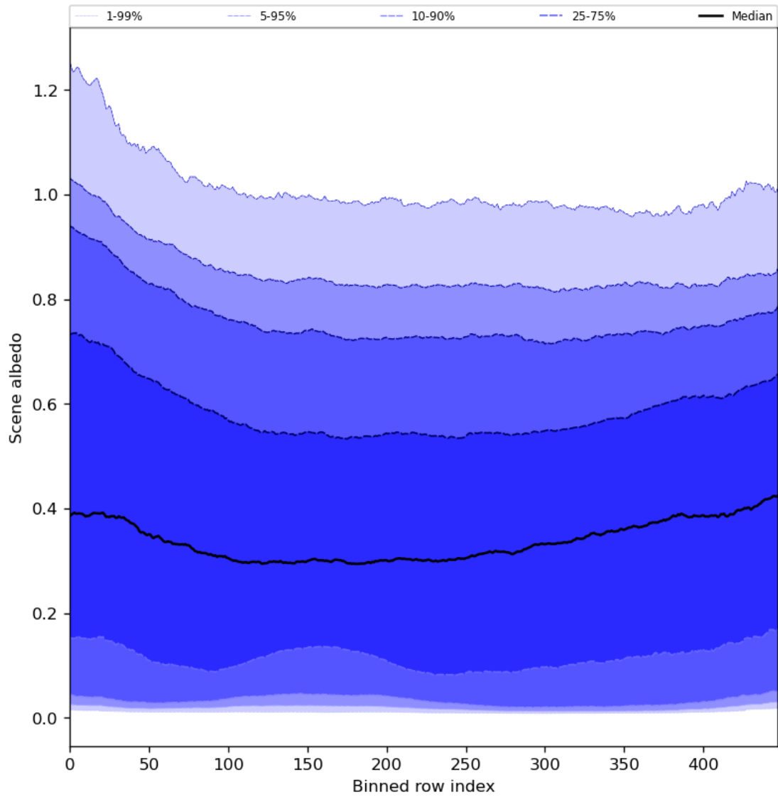
Figure 51: Along track statistics of “Scene albedo” for 2023-08-23 to 2023-08-25
