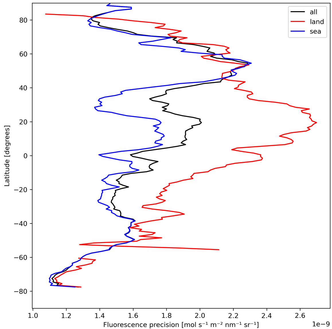
Figure 24: Zonal average of “Fluorescence precision” for 2023-08-23 to 2023-08-25.
