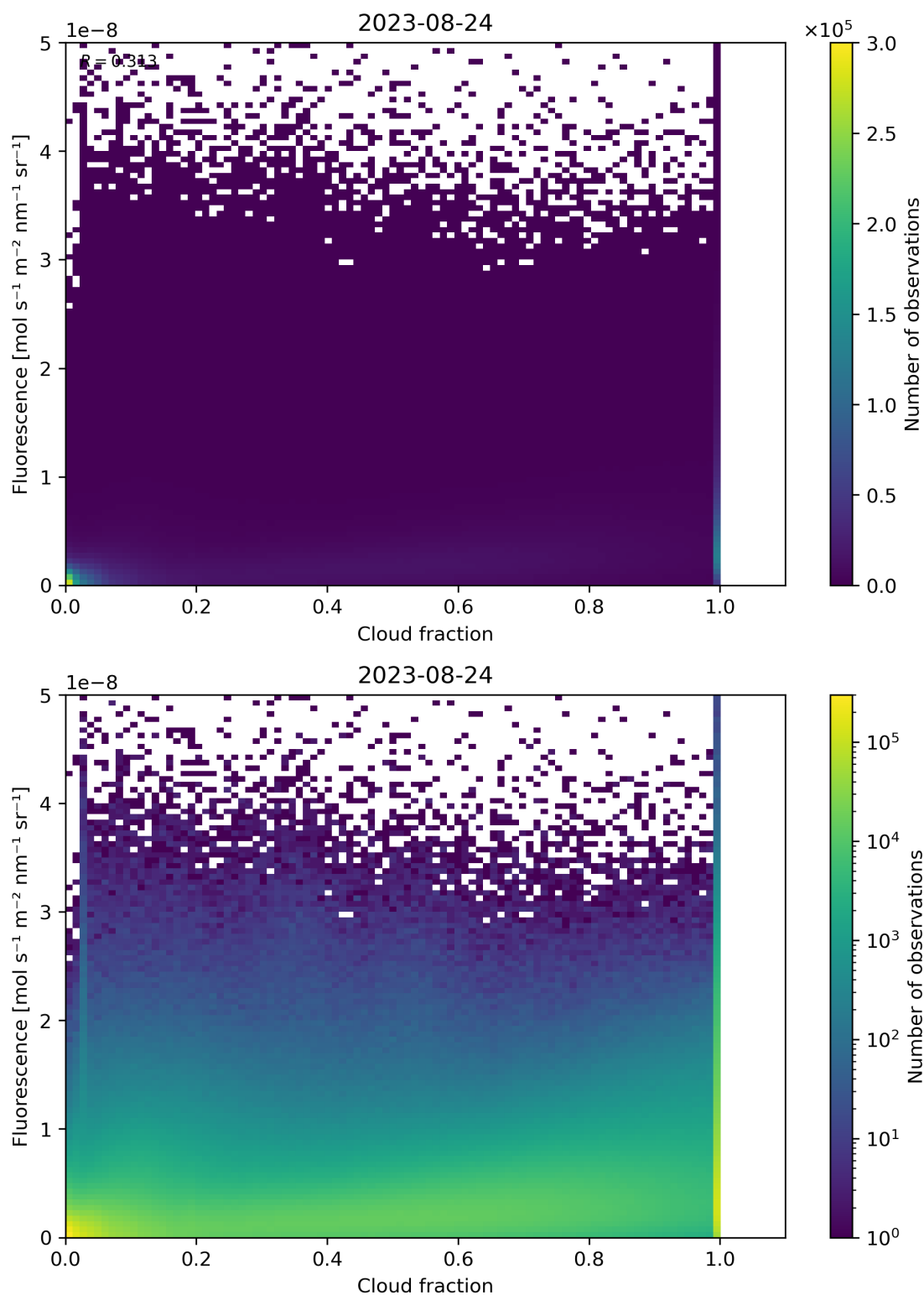
Figure 79: Scatter density plot of “Cloud fraction” against “Fluorescence” for 2023-08-23 to 2023-08-25.
