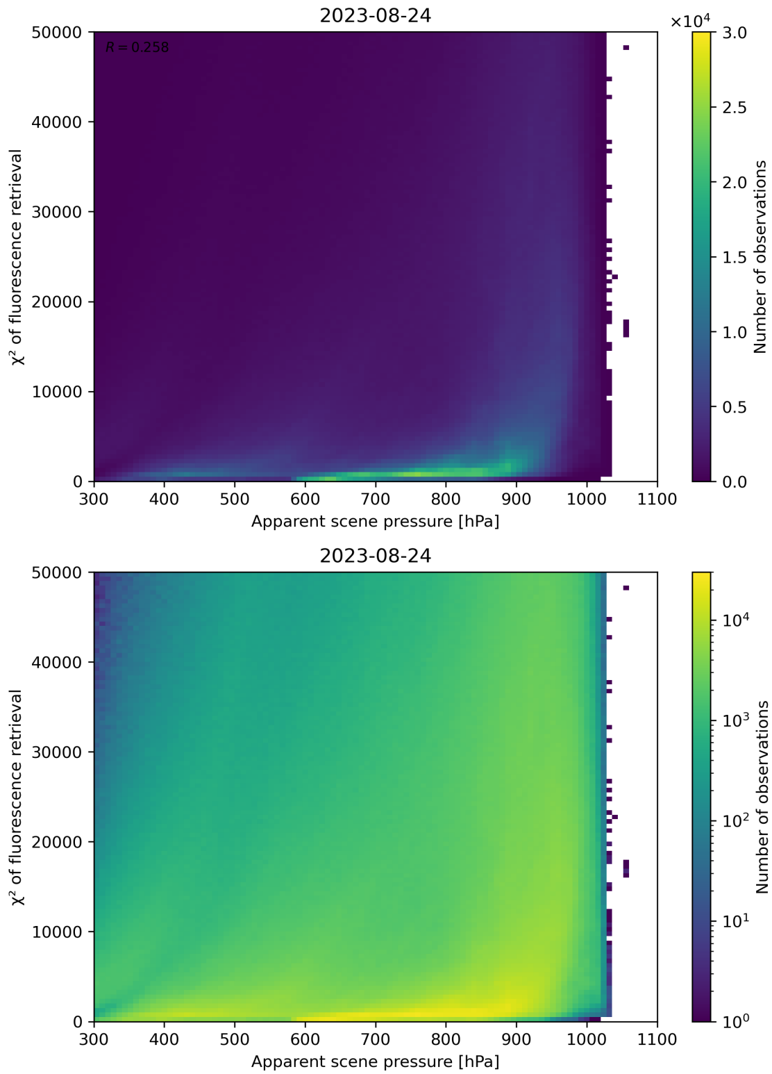
Figure 64: Scatter density plot of “Apparent scene pressure” against “ \chi^2 of fluorescence retrieval” for 2023-08-23 to 2023-08-25.
