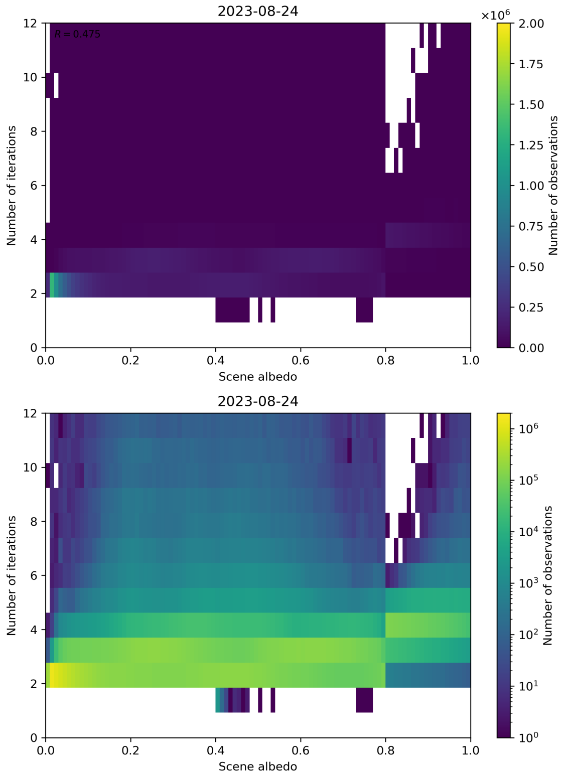
Figure 115: Scatter density plot of “Scene albedo” against “Number of iterations” for 2023-08-23 to 2023-08-25.
