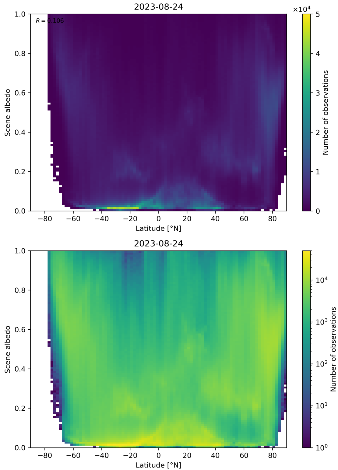
Figure 104: Scatter density plot of “Latitude” against “Scene albedo” for 2023-08-23 to 2023-08-25.
