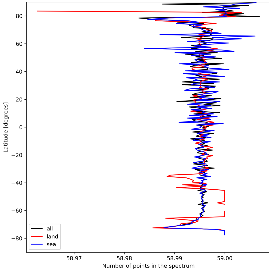
Figure 27: Zonal average of “Number of points in the spectrum” for 2023-08-23 to 2023-08-25.
