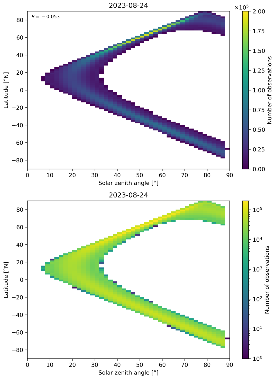
Figure 124: Scatter density plot of “Solar zenith angle” against “Latitude” for 2023-08-23 to 2023-08-25.
