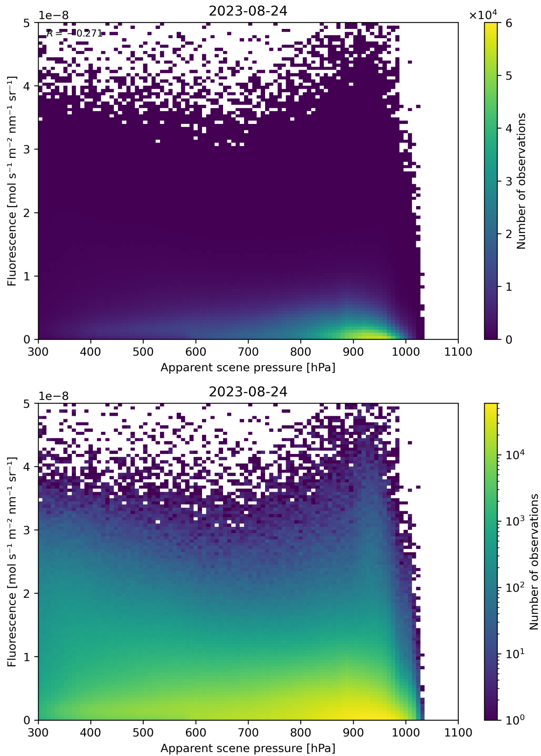
Figure 65: Scatter density plot of “Apparent scene pressure” against “Fluorescence” for 2023-08-23 to 2023-08-25.
