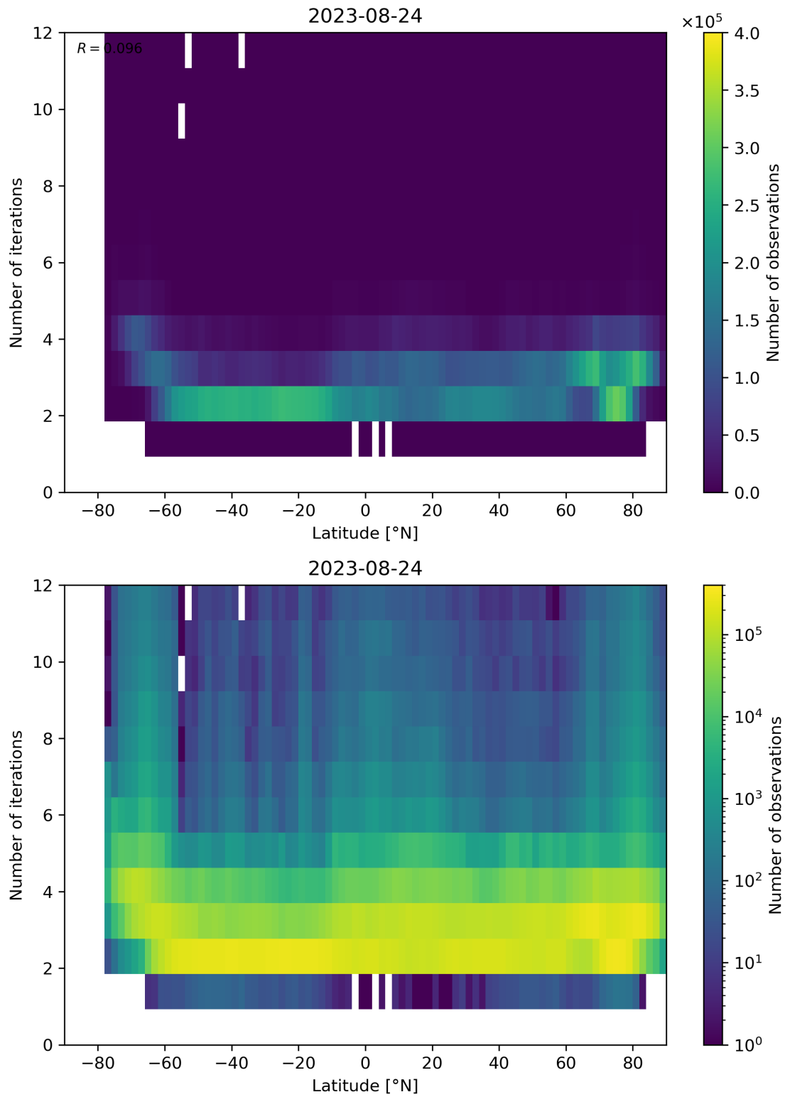
Figure 102: Scatter density plot of “Latitude” against “Number of iterations” for 2023-08-23 to 2023-08-25.
