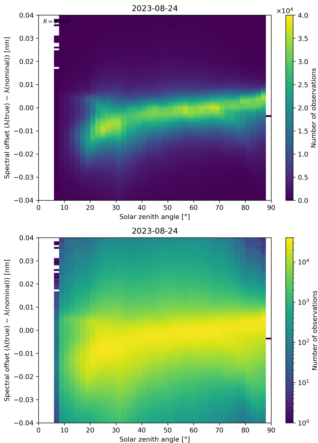
Figure 128: Scatter density plot of “Solar zenith angle” against “Spectral offset ( \lambda(\text{true}) - \lambda(\text{nominal}) )” for 2023-08-23 to 2023-08-25.
