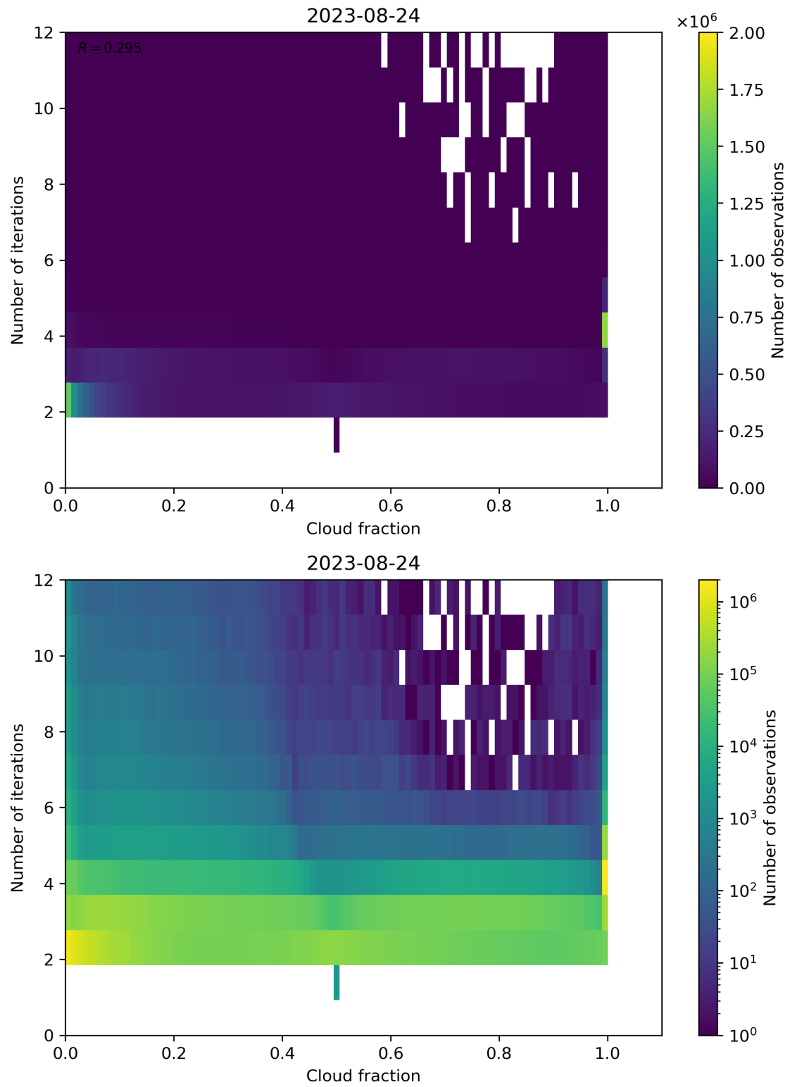
Figure 80: Scatter density plot of “Cloud fraction” against “Number of iterations” for 2023-08-23 to 2023-08-25.
