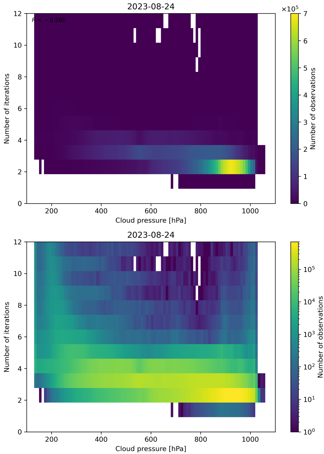
Figure 89: Scatter density plot of “Cloud pressure” against “Number of iterations” for 2023-08-23 to 2023-08-25.
