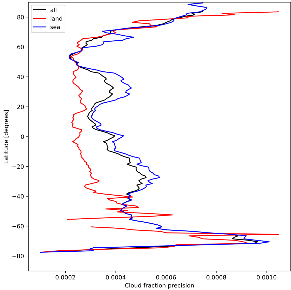
Figure 16: Zonal average of “Cloud fraction precision” for 2023-08-23 to 2023-08-25.
