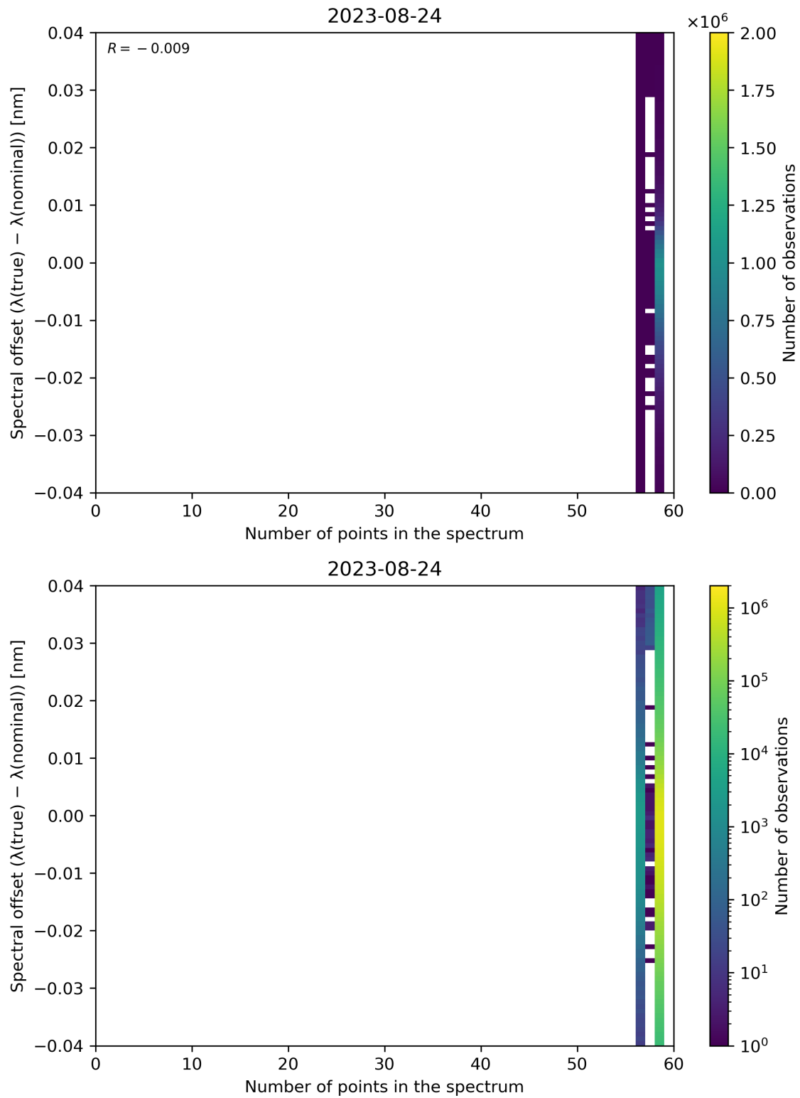
Figure 110: Scatter density plot of “Number of points in the spectrum” against “Spectral offset ( \lambda(\text{true}) - \lambda(\text{nominal}) )” for 2023-08-23 to 2023-08-25.
