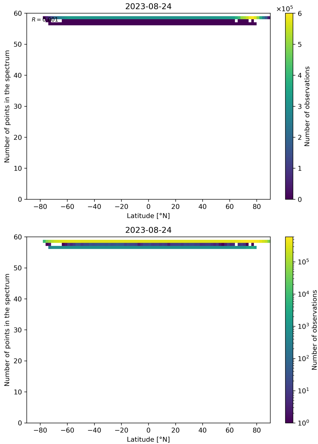
Figure 103: Scatter density plot of “Latitude” against “Number of points in the spectrum” for 2023-08-23 to 2023-08-25.
