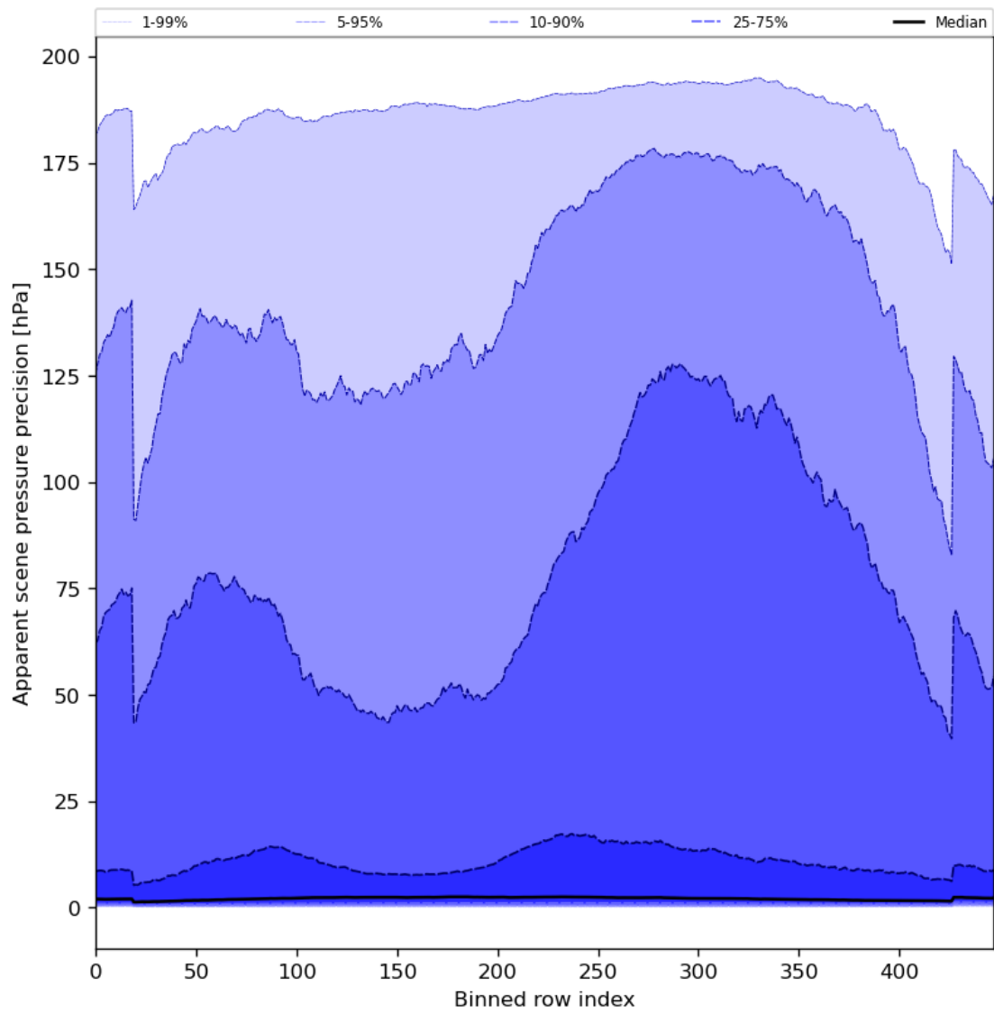
Figure 54: Along track statistics of “Apparent scene pressure precision” for 2023-08-23 to 2023-08-25
