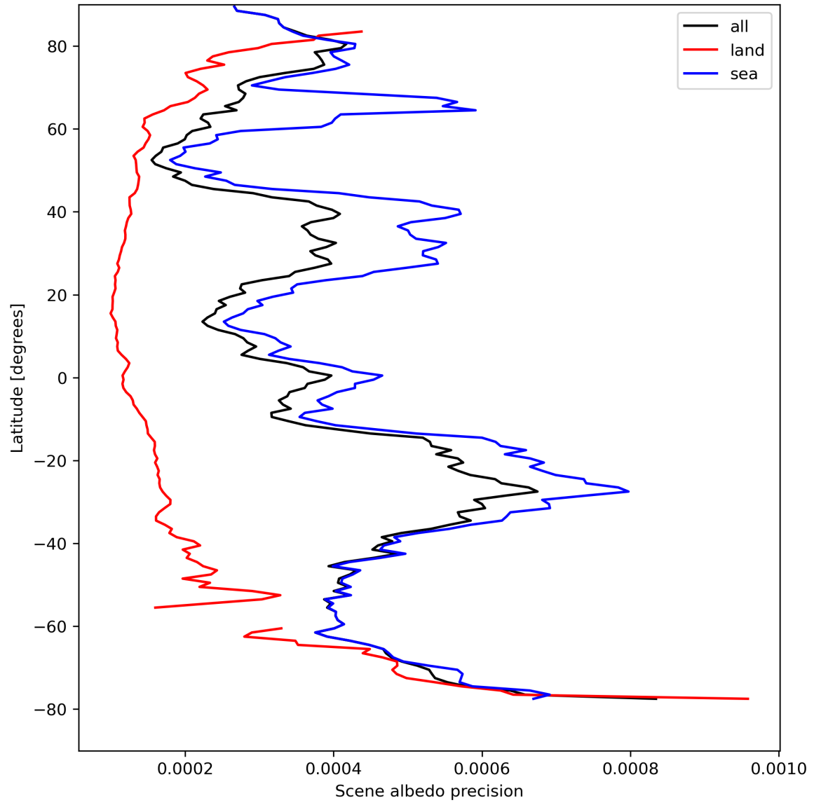
Figure 18: Zonal average of “Scene albedo precision” for 2023-08-23 to 2023-08-25.
