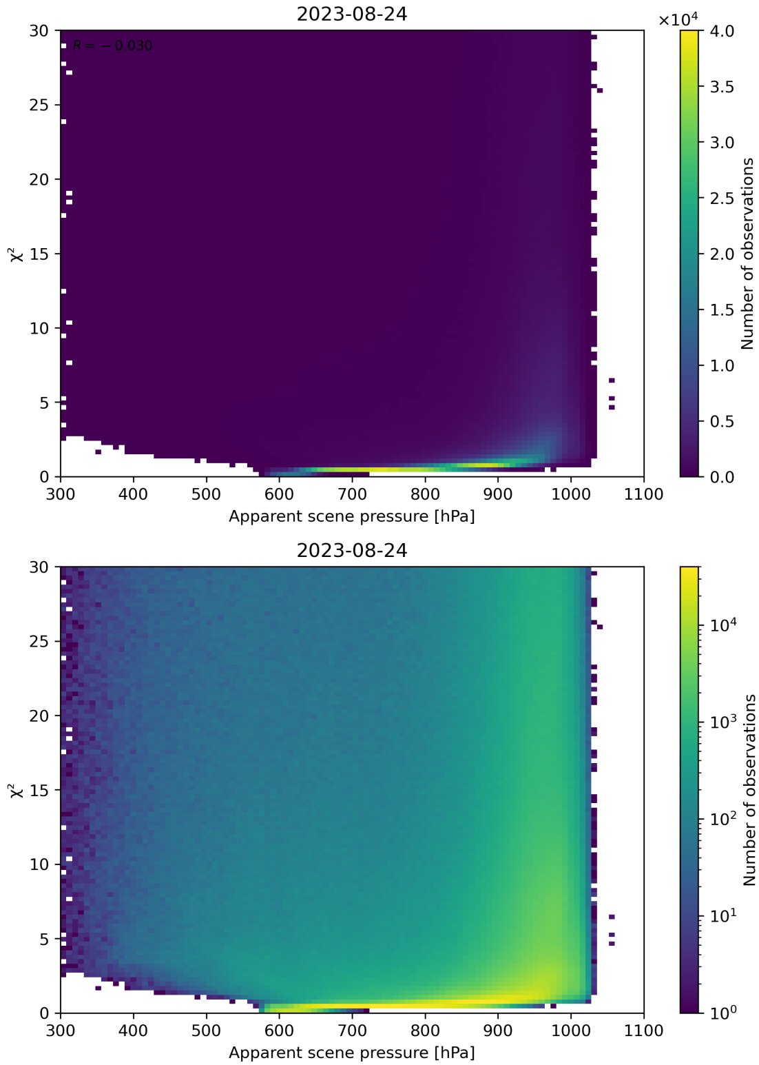
Figure 63: Scatter density plot of “Apparent scene pressure” against “ \chi^2 ” for 2023-08-23 to 2023-08-25.
