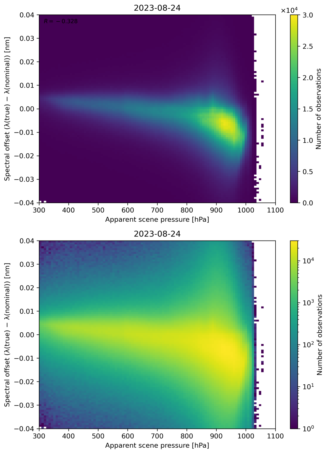
Figure 68: Scatter density plot of “Apparent scene pressure” against “Spectral offset ( \lambda(\text{true}) - \lambda(\text{nominal}) )” for 2023-08-23 to 2023-08-25.
