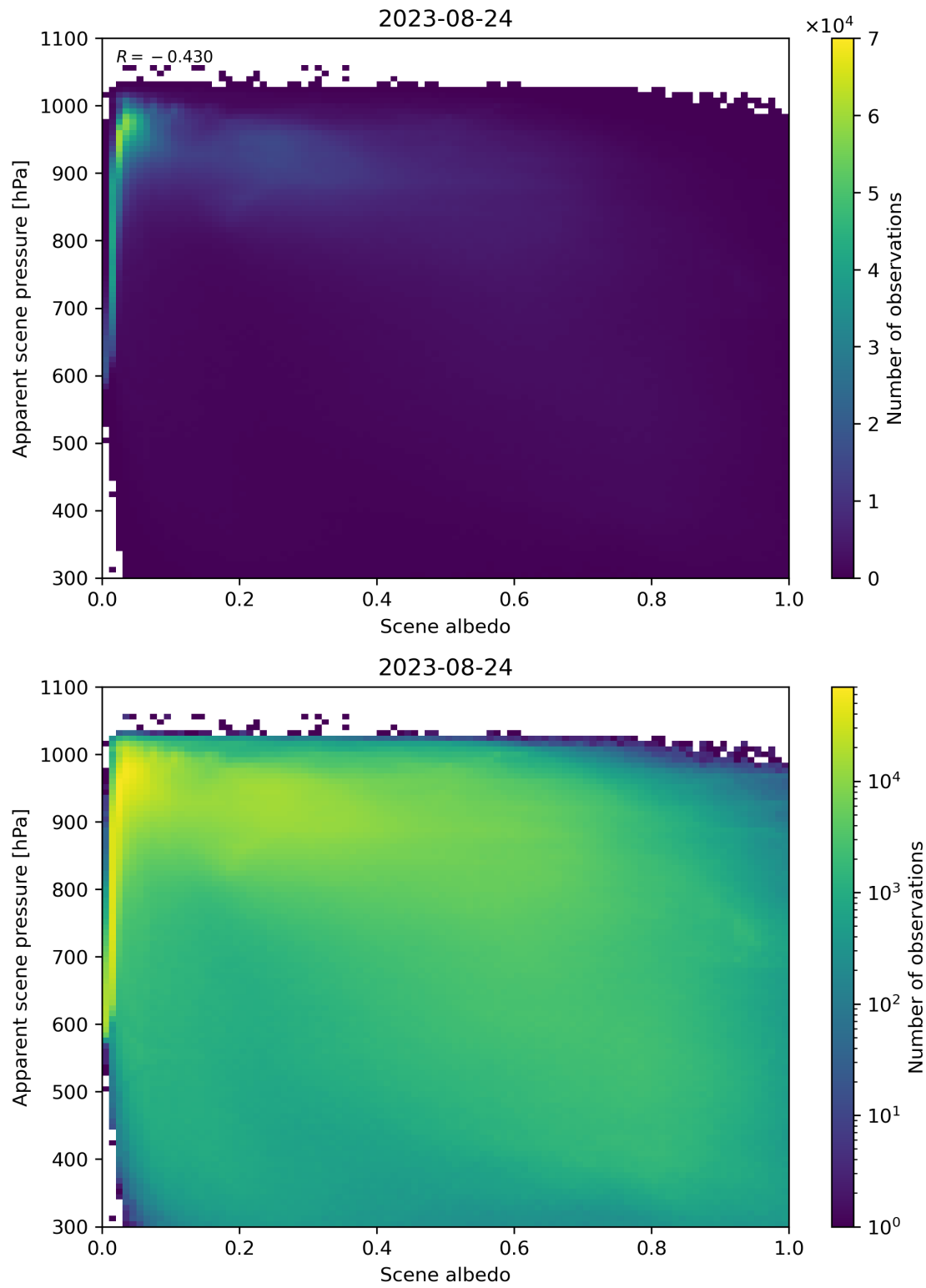
Figure 111: Scatter density plot of “Scene albedo” against “Apparent scene pressure” for 2023-08-23 to 2023-08-25.
