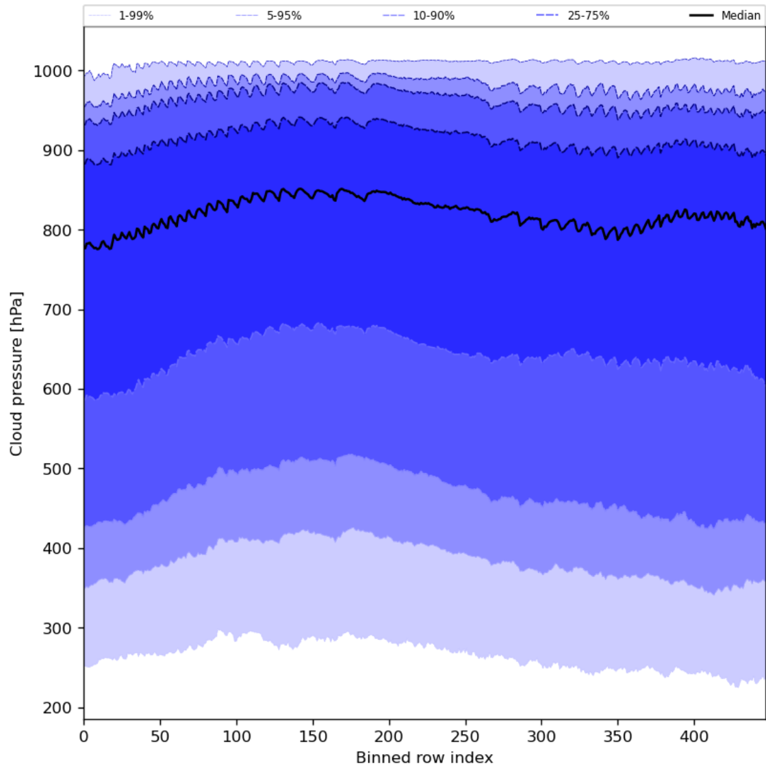
Figure 47: Along track statistics of “Cloud pressure” for 2023-08-23 to 2023-08-25
