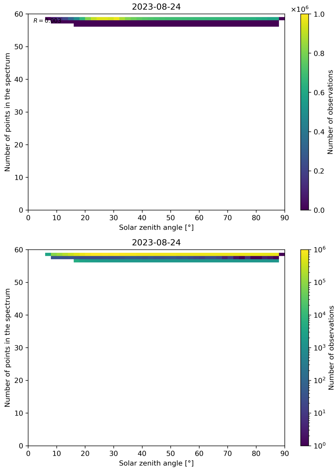
Figure 126: Scatter density plot of “Solar zenith angle” against “Number of points in the spectrum” for 2023-08-23 to 2023-08-25.
