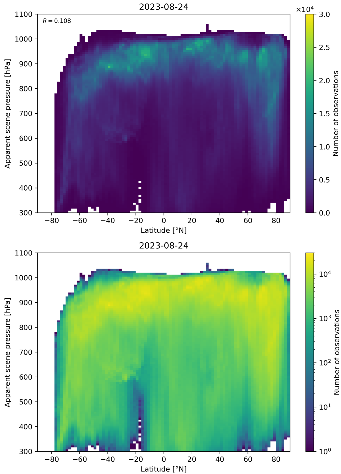
Figure 96: Scatter density plot of “Latitude” against “Apparent scene pressure” for 2023-08-23 to 2023-08-25.
