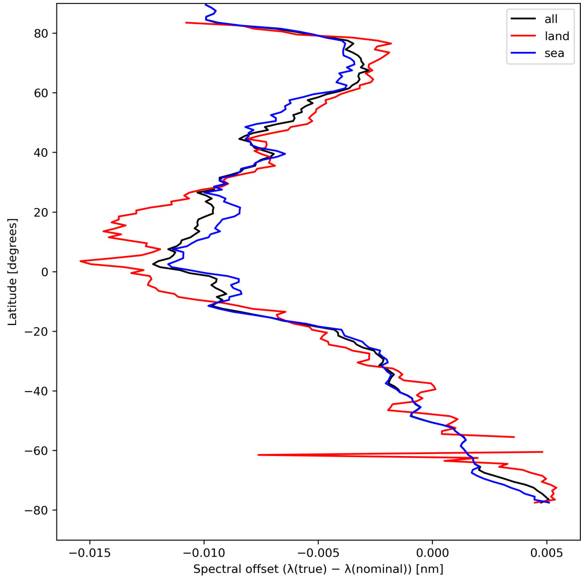
Figure 28: Zonal average of “Spectral offset ( \lambda(\text{true}) - \lambda(\text{nominal}) )” for 2023-08-23 to 2023-08-25.
