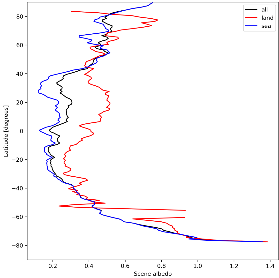
Figure 17: Zonal average of “Scene albedo” for 2023-08-23 to 2023-08-25.
