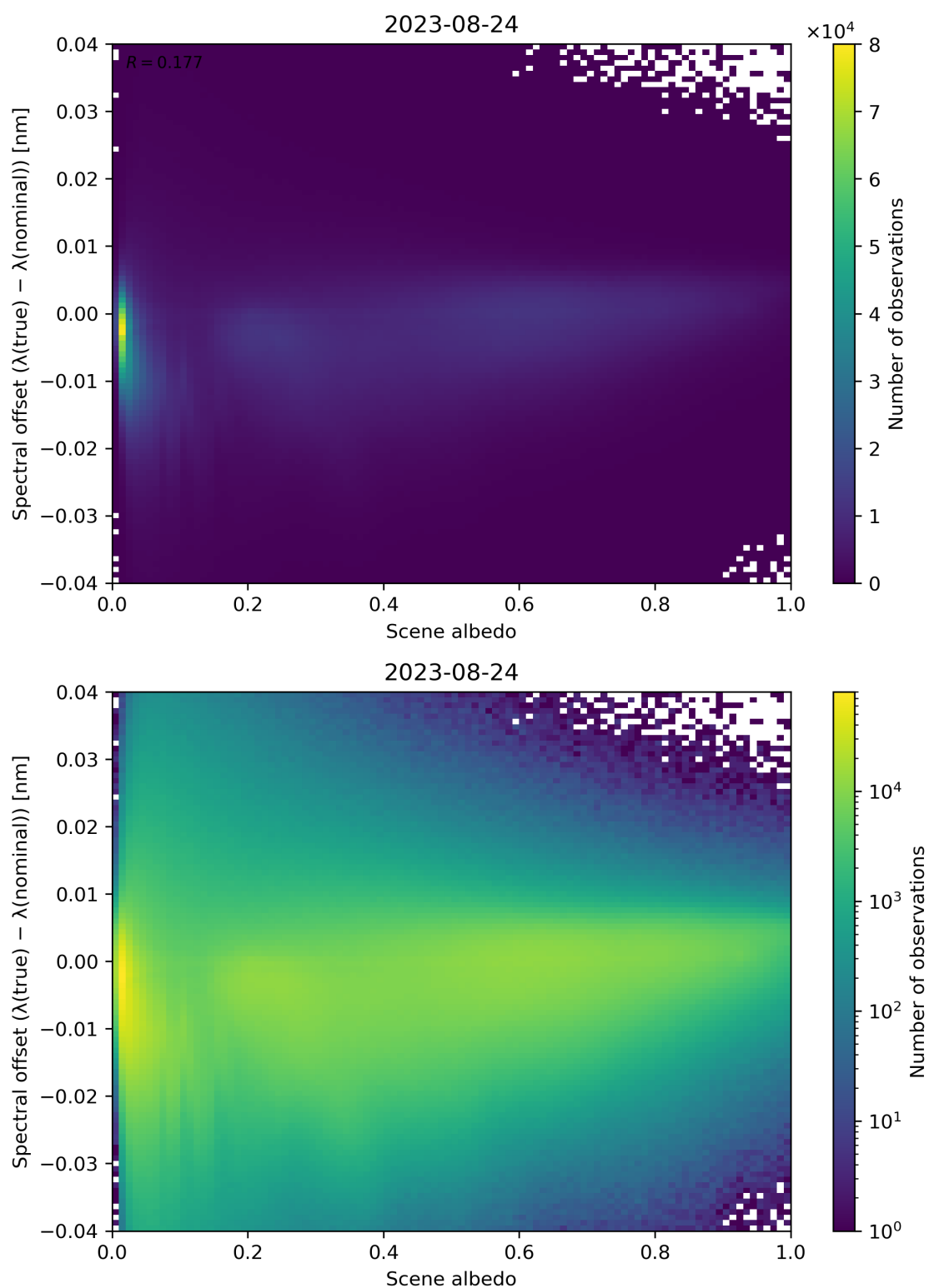
Figure 117: Scatter density plot of “Scene albedo” against “Spectral offset ( \lambda(\text{true}) - \lambda(\text{nominal}) )” for 2023-08-23 to 2023-08-25.
