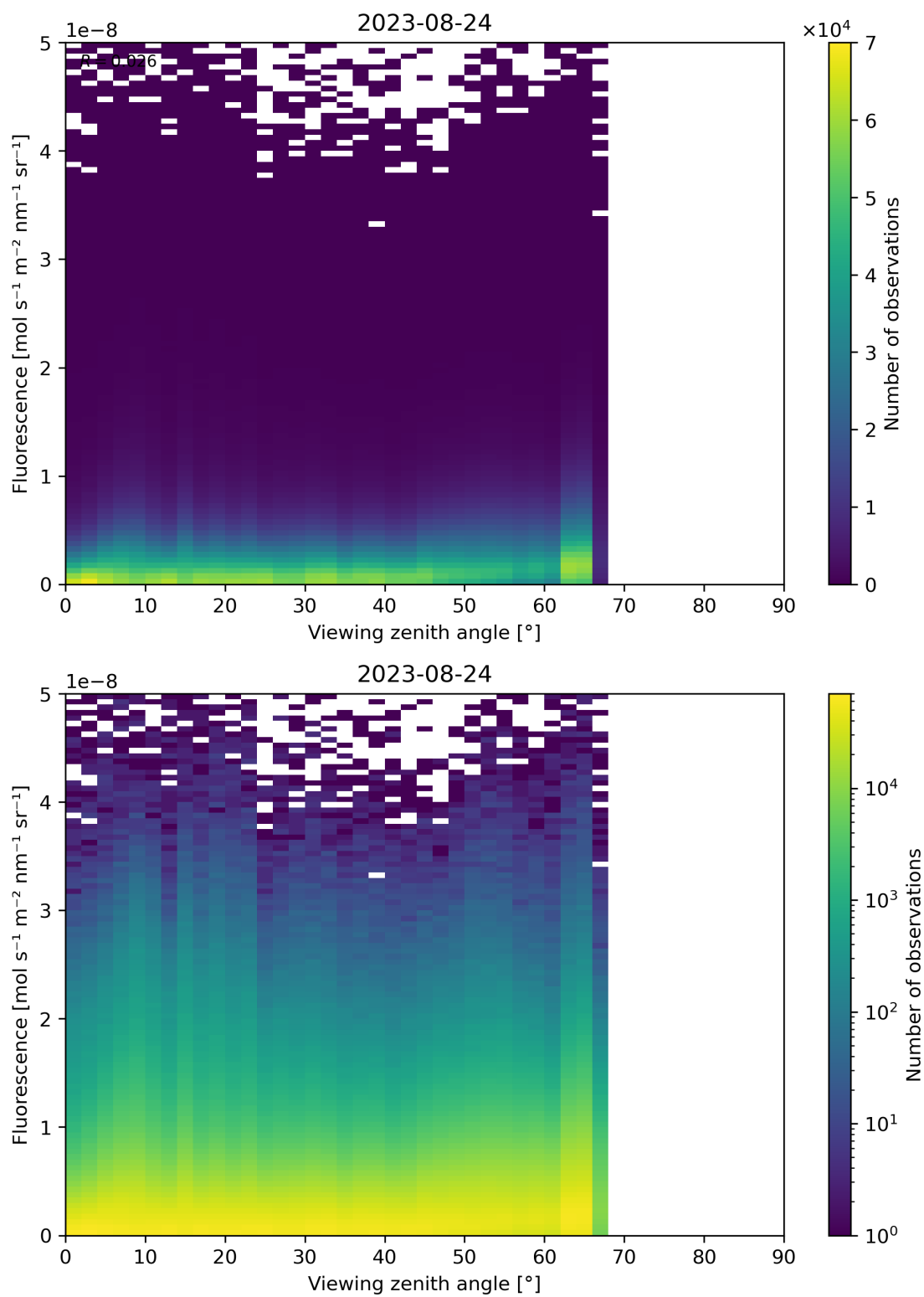
Figure 134: Scatter density plot of “Viewing zenith angle” against “Fluorescence” for 2023-08-23 to 2023-08-25.
