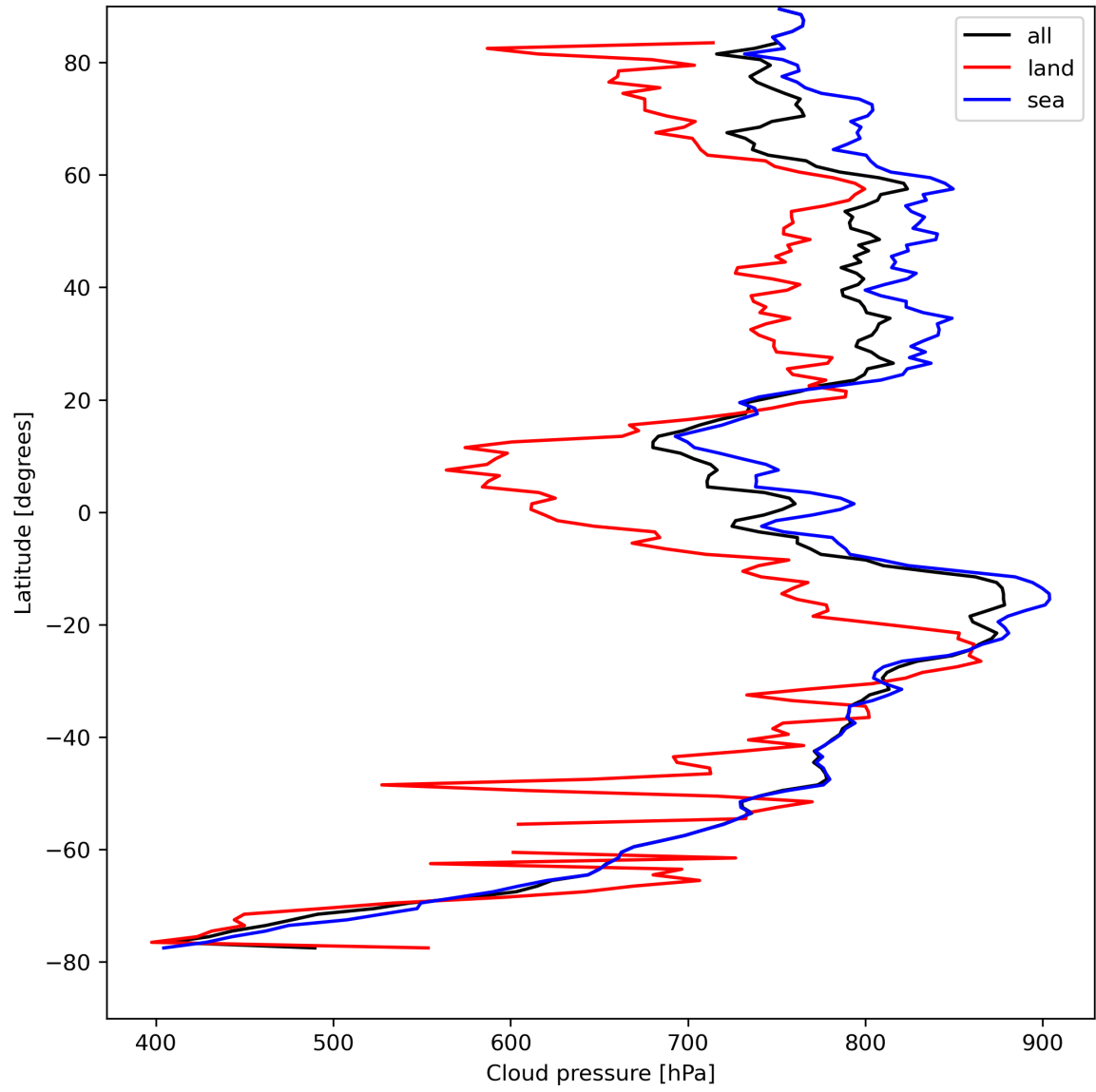
Figure 13: Zonal average of “Cloud pressure” for 2023-08-23 to 2023-08-25.
