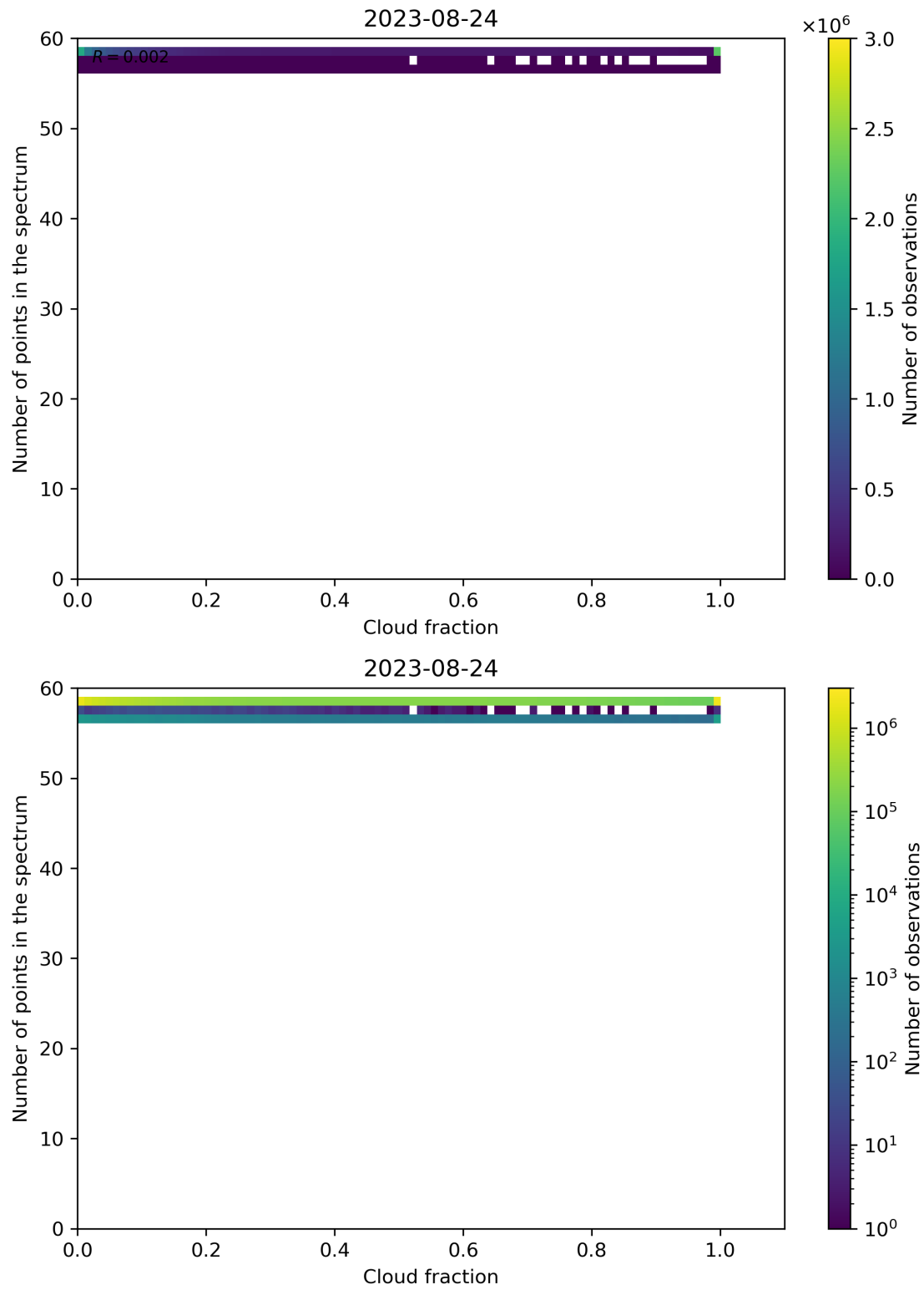
Figure 81: Scatter density plot of “Cloud fraction” against “Number of points in the spectrum” for 2023-08-23 to 2023-08-25.
