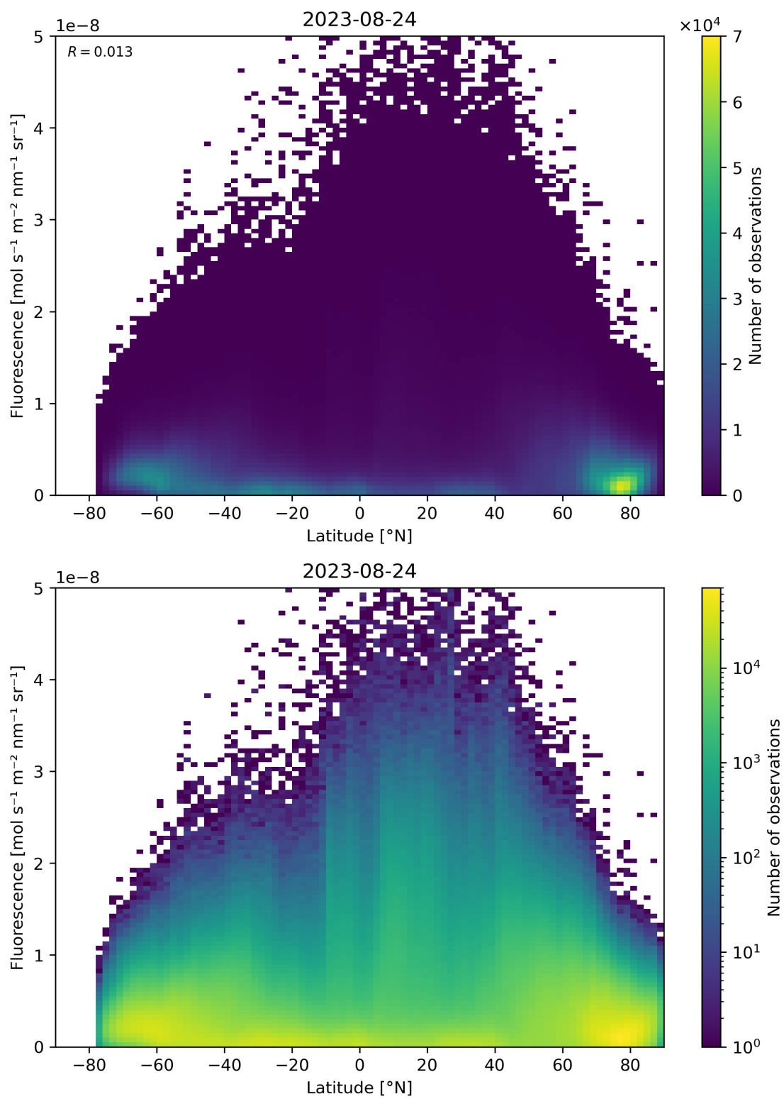
Figure 101: Scatter density plot of “Latitude” against “Fluorescence” for 2023-08-23 to 2023-08-25.
