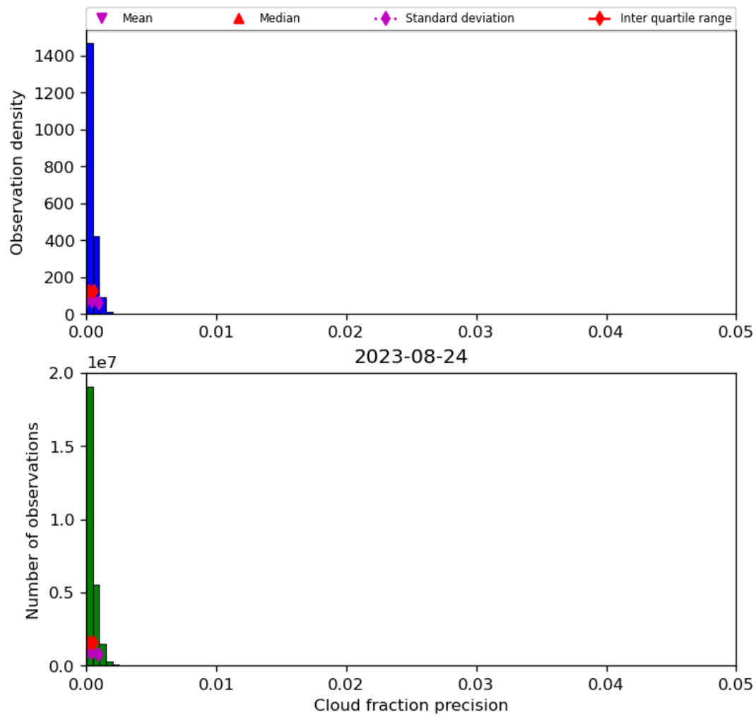
Figure 33: Histogram of “Cloud fraction precision” for 2023-08-23 to 2023-08-25
