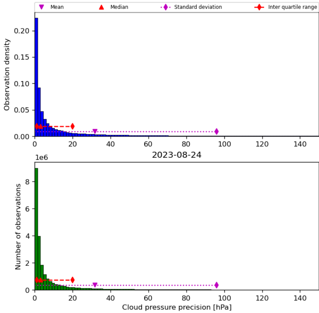
Figure 31: Histogram of “Cloud pressure precision” for 2023-08-23 to 2023-08-25
