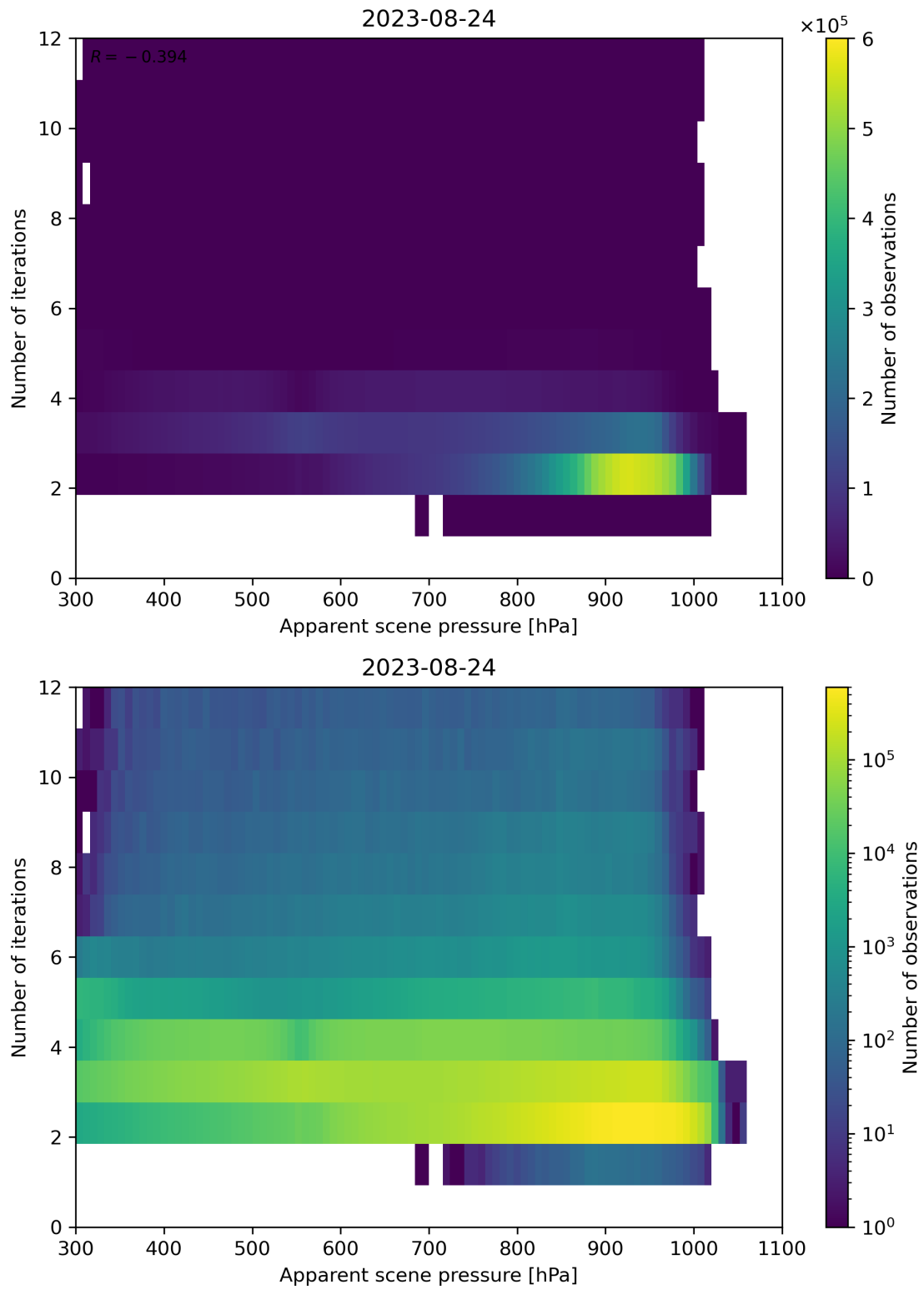
Figure 66: Scatter density plot of “Apparent scene pressure” against “Number of iterations” for 2023-08-23 to 2023-08-25.
