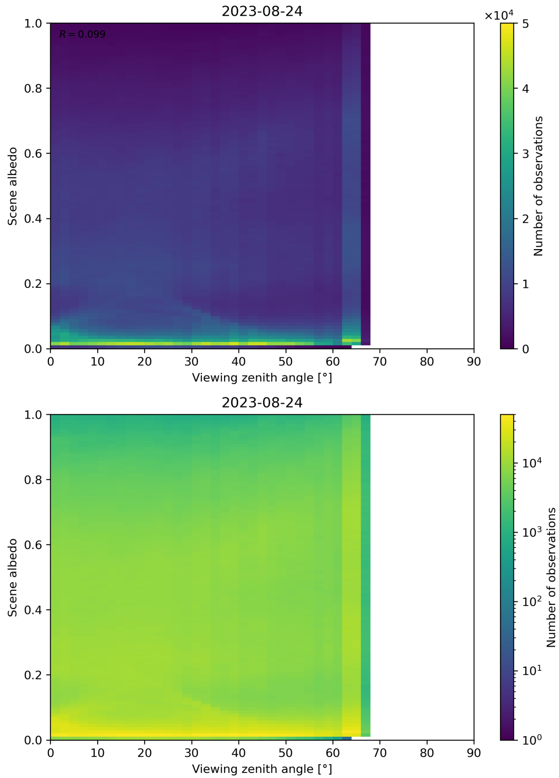
Figure 138: Scatter density plot of “Viewing zenith angle” against “Scene albedo” for 2023-08-23 to 2023-08-25.
