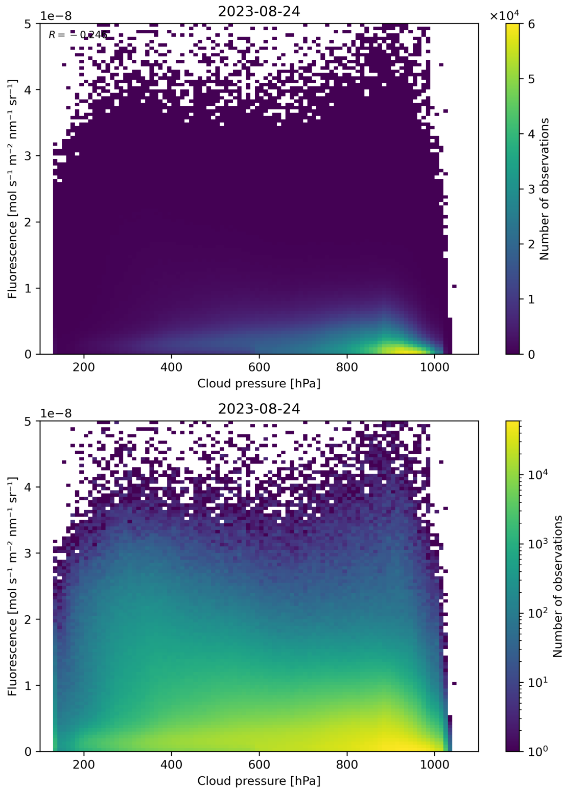
Figure 88: Scatter density plot of “Cloud pressure” against “Fluorescence” for 2023-08-23 to 2023-08-25.
