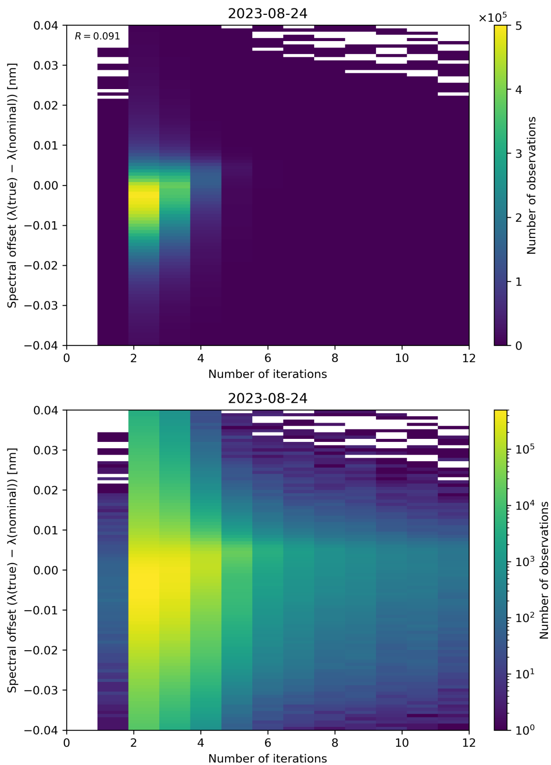
Figure 109: Scatter density plot of “Number of iterations” against “Spectral offset ( \lambda(\text{true}) - \lambda(\text{nominal}) )” for 2023-08-23 to 2023-08-25.
