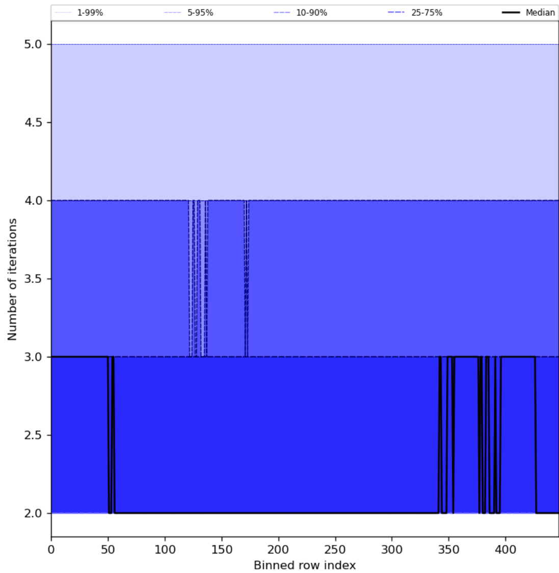
Figure 56: Along track statistics of “Number of iterations” for 2023-08-23 to 2023-08-25
