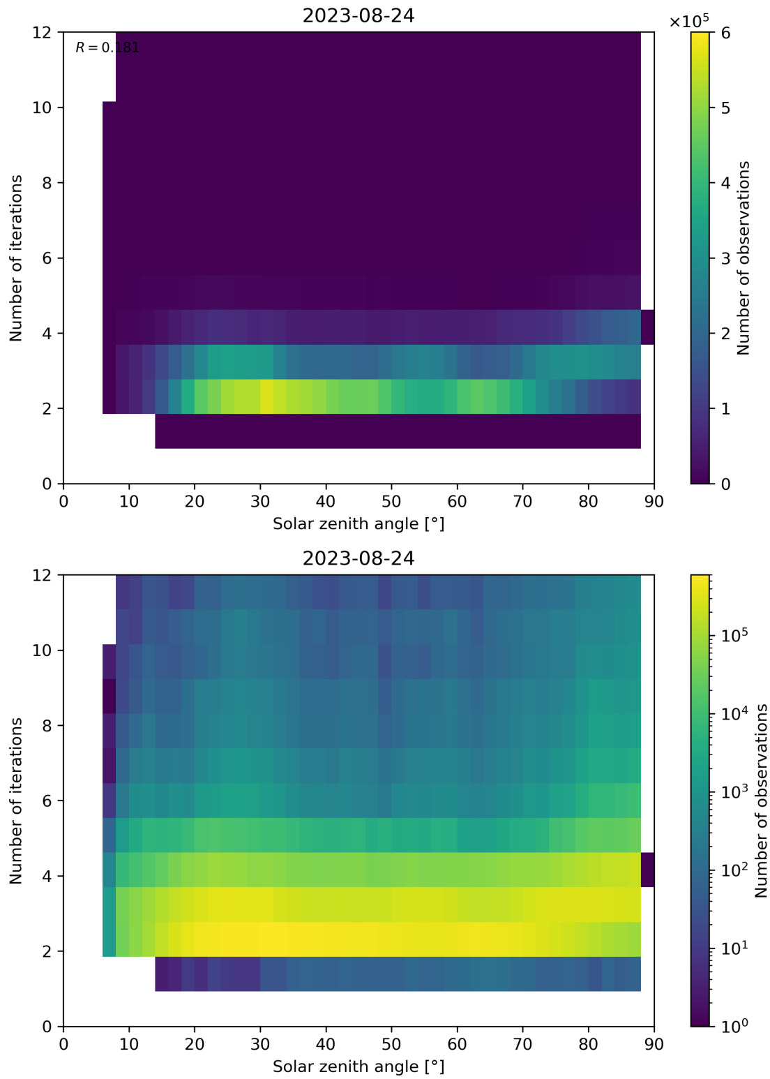
Figure 125: Scatter density plot of “Solar zenith angle” against “Number of iterations” for 2023-08-23 to 2023-08-25.
