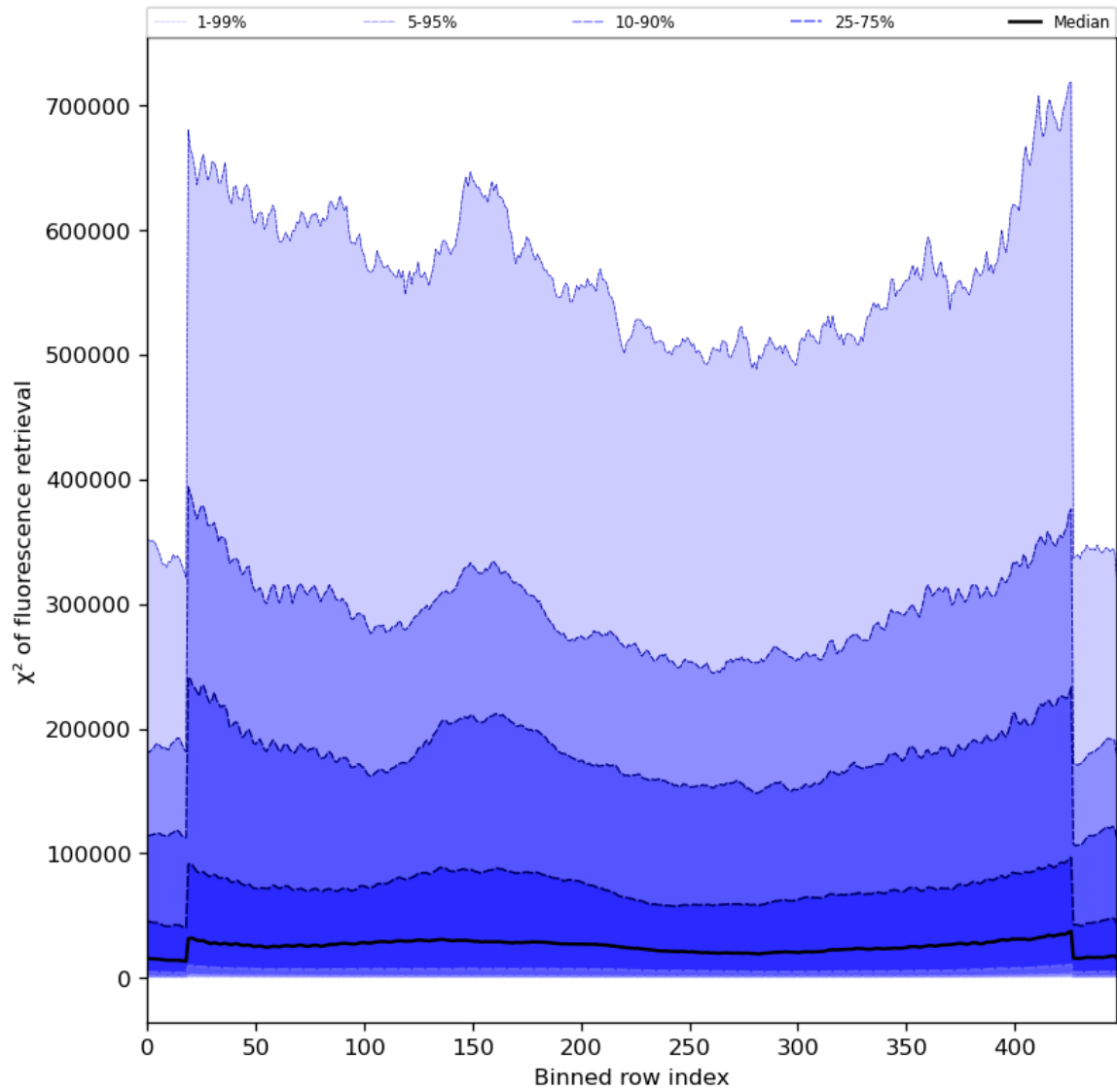
Figure 59: Along track statistics of “ \chi^2 of fluorescence retrieval” for 2023-08-23 to 2023-08-25
