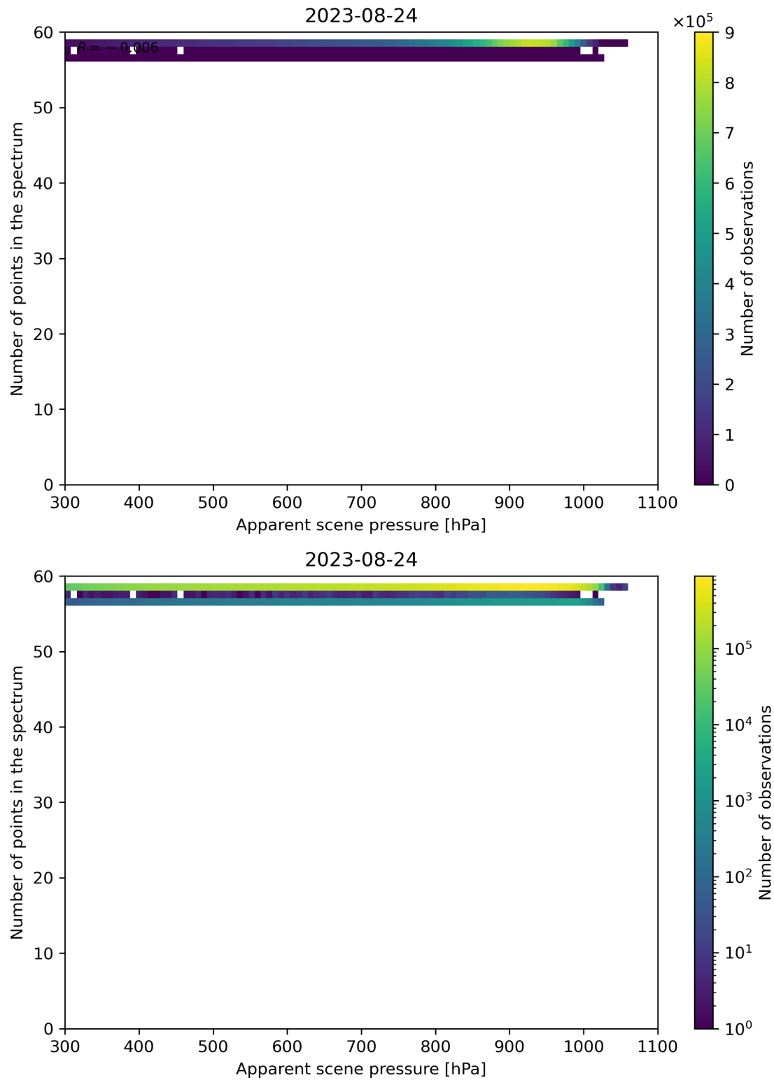
Figure 67: Scatter density plot of “Apparent scene pressure” against “Number of points in the spectrum” for 2023-08-23 to 2023-08-25.
