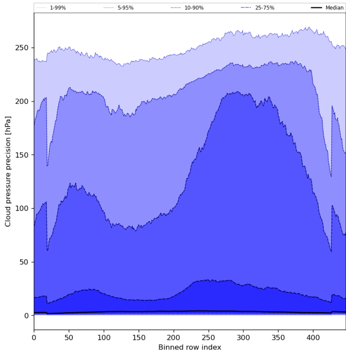
Figure 48: Along track statistics of “Cloud pressure precision” for 2023-08-23 to 2023-08-25
