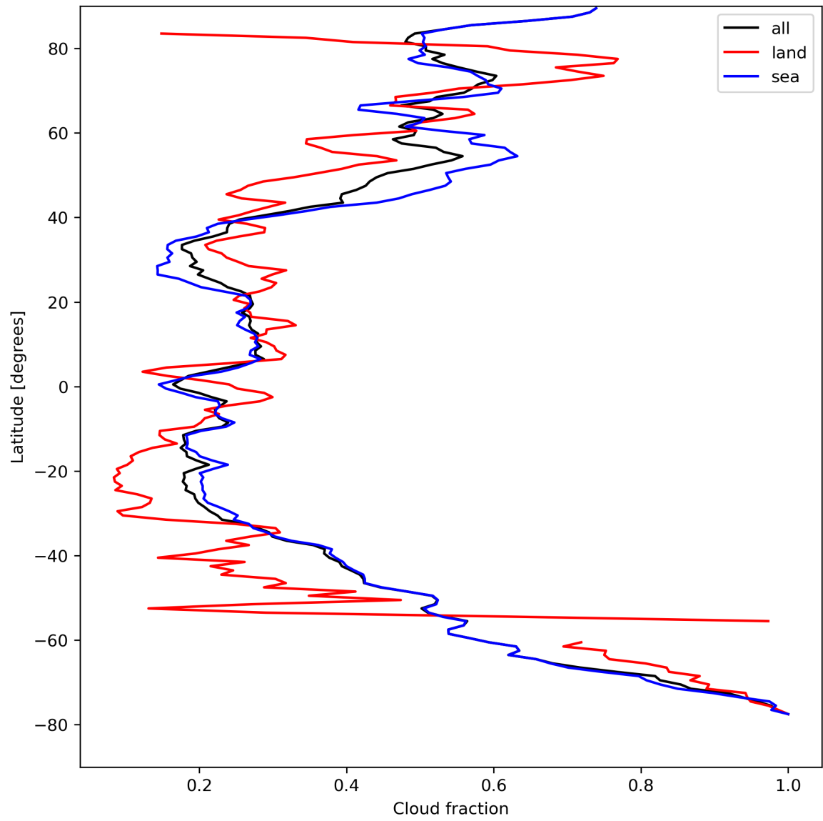
Figure 15: Zonal average of “Cloud fraction” for 2023-08-23 to 2023-08-25.
