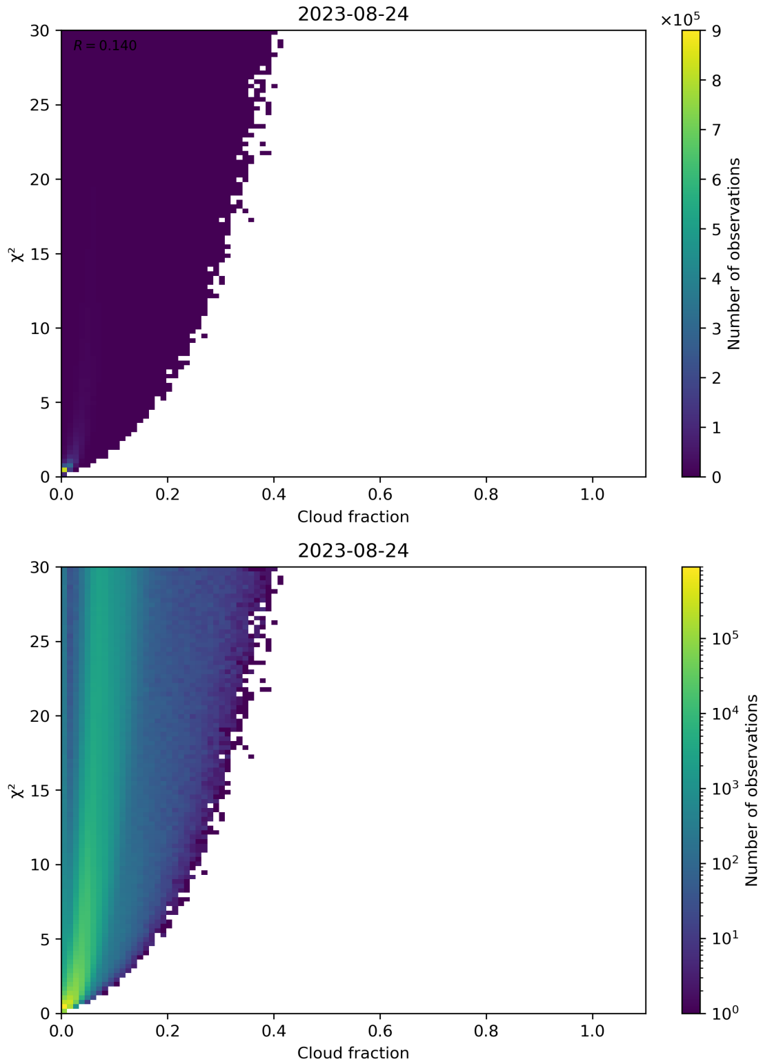
Figure 77: Scatter density plot of “Cloud fraction” against “ \chi^2 ” for 2023-08-23 to 2023-08-25.
