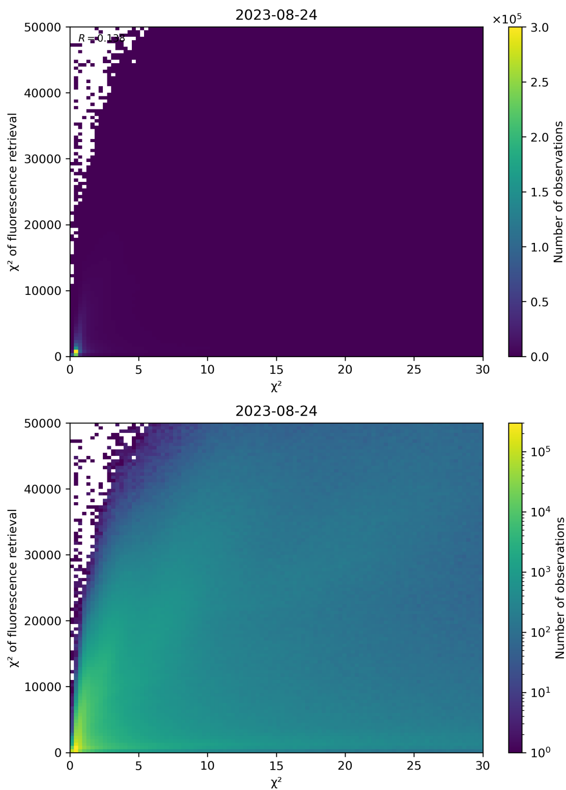
Figure 69: Scatter density plot of “ \chi^2 ” against “ \chi^2 of fluorescence retrieval” for 2023-08-23 to 2023-08-25.
