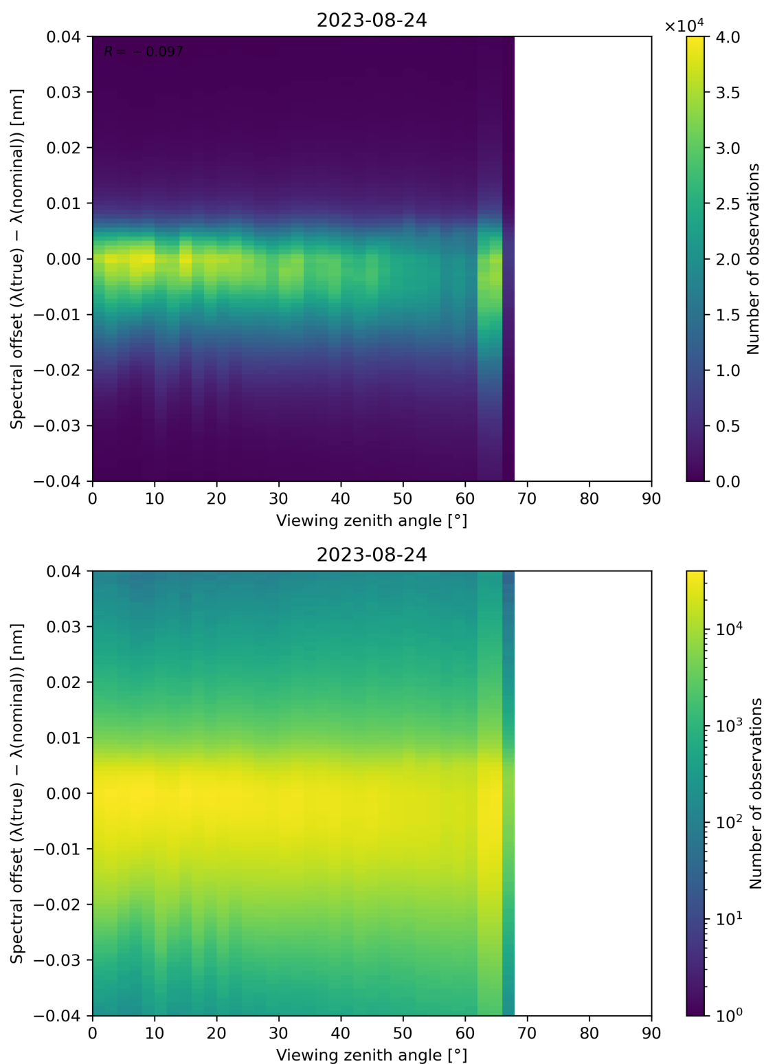
Figure 140: Scatter density plot of “Viewing zenith angle” against “Spectral offset ( \lambda(\text{true}) - \lambda(\text{nominal}) )” for 2023-08-23 to 2023-08-25.
