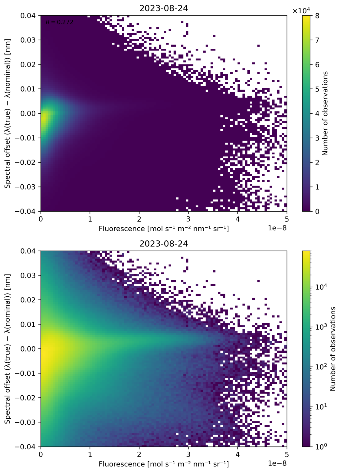
Figure 95: Scatter density plot of “Fluorescence” against “Spectral offset ( \lambda(\text{true}) - \lambda(\text{nominal}) )” for 2023-08-23 to 2023-08-25.
