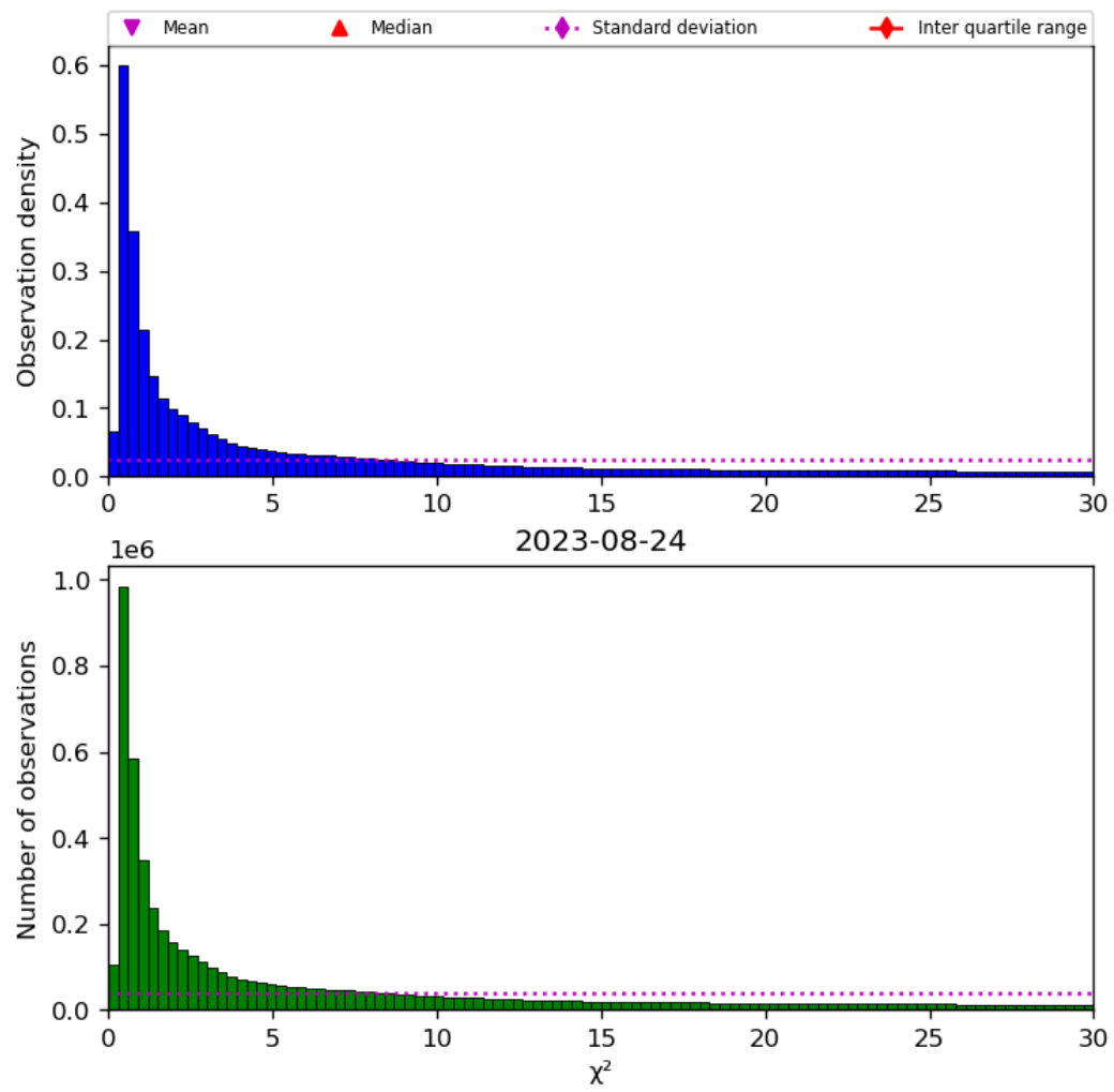
Figure 38: Histogram of “ \chi^2 ” for 2023-08-23 to 2023-08-25
