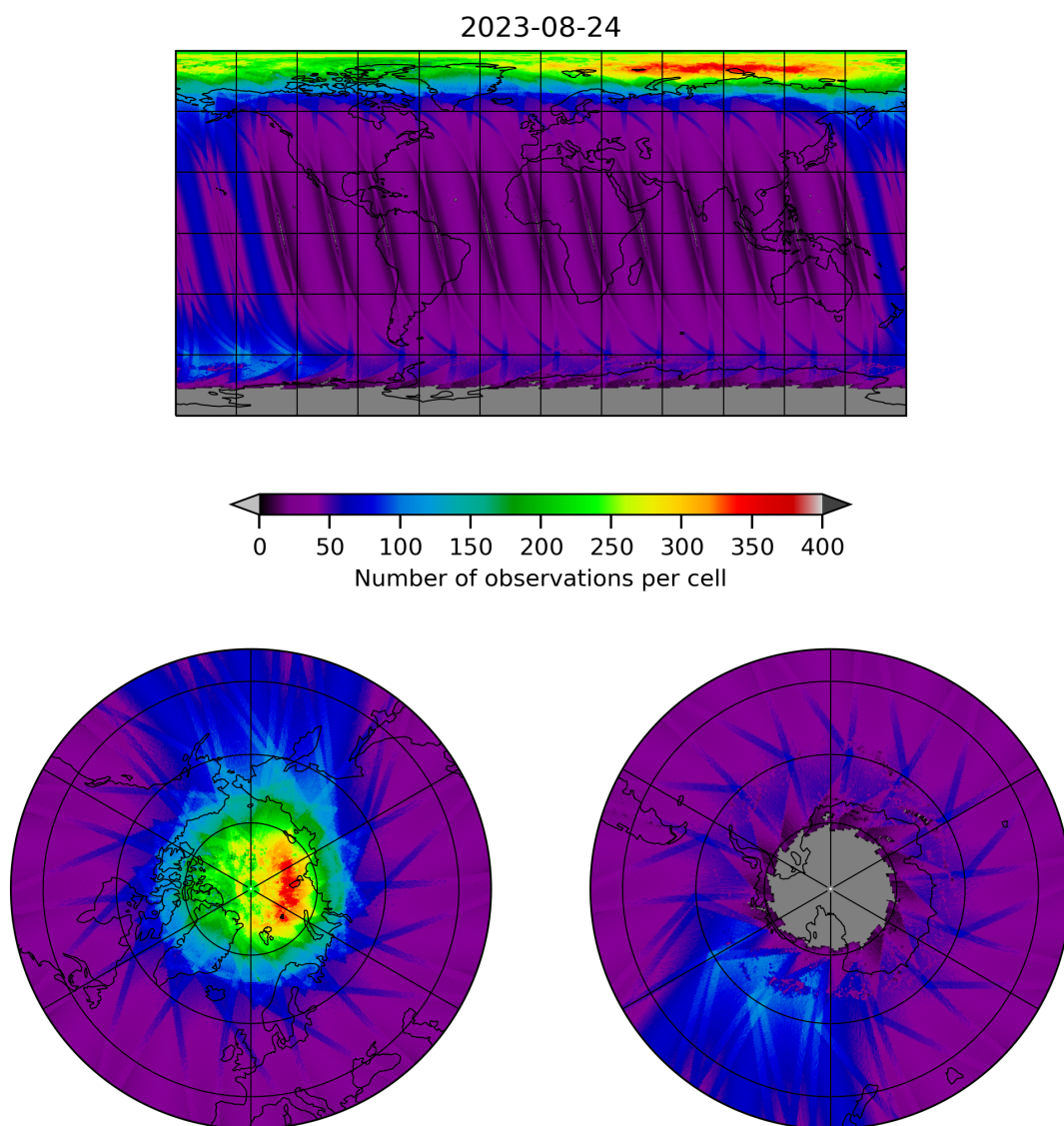
Figure 11: Map of the number of observations for 2023-08-23 to 2023-08-25
