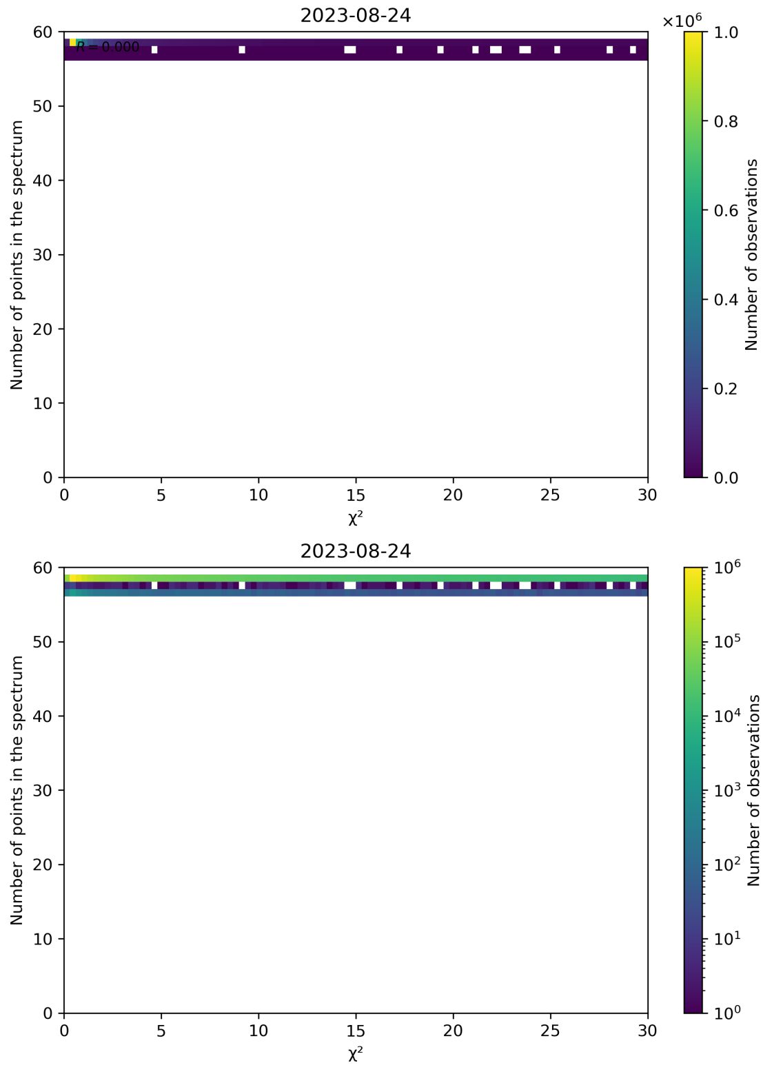
Figure 74: Scatter density plot of " \chi^2 " against "Number of points in the spectrum" for 2023-08-23 to 2023-08-25.
