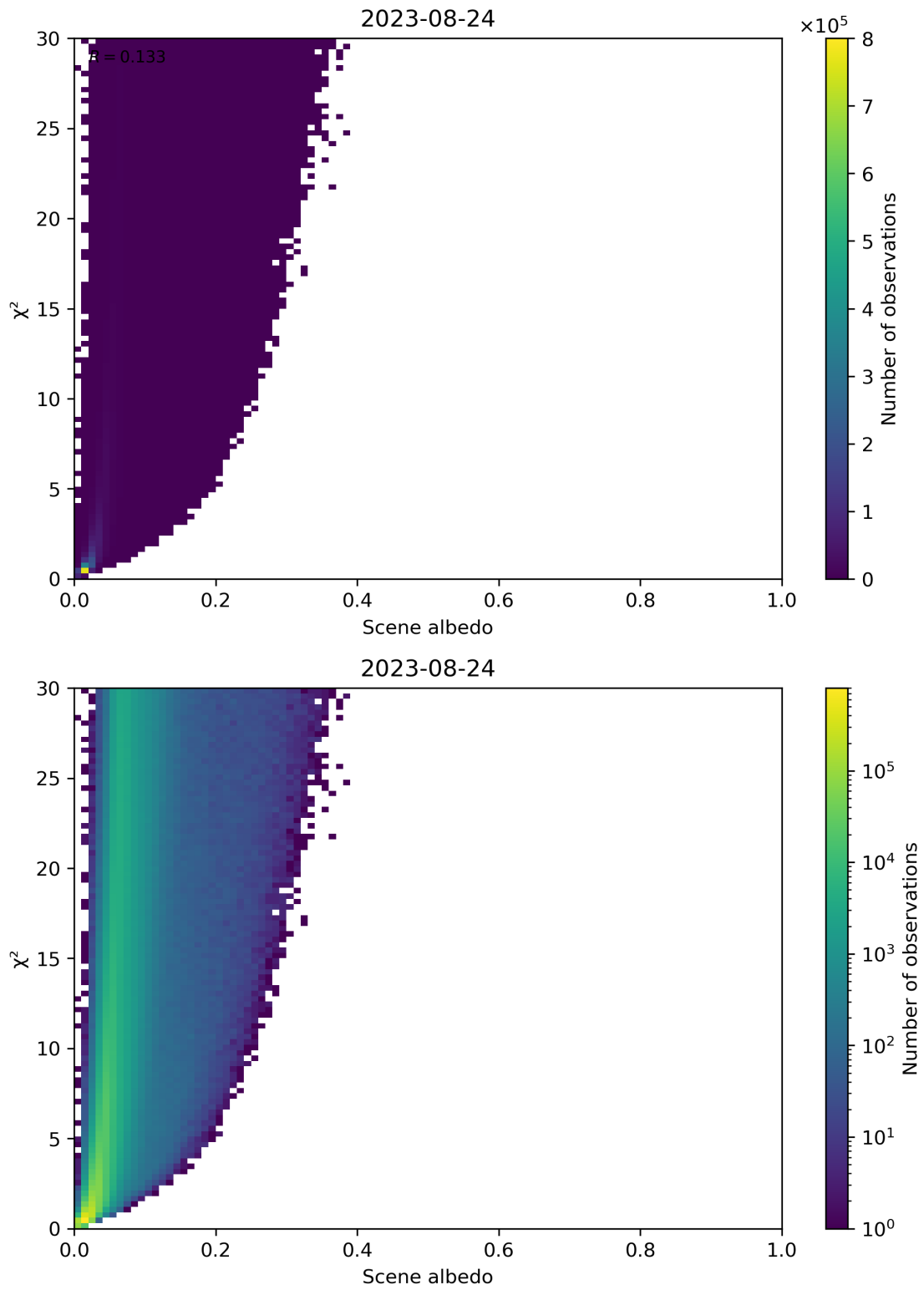
Figure 112: Scatter density plot of “Scene albedo” against “ \chi^2 ” for 2023-08-23 to 2023-08-25.
