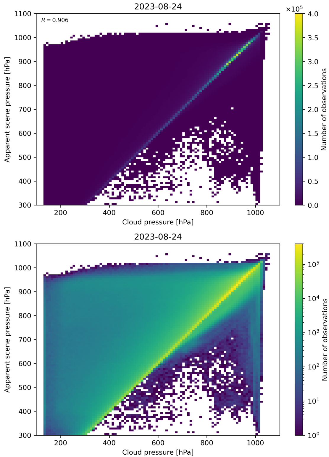
Figure 84: Scatter density plot of “Cloud pressure” against “Apparent scene pressure” for 2023-08-23 to 2023-08-25.
