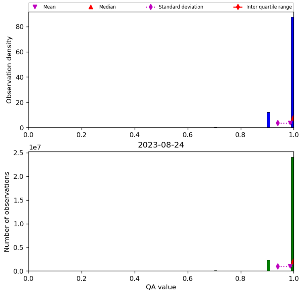
Figure 29: Histogram of “QA value” for 2023-08-23 to 2023-08-25
