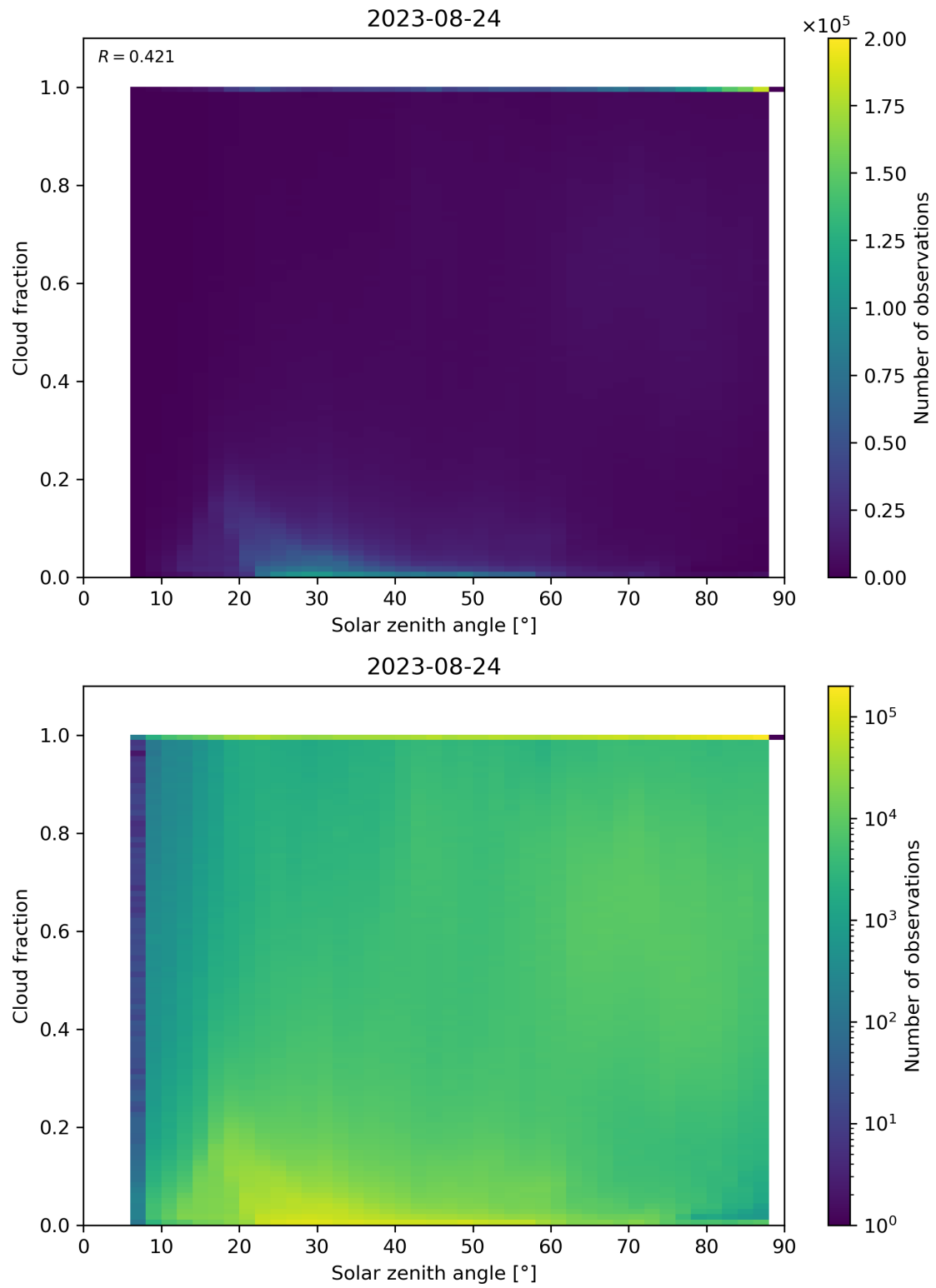
Figure 121: Scatter density plot of “Solar zenith angle” against “Cloud fraction” for 2023-08-23 to 2023-08-25.
