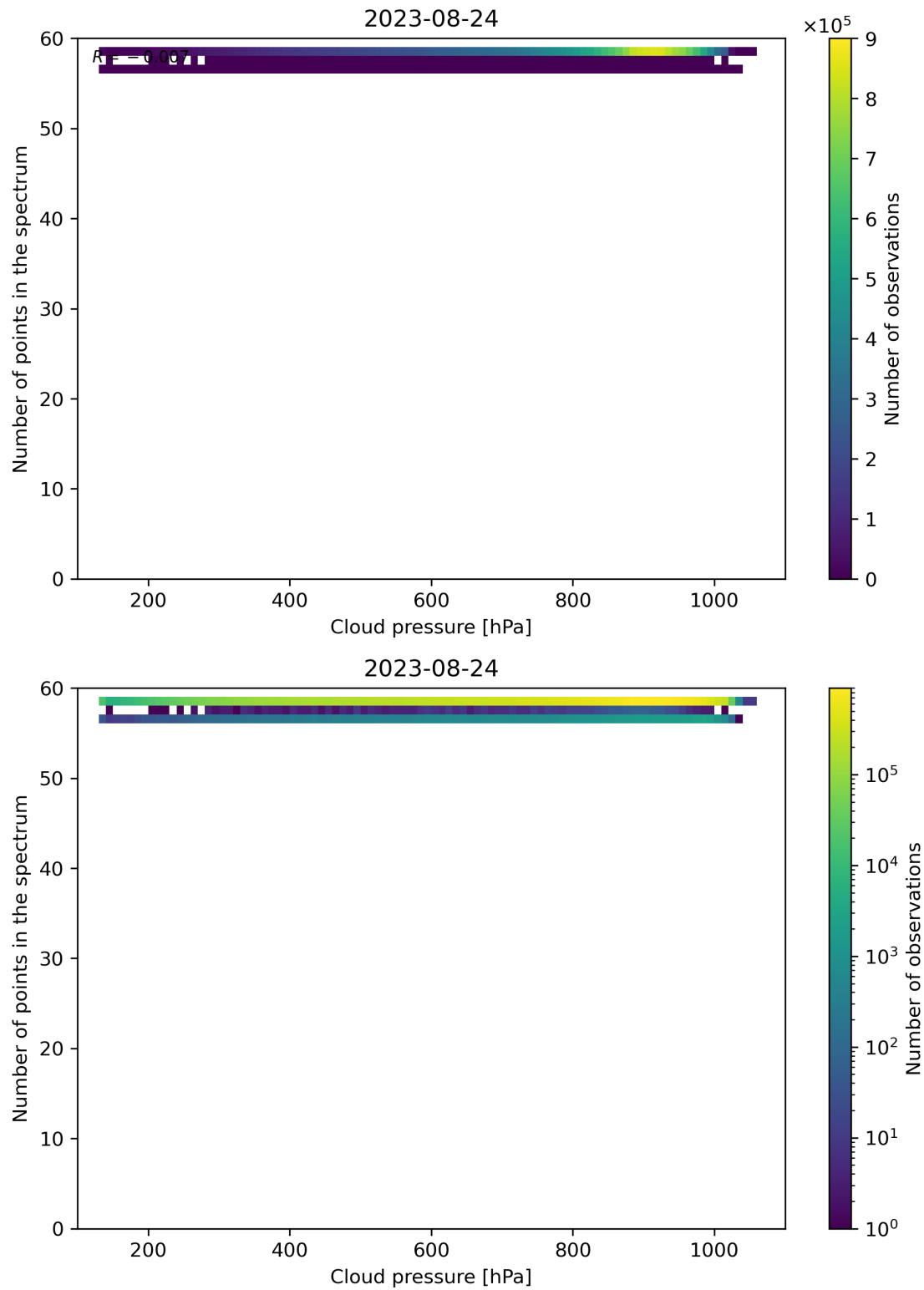
Figure 90: Scatter density plot of “Cloud pressure” against “Number of points in the spectrum” for 2023-08-23 to 2023-08-25.
