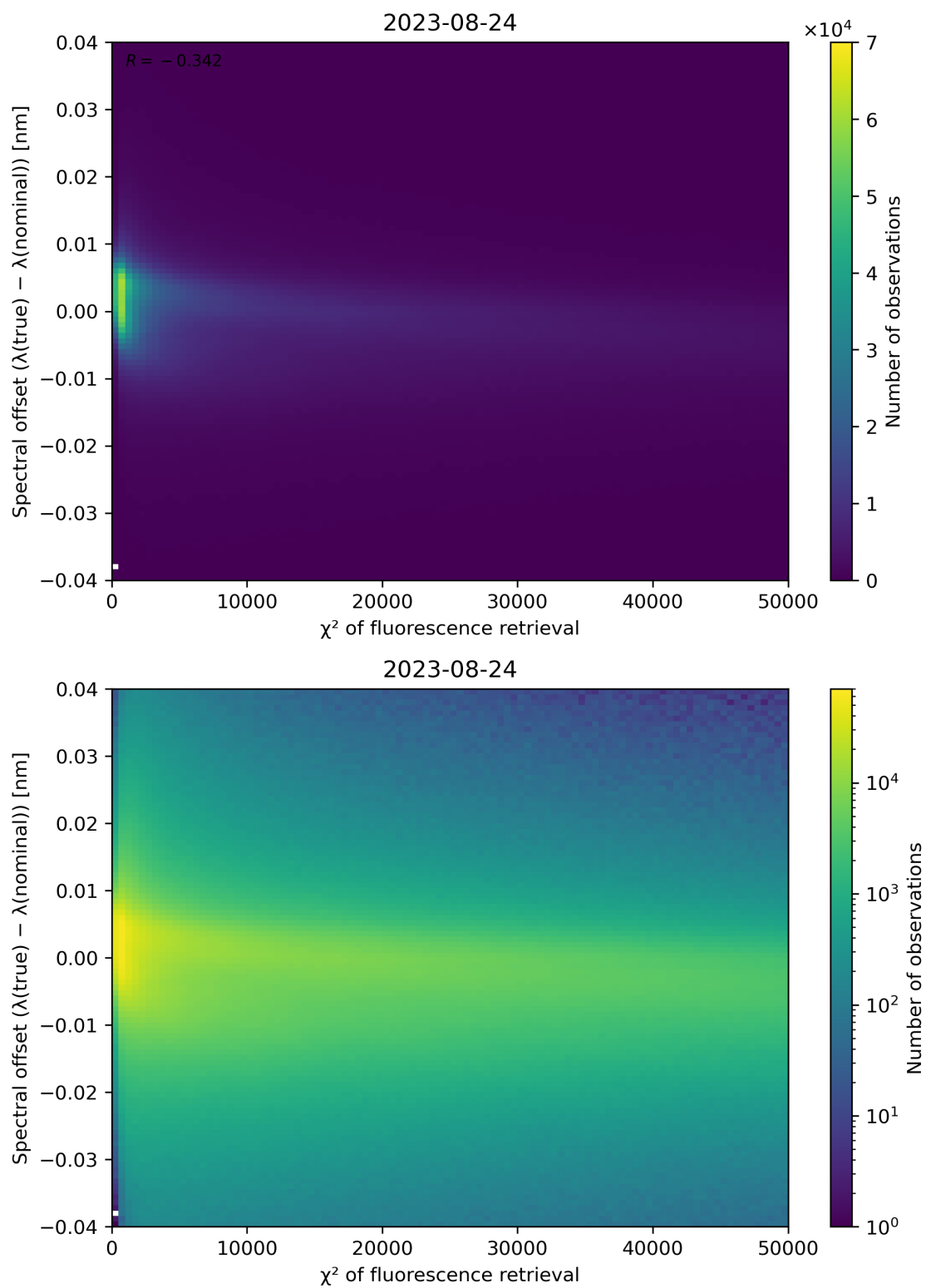
Figure 72: Scatter density plot of “ \chi^2 of fluorescence retrieval” against “Spectral offset ( \lambda(\text{true}) - \lambda(\text{nominal}) )” for 2023-08-23 to 2023-08-25.
