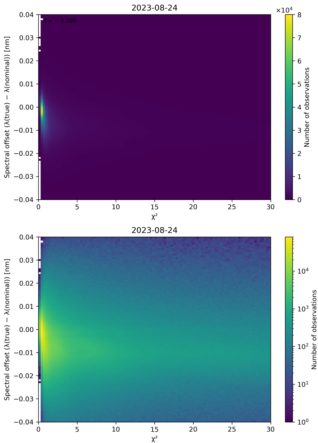
Figure 75: Scatter density plot of “ \chi^2 ” against “Spectral offset ( \lambda(\text{true}) - \lambda(\text{nominal}) )” for 2023-08-23 to 2023-08-25.
