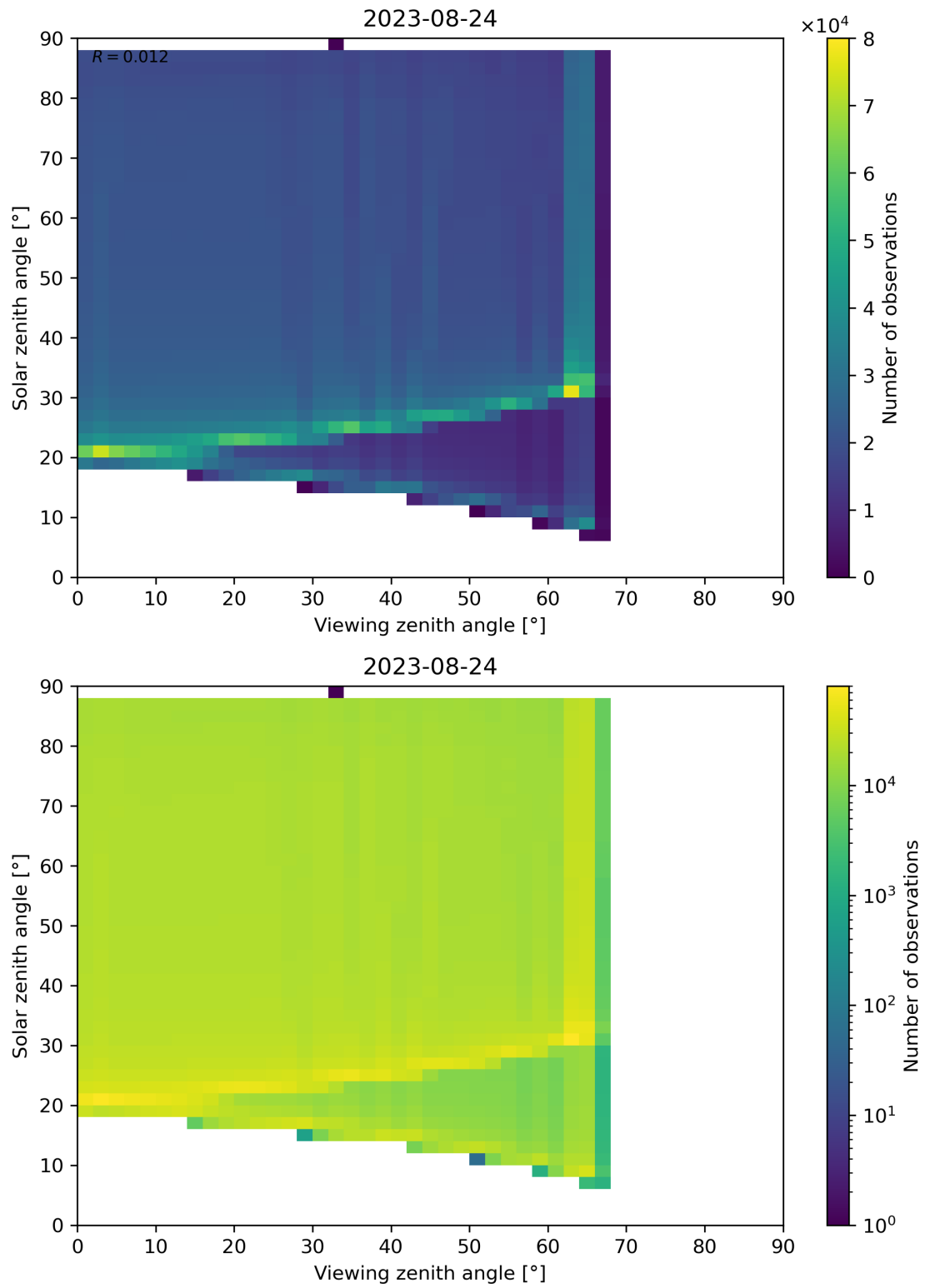
Figure 139: Scatter density plot of “Viewing zenith angle” against “Solar zenith angle” for 2023-08-23 to 2023-08-25.
