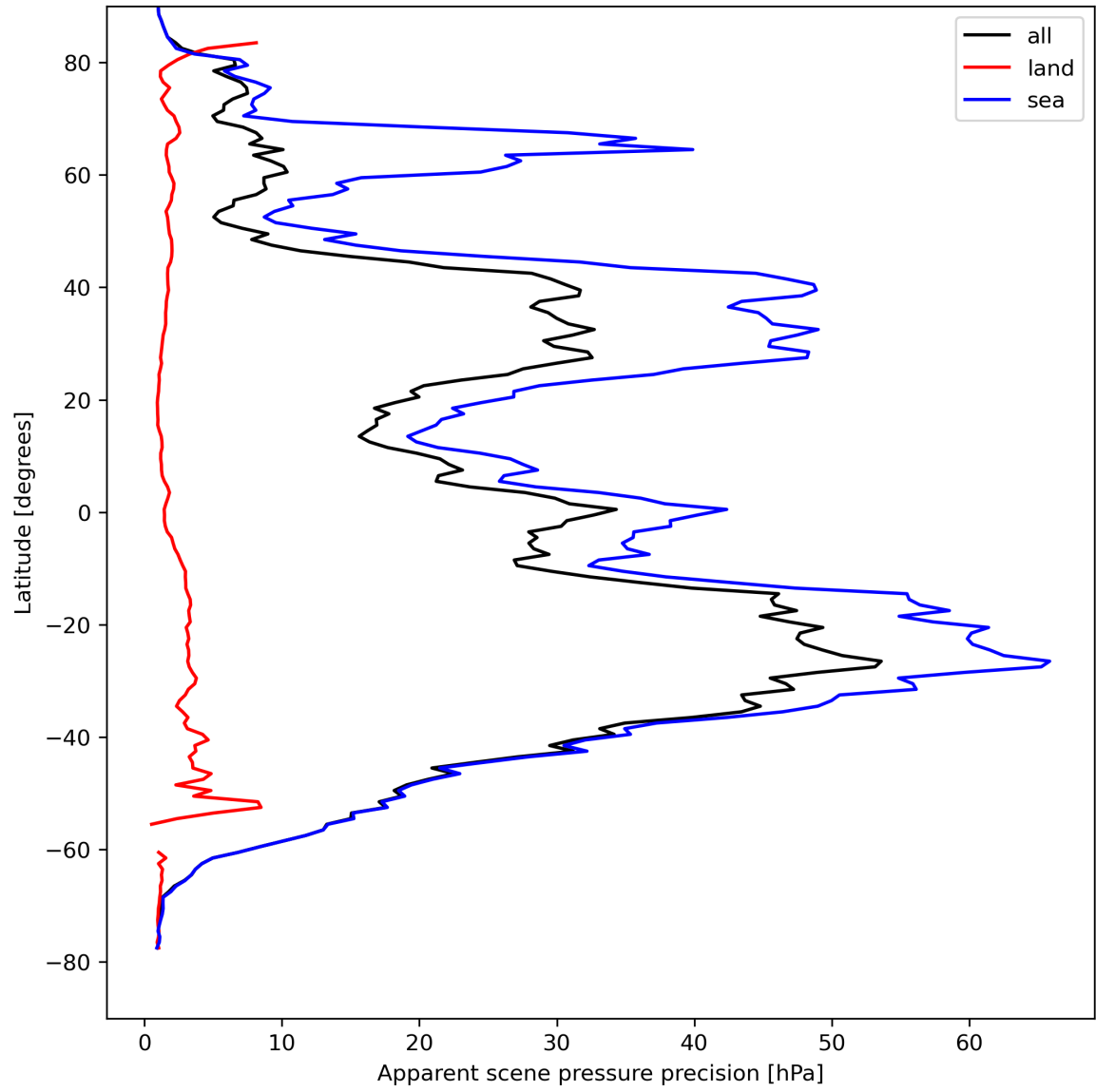
Figure 20: Zonal average of “Apparent scene pressure precision” for 2023-08-23 to 2023-08-25.
