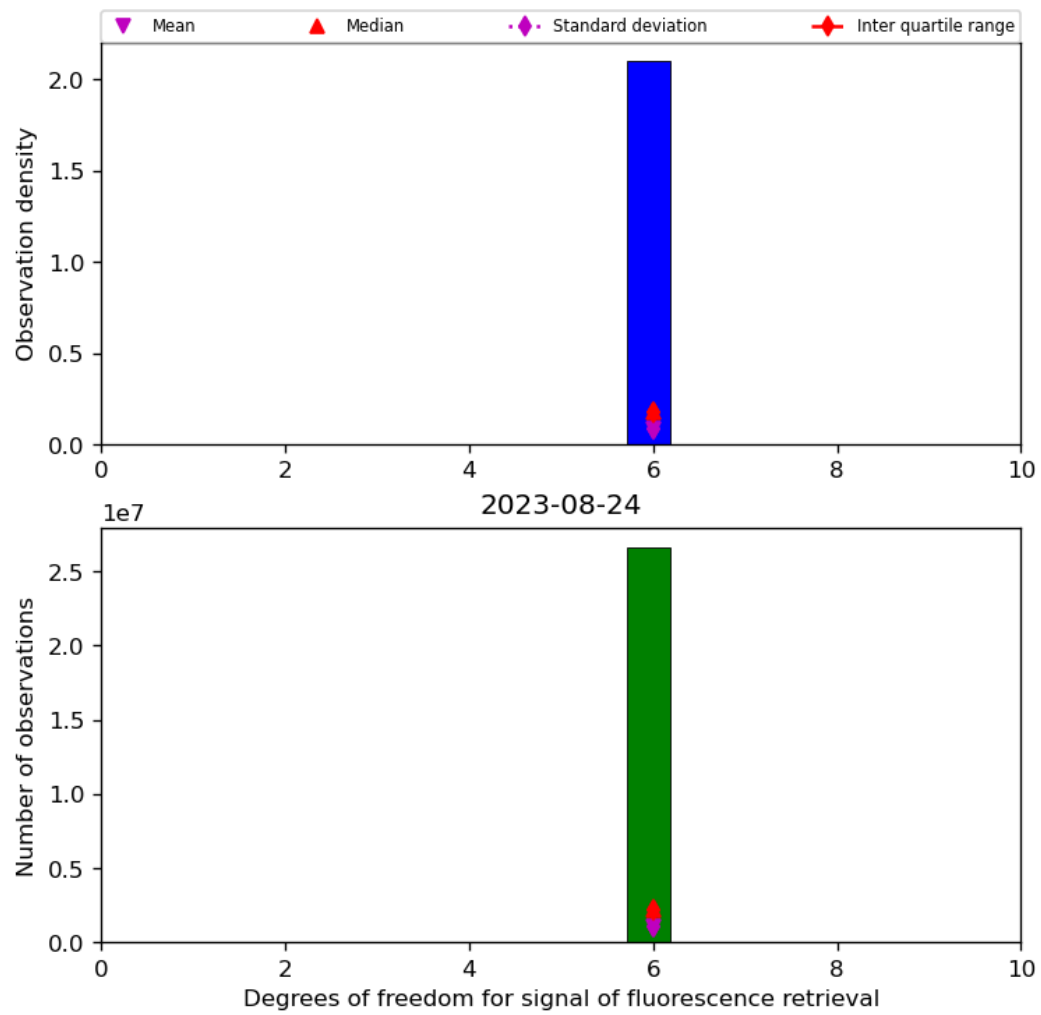
Figure 43: Histogram of “Degrees of freedom for signal of fluorescence retrieval” for 2023-08-23 to 2023-08-25
