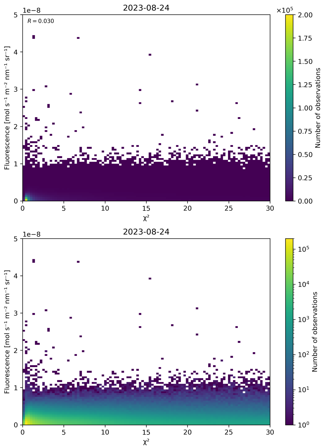
Figure 70: Scatter density plot of “ \chi^2 ” against “Fluorescence” for 2023-08-23 to 2023-08-25.
