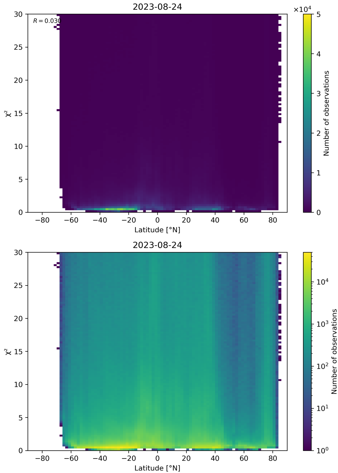
Figure 97: Scatter density plot of “Latitude” against “ \chi^2 ” for 2023-08-23 to 2023-08-25.
