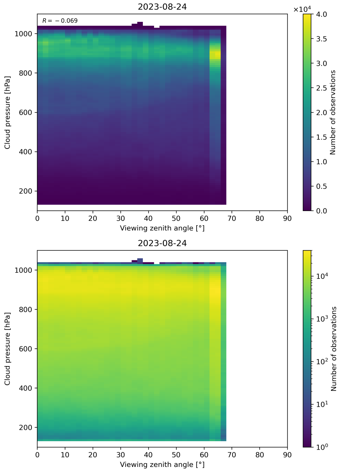
Figure 133: Scatter density plot of “Viewing zenith angle” against “Cloud pressure” for 2023-08-23 to 2023-08-25.
