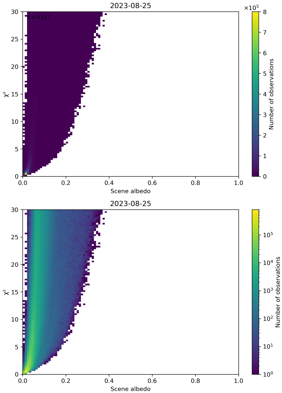
Figure 112: Scatter density plot of “Scene albedo” against “ \chi^2 ” for 2023-08-25 to 2023-08-26.
