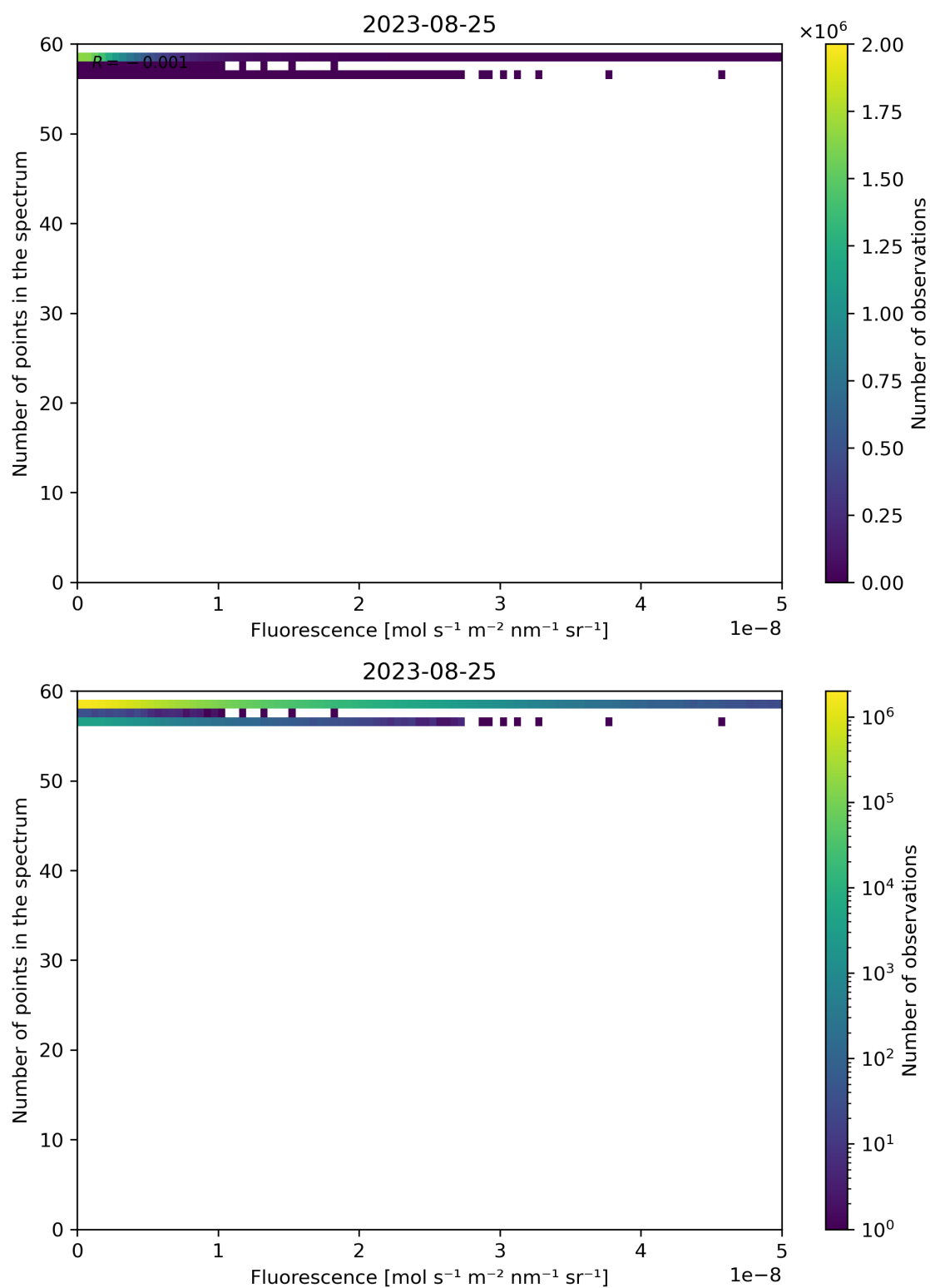
Figure 94: Scatter density plot of “Fluorescence” against “Number of points in the spectrum” for 2023-08-25 to 2023-08-26.
