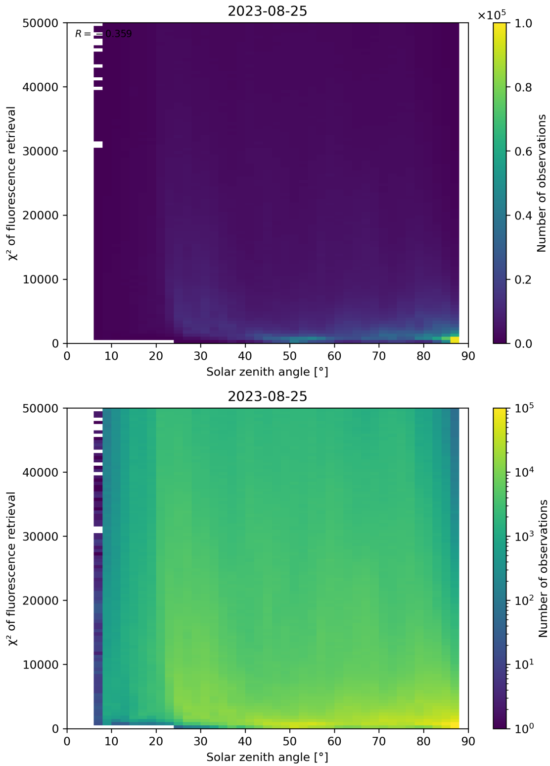
Figure 120: Scatter density plot of “Solar zenith angle” against “ \chi^2 of fluorescence retrieval” for 2023-08-25 to 2023-08-26.
