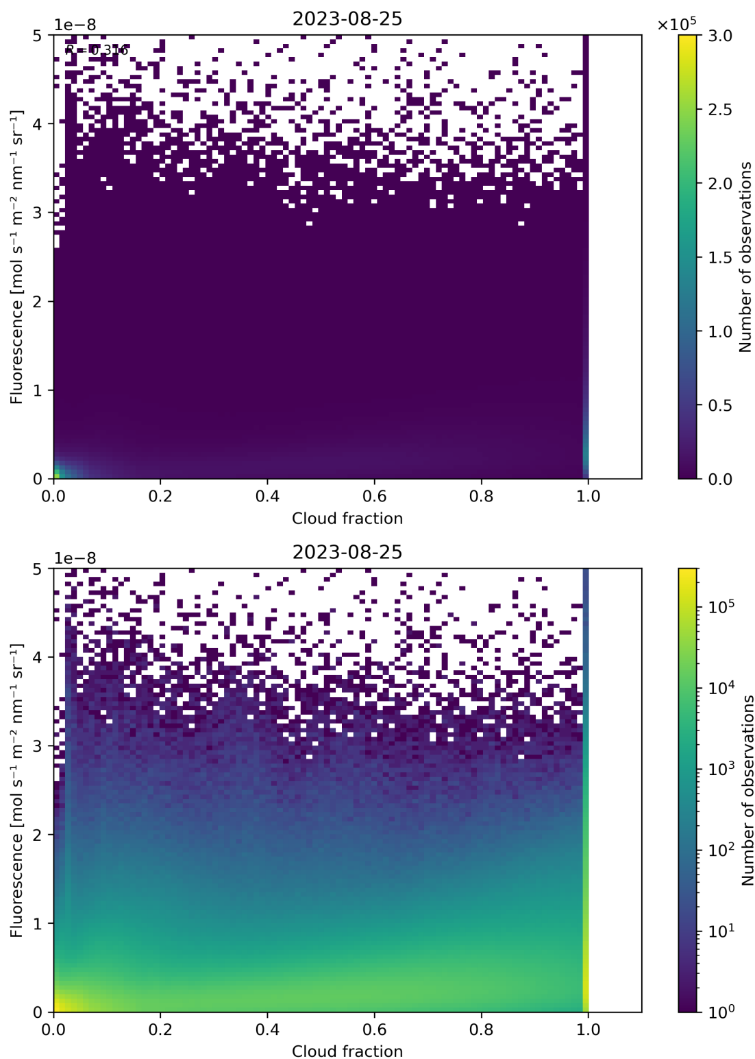
Figure 79: Scatter density plot of “Cloud fraction” against “Fluorescence” for 2023-08-25 to 2023-08-26.
