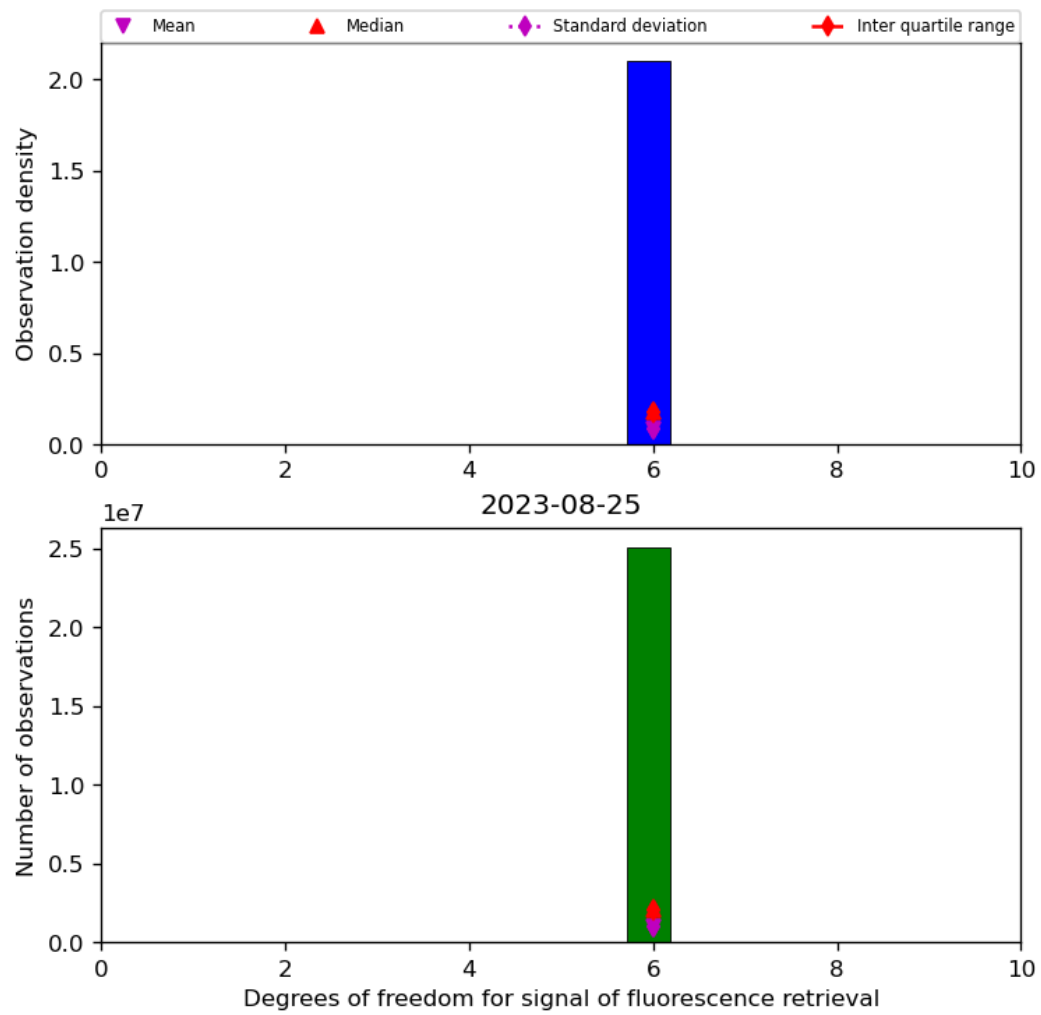
Figure 43: Histogram of “Degrees of freedom for signal of fluorescence retrieval” for 2023-08-25 to 2023-08-26
