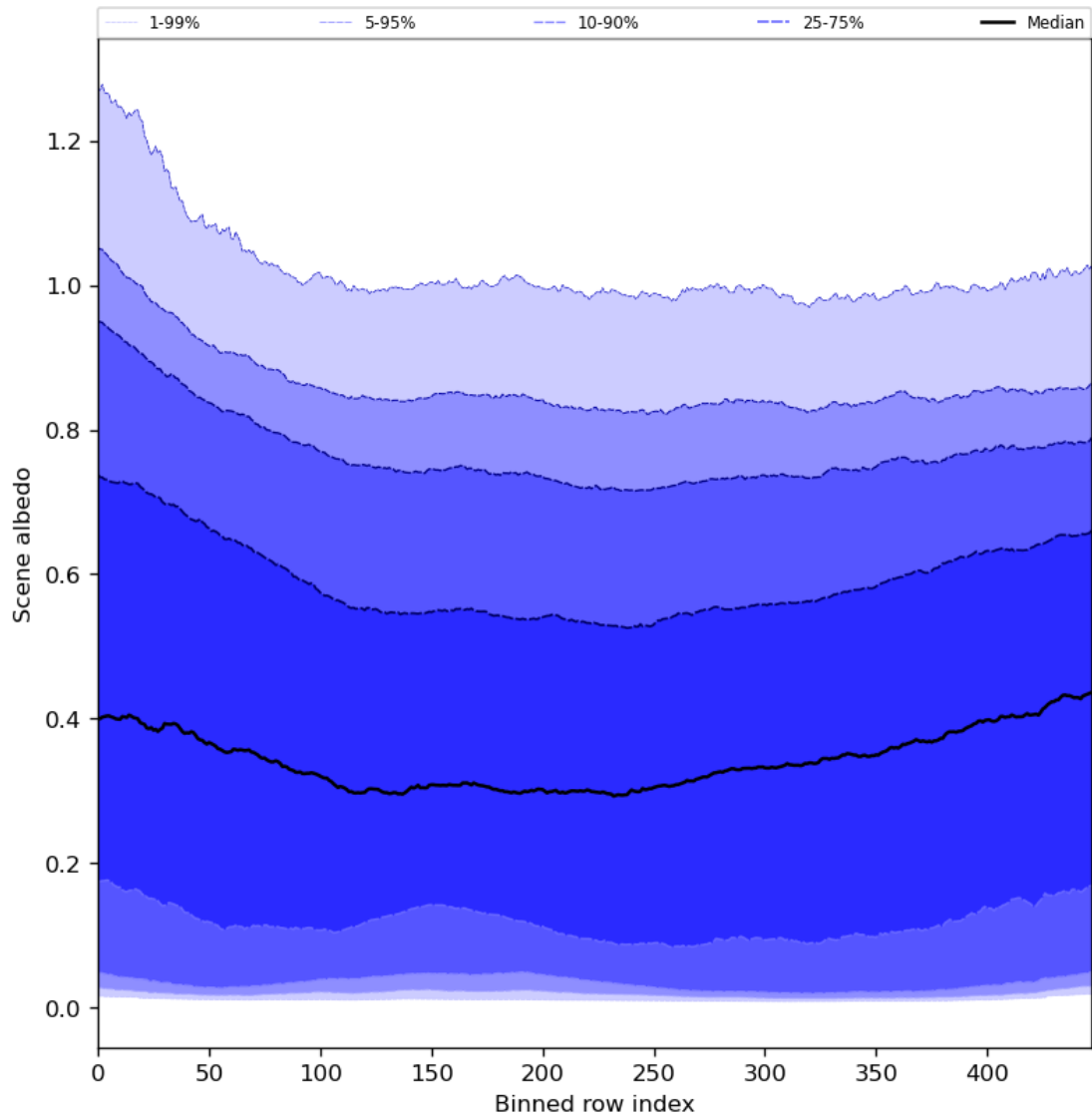
Figure 51: Along track statistics of “Scene albedo” for 2023-08-25 to 2023-08-26
