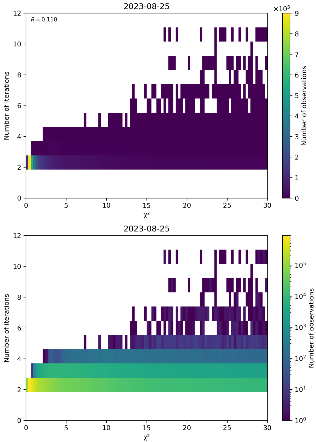
Figure 73: Scatter density plot of “ \chi^2 ” against “Number of iterations” for 2023-08-25 to 2023-08-26.
