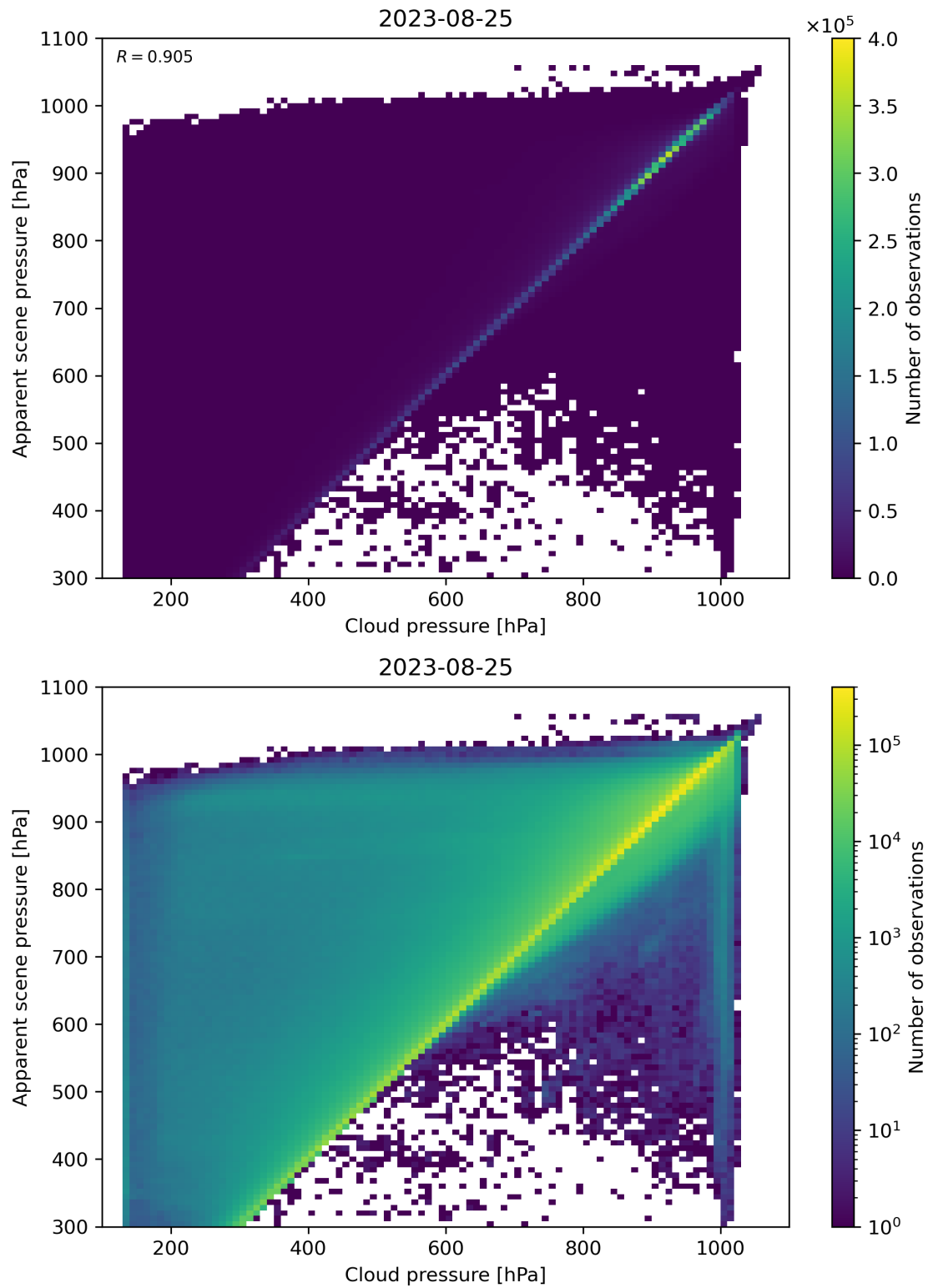
Figure 84: Scatter density plot of “Cloud pressure” against “Apparent scene pressure” for 2023-08-25 to 2023-08-26.
