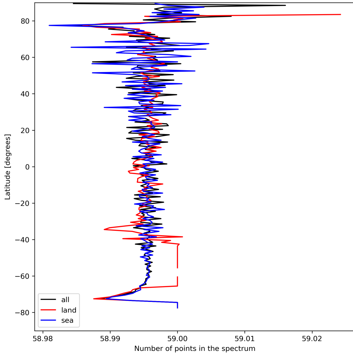
Figure 27: Zonal average of “Number of points in the spectrum” for 2023-08-25 to 2023-08-26.
