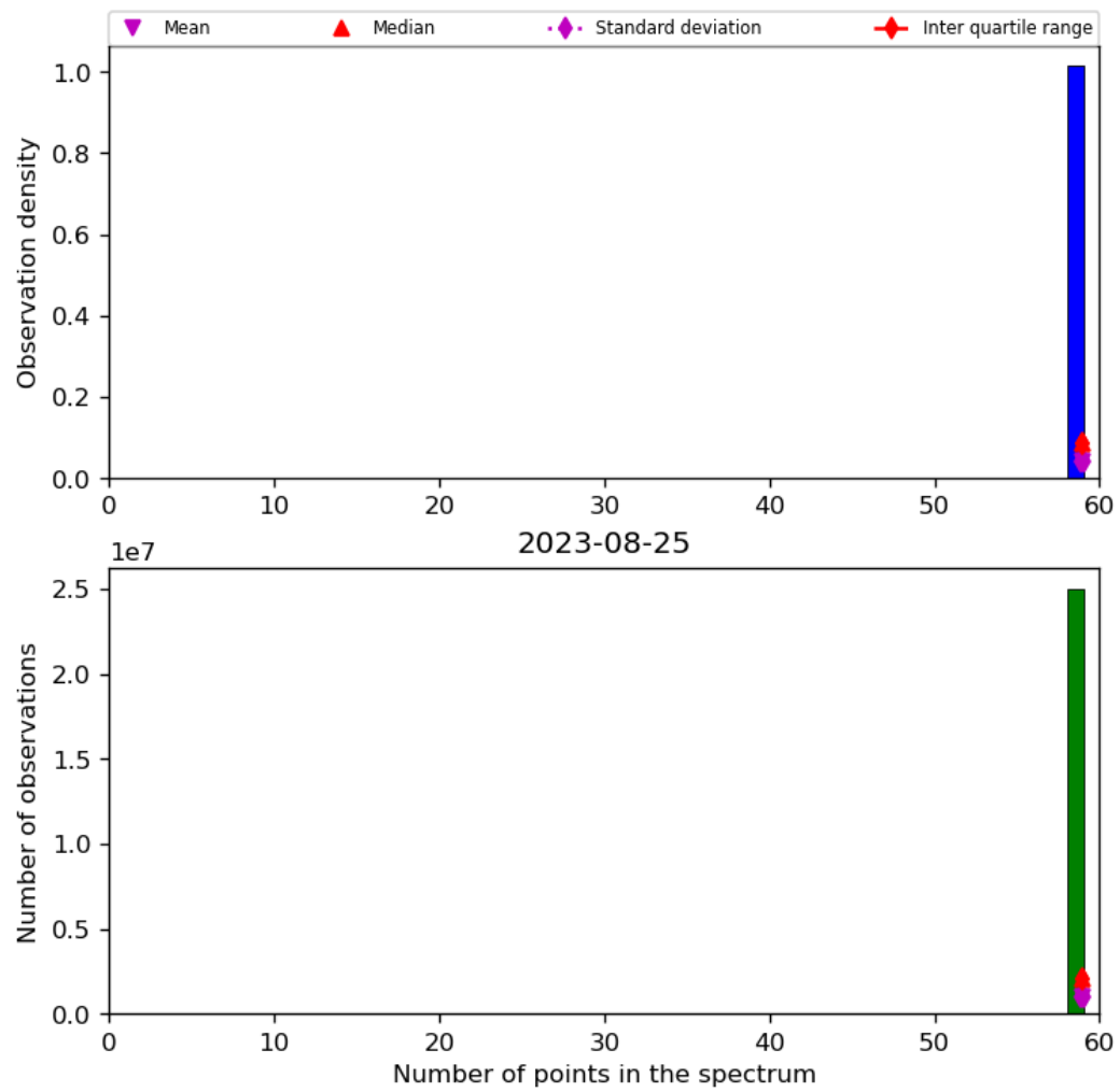
Figure 44: Histogram of “Number of points in the spectrum” for 2023-08-25 to 2023-08-26
