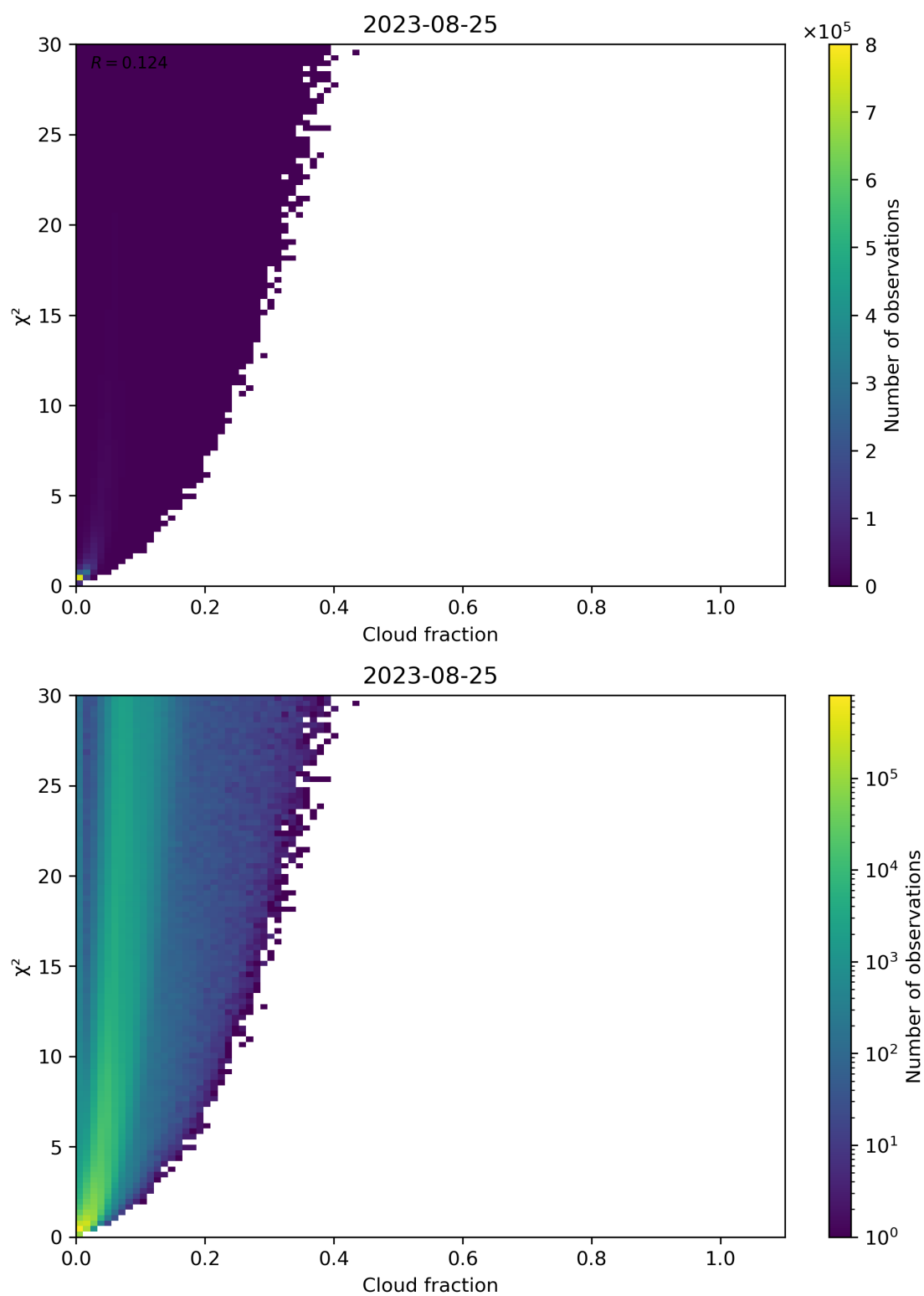
Figure 77: Scatter density plot of “Cloud fraction” against “ \chi^2 ” for 2023-08-25 to 2023-08-26.
