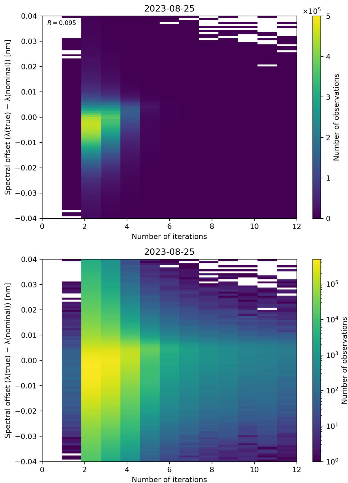
Figure 109: Scatter density plot of “Number of iterations” against “Spectral offset ( \lambda(\text{true}) - \lambda(\text{nominal}) )” for 2023-08-25 to 2023-08-26.
