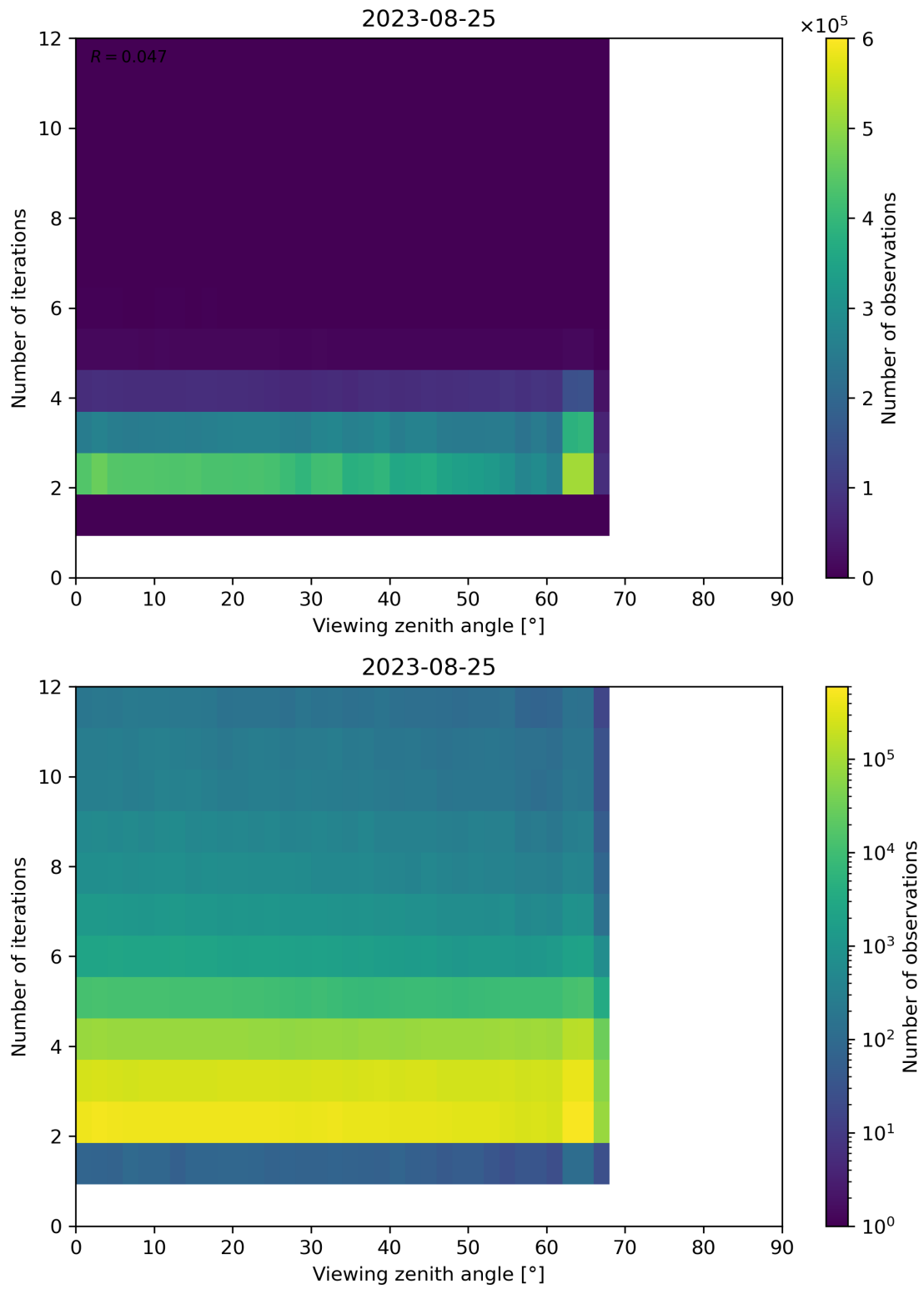
Figure 136: Scatter density plot of “Viewing zenith angle” against “Number of iterations” for 2023-08-25 to 2023-08-26.
