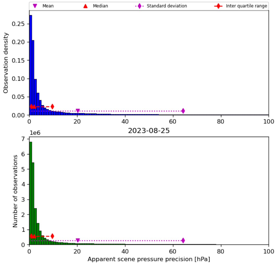
Figure 37: Histogram of “Apparent scene pressure precision” for 2023-08-25 to 2023-08-26
