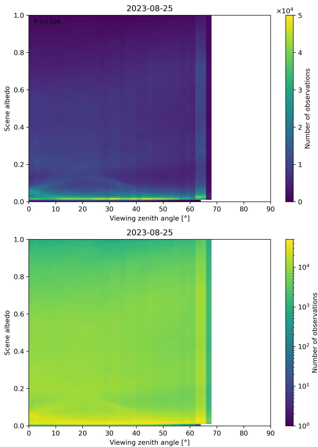
Figure 138: Scatter density plot of “Viewing zenith angle” against “Scene albedo” for 2023-08-25 to 2023-08-26.
