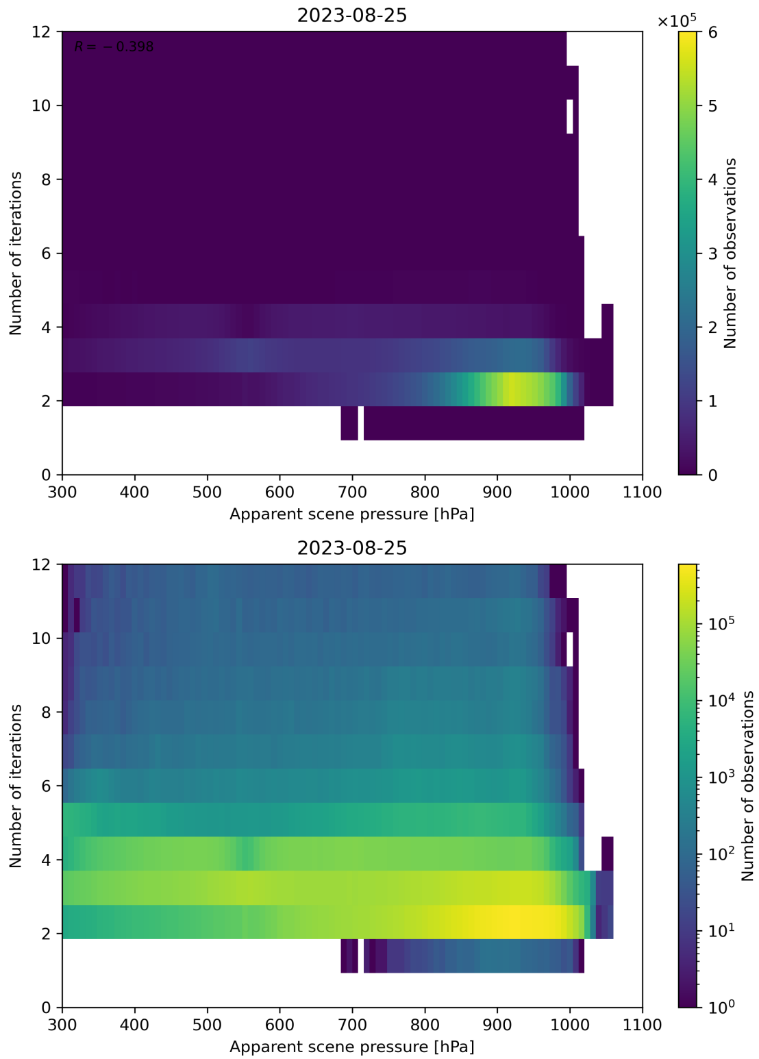
Figure 66: Scatter density plot of “Apparent scene pressure” against “Number of iterations” for 2023-08-25 to 2023-08-26.
