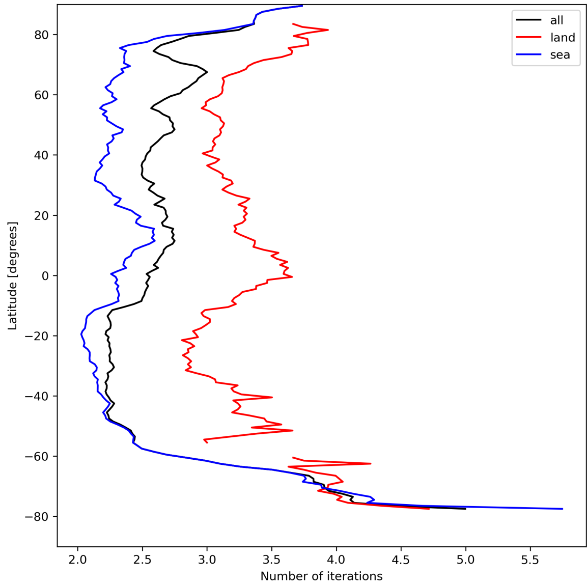
Figure 22: Zonal average of “Number of iterations” for 2023-08-25 to 2023-08-26.
