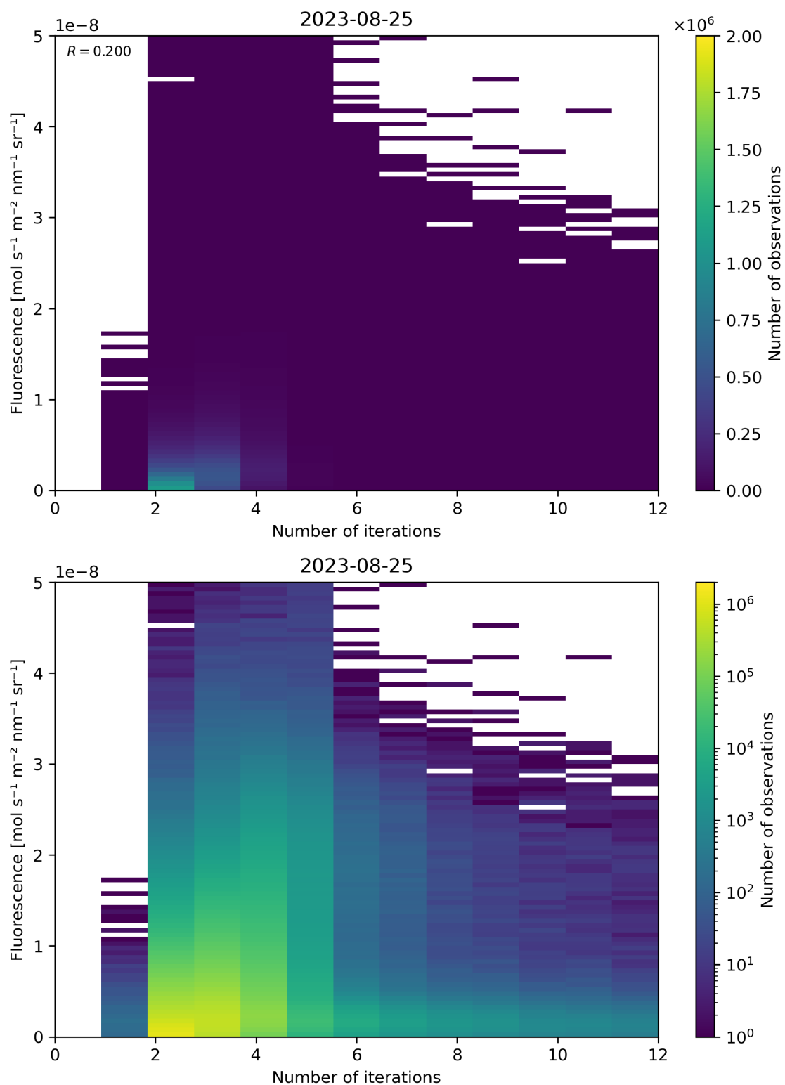
Figure 107: Scatter density plot of “Number of iterations” against “Fluorescence” for 2023-08-25 to 2023-08-26.
