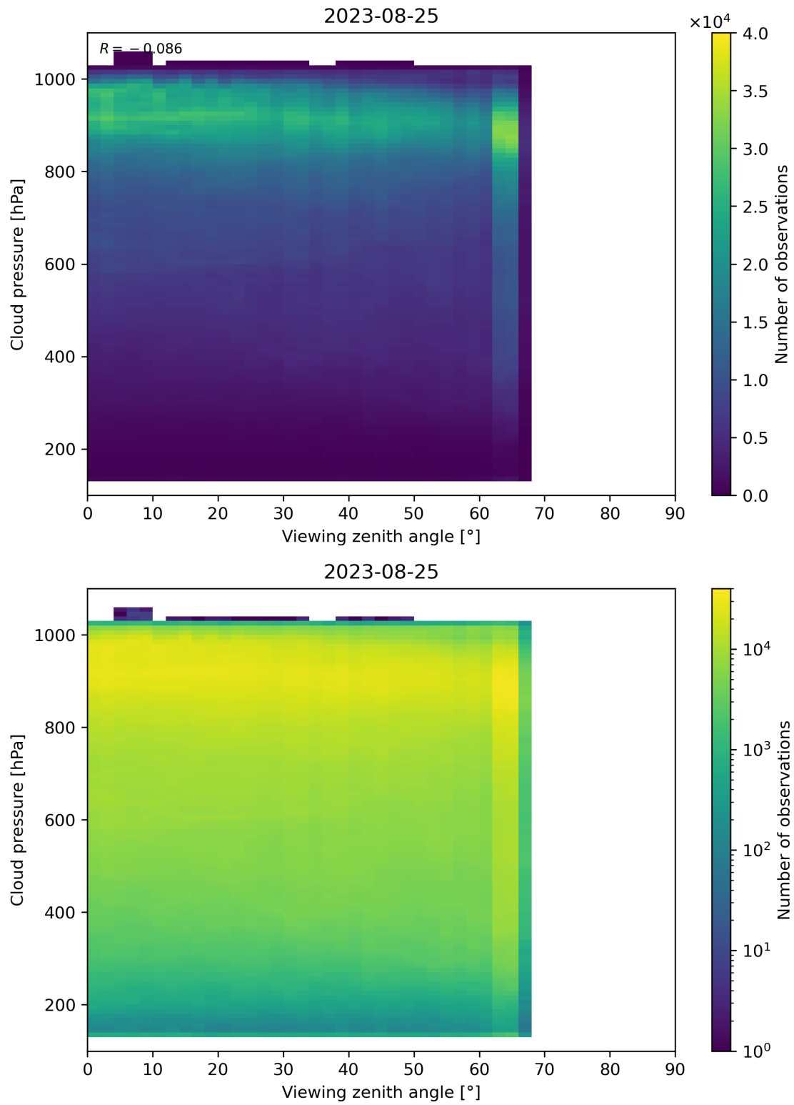
Figure 133: Scatter density plot of “Viewing zenith angle” against “Cloud pressure” for 2023-08-25 to 2023-08-26.
