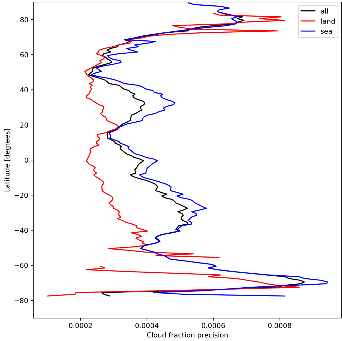
Figure 16: Zonal average of “Cloud fraction precision” for 2023-08-25 to 2023-08-26.
