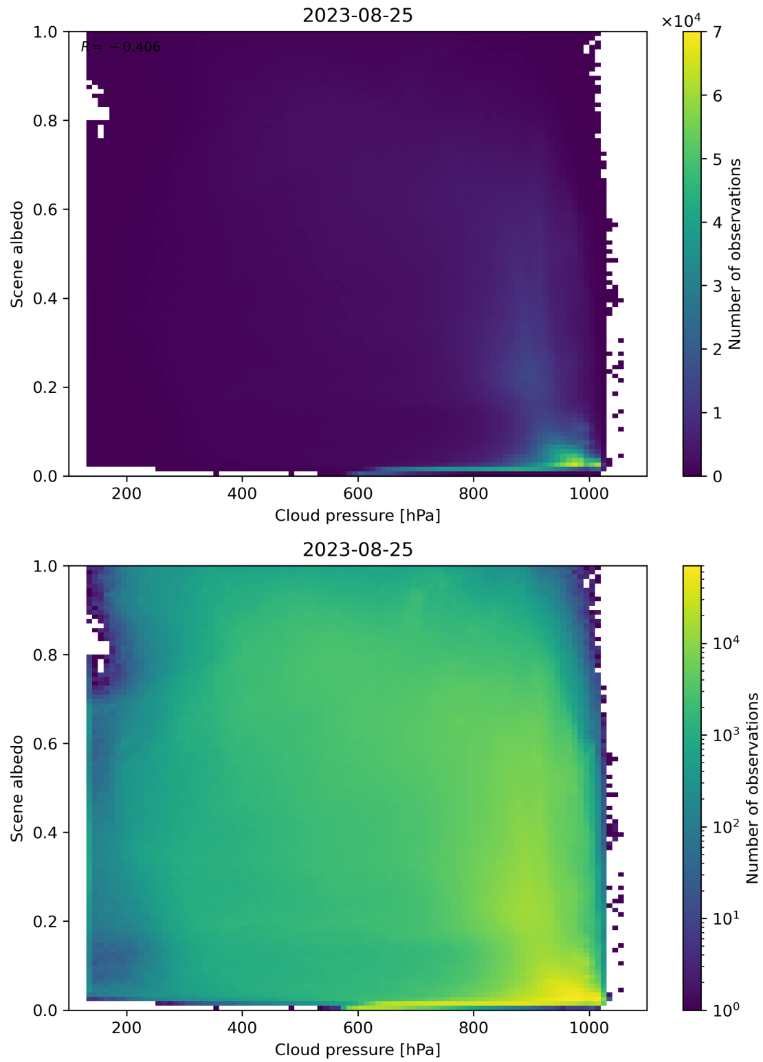
Figure 91: Scatter density plot of “Cloud pressure” against “Scene albedo” for 2023-08-25 to 2023-08-26.
