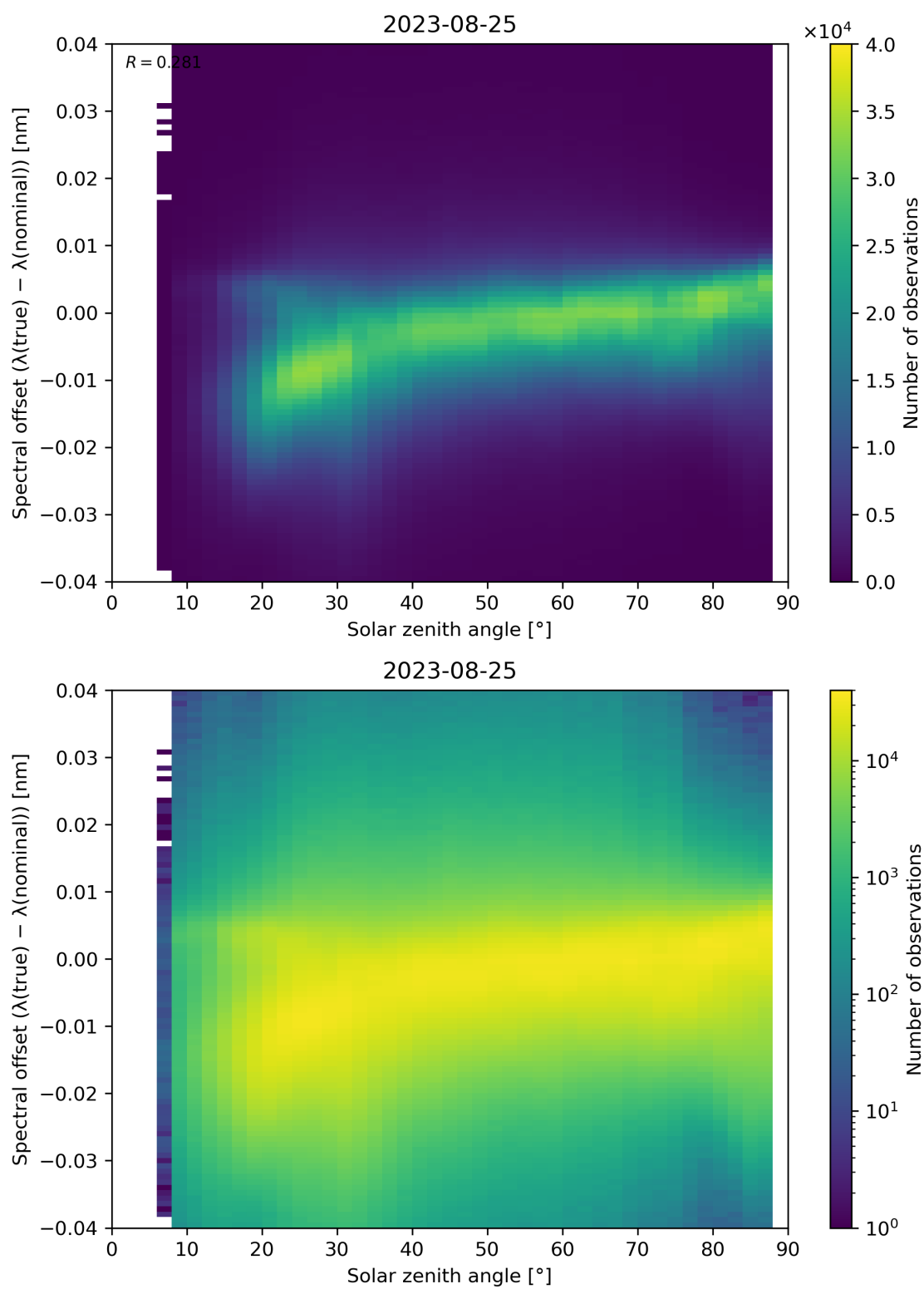
Figure 128: Scatter density plot of “Solar zenith angle” against “Spectral offset ( \lambda(\text{true}) - \lambda(\text{nominal}) )” for 2023-08-25 to 2023-08-26.
