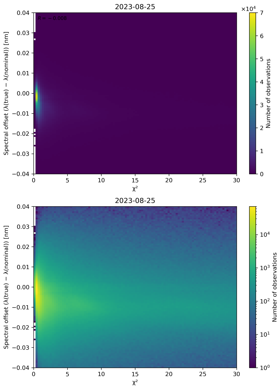
Figure 75: Scatter density plot of “ \chi^2 ” against “Spectral offset ( \lambda(\text{true}) - \lambda(\text{nominal}) )” for 2023-08-25 to 2023-08-26.
