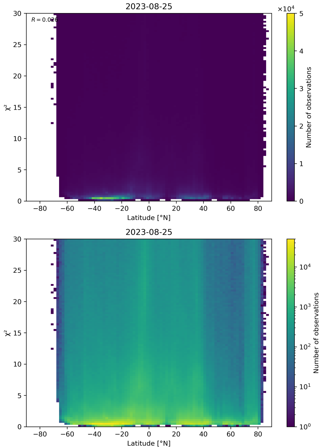
Figure 97: Scatter density plot of “Latitude” against “ \chi^2 ” for 2023-08-25 to 2023-08-26.
