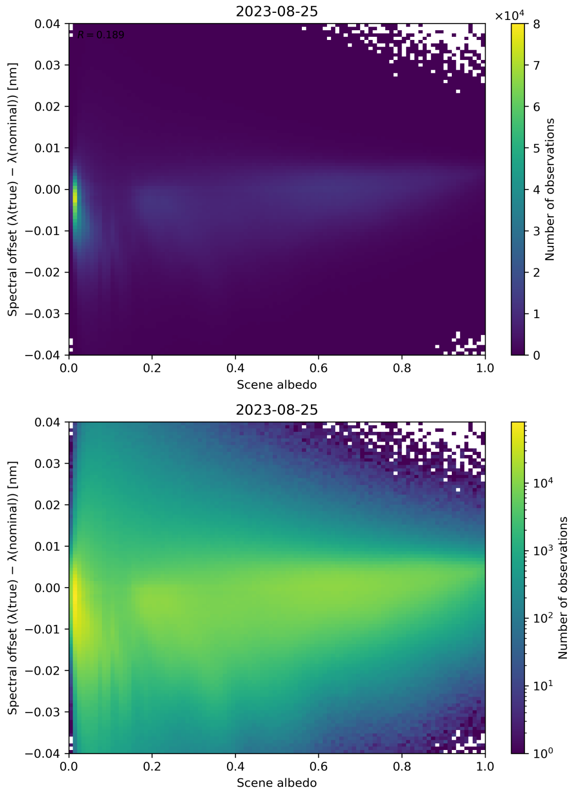
Figure 117: Scatter density plot of “Scene albedo” against “Spectral offset ( \lambda(\text{true}) - \lambda(\text{nominal}) )” for 2023-08-25 to 2023-08-26.
