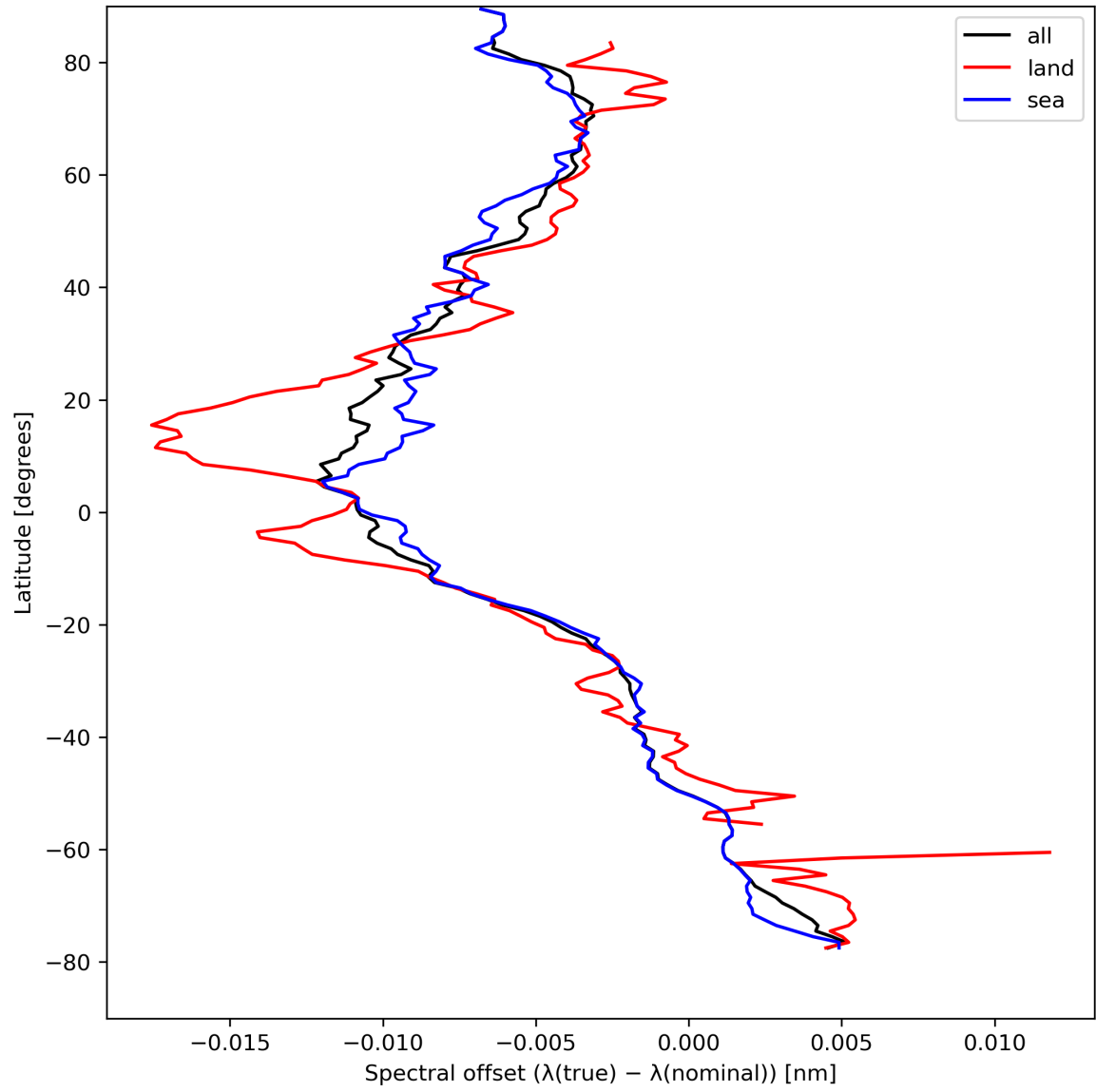
Figure 28: Zonal average of “Spectral offset ( \lambda(\text{true}) - \lambda(\text{nominal}) )” for 2023-08-25 to 2023-08-26.
