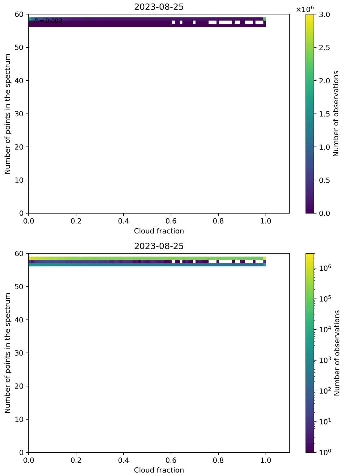
Figure 81: Scatter density plot of “Cloud fraction” against “Number of points in the spectrum” for 2023-08-25 to 2023-08-26.
