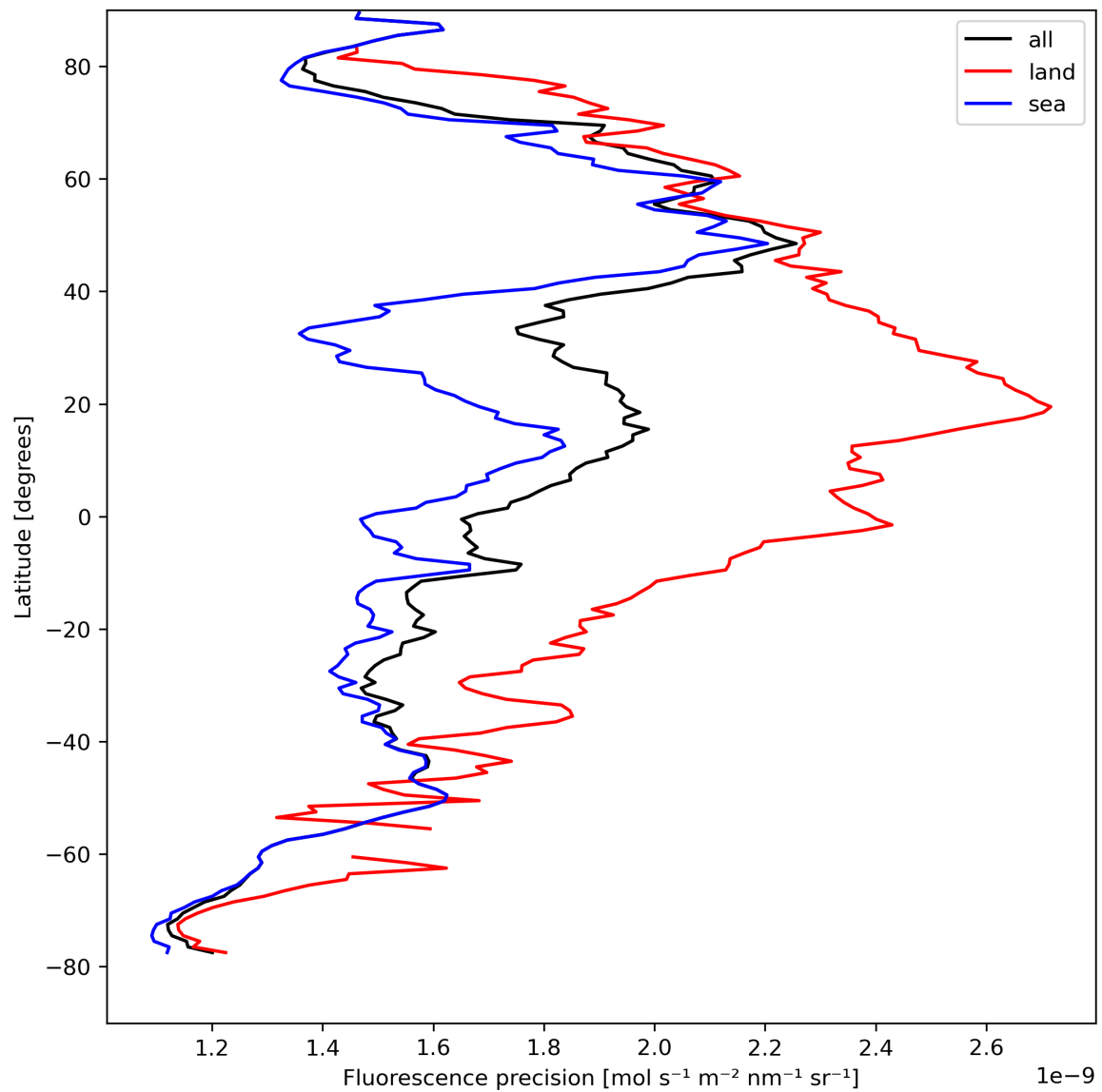
Figure 24: Zonal average of “Fluorescence precision” for 2023-08-25 to 2023-08-26.
