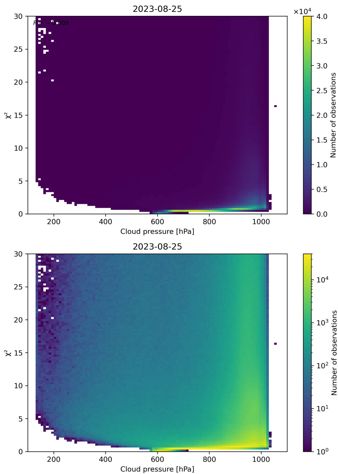
Figure 85: Scatter density plot of “Cloud pressure” against “ \chi^2 ” for 2023-08-25 to 2023-08-26.
