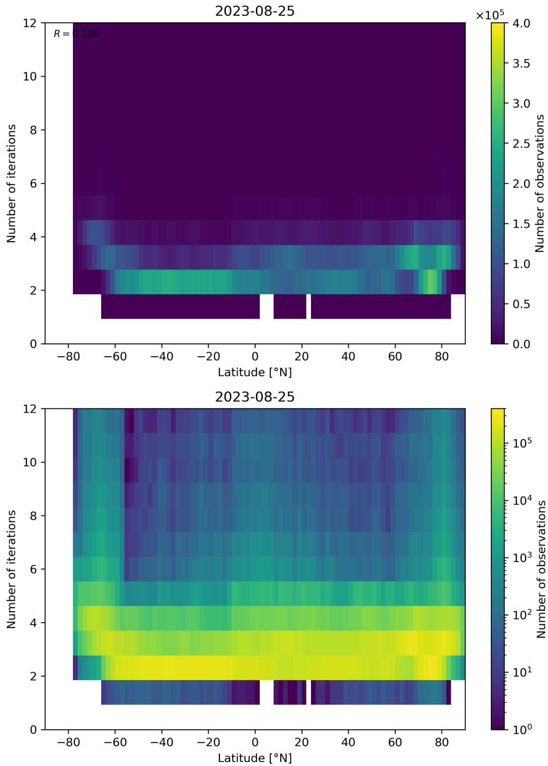
Figure 102: Scatter density plot of “Latitude” against “Number of iterations” for 2023-08-25 to 2023-08-26.
