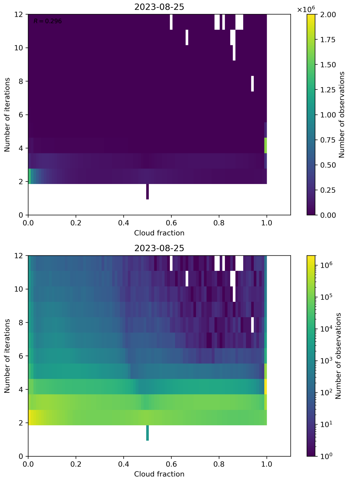
Figure 80: Scatter density plot of “Cloud fraction” against “Number of iterations” for 2023-08-25 to 2023-08-26.
