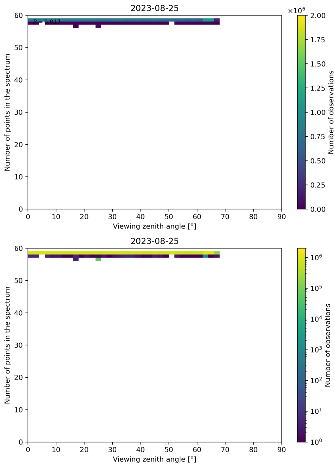
Figure 137: Scatter density plot of “Viewing zenith angle” against “Number of points in the spectrum” for 2023-08-25 to 2023-08-26.
