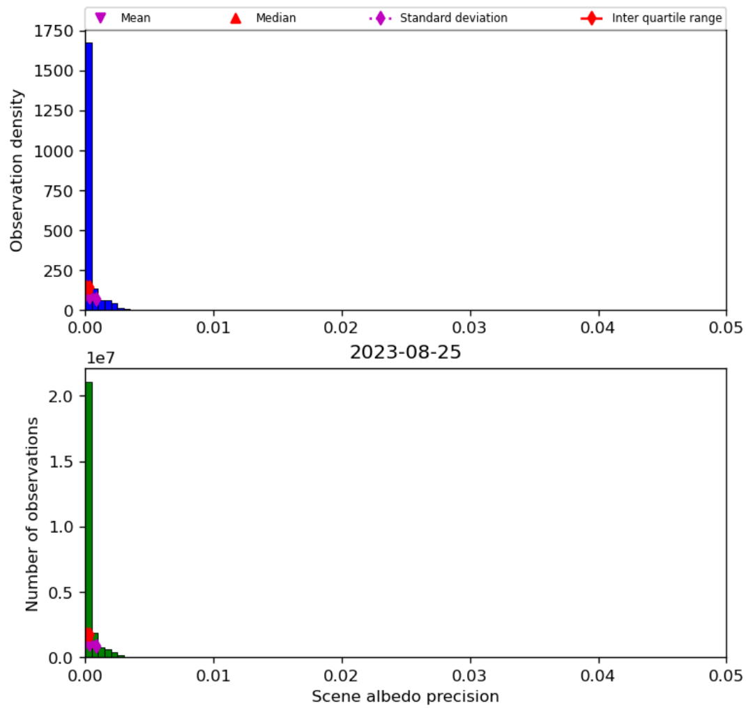
Figure 35: Histogram of “Scene albedo precision” for 2023-08-25 to 2023-08-26
