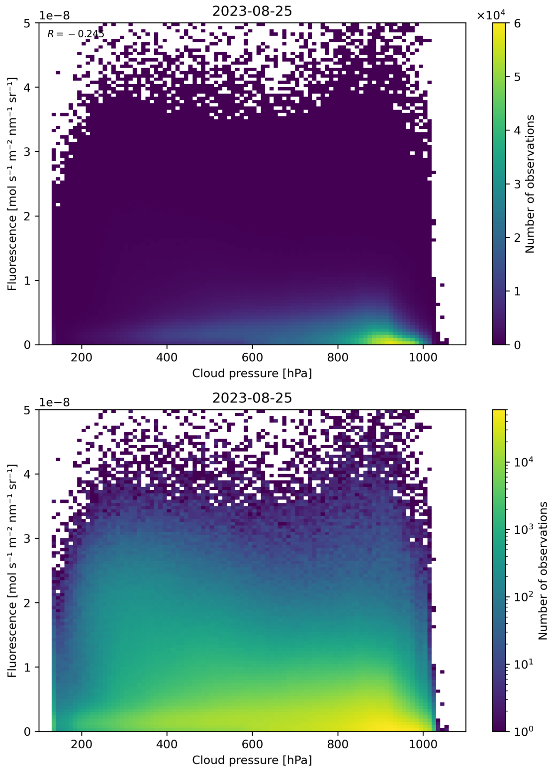
Figure 88: Scatter density plot of “Cloud pressure” against “Fluorescence” for 2023-08-25 to 2023-08-26.
