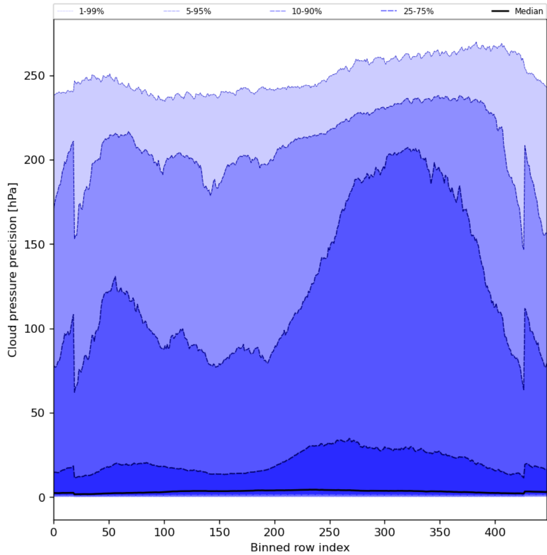
Figure 48: Along track statistics of “Cloud pressure precision” for 2023-08-25 to 2023-08-26
