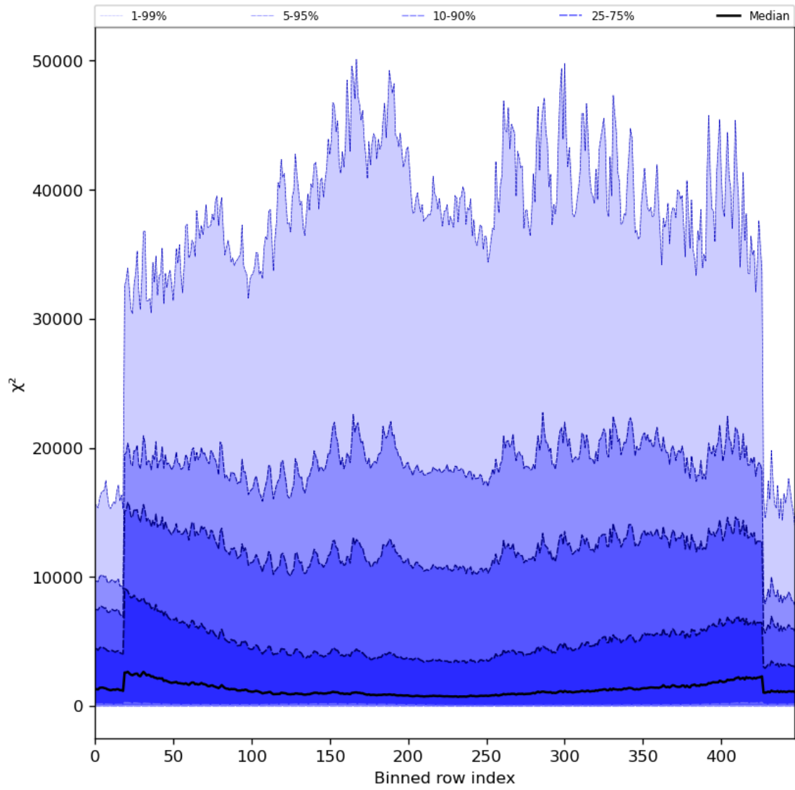
Figure 55: Along track statistics of “ \chi^2 ” for 2023-08-25 to 2023-08-26
