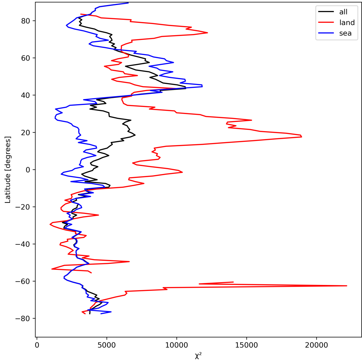
Figure 21: Zonal average of “ \chi^2 ” for 2023-08-25 to 2023-08-26.
