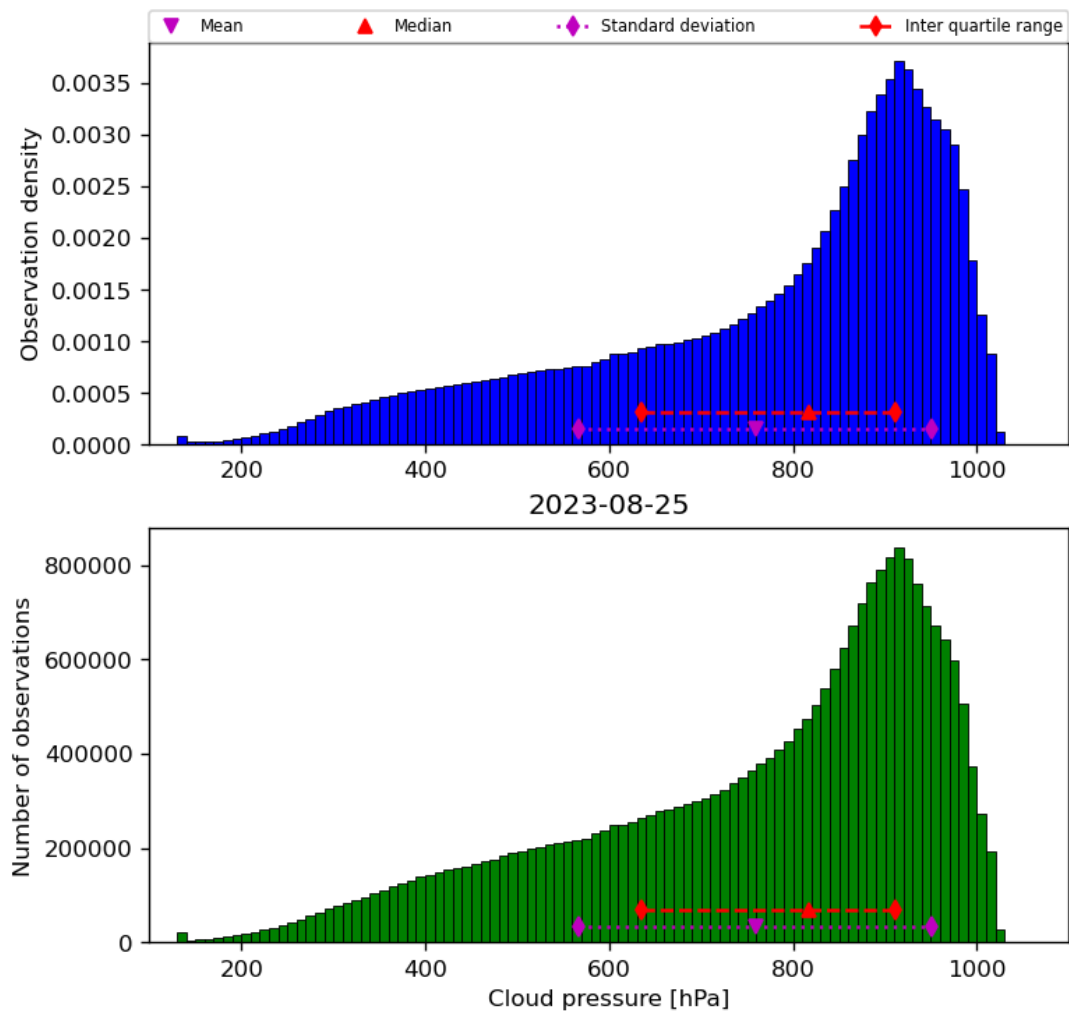
Figure 30: Histogram of “Cloud pressure” for 2023-08-25 to 2023-08-26
