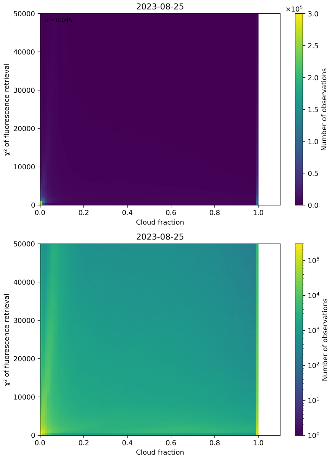
Figure 78: Scatter density plot of “Cloud fraction” against “ \chi^2 of fluorescence retrieval” for 2023-08-25 to 2023-08-26.
