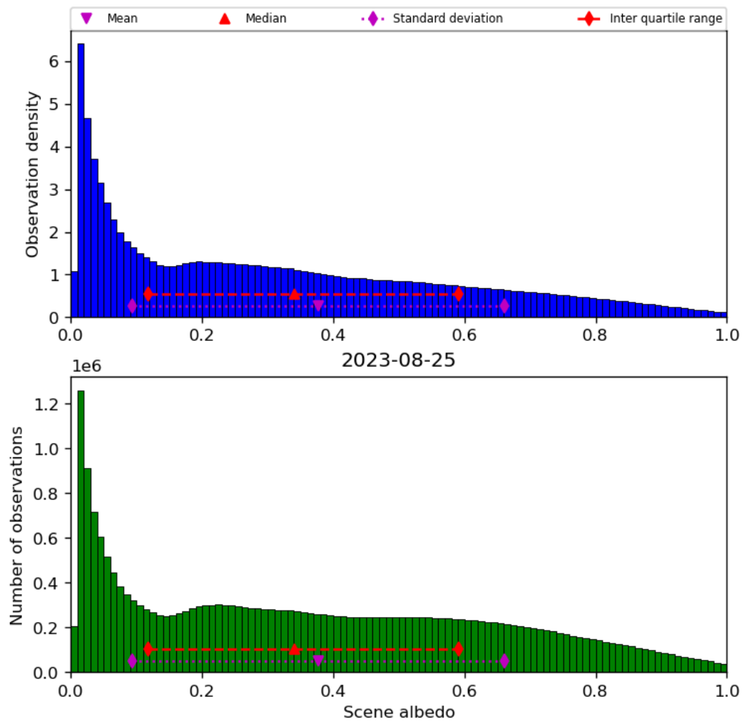
Figure 34: Histogram of “Scene albedo” for 2023-08-25 to 2023-08-26
