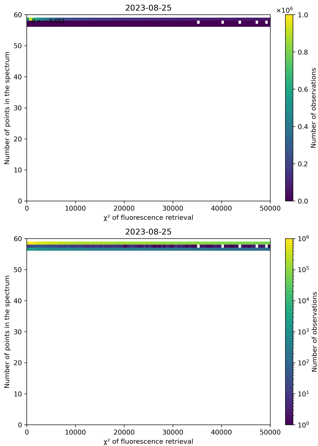
Figure 71: Scatter density plot of " \chi^2 of fluorescence retrieval" against "Number of points in the spectrum" for 2023-08-25 to 2023-08-26.
