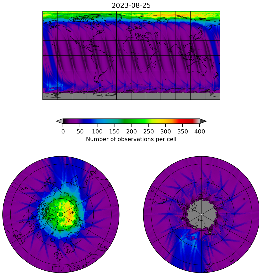
Figure 11: Map of the number of observations for 2023-08-25 to 2023-08-26
