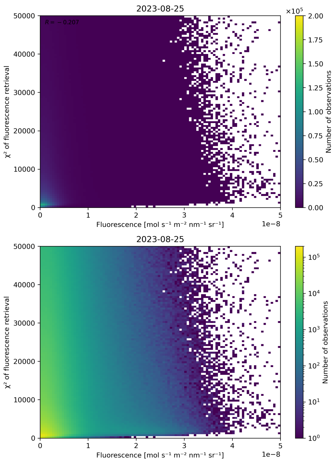
Figure 93: Scatter density plot of “Fluorescence” against “ \chi^2 of fluorescence retrieval” for 2023-08-25 to 2023-08-26.
