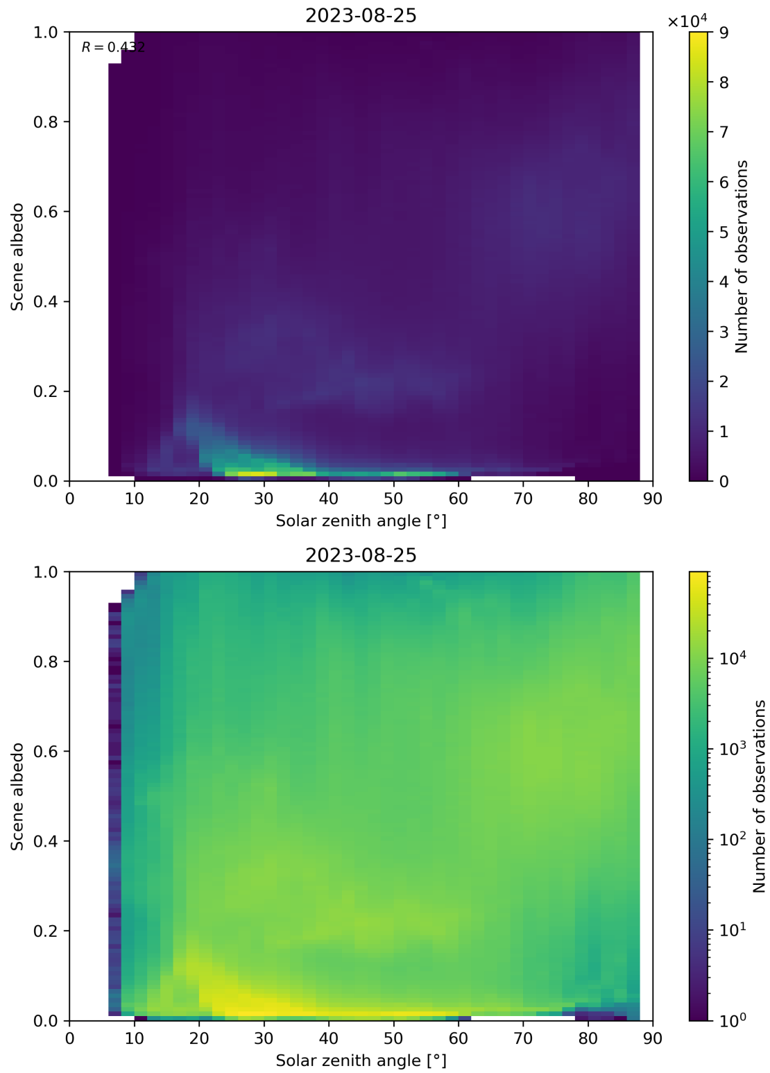
Figure 127: Scatter density plot of “Solar zenith angle” against “Scene albedo” for 2023-08-25 to 2023-08-26.
