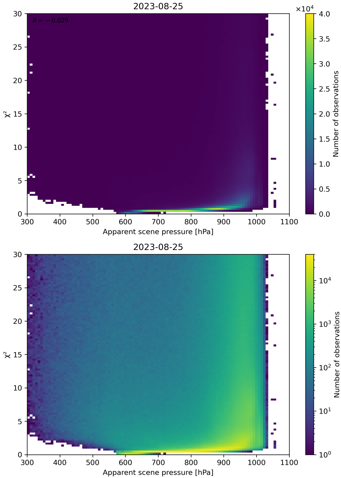
Figure 63: Scatter density plot of “Apparent scene pressure” against “ \chi^2 ” for 2023-08-25 to 2023-08-26.
