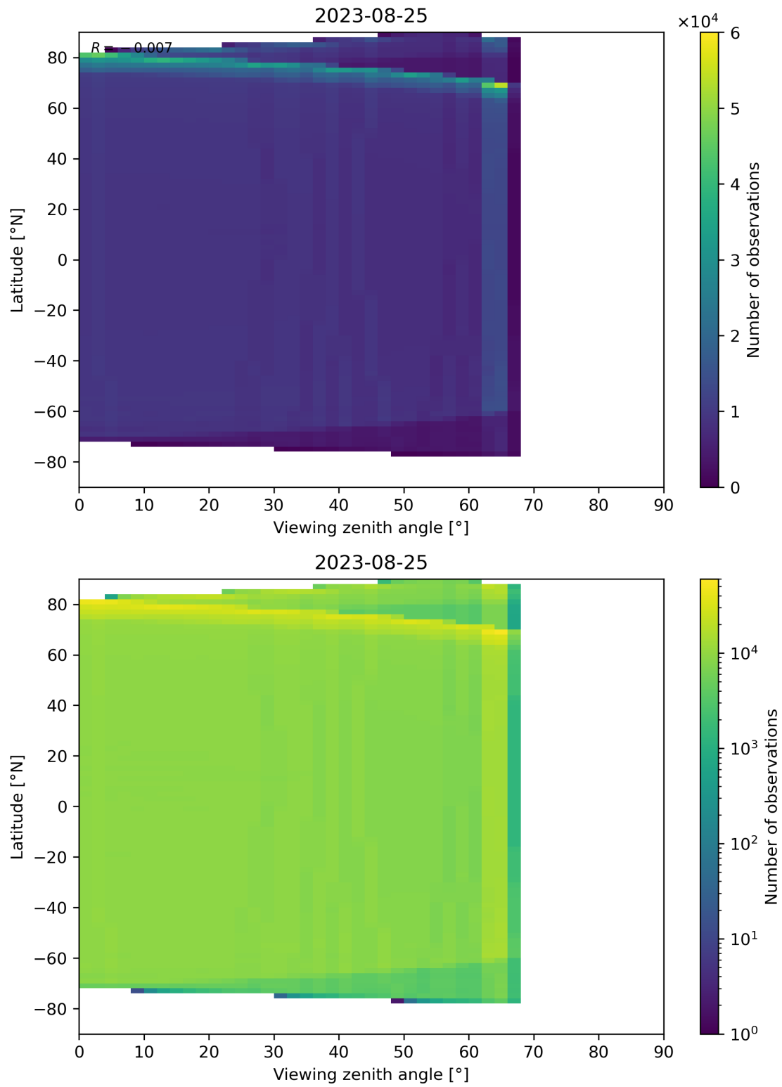
Figure 135: Scatter density plot of “Viewing zenith angle” against “Latitude” for 2023-08-25 to 2023-08-26.
