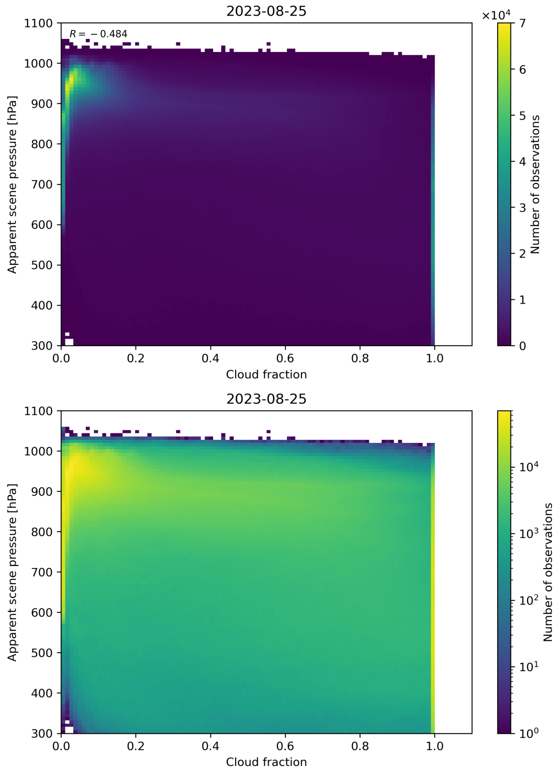
Figure 76: Scatter density plot of “Cloud fraction” against “Apparent scene pressure” for 2023-08-25 to 2023-08-26.
