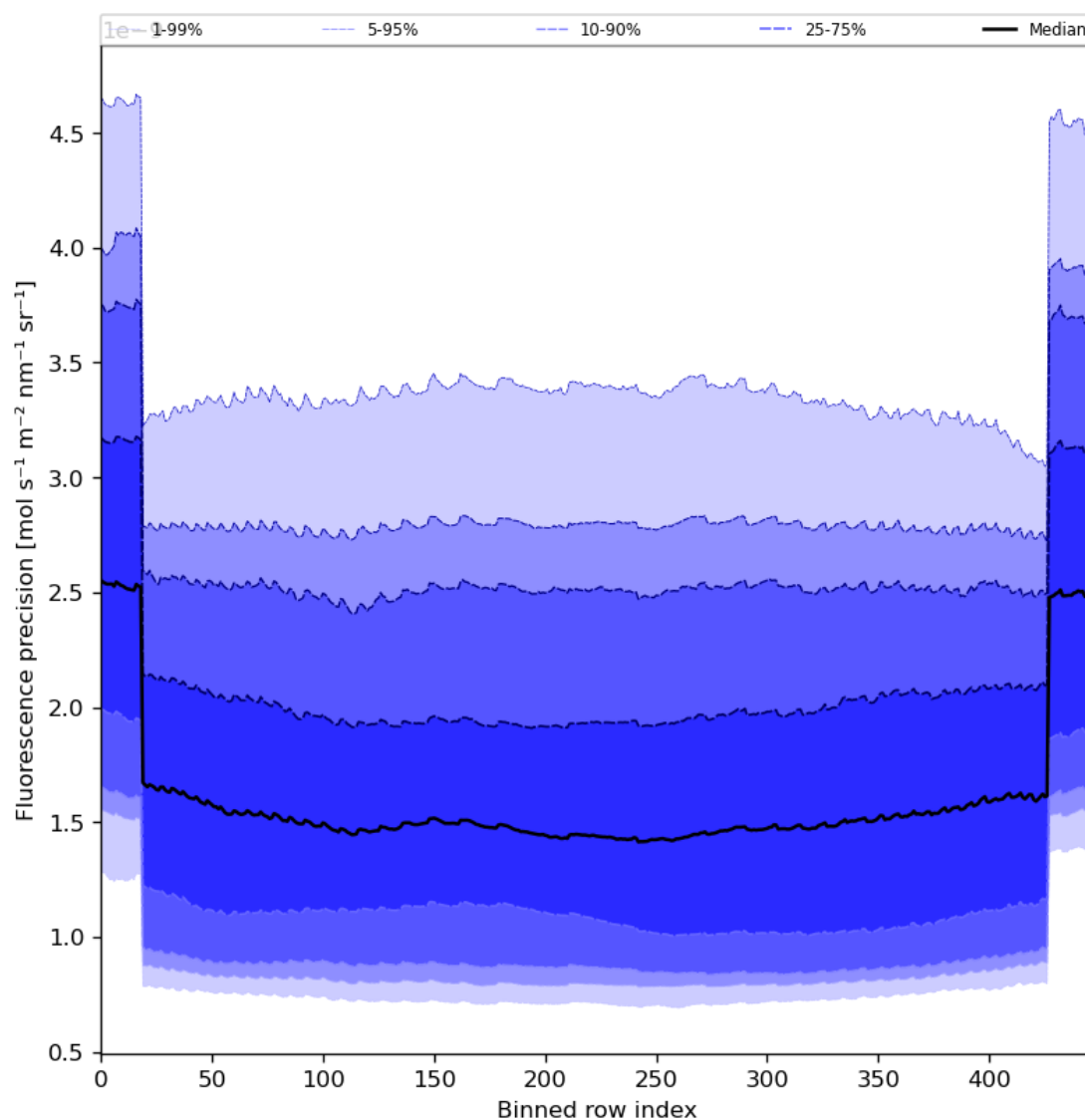
Figure 58: Along track statistics of “Fluorescence precision” for 2023-08-25 to 2023-08-26
