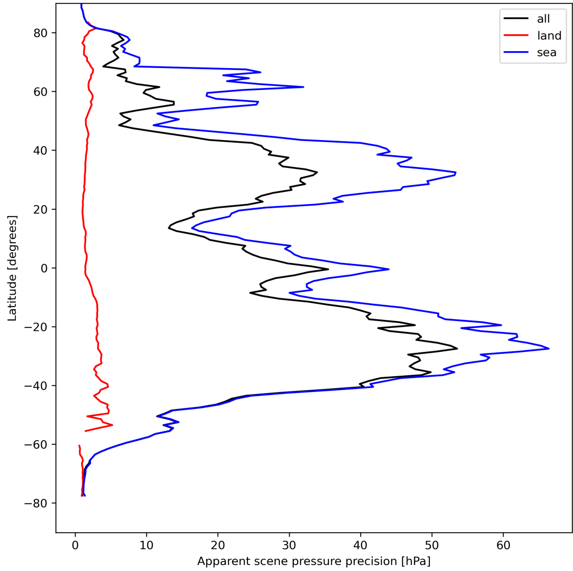
Figure 20: Zonal average of “Apparent scene pressure precision” for 2023-08-25 to 2023-08-26.
