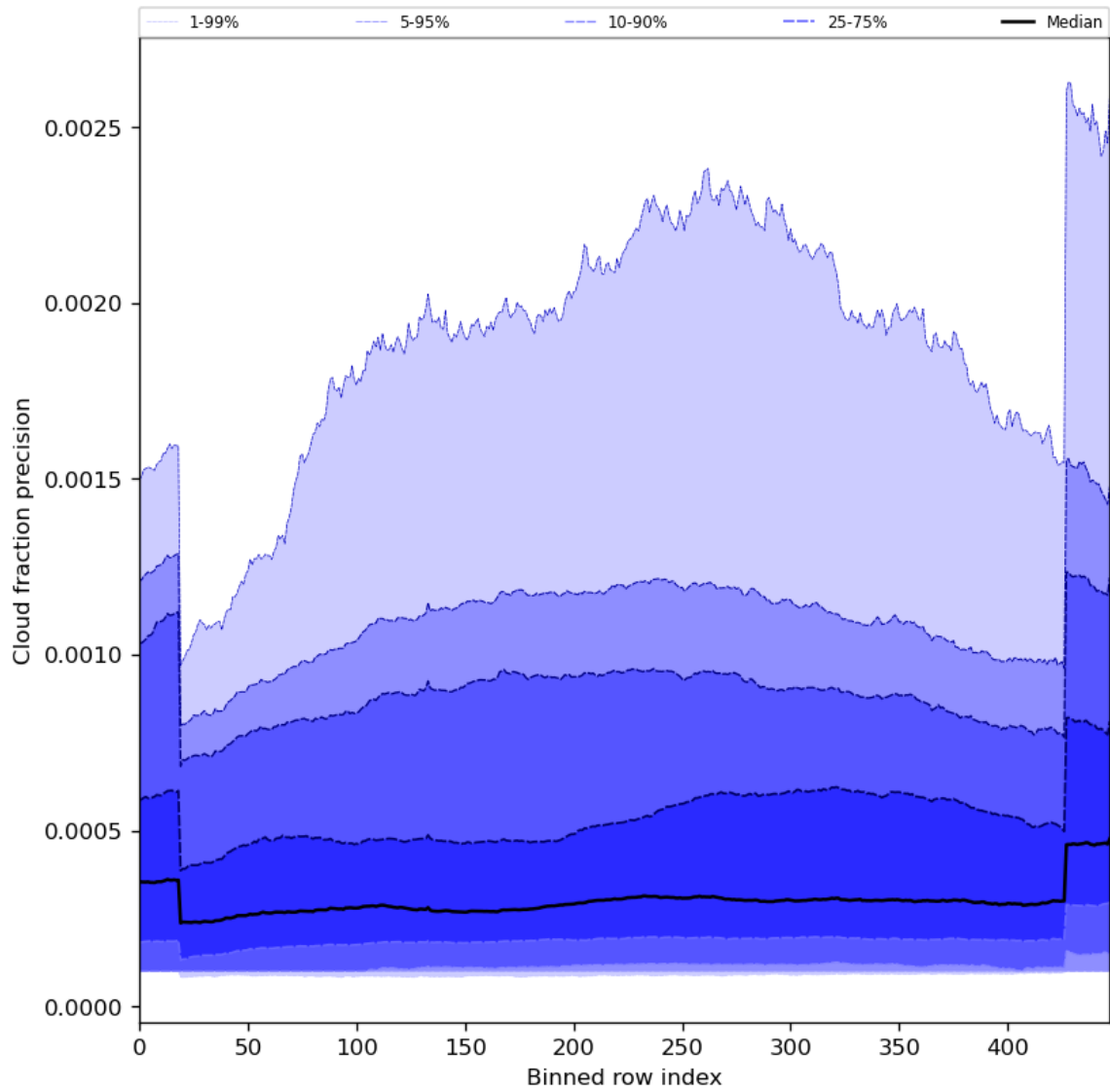
Figure 50: Along track statistics of “Cloud fraction precision” for 2023-08-25 to 2023-08-26
