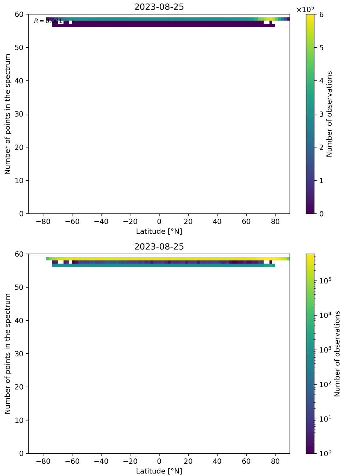
Figure 103: Scatter density plot of “Latitude” against “Number of points in the spectrum” for 2023-08-25 to 2023-08-26.
