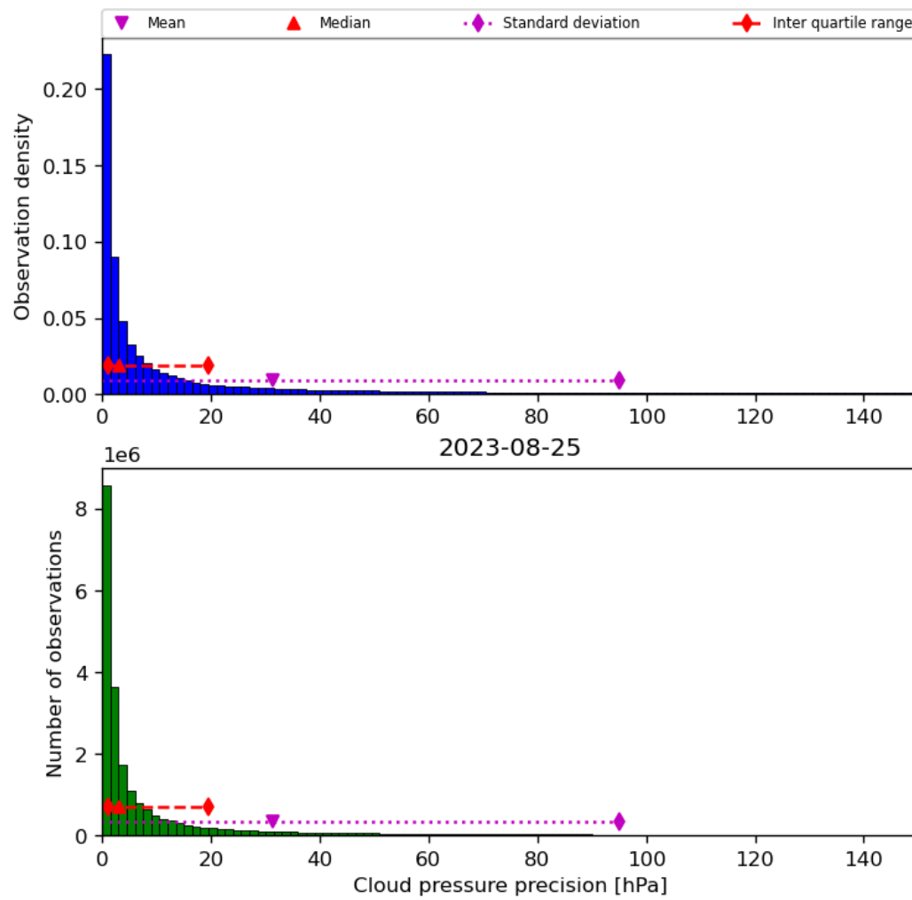
Figure 31: Histogram of “Cloud pressure precision” for 2023-08-25 to 2023-08-26
