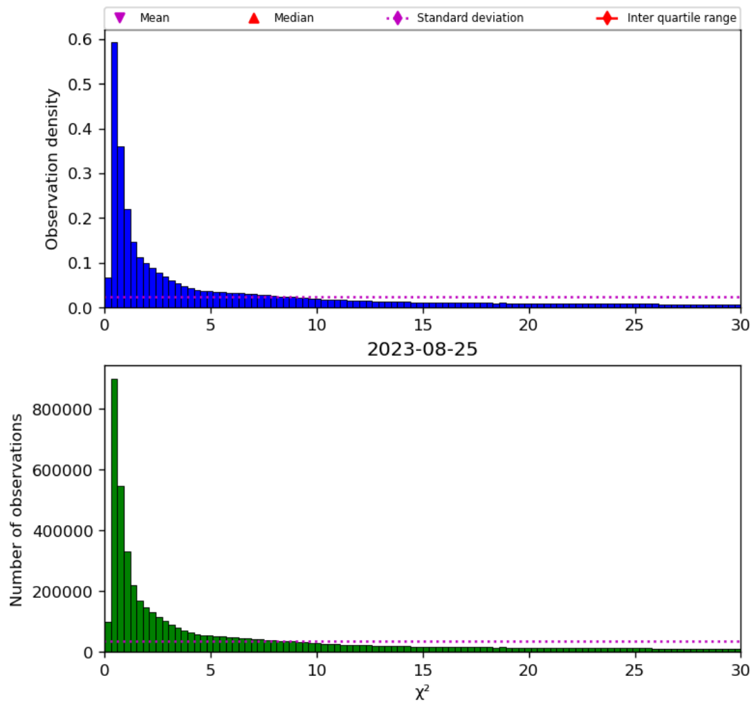
Figure 38: Histogram of “ \chi^2 ” for 2023-08-25 to 2023-08-26
