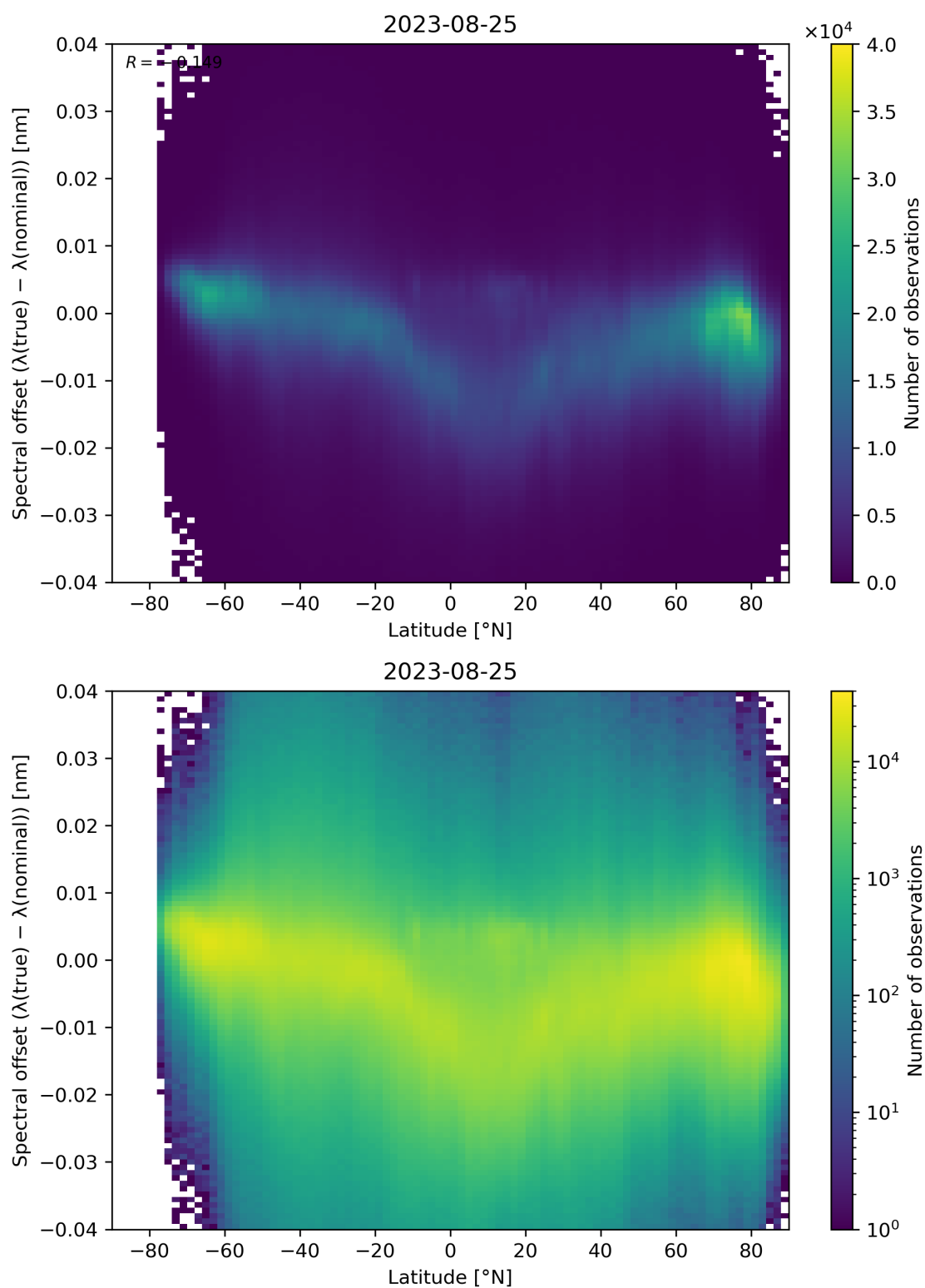
Figure 105: Scatter density plot of “Latitude” against “Spectral offset ( \lambda(\text{true}) - \lambda(\text{nominal}) )” for 2023-08-25 to 2023-08-26.
