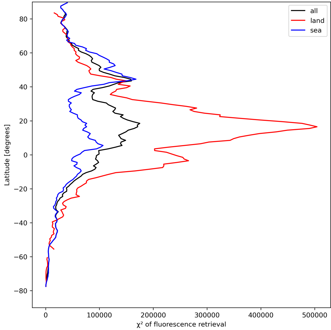
Figure 25: Zonal average of “ \chi^2 of fluorescence retrieval” for 2023-08-25 to 2023-08-26.
