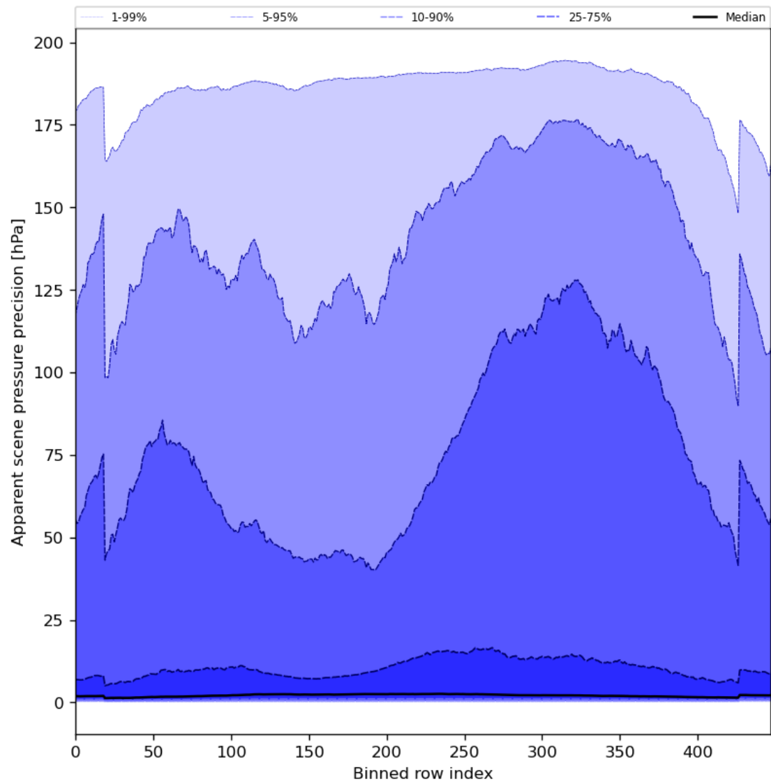
Figure 54: Along track statistics of “Apparent scene pressure precision” for 2023-08-25 to 2023-08-26
