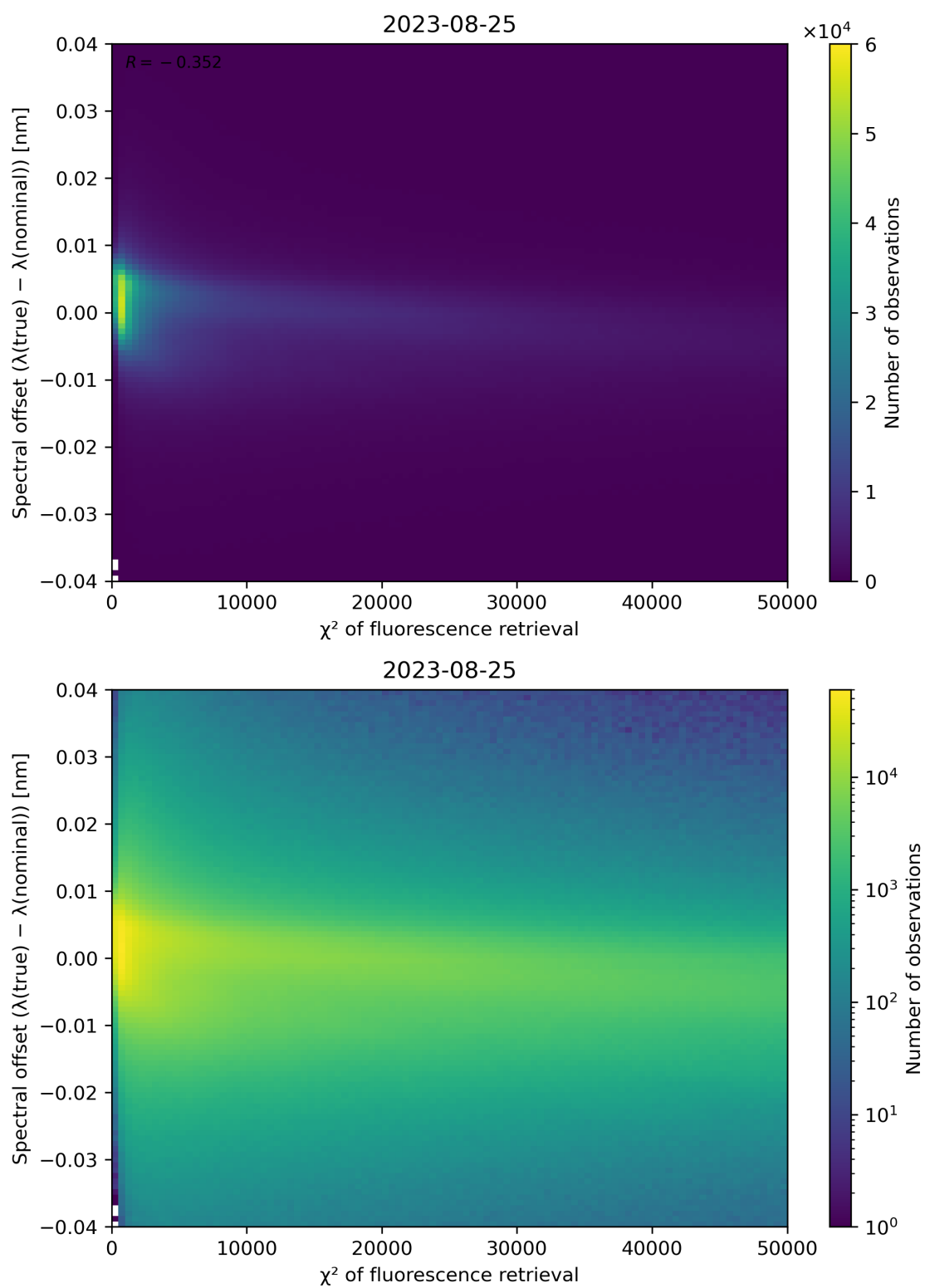
Figure 72: Scatter density plot of " \chi^2 of fluorescence retrieval" against "Spectral offset ( \lambda(\text{true}) - \lambda(\text{nominal}) )" for 2023-08-25 to 2023-08-26.
