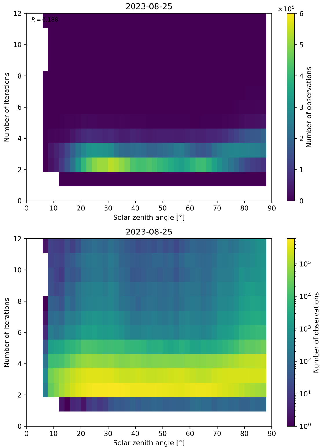
Figure 125: Scatter density plot of “Solar zenith angle” against “Number of iterations” for 2023-08-25 to 2023-08-26.
