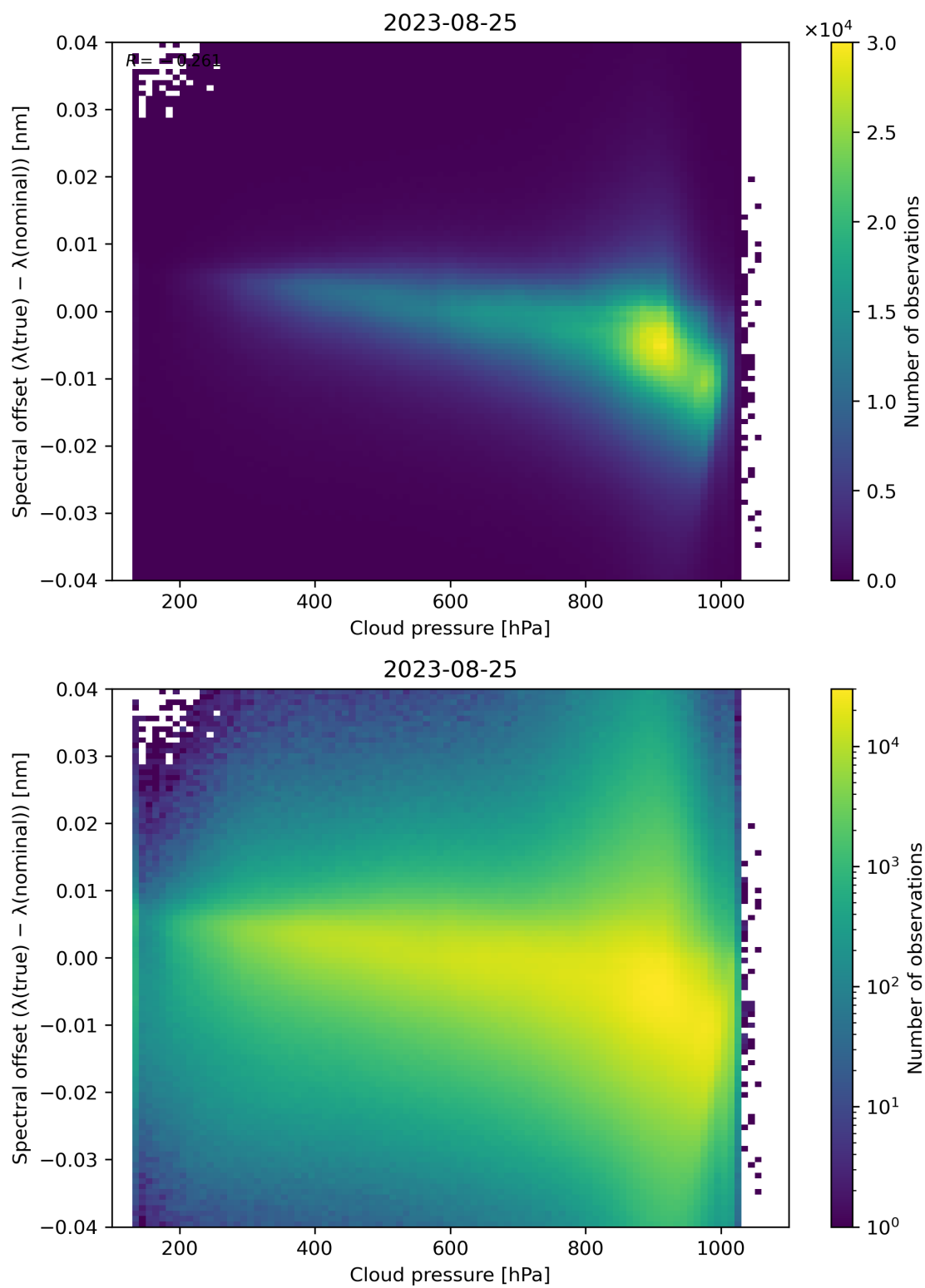
Figure 92: Scatter density plot of “Cloud pressure” against “Spectral offset ( \lambda(\text{true}) - \lambda(\text{nominal}) )” for 2023-08-25 to 2023-08-26.
