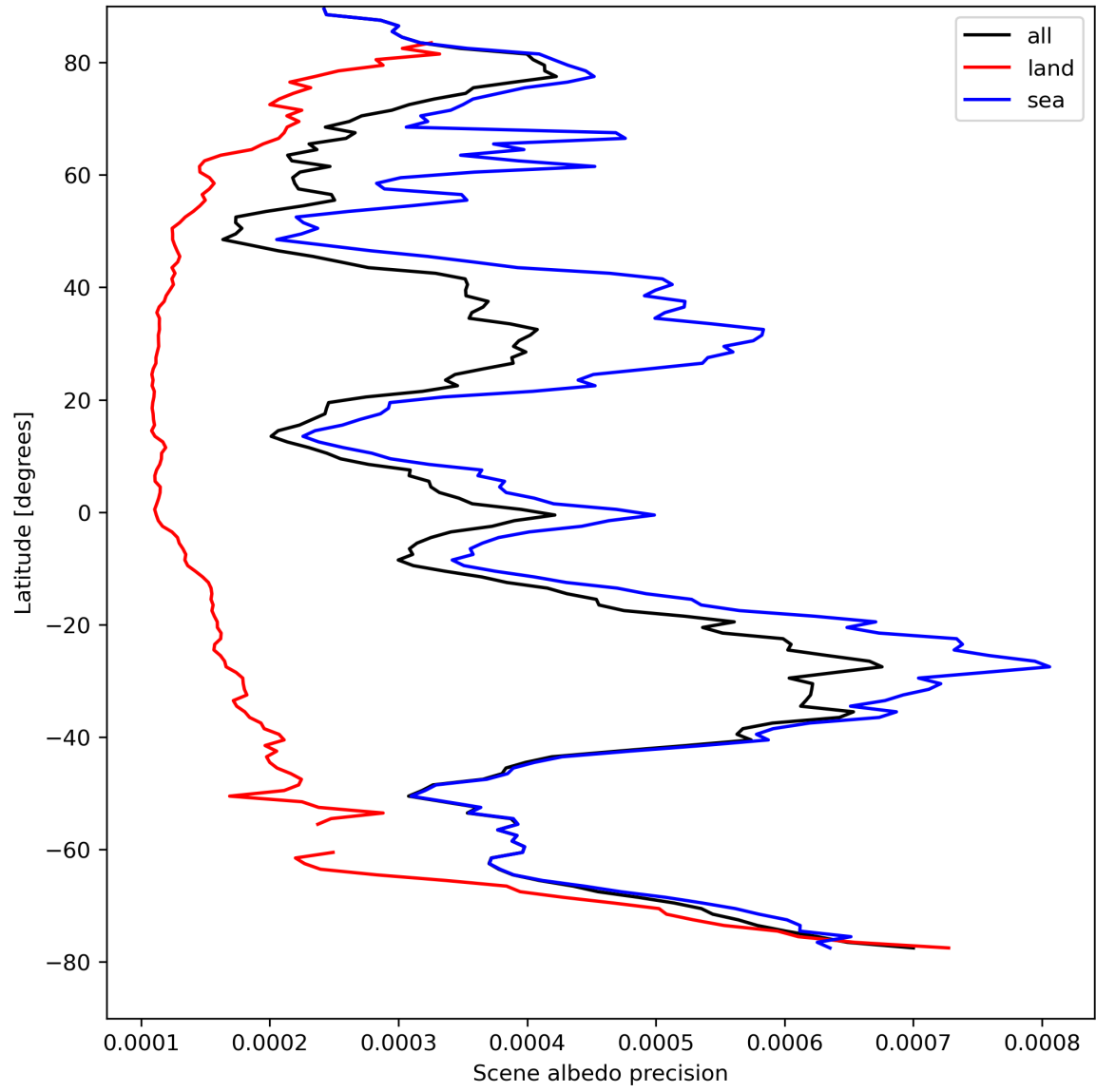
Figure 18: Zonal average of “Scene albedo precision” for 2023-08-25 to 2023-08-26.
