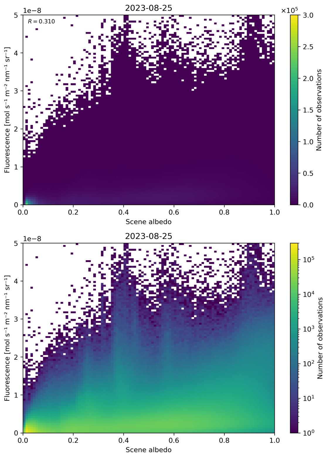
Figure 114: Scatter density plot of “Scene albedo” against “Fluorescence” for 2023-08-25 to 2023-08-26.
