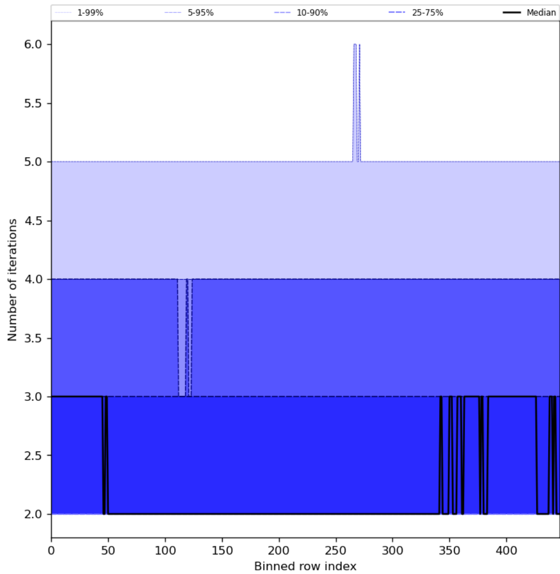
Figure 56: Along track statistics of “Number of iterations” for 2023-08-25 to 2023-08-26
