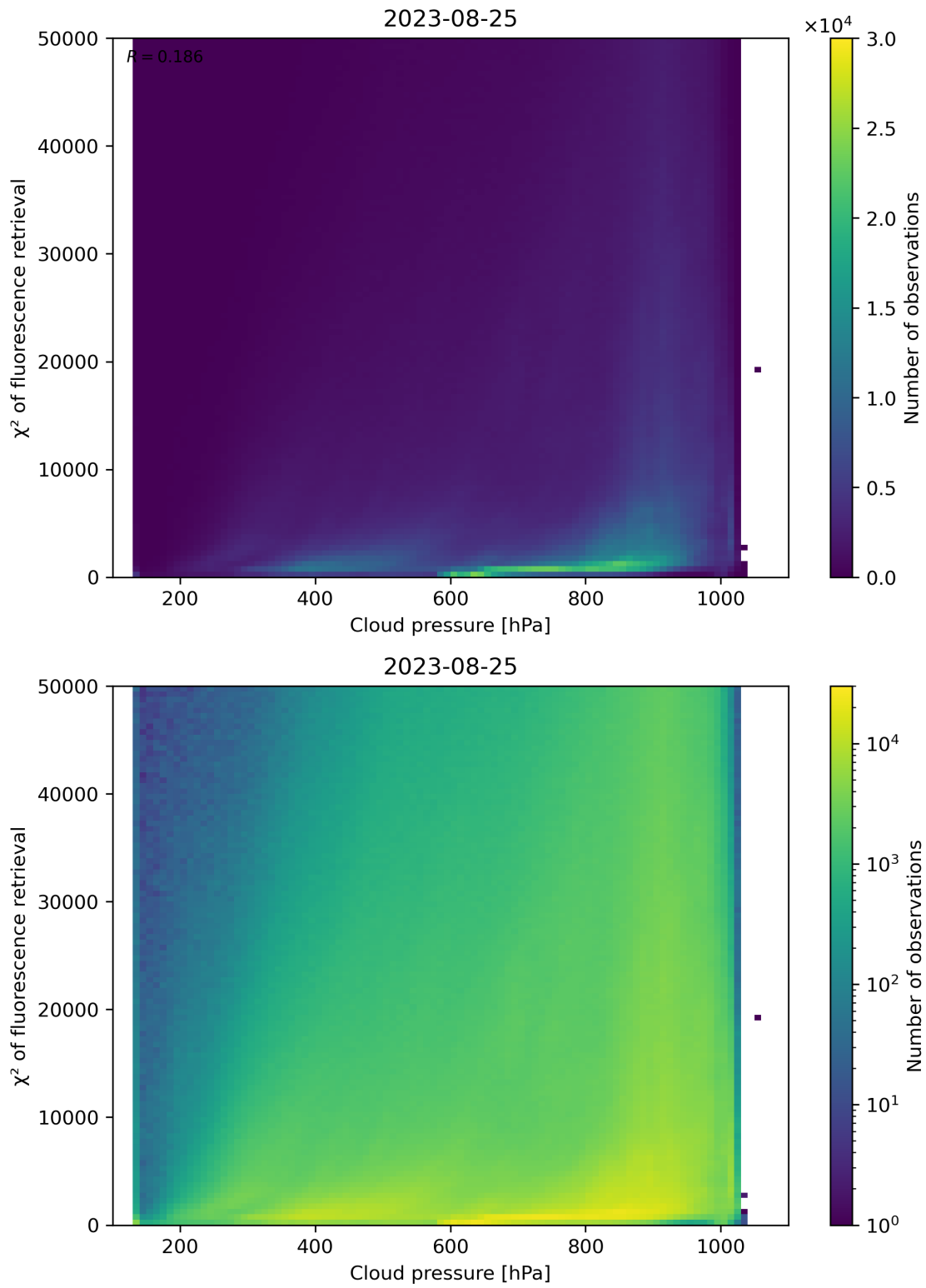
Figure 86: Scatter density plot of “Cloud pressure” against “ \chi^2 of fluorescence retrieval” for 2023-08-25 to 2023-08-26.
