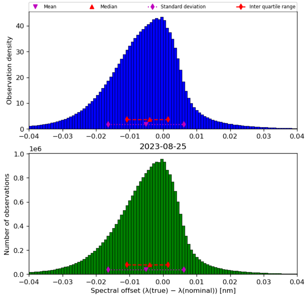
Figure 45: Histogram of “Spectral offset ( \lambda(\text{true}) - \lambda(\text{nominal}) )” for 2023-08-25 to 2023-08-26
