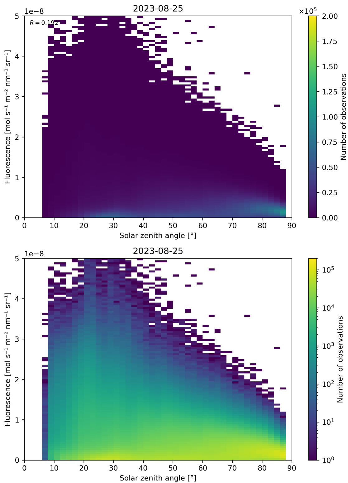
Figure 123: Scatter density plot of “Solar zenith angle” against “Fluorescence” for 2023-08-25 to 2023-08-26.
