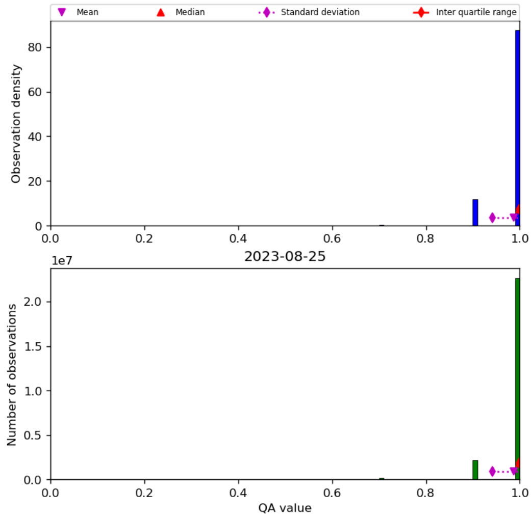
Figure 29: Histogram of “QA value” for 2023-08-25 to 2023-08-26
