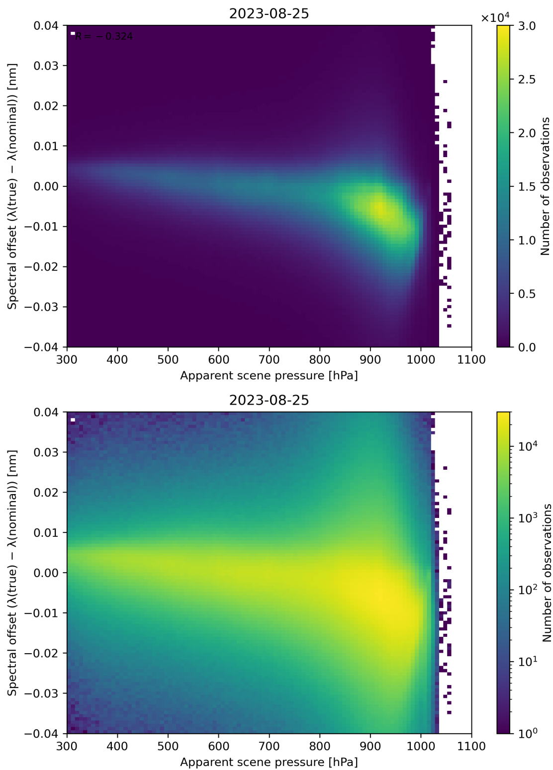
Figure 68: Scatter density plot of “Apparent scene pressure” against “Spectral offset ( \lambda(\text{true}) - \lambda(\text{nominal}) )” for 2023-08-25 to 2023-08-26.
