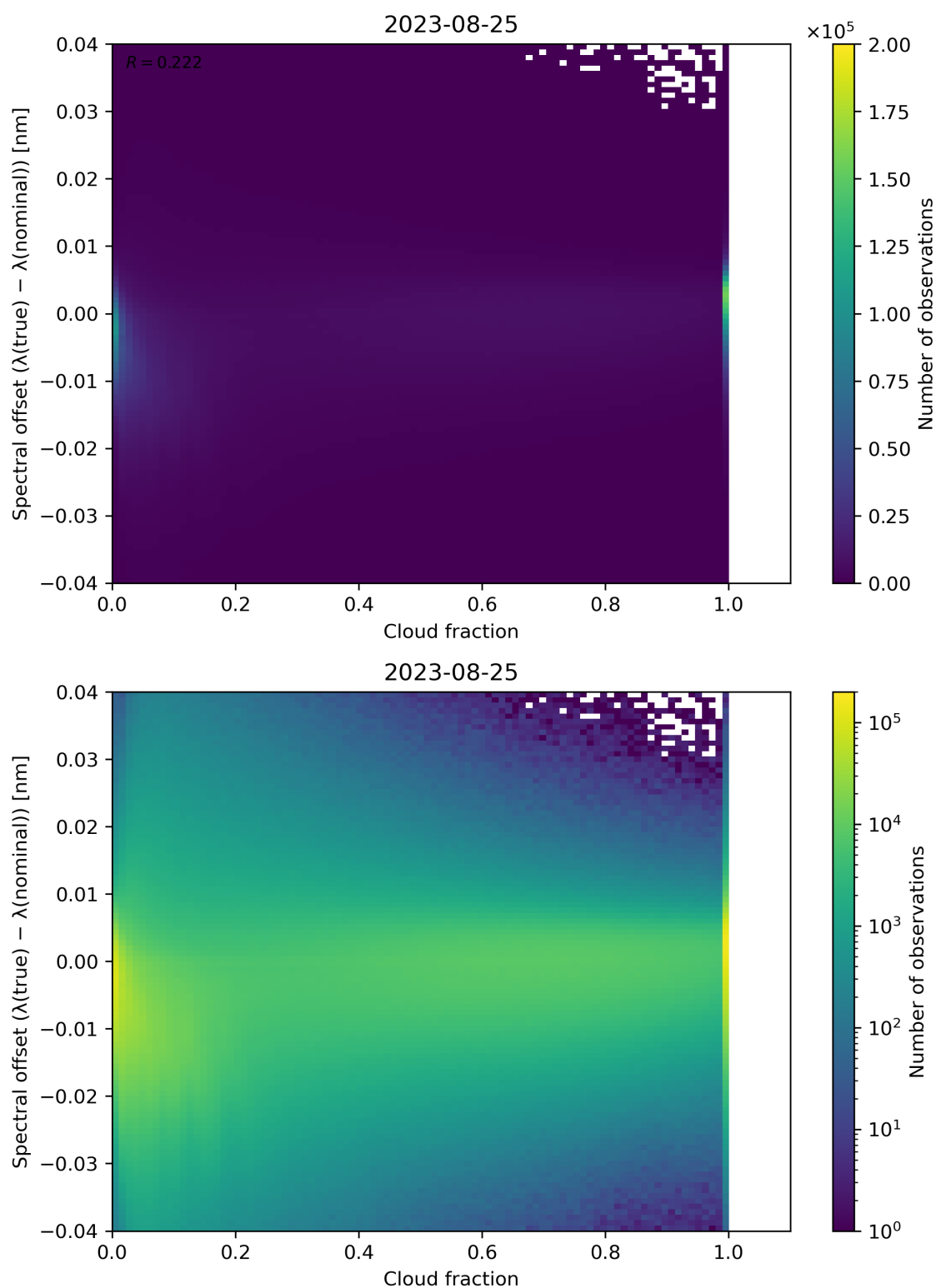
Figure 83: Scatter density plot of “Cloud fraction” against “Spectral offset ( \lambda(\text{true}) - \lambda(\text{nominal}) )” for 2023-08-25 to 2023-08-26.
