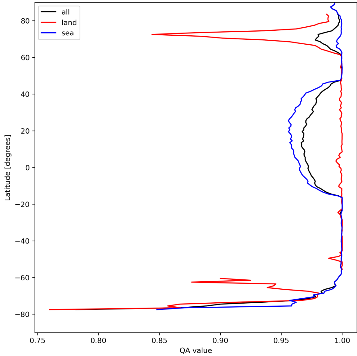
Figure 12: Zonal average of "QA value" for 2023-08-25 to 2023-08-26.
