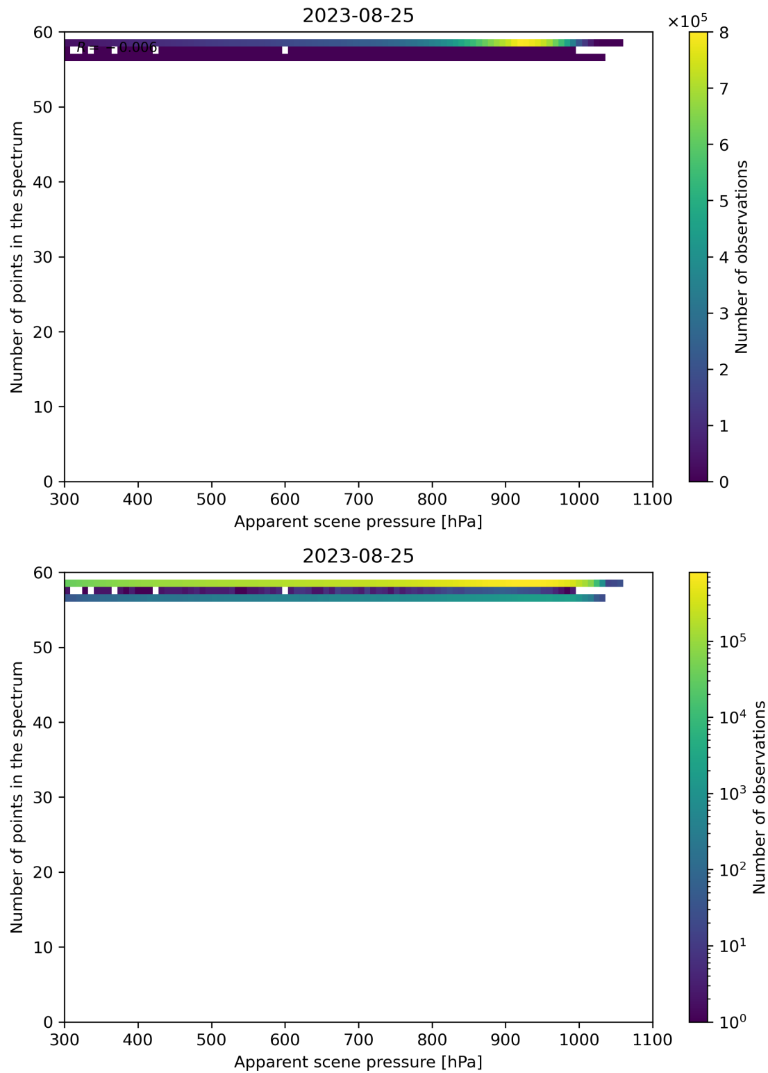
Figure 67: Scatter density plot of “Apparent scene pressure” against “Number of points in the spectrum” for 2023-08-25 to 2023-08-26.
