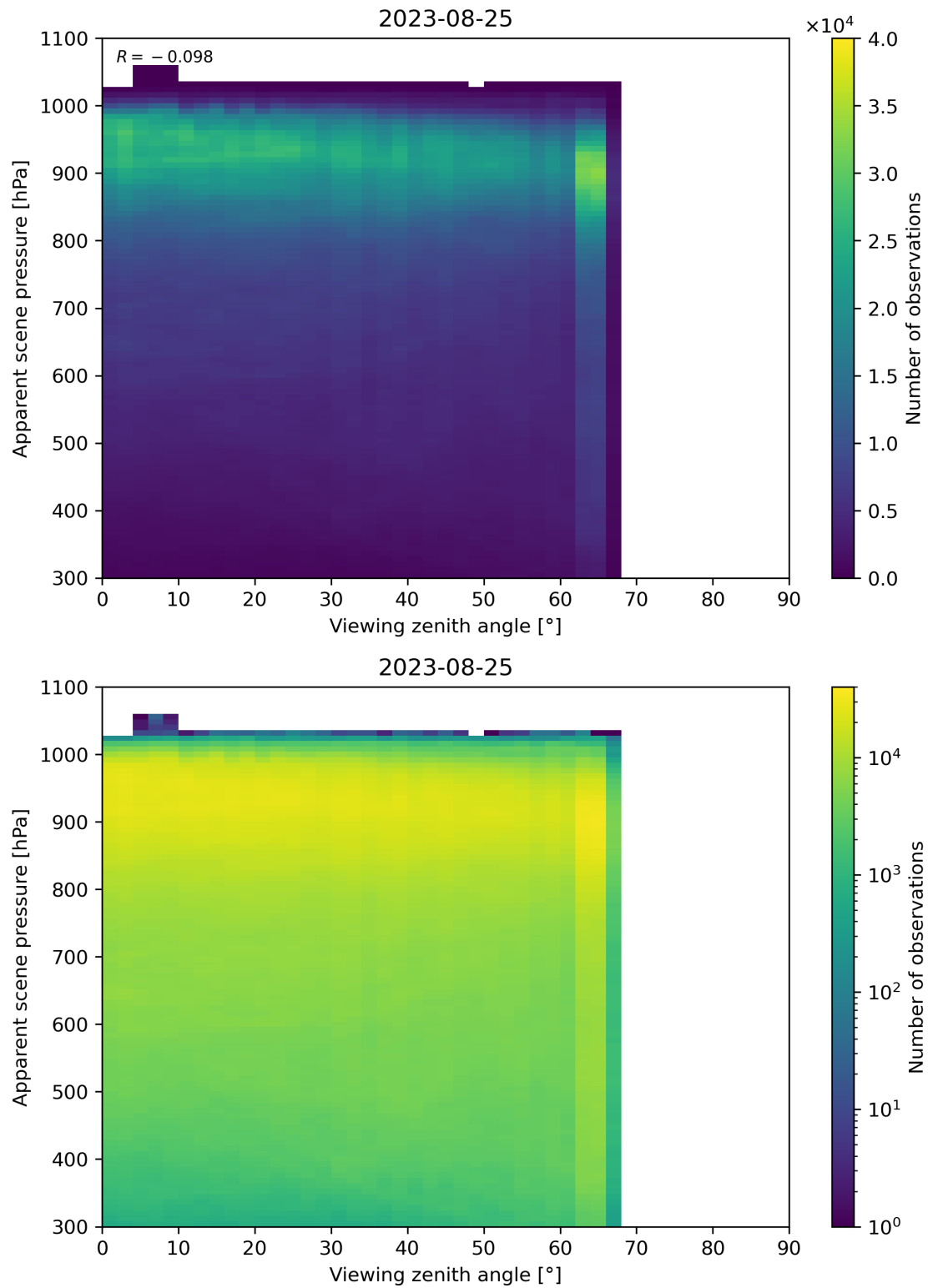
Figure 129: Scatter density plot of “Viewing zenith angle” against “Apparent scene pressure” for 2023-08-25 to 2023-08-26.
