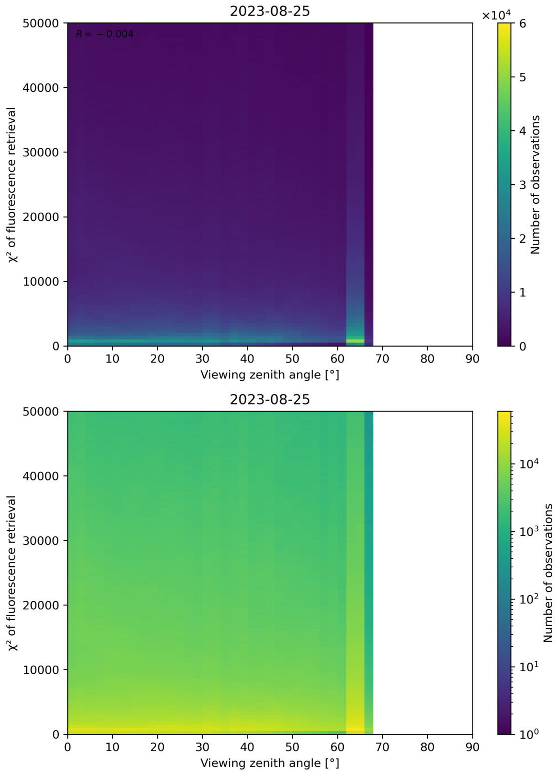
Figure 131: Scatter density plot of “Viewing zenith angle” against “ \chi^2 of fluorescence retrieval” for 2023-08-25 to 2023-08-26.
