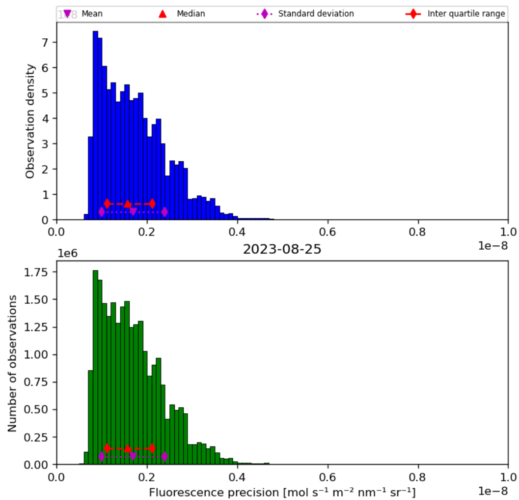
Figure 41: Histogram of “Fluorescence precision” for 2023-08-25 to 2023-08-26
