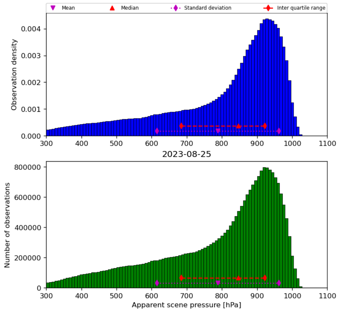
Figure 36: Histogram of “Apparent scene pressure” for 2023-08-25 to 2023-08-26
