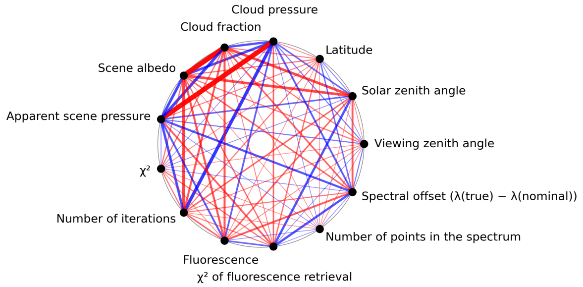
Figure 1: Map of correlation graph for 2023-08-25 to 2023-08-26.
