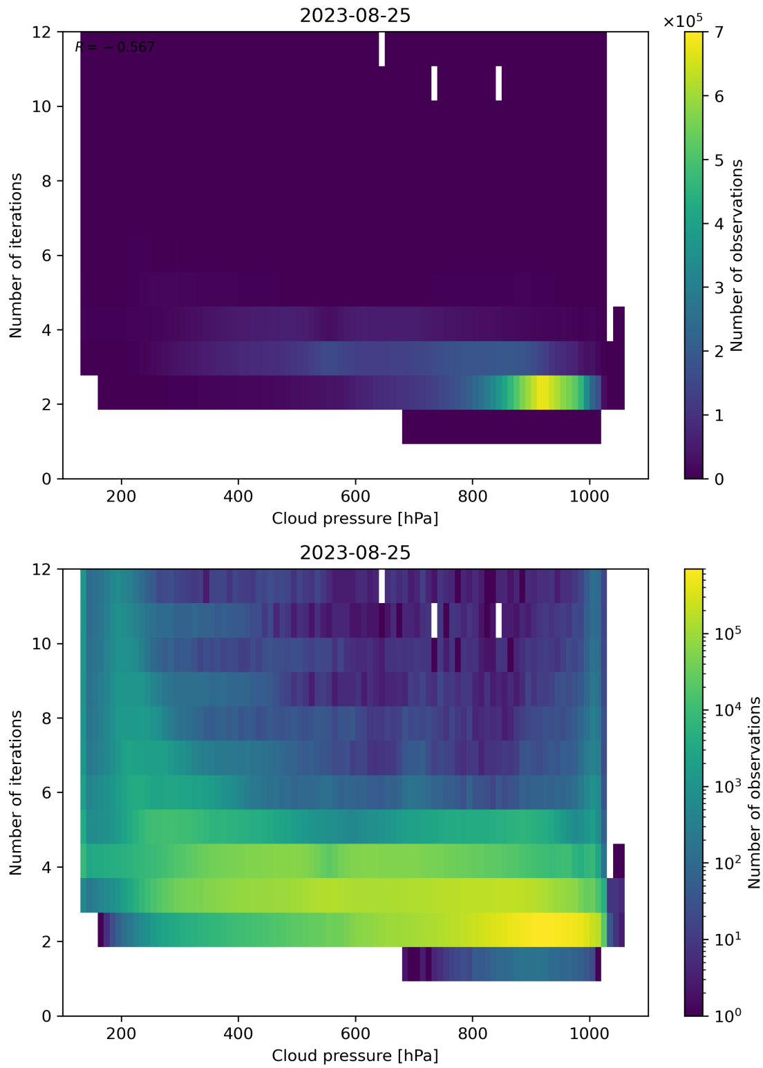
Figure 89: Scatter density plot of “Cloud pressure” against “Number of iterations” for 2023-08-25 to 2023-08-26.
