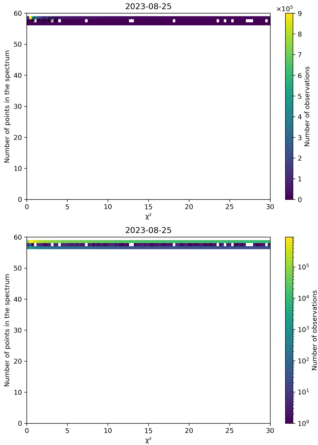
Figure 74: Scatter density plot of “ \chi^2 ” against “Number of points in the spectrum” for 2023-08-25 to 2023-08-26.
