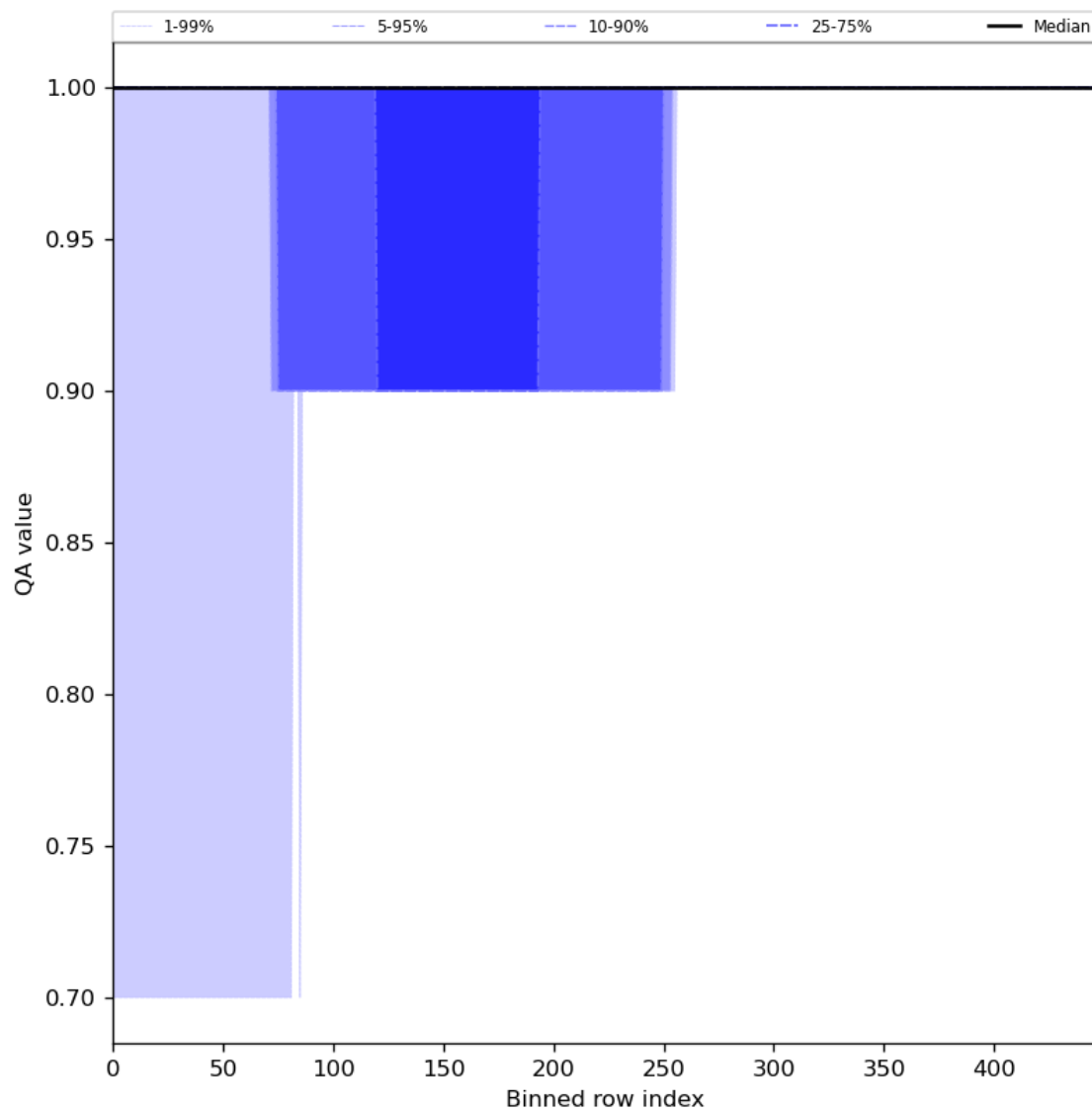
Figure 46: Along track statistics of “QA value” for 2023-08-25 to 2023-08-26
