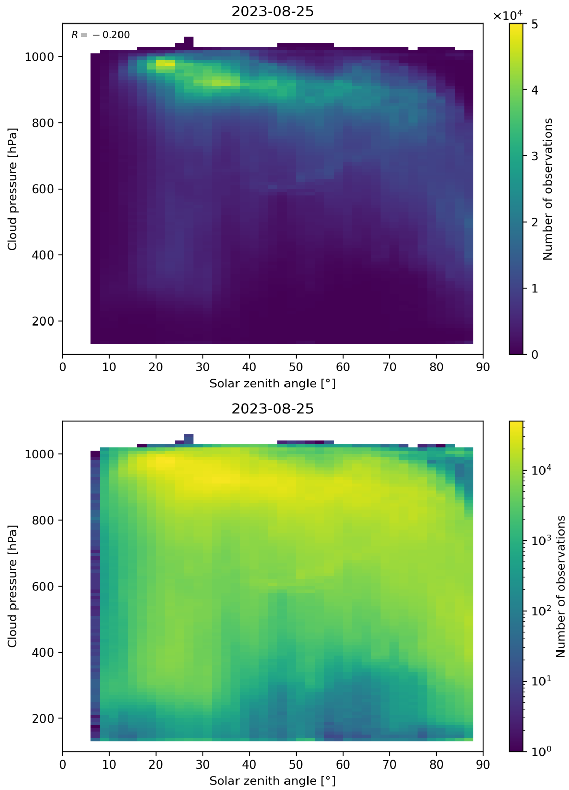
Figure 122: Scatter density plot of “Solar zenith angle” against “Cloud pressure” for 2023-08-25 to 2023-08-26.
