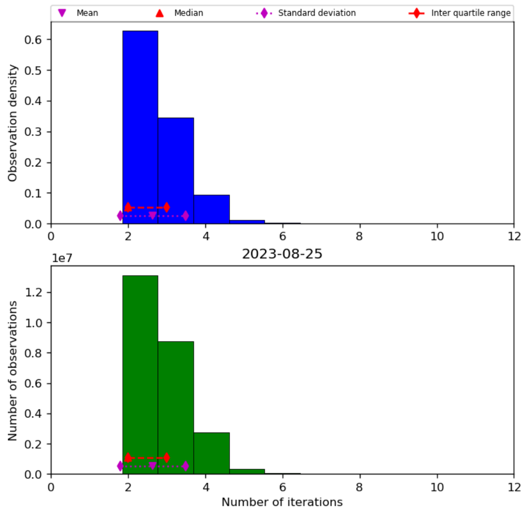
Figure 39: Histogram of “Number of iterations” for 2023-08-25 to 2023-08-26
