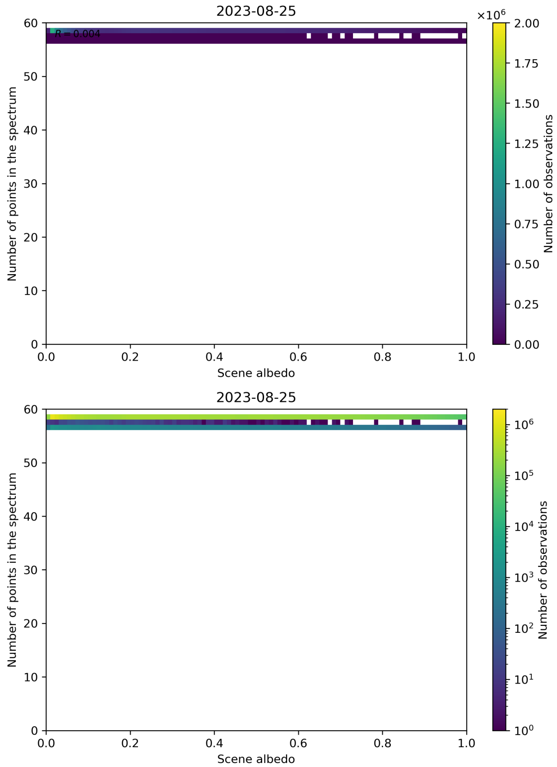
Figure 116: Scatter density plot of “Scene albedo” against “Number of points in the spectrum” for 2023-08-25 to 2023-08-26.
