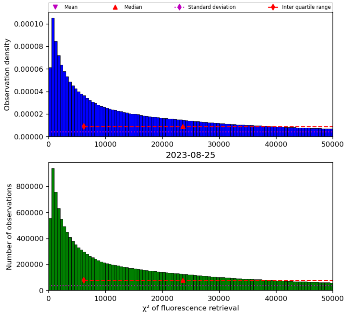
Figure 42: Histogram of “ \chi^2 of fluorescence retrieval” for 2023-08-25 to 2023-08-26
