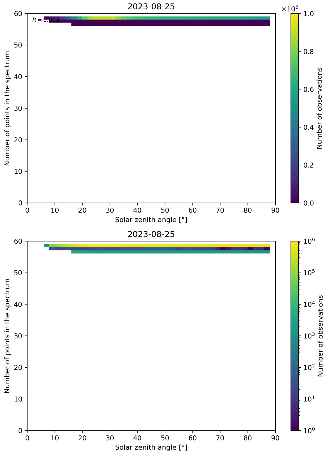
Figure 126: Scatter density plot of “Solar zenith angle” against “Number of points in the spectrum” for 2023-08-25 to 2023-08-26.
