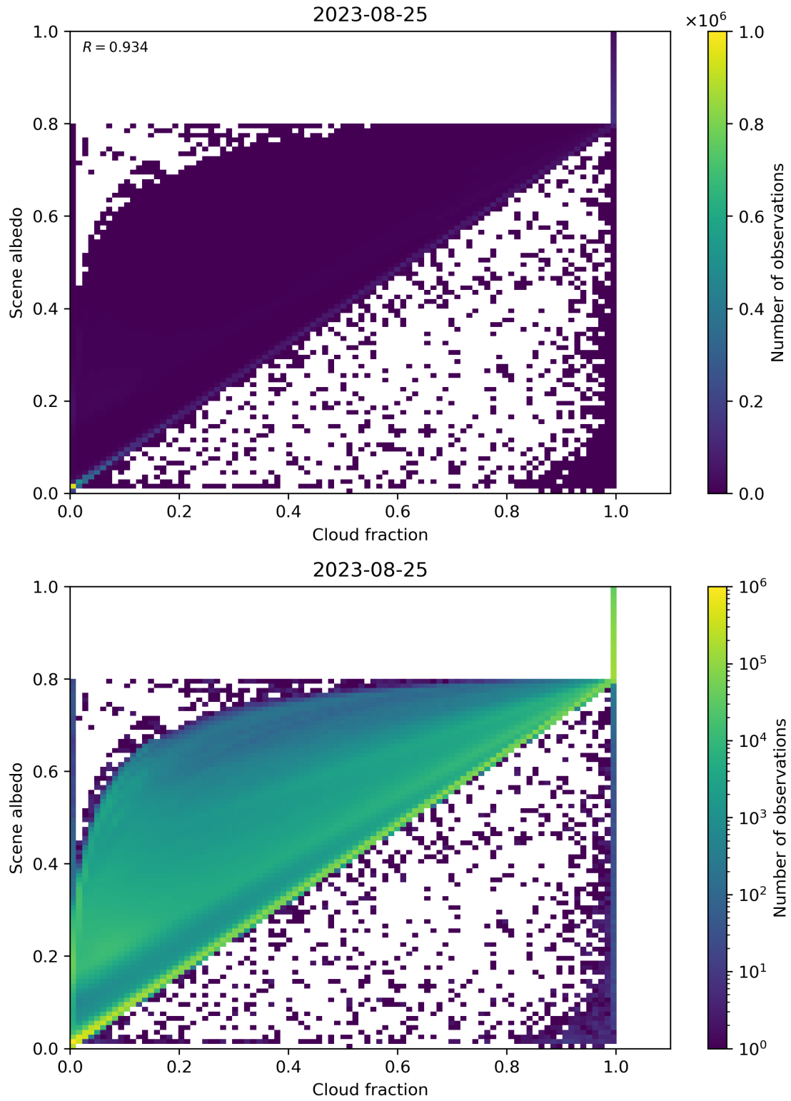
Figure 82: Scatter density plot of “Cloud fraction” against “Scene albedo” for 2023-08-25 to 2023-08-26.
