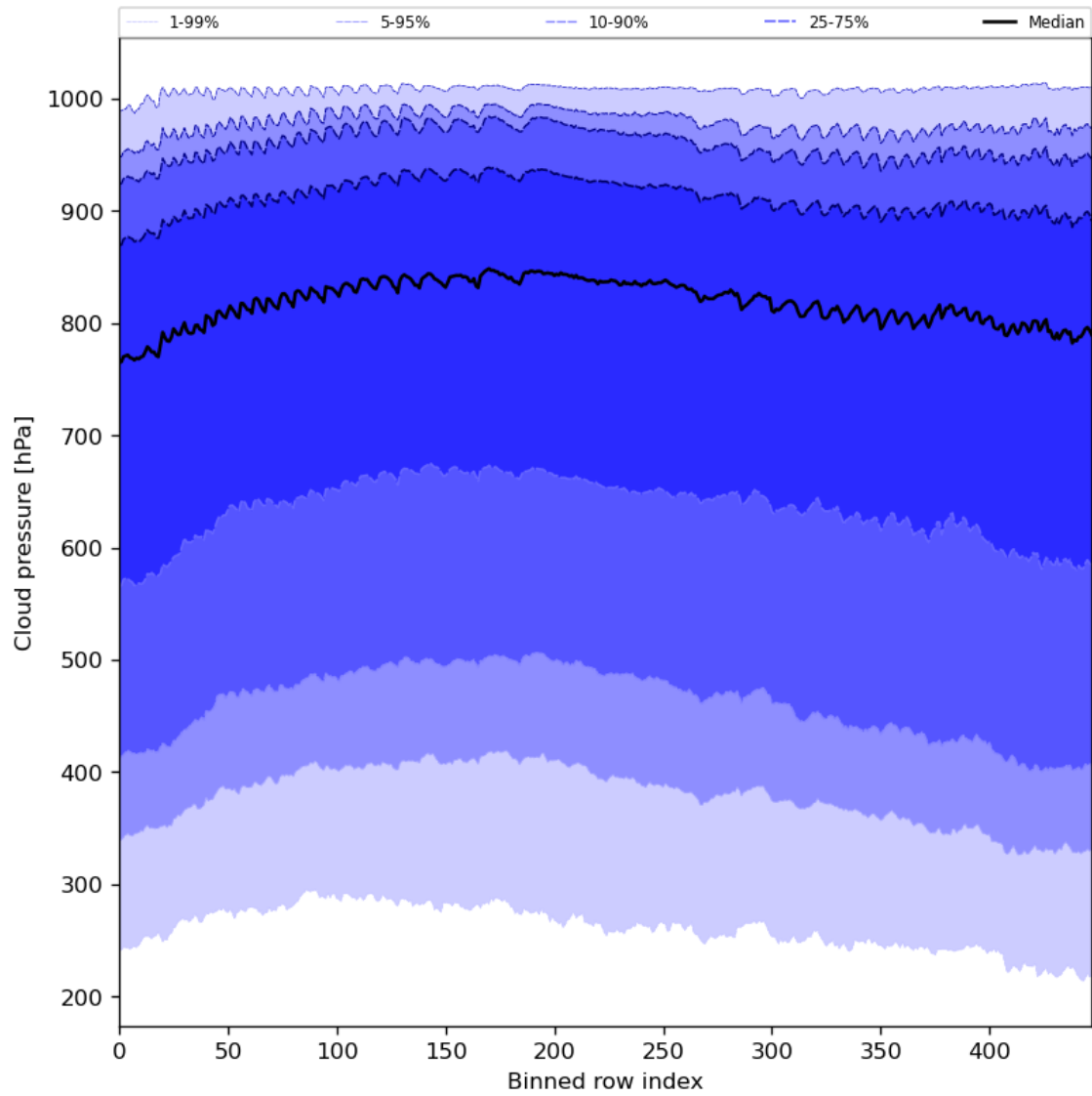
Figure 47: Along track statistics of “Cloud pressure” for 2023-08-25 to 2023-08-26
