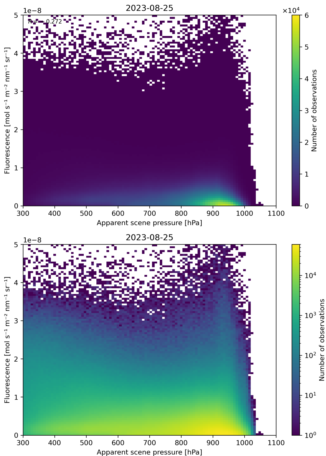
Figure 65: Scatter density plot of “Apparent scene pressure” against “Fluorescence” for 2023-08-25 to 2023-08-26.
