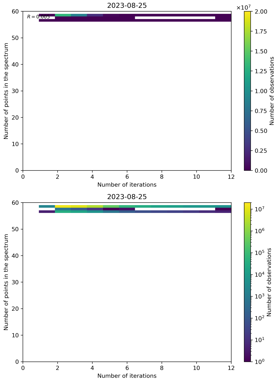
Figure 108: Scatter density plot of “Number of iterations” against “Number of points in the spectrum” for 2023-08-25 to 2023-08-26.
