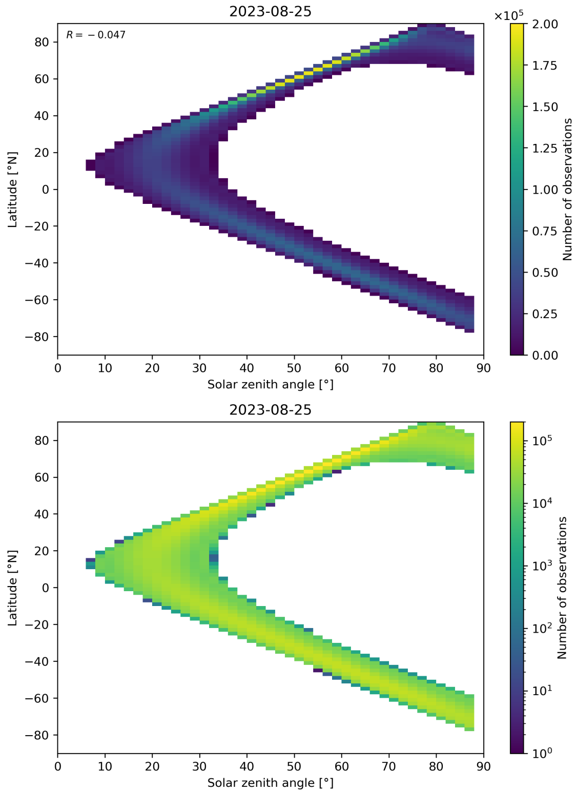
Figure 124: Scatter density plot of “Solar zenith angle” against “Latitude” for 2023-08-25 to 2023-08-26.
