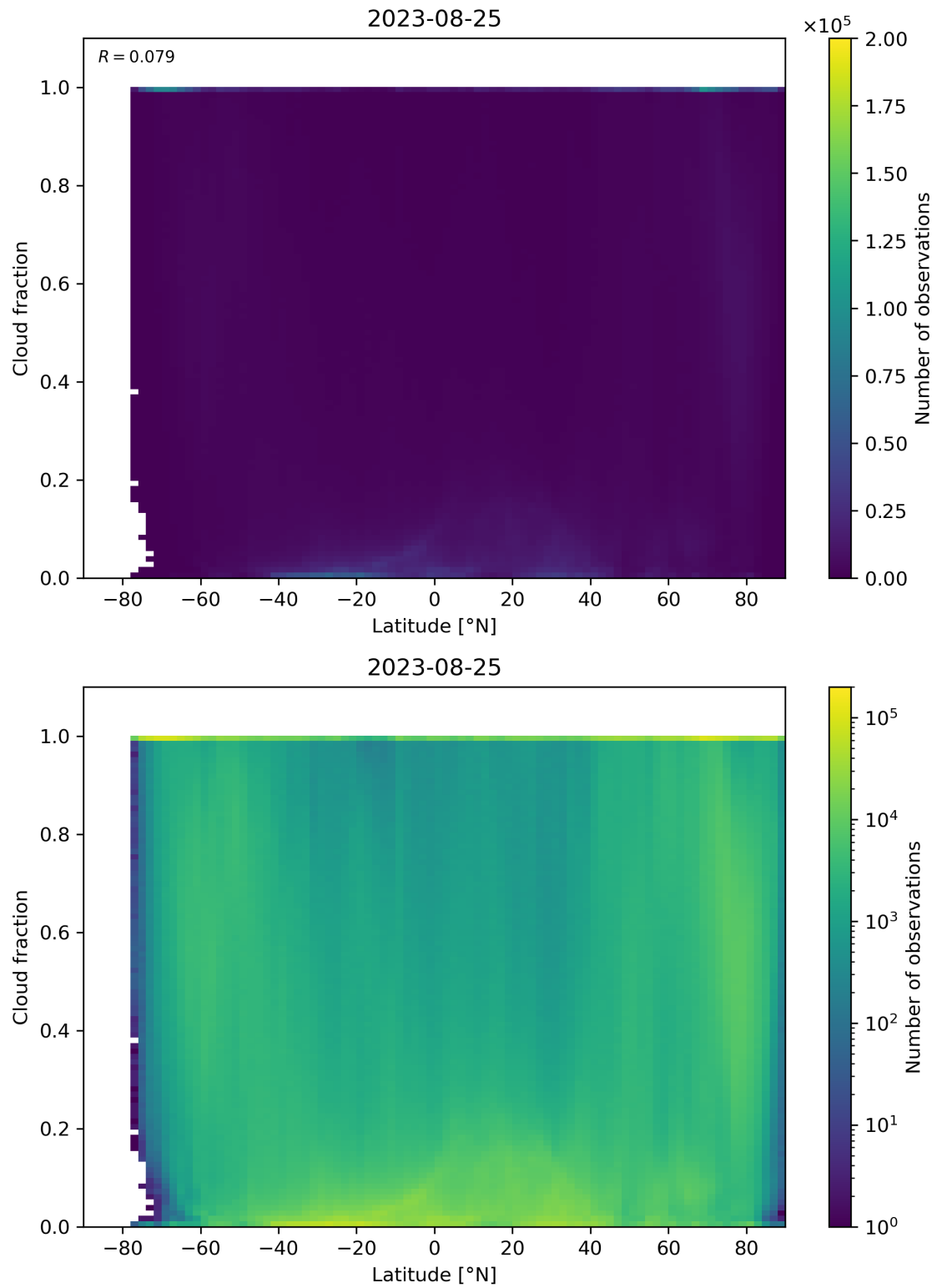
Figure 99: Scatter density plot of “Latitude” against “Cloud fraction” for 2023-08-25 to 2023-08-26.
