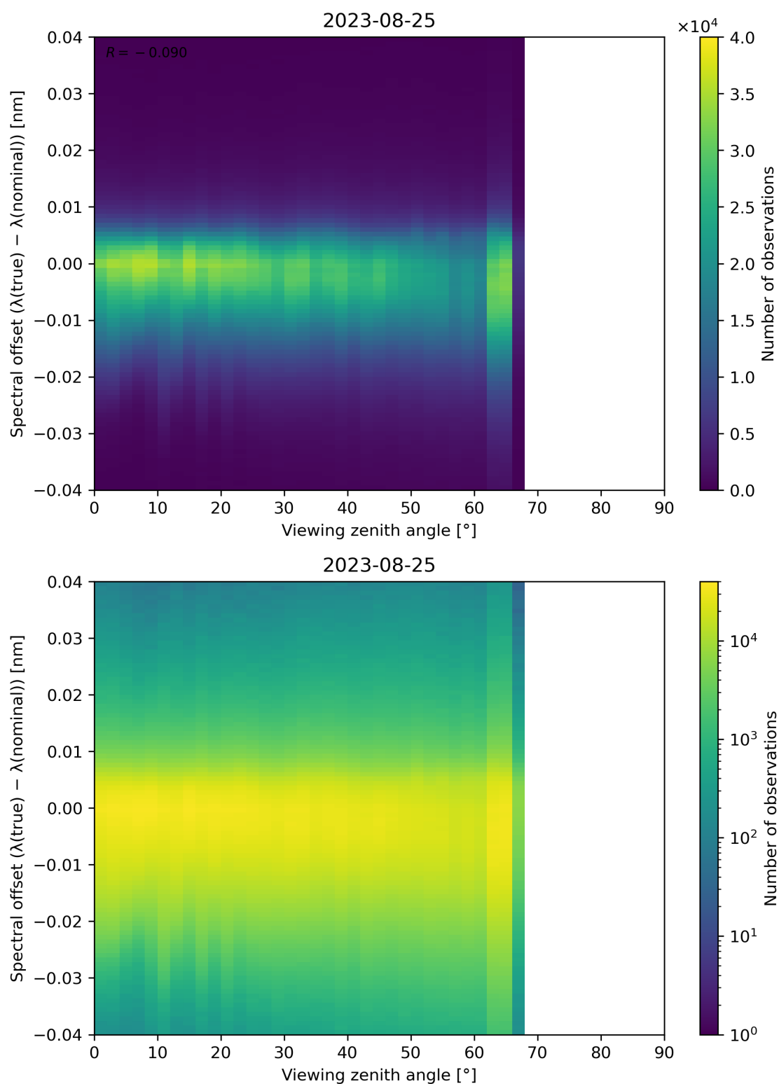
Figure 140: Scatter density plot of “Viewing zenith angle” against “Spectral offset ( \lambda(\text{true}) - \lambda(\text{nominal}) )” for 2023-08-25 to 2023-08-26.
