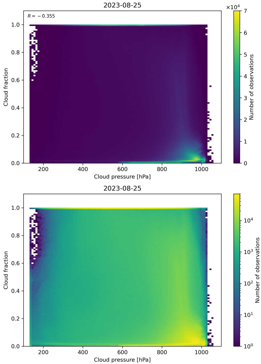
Figure 87: Scatter density plot of “Cloud pressure” against “Cloud fraction” for 2023-08-25 to 2023-08-26.
