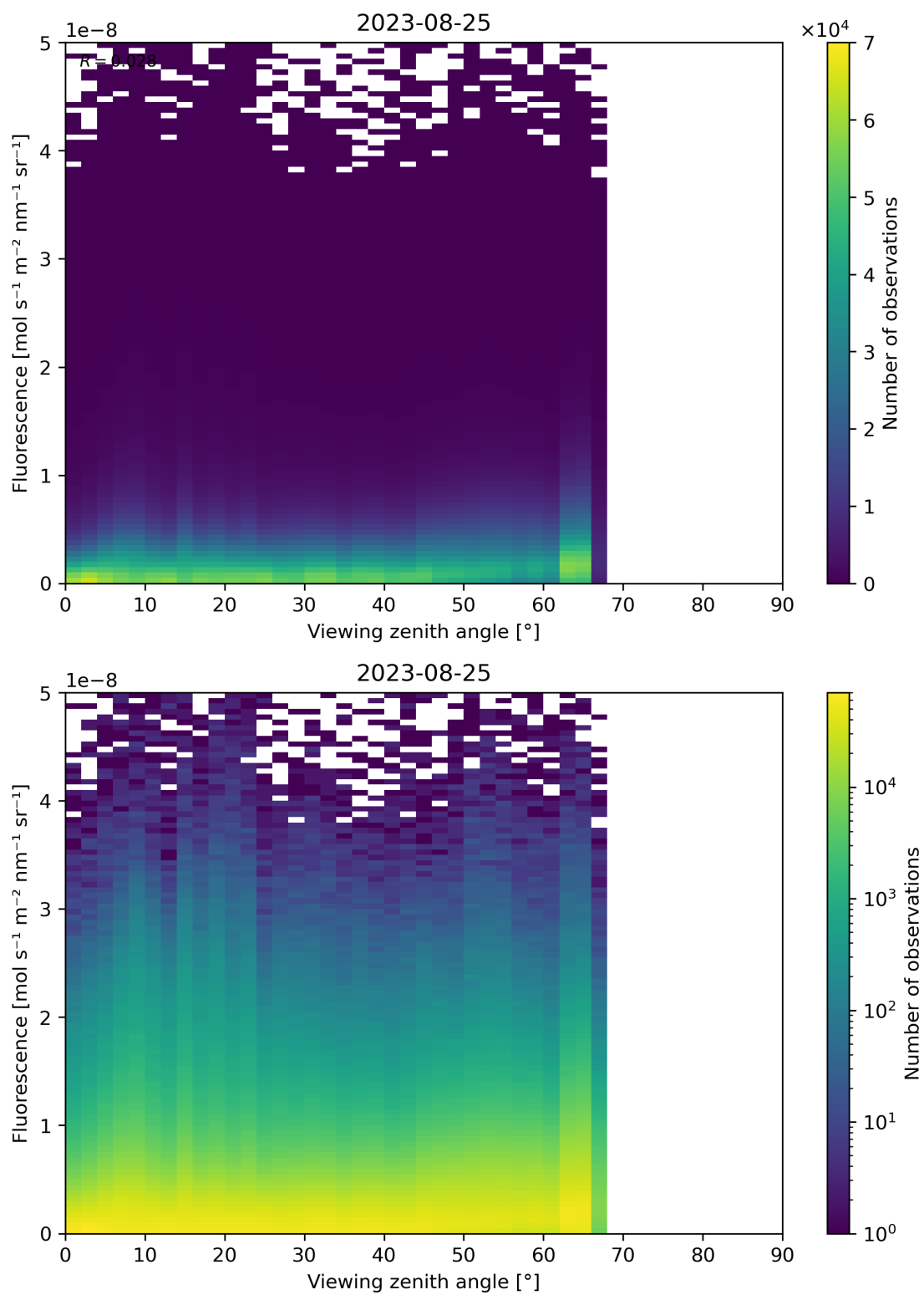
Figure 134: Scatter density plot of “Viewing zenith angle” against “Fluorescence” for 2023-08-25 to 2023-08-26.
