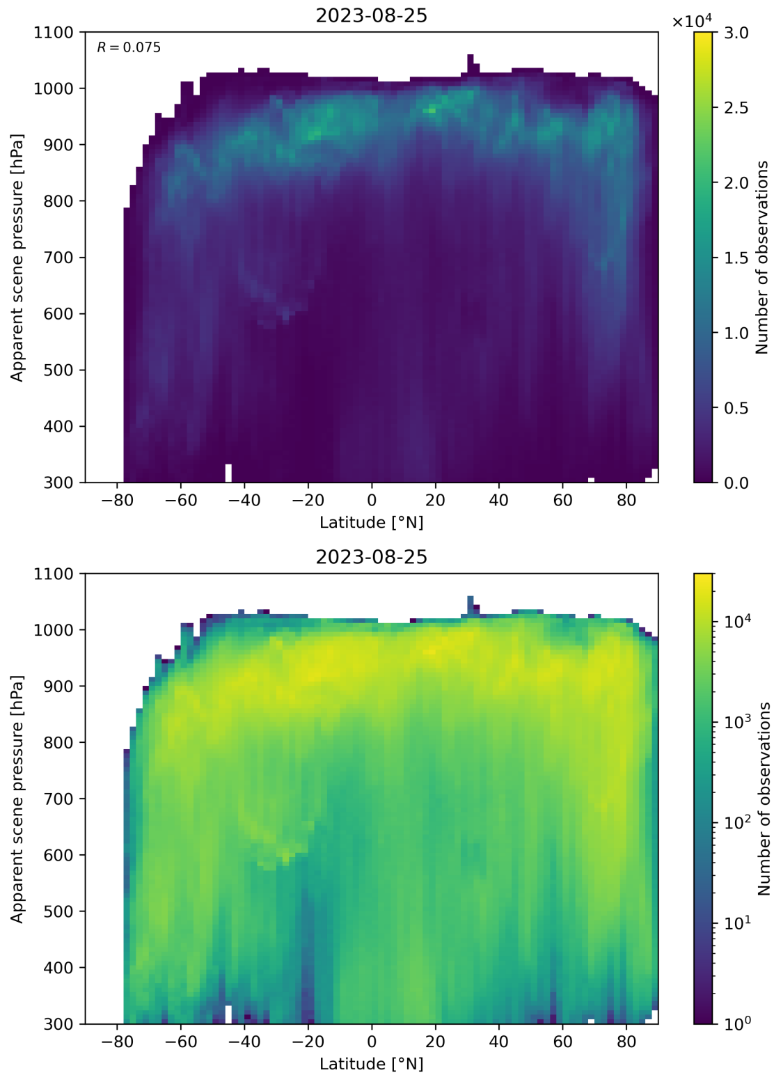
Figure 96: Scatter density plot of “Latitude” against “Apparent scene pressure” for 2023-08-25 to 2023-08-26.
