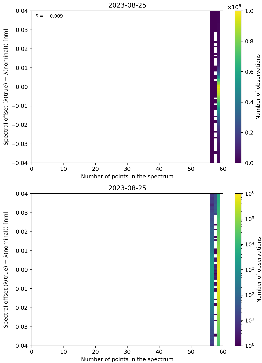
Figure 110: Scatter density plot of “Number of points in the spectrum” against “Spectral offset ( \lambda(\text{true}) - \lambda(\text{nominal}) )” for 2023-08-25 to 2023-08-26.
