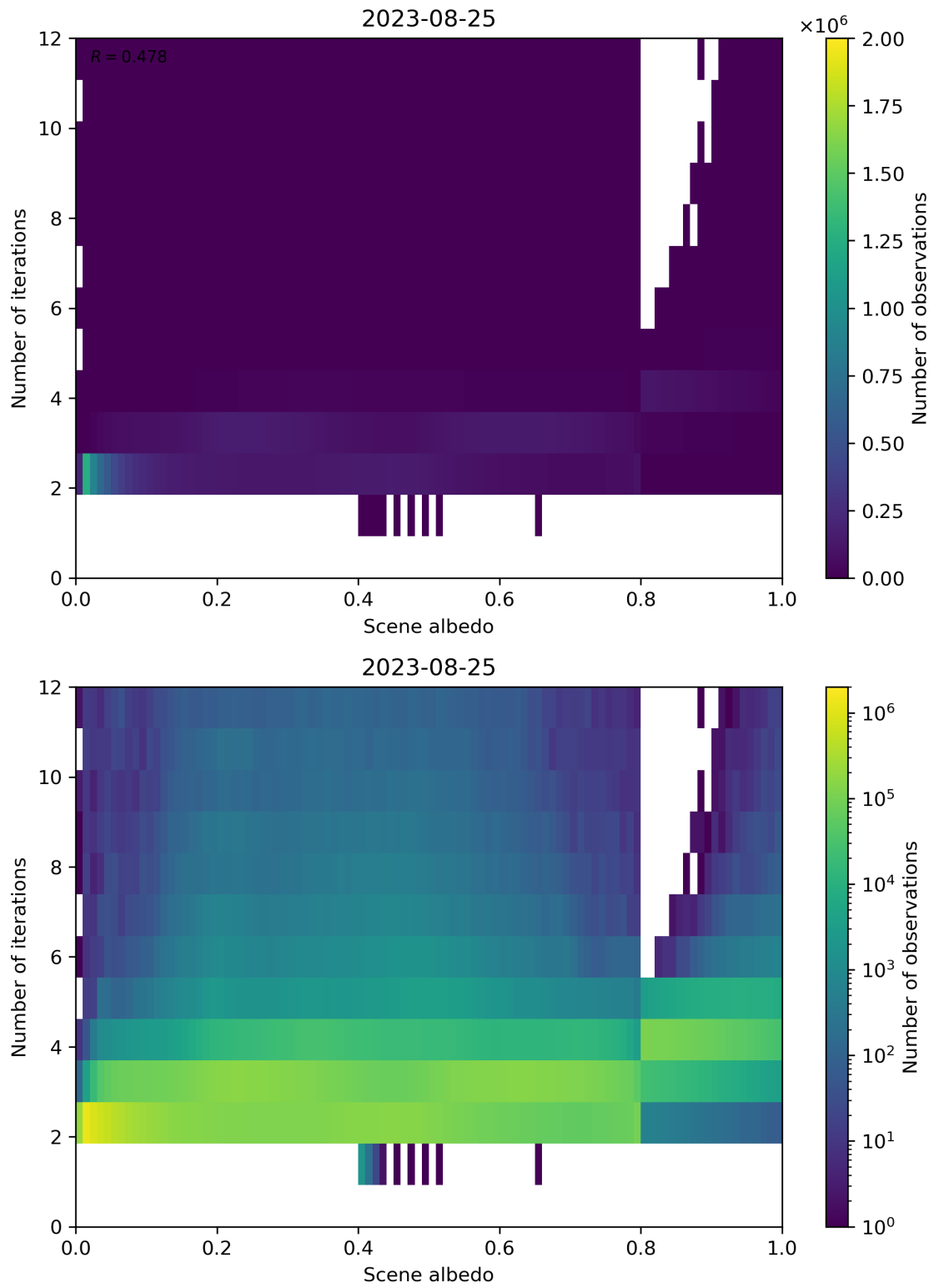
Figure 115: Scatter density plot of “Scene albedo” against “Number of iterations” for 2023-08-25 to 2023-08-26.
