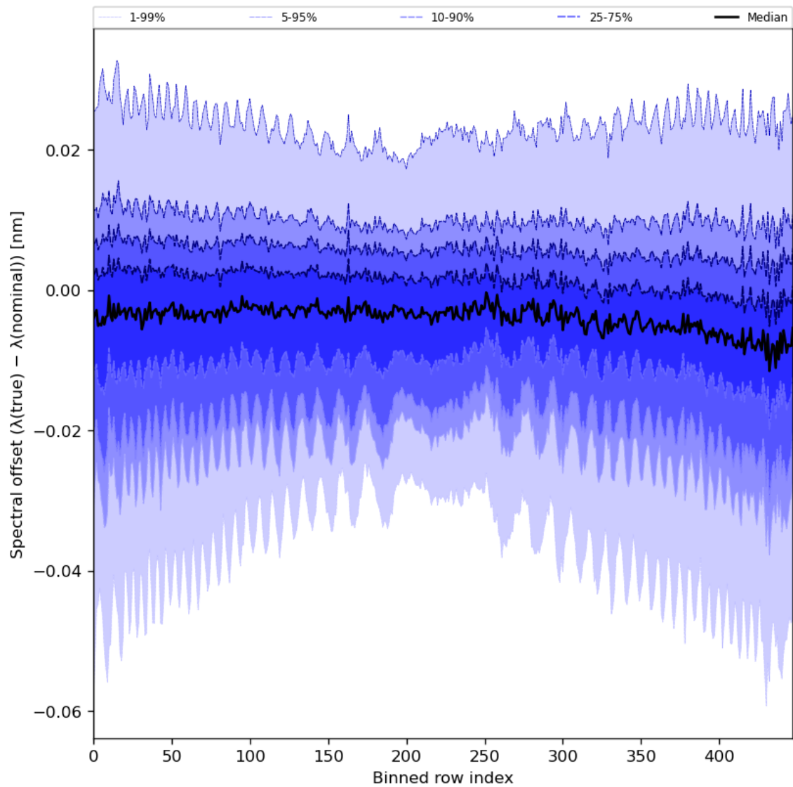
Figure 62: Along track statistics of “Spectral offset ( \lambda(\text{true}) - \lambda(\text{nominal}) )” for 2023-08-25 to 2023-08-26
