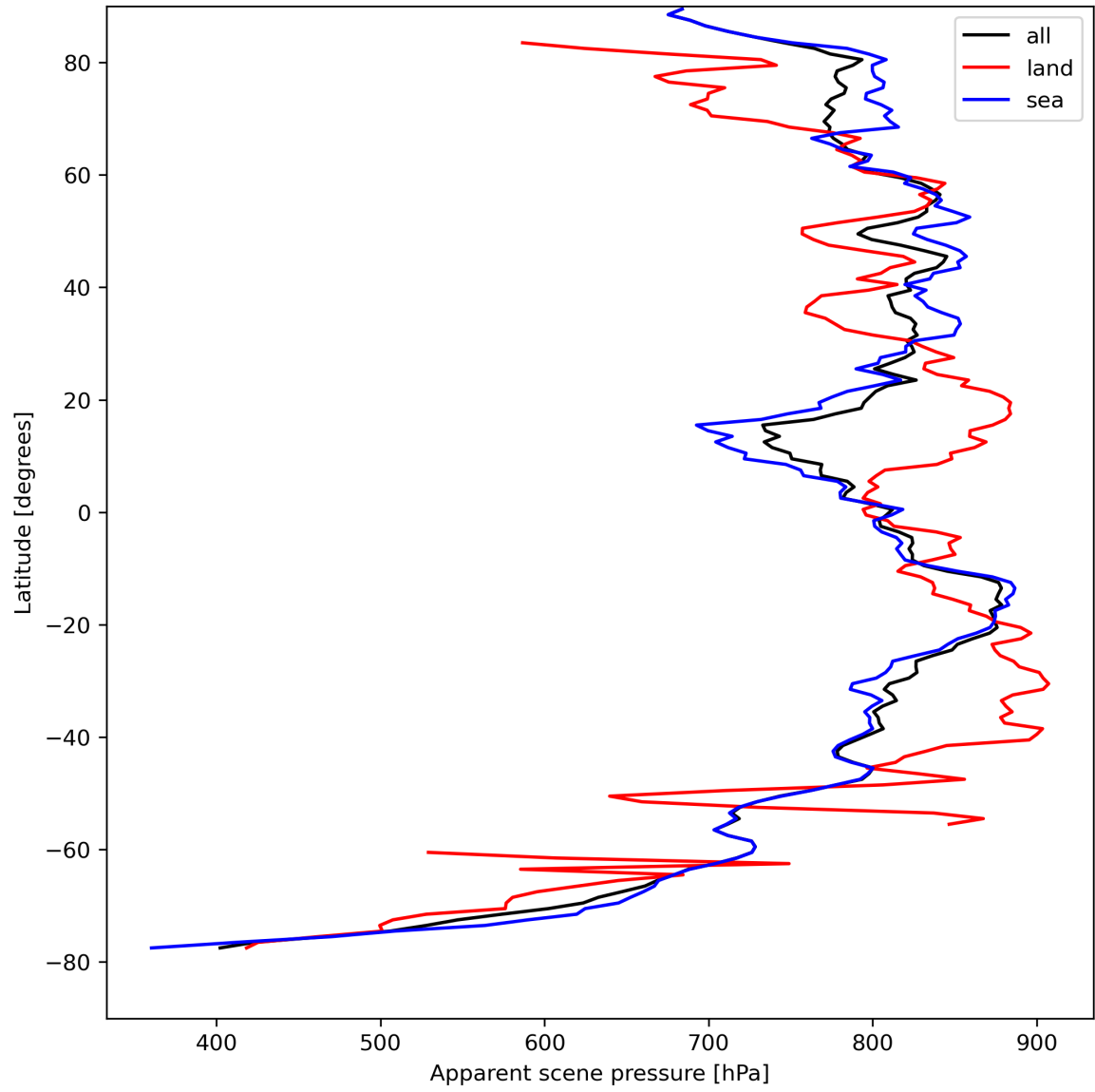
Figure 19: Zonal average of “Apparent scene pressure” for 2023-08-25 to 2023-08-26.
