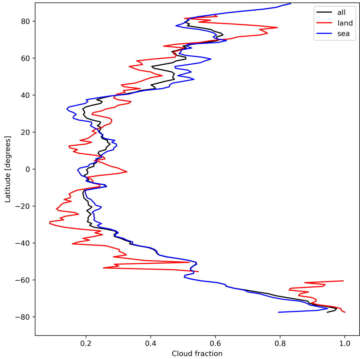
Figure 15: Zonal average of “Cloud fraction” for 2023-08-25 to 2023-08-26.
