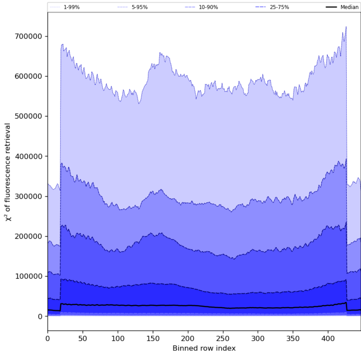
Figure 59: Along track statistics of “ \chi^2 of fluorescence retrieval” for 2023-08-25 to 2023-08-26
