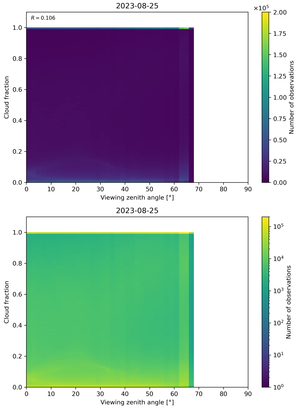
Figure 132: Scatter density plot of “Viewing zenith angle” against “Cloud fraction” for 2023-08-25 to 2023-08-26.
