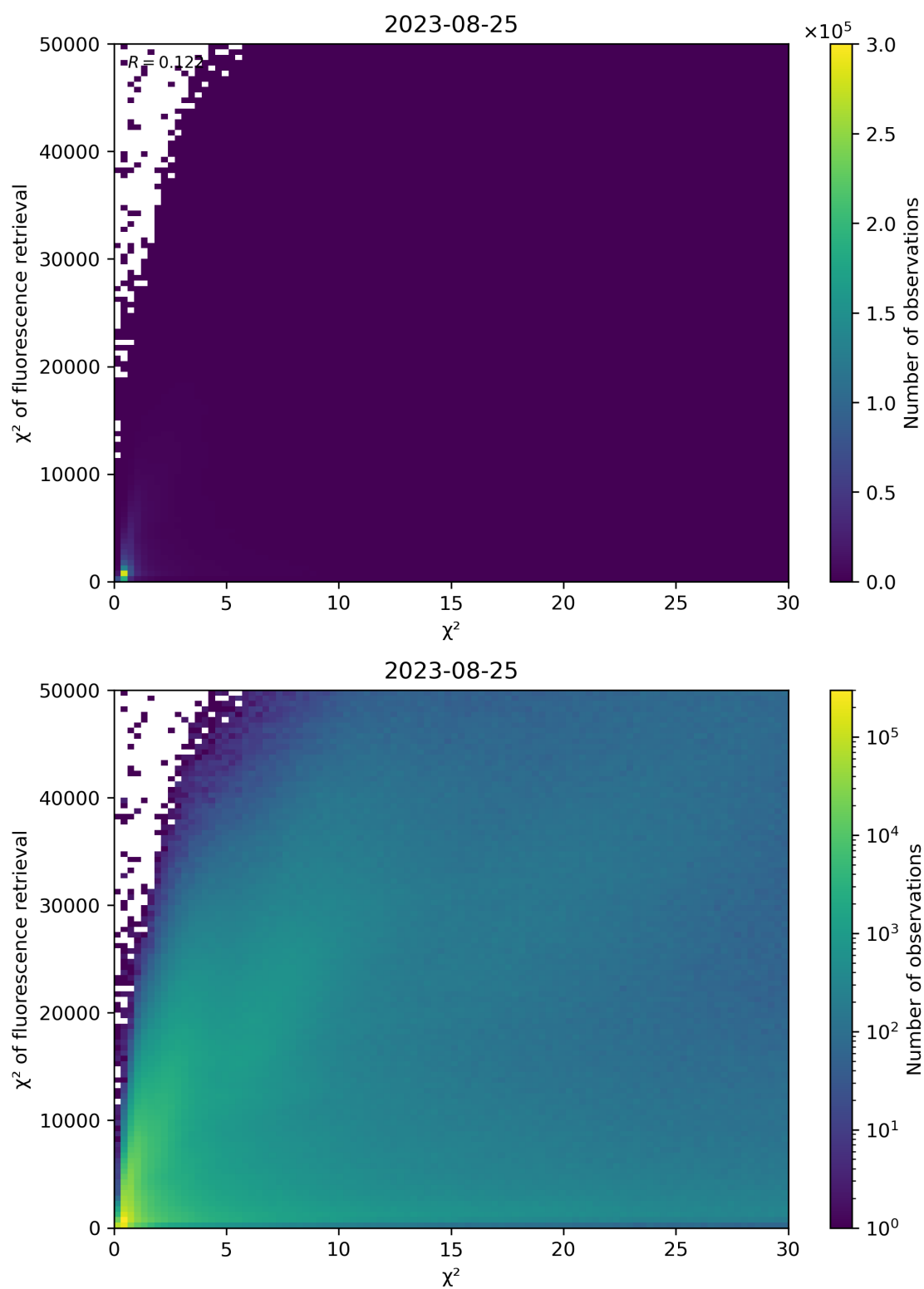
Figure 69: Scatter density plot of “ \chi^2 ” against “ \chi^2 of fluorescence retrieval” for 2023-08-25 to 2023-08-26.
