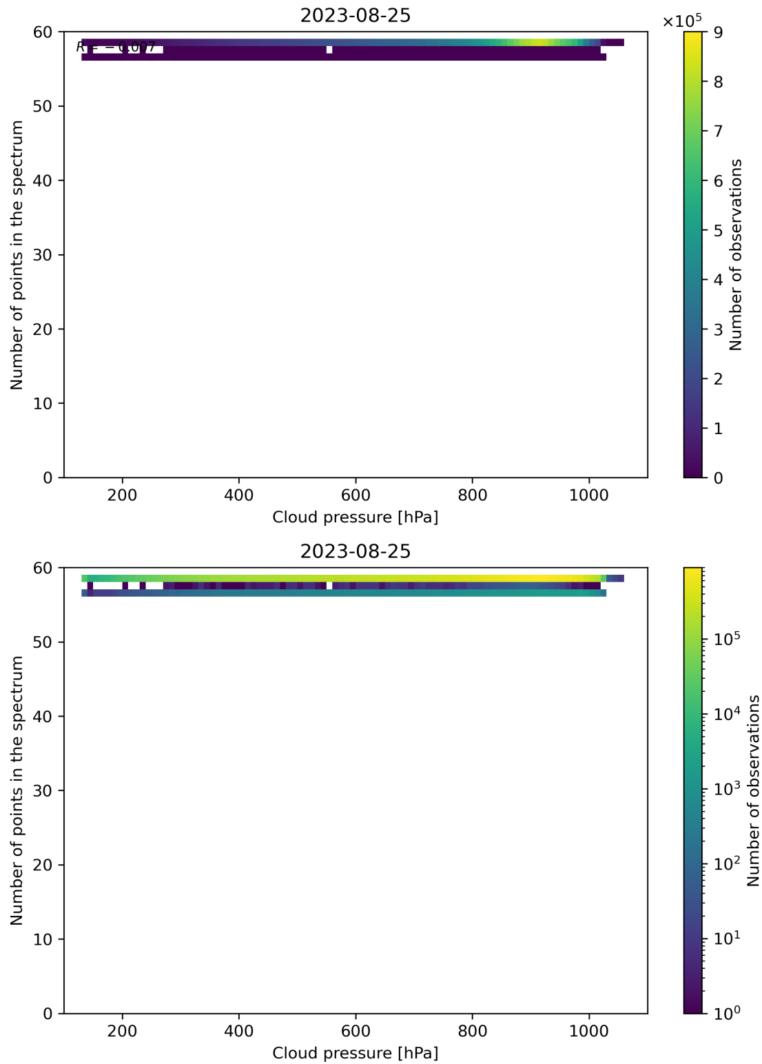
Figure 90: Scatter density plot of “Cloud pressure” against “Number of points in the spectrum” for 2023-08-25 to 2023-08-26.
