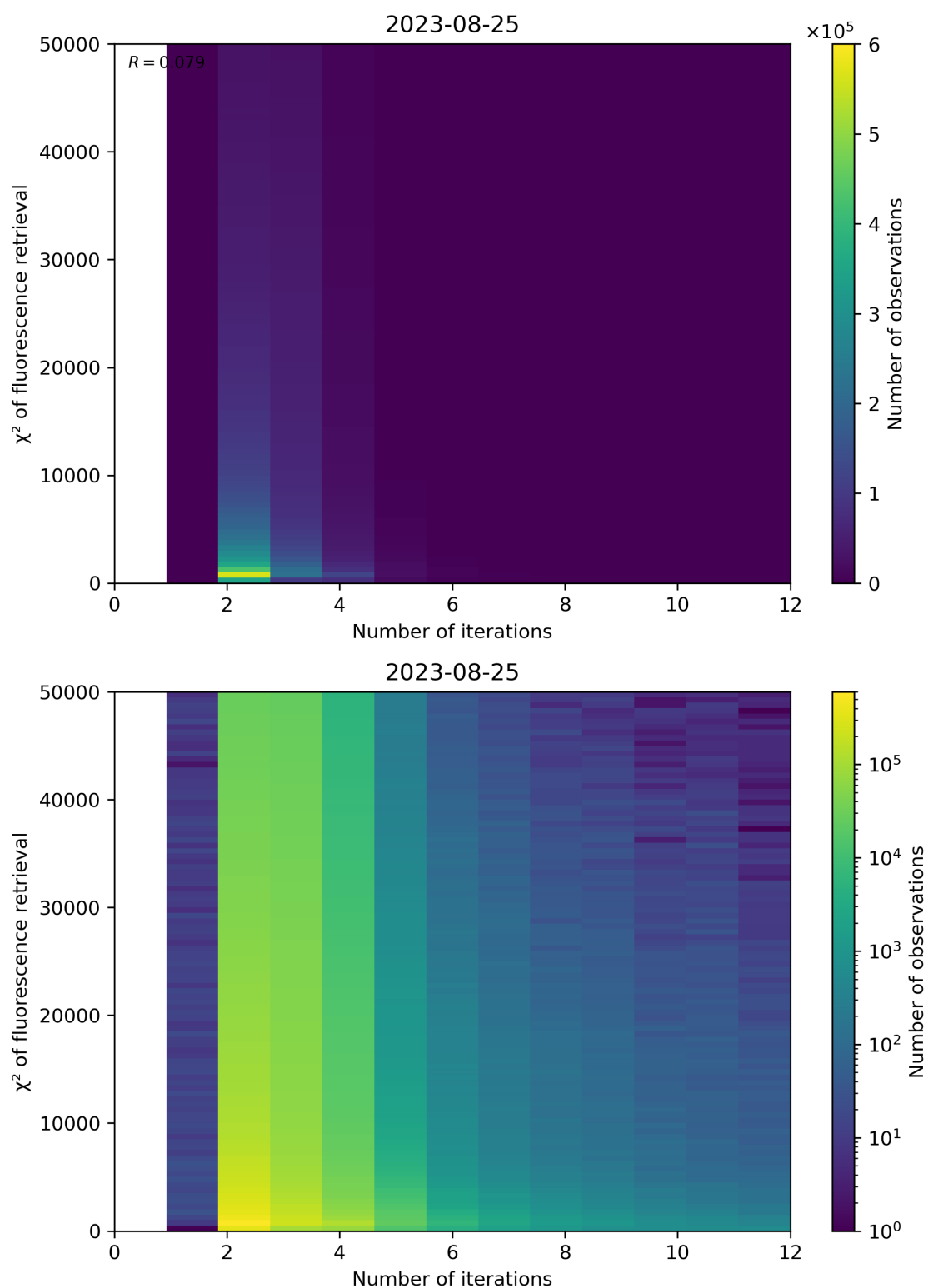
Figure 106: Scatter density plot of “Number of iterations” against “ \chi^2 of fluorescence retrieval” for 2023-08-25 to 2023-08-26.
