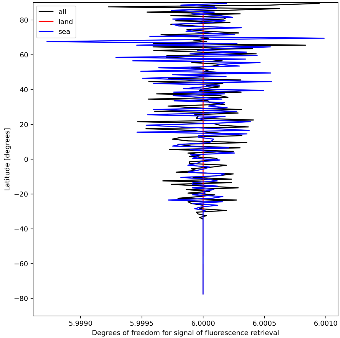
Figure 26: Zonal average of “Degrees of freedom for signal of fluorescence retrieval” for 2023-08-25 to 2023-08-26.
