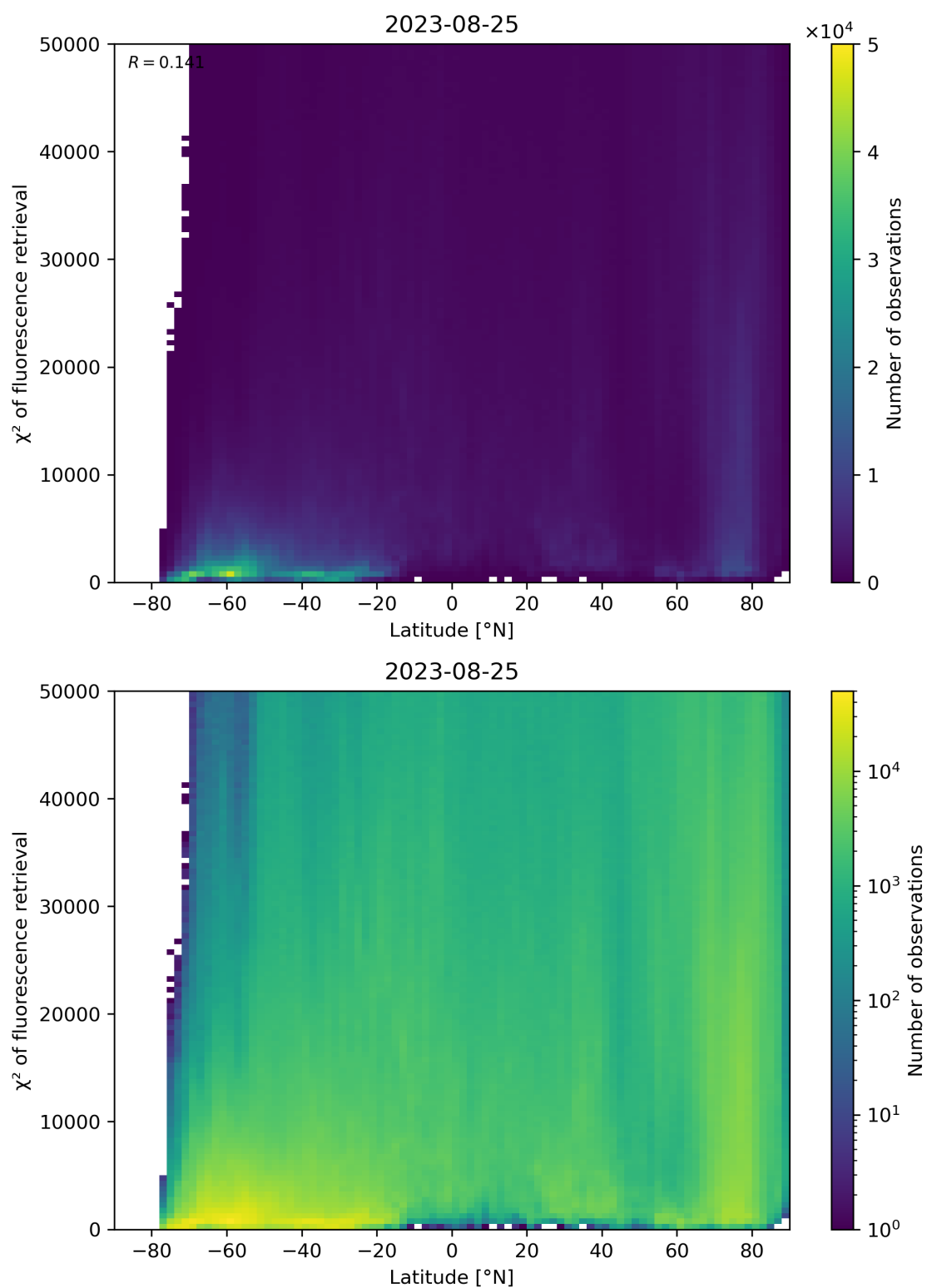
Figure 98: Scatter density plot of “Latitude” against “ \chi^2 of fluorescence retrieval” for 2023-08-25 to 2023-08-26.
