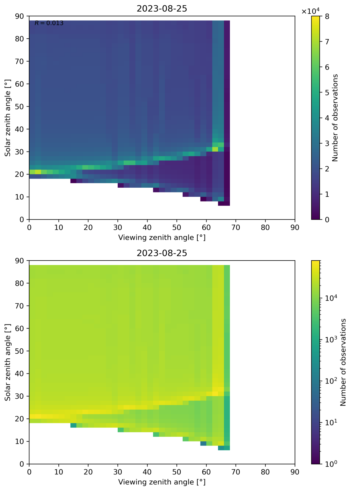
Figure 139: Scatter density plot of “Viewing zenith angle” against “Solar zenith angle” for 2023-08-25 to 2023-08-26.
