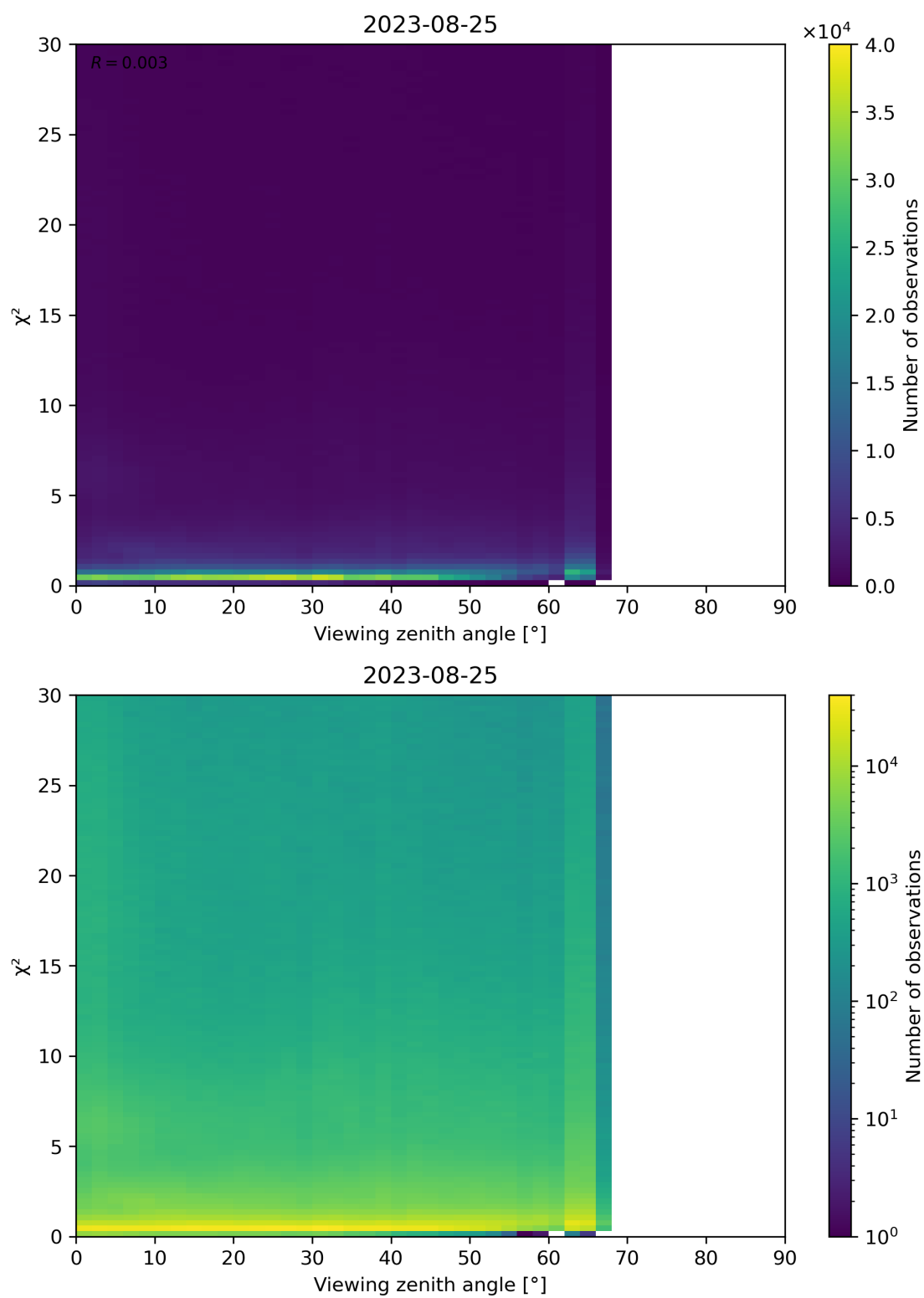
Figure 130: Scatter density plot of “Viewing zenith angle” against “ \chi^2 ” for 2023-08-25 to 2023-08-26.
