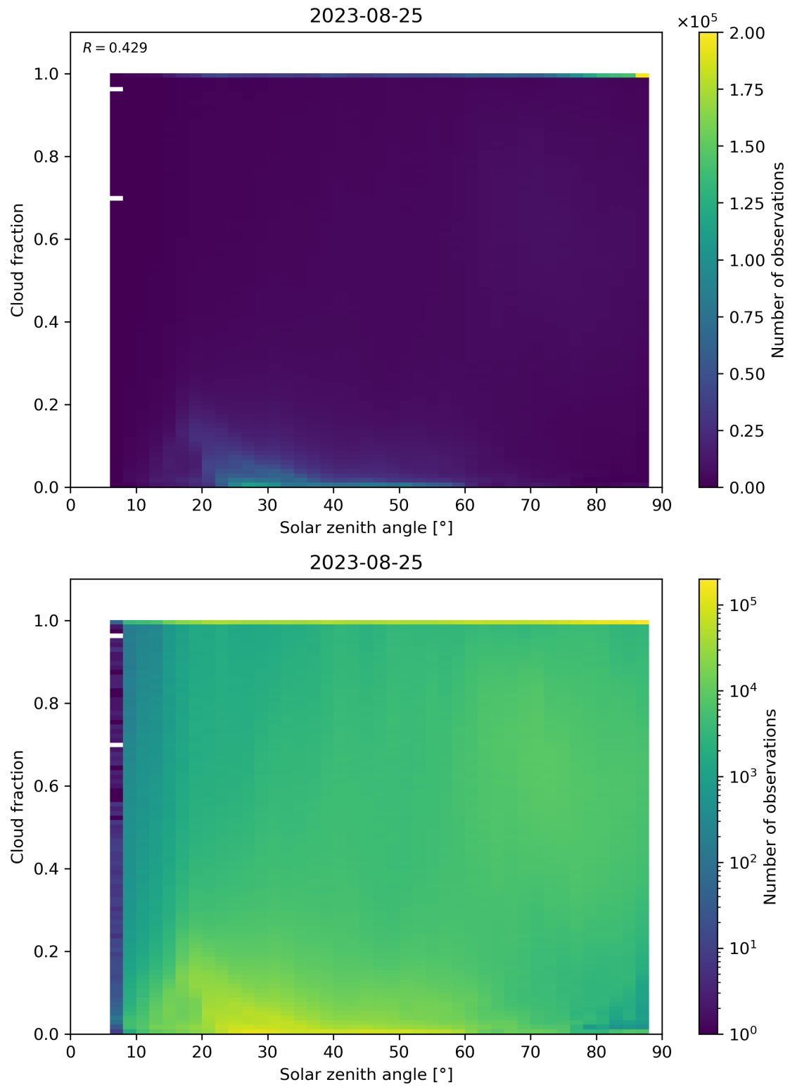
Figure 121: Scatter density plot of “Solar zenith angle” against “Cloud fraction” for 2023-08-25 to 2023-08-26.
