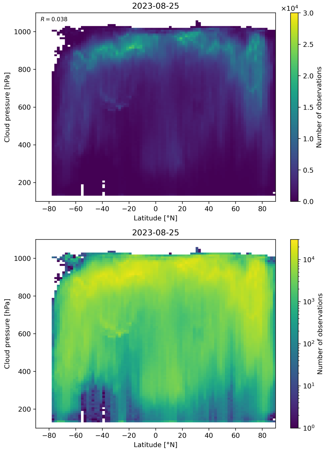
Figure 100: Scatter density plot of “Latitude” against “Cloud pressure” for 2023-08-25 to 2023-08-26.
