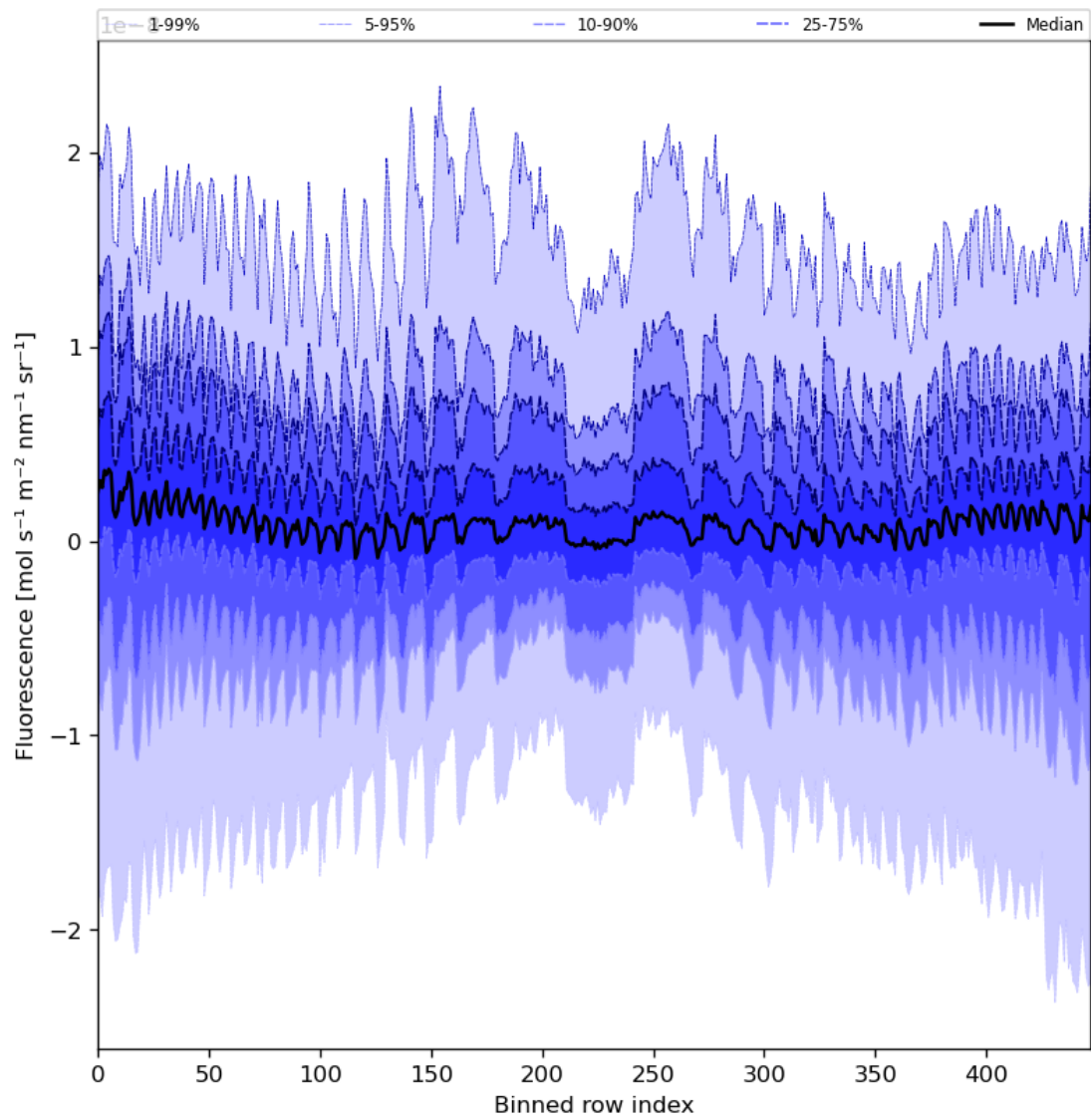
Figure 57: Along track statistics of "Fluorescence" for 2023-08-25 to 2023-08-26
