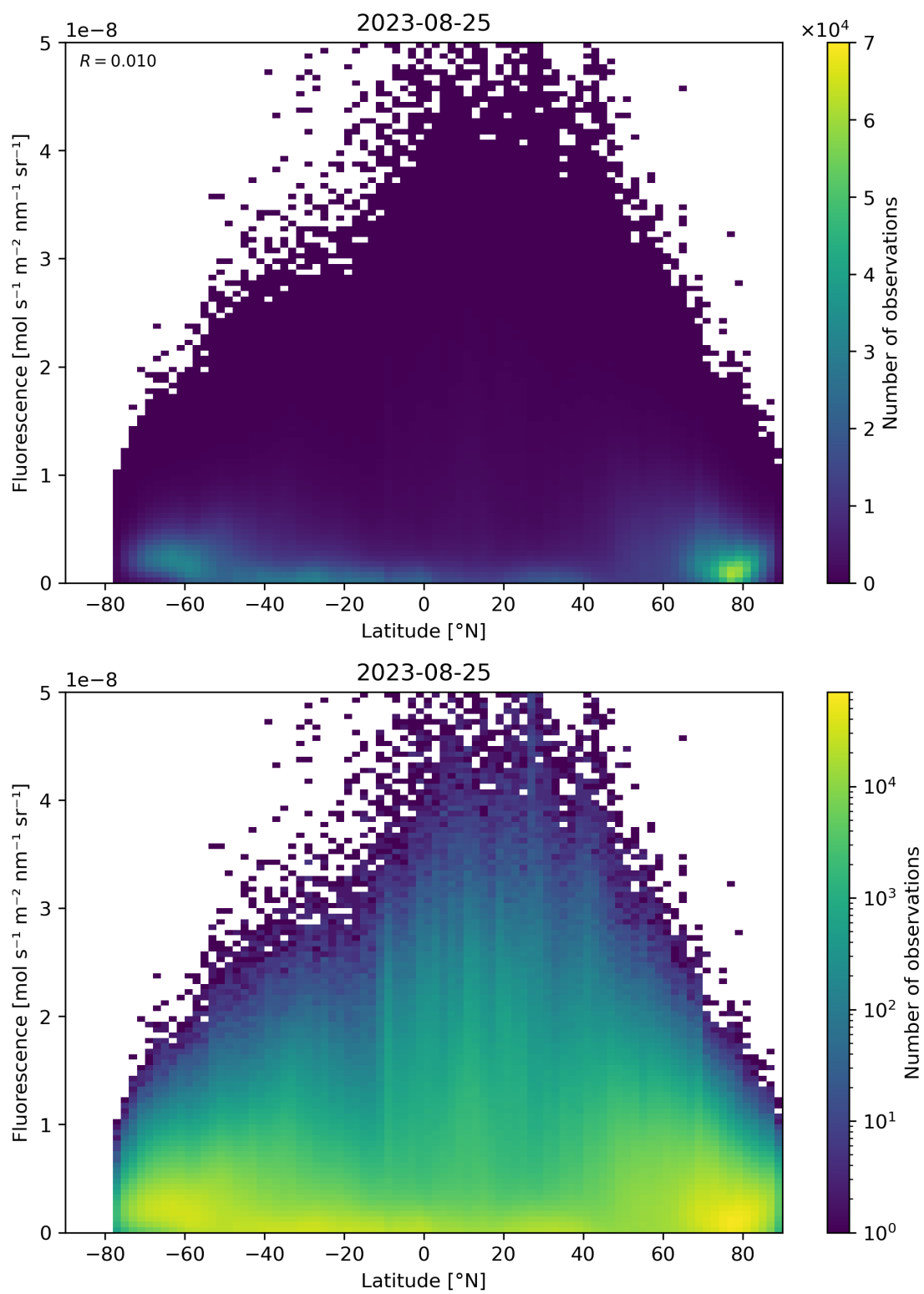
Figure 101: Scatter density plot of “Latitude” against “Fluorescence” for 2023-08-25 to 2023-08-26.
