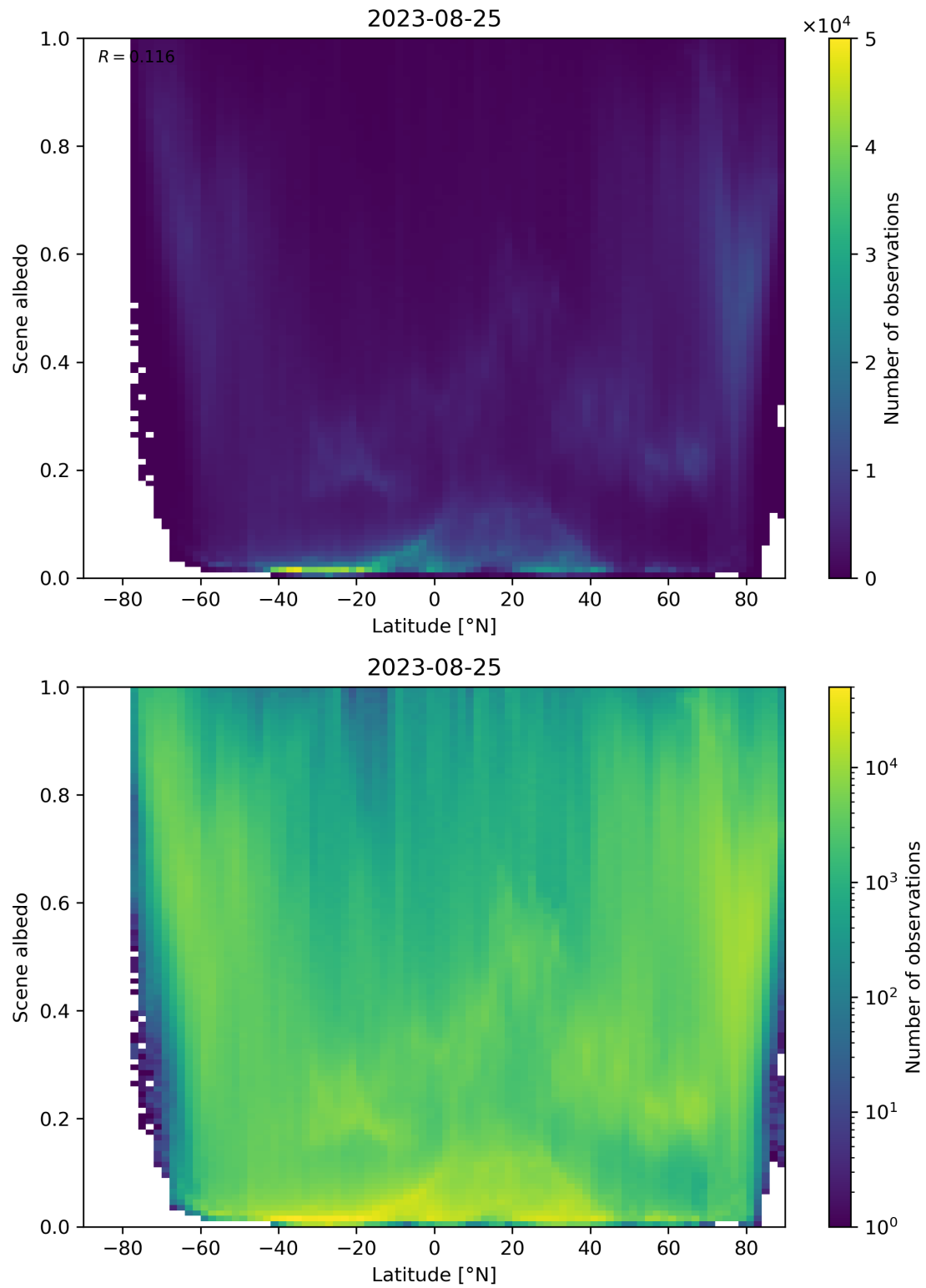
Figure 104: Scatter density plot of “Latitude” against “Scene albedo” for 2023-08-25 to 2023-08-26.
