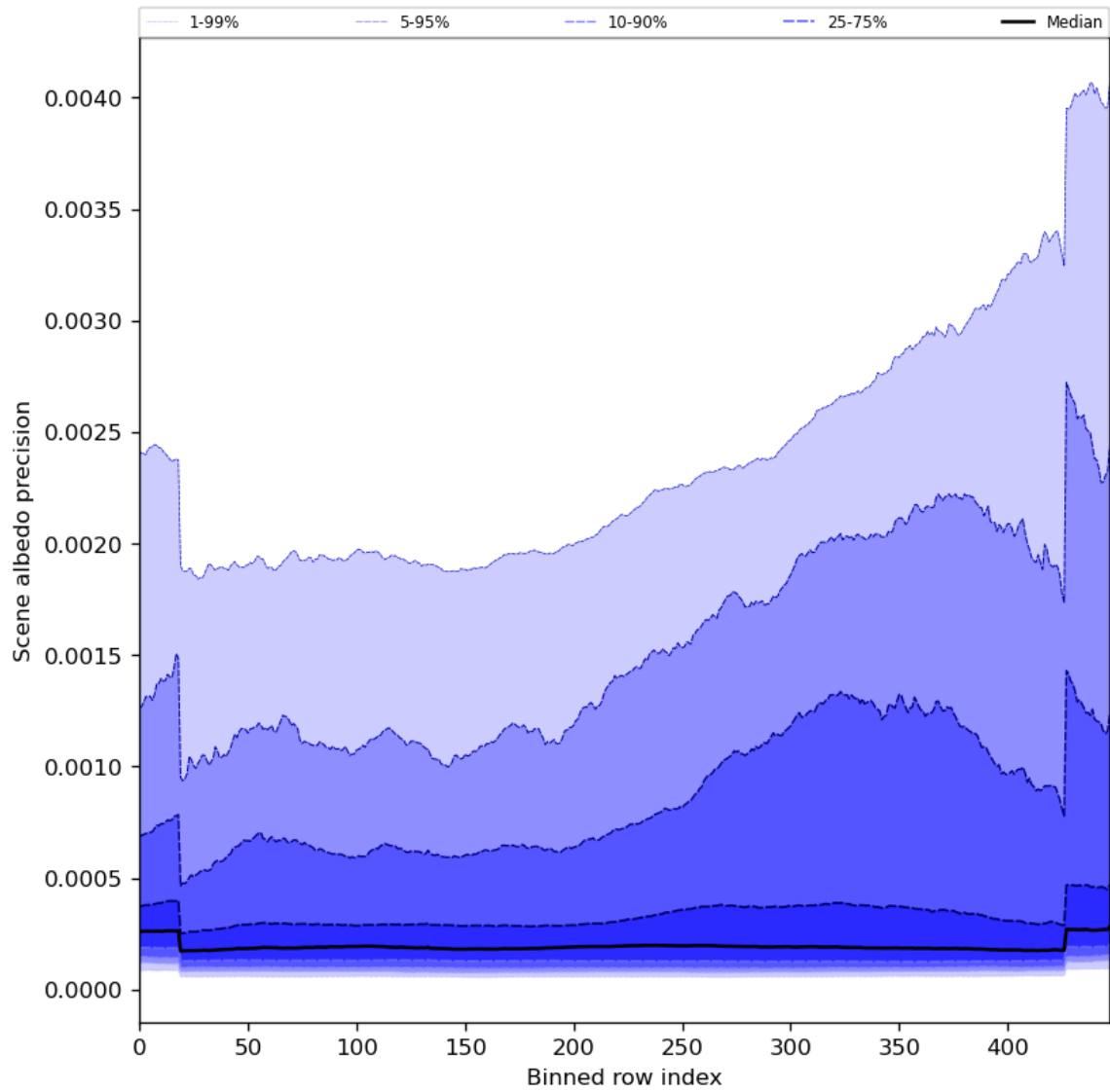
Figure 52: Along track statistics of “Scene albedo precision” for 2023-08-25 to 2023-08-26
