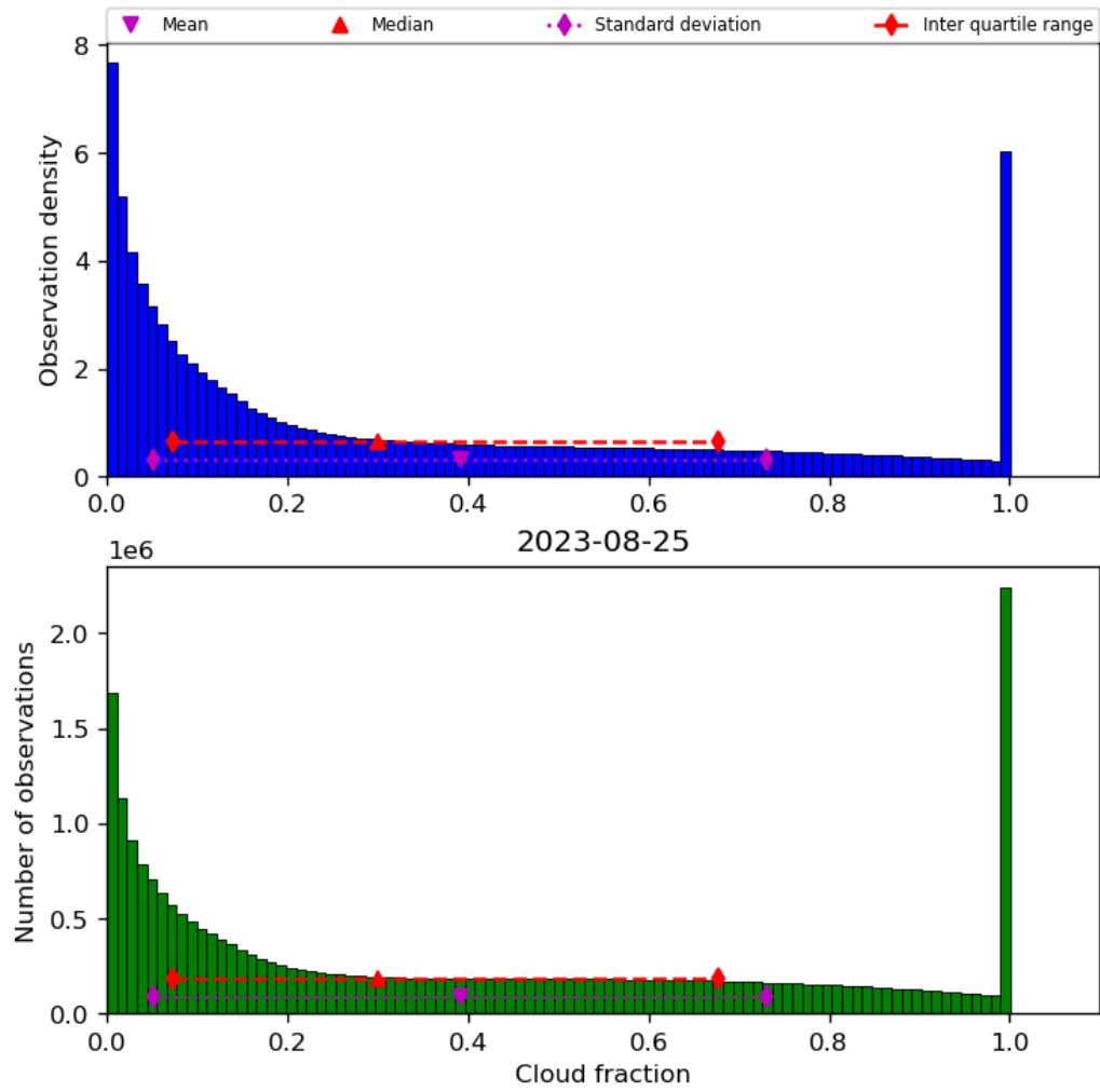
Figure 32: Histogram of “Cloud fraction” for 2023-08-25 to 2023-08-26
