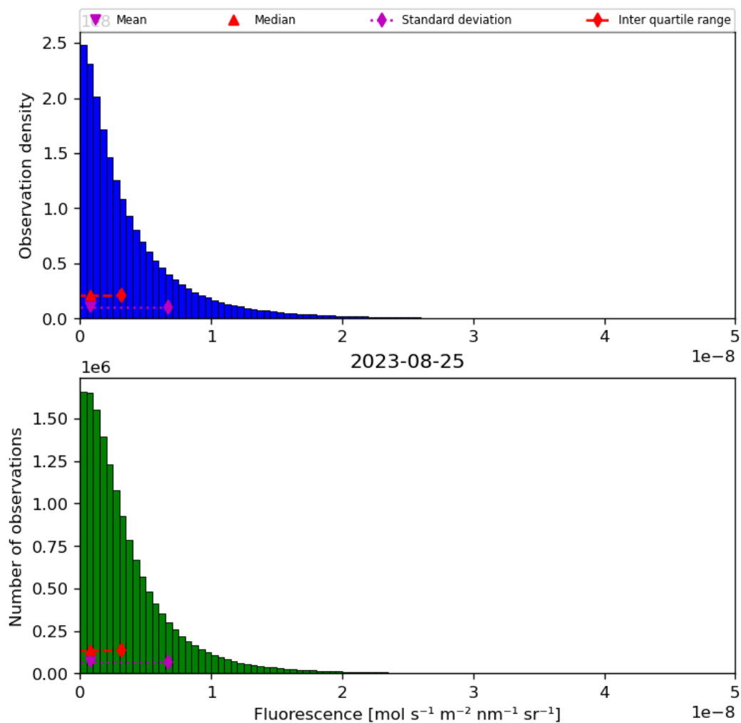
Figure 40: Histogram of “Fluorescence” for 2023-08-25 to 2023-08-26
