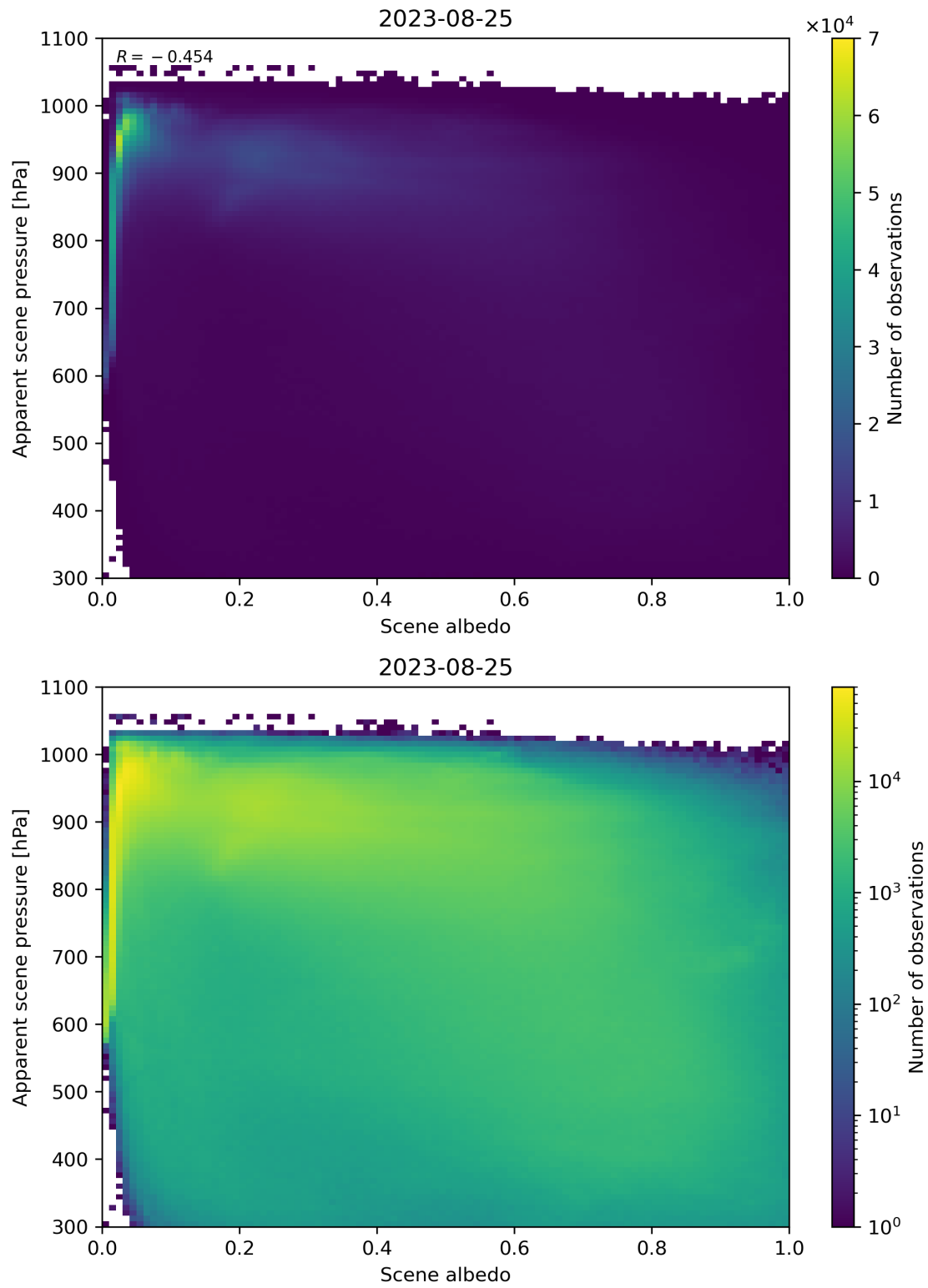
Figure 111: Scatter density plot of “Scene albedo” against “Apparent scene pressure” for 2023-08-25 to 2023-08-26.
