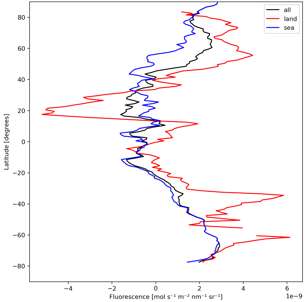
Figure 23: Zonal average of “Fluorescence” for 2023-08-25 to 2023-08-26.
