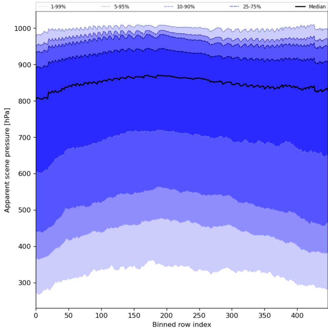
Figure 53: Along track statistics of “Apparent scene pressure” for 2023-08-25 to 2023-08-26
