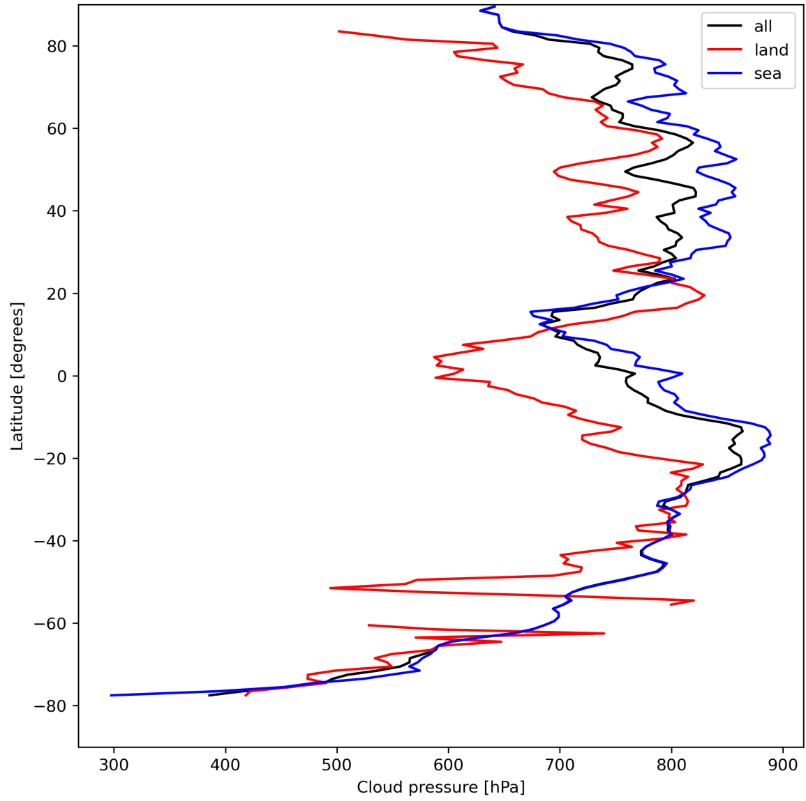
Figure 13: Zonal average of “Cloud pressure” for 2023-08-25 to 2023-08-26.
