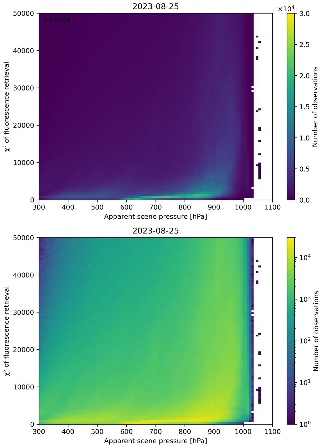
Figure 64: Scatter density plot of “Apparent scene pressure” against “ \chi^2 of fluorescence retrieval” for 2023-08-25 to 2023-08-26.
