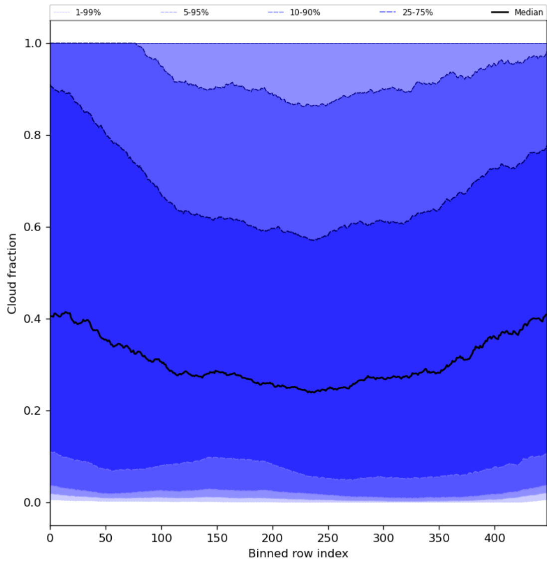
Figure 49: Along track statistics of “Cloud fraction” for 2023-08-25 to 2023-08-26
