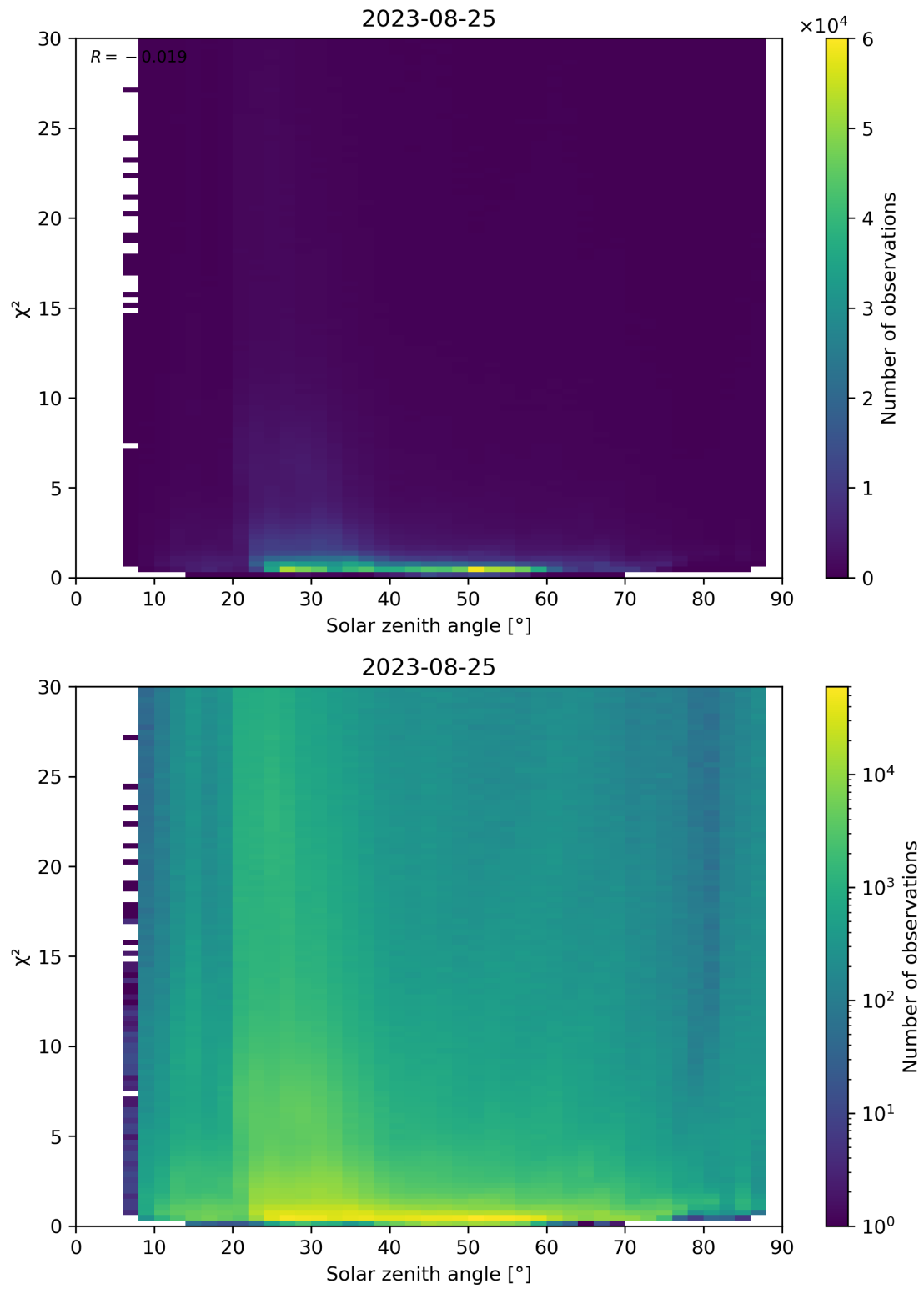
Figure 119: Scatter density plot of “Solar zenith angle” against “ \chi^2 ” for 2023-08-25 to 2023-08-26.
