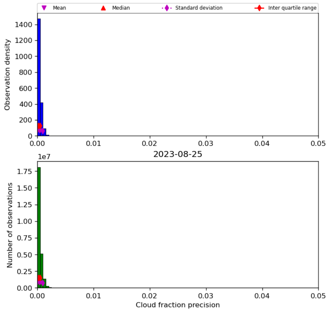
Figure 33: Histogram of “Cloud fraction precision” for 2023-08-25 to 2023-08-26
