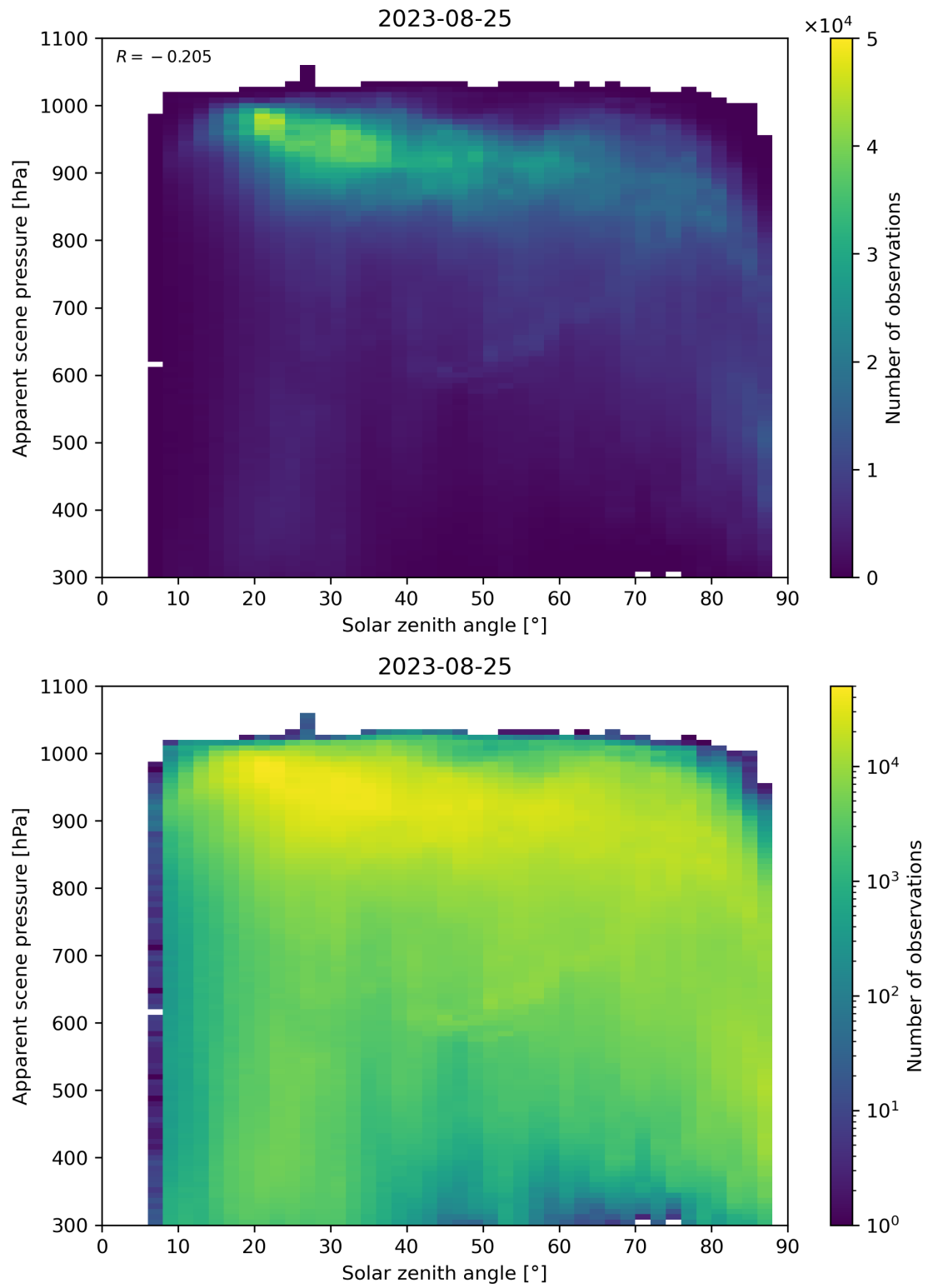
Figure 118: Scatter density plot of “Solar zenith angle” against “Apparent scene pressure” for 2023-08-25 to 2023-08-26.
