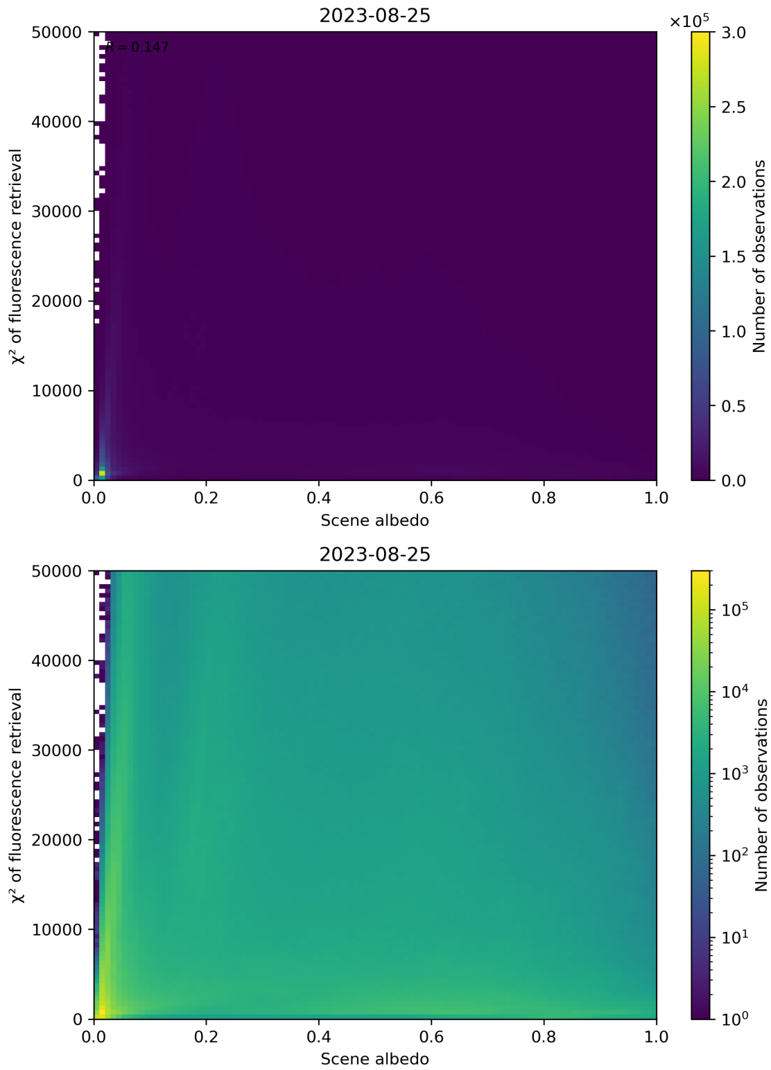
Figure 113: Scatter density plot of “Scene albedo” against “ \chi^2 of fluorescence retrieval” for 2023-08-25 to 2023-08-26.
