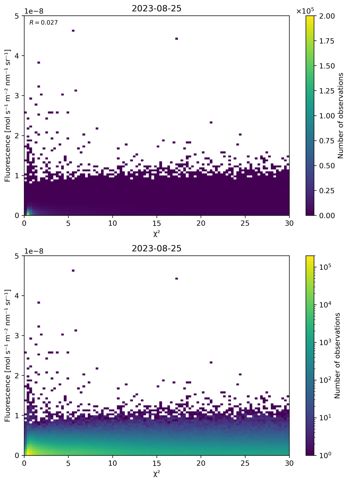
Figure 70: Scatter density plot of “ \chi^2 ” against “Fluorescence” for 2023-08-25 to 2023-08-26.
