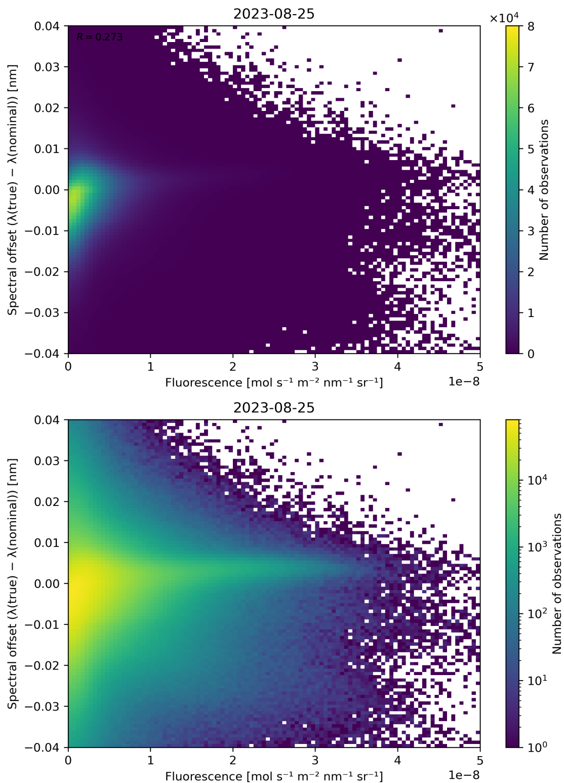
Figure 95: Scatter density plot of “Fluorescence” against “Spectral offset ( \lambda(\text{true}) - \lambda(\text{nominal}) )” for 2023-08-25 to 2023-08-26.
