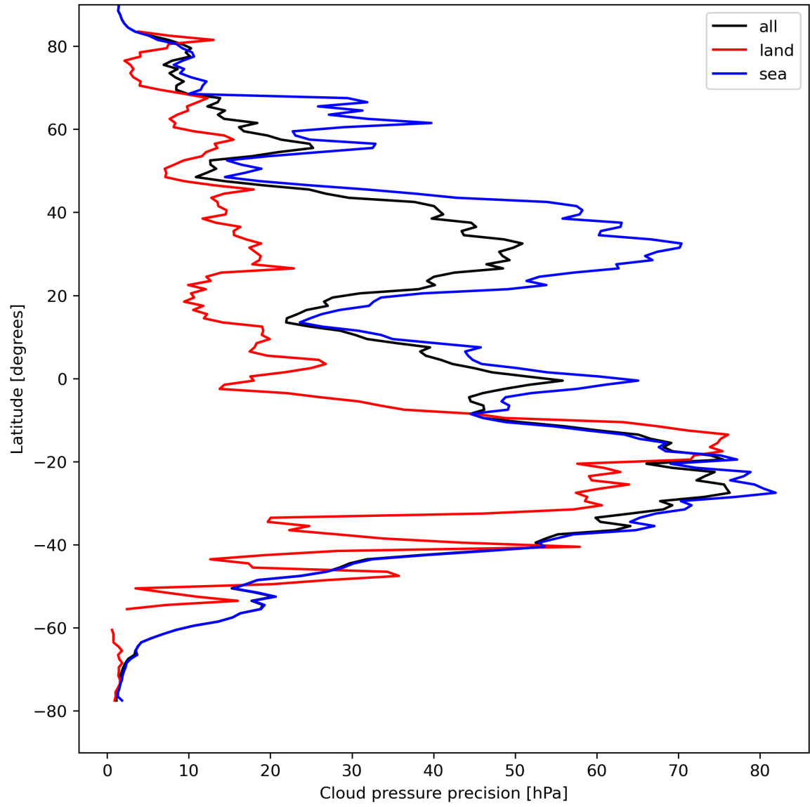
Figure 14: Zonal average of “Cloud pressure precision” for 2023-08-25 to 2023-08-26.
