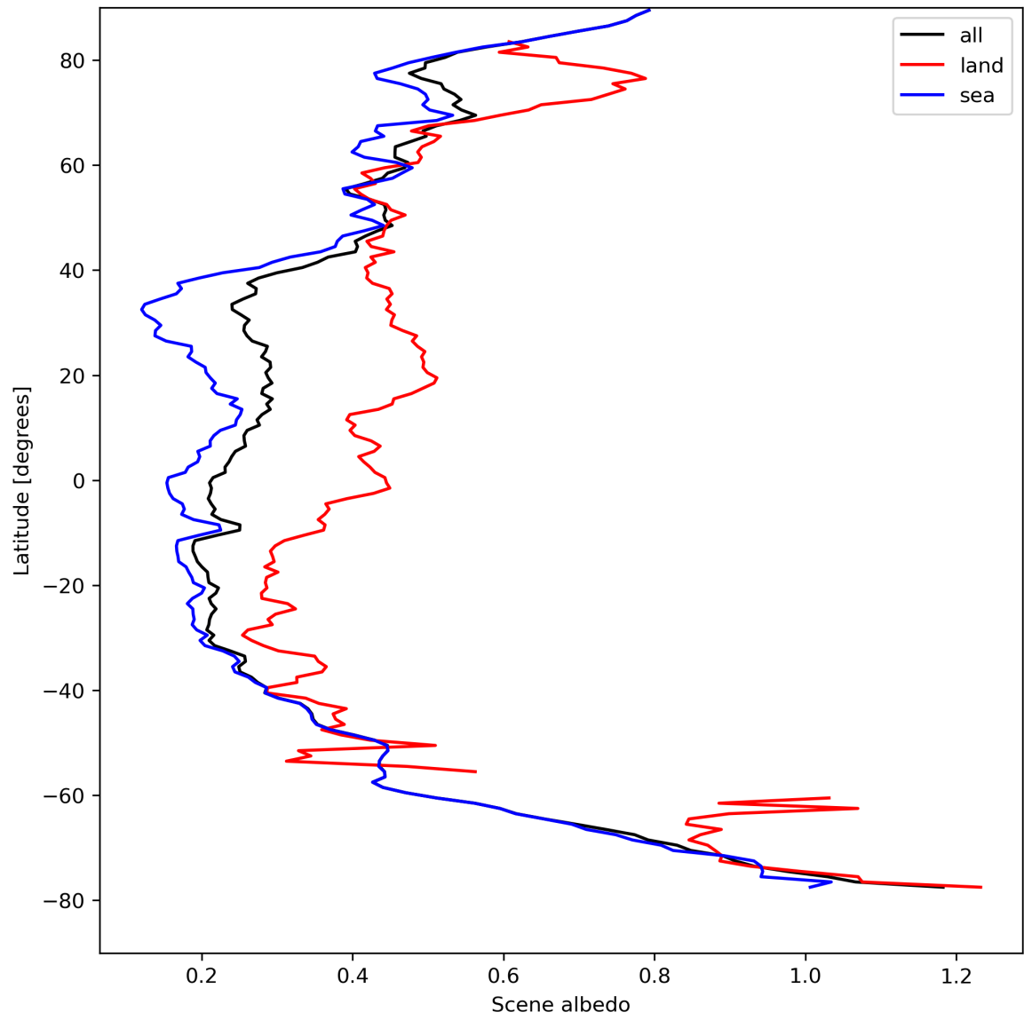
Figure 17: Zonal average of “Scene albedo” for 2023-08-25 to 2023-08-26.
