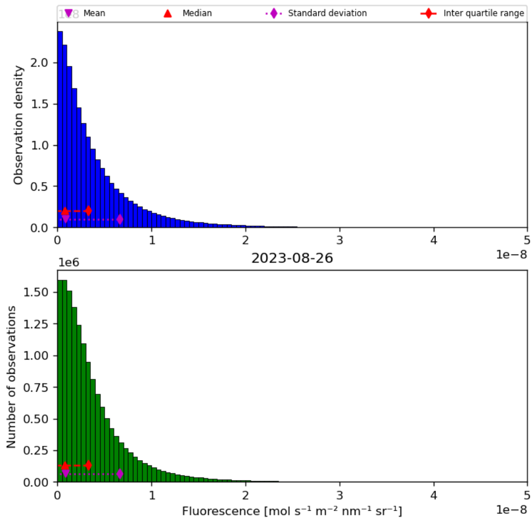
Figure 40: Histogram of “Fluorescence” for 2023-08-25 to 2023-08-27
