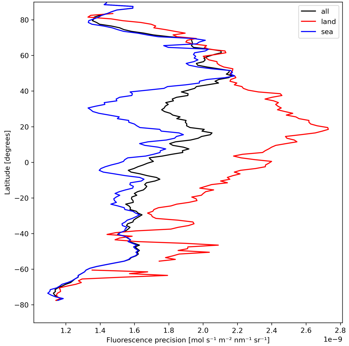
Figure 24: Zonal average of “Fluorescence precision” for 2023-08-25 to 2023-08-27.
