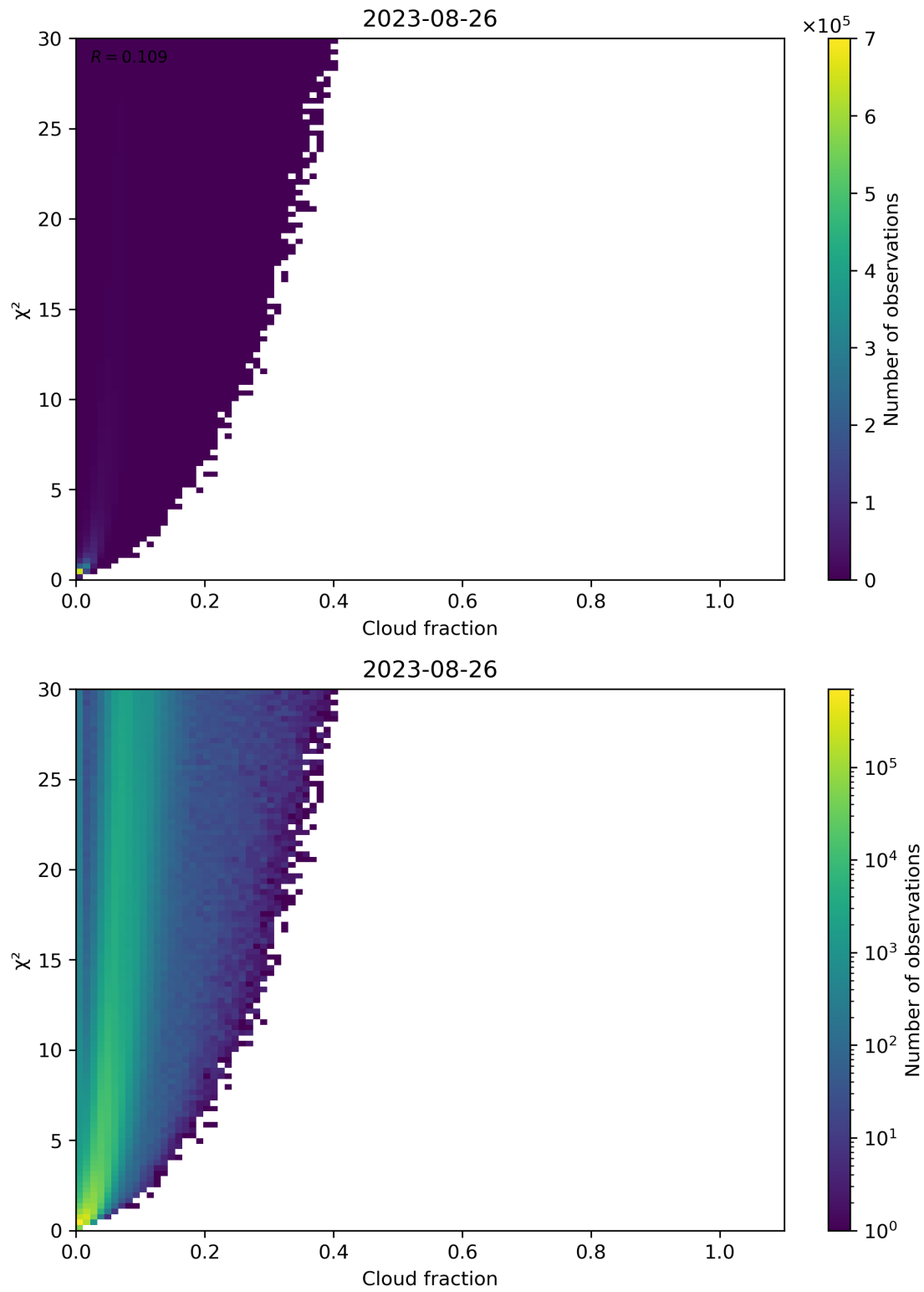
Figure 77: Scatter density plot of “Cloud fraction” against “ \chi^2 ” for 2023-08-25 to 2023-08-27.
