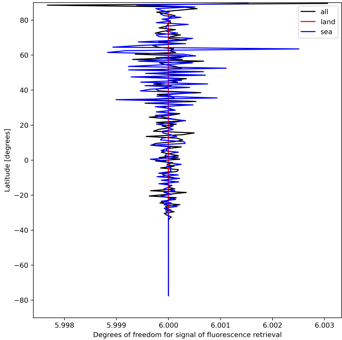
Figure 26: Zonal average of “Degrees of freedom for signal of fluorescence retrieval” for 2023-08-25 to 2023-08-27.
