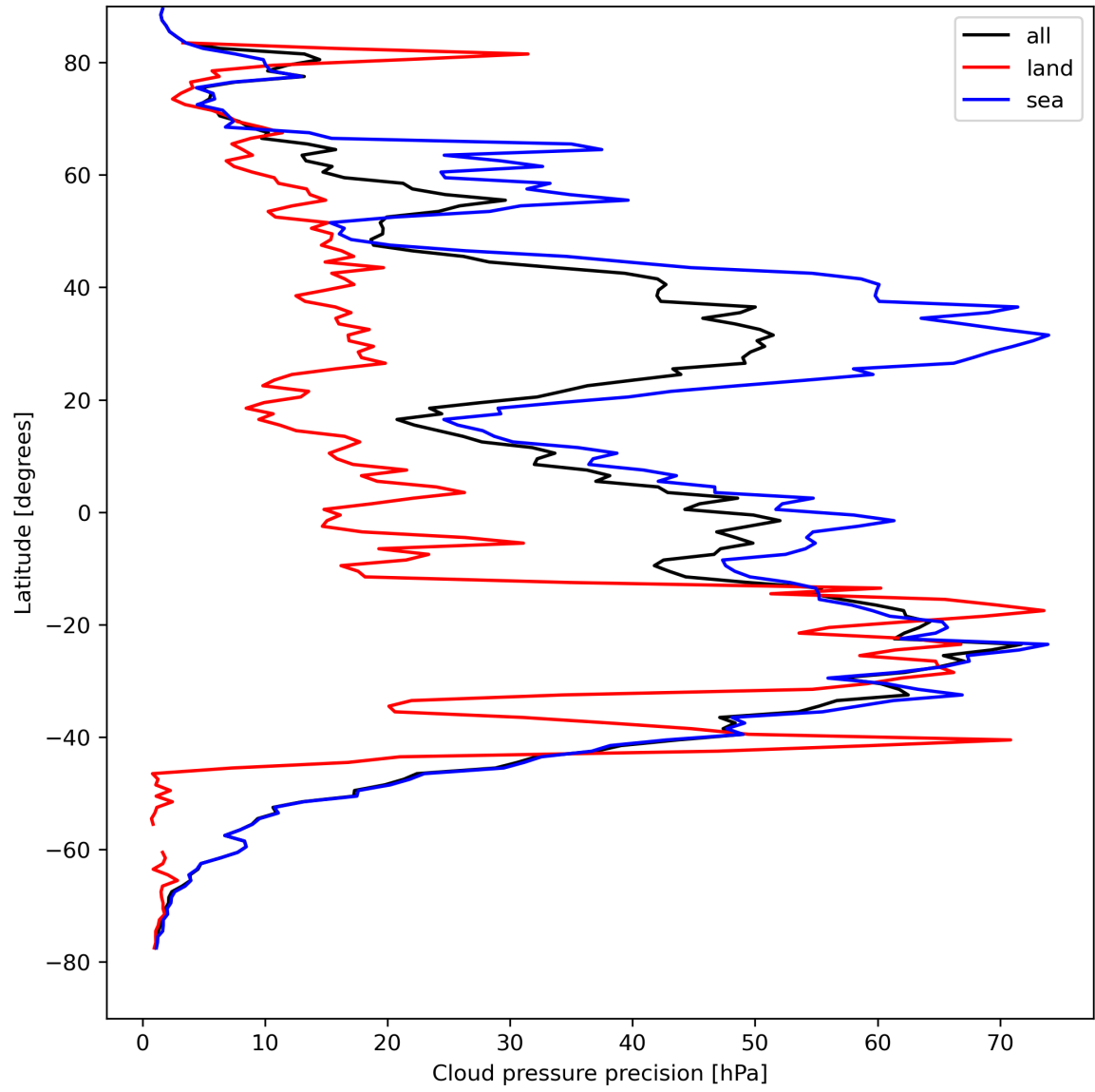
Figure 14: Zonal average of “Cloud pressure precision” for 2023-08-25 to 2023-08-27.
