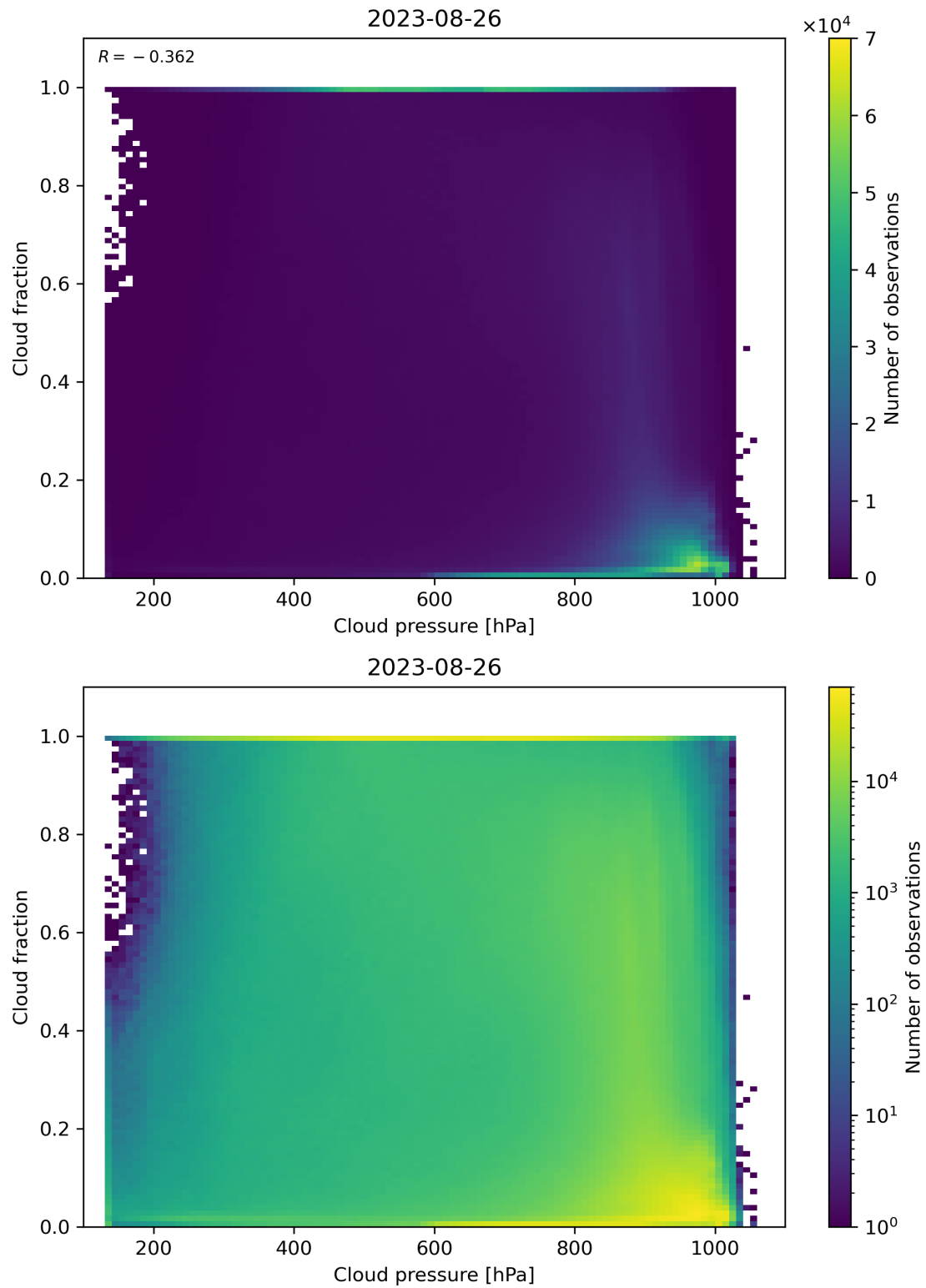
Figure 87: Scatter density plot of “Cloud pressure” against “Cloud fraction” for 2023-08-25 to 2023-08-27.
