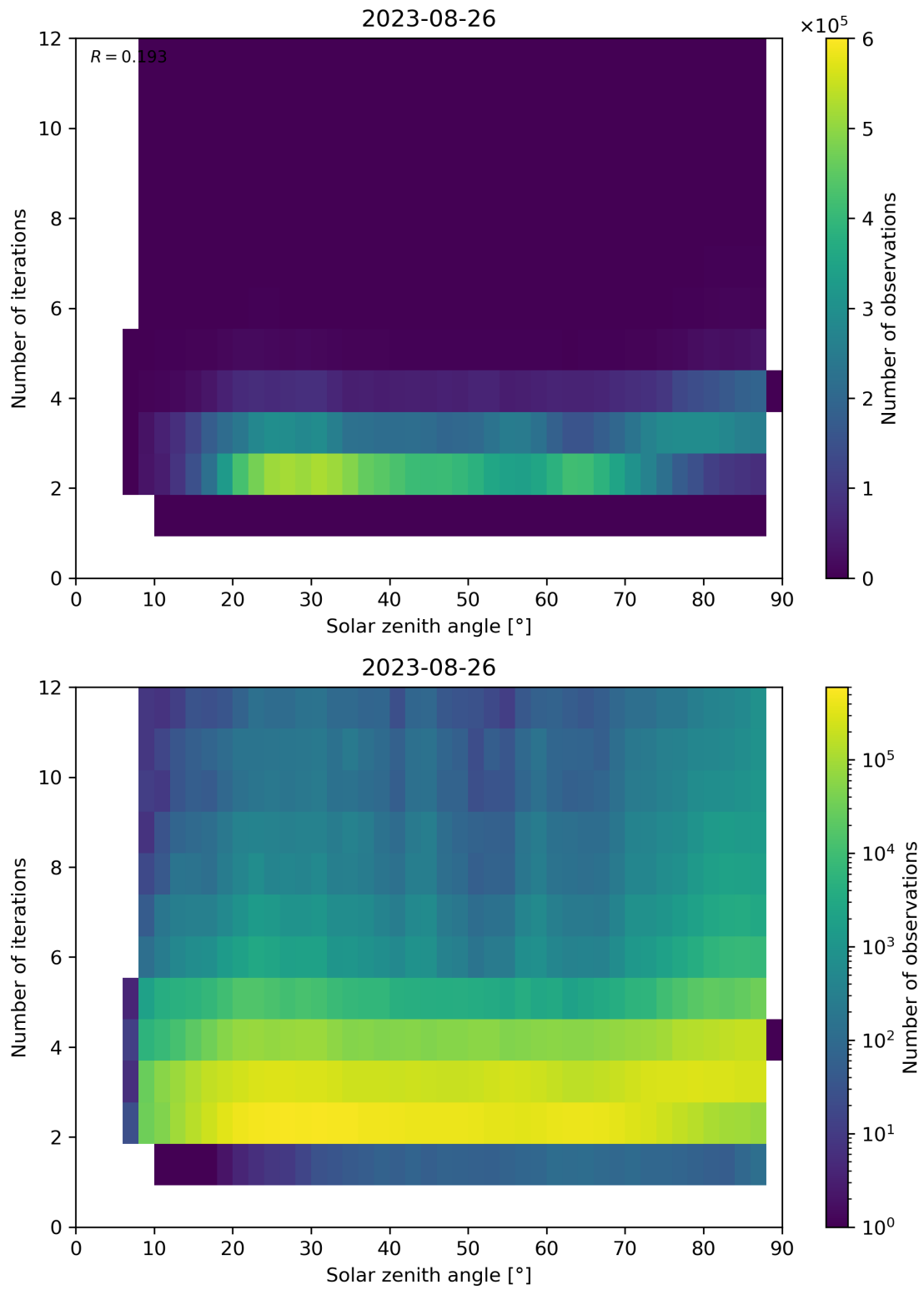
Figure 125: Scatter density plot of “Solar zenith angle” against “Number of iterations” for 2023-08-25 to 2023-08-27.
