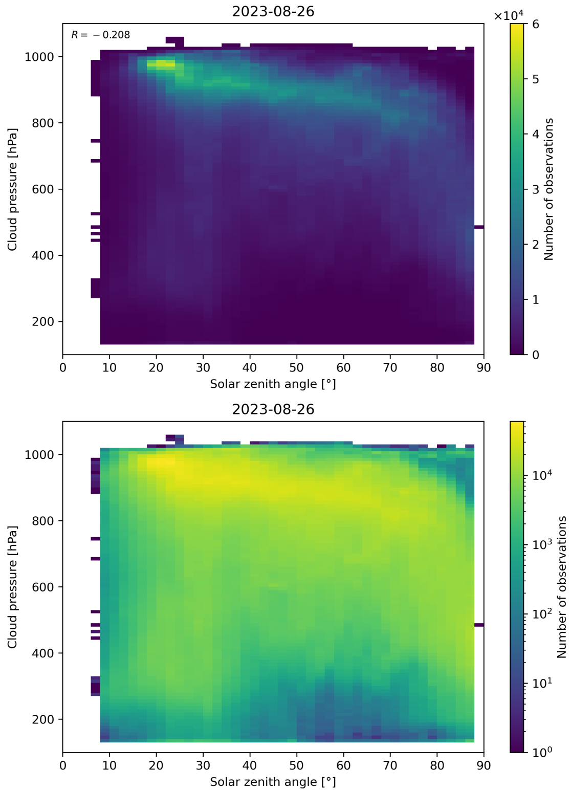
Figure 122: Scatter density plot of “Solar zenith angle” against “Cloud pressure” for 2023-08-25 to 2023-08-27.
