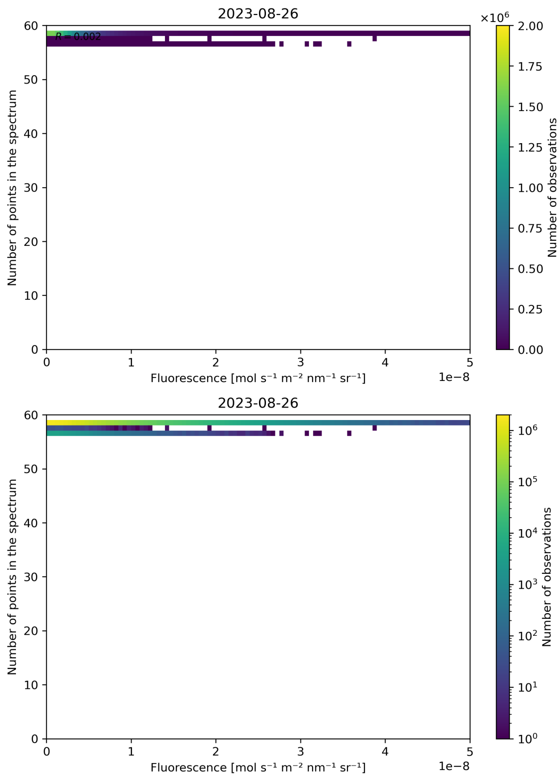
Figure 94: Scatter density plot of “Fluorescence” against “Number of points in the spectrum” for 2023-08-25 to 2023-08-27.
