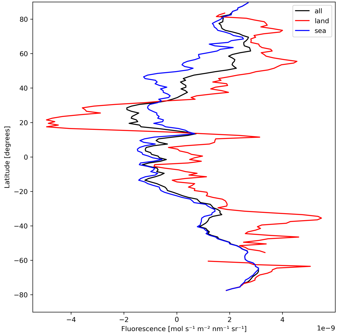
Figure 23: Zonal average of “Fluorescence” for 2023-08-25 to 2023-08-27.
