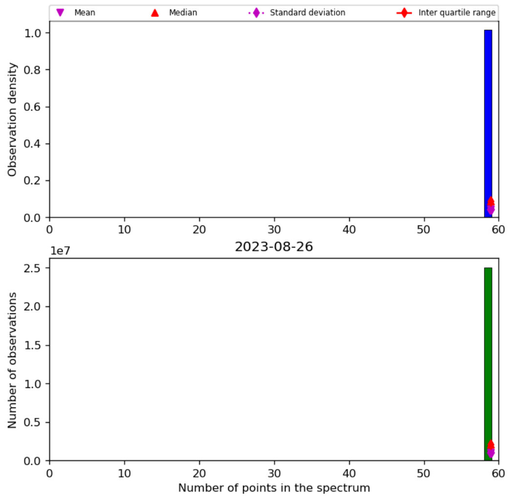
Figure 44: Histogram of “Number of points in the spectrum” for 2023-08-25 to 2023-08-27
