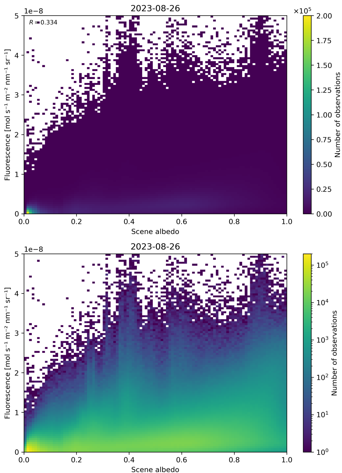
Figure 114: Scatter density plot of “Scene albedo” against “Fluorescence” for 2023-08-25 to 2023-08-27.
