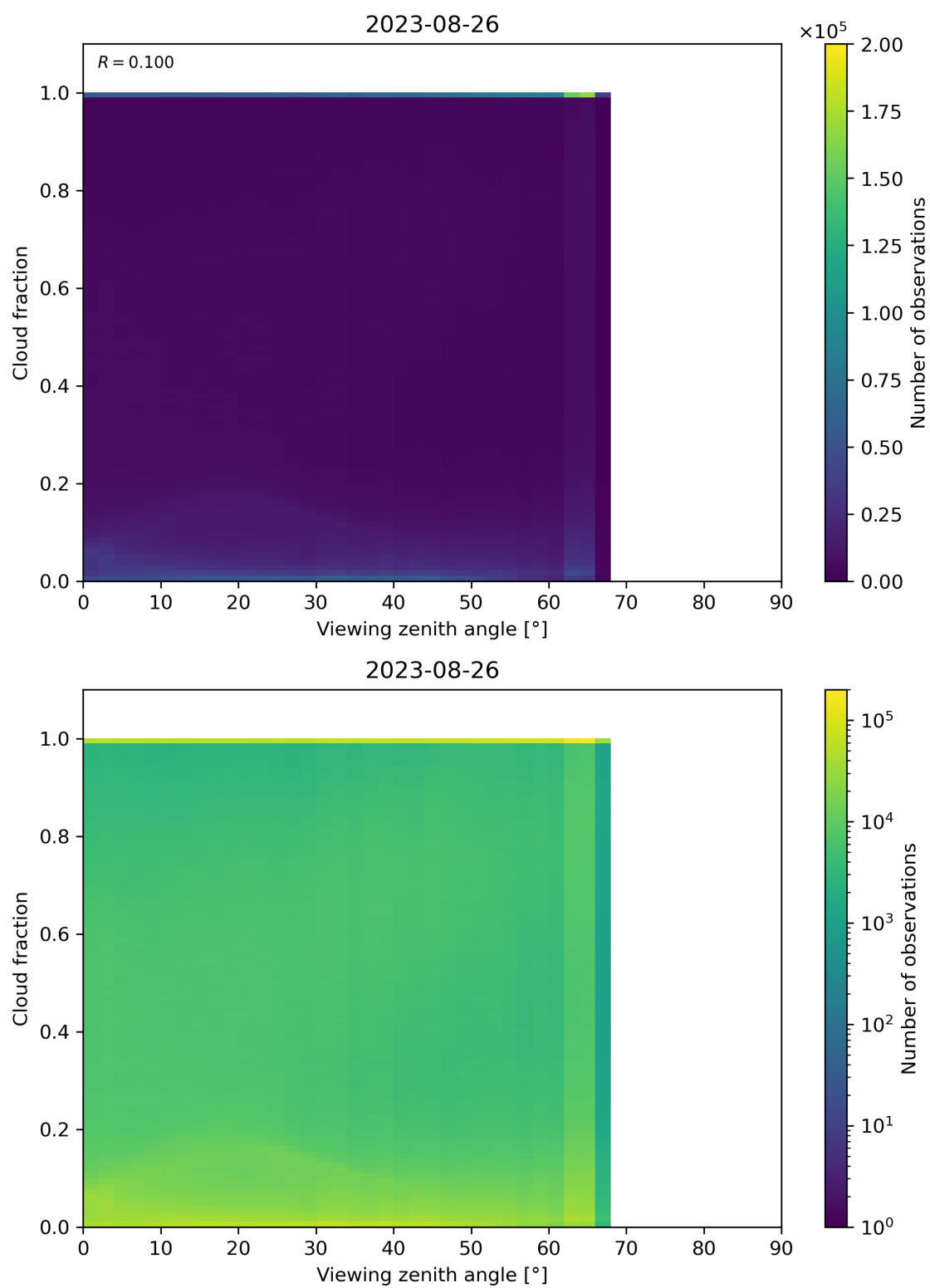
Figure 132: Scatter density plot of “Viewing zenith angle” against “Cloud fraction” for 2023-08-25 to 2023-08-27.
