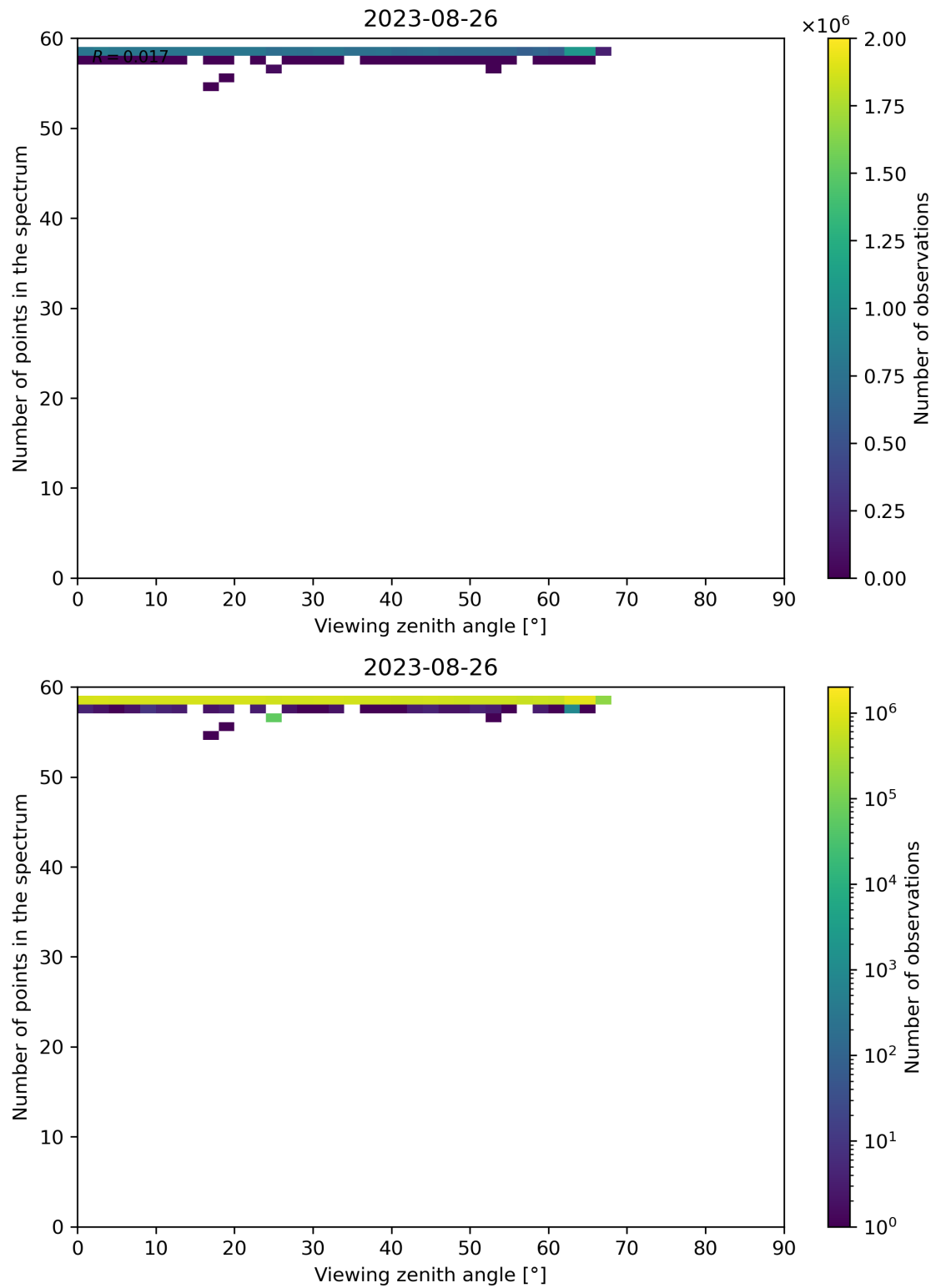
Figure 137: Scatter density plot of “Viewing zenith angle” against “Number of points in the spectrum” for 2023-08-25 to 2023-08-27.
