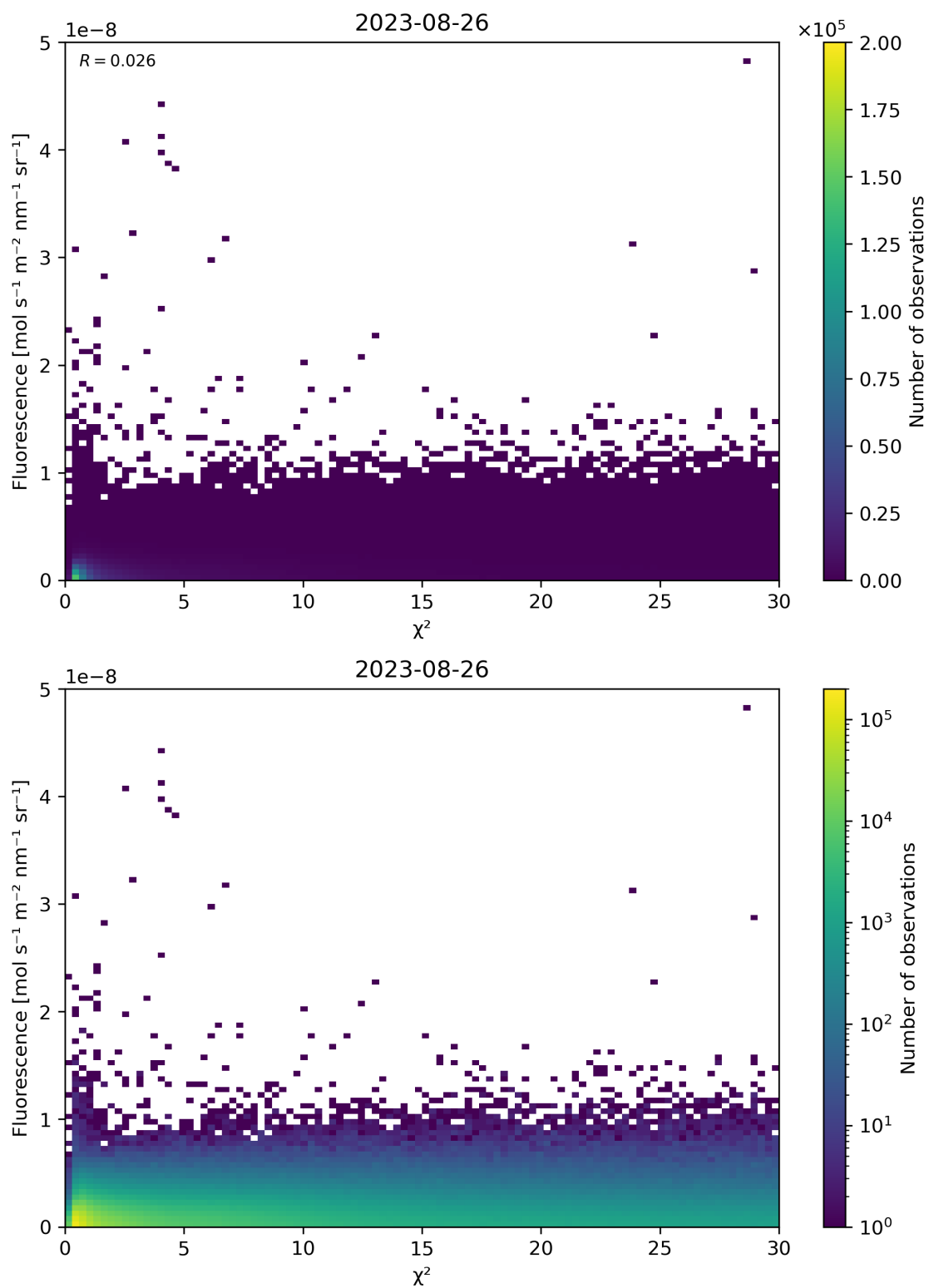
Figure 70: Scatter density plot of “ \chi^2 ” against “Fluorescence” for 2023-08-25 to 2023-08-27.
