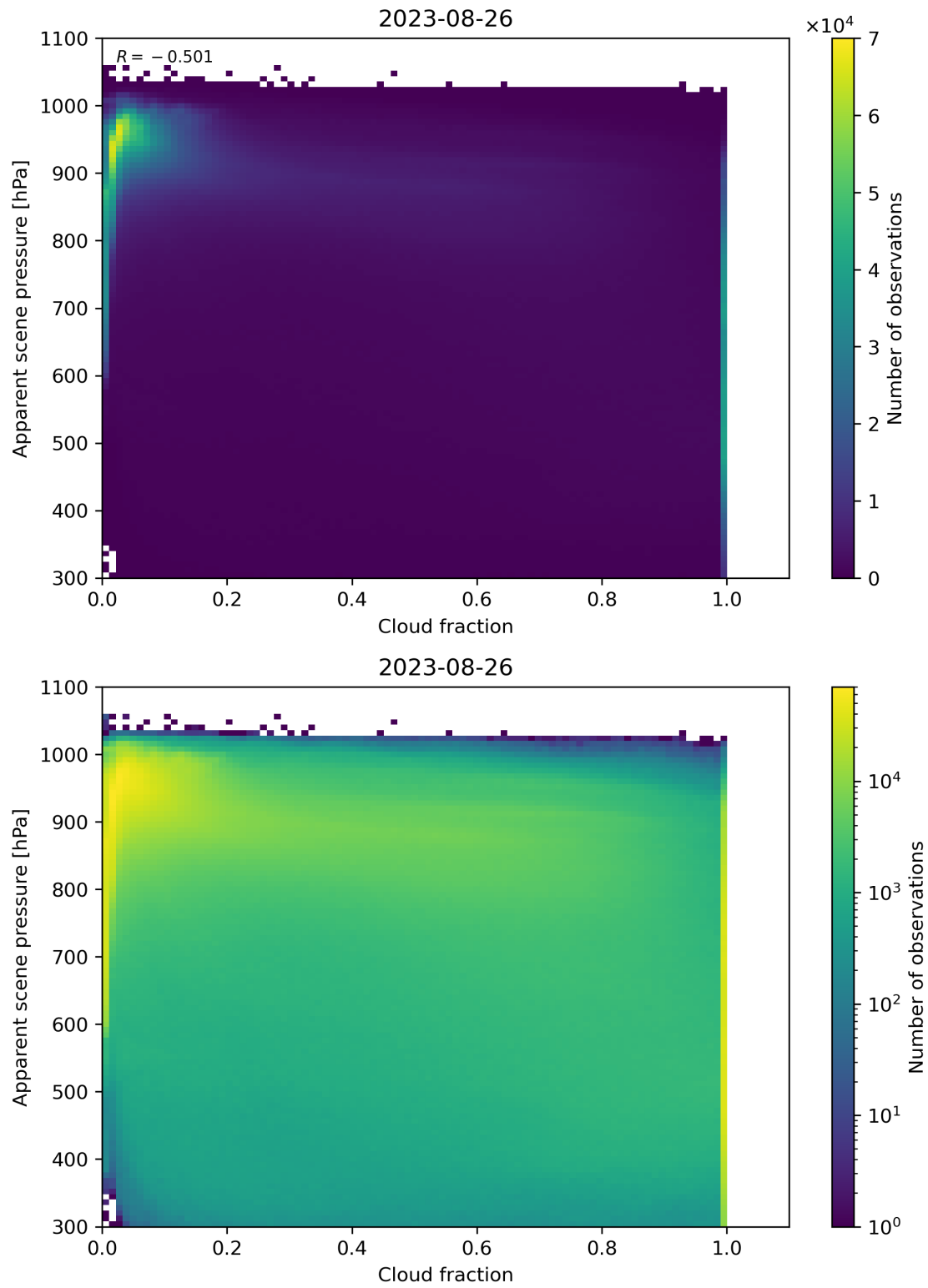
Figure 76: Scatter density plot of “Cloud fraction” against “Apparent scene pressure” for 2023-08-25 to 2023-08-27.
