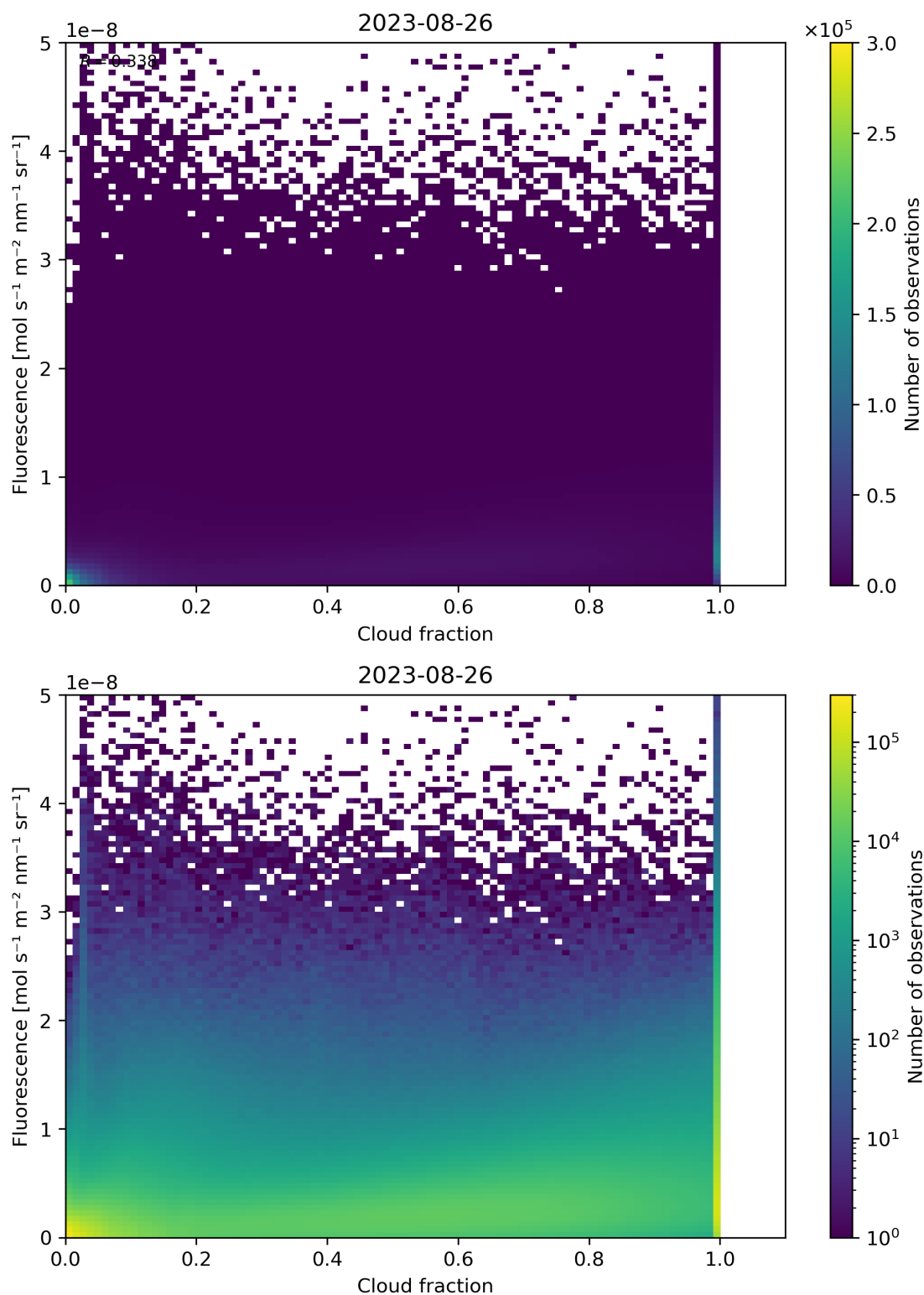
Figure 79: Scatter density plot of “Cloud fraction” against “Fluorescence” for 2023-08-25 to 2023-08-27.
