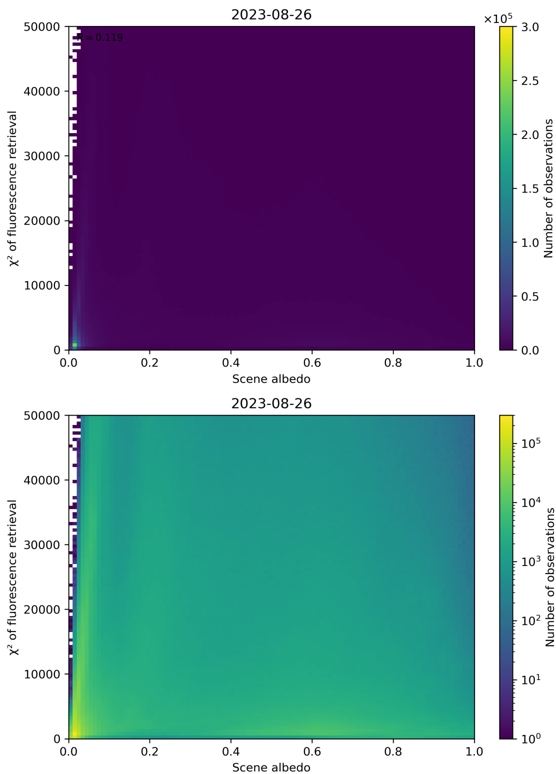
Figure 113: Scatter density plot of “Scene albedo” against “ \chi^2 of fluorescence retrieval” for 2023-08-25 to 2023-08-27.
