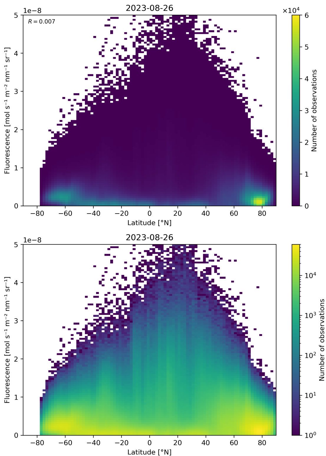
Figure 101: Scatter density plot of “Latitude” against “Fluorescence” for 2023-08-25 to 2023-08-27.
