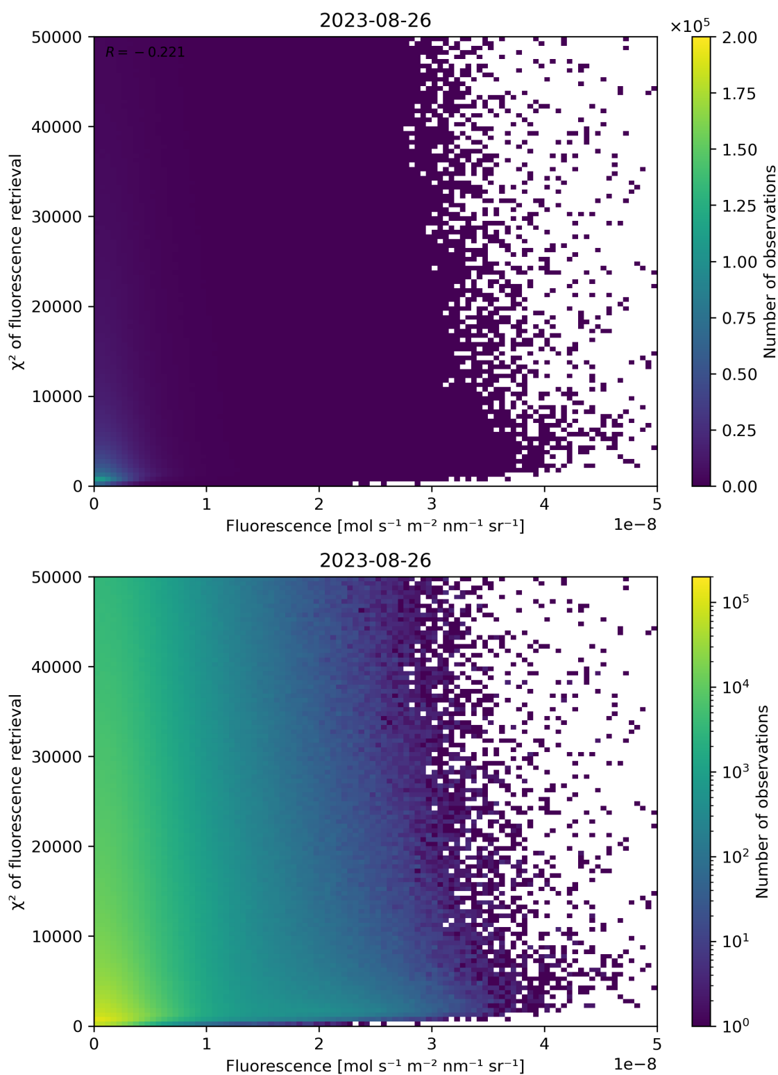
Figure 93: Scatter density plot of “Fluorescence” against “ \chi^2 of fluorescence retrieval” for 2023-08-25 to 2023-08-27.
