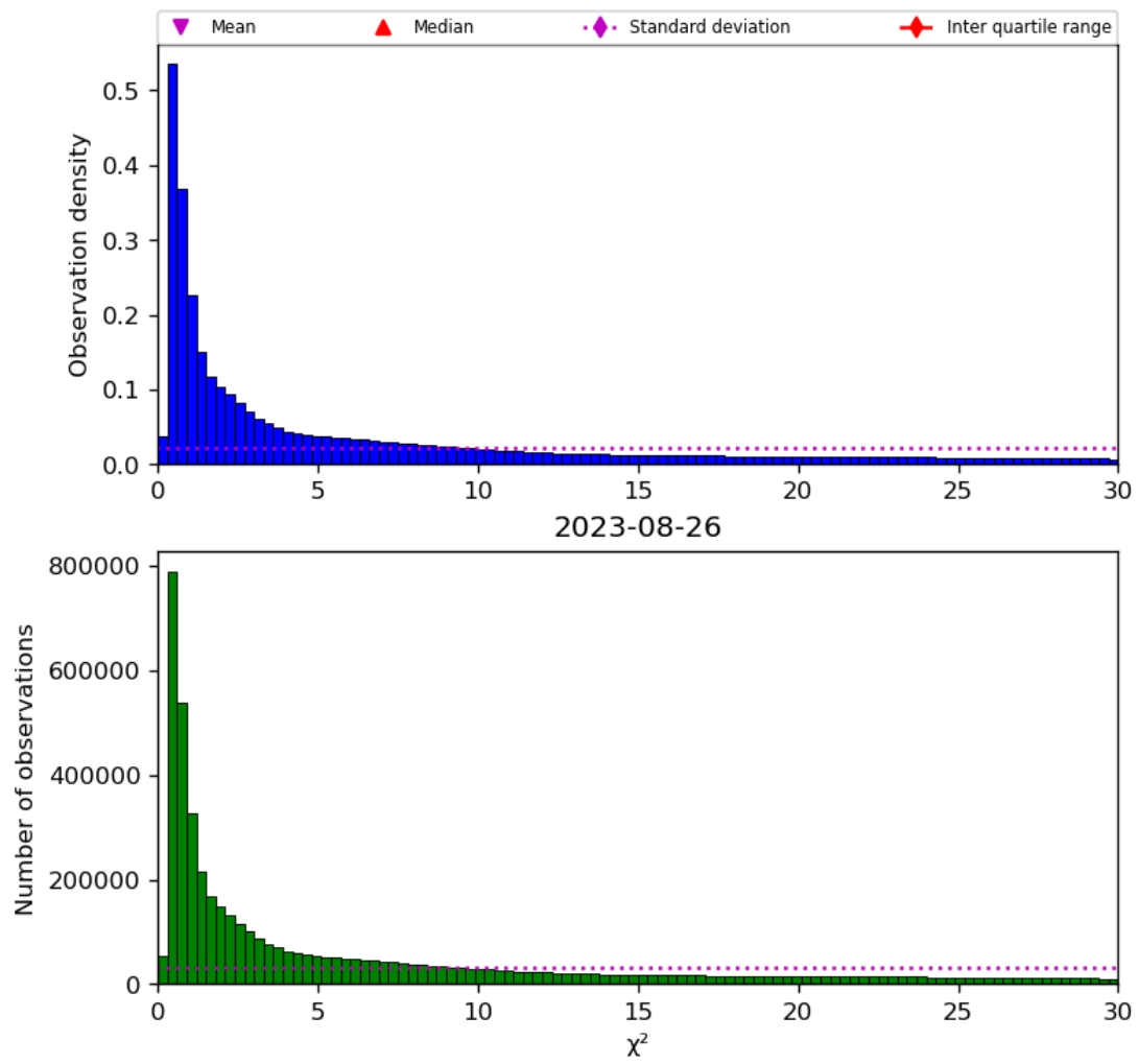
Figure 38: Histogram of “ \chi^2 ” for 2023-08-25 to 2023-08-27
