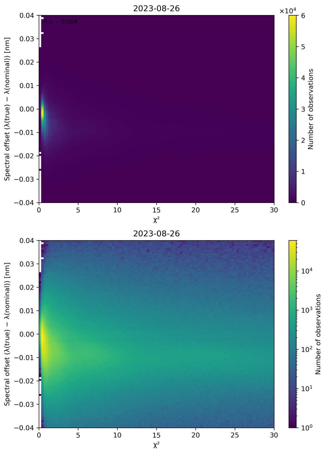
Figure 75: Scatter density plot of " \chi^2 " against "Spectral offset ( \lambda(\text{true}) - \lambda(\text{nominal}) )" for 2023-08-25 to 2023-08-27.
