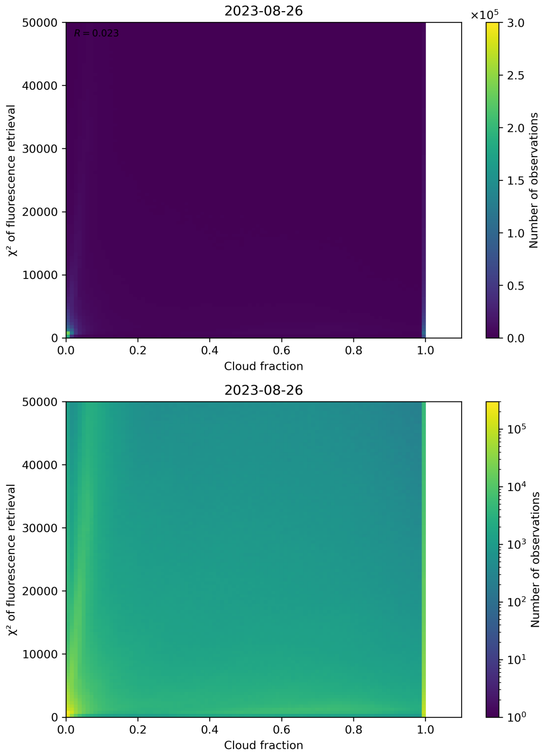
Figure 78: Scatter density plot of “Cloud fraction” against “ \chi^2 of fluorescence retrieval” for 2023-08-25 to 2023-08-27.
