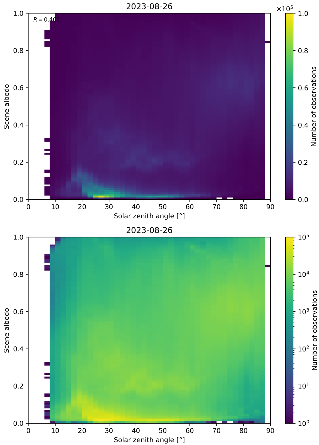
Figure 127: Scatter density plot of “Solar zenith angle” against “Scene albedo” for 2023-08-25 to 2023-08-27.
