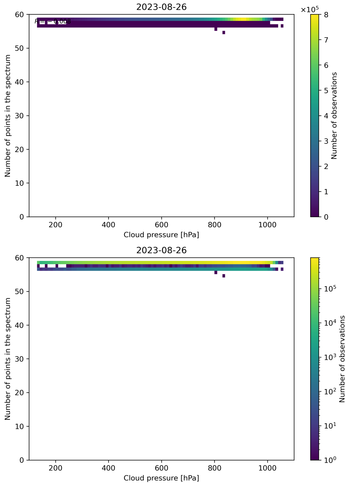
Figure 90: Scatter density plot of “Cloud pressure” against “Number of points in the spectrum” for 2023-08-25 to 2023-08-27.
