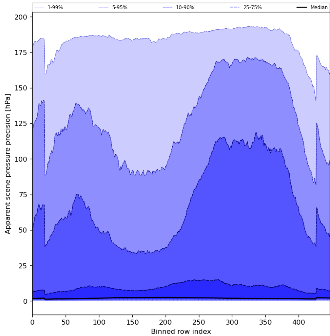
Figure 54: Along track statistics of “Apparent scene pressure precision” for 2023-08-25 to 2023-08-27
