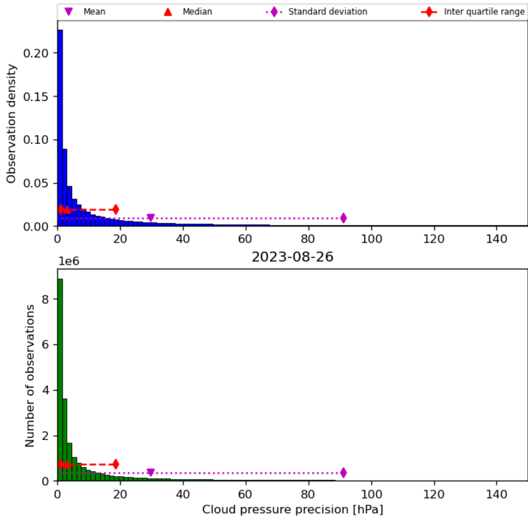
Figure 31: Histogram of “Cloud pressure precision” for 2023-08-25 to 2023-08-27
