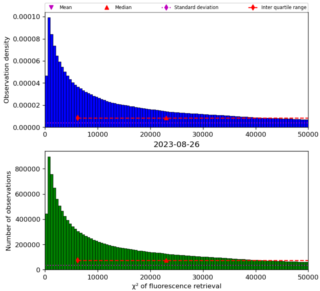
Figure 42: Histogram of “ \chi^2 of fluorescence retrieval” for 2023-08-25 to 2023-08-27
