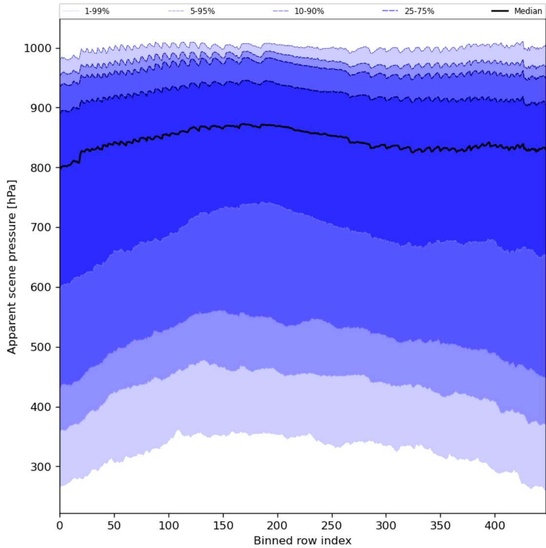
Figure 53: Along track statistics of “Apparent scene pressure” for 2023-08-25 to 2023-08-27
