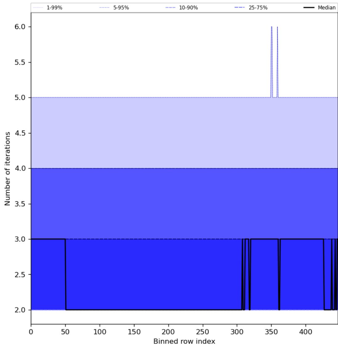
Figure 56: Along track statistics of “Number of iterations” for 2023-08-25 to 2023-08-27
