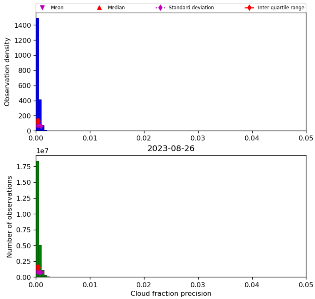
Figure 33: Histogram of “Cloud fraction precision” for 2023-08-25 to 2023-08-27
