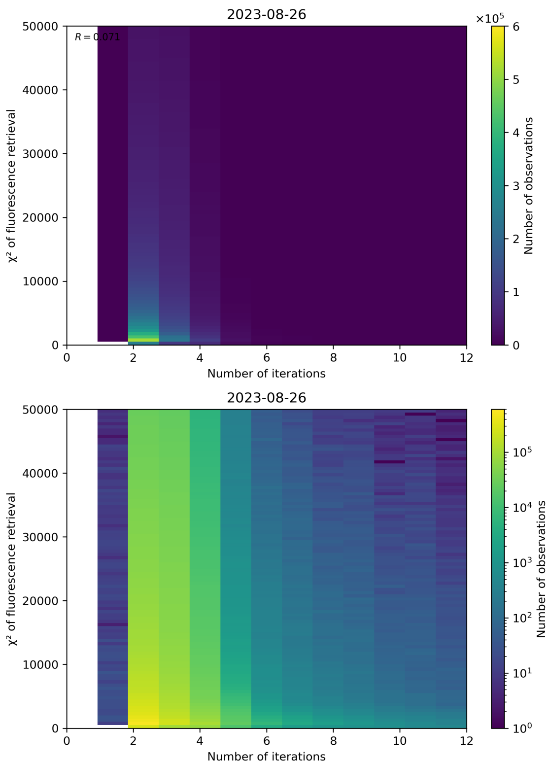
Figure 106: Scatter density plot of “Number of iterations” against “ \chi^2 of fluorescence retrieval” for 2023-08-25 to 2023-08-27.
