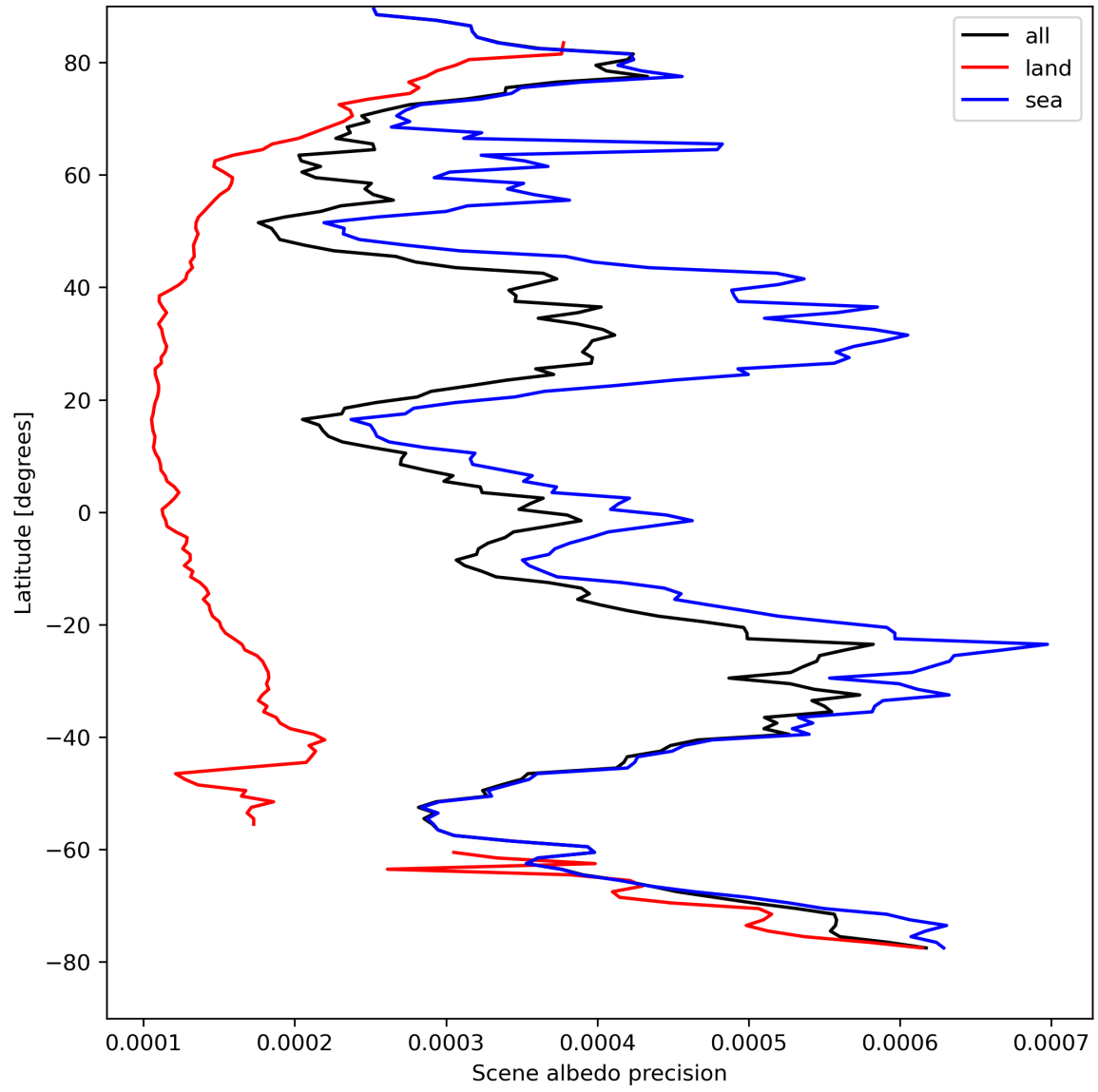
Figure 18: Zonal average of “Scene albedo precision” for 2023-08-25 to 2023-08-27.
