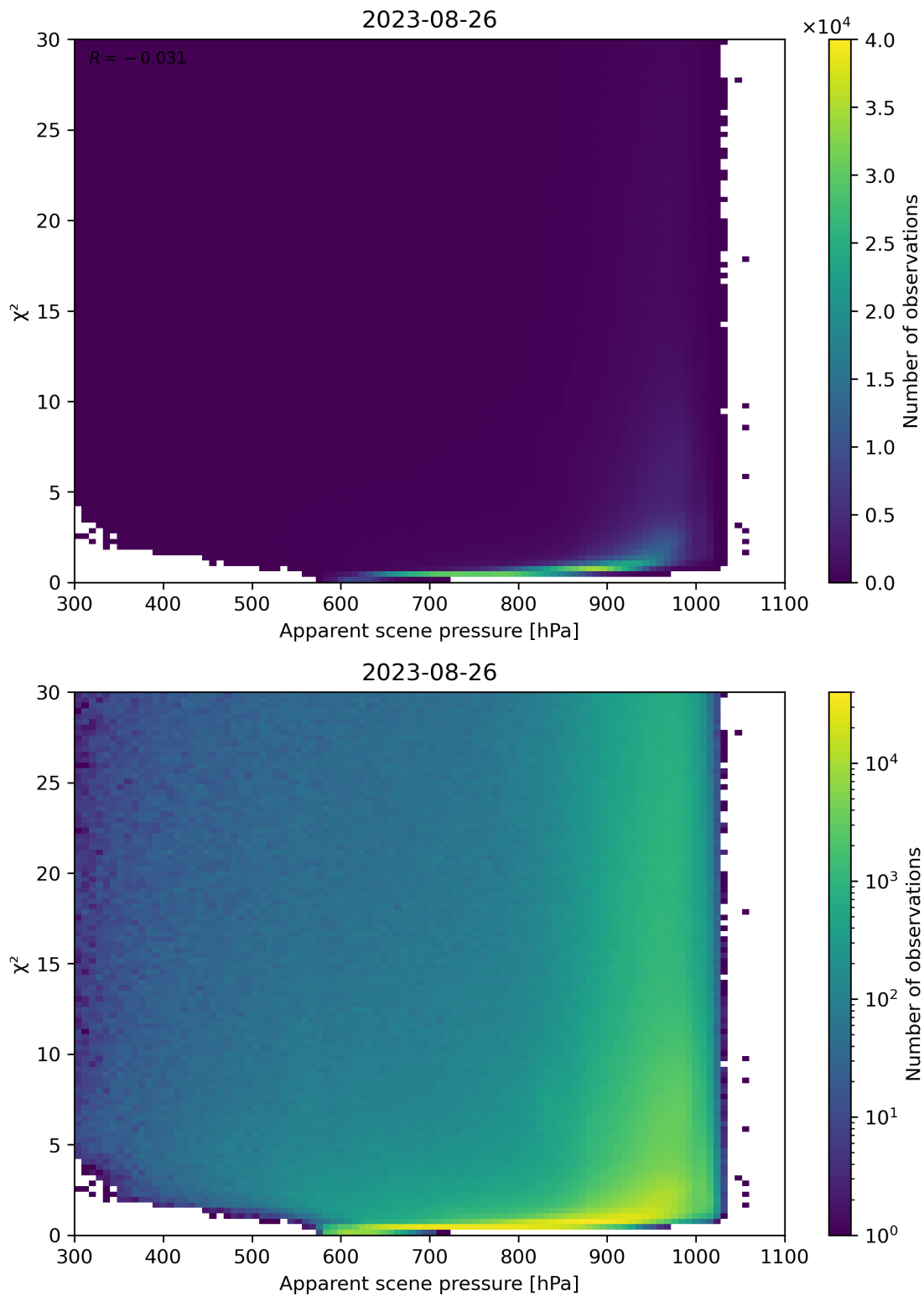
Figure 63: Scatter density plot of “Apparent scene pressure” against “ \chi^2 ” for 2023-08-25 to 2023-08-27.
