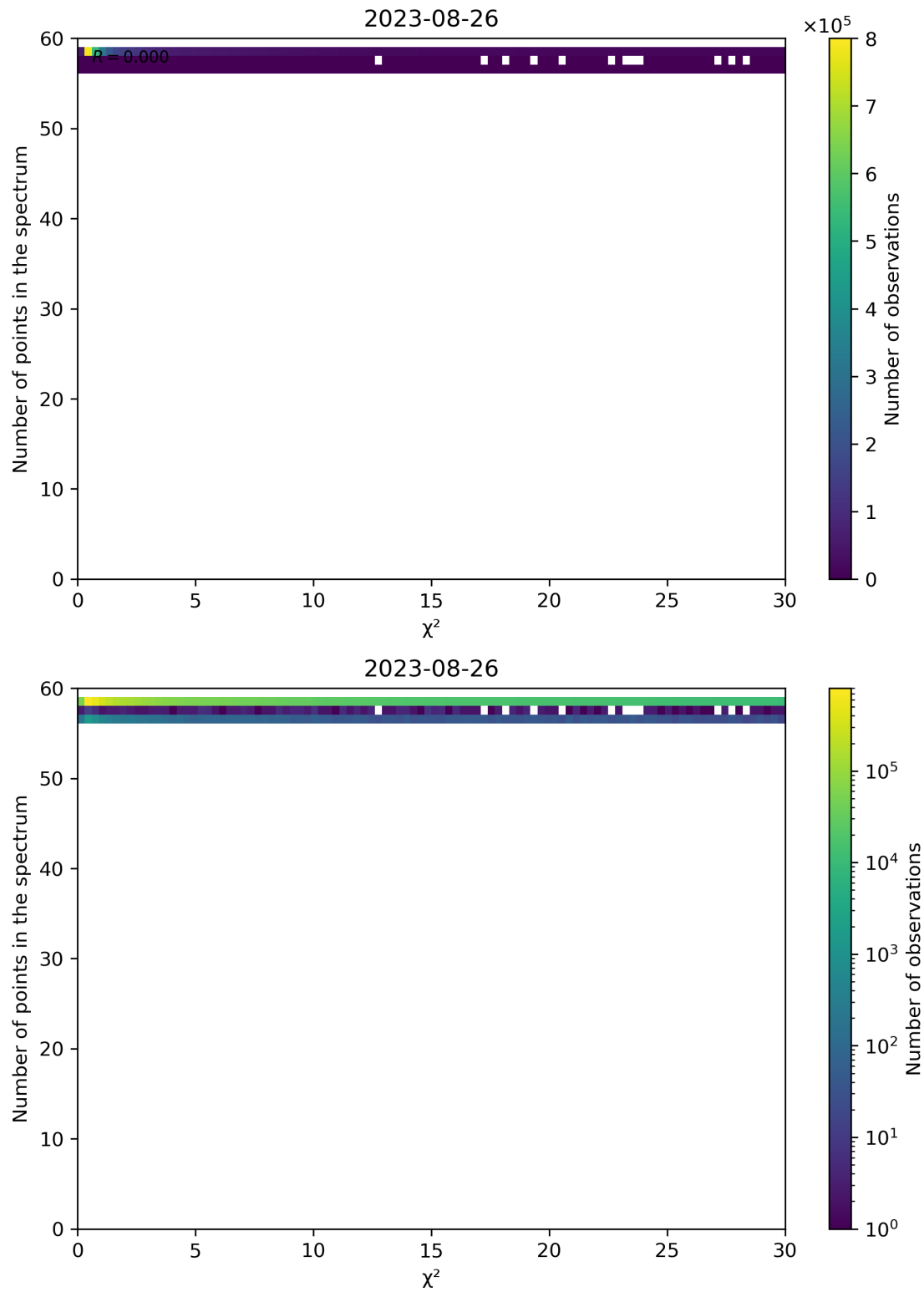
Figure 74: Scatter density plot of " \chi^2 " against "Number of points in the spectrum" for 2023-08-25 to 2023-08-27.
