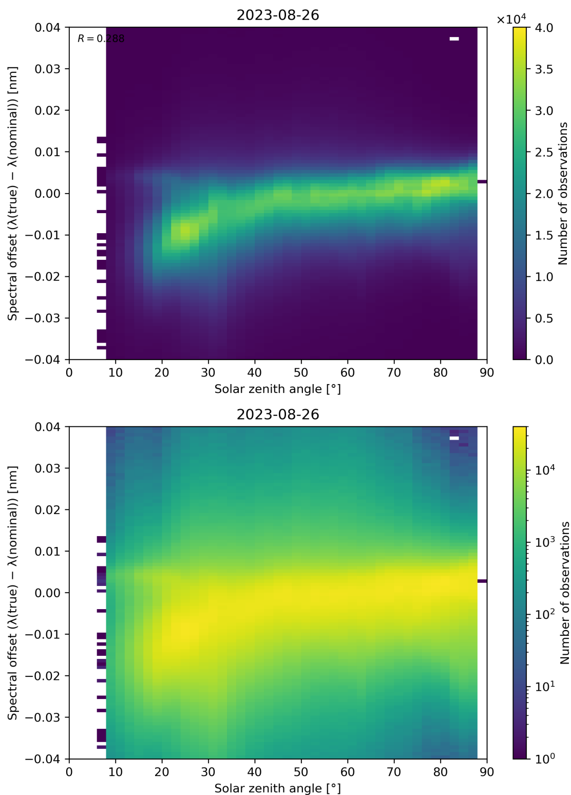
Figure 128: Scatter density plot of “Solar zenith angle” against “Spectral offset ( \lambda(\text{true}) - \lambda(\text{nominal}) )” for 2023-08-25 to 2023-08-27.
