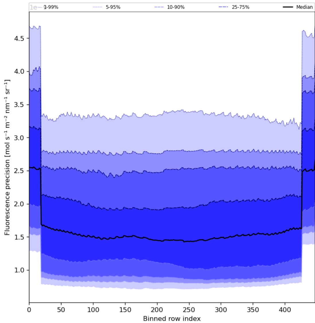
Figure 58: Along track statistics of “Fluorescence precision” for 2023-08-25 to 2023-08-27
