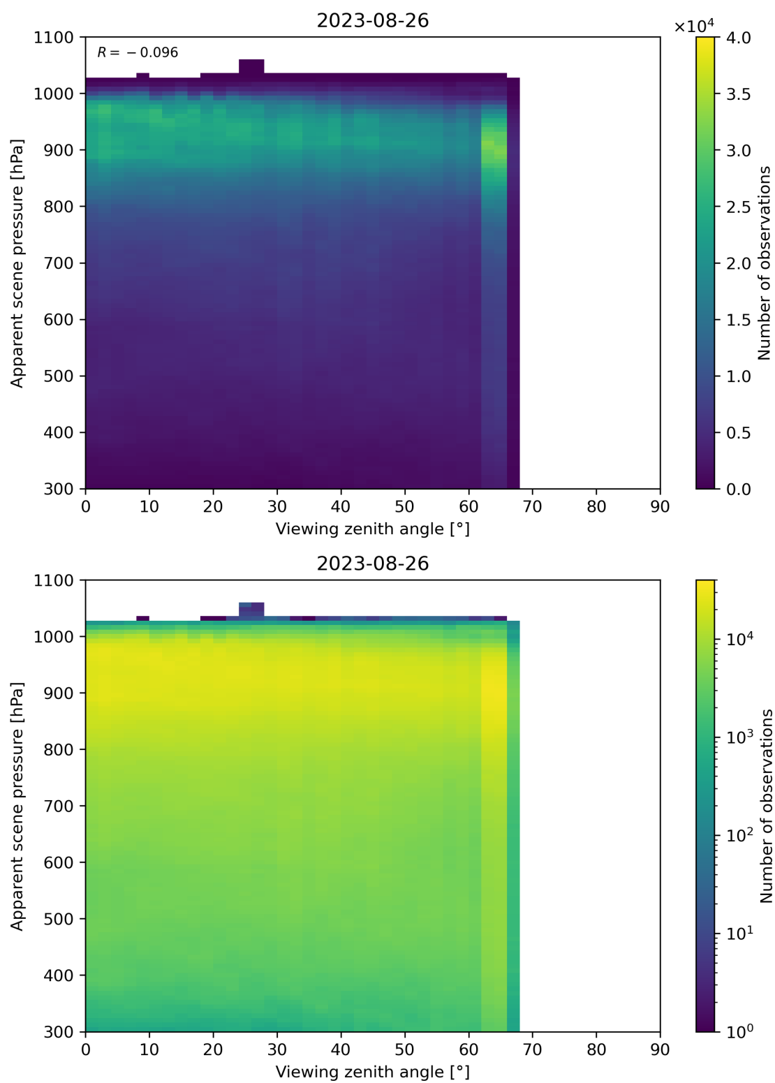
Figure 129: Scatter density plot of “Viewing zenith angle” against “Apparent scene pressure” for 2023-08-25 to 2023-08-27.
