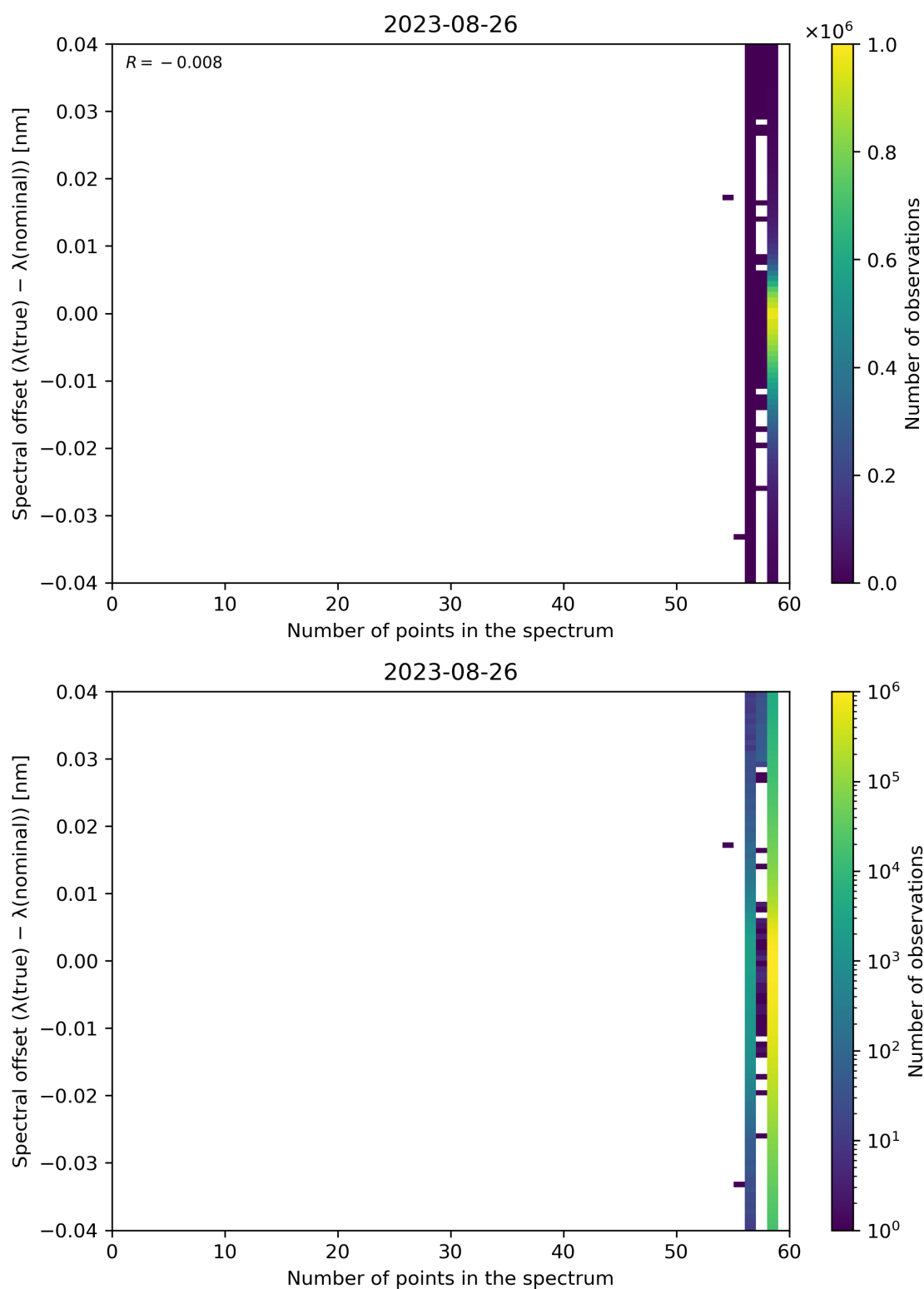
Figure 110: Scatter density plot of “Number of points in the spectrum” against “Spectral offset ( \lambda(\text{true}) - \lambda(\text{nominal}) )” for 2023-08-25 to 2023-08-27.
