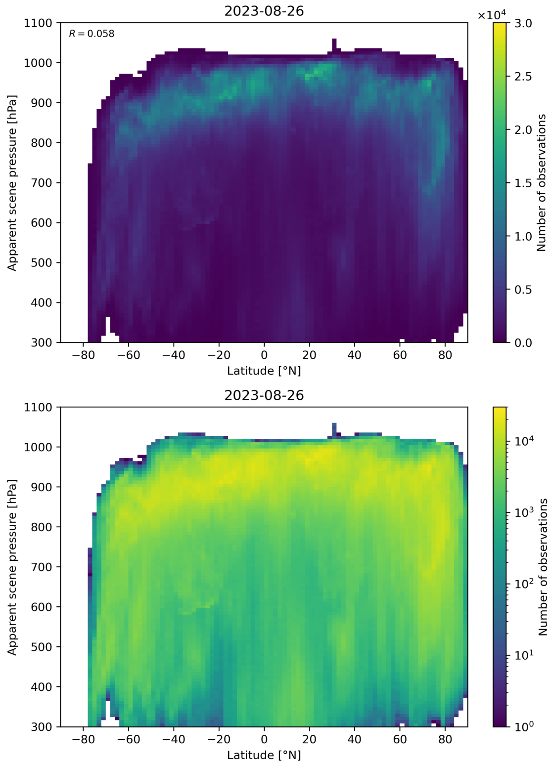
Figure 96: Scatter density plot of “Latitude” against “Apparent scene pressure” for 2023-08-25 to 2023-08-27.
