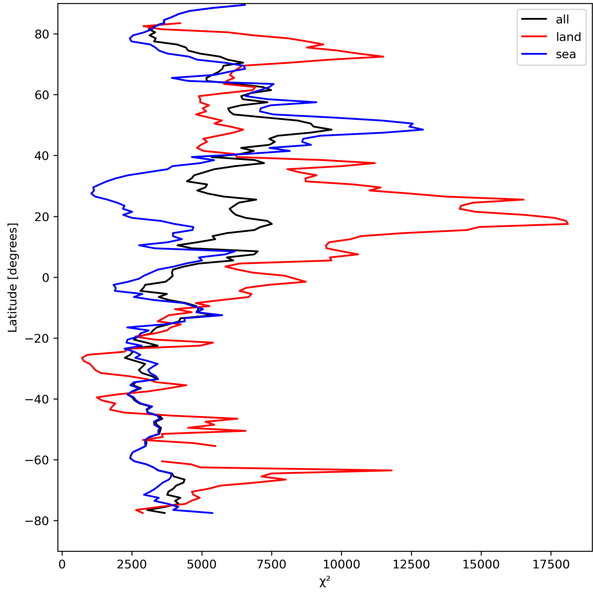
Figure 21: Zonal average of “ \chi^2 ” for 2023-08-25 to 2023-08-27.
