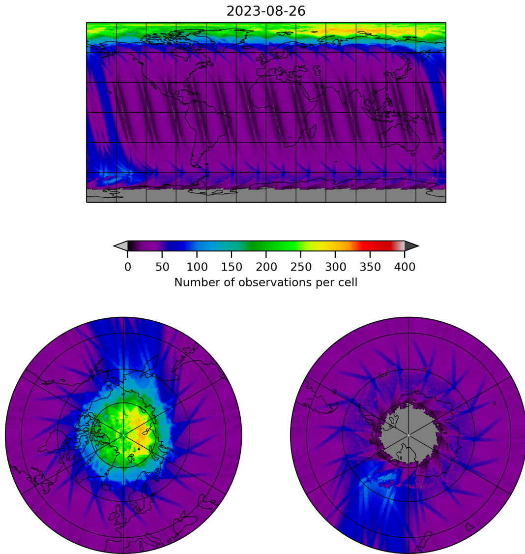
Figure 11: Map of the number of observations for 2023-08-25 to 2023-08-27
