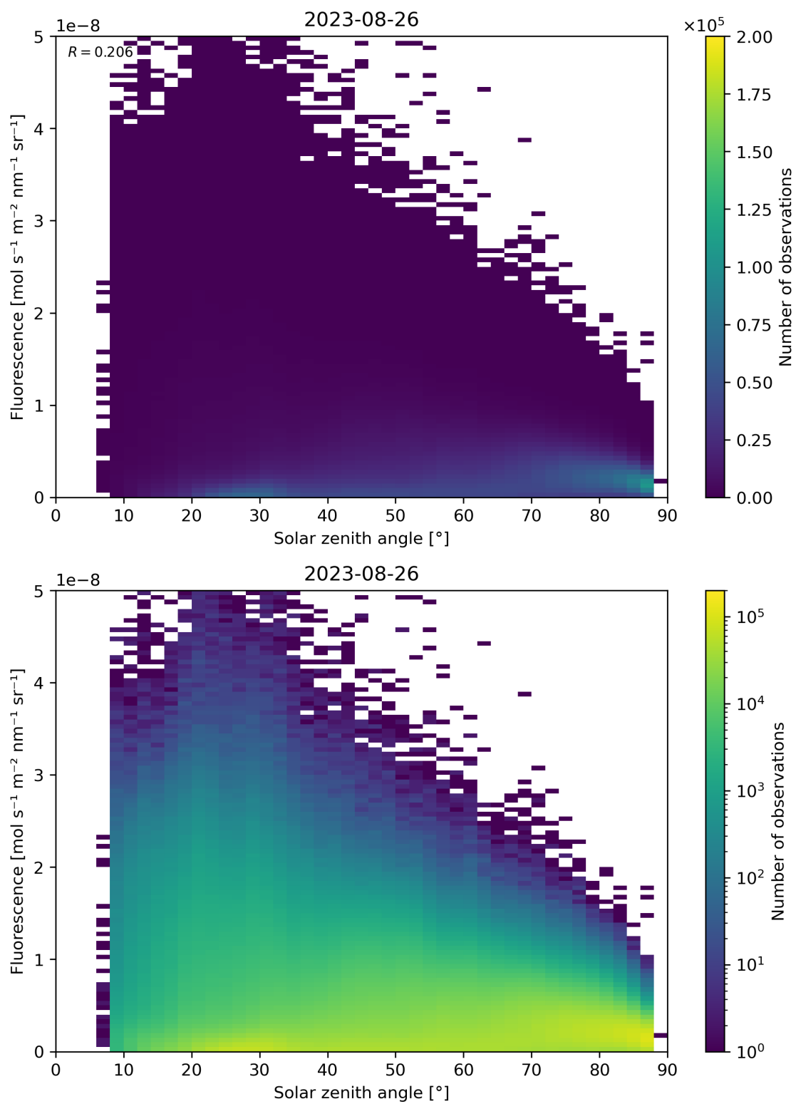
Figure 123: Scatter density plot of “Solar zenith angle” against “Fluorescence” for 2023-08-25 to 2023-08-27.
