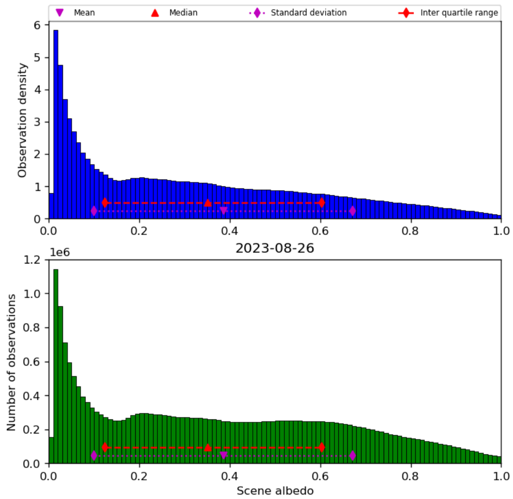
Figure 34: Histogram of “Scene albedo” for 2023-08-25 to 2023-08-27
