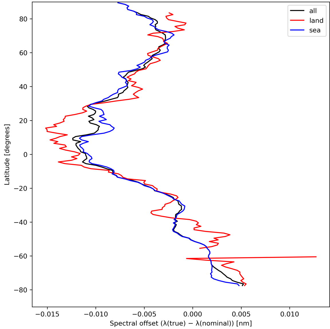
Figure 28: Zonal average of “Spectral offset ( \lambda(\text{true}) - \lambda(\text{nominal}) )” for 2023-08-25 to 2023-08-27.
