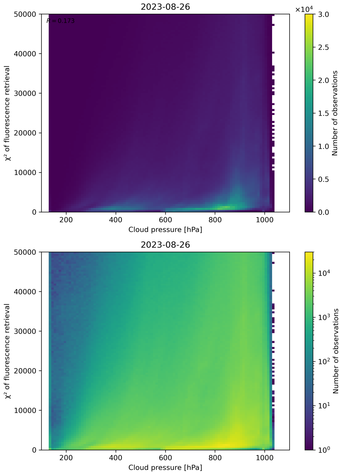
Figure 86: Scatter density plot of “Cloud pressure” against “ \chi^2 of fluorescence retrieval” for 2023-08-25 to 2023-08-27.
