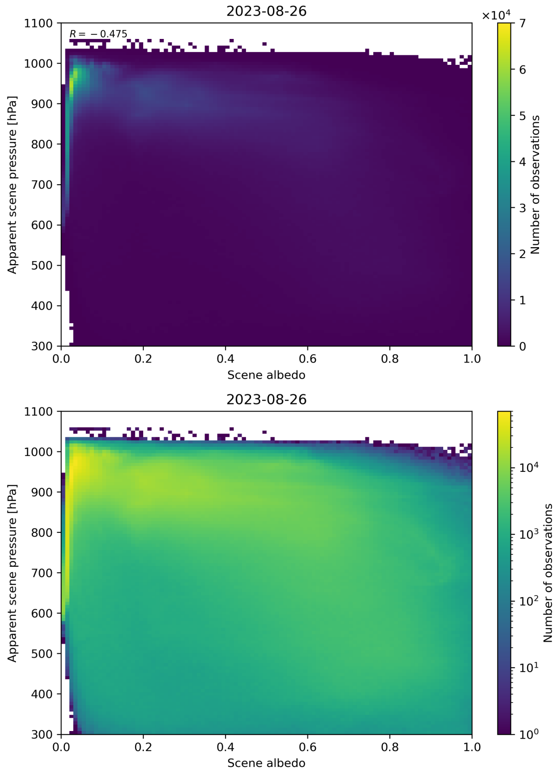
Figure 111: Scatter density plot of “Scene albedo” against “Apparent scene pressure” for 2023-08-25 to 2023-08-27.
