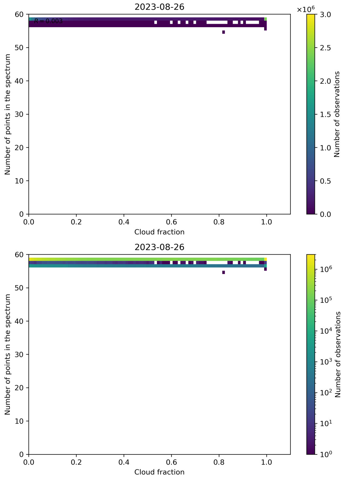
Figure 81: Scatter density plot of “Cloud fraction” against “Number of points in the spectrum” for 2023-08-25 to 2023-08-27.
