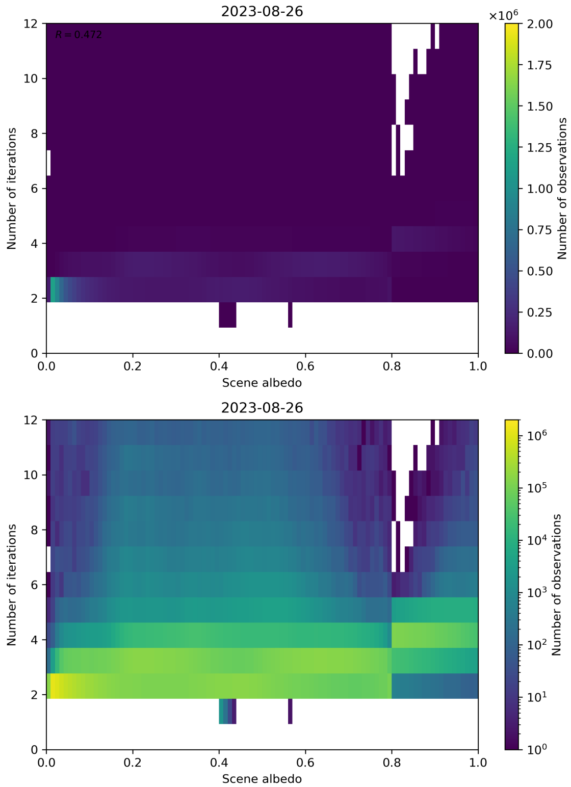
Figure 115: Scatter density plot of “Scene albedo” against “Number of iterations” for 2023-08-25 to 2023-08-27.
