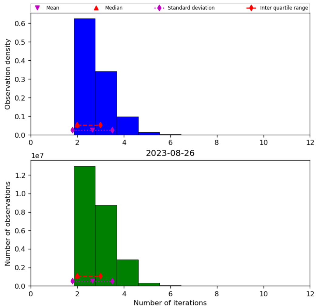
Figure 39: Histogram of “Number of iterations” for 2023-08-25 to 2023-08-27
