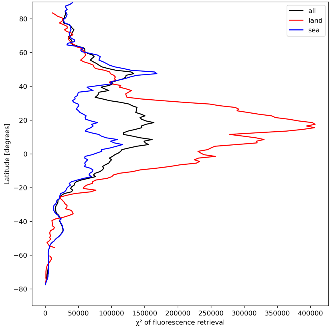
Figure 25: Zonal average of “ \chi^2 of fluorescence retrieval” for 2023-08-25 to 2023-08-27.
