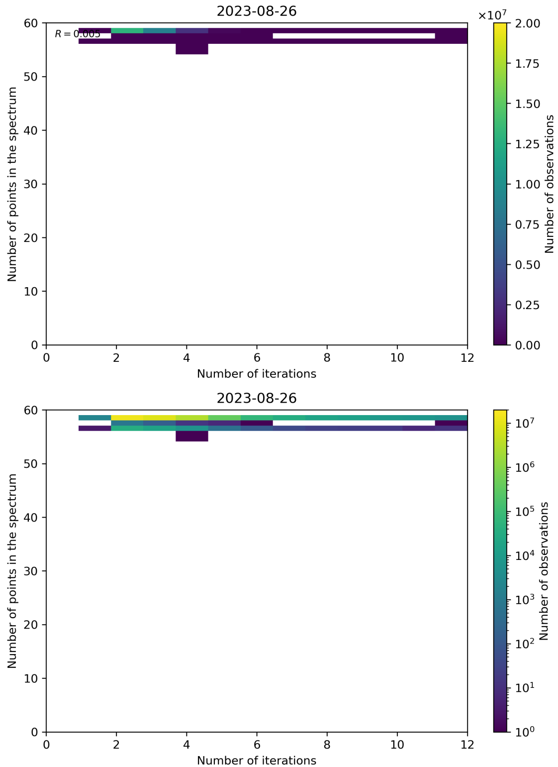
Figure 108: Scatter density plot of “Number of iterations” against “Number of points in the spectrum” for 2023-08-25 to 2023-08-27.
