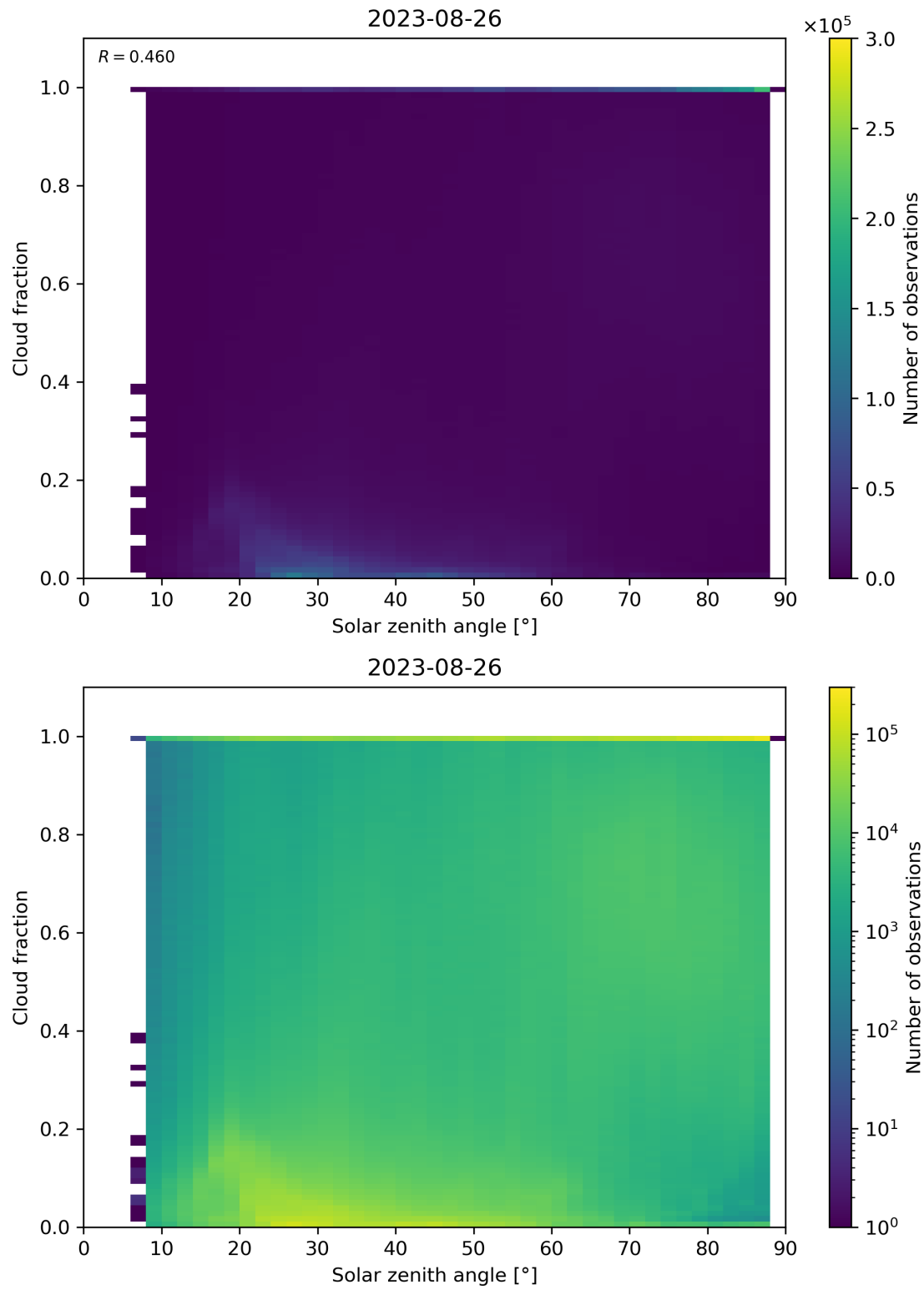
Figure 121: Scatter density plot of “Solar zenith angle” against “Cloud fraction” for 2023-08-25 to 2023-08-27.
