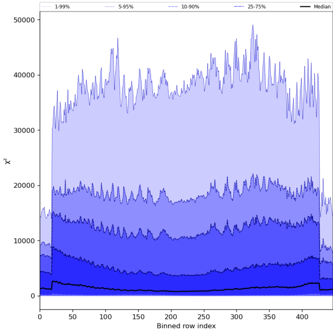
Figure 55: Along track statistics of “ \chi^2 ” for 2023-08-25 to 2023-08-27
