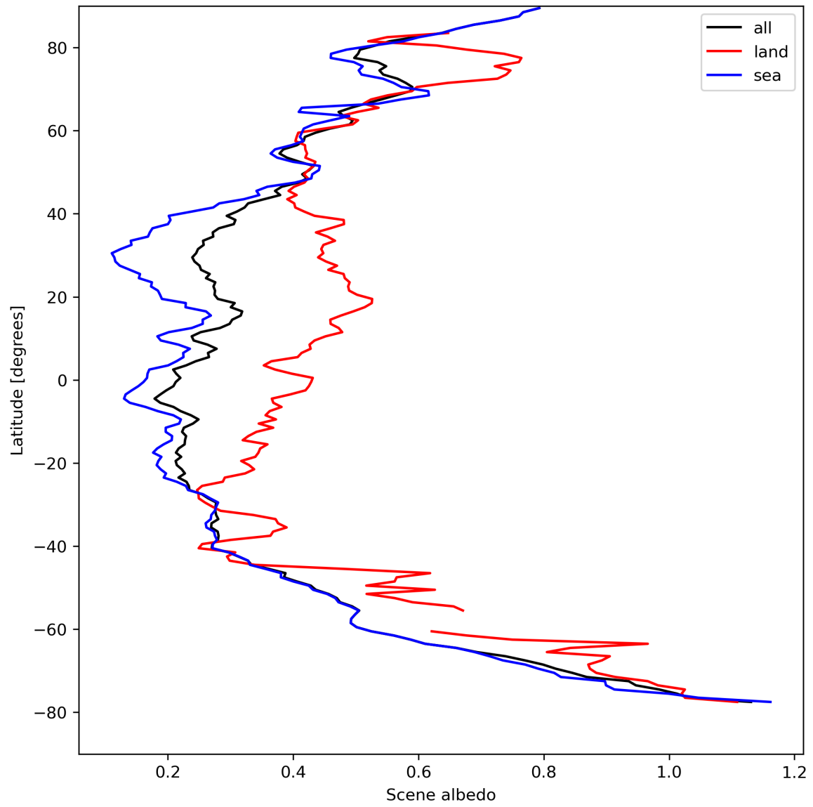
Figure 17: Zonal average of “Scene albedo” for 2023-08-25 to 2023-08-27.
