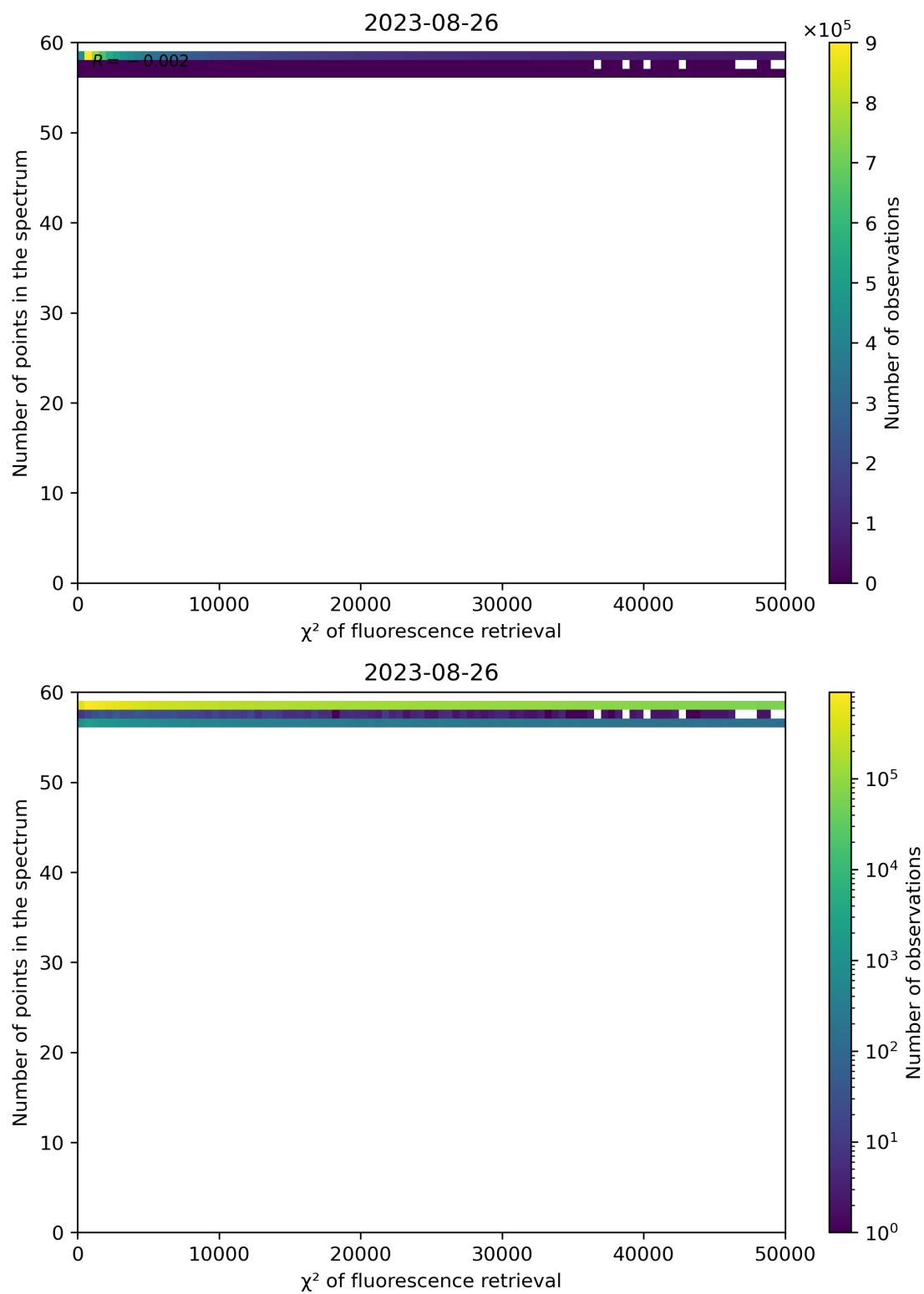
Figure 71: Scatter density plot of " \chi^2 of fluorescence retrieval" against "Number of points in the spectrum" for 2023-08-25 to 2023-08-27.
