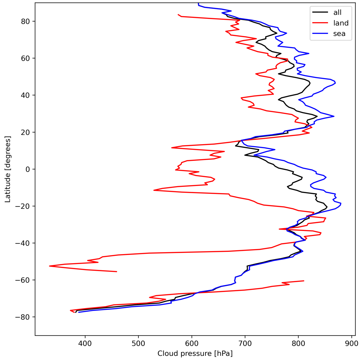
Figure 13: Zonal average of “Cloud pressure” for 2023-08-25 to 2023-08-27.
