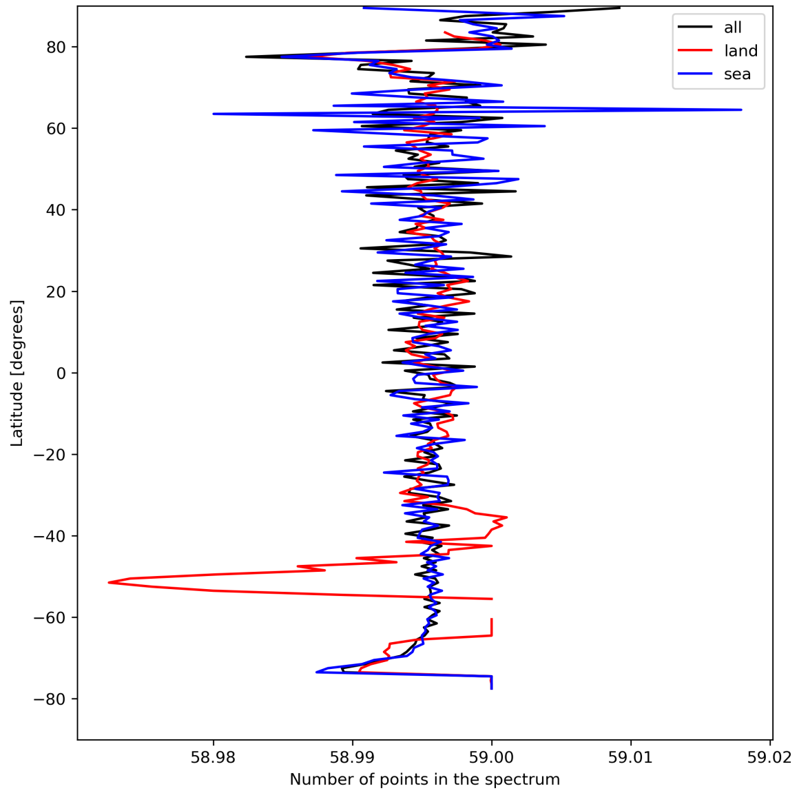
Figure 27: Zonal average of “Number of points in the spectrum” for 2023-08-25 to 2023-08-27.
