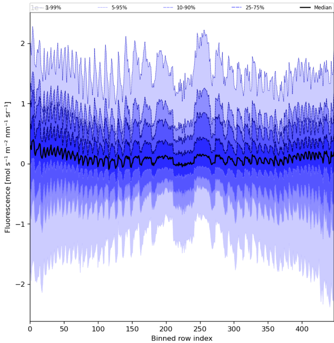
Figure 57: Along track statistics of “Fluorescence” for 2023-08-25 to 2023-08-27
