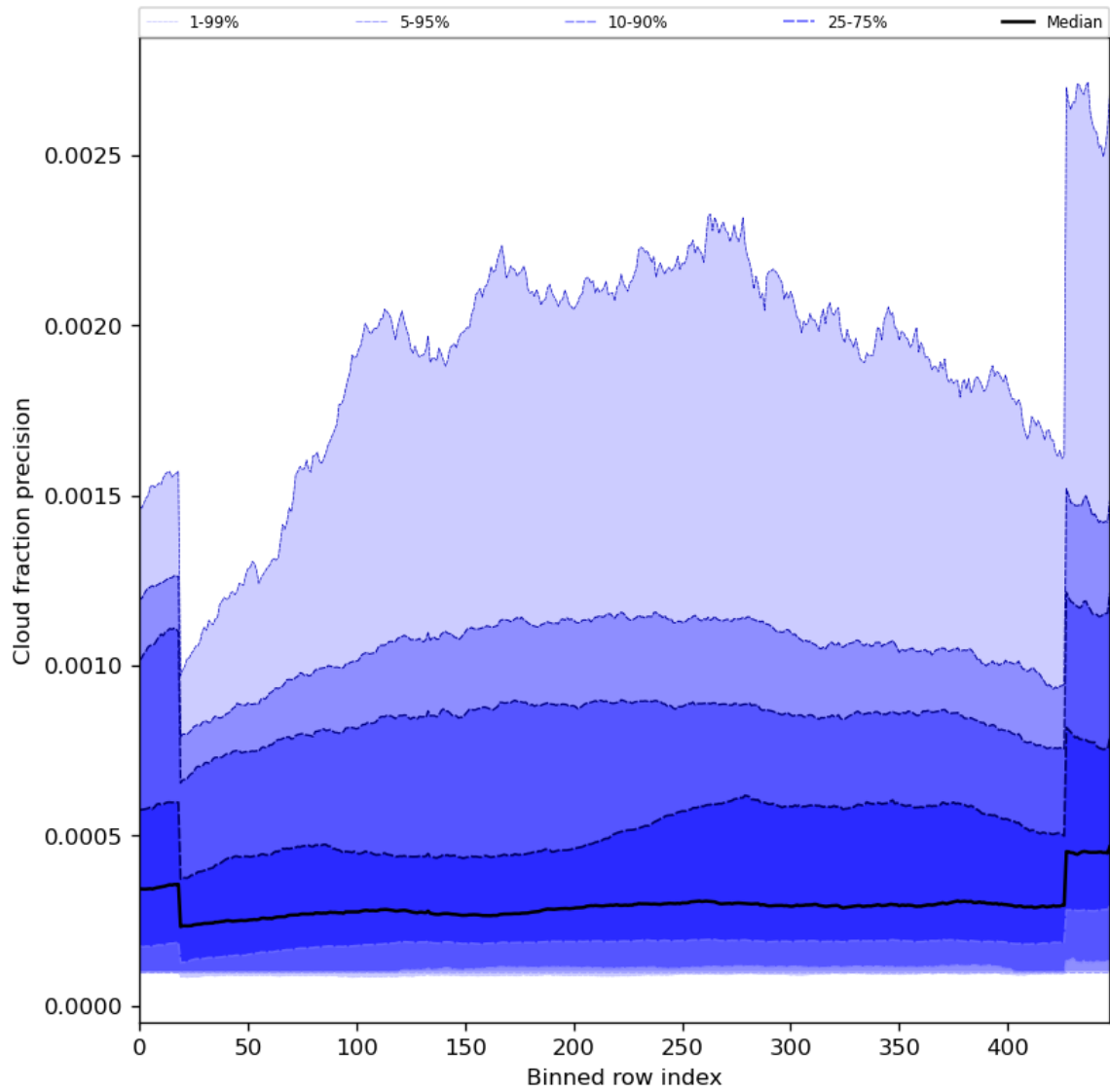
Figure 50: Along track statistics of “Cloud fraction precision” for 2023-08-25 to 2023-08-27
