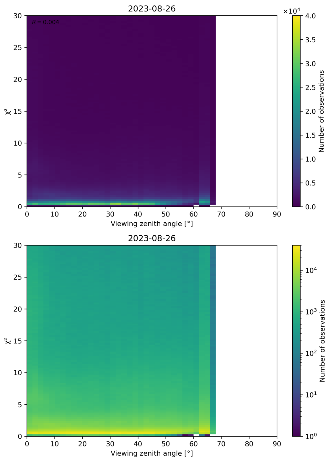
Figure 130: Scatter density plot of “Viewing zenith angle” against “ \chi^2 ” for 2023-08-25 to 2023-08-27.
