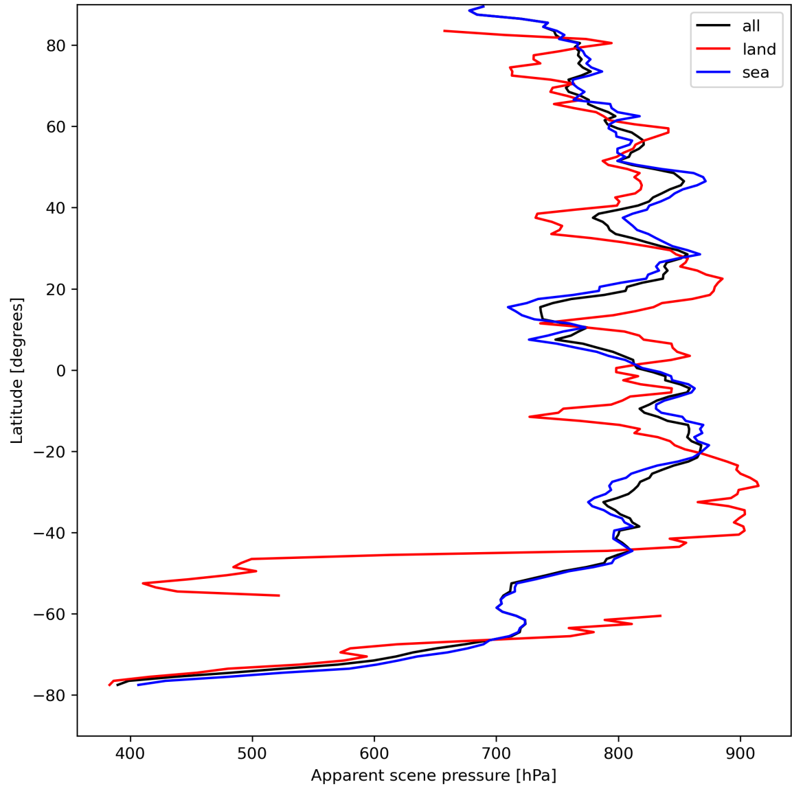
Figure 19: Zonal average of “Apparent scene pressure” for 2023-08-25 to 2023-08-27.
