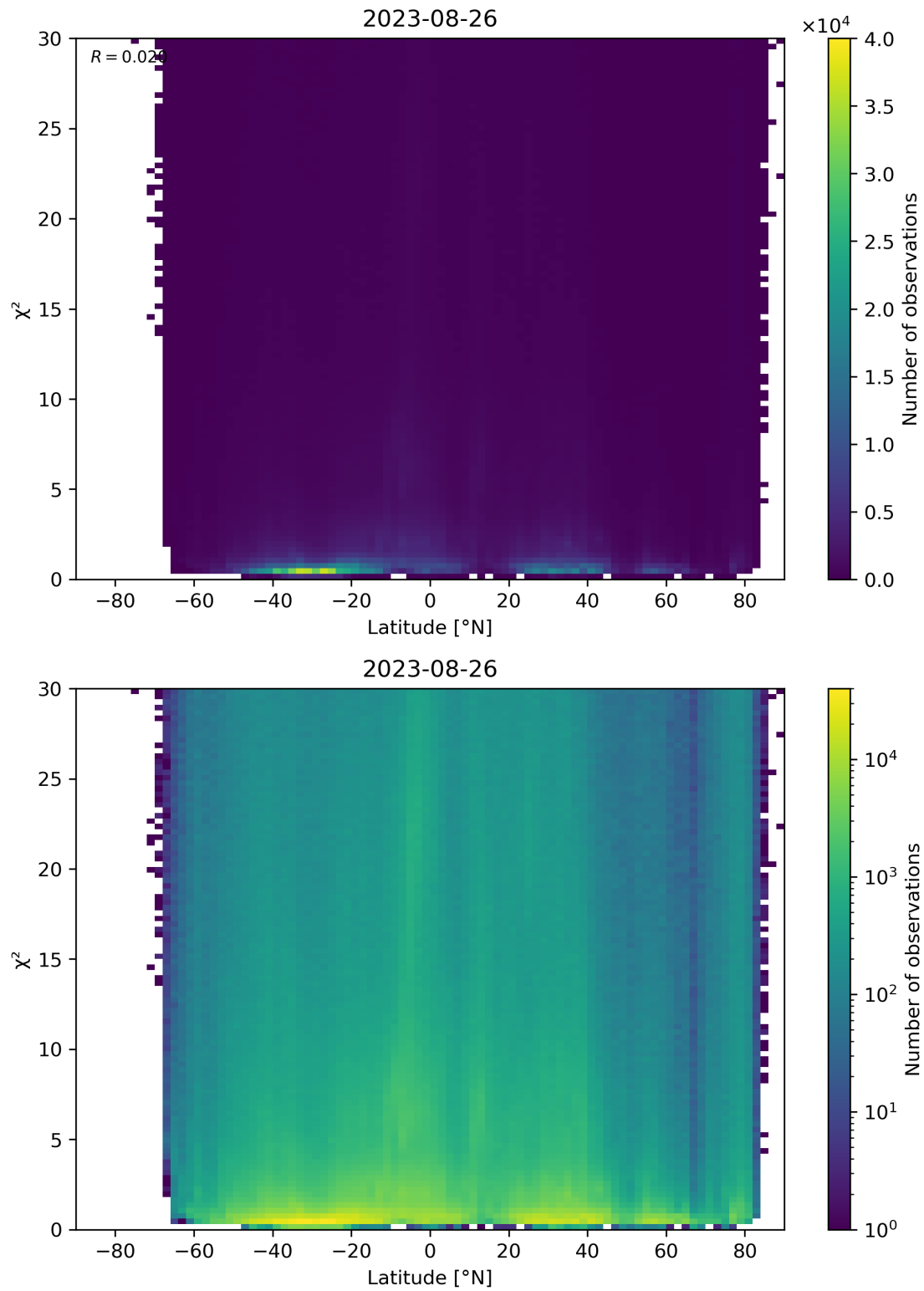
Figure 97: Scatter density plot of “Latitude” against “ \chi^2 ” for 2023-08-25 to 2023-08-27.
