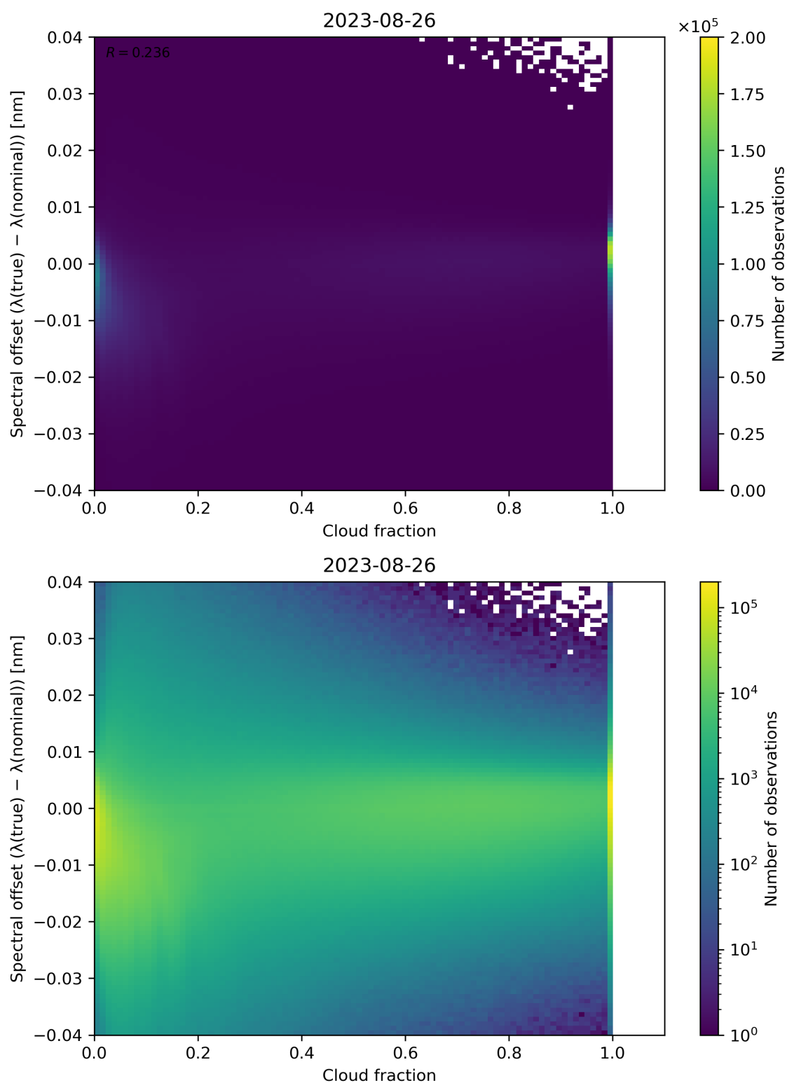
Figure 83: Scatter density plot of “Cloud fraction” against “Spectral offset ( \lambda(\text{true}) - \lambda(\text{nominal}) )” for 2023-08-25 to 2023-08-27.
