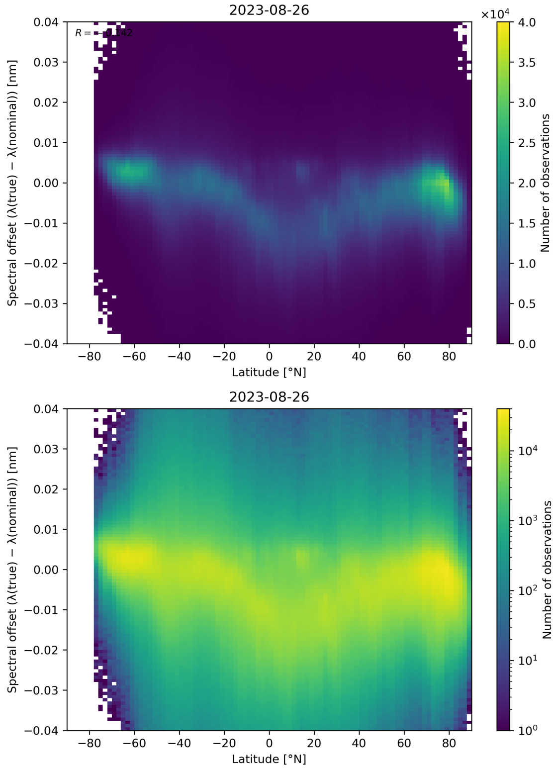
Figure 105: Scatter density plot of “Latitude” against “Spectral offset ( \lambda(\text{true}) - \lambda(\text{nominal}) )” for 2023-08-25 to 2023-08-27.
