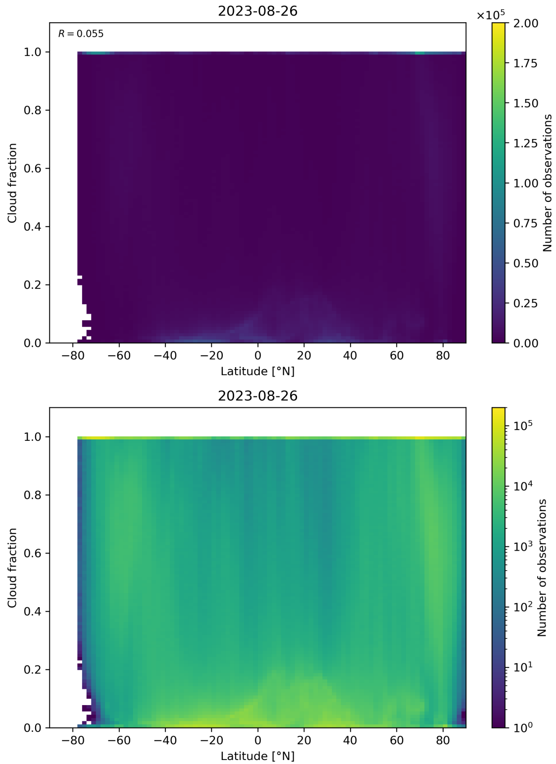
Figure 99: Scatter density plot of “Latitude” against “Cloud fraction” for 2023-08-25 to 2023-08-27.
