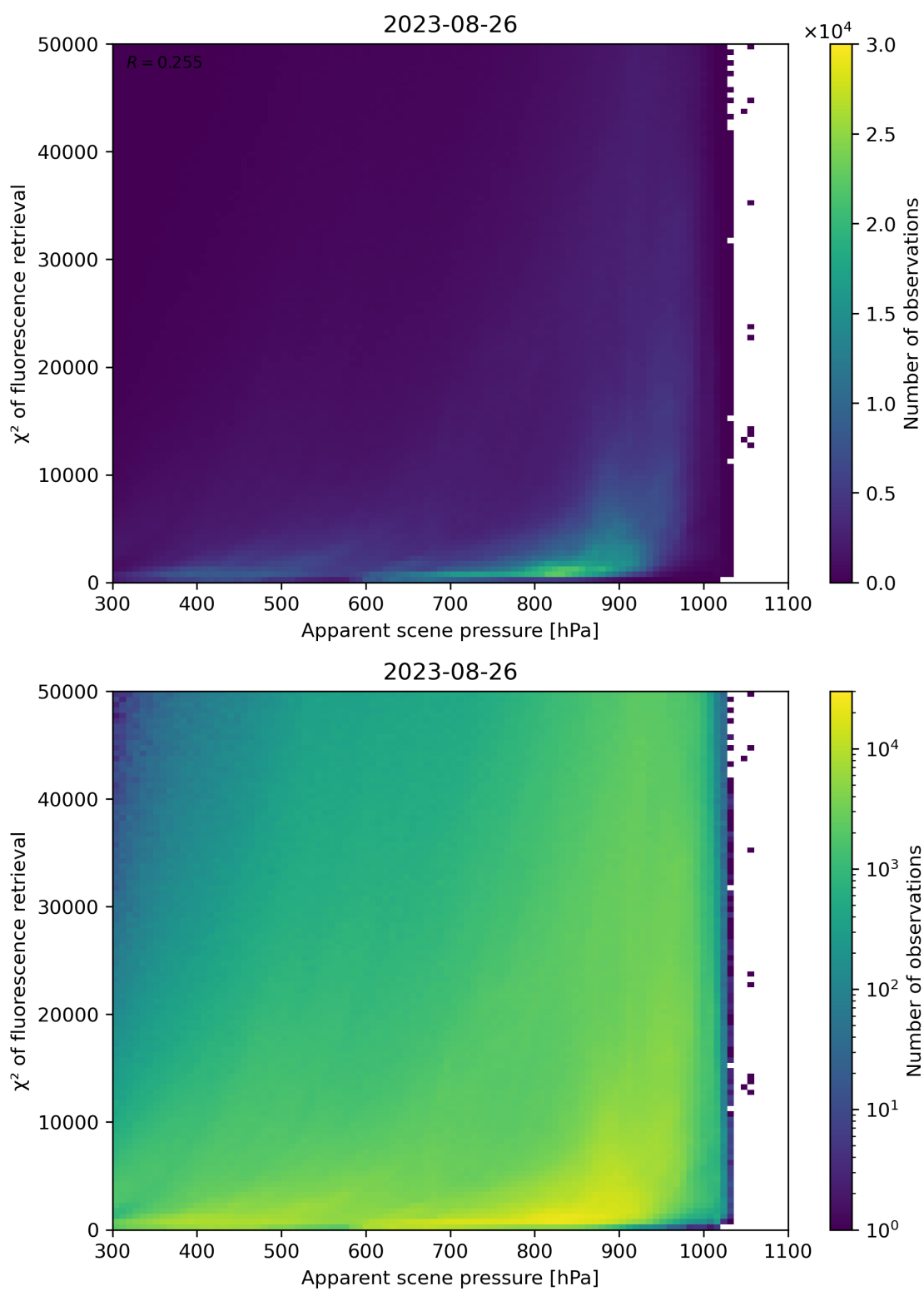
Figure 64: Scatter density plot of “Apparent scene pressure” against “ \chi^2 of fluorescence retrieval” for 2023-08-25 to 2023-08-27.
