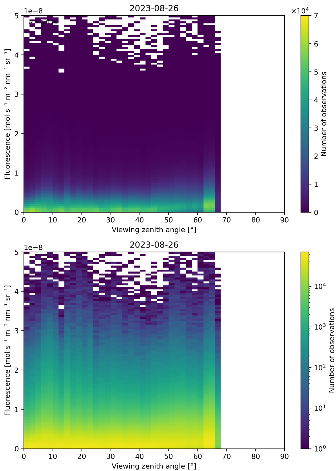
Figure 134: Scatter density plot of “Viewing zenith angle” against “Fluorescence” for 2023-08-25 to 2023-08-27.
