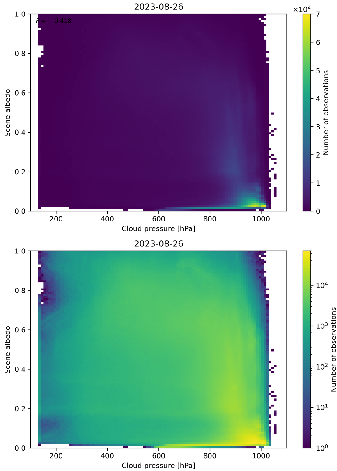
Figure 91: Scatter density plot of “Cloud pressure” against “Scene albedo” for 2023-08-25 to 2023-08-27.
