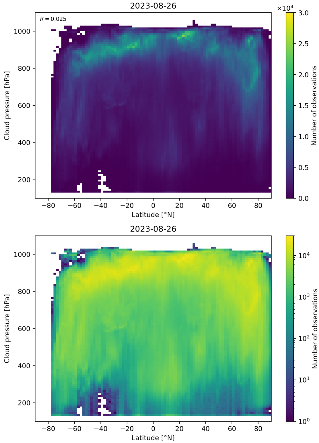
Figure 100: Scatter density plot of “Latitude” against “Cloud pressure” for 2023-08-25 to 2023-08-27.
