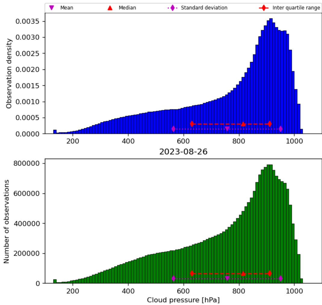
Figure 30: Histogram of “Cloud pressure” for 2023-08-25 to 2023-08-27
