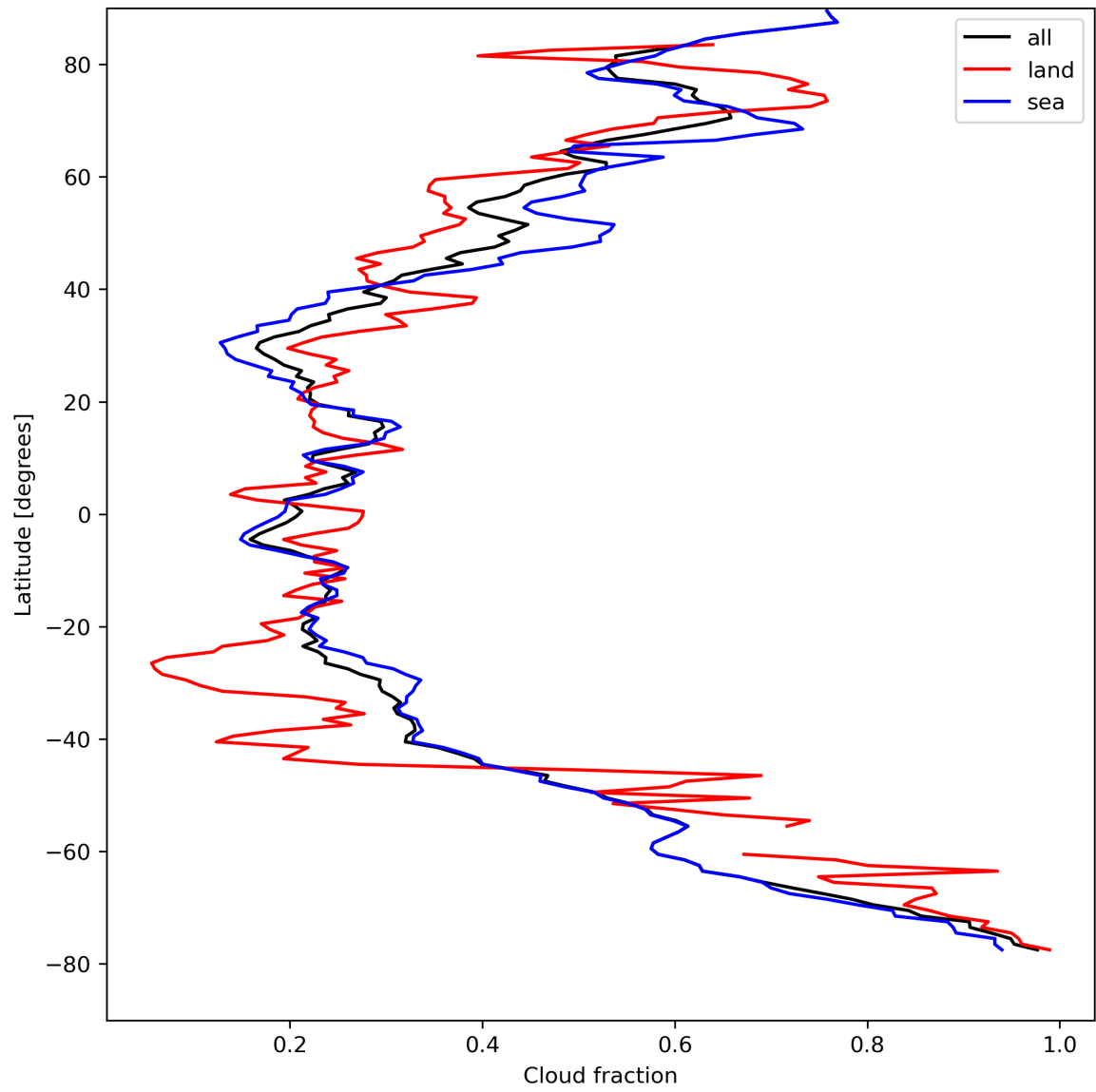
Figure 15: Zonal average of “Cloud fraction” for 2023-08-25 to 2023-08-27.
