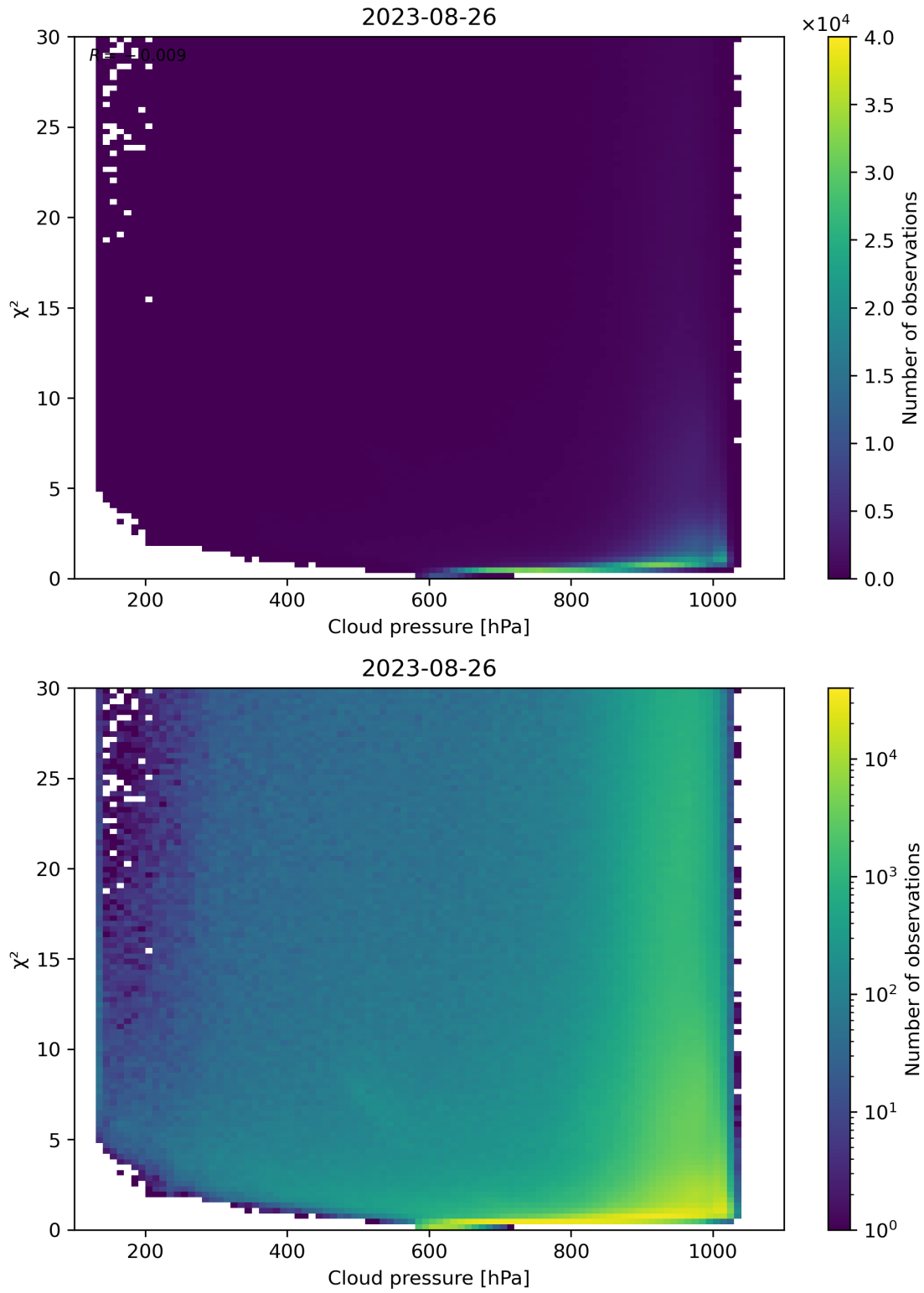
Figure 85: Scatter density plot of “Cloud pressure” against “ \chi^2 ” for 2023-08-25 to 2023-08-27.
