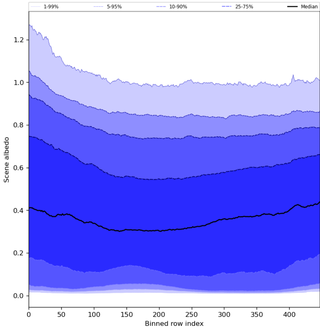
Figure 51: Along track statistics of “Scene albedo” for 2023-08-25 to 2023-08-27
