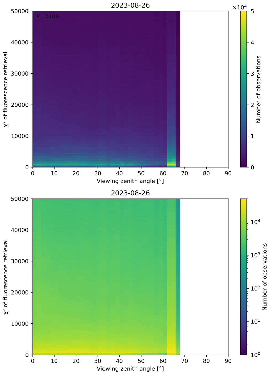
Figure 131: Scatter density plot of “Viewing zenith angle” against “ \chi^2 of fluorescence retrieval” for 2023-08-25 to 2023-08-27.
