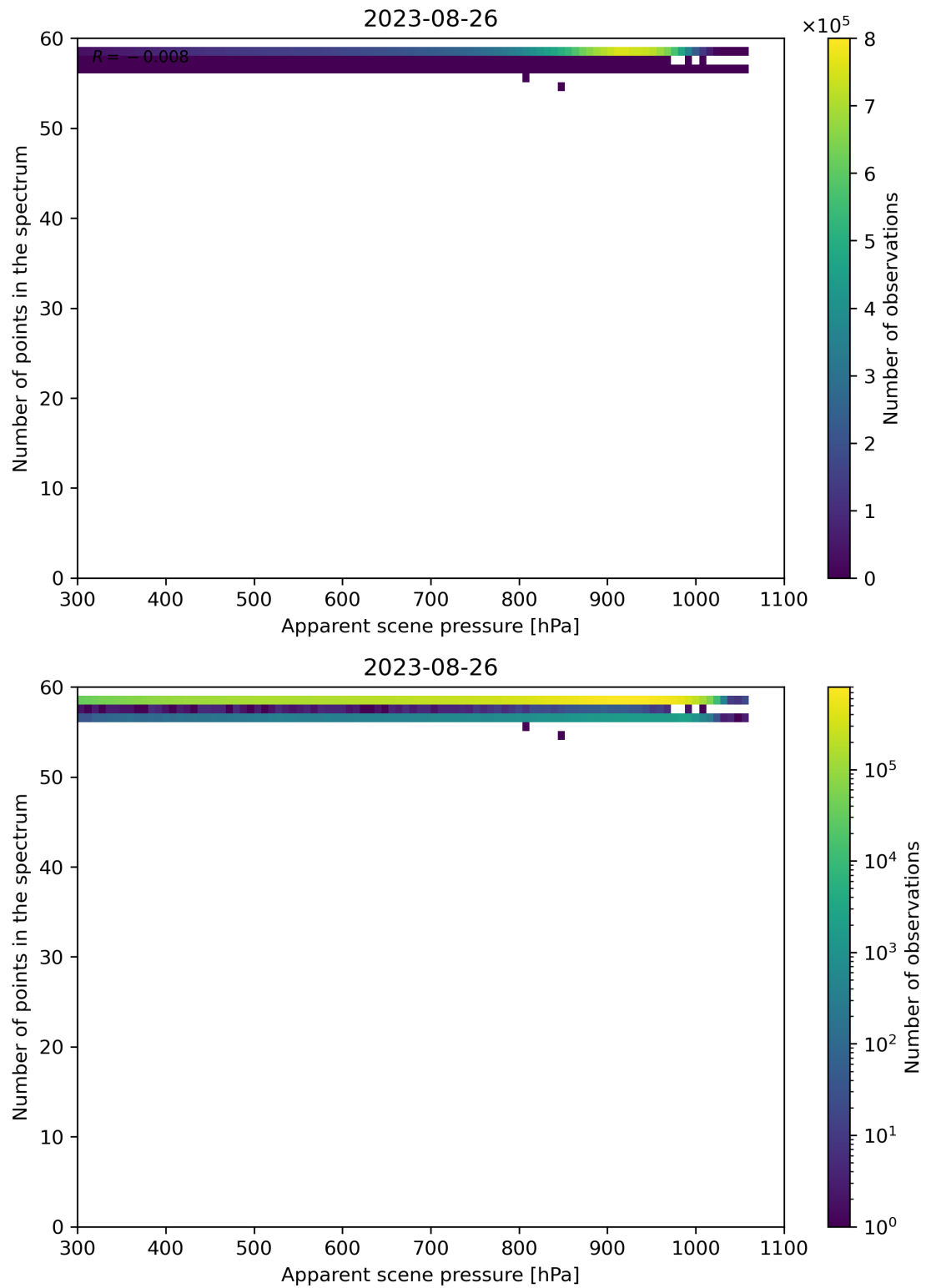
Figure 67: Scatter density plot of “Apparent scene pressure” against “Number of points in the spectrum” for 2023-08-25 to 2023-08-27.
