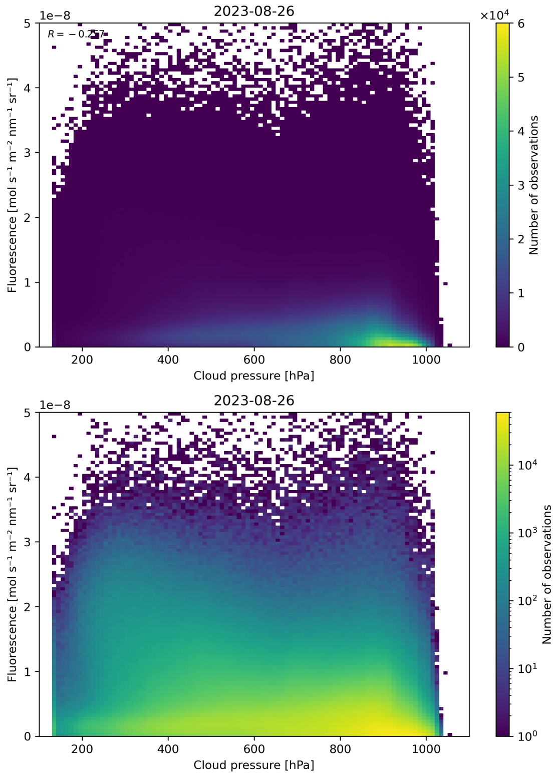
Figure 88: Scatter density plot of “Cloud pressure” against “Fluorescence” for 2023-08-25 to 2023-08-27.
