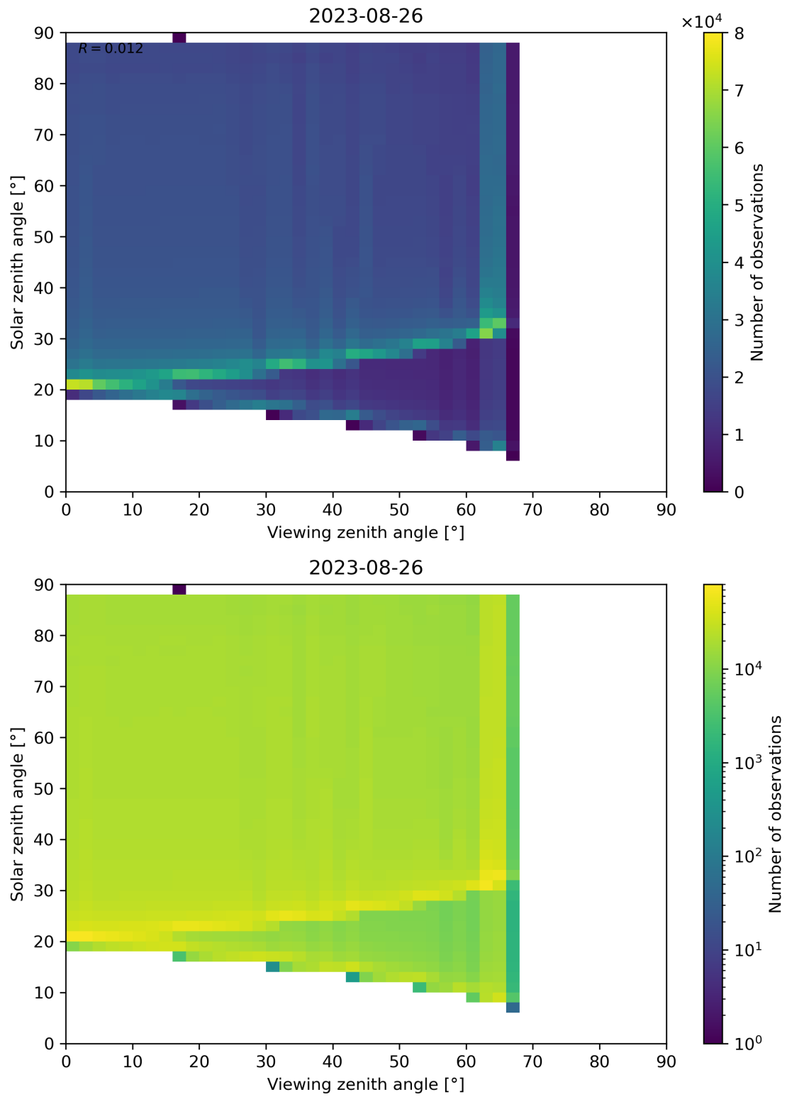
Figure 139: Scatter density plot of “Viewing zenith angle” against “Solar zenith angle” for 2023-08-25 to 2023-08-27.
