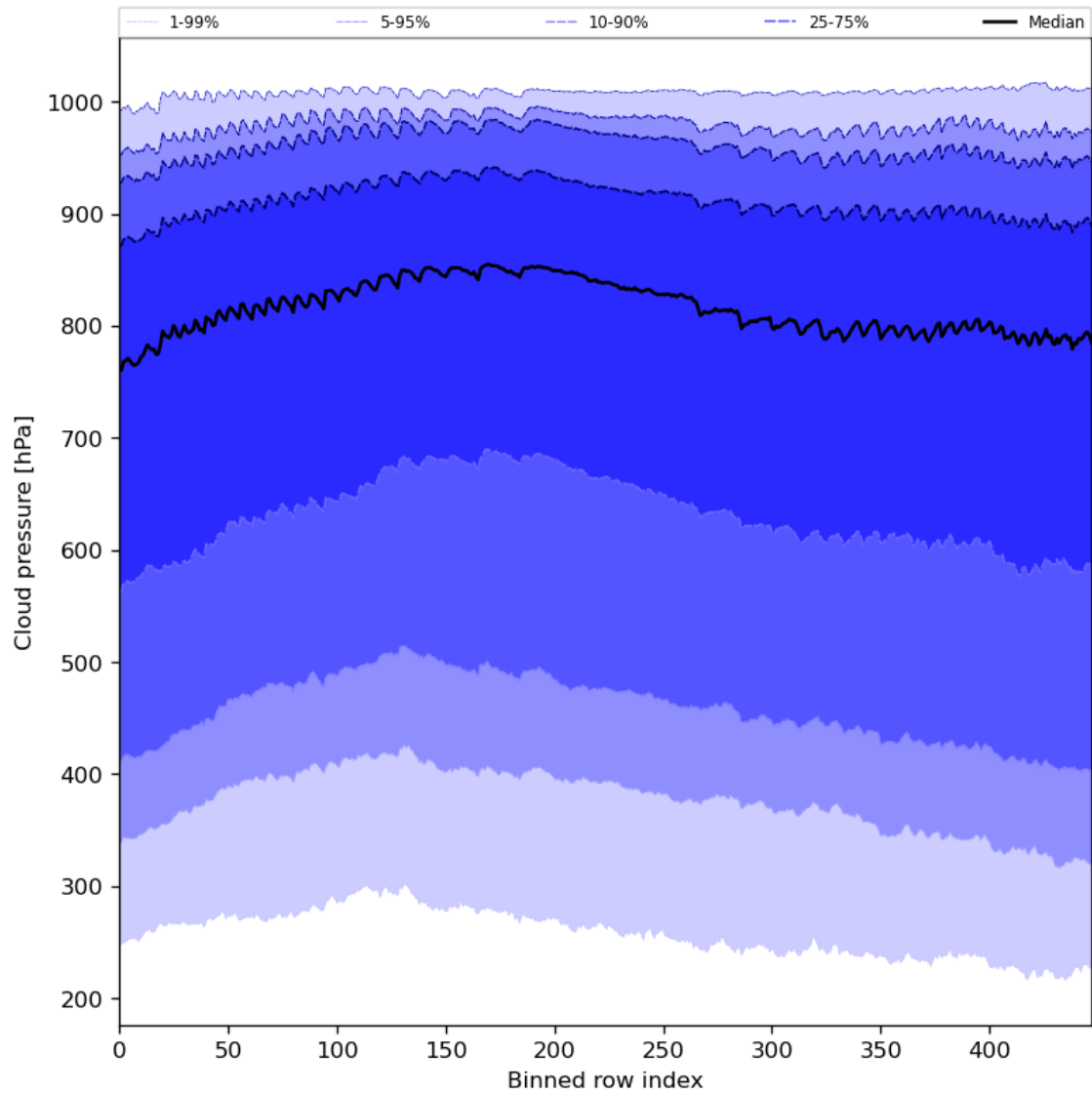
Figure 47: Along track statistics of “Cloud pressure” for 2023-08-25 to 2023-08-27
