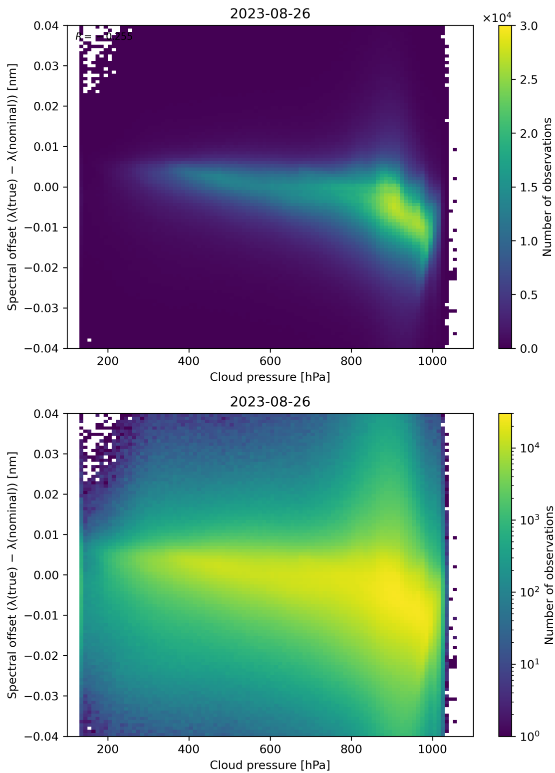
Figure 92: Scatter density plot of “Cloud pressure” against “Spectral offset ( \lambda(\text{true}) - \lambda(\text{nominal}) )” for 2023-08-25 to 2023-08-27.
