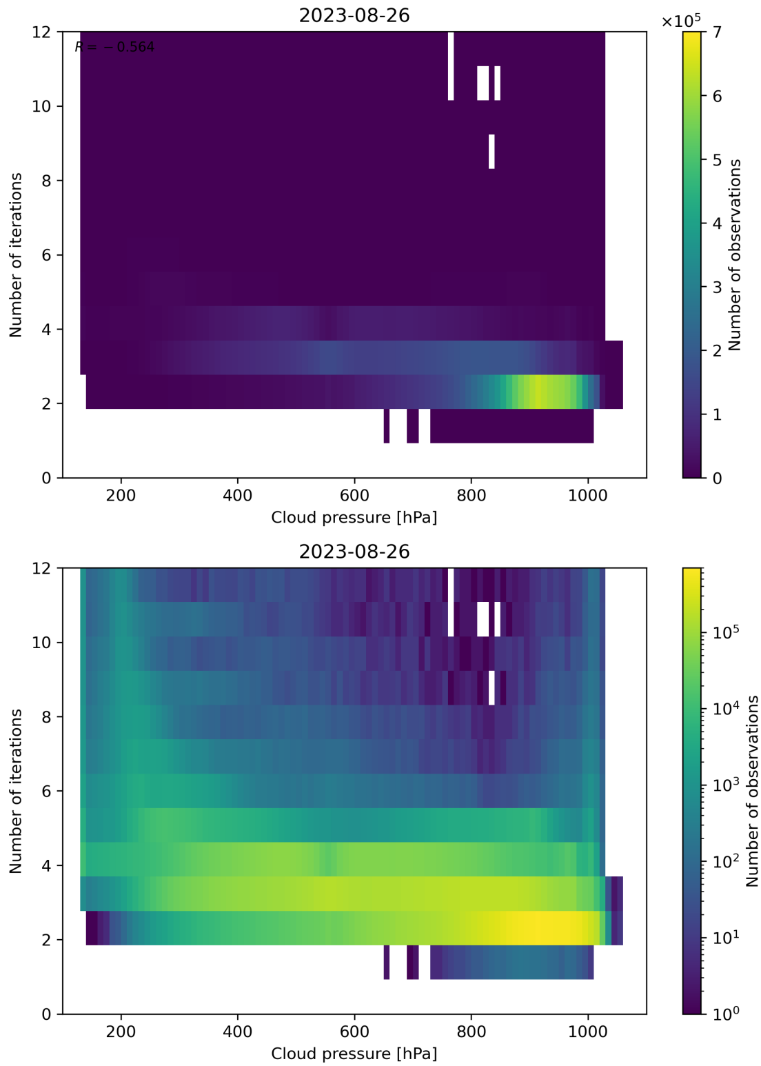
Figure 89: Scatter density plot of “Cloud pressure” against “Number of iterations” for 2023-08-25 to 2023-08-27.
