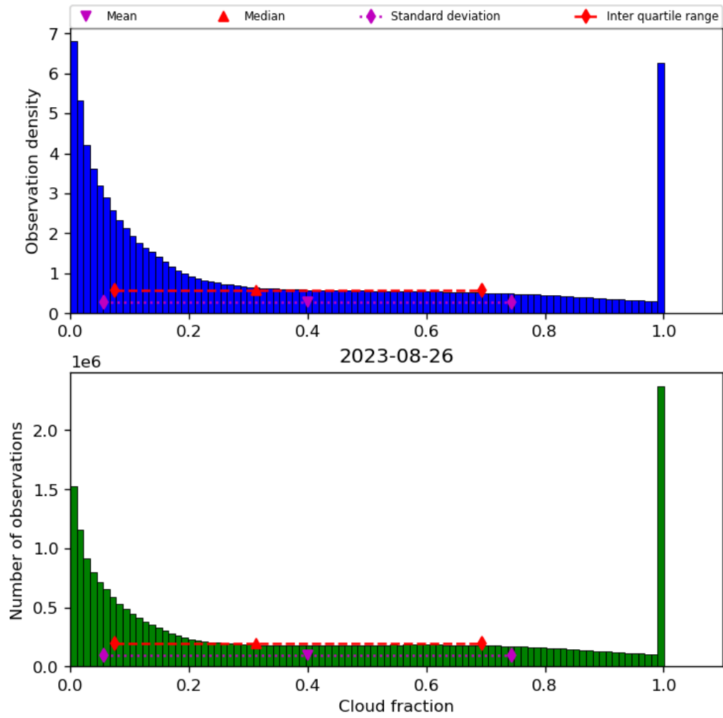
Figure 32: Histogram of “Cloud fraction” for 2023-08-25 to 2023-08-27
