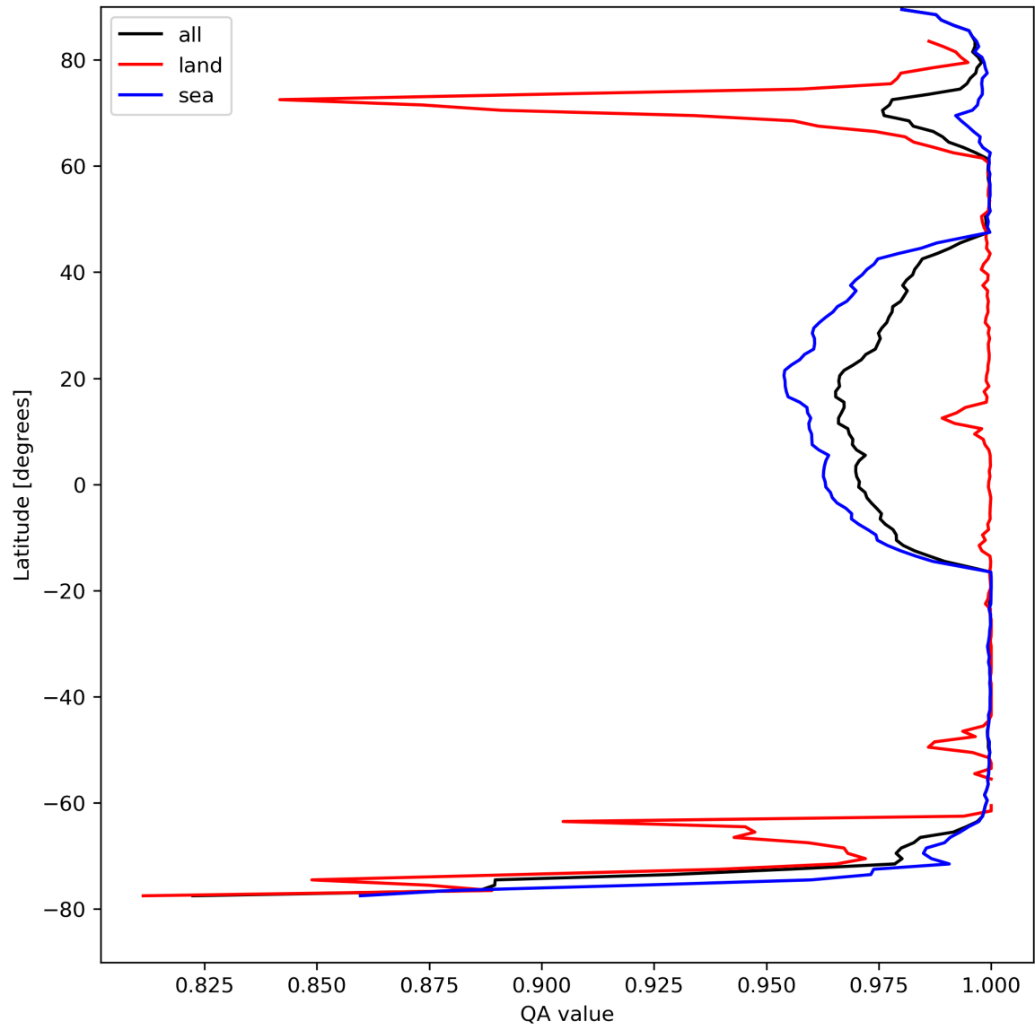
Figure 12: Zonal average of “QA value” for 2023-08-25 to 2023-08-27.
