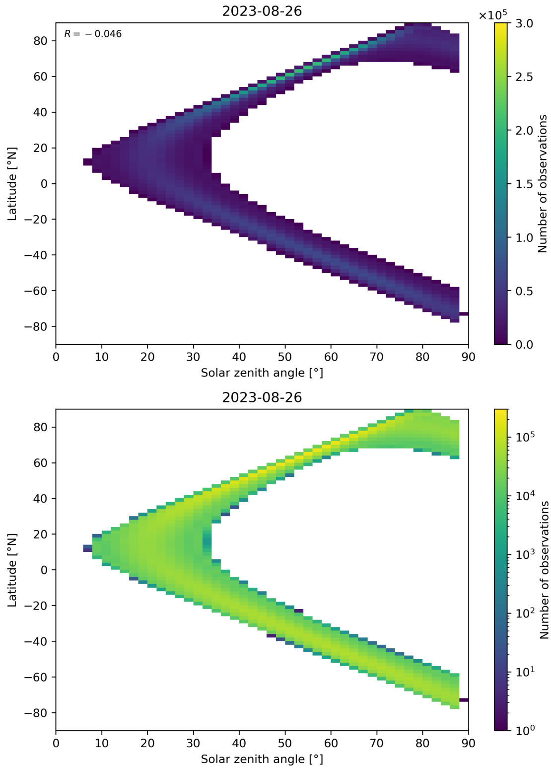
Figure 124: Scatter density plot of “Solar zenith angle” against “Latitude” for 2023-08-25 to 2023-08-27.
