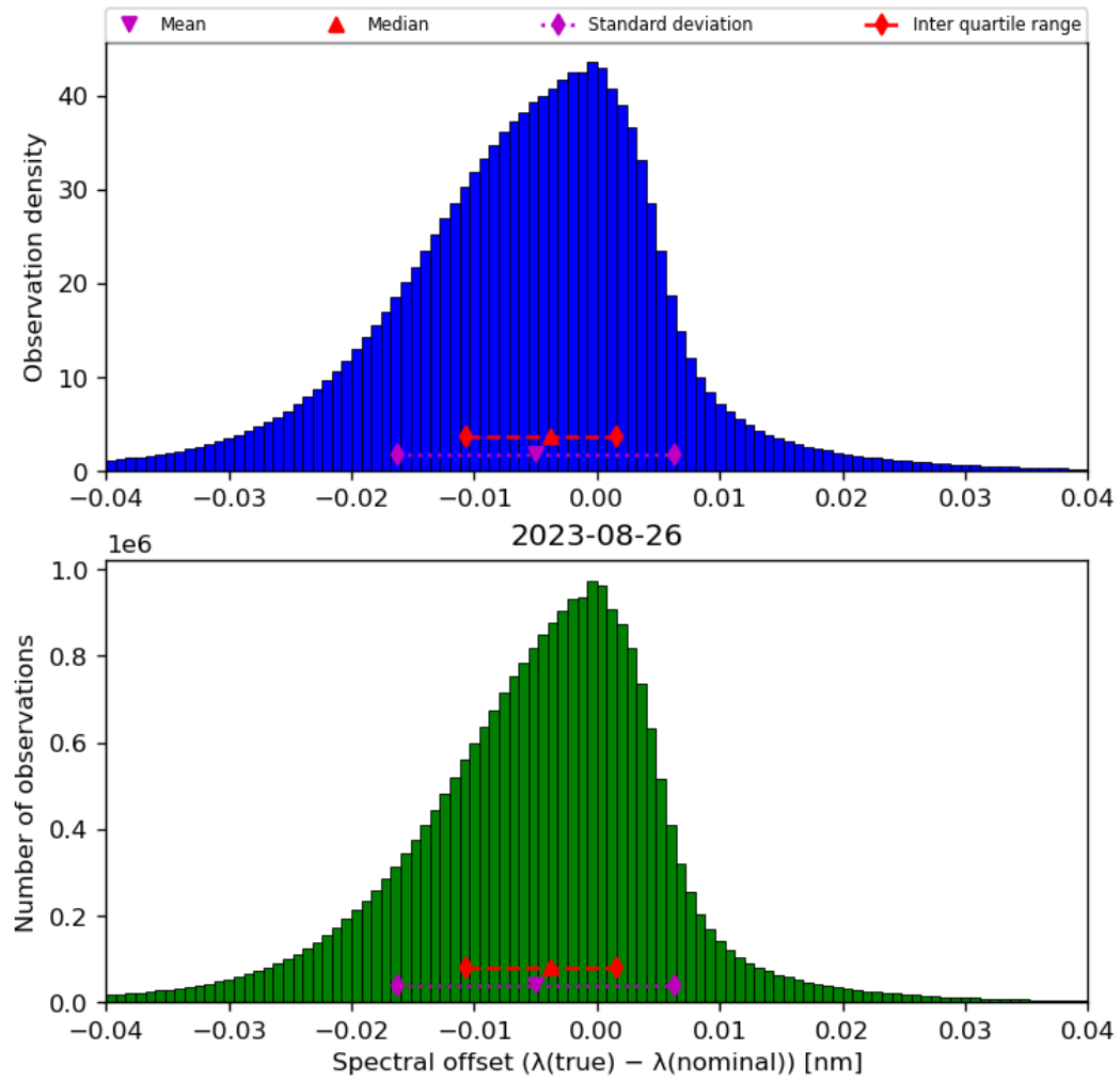
Figure 45: Histogram of “Spectral offset ( \lambda(\text{true}) - \lambda(\text{nominal}) )” for 2023-08-25 to 2023-08-27
