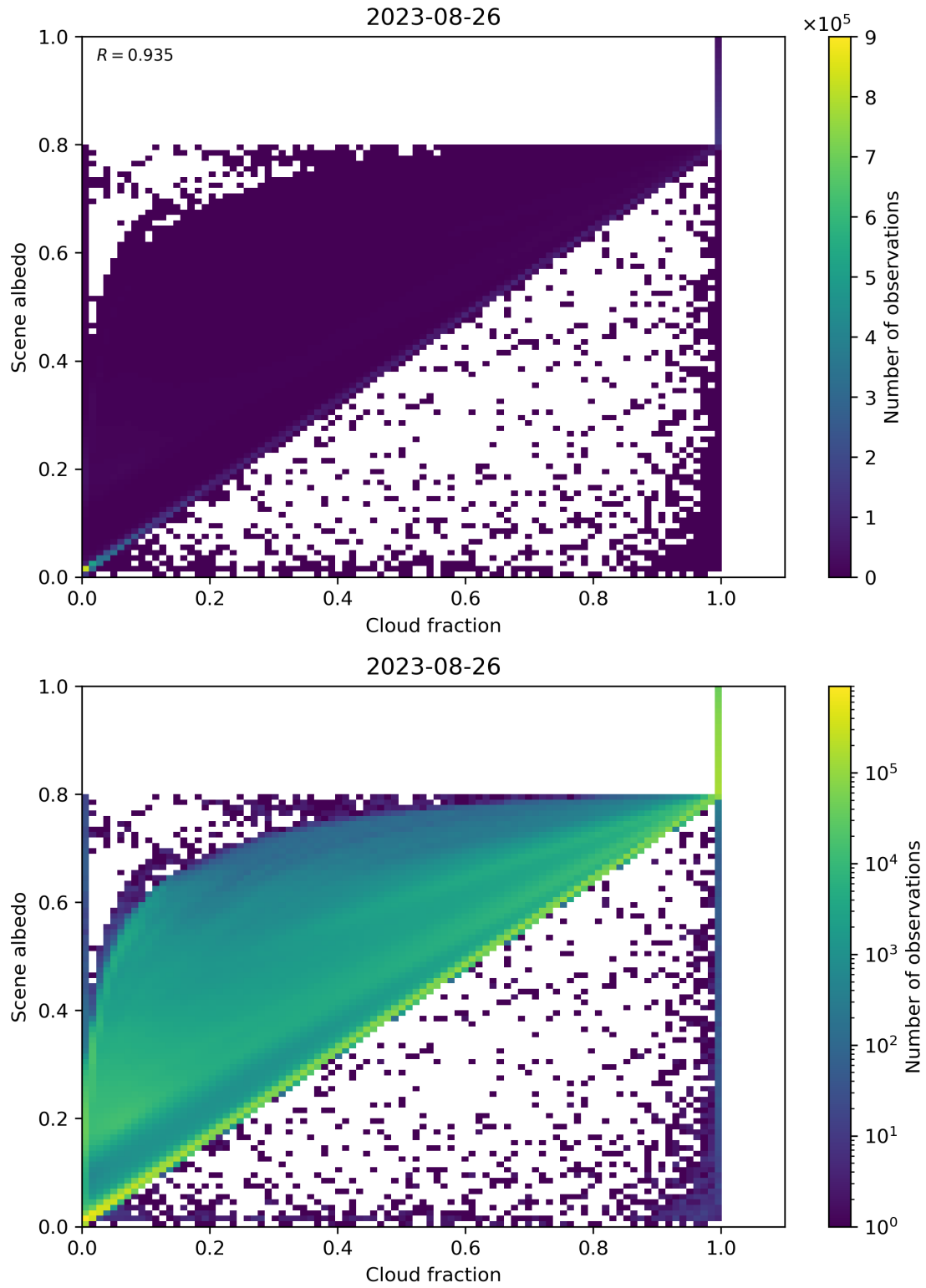
Figure 82: Scatter density plot of “Cloud fraction” against “Scene albedo” for 2023-08-25 to 2023-08-27.
