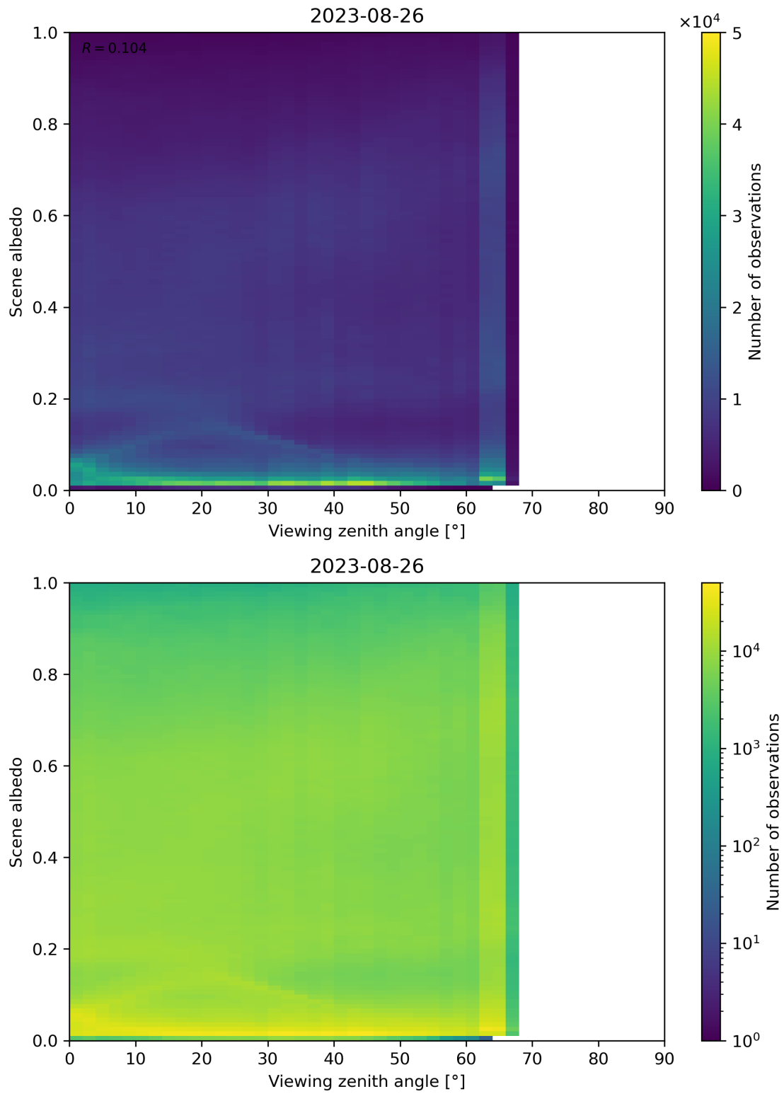
Figure 138: Scatter density plot of “Viewing zenith angle” against “Scene albedo” for 2023-08-25 to 2023-08-27.
