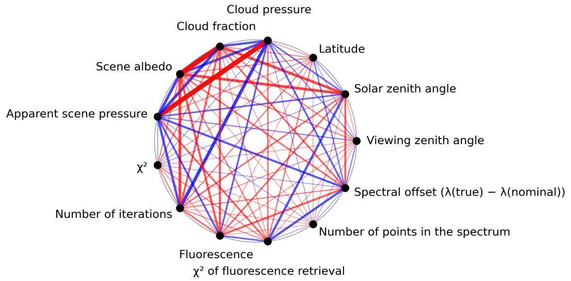
Figure 1: Map of correlation graph for 2023-08-25 to 2023-08-27.
