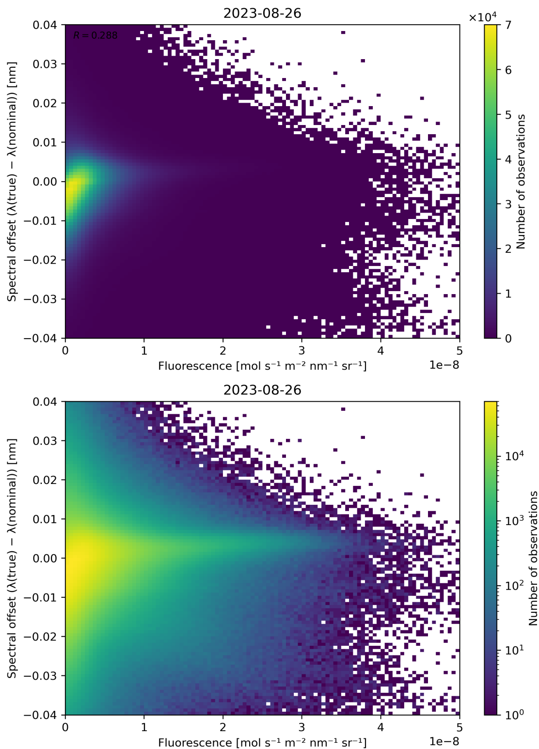
Figure 95: Scatter density plot of “Fluorescence” against “Spectral offset ( \lambda(\text{true}) - \lambda(\text{nominal}) )” for 2023-08-25 to 2023-08-27.
