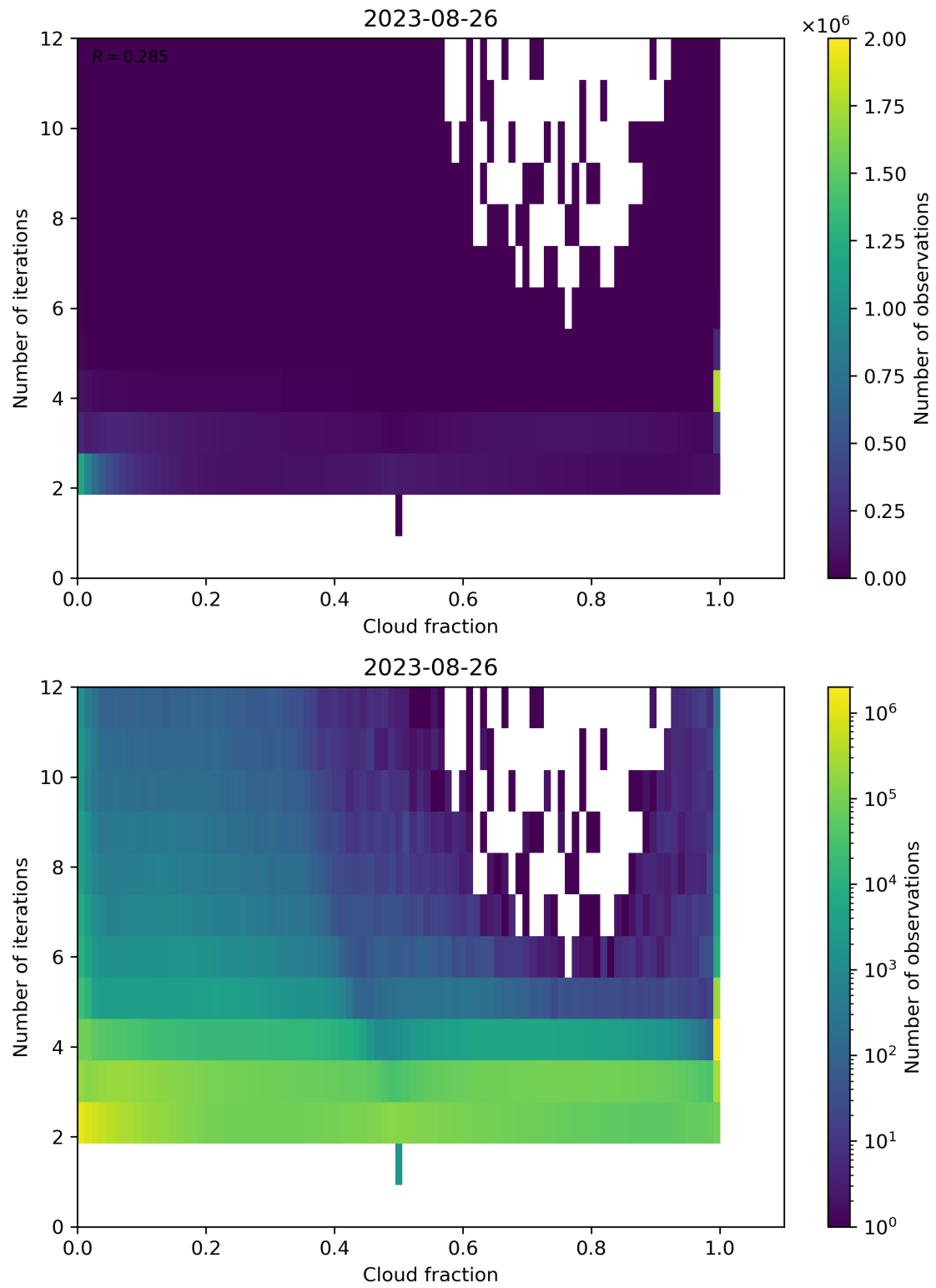
Figure 80: Scatter density plot of “Cloud fraction” against “Number of iterations” for 2023-08-25 to 2023-08-27.
