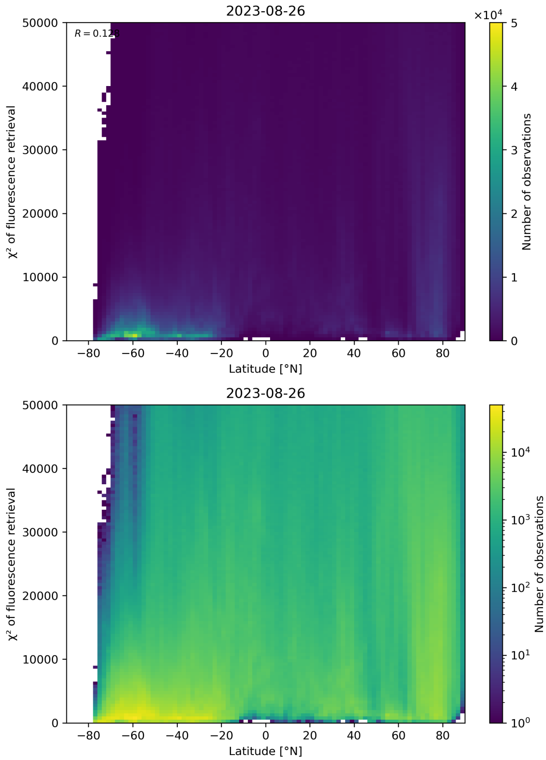
Figure 98: Scatter density plot of “Latitude” against “ \chi^2 of fluorescence retrieval” for 2023-08-25 to 2023-08-27.
