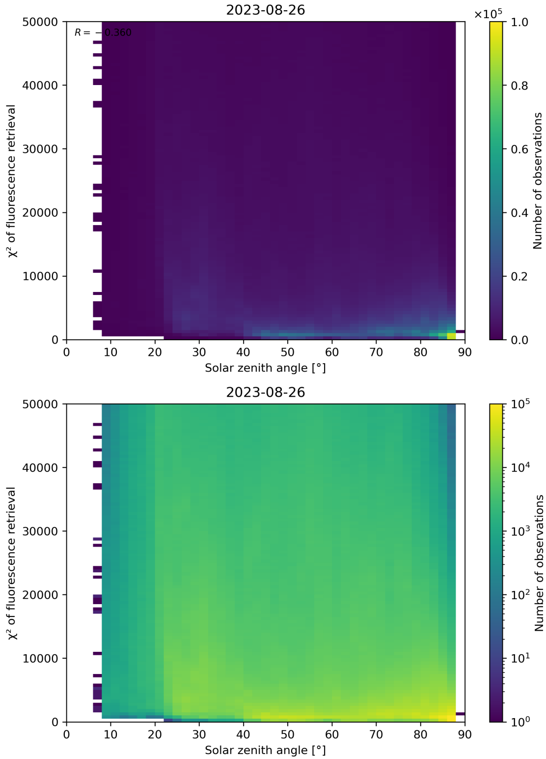
Figure 120: Scatter density plot of “Solar zenith angle” against “ \chi^2 of fluorescence retrieval” for 2023-08-25 to 2023-08-27.
