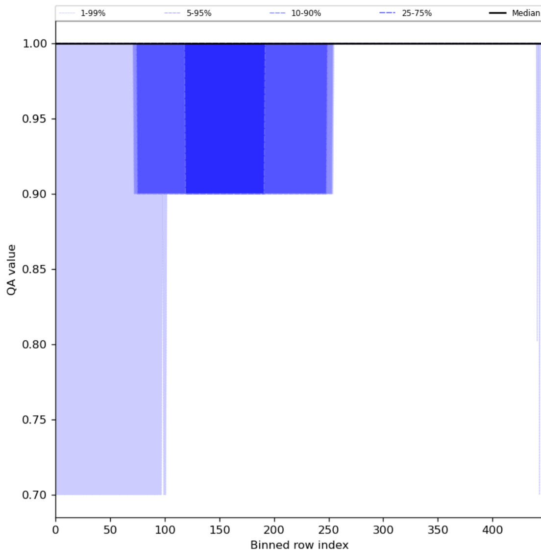
Figure 46: Along track statistics of “QA value” for 2023-08-25 to 2023-08-27
