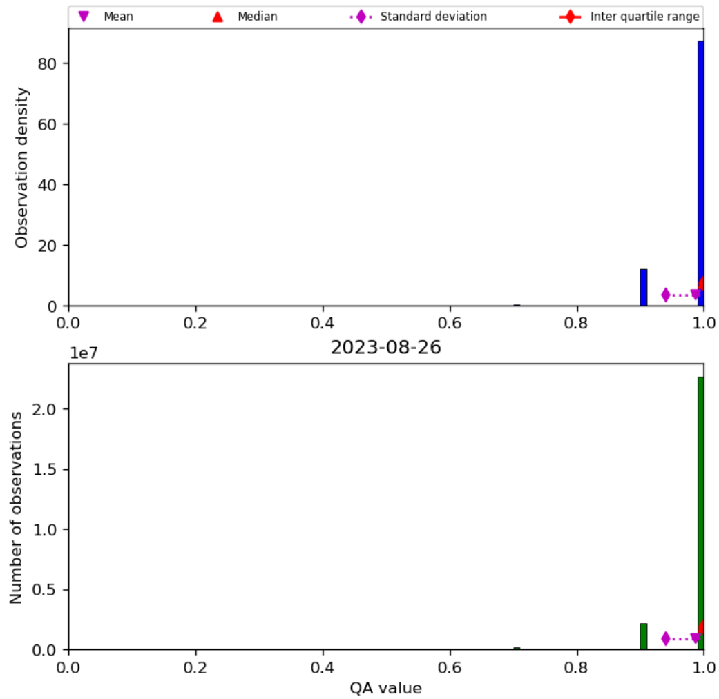
Figure 29: Histogram of “QA value” for 2023-08-25 to 2023-08-27
