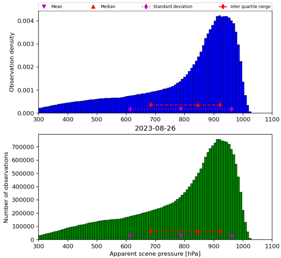
Figure 36: Histogram of “Apparent scene pressure” for 2023-08-25 to 2023-08-27
