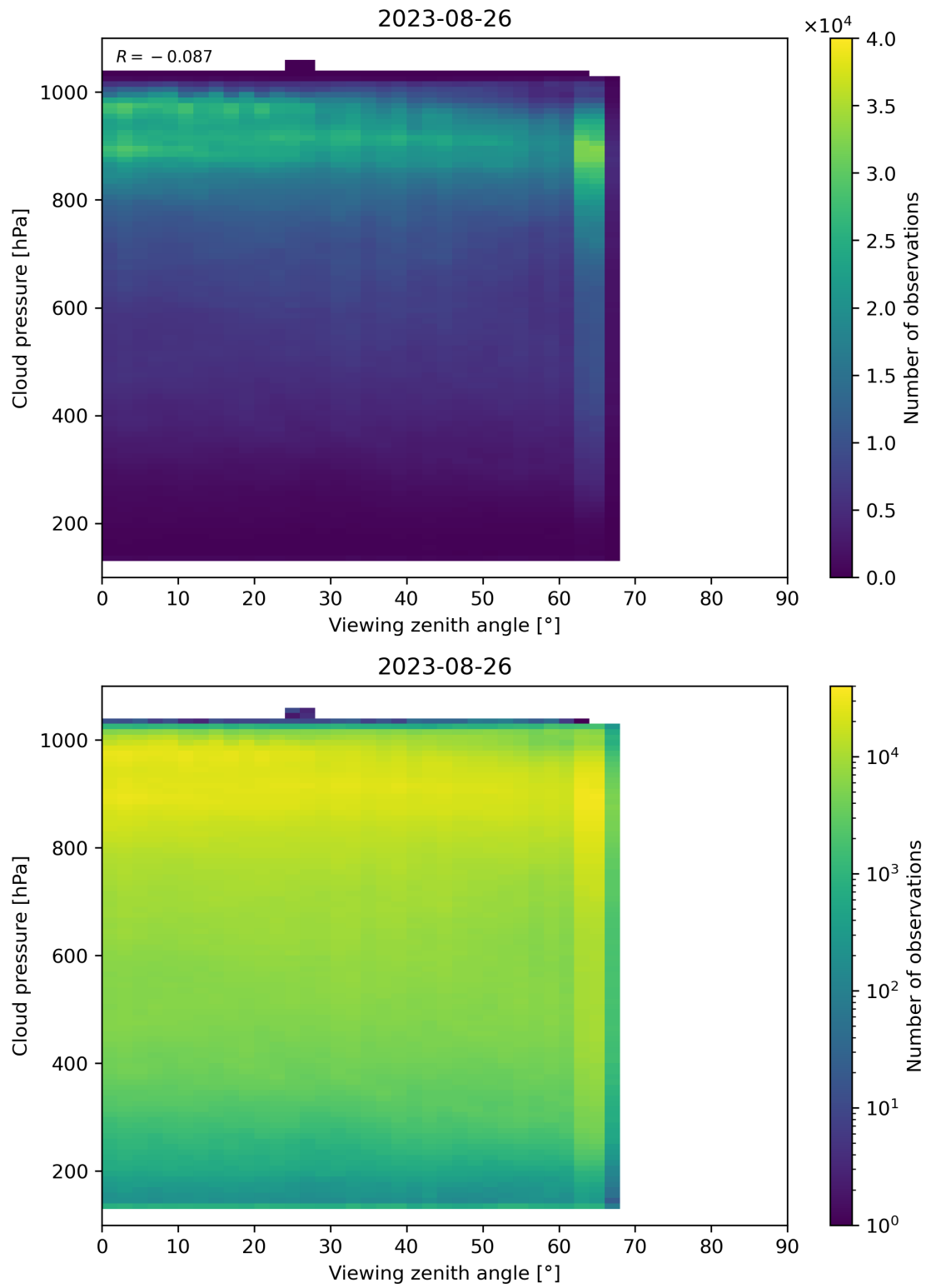
Figure 133: Scatter density plot of “Viewing zenith angle” against “Cloud pressure” for 2023-08-25 to 2023-08-27.
