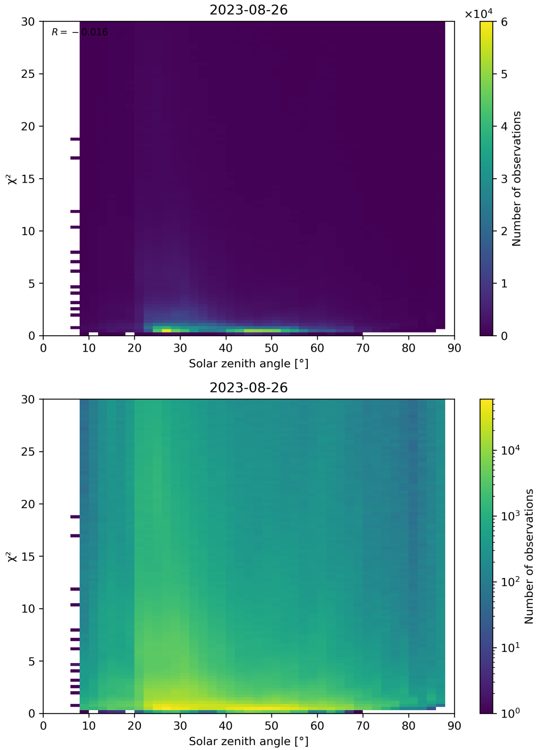
Figure 119: Scatter density plot of “Solar zenith angle” against “ \chi^2 ” for 2023-08-25 to 2023-08-27.
