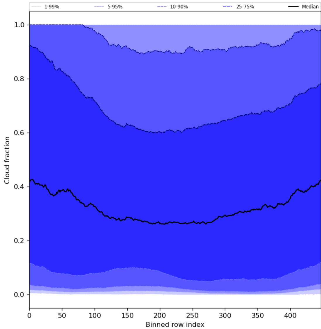
Figure 49: Along track statistics of “Cloud fraction” for 2023-08-25 to 2023-08-27
