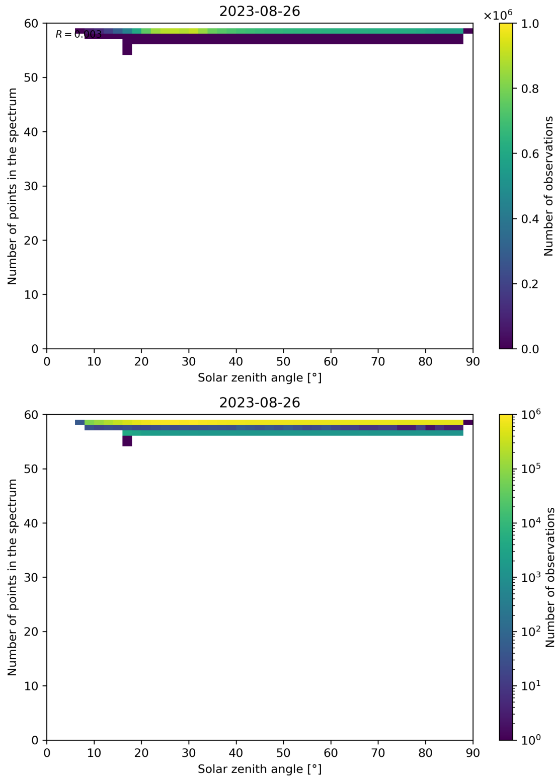
Figure 126: Scatter density plot of “Solar zenith angle” against “Number of points in the spectrum” for 2023-08-25 to 2023-08-27.
