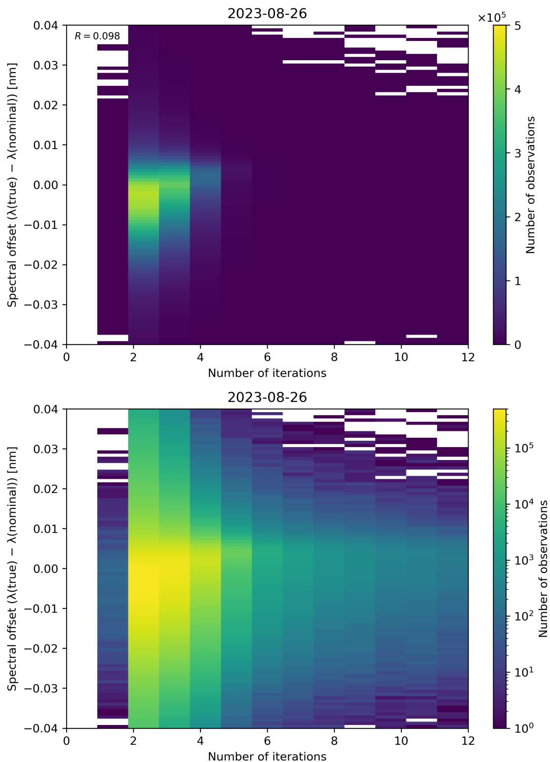
Figure 109: Scatter density plot of “Number of iterations” against “Spectral offset ( \lambda(\text{true}) - \lambda(\text{nominal}) )” for 2023-08-25 to 2023-08-27.
