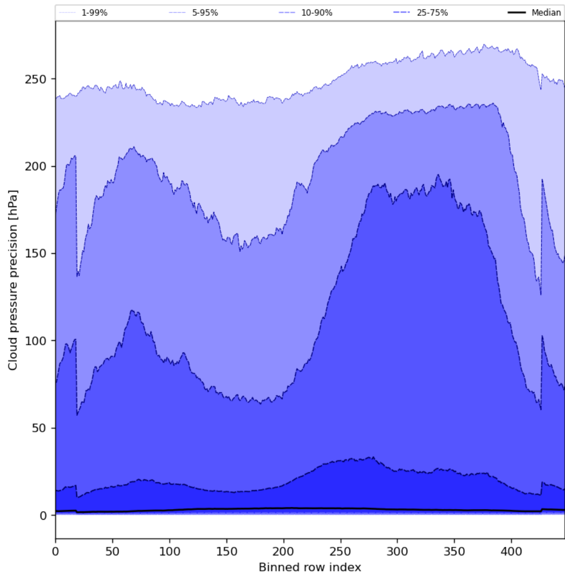
Figure 48: Along track statistics of “Cloud pressure precision” for 2023-08-25 to 2023-08-27
