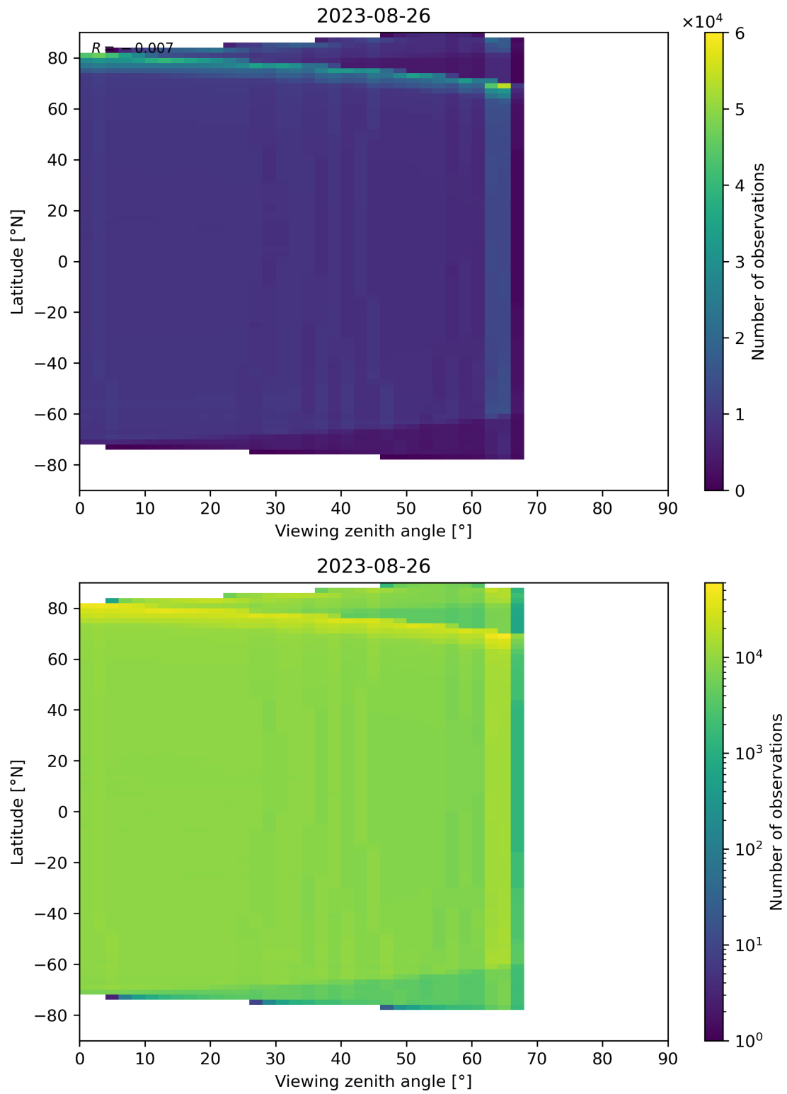
Figure 135: Scatter density plot of “Viewing zenith angle” against “Latitude” for 2023-08-25 to 2023-08-27.
