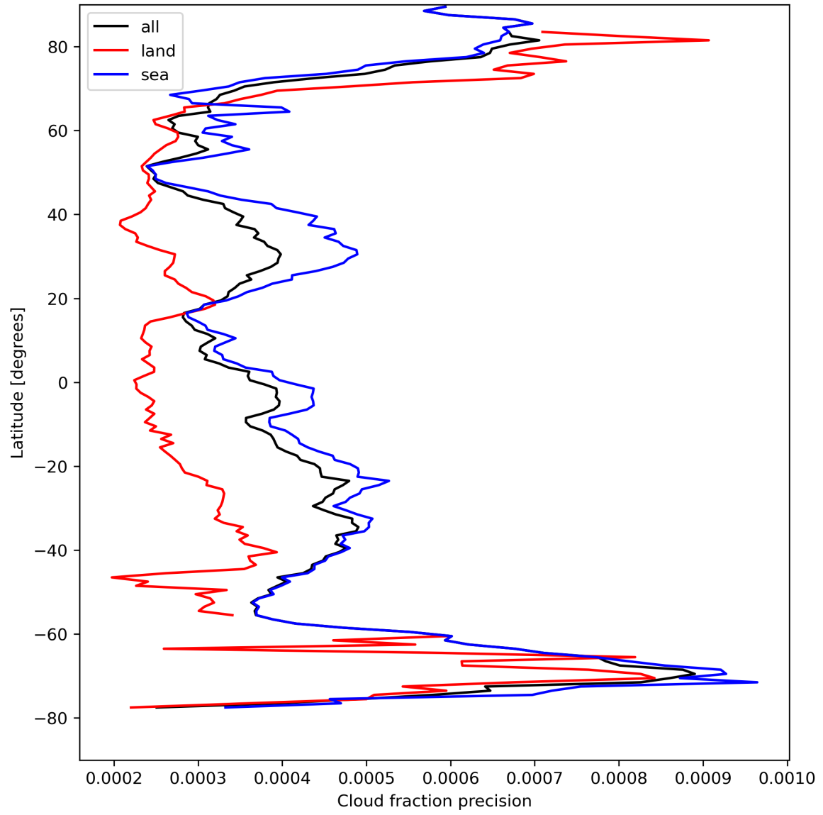
Figure 16: Zonal average of “Cloud fraction precision” for 2023-08-25 to 2023-08-27.
