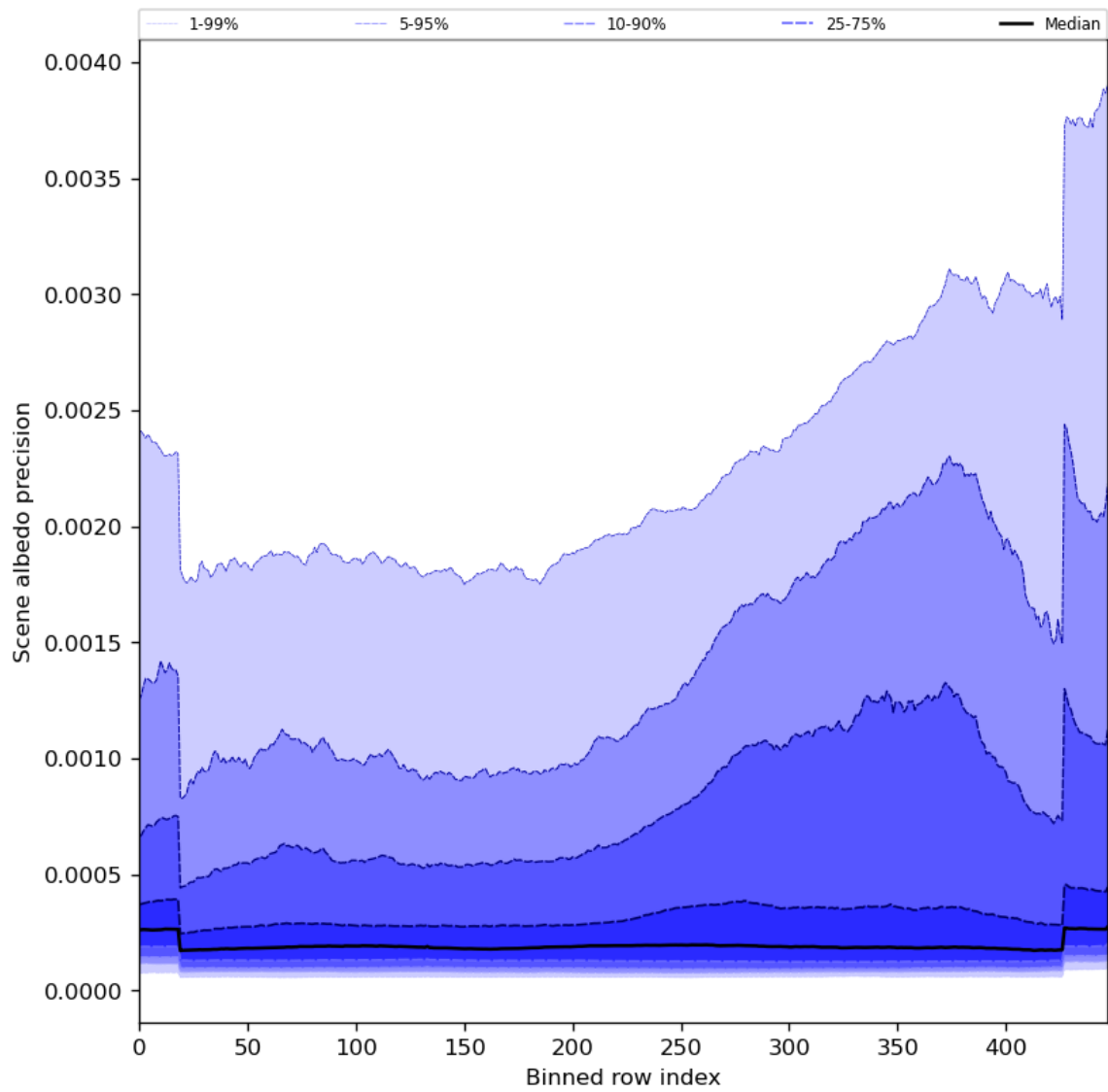
Figure 52: Along track statistics of “Scene albedo precision” for 2023-08-25 to 2023-08-27
