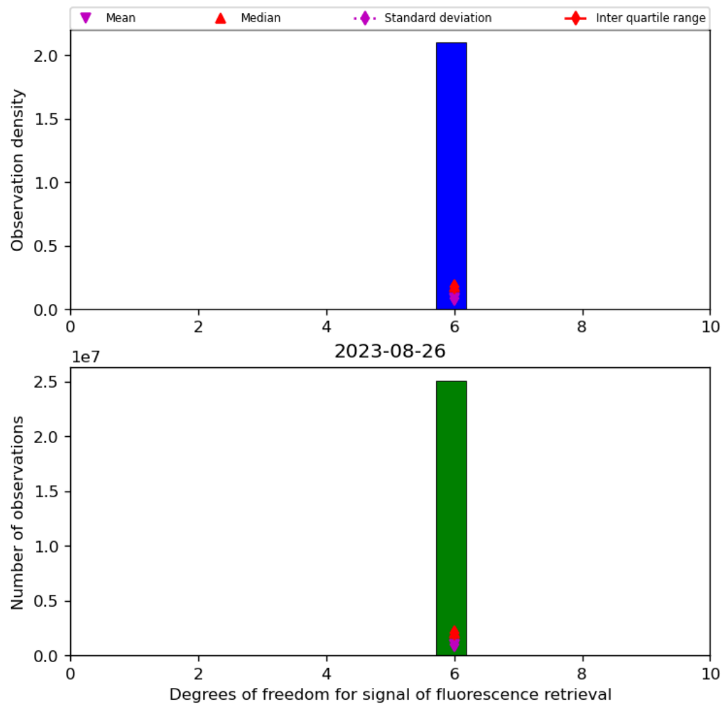
Figure 43: Histogram of “Degrees of freedom for signal of fluorescence retrieval” for 2023-08-25 to 2023-08-27
