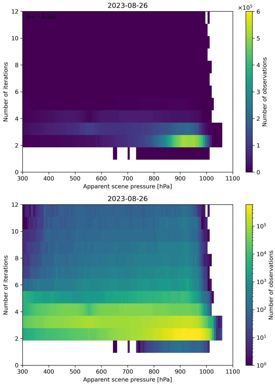
Figure 66: Scatter density plot of “Apparent scene pressure” against “Number of iterations” for 2023-08-25 to 2023-08-27.
