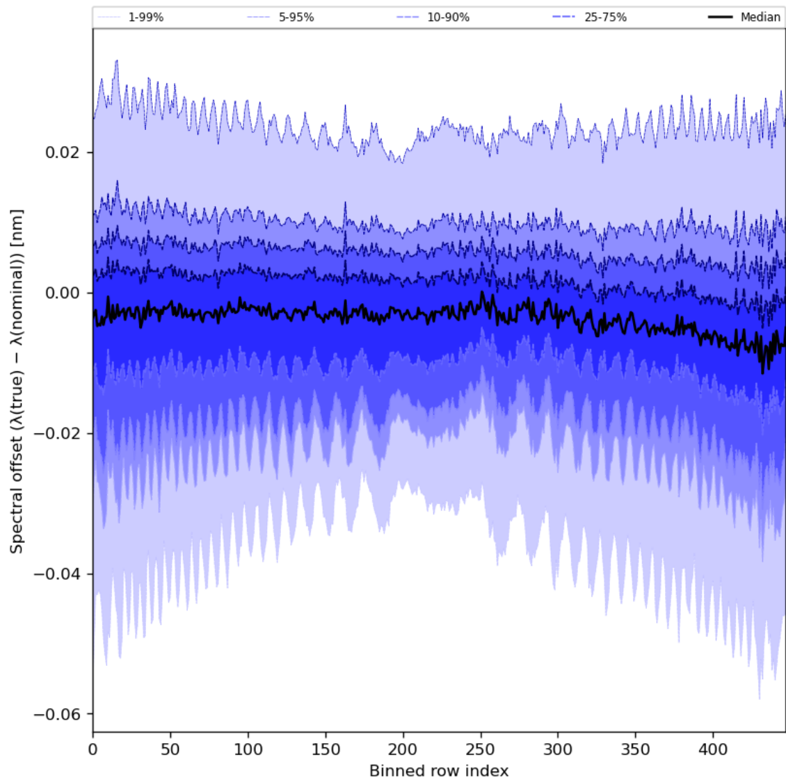
Figure 62: Along track statistics of “Spectral offset ( \lambda(\text{true}) - \lambda(\text{nominal}) )” for 2023-08-25 to 2023-08-27
