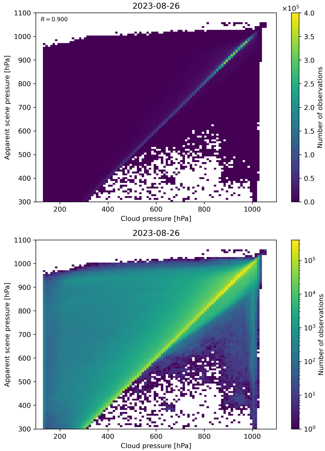
Figure 84: Scatter density plot of “Cloud pressure” against “Apparent scene pressure” for 2023-08-25 to 2023-08-27.
