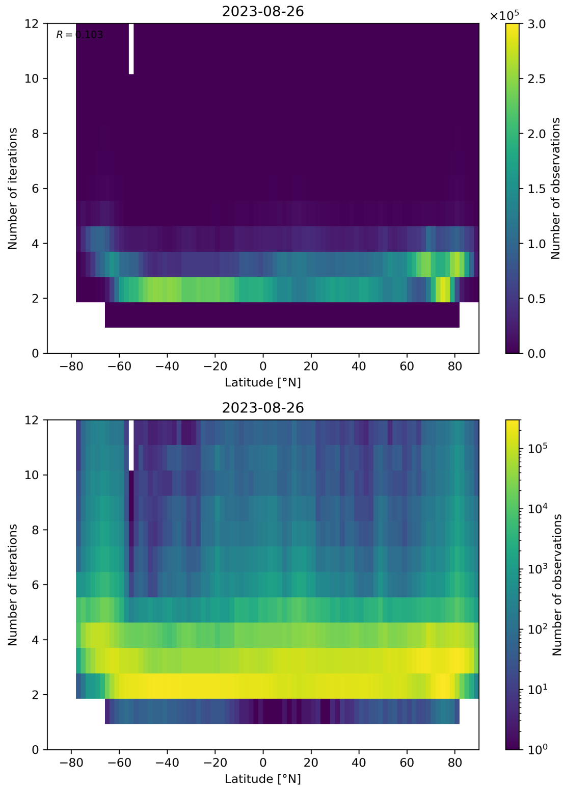
Figure 102: Scatter density plot of “Latitude” against “Number of iterations” for 2023-08-25 to 2023-08-27.
