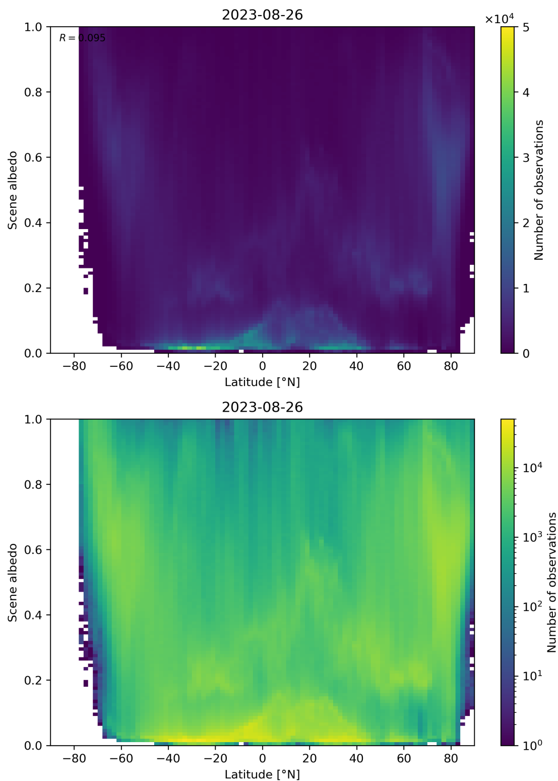
Figure 104: Scatter density plot of “Latitude” against “Scene albedo” for 2023-08-25 to 2023-08-27.
