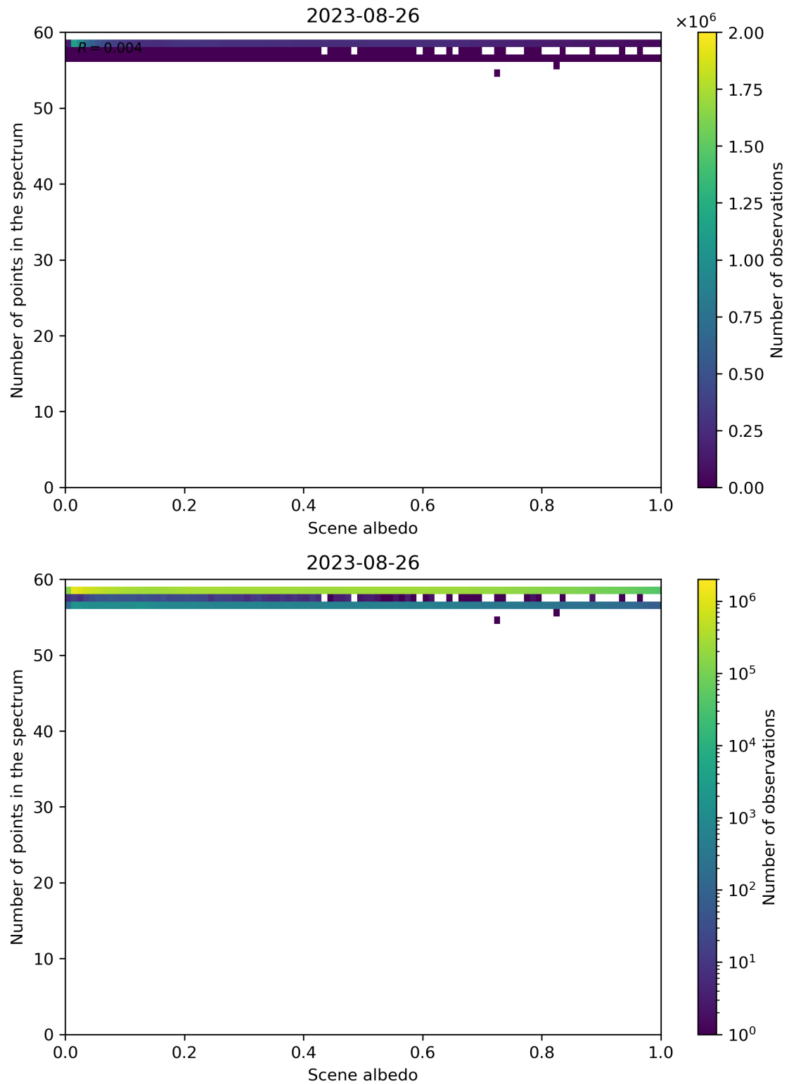
Figure 116: Scatter density plot of “Scene albedo” against “Number of points in the spectrum” for 2023-08-25 to 2023-08-27.
