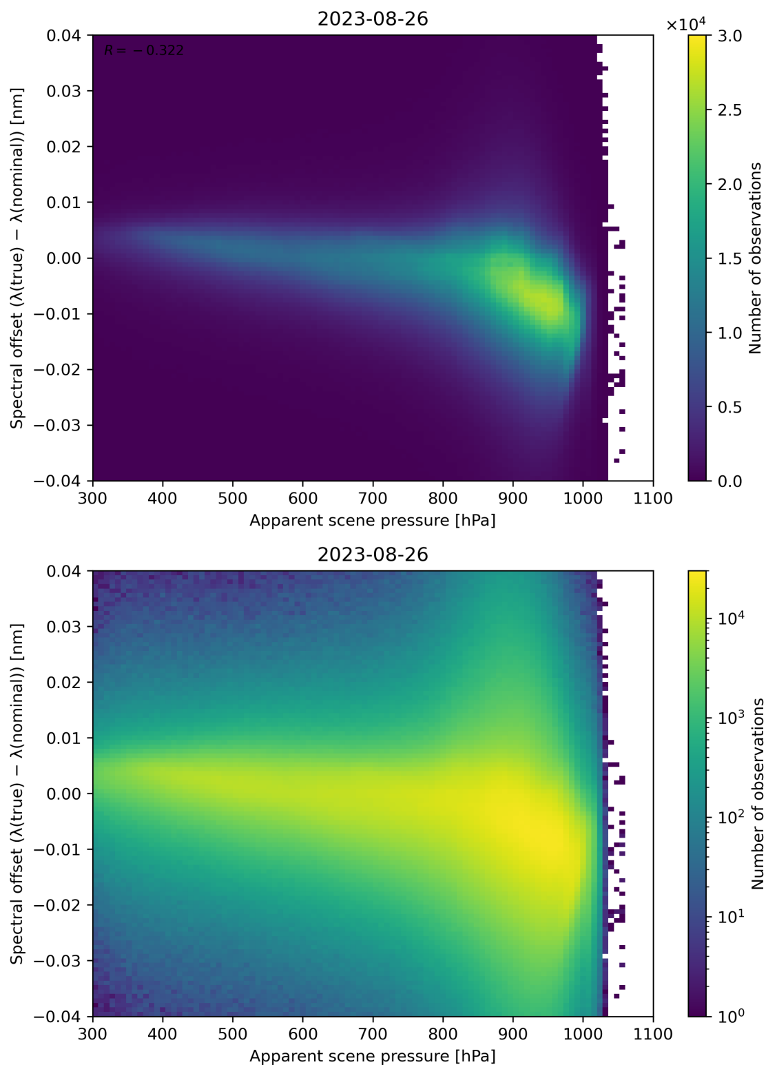
Figure 68: Scatter density plot of “Apparent scene pressure” against “Spectral offset ( \lambda(\text{true}) - \lambda(\text{nominal}) )” for 2023-08-25 to 2023-08-27.
