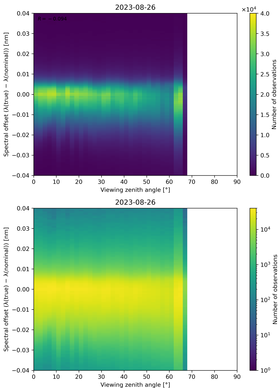
Figure 140: Scatter density plot of “Viewing zenith angle” against “Spectral offset ( \lambda(\text{true}) - \lambda(\text{nominal}) )” for 2023-08-25 to 2023-08-27.
