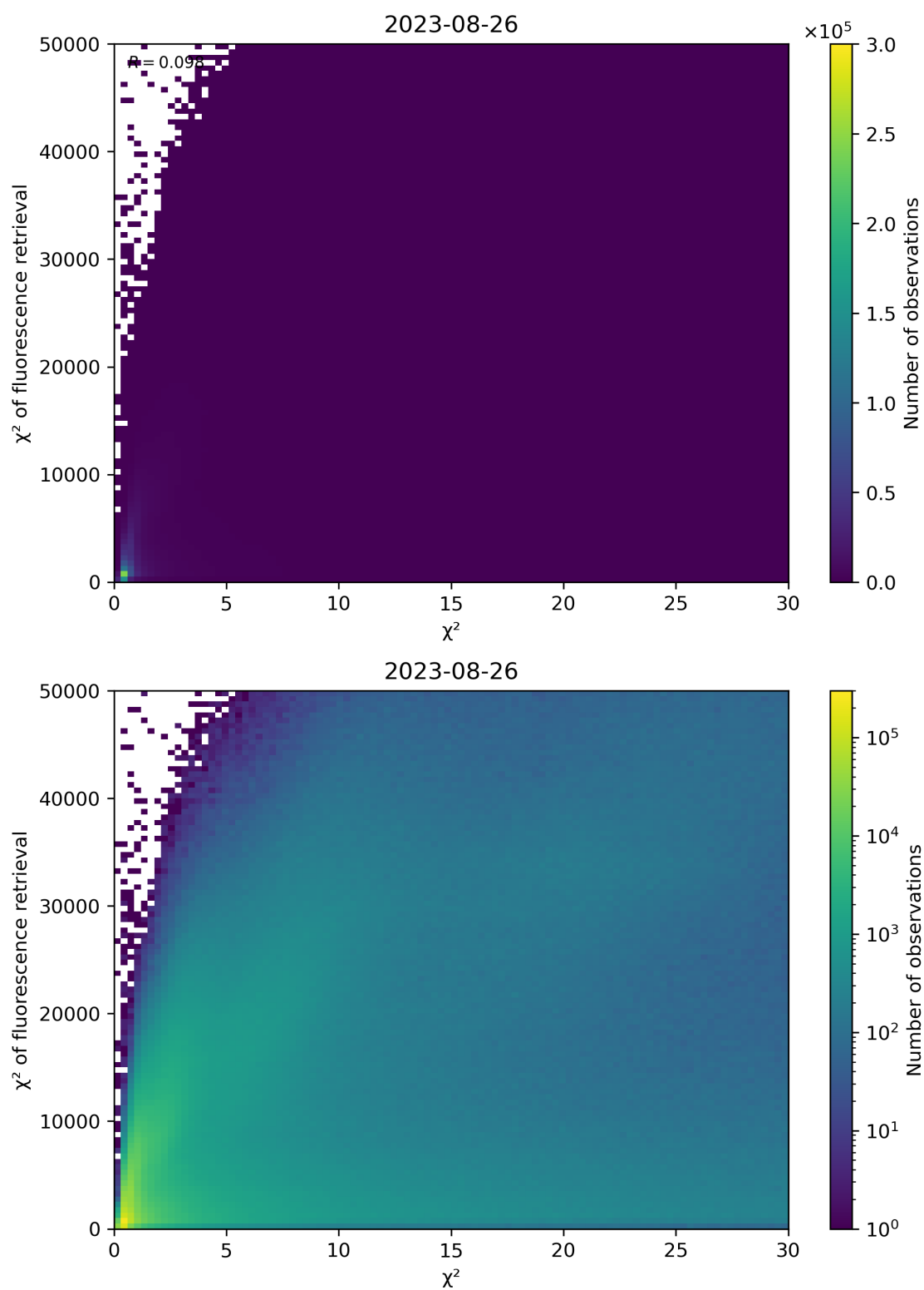
Figure 69: Scatter density plot of “ \chi^2 ” against “ \chi^2 of fluorescence retrieval” for 2023-08-25 to 2023-08-27.
