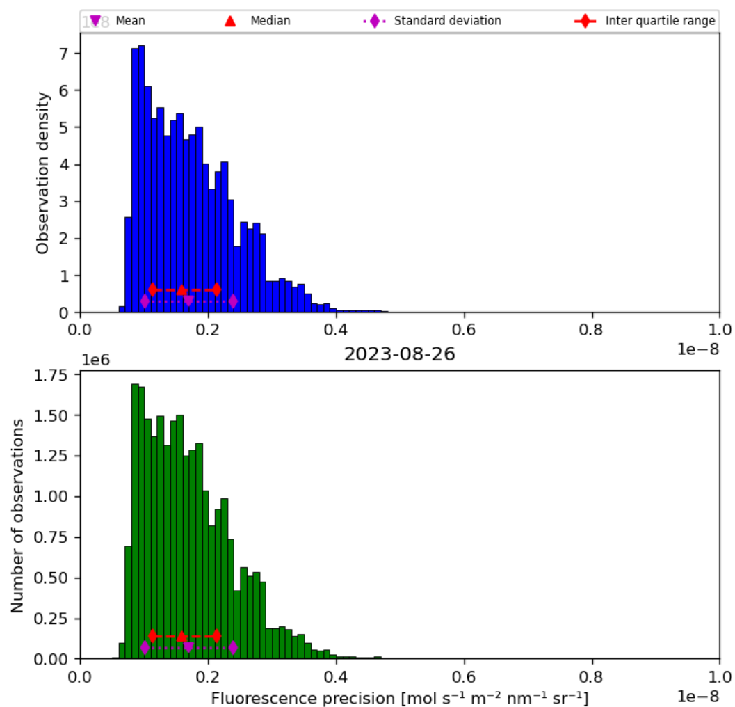
Figure 41: Histogram of “Fluorescence precision” for 2023-08-25 to 2023-08-27
