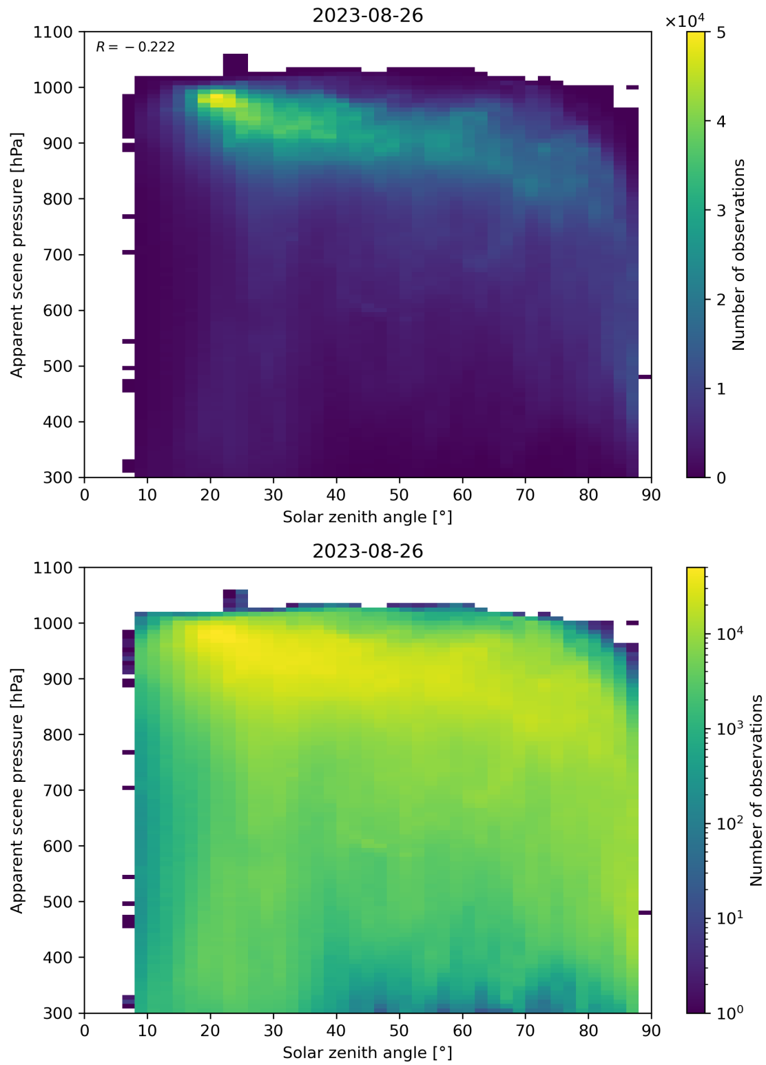
Figure 118: Scatter density plot of “Solar zenith angle” against “Apparent scene pressure” for 2023-08-25 to 2023-08-27.
