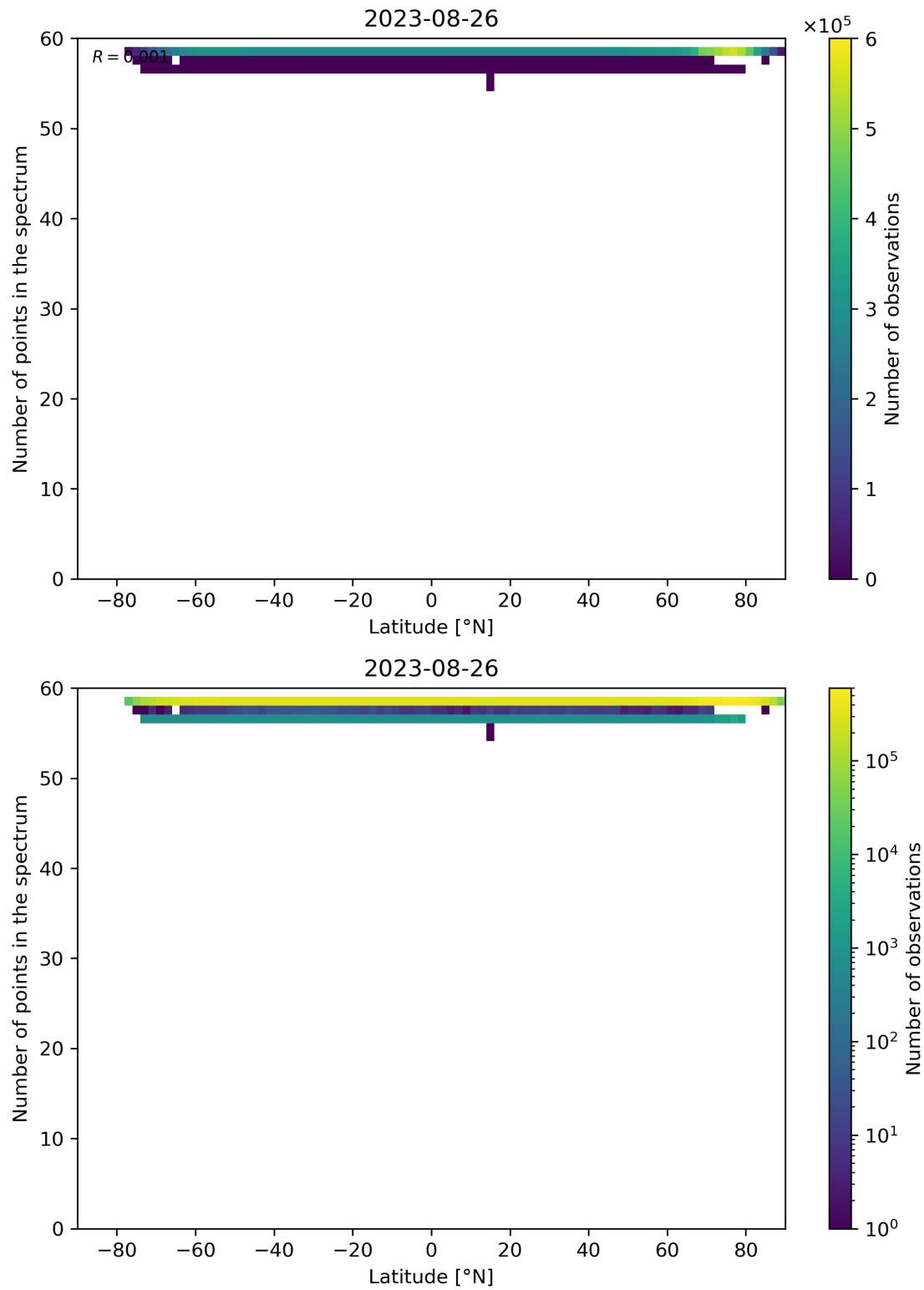
Figure 103: Scatter density plot of “Latitude” against “Number of points in the spectrum” for 2023-08-25 to 2023-08-27.
