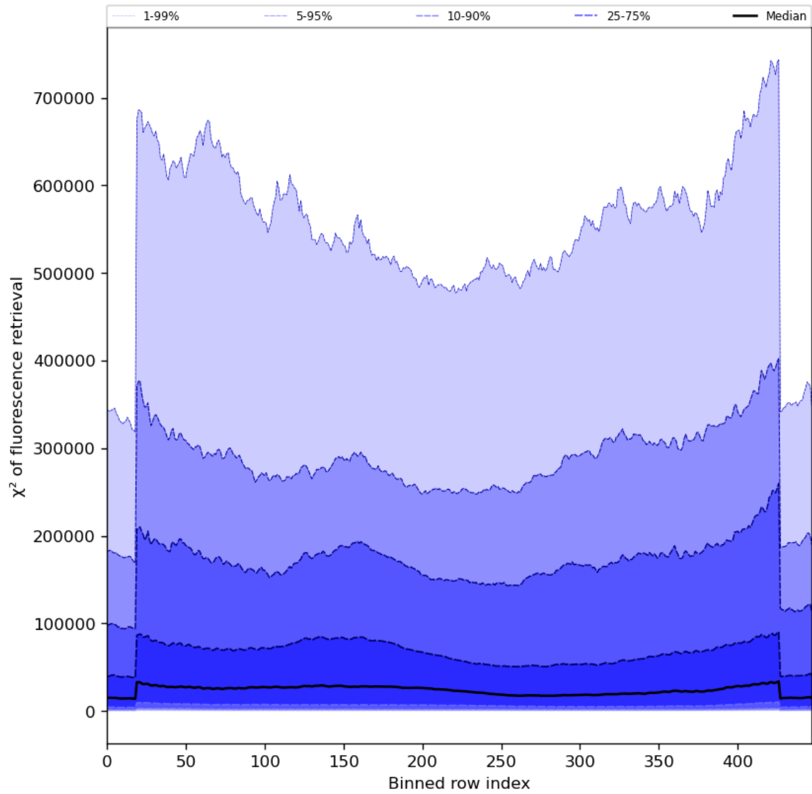
Figure 59: Along track statistics of “ \chi^2 of fluorescence retrieval” for 2023-08-25 to 2023-08-27
