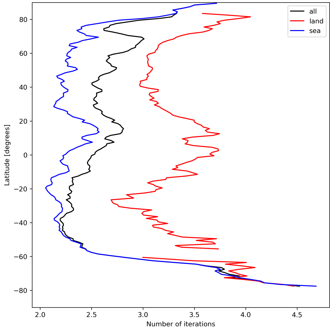
Figure 22: Zonal average of “Number of iterations” for 2023-08-25 to 2023-08-27.
