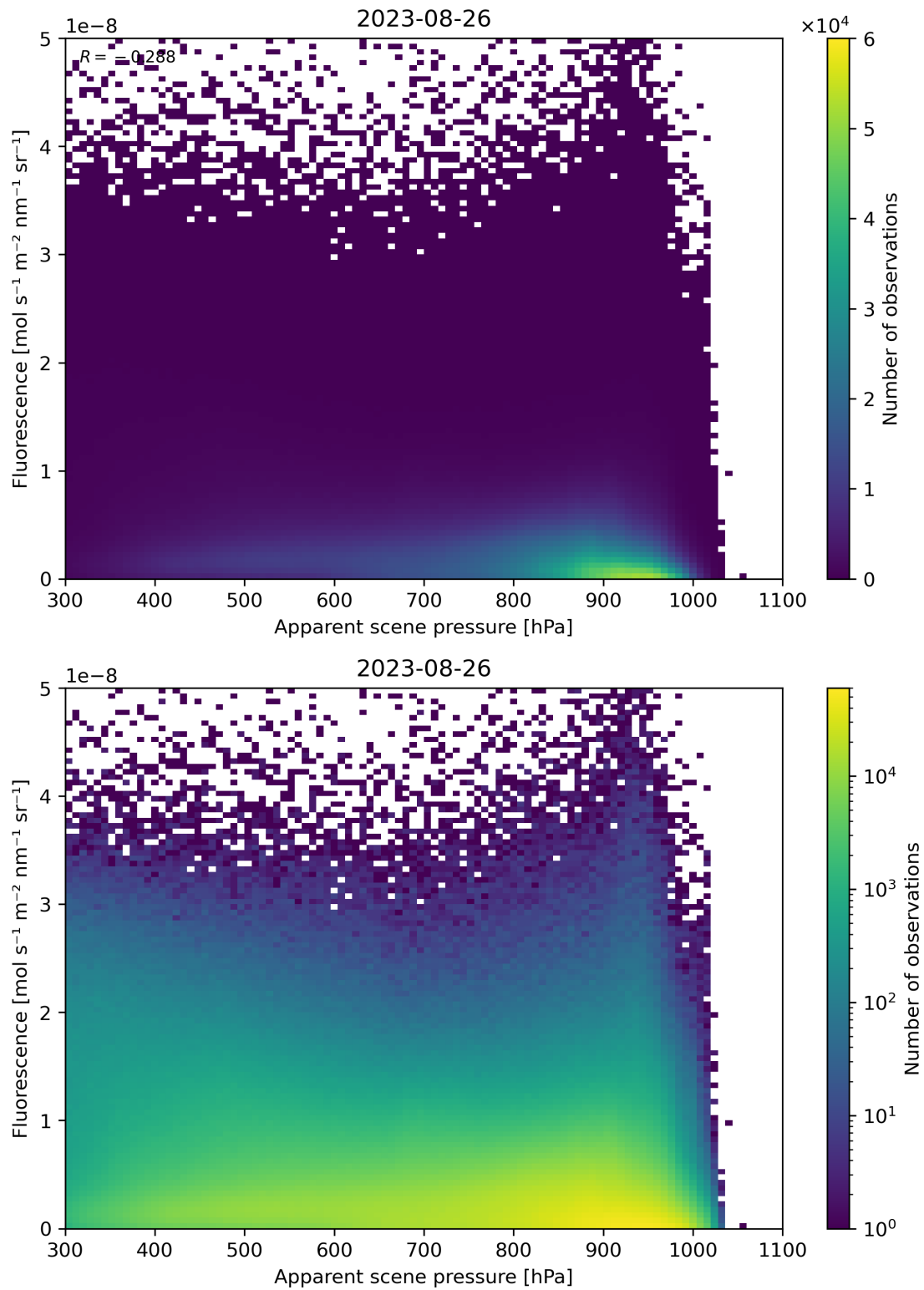
Figure 65: Scatter density plot of “Apparent scene pressure” against “Fluorescence” for 2023-08-25 to 2023-08-27.
