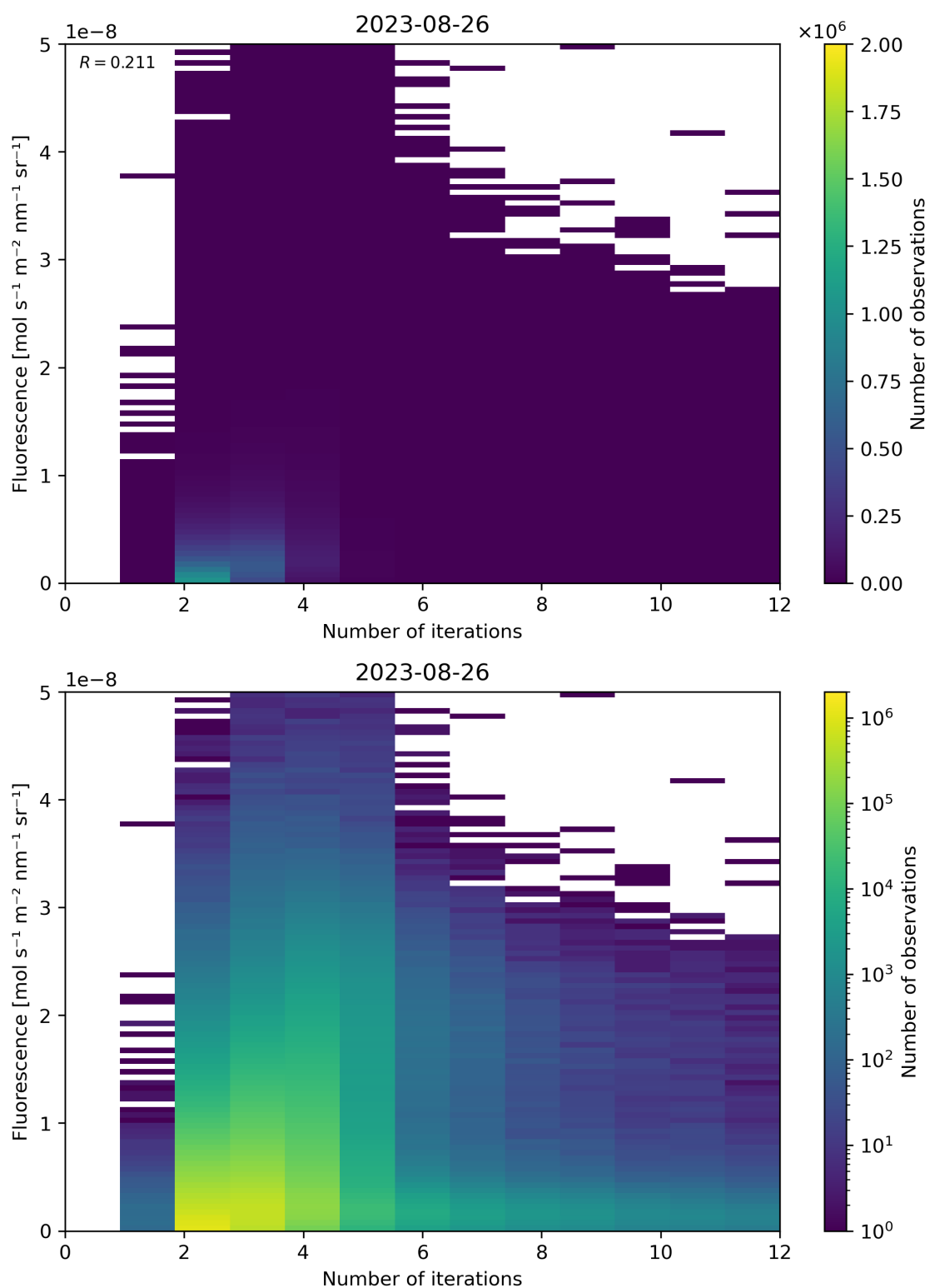
Figure 107: Scatter density plot of “Number of iterations” against “Fluorescence” for 2023-08-25 to 2023-08-27.
