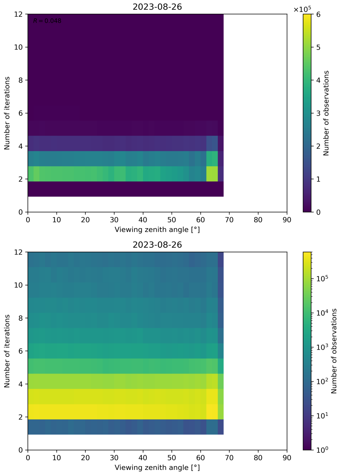
Figure 136: Scatter density plot of “Viewing zenith angle” against “Number of iterations” for 2023-08-25 to 2023-08-27.
