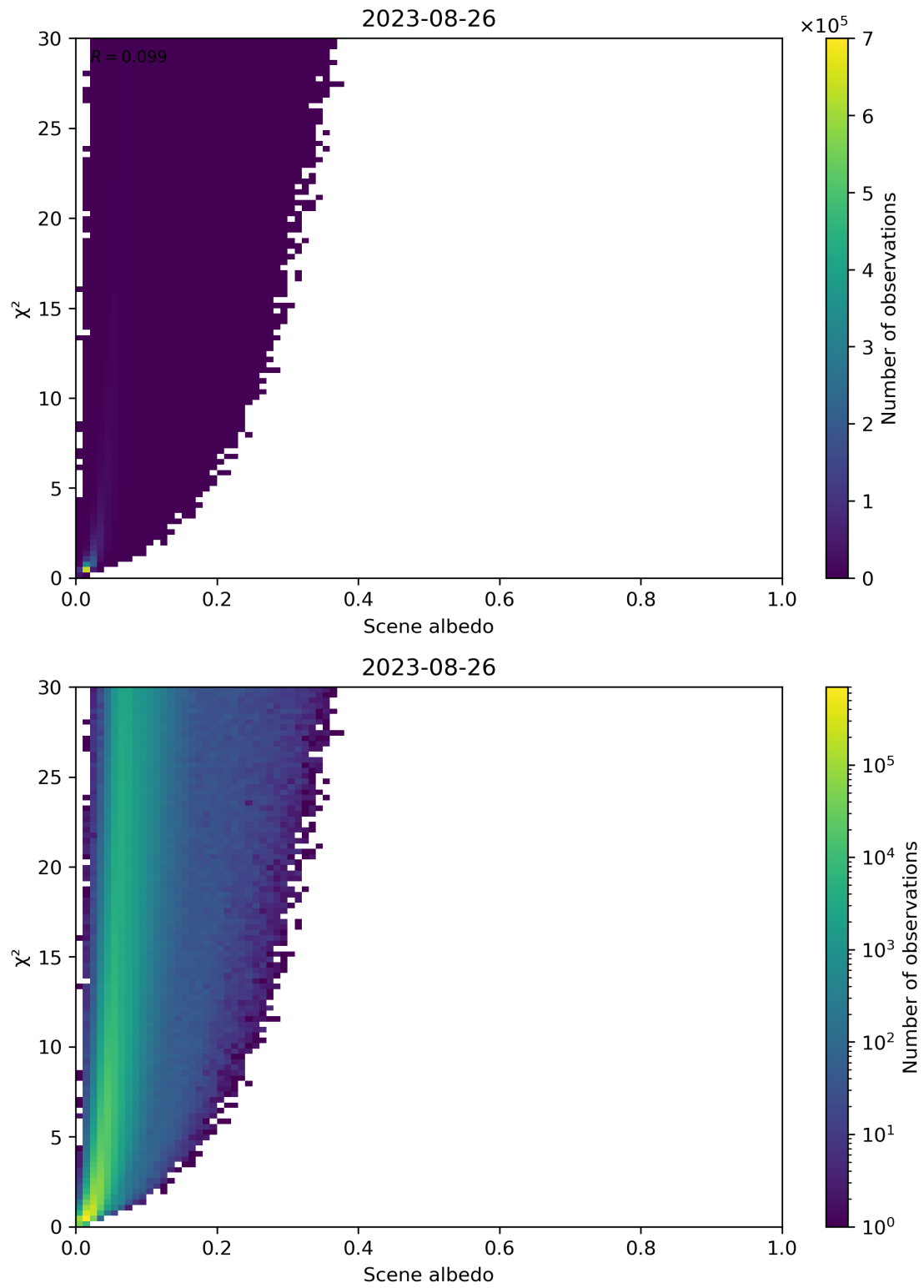
Figure 112: Scatter density plot of “Scene albedo” against “ \chi^2 ” for 2023-08-25 to 2023-08-27.
