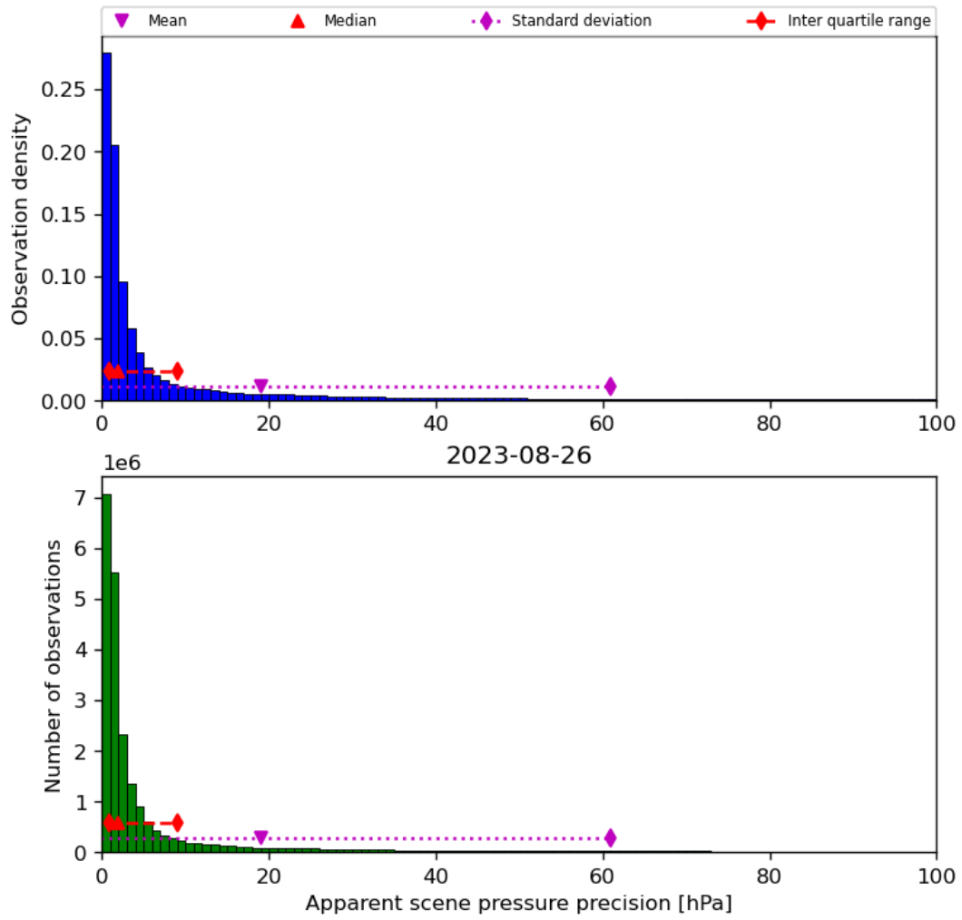
Figure 37: Histogram of “Apparent scene pressure precision” for 2023-08-25 to 2023-08-27
