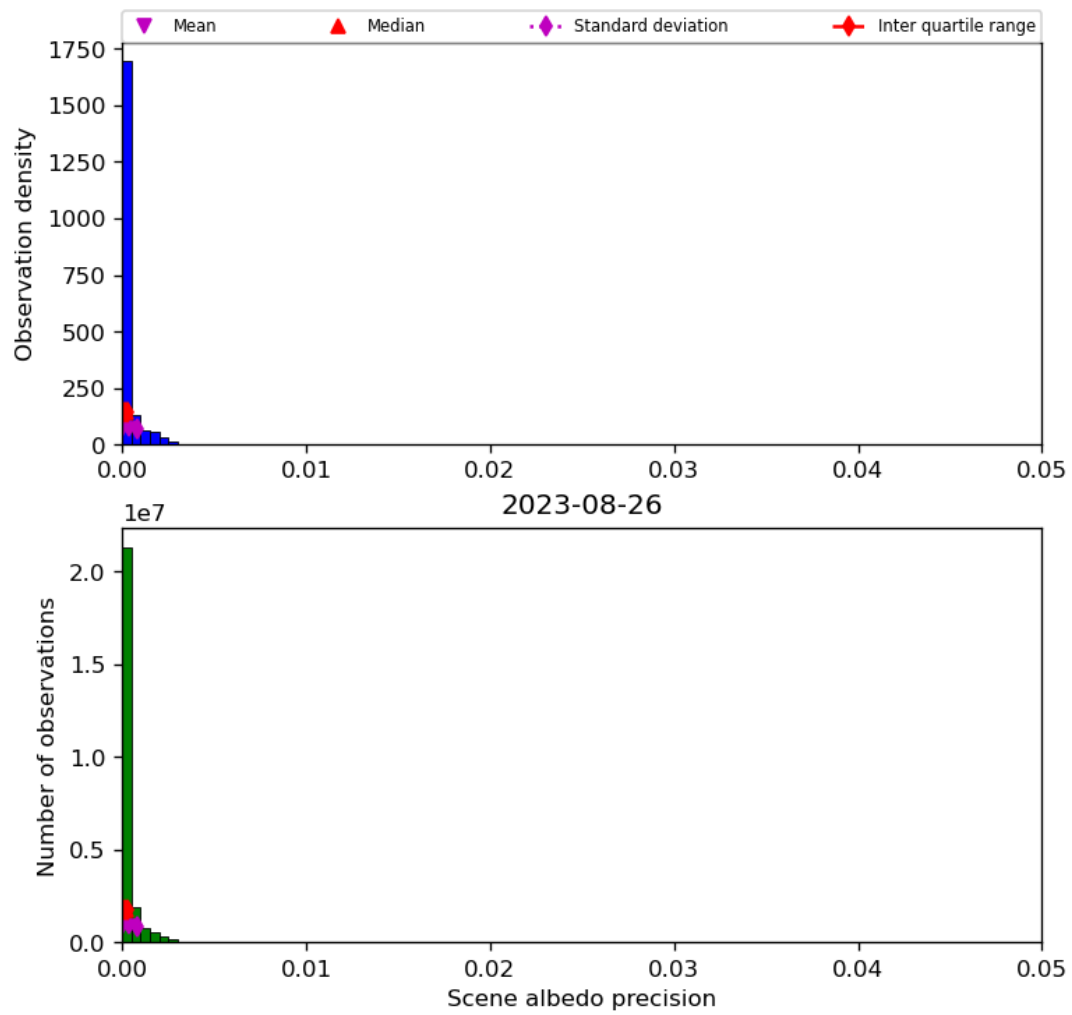
Figure 35: Histogram of “Scene albedo precision” for 2023-08-25 to 2023-08-27
