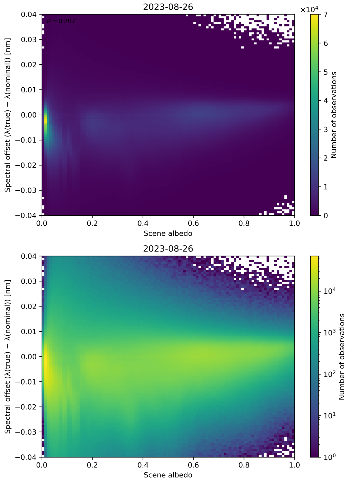
Figure 117: Scatter density plot of “Scene albedo” against “Spectral offset ( \lambda(\text{true}) - \lambda(\text{nominal}) )” for 2023-08-25 to 2023-08-27.
