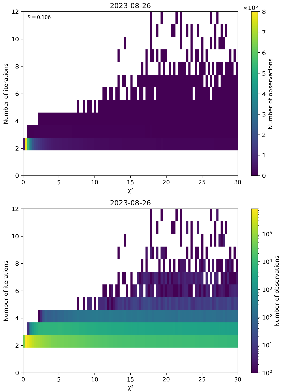
Figure 73: Scatter density plot of “ \chi^2 ” against “Number of iterations” for 2023-08-25 to 2023-08-27.
