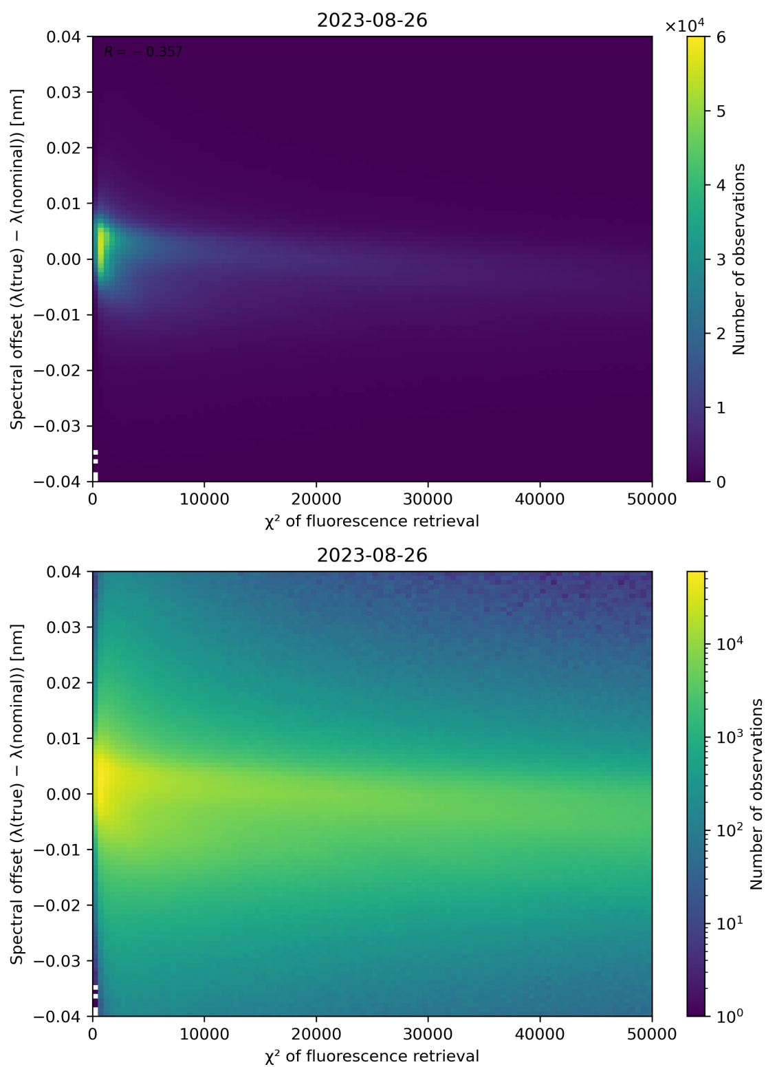
Figure 72: Scatter density plot of “ \chi^2 of fluorescence retrieval” against “Spectral offset ( \lambda(\text{true}) - \lambda(\text{nominal}) )” for 2023-08-25 to 2023-08-27.
