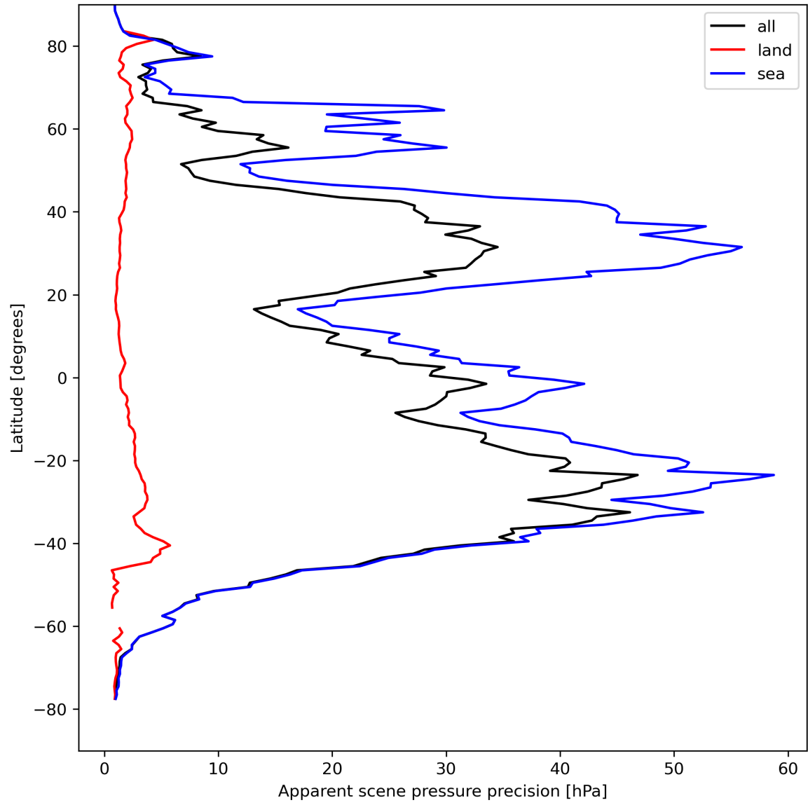
Figure 20: Zonal average of “Apparent scene pressure precision” for 2023-08-25 to 2023-08-27.
