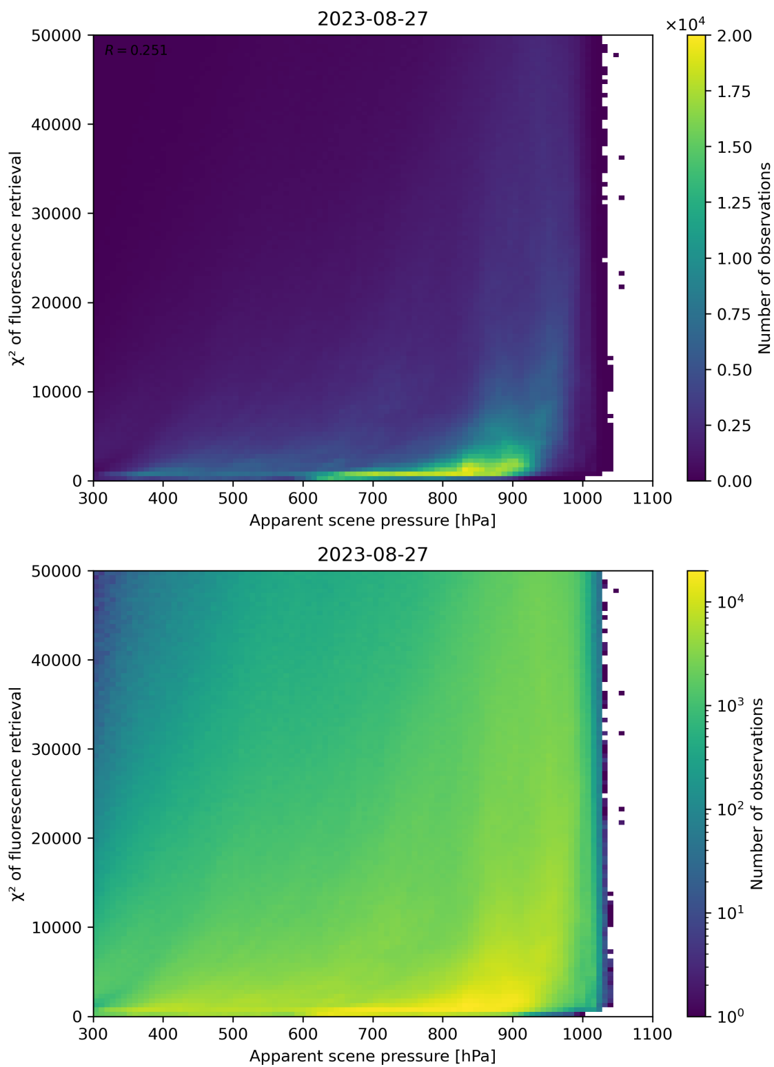
Figure 64: Scatter density plot of “Apparent scene pressure” against “ \chi^2 of fluorescence retrieval” for 2023-08-26 to 2023-08-28.
