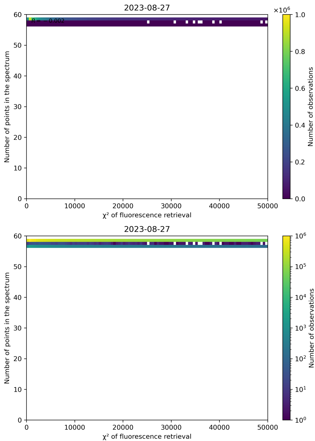
Figure 71: Scatter density plot of " \chi^2 of fluorescence retrieval" against "Number of points in the spectrum" for 2023-08-26 to 2023-08-28.
