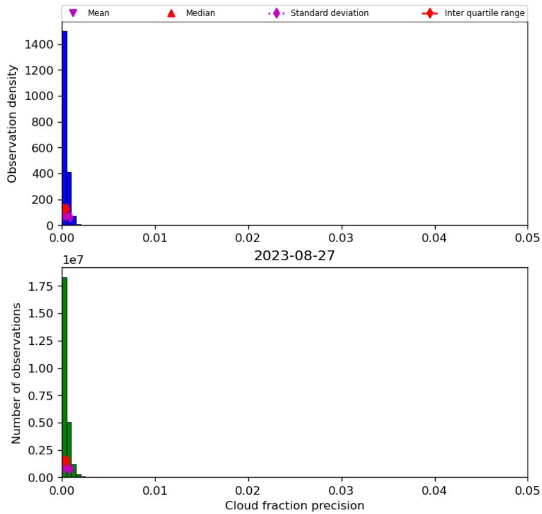
Figure 33: Histogram of “Cloud fraction precision” for 2023-08-26 to 2023-08-28
