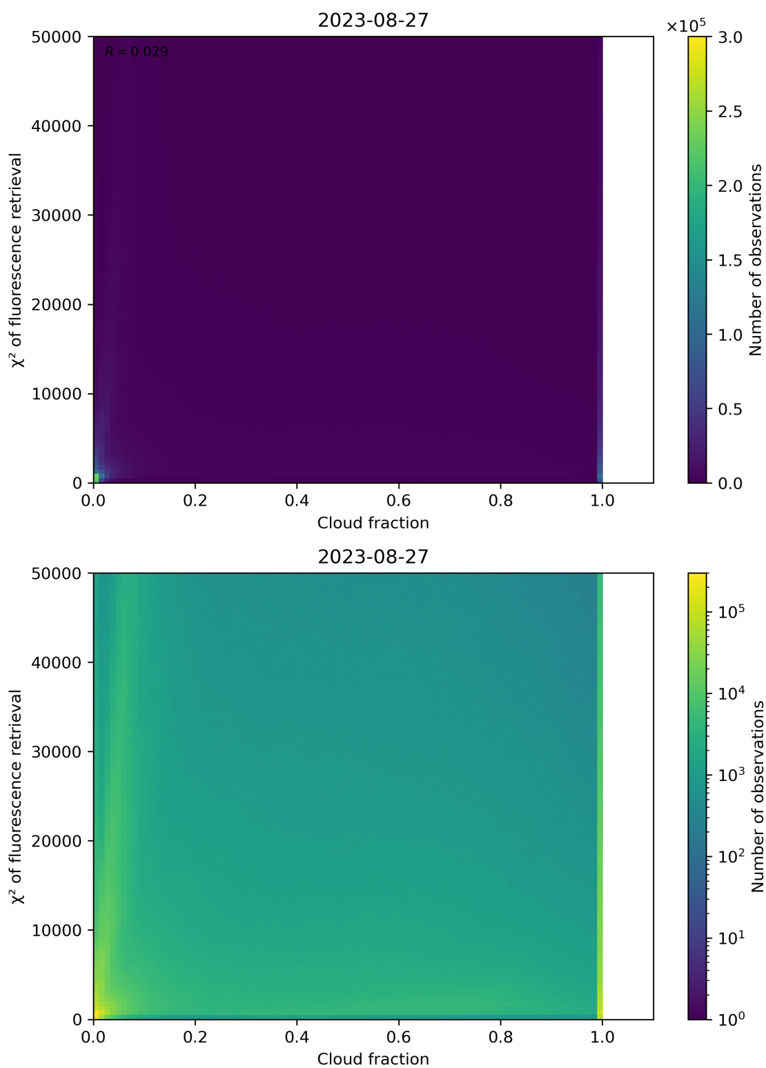
Figure 78: Scatter density plot of “Cloud fraction” against “ \chi^2 of fluorescence retrieval” for 2023-08-26 to 2023-08-28.
