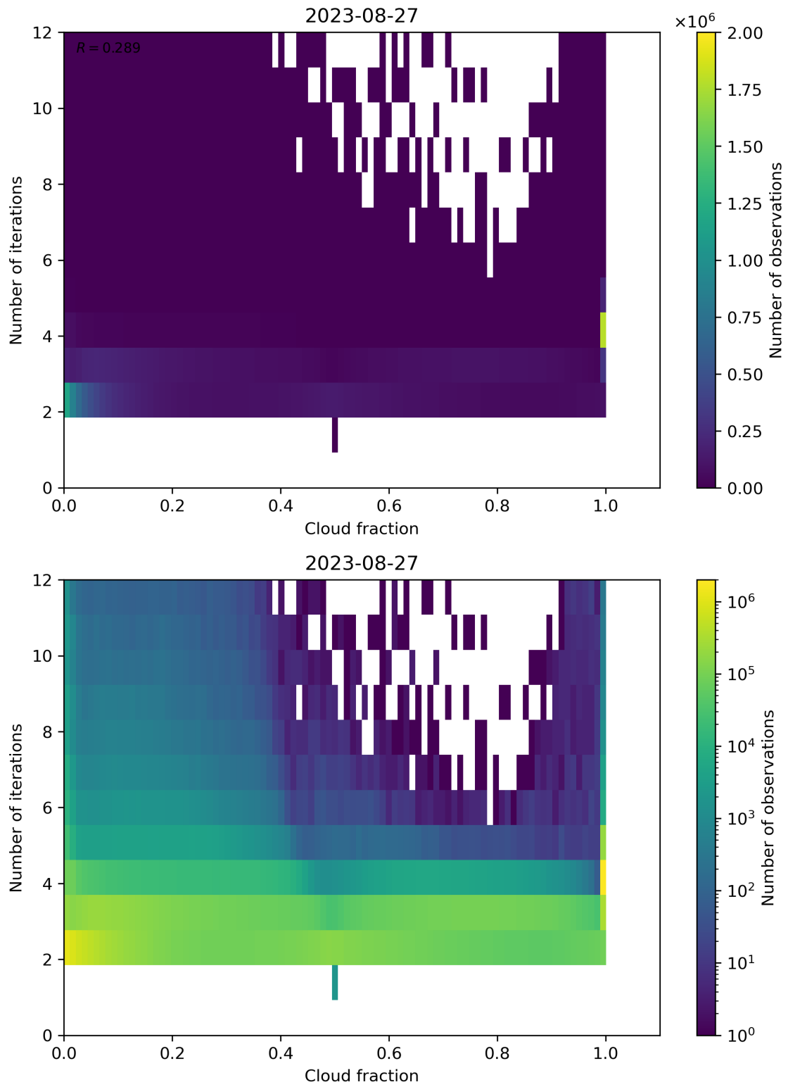
Figure 80: Scatter density plot of “Cloud fraction” against “Number of iterations” for 2023-08-26 to 2023-08-28.
