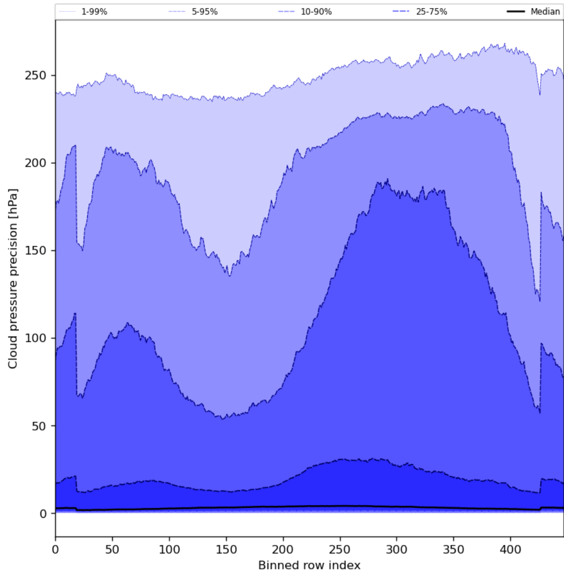
Figure 48: Along track statistics of “Cloud pressure precision” for 2023-08-26 to 2023-08-28
