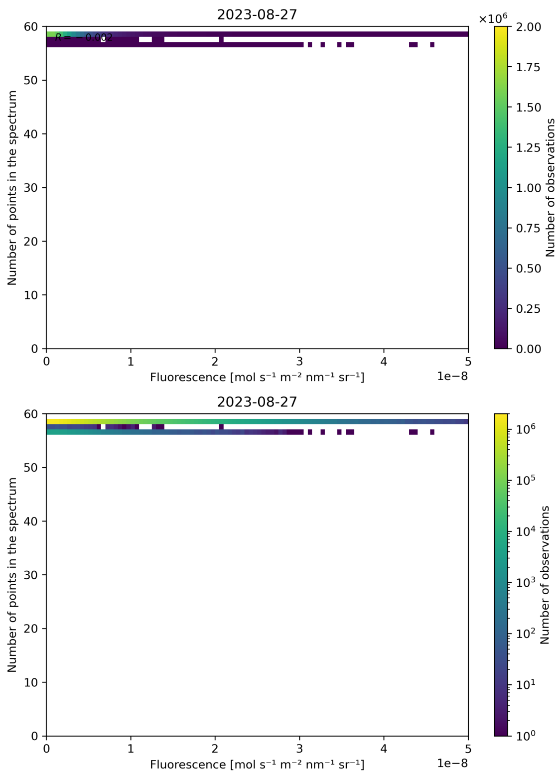
Figure 94: Scatter density plot of “Fluorescence” against “Number of points in the spectrum” for 2023-08-26 to 2023-08-28.
