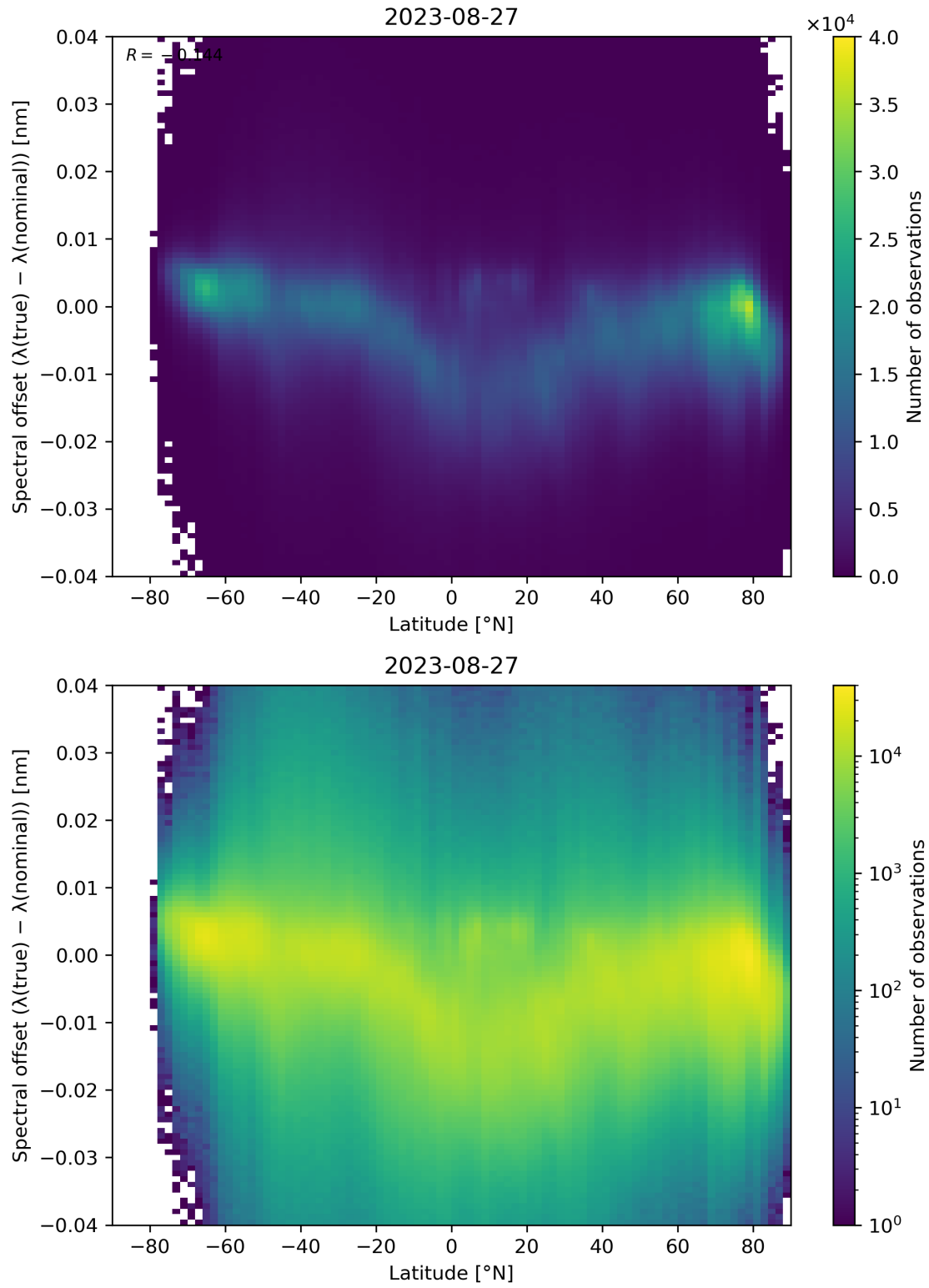
Figure 105: Scatter density plot of “Latitude” against “Spectral offset ( \lambda(\text{true}) - \lambda(\text{nominal}) )” for 2023-08-26 to 2023-08-28.
