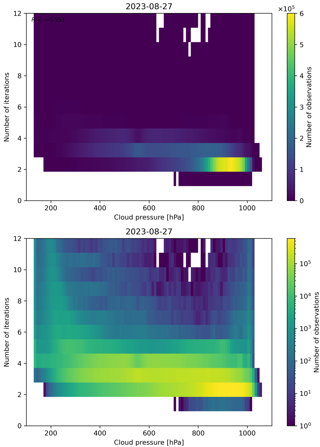
Figure 89: Scatter density plot of “Cloud pressure” against “Number of iterations” for 2023-08-26 to 2023-08-28.
