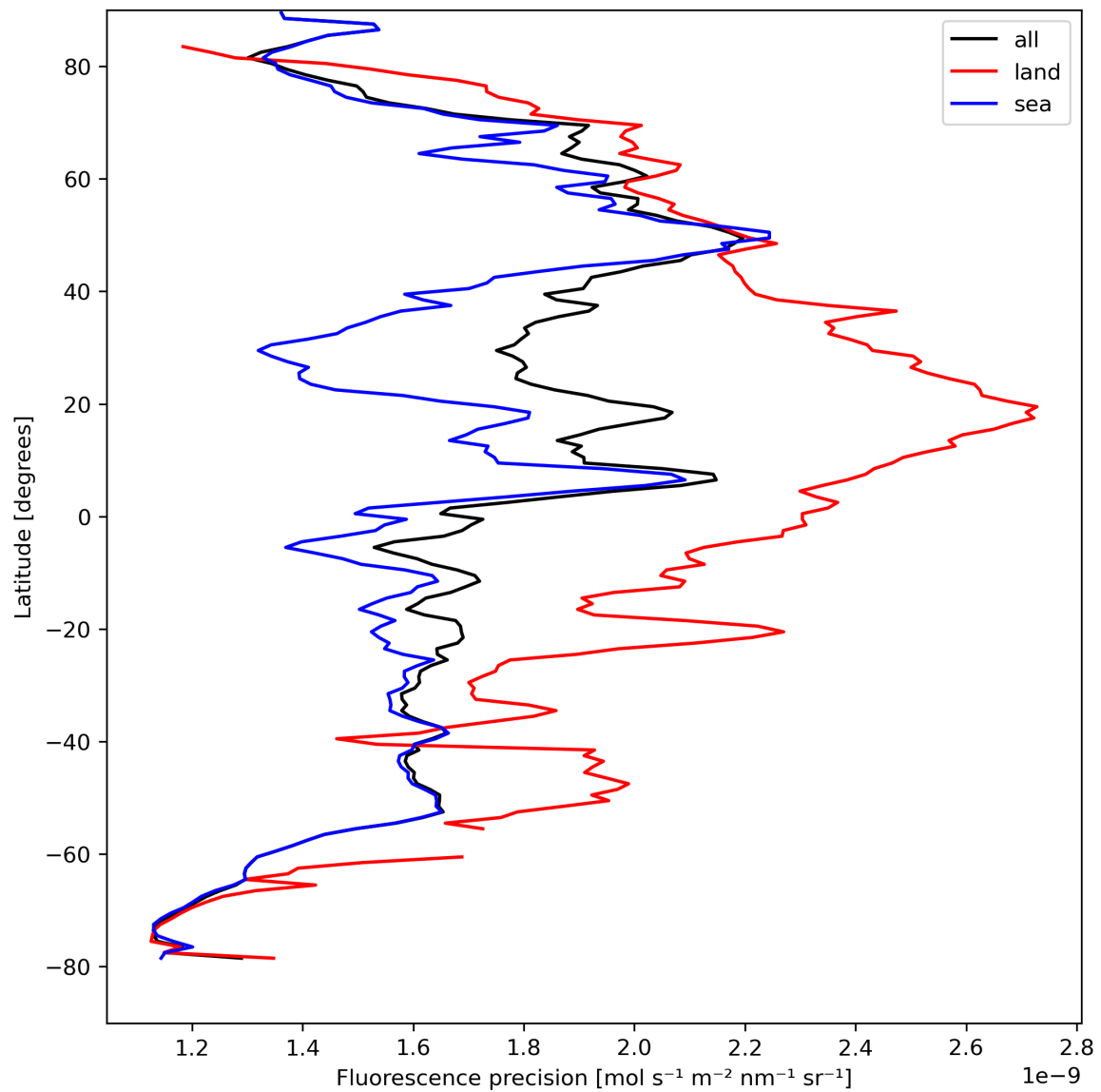
Figure 24: Zonal average of “Fluorescence precision” for 2023-08-26 to 2023-08-28.
