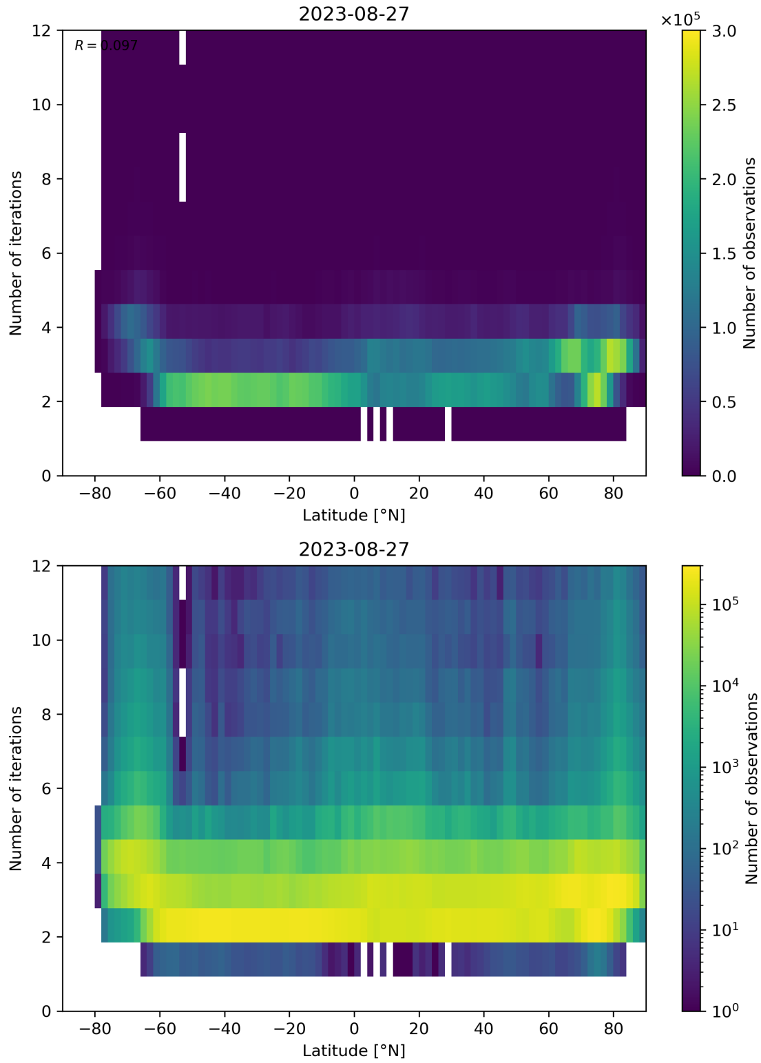
Figure 102: Scatter density plot of “Latitude” against “Number of iterations” for 2023-08-26 to 2023-08-28.
