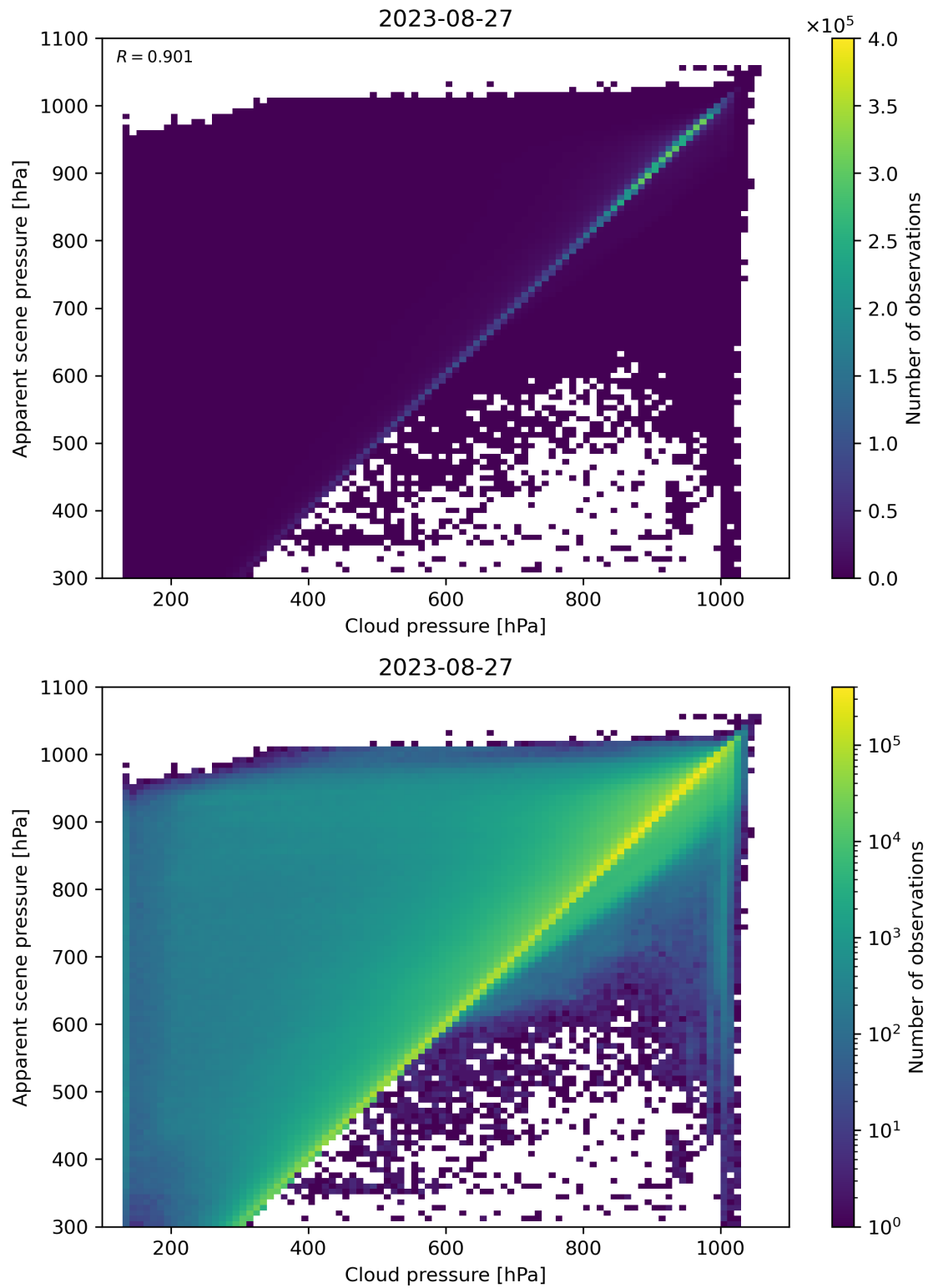
Figure 84: Scatter density plot of “Cloud pressure” against “Apparent scene pressure” for 2023-08-26 to 2023-08-28.
