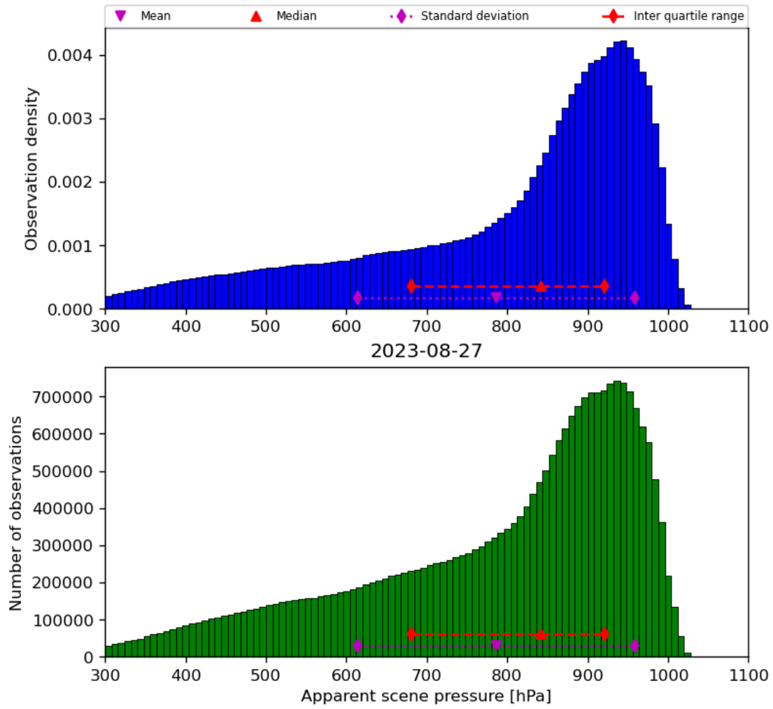
Figure 36: Histogram of “Apparent scene pressure” for 2023-08-26 to 2023-08-28
