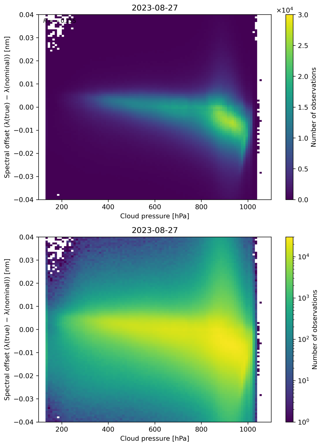
Figure 92: Scatter density plot of “Cloud pressure” against “Spectral offset ( \lambda(\text{true}) - \lambda(\text{nominal}) )” for 2023-08-26 to 2023-08-28.
