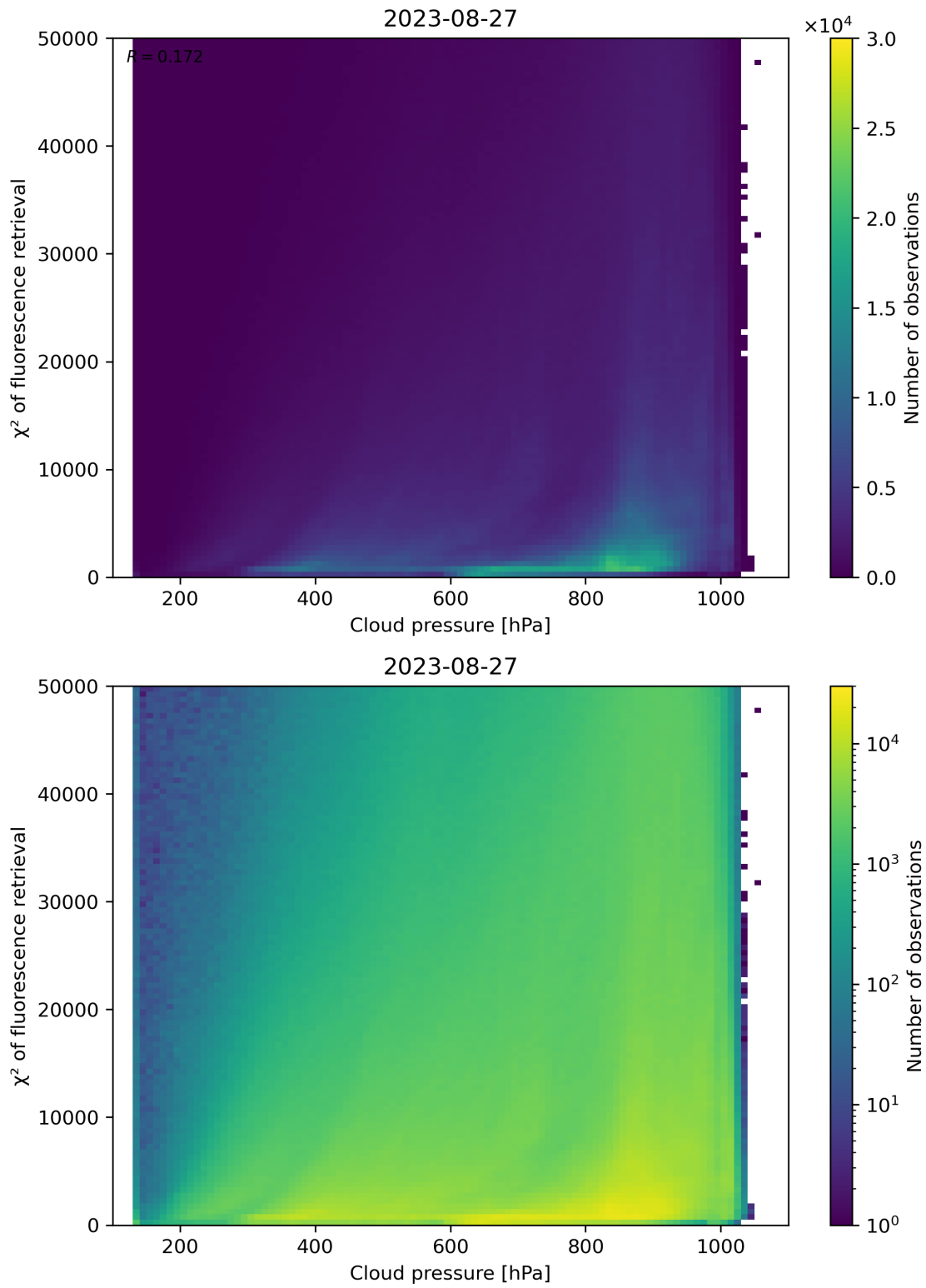
Figure 86: Scatter density plot of “Cloud pressure” against “ \chi^2 of fluorescence retrieval” for 2023-08-26 to 2023-08-28.
