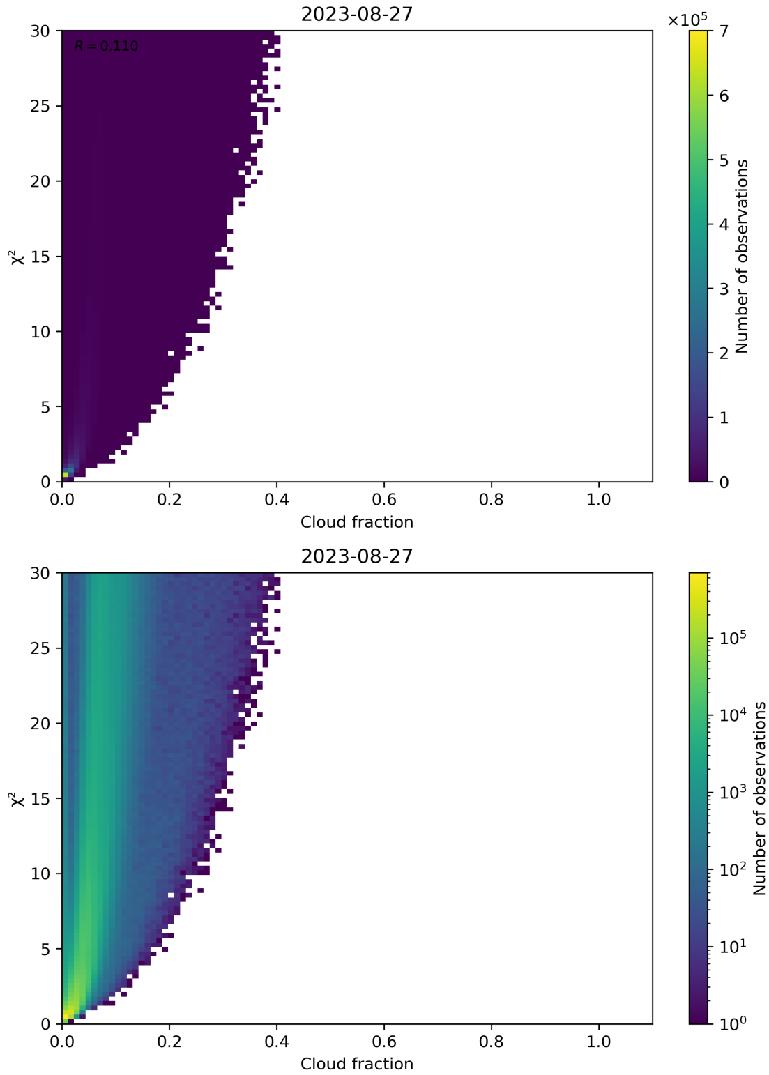
Figure 77: Scatter density plot of “Cloud fraction” against “ \chi^2 ” for 2023-08-26 to 2023-08-28.
