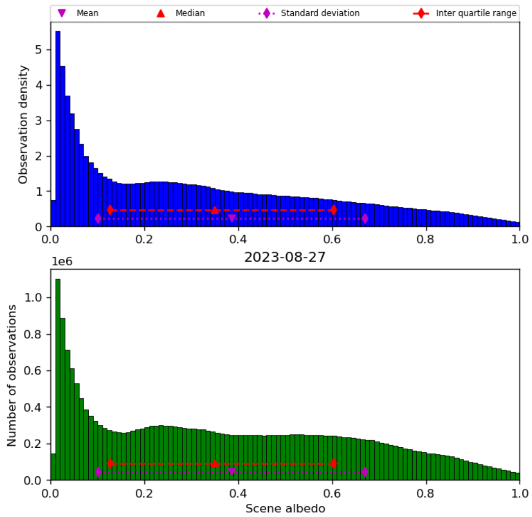
Figure 34: Histogram of “Scene albedo” for 2023-08-26 to 2023-08-28
