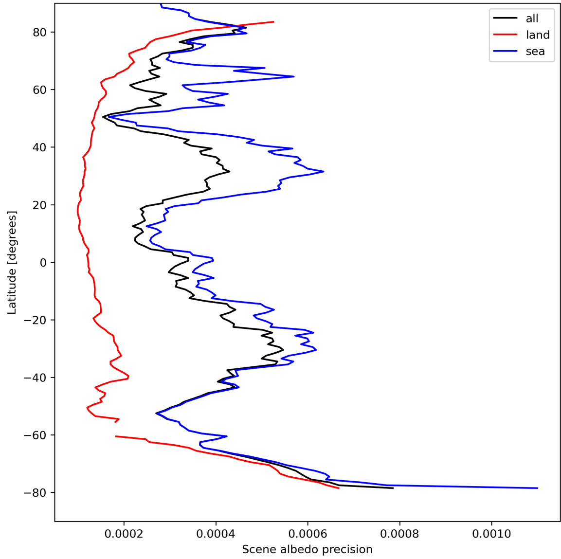
Figure 18: Zonal average of “Scene albedo precision” for 2023-08-26 to 2023-08-28.
