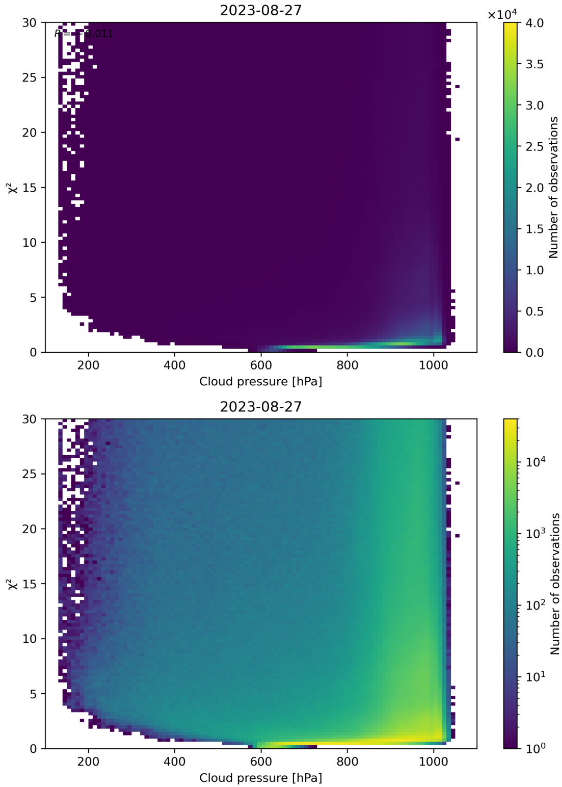
Figure 85: Scatter density plot of “Cloud pressure” against “ \chi^2 ” for 2023-08-26 to 2023-08-28.
