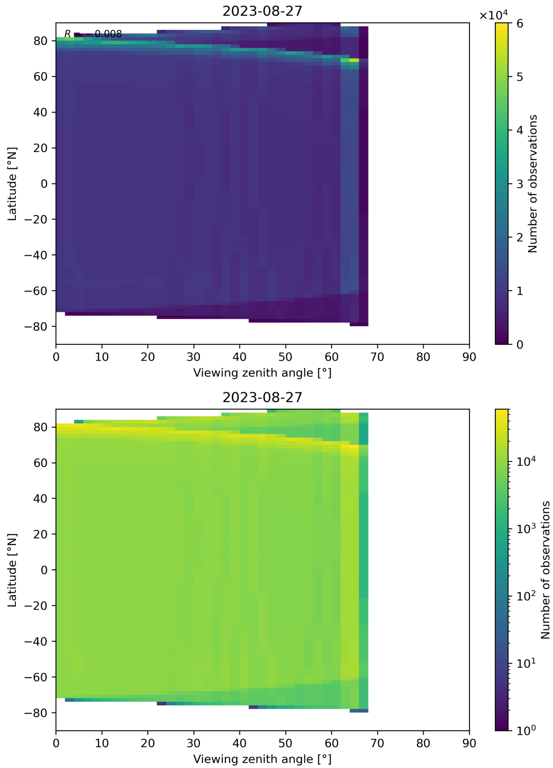
Figure 135: Scatter density plot of “Viewing zenith angle” against “Latitude” for 2023-08-26 to 2023-08-28.
