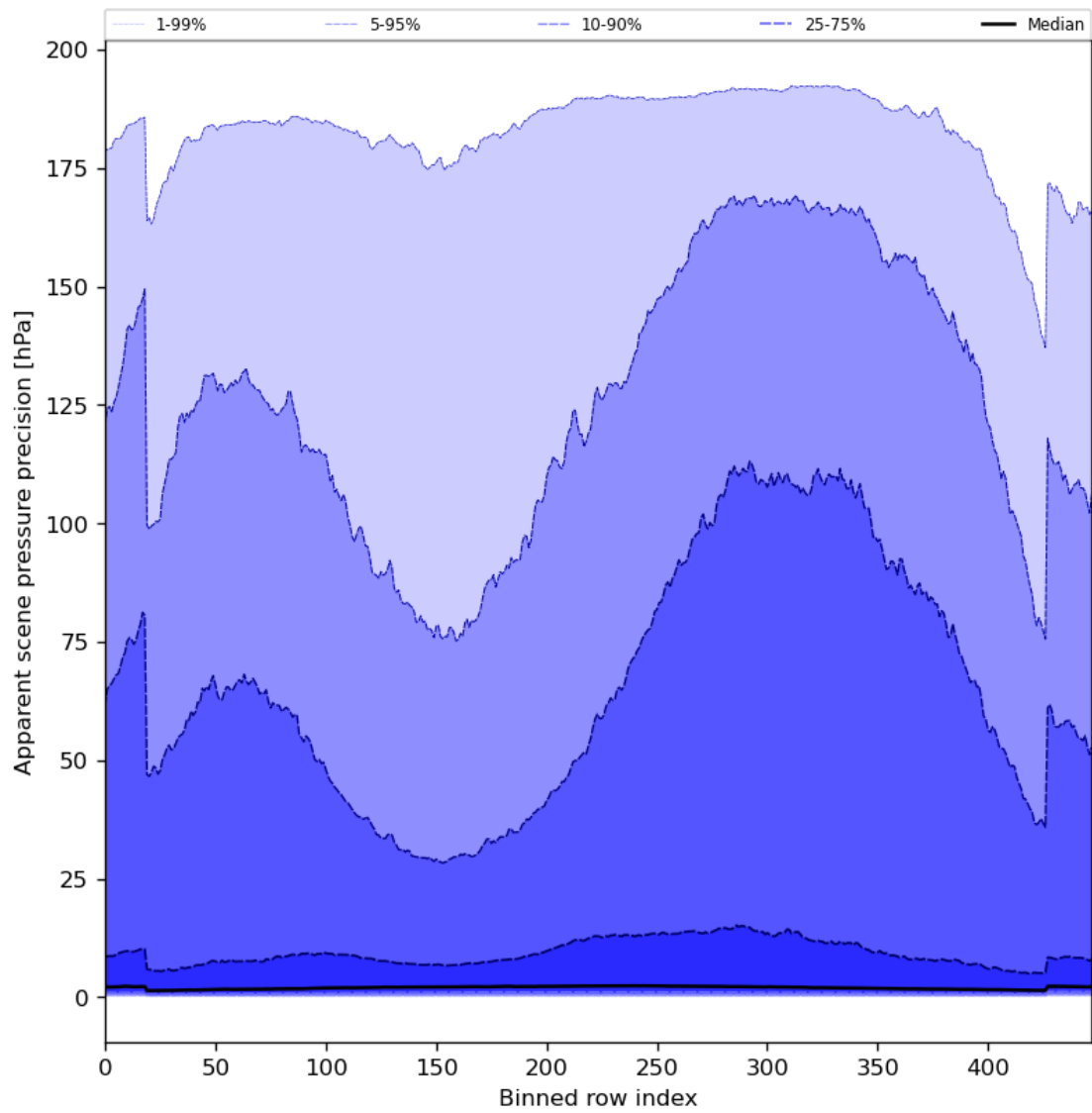
Figure 54: Along track statistics of “Apparent scene pressure precision” for 2023-08-26 to 2023-08-28
