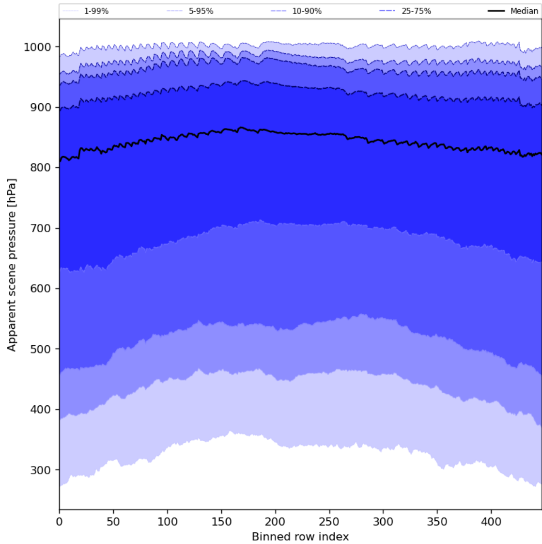
Figure 53: Along track statistics of “Apparent scene pressure” for 2023-08-26 to 2023-08-28
