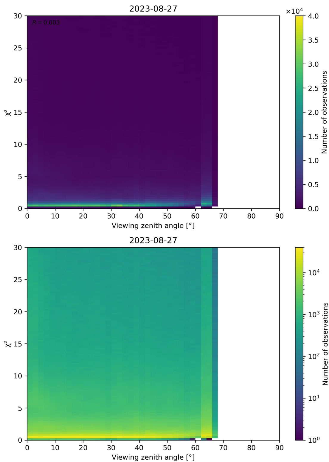
Figure 130: Scatter density plot of “Viewing zenith angle” against “ \chi^2 ” for 2023-08-26 to 2023-08-28.
