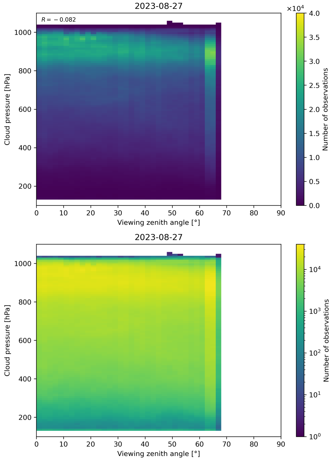
Figure 133: Scatter density plot of “Viewing zenith angle” against “Cloud pressure” for 2023-08-26 to 2023-08-28.
