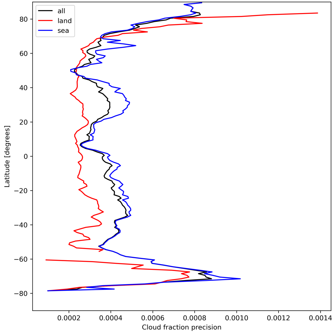
Figure 16: Zonal average of “Cloud fraction precision” for 2023-08-26 to 2023-08-28.
