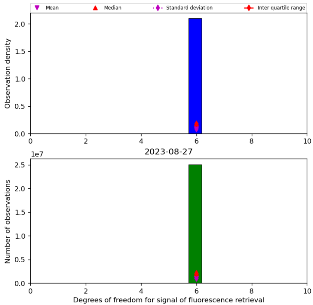
Figure 43: Histogram of "Degrees of freedom for signal of fluorescence retrieval" for 2023-08-26 to 2023-08-28
