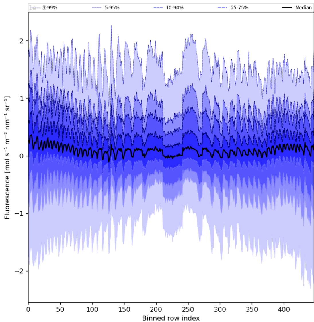
Figure 57: Along track statistics of “Fluorescence” for 2023-08-26 to 2023-08-28
