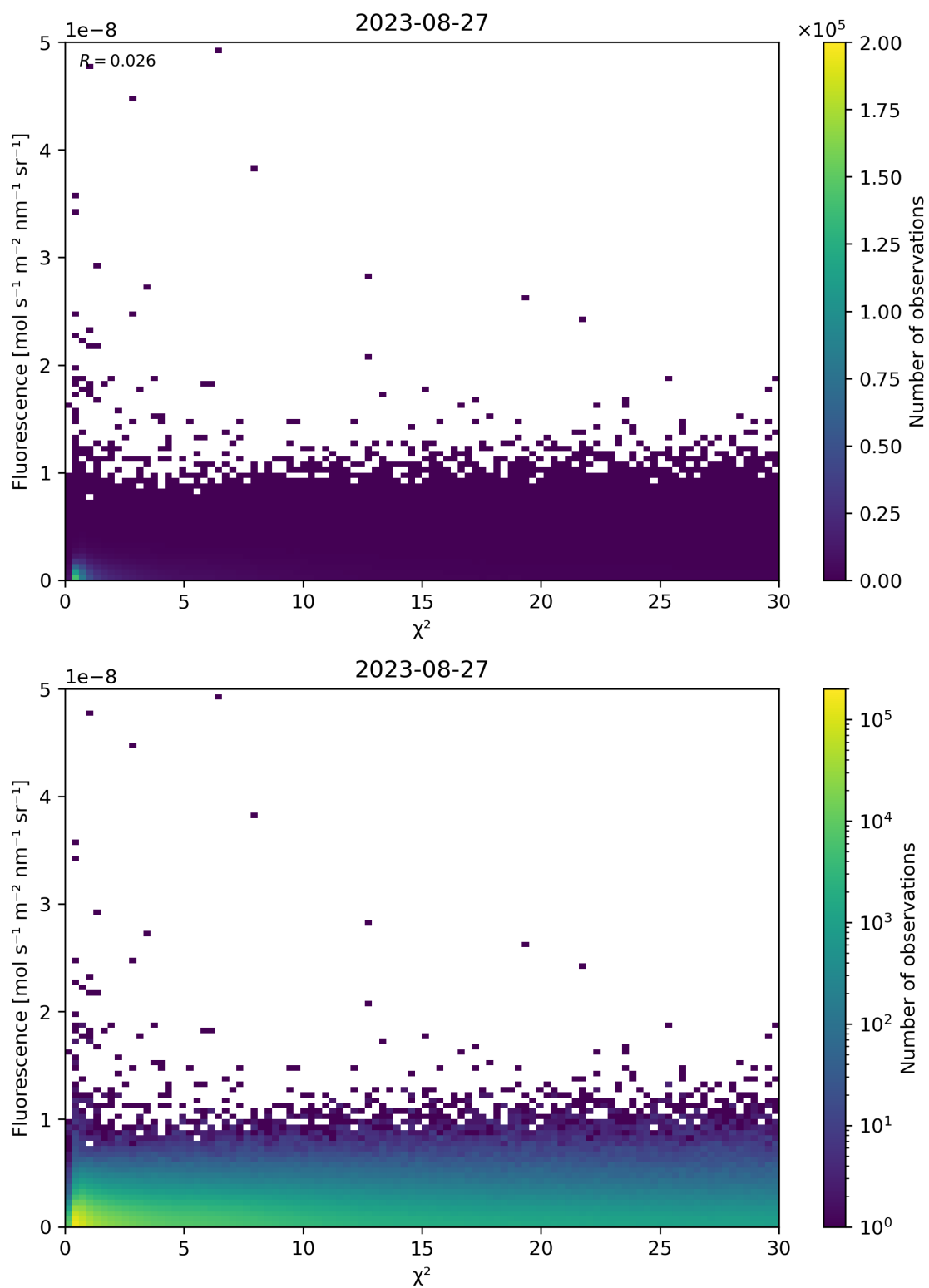
Figure 70: Scatter density plot of “ \chi^2 ” against “Fluorescence” for 2023-08-26 to 2023-08-28.
