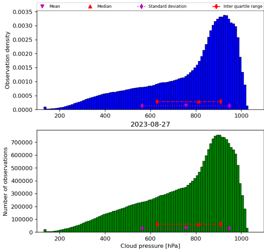
Figure 30: Histogram of “Cloud pressure” for 2023-08-26 to 2023-08-28
