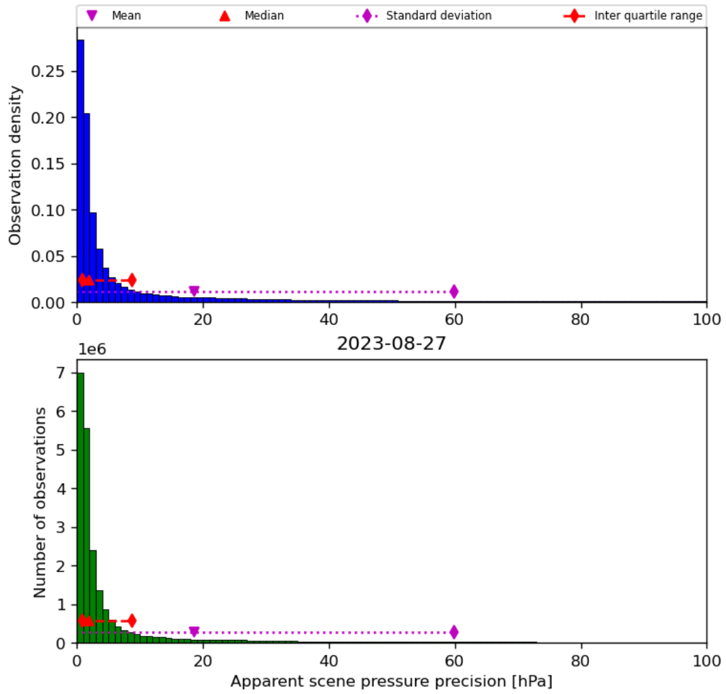
Figure 37: Histogram of “Apparent scene pressure precision” for 2023-08-26 to 2023-08-28
