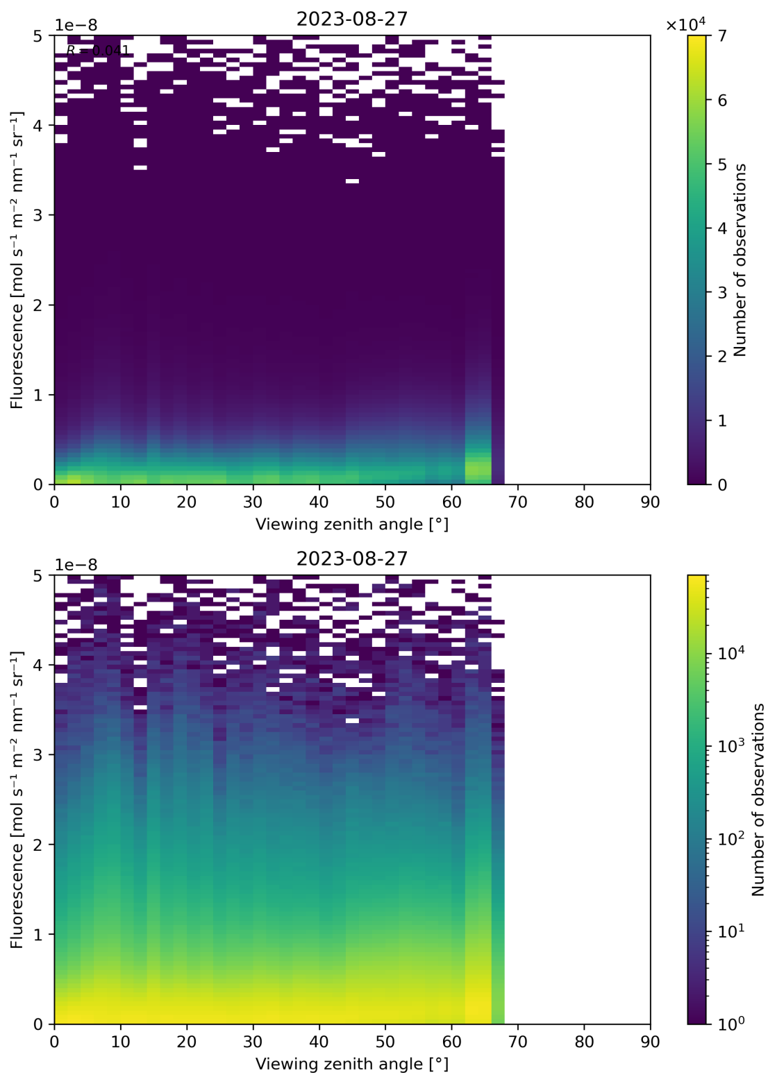
Figure 134: Scatter density plot of “Viewing zenith angle” against “Fluorescence” for 2023-08-26 to 2023-08-28.
