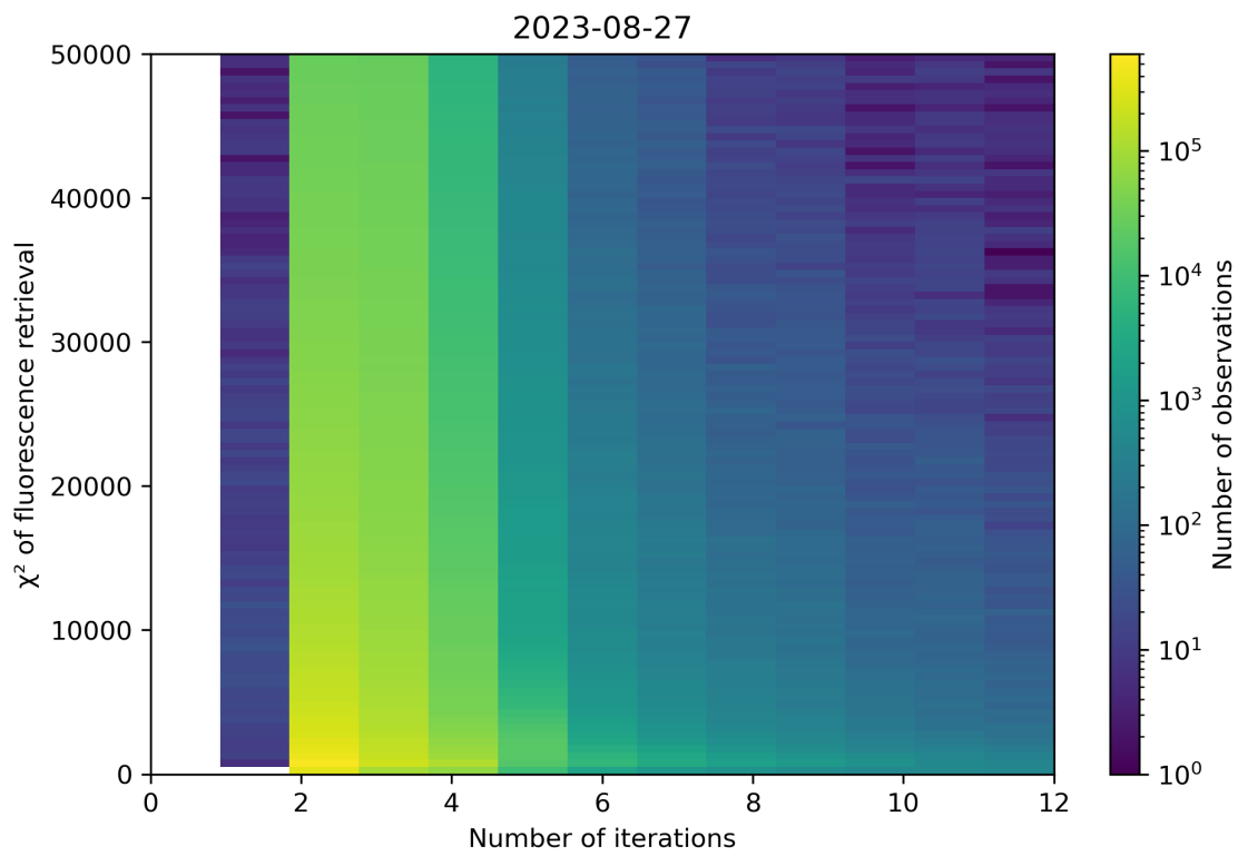
Figure 106: Scatter density plot of “Number of iterations” against “ \chi^2 of fluorescence retrieval” for 2023-08-26 to 2023-08-28.
