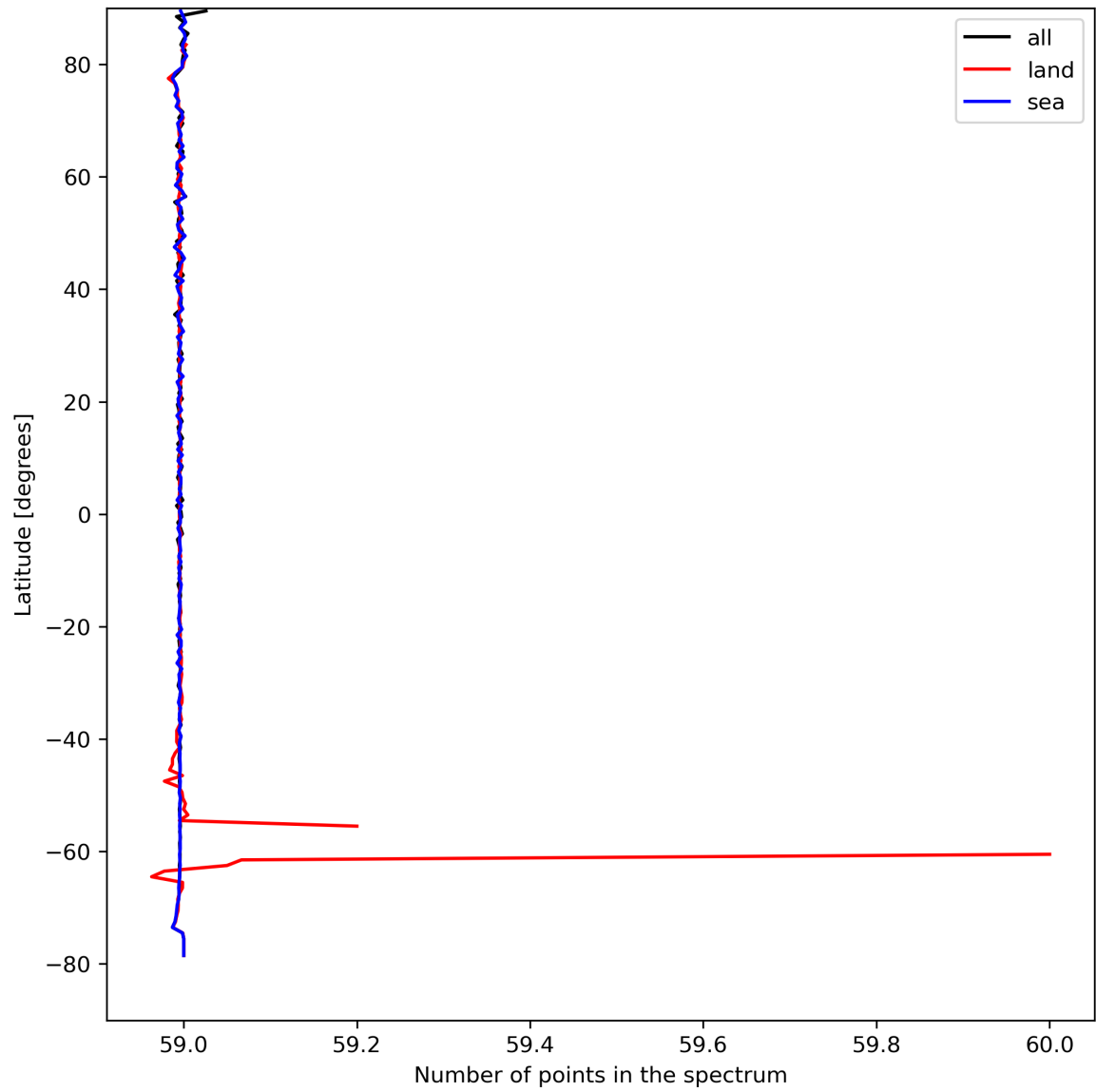
Figure 27: Zonal average of “Number of points in the spectrum” for 2023-08-26 to 2023-08-28.
