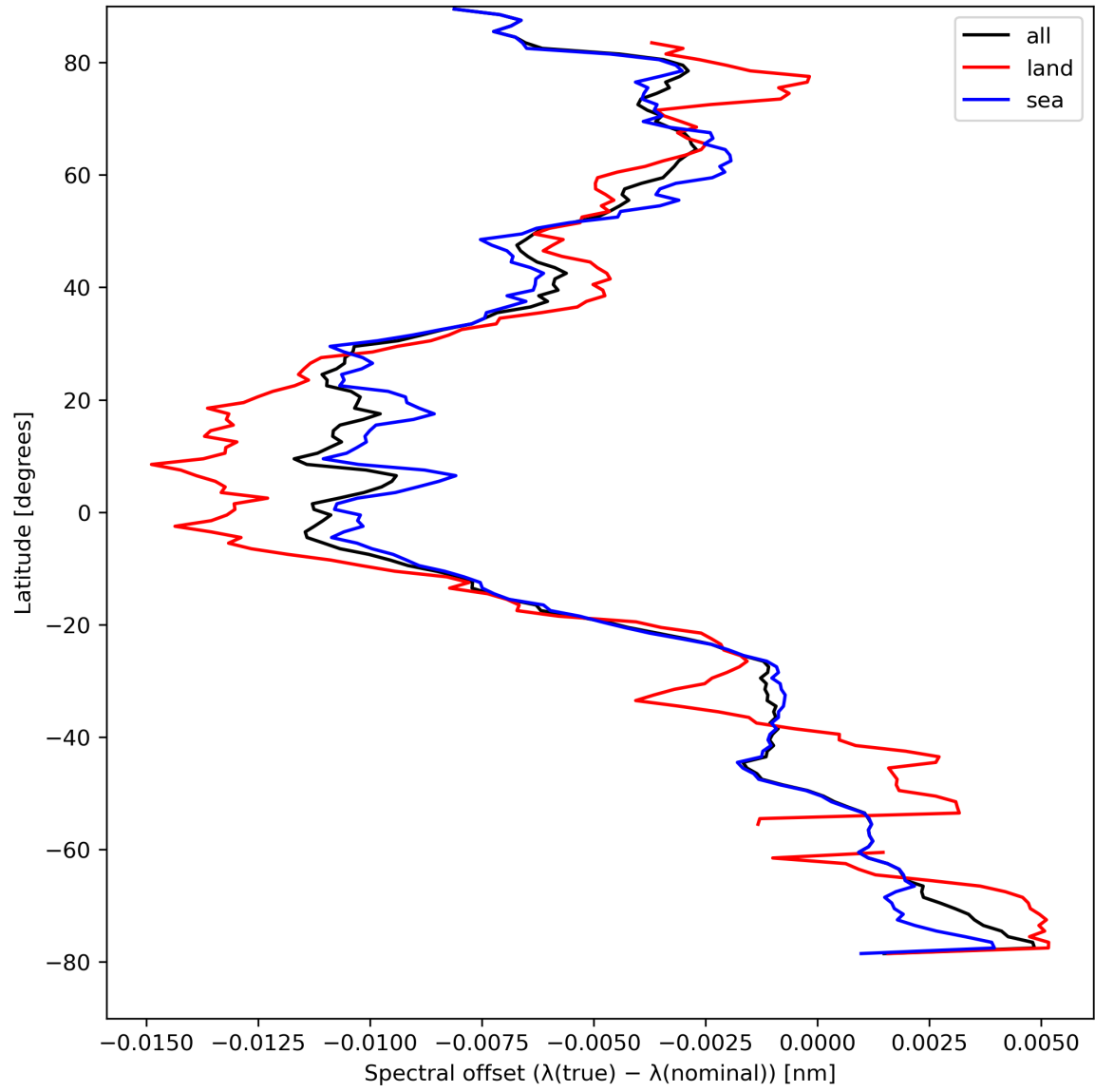
Figure 28: Zonal average of “Spectral offset ( \lambda(\text{true}) - \lambda(\text{nominal}) )” for 2023-08-26 to 2023-08-28.
