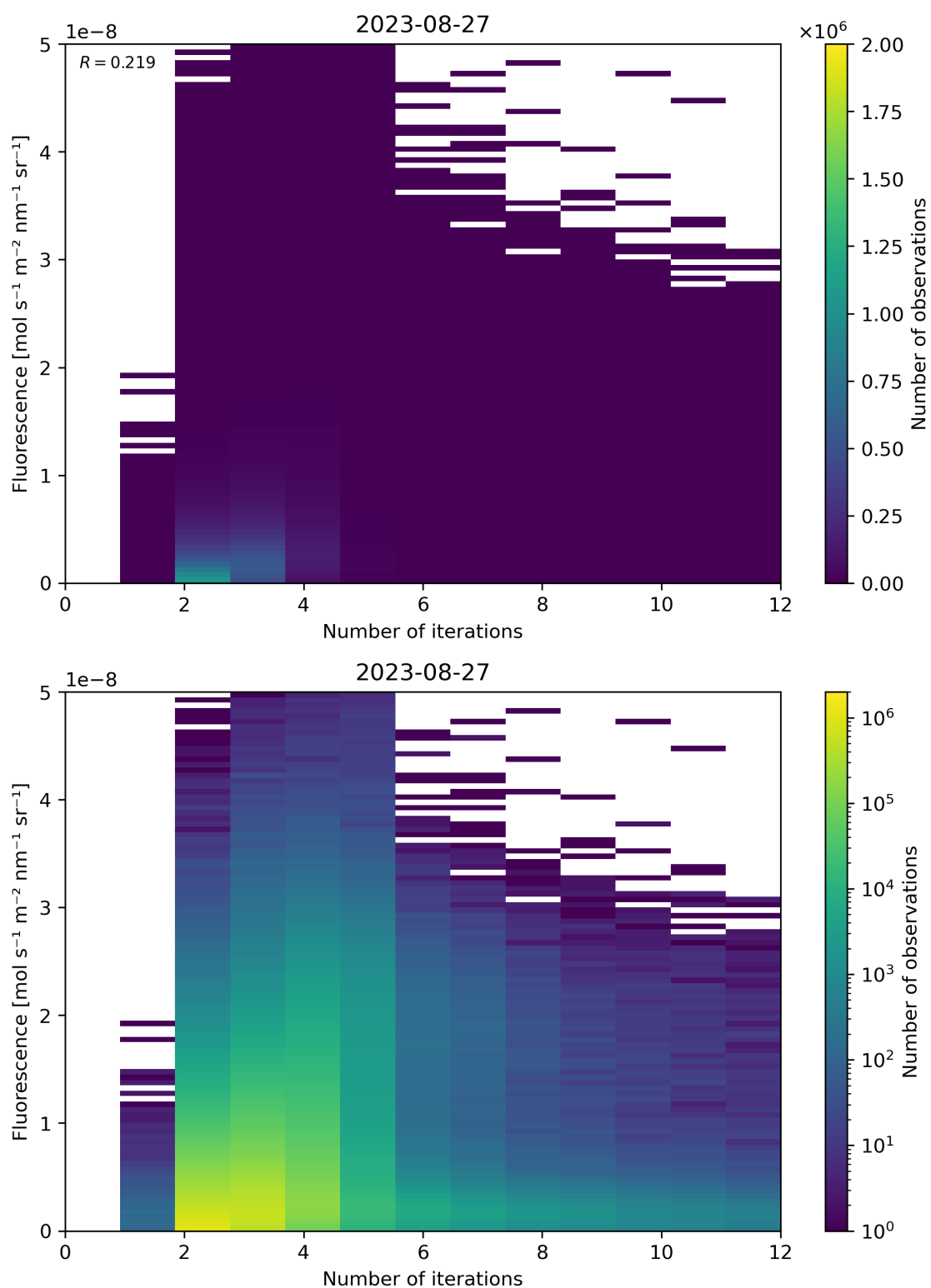
Figure 107: Scatter density plot of “Number of iterations” against “Fluorescence” for 2023-08-26 to 2023-08-28.
