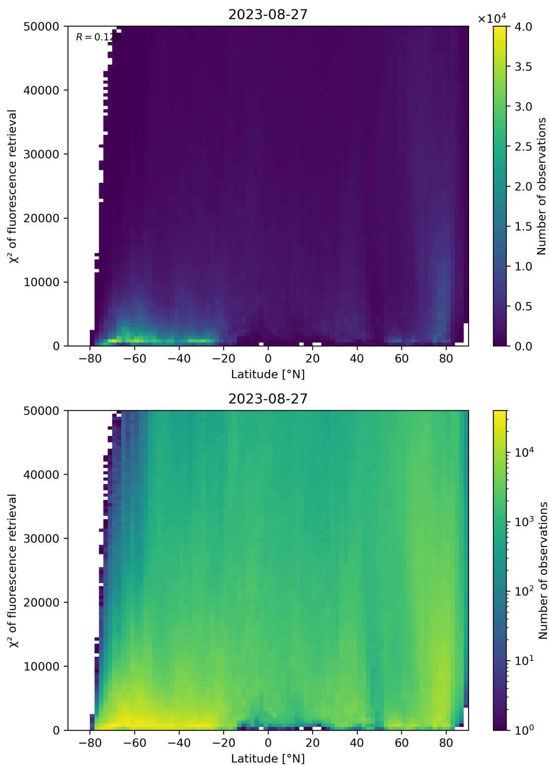
Figure 98: Scatter density plot of “Latitude” against “ \chi^2 of fluorescence retrieval” for 2023-08-26 to 2023-08-28.
