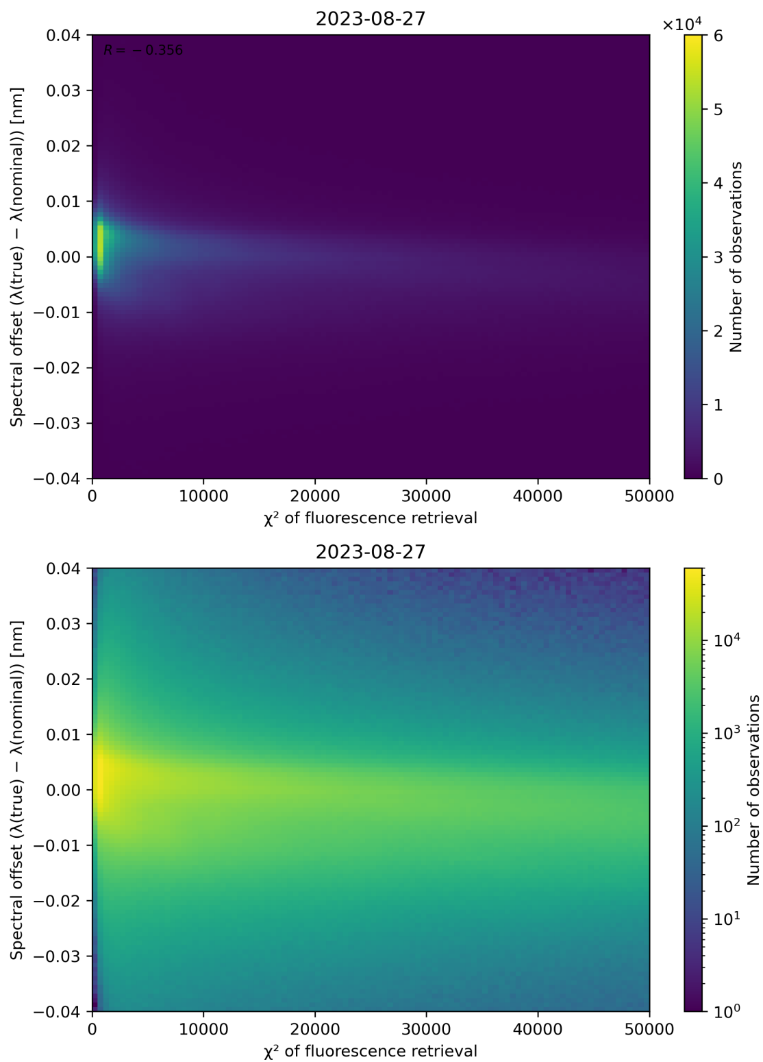
Figure 72: Scatter density plot of " \chi^2 of fluorescence retrieval" against "Spectral offset ( \lambda(\text{true}) - \lambda(\text{nominal})) " for 2023-08-26 to 2023-08-28.
