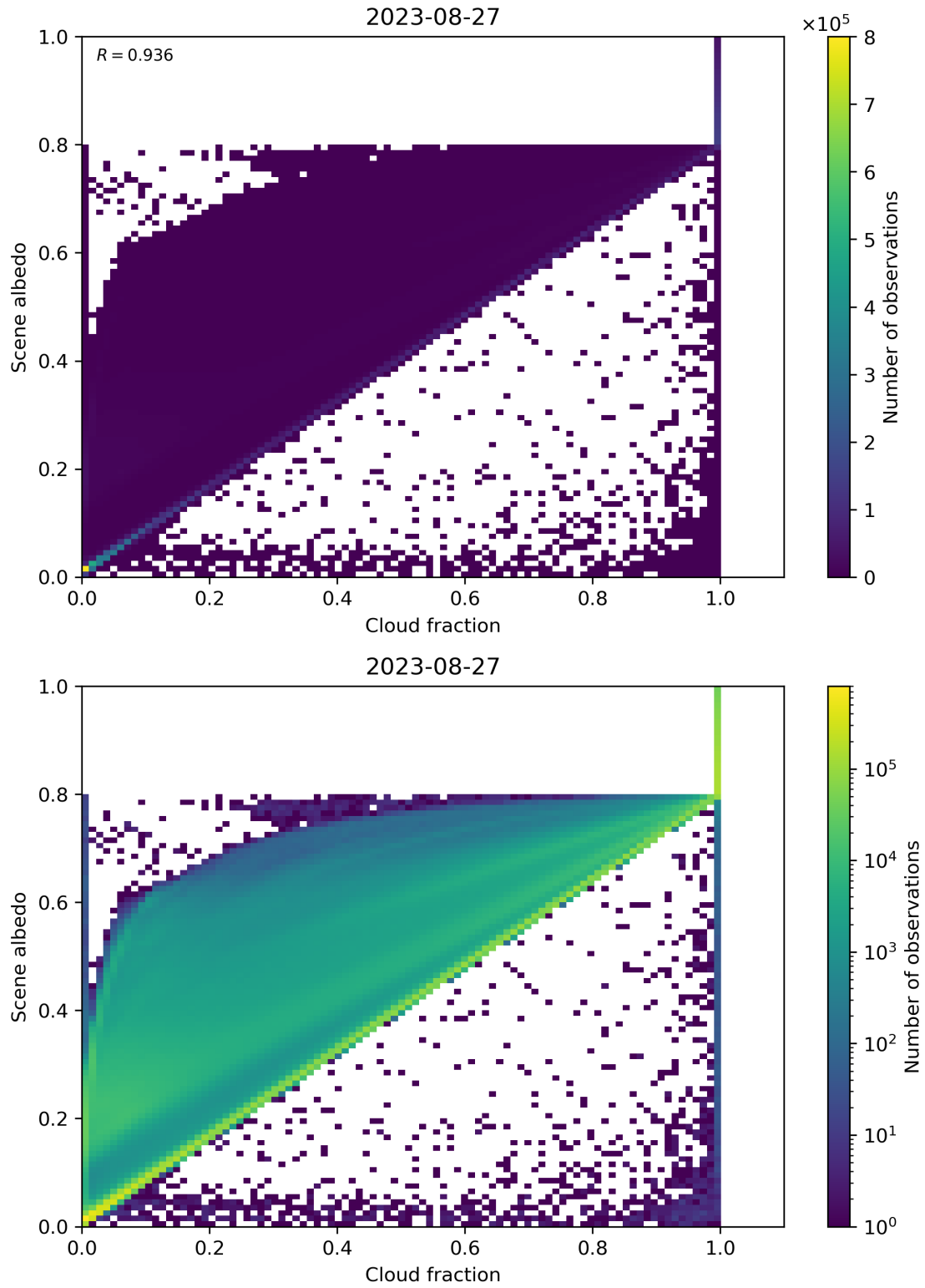
Figure 82: Scatter density plot of “Cloud fraction” against “Scene albedo” for 2023-08-26 to 2023-08-28.
