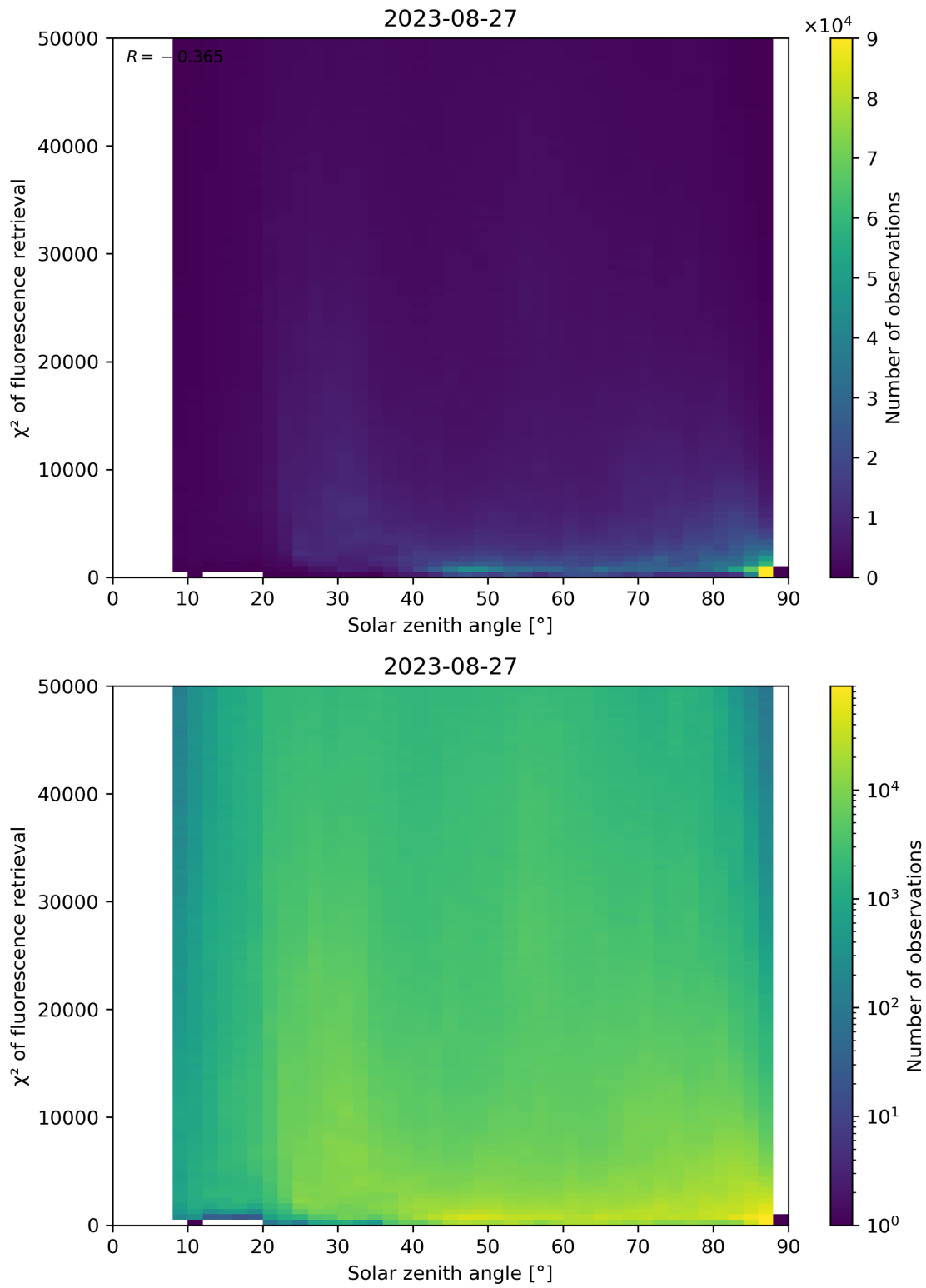
Figure 120: Scatter density plot of “Solar zenith angle” against “ \chi^2 of fluorescence retrieval” for 2023-08-26 to 2023-08-28.
