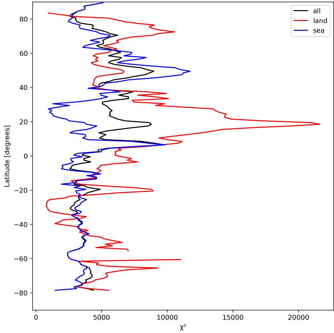
Figure 21: Zonal average of “ \chi^2 ” for 2023-08-26 to 2023-08-28.
