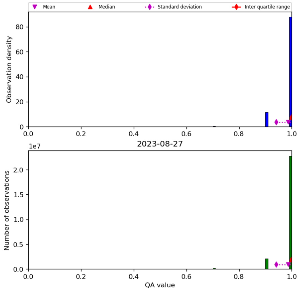
Figure 29: Histogram of “QA value” for 2023-08-26 to 2023-08-28
