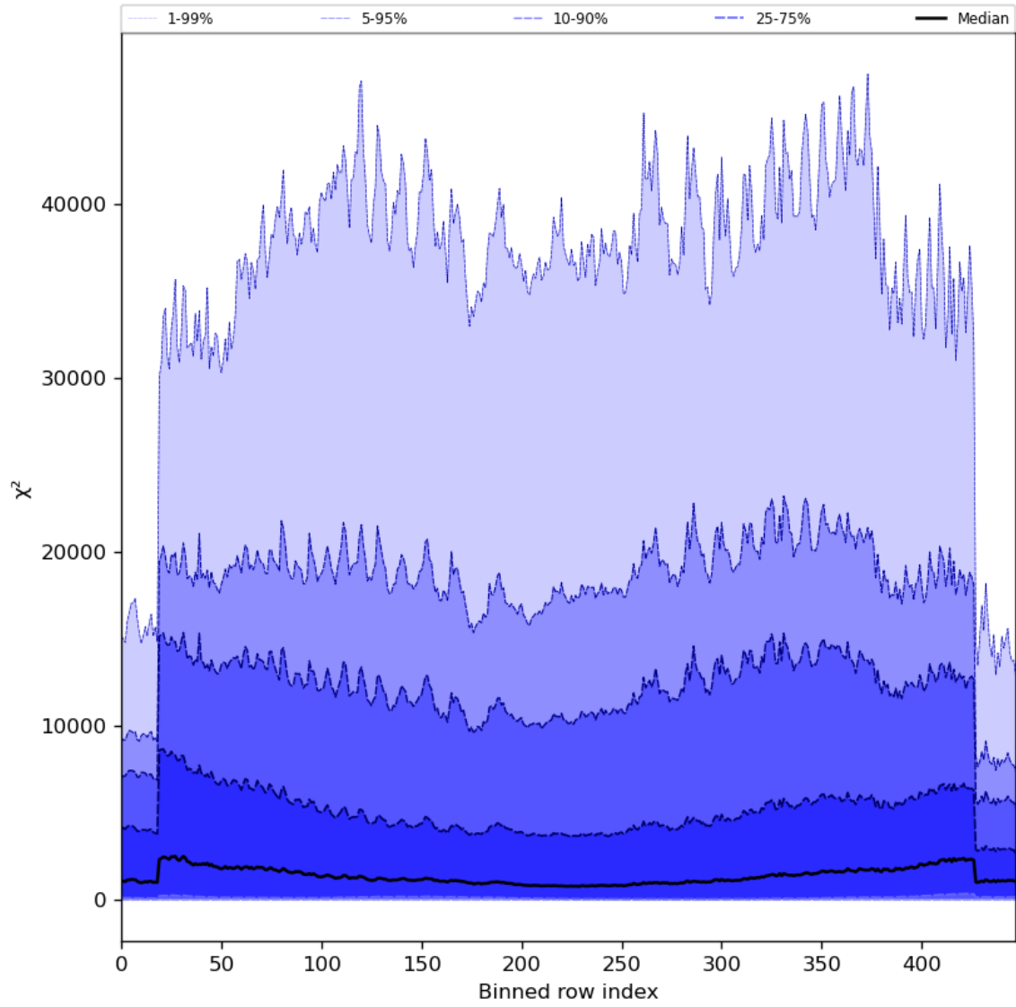
Figure 55: Along track statistics of “ \chi^2 ” for 2023-08-26 to 2023-08-28
