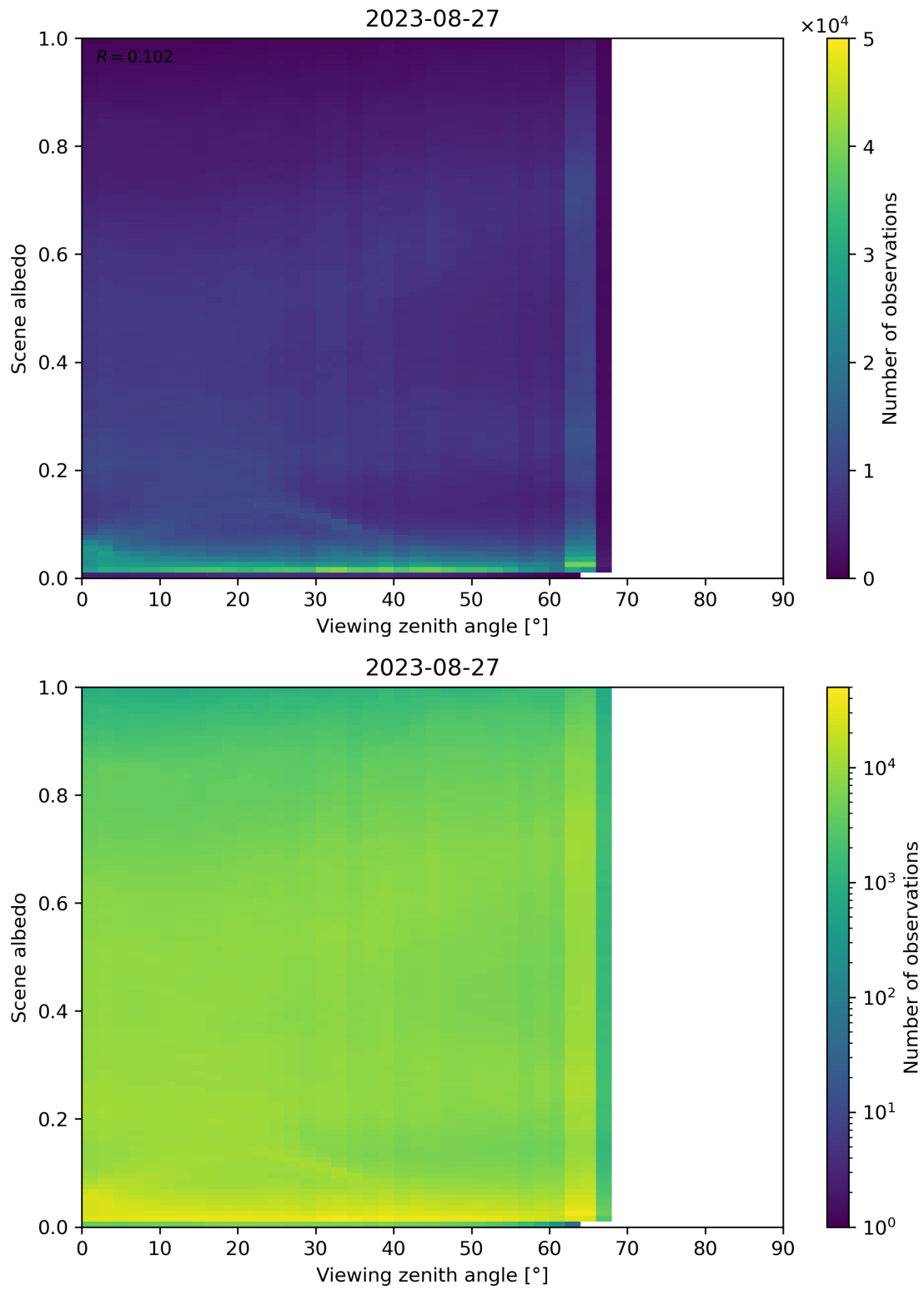
Figure 138: Scatter density plot of “Viewing zenith angle” against “Scene albedo” for 2023-08-26 to 2023-08-28.
