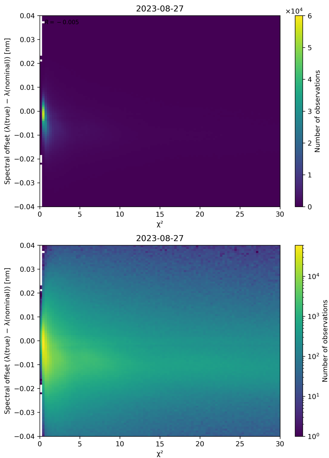
Figure 75: Scatter density plot of “ \chi^2 ” against “Spectral offset ( \lambda(\text{true}) - \lambda(\text{nominal}) )” for 2023-08-26 to 2023-08-28.
