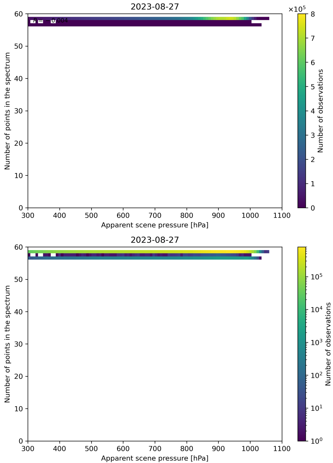
Figure 67: Scatter density plot of “Apparent scene pressure” against “Number of points in the spectrum” for 2023-08-26 to 2023-08-28.
