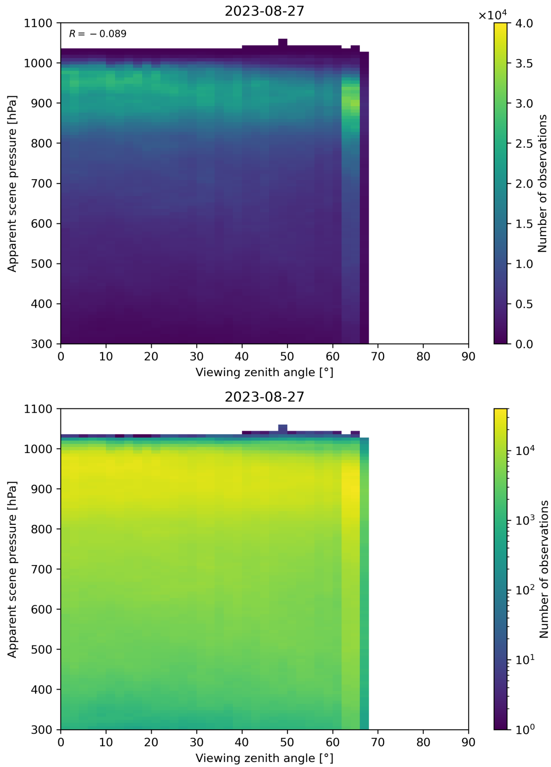
Figure 129: Scatter density plot of “Viewing zenith angle” against “Apparent scene pressure” for 2023-08-26 to 2023-08-28.
