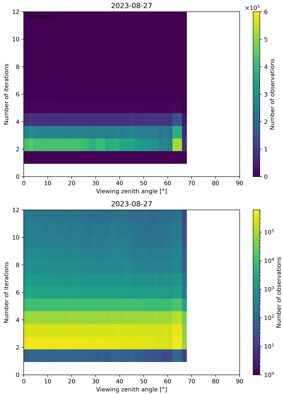
Figure 136: Scatter density plot of “Viewing zenith angle” against “Number of iterations” for 2023-08-26 to 2023-08-28.
