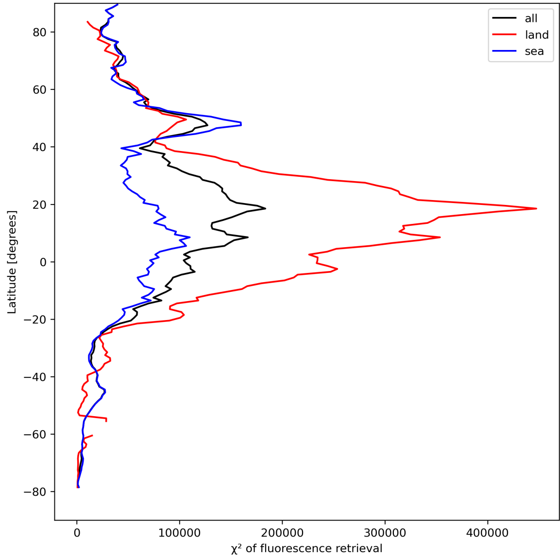
Figure 25: Zonal average of “ \chi^2 of fluorescence retrieval” for 2023-08-26 to 2023-08-28.
