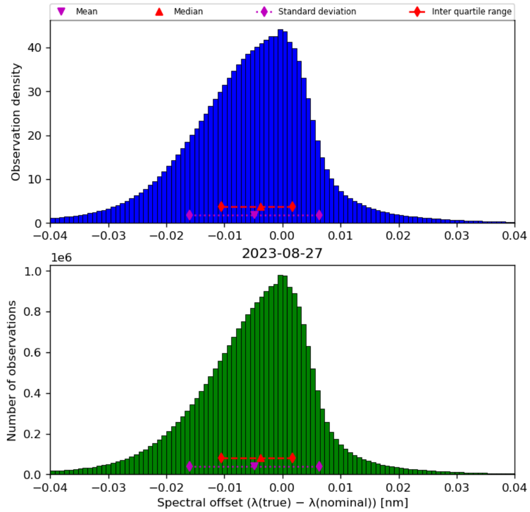
Figure 45: Histogram of “Spectral offset ( \lambda(\text{true}) - \lambda(\text{nominal}) )” for 2023-08-26 to 2023-08-28
