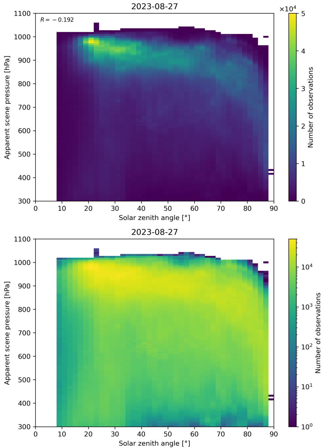
Figure 118: Scatter density plot of “Solar zenith angle” against “Apparent scene pressure” for 2023-08-26 to 2023-08-28.
