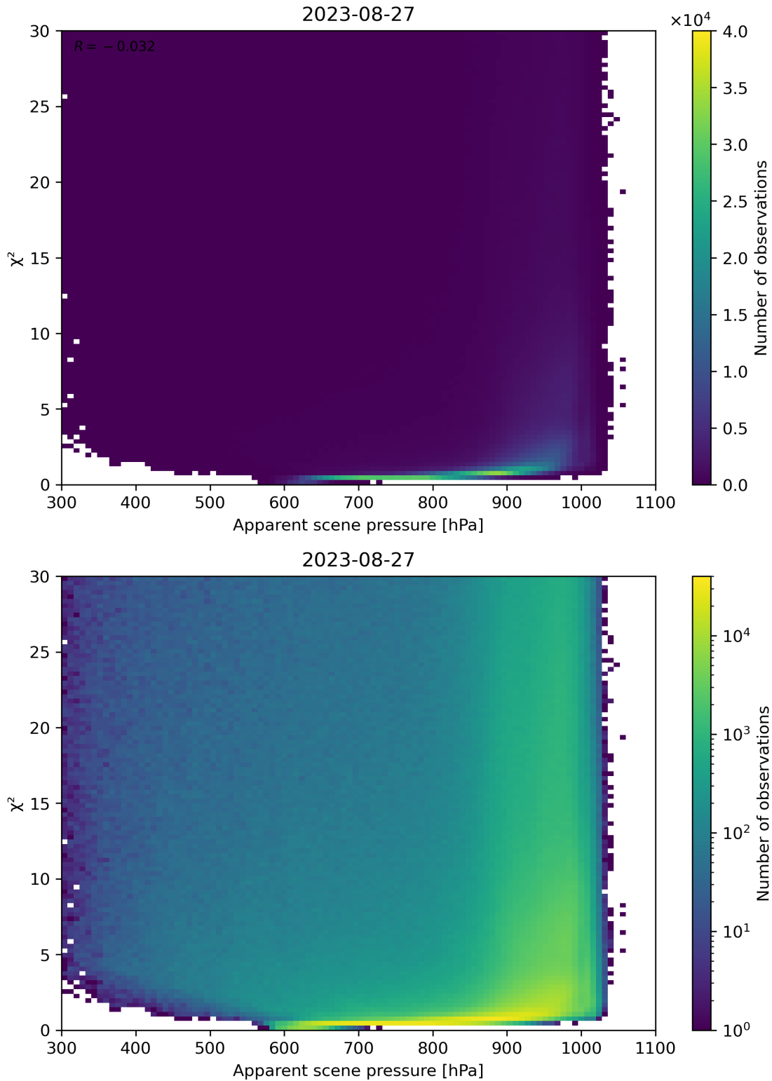
Figure 63: Scatter density plot of “Apparent scene pressure” against “ \chi^2 ” for 2023-08-26 to 2023-08-28.
