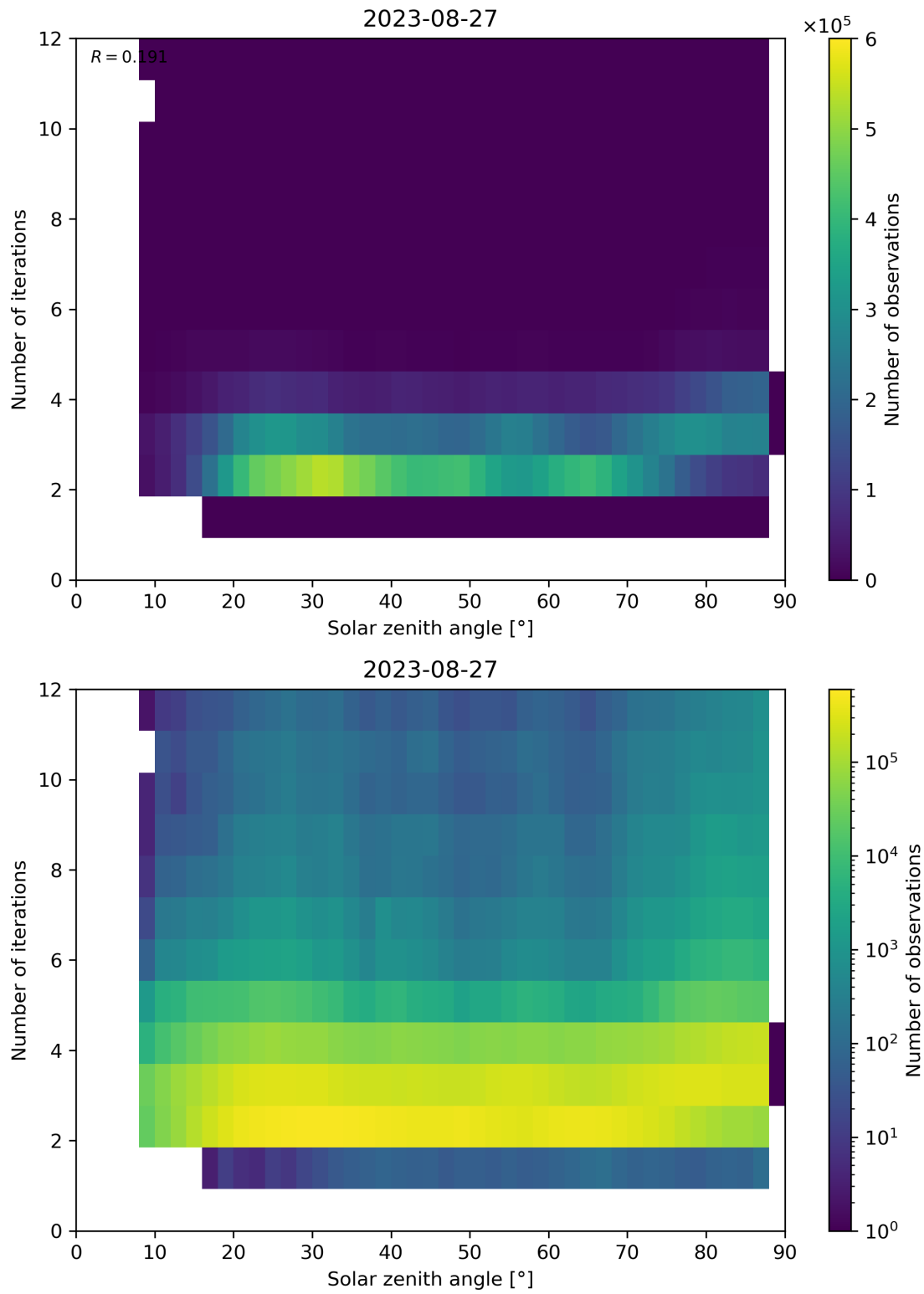
Figure 125: Scatter density plot of “Solar zenith angle” against “Number of iterations” for 2023-08-26 to 2023-08-28.
