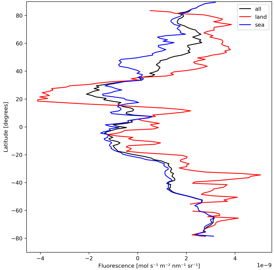
Figure 23: Zonal average of “Fluorescence” for 2023-08-26 to 2023-08-28.
