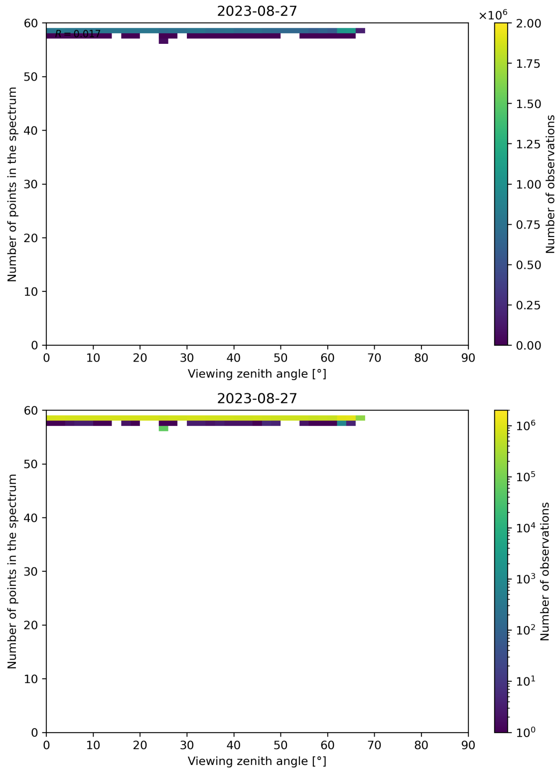
Figure 137: Scatter density plot of “Viewing zenith angle” against “Number of points in the spectrum” for 2023-08-26 to 2023-08-28.
