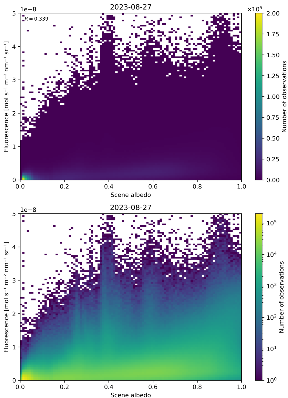
Figure 114: Scatter density plot of “Scene albedo” against “Fluorescence” for 2023-08-26 to 2023-08-28.
