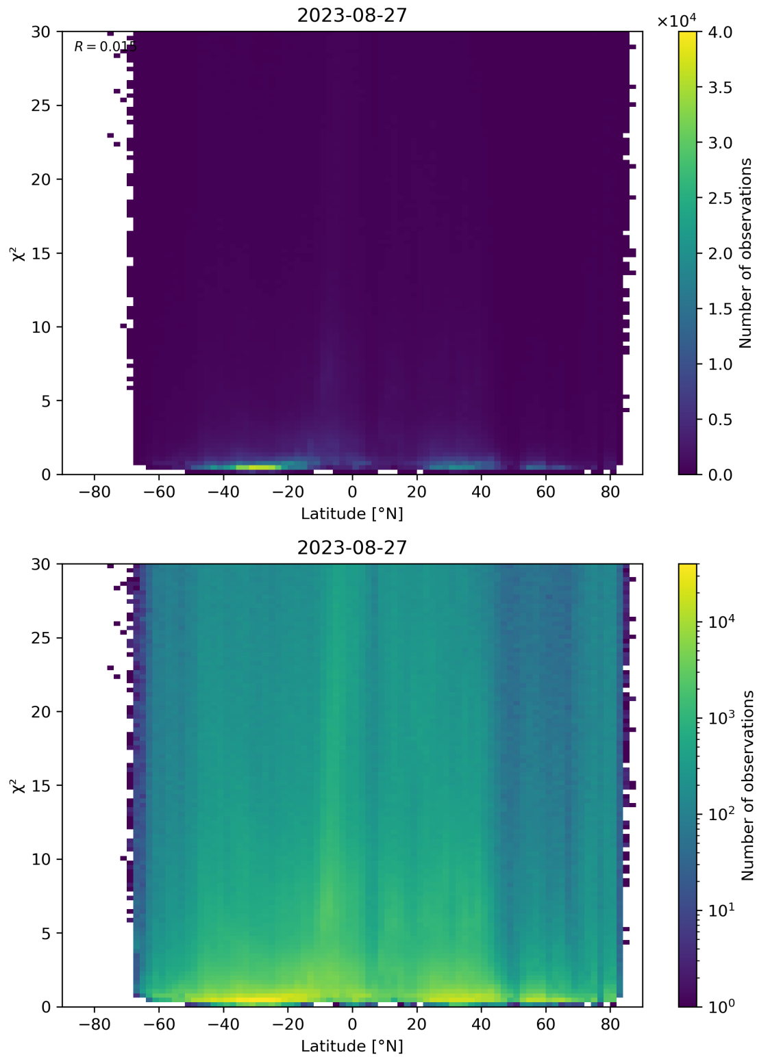
Figure 97: Scatter density plot of “Latitude” against “ \chi^2 ” for 2023-08-26 to 2023-08-28.
