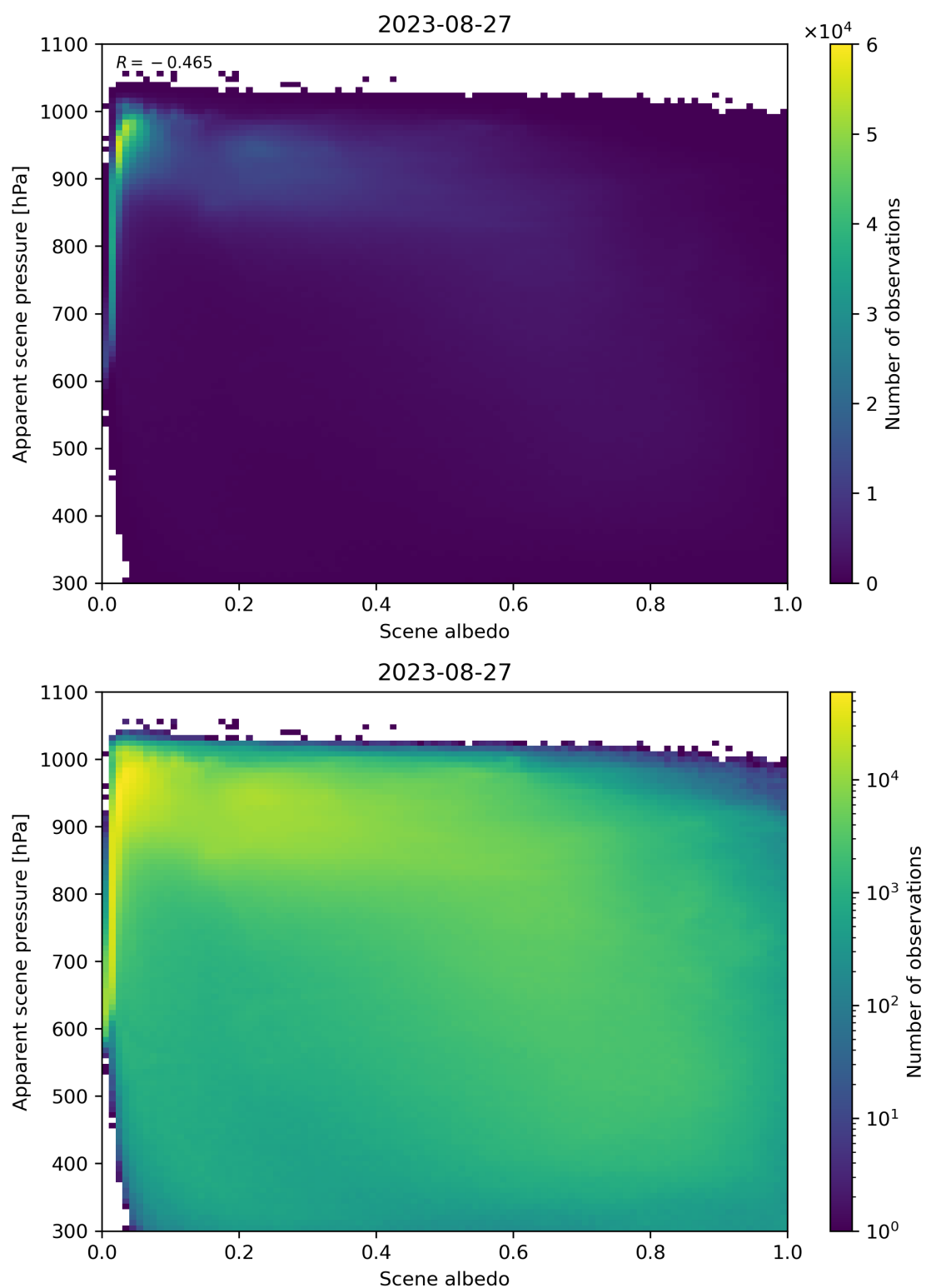
Figure 111: Scatter density plot of “Scene albedo” against “Apparent scene pressure” for 2023-08-26 to 2023-08-28.
