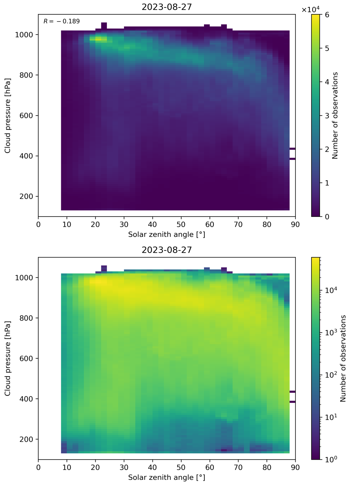
Figure 122: Scatter density plot of “Solar zenith angle” against “Cloud pressure” for 2023-08-26 to 2023-08-28.
