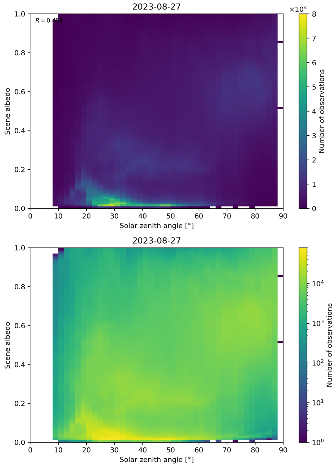
Figure 127: Scatter density plot of “Solar zenith angle” against “Scene albedo” for 2023-08-26 to 2023-08-28.
