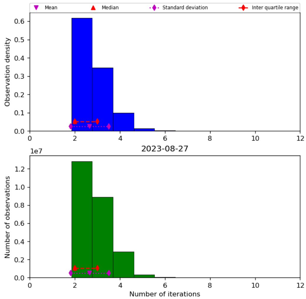
Figure 39: Histogram of “Number of iterations” for 2023-08-26 to 2023-08-28
