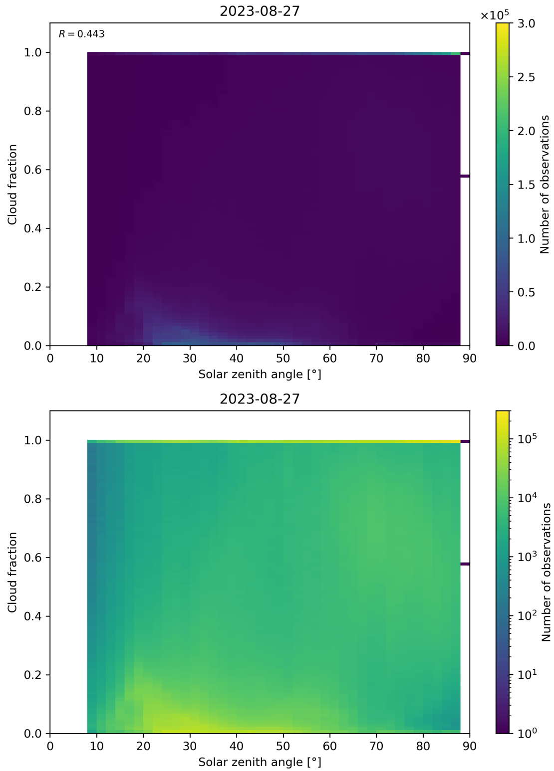
Figure 121: Scatter density plot of “Solar zenith angle” against “Cloud fraction” for 2023-08-26 to 2023-08-28.
