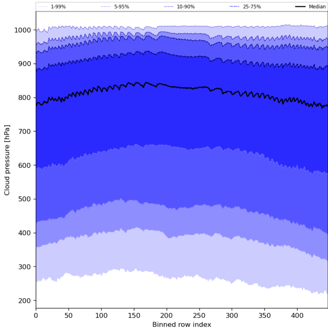
Figure 47: Along track statistics of “Cloud pressure” for 2023-08-26 to 2023-08-28
