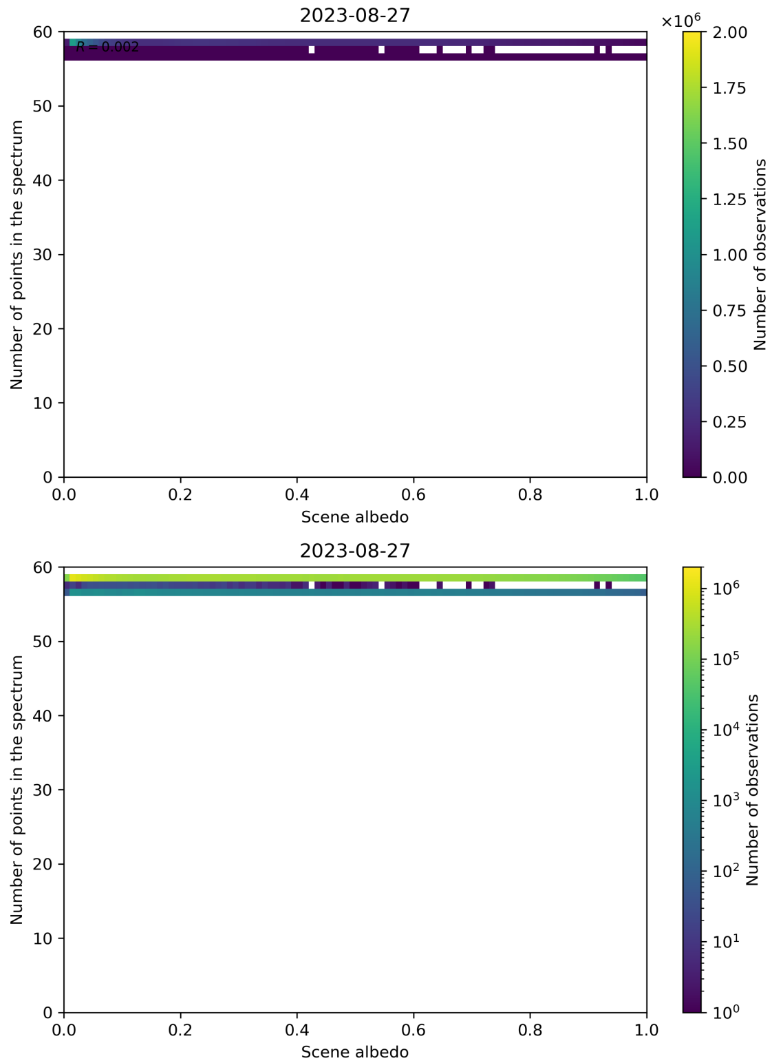
Figure 116: Scatter density plot of “Scene albedo” against “Number of points in the spectrum” for 2023-08-26 to 2023-08-28.
