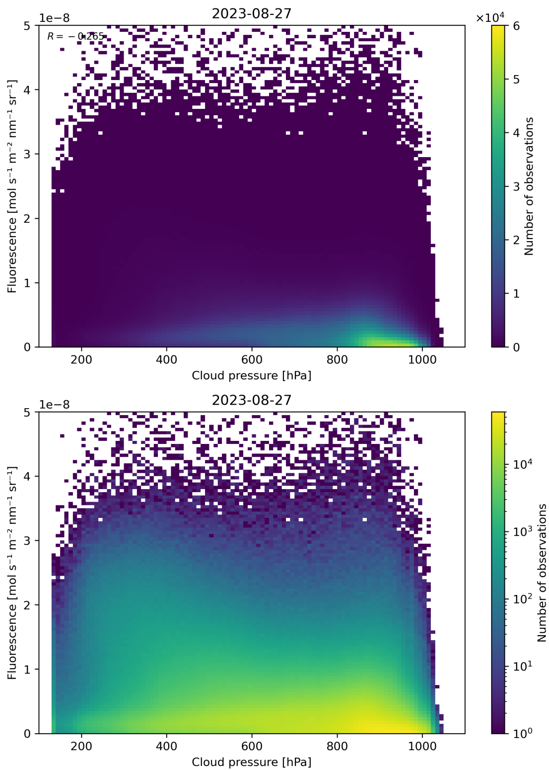
Figure 88: Scatter density plot of “Cloud pressure” against “Fluorescence” for 2023-08-26 to 2023-08-28.
