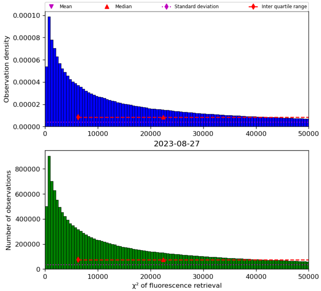
Figure 42: Histogram of “ \chi^2 of fluorescence retrieval” for 2023-08-26 to 2023-08-28
