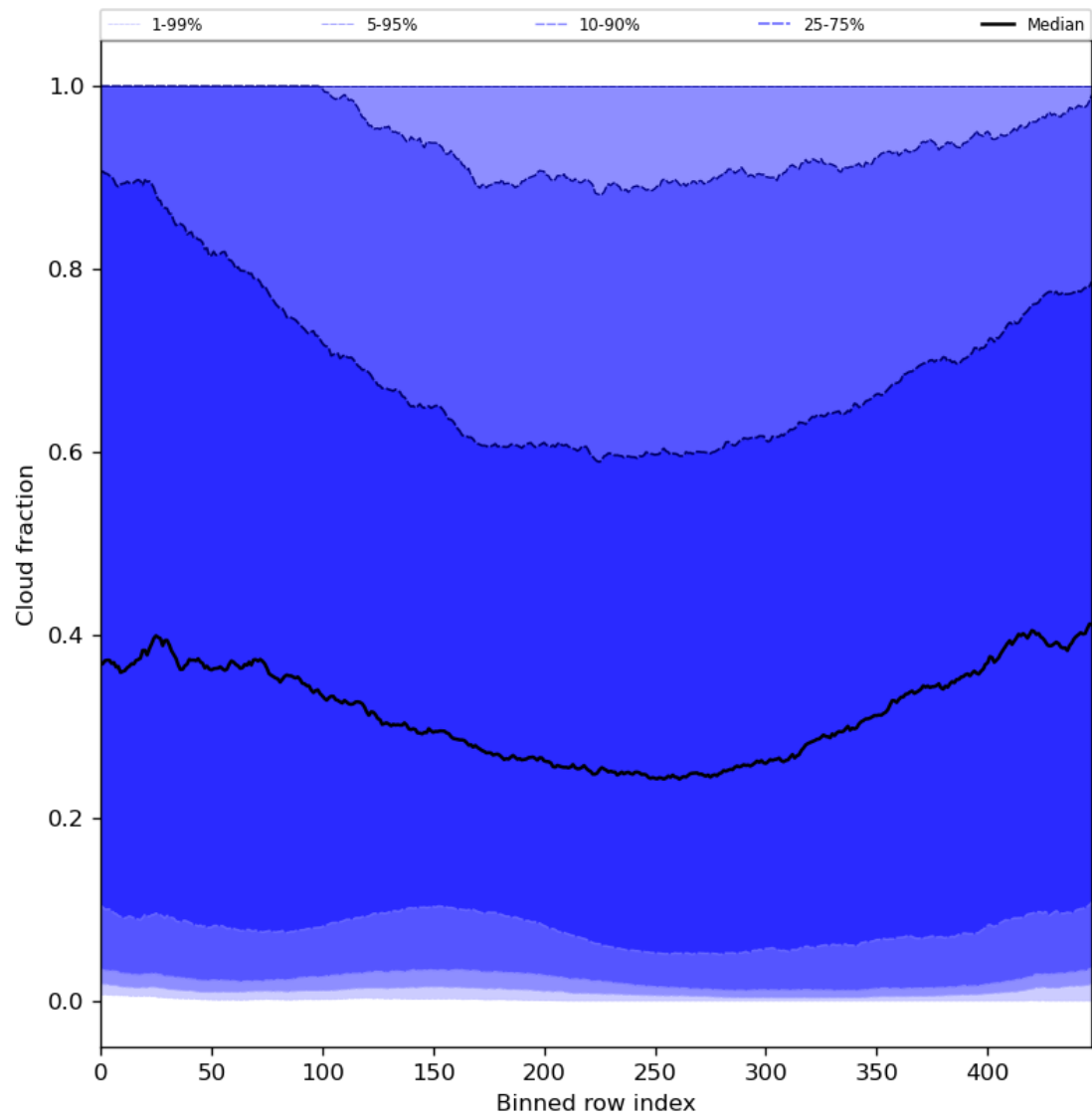
Figure 49: Along track statistics of “Cloud fraction” for 2023-08-26 to 2023-08-28
