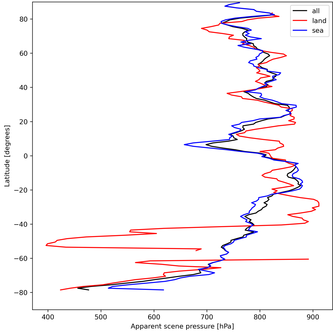
Figure 19: Zonal average of “Apparent scene pressure” for 2023-08-26 to 2023-08-28.
