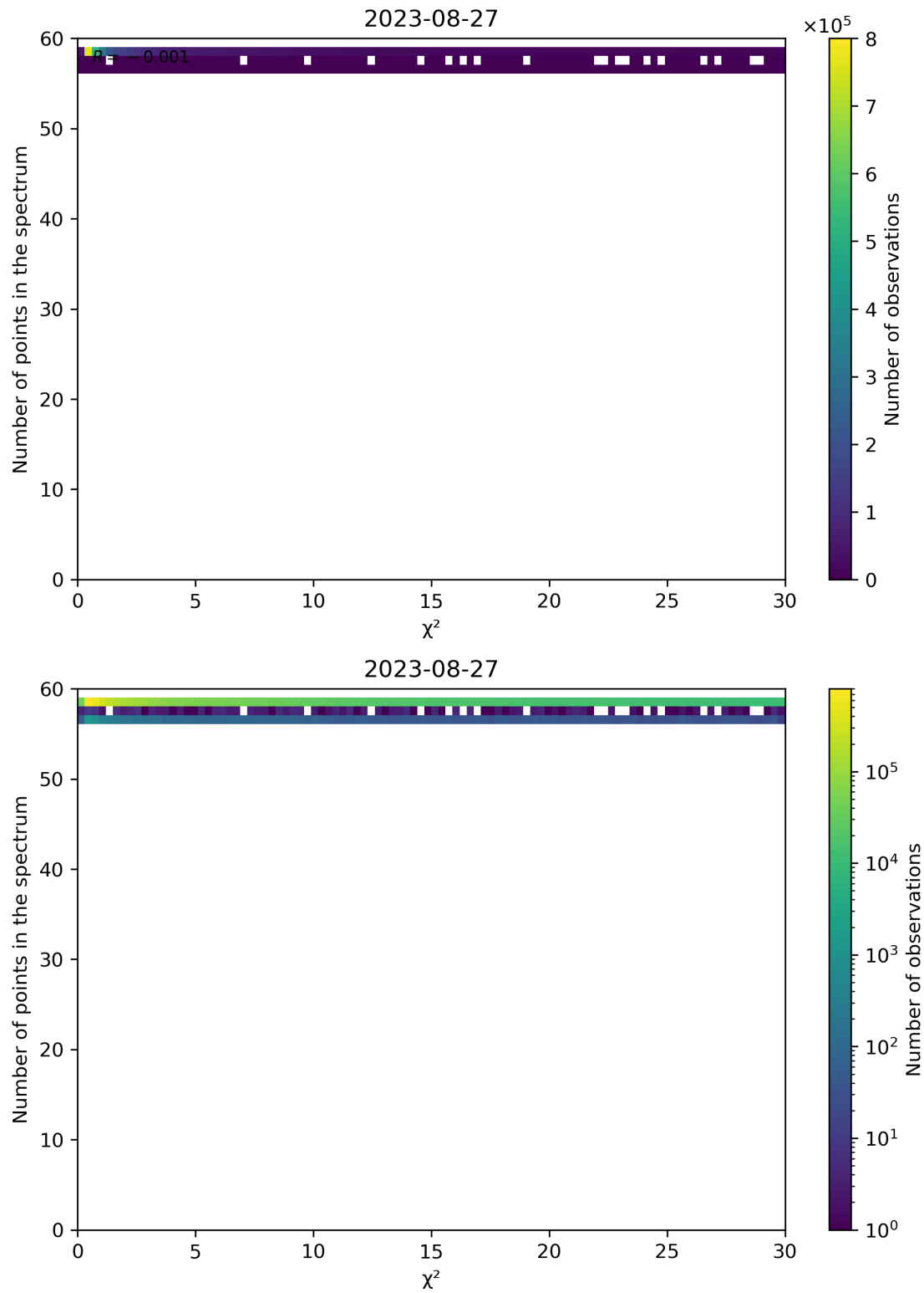
Figure 74: Scatter density plot of " \chi^2 " against "Number of points in the spectrum" for 2023-08-26 to 2023-08-28.
