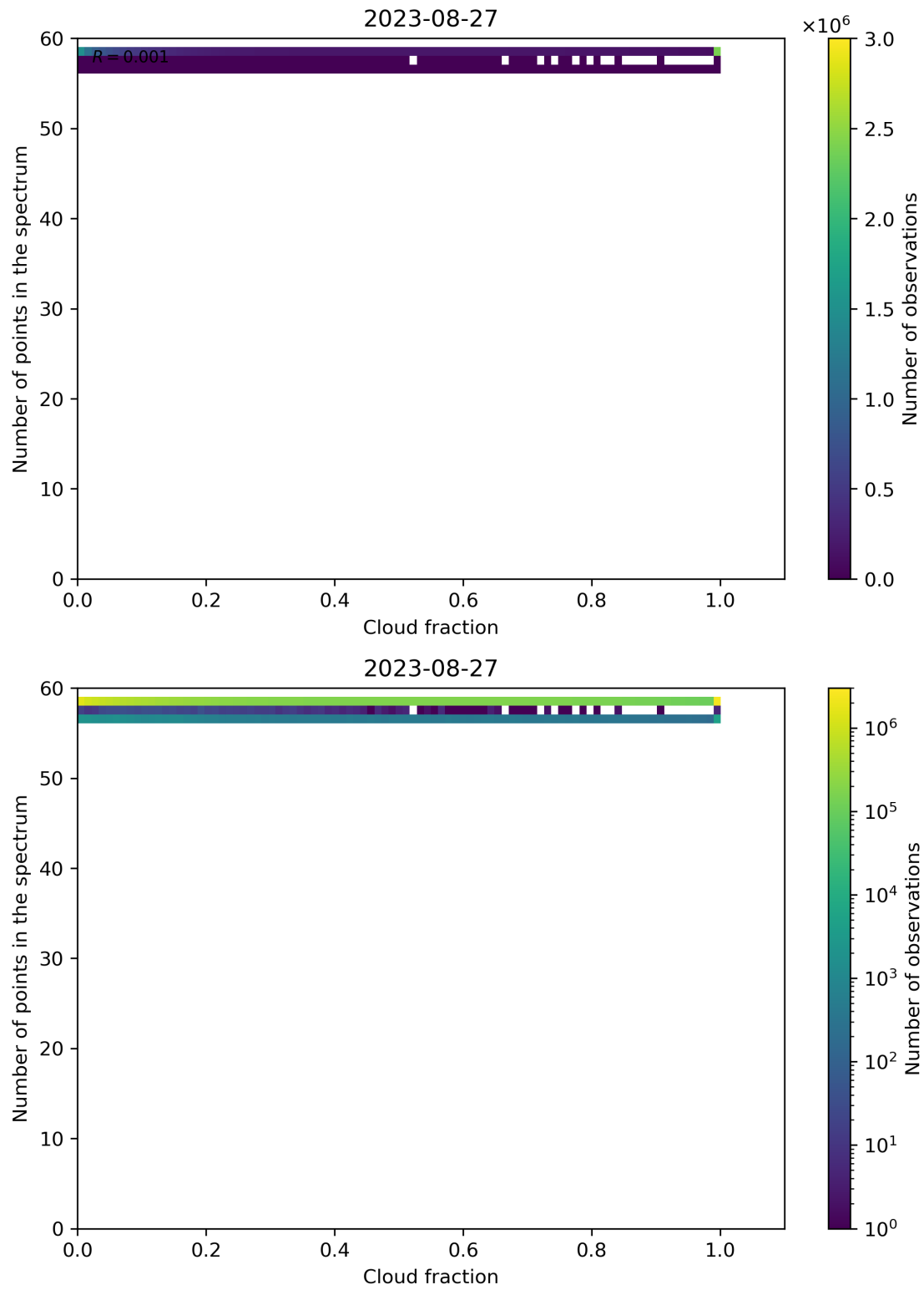
Figure 81: Scatter density plot of “Cloud fraction” against “Number of points in the spectrum” for 2023-08-26 to 2023-08-28.
