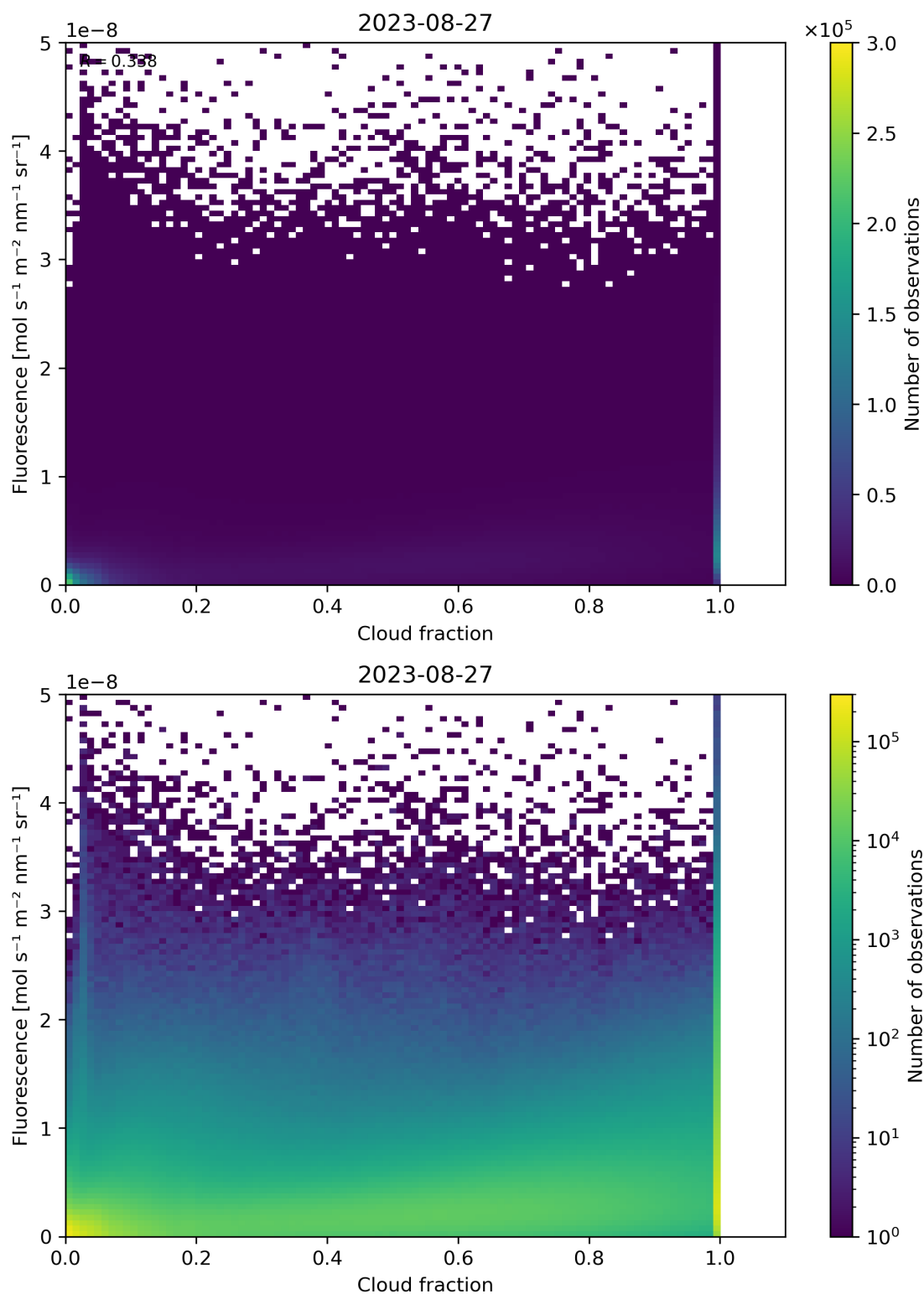
Figure 79: Scatter density plot of “Cloud fraction” against “Fluorescence” for 2023-08-26 to 2023-08-28.
