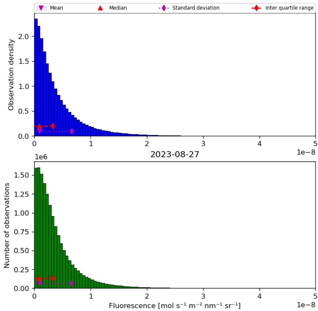
Figure 40: Histogram of “Fluorescence” for 2023-08-26 to 2023-08-28
