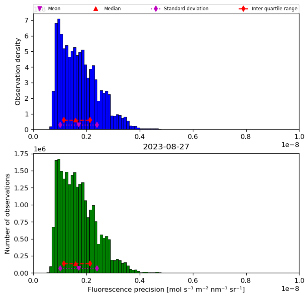
Figure 41: Histogram of “Fluorescence precision” for 2023-08-26 to 2023-08-28
