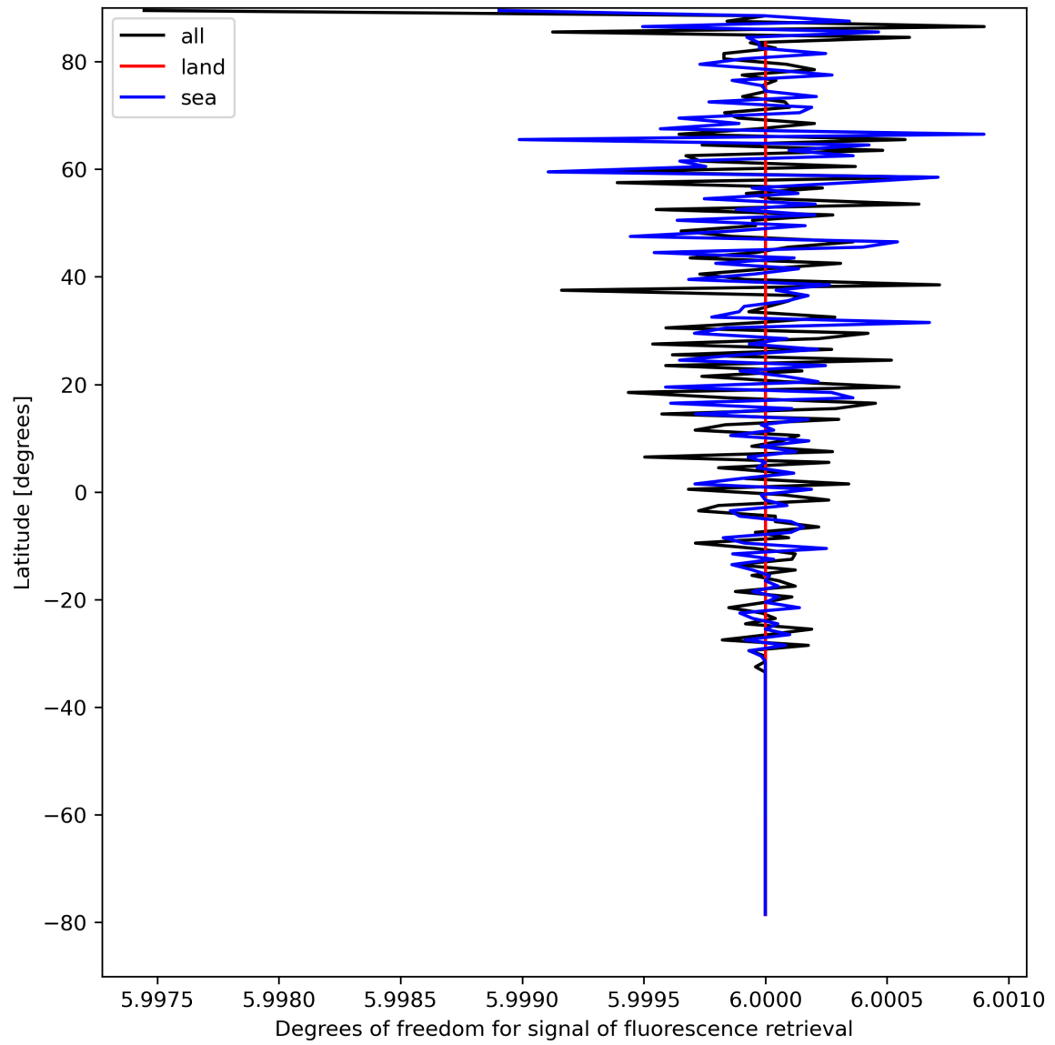
Figure 26: Zonal average of “Degrees of freedom for signal of fluorescence retrieval” for 2023-08-26 to 2023-08-28.
