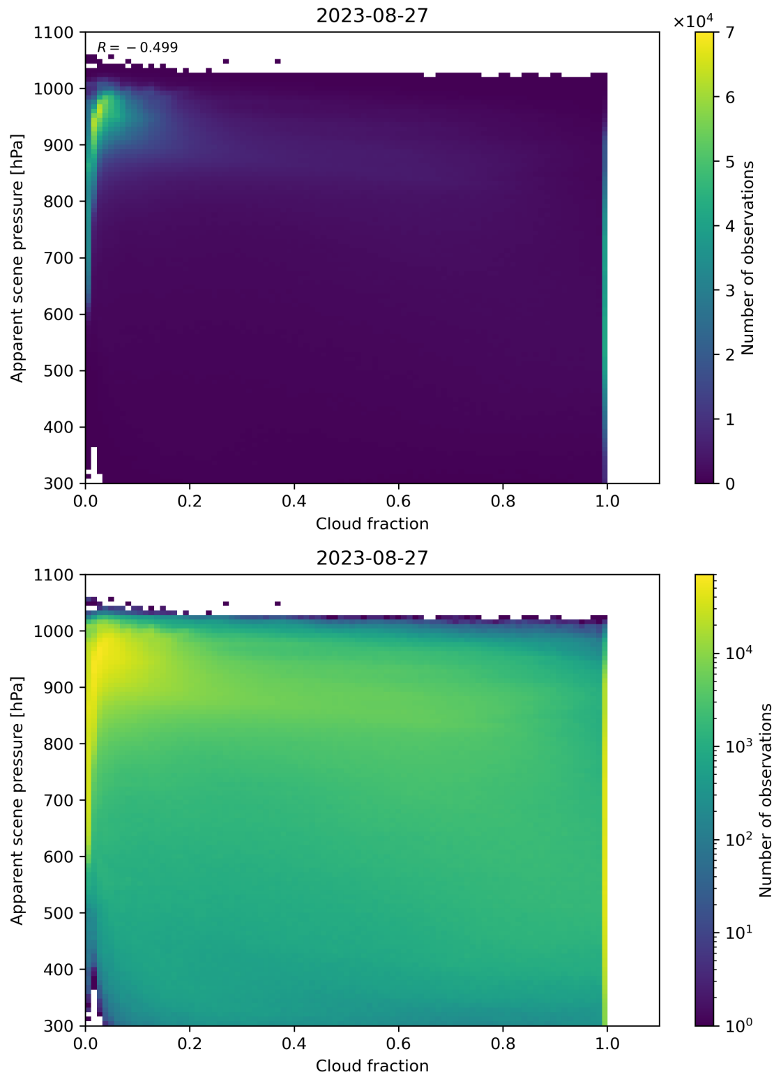
Figure 76: Scatter density plot of “Cloud fraction” against “Apparent scene pressure” for 2023-08-26 to 2023-08-28.
