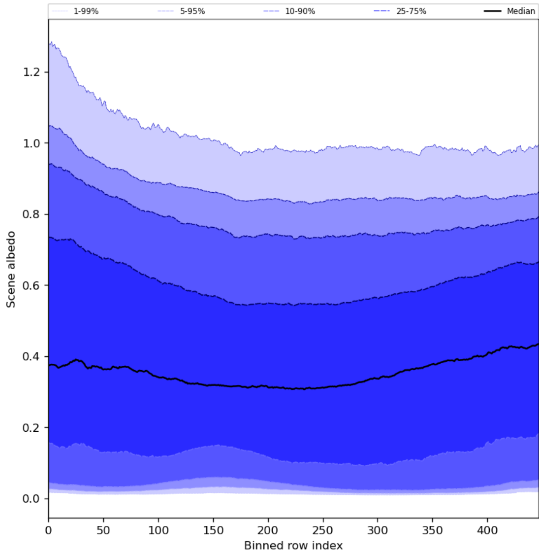
Figure 51: Along track statistics of “Scene albedo” for 2023-08-26 to 2023-08-28
