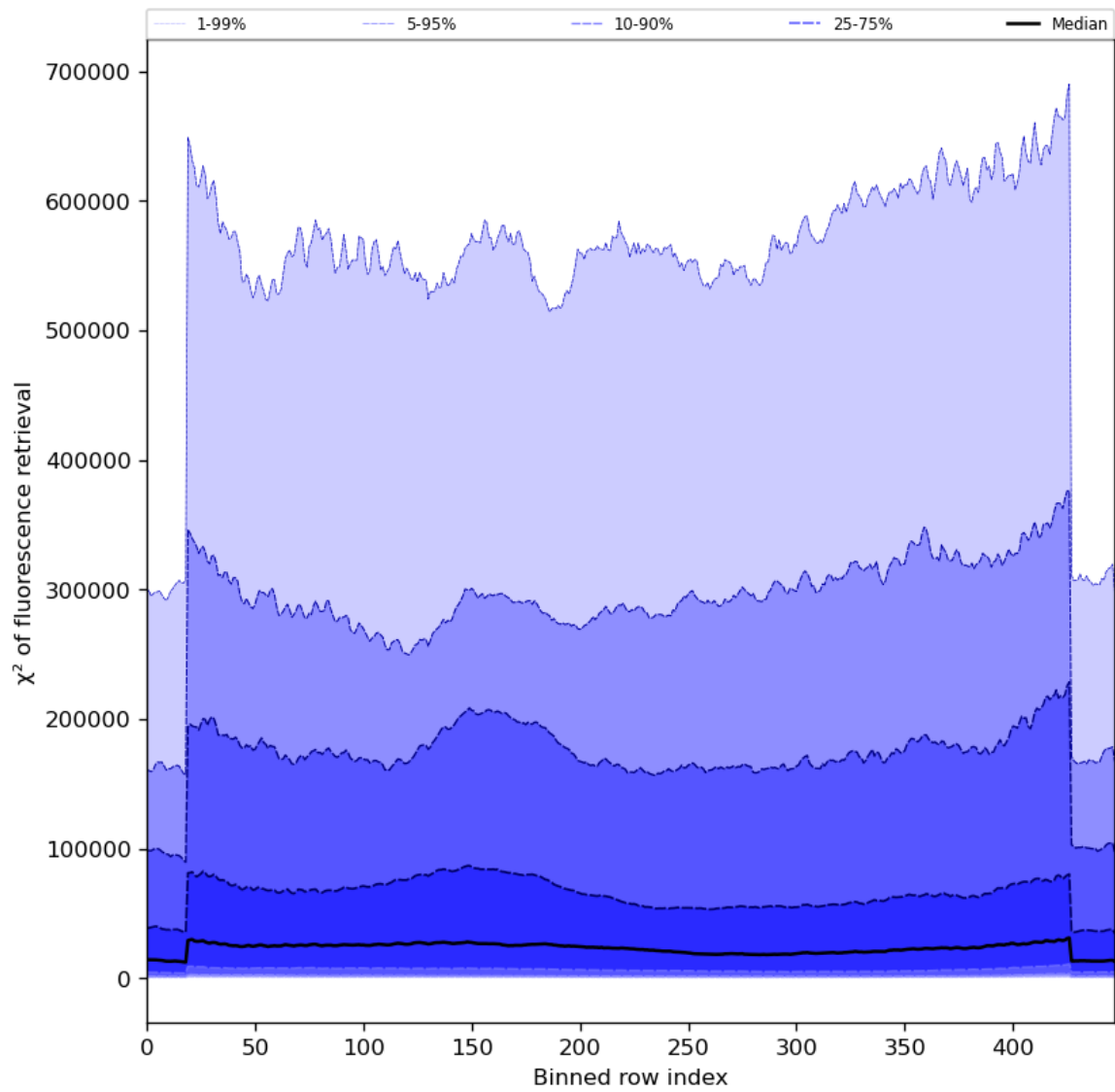
Figure 59: Along track statistics of “ \chi^2 of fluorescence retrieval” for 2023-08-26 to 2023-08-28
