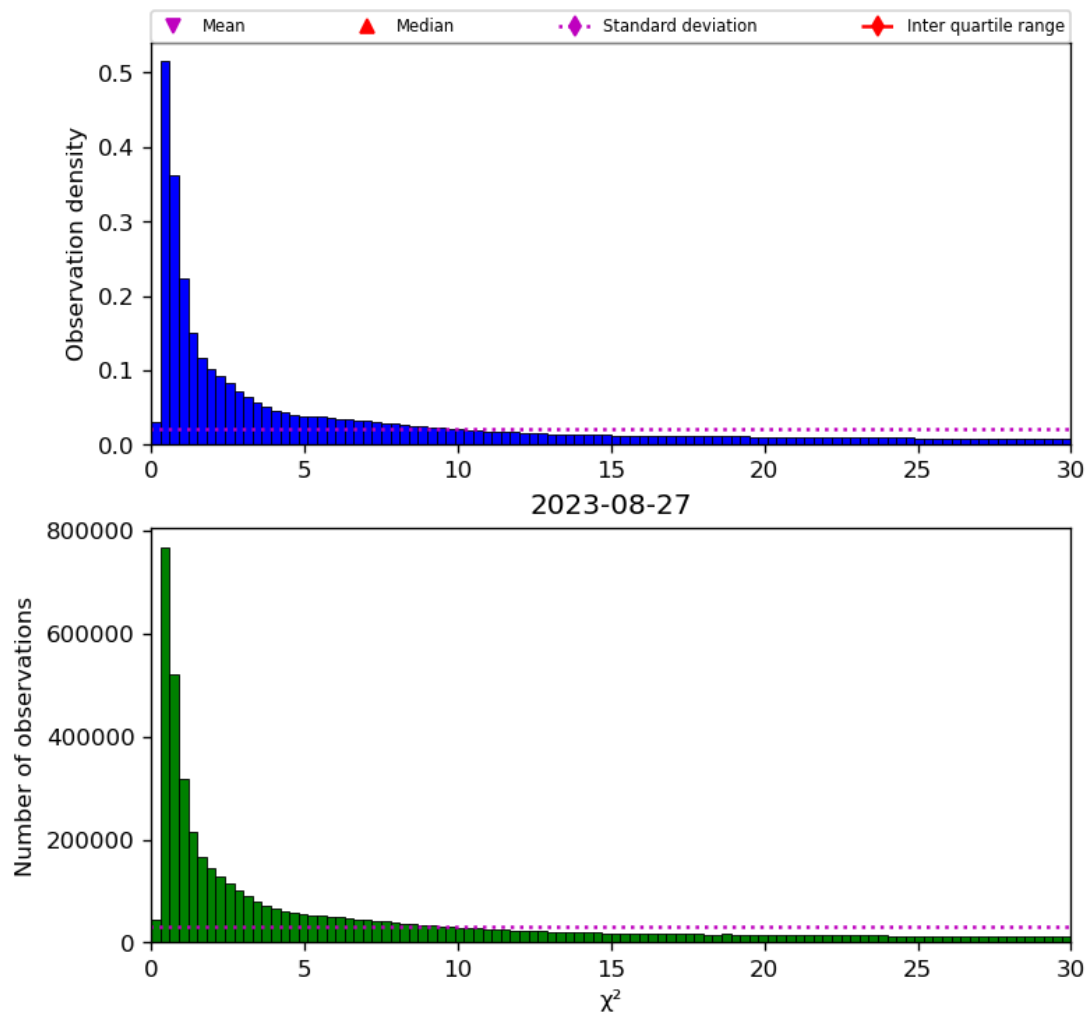
Figure 38: Histogram of “ \chi^2 ” for 2023-08-26 to 2023-08-28
