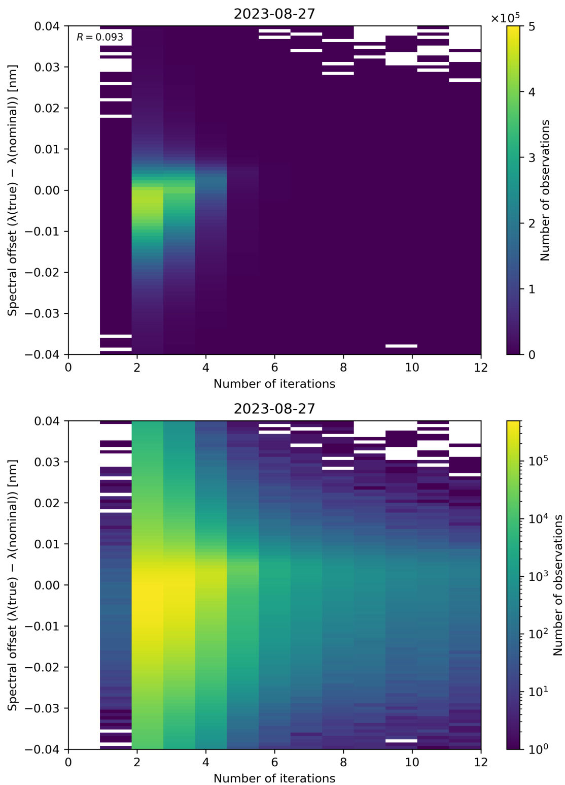
Figure 109: Scatter density plot of “Number of iterations” against “Spectral offset ( \lambda(\text{true}) - \lambda(\text{nominal}) )” for 2023-08-26 to 2023-08-28.
