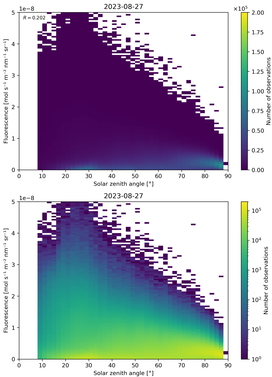
Figure 123: Scatter density plot of “Solar zenith angle” against “Fluorescence” for 2023-08-26 to 2023-08-28.
