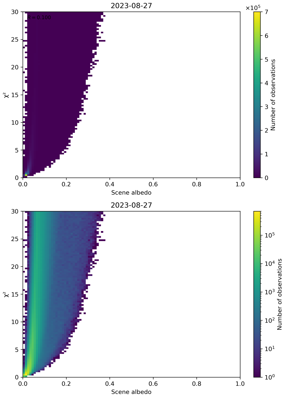
Figure 112: Scatter density plot of “Scene albedo” against “ \chi^2 ” for 2023-08-26 to 2023-08-28.
