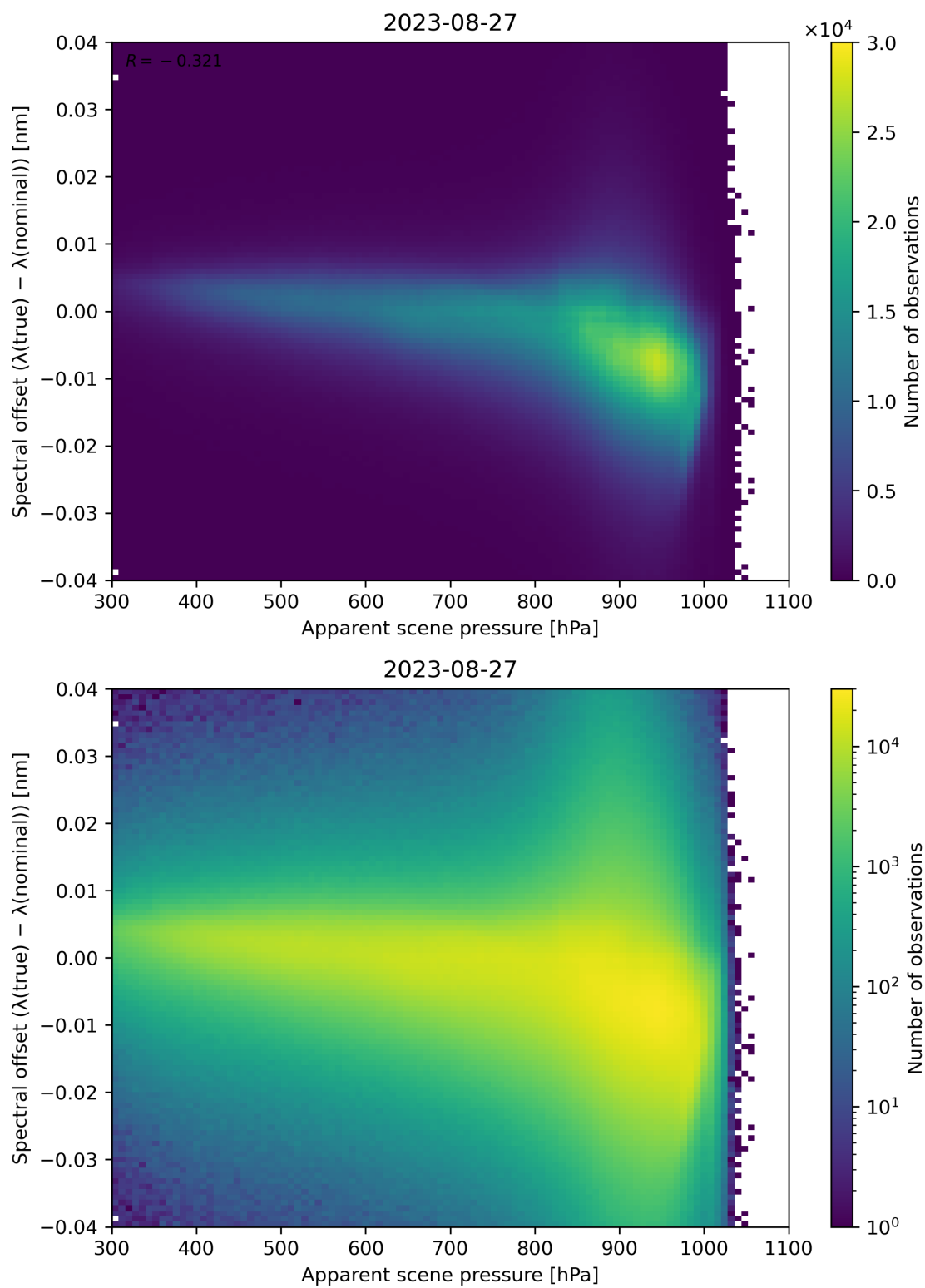
Figure 68: Scatter density plot of “Apparent scene pressure” against “Spectral offset ( \lambda(\text{true}) - \lambda(\text{nominal}) )” for 2023-08-26 to 2023-08-28.
