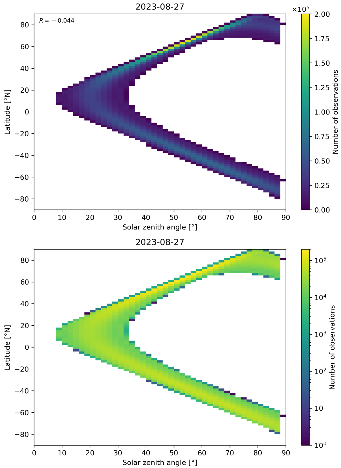
Figure 124: Scatter density plot of “Solar zenith angle” against “Latitude” for 2023-08-26 to 2023-08-28.
