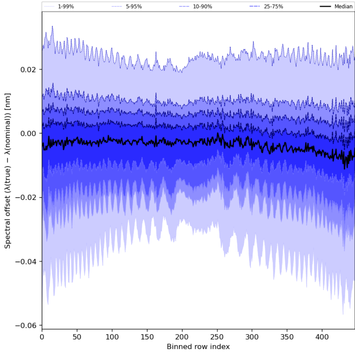
Figure 62: Along track statistics of “Spectral offset ( \lambda(\text{true}) - \lambda(\text{nominal}) )” for 2023-08-26 to 2023-08-28
