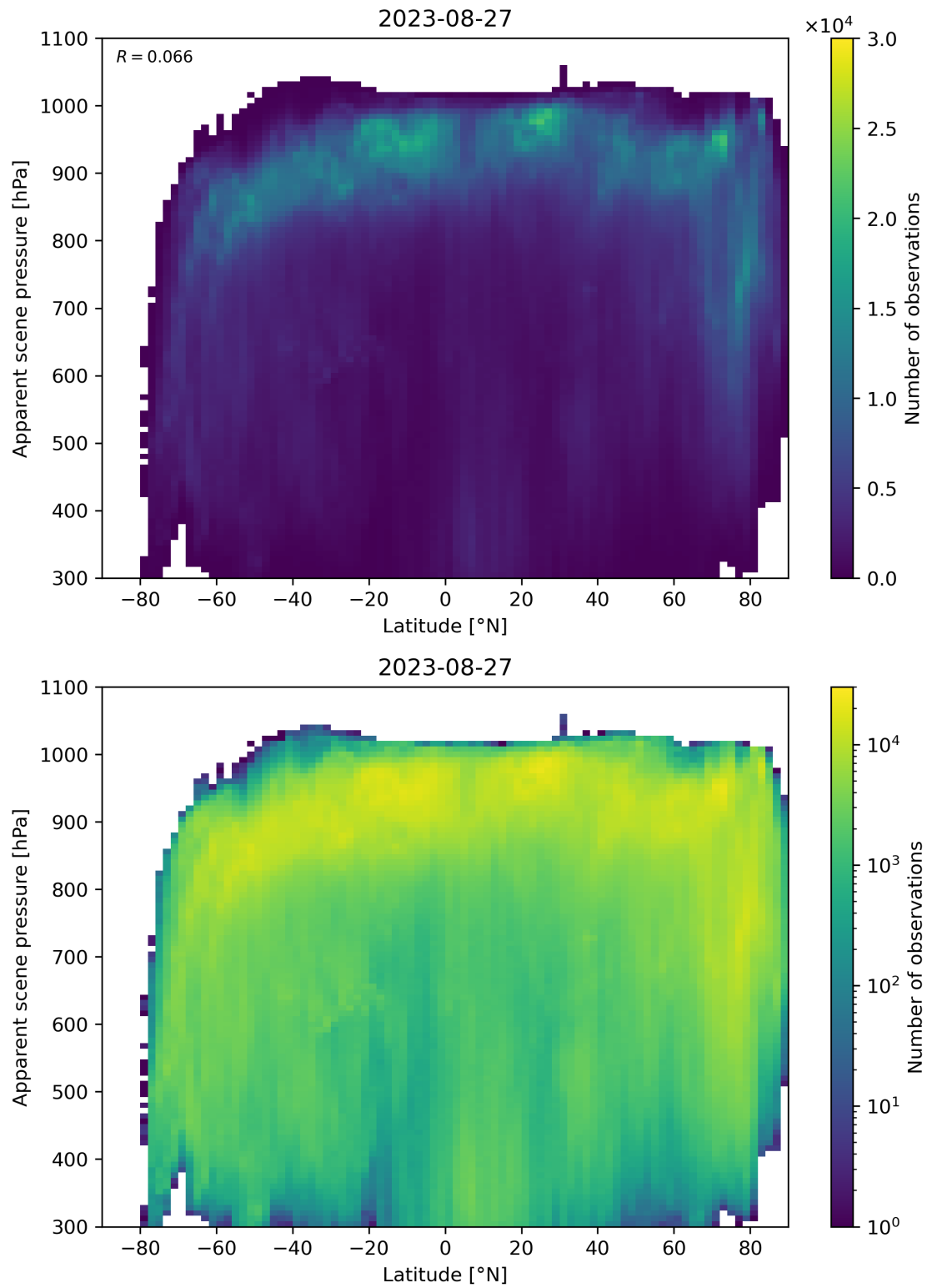
Figure 96: Scatter density plot of “Latitude” against “Apparent scene pressure” for 2023-08-26 to 2023-08-28.
