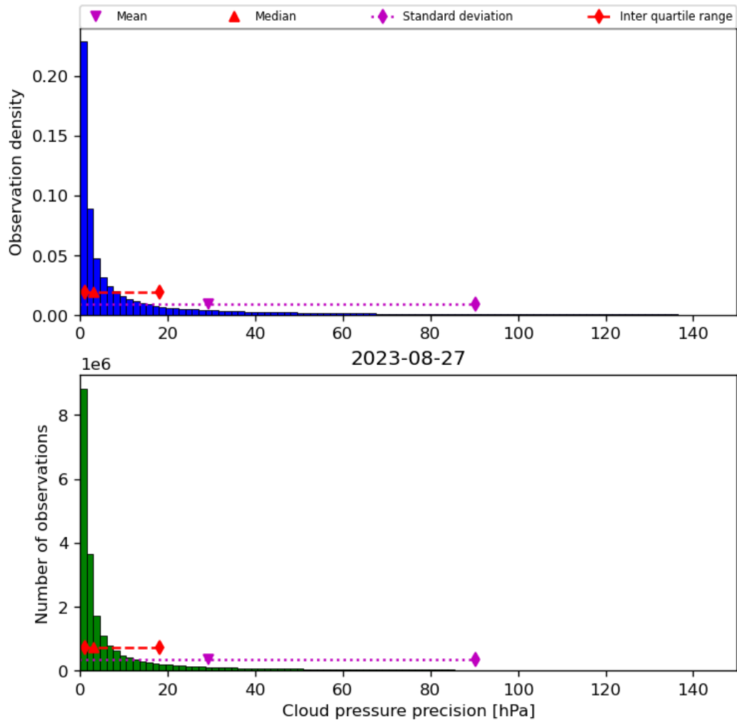
Figure 31: Histogram of “Cloud pressure precision” for 2023-08-26 to 2023-08-28
