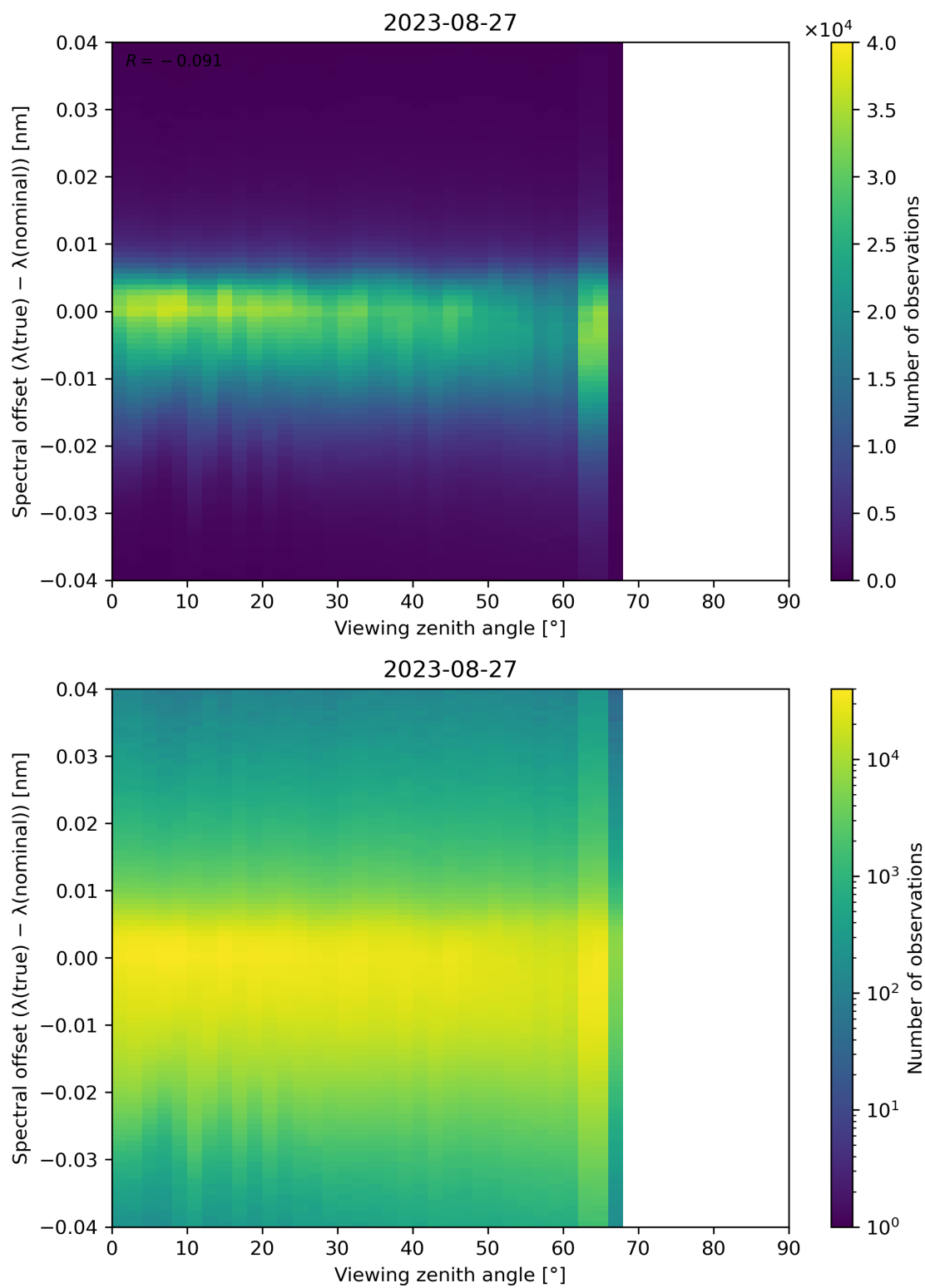
Figure 140: Scatter density plot of “Viewing zenith angle” against “Spectral offset ( \lambda(\text{true}) - \lambda(\text{nominal}) )” for 2023-08-26 to 2023-08-28.
