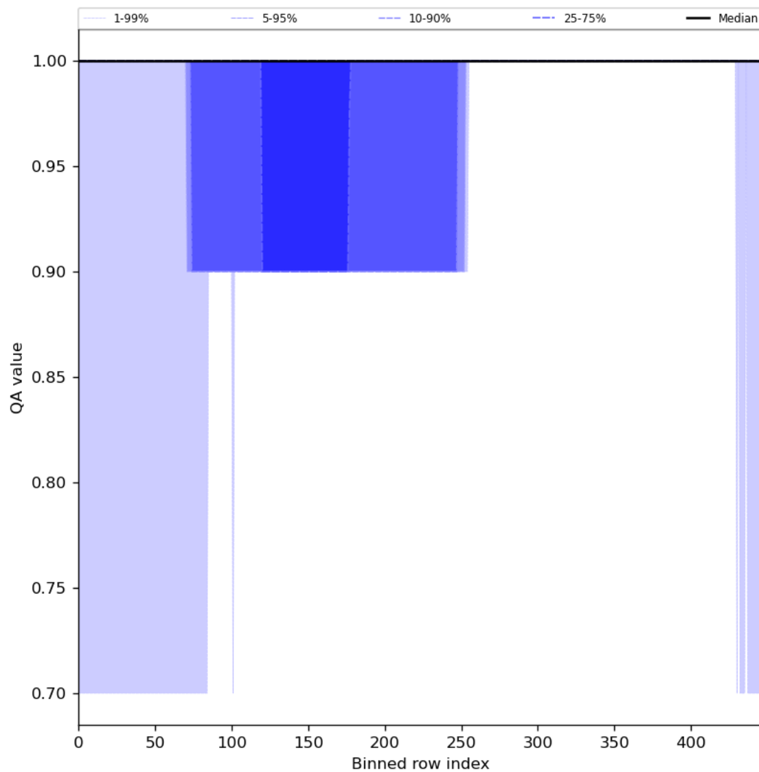
Figure 46: Along track statistics of “QA value” for 2023-08-26 to 2023-08-28
