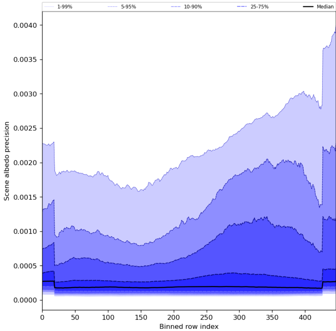
Figure 52: Along track statistics of “Scene albedo precision” for 2023-08-26 to 2023-08-28
