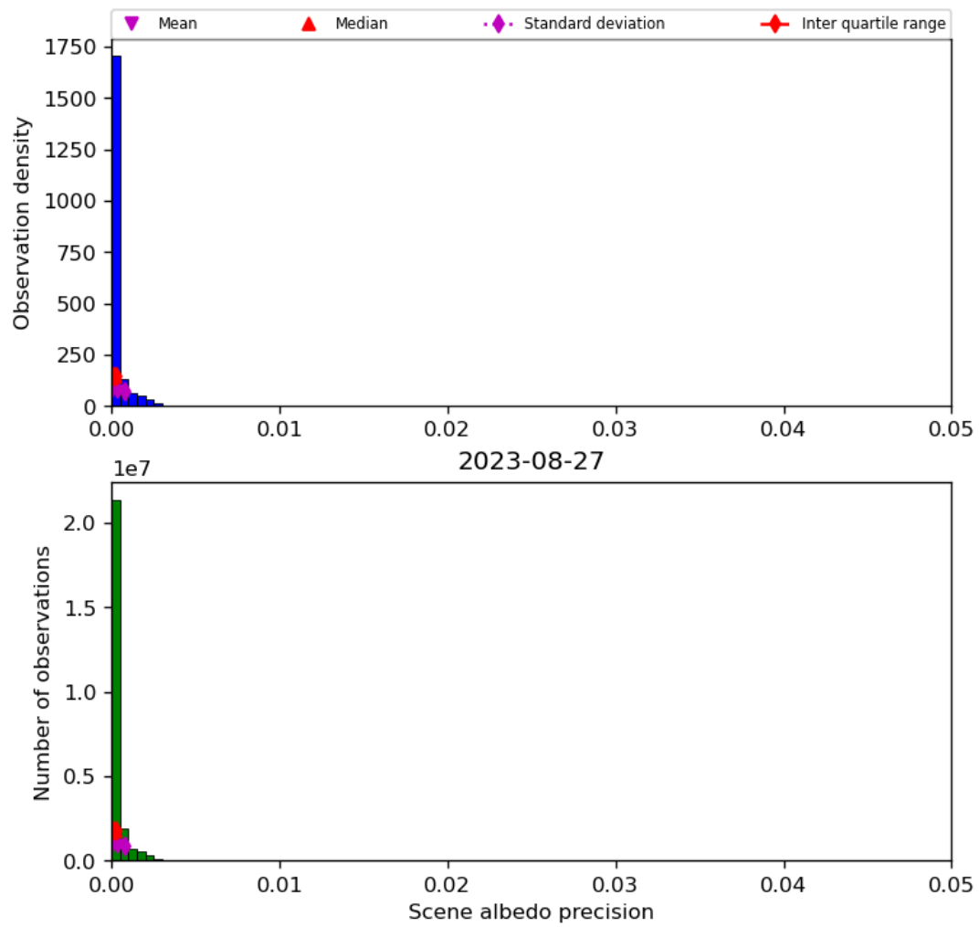
Figure 35: Histogram of “Scene albedo precision” for 2023-08-26 to 2023-08-28
