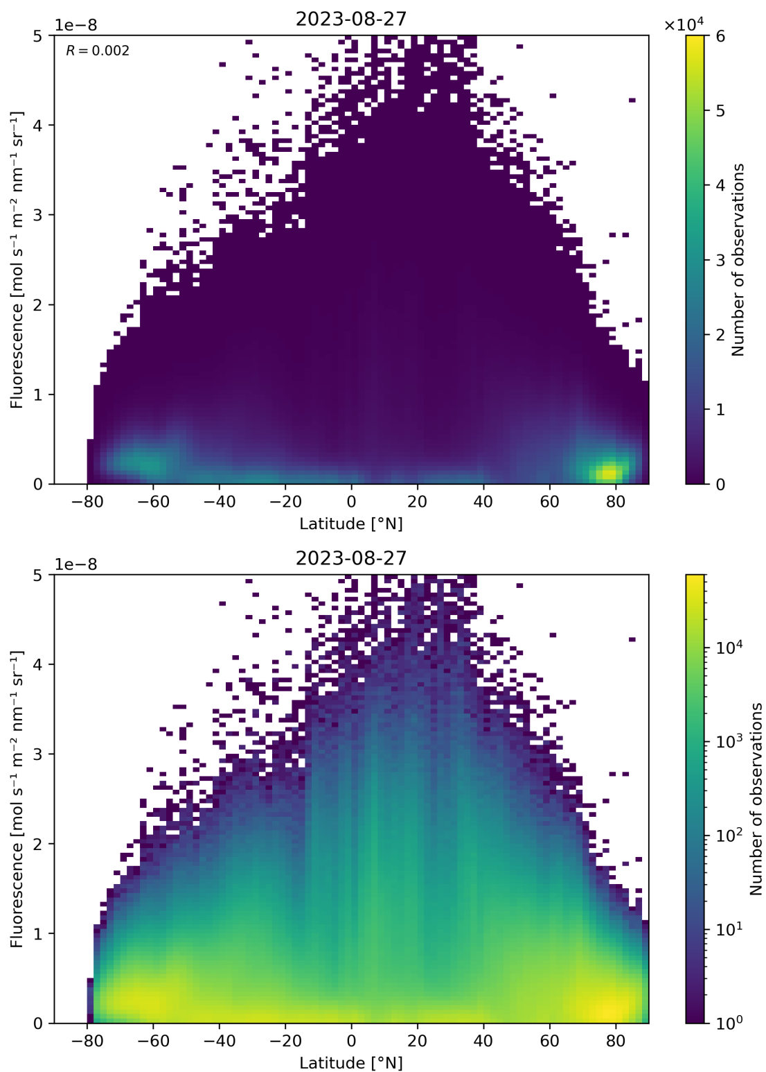
Figure 101: Scatter density plot of “Latitude” against “Fluorescence” for 2023-08-26 to 2023-08-28.
