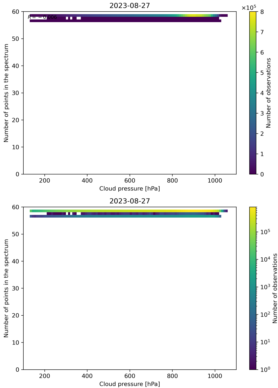
Figure 90: Scatter density plot of “Cloud pressure” against “Number of points in the spectrum” for 2023-08-26 to 2023-08-28.
