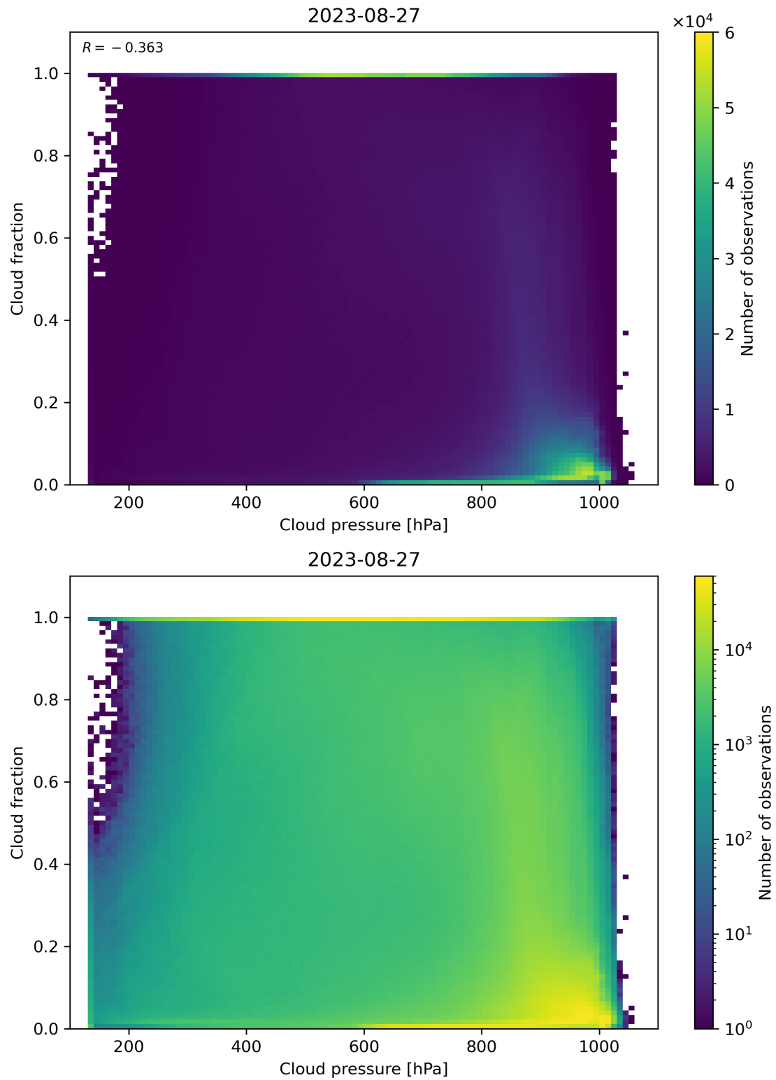
Figure 87: Scatter density plot of “Cloud pressure” against “Cloud fraction” for 2023-08-26 to 2023-08-28.
