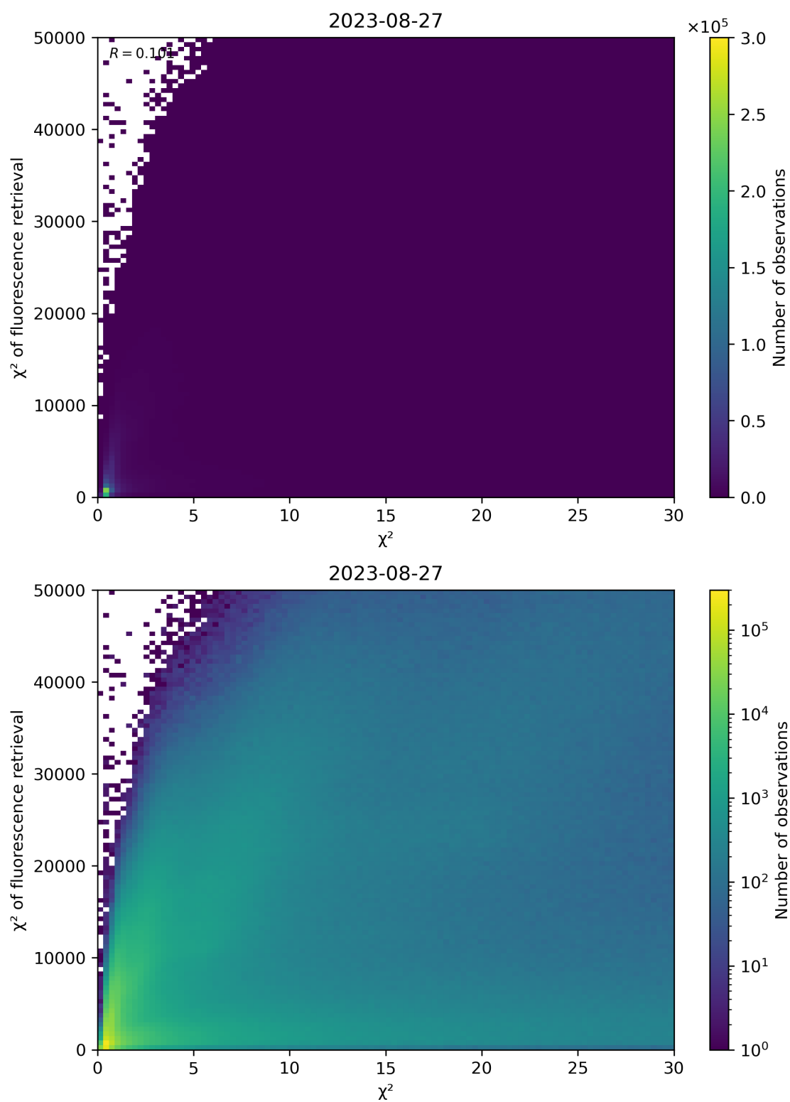
Figure 69: Scatter density plot of “ \chi^2 ” against “ \chi^2 of fluorescence retrieval” for 2023-08-26 to 2023-08-28.
