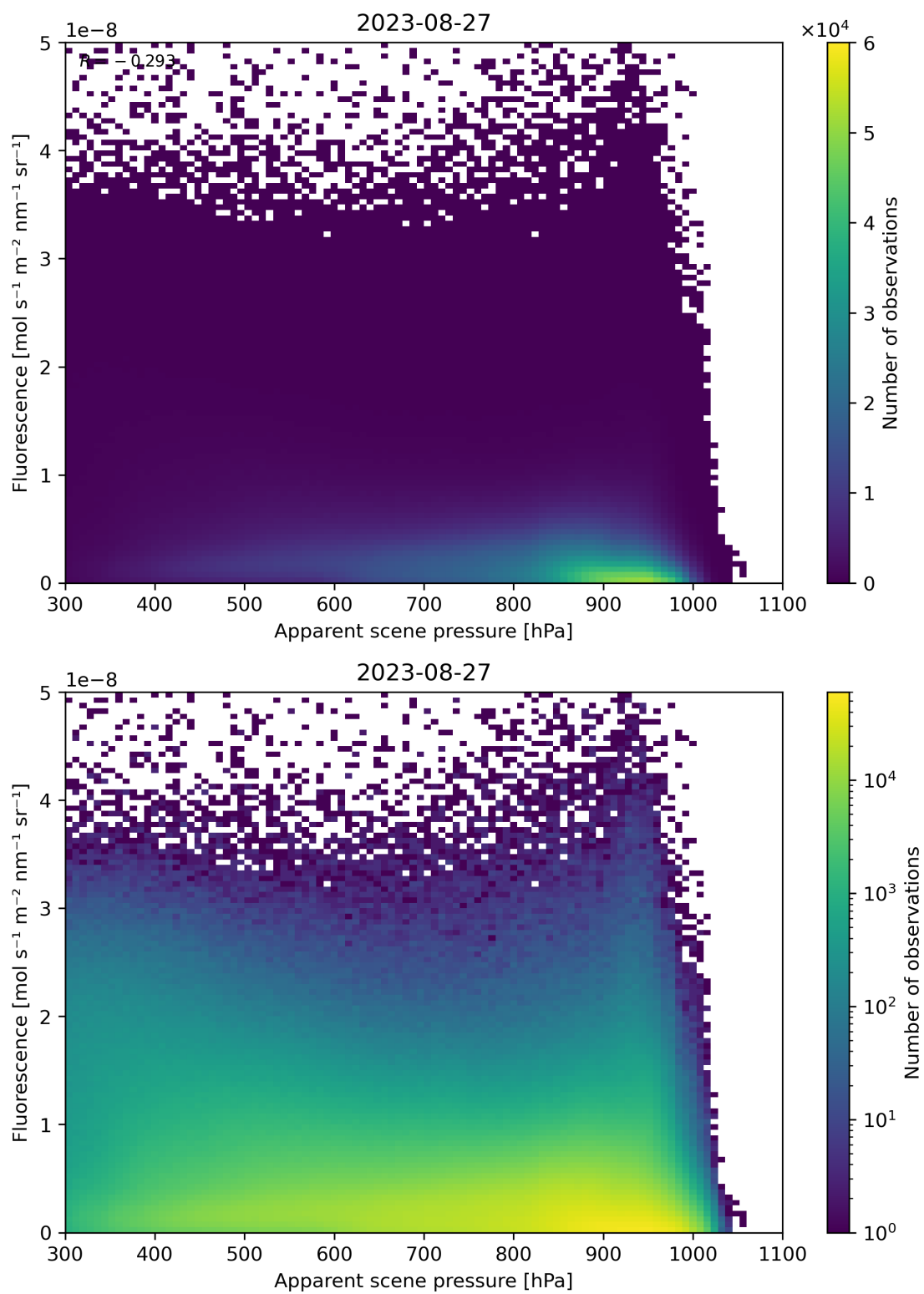
Figure 65: Scatter density plot of “Apparent scene pressure” against “Fluorescence” for 2023-08-26 to 2023-08-28.
