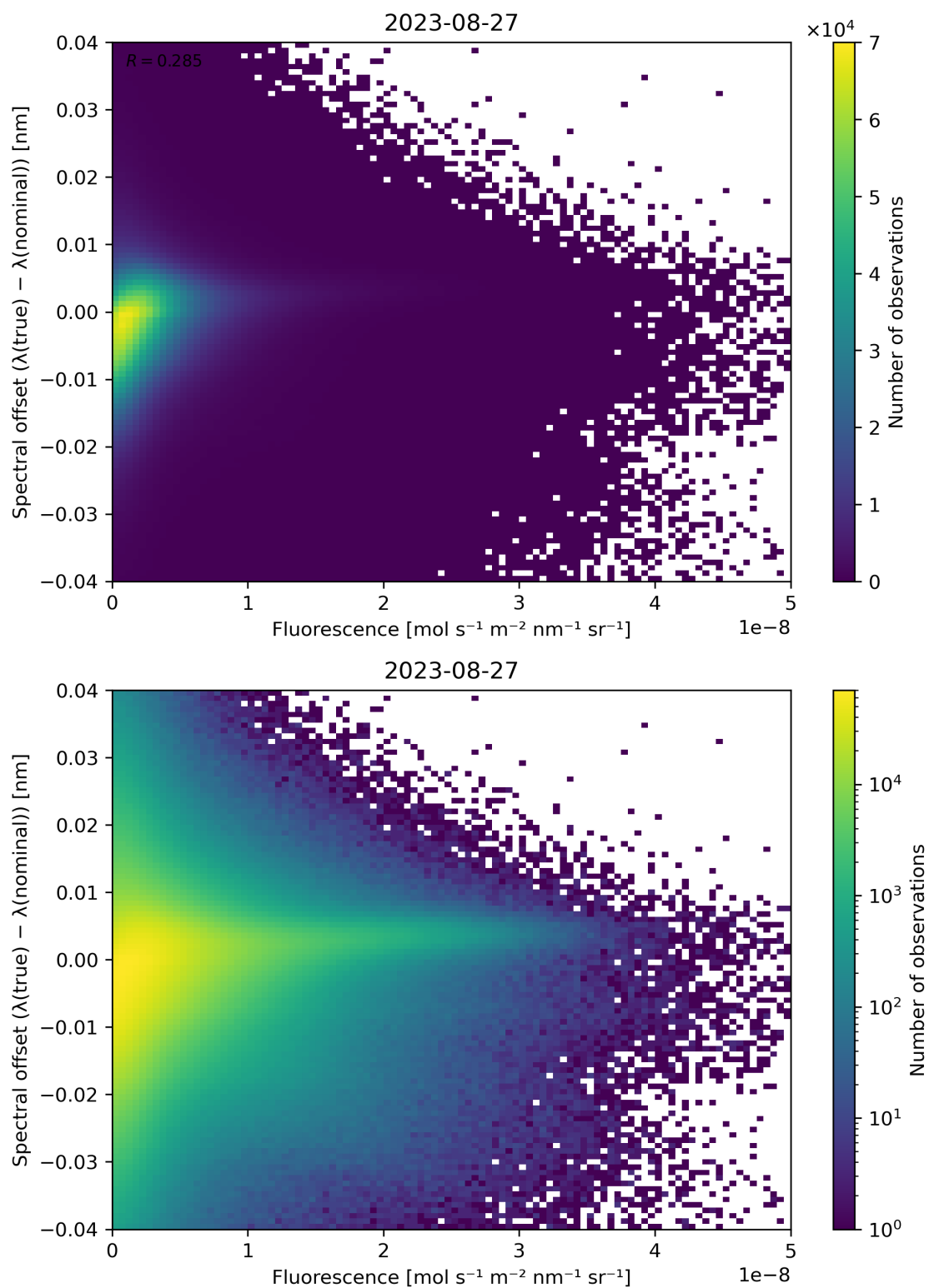
Figure 95: Scatter density plot of “Fluorescence” against “Spectral offset ( \lambda(\text{true}) - \lambda(\text{nominal}) )” for 2023-08-26 to 2023-08-28.
