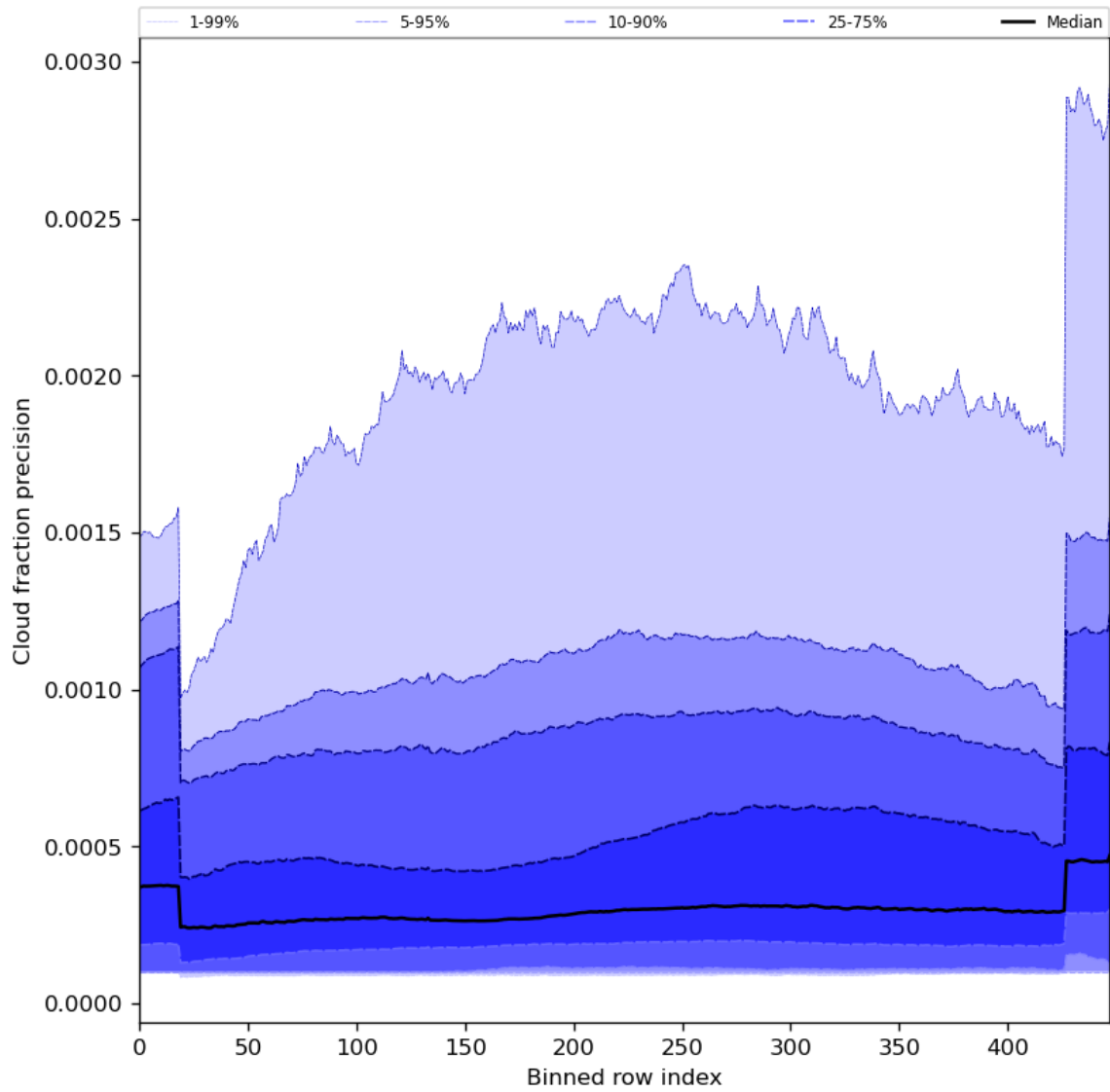
Figure 50: Along track statistics of “Cloud fraction precision” for 2023-08-26 to 2023-08-28
