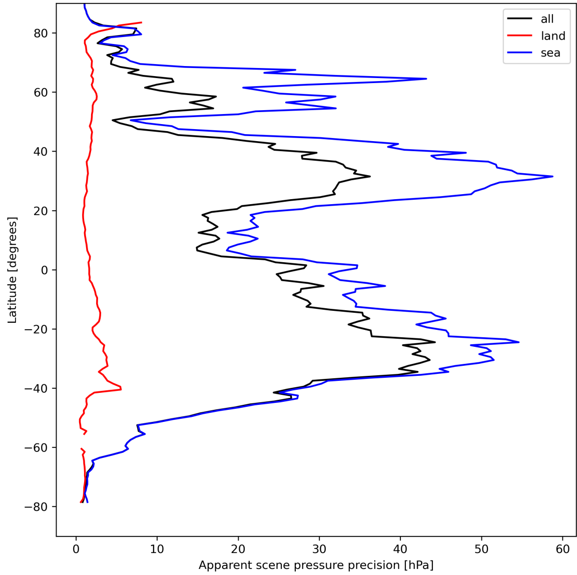
Figure 20: Zonal average of “Apparent scene pressure precision” for 2023-08-26 to 2023-08-28.
