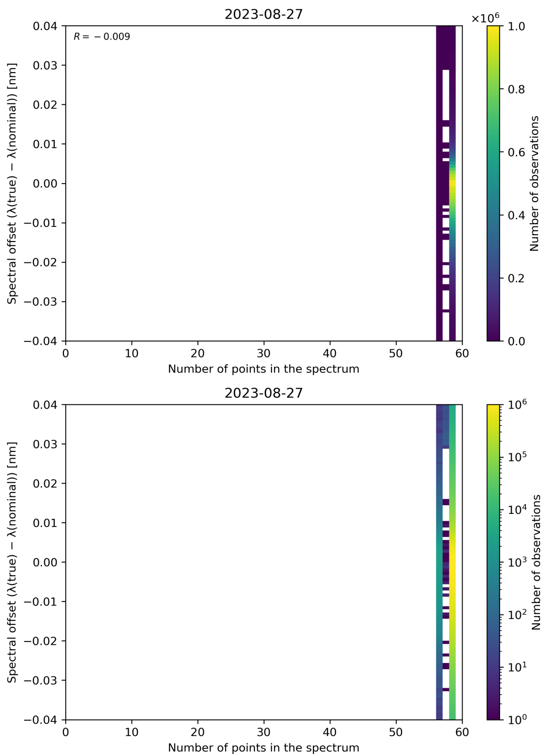
Figure 110: Scatter density plot of “Number of points in the spectrum” against “Spectral offset ( \lambda(\text{true}) - \lambda(\text{nominal}) )” for 2023-08-26 to 2023-08-28.
