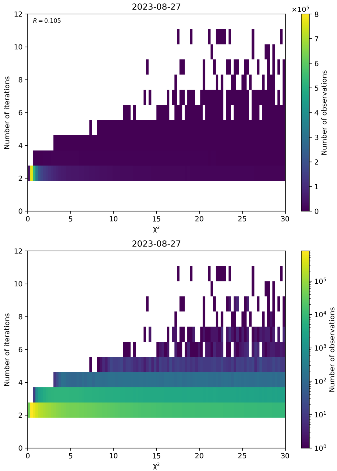
Figure 73: Scatter density plot of “ \chi^2 ” against “Number of iterations” for 2023-08-26 to 2023-08-28.
