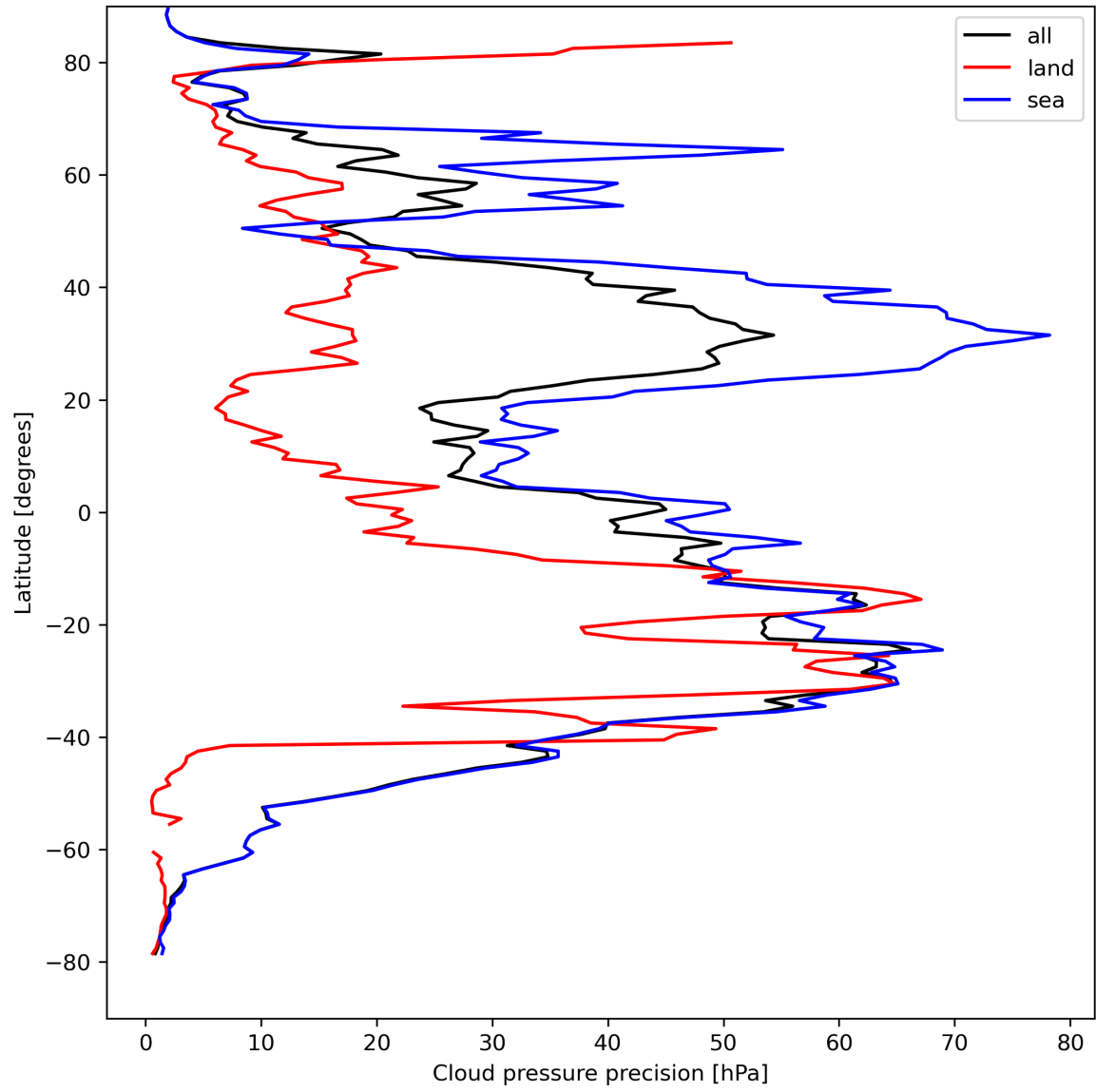
Figure 14: Zonal average of “Cloud pressure precision” for 2023-08-26 to 2023-08-28.
