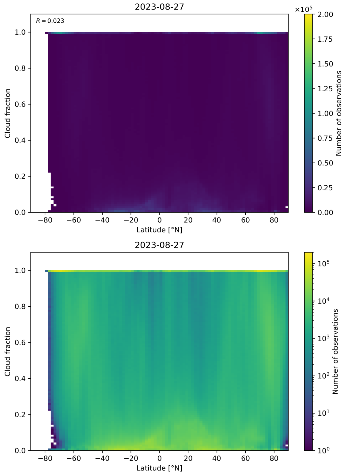
Figure 99: Scatter density plot of “Latitude” against “Cloud fraction” for 2023-08-26 to 2023-08-28.
