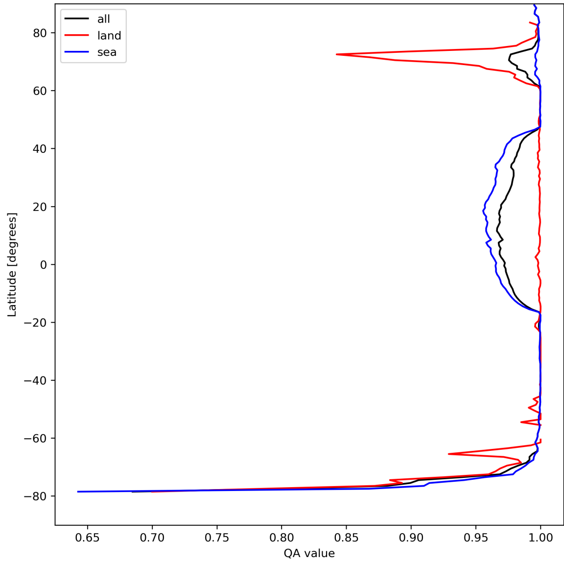
Figure 12: Zonal average of "QA value" for 2023-08-26 to 2023-08-28.
