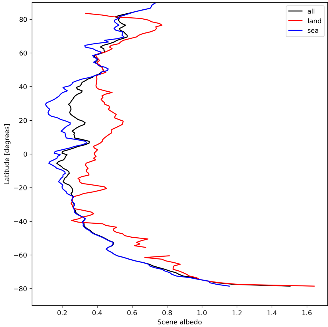
Figure 17: Zonal average of “Scene albedo” for 2023-08-26 to 2023-08-28.
