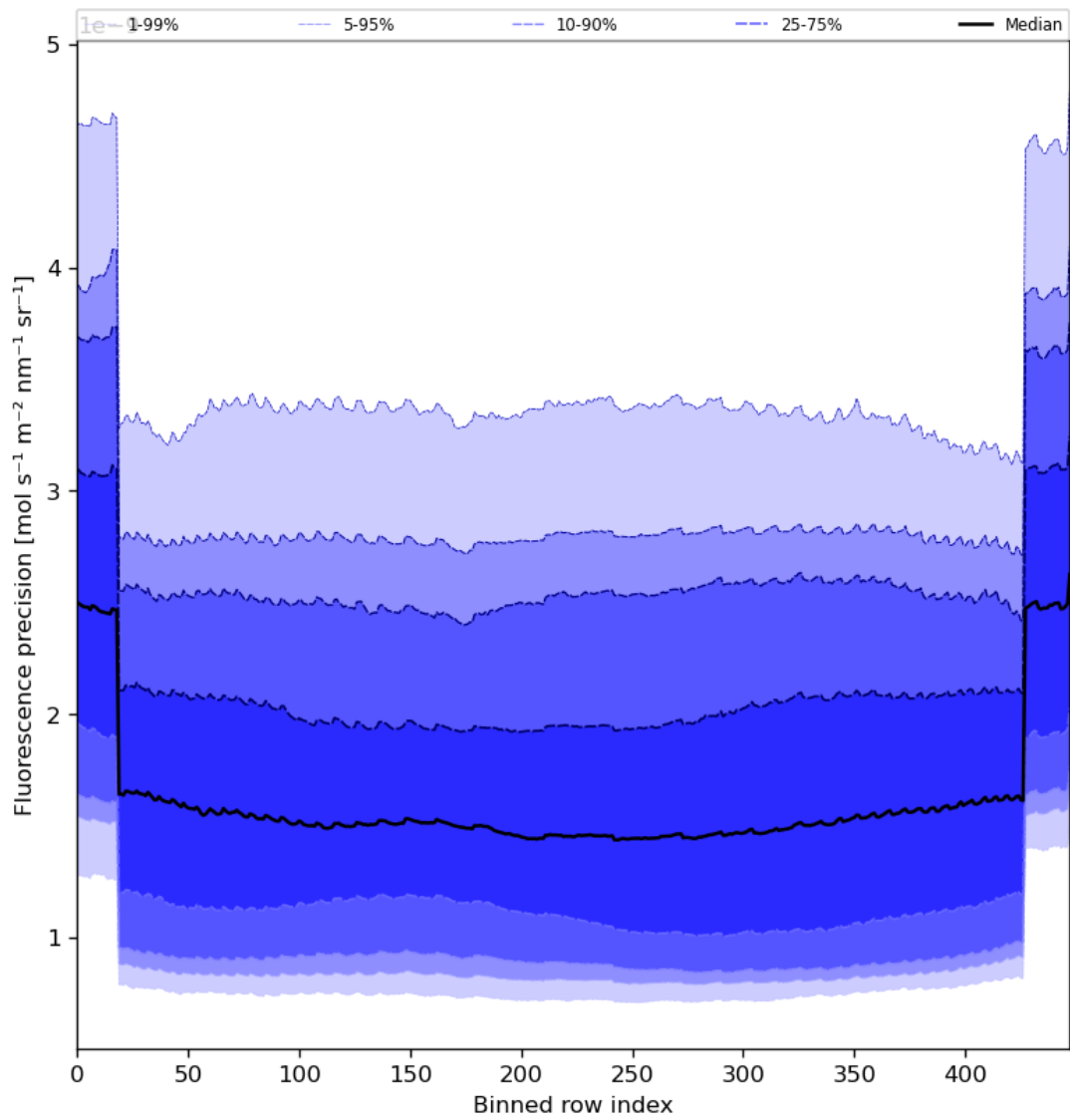
Figure 58: Along track statistics of “Fluorescence precision” for 2023-08-26 to 2023-08-28
