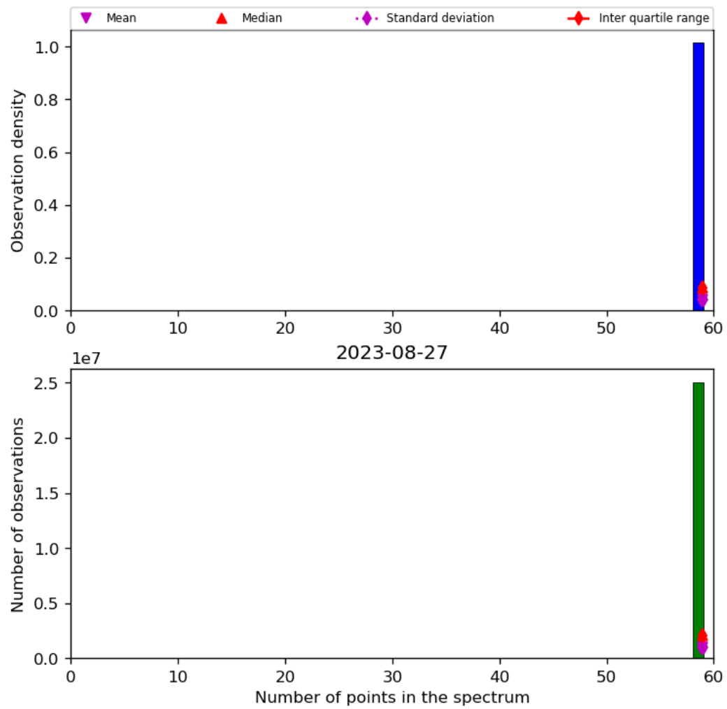
Figure 44: Histogram of “Number of points in the spectrum” for 2023-08-26 to 2023-08-28
