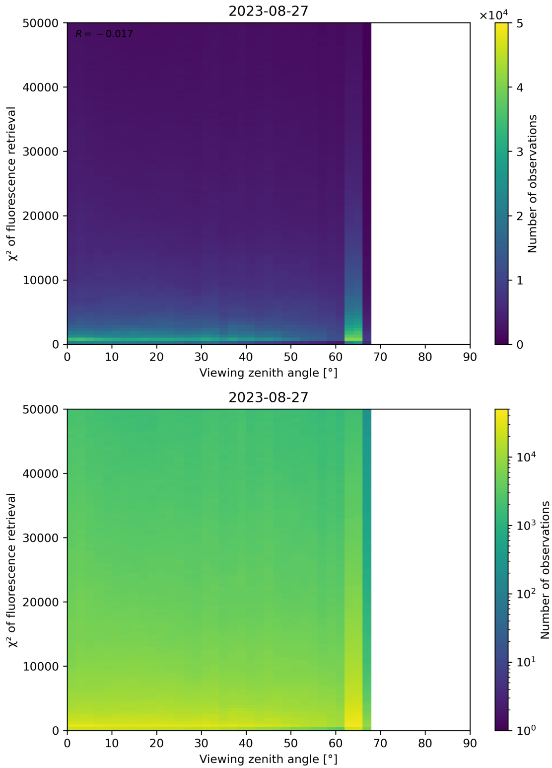
Figure 131: Scatter density plot of “Viewing zenith angle” against “ \chi^2 of fluorescence retrieval” for 2023-08-26 to 2023-08-28.
