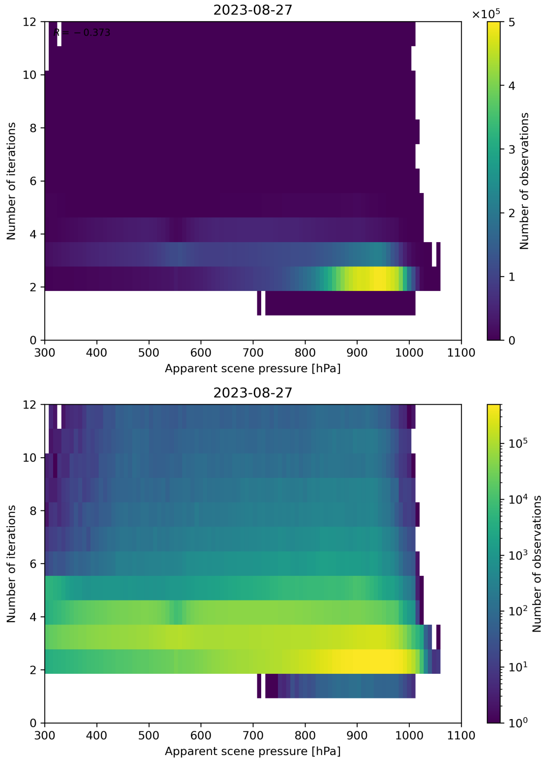
Figure 66: Scatter density plot of “Apparent scene pressure” against “Number of iterations” for 2023-08-26 to 2023-08-28.
