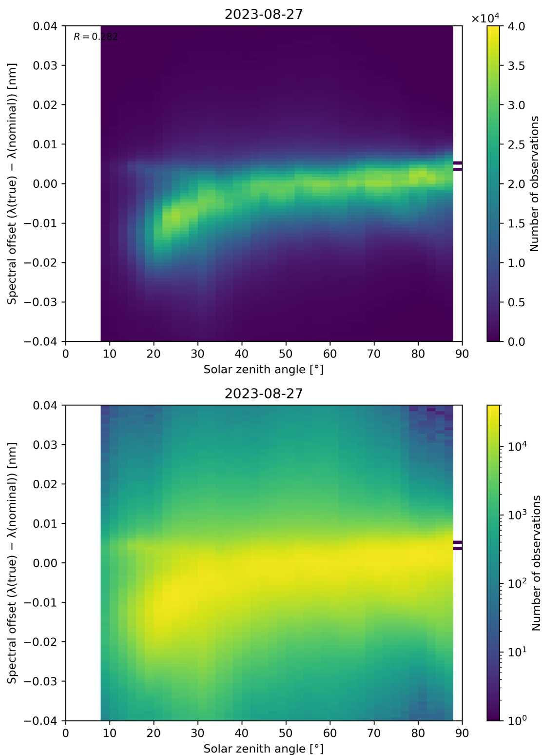
Figure 128: Scatter density plot of “Solar zenith angle” against “Spectral offset ( \lambda(\text{true}) - \lambda(\text{nominal}) )” for 2023-08-26 to 2023-08-28.
