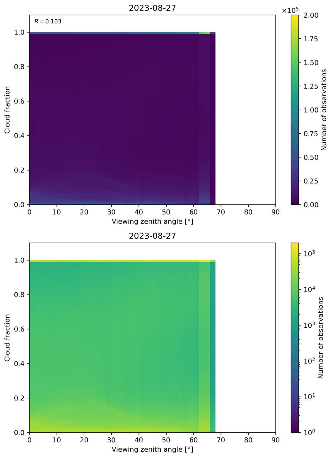
Figure 132: Scatter density plot of “Viewing zenith angle” against “Cloud fraction” for 2023-08-26 to 2023-08-28.
