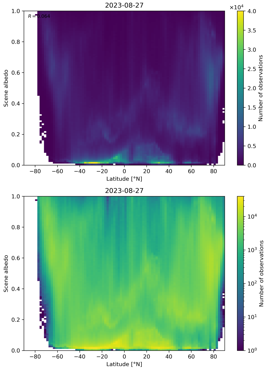
Figure 104: Scatter density plot of “Latitude” against “Scene albedo” for 2023-08-26 to 2023-08-28.
