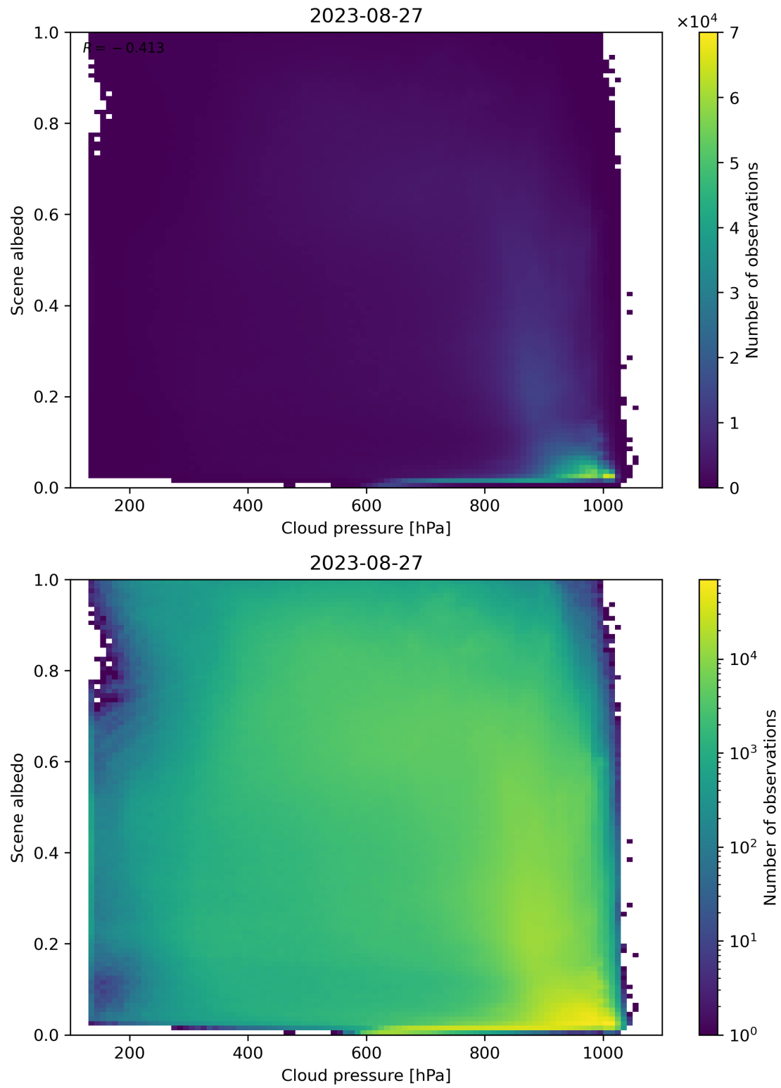
Figure 91: Scatter density plot of “Cloud pressure” against “Scene albedo” for 2023-08-26 to 2023-08-28.
