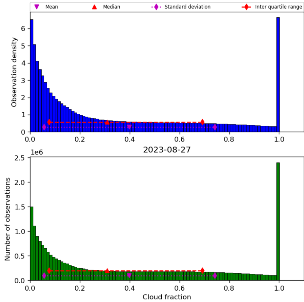
Figure 32: Histogram of “Cloud fraction” for 2023-08-26 to 2023-08-28
