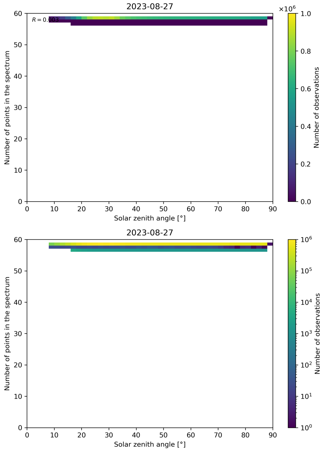
Figure 126: Scatter density plot of “Solar zenith angle” against “Number of points in the spectrum” for 2023-08-26 to 2023-08-28.
