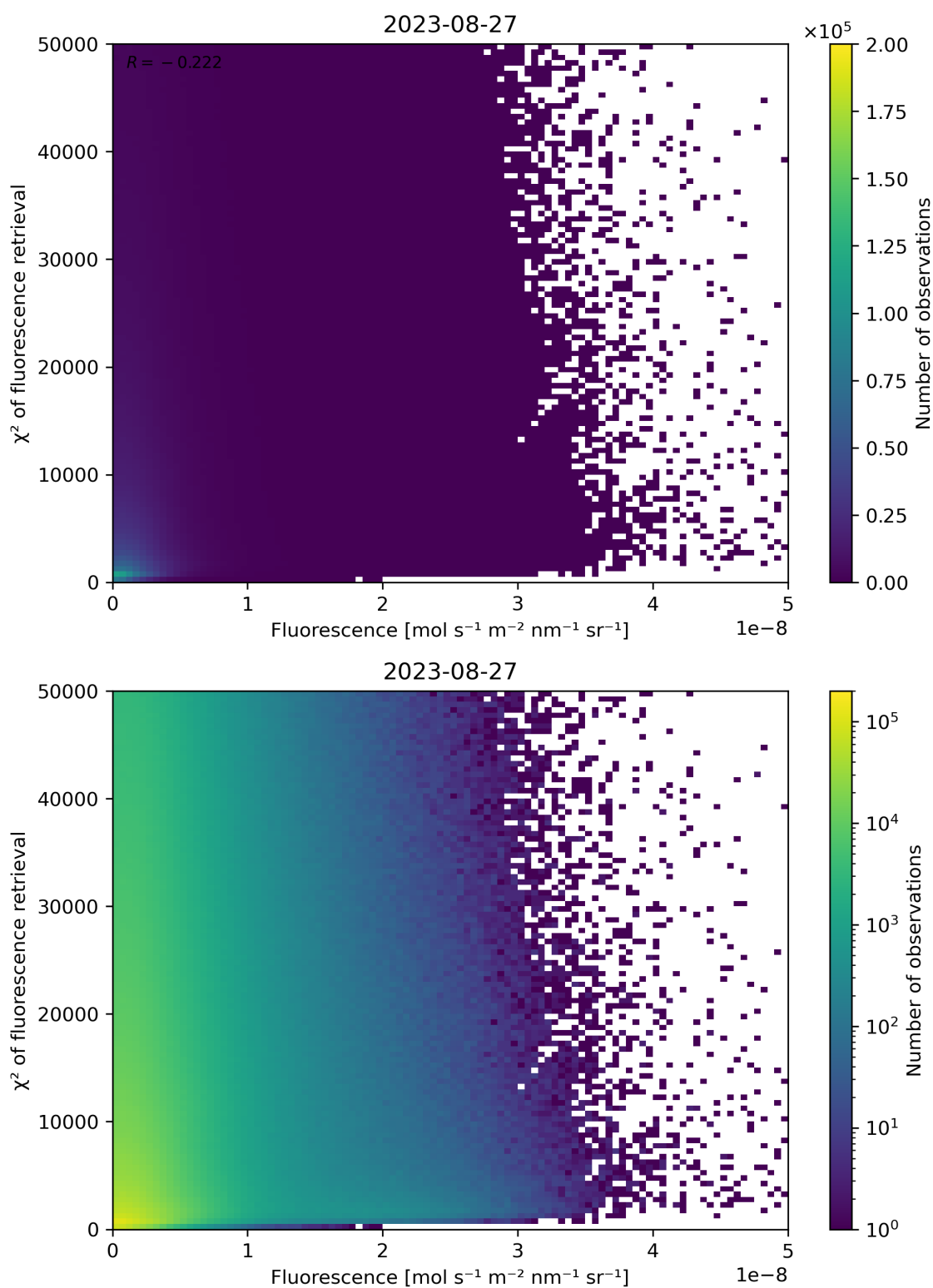
Figure 93: Scatter density plot of “Fluorescence” against “ \chi^2 of fluorescence retrieval” for 2023-08-26 to 2023-08-28.
