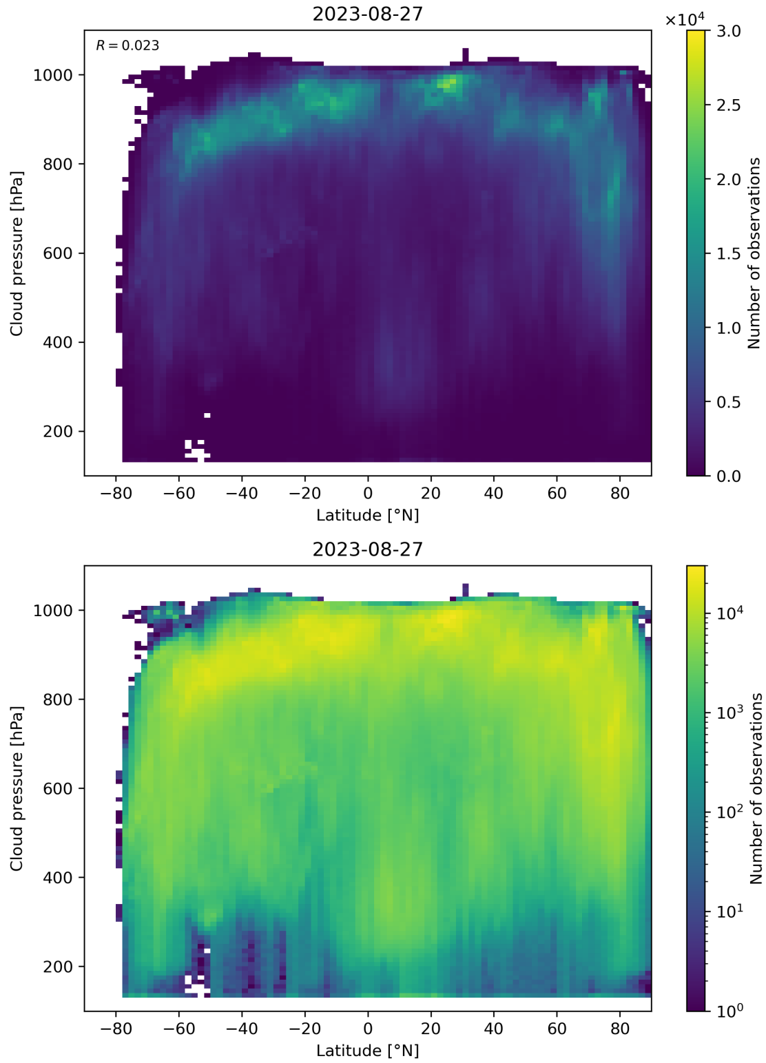
Figure 100: Scatter density plot of “Latitude” against “Cloud pressure” for 2023-08-26 to 2023-08-28.
