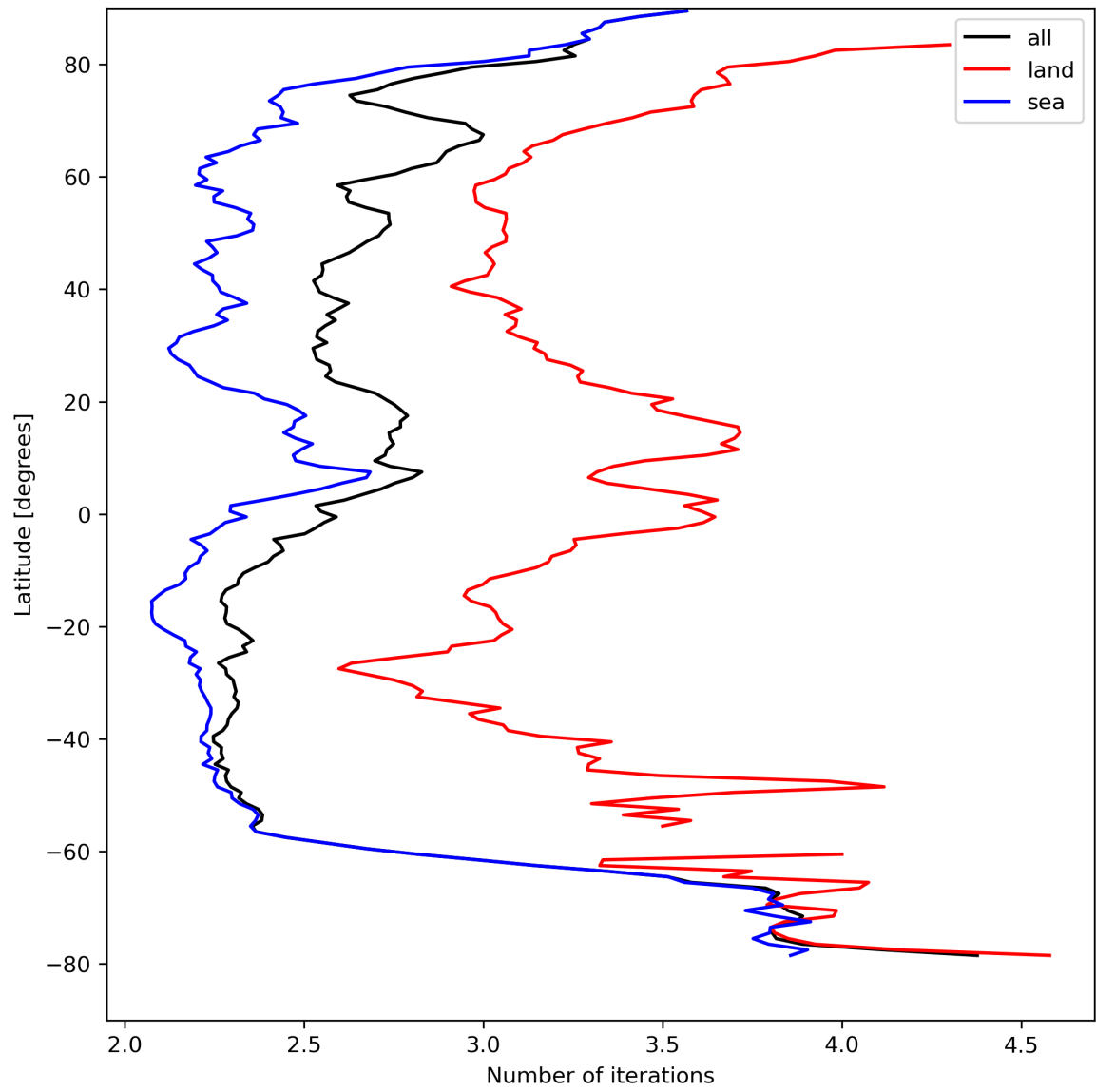
Figure 22: Zonal average of “Number of iterations” for 2023-08-26 to 2023-08-28.
