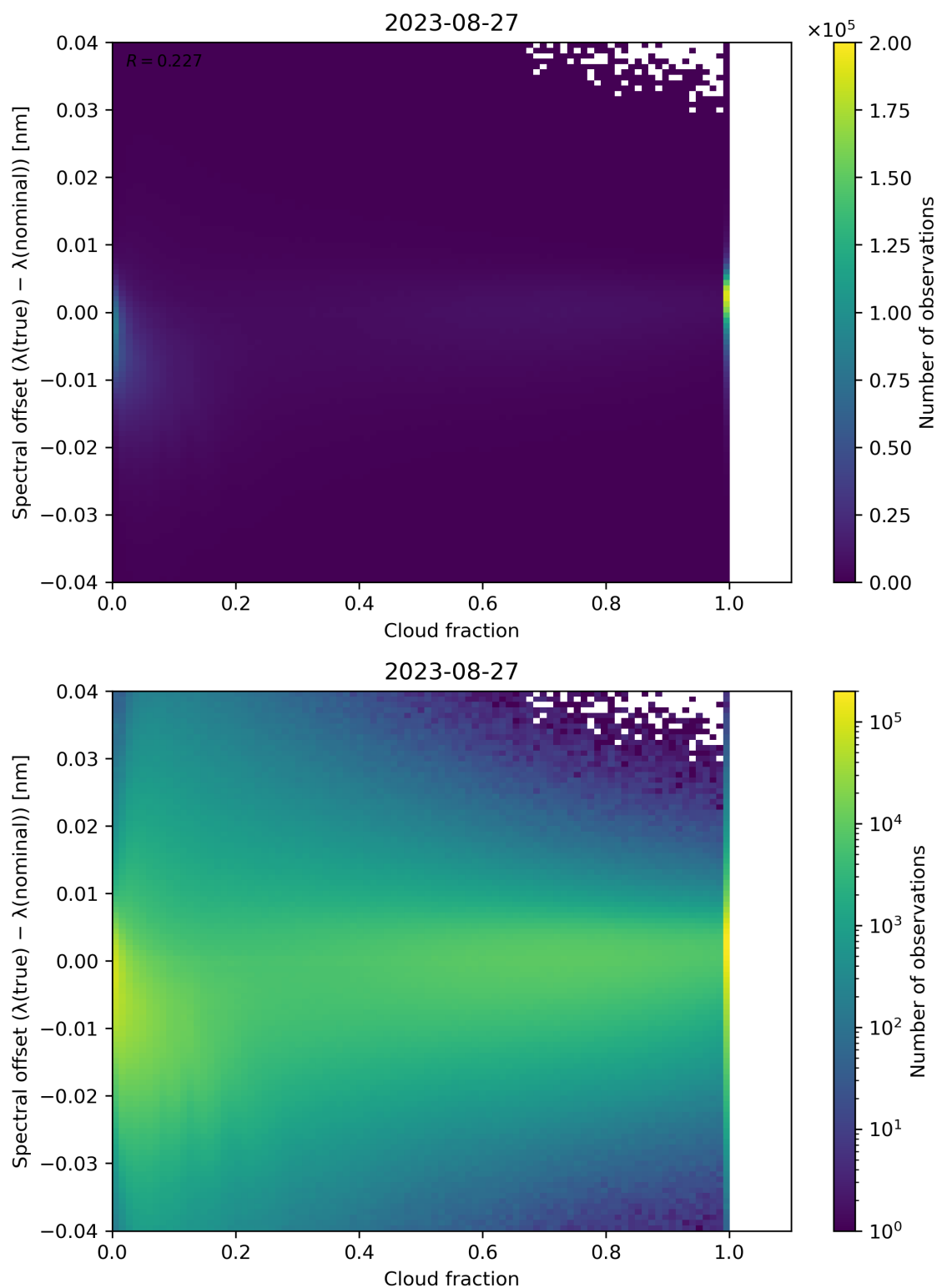
Figure 83: Scatter density plot of “Cloud fraction” against “Spectral offset ( \lambda(\text{true}) - \lambda(\text{nominal}) )” for 2023-08-26 to 2023-08-28.
