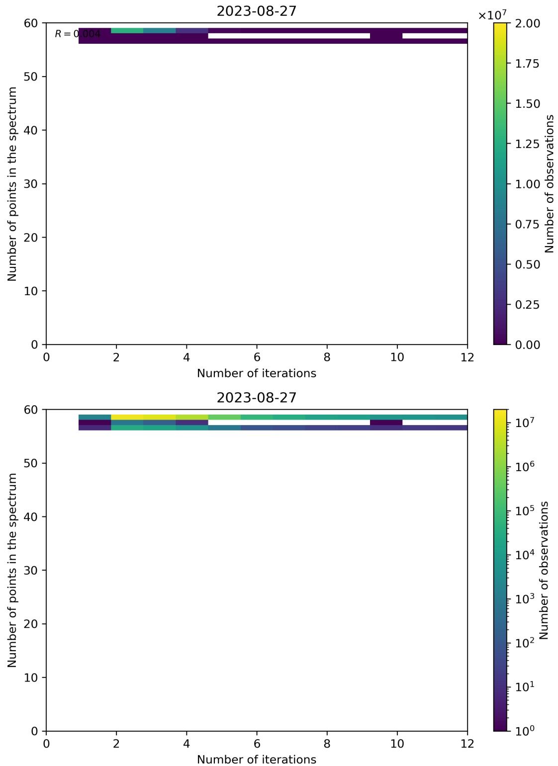
Figure 108: Scatter density plot of “Number of iterations” against “Number of points in the spectrum” for 2023-08-26 to 2023-08-28.
