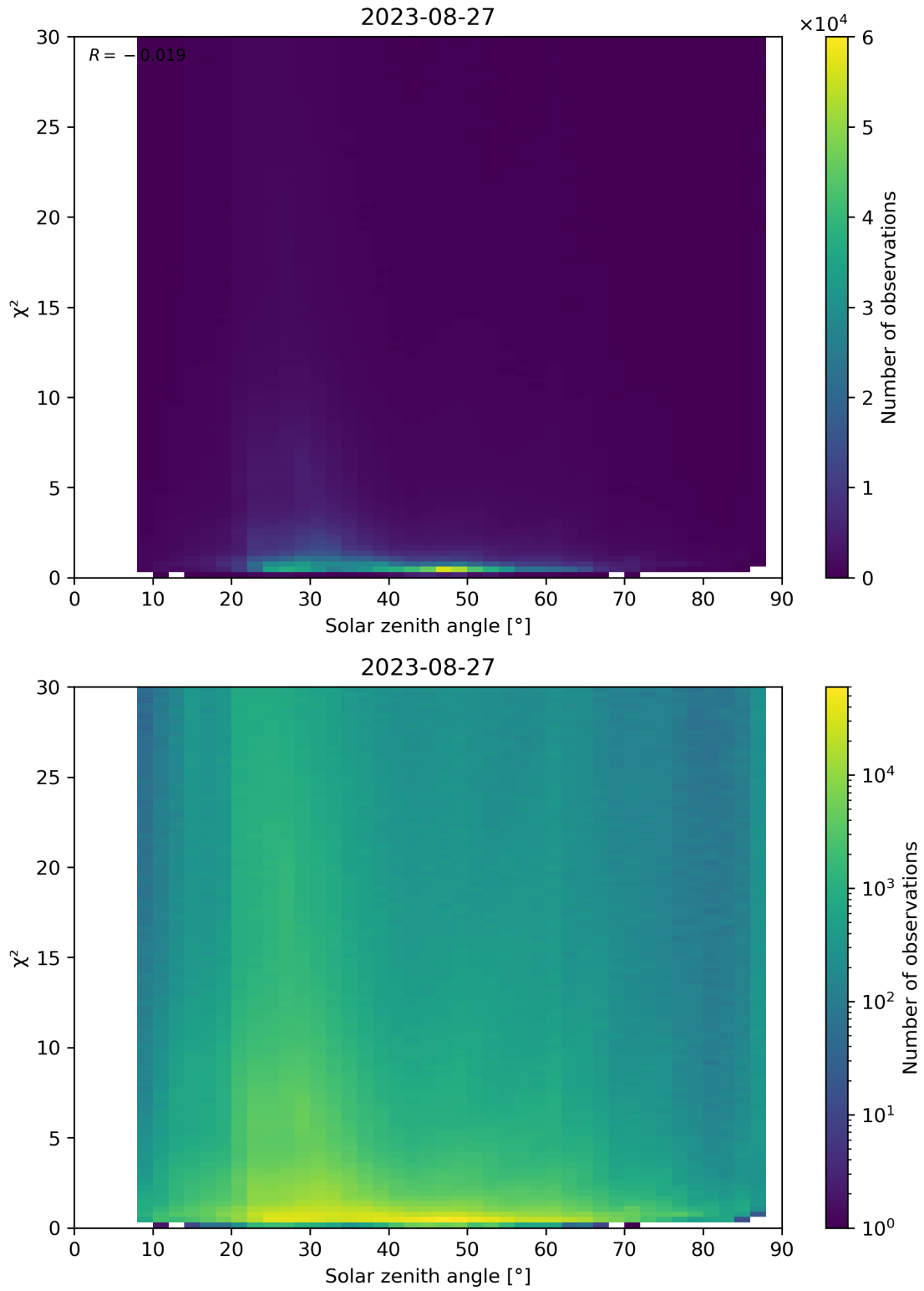
Figure 119: Scatter density plot of “Solar zenith angle” against “ \chi^2 ” for 2023-08-26 to 2023-08-28.
