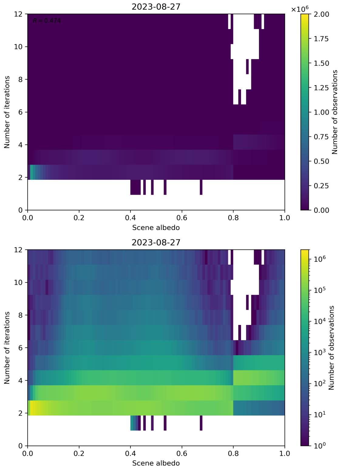
Figure 115: Scatter density plot of “Scene albedo” against “Number of iterations” for 2023-08-26 to 2023-08-28.
