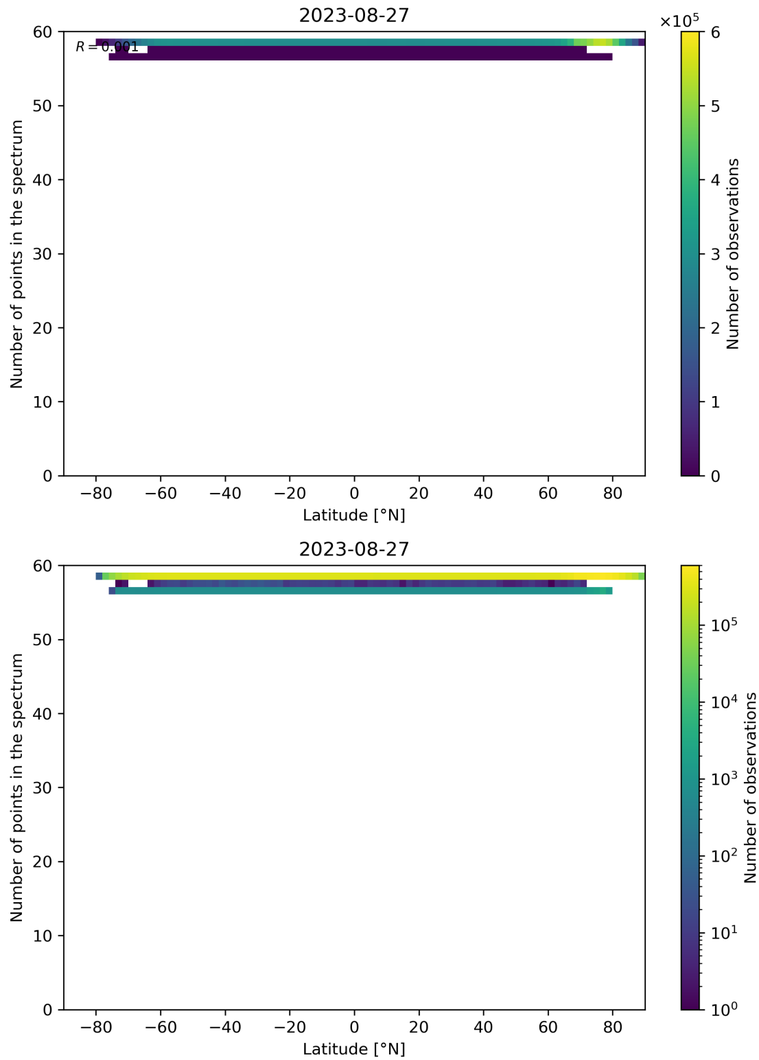
Figure 103: Scatter density plot of “Latitude” against “Number of points in the spectrum” for 2023-08-26 to 2023-08-28.
