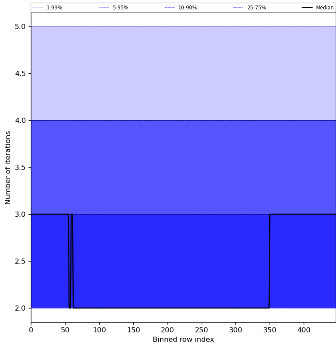
Figure 56: Along track statistics of “Number of iterations” for 2023-08-26 to 2023-08-28
