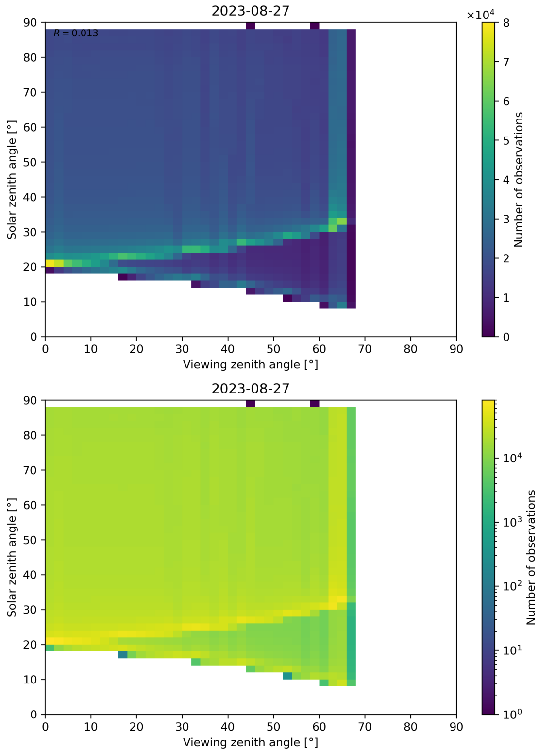
Figure 139: Scatter density plot of “Viewing zenith angle” against “Solar zenith angle” for 2023-08-26 to 2023-08-28.
