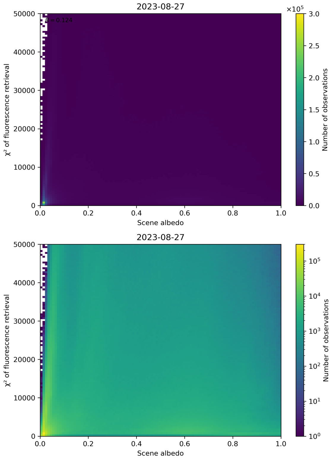
Figure 113: Scatter density plot of “Scene albedo” against “ \chi^2 of fluorescence retrieval” for 2023-08-26 to 2023-08-28.
