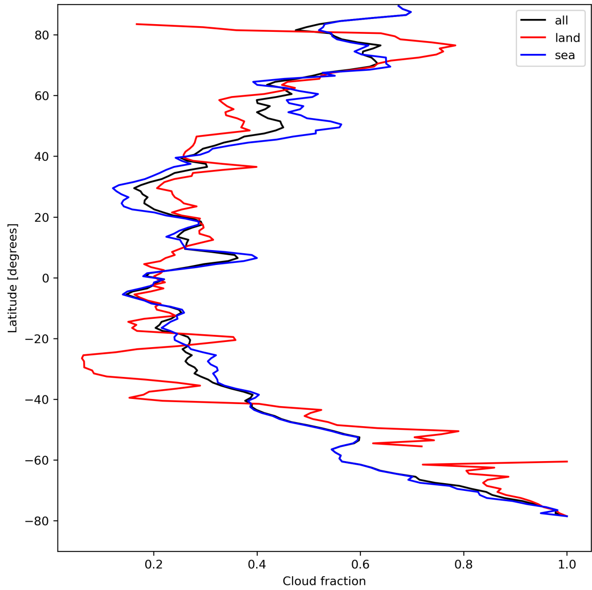
Figure 15: Zonal average of “Cloud fraction” for 2023-08-26 to 2023-08-28.
