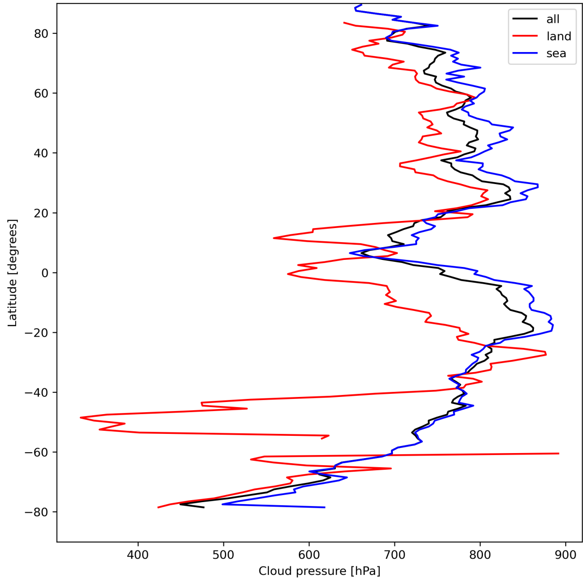
Figure 13: Zonal average of “Cloud pressure” for 2023-08-26 to 2023-08-28.
