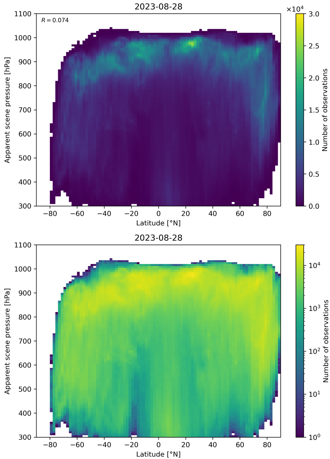
Figure 96: Scatter density plot of “Latitude” against “Apparent scene pressure” for 2023-08-27 to 2023-08-29.
