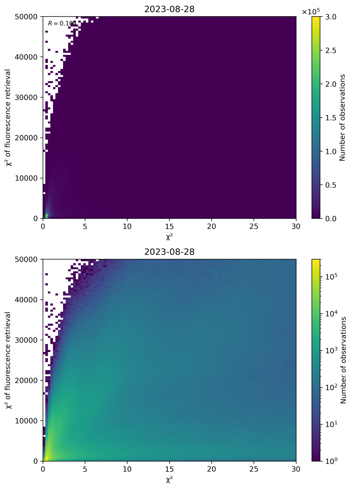
Figure 69: Scatter density plot of “ \chi^2 ” against “ \chi^2 of fluorescence retrieval” for 2023-08-27 to 2023-08-29.
