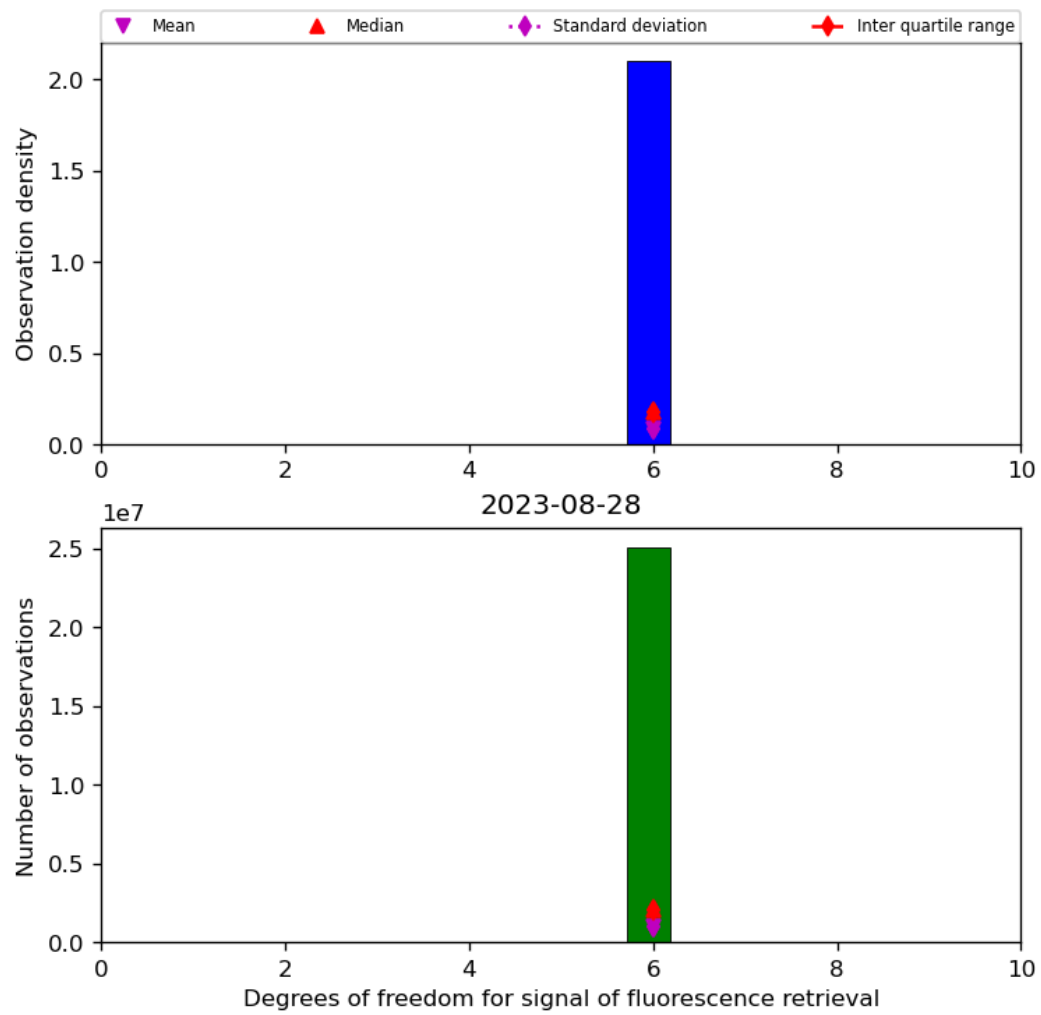
Figure 43: Histogram of “Degrees of freedom for signal of fluorescence retrieval” for 2023-08-27 to 2023-08-29
