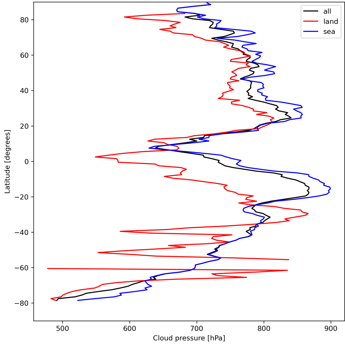
Figure 13: Zonal average of “Cloud pressure” for 2023-08-27 to 2023-08-29.
