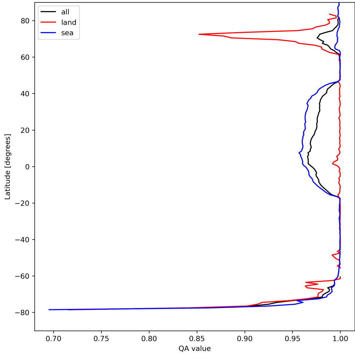
Figure 12: Zonal average of “QA value” for 2023-08-27 to 2023-08-29.
