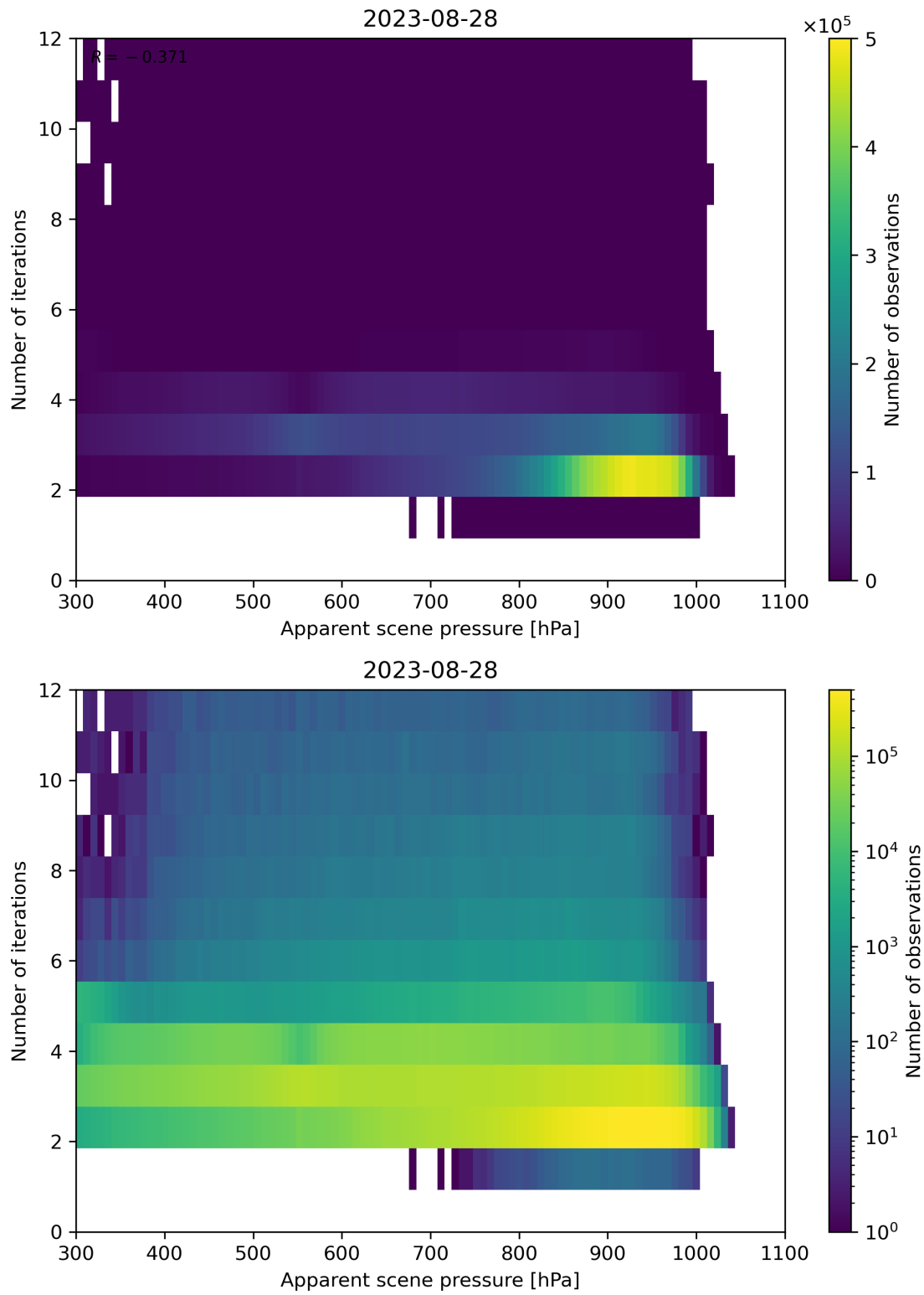
Figure 66: Scatter density plot of “Apparent scene pressure” against “Number of iterations” for 2023-08-27 to 2023-08-29.
