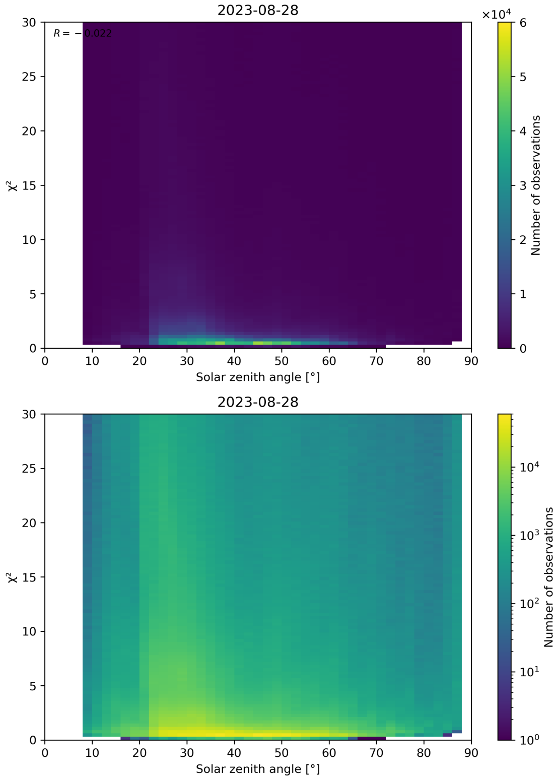
Figure 119: Scatter density plot of “Solar zenith angle” against “ \chi^2 ” for 2023-08-27 to 2023-08-29.
