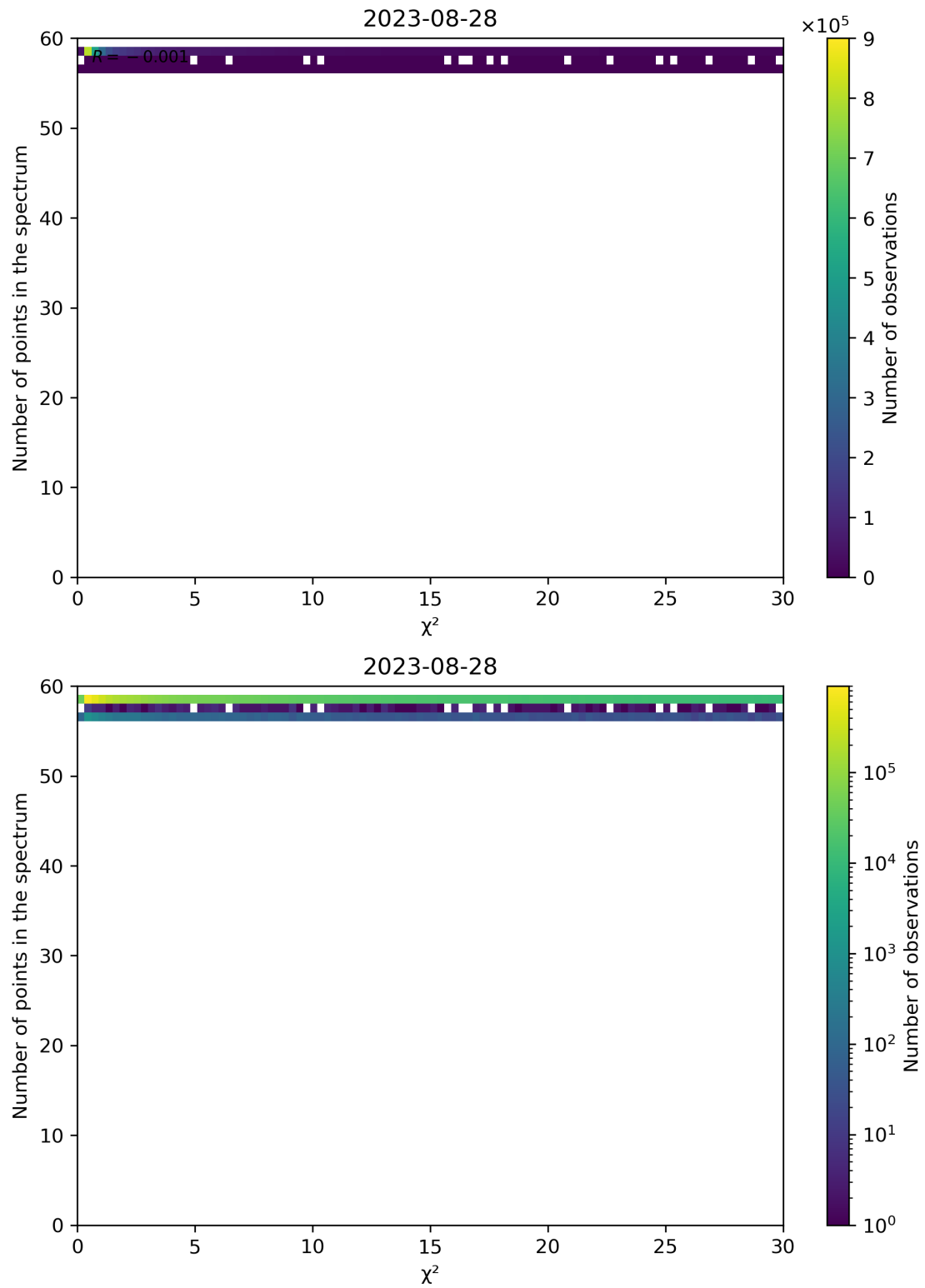
Figure 74: Scatter density plot of “ \chi^2 ” against “Number of points in the spectrum” for 2023-08-27 to 2023-08-29.
