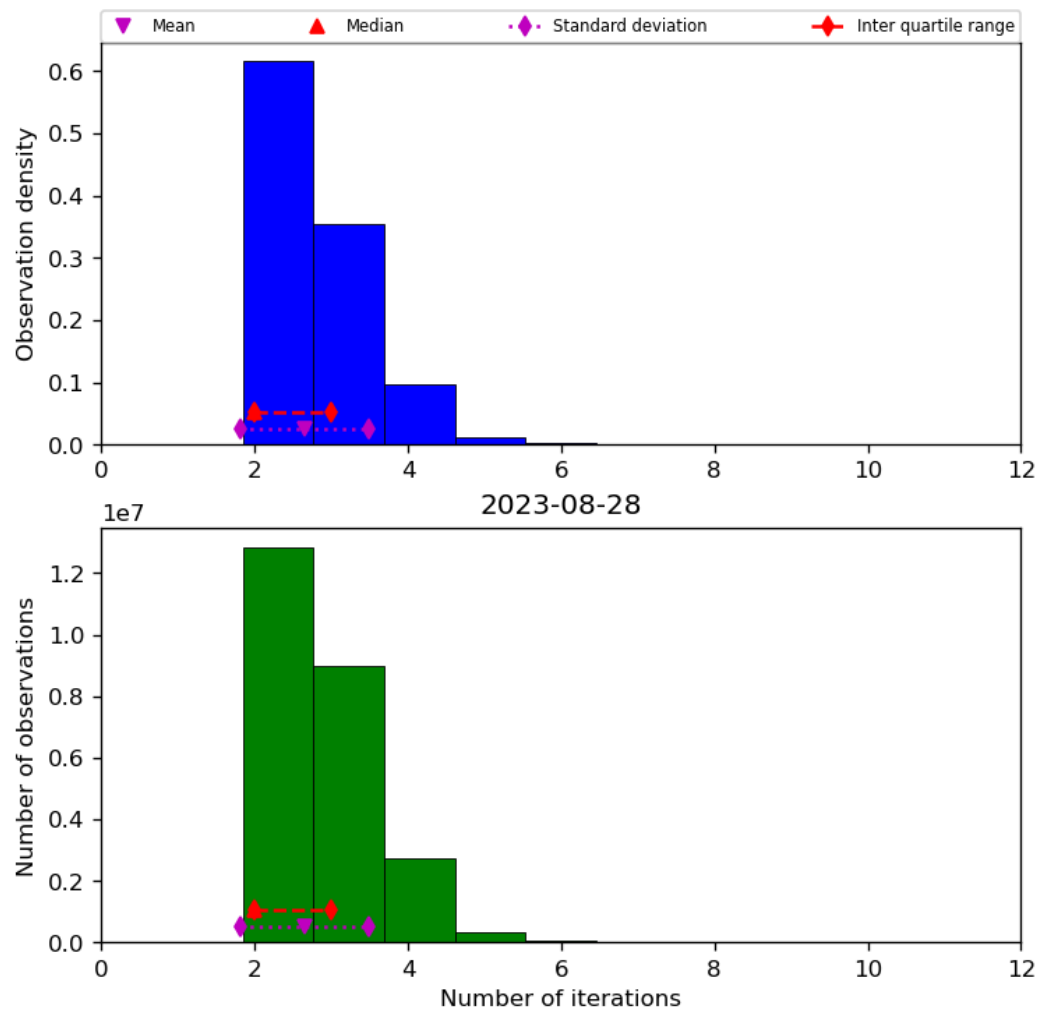
Figure 39: Histogram of “Number of iterations” for 2023-08-27 to 2023-08-29
