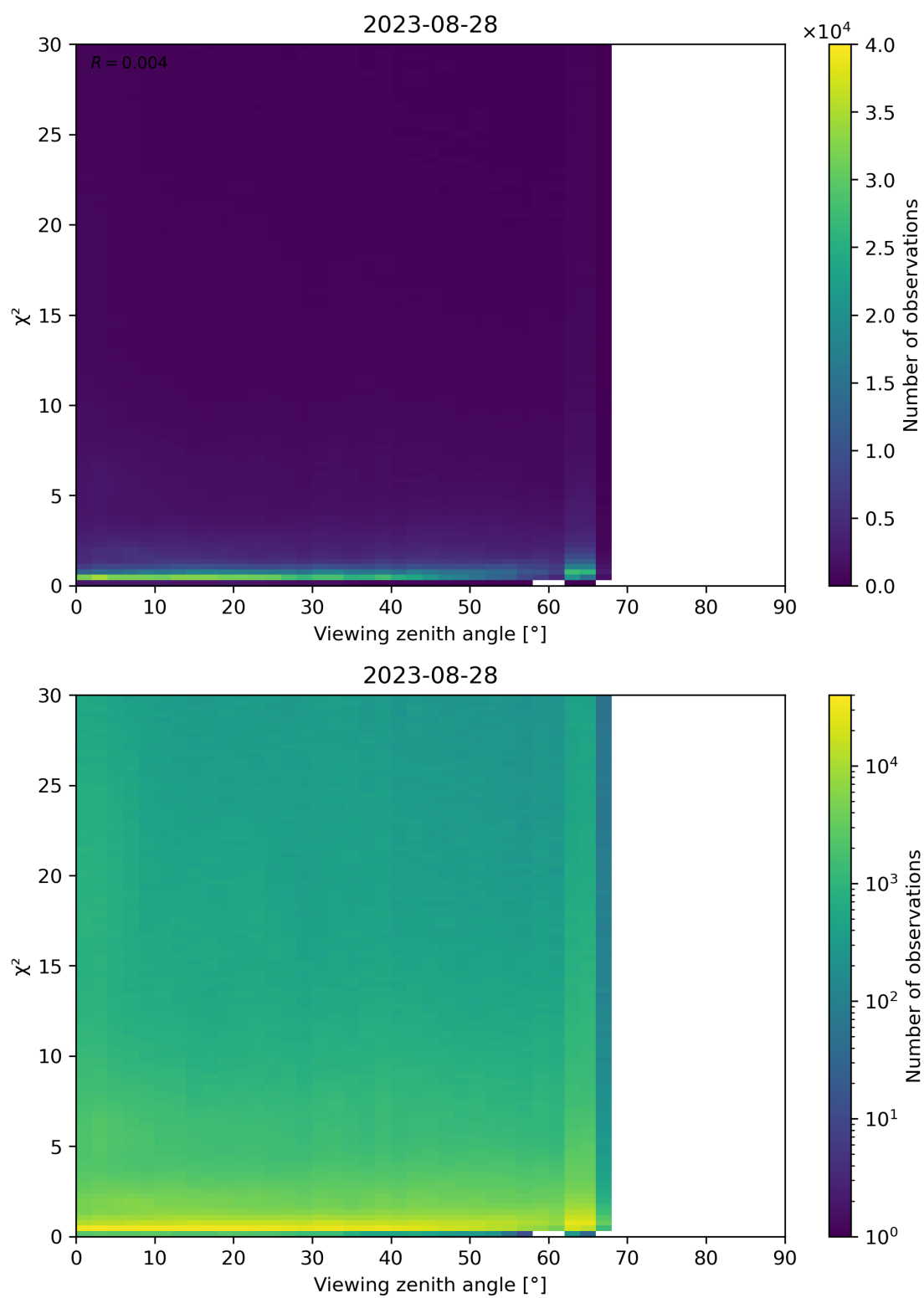
Figure 130: Scatter density plot of “Viewing zenith angle” against “ \chi^2 ” for 2023-08-27 to 2023-08-29.
