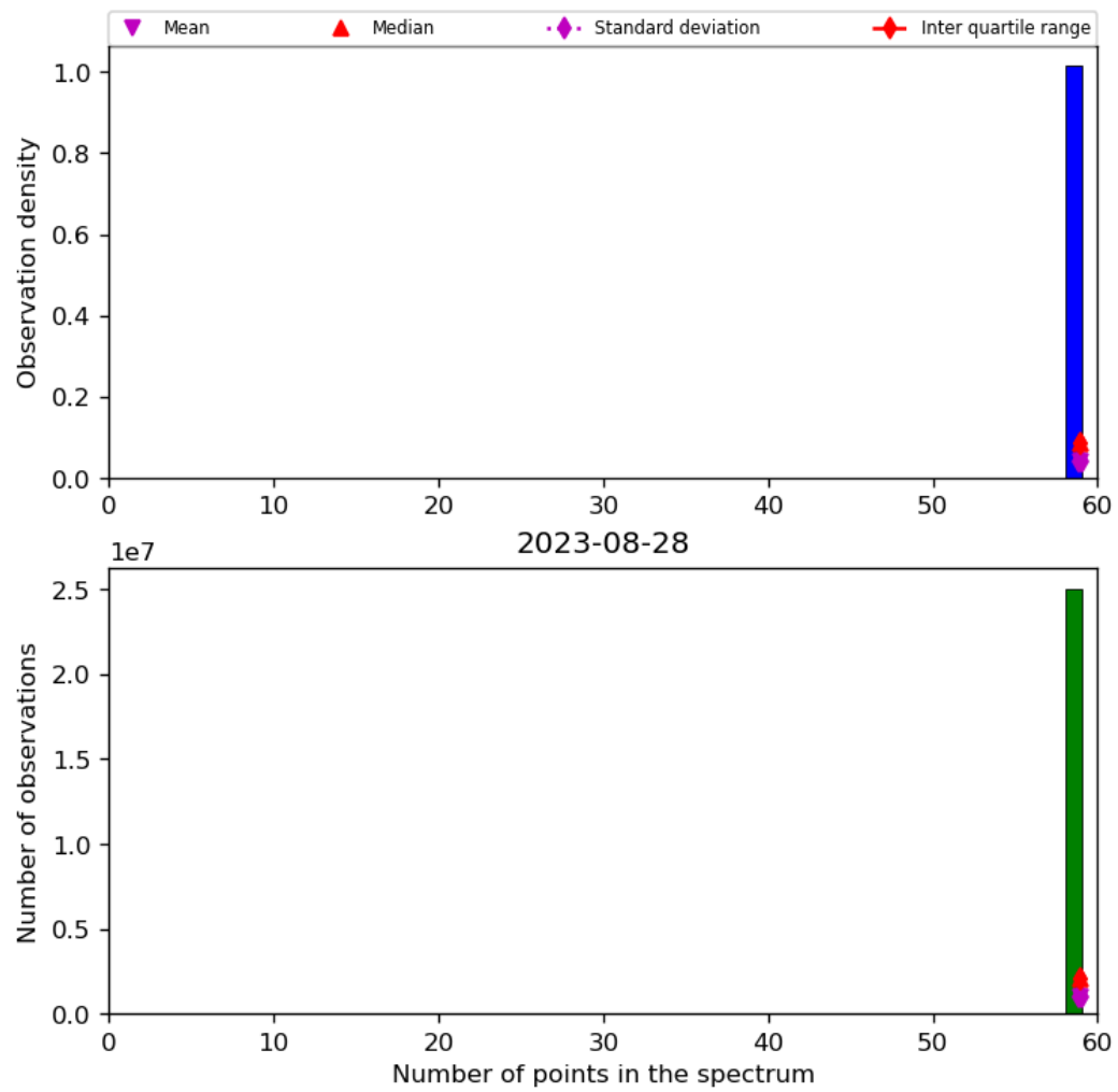
Figure 44: Histogram of “Number of points in the spectrum” for 2023-08-27 to 2023-08-29
