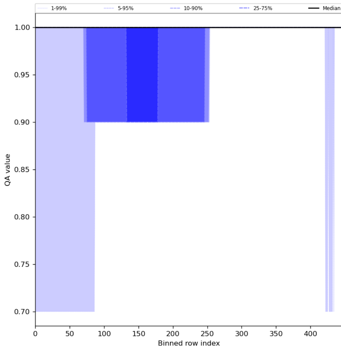
Figure 46: Along track statistics of “QA value” for 2023-08-27 to 2023-08-29
