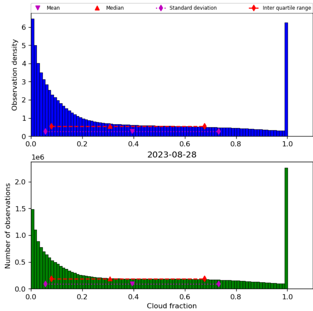
Figure 32: Histogram of “Cloud fraction” for 2023-08-27 to 2023-08-29
