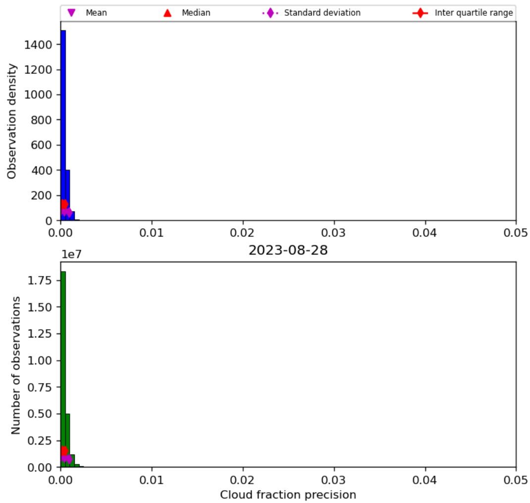
Figure 33: Histogram of “Cloud fraction precision” for 2023-08-27 to 2023-08-29
