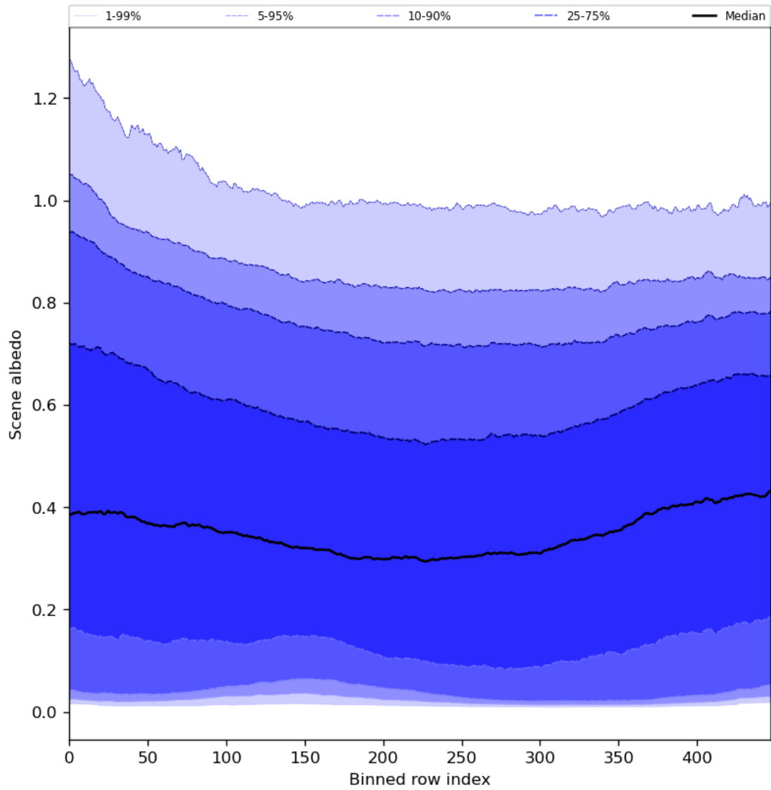
Figure 51: Along track statistics of “Scene albedo” for 2023-08-27 to 2023-08-29
