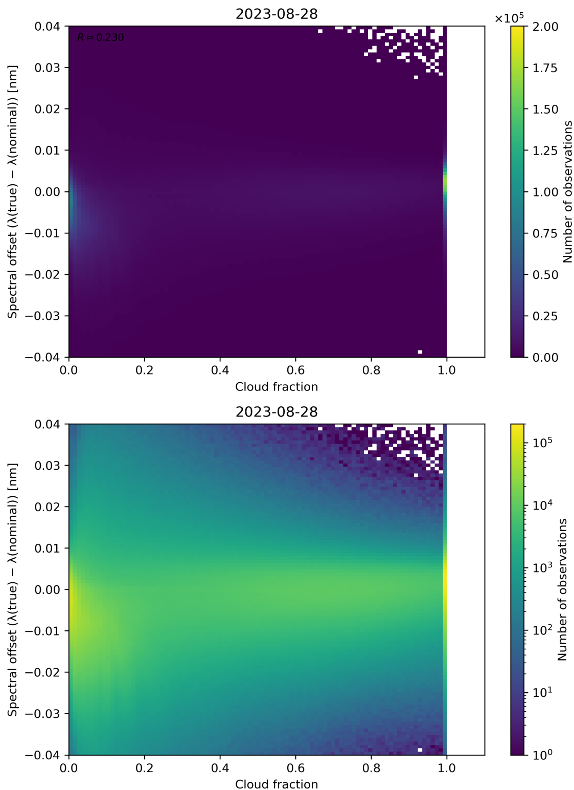
Figure 83: Scatter density plot of “Cloud fraction” against “Spectral offset ( \lambda(\text{true}) - \lambda(\text{nominal}) )” for 2023-08-27 to 2023-08-29.
