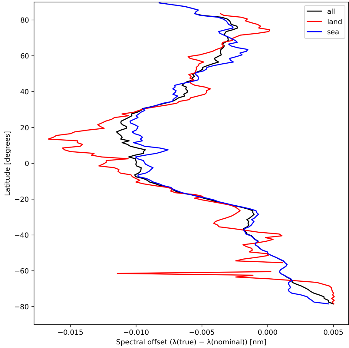
Figure 28: Zonal average of “Spectral offset ( \lambda(\text{true}) - \lambda(\text{nominal}) )” for 2023-08-27 to 2023-08-29.
