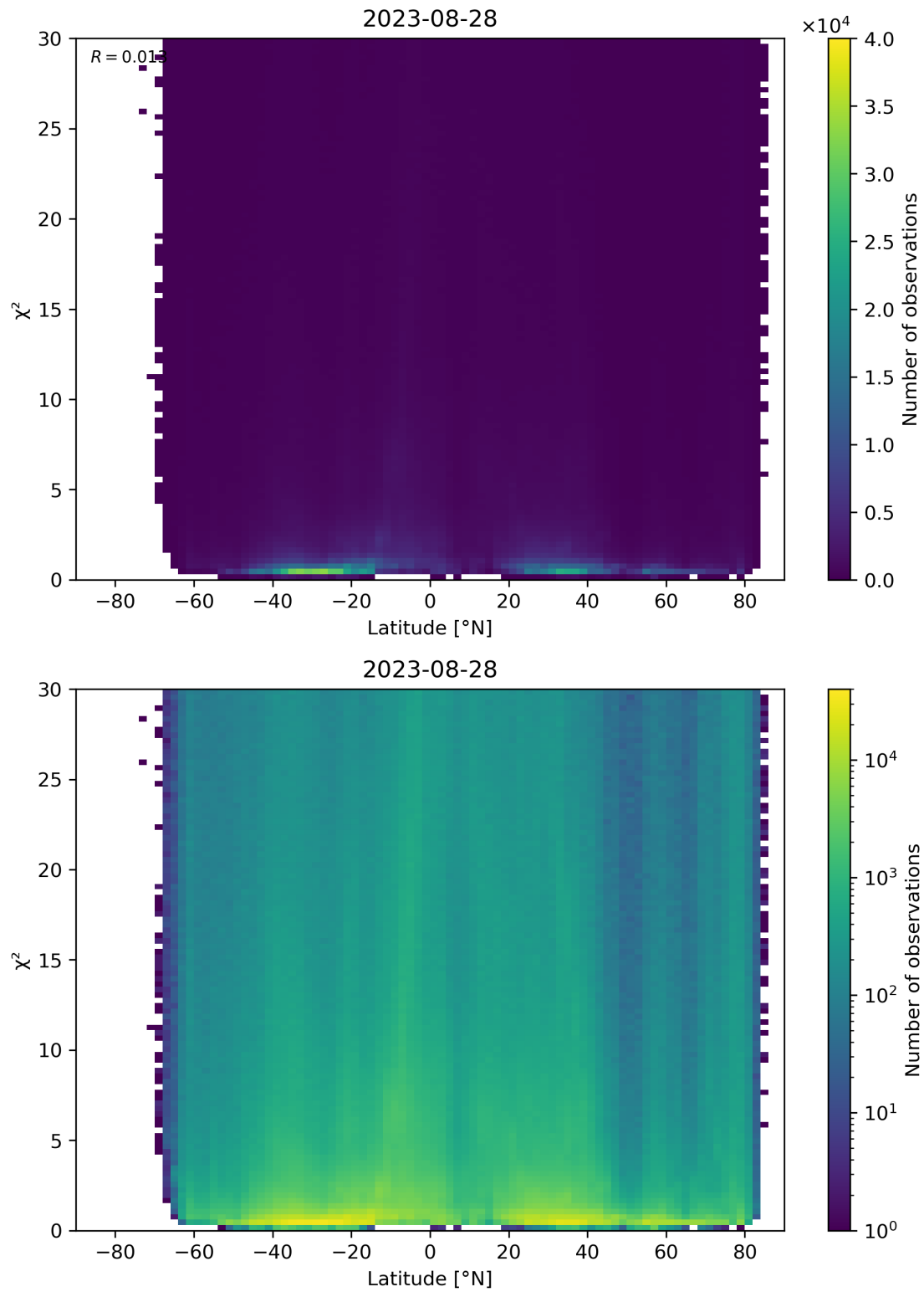
Figure 97: Scatter density plot of “Latitude” against “ \chi^2 ” for 2023-08-27 to 2023-08-29.
