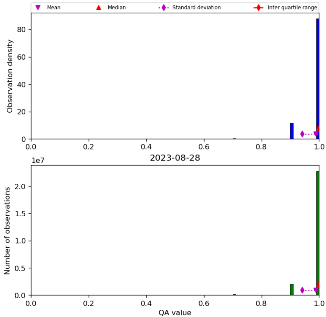
Figure 29: Histogram of “QA value” for 2023-08-27 to 2023-08-29
