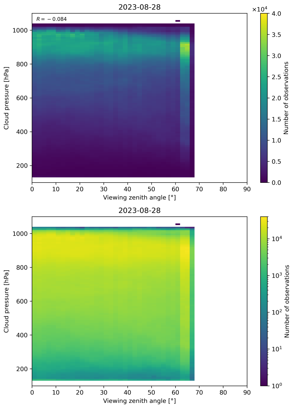
Figure 133: Scatter density plot of “Viewing zenith angle” against “Cloud pressure” for 2023-08-27 to 2023-08-29.
