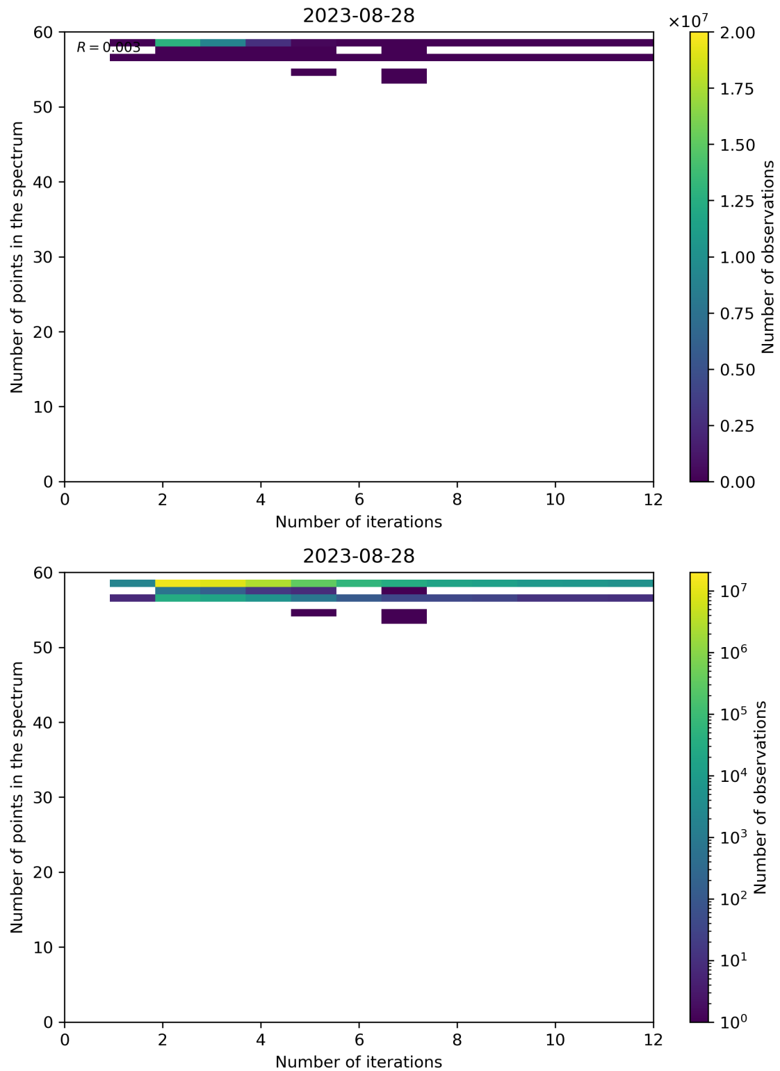
Figure 108: Scatter density plot of “Number of iterations” against “Number of points in the spectrum” for 2023-08-27 to 2023-08-29.
