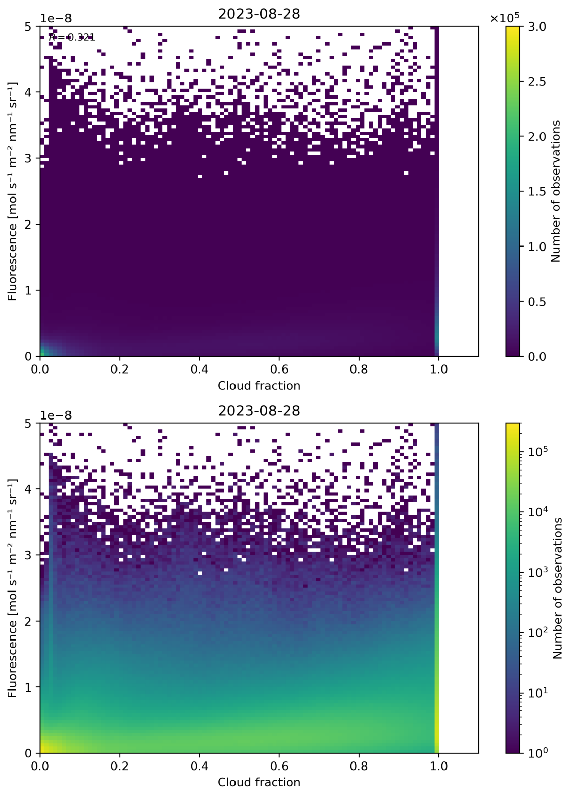
Figure 79: Scatter density plot of “Cloud fraction” against “Fluorescence” for 2023-08-27 to 2023-08-29.
