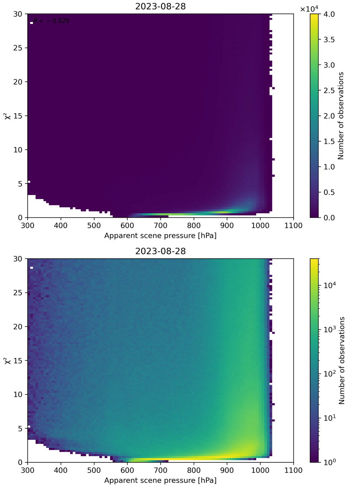
Figure 63: Scatter density plot of “Apparent scene pressure” against “ \chi^2 ” for 2023-08-27 to 2023-08-29.
