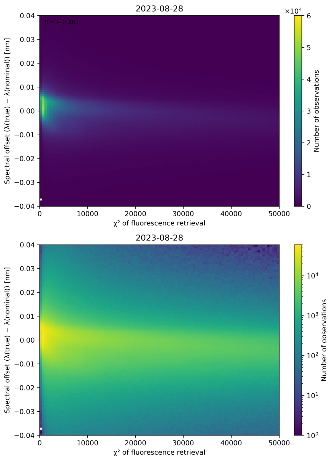
Figure 72: Scatter density plot of " \chi^2 of fluorescence retrieval" against "Spectral offset ( \lambda(\text{true}) - \lambda(\text{nominal})) " for 2023-08-27 to 2023-08-29.
