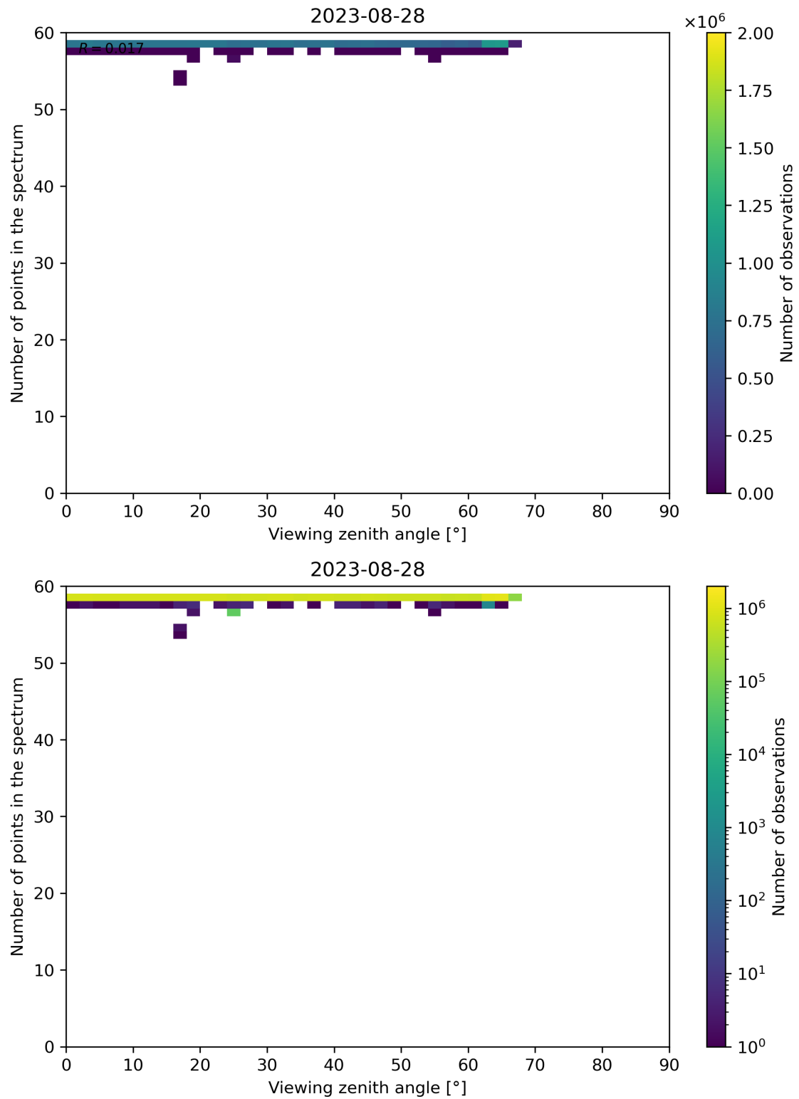
Figure 137: Scatter density plot of “Viewing zenith angle” against “Number of points in the spectrum” for 2023-08-27 to 2023-08-29.
