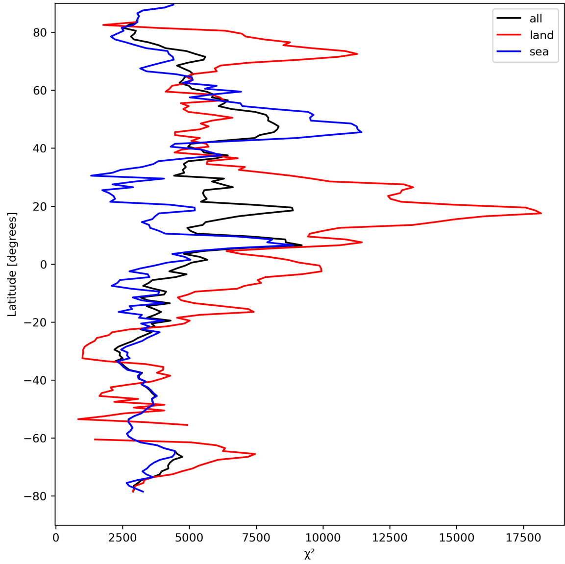
Figure 21: Zonal average of “ \chi^2 ” for 2023-08-27 to 2023-08-29.
