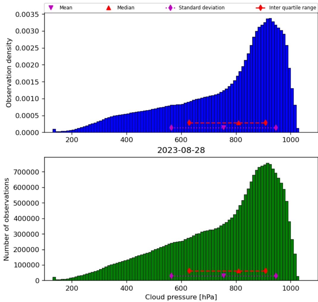
Figure 30: Histogram of “Cloud pressure” for 2023-08-27 to 2023-08-29
