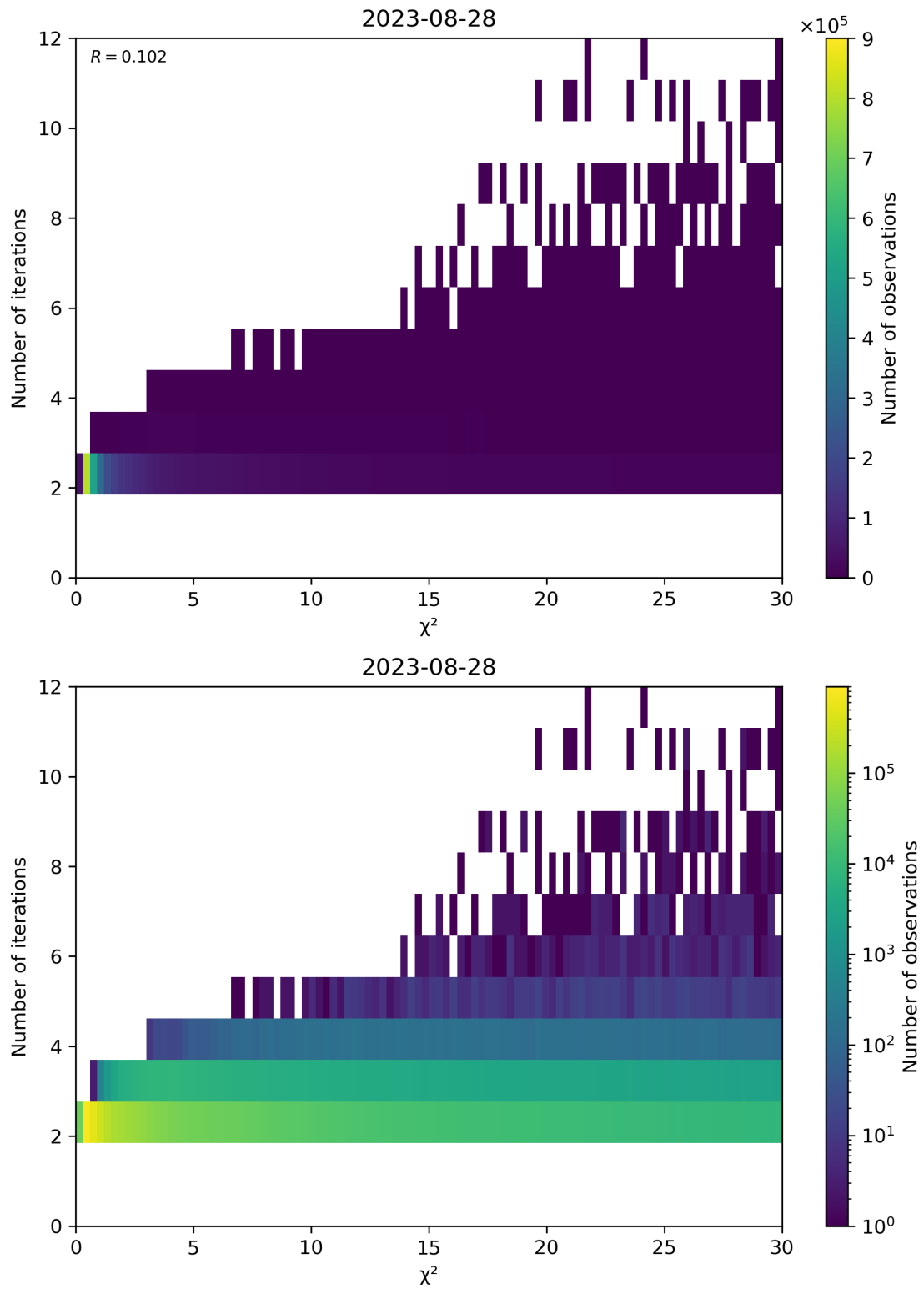
Figure 73: Scatter density plot of “ \chi^2 ” against “Number of iterations” for 2023-08-27 to 2023-08-29.
