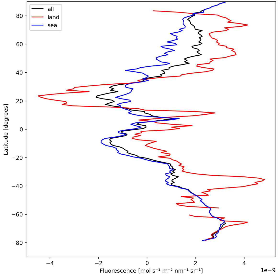
Figure 23: Zonal average of “Fluorescence” for 2023-08-27 to 2023-08-29.
