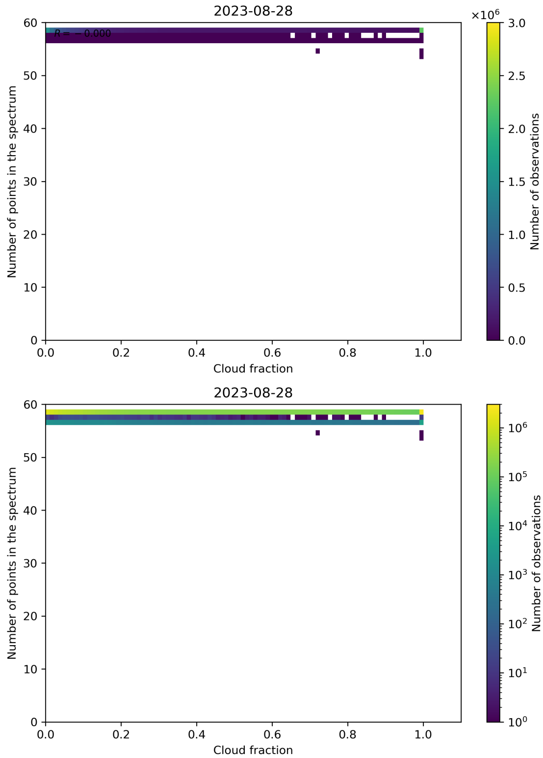
Figure 81: Scatter density plot of “Cloud fraction” against “Number of points in the spectrum” for 2023-08-27 to 2023-08-29.
