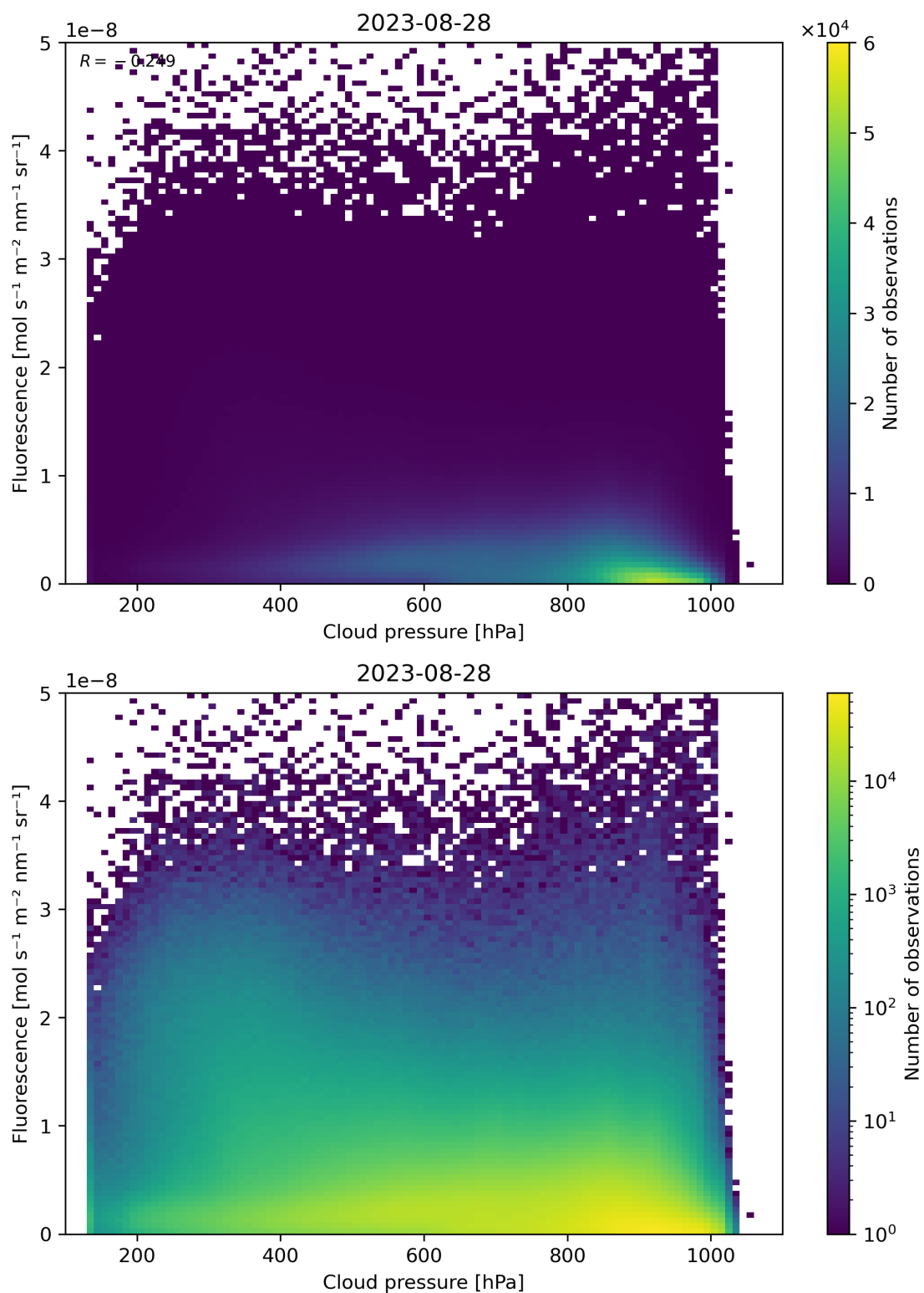
Figure 88: Scatter density plot of “Cloud pressure” against “Fluorescence” for 2023-08-27 to 2023-08-29.
