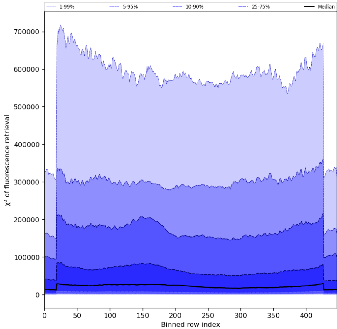
Figure 59: Along track statistics of “ \chi^2 of fluorescence retrieval” for 2023-08-27 to 2023-08-29
