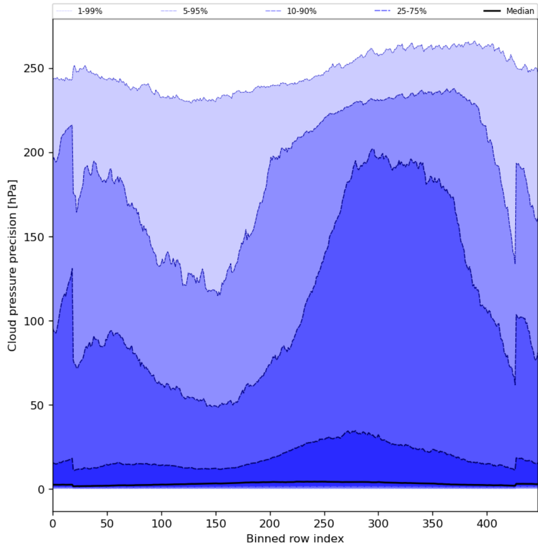
Figure 48: Along track statistics of “Cloud pressure precision” for 2023-08-27 to 2023-08-29
