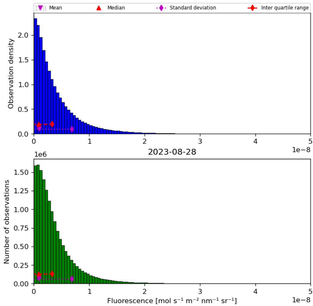
Figure 40: Histogram of “Fluorescence” for 2023-08-27 to 2023-08-29
