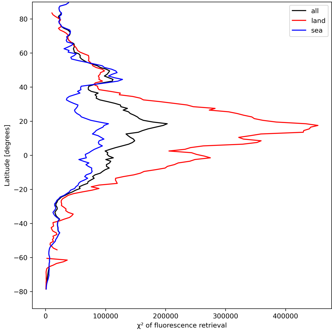
Figure 25: Zonal average of “ \chi^2 of fluorescence retrieval” for 2023-08-27 to 2023-08-29.
