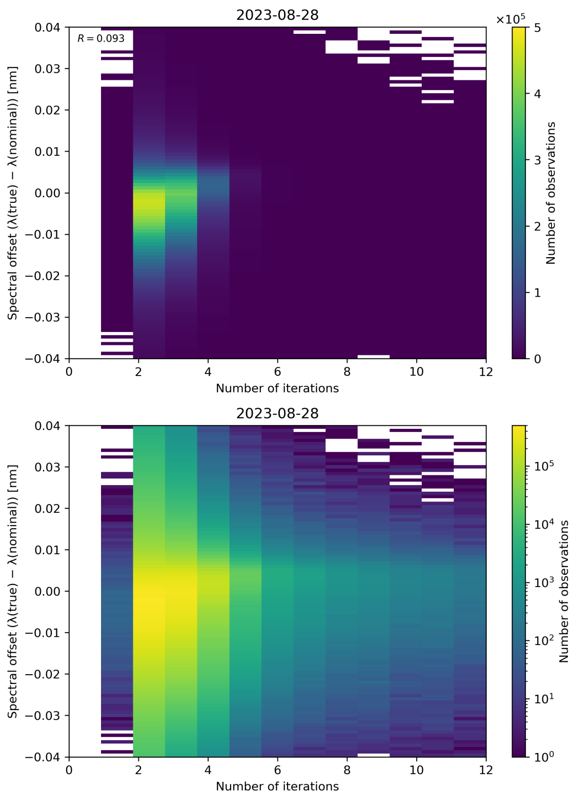
Figure 109: Scatter density plot of “Number of iterations” against “Spectral offset ( \lambda(\text{true}) - \lambda(\text{nominal}) )” for 2023-08-27 to 2023-08-29.
