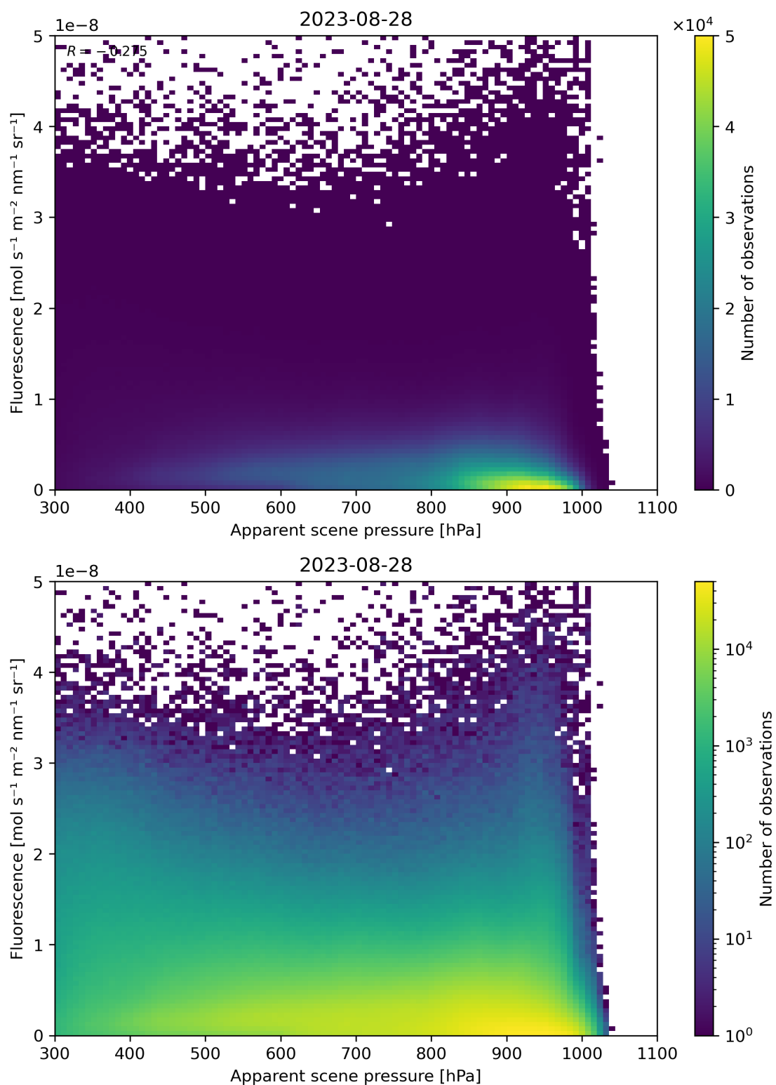
Figure 65: Scatter density plot of “Apparent scene pressure” against “Fluorescence” for 2023-08-27 to 2023-08-29.
