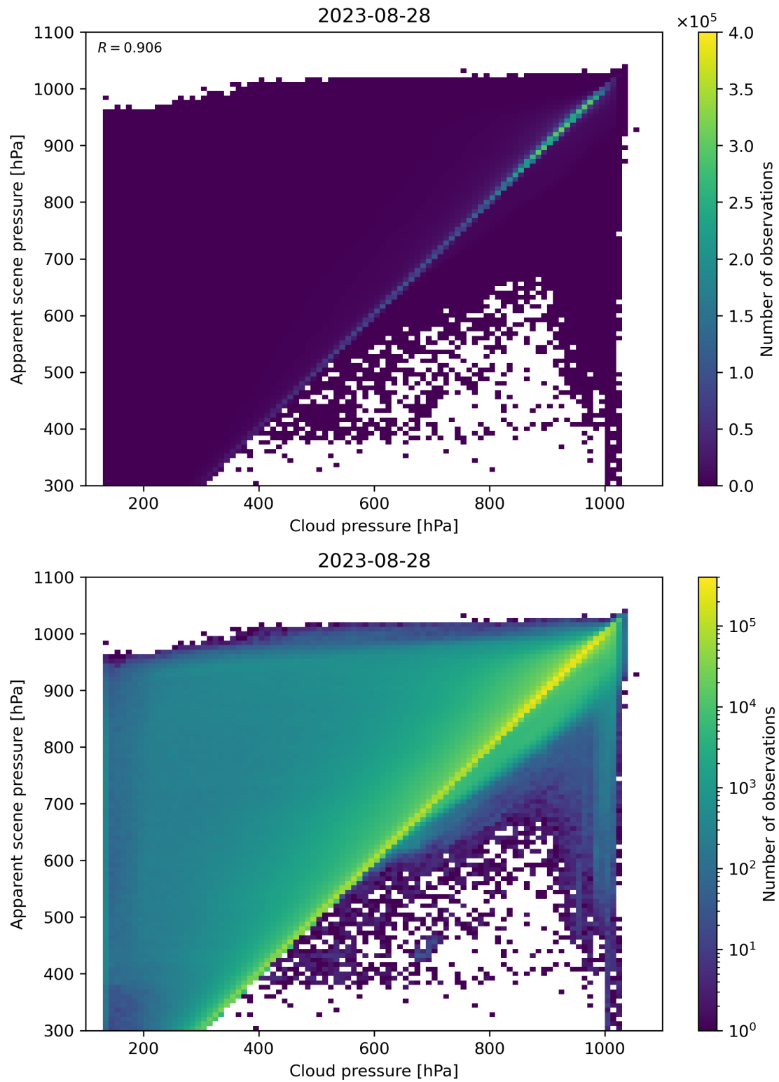
Figure 84: Scatter density plot of “Cloud pressure” against “Apparent scene pressure” for 2023-08-27 to 2023-08-29.
