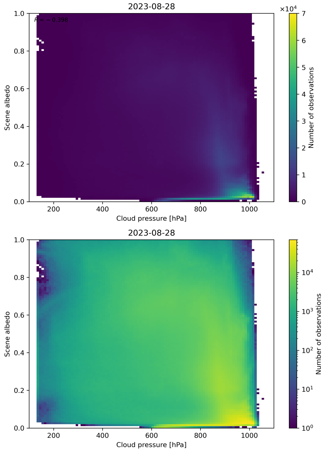
Figure 91: Scatter density plot of “Cloud pressure” against “Scene albedo” for 2023-08-27 to 2023-08-29.
