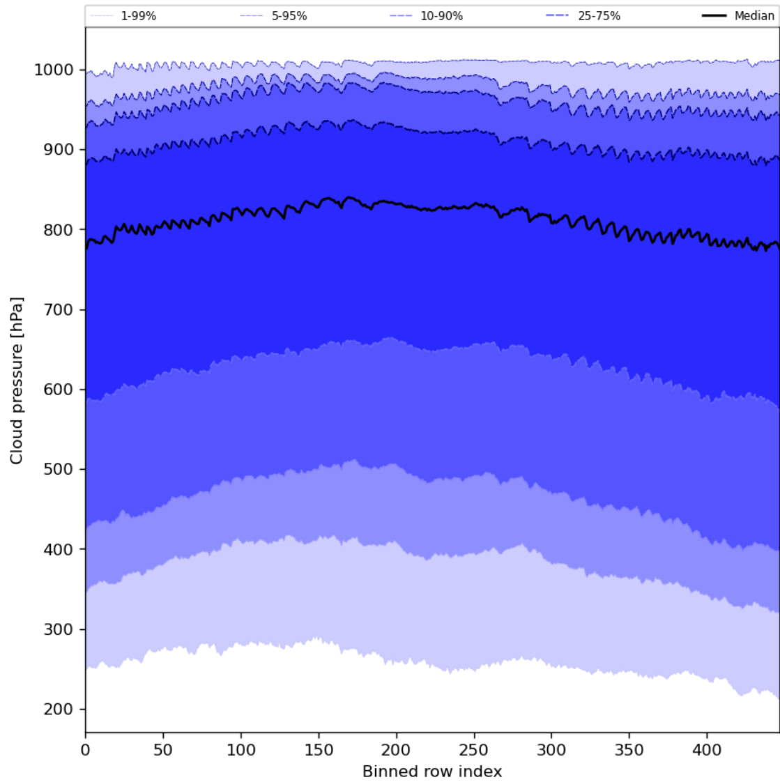
Figure 47: Along track statistics of “Cloud pressure” for 2023-08-27 to 2023-08-29
