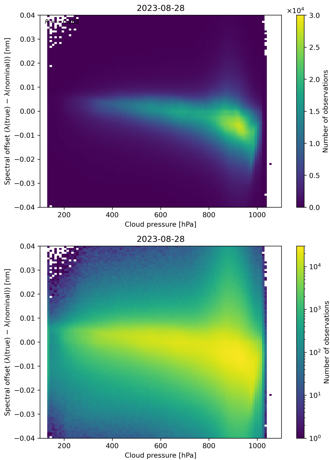
Figure 92: Scatter density plot of “Cloud pressure” against “Spectral offset ( \lambda(\text{true}) - \lambda(\text{nominal}) )” for 2023-08-27 to 2023-08-29.
