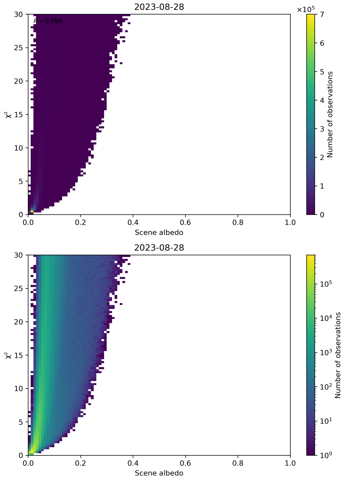
Figure 112: Scatter density plot of “Scene albedo” against “ \chi^2 ” for 2023-08-27 to 2023-08-29.
