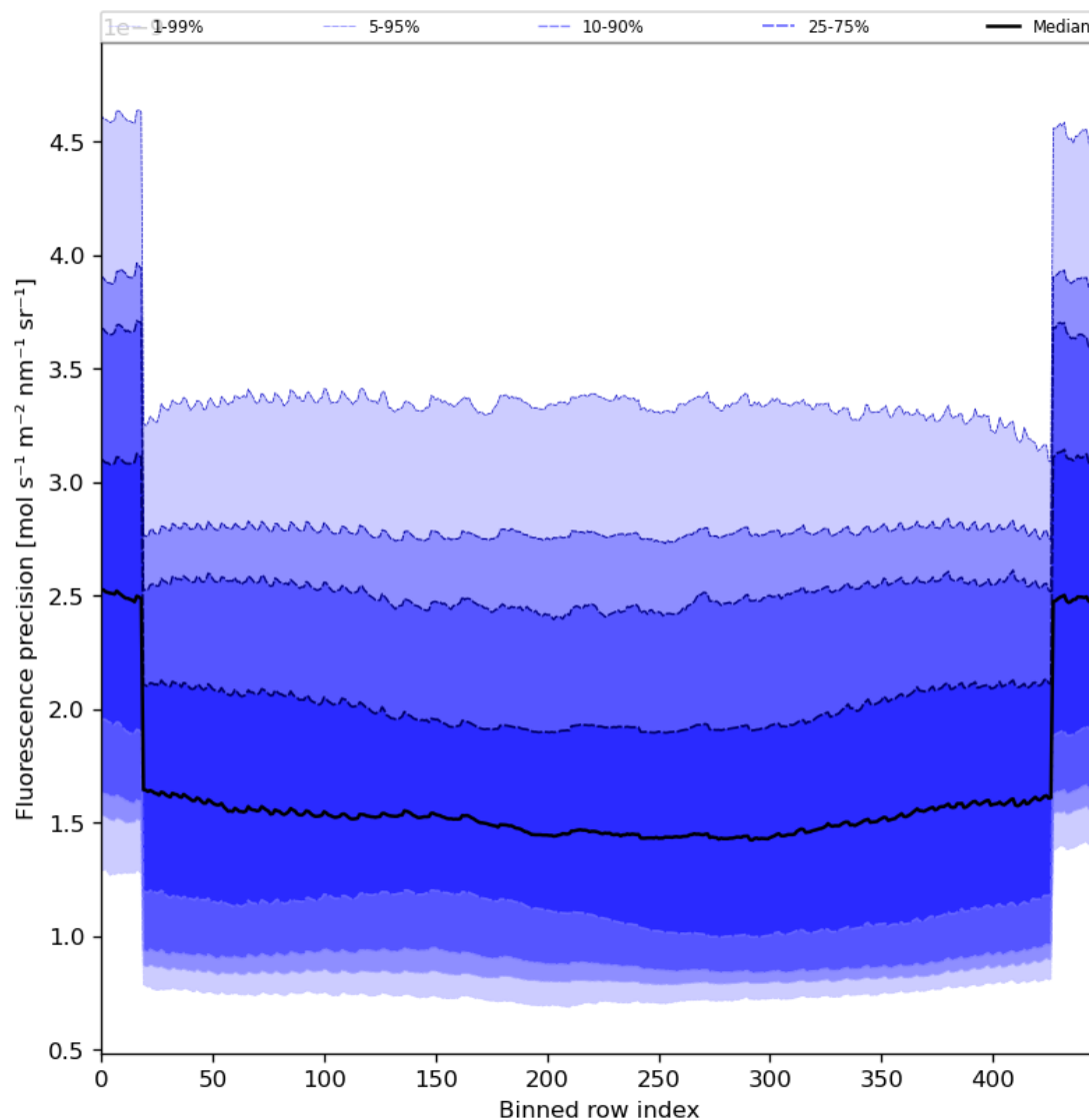
Figure 58: Along track statistics of “Fluorescence precision” for 2023-08-27 to 2023-08-29
