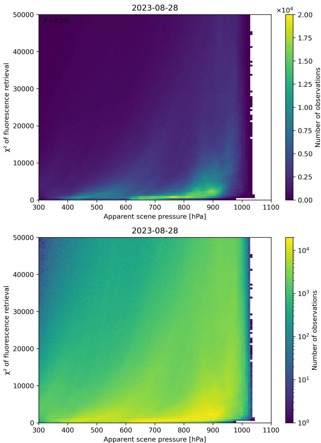
Figure 64: Scatter density plot of “Apparent scene pressure” against “ \chi^2 of fluorescence retrieval” for 2023-08-27 to 2023-08-29.
