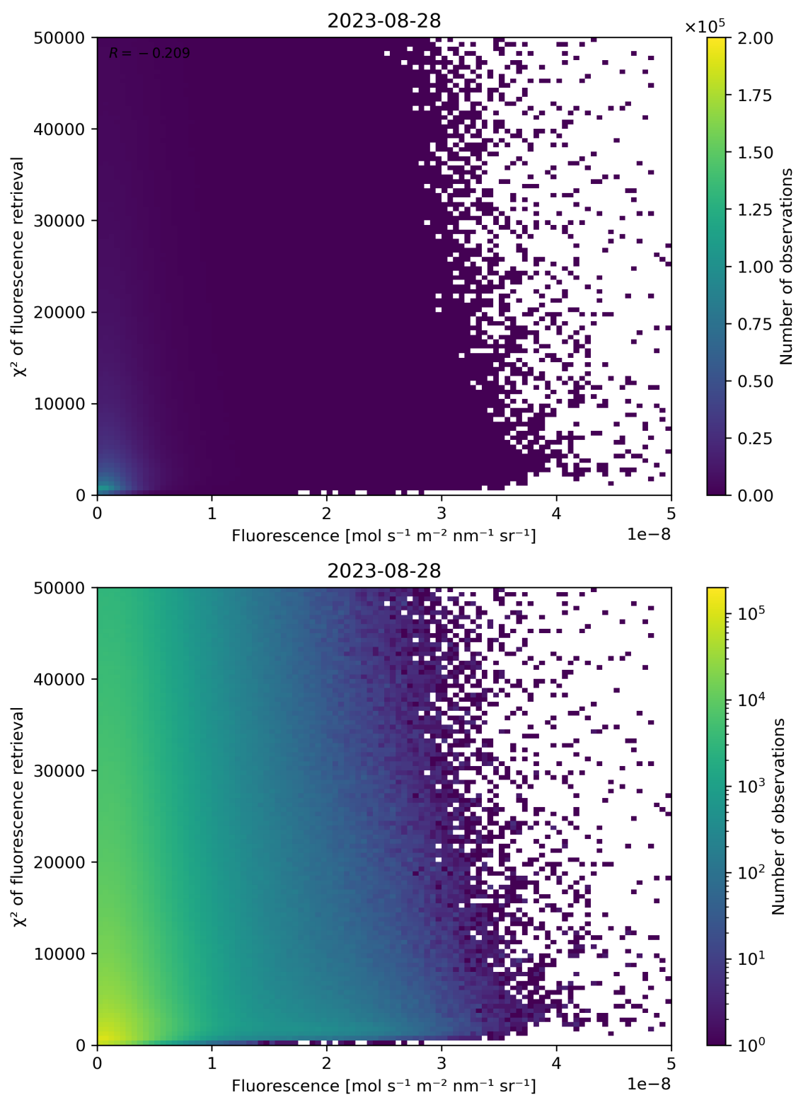
Figure 93: Scatter density plot of “Fluorescence” against “ \chi^2 of fluorescence retrieval” for 2023-08-27 to 2023-08-29.
