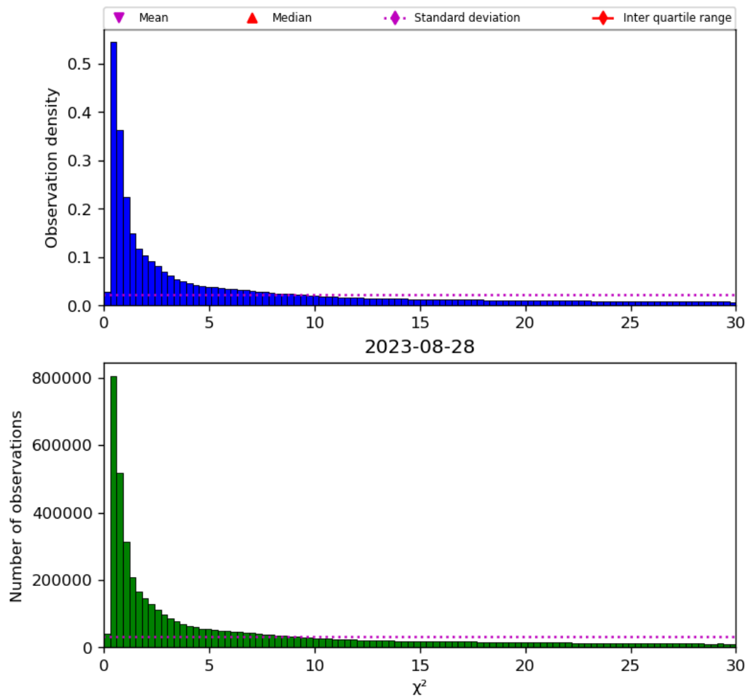
Figure 38: Histogram of “ \chi^2 ” for 2023-08-27 to 2023-08-29
