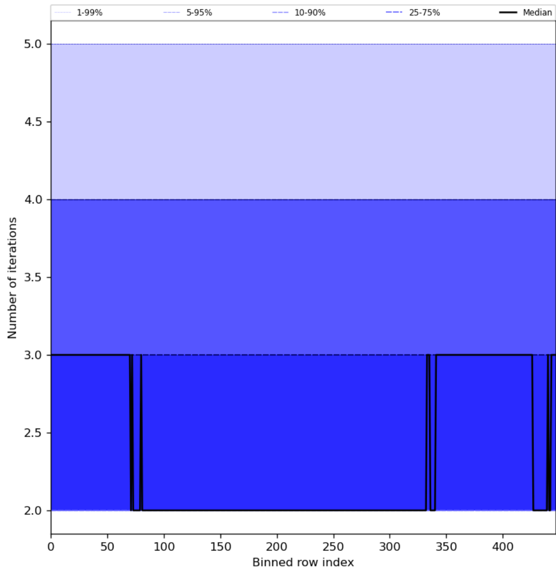
Figure 56: Along track statistics of “Number of iterations” for 2023-08-27 to 2023-08-29
