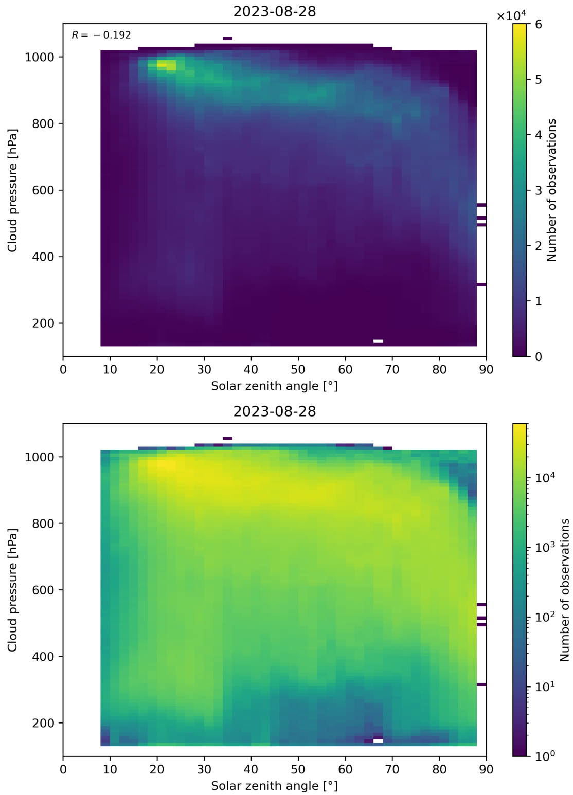
Figure 122: Scatter density plot of “Solar zenith angle” against “Cloud pressure” for 2023-08-27 to 2023-08-29.
