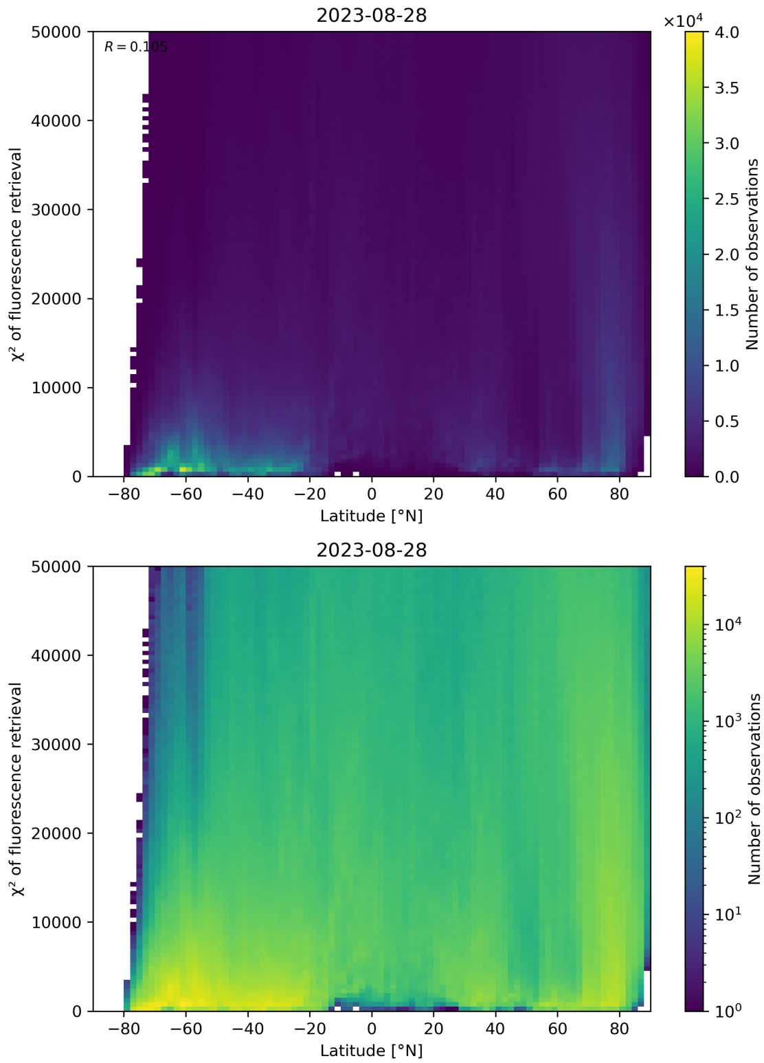
Figure 98: Scatter density plot of “Latitude” against “ \chi^2 of fluorescence retrieval” for 2023-08-27 to 2023-08-29.
