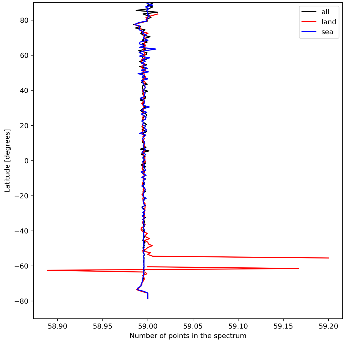
Figure 27: Zonal average of “Number of points in the spectrum” for 2023-08-27 to 2023-08-29.
