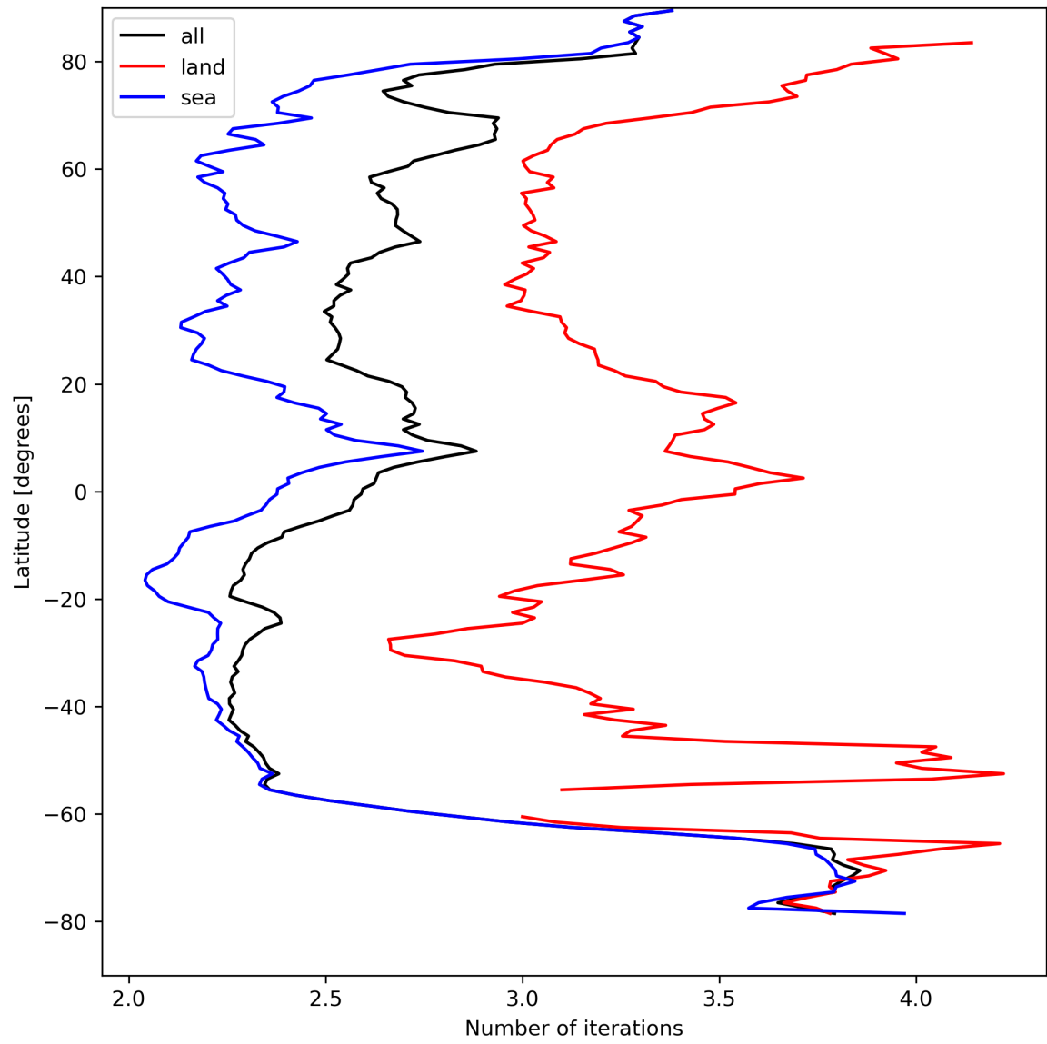
Figure 22: Zonal average of “Number of iterations” for 2023-08-27 to 2023-08-29.
