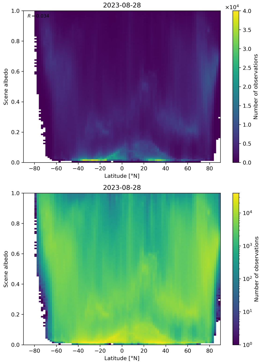
Figure 104: Scatter density plot of “Latitude” against “Scene albedo” for 2023-08-27 to 2023-08-29.
