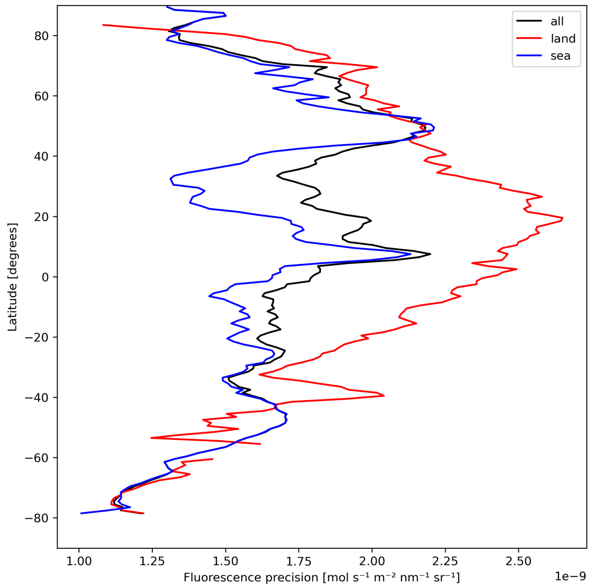
Figure 24: Zonal average of “Fluorescence precision” for 2023-08-27 to 2023-08-29.
