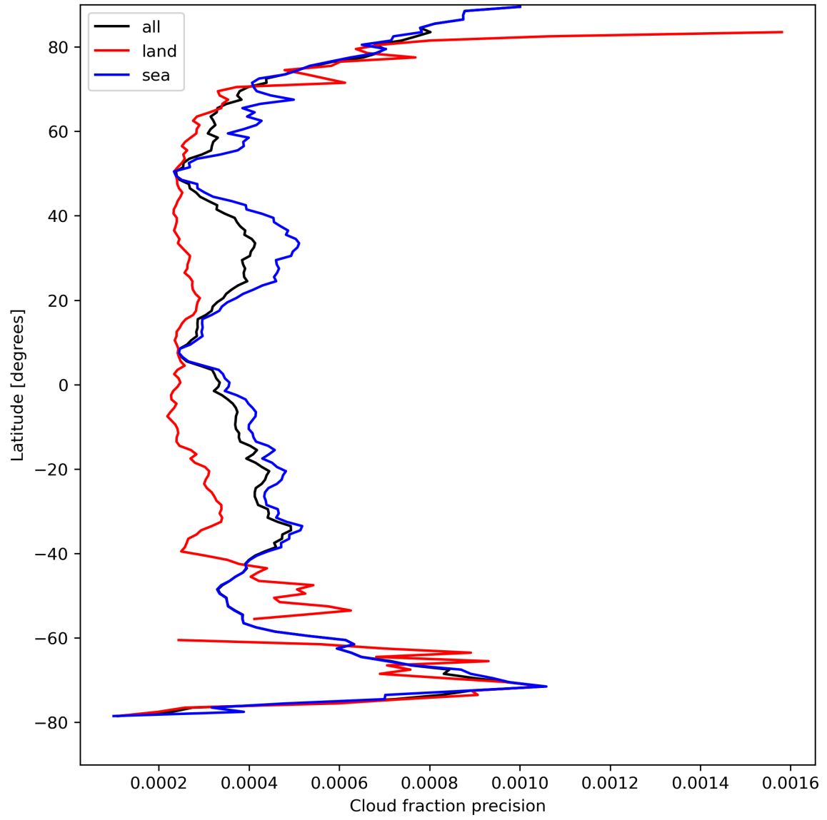
Figure 16: Zonal average of “Cloud fraction precision” for 2023-08-27 to 2023-08-29.
