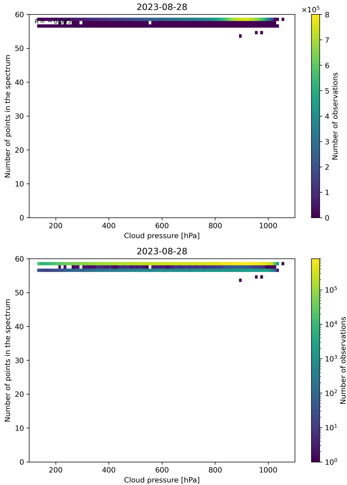
Figure 90: Scatter density plot of “Cloud pressure” against “Number of points in the spectrum” for 2023-08-27 to 2023-08-29.
