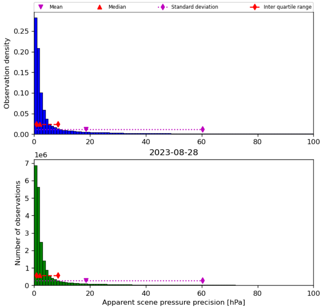
Figure 37: Histogram of “Apparent scene pressure precision” for 2023-08-27 to 2023-08-29
