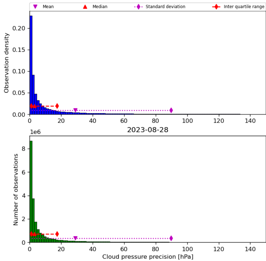
Figure 31: Histogram of “Cloud pressure precision” for 2023-08-27 to 2023-08-29
