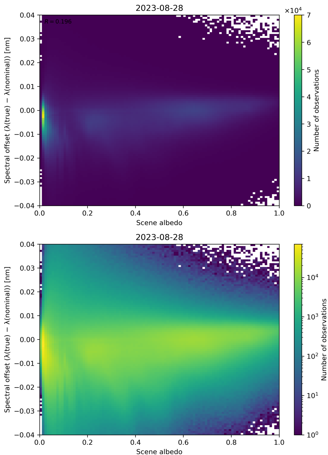
Figure 117: Scatter density plot of “Scene albedo” against “Spectral offset ( \lambda(\text{true}) - \lambda(\text{nominal}) )” for 2023-08-27 to 2023-08-29.
