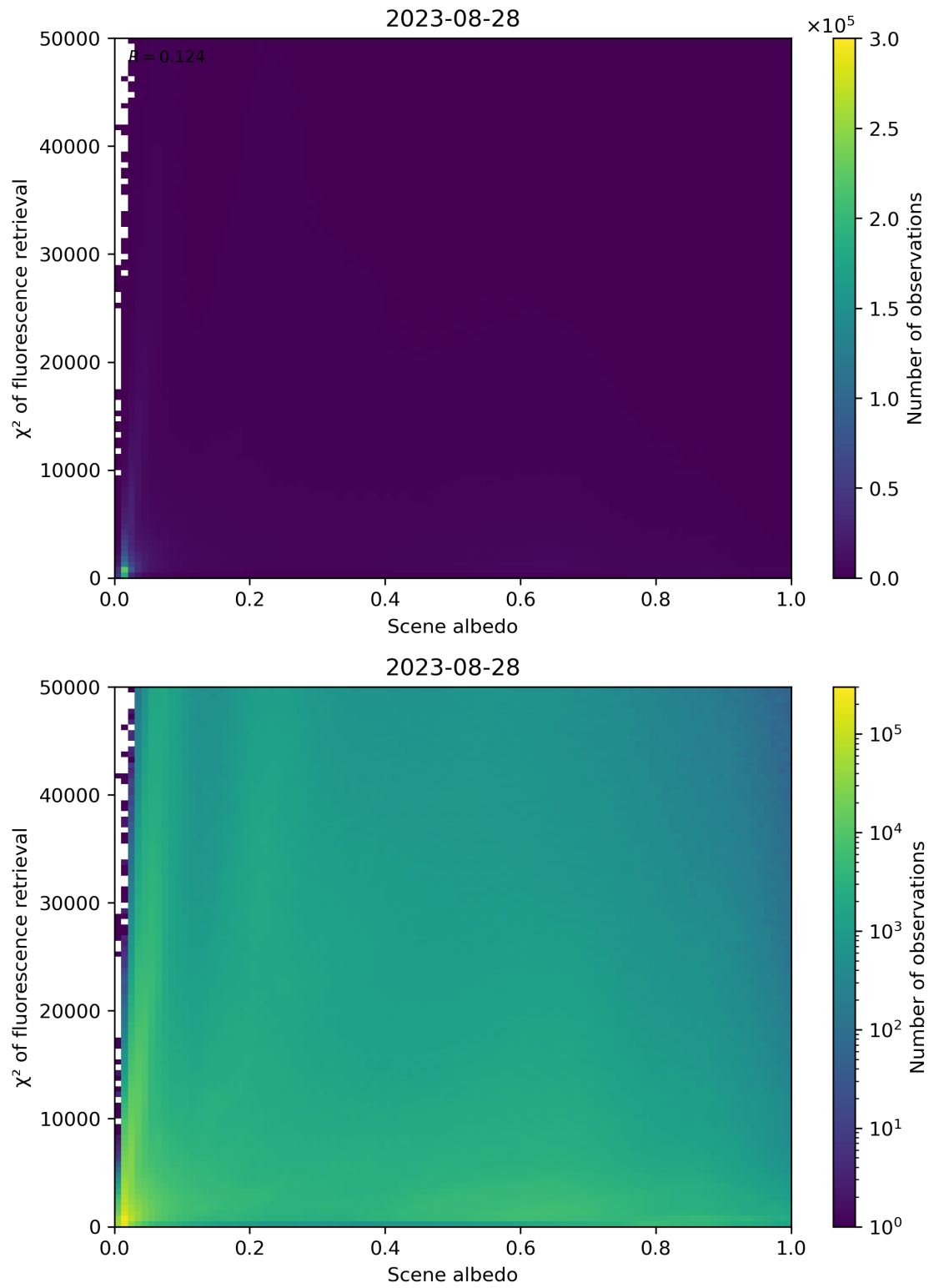
Figure 113: Scatter density plot of “Scene albedo” against “ \chi^2 of fluorescence retrieval” for 2023-08-27 to 2023-08-29.
