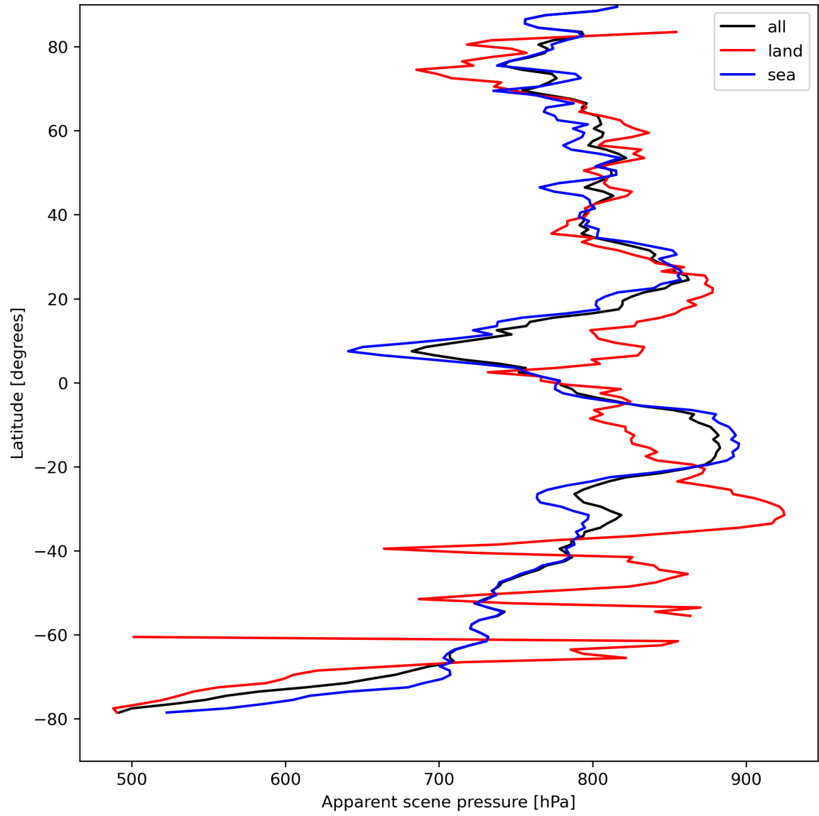
Figure 19: Zonal average of “Apparent scene pressure” for 2023-08-27 to 2023-08-29.
