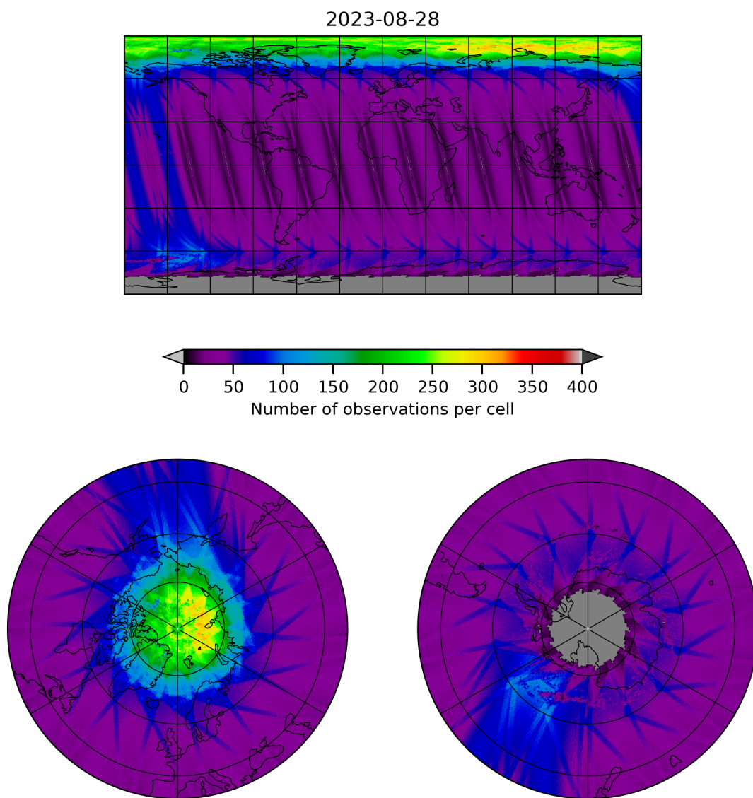
Figure 11: Map of the number of observations for 2023-08-27 to 2023-08-29
