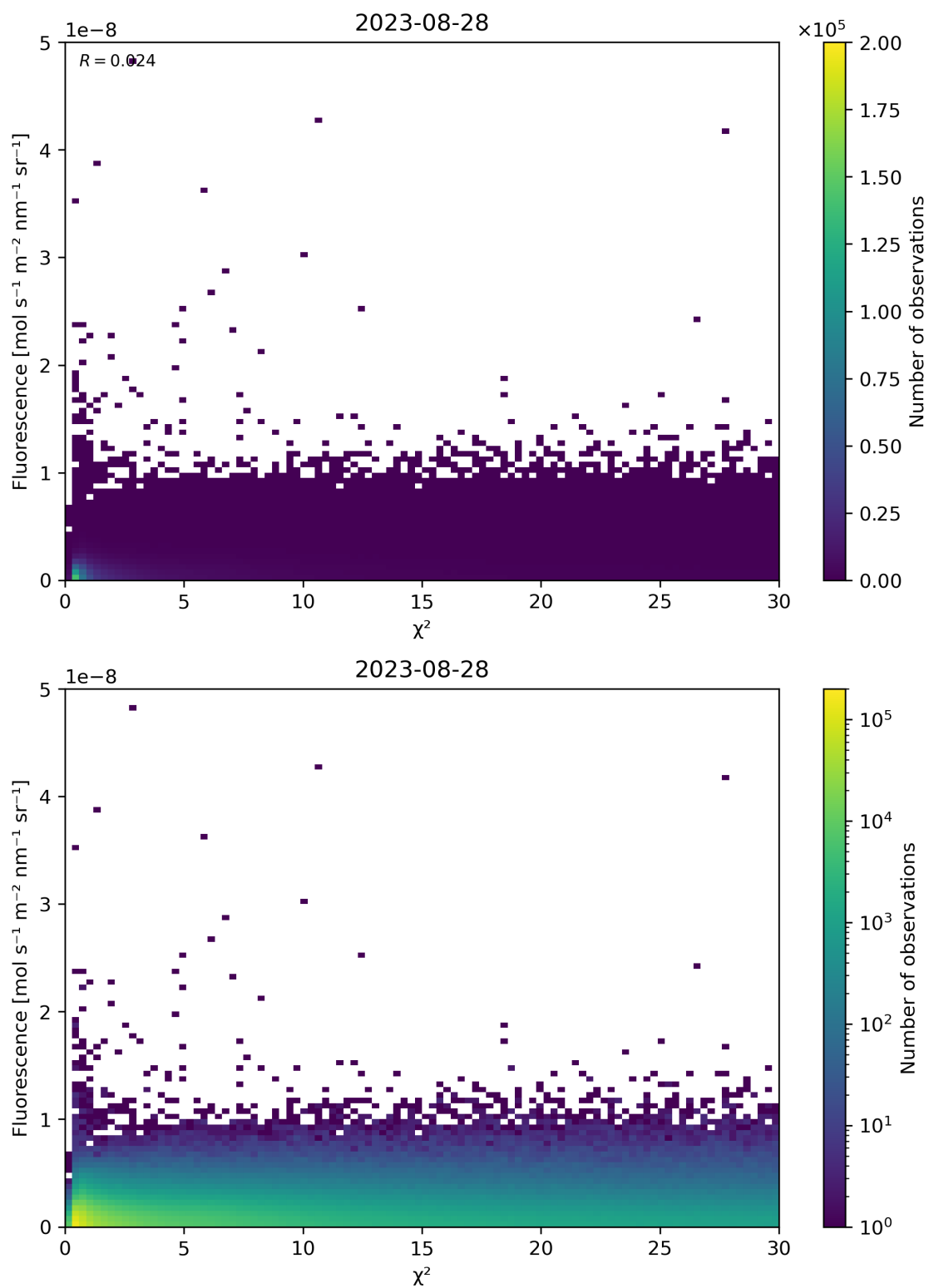
Figure 70: Scatter density plot of “ \chi^2 ” against “Fluorescence” for 2023-08-27 to 2023-08-29.
