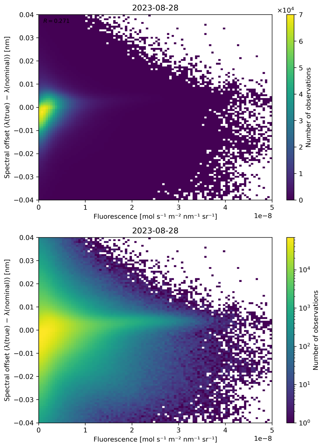
Figure 95: Scatter density plot of “Fluorescence” against “Spectral offset ( \lambda(\text{true}) - \lambda(\text{nominal}) )” for 2023-08-27 to 2023-08-29.
