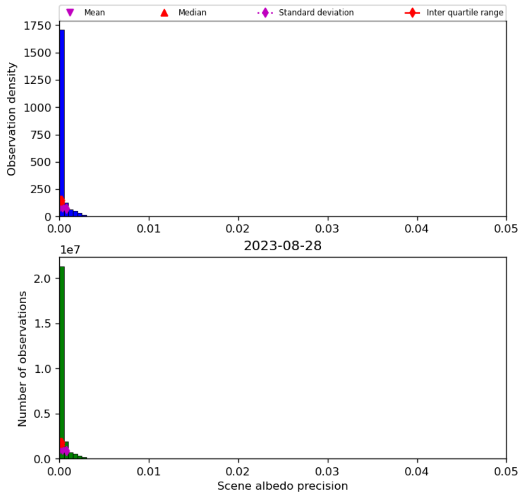
Figure 35: Histogram of “Scene albedo precision” for 2023-08-27 to 2023-08-29
