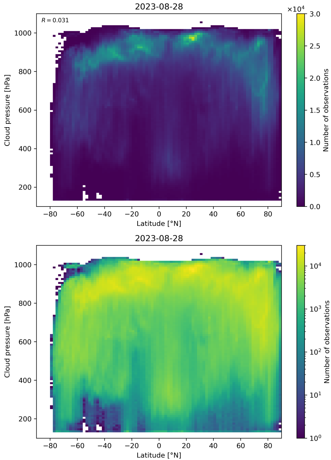
Figure 100: Scatter density plot of “Latitude” against “Cloud pressure” for 2023-08-27 to 2023-08-29.
