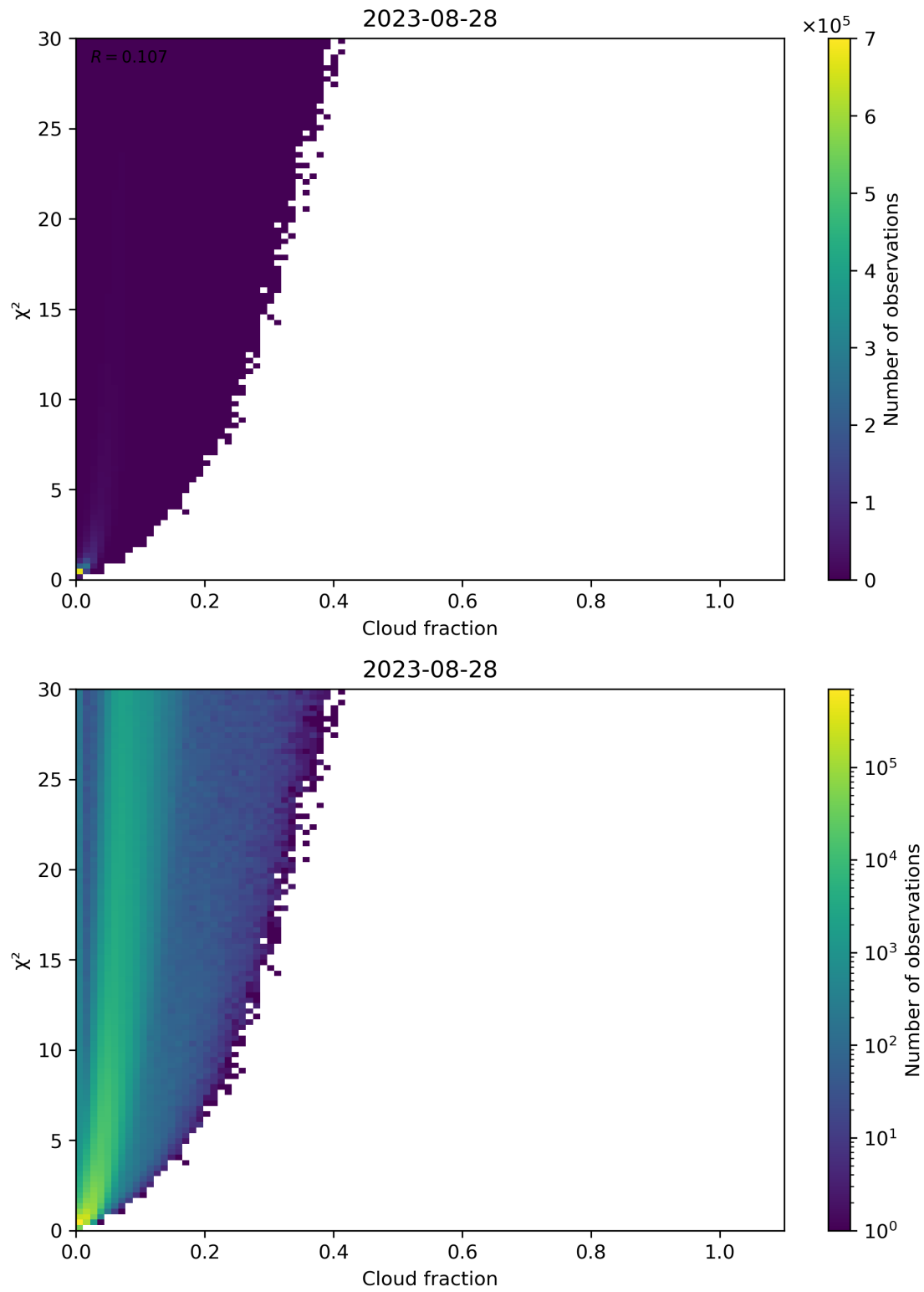
Figure 77: Scatter density plot of “Cloud fraction” against “ \chi^2 ” for 2023-08-27 to 2023-08-29.
