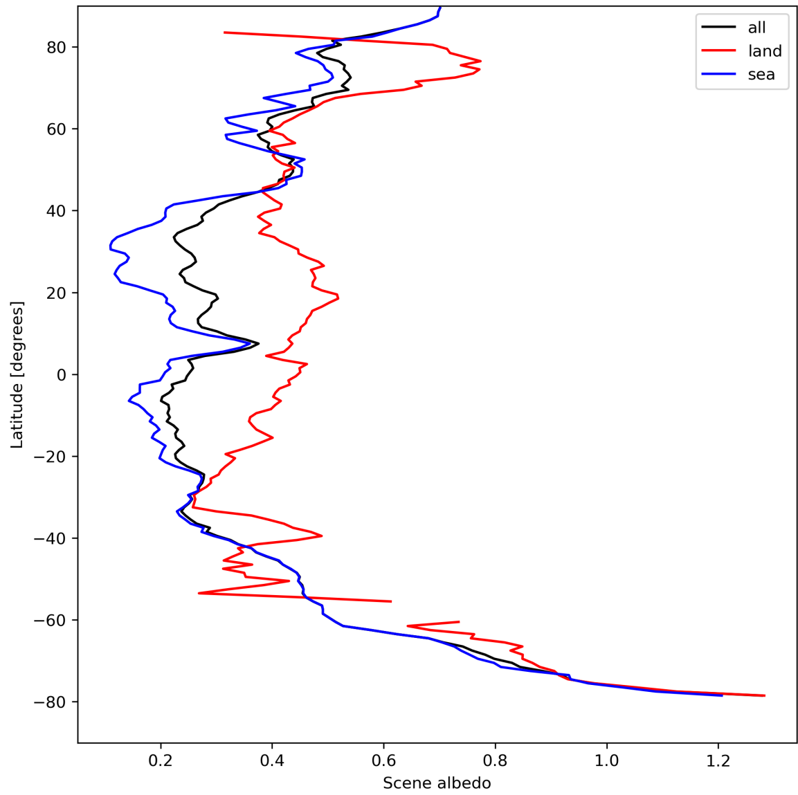
Figure 17: Zonal average of “Scene albedo” for 2023-08-27 to 2023-08-29.
