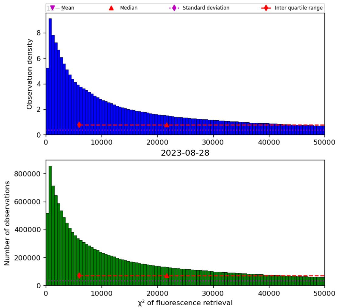
Figure 42: Histogram of “ \chi^2 of fluorescence retrieval” for 2023-08-27 to 2023-08-29
