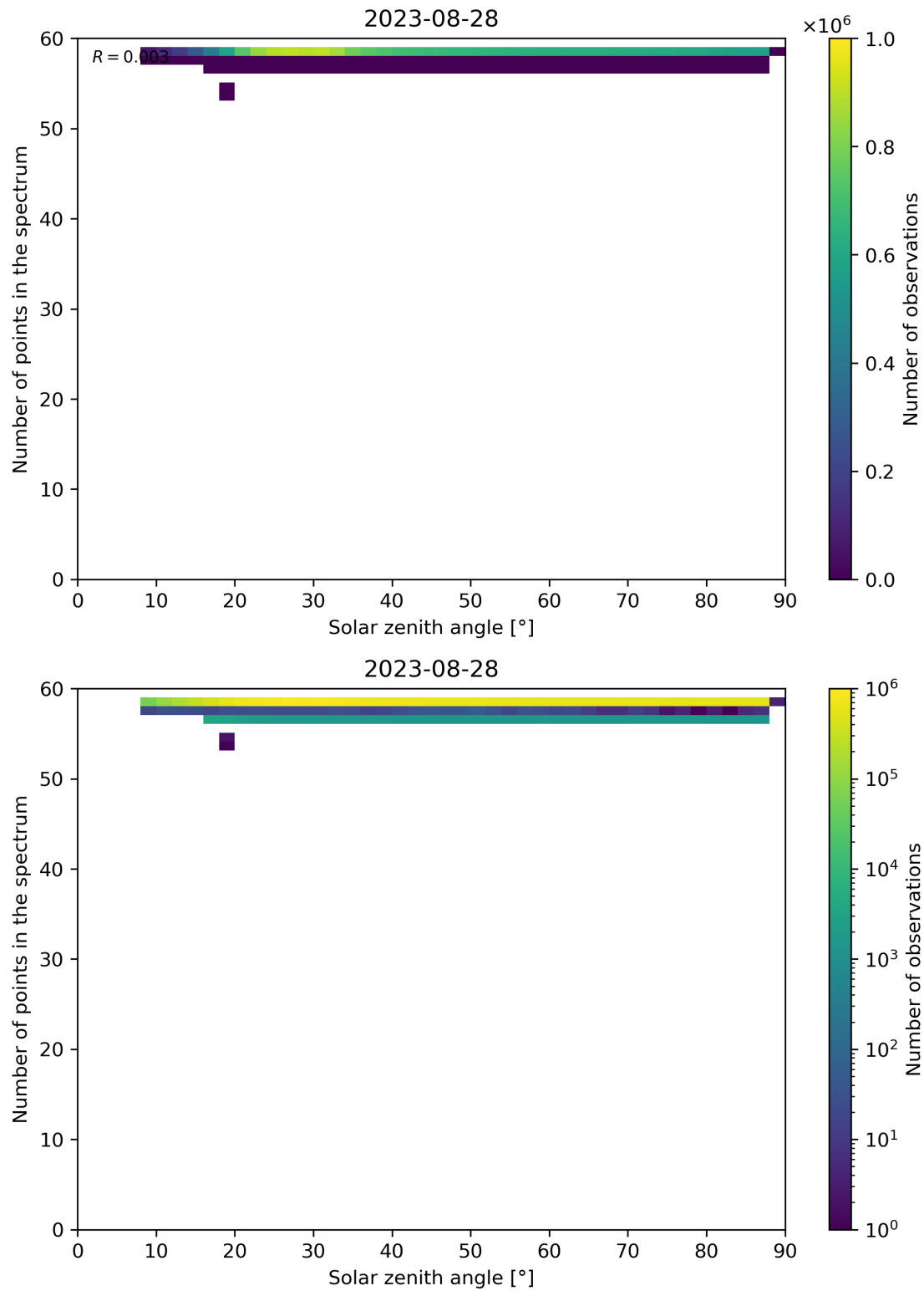
Figure 126: Scatter density plot of “Solar zenith angle” against “Number of points in the spectrum” for 2023-08-27 to 2023-08-29.
