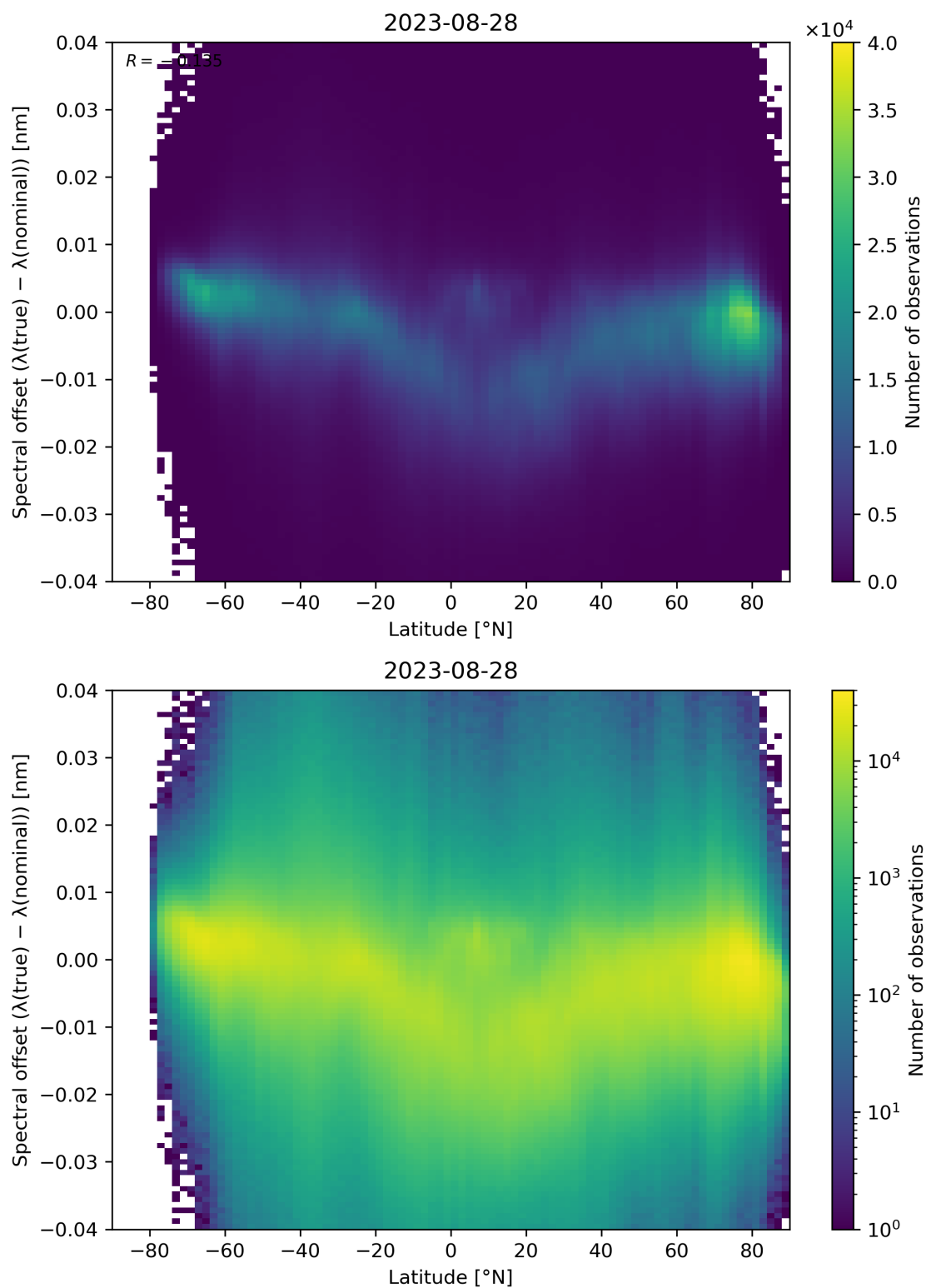
Figure 105: Scatter density plot of “Latitude” against “Spectral offset ( \lambda(\text{true}) - \lambda(\text{nominal}) )” for 2023-08-27 to 2023-08-29.
