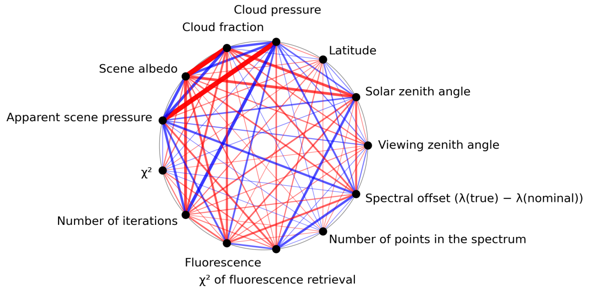
Figure 1: Map of correlation graph for 2023-08-27 to 2023-08-29.
