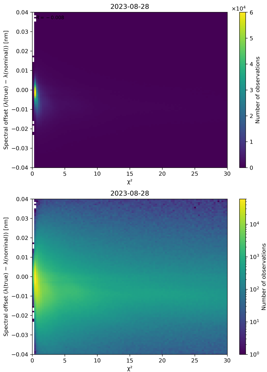
Figure 75: Scatter density plot of “ \chi^2 ” against “Spectral offset ( \lambda(\text{true}) - \lambda(\text{nominal}) )” for 2023-08-27 to 2023-08-29.
