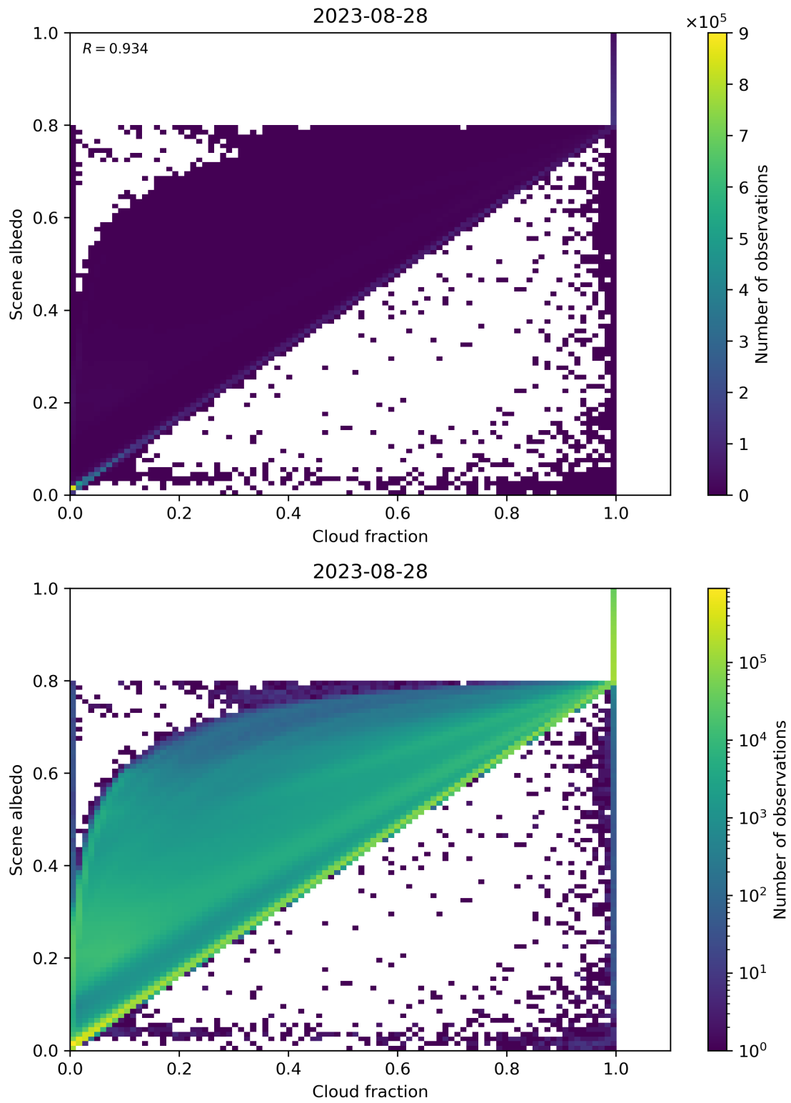
Figure 82: Scatter density plot of “Cloud fraction” against “Scene albedo” for 2023-08-27 to 2023-08-29.
