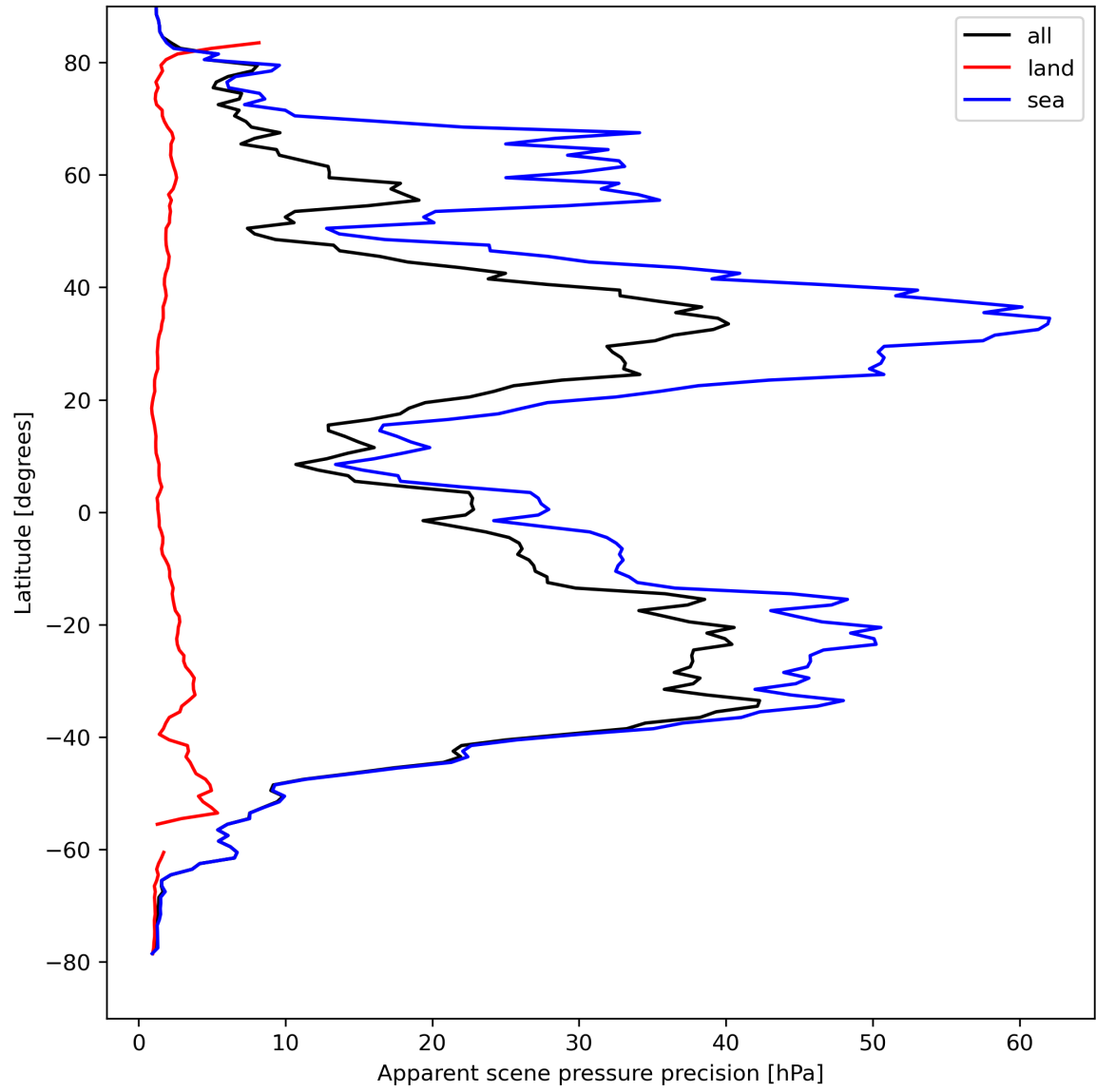
Figure 20: Zonal average of “Apparent scene pressure precision” for 2023-08-27 to 2023-08-29.
