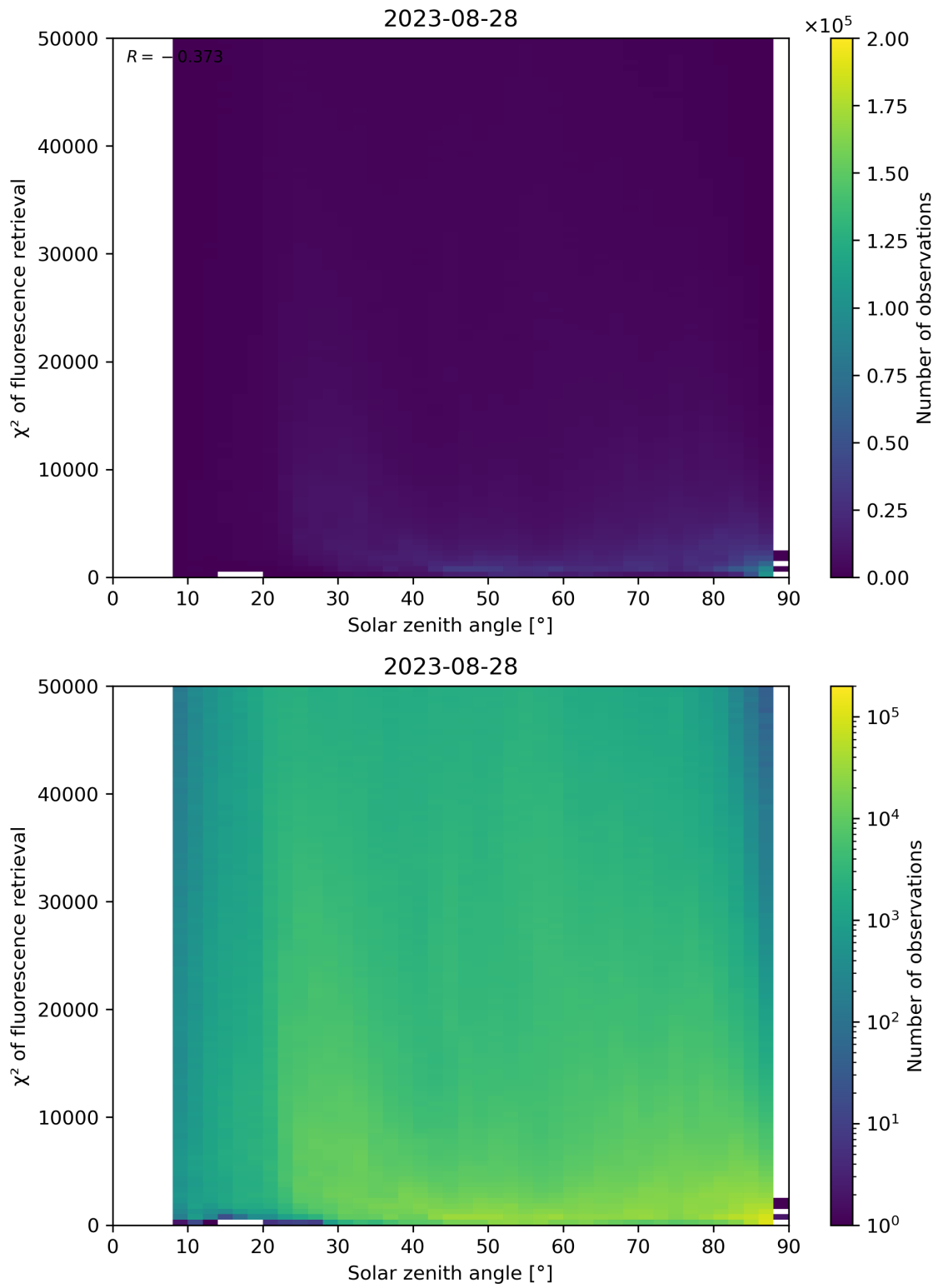
Figure 120: Scatter density plot of “Solar zenith angle” against “ \chi^2 of fluorescence retrieval” for 2023-08-27 to 2023-08-29.
