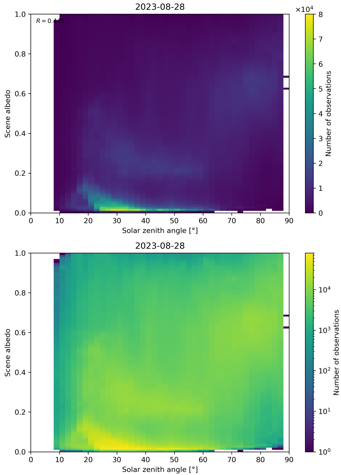
Figure 127: Scatter density plot of “Solar zenith angle” against “Scene albedo” for 2023-08-27 to 2023-08-29.
