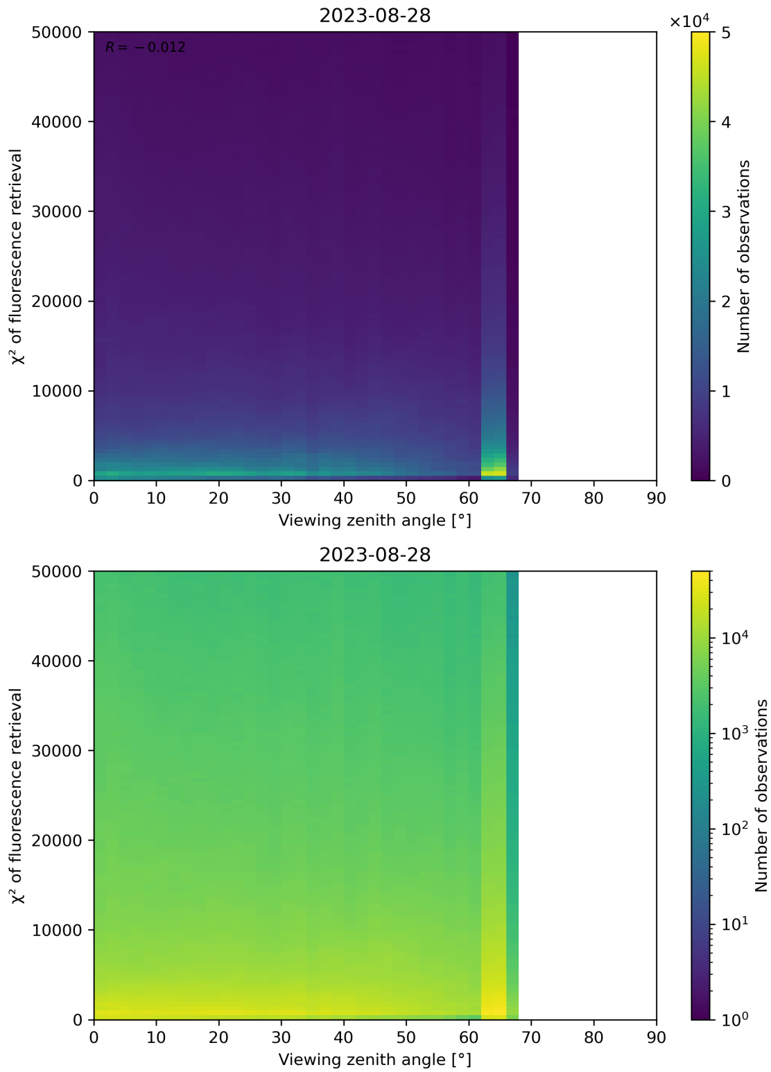
Figure 131: Scatter density plot of “Viewing zenith angle” against “ \chi^2 of fluorescence retrieval” for 2023-08-27 to 2023-08-29.
