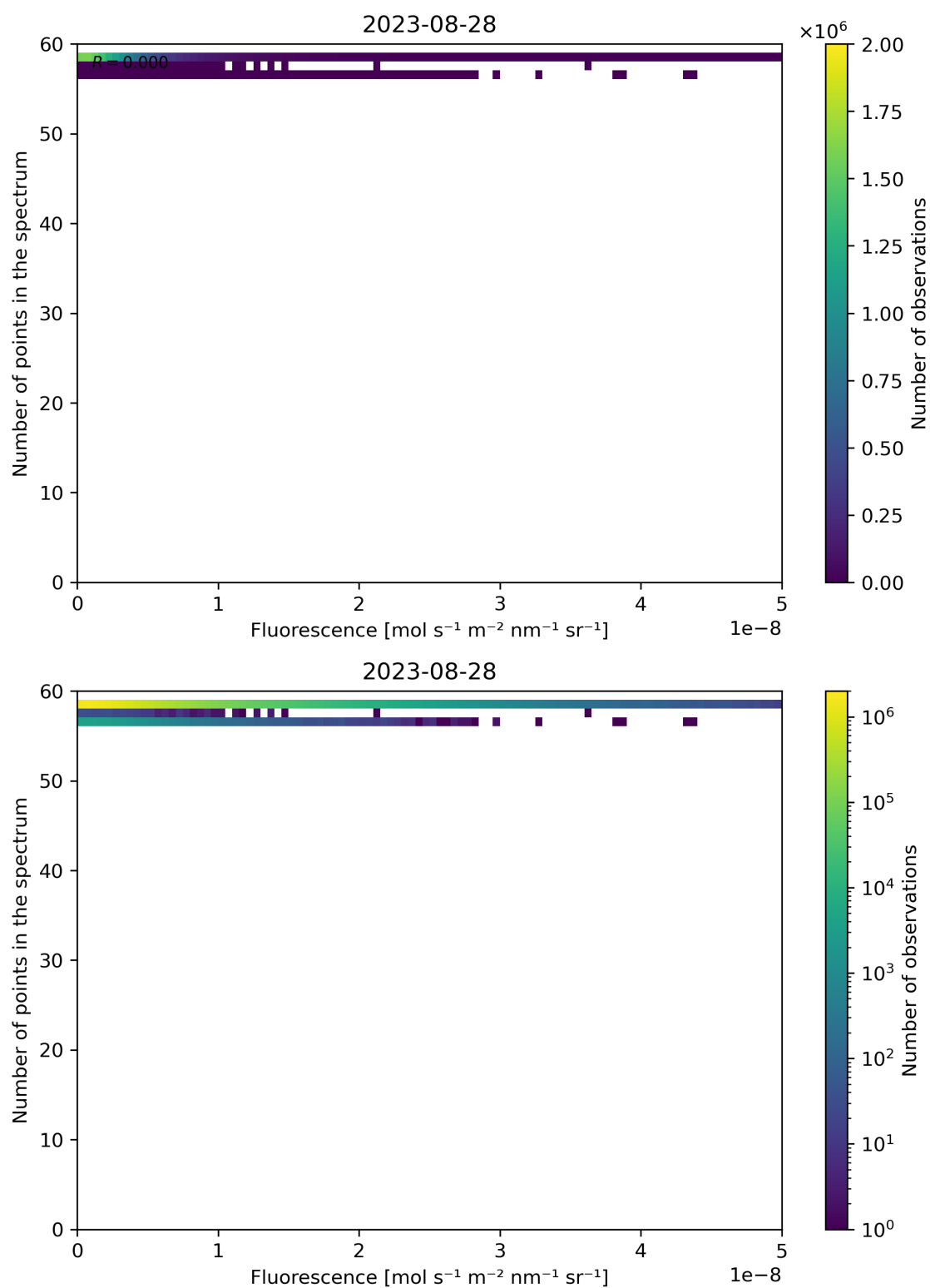
Figure 94: Scatter density plot of “Fluorescence” against “Number of points in the spectrum” for 2023-08-27 to 2023-08-29.
