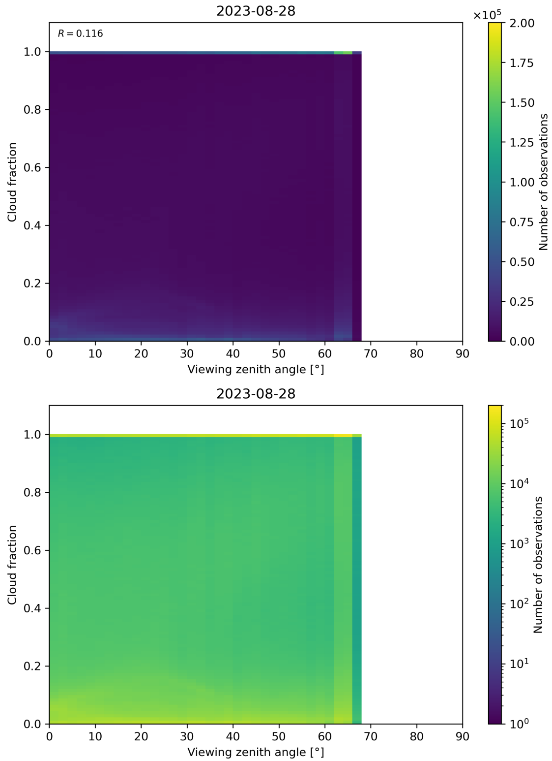
Figure 132: Scatter density plot of “Viewing zenith angle” against “Cloud fraction” for 2023-08-27 to 2023-08-29.
