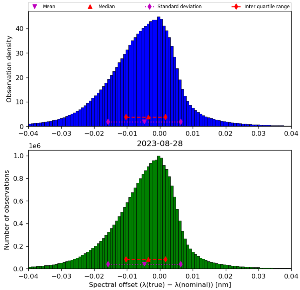
Figure 45: Histogram of “Spectral offset ( \lambda(\text{true}) - \lambda(\text{nominal}) )” for 2023-08-27 to 2023-08-29
