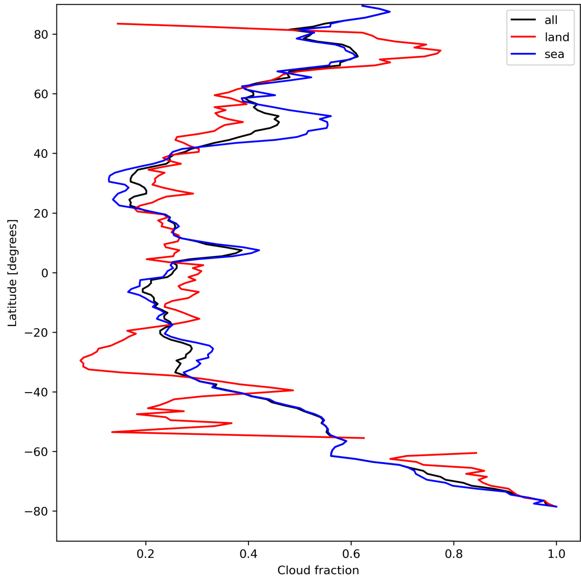
Figure 15: Zonal average of “Cloud fraction” for 2023-08-27 to 2023-08-29.
