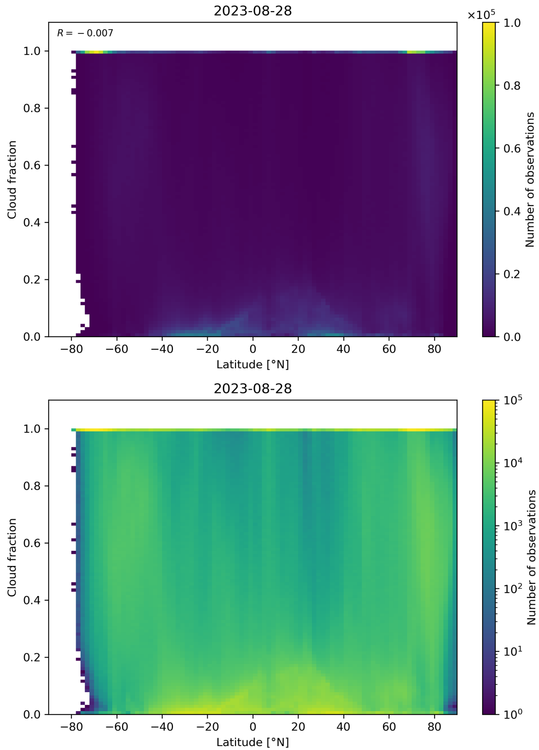
Figure 99: Scatter density plot of “Latitude” against “Cloud fraction” for 2023-08-27 to 2023-08-29.
