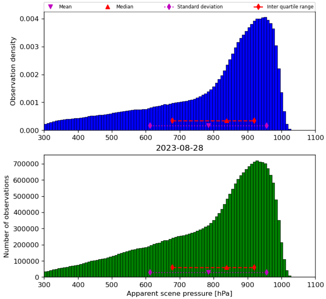
Figure 36: Histogram of “Apparent scene pressure” for 2023-08-27 to 2023-08-29
