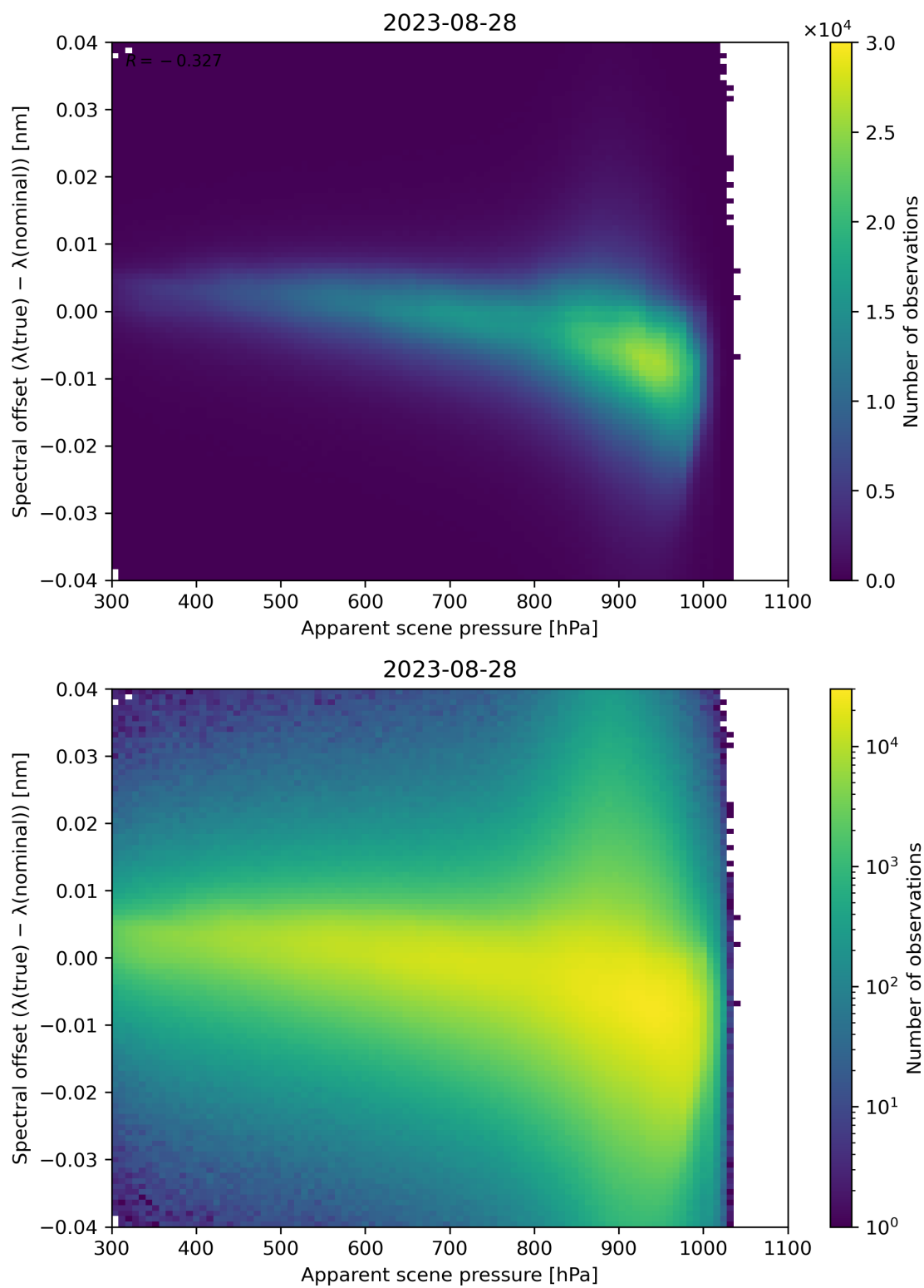
Figure 68: Scatter density plot of “Apparent scene pressure” against “Spectral offset ( \lambda(\text{true}) - \lambda(\text{nominal}) )” for 2023-08-27 to 2023-08-29.
