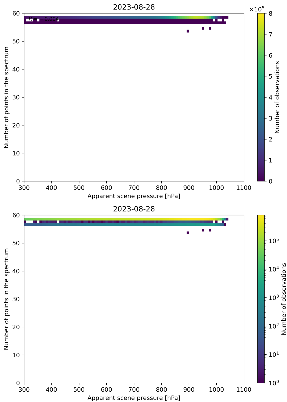
Figure 67: Scatter density plot of “Apparent scene pressure” against “Number of points in the spectrum” for 2023-08-27 to 2023-08-29.
