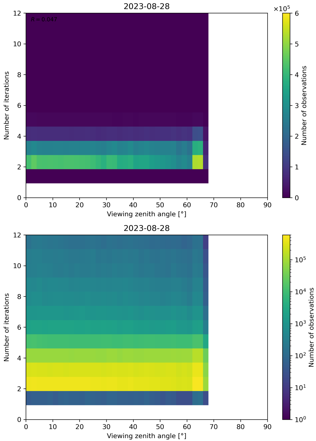
Figure 136: Scatter density plot of “Viewing zenith angle” against “Number of iterations” for 2023-08-27 to 2023-08-29.
