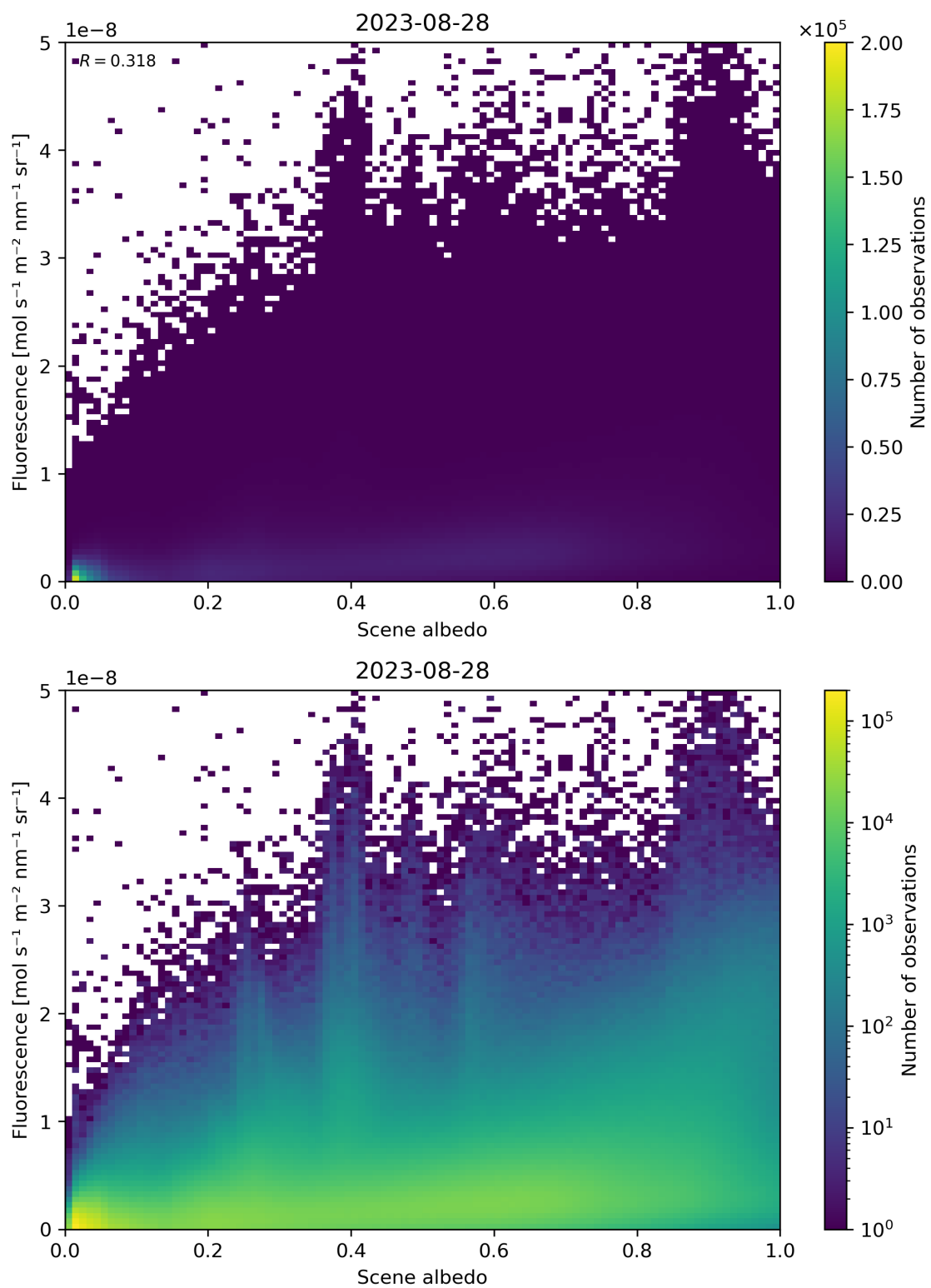
Figure 114: Scatter density plot of “Scene albedo” against “Fluorescence” for 2023-08-27 to 2023-08-29.
