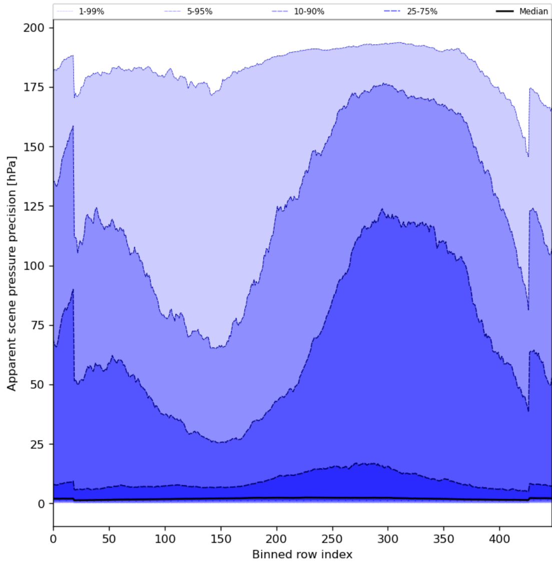
Figure 54: Along track statistics of “Apparent scene pressure precision” for 2023-08-27 to 2023-08-29
