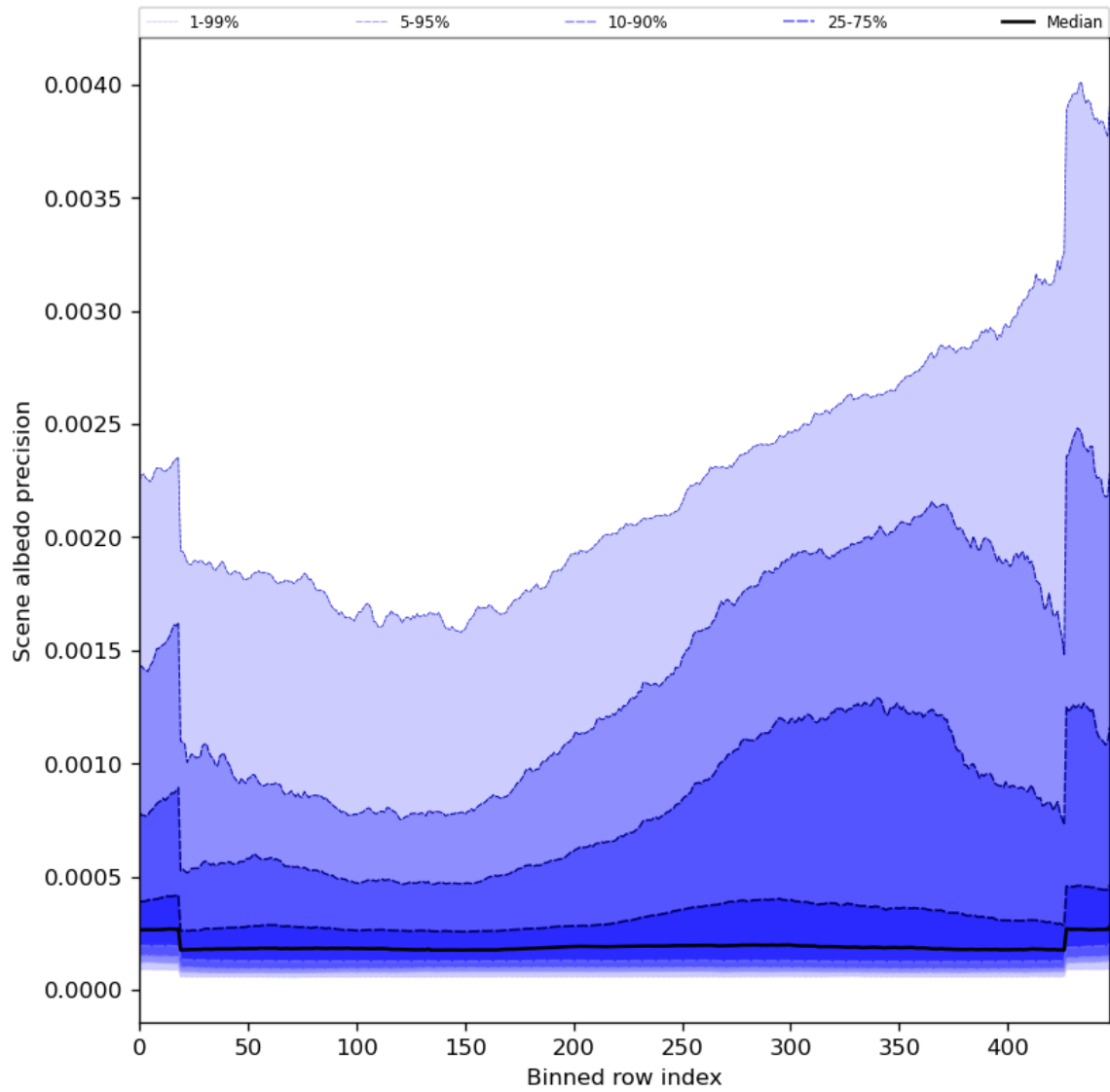
Figure 52: Along track statistics of “Scene albedo precision” for 2023-08-27 to 2023-08-29
