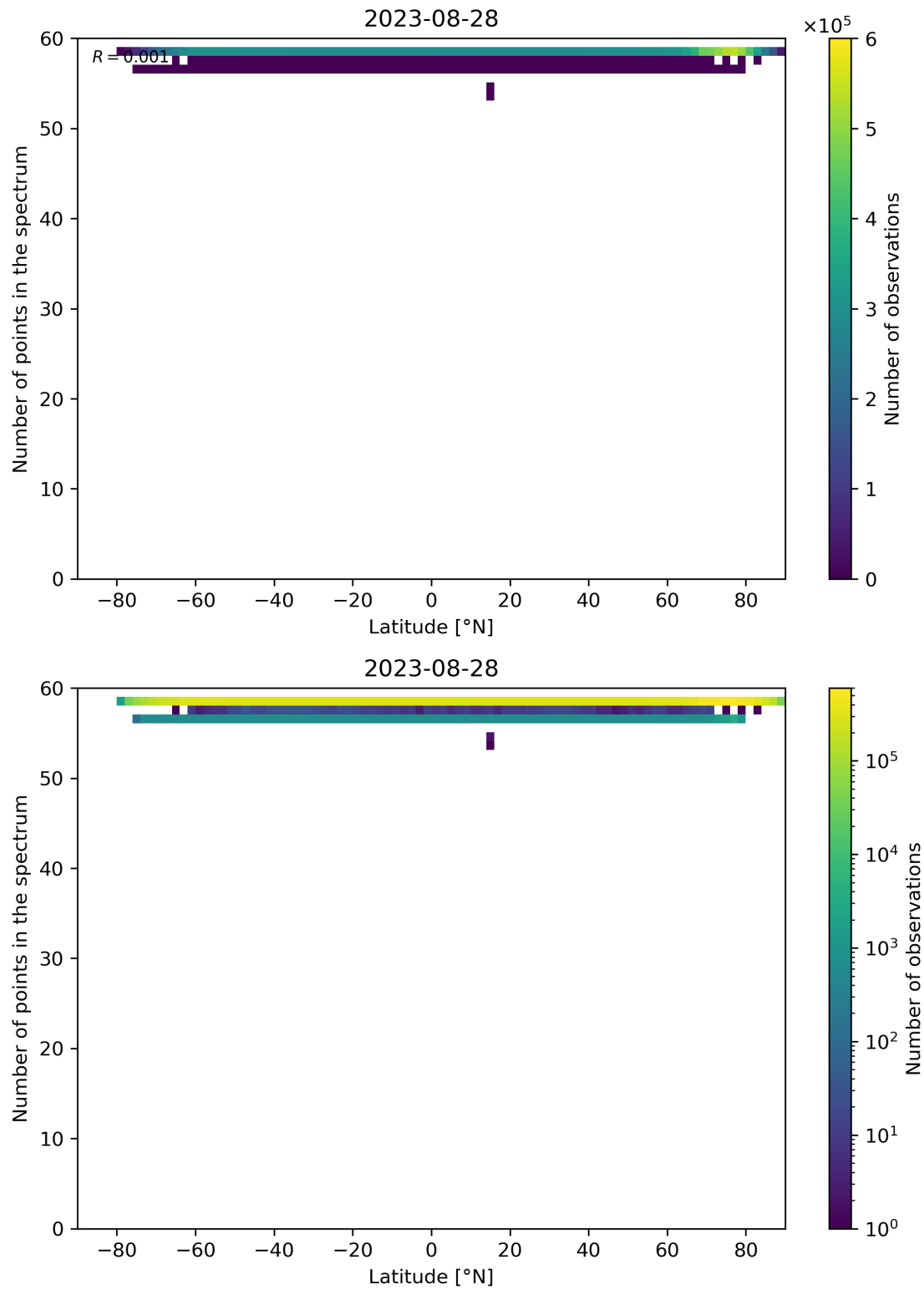
Figure 103: Scatter density plot of “Latitude” against “Number of points in the spectrum” for 2023-08-27 to 2023-08-29.
