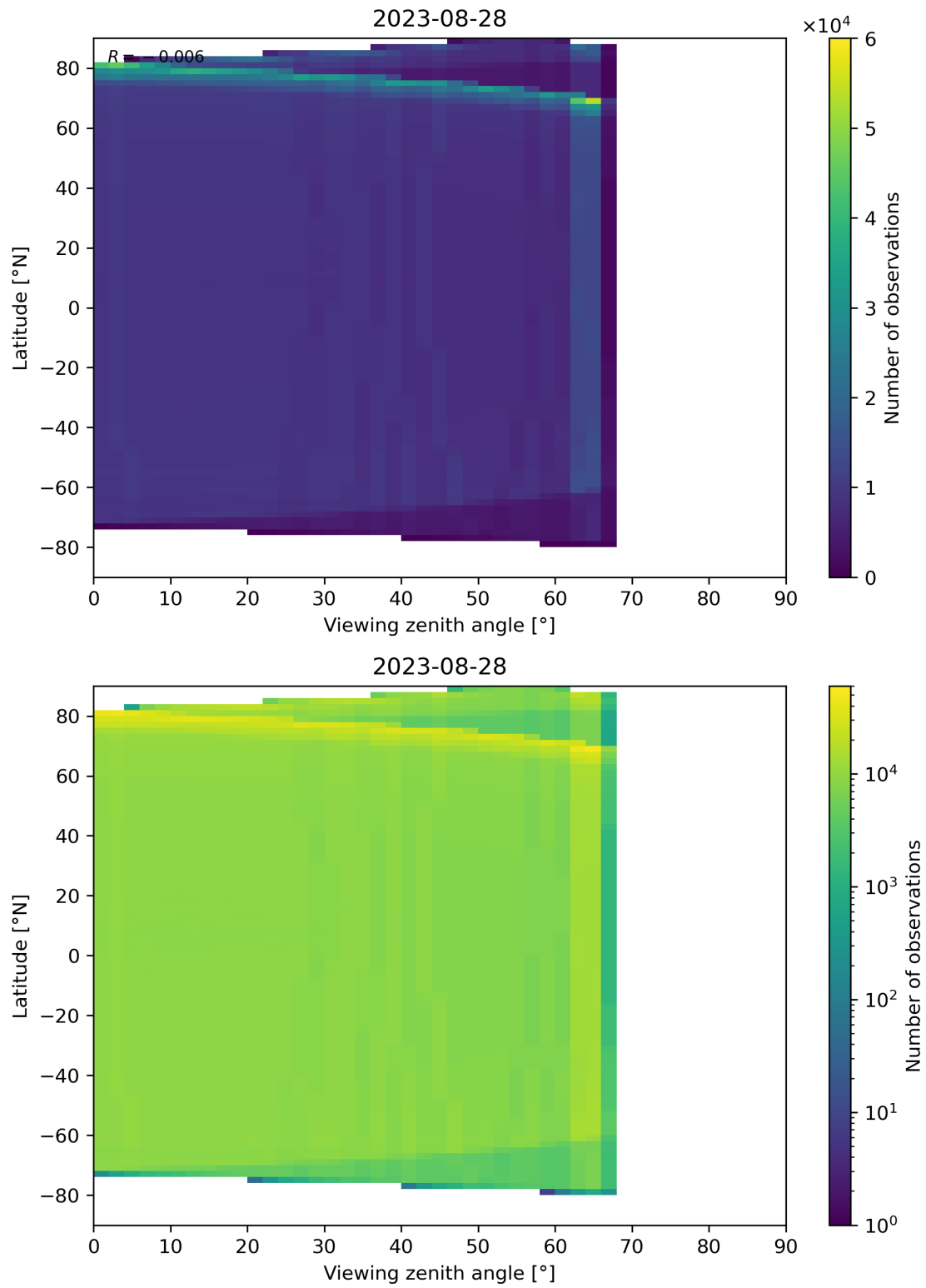
Figure 135: Scatter density plot of “Viewing zenith angle” against “Latitude” for 2023-08-27 to 2023-08-29.
