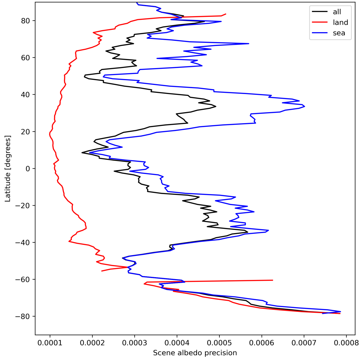
Figure 18: Zonal average of “Scene albedo precision” for 2023-08-27 to 2023-08-29.
