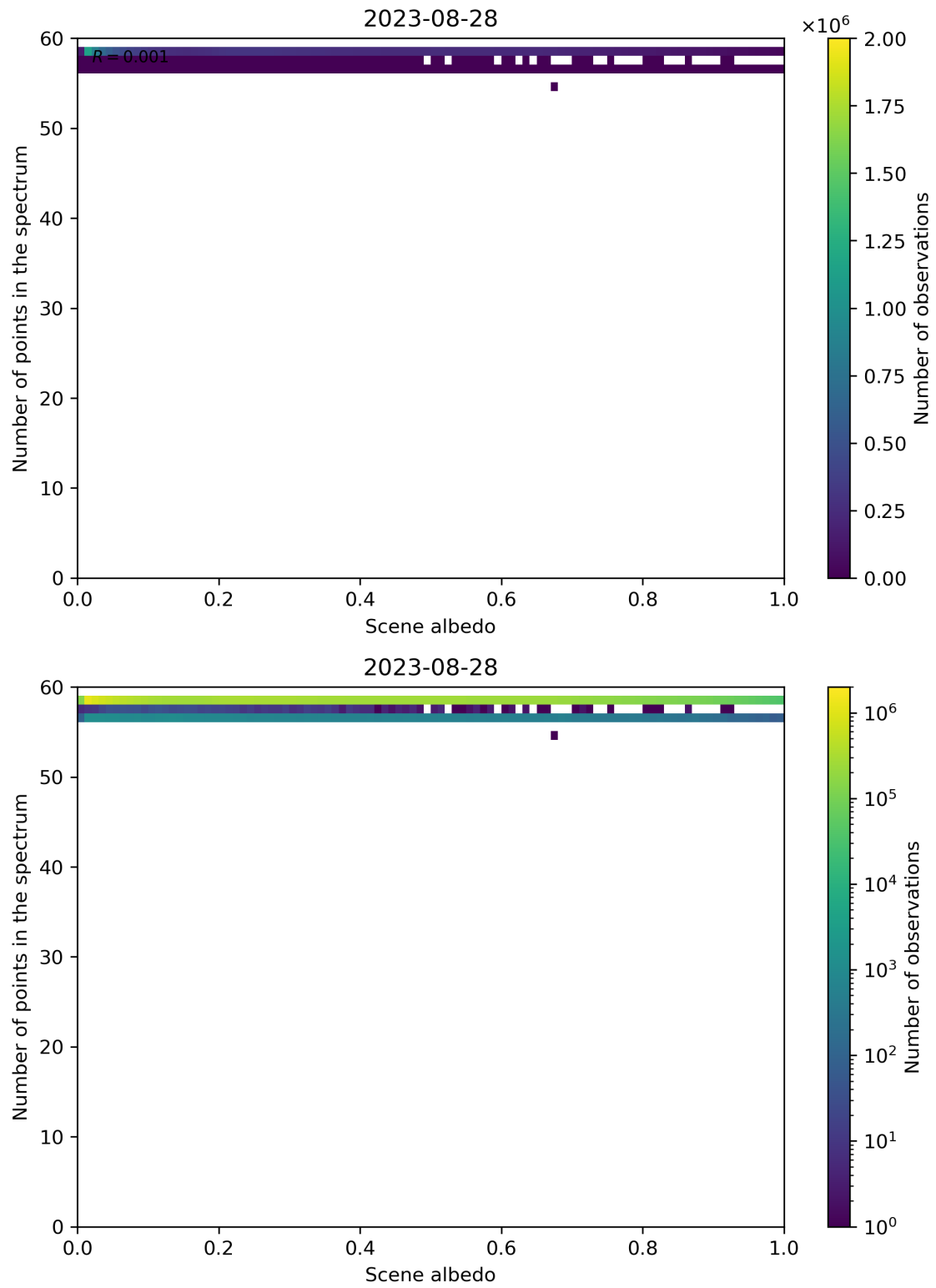
Figure 116: Scatter density plot of “Scene albedo” against “Number of points in the spectrum” for 2023-08-27 to 2023-08-29.
