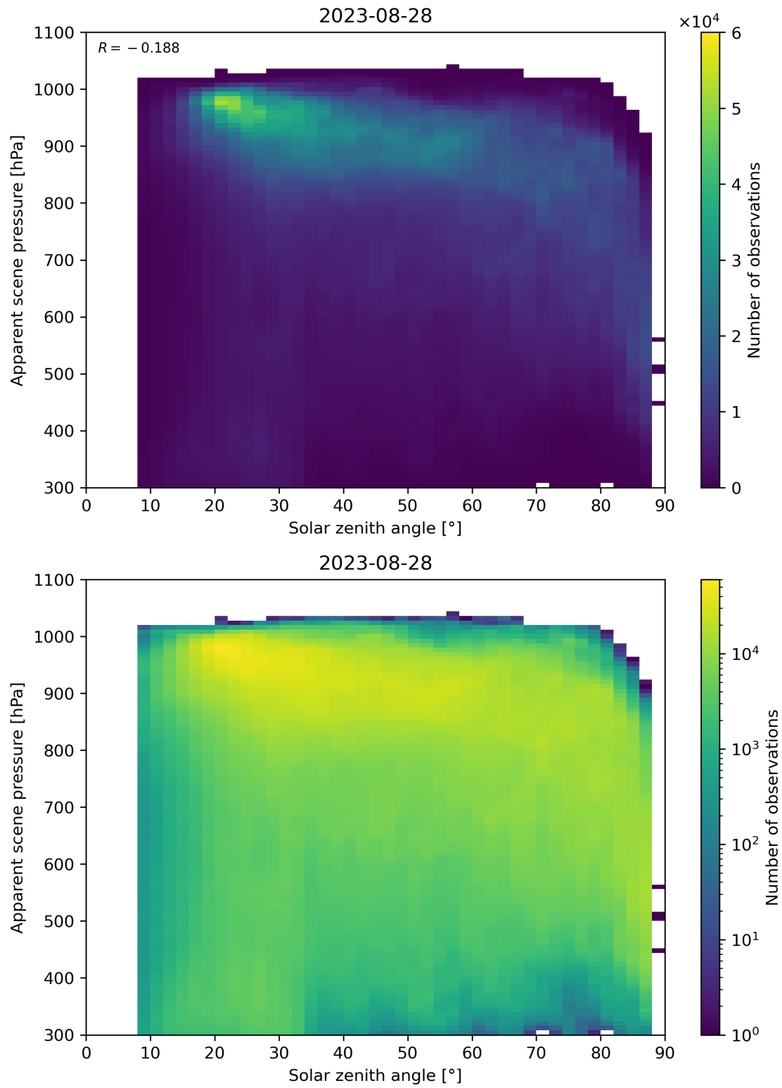
Figure 118: Scatter density plot of “Solar zenith angle” against “Apparent scene pressure” for 2023-08-27 to 2023-08-29.
