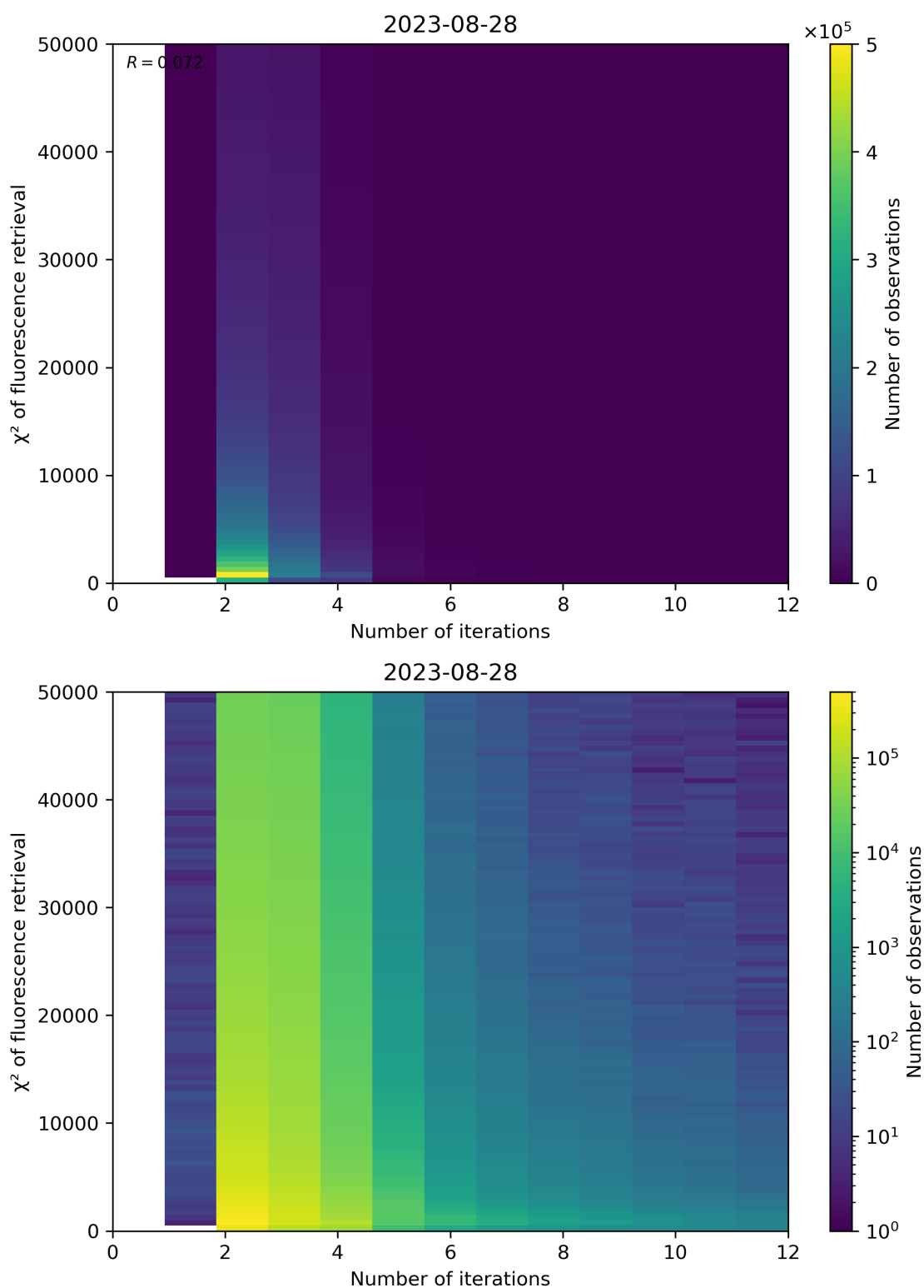
Figure 106: Scatter density plot of “Number of iterations” against “ \chi^2 of fluorescence retrieval” for 2023-08-27 to 2023-08-29.
