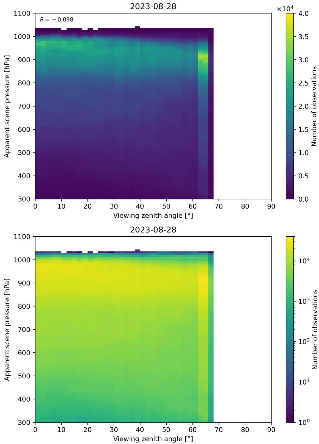
Figure 129: Scatter density plot of “Viewing zenith angle” against “Apparent scene pressure” for 2023-08-27 to 2023-08-29.
