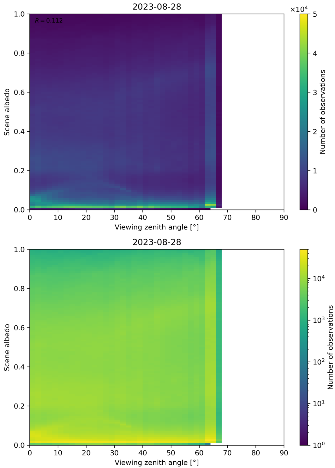
Figure 138: Scatter density plot of “Viewing zenith angle” against “Scene albedo” for 2023-08-27 to 2023-08-29.
