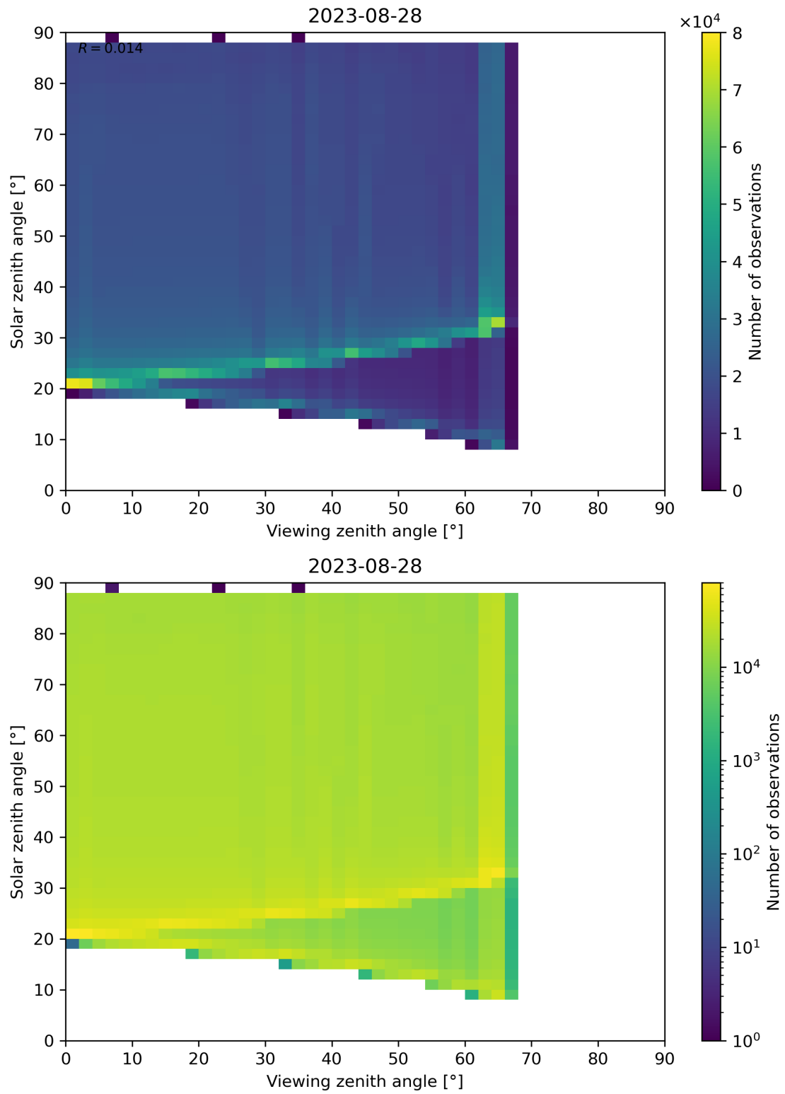
Figure 139: Scatter density plot of “Viewing zenith angle” against “Solar zenith angle” for 2023-08-27 to 2023-08-29.
