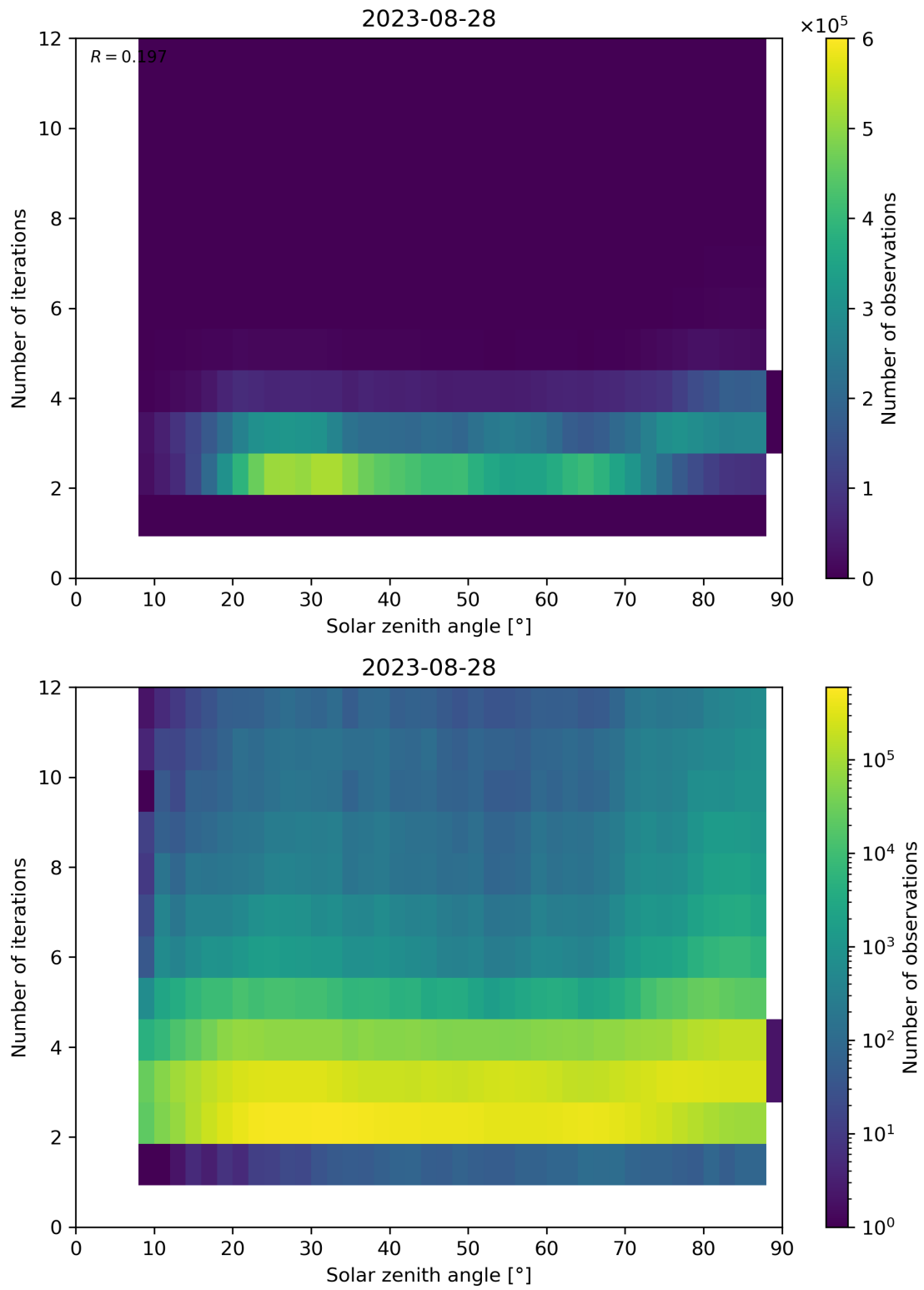
Figure 125: Scatter density plot of “Solar zenith angle” against “Number of iterations” for 2023-08-27 to 2023-08-29.
