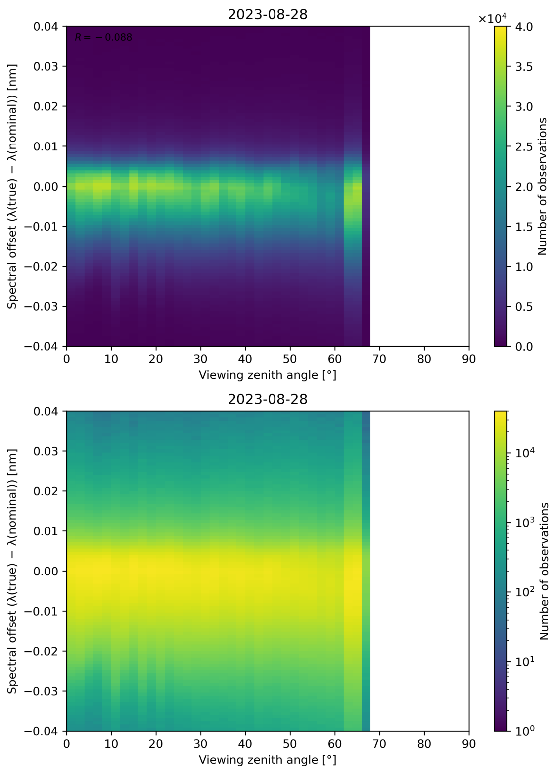
Figure 140: Scatter density plot of “Viewing zenith angle” against “Spectral offset ( \lambda(\text{true}) - \lambda(\text{nominal}) )” for 2023-08-27 to 2023-08-29.
