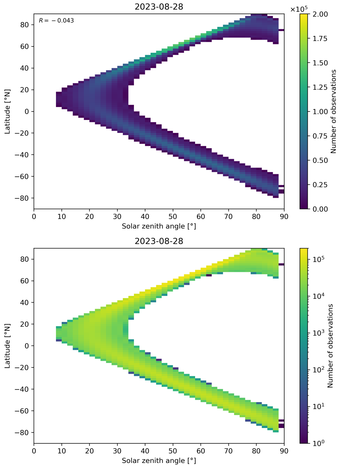
Figure 124: Scatter density plot of “Solar zenith angle” against “Latitude” for 2023-08-27 to 2023-08-29.
