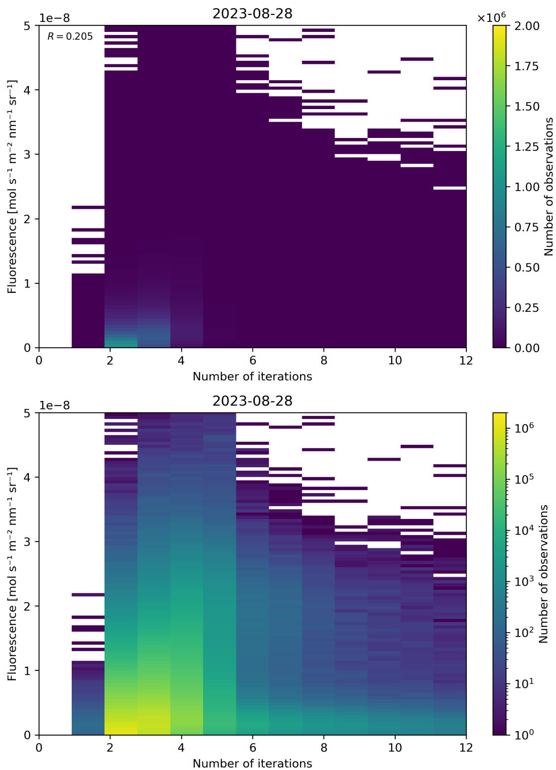
Figure 107: Scatter density plot of “Number of iterations” against “Fluorescence” for 2023-08-27 to 2023-08-29.
