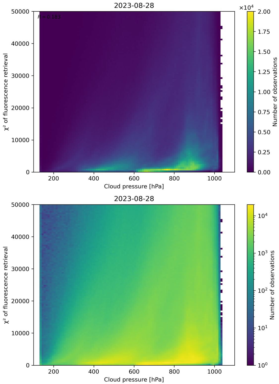
Figure 86: Scatter density plot of “Cloud pressure” against “ \chi^2 of fluorescence retrieval” for 2023-08-27 to 2023-08-29.
