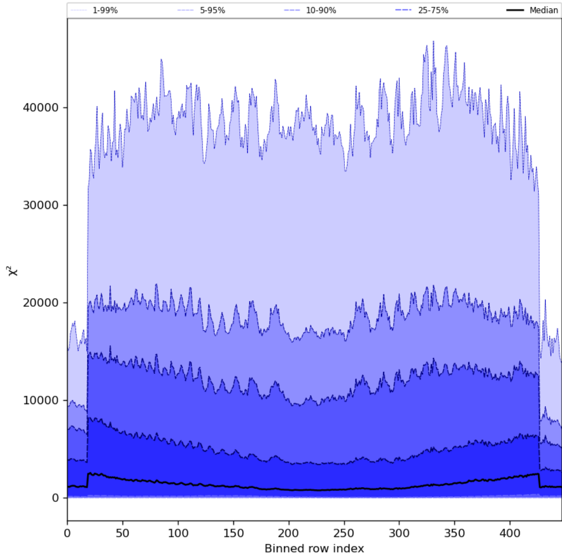
Figure 55: Along track statistics of “ \chi^2 ” for 2023-08-27 to 2023-08-29
