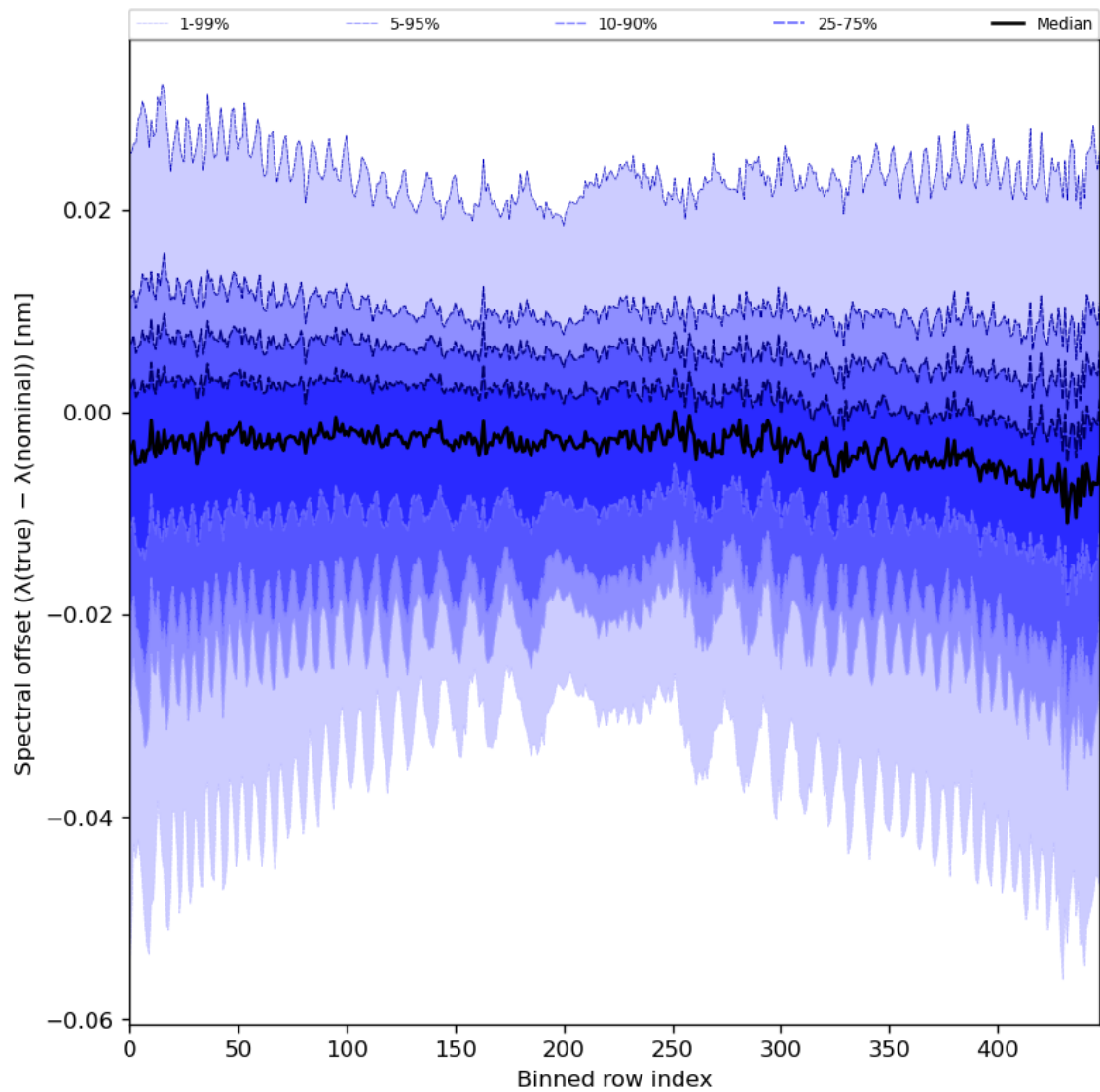
Figure 62: Along track statistics of “Spectral offset ( \lambda(\text{true}) - \lambda(\text{nominal}) )” for 2023-08-27 to 2023-08-29
