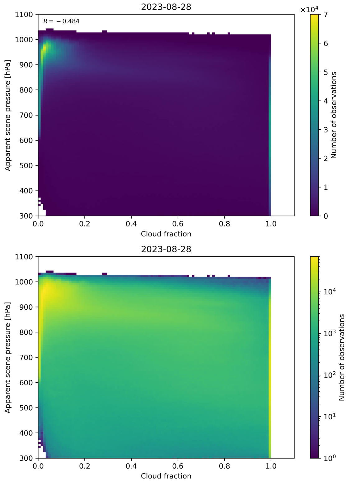
Figure 76: Scatter density plot of “Cloud fraction” against “Apparent scene pressure” for 2023-08-27 to 2023-08-29.
