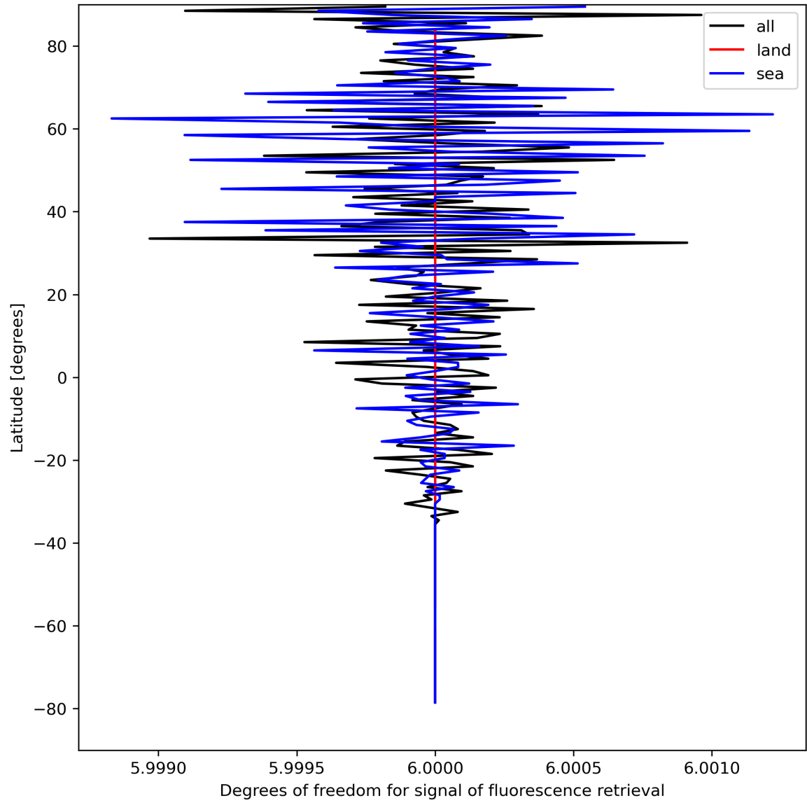
Figure 26: Zonal average of “Degrees of freedom for signal of fluorescence retrieval” for 2023-08-27 to 2023-08-29.
