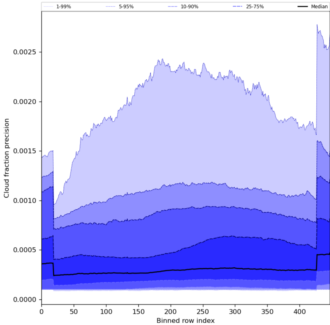
Figure 50: Along track statistics of “Cloud fraction precision” for 2023-08-27 to 2023-08-29
