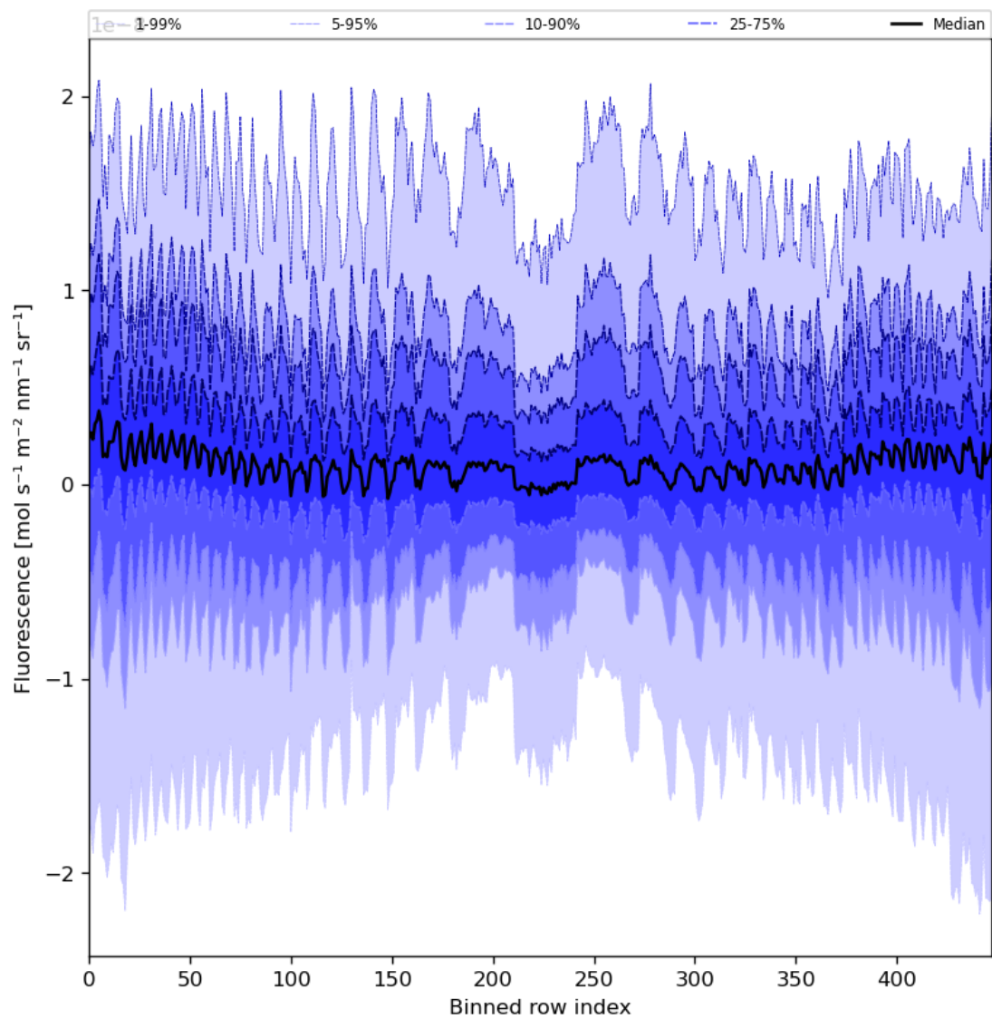
Figure 57: Along track statistics of “Fluorescence” for 2023-08-27 to 2023-08-29
