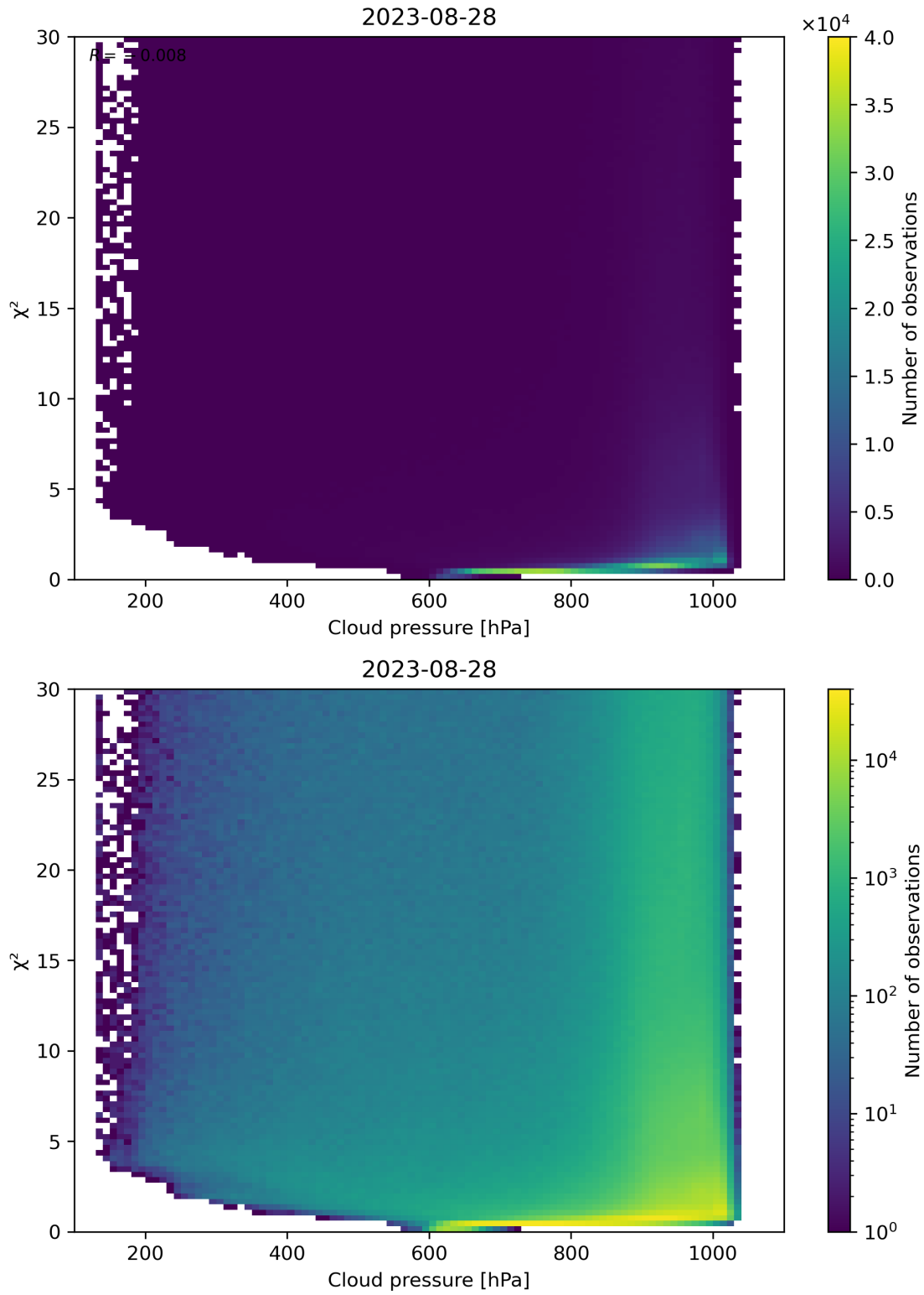
Figure 85: Scatter density plot of “Cloud pressure” against “ \chi^2 ” for 2023-08-27 to 2023-08-29.
