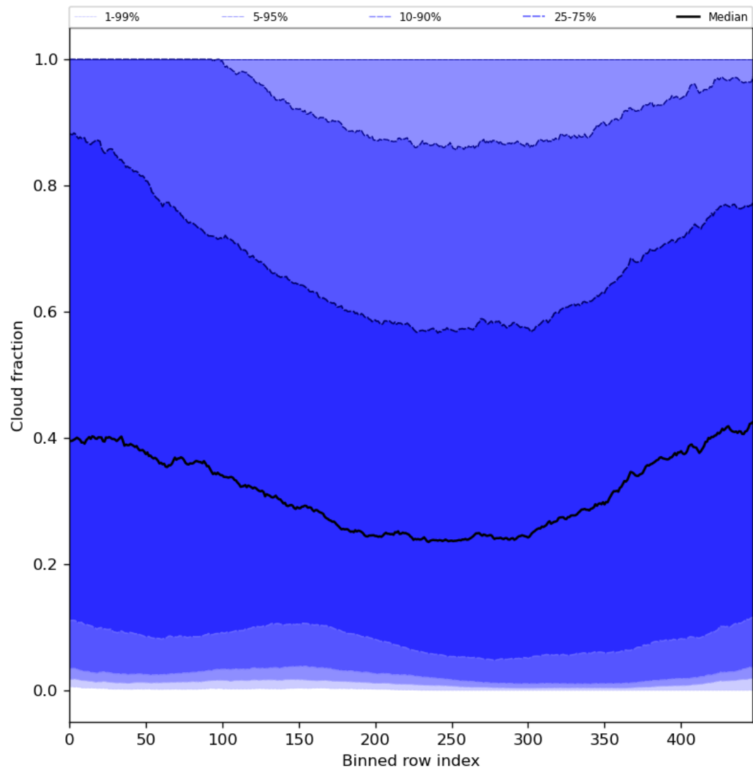
Figure 49: Along track statistics of “Cloud fraction” for 2023-08-27 to 2023-08-29
