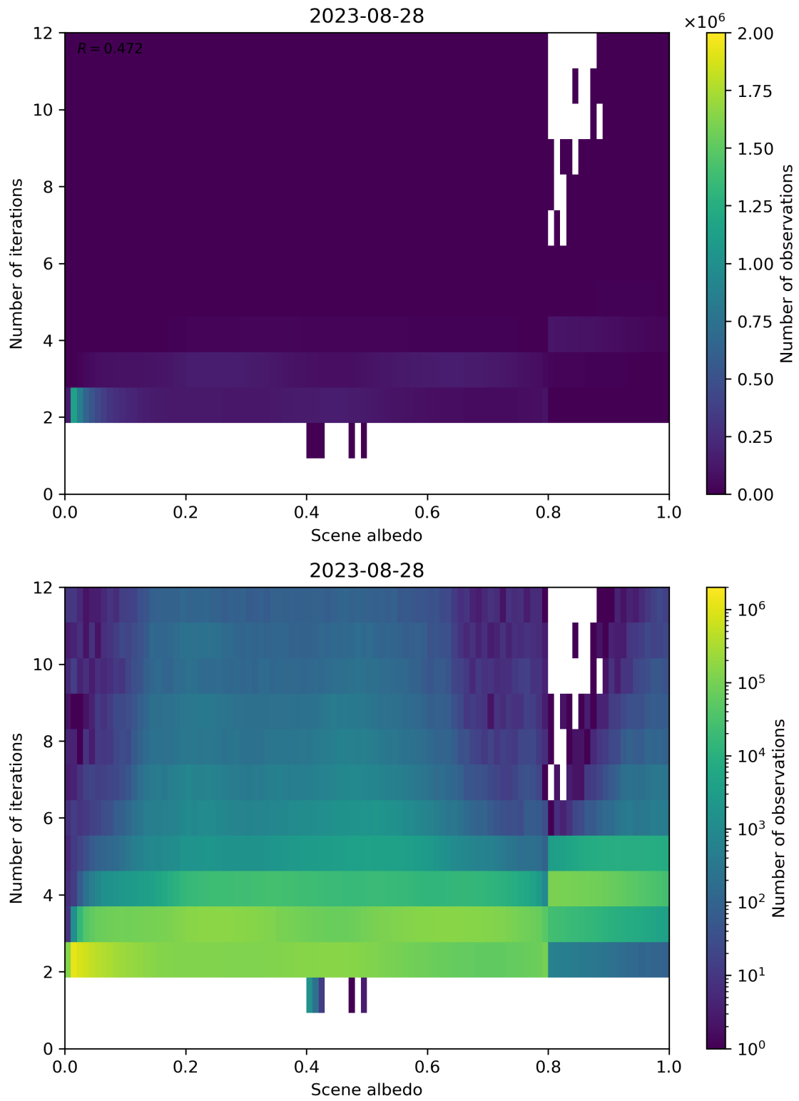
Figure 115: Scatter density plot of “Scene albedo” against “Number of iterations” for 2023-08-27 to 2023-08-29.
