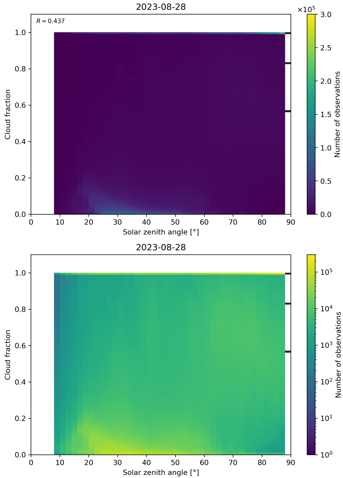
Figure 121: Scatter density plot of “Solar zenith angle” against “Cloud fraction” for 2023-08-27 to 2023-08-29.
