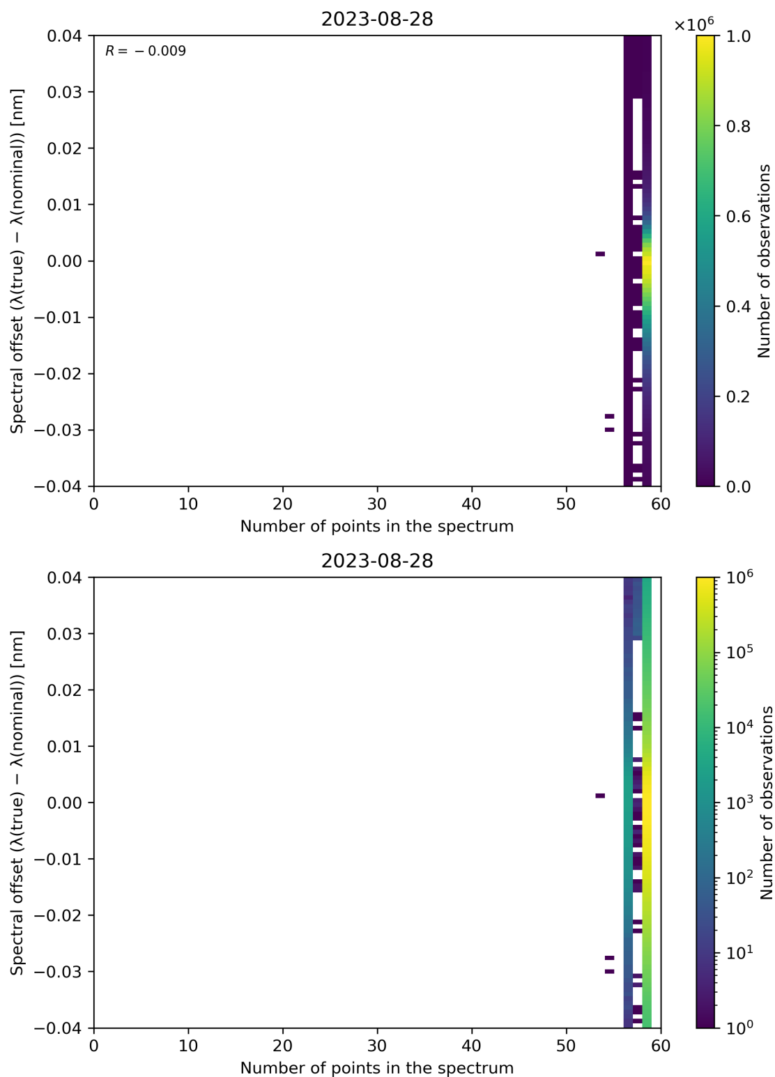
Figure 110: Scatter density plot of “Number of points in the spectrum” against “Spectral offset ( \lambda(\text{true}) - \lambda(\text{nominal}) )” for 2023-08-27 to 2023-08-29.
