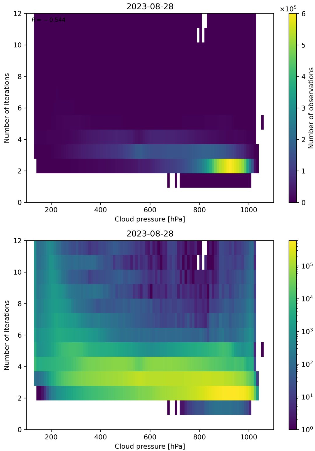
Figure 89: Scatter density plot of “Cloud pressure” against “Number of iterations” for 2023-08-27 to 2023-08-29.
