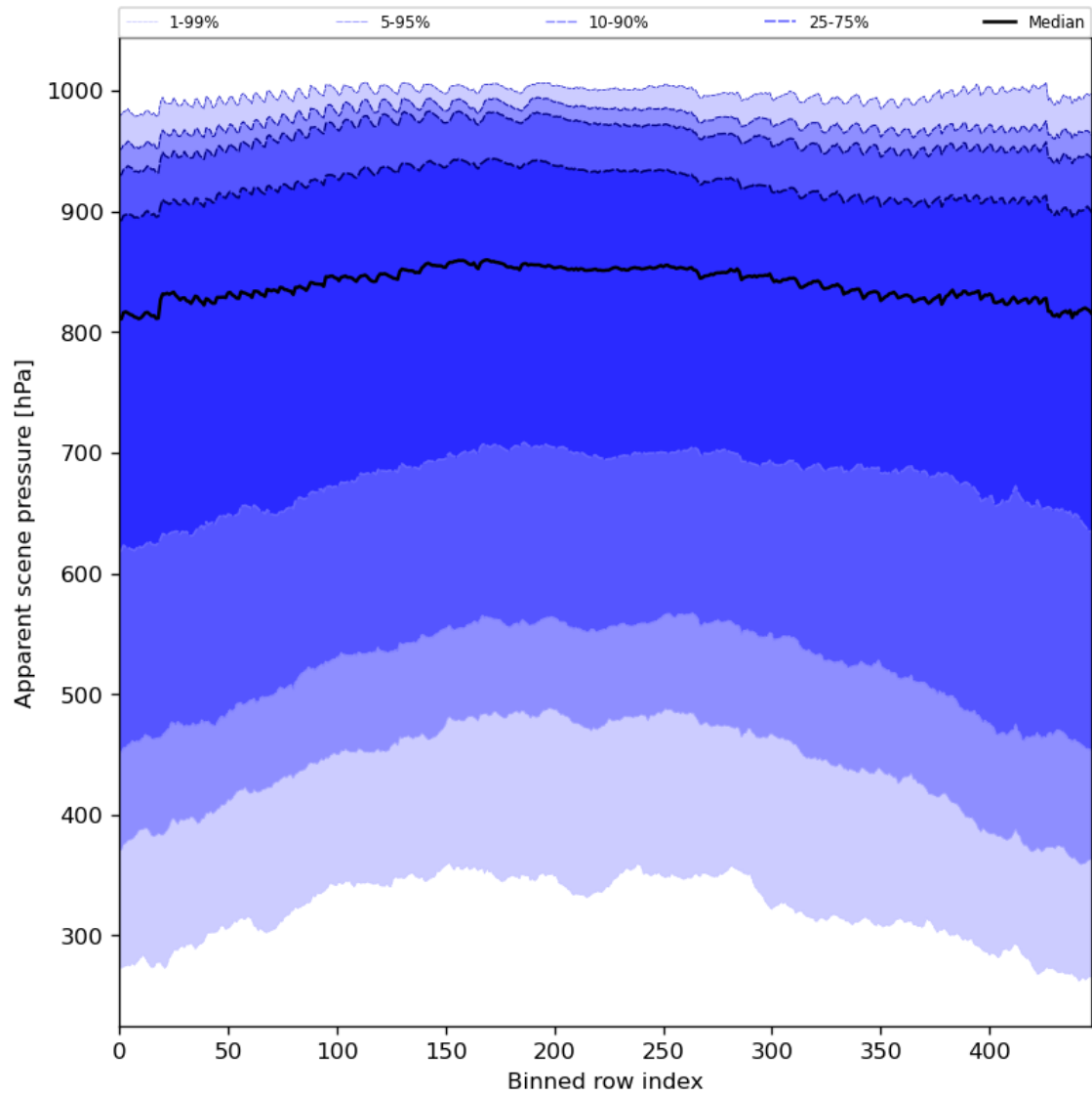
Figure 53: Along track statistics of “Apparent scene pressure” for 2023-08-27 to 2023-08-29
