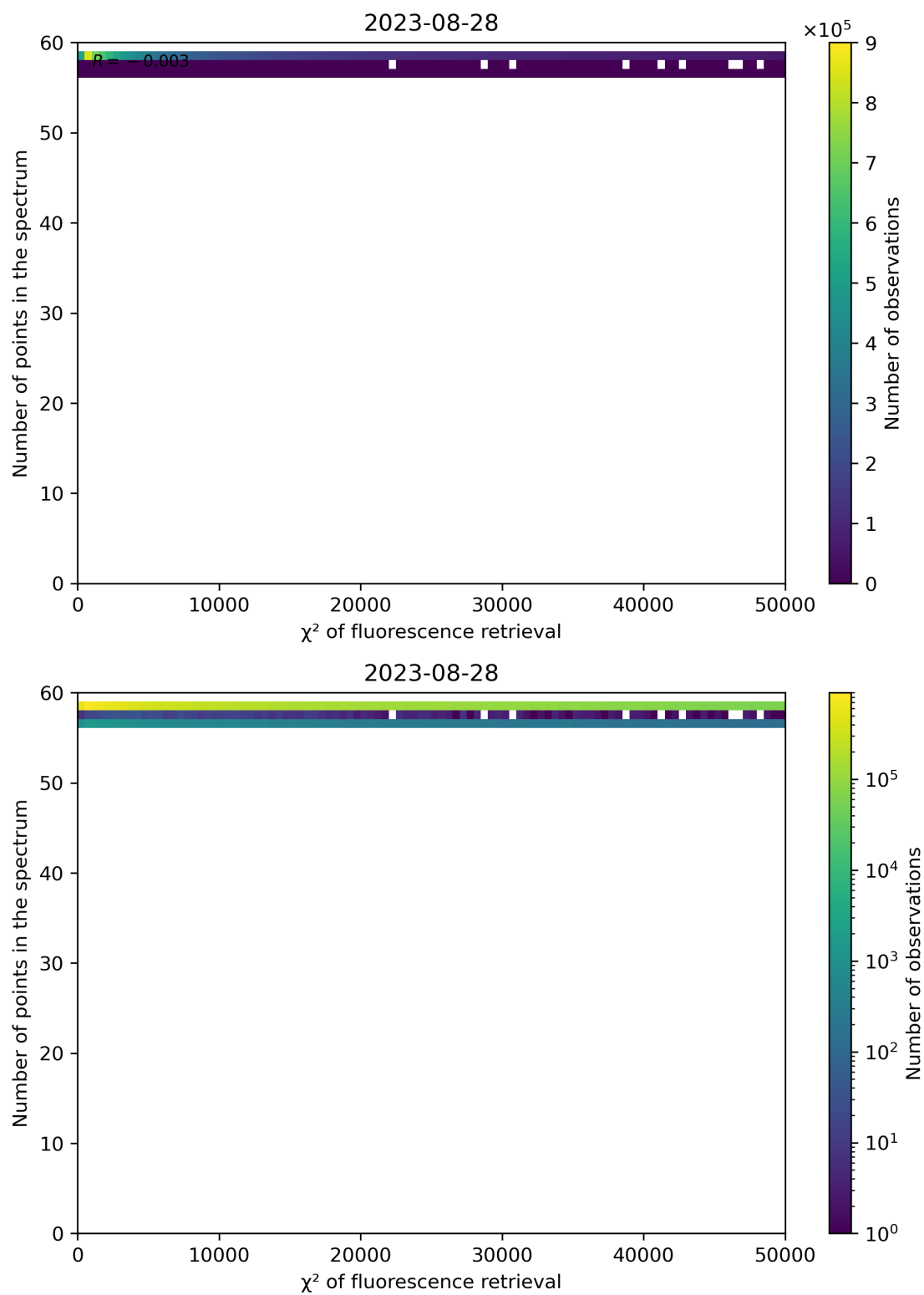
Figure 71: Scatter density plot of " \chi^2 of fluorescence retrieval" against "Number of points in the spectrum" for 2023-08-27 to 2023-08-29.
