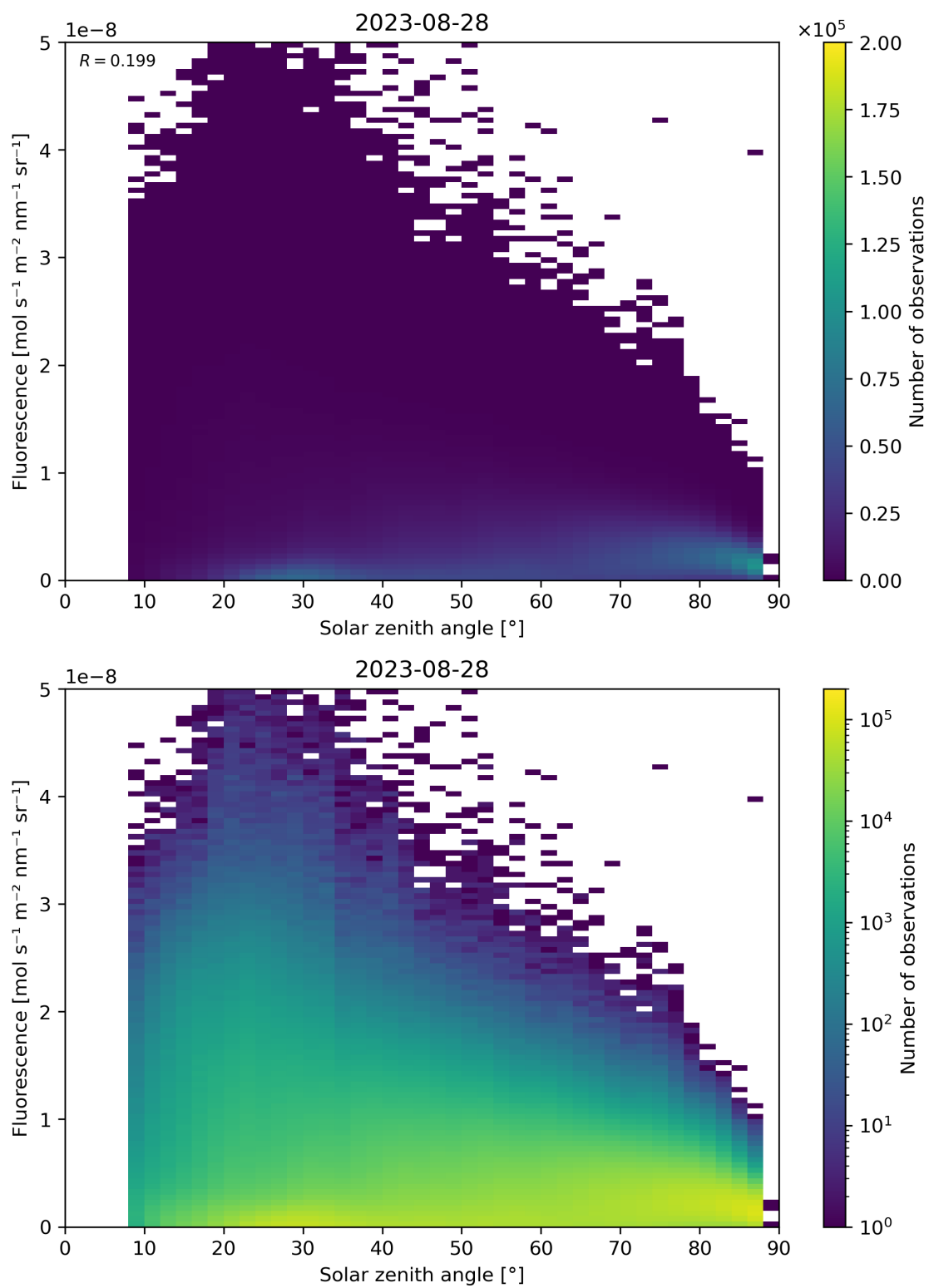
Figure 123: Scatter density plot of “Solar zenith angle” against “Fluorescence” for 2023-08-27 to 2023-08-29.
