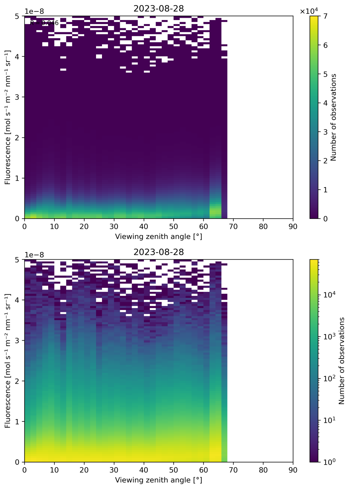
Figure 134: Scatter density plot of “Viewing zenith angle” against “Fluorescence” for 2023-08-27 to 2023-08-29.
