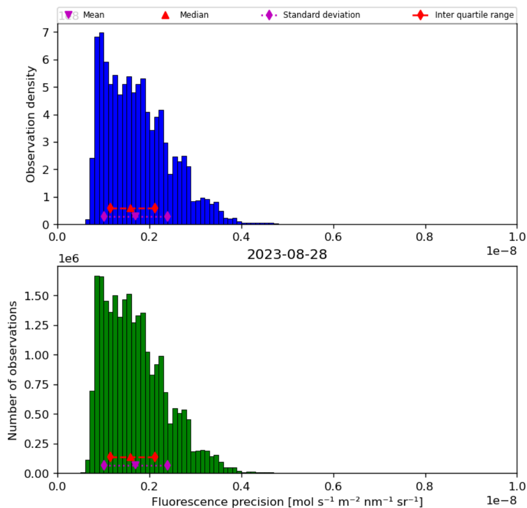
Figure 41: Histogram of “Fluorescence precision” for 2023-08-27 to 2023-08-29
