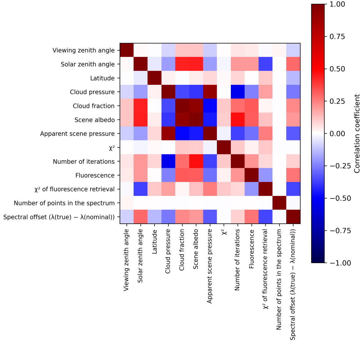
Figure 2: Map of correlation matrix for 2023-08-27 to 2023-08-29.
