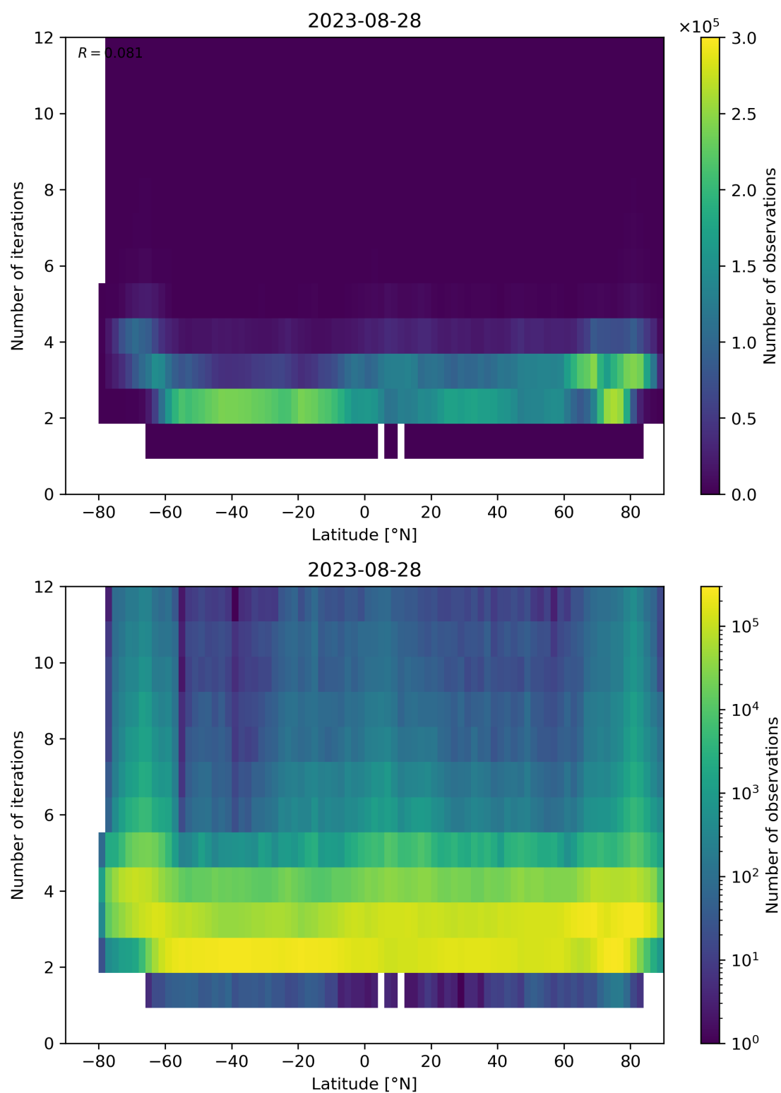
Figure 102: Scatter density plot of “Latitude” against “Number of iterations” for 2023-08-27 to 2023-08-29.
