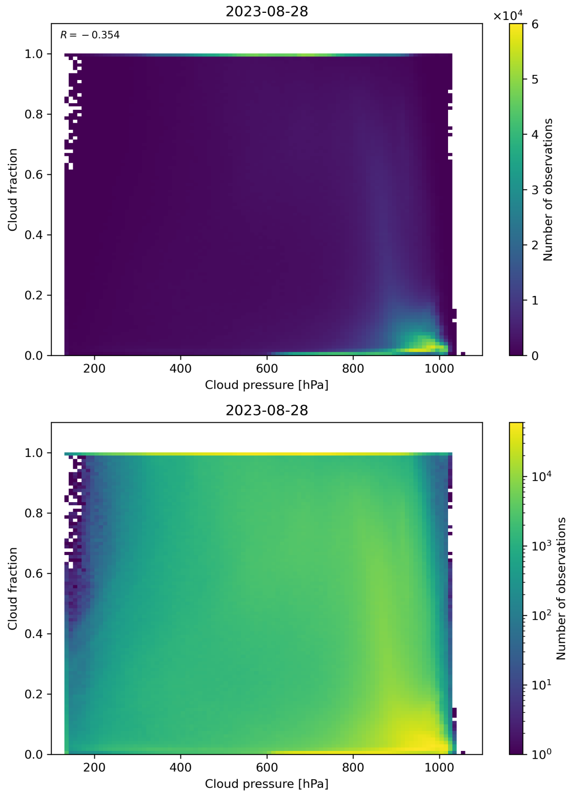
Figure 87: Scatter density plot of “Cloud pressure” against “Cloud fraction” for 2023-08-27 to 2023-08-29.
