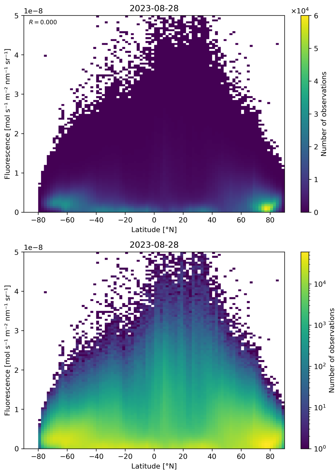
Figure 101: Scatter density plot of “Latitude” against “Fluorescence” for 2023-08-27 to 2023-08-29.
