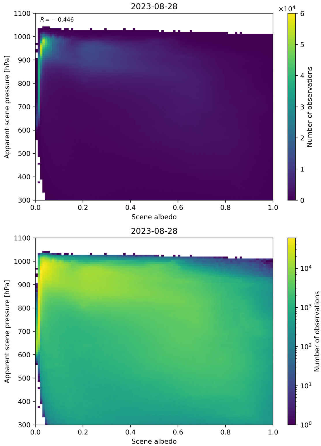
Figure 111: Scatter density plot of “Scene albedo” against “Apparent scene pressure” for 2023-08-27 to 2023-08-29.
