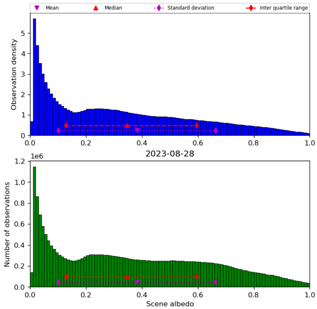
Figure 34: Histogram of “Scene albedo” for 2023-08-27 to 2023-08-29
