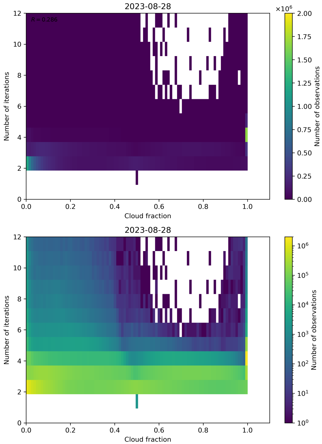
Figure 80: Scatter density plot of “Cloud fraction” against “Number of iterations” for 2023-08-27 to 2023-08-29.
