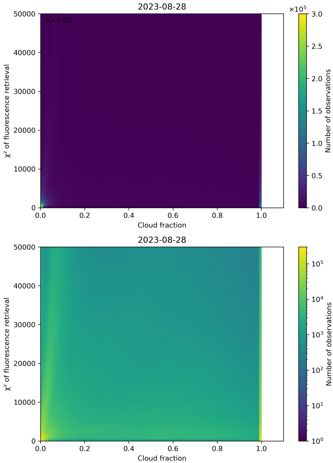
Figure 78: Scatter density plot of “Cloud fraction” against “ \chi^2 of fluorescence retrieval” for 2023-08-27 to 2023-08-29.
