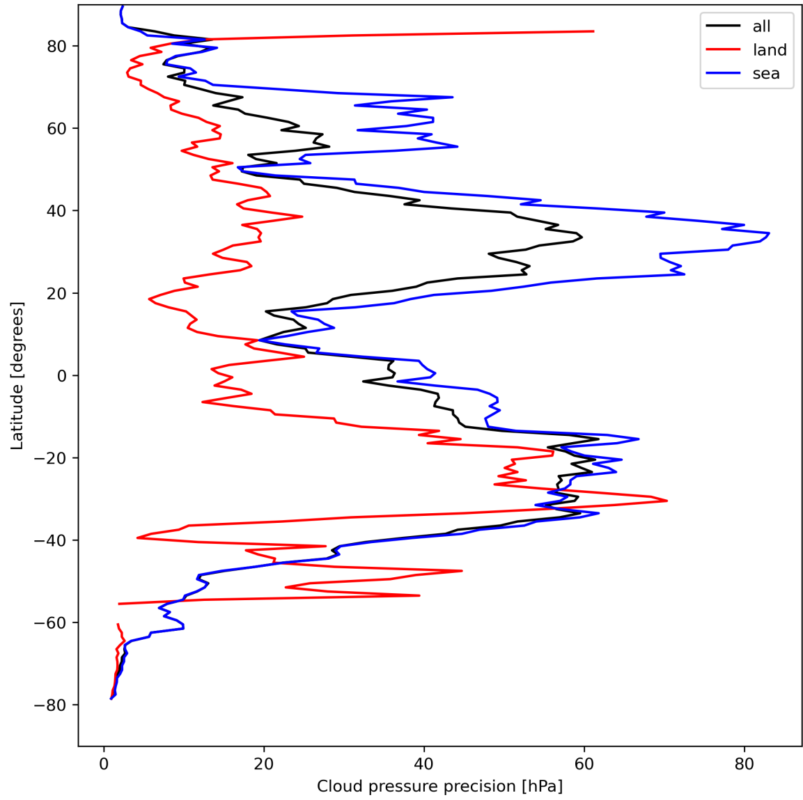
Figure 14: Zonal average of “Cloud pressure precision” for 2023-08-27 to 2023-08-29.
