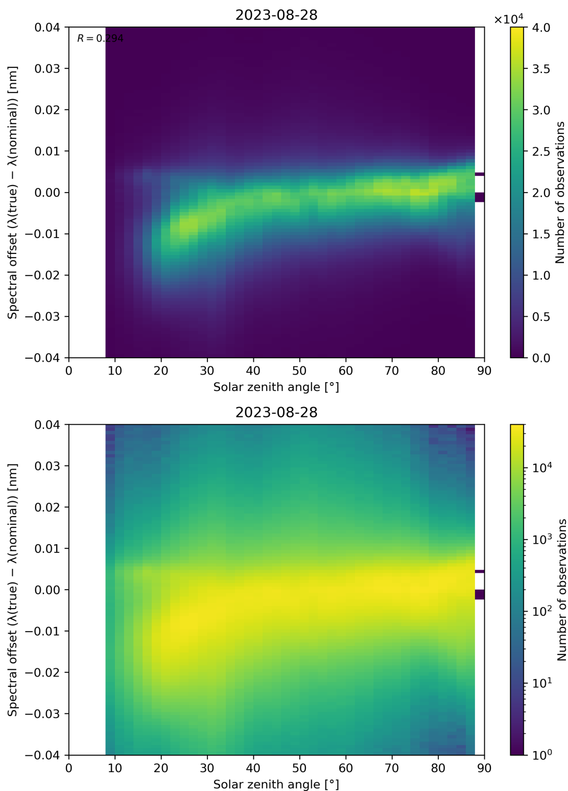
Figure 128: Scatter density plot of “Solar zenith angle” against “Spectral offset ( \lambda(\text{true}) - \lambda(\text{nominal}) )” for 2023-08-27 to 2023-08-29.
