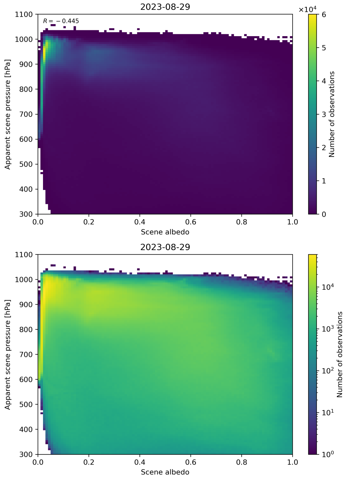
Figure 111: Scatter density plot of “Scene albedo” against “Apparent scene pressure” for 2023-08-28 to 2023-08-30.
