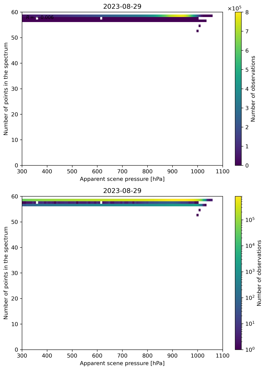
Figure 67: Scatter density plot of “Apparent scene pressure” against “Number of points in the spectrum” for 2023-08-28 to 2023-08-30.
