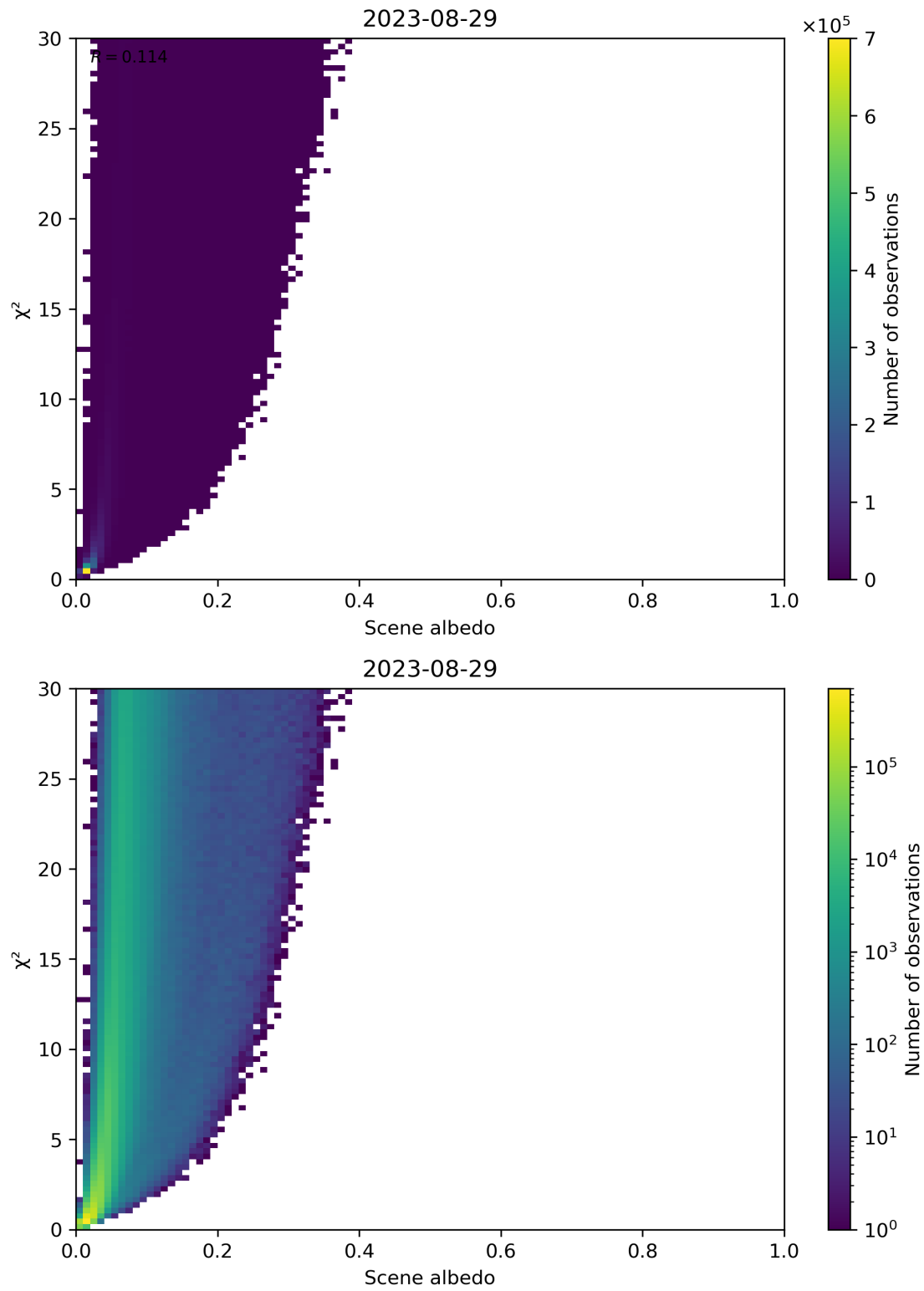
Figure 112: Scatter density plot of “Scene albedo” against “ \chi^2 ” for 2023-08-28 to 2023-08-30.
