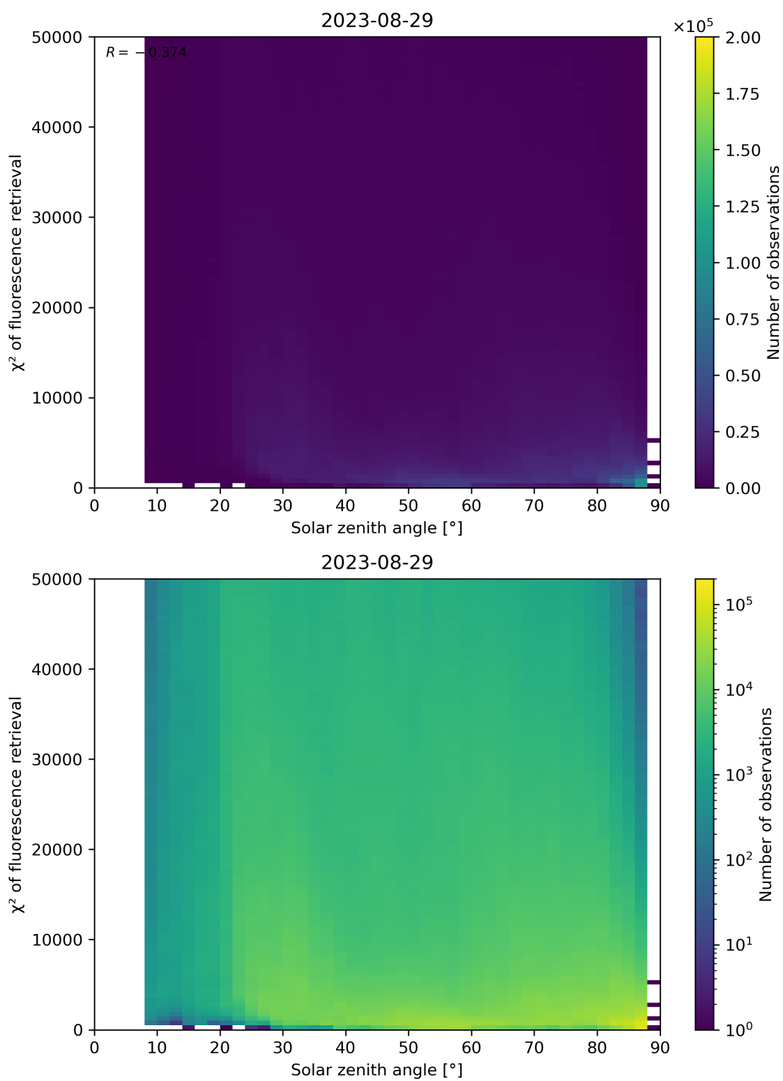
Figure 120: Scatter density plot of “Solar zenith angle” against “ \chi^2 of fluorescence retrieval” for 2023-08-28 to 2023-08-30.
