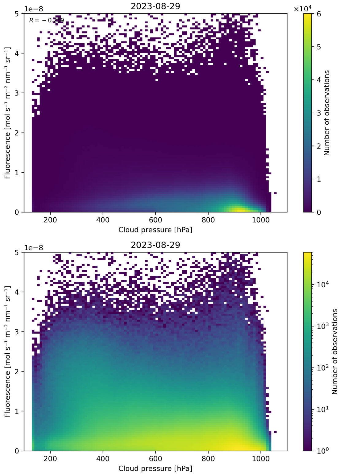
Figure 88: Scatter density plot of “Cloud pressure” against “Fluorescence” for 2023-08-28 to 2023-08-30.
