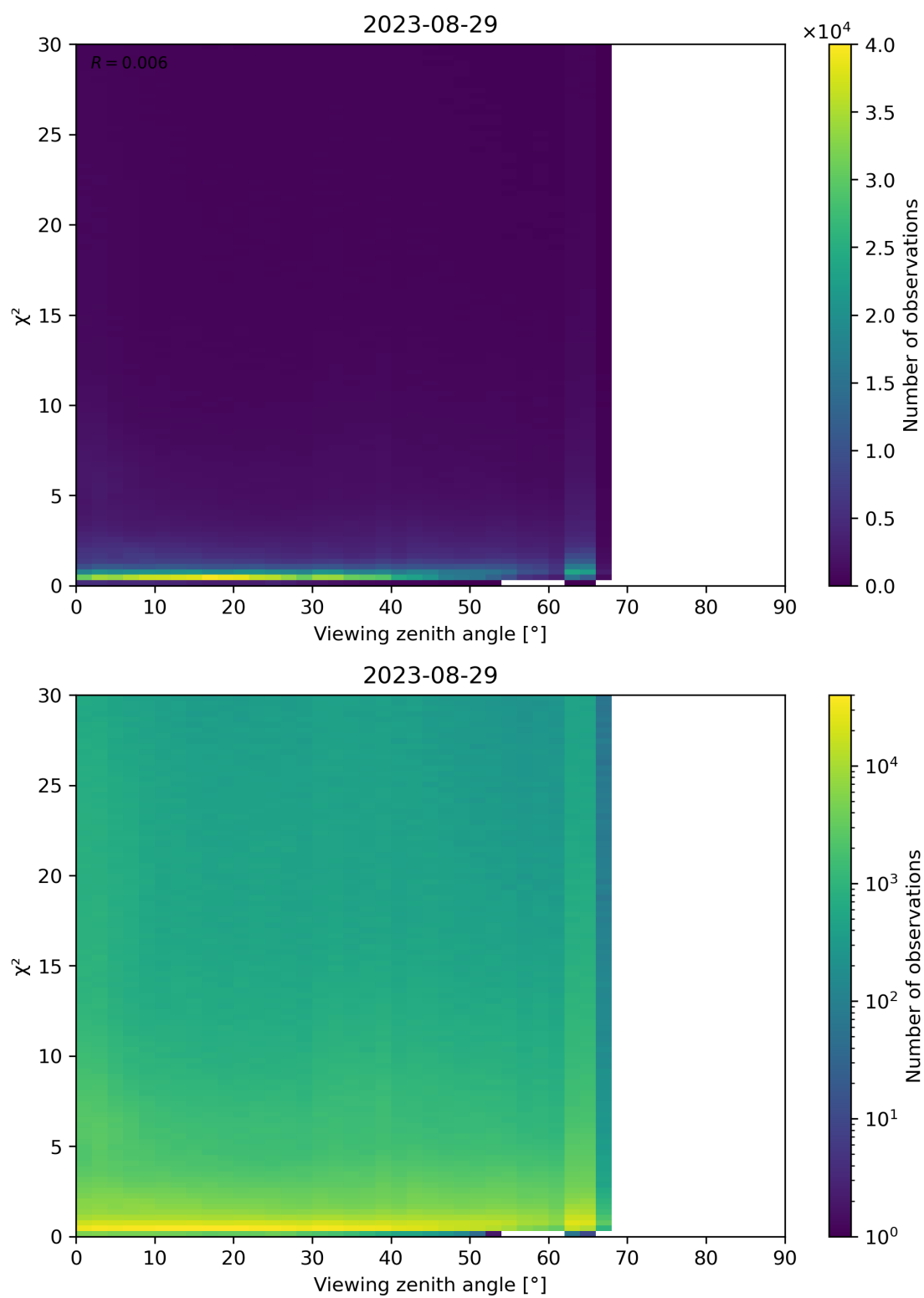
Figure 130: Scatter density plot of “Viewing zenith angle” against “ \chi^2 ” for 2023-08-28 to 2023-08-30.
