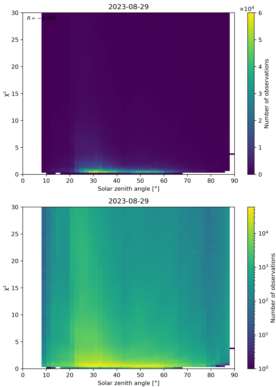
Figure 119: Scatter density plot of “Solar zenith angle” against “ \chi^2 ” for 2023-08-28 to 2023-08-30.
