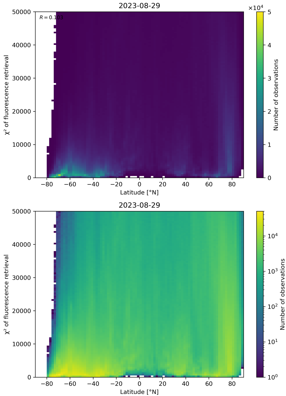
Figure 98: Scatter density plot of “Latitude” against “ \chi^2 of fluorescence retrieval” for 2023-08-28 to 2023-08-30.
