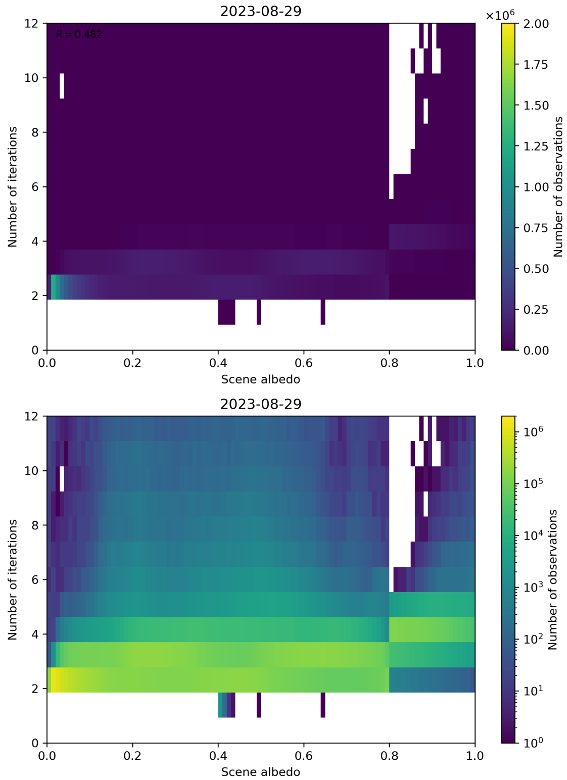
Figure 115: Scatter density plot of “Scene albedo” against “Number of iterations” for 2023-08-28 to 2023-08-30.
