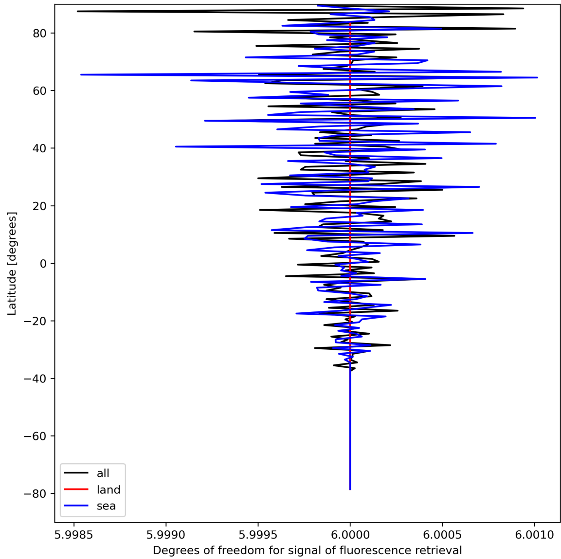
Figure 26: Zonal average of “Degrees of freedom for signal of fluorescence retrieval” for 2023-08-28 to 2023-08-30.
