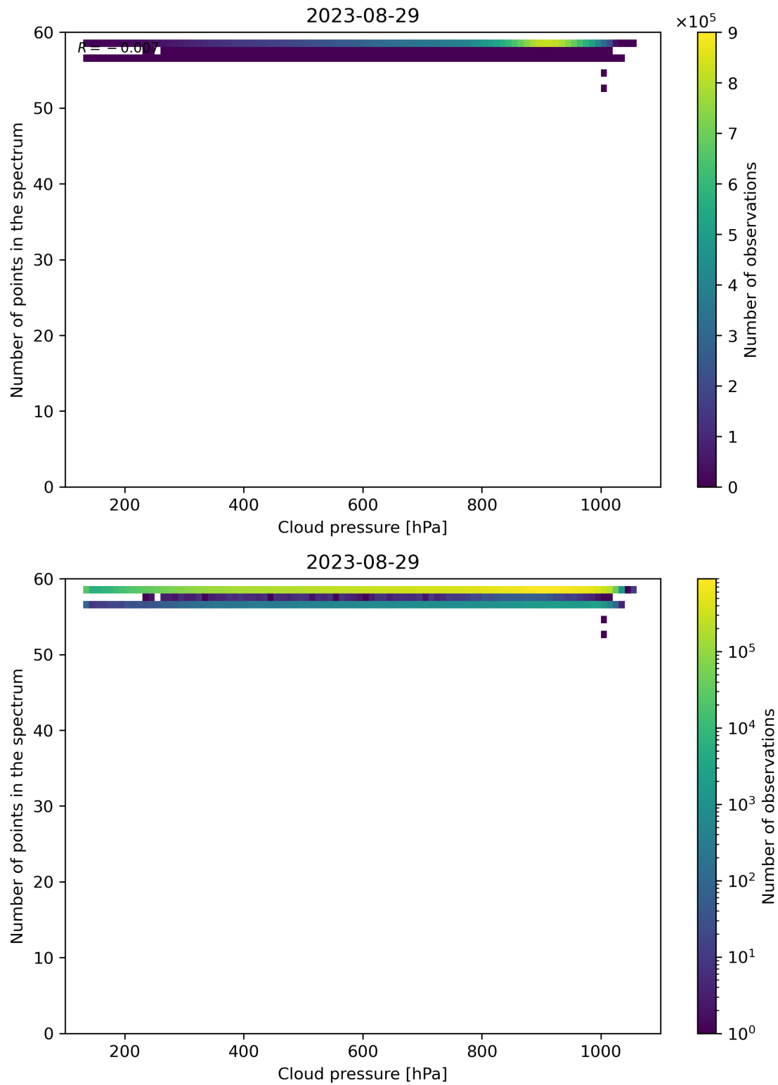
Figure 90: Scatter density plot of “Cloud pressure” against “Number of points in the spectrum” for 2023-08-28 to 2023-08-30.
