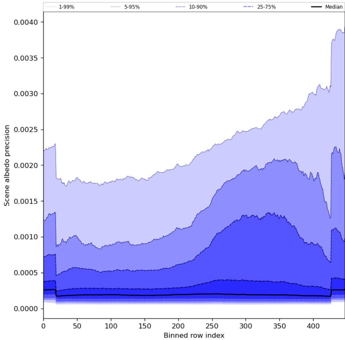
Figure 52: Along track statistics of “Scene albedo precision” for 2023-08-28 to 2023-08-30
