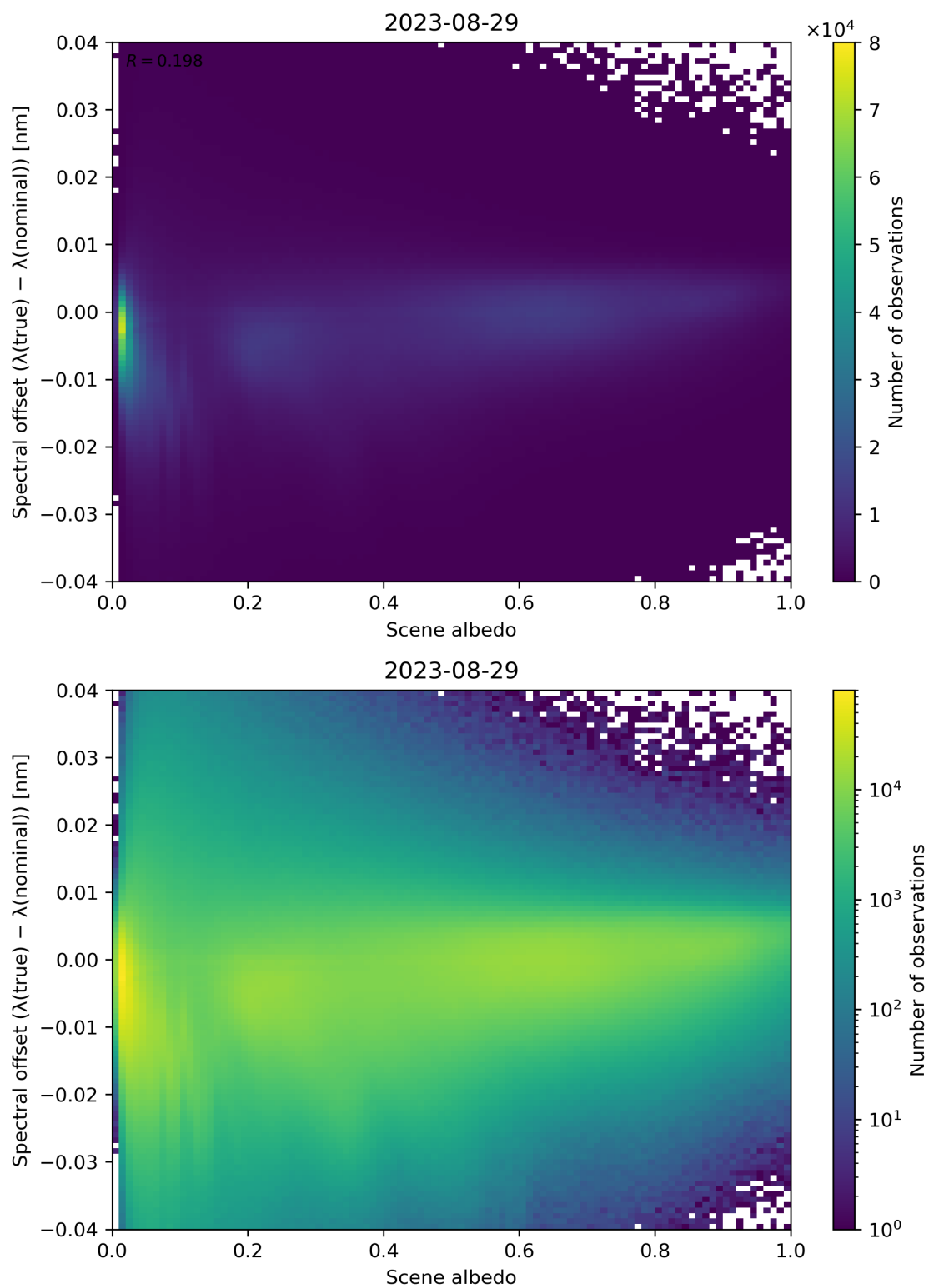
Figure 117: Scatter density plot of “Scene albedo” against “Spectral offset ( \lambda(\text{true}) - \lambda(\text{nominal}) )” for 2023-08-28 to 2023-08-30.
