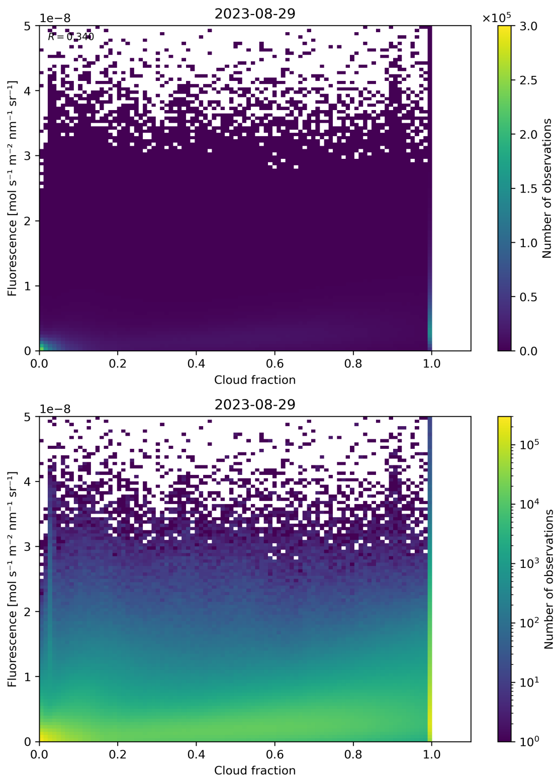
Figure 79: Scatter density plot of “Cloud fraction” against “Fluorescence” for 2023-08-28 to 2023-08-30.
