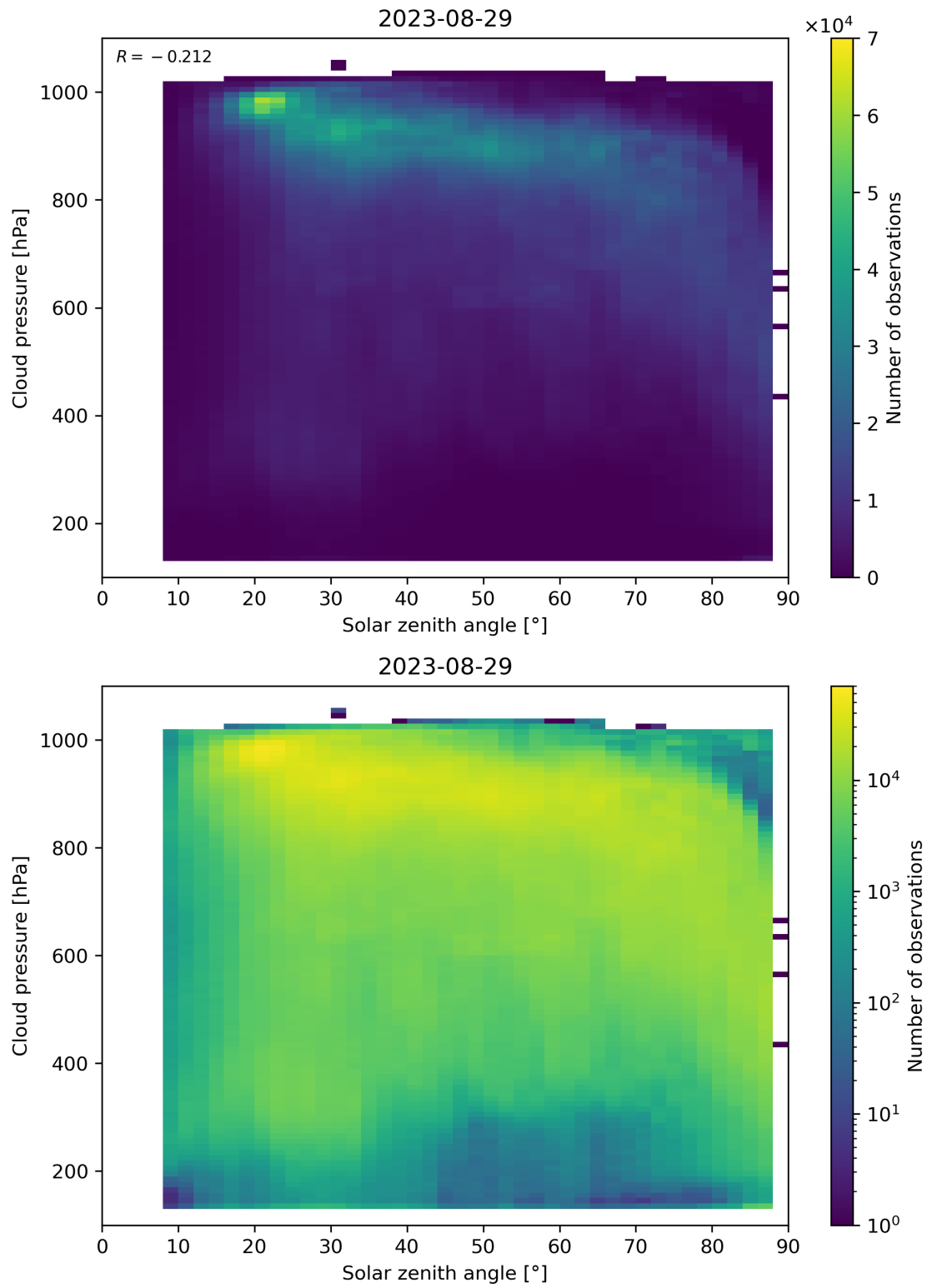
Figure 122: Scatter density plot of “Solar zenith angle” against “Cloud pressure” for 2023-08-28 to 2023-08-30.
