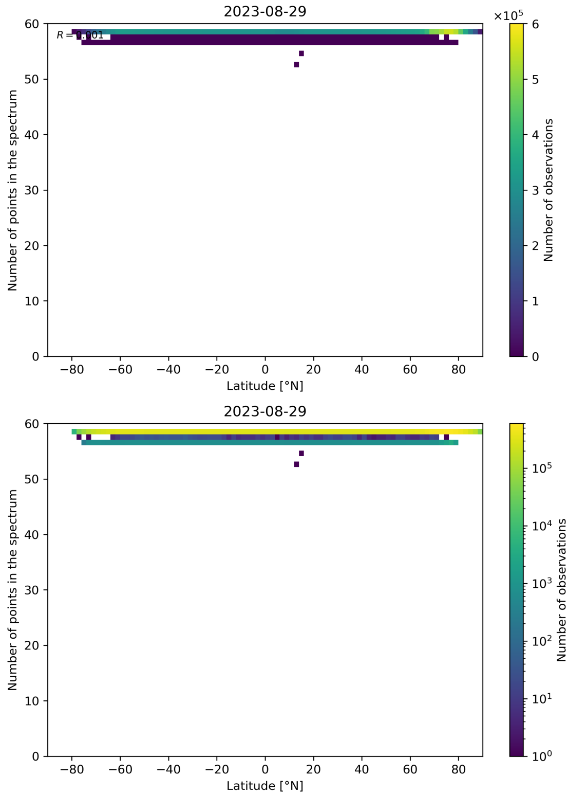
Figure 103: Scatter density plot of “Latitude” against “Number of points in the spectrum” for 2023-08-28 to 2023-08-30.
