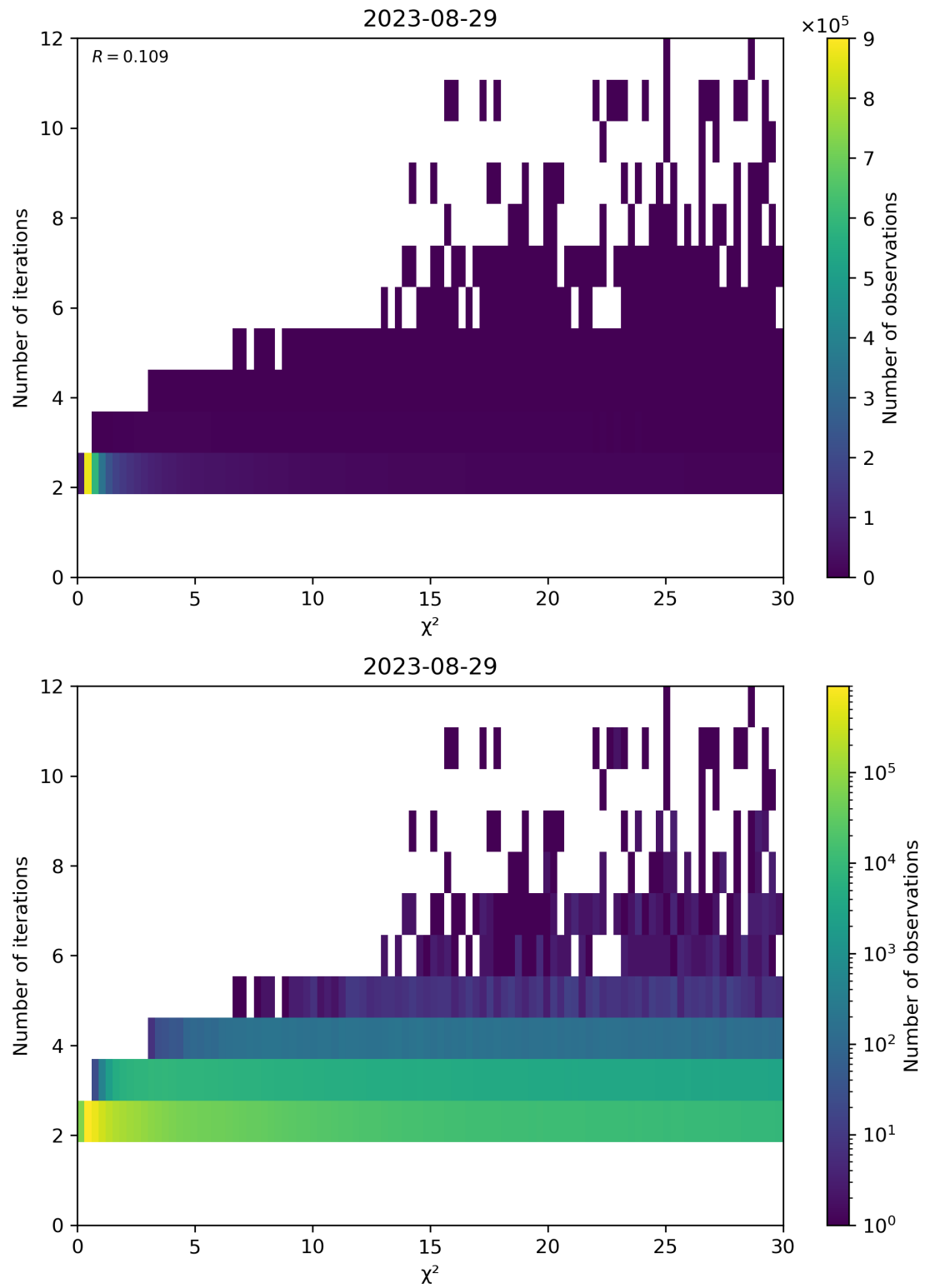
Figure 73: Scatter density plot of “ \chi^2 ” against “Number of iterations” for 2023-08-28 to 2023-08-30.
