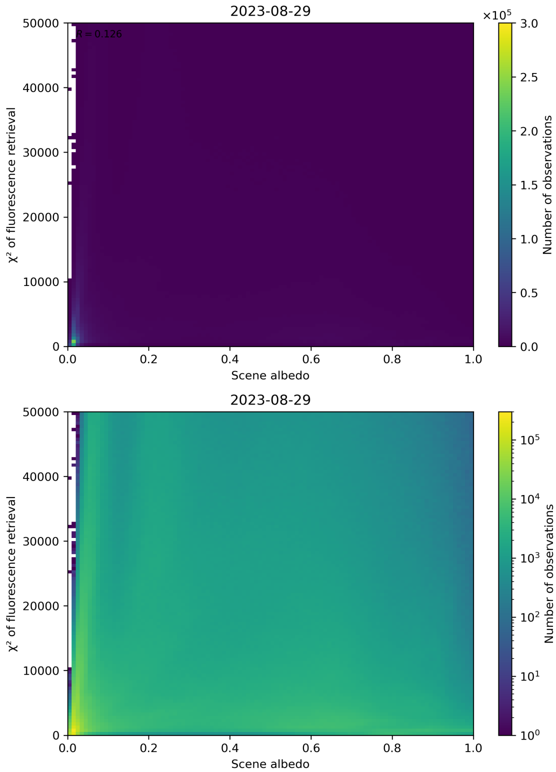
Figure 113: Scatter density plot of “Scene albedo” against “ \chi^2 of fluorescence retrieval” for 2023-08-28 to 2023-08-30.
