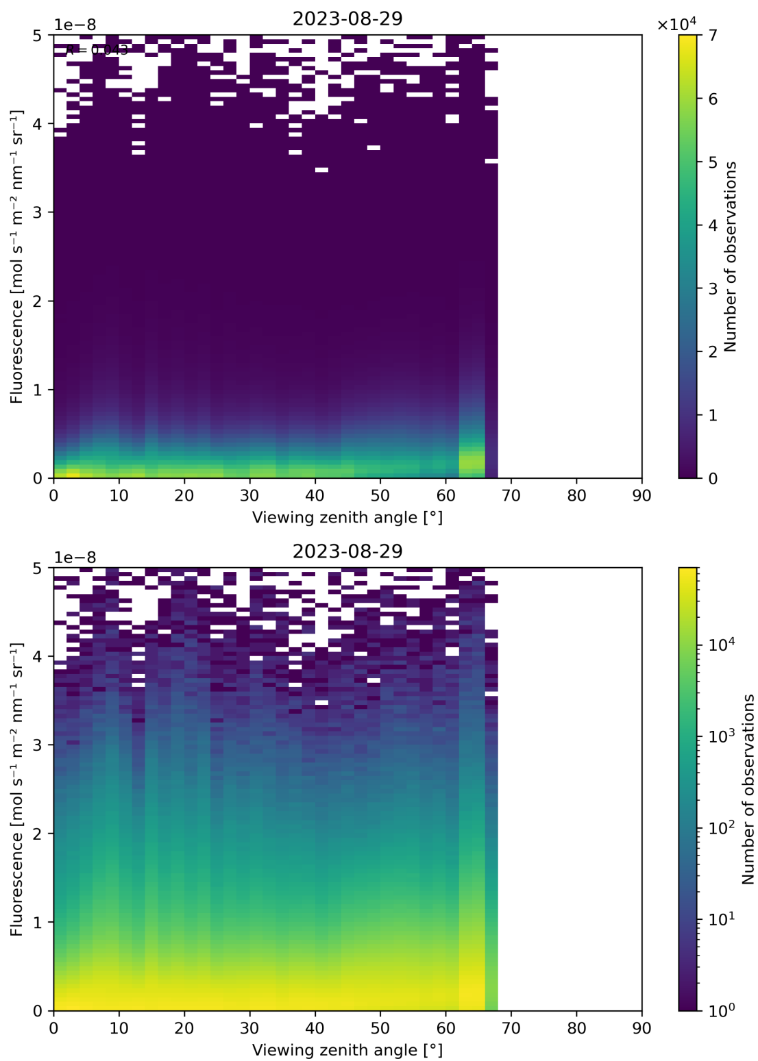
Figure 134: Scatter density plot of “Viewing zenith angle” against “Fluorescence” for 2023-08-28 to 2023-08-30.
