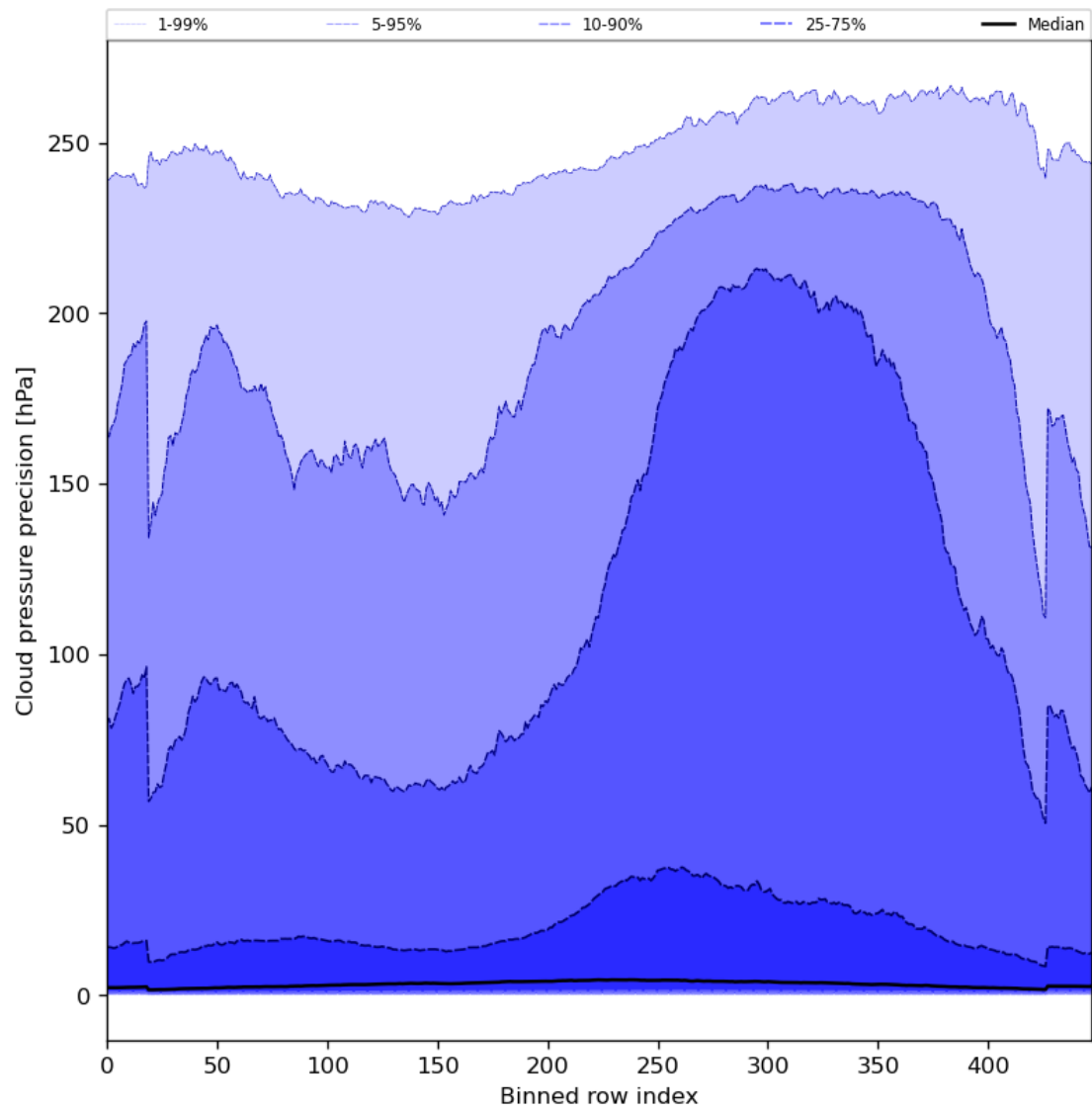
Figure 48: Along track statistics of “Cloud pressure precision” for 2023-08-28 to 2023-08-30
