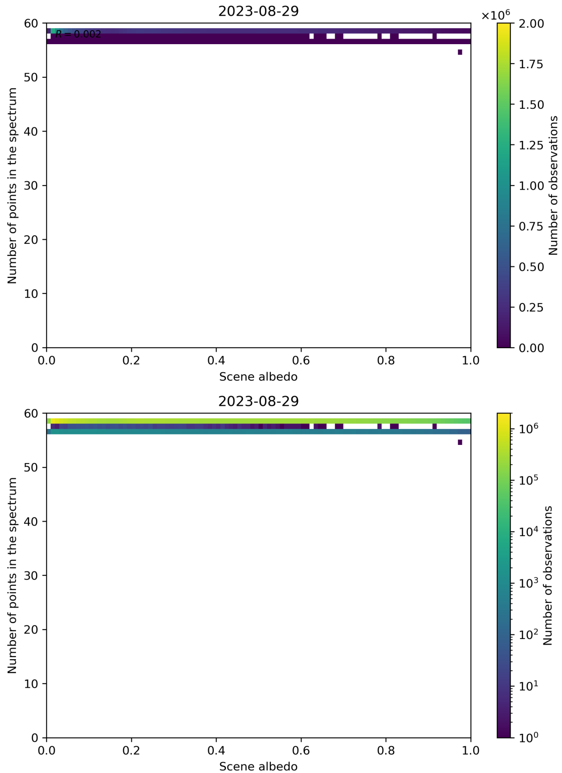
Figure 116: Scatter density plot of “Scene albedo” against “Number of points in the spectrum” for 2023-08-28 to 2023-08-30.
