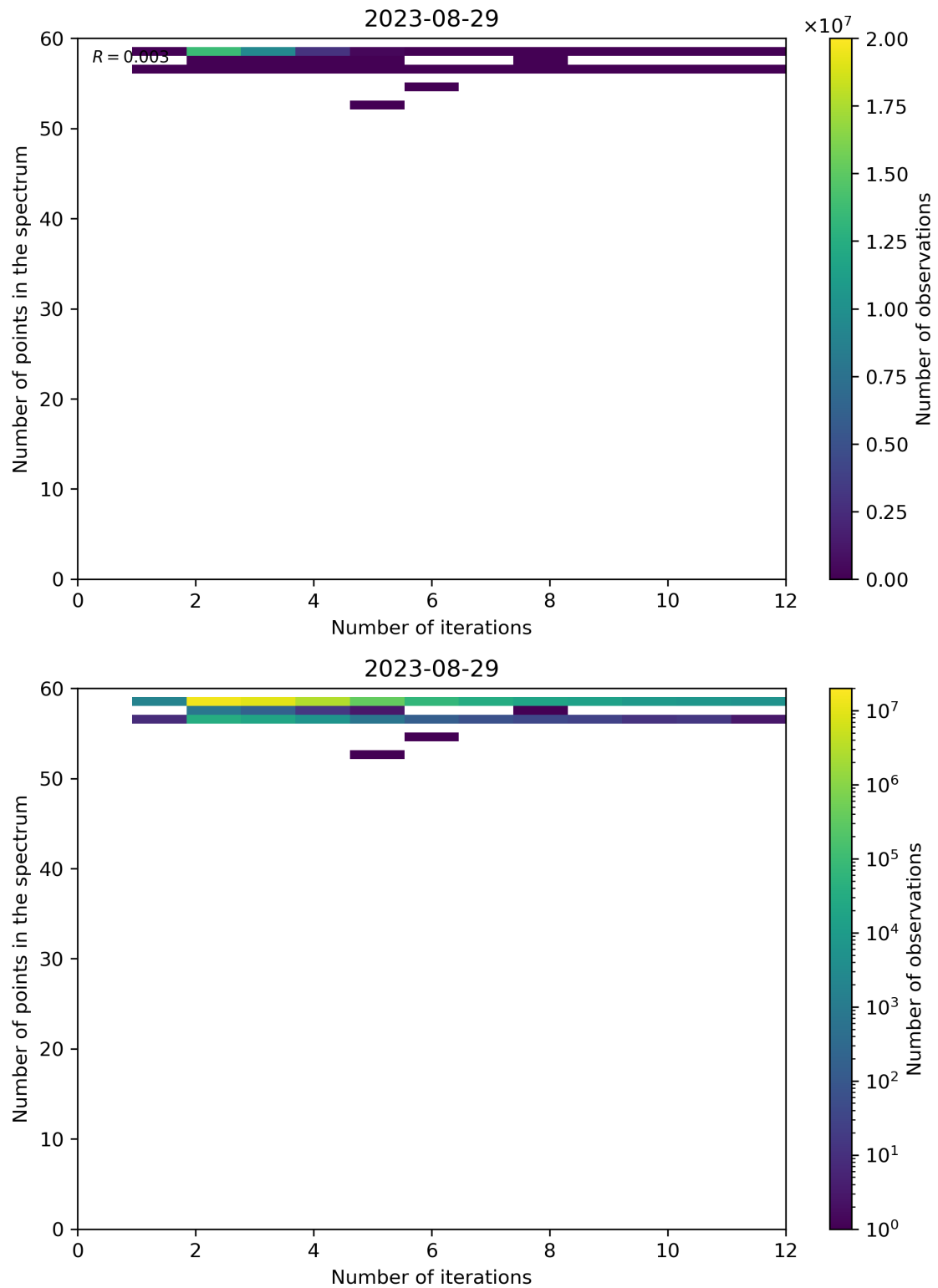
Figure 108: Scatter density plot of “Number of iterations” against “Number of points in the spectrum” for 2023-08-28 to 2023-08-30.
