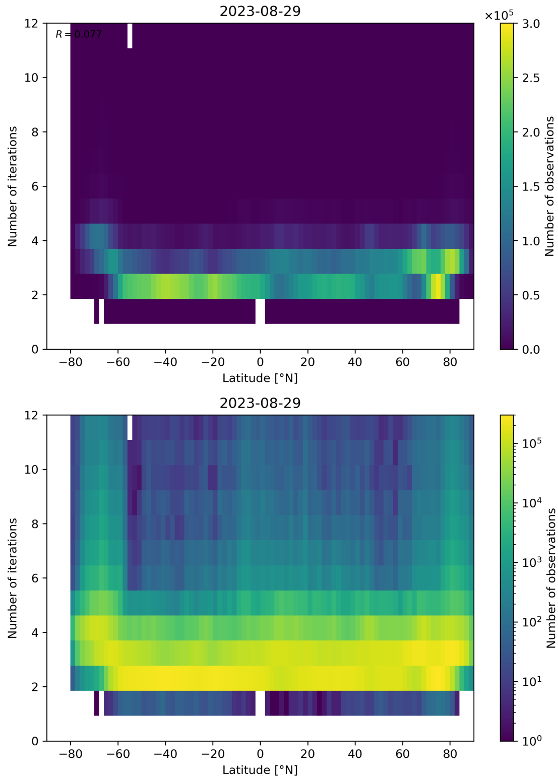
Figure 102: Scatter density plot of “Latitude” against “Number of iterations” for 2023-08-28 to 2023-08-30.
