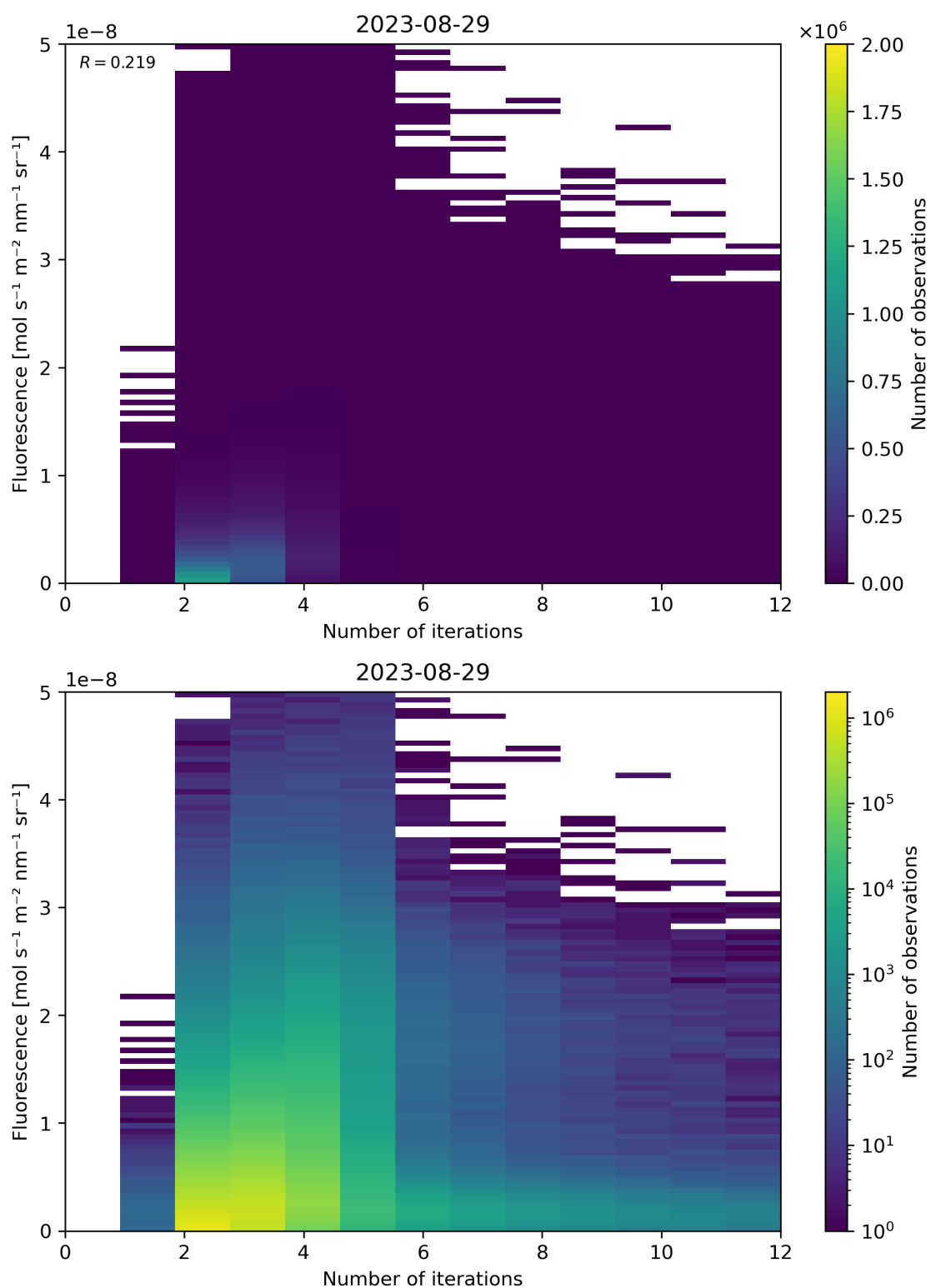
Figure 107: Scatter density plot of “Number of iterations” against “Fluorescence” for 2023-08-28 to 2023-08-30.
