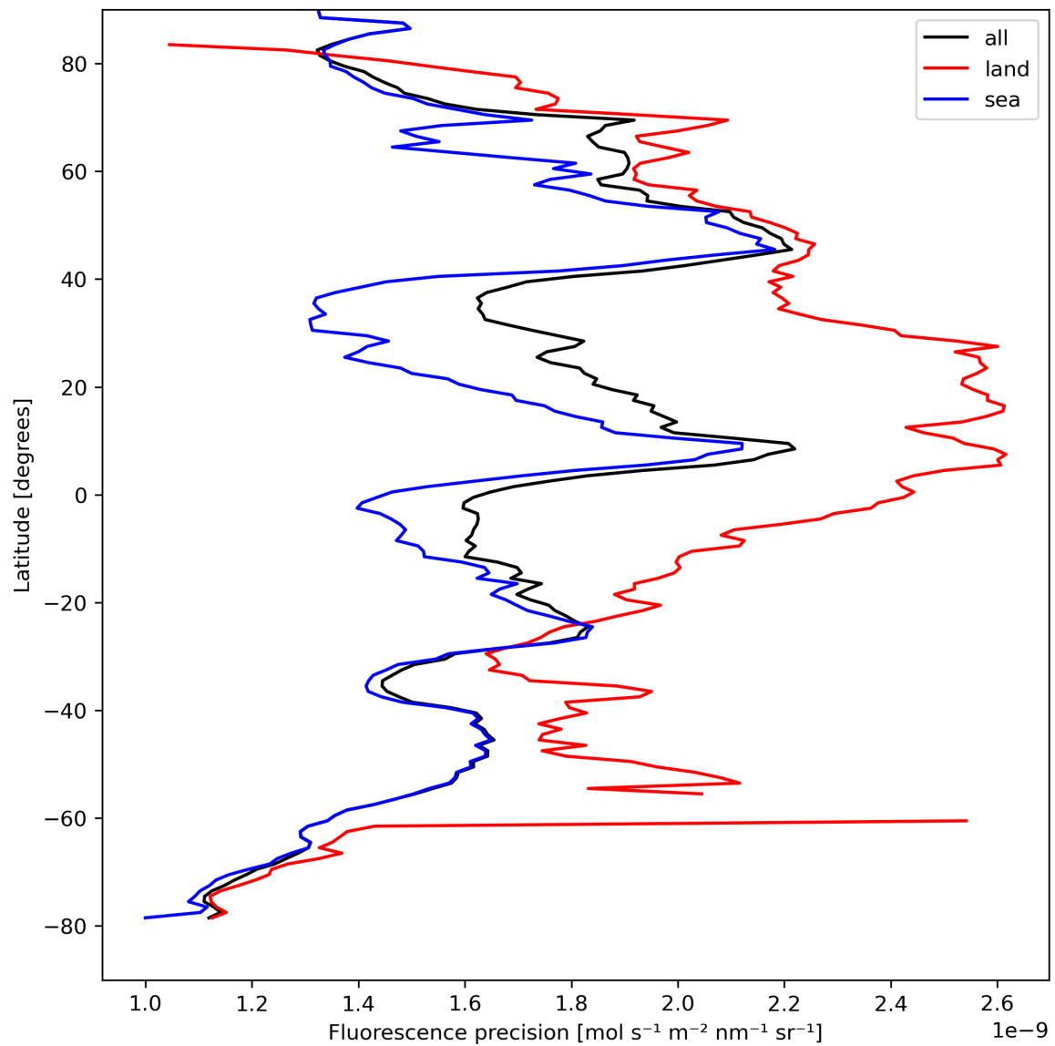
Figure 24: Zonal average of “Fluorescence precision” for 2023-08-28 to 2023-08-30.
