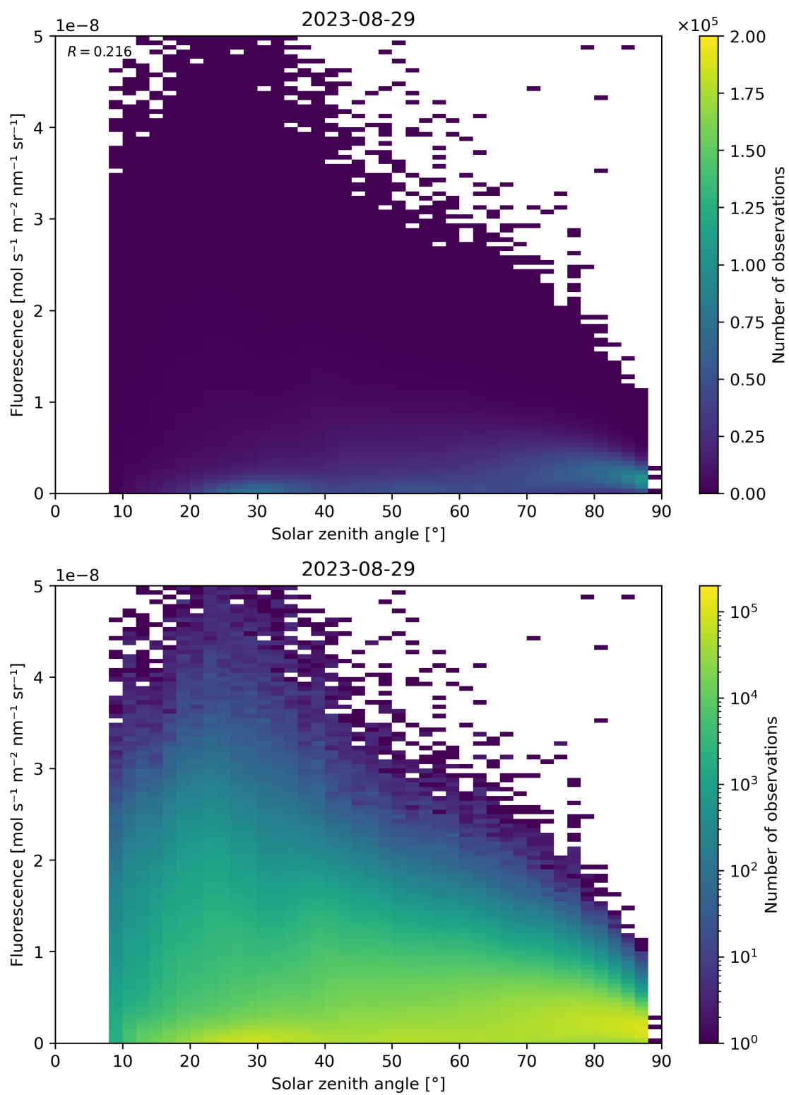
Figure 123: Scatter density plot of “Solar zenith angle” against “Fluorescence” for 2023-08-28 to 2023-08-30.
