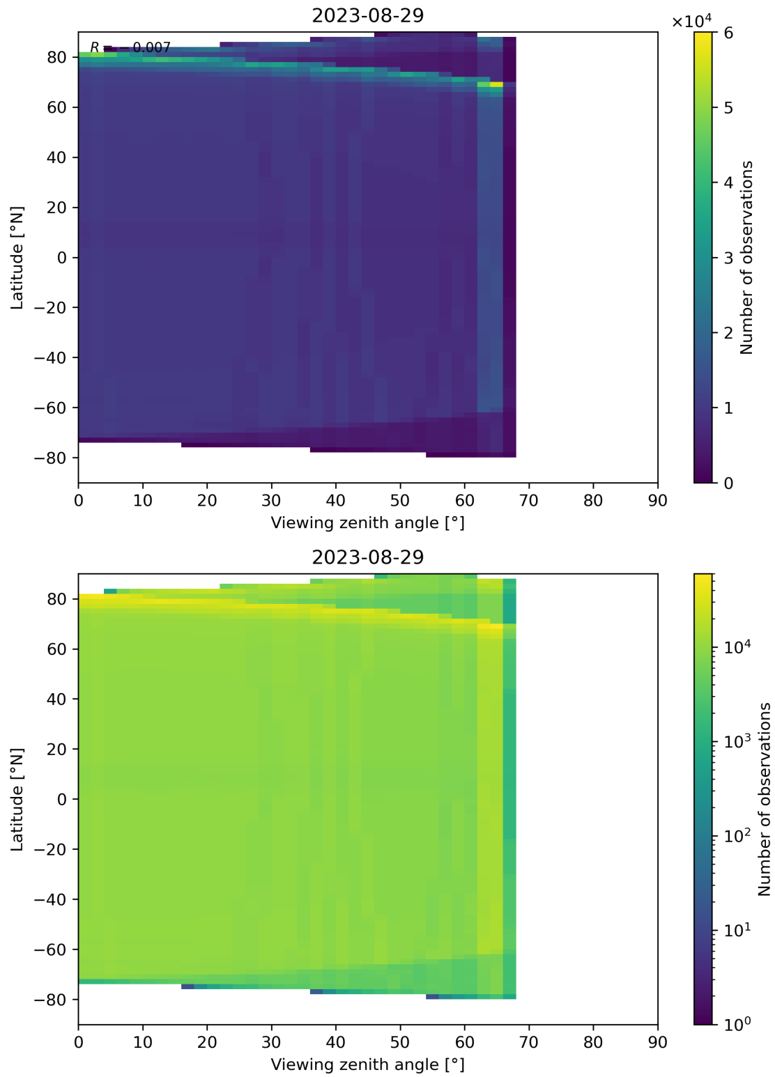
Figure 135: Scatter density plot of “Viewing zenith angle” against “Latitude” for 2023-08-28 to 2023-08-30.
