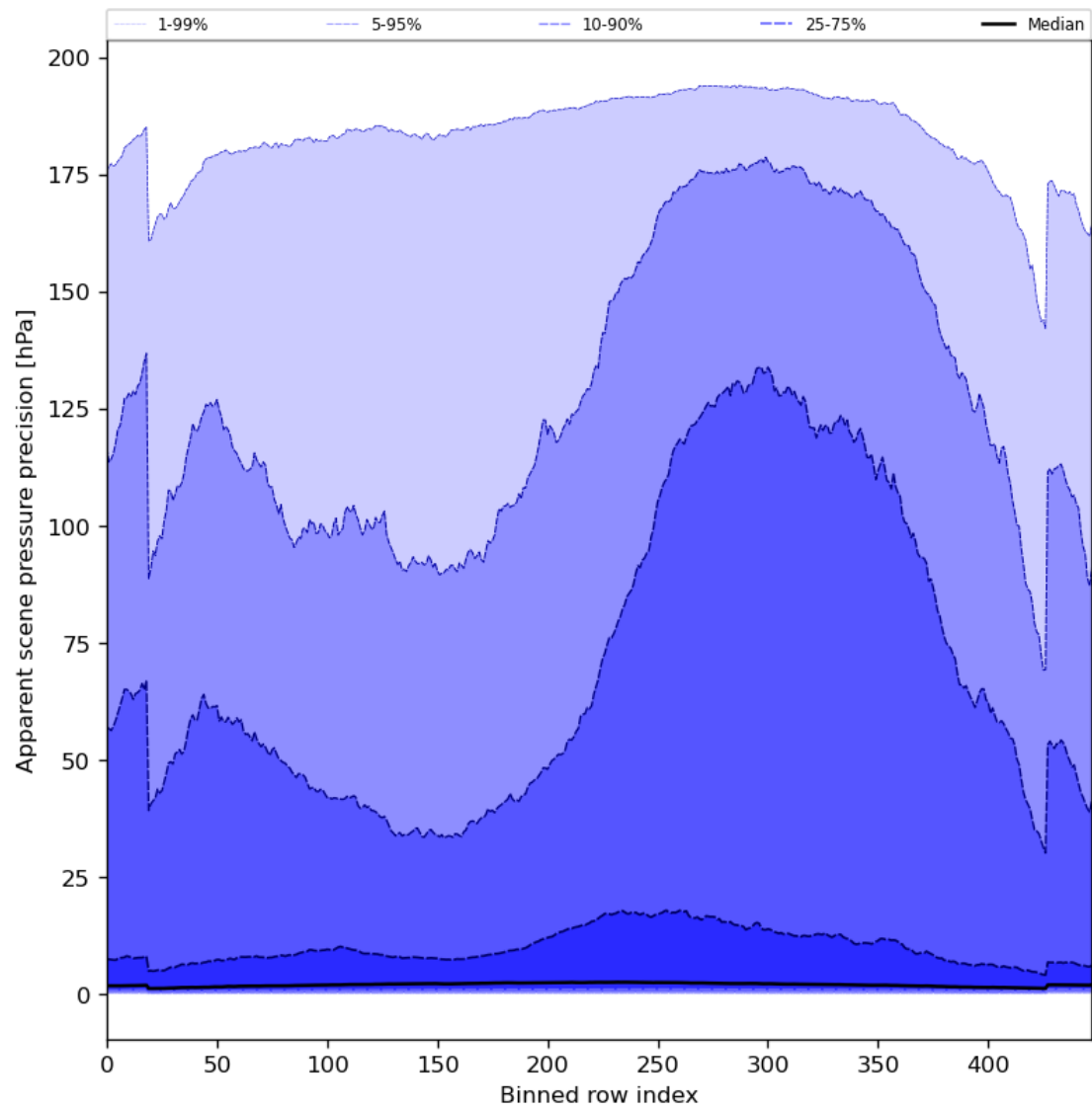
Figure 54: Along track statistics of “Apparent scene pressure precision” for 2023-08-28 to 2023-08-30
