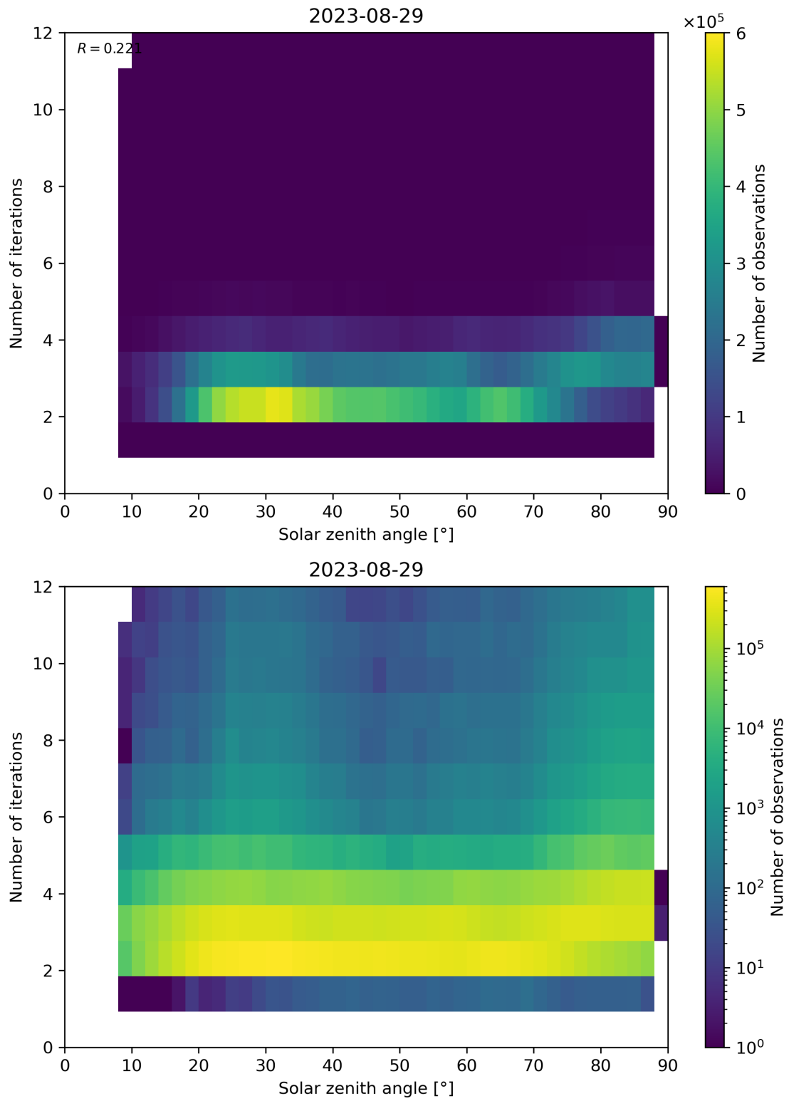
Figure 125: Scatter density plot of “Solar zenith angle” against “Number of iterations” for 2023-08-28 to 2023-08-30.
