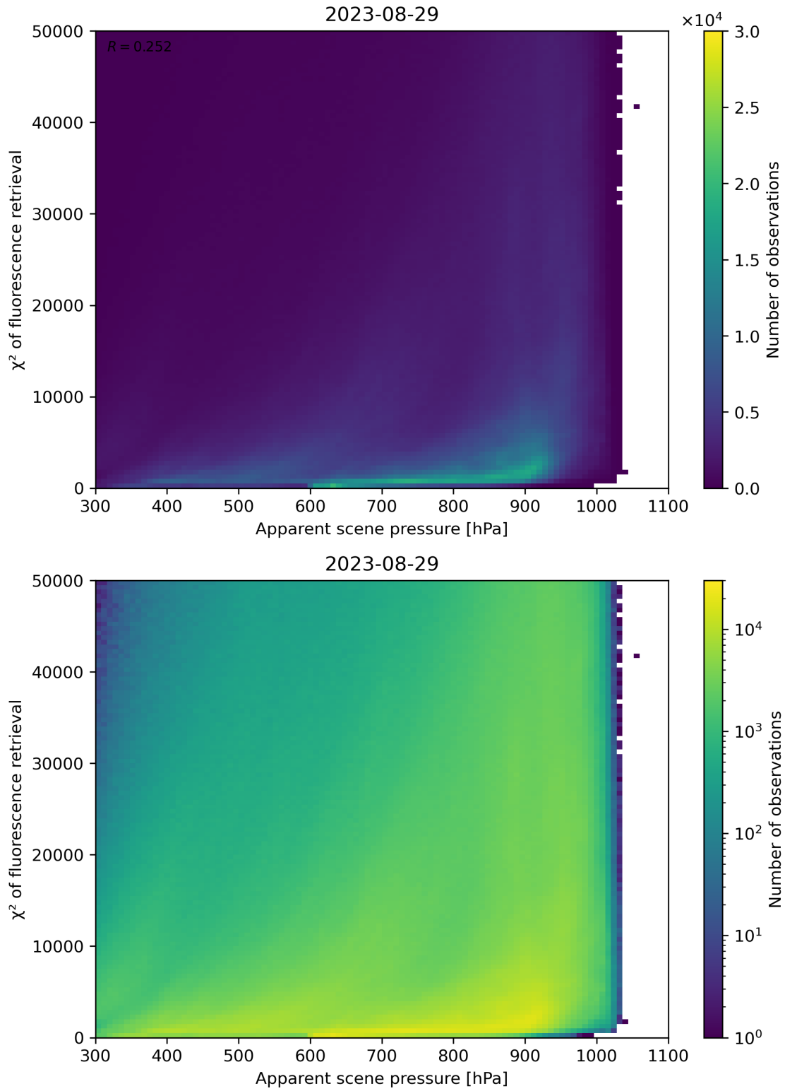
Figure 64: Scatter density plot of “Apparent scene pressure” against “ \chi^2 of fluorescence retrieval” for 2023-08-28 to 2023-08-30.
