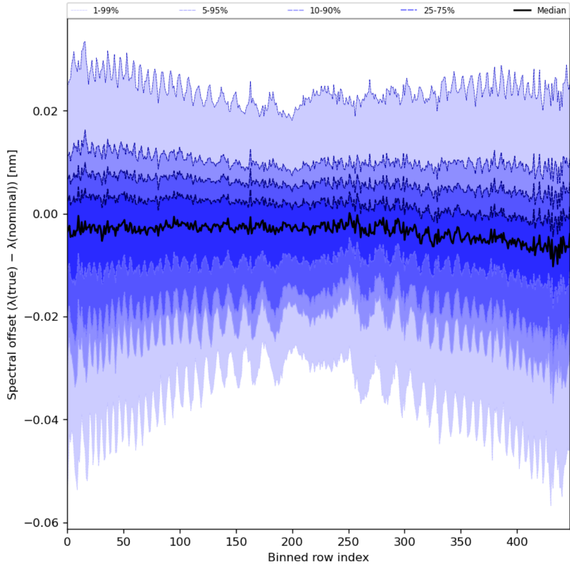
Figure 62: Along track statistics of “Spectral offset ( \lambda(\text{true}) - \lambda(\text{nominal}) )” for 2023-08-28 to 2023-08-30
