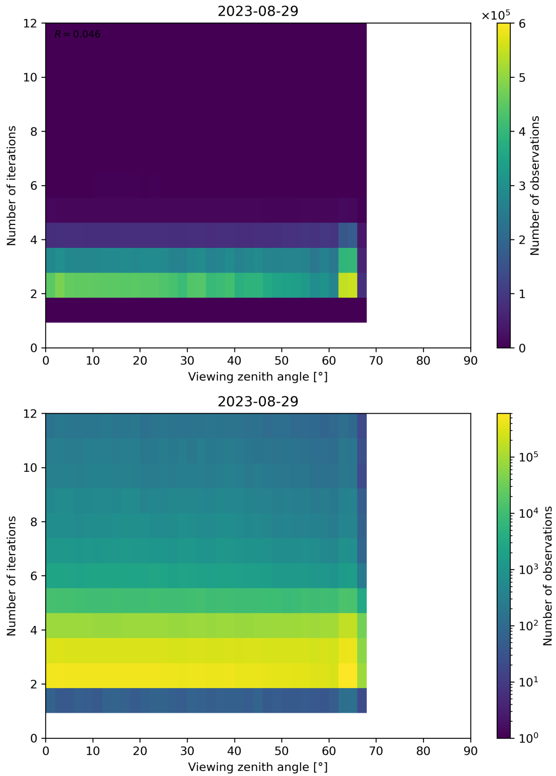
Figure 136: Scatter density plot of “Viewing zenith angle” against “Number of iterations” for 2023-08-28 to 2023-08-30.
