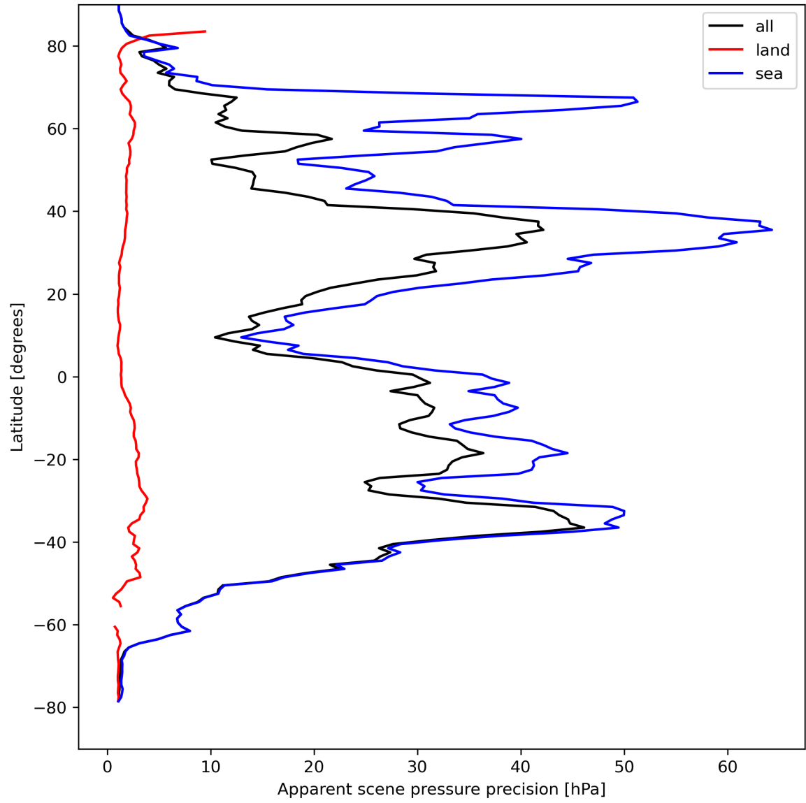
Figure 20: Zonal average of “Apparent scene pressure precision” for 2023-08-28 to 2023-08-30.
