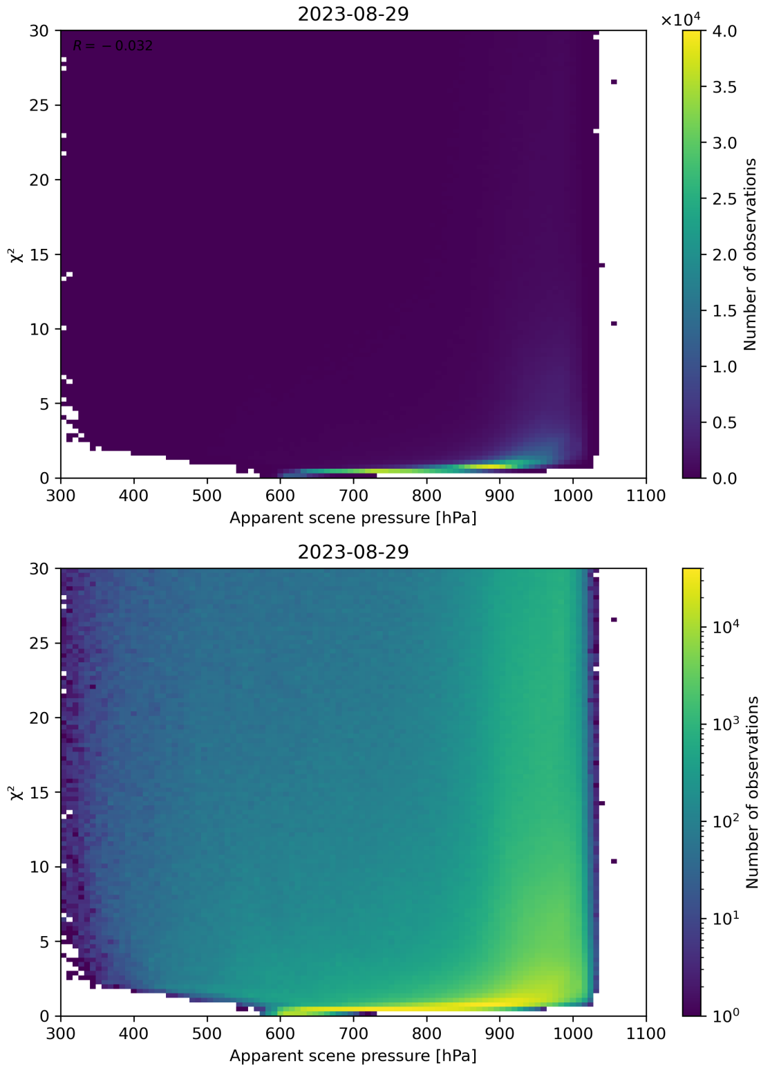
Figure 63: Scatter density plot of “Apparent scene pressure” against “ \chi^2 ” for 2023-08-28 to 2023-08-30.
