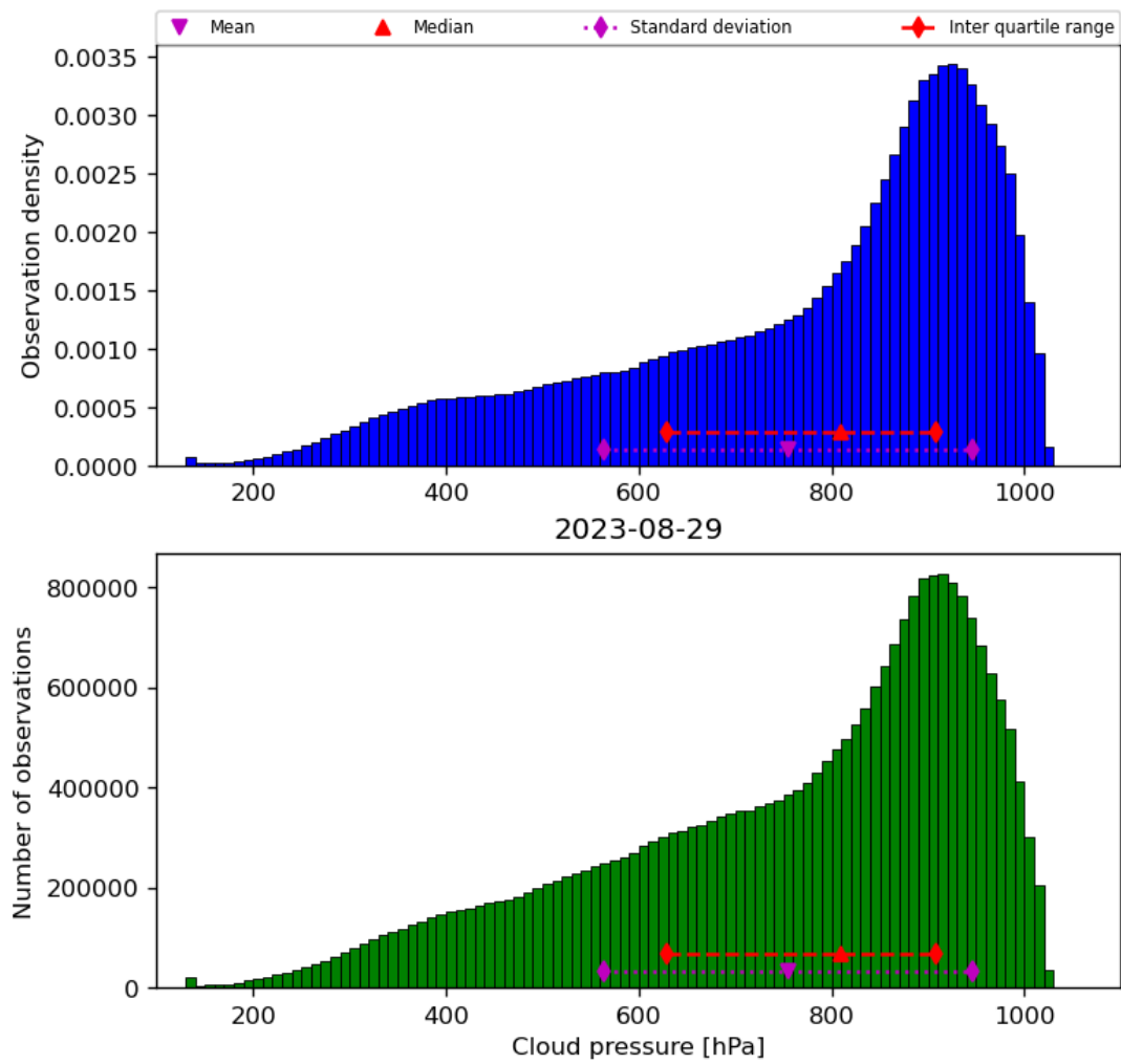
Figure 30: Histogram of “Cloud pressure” for 2023-08-28 to 2023-08-30
