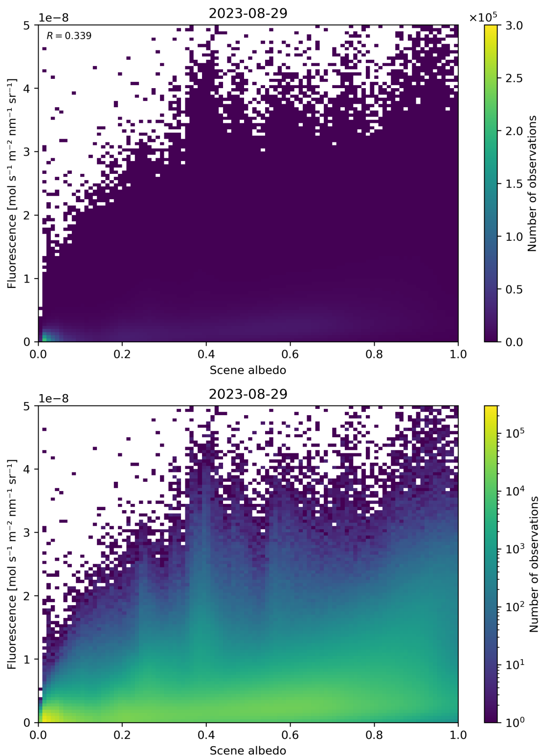
Figure 114: Scatter density plot of “Scene albedo” against “Fluorescence” for 2023-08-28 to 2023-08-30.
