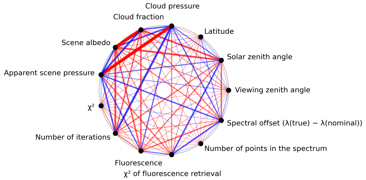
Figure 1: Map of correlation graph for 2023-08-28 to 2023-08-30.
