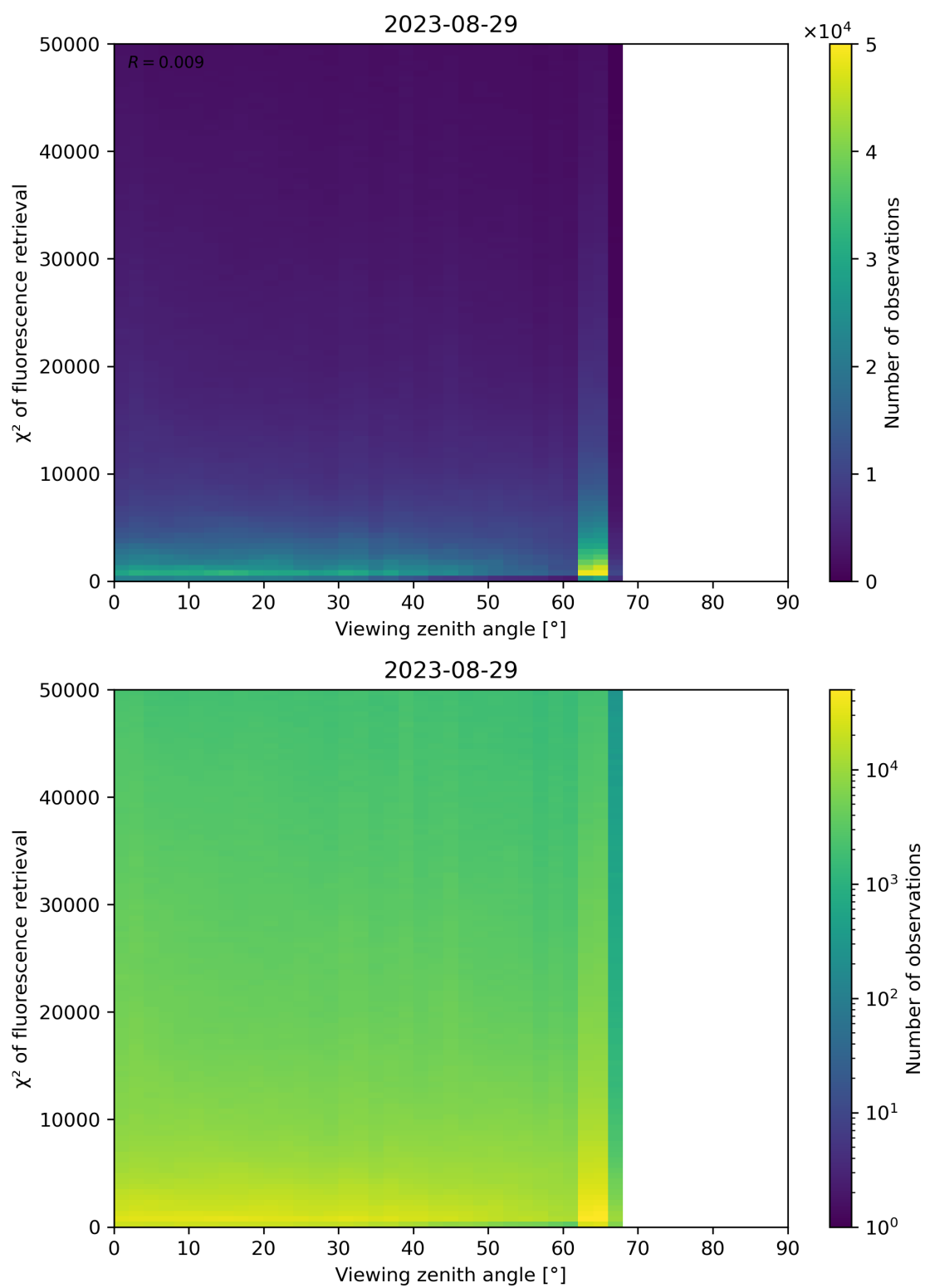
Figure 131: Scatter density plot of “Viewing zenith angle” against “ \chi^2 of fluorescence retrieval” for 2023-08-28 to 2023-08-30.
