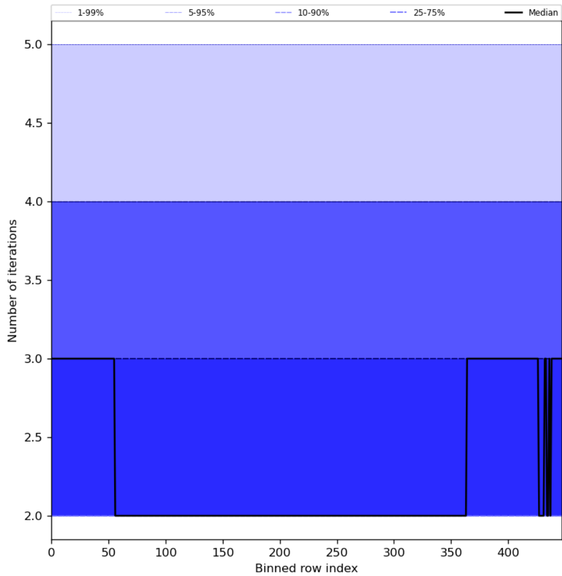
Figure 56: Along track statistics of “Number of iterations” for 2023-08-28 to 2023-08-30
