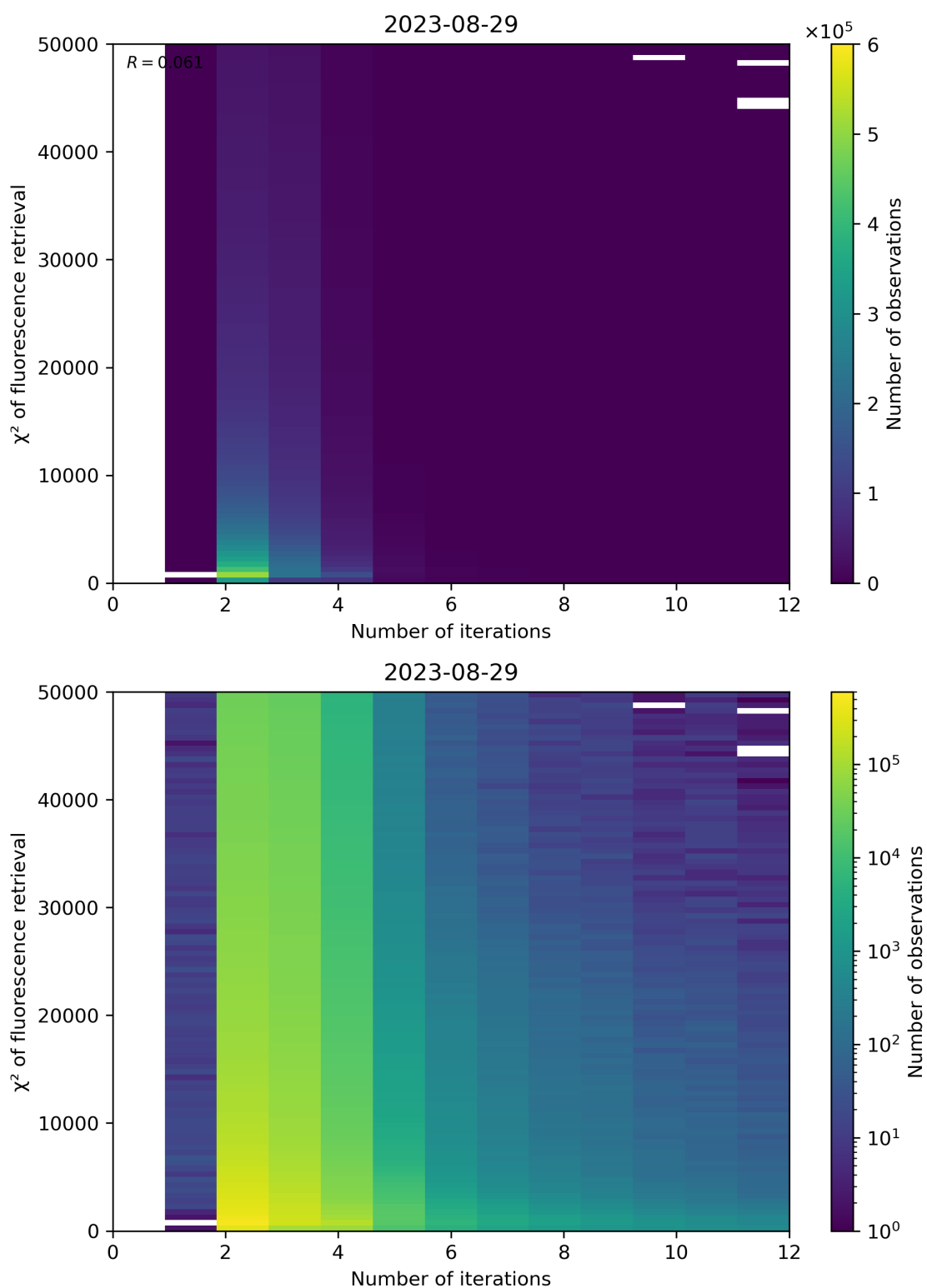
Figure 106: Scatter density plot of “Number of iterations” against “ \chi^2 of fluorescence retrieval” for 2023-08-28 to 2023-08-30.
