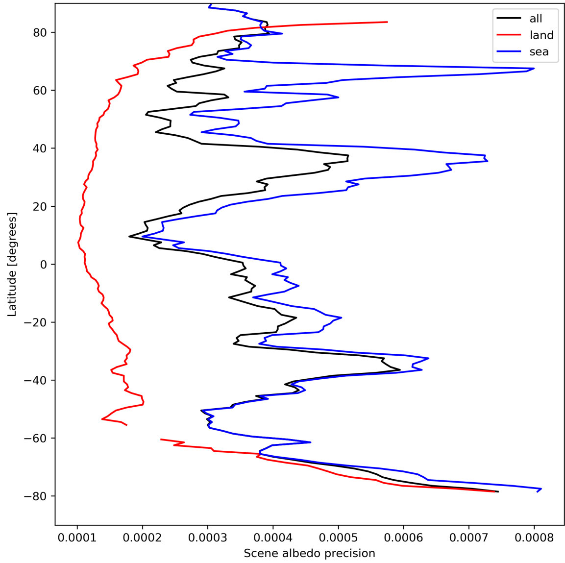
Figure 18: Zonal average of “Scene albedo precision” for 2023-08-28 to 2023-08-30.
