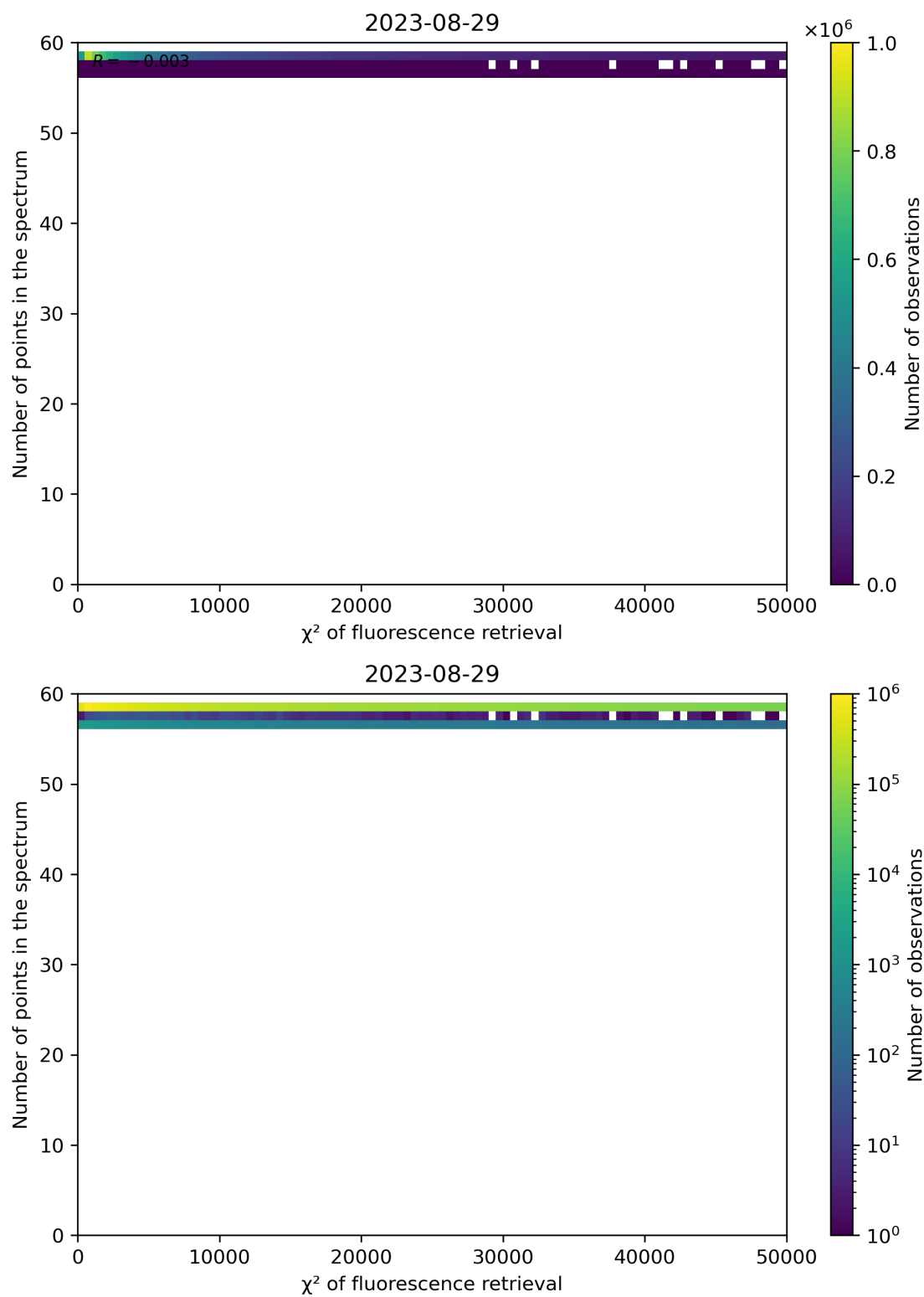
Figure 71: Scatter density plot of “ \chi^2 of fluorescence retrieval” against “Number of points in the spectrum” for 2023-08-28 to 2023-08-30.
