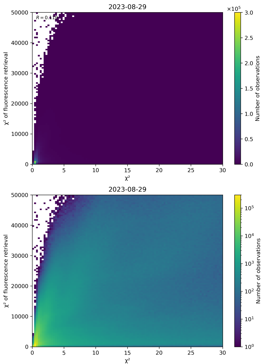
Figure 69: Scatter density plot of “ \chi^2 ” against “ \chi^2 of fluorescence retrieval” for 2023-08-28 to 2023-08-30.
