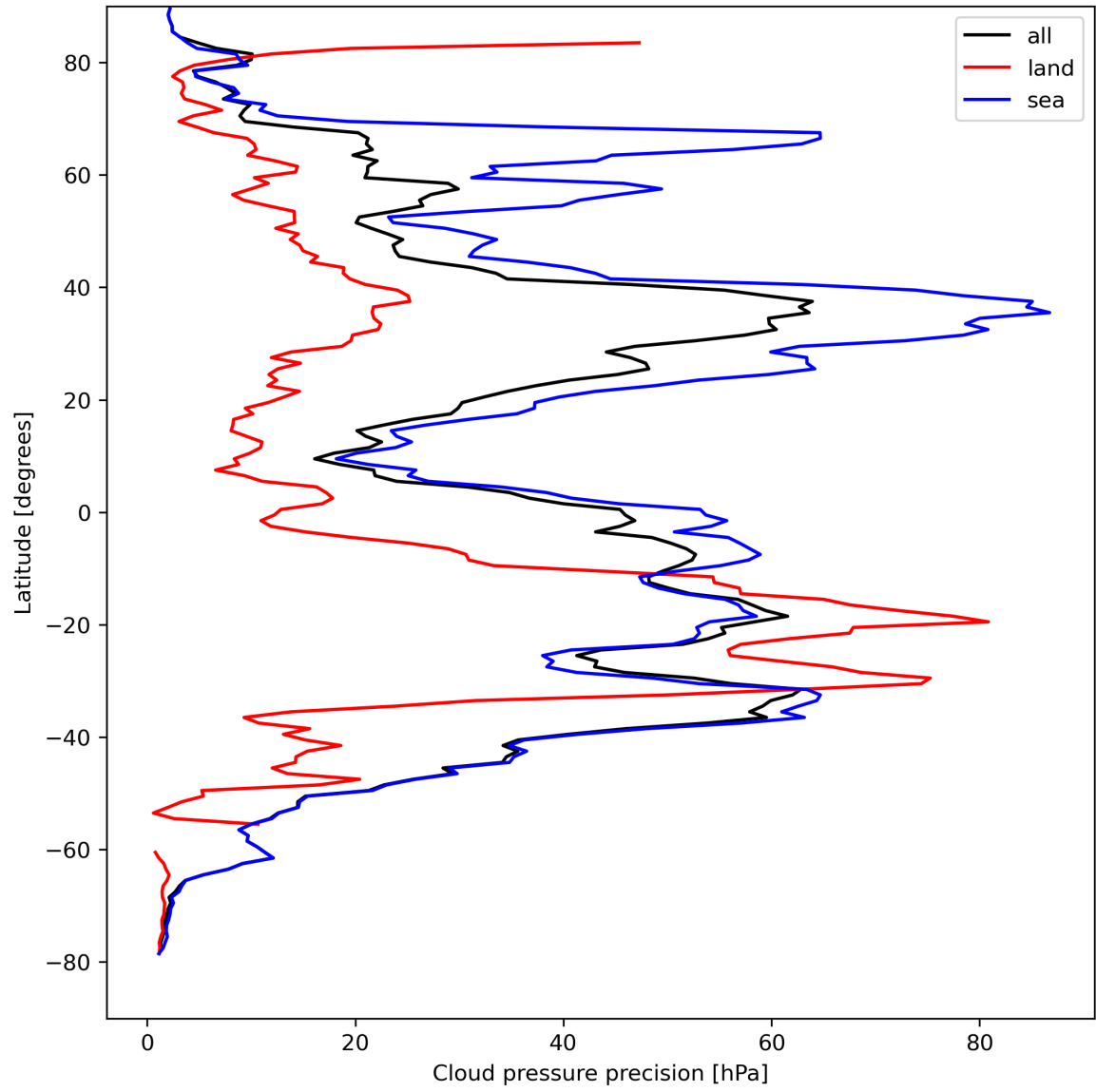
Figure 14: Zonal average of “Cloud pressure precision” for 2023-08-28 to 2023-08-30.
