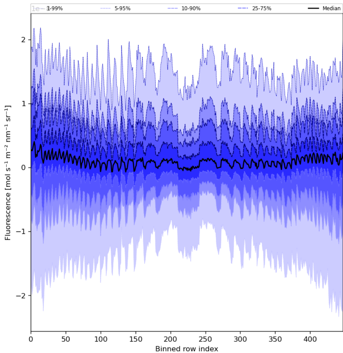
Figure 57: Along track statistics of “Fluorescence” for 2023-08-28 to 2023-08-30
