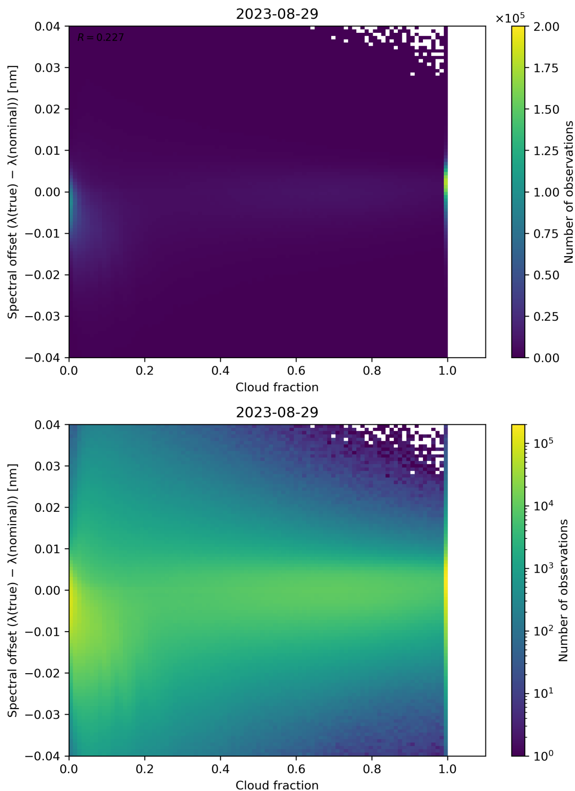
Figure 83: Scatter density plot of “Cloud fraction” against “Spectral offset ( \lambda(\text{true}) - \lambda(\text{nominal}) )” for 2023-08-28 to 2023-08-30.
