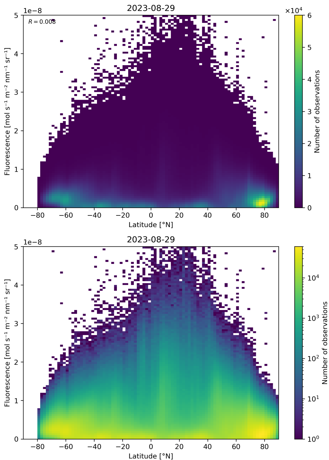
Figure 101: Scatter density plot of “Latitude” against “Fluorescence” for 2023-08-28 to 2023-08-30.
