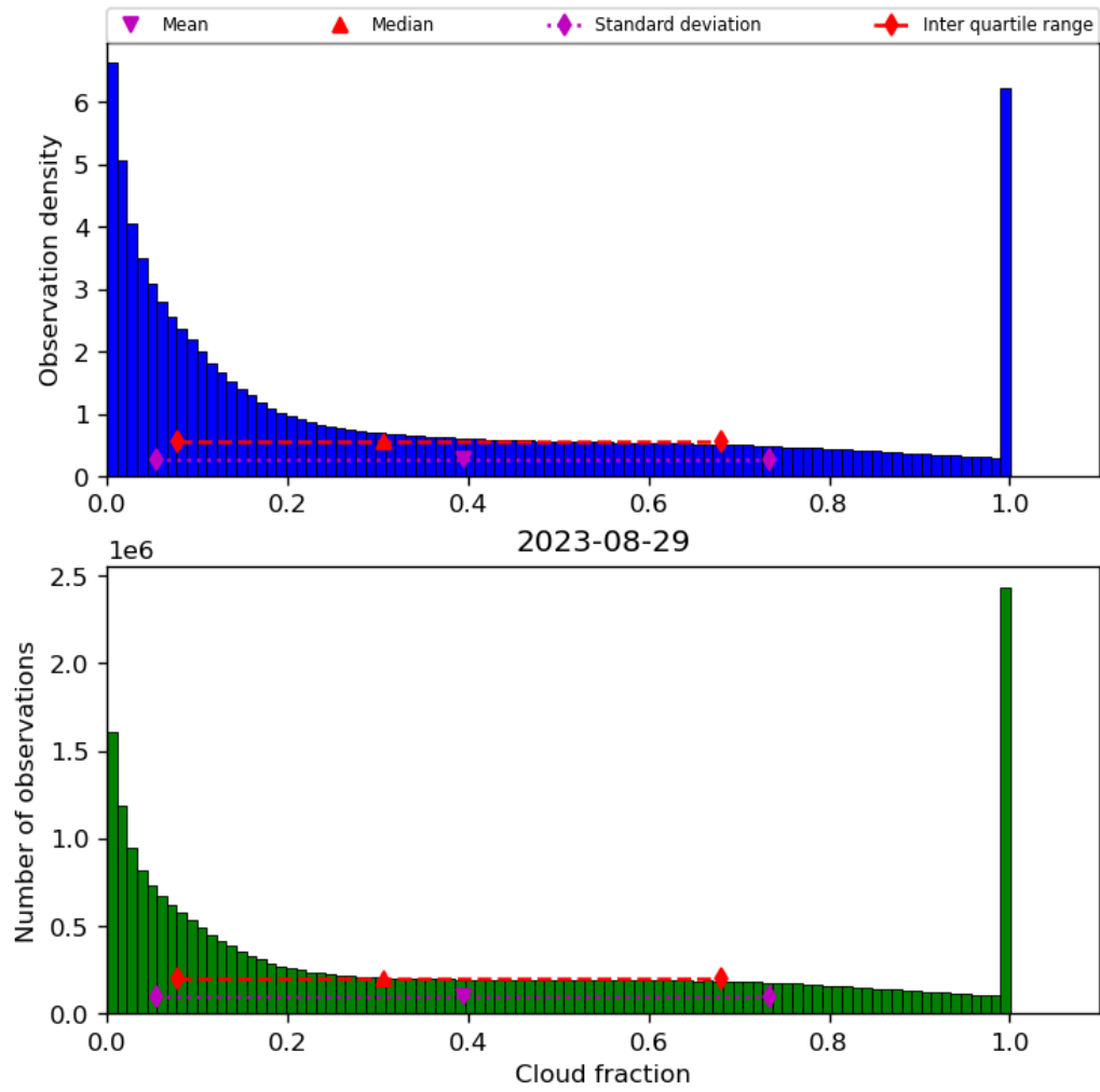
Figure 32: Histogram of “Cloud fraction” for 2023-08-28 to 2023-08-30
