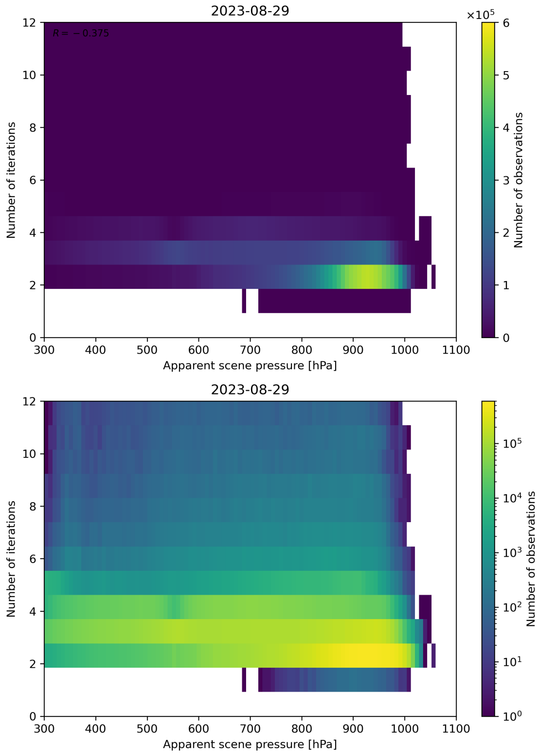
Figure 66: Scatter density plot of “Apparent scene pressure” against “Number of iterations” for 2023-08-28 to 2023-08-30.
