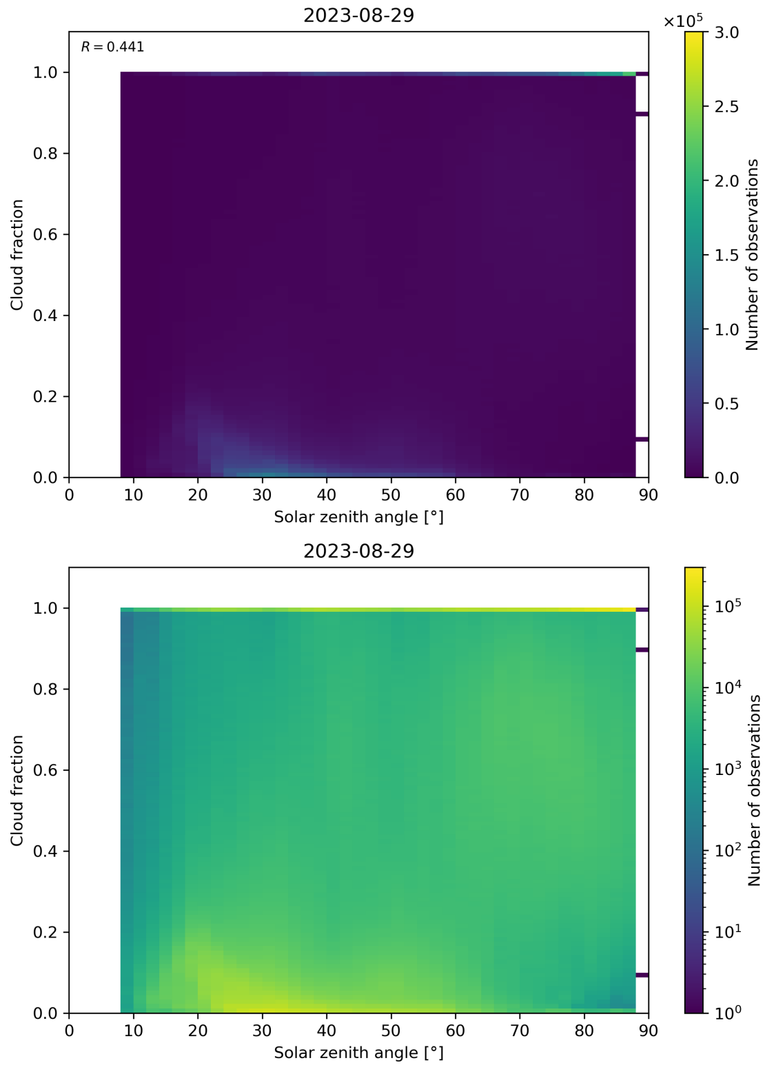
Figure 121: Scatter density plot of “Solar zenith angle” against “Cloud fraction” for 2023-08-28 to 2023-08-30.
