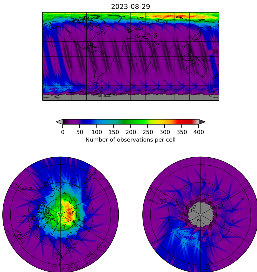
Figure 11: Map of the number of observations for 2023-08-28 to 2023-08-30
