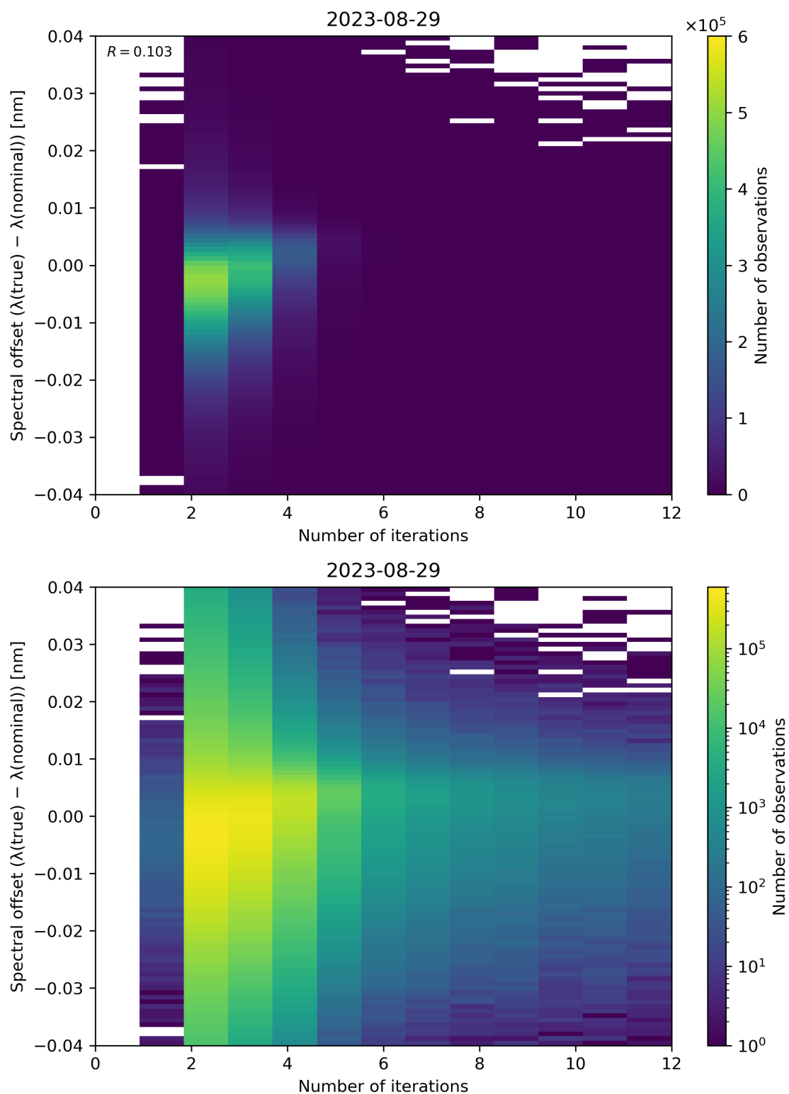
Figure 109: Scatter density plot of “Number of iterations” against “Spectral offset ( \lambda(\text{true}) - \lambda(\text{nominal}) )” for 2023-08-28 to 2023-08-30.
