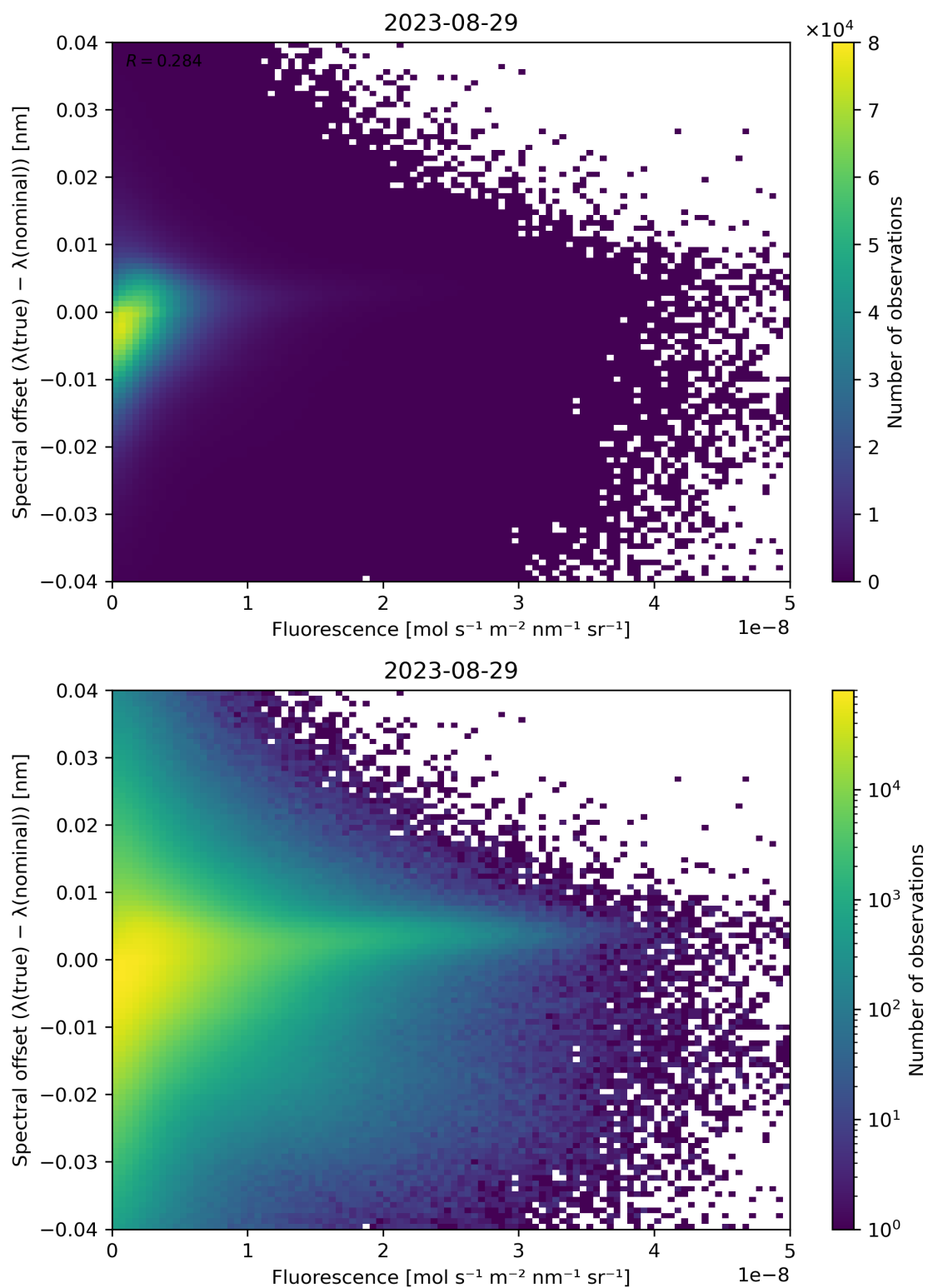
Figure 95: Scatter density plot of “Fluorescence” against “Spectral offset ( \lambda(\text{true}) - \lambda(\text{nominal}) )” for 2023-08-28 to 2023-08-30.
