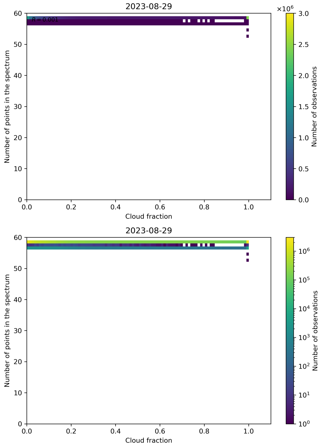
Figure 81: Scatter density plot of “Cloud fraction” against “Number of points in the spectrum” for 2023-08-28 to 2023-08-30.
