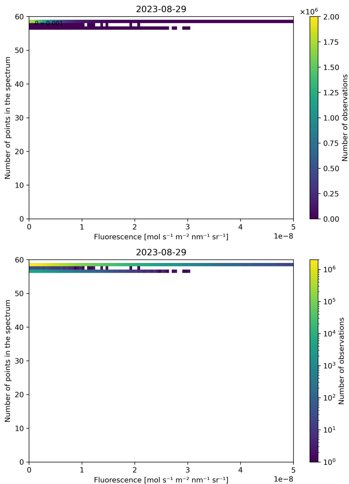
Figure 94: Scatter density plot of “Fluorescence” against “Number of points in the spectrum” for 2023-08-28 to 2023-08-30.
