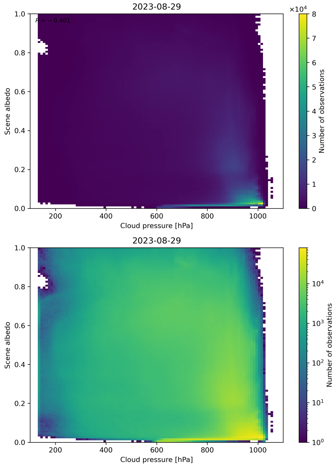
Figure 91: Scatter density plot of “Cloud pressure” against “Scene albedo” for 2023-08-28 to 2023-08-30.
