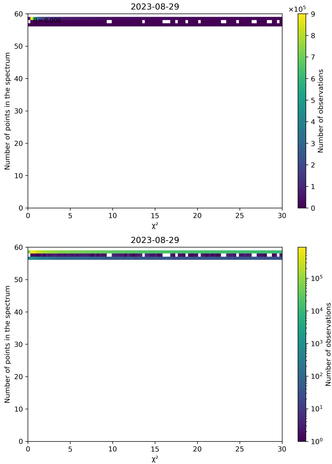
Figure 74: Scatter density plot of " \chi^2 " against "Number of points in the spectrum" for 2023-08-28 to 2023-08-30.
