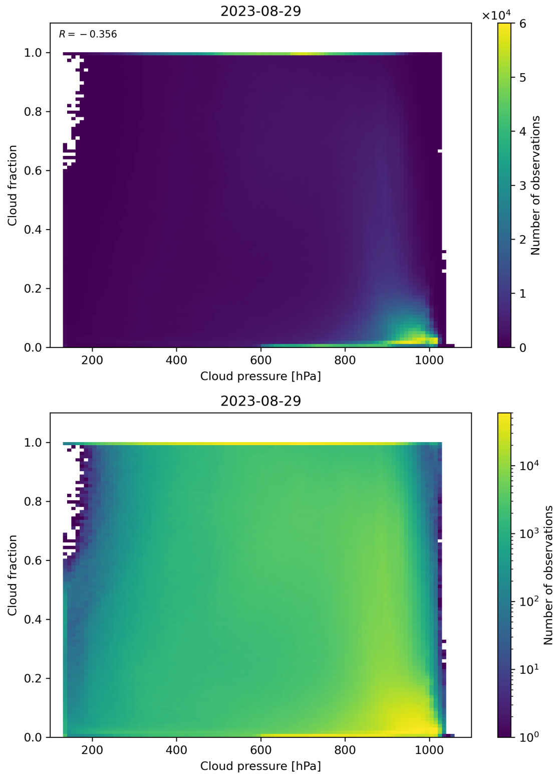
Figure 87: Scatter density plot of “Cloud pressure” against “Cloud fraction” for 2023-08-28 to 2023-08-30.
