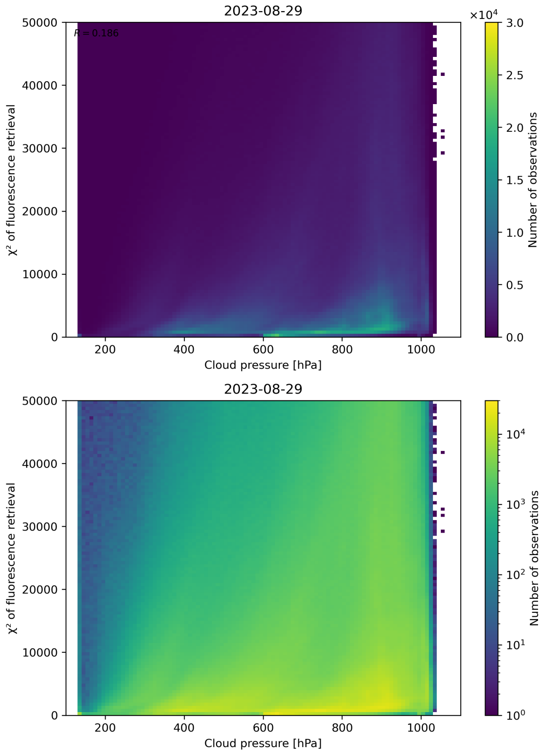
Figure 86: Scatter density plot of “Cloud pressure” against “ \chi^2 of fluorescence retrieval” for 2023-08-28 to 2023-08-30.
