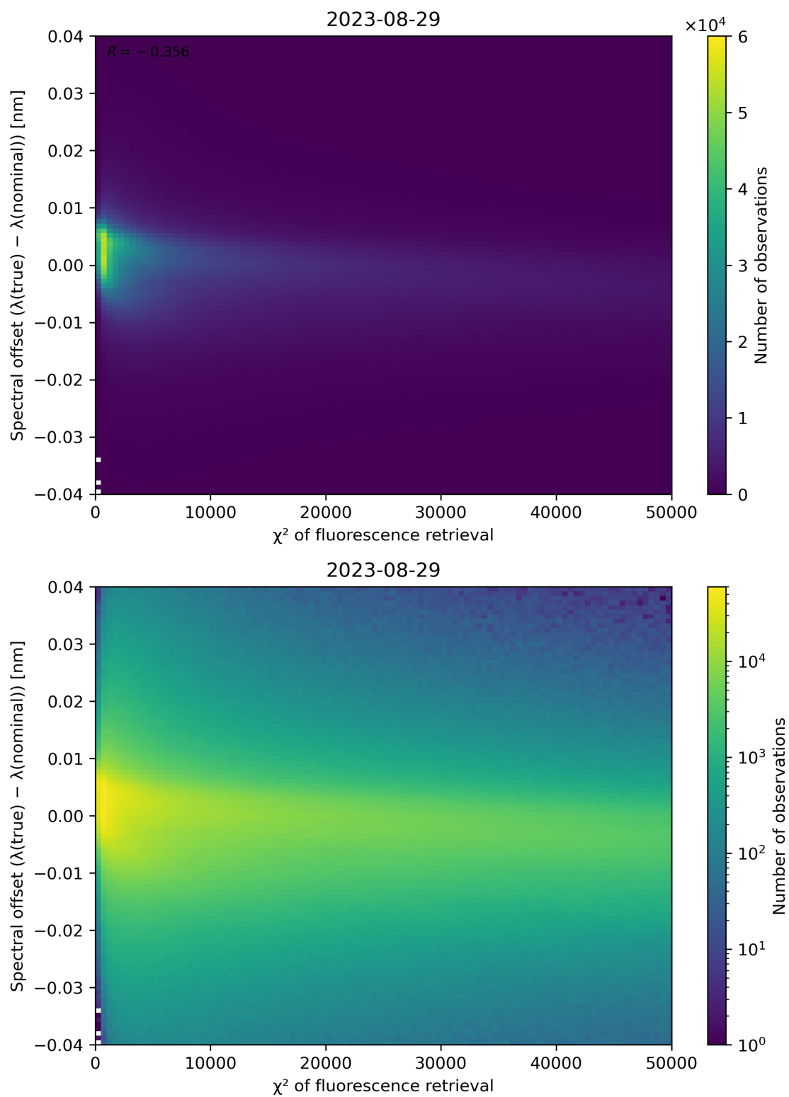
Figure 72: Scatter density plot of " \chi^2 of fluorescence retrieval" against "Spectral offset ( \lambda(\text{true}) - \lambda(\text{nominal})) " for 2023-08-28 to 2023-08-30.
