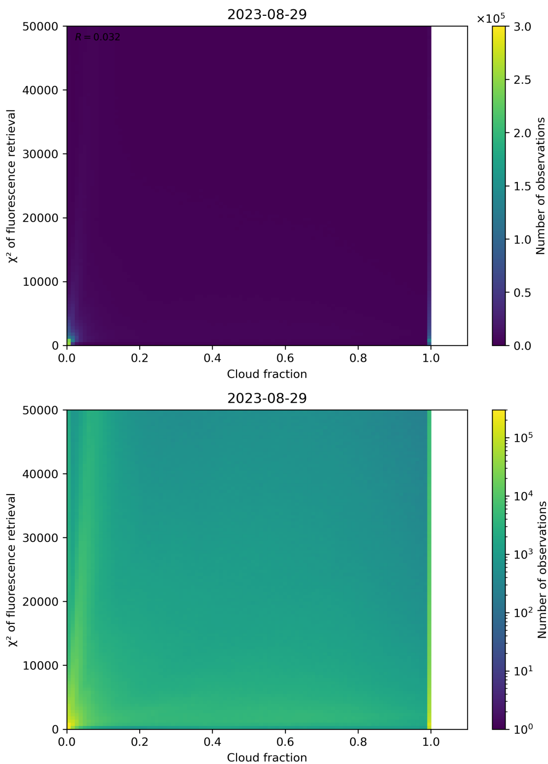
Figure 78: Scatter density plot of “Cloud fraction” against “ \chi^2 of fluorescence retrieval” for 2023-08-28 to 2023-08-30.
