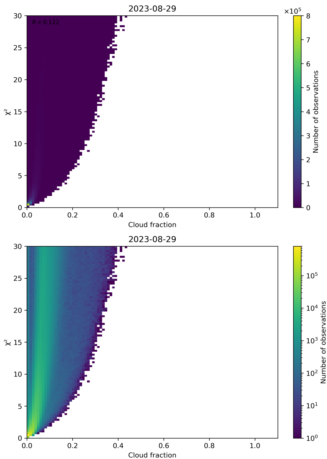
Figure 77: Scatter density plot of “Cloud fraction” against “ \chi^2 ” for 2023-08-28 to 2023-08-30.
