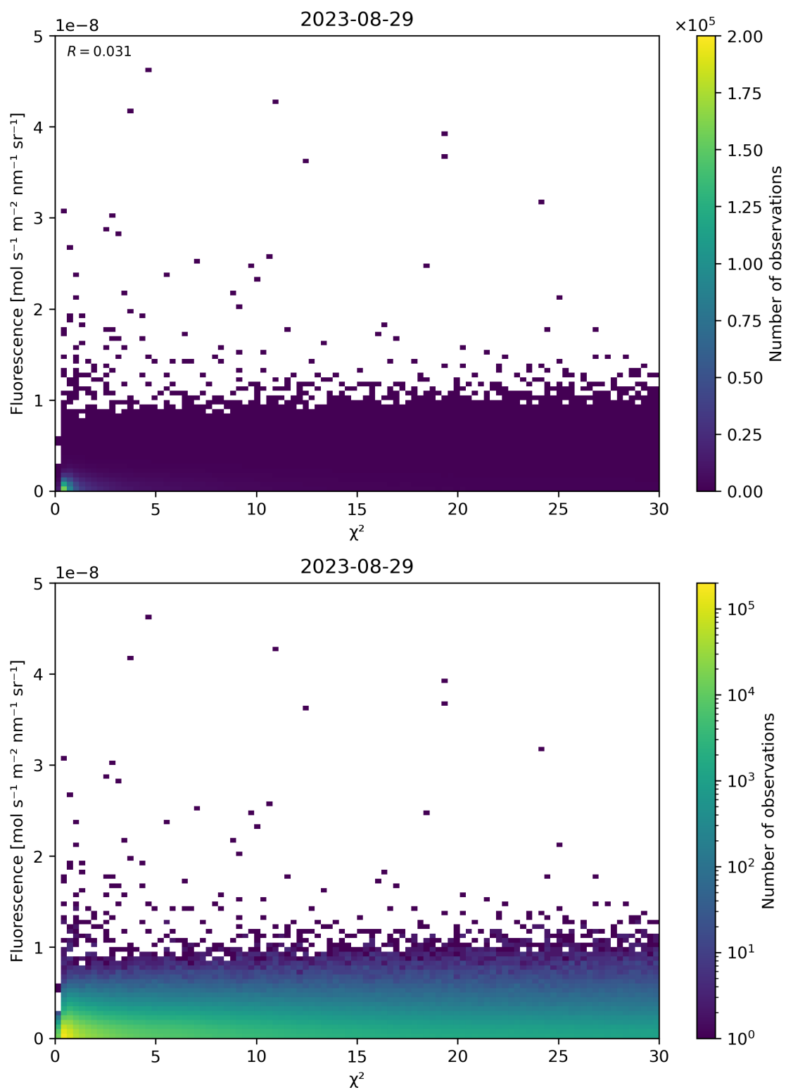
Figure 70: Scatter density plot of “ \chi^2 ” against “Fluorescence” for 2023-08-28 to 2023-08-30.
