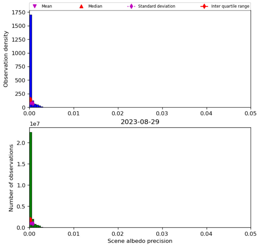
Figure 35: Histogram of “Scene albedo precision” for 2023-08-28 to 2023-08-30
