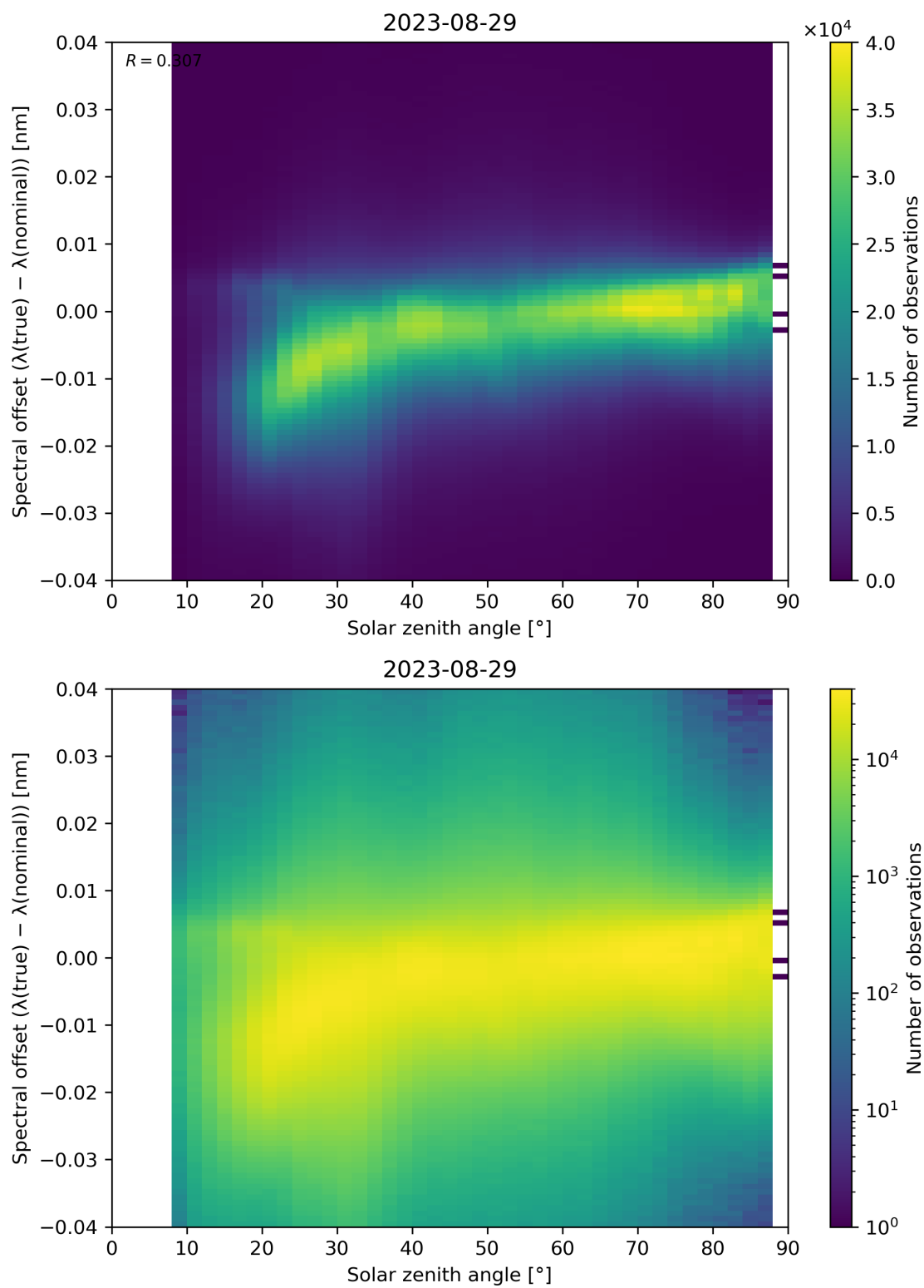
Figure 128: Scatter density plot of “Solar zenith angle” against “Spectral offset ( \lambda(\text{true}) - \lambda(\text{nominal}) )” for 2023-08-28 to 2023-08-30.
