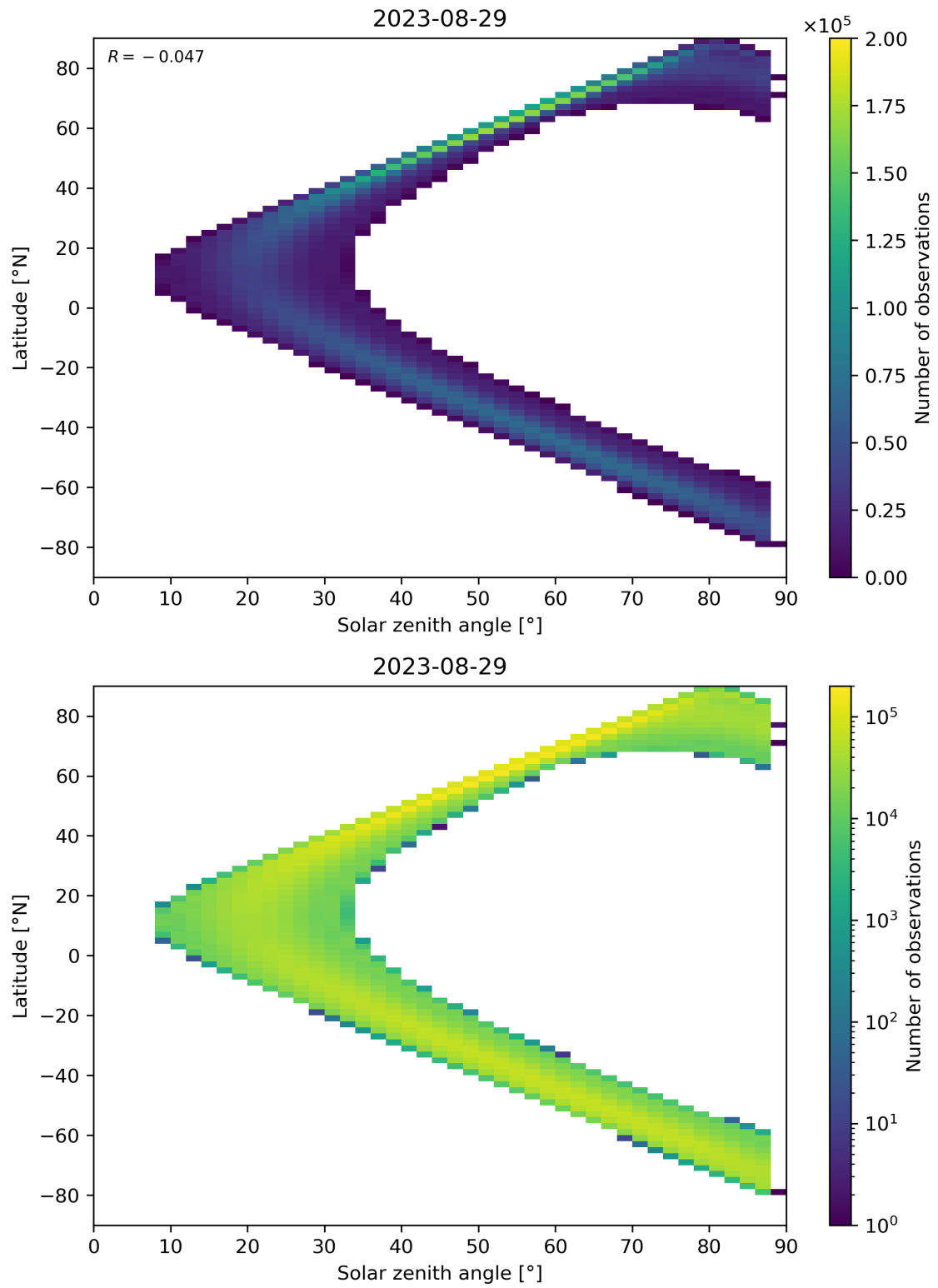
Figure 124: Scatter density plot of “Solar zenith angle” against “Latitude” for 2023-08-28 to 2023-08-30.
