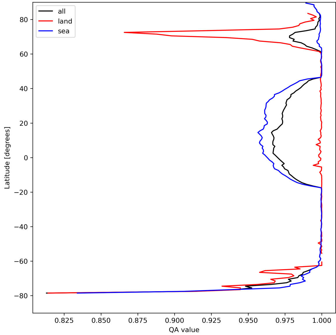
Figure 12: Zonal average of “QA value” for 2023-08-28 to 2023-08-30.
