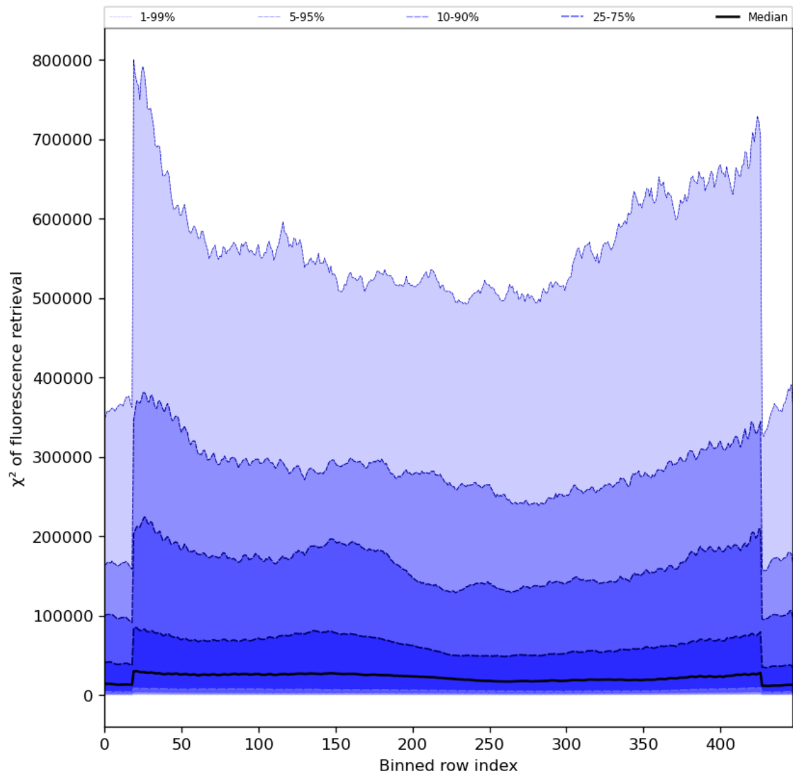
Figure 59: Along track statistics of “ \chi^2 of fluorescence retrieval” for 2023-08-28 to 2023-08-30
