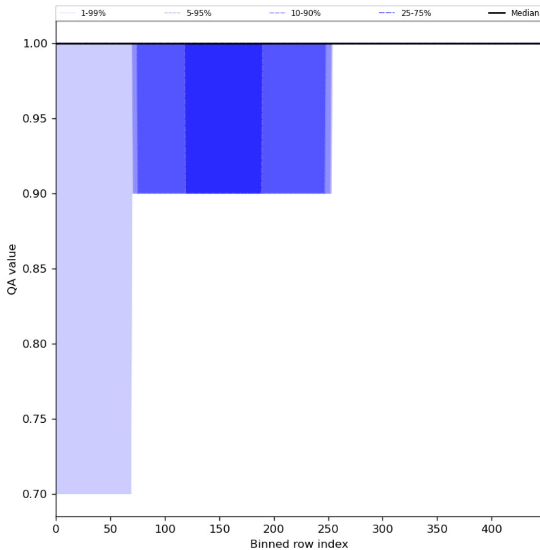
Figure 46: Along track statistics of “QA value” for 2023-08-28 to 2023-08-30
