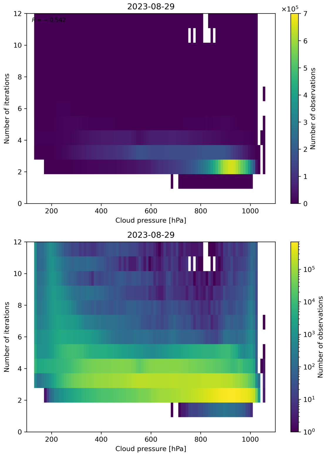
Figure 89: Scatter density plot of “Cloud pressure” against “Number of iterations” for 2023-08-28 to 2023-08-30.
