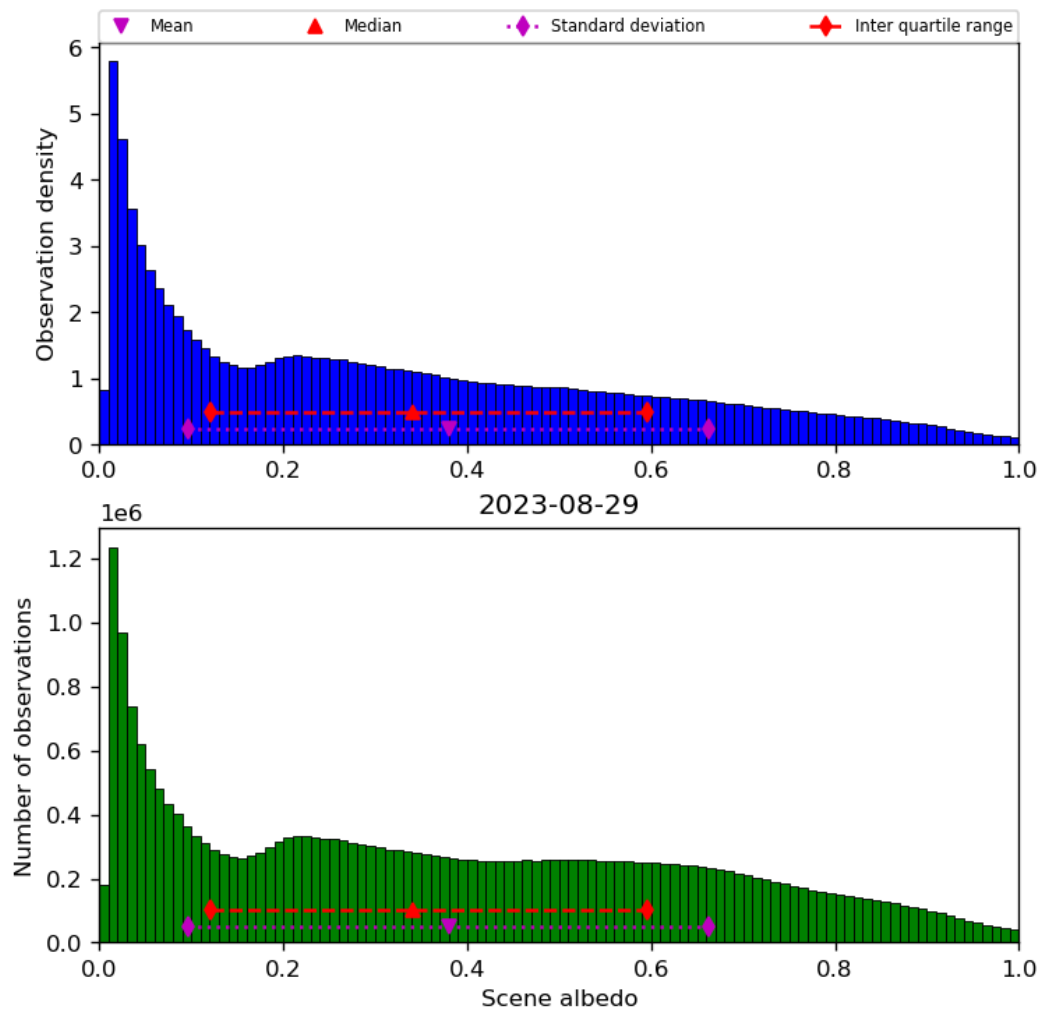
Figure 34: Histogram of “Scene albedo” for 2023-08-28 to 2023-08-30
