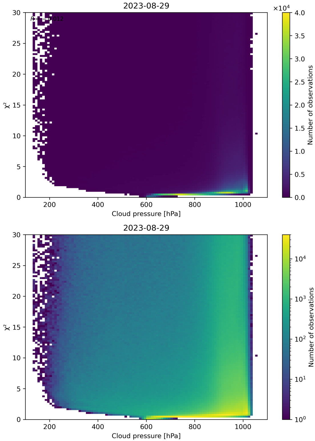
Figure 85: Scatter density plot of “Cloud pressure” against “ \chi^2 ” for 2023-08-28 to 2023-08-30.
