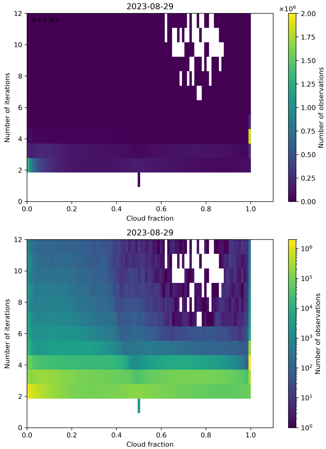
Figure 80: Scatter density plot of “Cloud fraction” against “Number of iterations” for 2023-08-28 to 2023-08-30.
