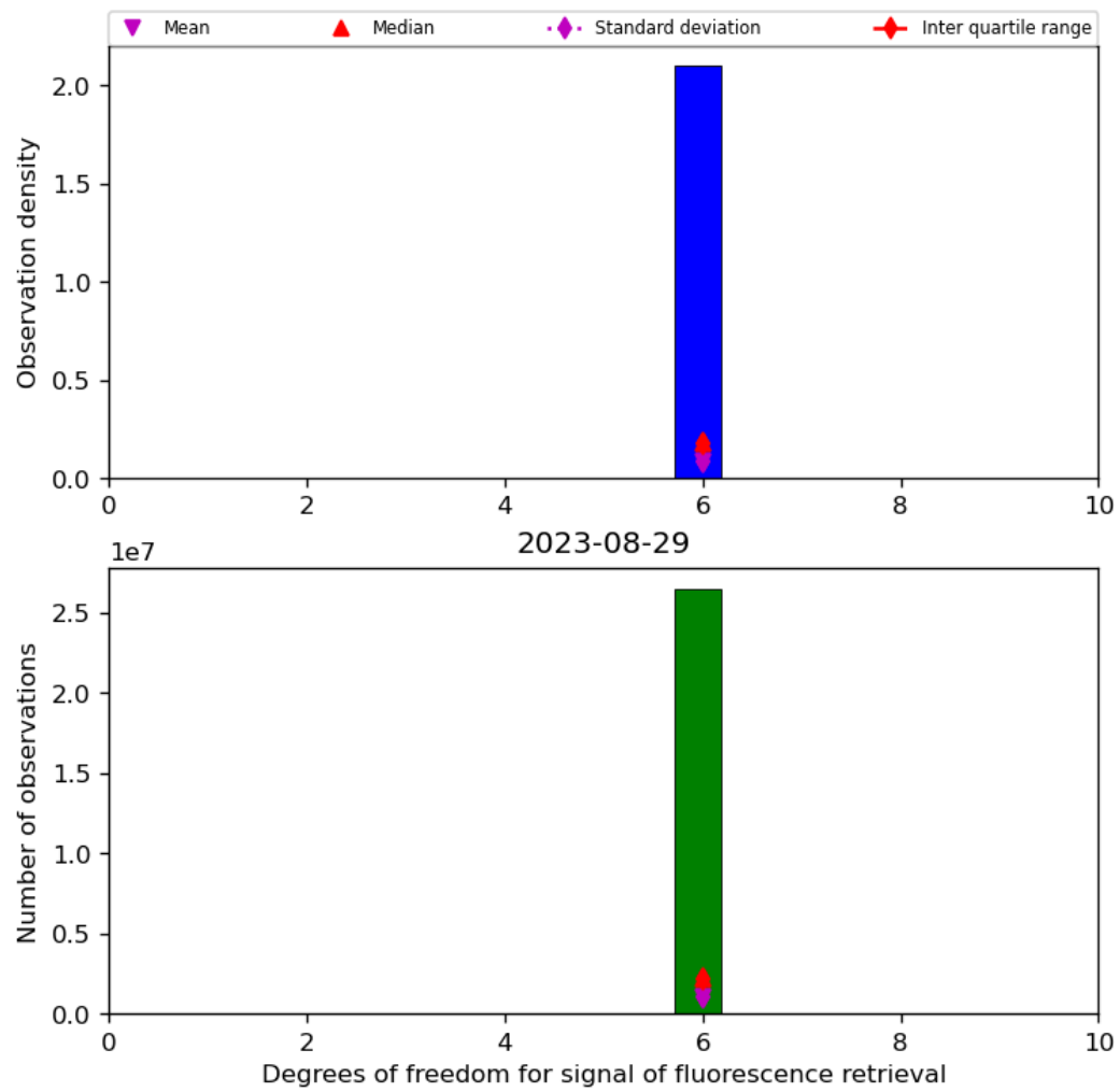
Figure 43: Histogram of “Degrees of freedom for signal of fluorescence retrieval” for 2023-08-28 to 2023-08-30
