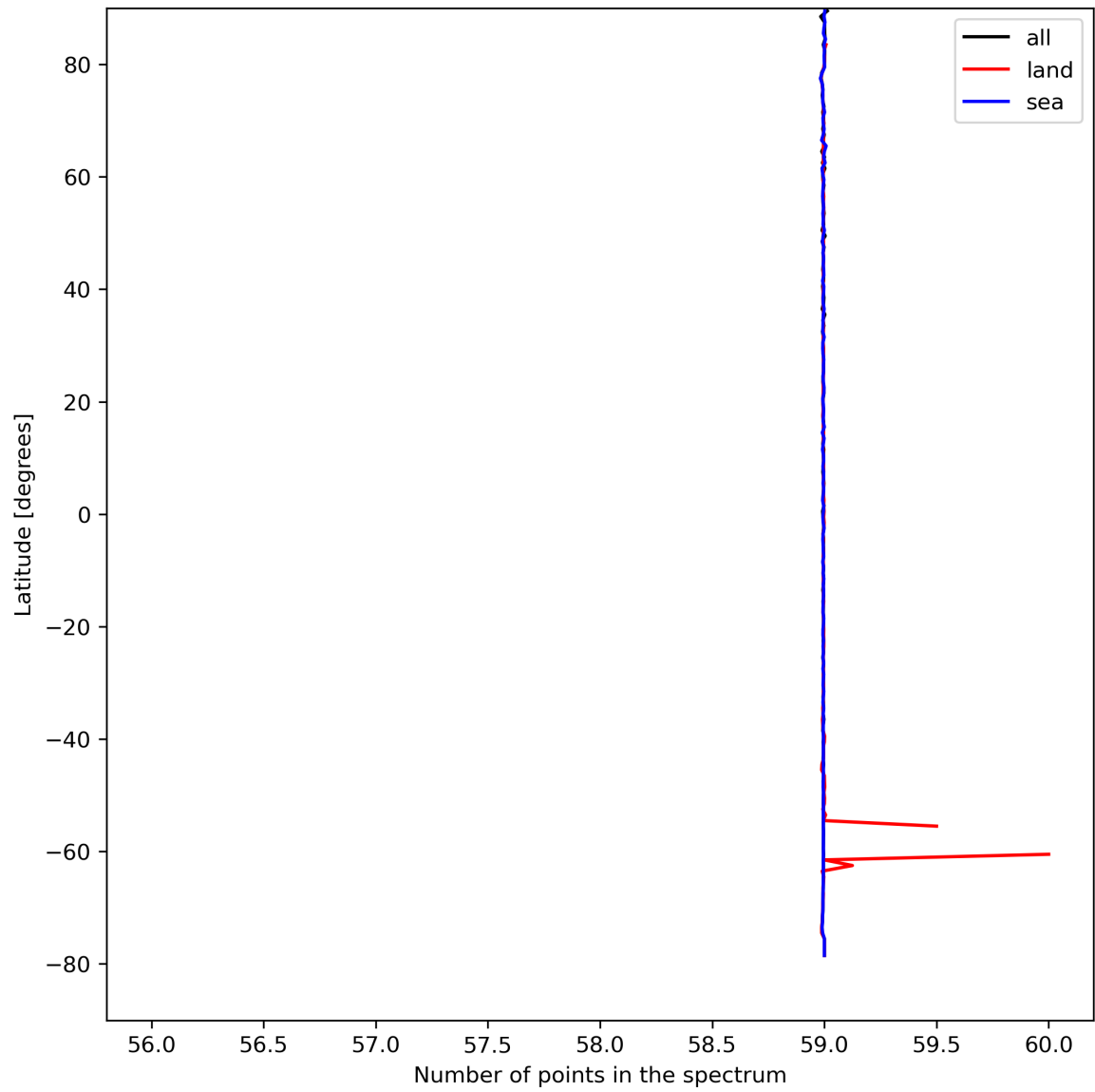
Figure 27: Zonal average of “Number of points in the spectrum” for 2023-08-28 to 2023-08-30.
