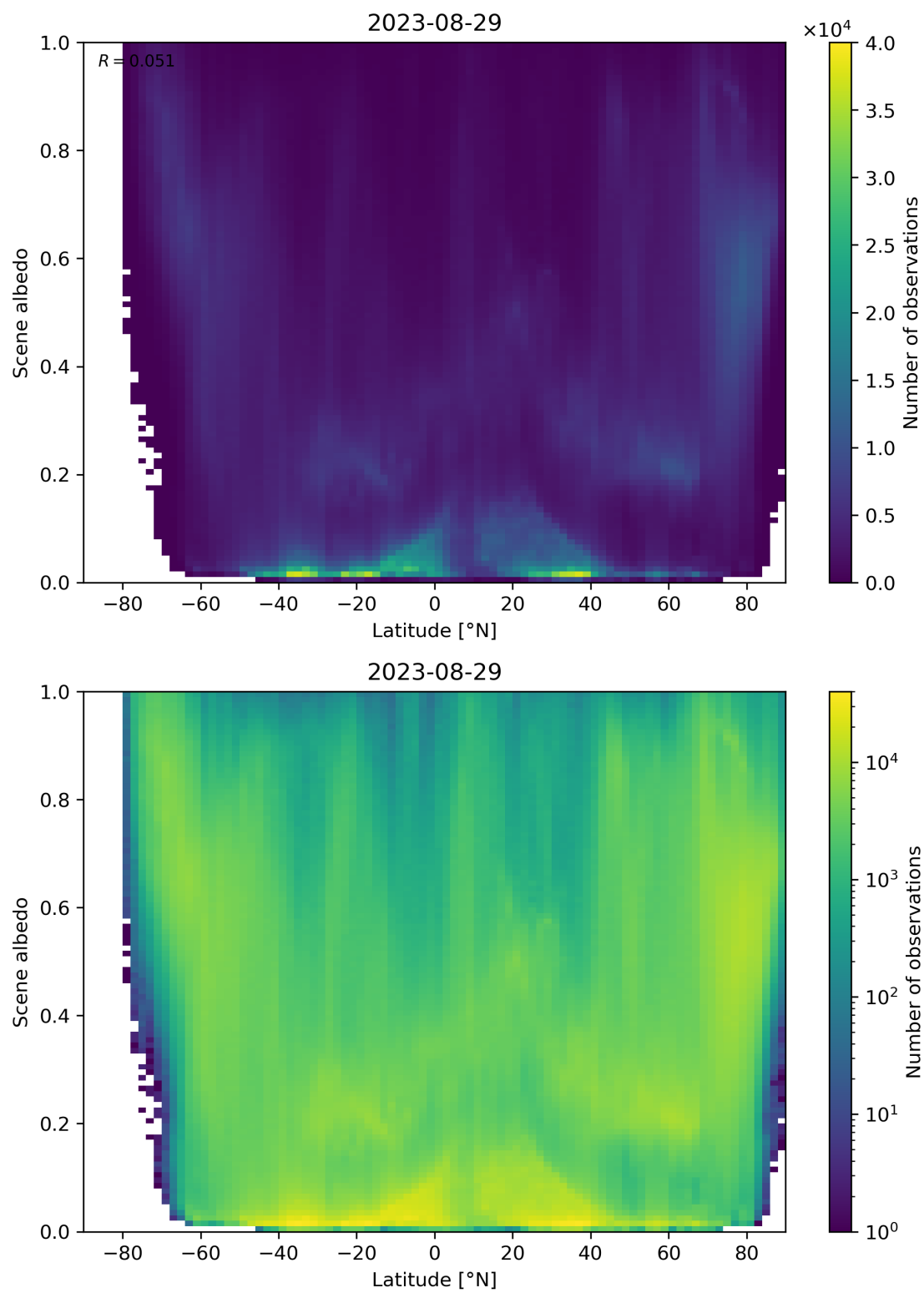
Figure 104: Scatter density plot of “Latitude” against “Scene albedo” for 2023-08-28 to 2023-08-30.
