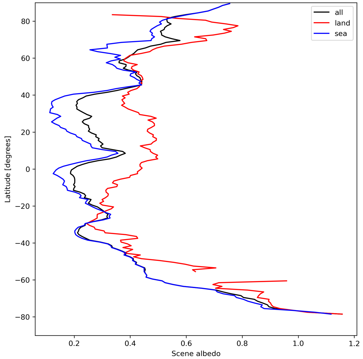
Figure 17: Zonal average of “Scene albedo” for 2023-08-28 to 2023-08-30.
