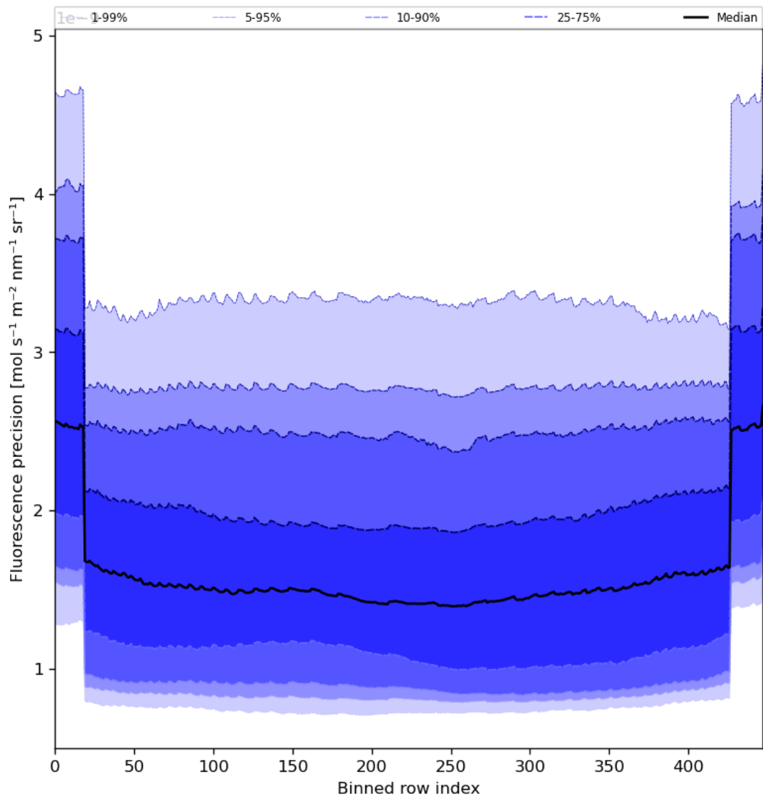
Figure 58: Along track statistics of “Fluorescence precision” for 2023-08-28 to 2023-08-30
