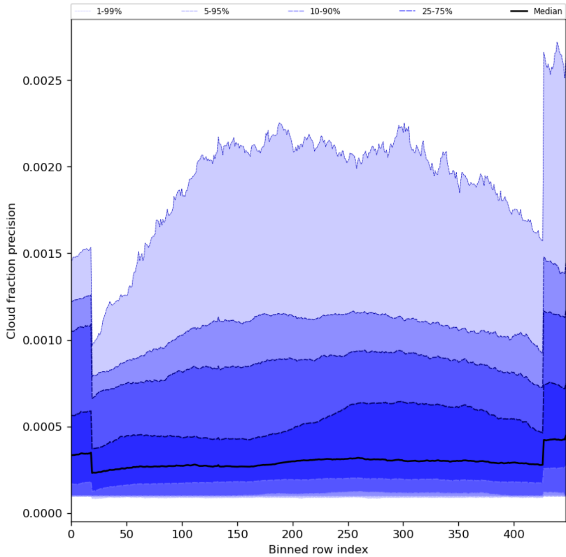
Figure 50: Along track statistics of “Cloud fraction precision” for 2023-08-28 to 2023-08-30
