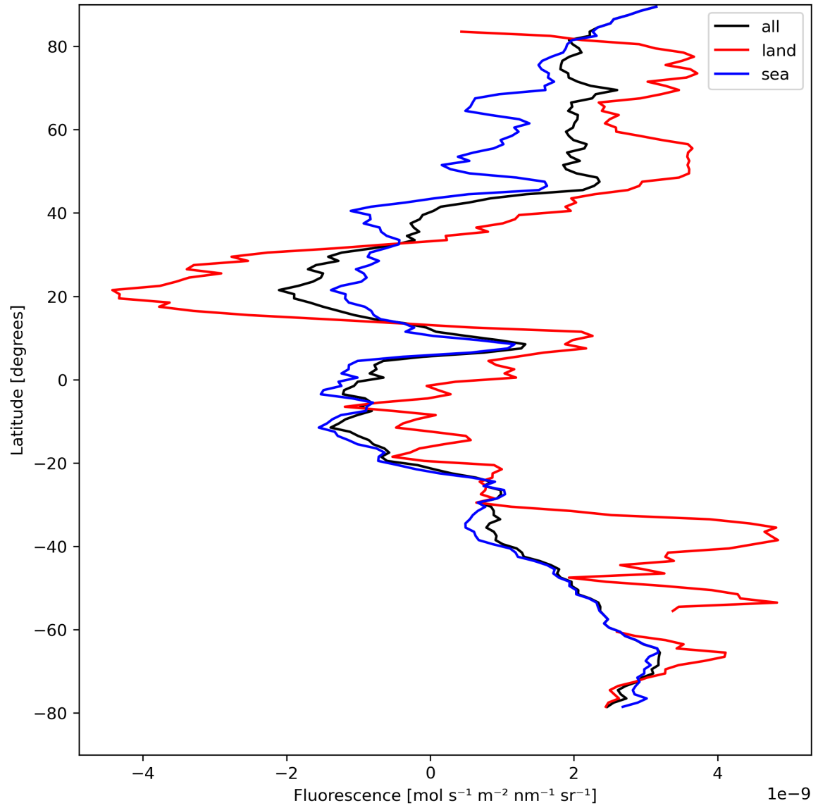
Figure 23: Zonal average of “Fluorescence” for 2023-08-28 to 2023-08-30.
