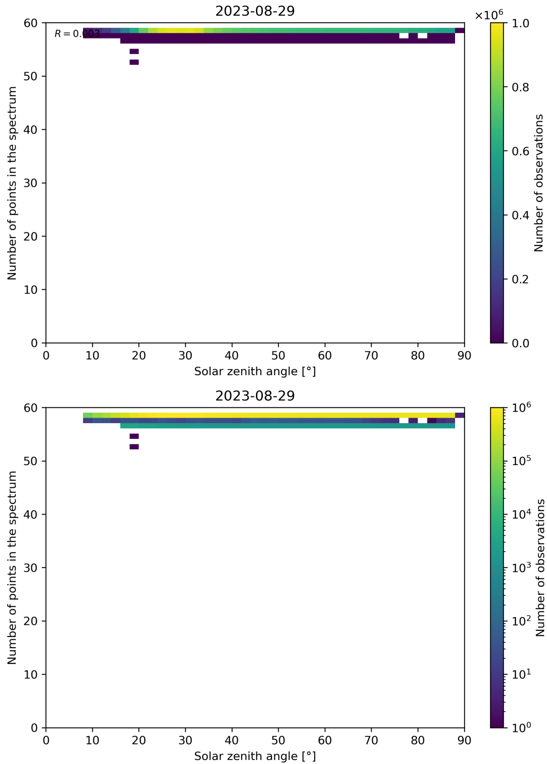
Figure 126: Scatter density plot of “Solar zenith angle” against “Number of points in the spectrum” for 2023-08-28 to 2023-08-30.
