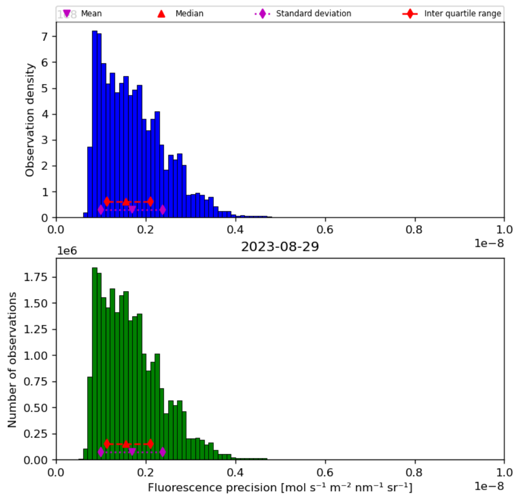
Figure 41: Histogram of “Fluorescence precision” for 2023-08-28 to 2023-08-30
