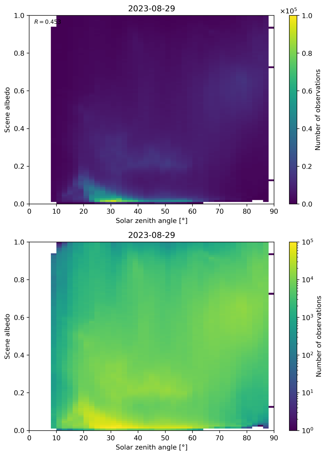
Figure 127: Scatter density plot of “Solar zenith angle” against “Scene albedo” for 2023-08-28 to 2023-08-30.
