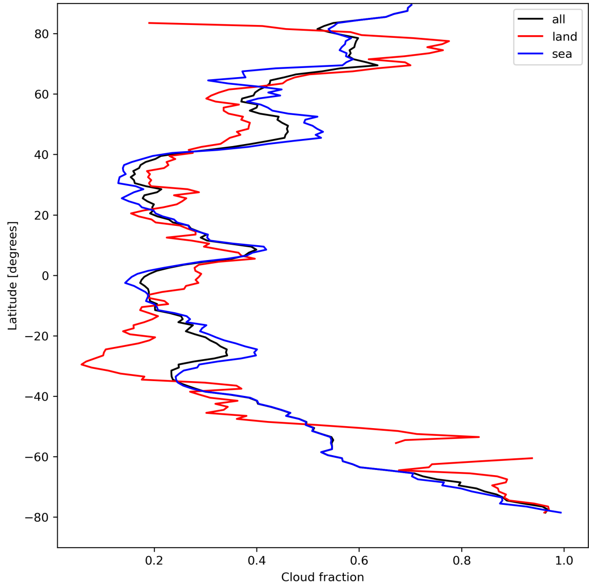
Figure 15: Zonal average of “Cloud fraction” for 2023-08-28 to 2023-08-30.
