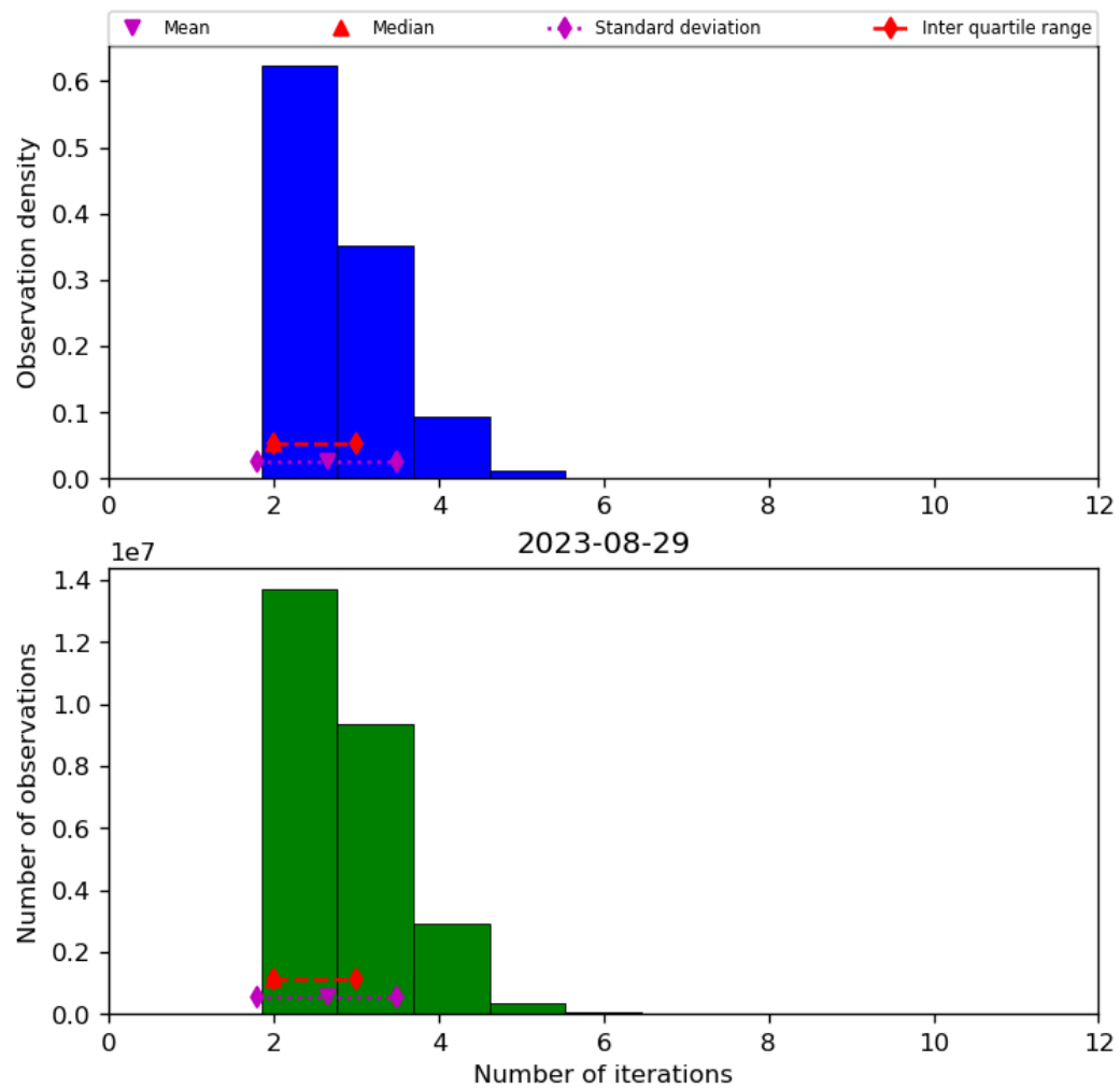
Figure 39: Histogram of “Number of iterations” for 2023-08-28 to 2023-08-30
