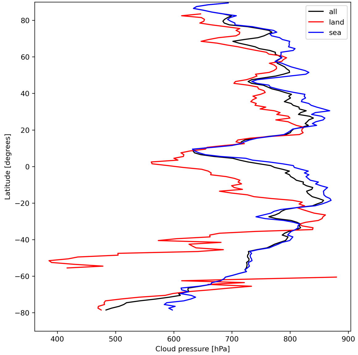
Figure 13: Zonal average of “Cloud pressure” for 2023-08-28 to 2023-08-30.
