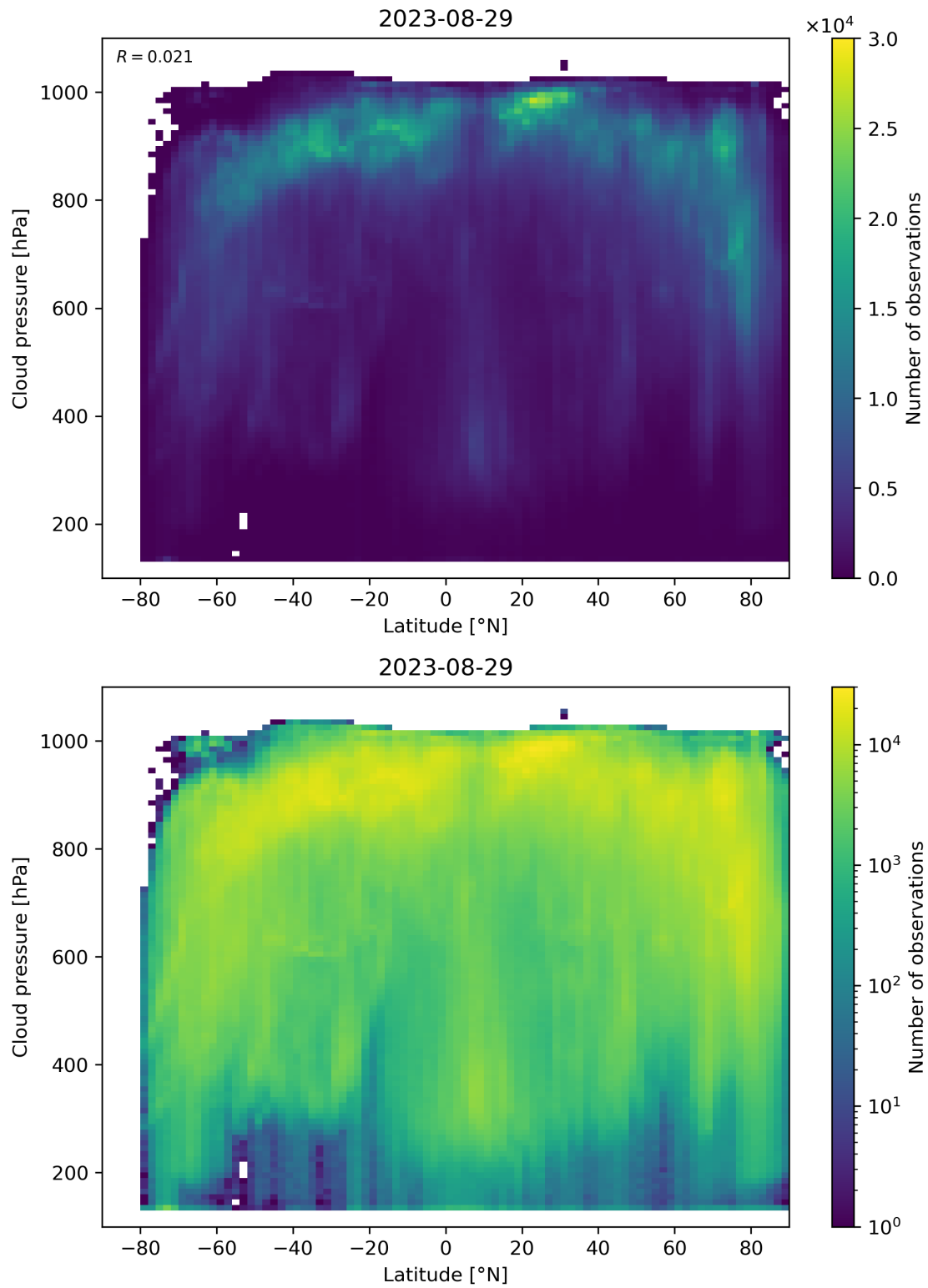
Figure 100: Scatter density plot of “Latitude” against “Cloud pressure” for 2023-08-28 to 2023-08-30.
