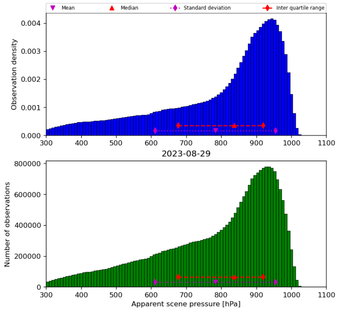
Figure 36: Histogram of “Apparent scene pressure” for 2023-08-28 to 2023-08-30
