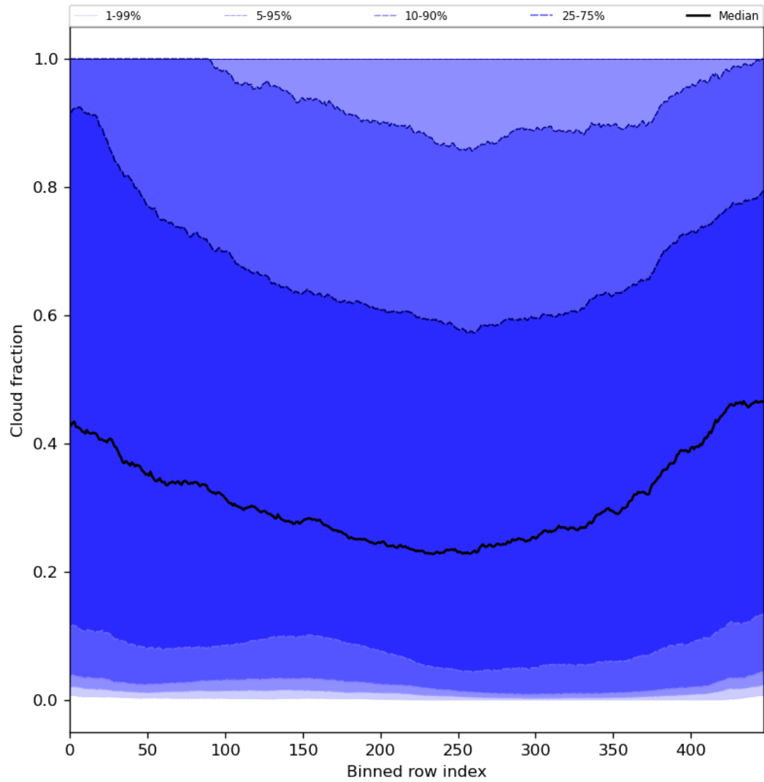
Figure 49: Along track statistics of “Cloud fraction” for 2023-08-28 to 2023-08-30
