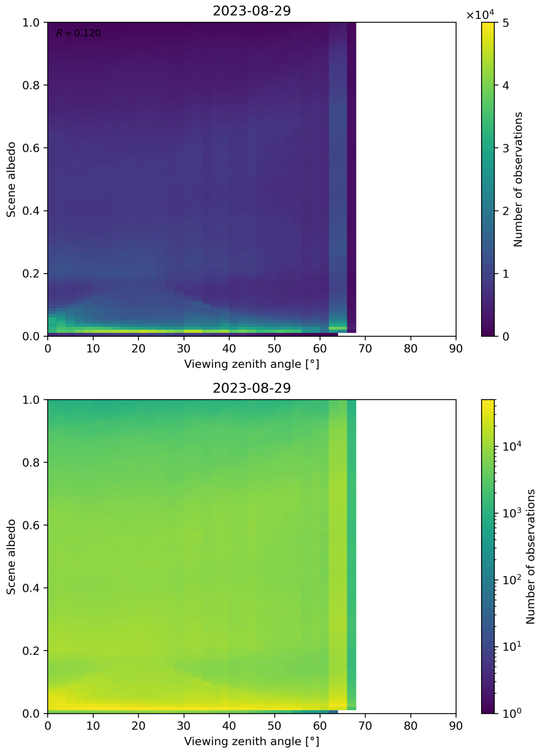
Figure 138: Scatter density plot of “Viewing zenith angle” against “Scene albedo” for 2023-08-28 to 2023-08-30.
