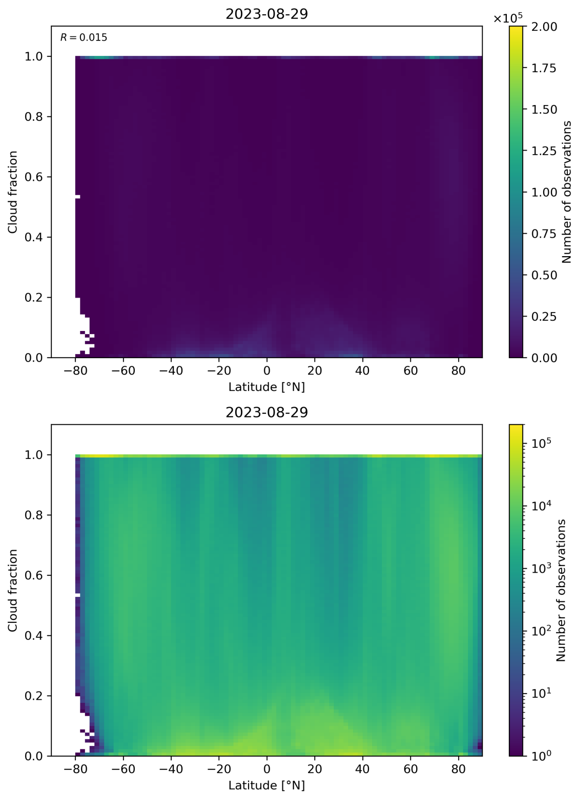
Figure 99: Scatter density plot of “Latitude” against “Cloud fraction” for 2023-08-28 to 2023-08-30.
