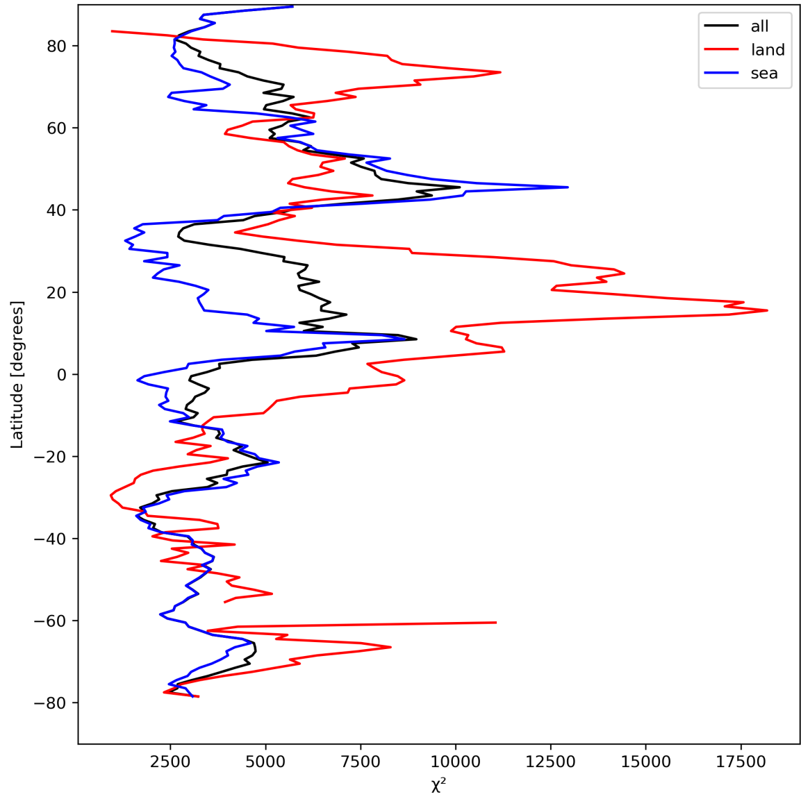
Figure 21: Zonal average of “ \chi^2 ” for 2023-08-28 to 2023-08-30.
