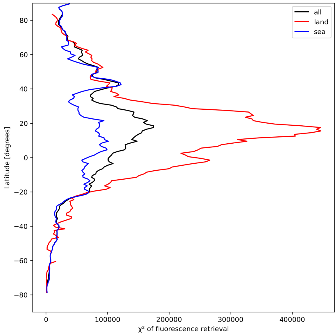
Figure 25: Zonal average of “ \chi^2 of fluorescence retrieval” for 2023-08-28 to 2023-08-30.
