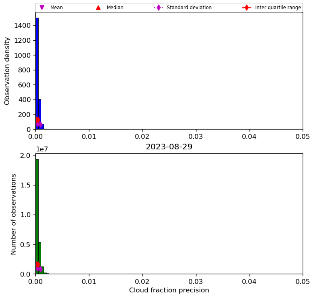
Figure 33: Histogram of “Cloud fraction precision” for 2023-08-28 to 2023-08-30
