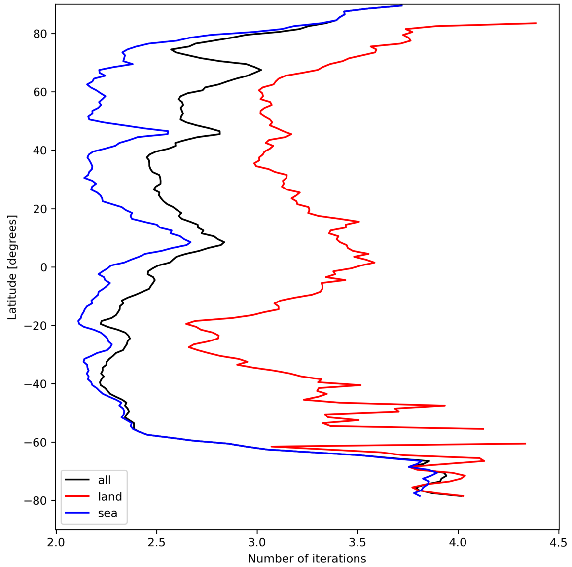
Figure 22: Zonal average of “Number of iterations” for 2023-08-28 to 2023-08-30.
