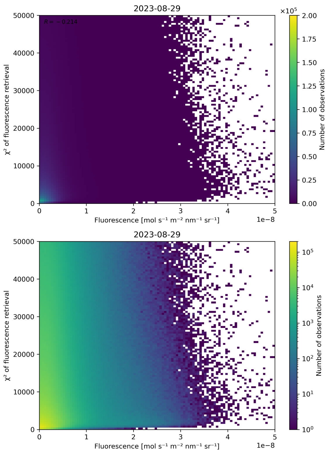
Figure 93: Scatter density plot of “Fluorescence” against “ \chi^2 of fluorescence retrieval” for 2023-08-28 to 2023-08-30.
