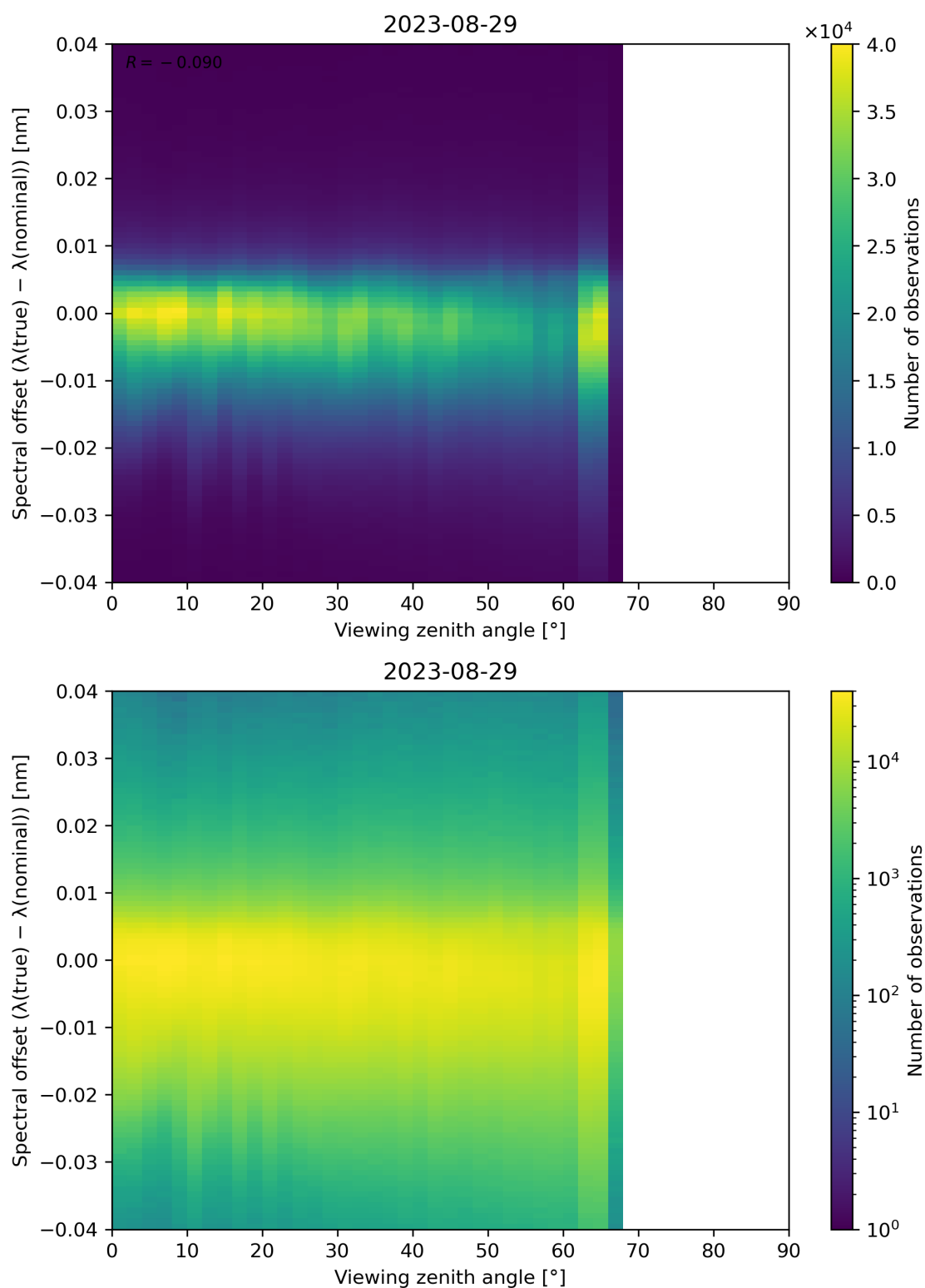
Figure 140: Scatter density plot of “Viewing zenith angle” against “Spectral offset ( \lambda(\text{true}) - \lambda(\text{nominal}) )” for 2023-08-28 to 2023-08-30.
