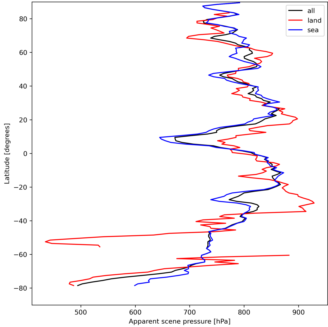
Figure 19: Zonal average of “Apparent scene pressure” for 2023-08-28 to 2023-08-30.
