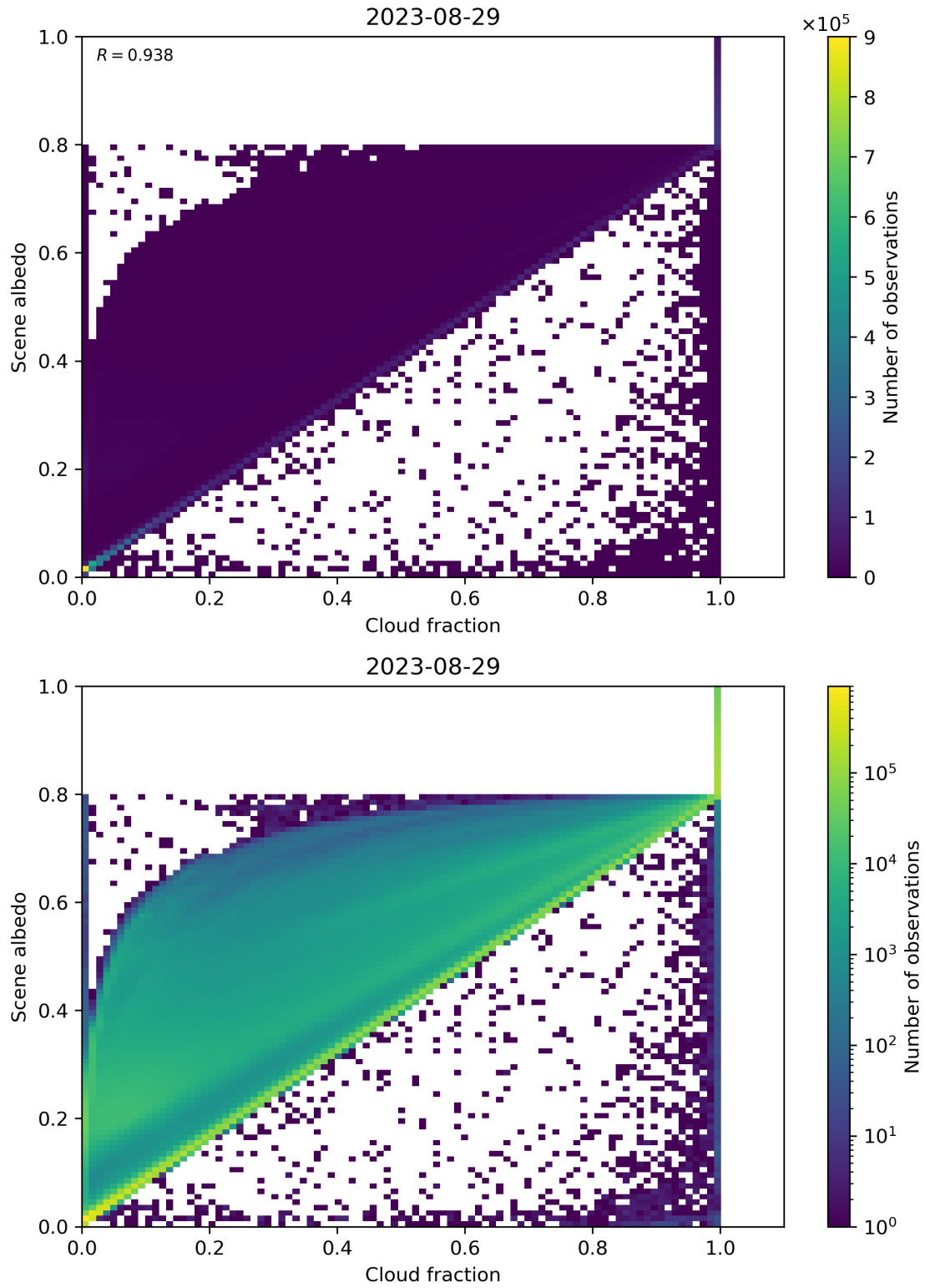
Figure 82: Scatter density plot of “Cloud fraction” against “Scene albedo” for 2023-08-28 to 2023-08-30.
