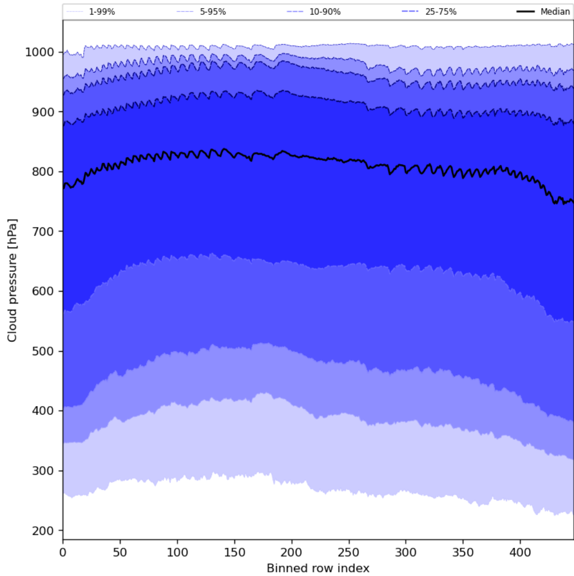
Figure 47: Along track statistics of “Cloud pressure” for 2023-08-28 to 2023-08-30
