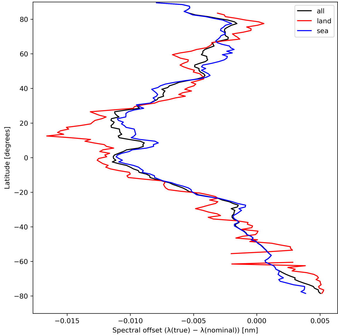
Figure 28: Zonal average of “Spectral offset ( \lambda(\text{true}) - \lambda(\text{nominal}) )” for 2023-08-28 to 2023-08-30.
