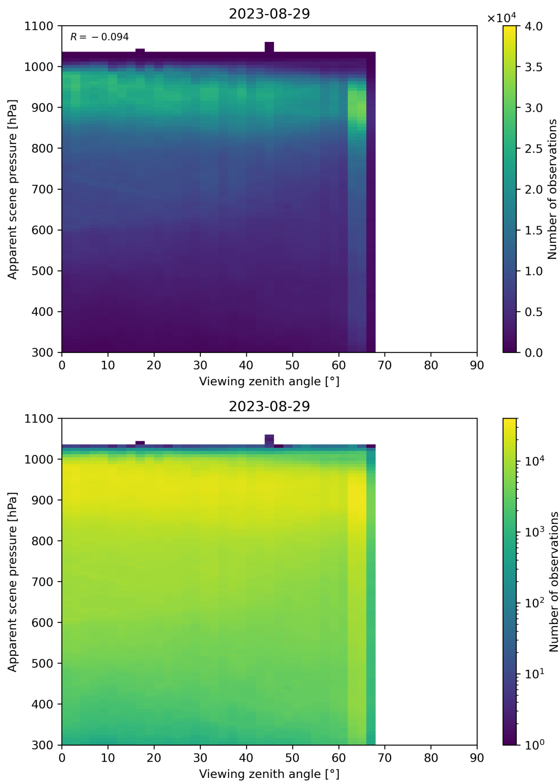
Figure 129: Scatter density plot of “Viewing zenith angle” against “Apparent scene pressure” for 2023-08-28 to 2023-08-30.
