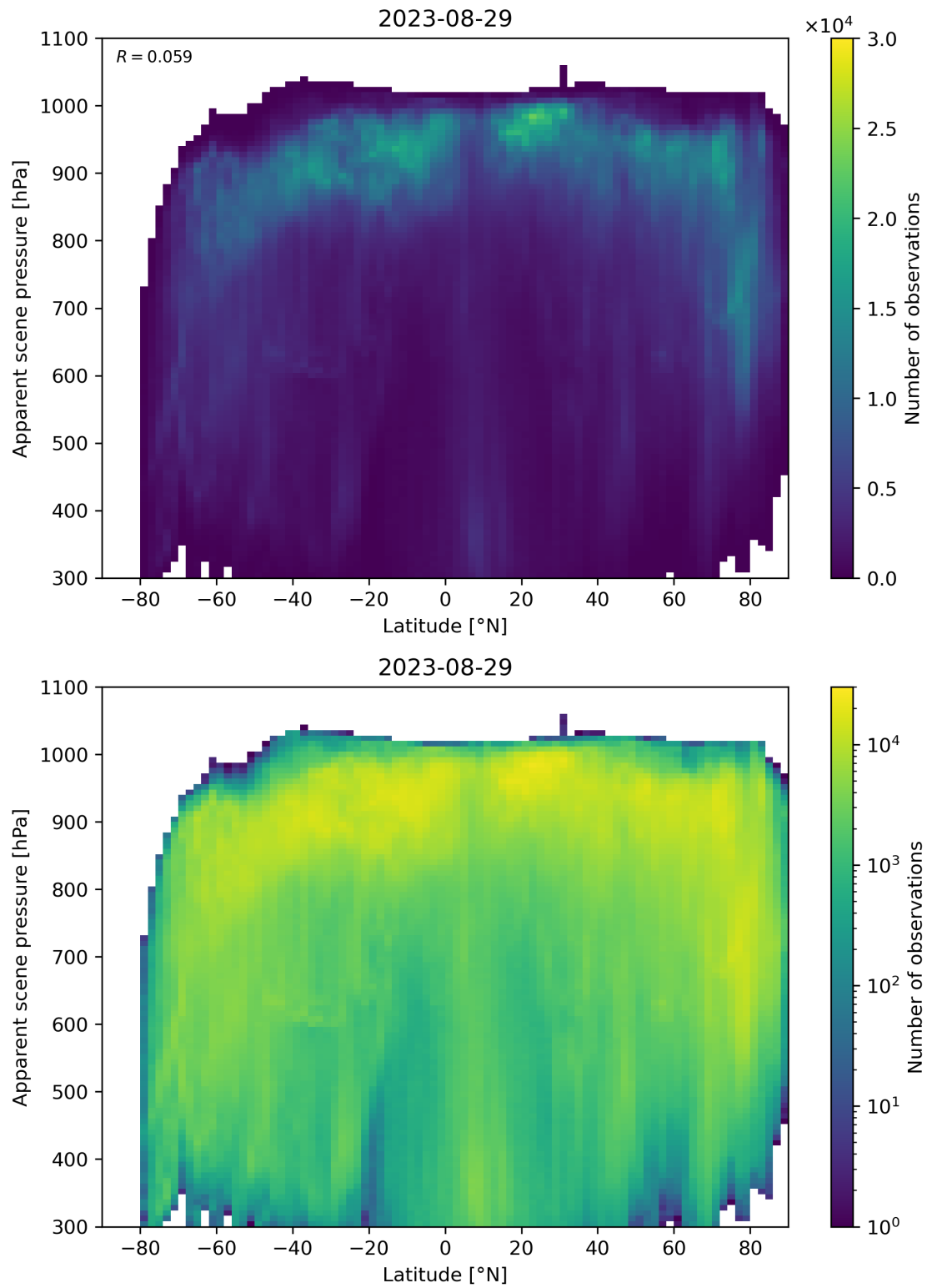
Figure 96: Scatter density plot of “Latitude” against “Apparent scene pressure” for 2023-08-28 to 2023-08-30.
