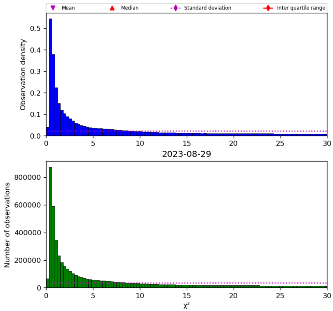
Figure 38: Histogram of " \chi^2 " for 2023-08-28 to 2023-08-30
