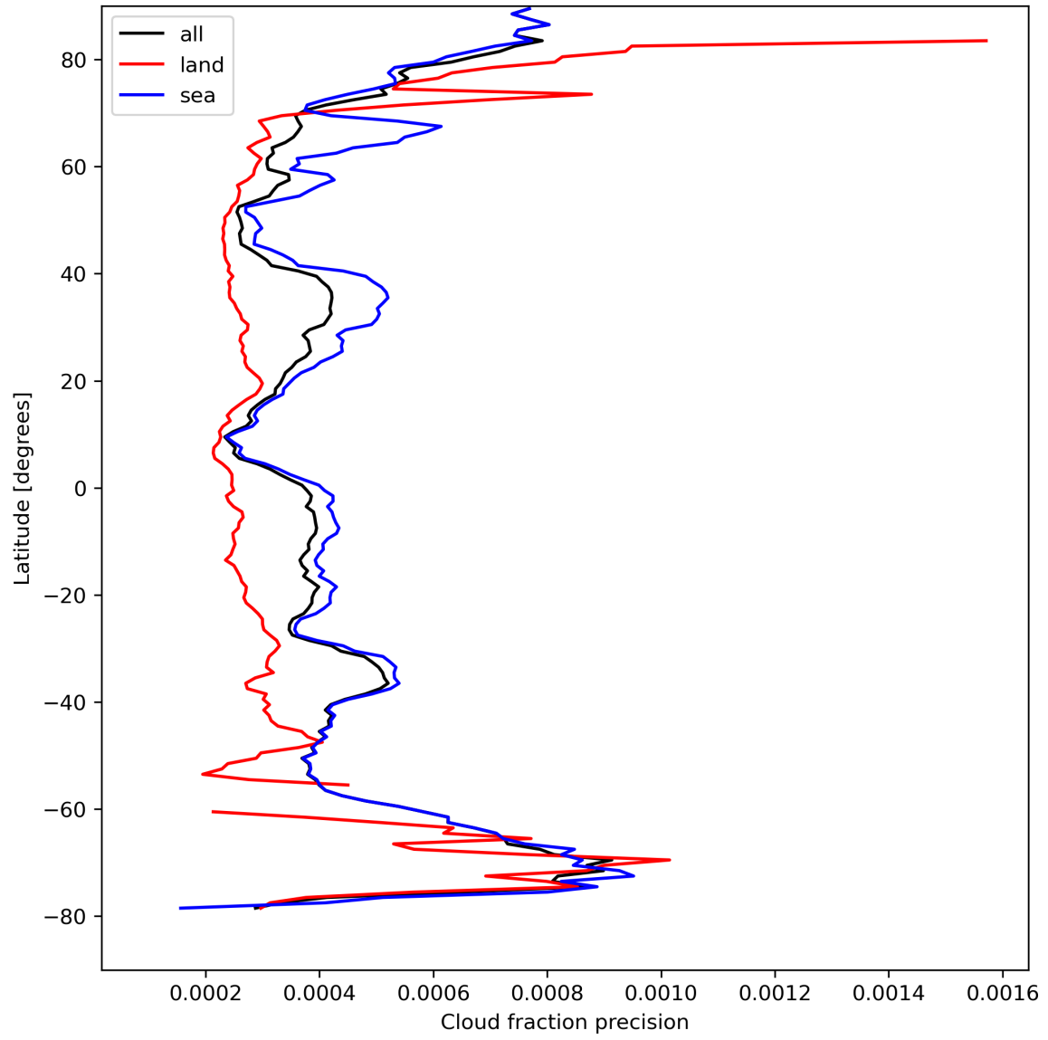
Figure 16: Zonal average of “Cloud fraction precision” for 2023-08-28 to 2023-08-30.
