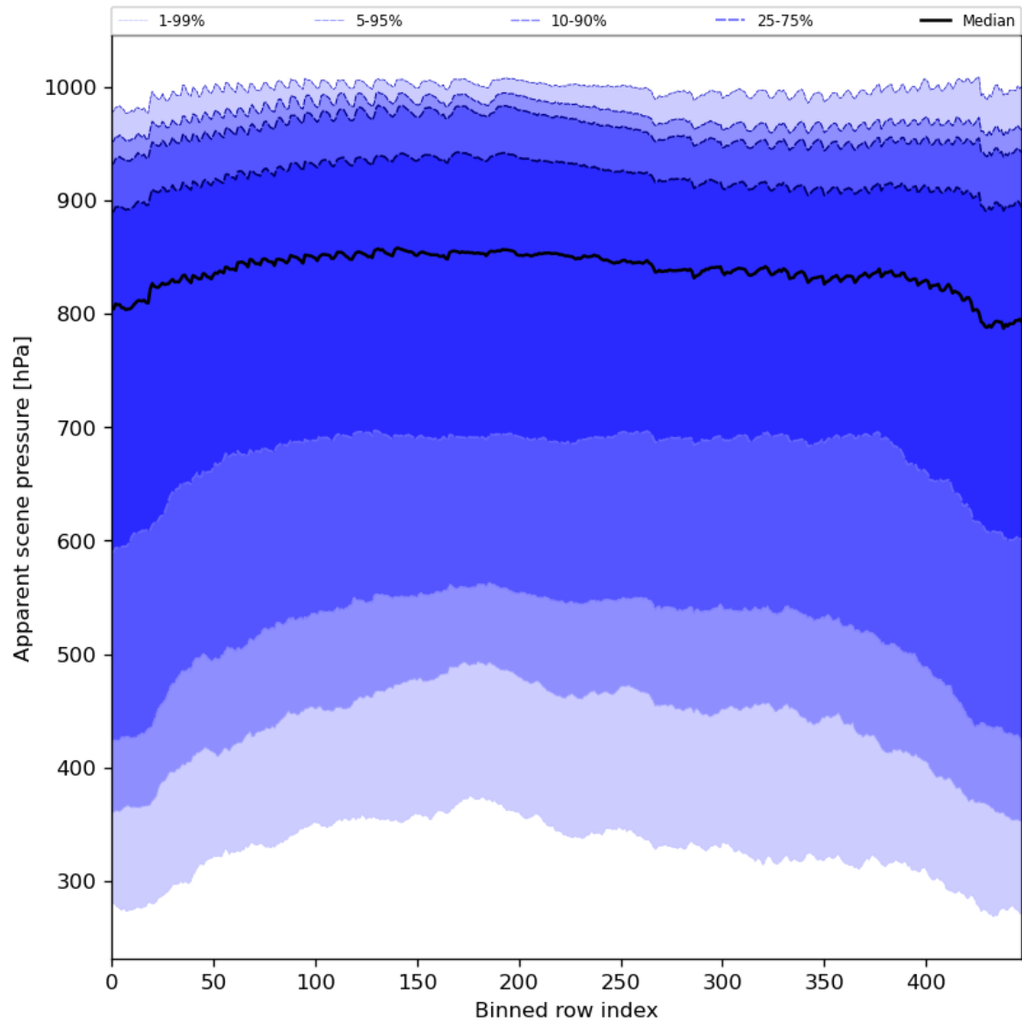
Figure 53: Along track statistics of “Apparent scene pressure” for 2023-08-28 to 2023-08-30
