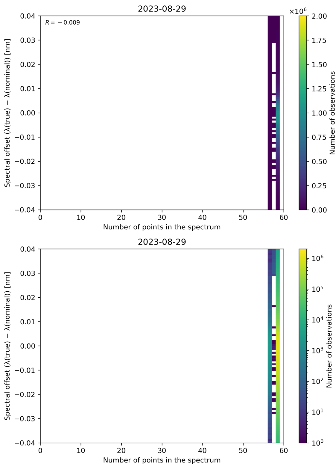
Figure 110: Scatter density plot of “Number of points in the spectrum” against “Spectral offset ( \lambda(\text{true}) - \lambda(\text{nominal}) )” for 2023-08-28 to 2023-08-30.
