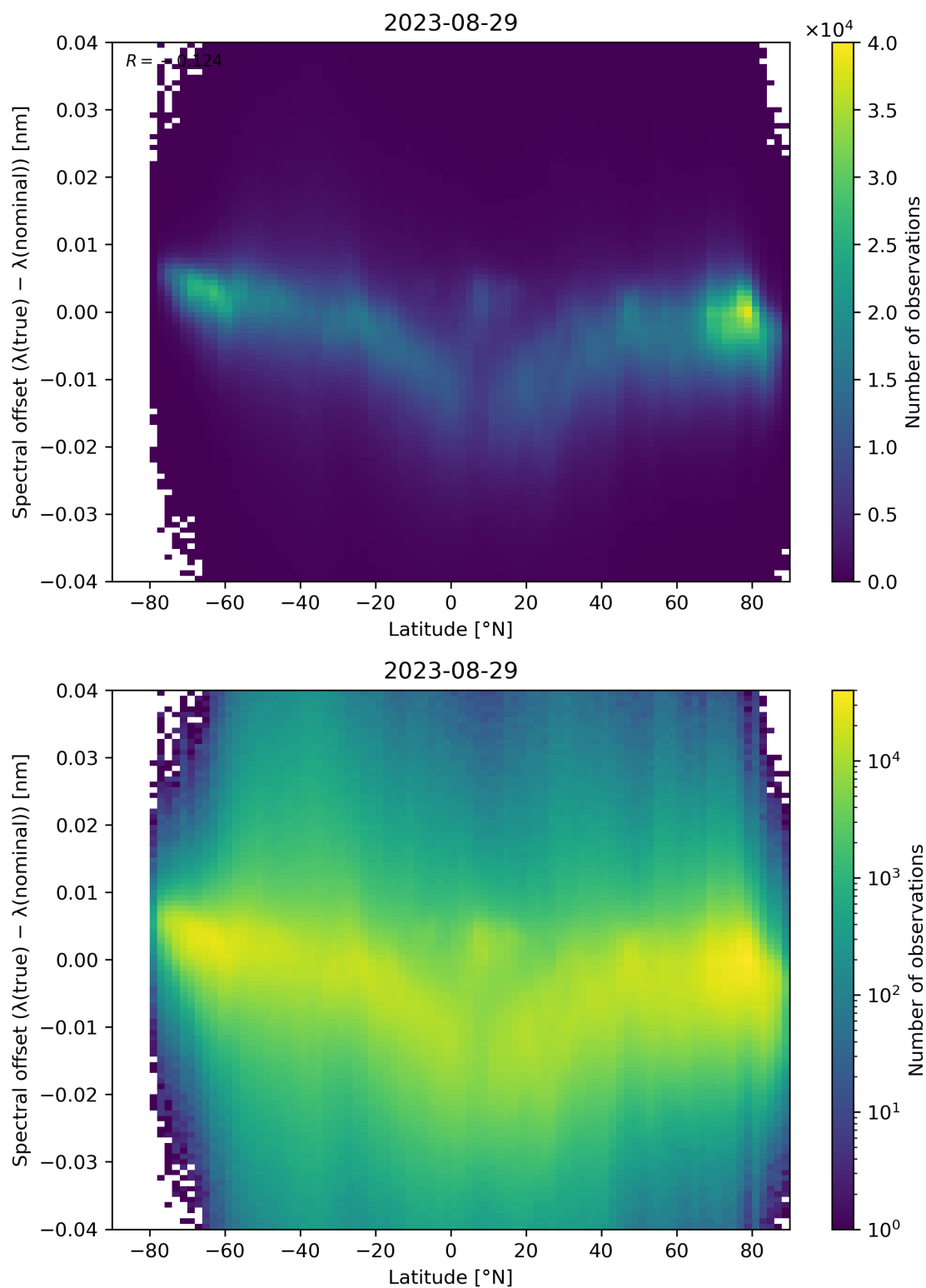
Figure 105: Scatter density plot of “Latitude” against “Spectral offset ( \lambda(\text{true}) - \lambda(\text{nominal}) )” for 2023-08-28 to 2023-08-30.
