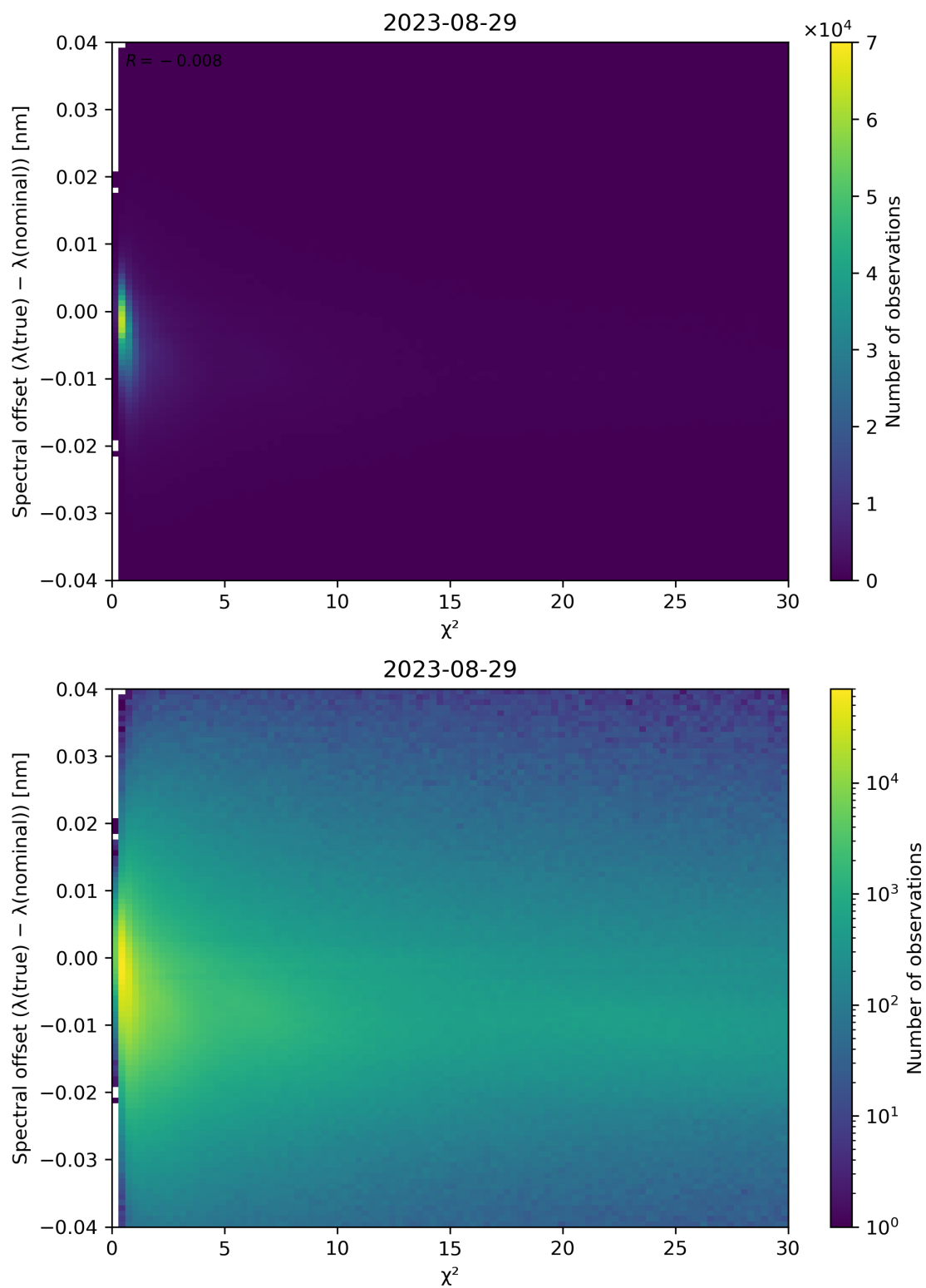
Figure 75: Scatter density plot of “ \chi^2 ” against “Spectral offset ( \lambda(\text{true}) - \lambda(\text{nominal}) )” for 2023-08-28 to 2023-08-30.
