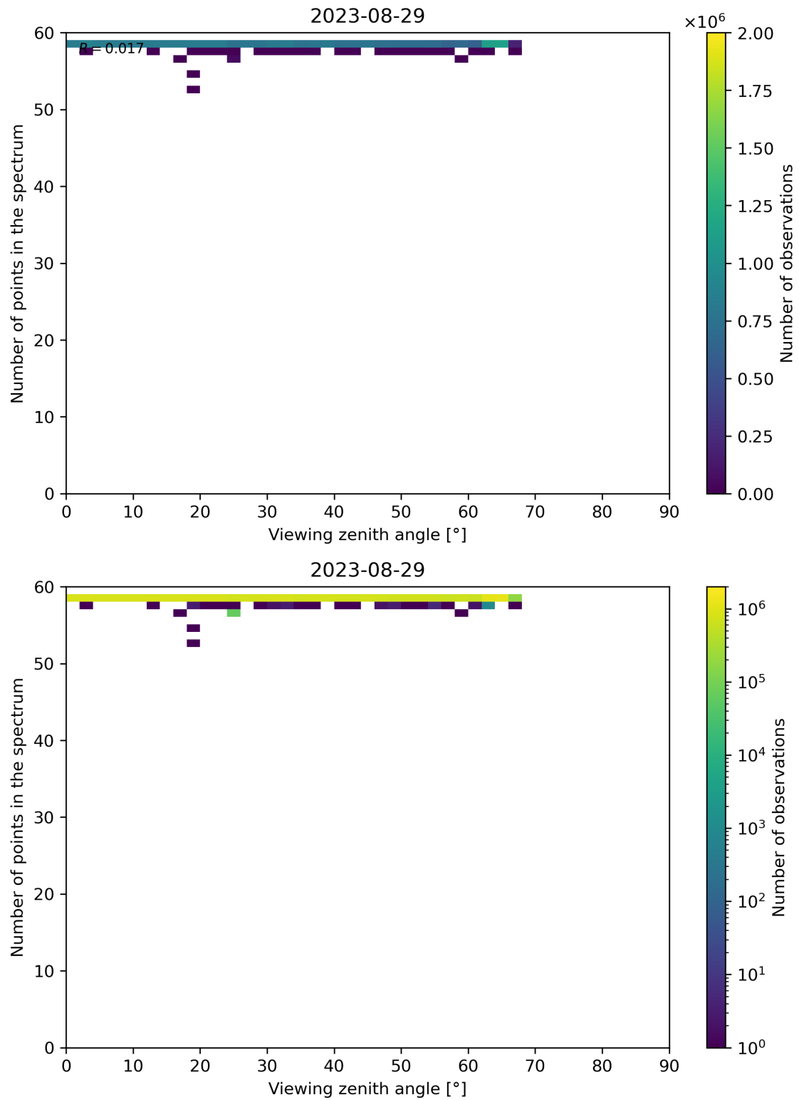
Figure 137: Scatter density plot of “Viewing zenith angle” against “Number of points in the spectrum” for 2023-08-28 to 2023-08-30.
