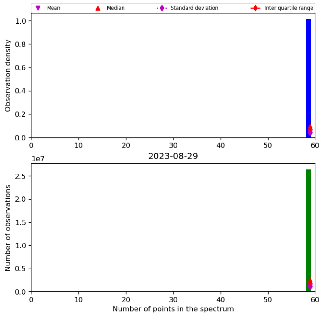
Figure 44: Histogram of “Number of points in the spectrum” for 2023-08-28 to 2023-08-30
