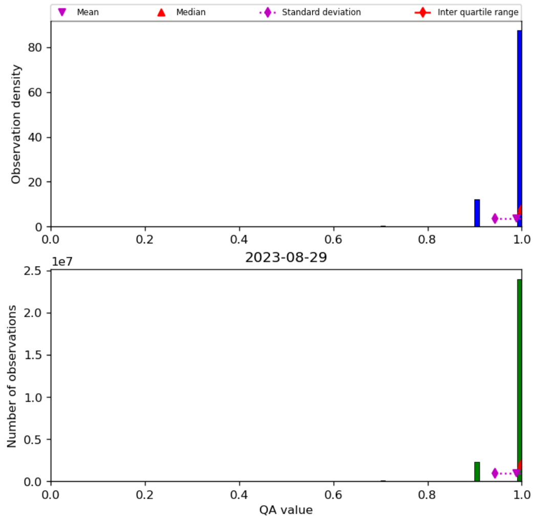
Figure 29: Histogram of “QA value” for 2023-08-28 to 2023-08-30
