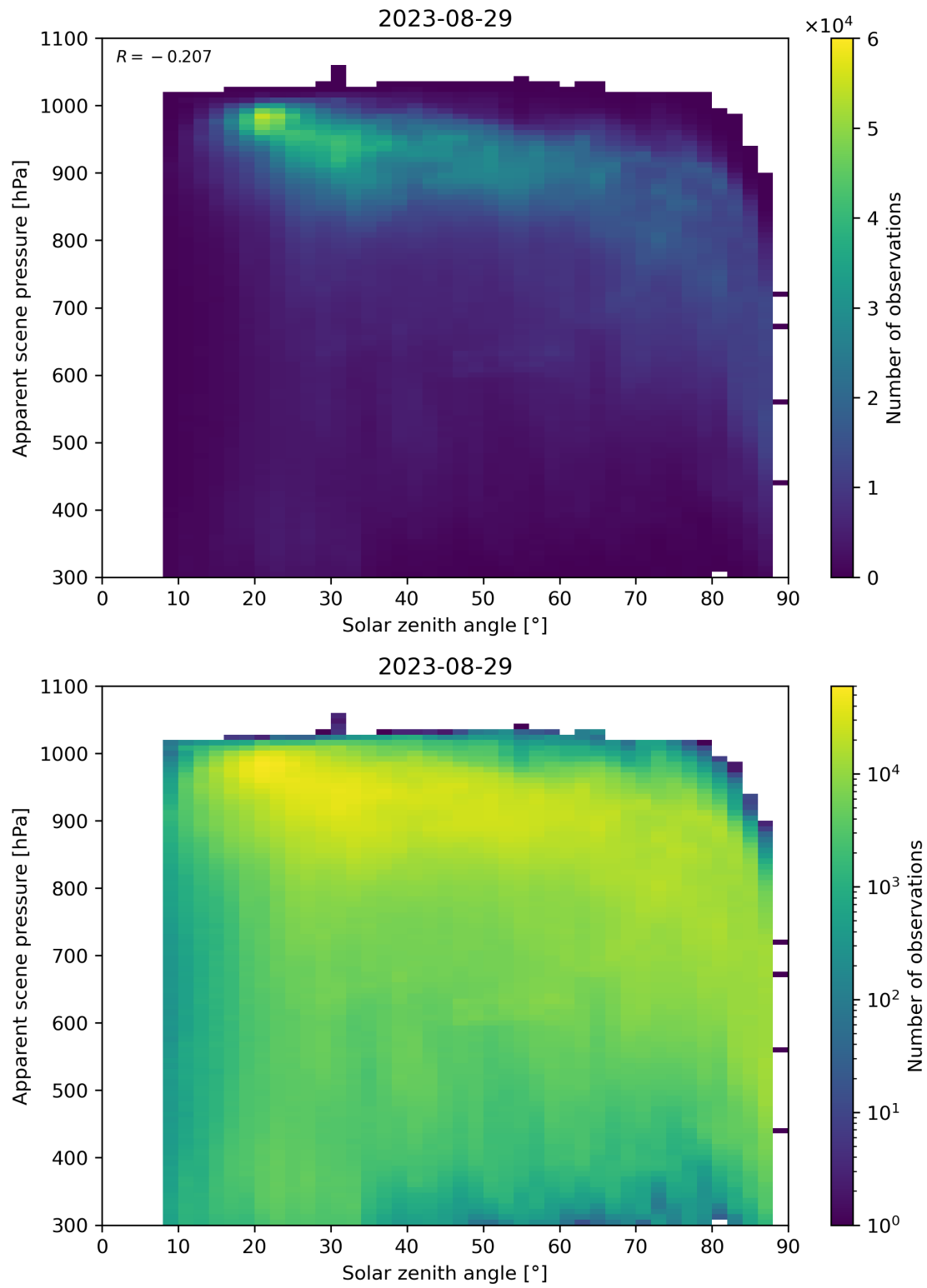
Figure 118: Scatter density plot of “Solar zenith angle” against “Apparent scene pressure” for 2023-08-28 to 2023-08-30.
