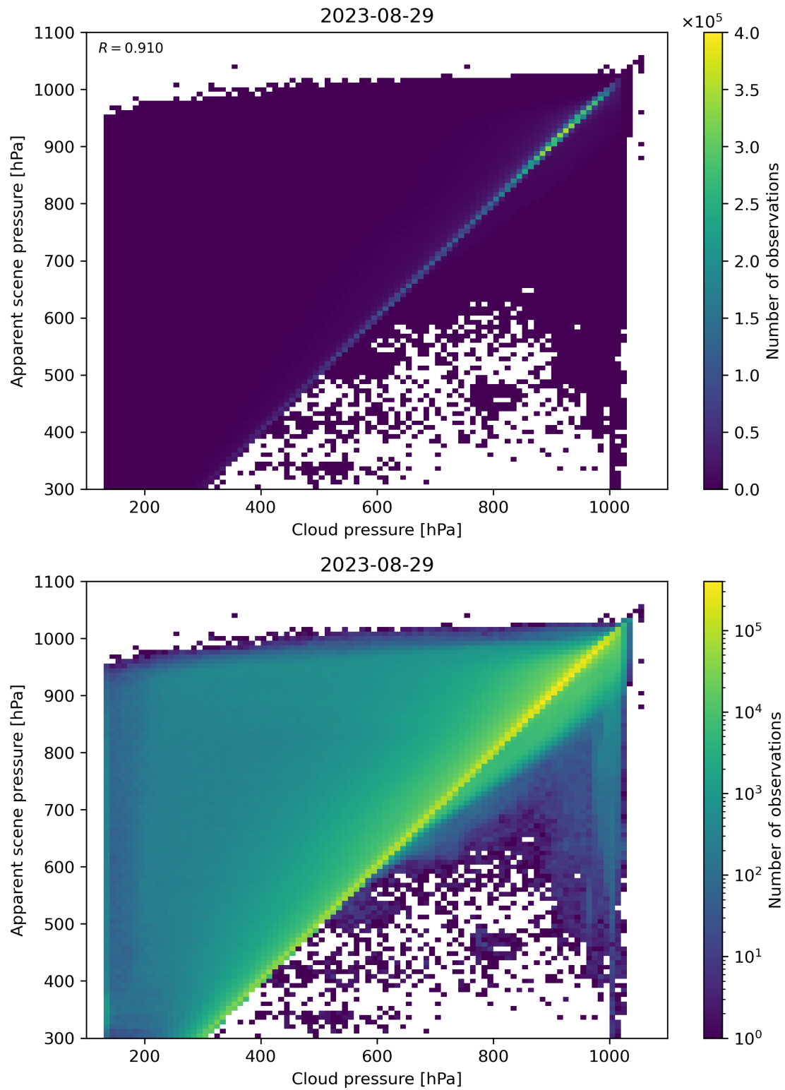
Figure 84: Scatter density plot of “Cloud pressure” against “Apparent scene pressure” for 2023-08-28 to 2023-08-30.
