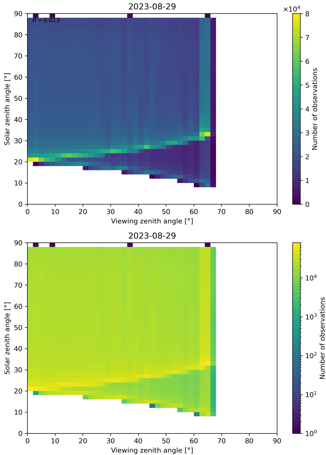
Figure 139: Scatter density plot of “Viewing zenith angle” against “Solar zenith angle” for 2023-08-28 to 2023-08-30.
