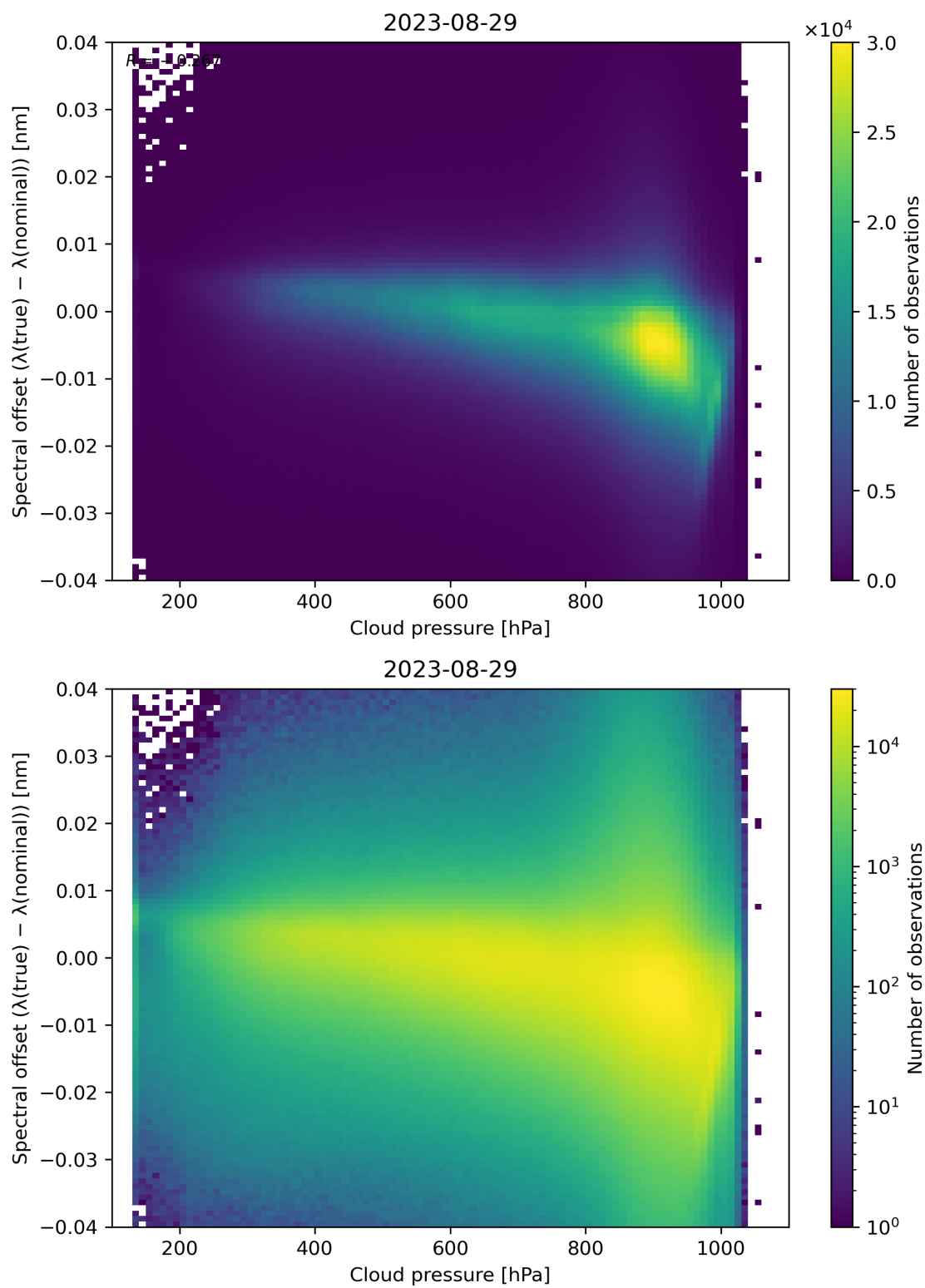
Figure 92: Scatter density plot of “Cloud pressure” against “Spectral offset ( \lambda(\text{true}) - \lambda(\text{nominal}) )” for 2023-08-28 to 2023-08-30.
