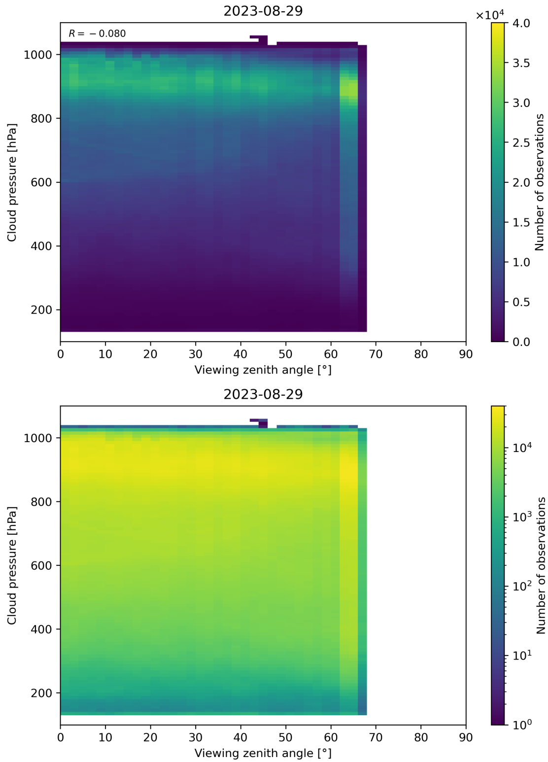
Figure 133: Scatter density plot of “Viewing zenith angle” against “Cloud pressure” for 2023-08-28 to 2023-08-30.
