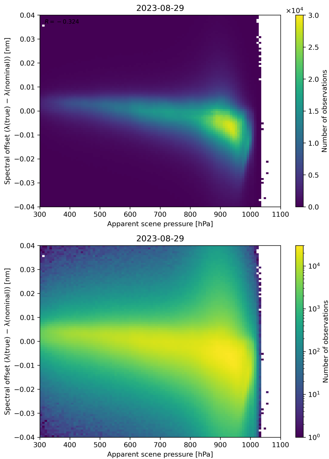
Figure 68: Scatter density plot of “Apparent scene pressure” against “Spectral offset ( \lambda(\text{true}) - \lambda(\text{nominal}) )” for 2023-08-28 to 2023-08-30.
