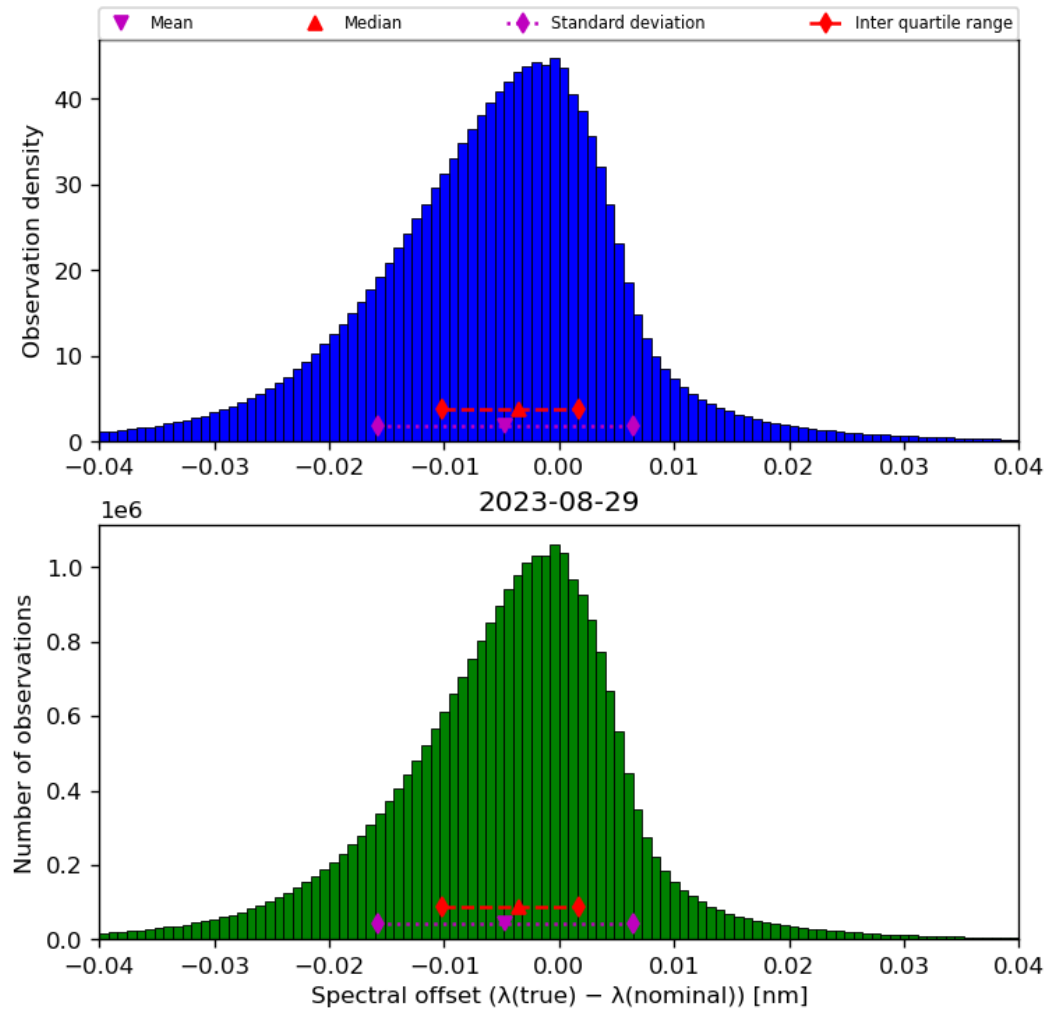
Figure 45: Histogram of “Spectral offset ( \lambda(\text{true}) - \lambda(\text{nominal}) )” for 2023-08-28 to 2023-08-30
