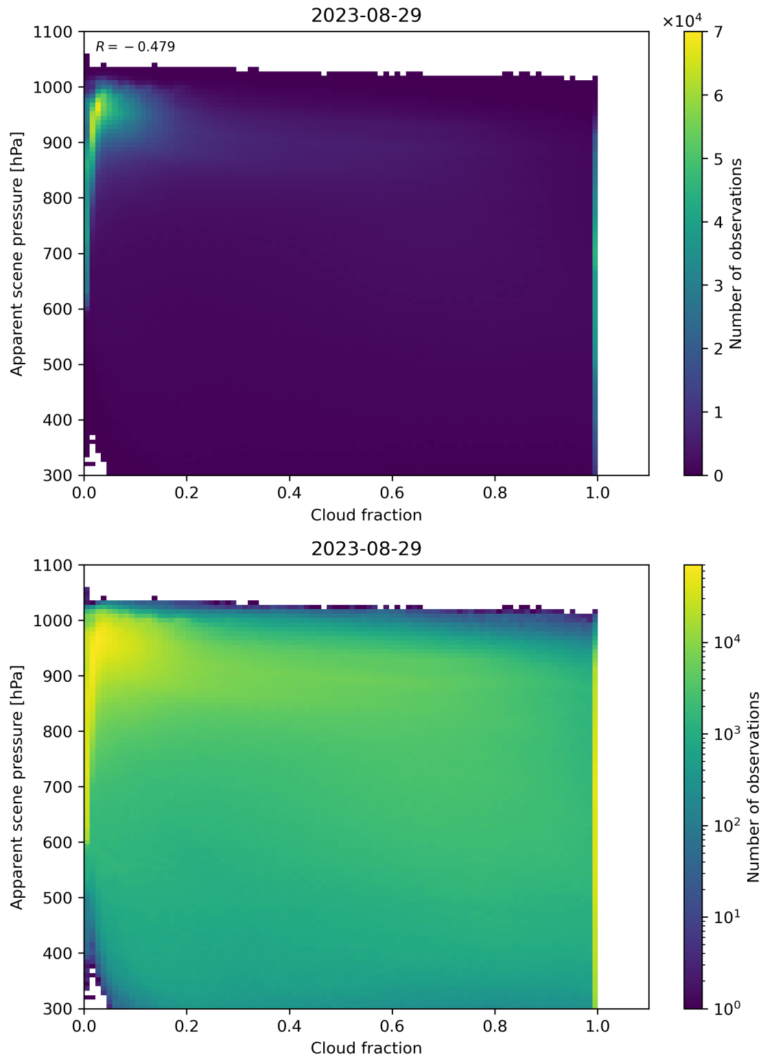
Figure 76: Scatter density plot of “Cloud fraction” against “Apparent scene pressure” for 2023-08-28 to 2023-08-30.
