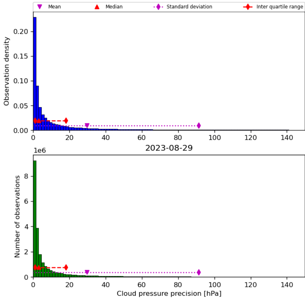
Figure 31: Histogram of “Cloud pressure precision” for 2023-08-28 to 2023-08-30
