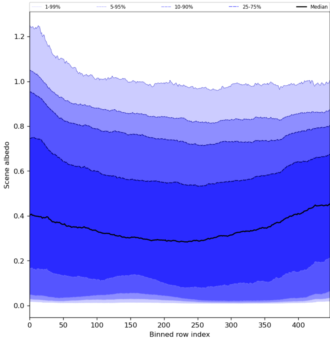
Figure 51: Along track statistics of “Scene albedo” for 2023-08-28 to 2023-08-30
