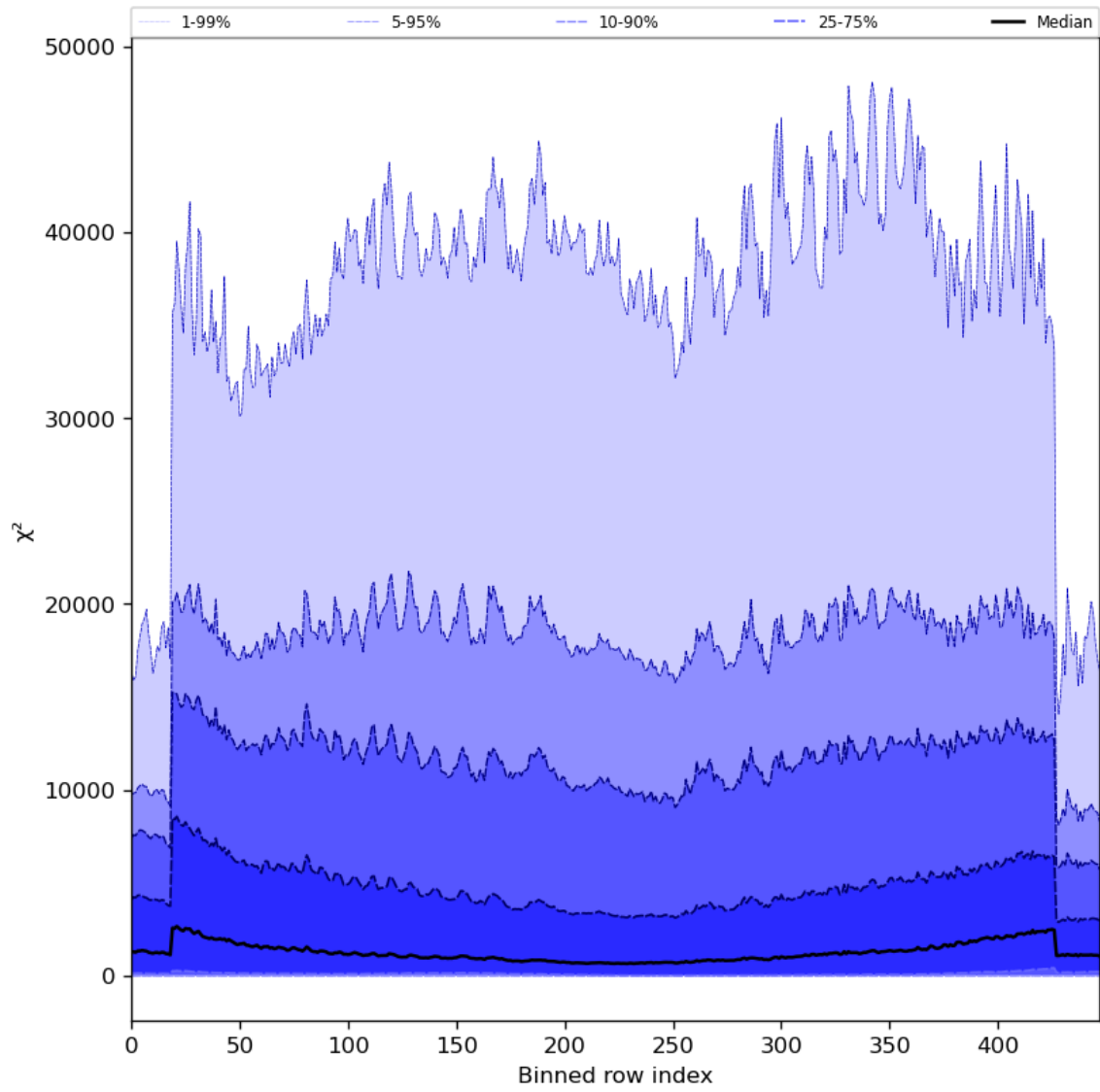
Figure 55: Along track statistics of “ \chi^2 ” for 2023-08-28 to 2023-08-30
