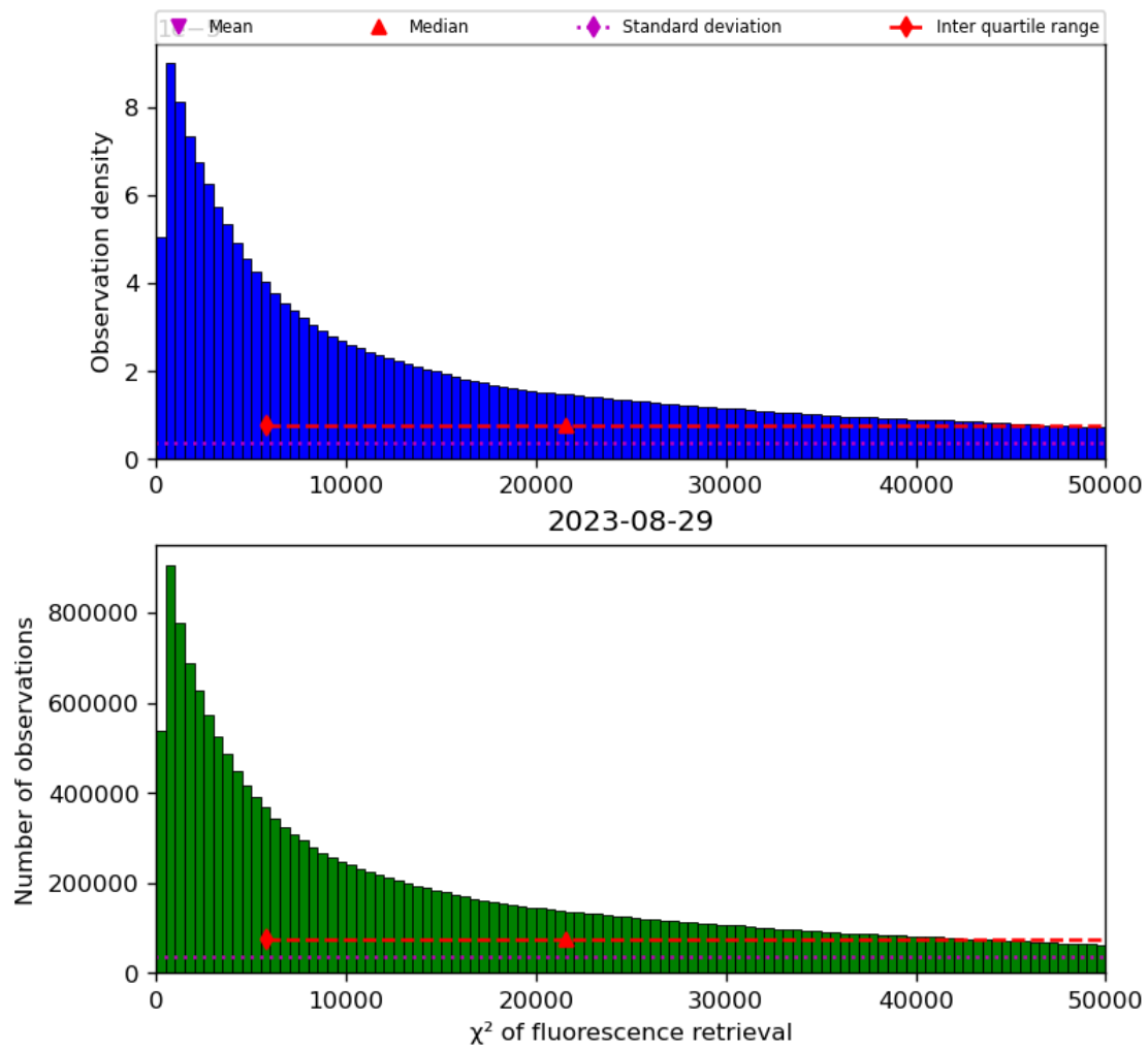
Figure 42: Histogram of “ \chi^2 of fluorescence retrieval” for 2023-08-28 to 2023-08-30
