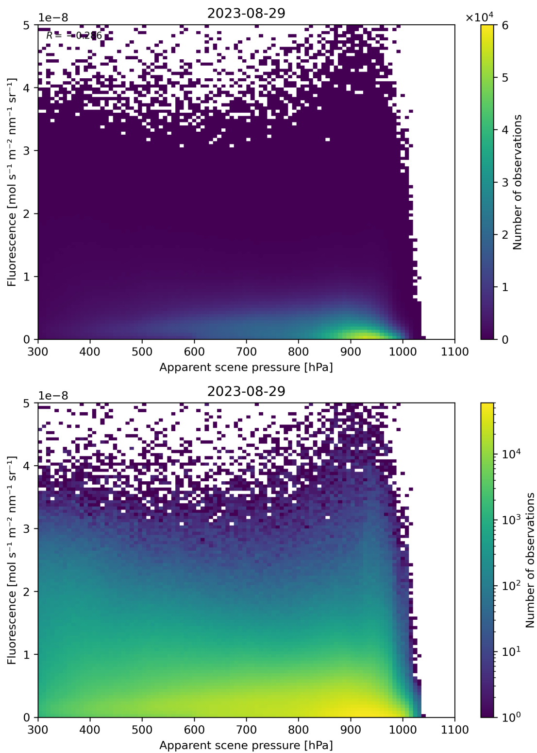
Figure 65: Scatter density plot of “Apparent scene pressure” against “Fluorescence” for 2023-08-28 to 2023-08-30.
