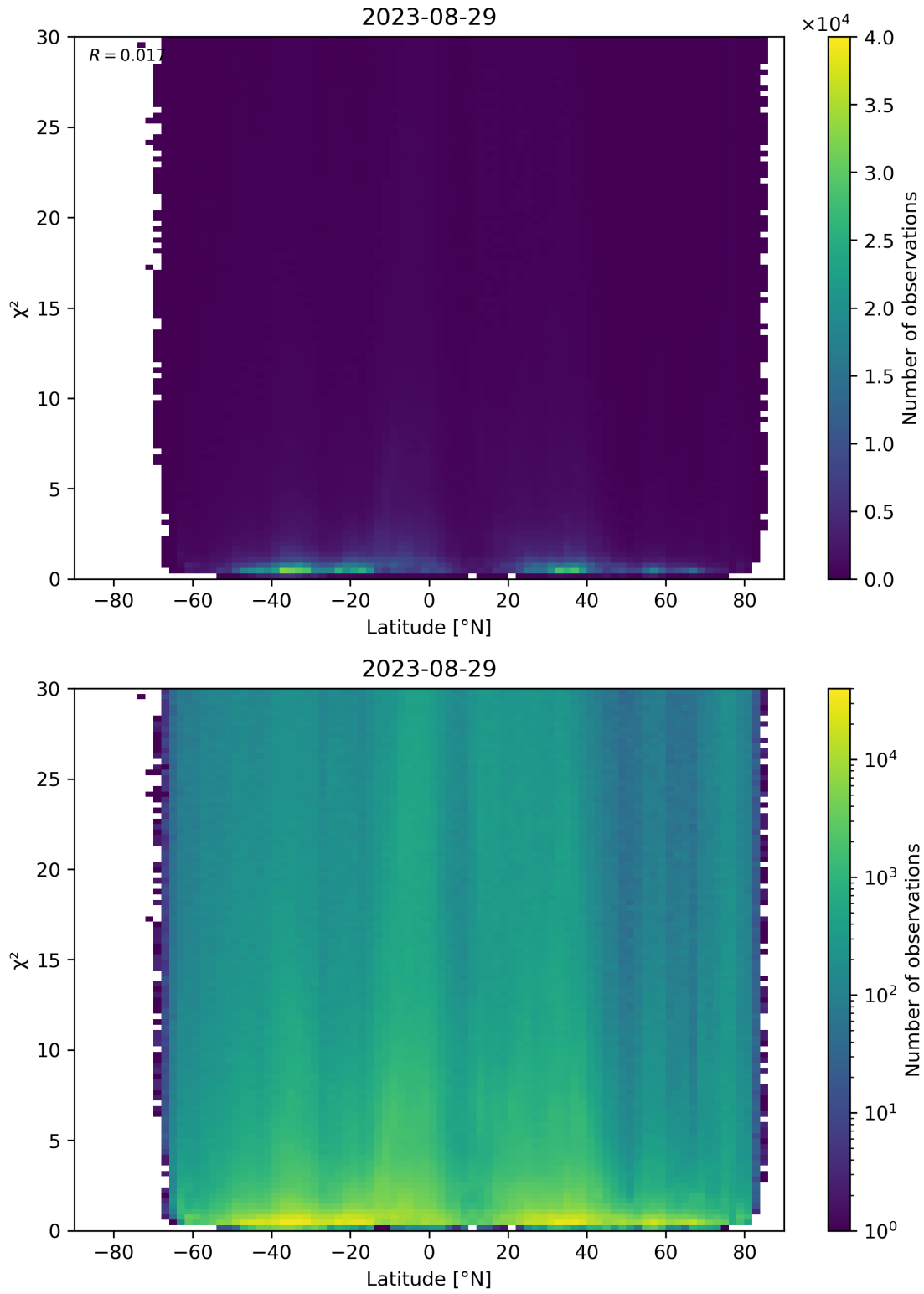
Figure 97: Scatter density plot of “Latitude” against “ \chi^2 ” for 2023-08-28 to 2023-08-30.
