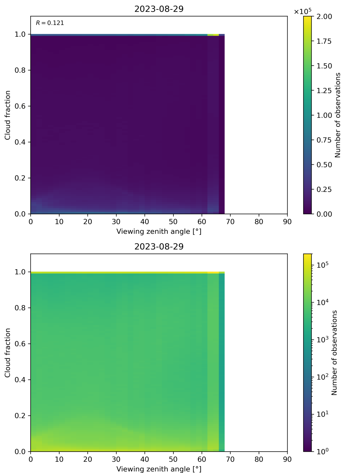
Figure 132: Scatter density plot of “Viewing zenith angle” against “Cloud fraction” for 2023-08-28 to 2023-08-30.
