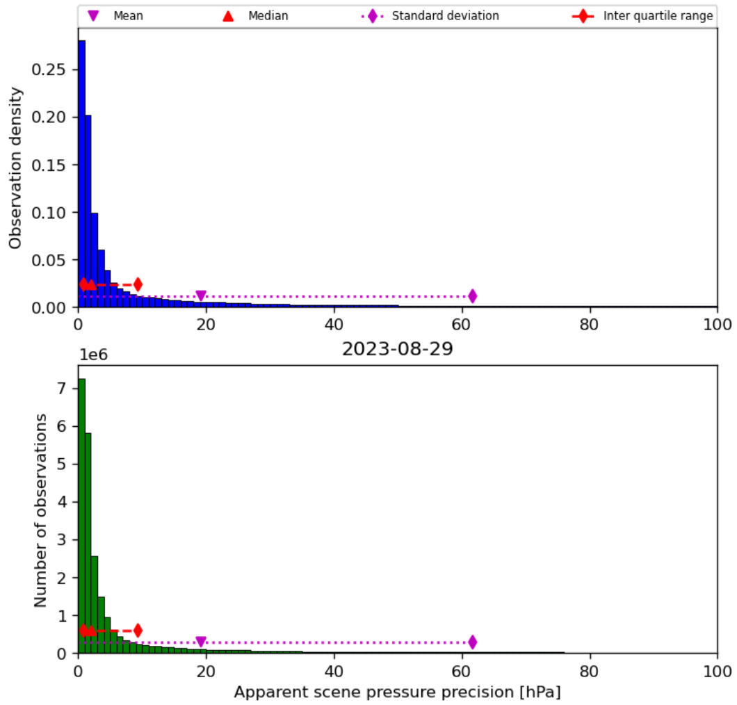
Figure 37: Histogram of “Apparent scene pressure precision” for 2023-08-28 to 2023-08-30
