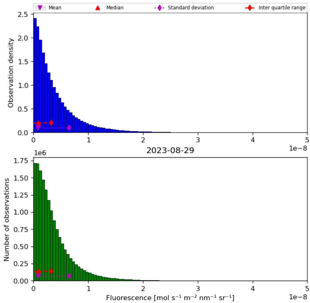
Figure 40: Histogram of “Fluorescence” for 2023-08-28 to 2023-08-30
