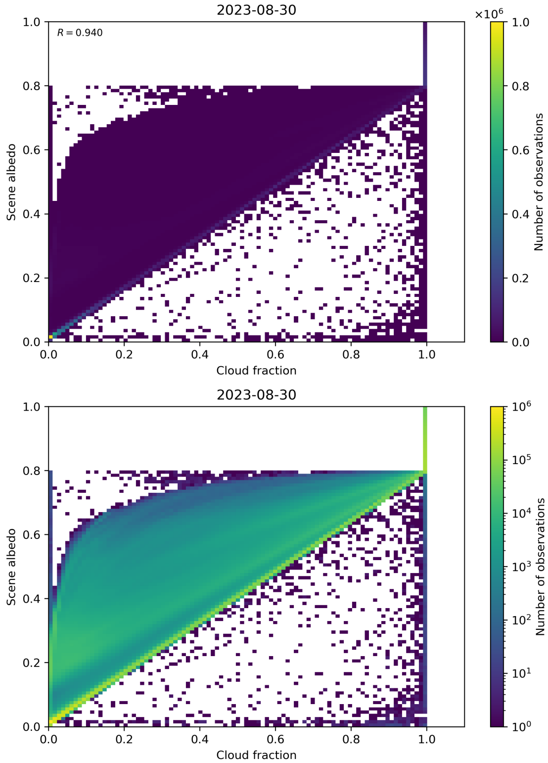
Figure 82: Scatter density plot of “Cloud fraction” against “Scene albedo” for 2023-08-30 to 2023-08-31.
