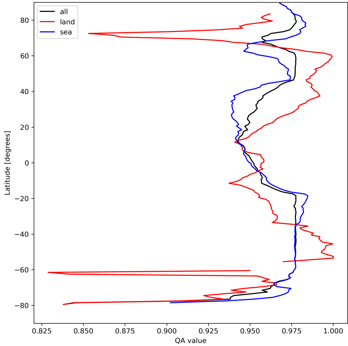
Figure 12: Zonal average of “QA value” for 2023-08-30 to 2023-08-31.
