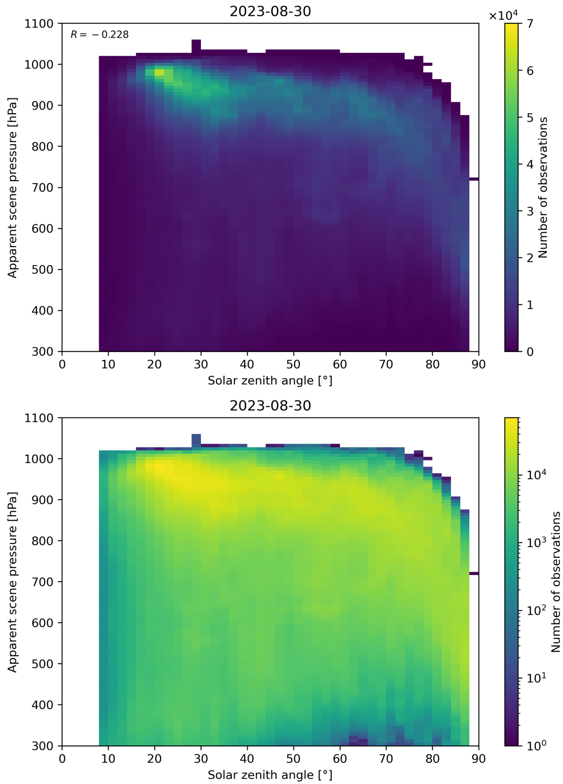
Figure 118: Scatter density plot of “Solar zenith angle” against “Apparent scene pressure” for 2023-08-30 to 2023-08-31.
