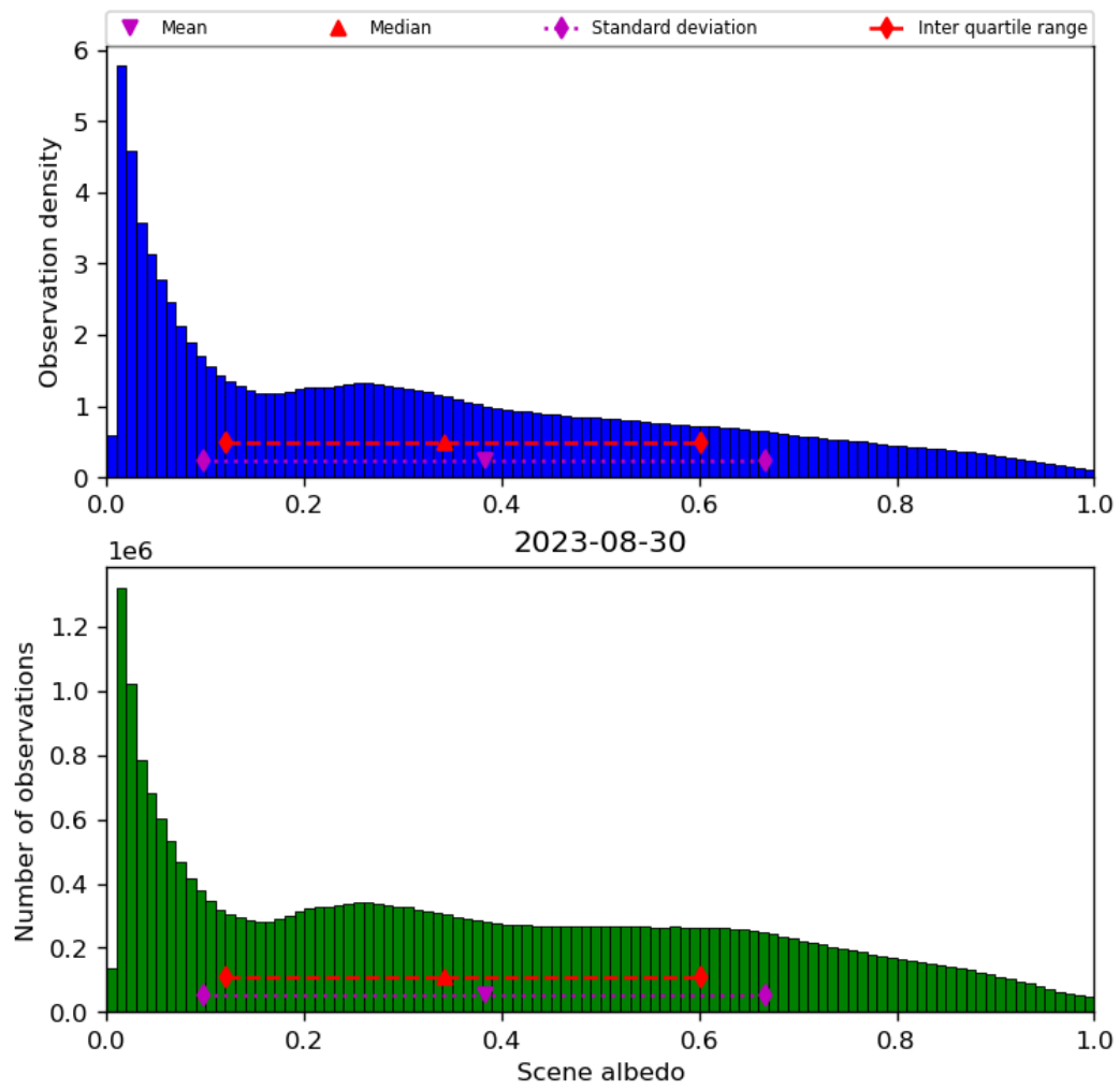
Figure 34: Histogram of “Scene albedo” for 2023-08-30 to 2023-08-31
