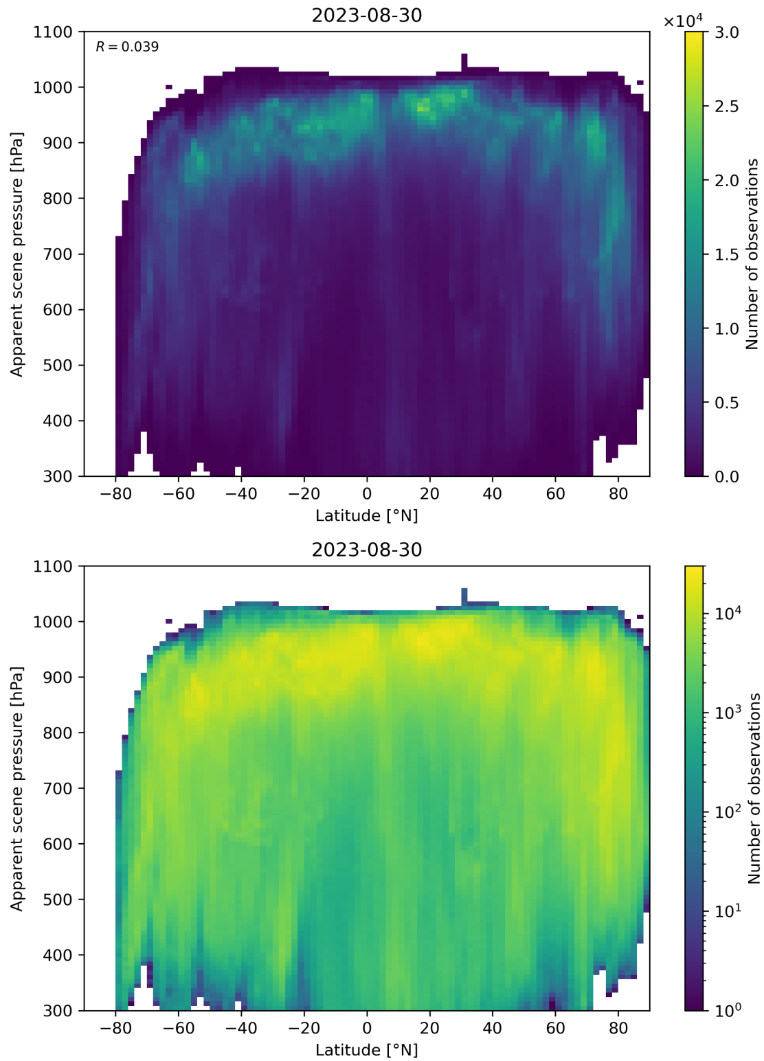
Figure 96: Scatter density plot of “Latitude” against “Apparent scene pressure” for 2023-08-30 to 2023-08-31.
