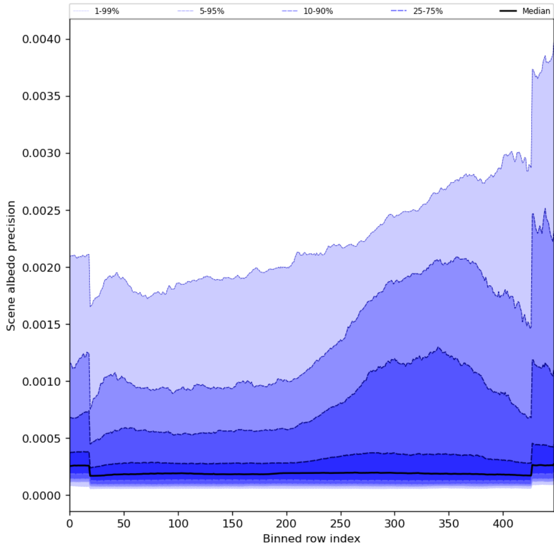
Figure 52: Along track statistics of “Scene albedo precision” for 2023-08-30 to 2023-08-31
