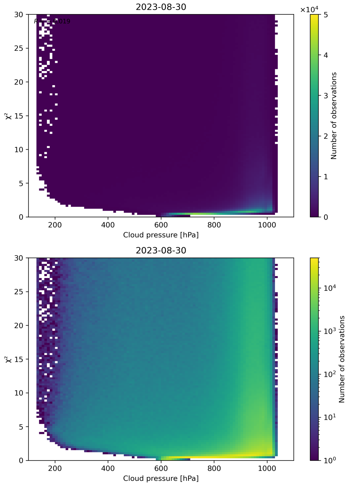
Figure 85: Scatter density plot of “Cloud pressure” against “ \chi^2 ” for 2023-08-30 to 2023-08-31.
