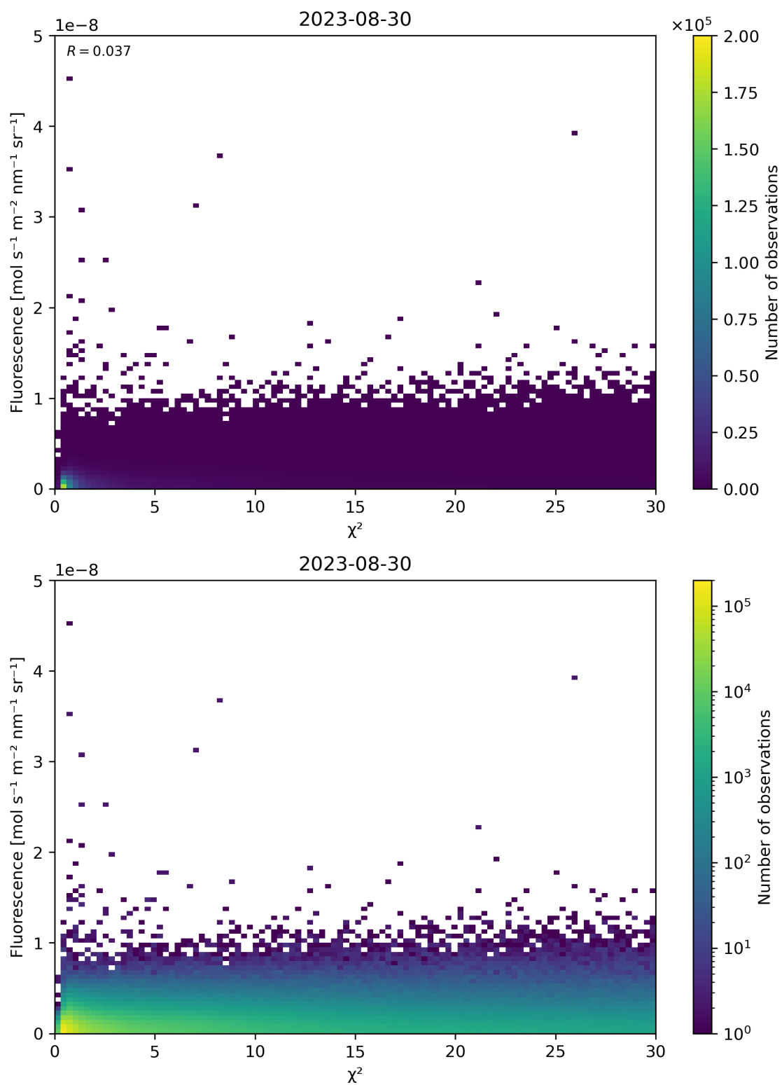
Figure 70: Scatter density plot of “ \chi^2 ” against “Fluorescence” for 2023-08-30 to 2023-08-31.
