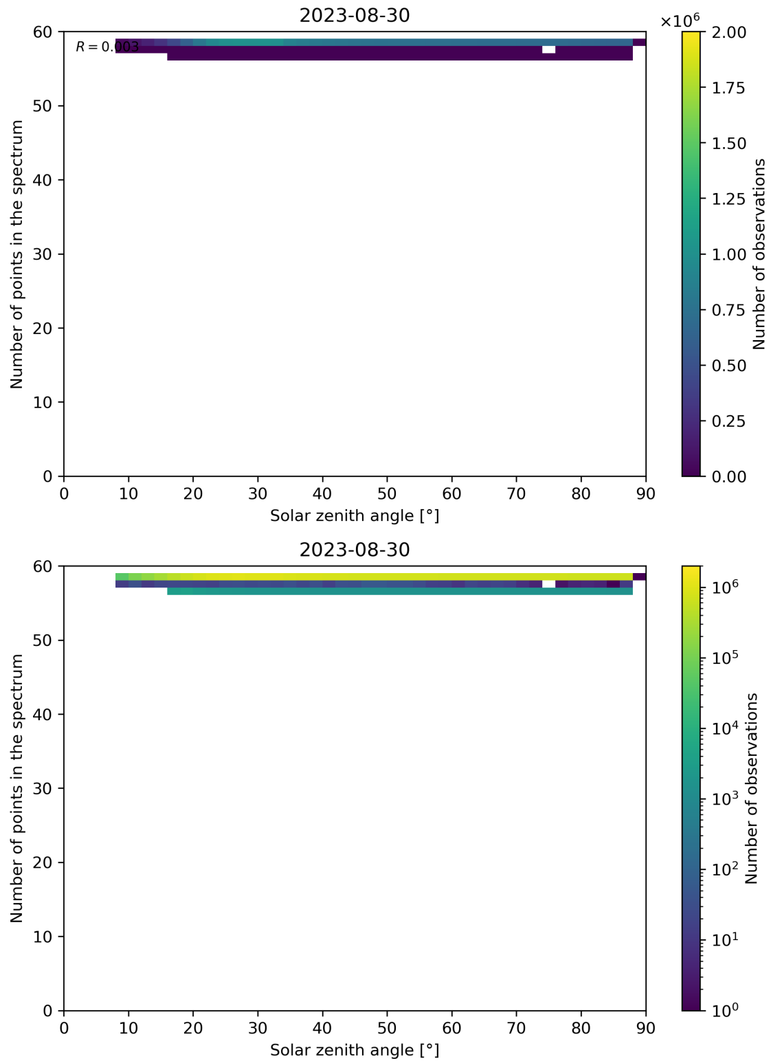
Figure 126: Scatter density plot of “Solar zenith angle” against “Number of points in the spectrum” for 2023-08-30 to 2023-08-31.
