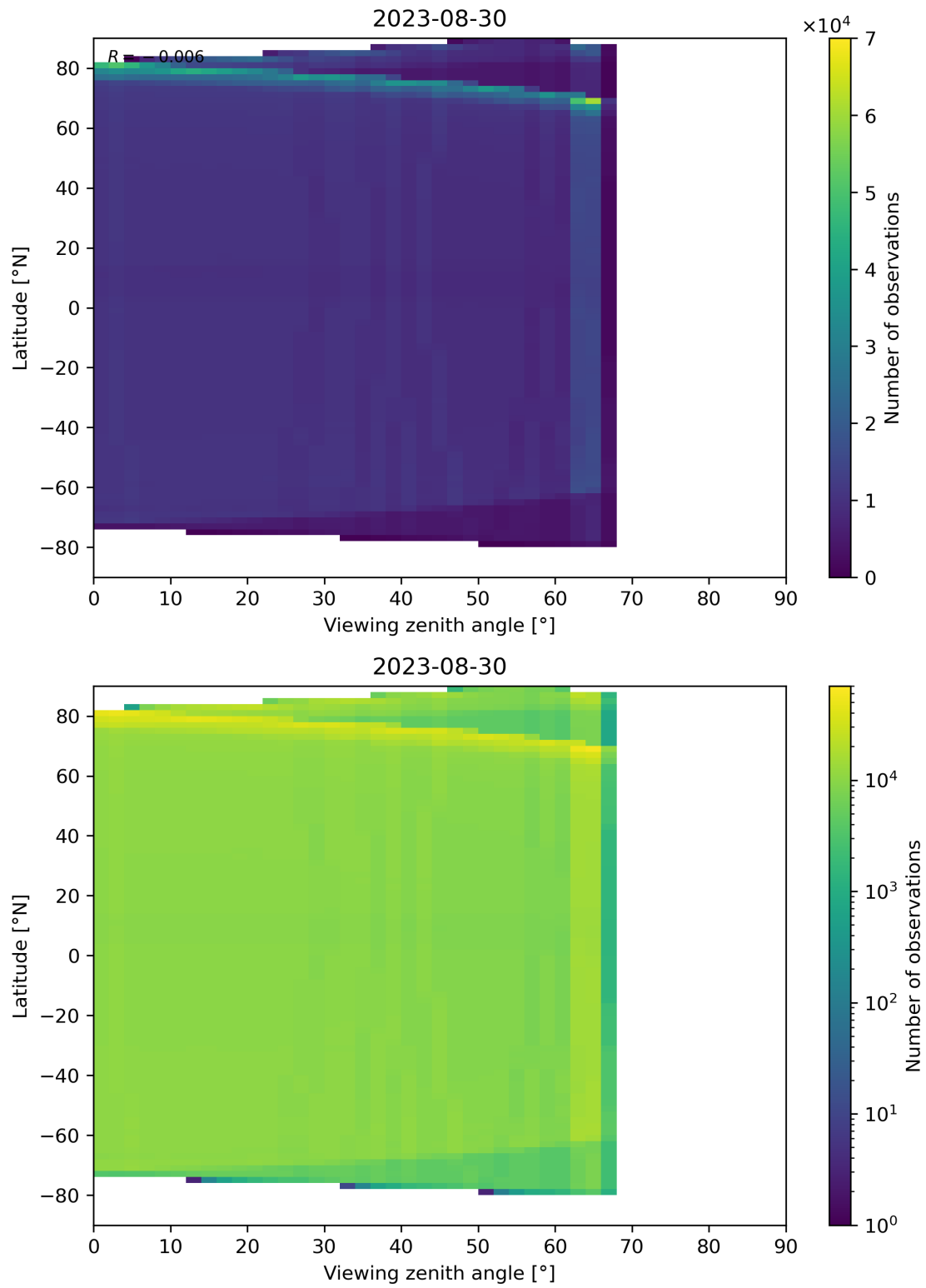
Figure 135: Scatter density plot of “Viewing zenith angle” against “Latitude” for 2023-08-30 to 2023-08-31.
