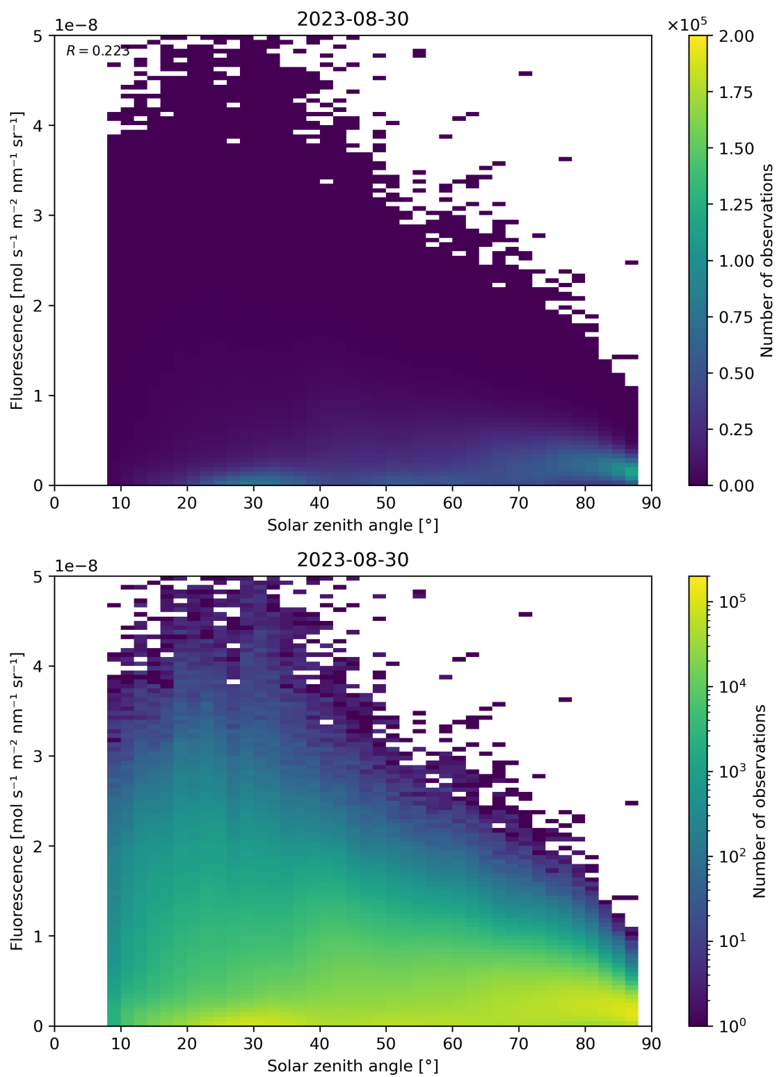
Figure 123: Scatter density plot of “Solar zenith angle” against “Fluorescence” for 2023-08-30 to 2023-08-31.
