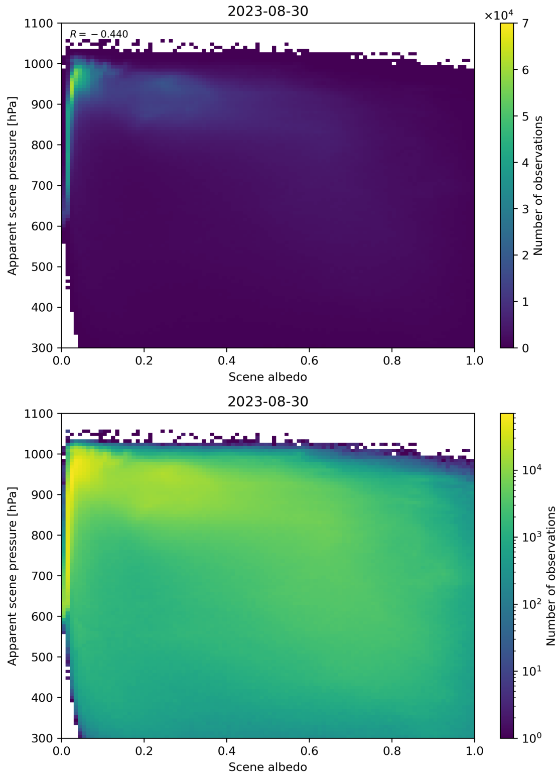
Figure 111: Scatter density plot of “Scene albedo” against “Apparent scene pressure” for 2023-08-30 to 2023-08-31.
