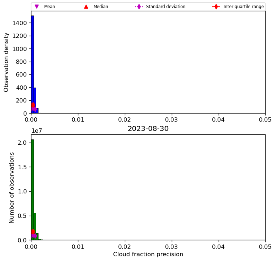
Figure 33: Histogram of “Cloud fraction precision” for 2023-08-30 to 2023-08-31
