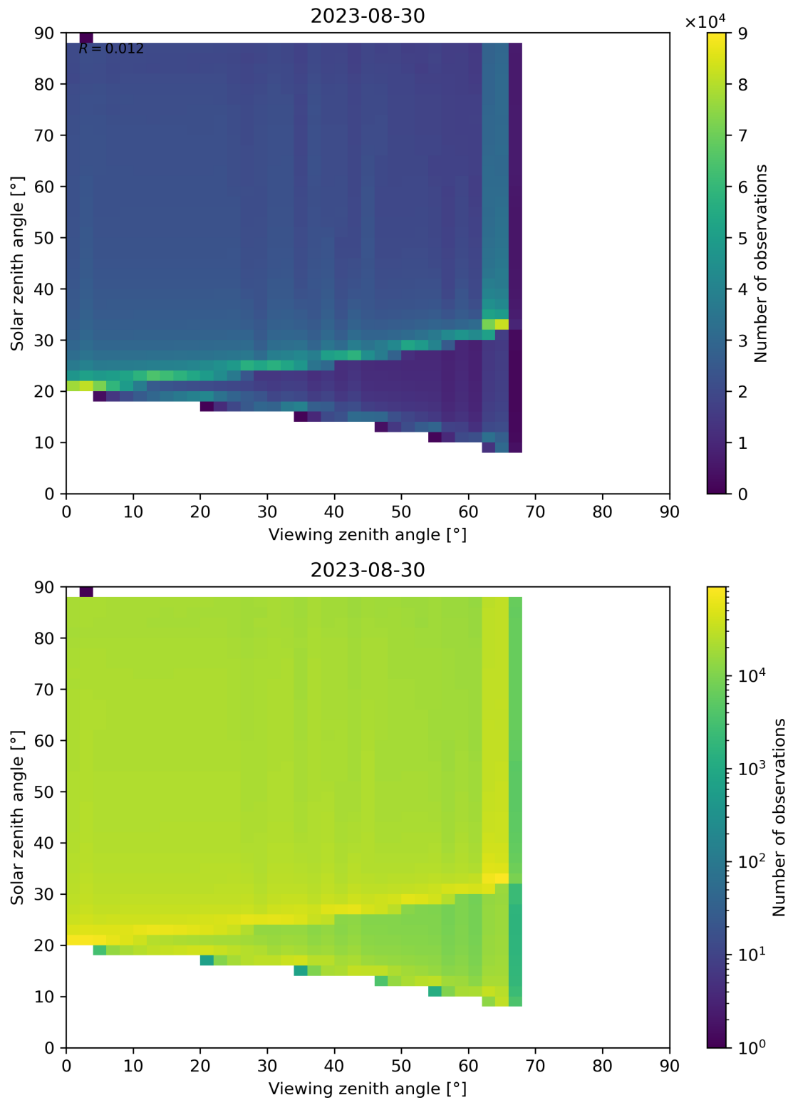
Figure 139: Scatter density plot of “Viewing zenith angle” against “Solar zenith angle” for 2023-08-30 to 2023-08-31.
