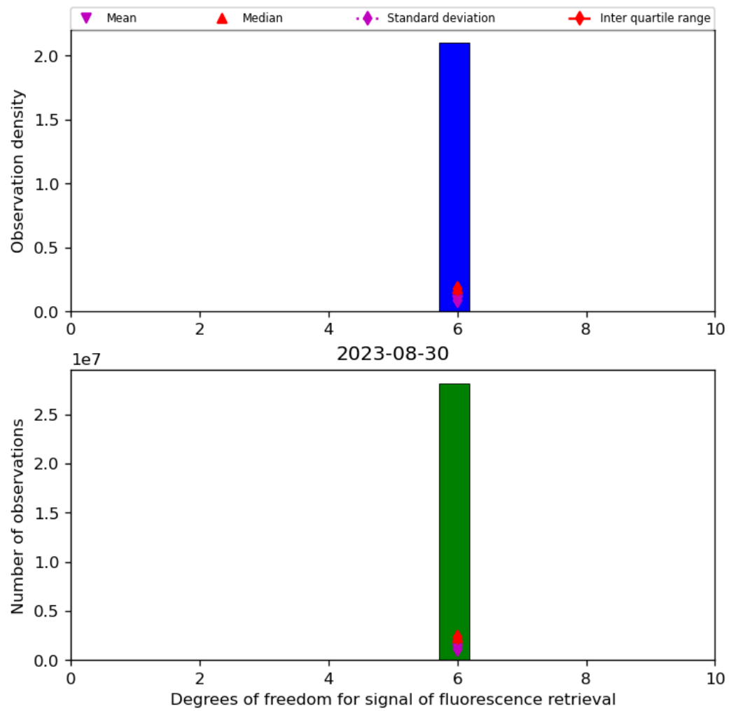
Figure 43: Histogram of “Degrees of freedom for signal of fluorescence retrieval” for 2023-08-30 to 2023-08-31
