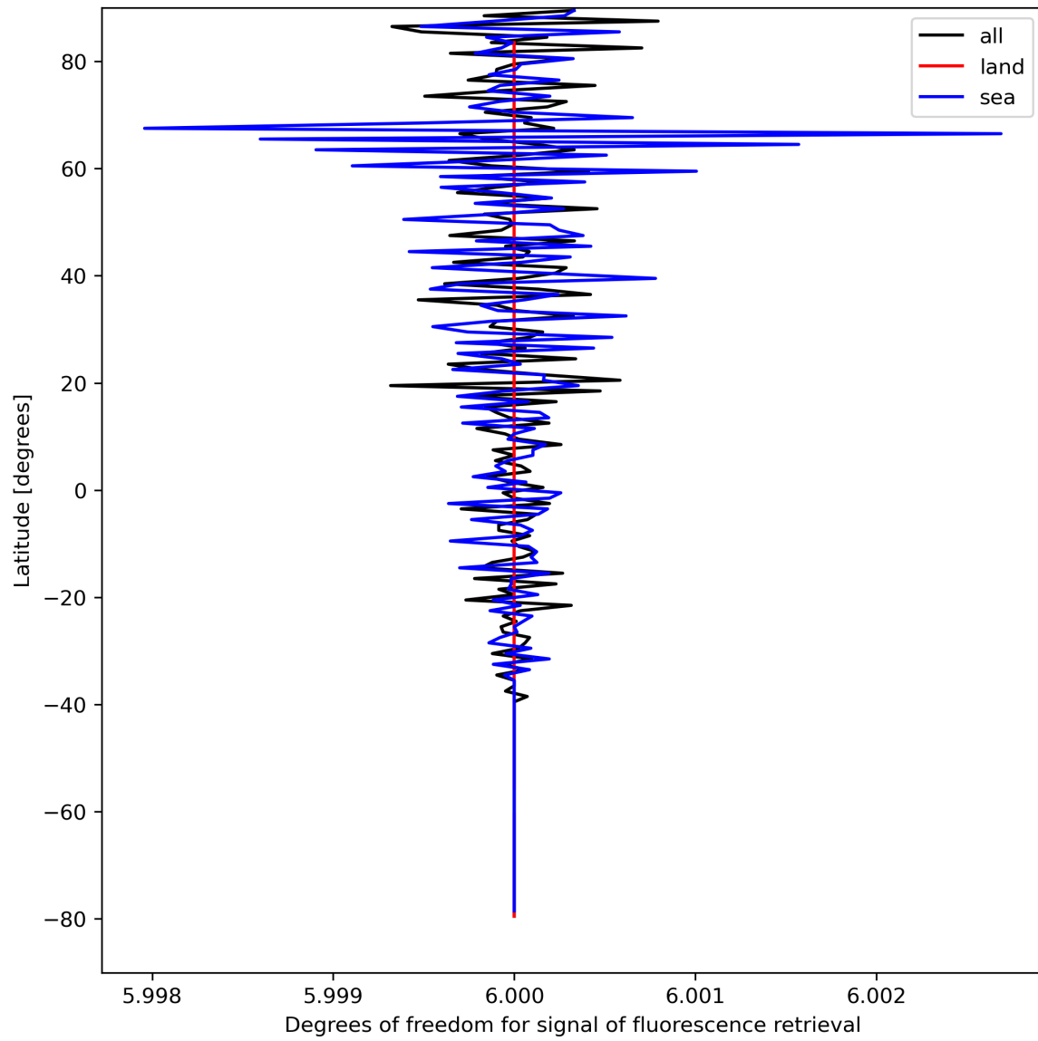
Figure 26: Zonal average of “Degrees of freedom for signal of fluorescence retrieval” for 2023-08-30 to 2023-08-31.
