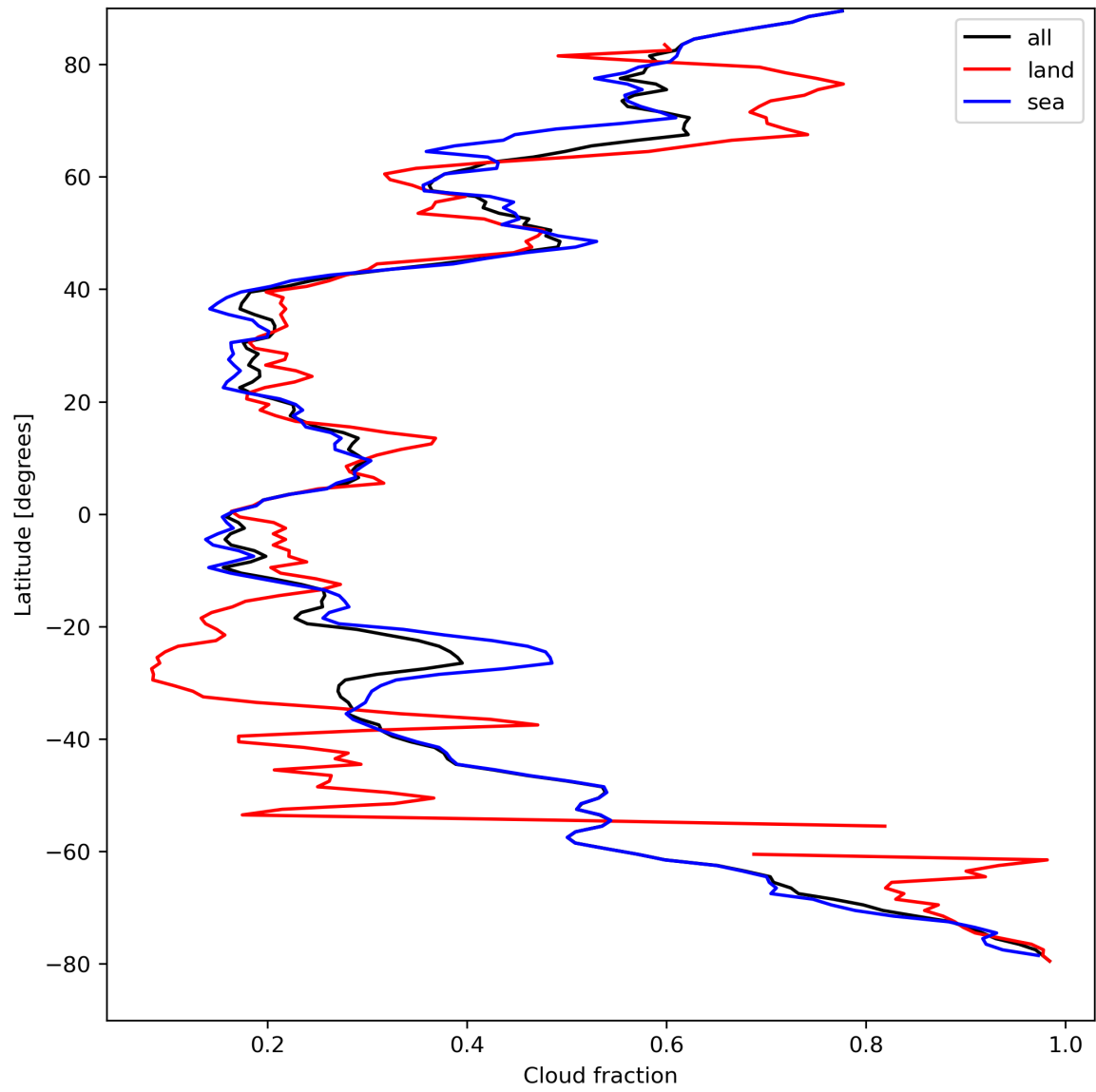
Figure 15: Zonal average of “Cloud fraction” for 2023-08-30 to 2023-08-31.
