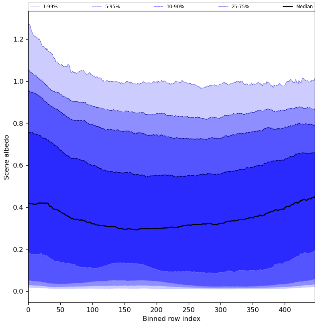
Figure 51: Along track statistics of “Scene albedo” for 2023-08-30 to 2023-08-31
