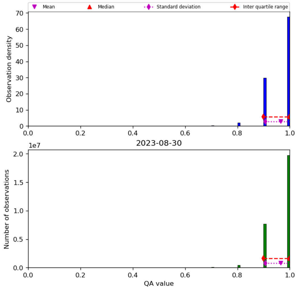
Figure 29: Histogram of “QA value” for 2023-08-30 to 2023-08-31
