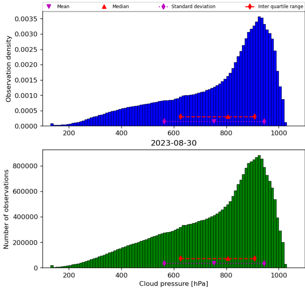
Figure 30: Histogram of “Cloud pressure” for 2023-08-30 to 2023-08-31
