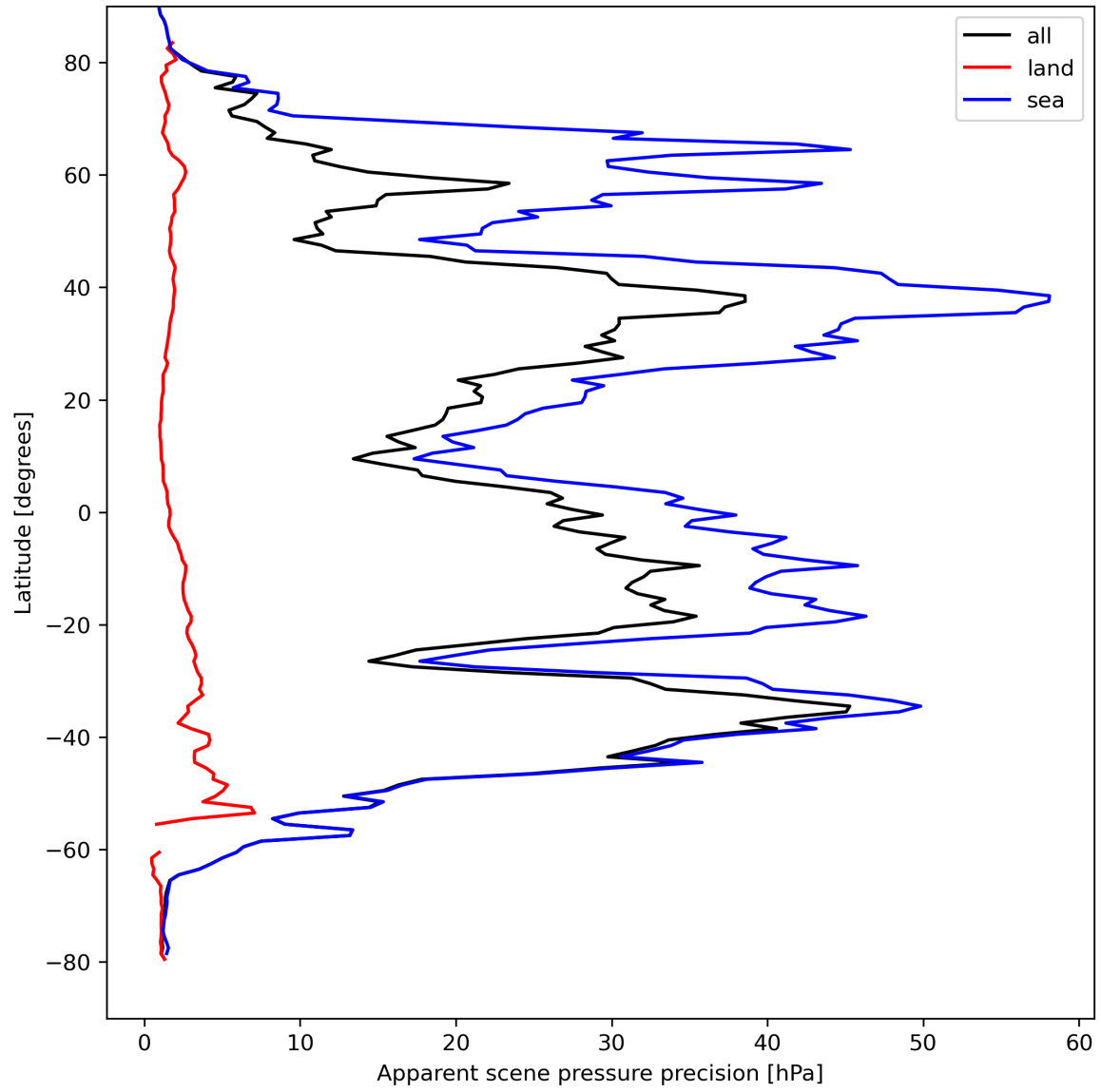
Figure 20: Zonal average of “Apparent scene pressure precision” for 2023-08-30 to 2023-08-31.
