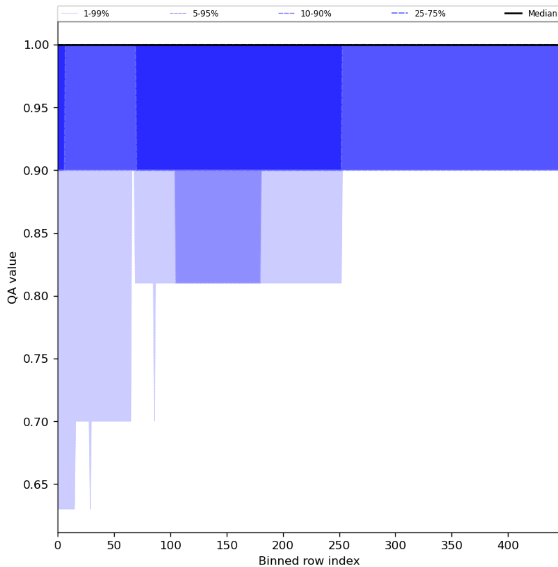
Figure 46: Along track statistics of “QA value” for 2023-08-30 to 2023-08-31
