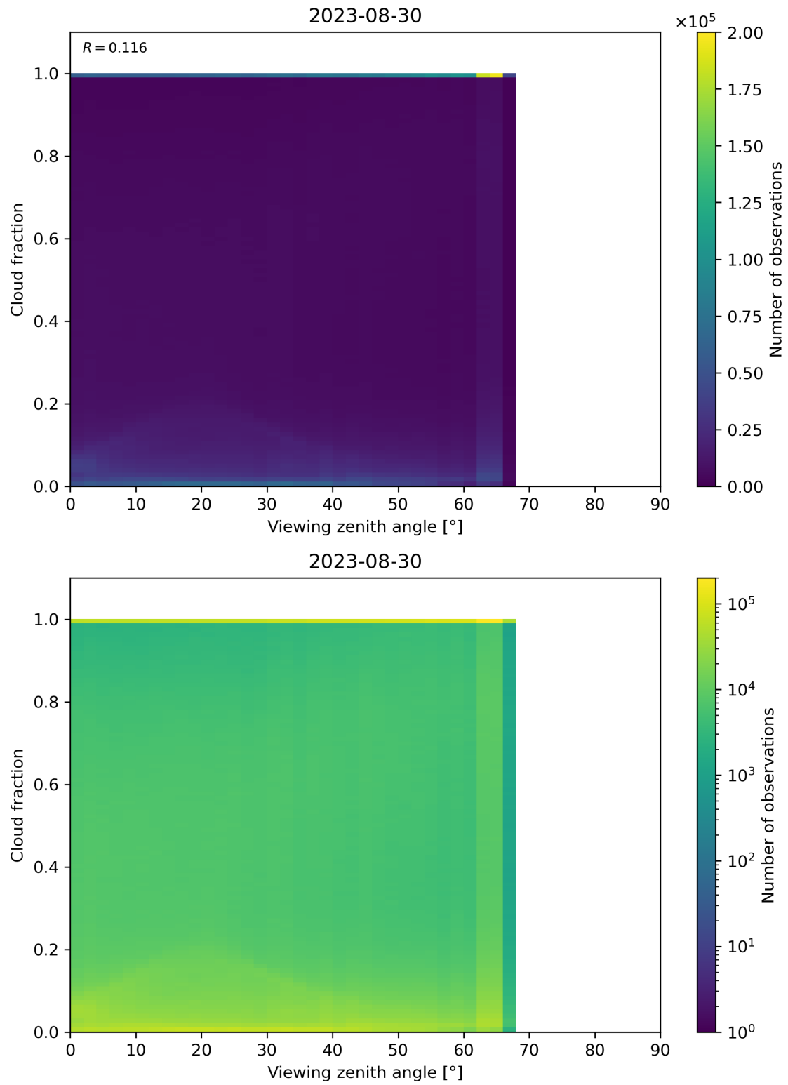
Figure 132: Scatter density plot of “Viewing zenith angle” against “Cloud fraction” for 2023-08-30 to 2023-08-31.
