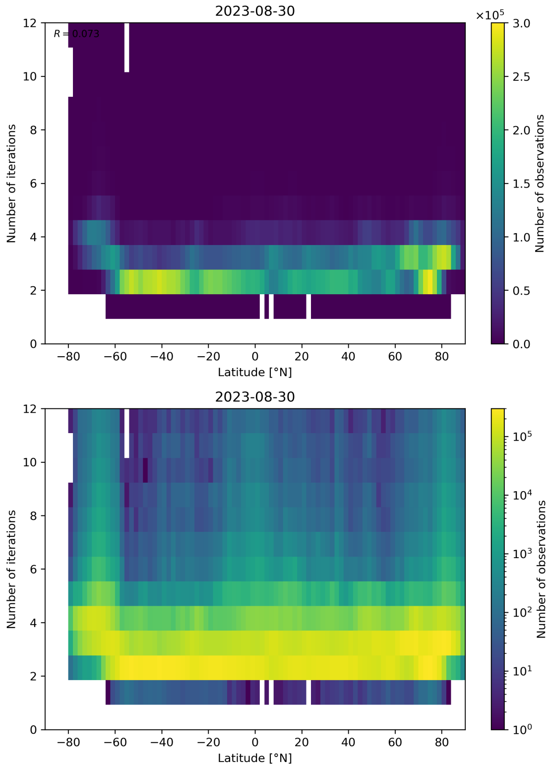
Figure 102: Scatter density plot of “Latitude” against “Number of iterations” for 2023-08-30 to 2023-08-31.
