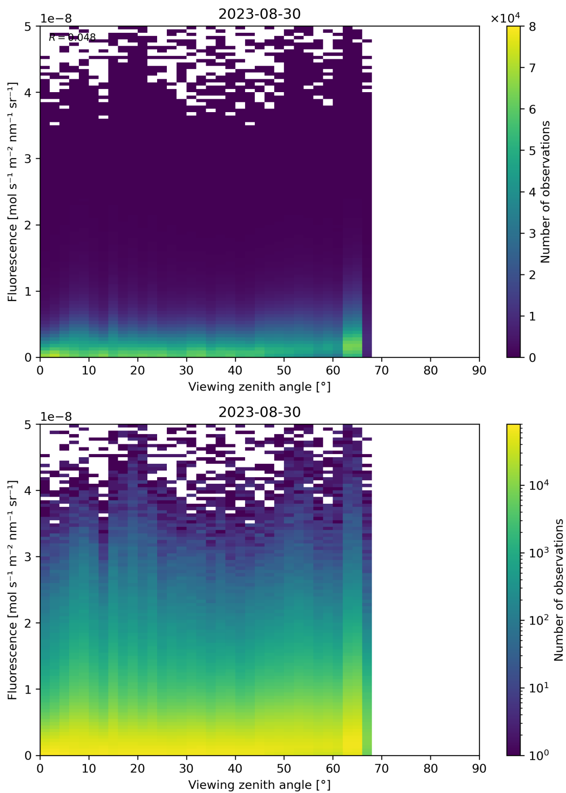
Figure 134: Scatter density plot of “Viewing zenith angle” against “Fluorescence” for 2023-08-30 to 2023-08-31.
