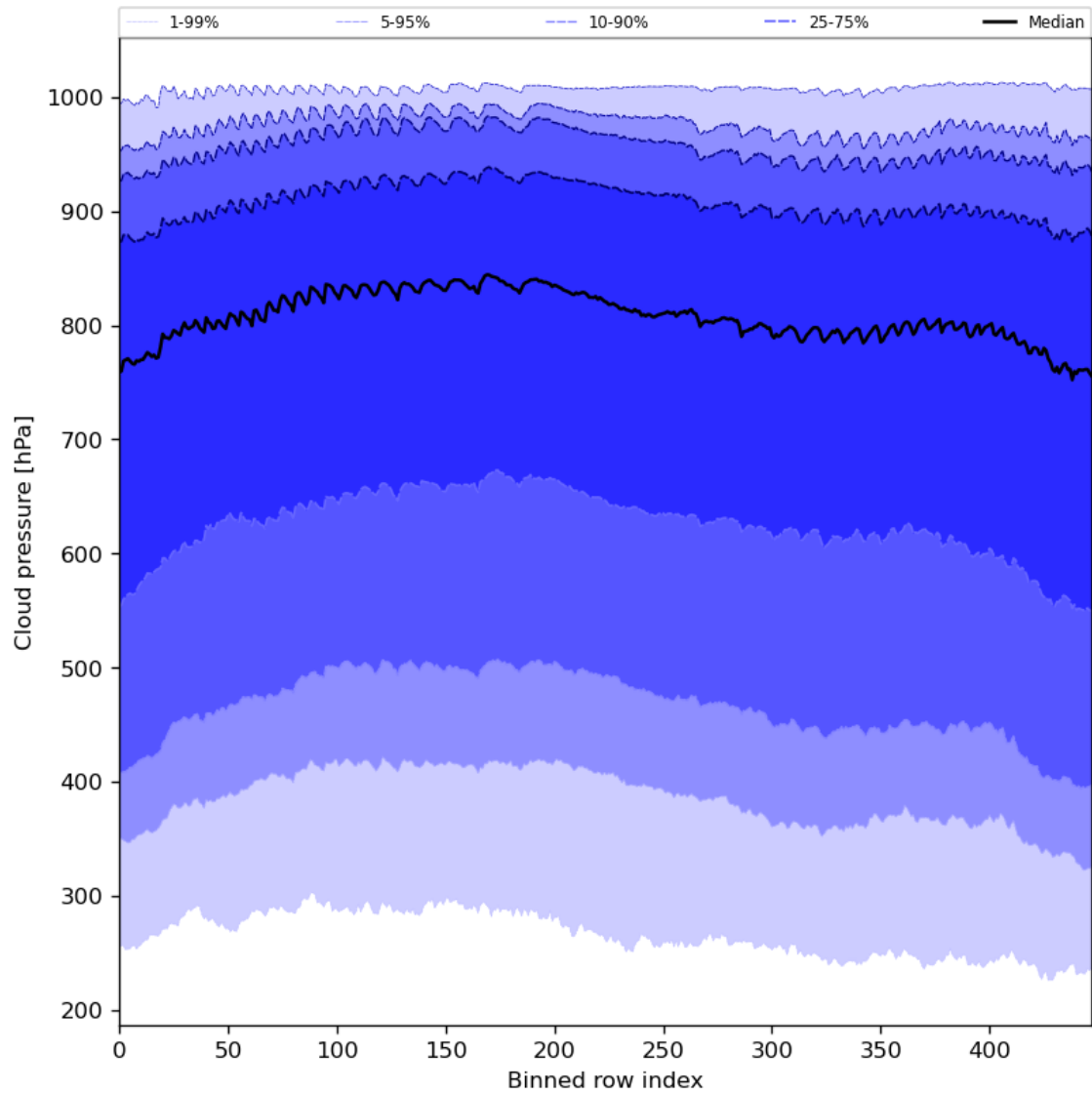
Figure 47: Along track statistics of “Cloud pressure” for 2023-08-30 to 2023-08-31
