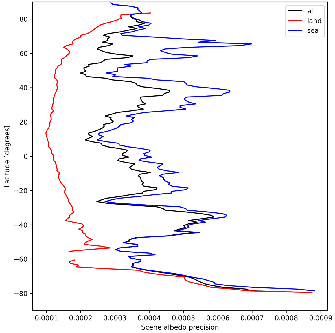
Figure 18: Zonal average of “Scene albedo precision” for 2023-08-30 to 2023-08-31.
