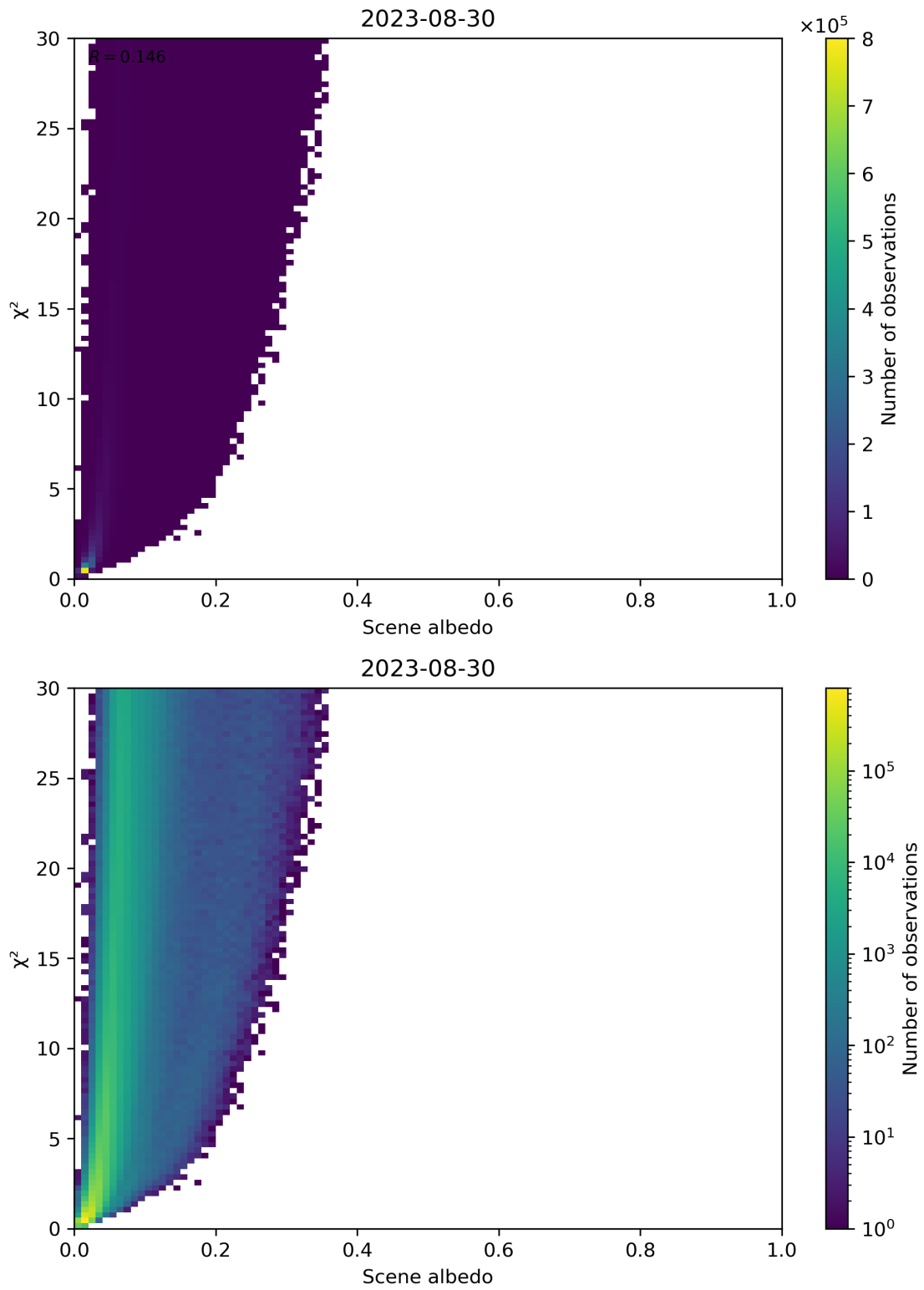
Figure 112: Scatter density plot of “Scene albedo” against “ \chi^2 ” for 2023-08-30 to 2023-08-31.
