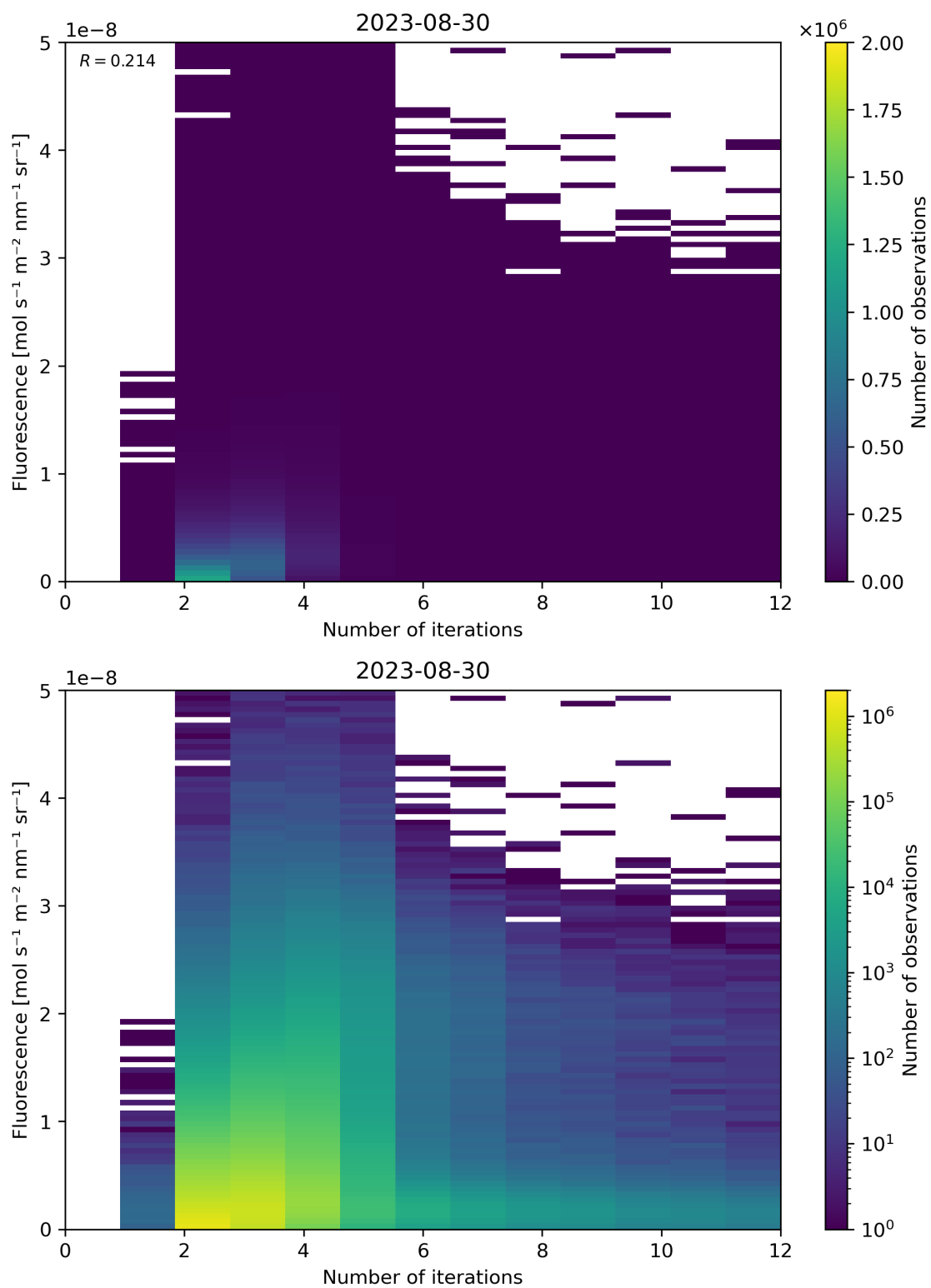
Figure 107: Scatter density plot of “Number of iterations” against “Fluorescence” for 2023-08-30 to 2023-08-31.
