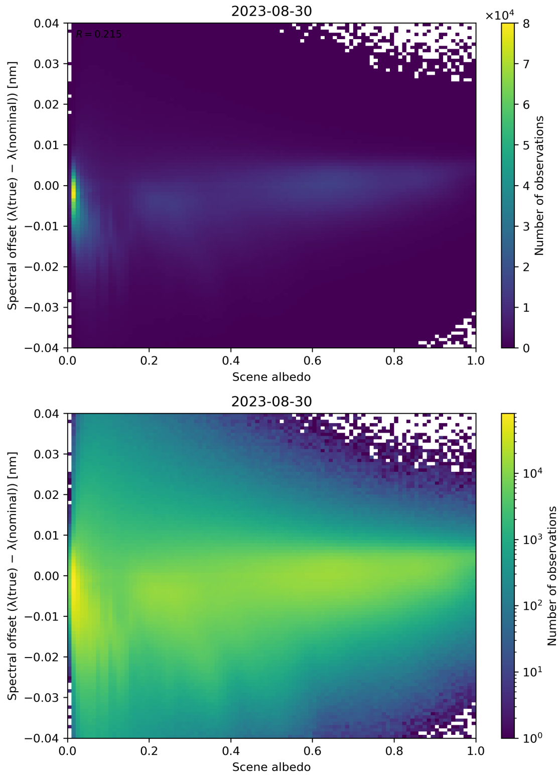
Figure 117: Scatter density plot of “Scene albedo” against “Spectral offset ( \lambda(\text{true}) - \lambda(\text{nominal}) )” for 2023-08-30 to 2023-08-31.
