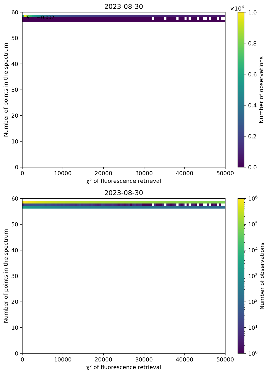
Figure 71: Scatter density plot of " \chi^2 of fluorescence retrieval" against "Number of points in the spectrum" for 2023-08-30 to 2023-08-31.
