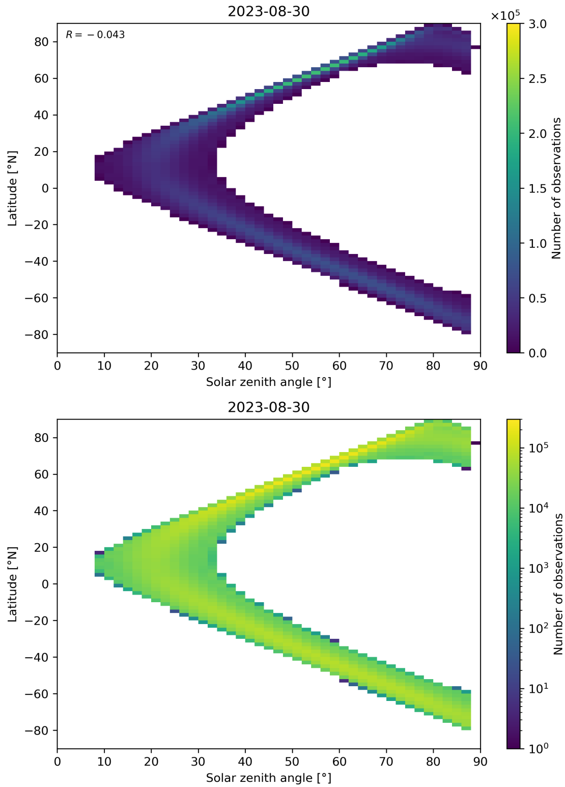
Figure 124: Scatter density plot of “Solar zenith angle” against “Latitude” for 2023-08-30 to 2023-08-31.
