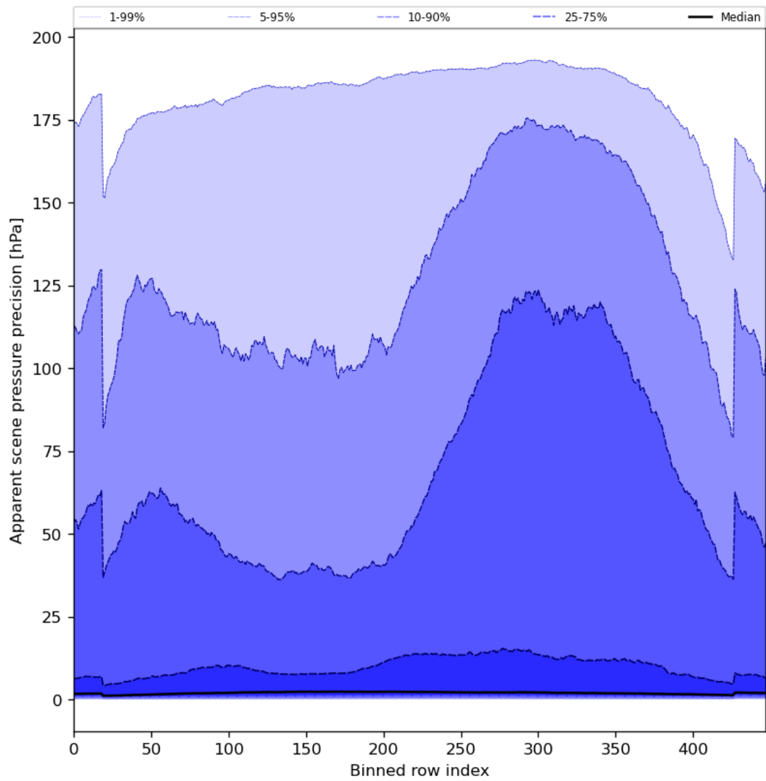
Figure 54: Along track statistics of “Apparent scene pressure precision” for 2023-08-30 to 2023-08-31
