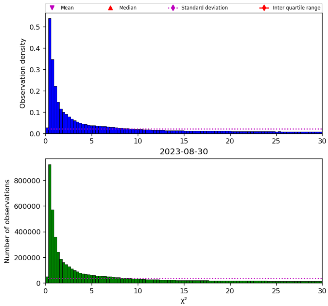
Figure 38: Histogram of “ \chi^2 ” for 2023-08-30 to 2023-08-31
