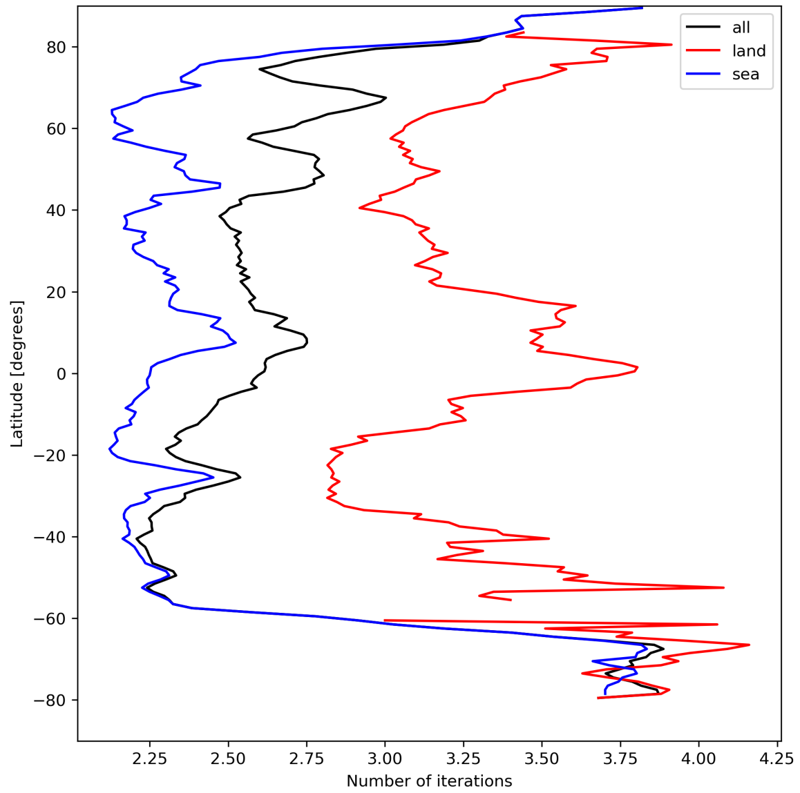
Figure 22: Zonal average of “Number of iterations” for 2023-08-30 to 2023-08-31.
