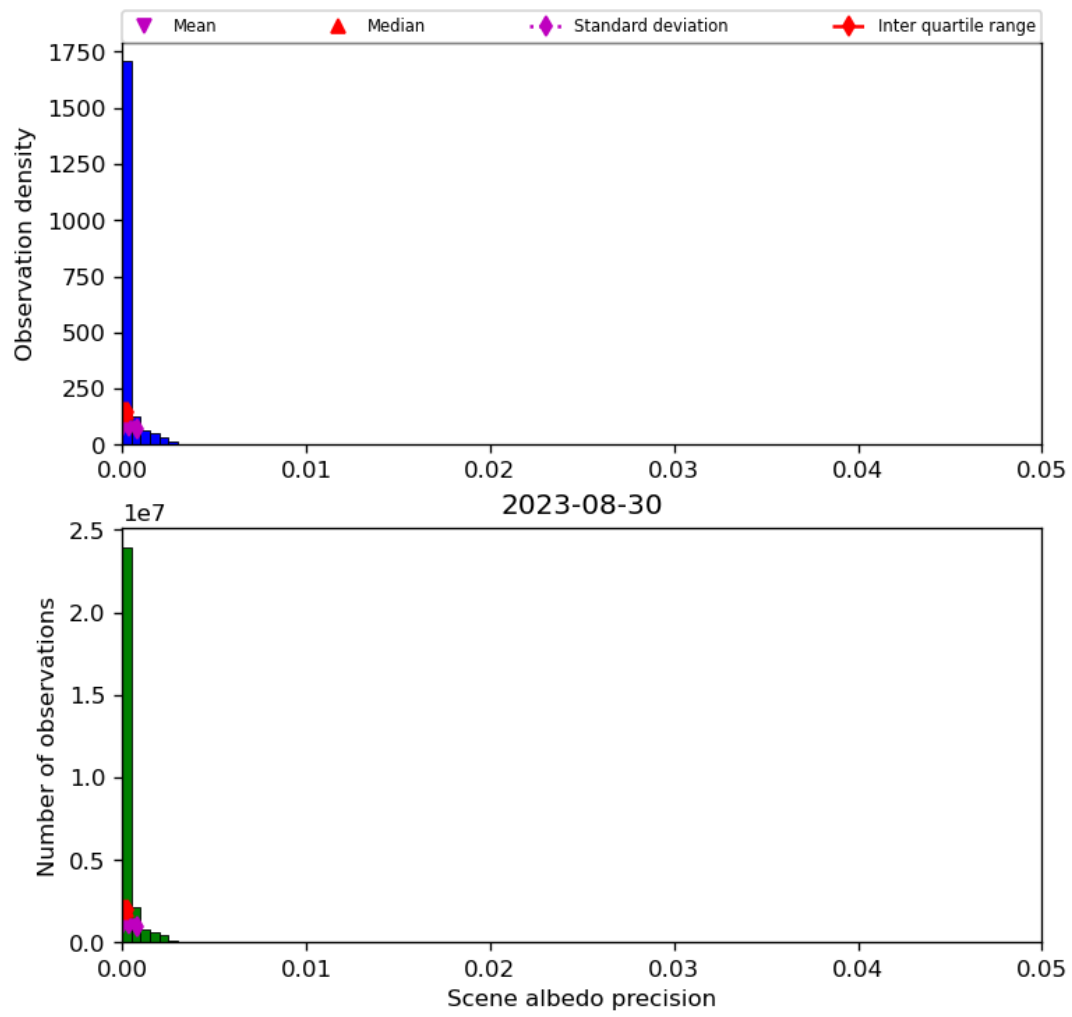
Figure 35: Histogram of “Scene albedo precision” for 2023-08-30 to 2023-08-31
