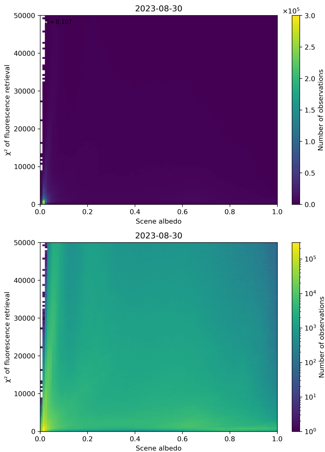
Figure 113: Scatter density plot of “Scene albedo” against “ \chi^2 of fluorescence retrieval” for 2023-08-30 to 2023-08-31.
