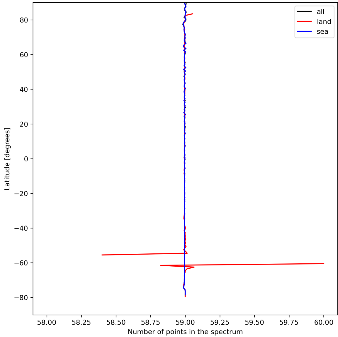
Figure 27: Zonal average of “Number of points in the spectrum” for 2023-08-30 to 2023-08-31.
