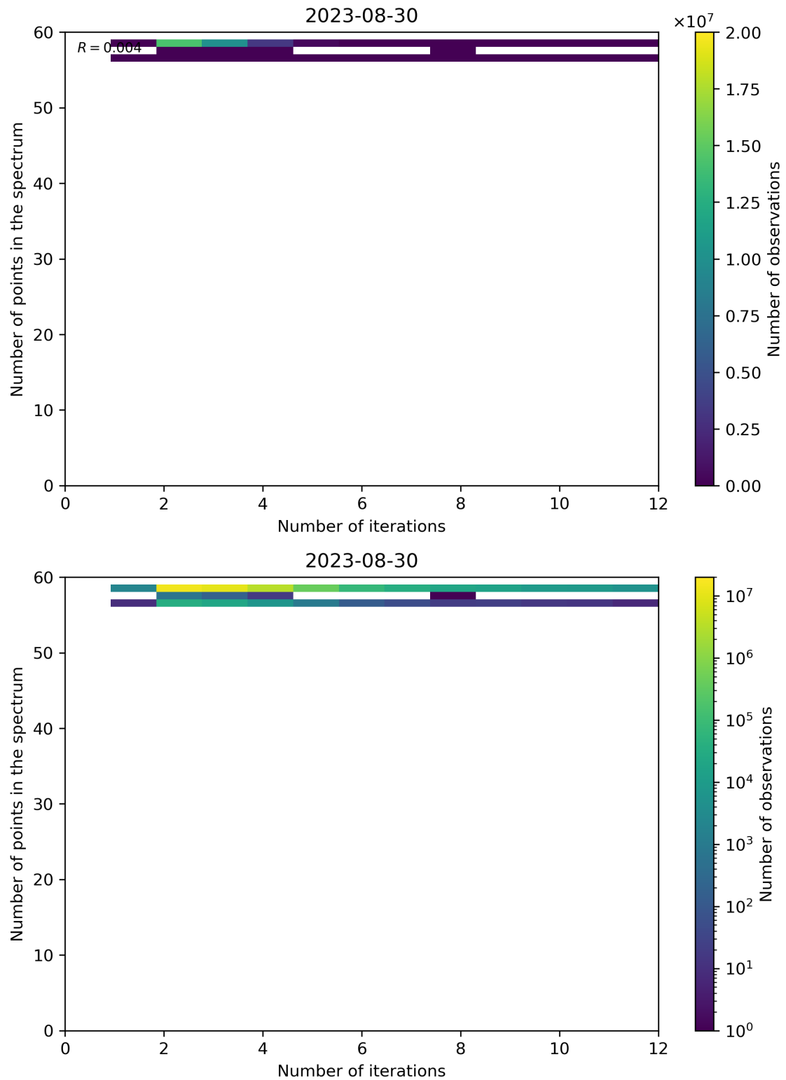
Figure 108: Scatter density plot of “Number of iterations” against “Number of points in the spectrum” for 2023-08-30 to 2023-08-31.
