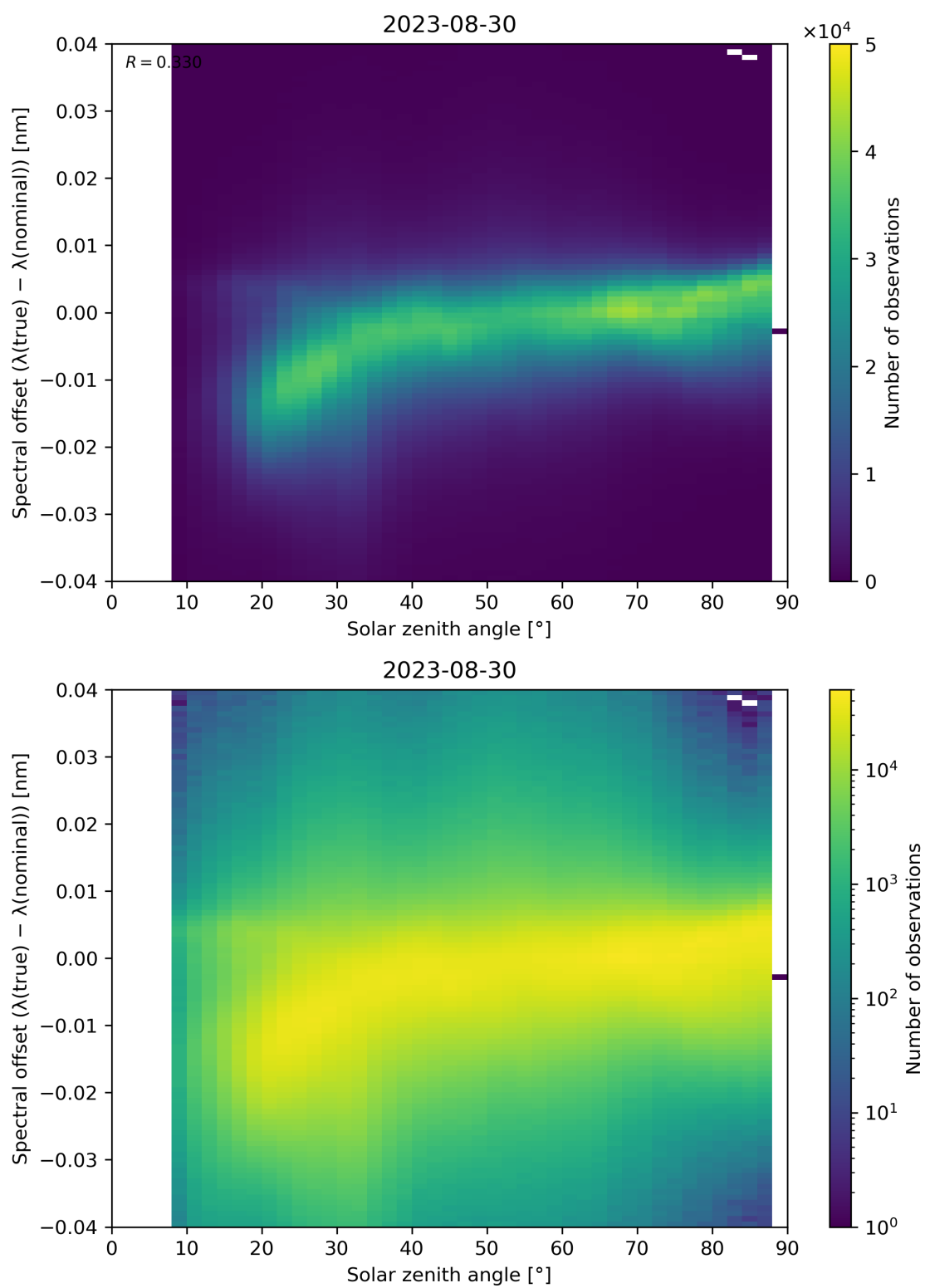
Figure 128: Scatter density plot of “Solar zenith angle” against “Spectral offset ( \lambda(\text{true}) - \lambda(\text{nominal}) )” for 2023-08-30 to 2023-08-31.
