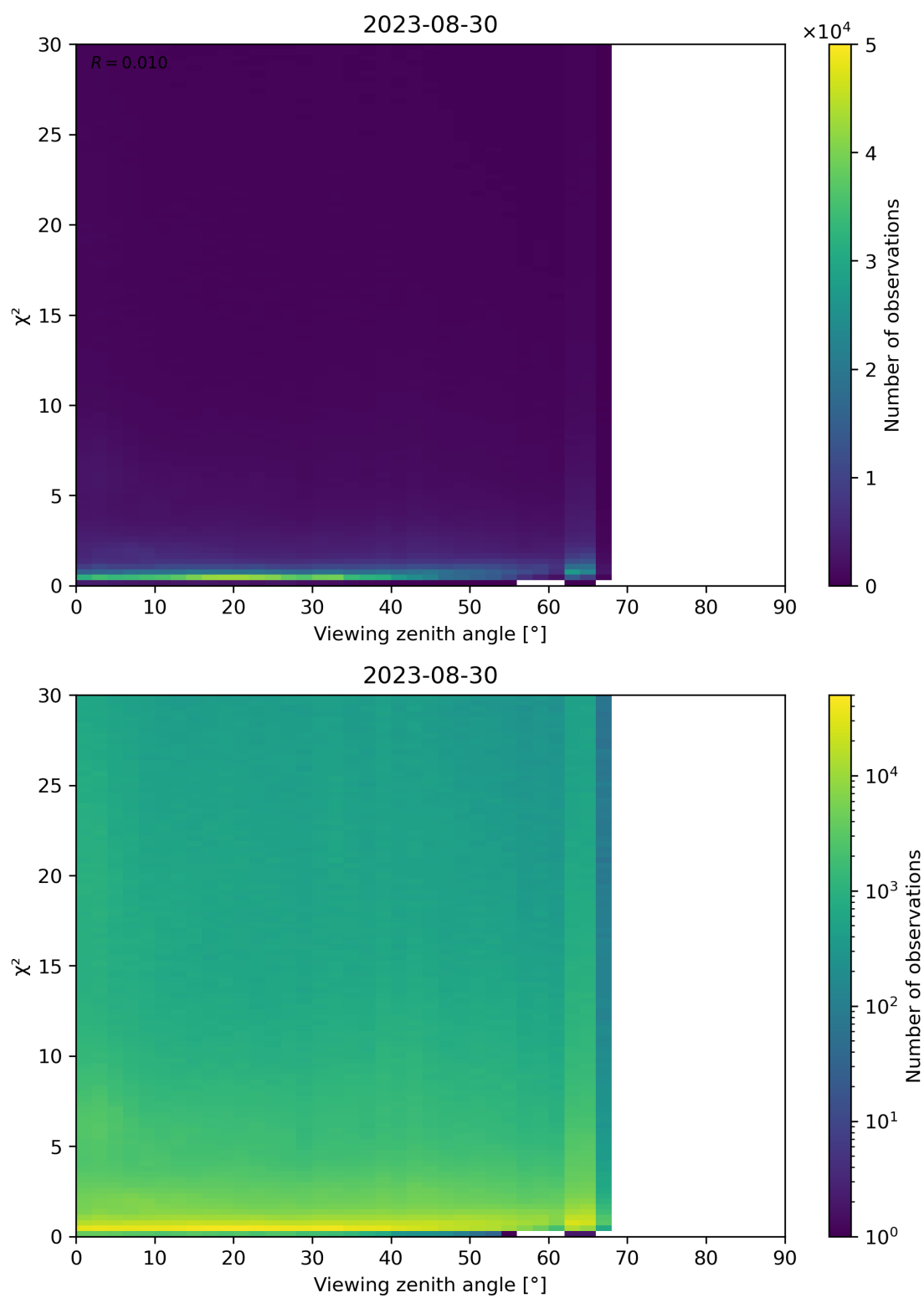
Figure 130: Scatter density plot of “Viewing zenith angle” against “ \chi^2 ” for 2023-08-30 to 2023-08-31.
