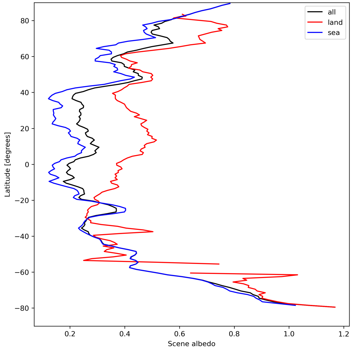
Figure 17: Zonal average of “Scene albedo” for 2023-08-30 to 2023-08-31.
