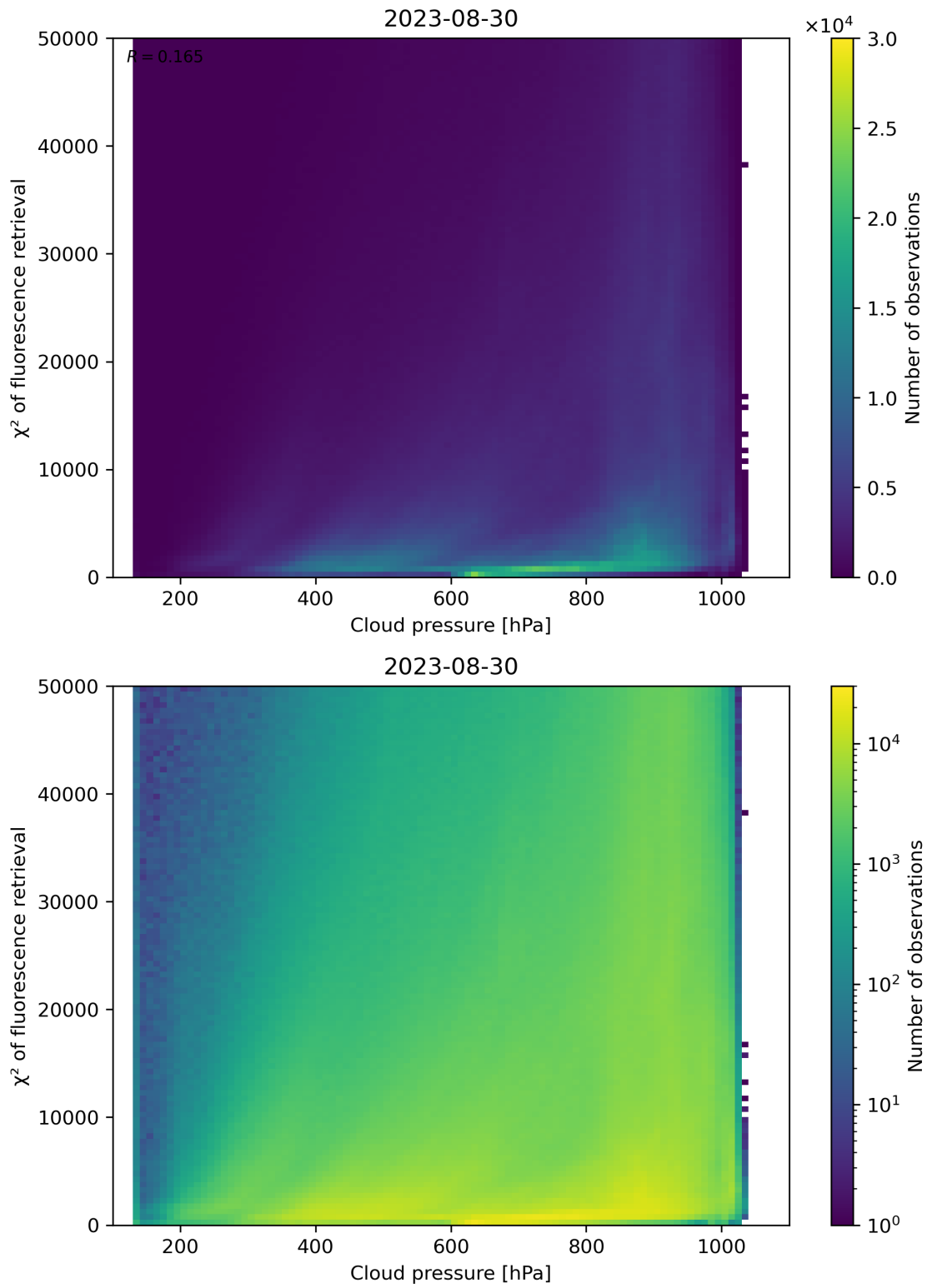
Figure 86: Scatter density plot of “Cloud pressure” against “ \chi^2 of fluorescence retrieval” for 2023-08-30 to 2023-08-31.
