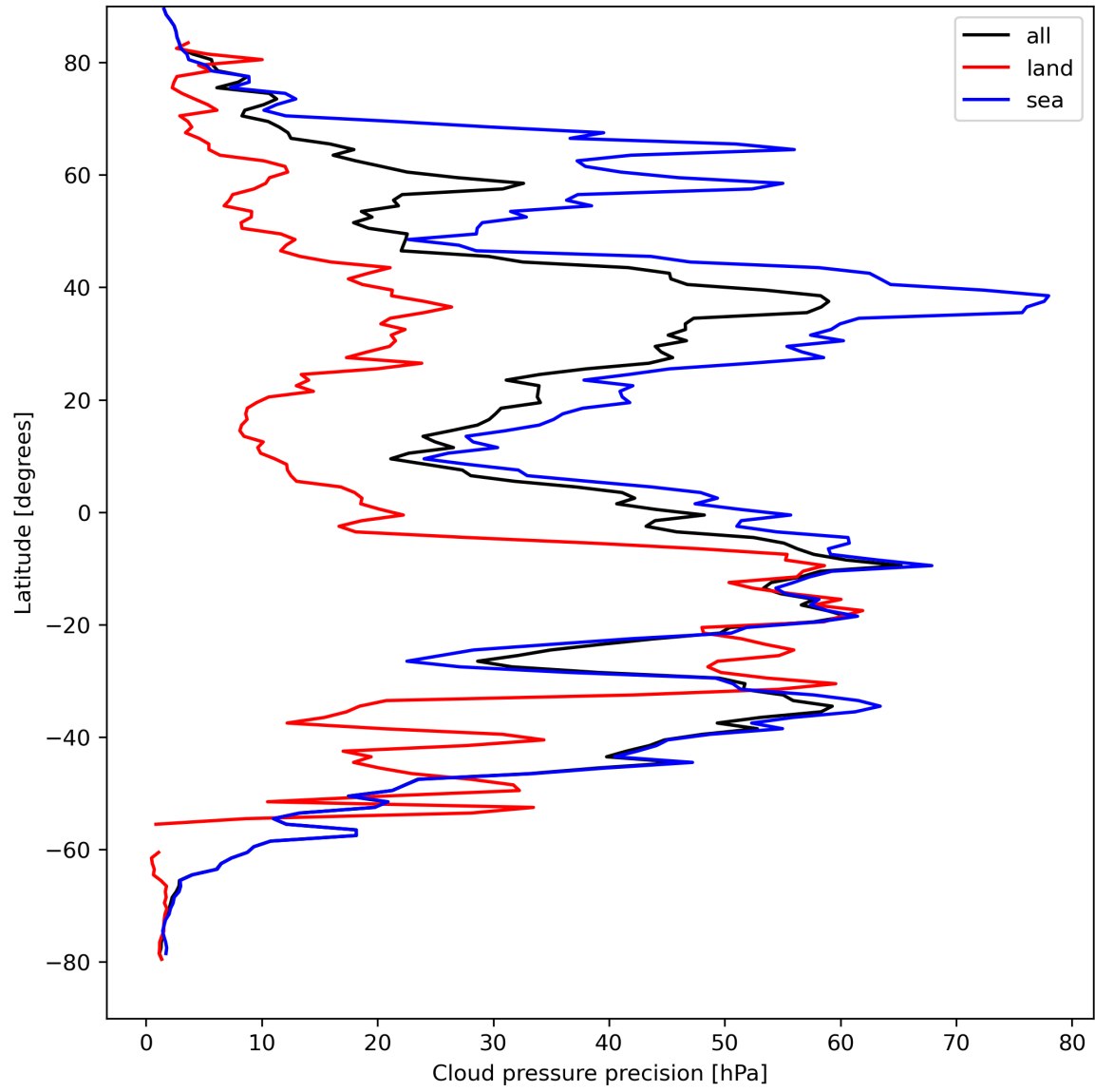
Figure 14: Zonal average of “Cloud pressure precision” for 2023-08-30 to 2023-08-31.
