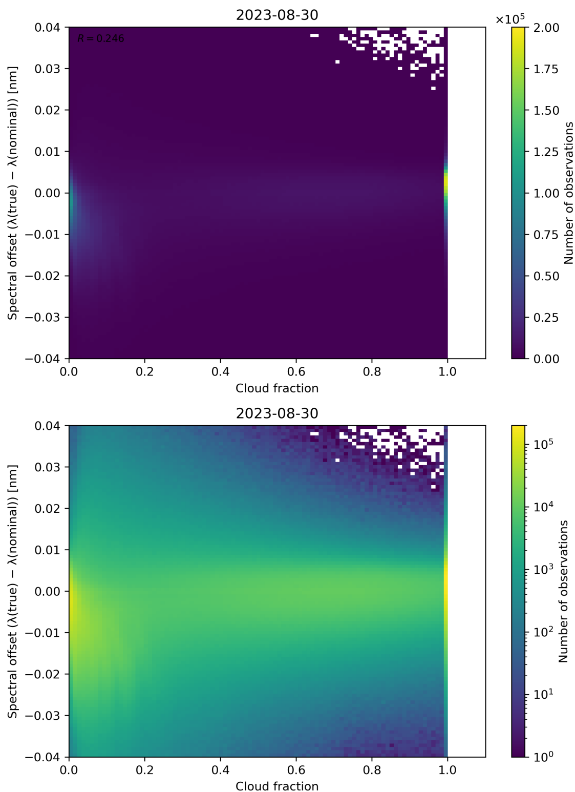
Figure 83: Scatter density plot of “Cloud fraction” against “Spectral offset ( \lambda(\text{true}) - \lambda(\text{nominal}) )” for 2023-08-30 to 2023-08-31.
