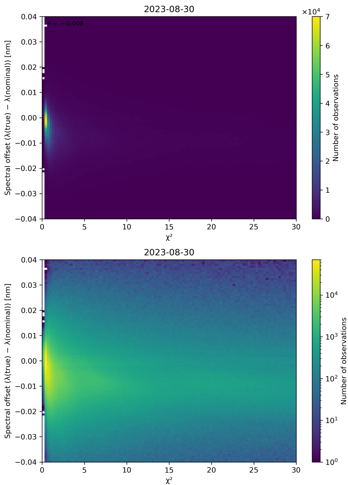
Figure 75: Scatter density plot of “ \chi^2 ” against “Spectral offset ( \lambda(\text{true}) - \lambda(\text{nominal}) )” for 2023-08-30 to 2023-08-31.
