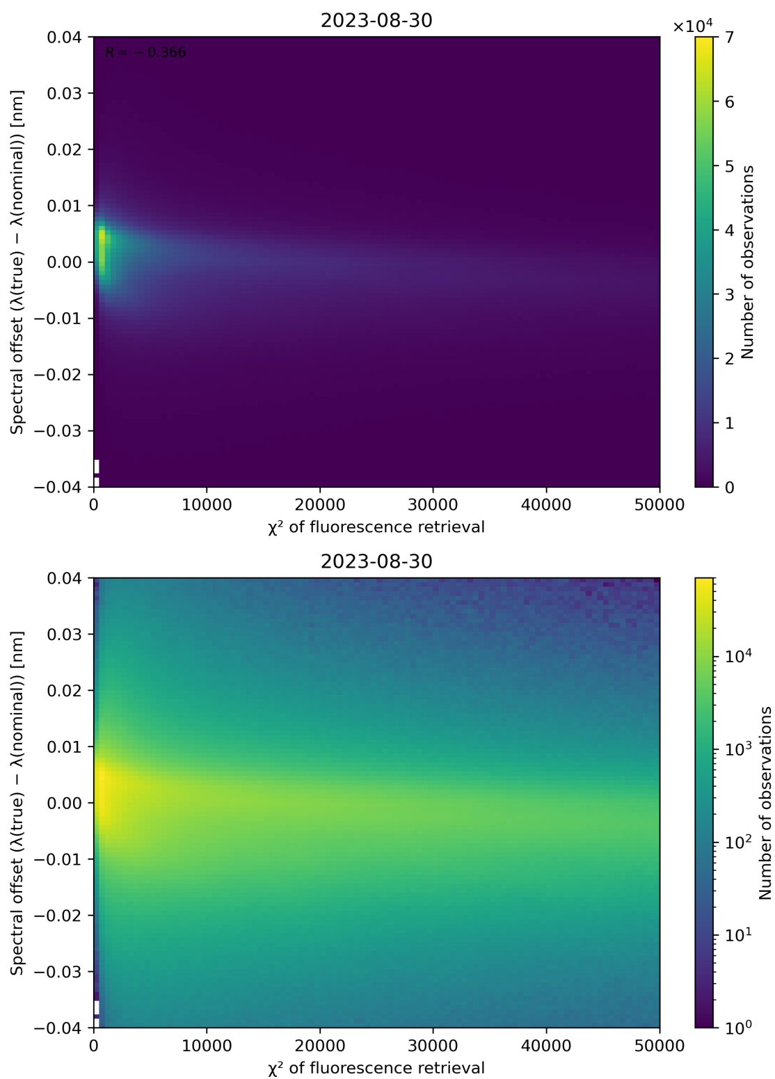
Figure 72: Scatter density plot of " \chi^2 of fluorescence retrieval" against "Spectral offset ( \lambda(\text{true}) - \lambda(\text{nominal}) )" for 2023-08-30 to 2023-08-31.
