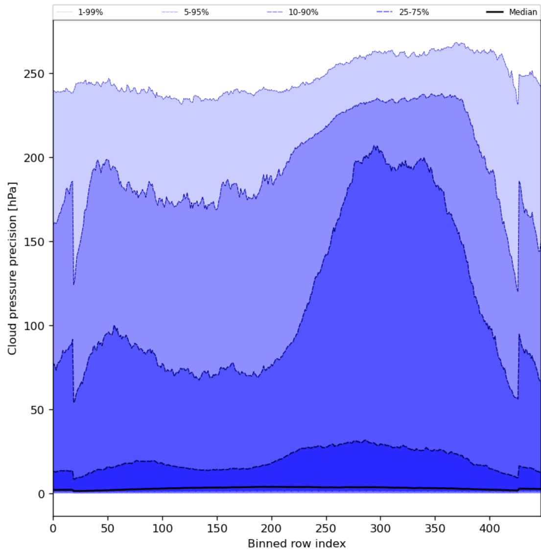
Figure 48: Along track statistics of “Cloud pressure precision” for 2023-08-30 to 2023-08-31
