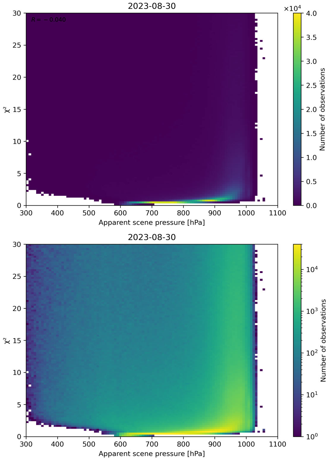
Figure 63: Scatter density plot of “Apparent scene pressure” against “ \chi^2 ” for 2023-08-30 to 2023-08-31.
