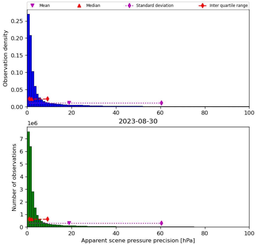
Figure 37: Histogram of “Apparent scene pressure precision” for 2023-08-30 to 2023-08-31
