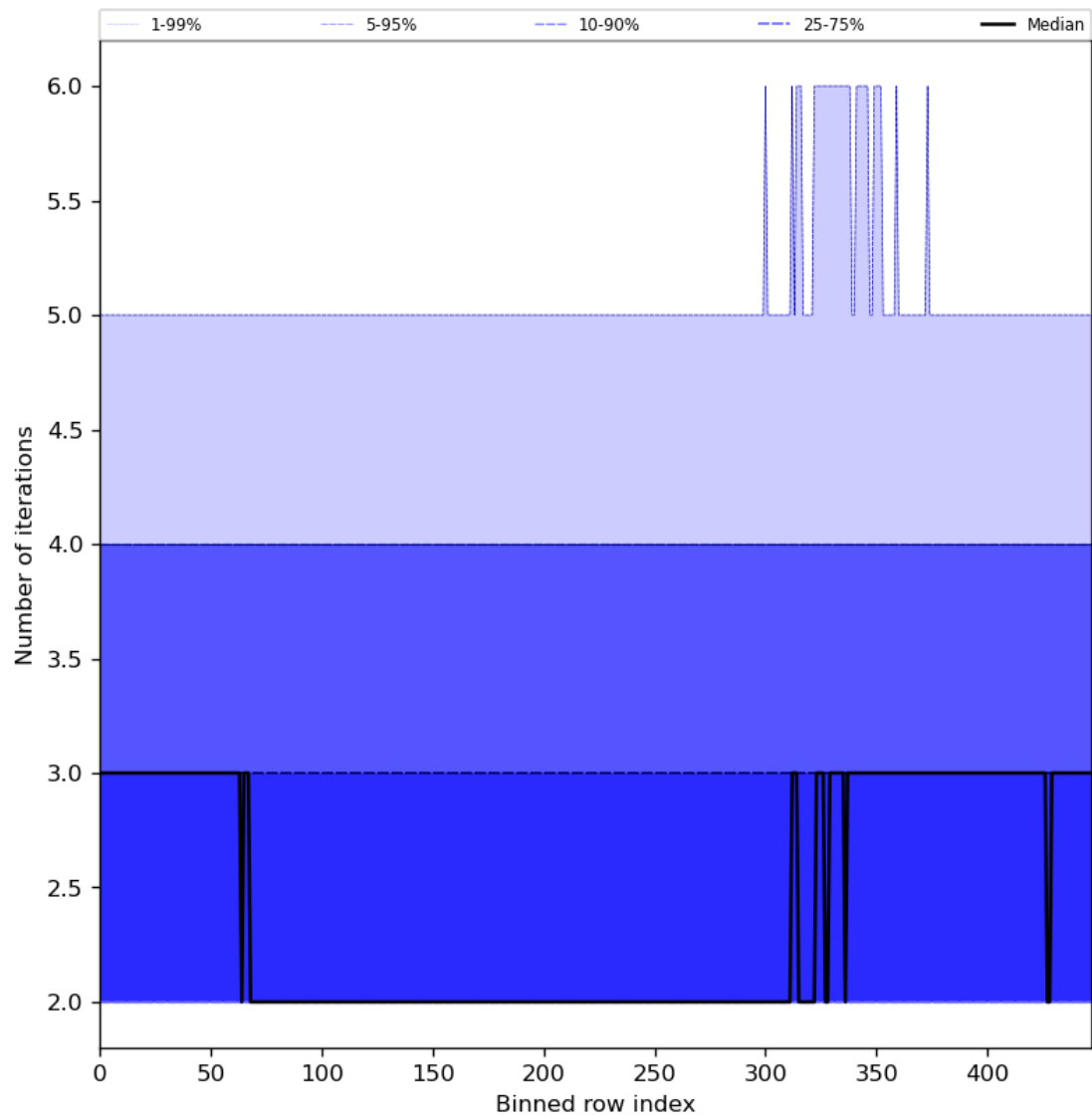
Figure 56: Along track statistics of “Number of iterations” for 2023-08-30 to 2023-08-31
