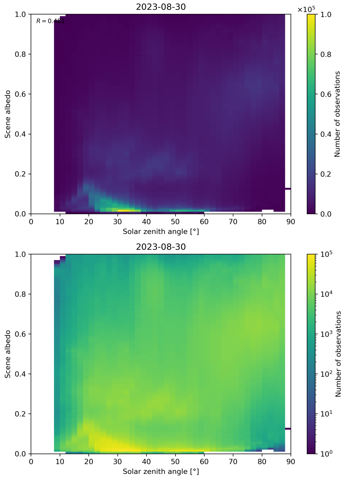
Figure 127: Scatter density plot of “Solar zenith angle” against “Scene albedo” for 2023-08-30 to 2023-08-31.
