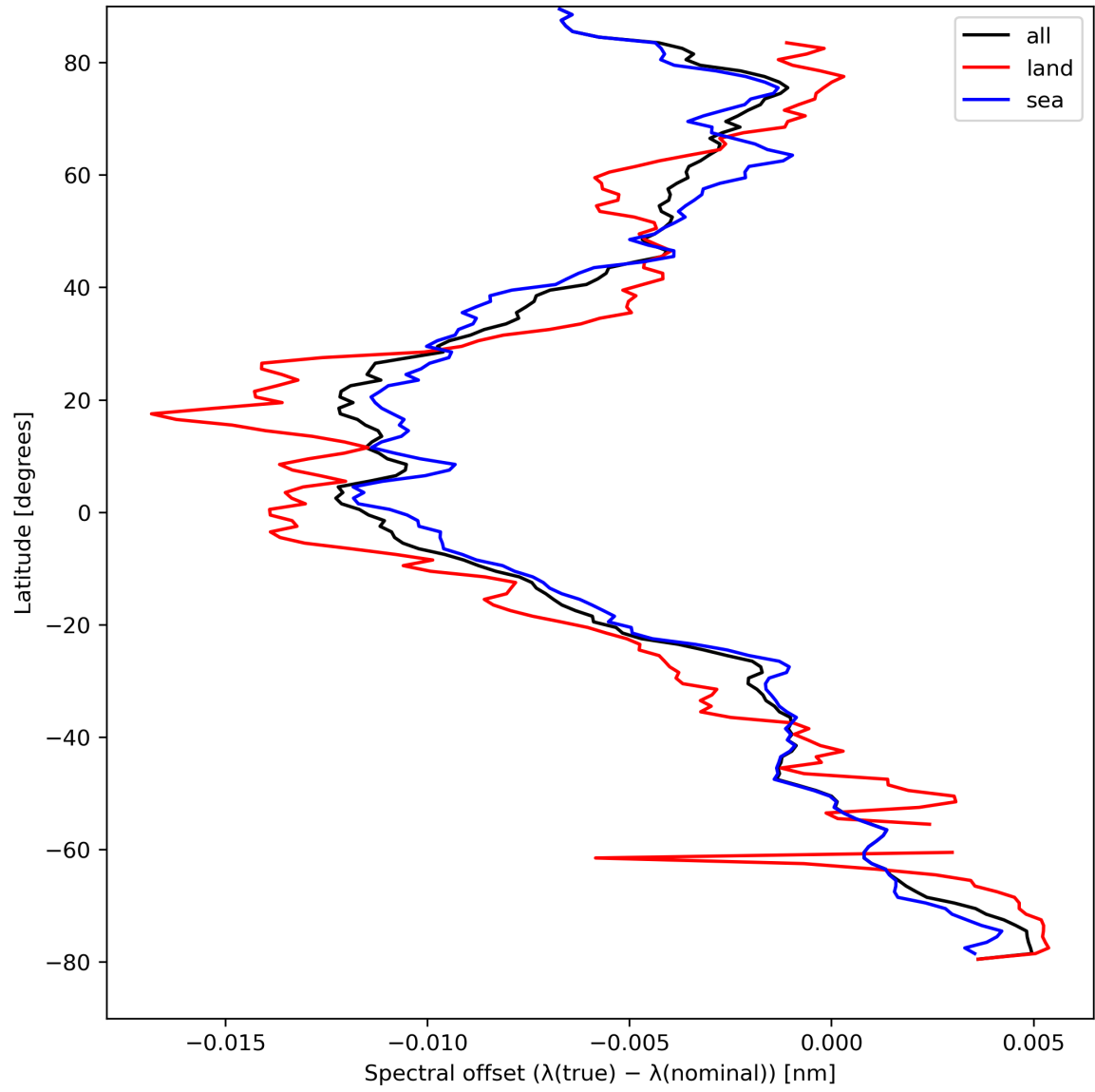
Figure 28: Zonal average of “Spectral offset ( \lambda(\text{true}) - \lambda(\text{nominal}) )” for 2023-08-30 to 2023-08-31.
