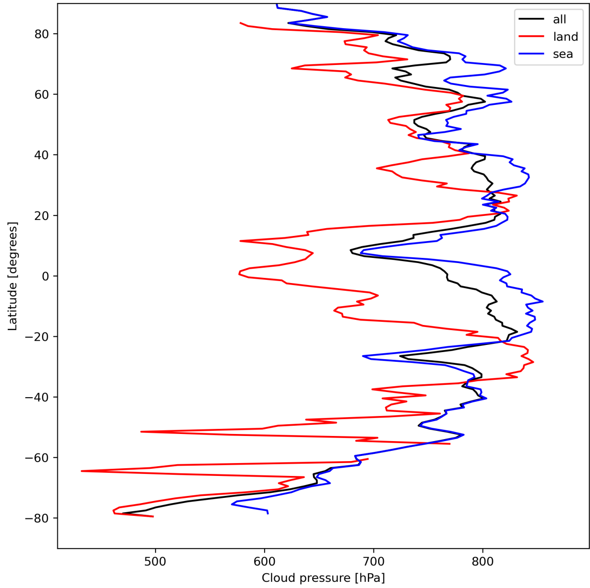
Figure 13: Zonal average of “Cloud pressure” for 2023-08-30 to 2023-08-31.
