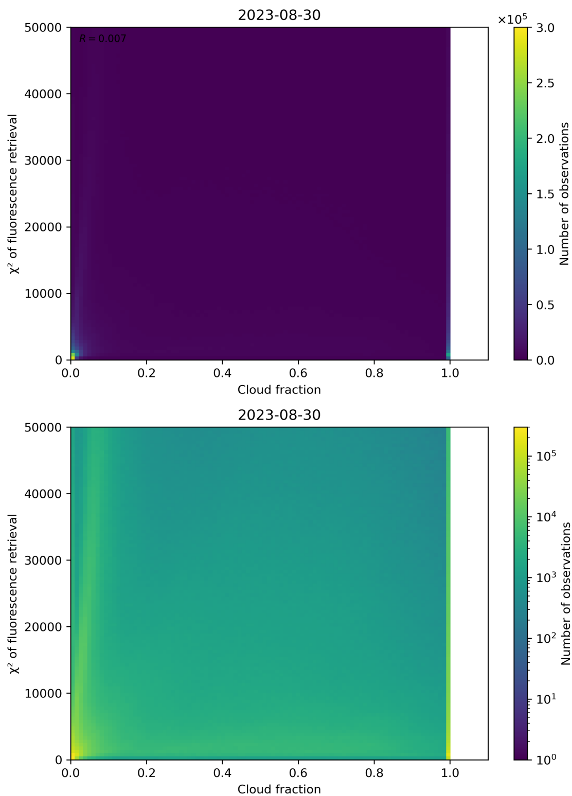
Figure 78: Scatter density plot of “Cloud fraction” against “ \chi^2 of fluorescence retrieval” for 2023-08-30 to 2023-08-31.
