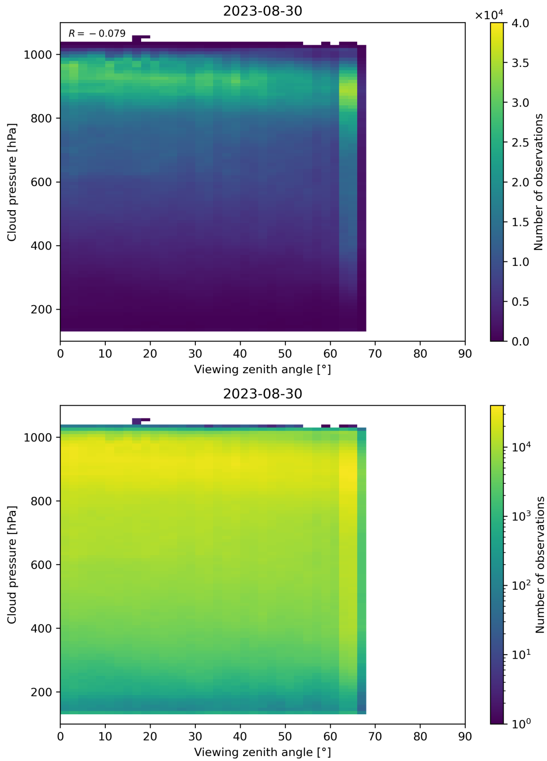
Figure 133: Scatter density plot of “Viewing zenith angle” against “Cloud pressure” for 2023-08-30 to 2023-08-31.
