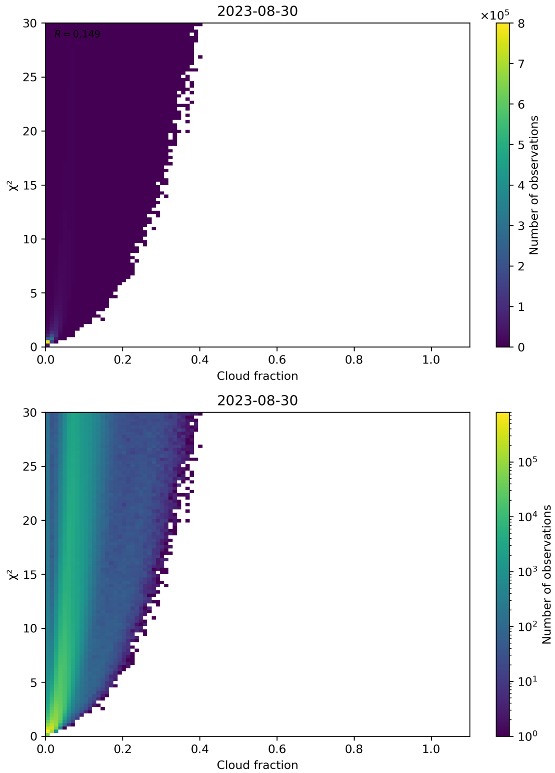
Figure 77: Scatter density plot of “Cloud fraction” against “ \chi^2 ” for 2023-08-30 to 2023-08-31.
