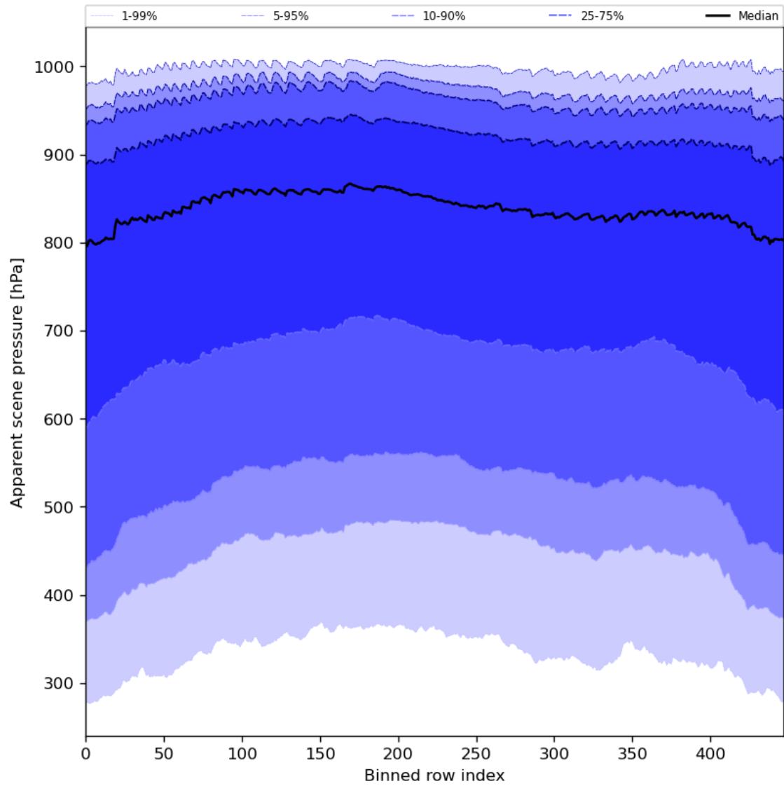
Figure 53: Along track statistics of “Apparent scene pressure” for 2023-08-30 to 2023-08-31
