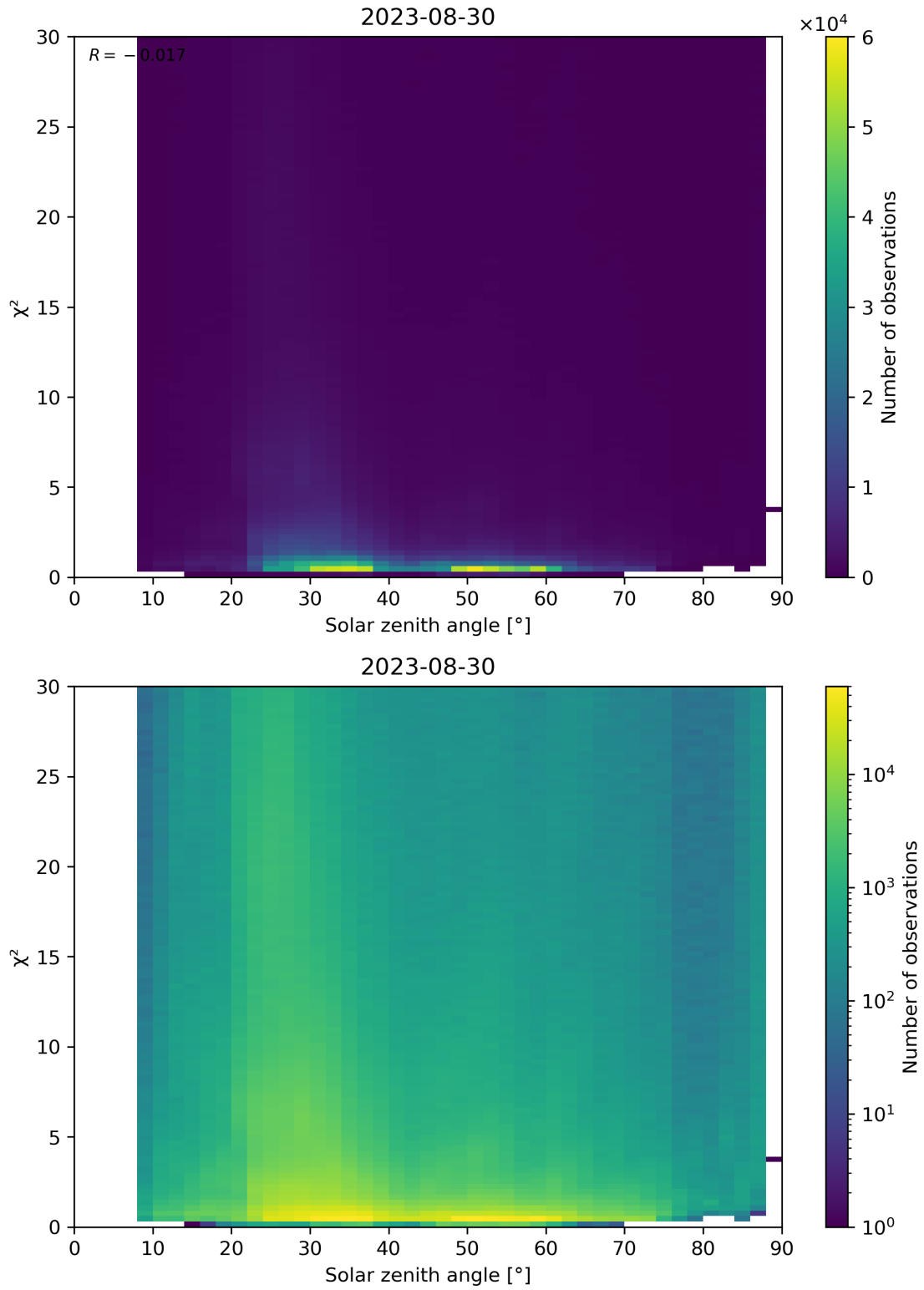
Figure 119: Scatter density plot of “Solar zenith angle” against “ \chi^2 ” for 2023-08-30 to 2023-08-31.
