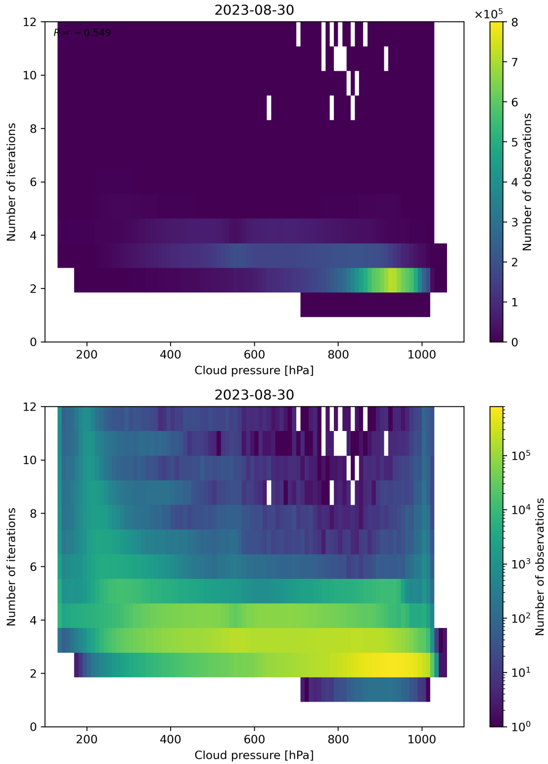
Figure 89: Scatter density plot of “Cloud pressure” against “Number of iterations” for 2023-08-30 to 2023-08-31.
