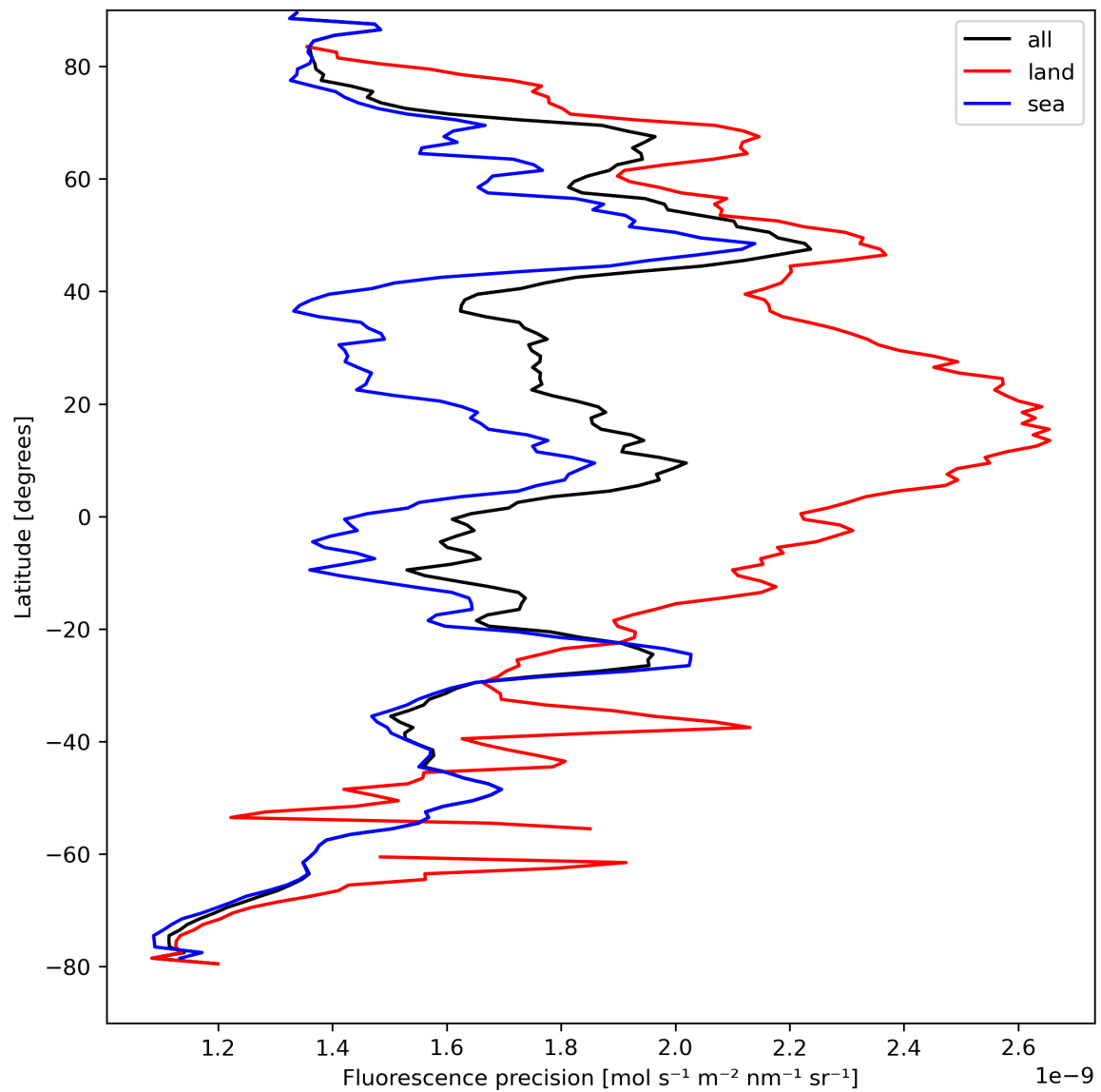
Figure 24: Zonal average of “Fluorescence precision” for 2023-08-30 to 2023-08-31.
