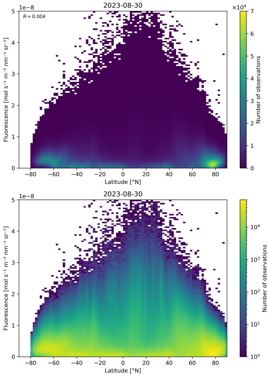
Figure 101: Scatter density plot of “Latitude” against “Fluorescence” for 2023-08-30 to 2023-08-31.
