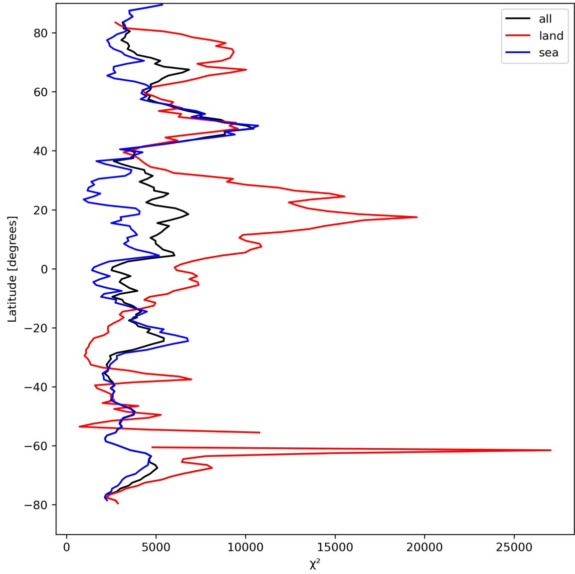
Figure 21: Zonal average of “ \chi^2 ” for 2023-08-30 to 2023-08-31.
