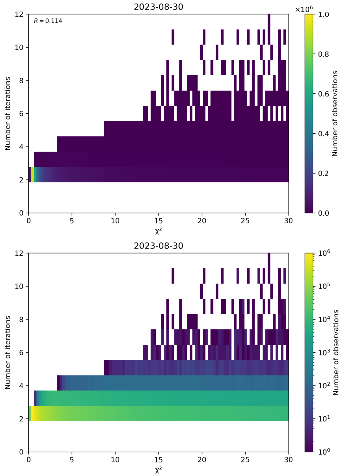
Figure 73: Scatter density plot of " \chi^2 " against "Number of iterations" for 2023-08-30 to 2023-08-31.
