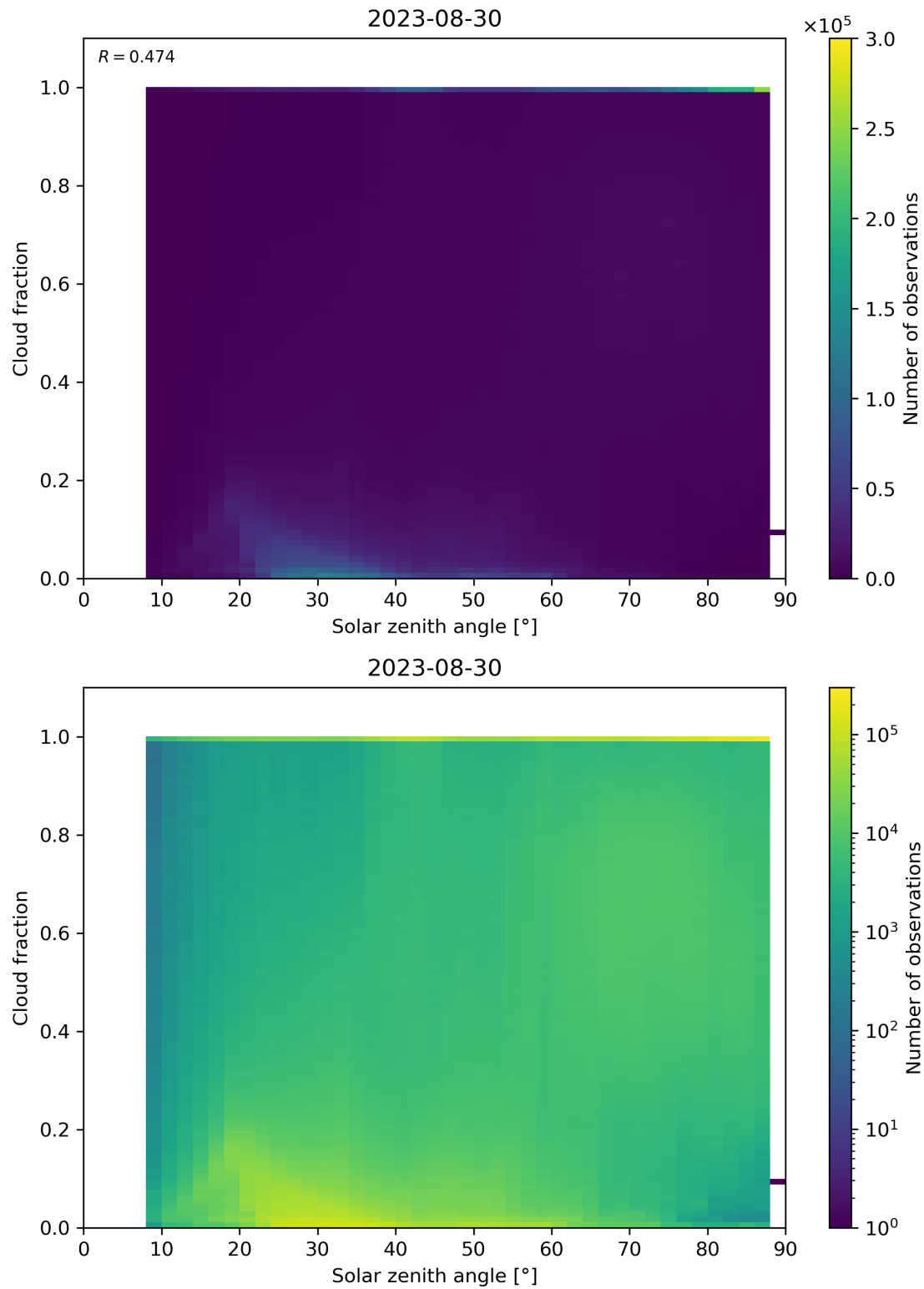
Figure 121: Scatter density plot of “Solar zenith angle” against “Cloud fraction” for 2023-08-30 to 2023-08-31.
