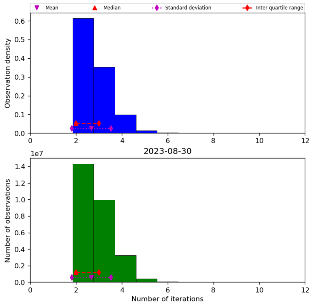
Figure 39: Histogram of “Number of iterations” for 2023-08-30 to 2023-08-31
