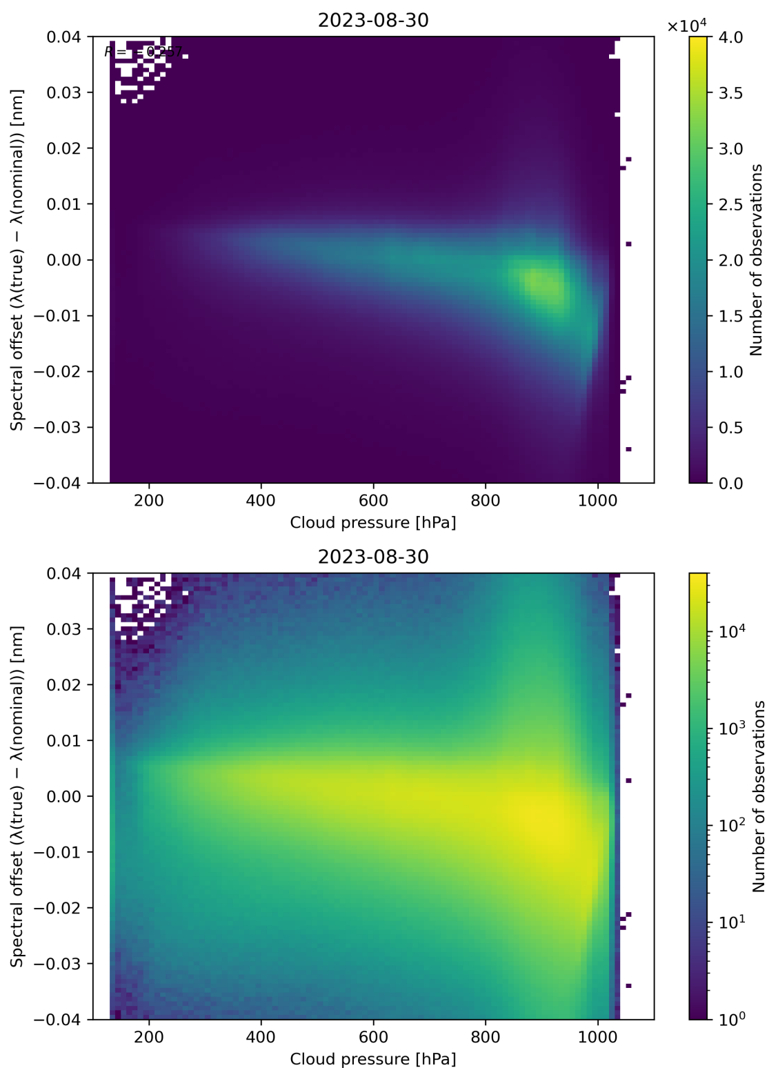
Figure 92: Scatter density plot of “Cloud pressure” against “Spectral offset ( \lambda(\text{true}) - \lambda(\text{nominal}) )” for 2023-08-30 to 2023-08-31.
