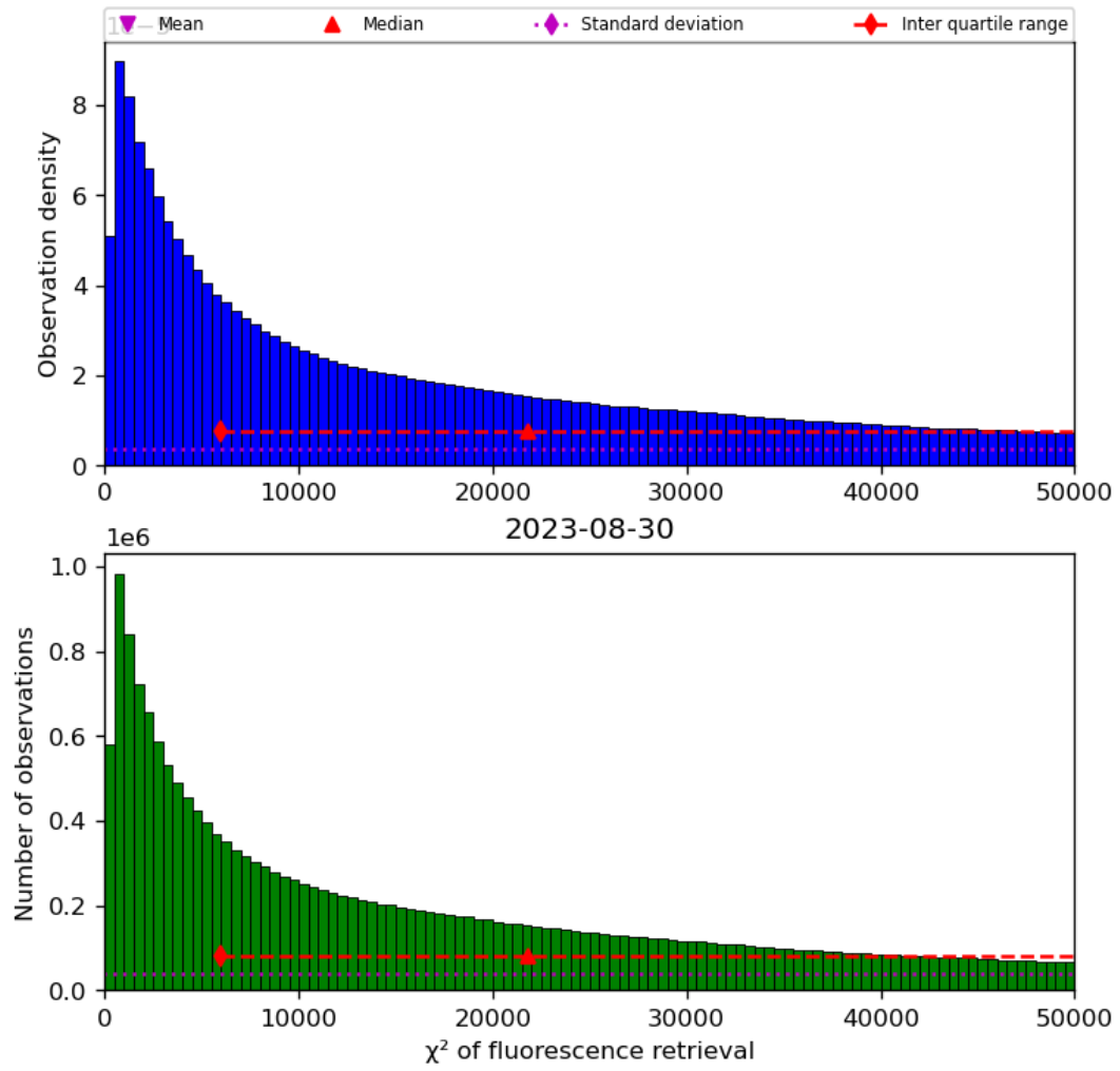
Figure 42: Histogram of “ \chi^2 of fluorescence retrieval” for 2023-08-30 to 2023-08-31
