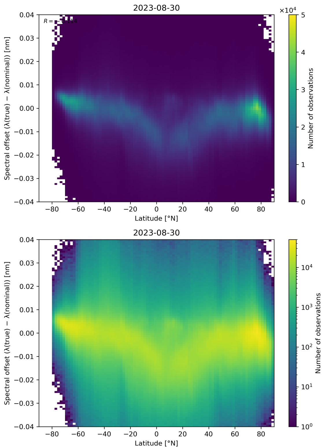
Figure 105: Scatter density plot of “Latitude” against “Spectral offset ( \lambda(\text{true}) - \lambda(\text{nominal}) )” for 2023-08-30 to 2023-08-31.
