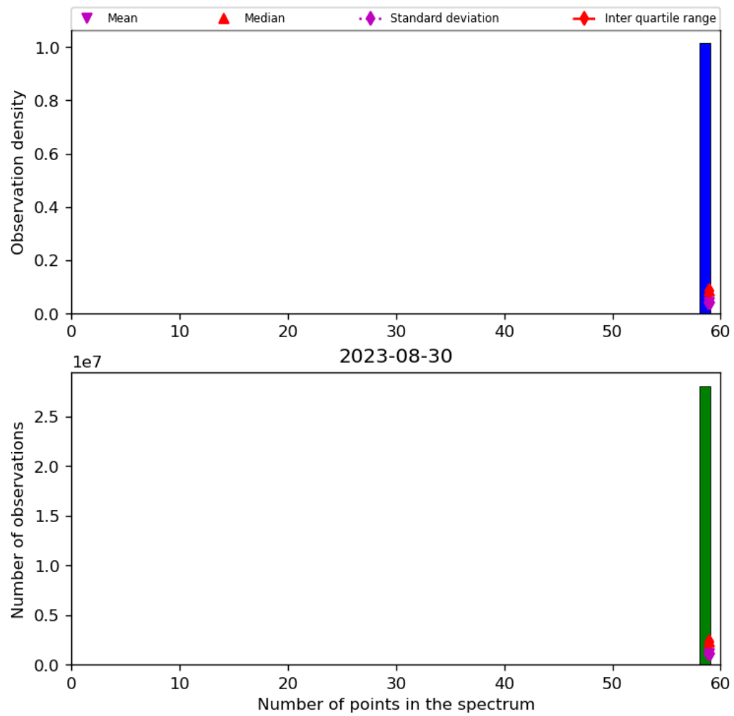
Figure 44: Histogram of “Number of points in the spectrum” for 2023-08-30 to 2023-08-31
