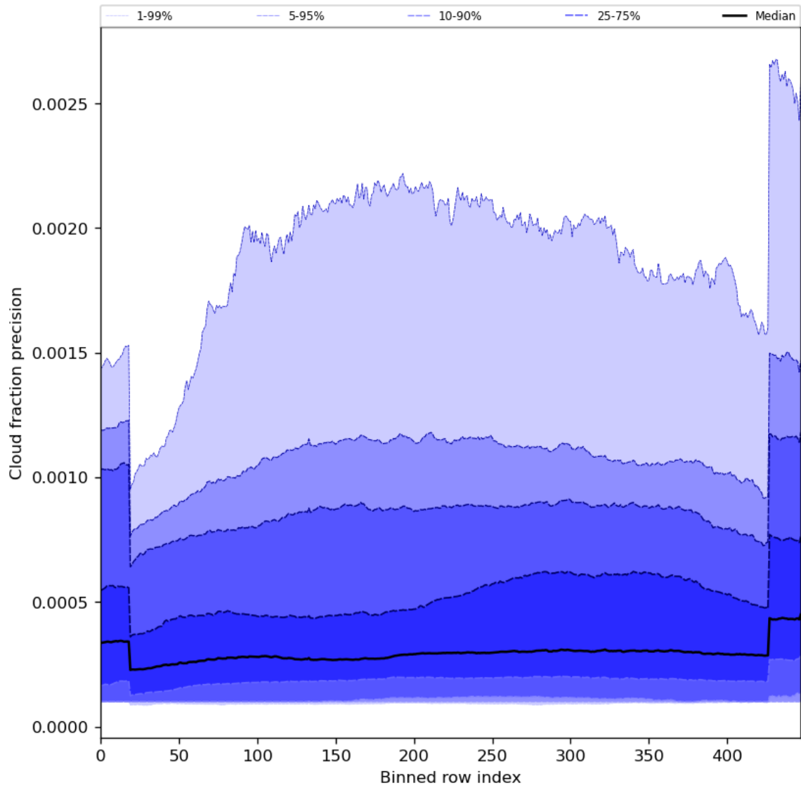
Figure 50: Along track statistics of “Cloud fraction precision” for 2023-08-30 to 2023-08-31
