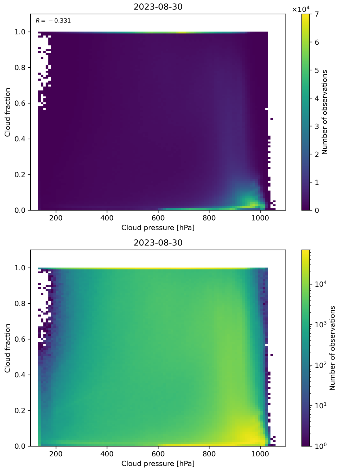
Figure 87: Scatter density plot of “Cloud pressure” against “Cloud fraction” for 2023-08-30 to 2023-08-31.
