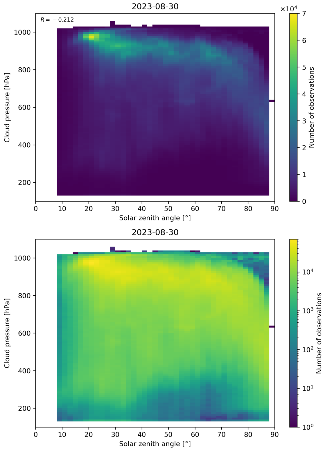
Figure 122: Scatter density plot of “Solar zenith angle” against “Cloud pressure” for 2023-08-30 to 2023-08-31.
