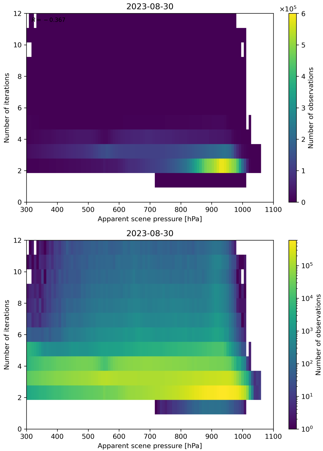
Figure 66: Scatter density plot of “Apparent scene pressure” against “Number of iterations” for 2023-08-30 to 2023-08-31.
