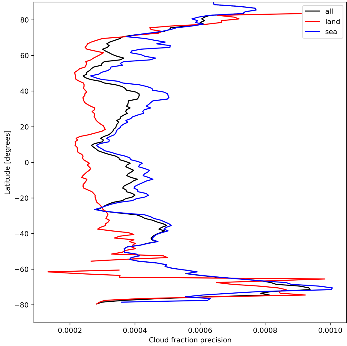
Figure 16: Zonal average of “Cloud fraction precision” for 2023-08-30 to 2023-08-31.
