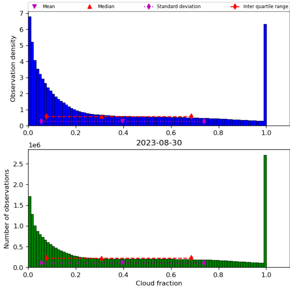
Figure 32: Histogram of “Cloud fraction” for 2023-08-30 to 2023-08-31
