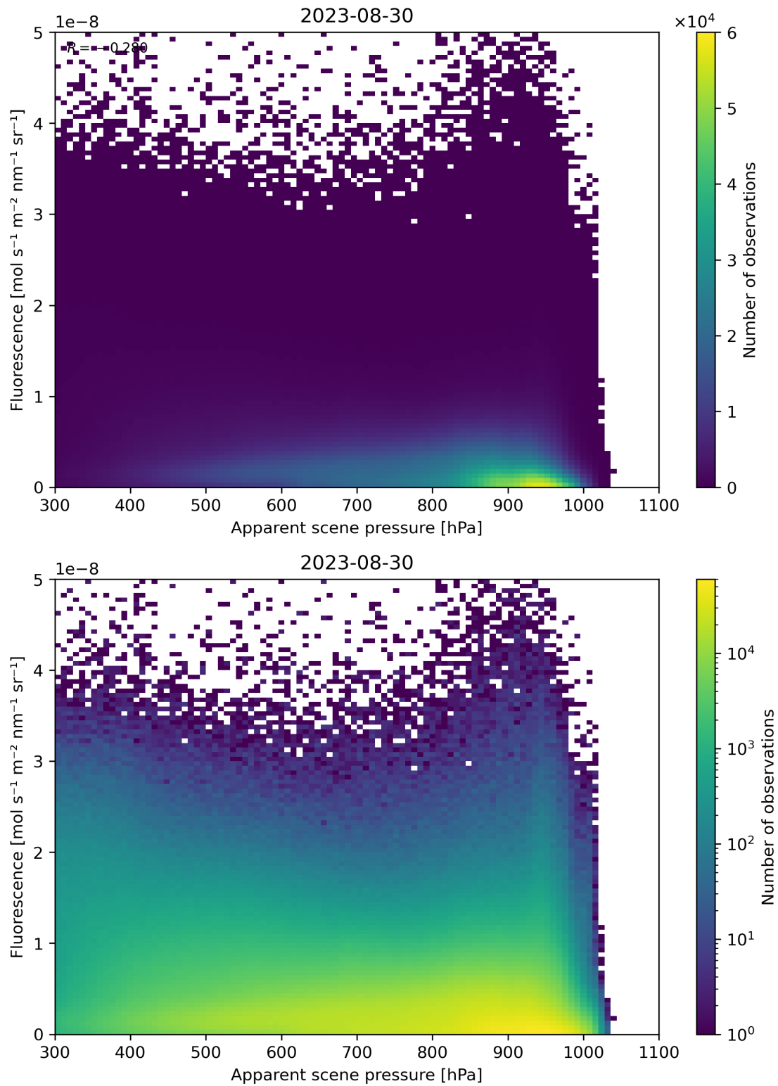
Figure 65: Scatter density plot of “Apparent scene pressure” against “Fluorescence” for 2023-08-30 to 2023-08-31.
