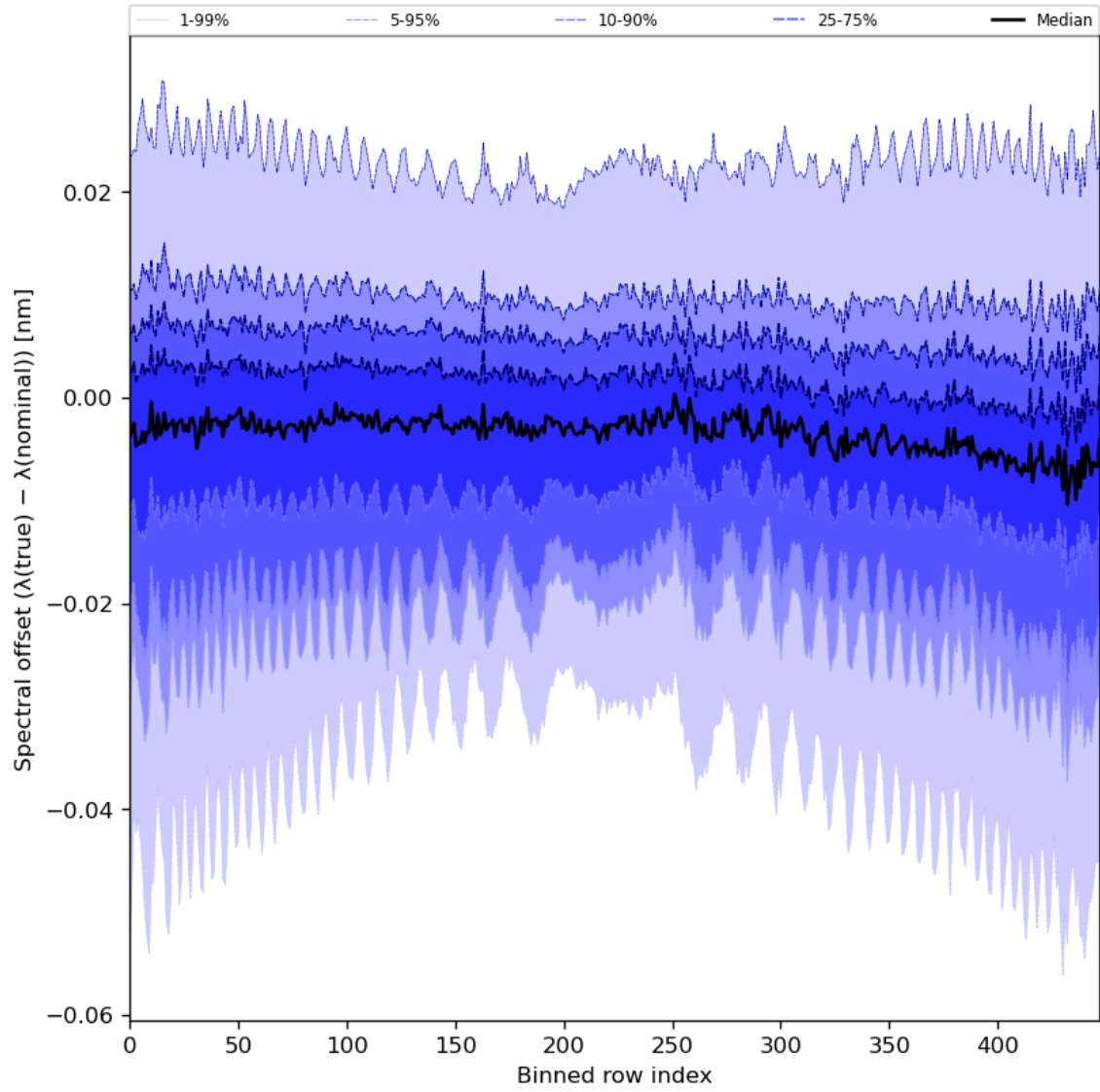
Figure 62: Along track statistics of “Spectral offset ( \lambda(\text{true}) - \lambda(\text{nominal}) )” for 2023-08-30 to 2023-08-31
