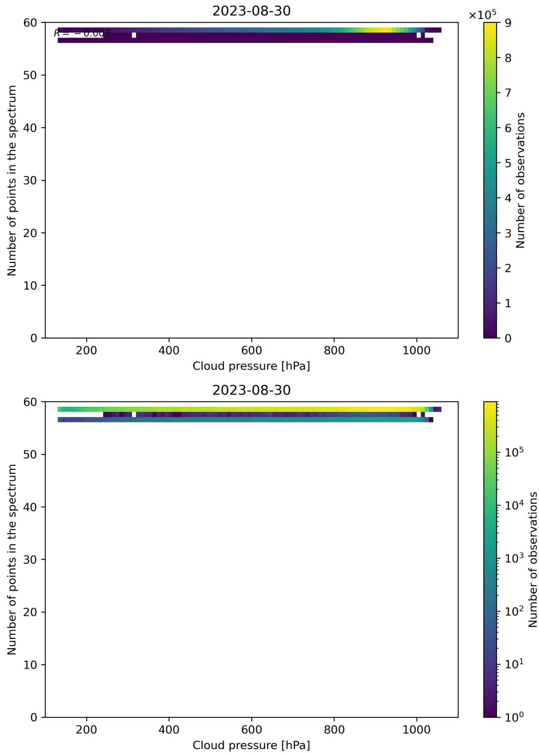
Figure 90: Scatter density plot of “Cloud pressure” against “Number of points in the spectrum” for 2023-08-30 to 2023-08-31.
