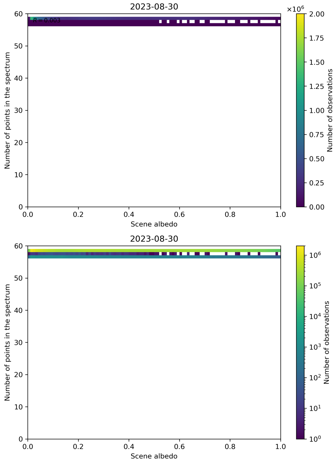
Figure 116: Scatter density plot of “Scene albedo” against “Number of points in the spectrum” for 2023-08-30 to 2023-08-31.
