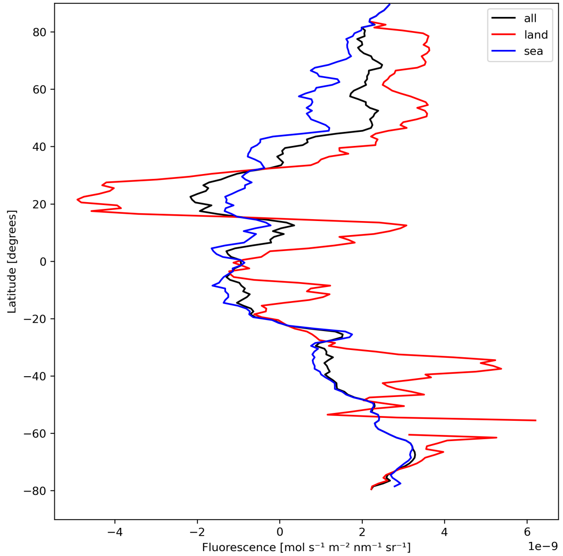
Figure 23: Zonal average of “Fluorescence” for 2023-08-30 to 2023-08-31.
