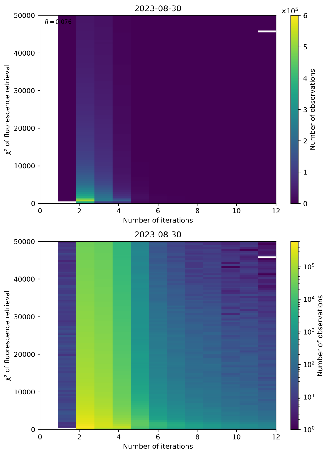
Figure 106: Scatter density plot of “Number of iterations” against “ \chi^2 of fluorescence retrieval” for 2023-08-30 to 2023-08-31.
