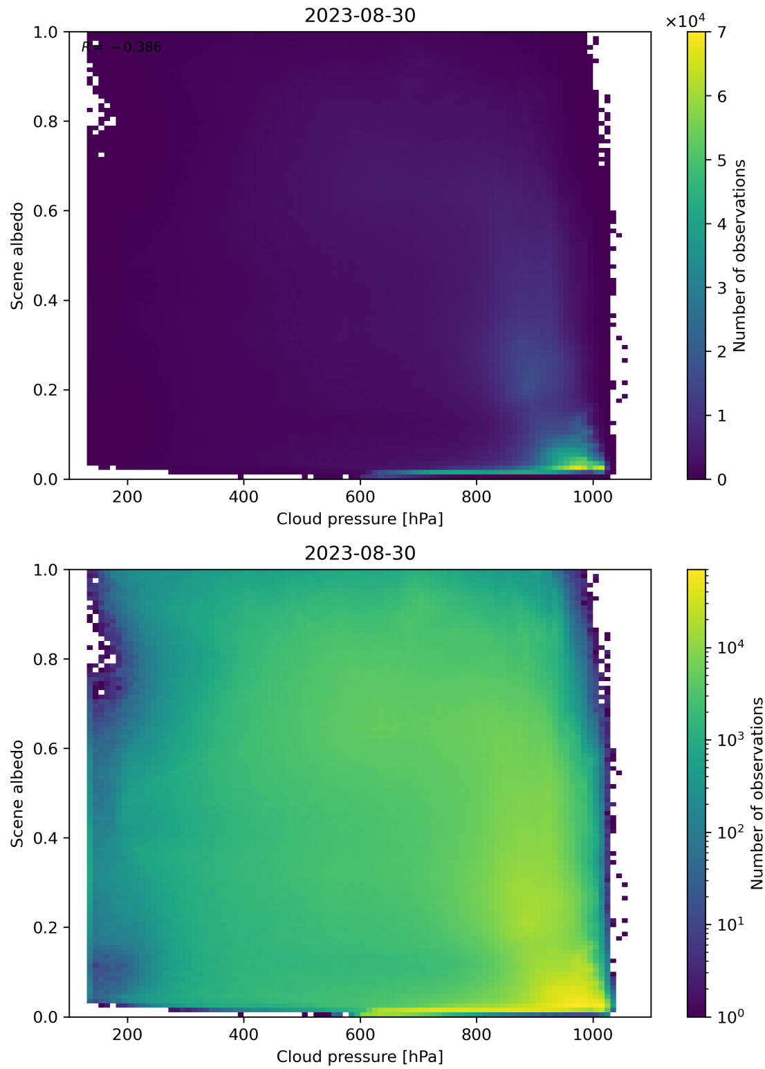
Figure 91: Scatter density plot of “Cloud pressure” against “Scene albedo” for 2023-08-30 to 2023-08-31.
