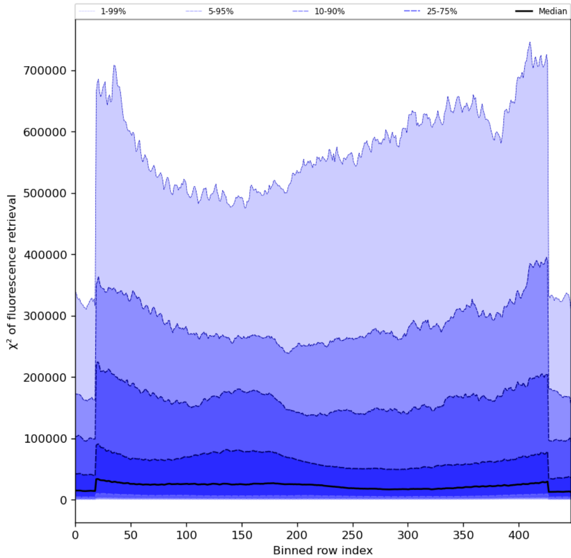
Figure 59: Along track statistics of “ \chi^2 of fluorescence retrieval” for 2023-08-30 to 2023-08-31
