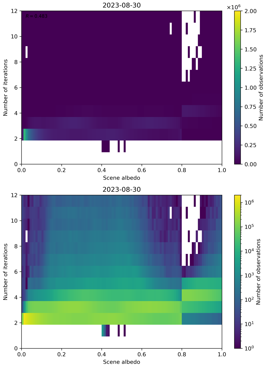
Figure 115: Scatter density plot of “Scene albedo” against “Number of iterations” for 2023-08-30 to 2023-08-31.
