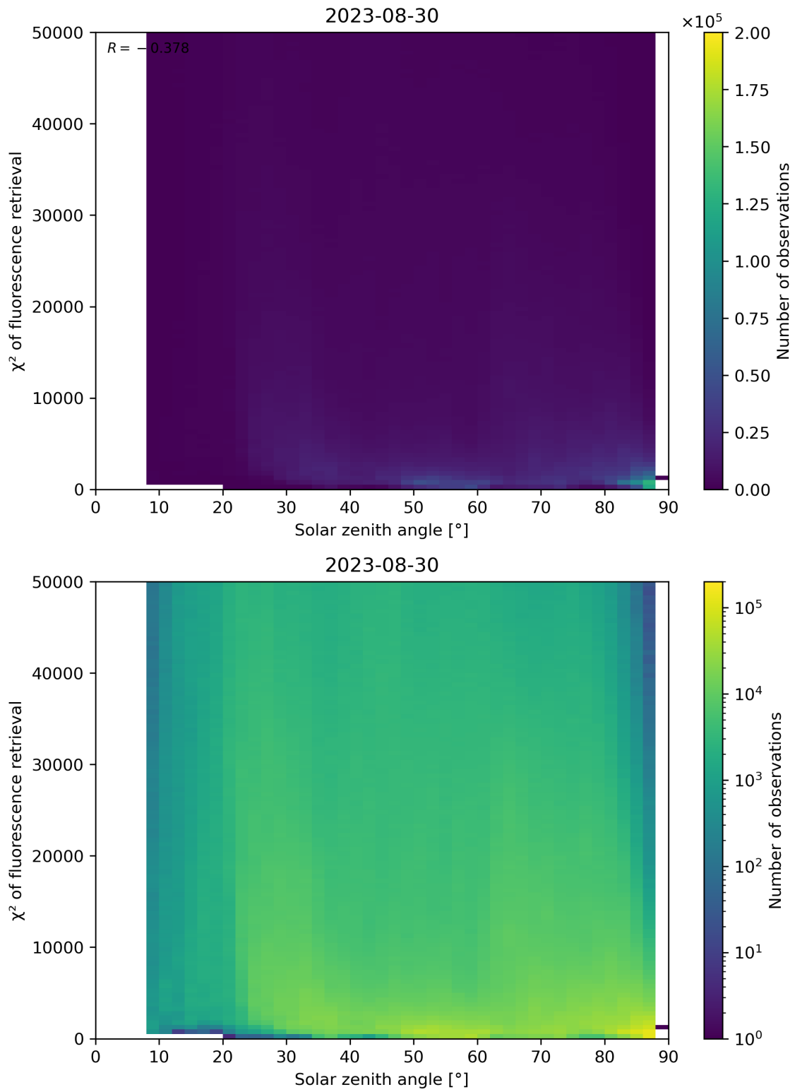
Figure 120: Scatter density plot of “Solar zenith angle” against “ \chi^2 of fluorescence retrieval” for 2023-08-30 to 2023-08-31.
