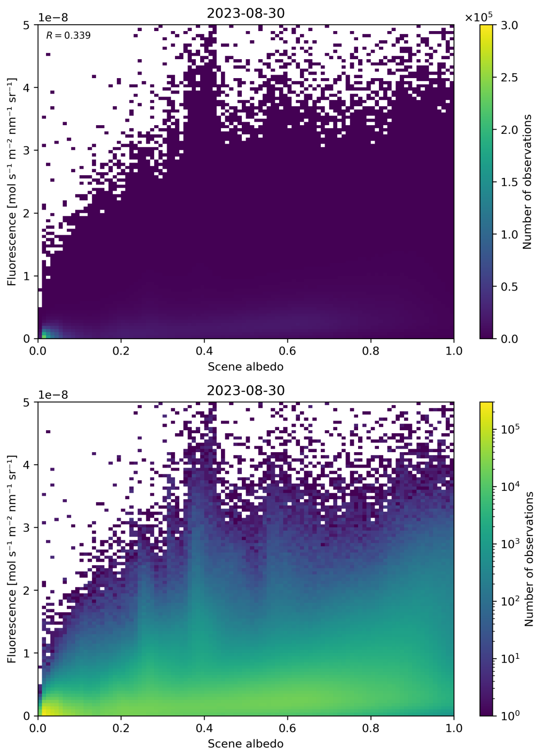
Figure 114: Scatter density plot of “Scene albedo” against “Fluorescence” for 2023-08-30 to 2023-08-31.
