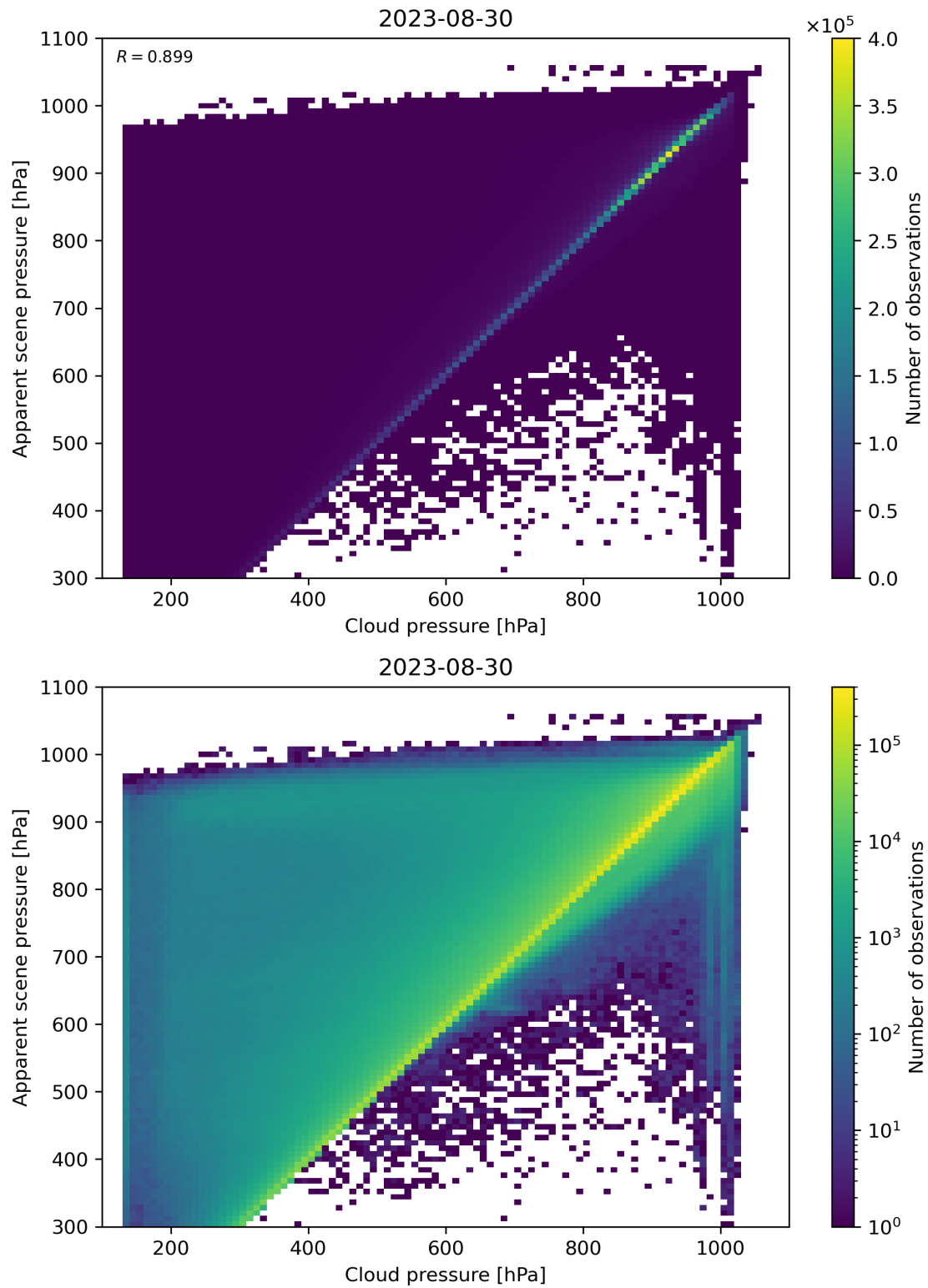
Figure 84: Scatter density plot of “Cloud pressure” against “Apparent scene pressure” for 2023-08-30 to 2023-08-31.
