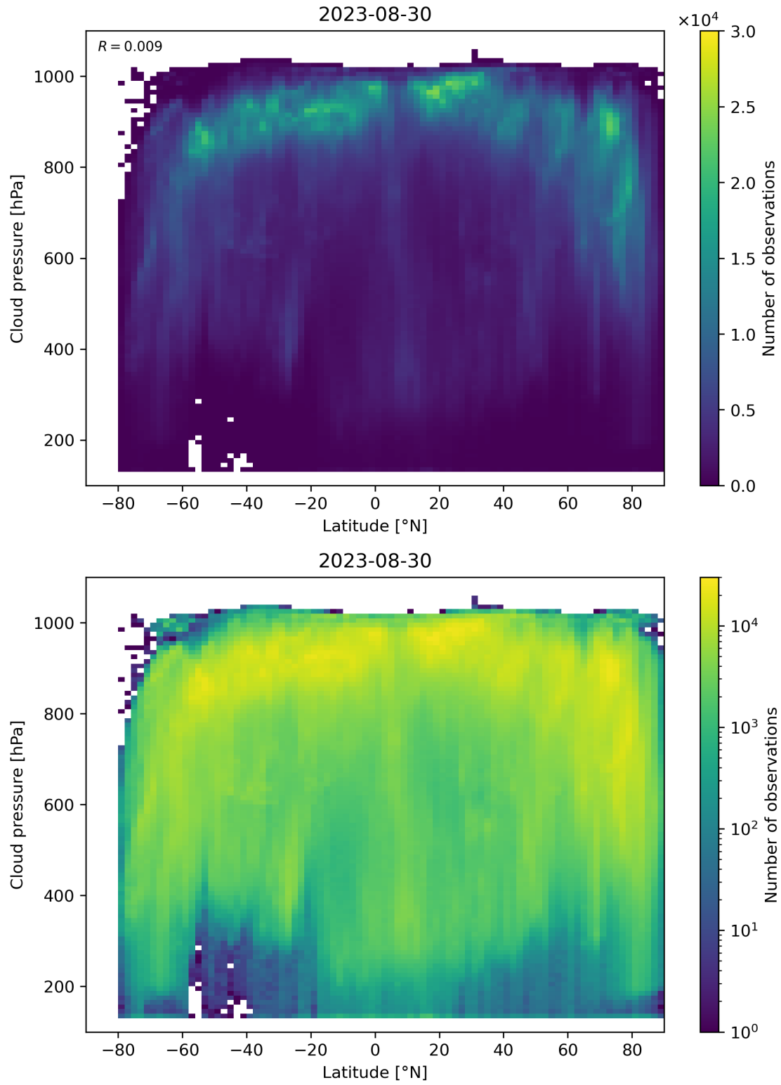
Figure 100: Scatter density plot of “Latitude” against “Cloud pressure” for 2023-08-30 to 2023-08-31.
