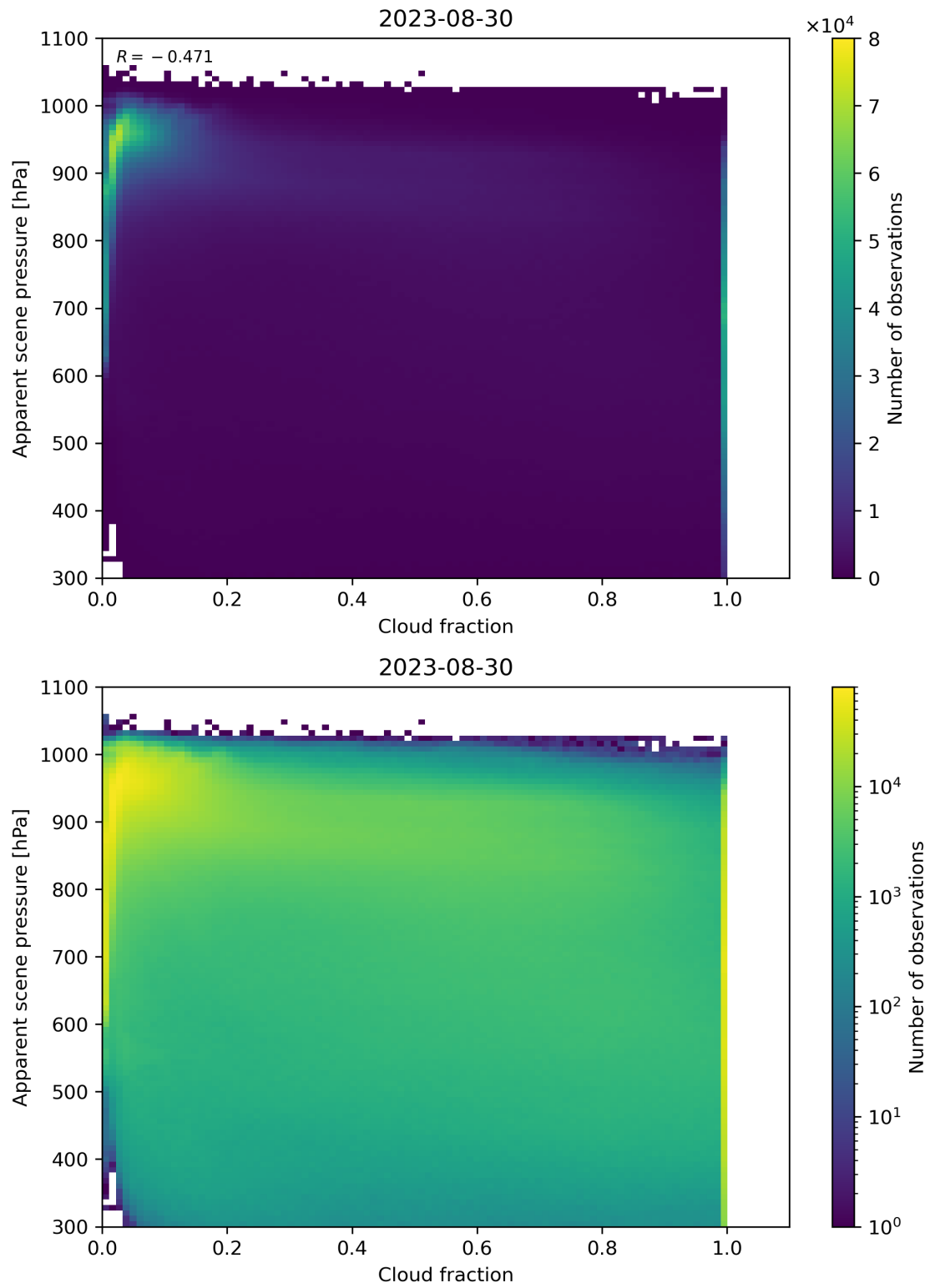
Figure 76: Scatter density plot of “Cloud fraction” against “Apparent scene pressure” for 2023-08-30 to 2023-08-31.
