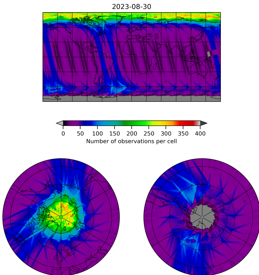
Figure 11: Map of the number of observations for 2023-08-30 to 2023-08-31
