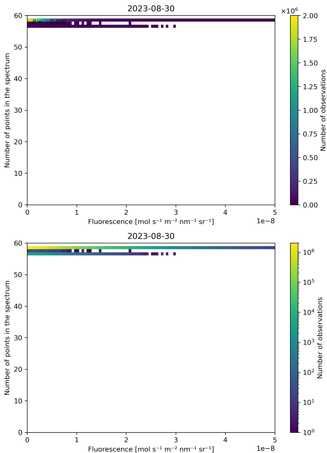
Figure 94: Scatter density plot of “Fluorescence” against “Number of points in the spectrum” for 2023-08-30 to 2023-08-31.
