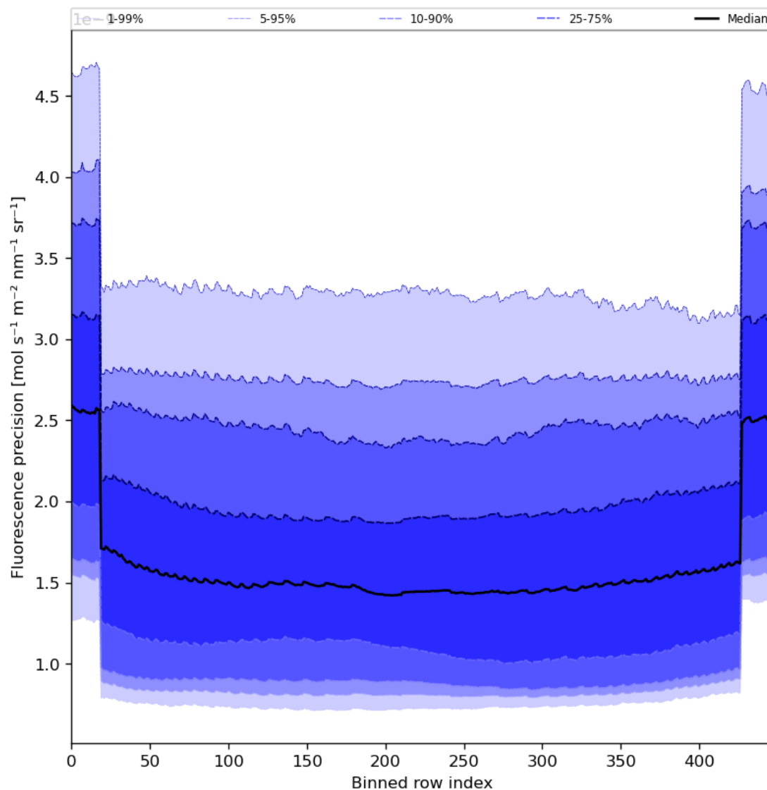
Figure 58: Along track statistics of “Fluorescence precision” for 2023-08-30 to 2023-08-31
