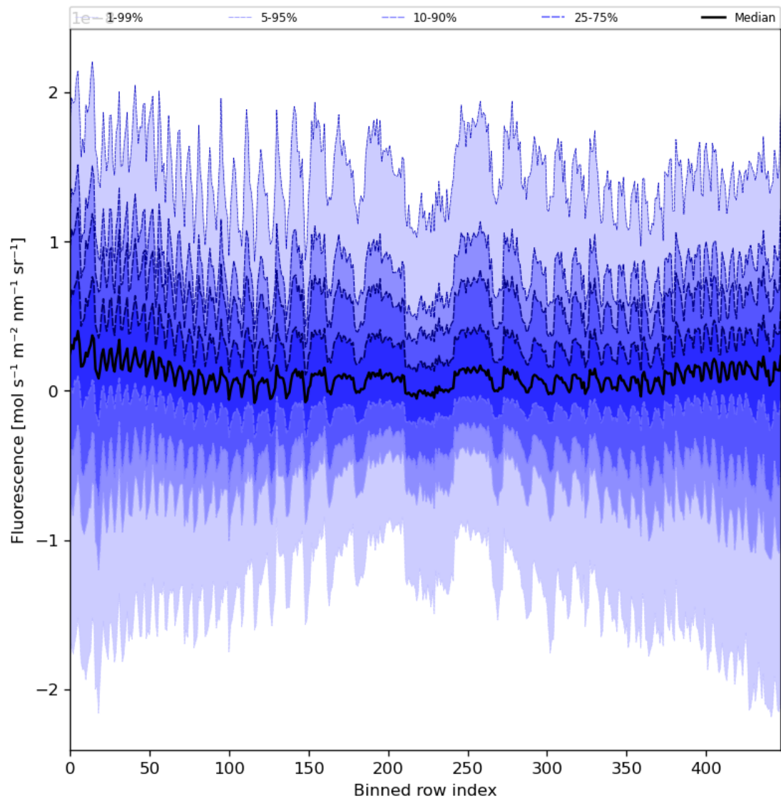
Figure 57: Along track statistics of “Fluorescence” for 2023-08-30 to 2023-08-31
