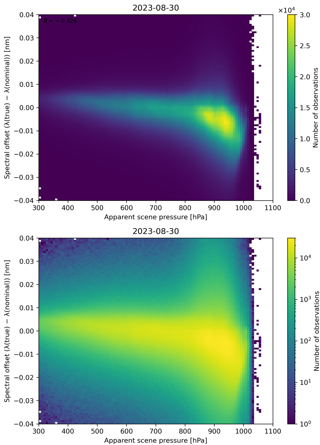
Figure 68: Scatter density plot of “Apparent scene pressure” against “Spectral offset ( \lambda(\text{true}) - \lambda(\text{nominal}) )” for 2023-08-30 to 2023-08-31.
