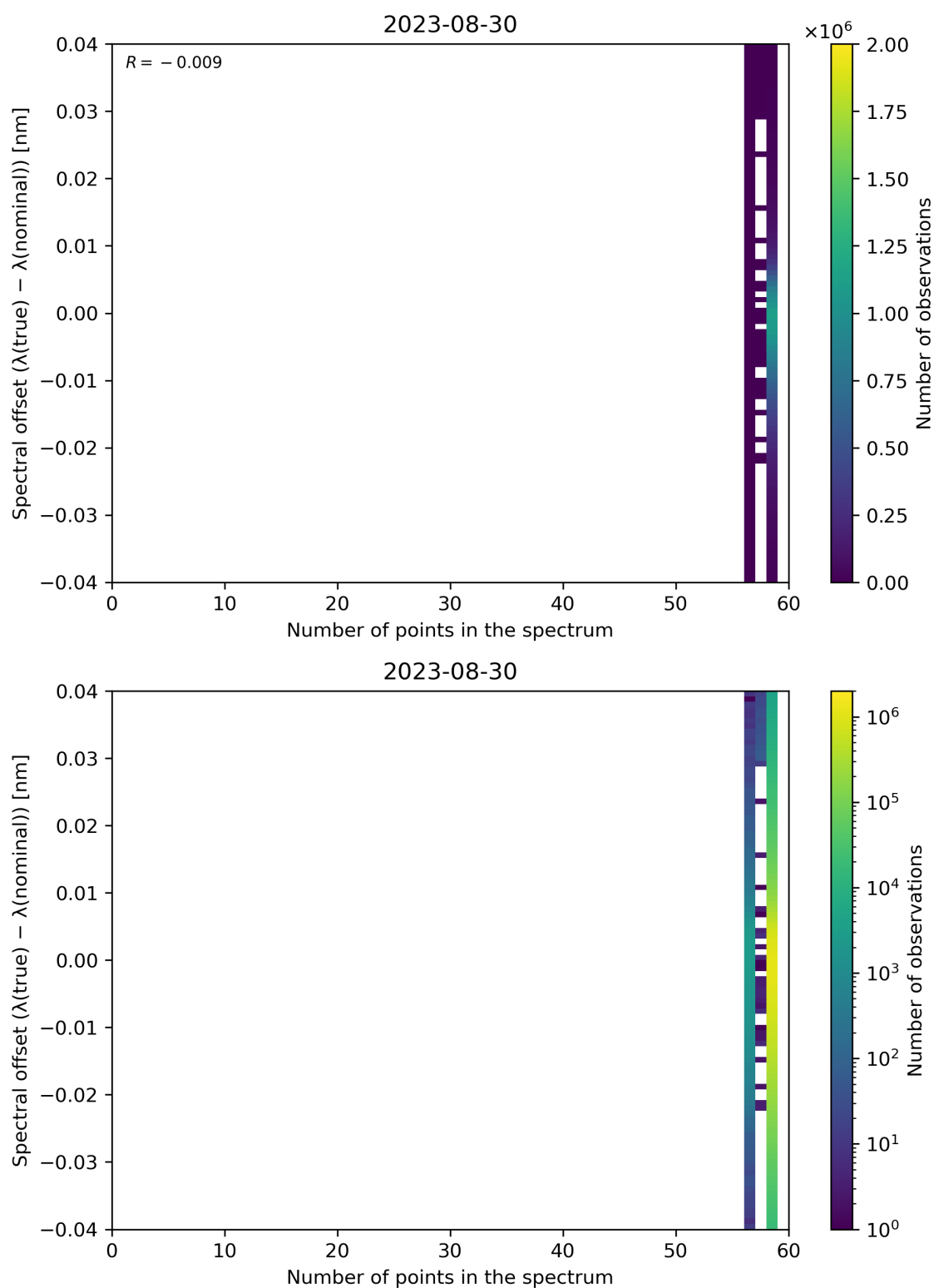
Figure 110: Scatter density plot of “Number of points in the spectrum” against “Spectral offset ( \lambda(\text{true}) - \lambda(\text{nominal}) )” for 2023-08-30 to 2023-08-31.
