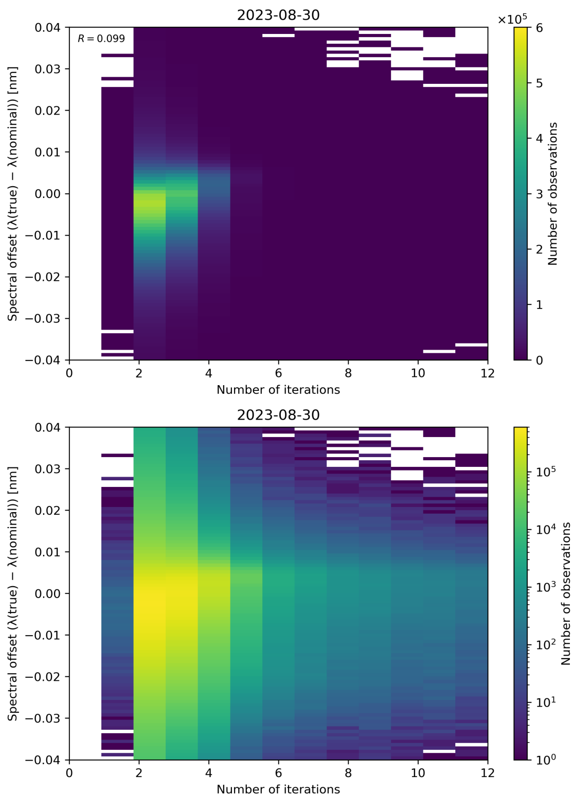
Figure 109: Scatter density plot of “Number of iterations” against “Spectral offset ( \lambda(\text{true}) - \lambda(\text{nominal}) )” for 2023-08-30 to 2023-08-31.
