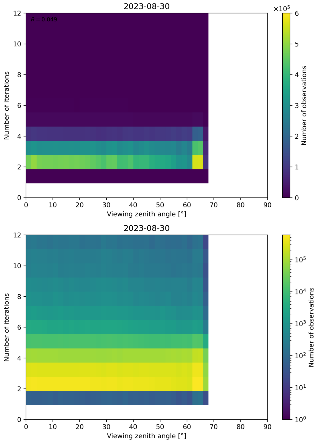
Figure 136: Scatter density plot of “Viewing zenith angle” against “Number of iterations” for 2023-08-30 to 2023-08-31.
