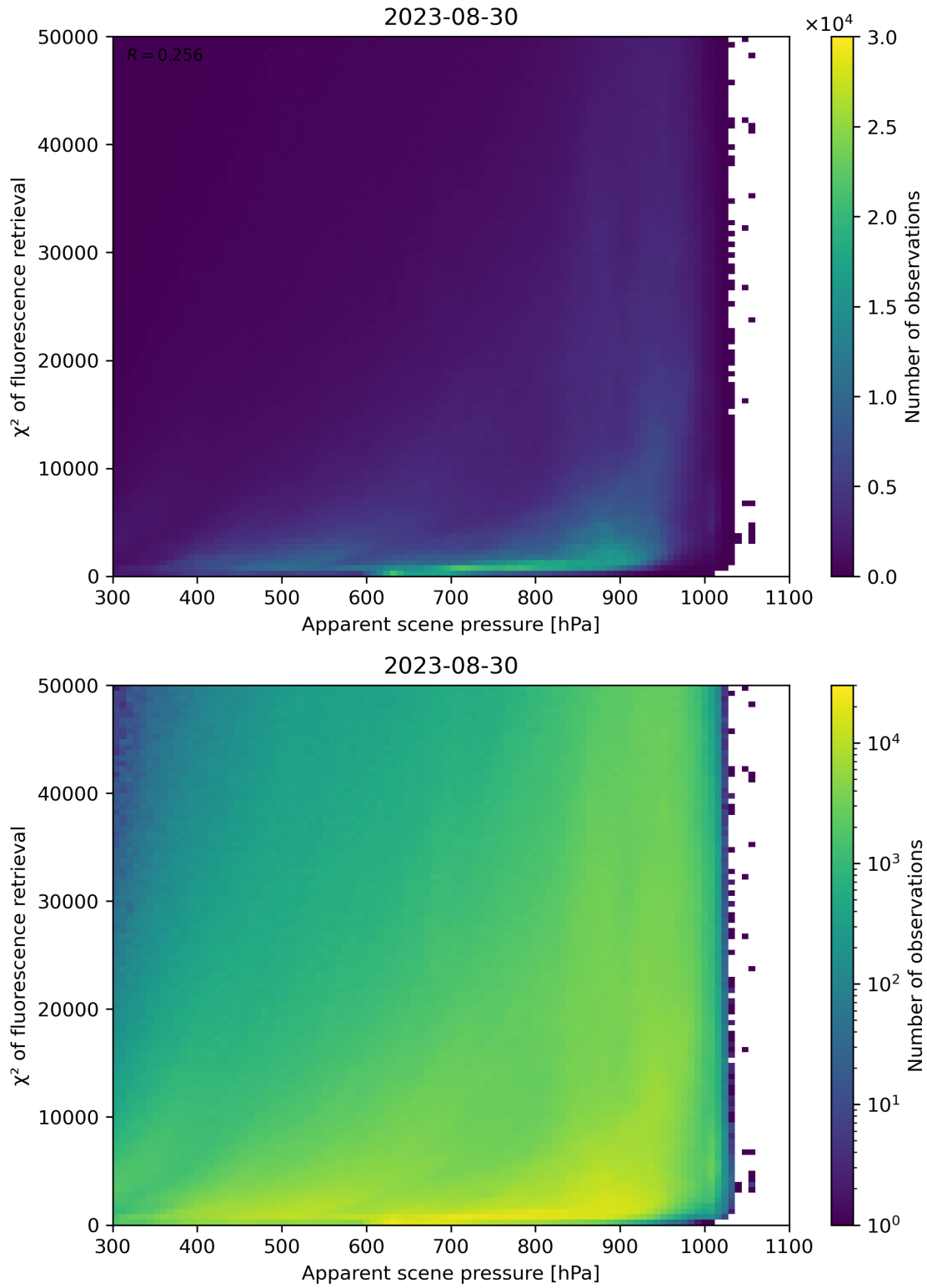
Figure 64: Scatter density plot of “Apparent scene pressure” against “ \chi^2 of fluorescence retrieval” for 2023-08-30 to 2023-08-31.
