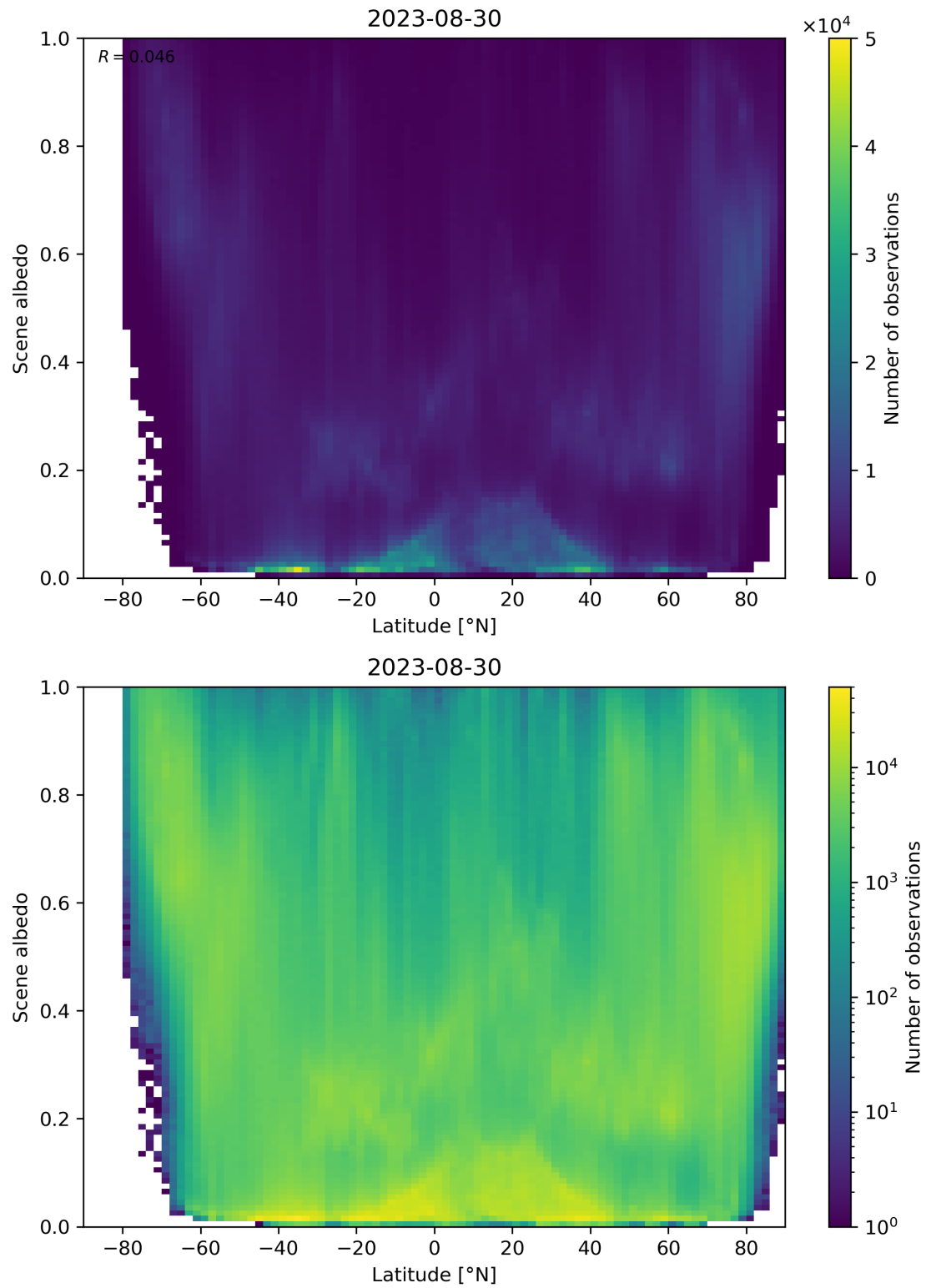
Figure 104: Scatter density plot of “Latitude” against “Scene albedo” for 2023-08-30 to 2023-08-31.
