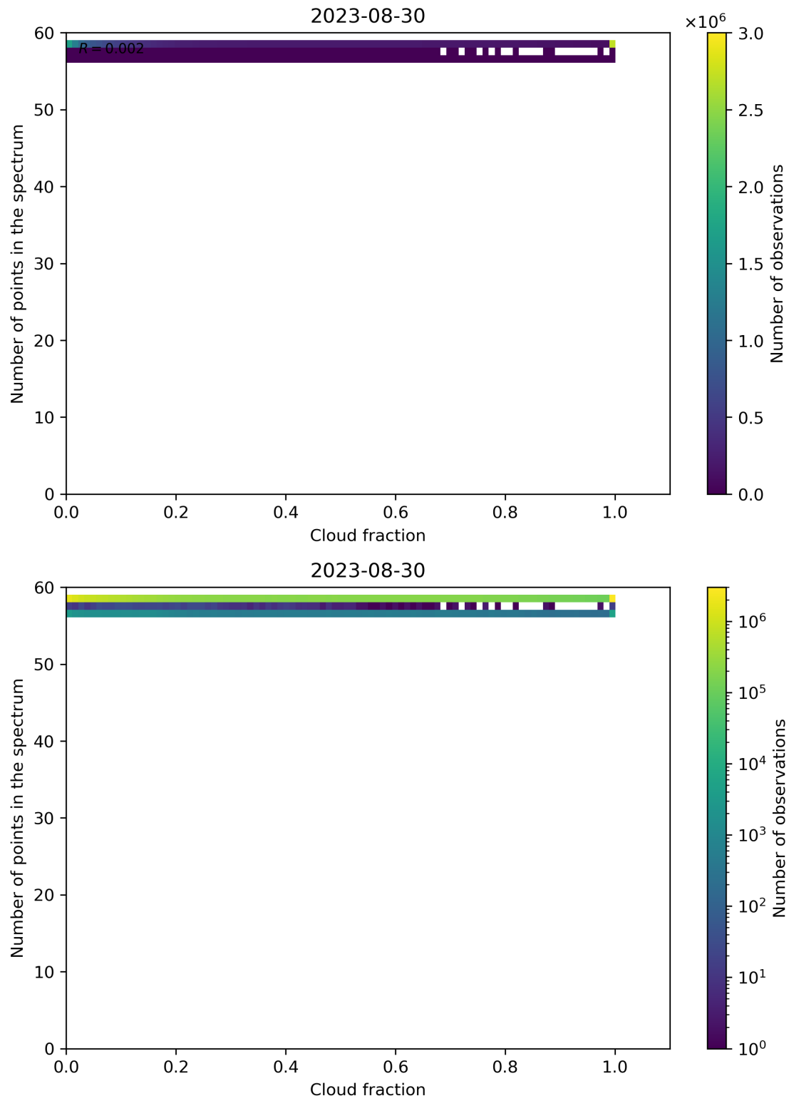
Figure 81: Scatter density plot of “Cloud fraction” against “Number of points in the spectrum” for 2023-08-30 to 2023-08-31.
