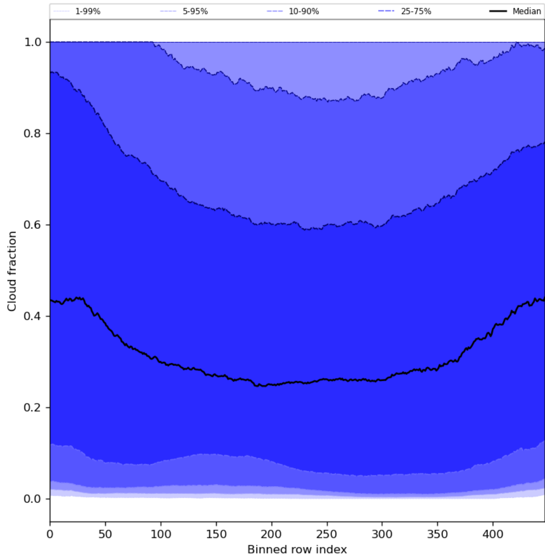
Figure 49: Along track statistics of “Cloud fraction” for 2023-08-30 to 2023-08-31
