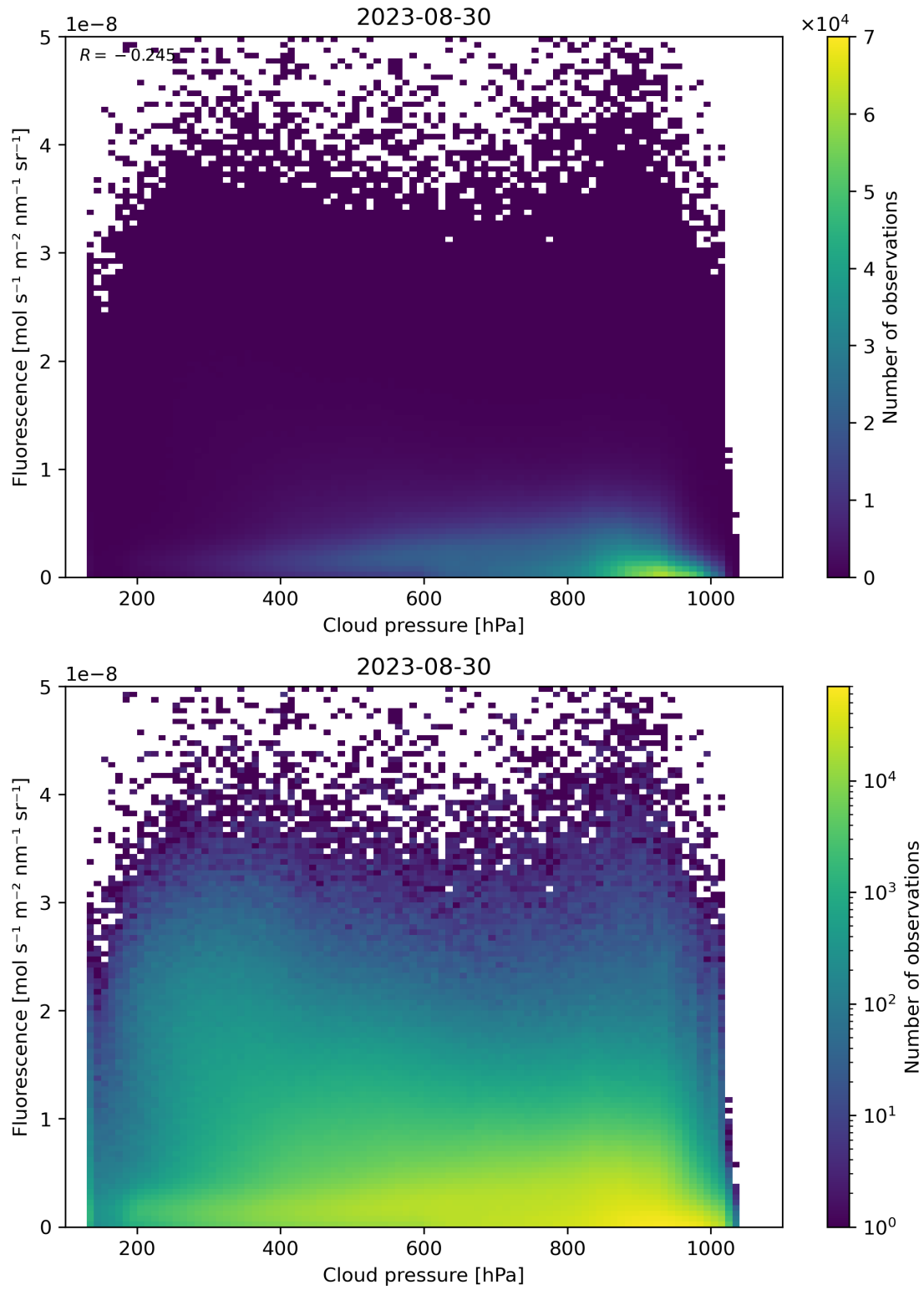
Figure 88: Scatter density plot of “Cloud pressure” against “Fluorescence” for 2023-08-30 to 2023-08-31.
