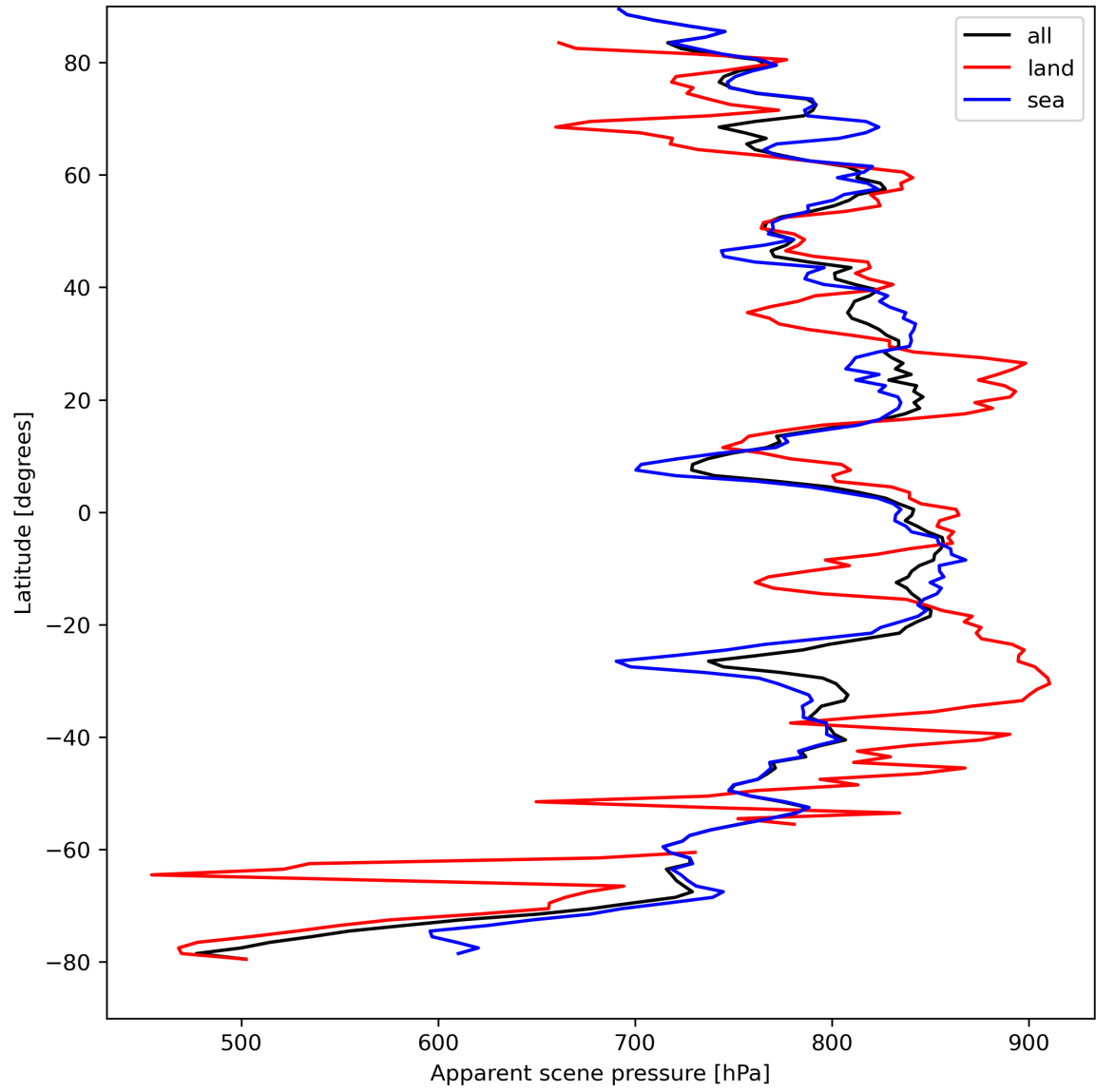
Figure 19: Zonal average of “Apparent scene pressure” for 2023-08-30 to 2023-08-31.
