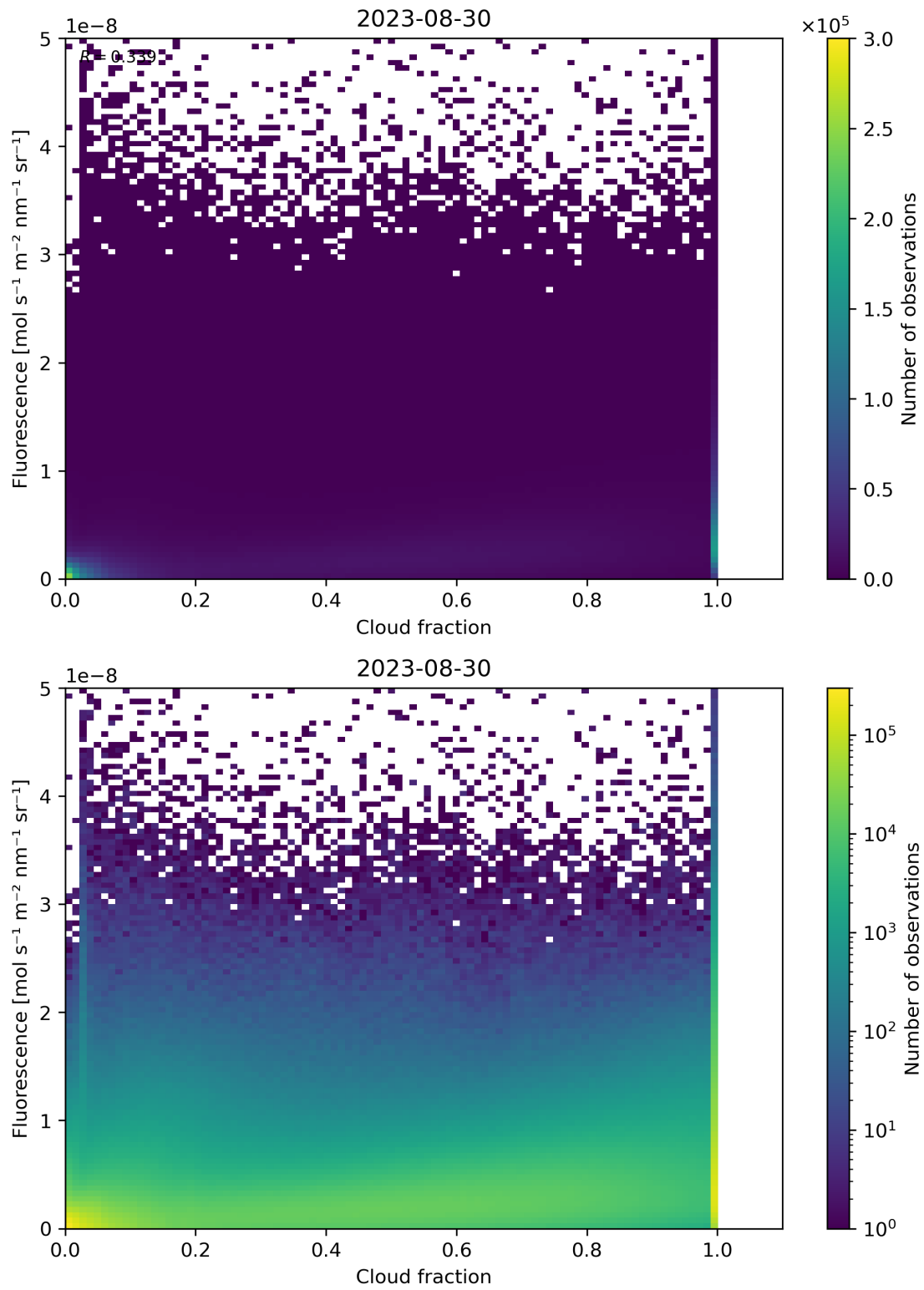
Figure 79: Scatter density plot of “Cloud fraction” against “Fluorescence” for 2023-08-30 to 2023-08-31.
