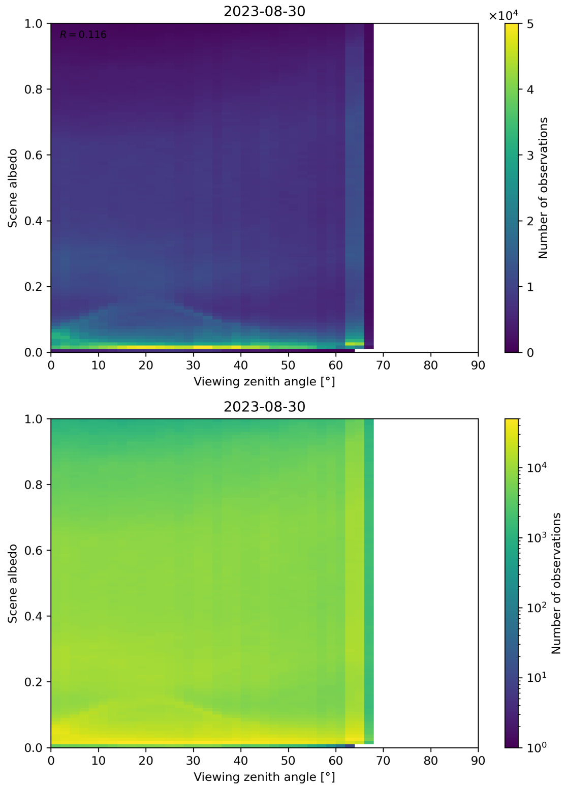
Figure 138: Scatter density plot of “Viewing zenith angle” against “Scene albedo” for 2023-08-30 to 2023-08-31.
