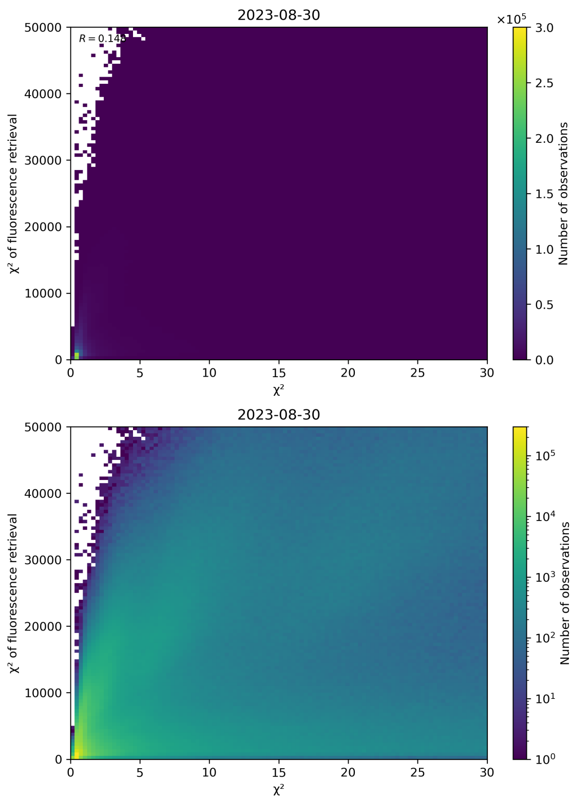
Figure 69: Scatter density plot of “ \chi^2 ” against “ \chi^2 of fluorescence retrieval” for 2023-08-30 to 2023-08-31.
