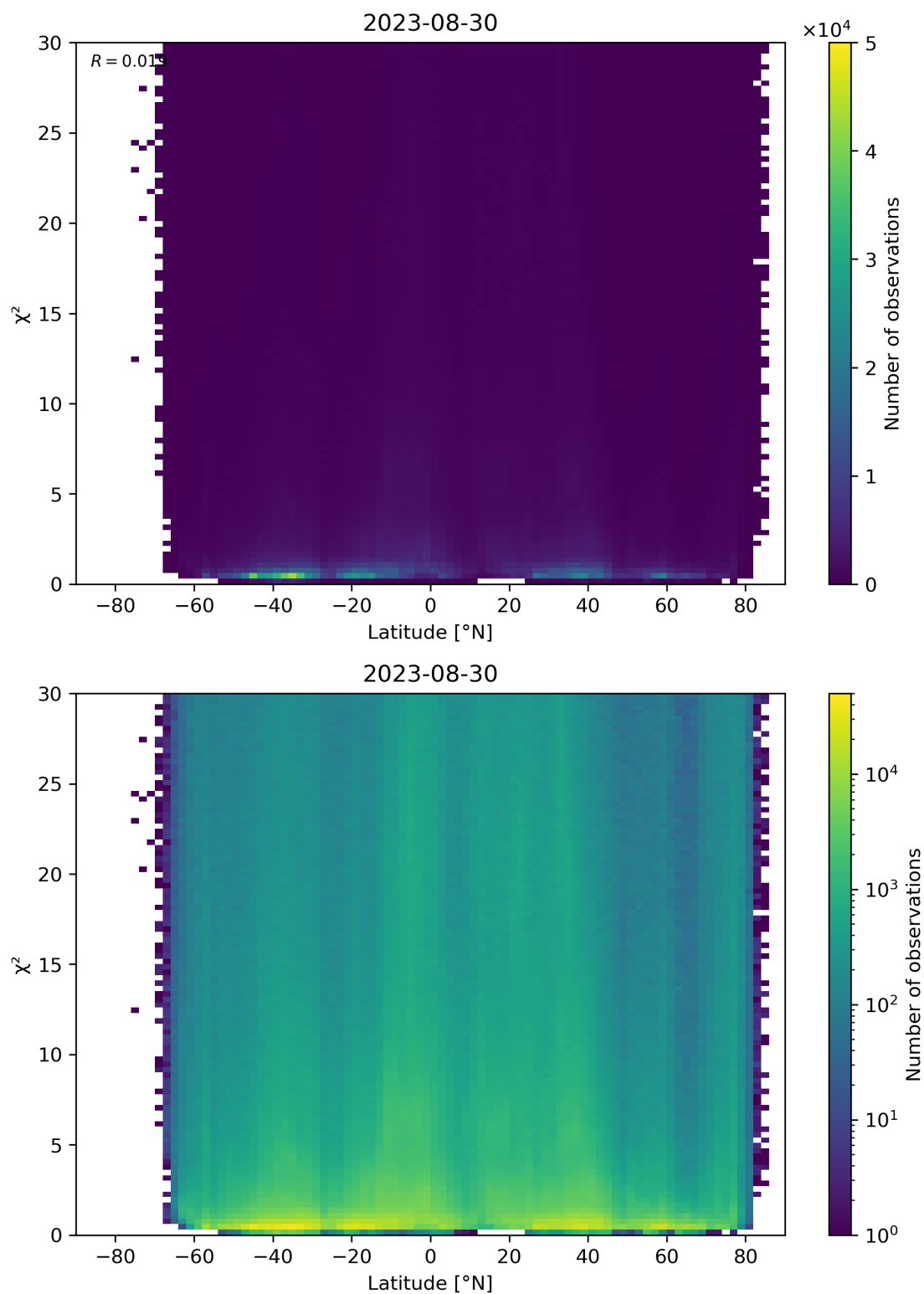
Figure 97: Scatter density plot of “Latitude” against “ \chi^2 ” for 2023-08-30 to 2023-08-31.
