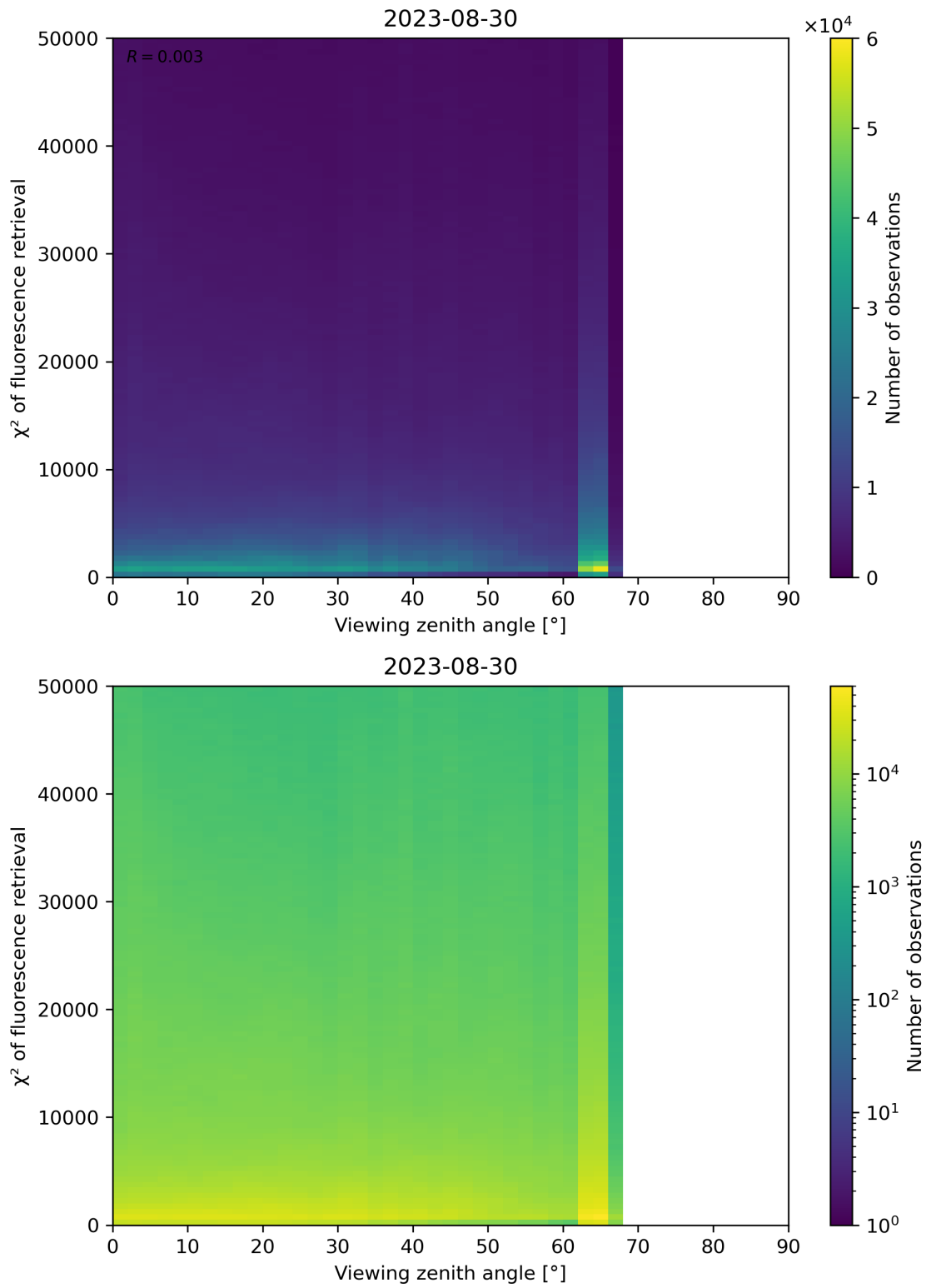
Figure 131: Scatter density plot of “Viewing zenith angle” against “ \chi^2 of fluorescence retrieval” for 2023-08-30 to 2023-08-31.
