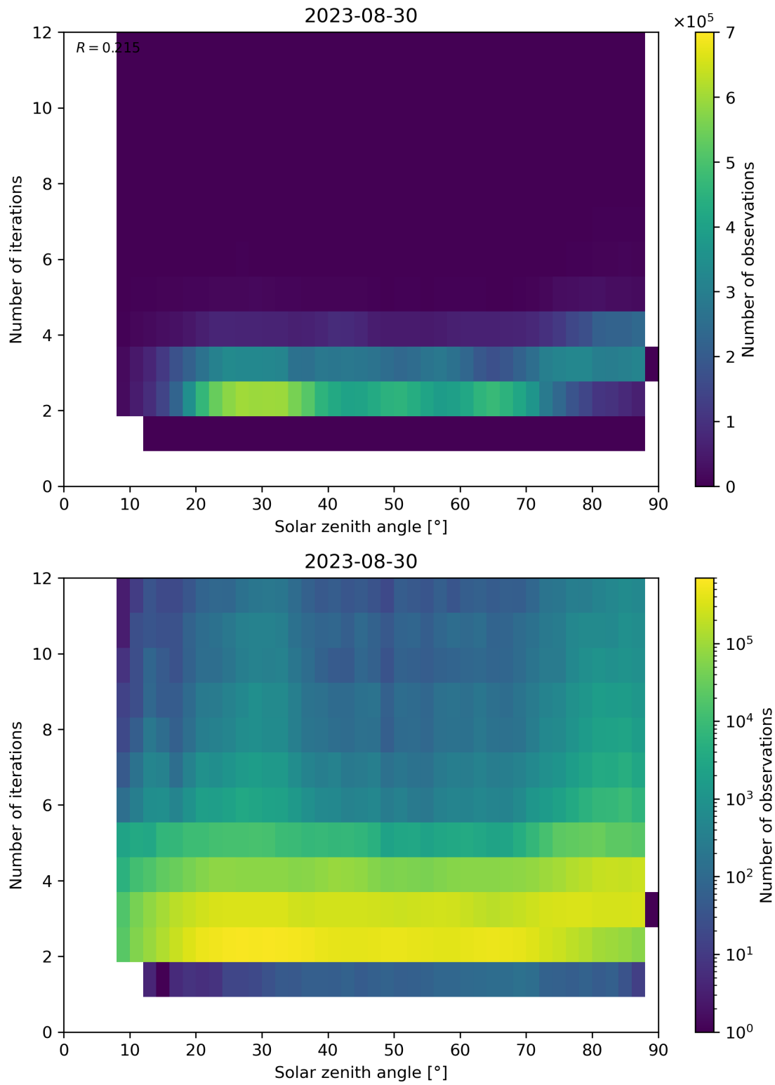
Figure 125: Scatter density plot of “Solar zenith angle” against “Number of iterations” for 2023-08-30 to 2023-08-31.
