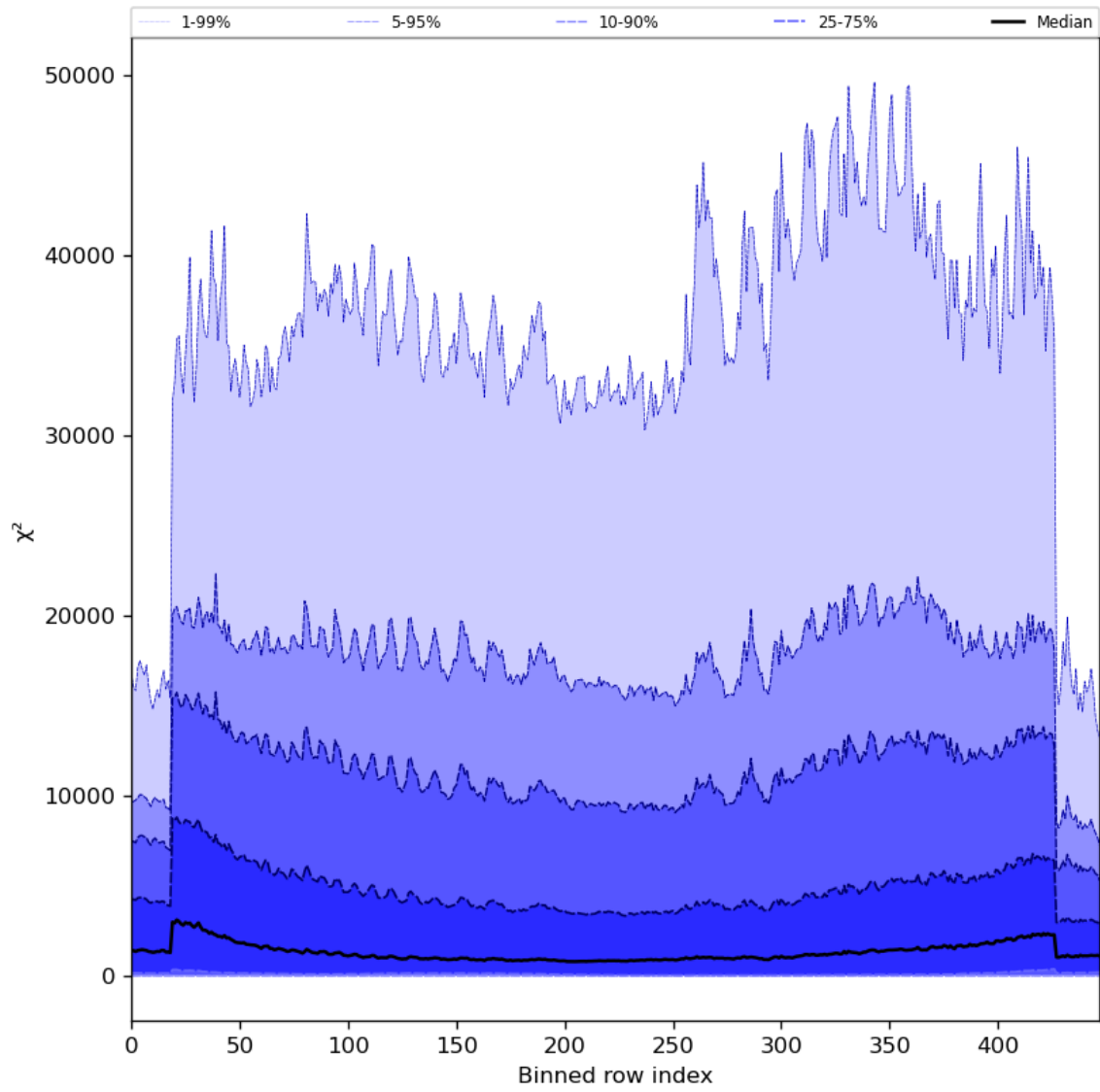
Figure 55: Along track statistics of “ \chi^2 ” for 2023-08-30 to 2023-08-31
