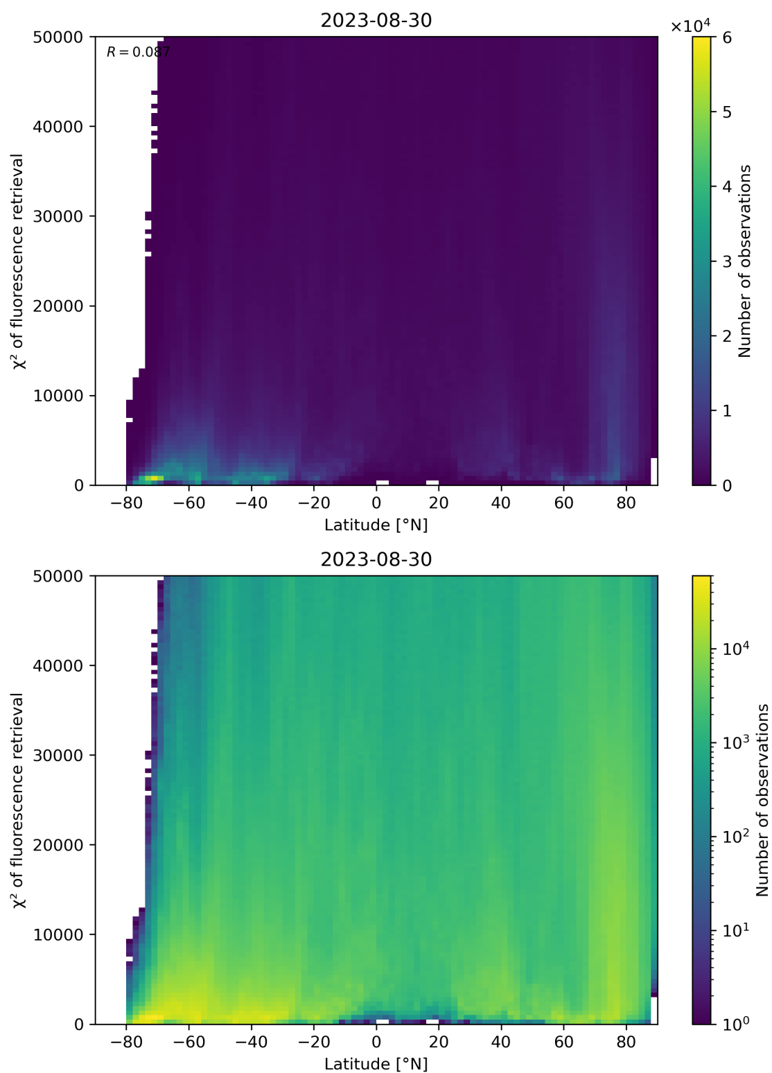
Figure 98: Scatter density plot of “Latitude” against “ \chi^2 of fluorescence retrieval” for 2023-08-30 to 2023-08-31.
