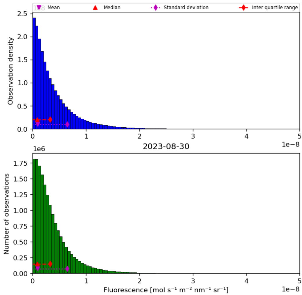
Figure 40: Histogram of “Fluorescence” for 2023-08-30 to 2023-08-31
