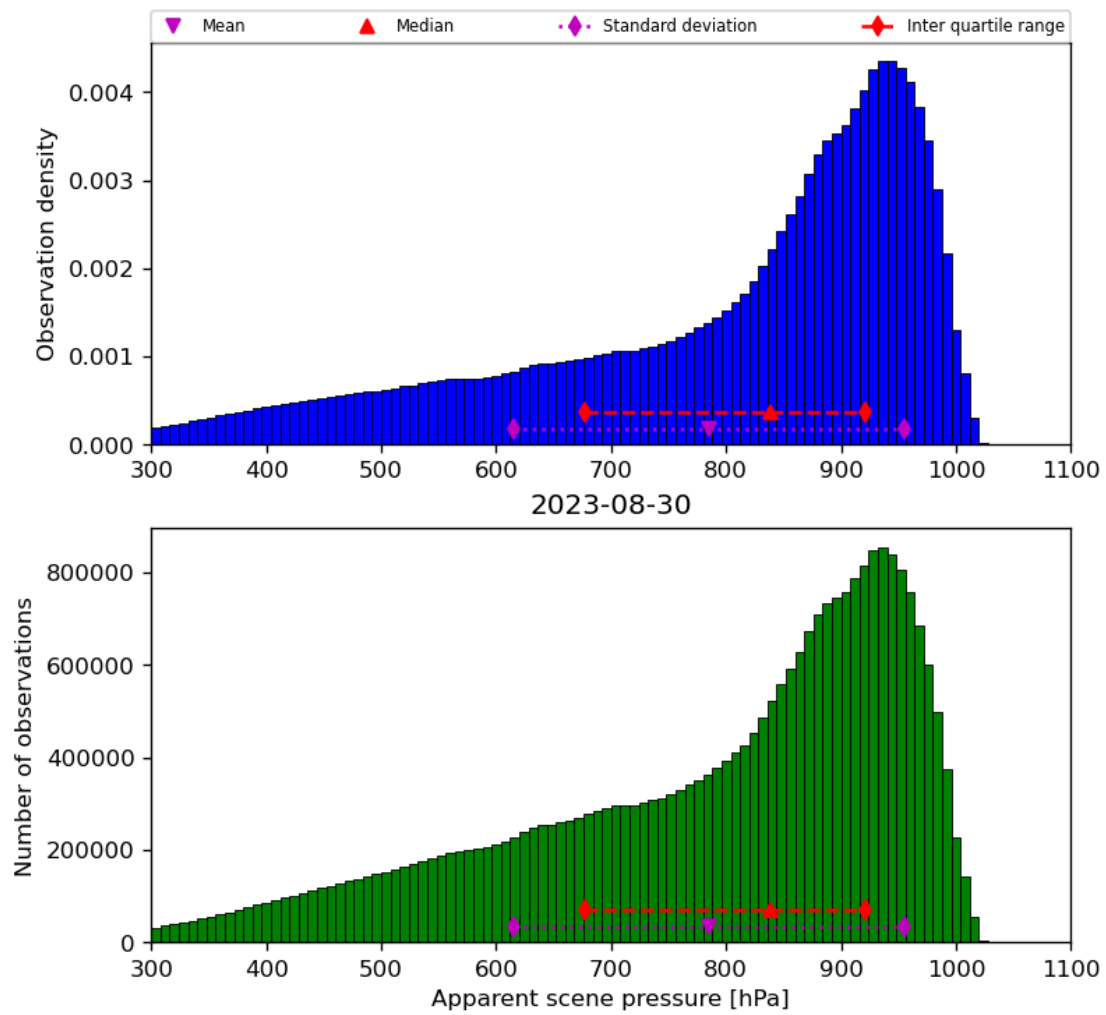
Figure 36: Histogram of “Apparent scene pressure” for 2023-08-30 to 2023-08-31
