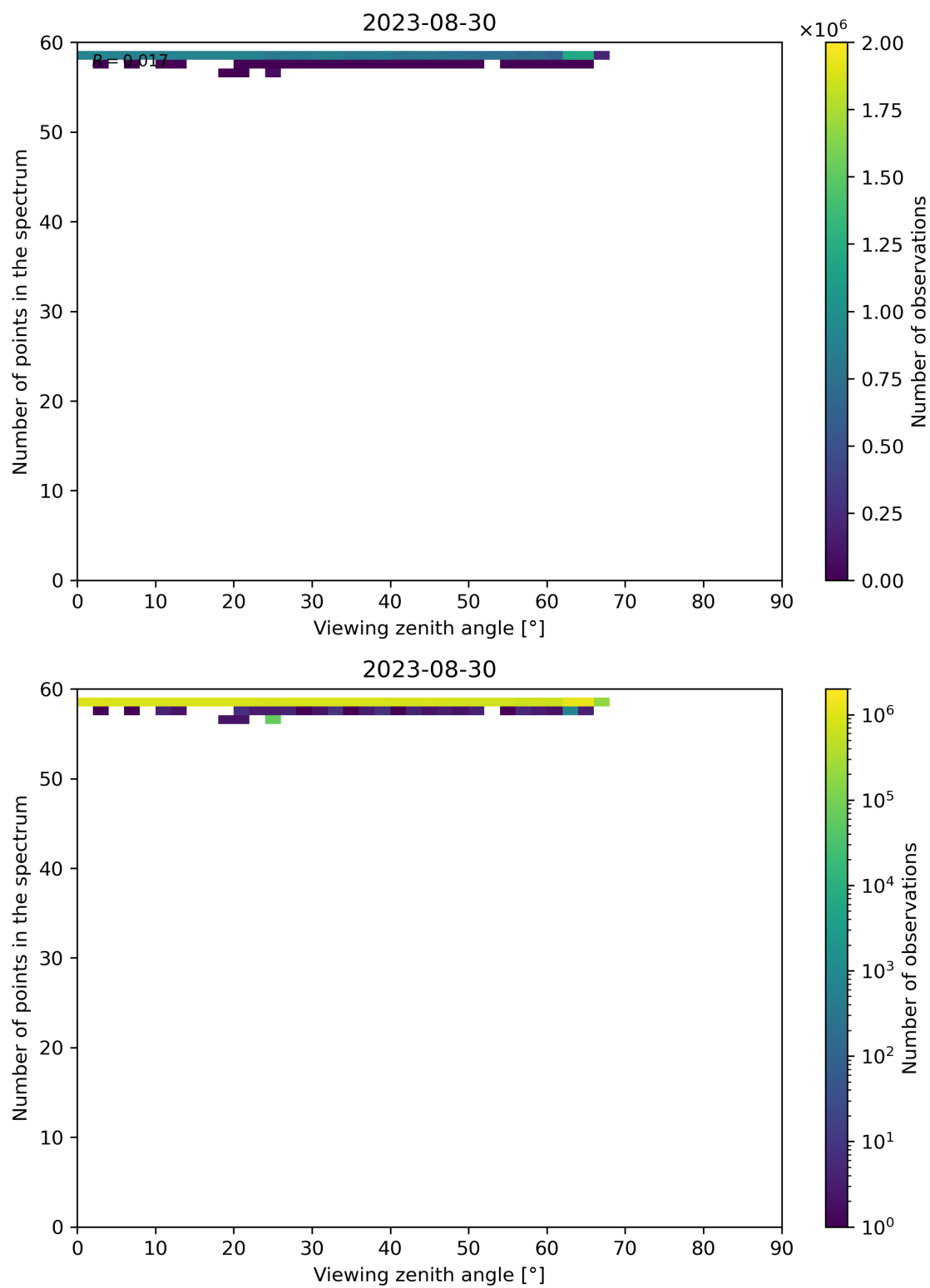
Figure 137: Scatter density plot of “Viewing zenith angle” against “Number of points in the spectrum” for 2023-08-30 to 2023-08-31.
