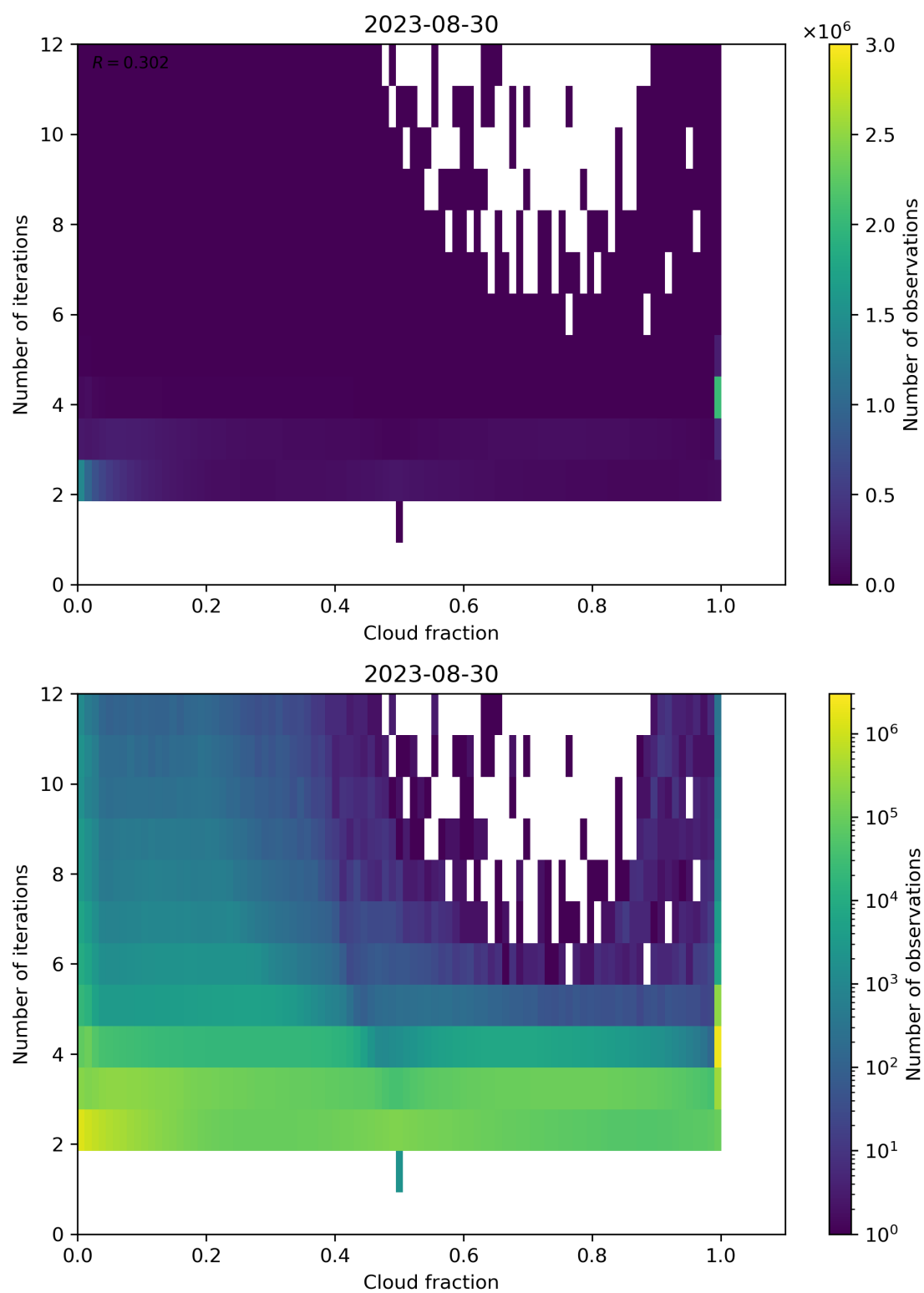
Figure 80: Scatter density plot of “Cloud fraction” against “Number of iterations” for 2023-08-30 to 2023-08-31.
