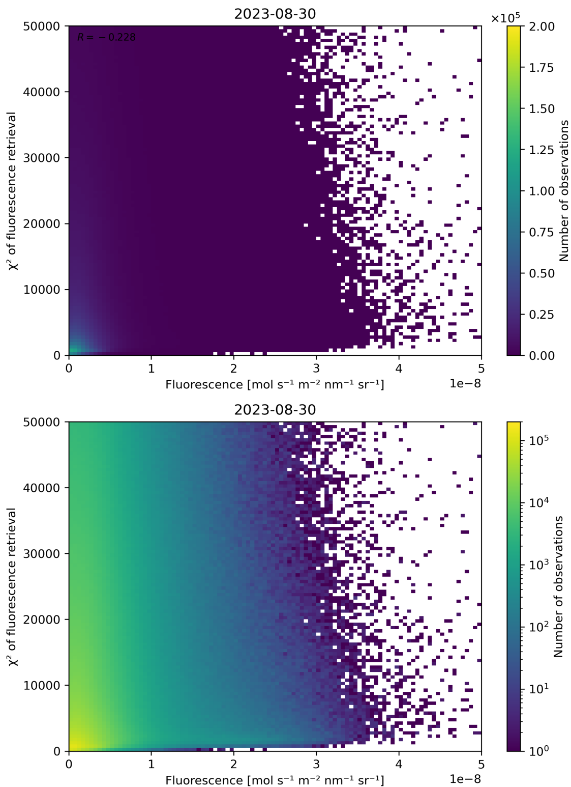
Figure 93: Scatter density plot of “Fluorescence” against “ \chi^2 of fluorescence retrieval” for 2023-08-30 to 2023-08-31.
