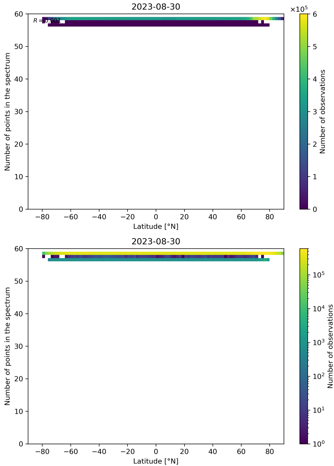
Figure 103: Scatter density plot of “Latitude” against “Number of points in the spectrum” for 2023-08-30 to 2023-08-31.
