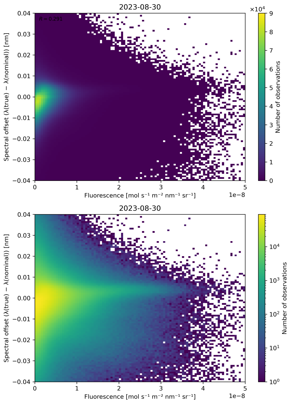
Figure 95: Scatter density plot of “Fluorescence” against “Spectral offset ( \lambda(\text{true}) - \lambda(\text{nominal}) )” for 2023-08-30 to 2023-08-31.
