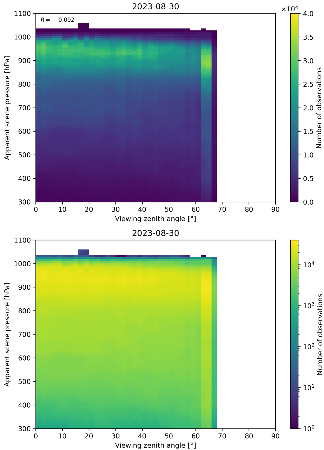
Figure 129: Scatter density plot of “Viewing zenith angle” against “Apparent scene pressure” for 2023-08-30 to 2023-08-31.
