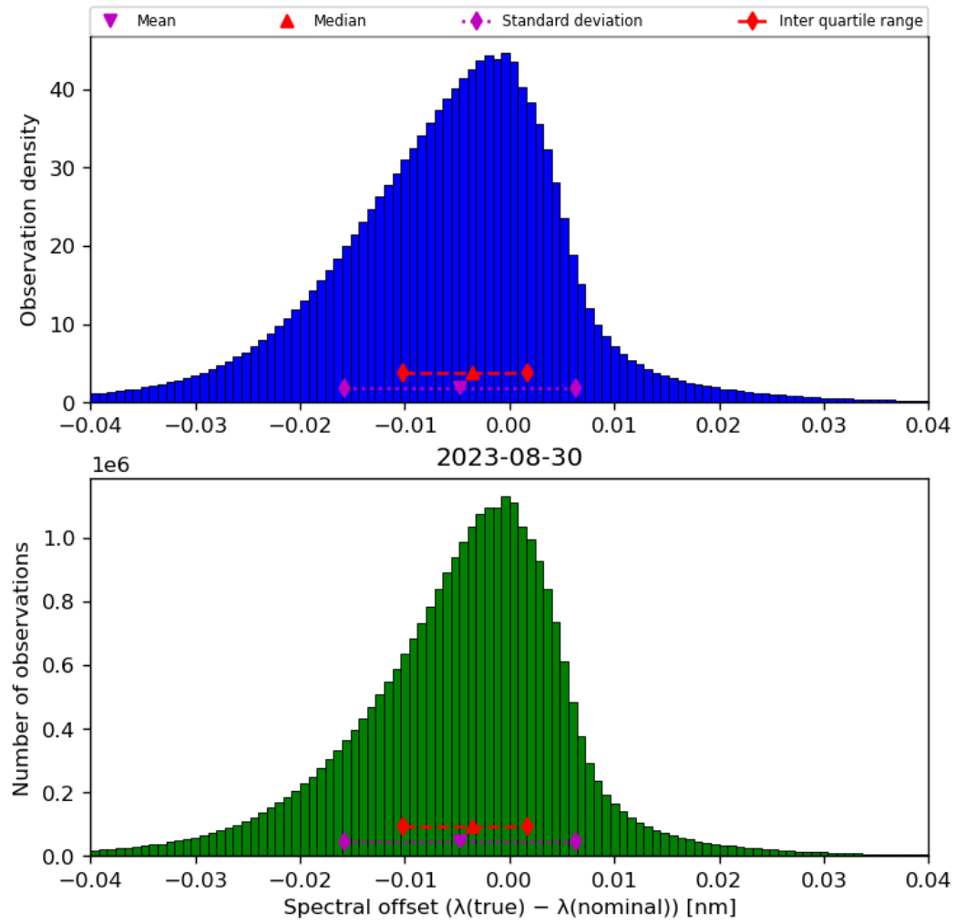
Figure 45: Histogram of “Spectral offset ( \lambda(\text{true}) - \lambda(\text{nominal}) )” for 2023-08-30 to 2023-08-31
