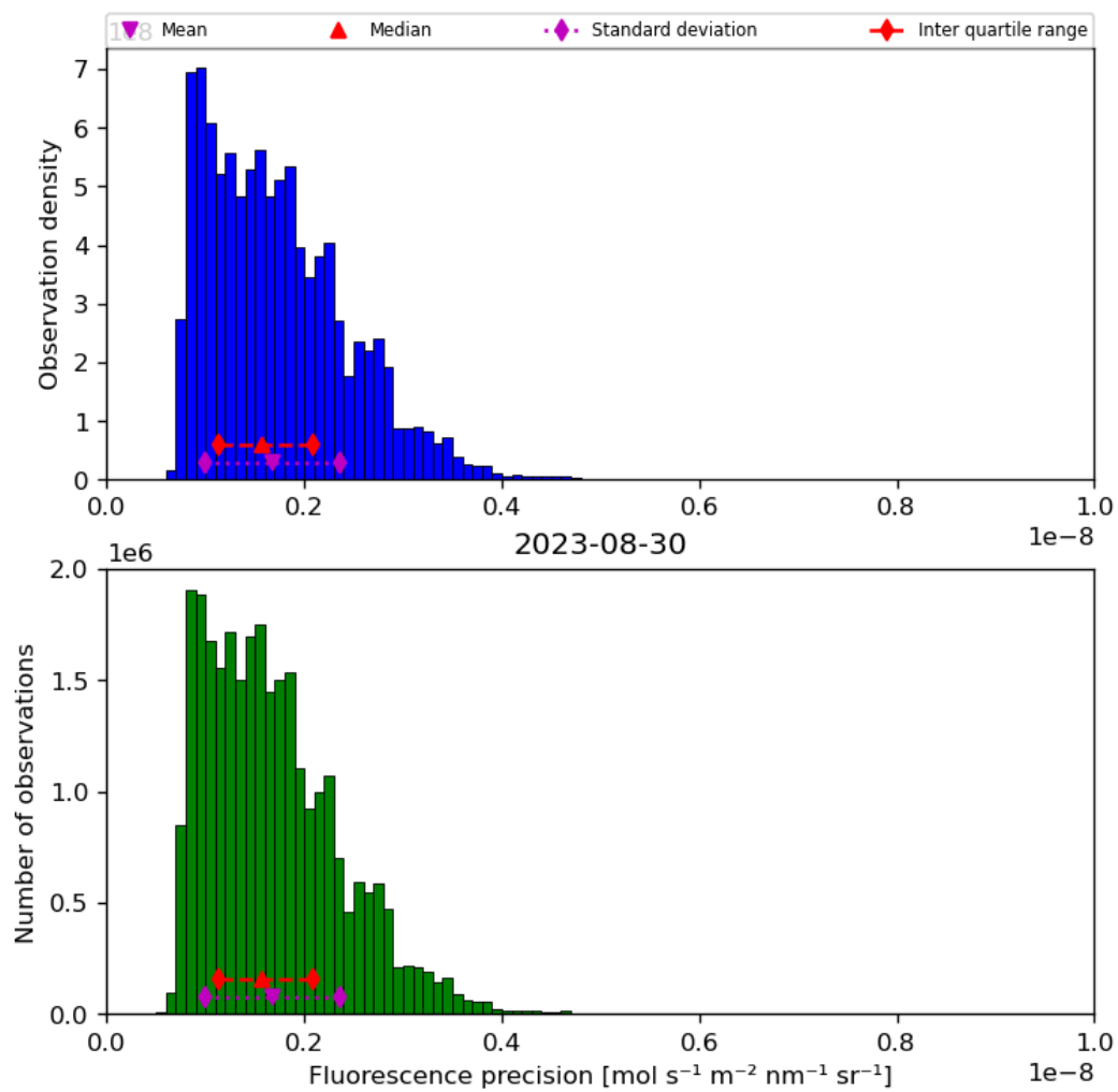
Figure 41: Histogram of “Fluorescence precision” for 2023-08-30 to 2023-08-31
