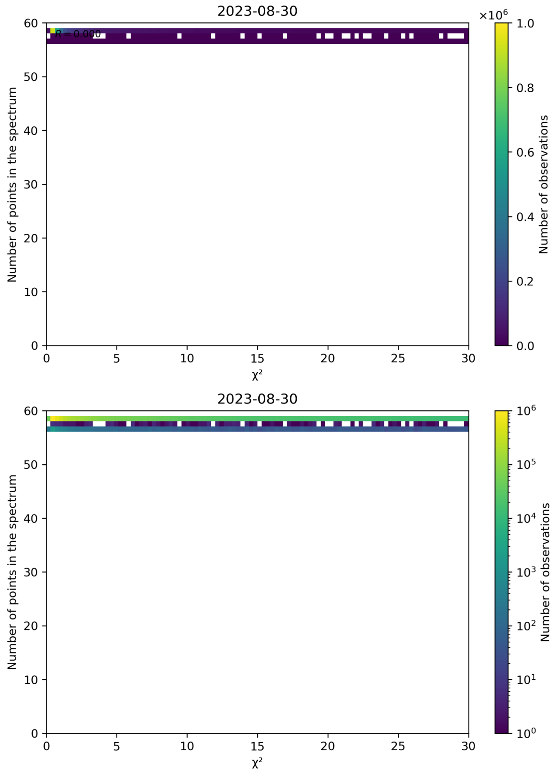
Figure 74: Scatter density plot of “ \chi^2 ” against “Number of points in the spectrum” for 2023-08-30 to 2023-08-31.
