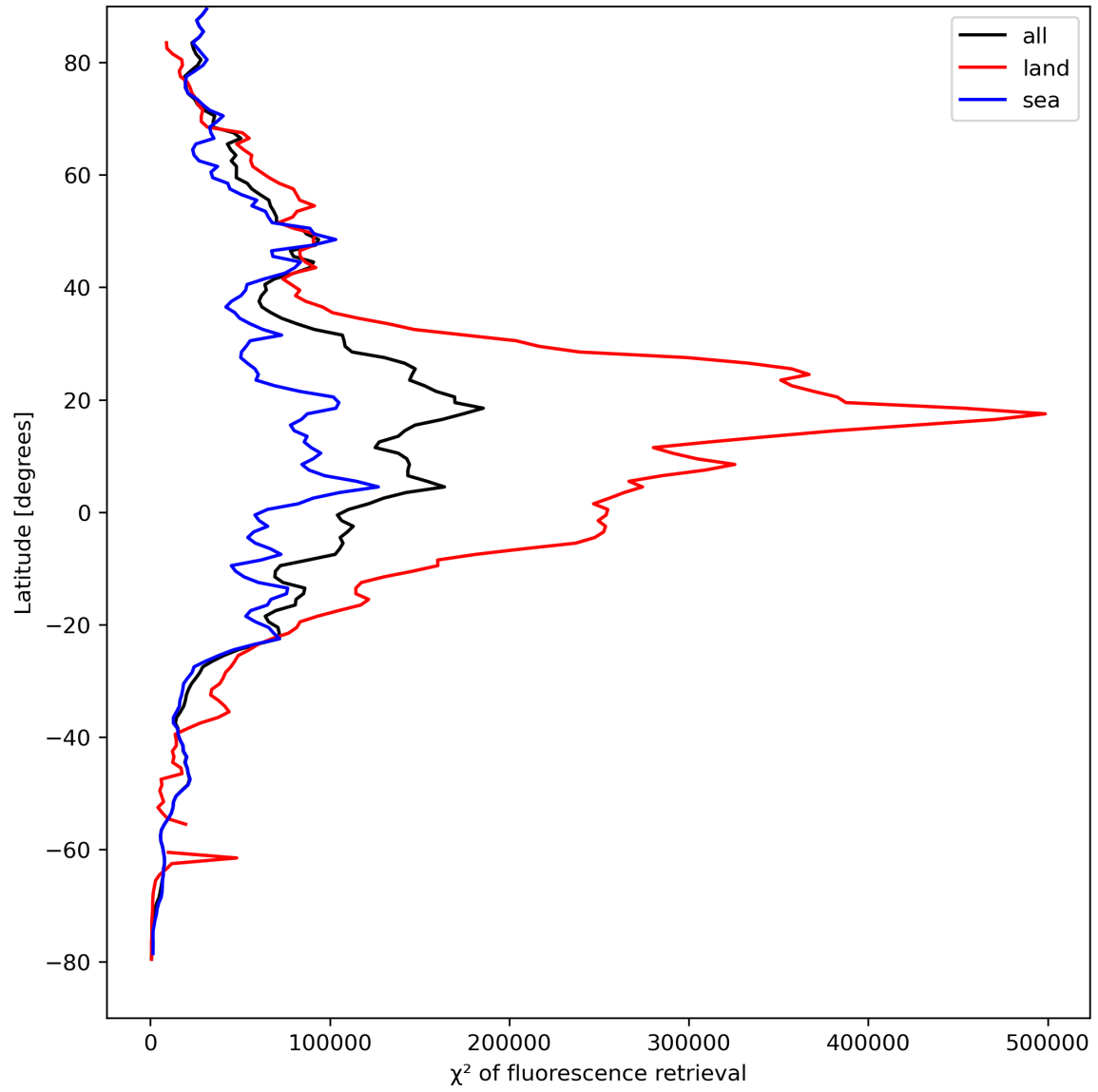
Figure 25: Zonal average of “ \chi^2 of fluorescence retrieval” for 2023-08-30 to 2023-08-31.
