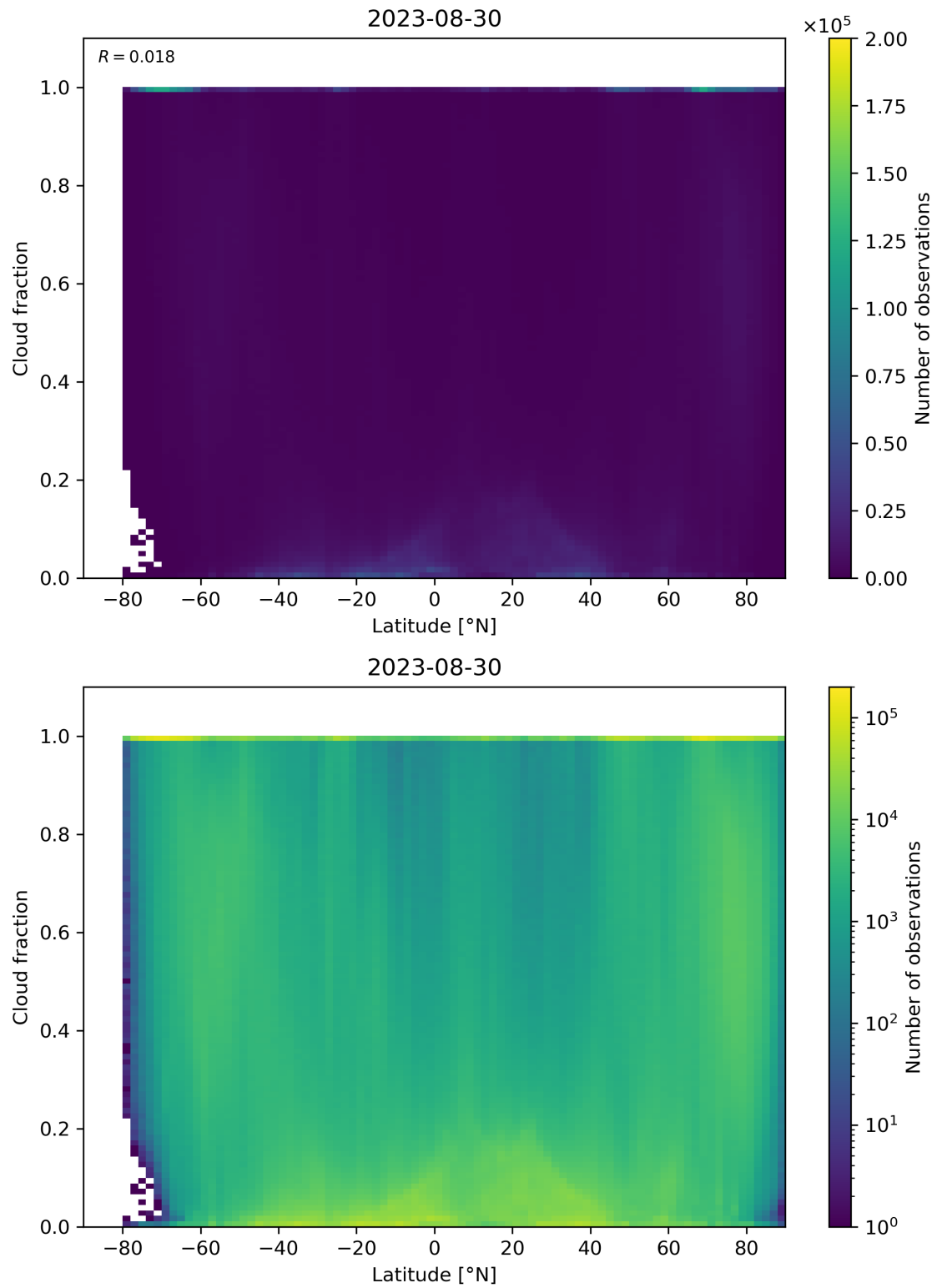
Figure 99: Scatter density plot of “Latitude” against “Cloud fraction” for 2023-08-30 to 2023-08-31.
