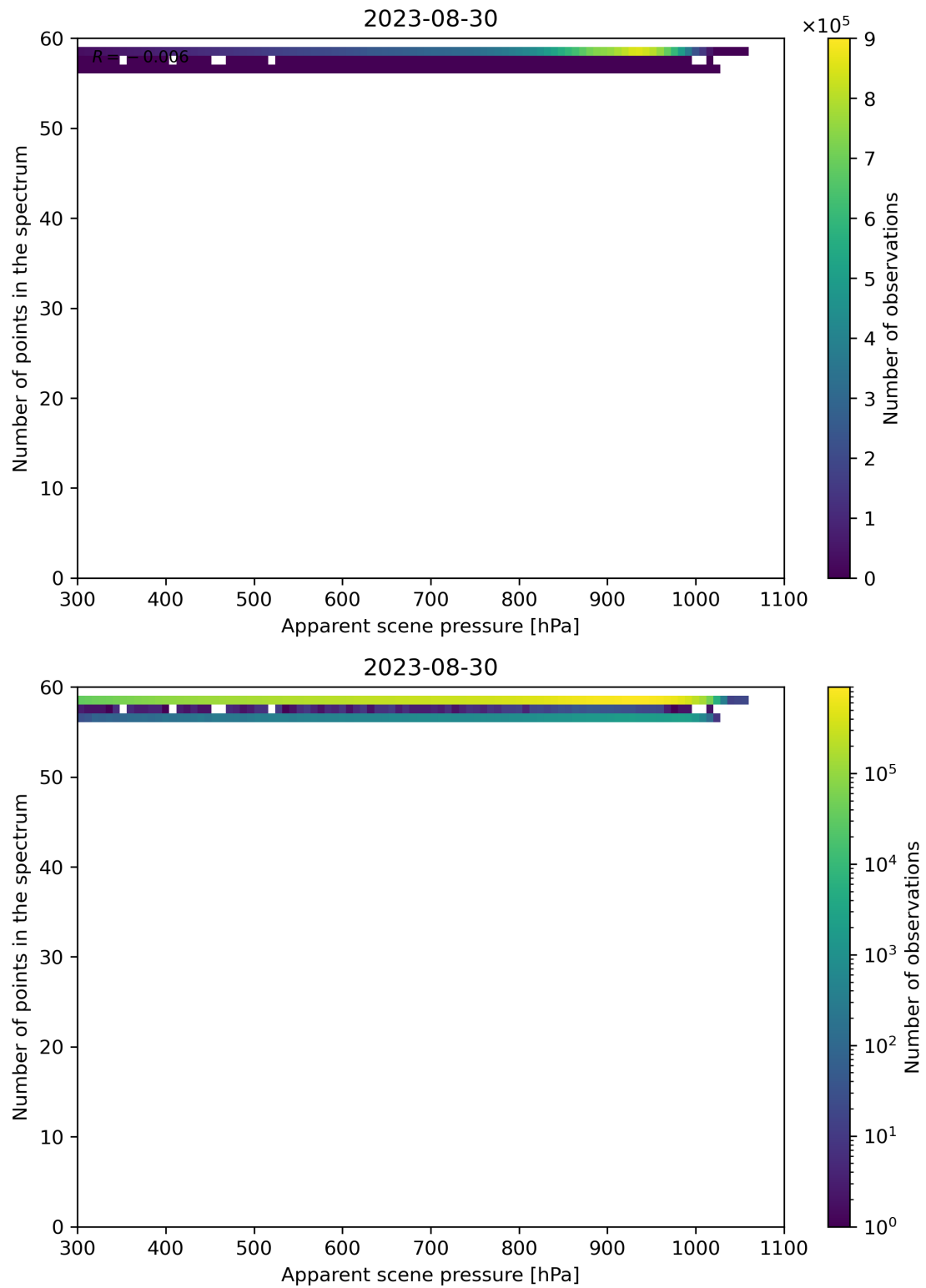
Figure 67: Scatter density plot of “Apparent scene pressure” against “Number of points in the spectrum” for 2023-08-30 to 2023-08-31.
