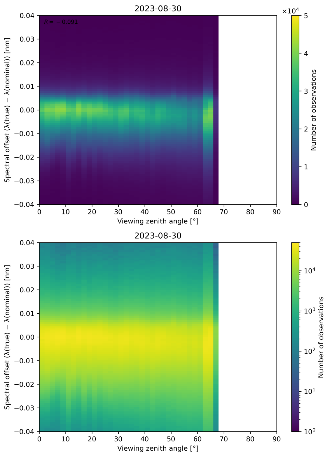
Figure 140: Scatter density plot of “Viewing zenith angle” against “Spectral offset ( \lambda(\text{true}) - \lambda(\text{nominal}) )” for 2023-08-30 to 2023-08-31.
