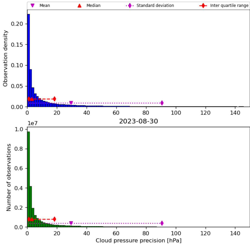
Figure 31: Histogram of “Cloud pressure precision” for 2023-08-30 to 2023-08-31
