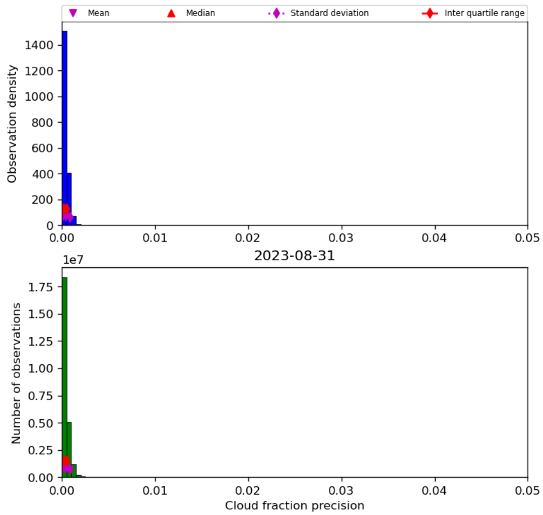
Figure 33: Histogram of “Cloud fraction precision” for 2023-08-30 to 2023-09-01
