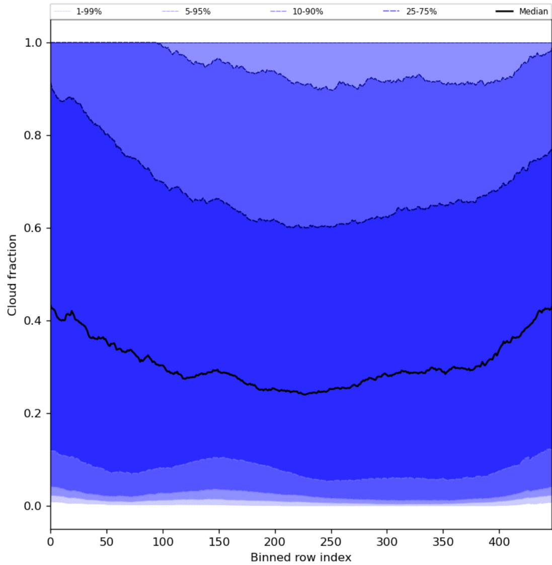
Figure 49: Along track statistics of “Cloud fraction” for 2023-08-30 to 2023-09-01
