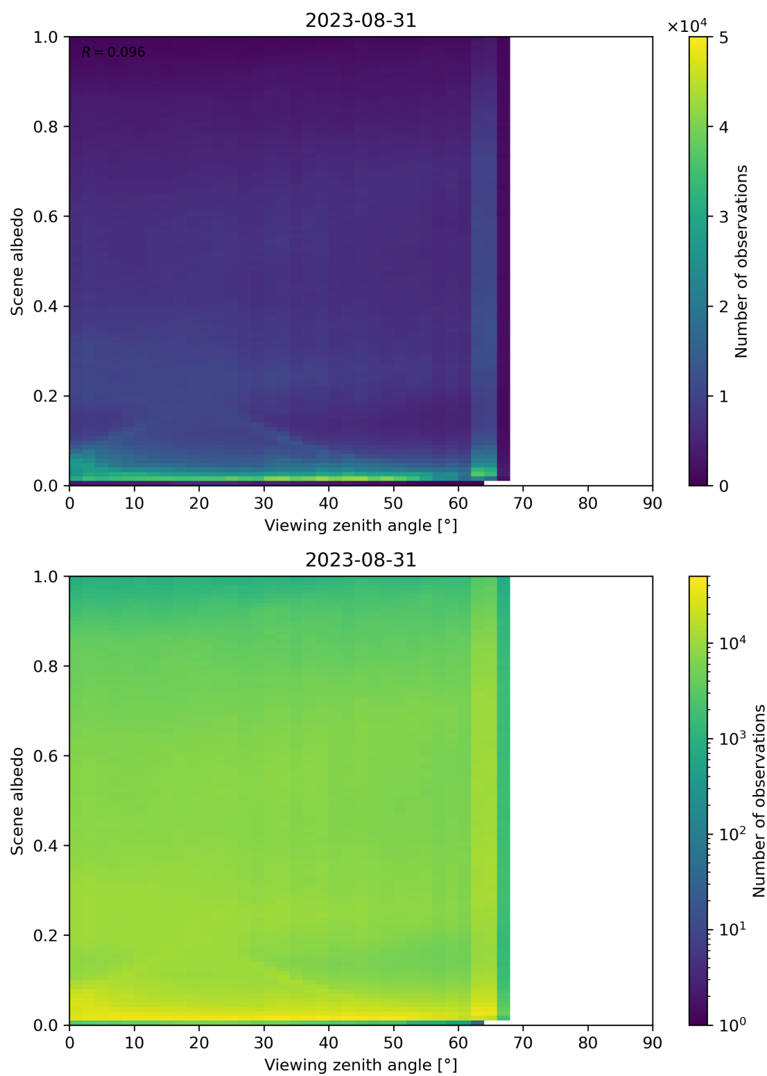
Figure 138: Scatter density plot of “Viewing zenith angle” against “Scene albedo” for 2023-08-30 to 2023-09-01.
