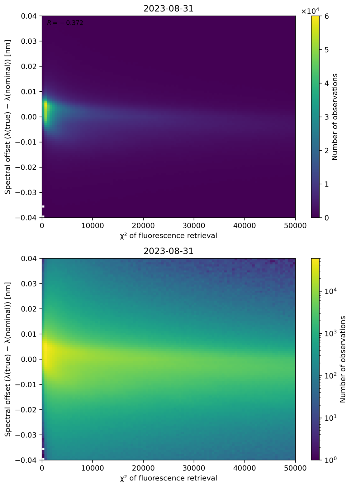
Figure 72: Scatter density plot of " \chi^2 of fluorescence retrieval" against "Spectral offset ( \lambda(\text{true}) - \lambda(\text{nominal}) )" for 2023-08-30 to 2023-09-01.
