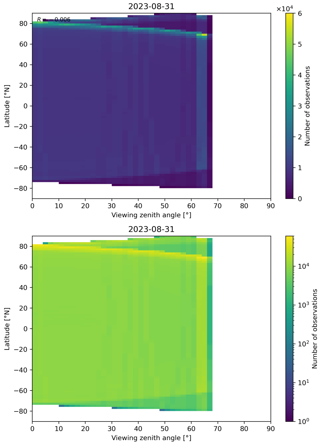
Figure 135: Scatter density plot of “Viewing zenith angle” against “Latitude” for 2023-08-30 to 2023-09-01.
