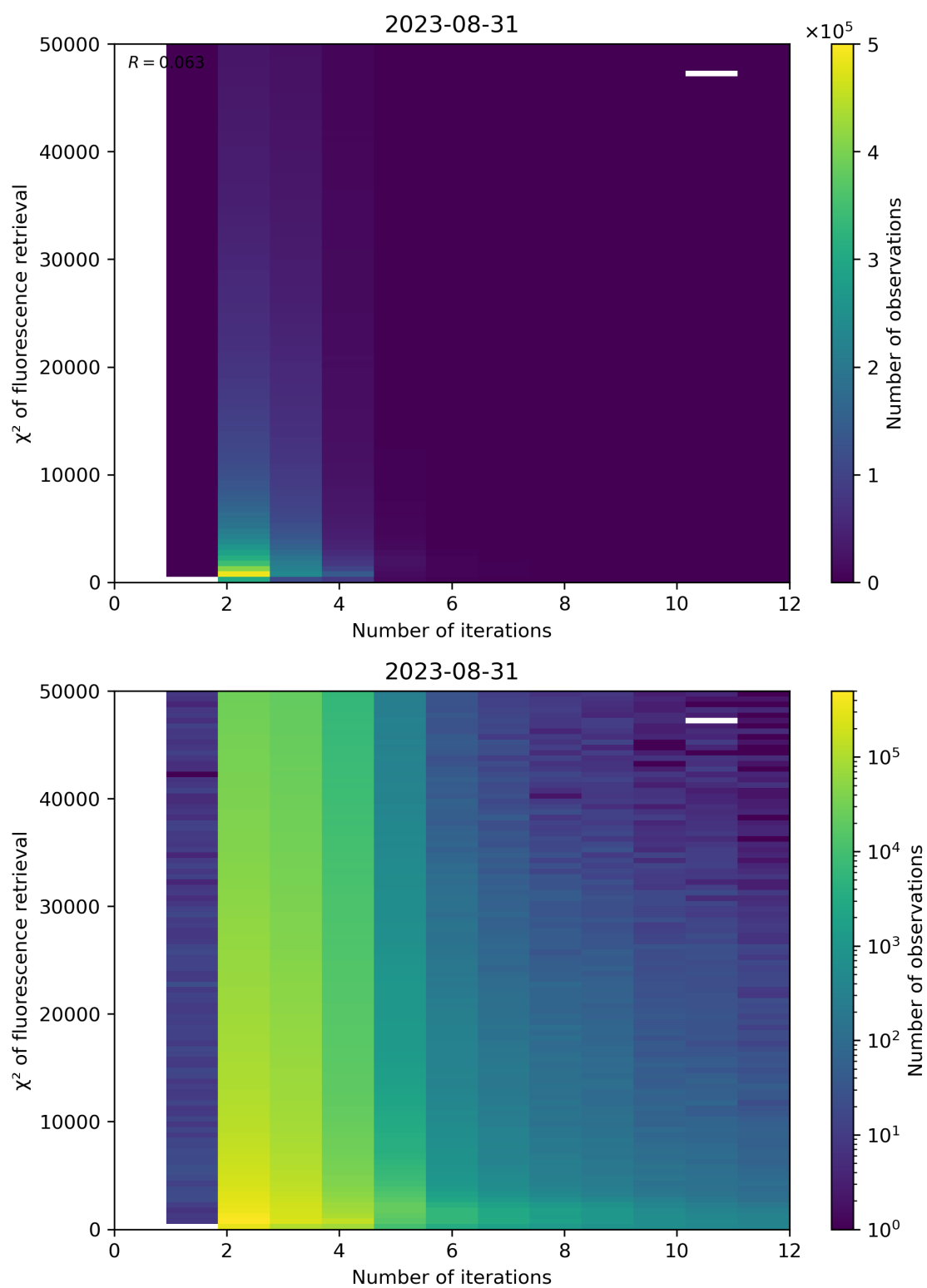
Figure 106: Scatter density plot of “Number of iterations” against “ \chi^2 of fluorescence retrieval” for 2023-08-30 to 2023-09-01.
