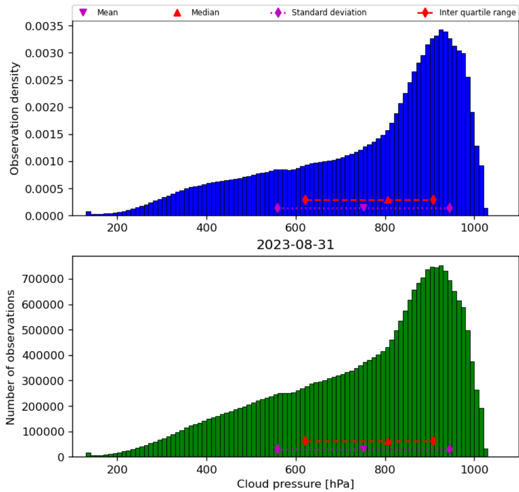
Figure 30: Histogram of “Cloud pressure” for 2023-08-30 to 2023-09-01
