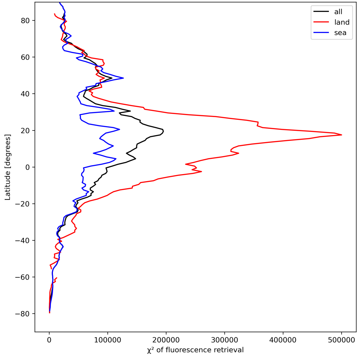
Figure 25: Zonal average of “ \chi^2 of fluorescence retrieval” for 2023-08-30 to 2023-09-01.
