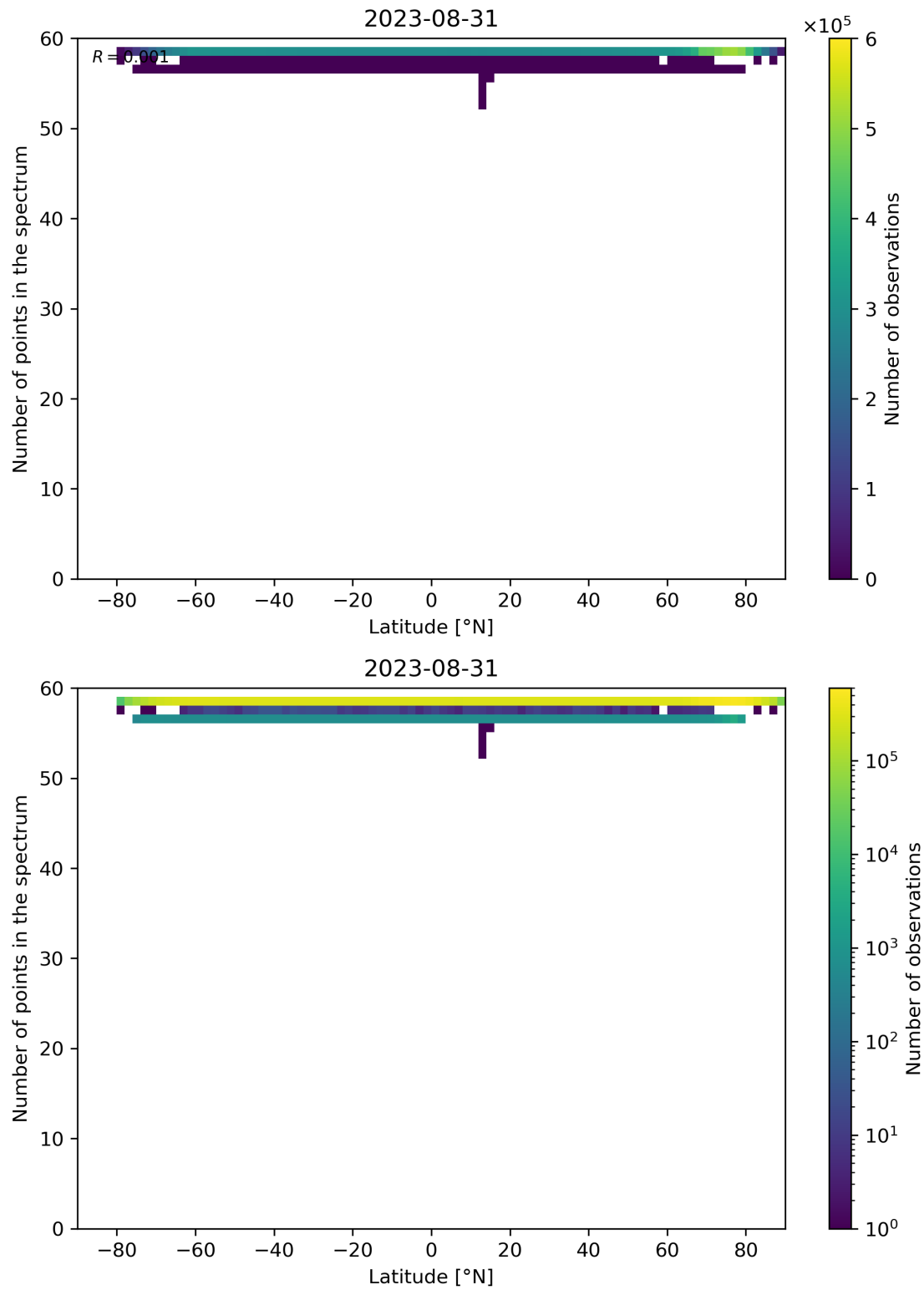
Figure 103: Scatter density plot of “Latitude” against “Number of points in the spectrum” for 2023-08-30 to 2023-09-01.
