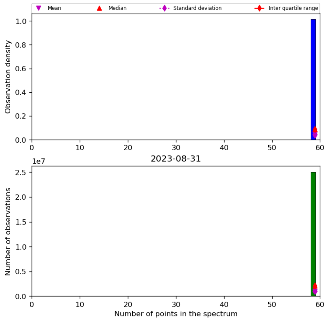
Figure 44: Histogram of “Number of points in the spectrum” for 2023-08-30 to 2023-09-01
