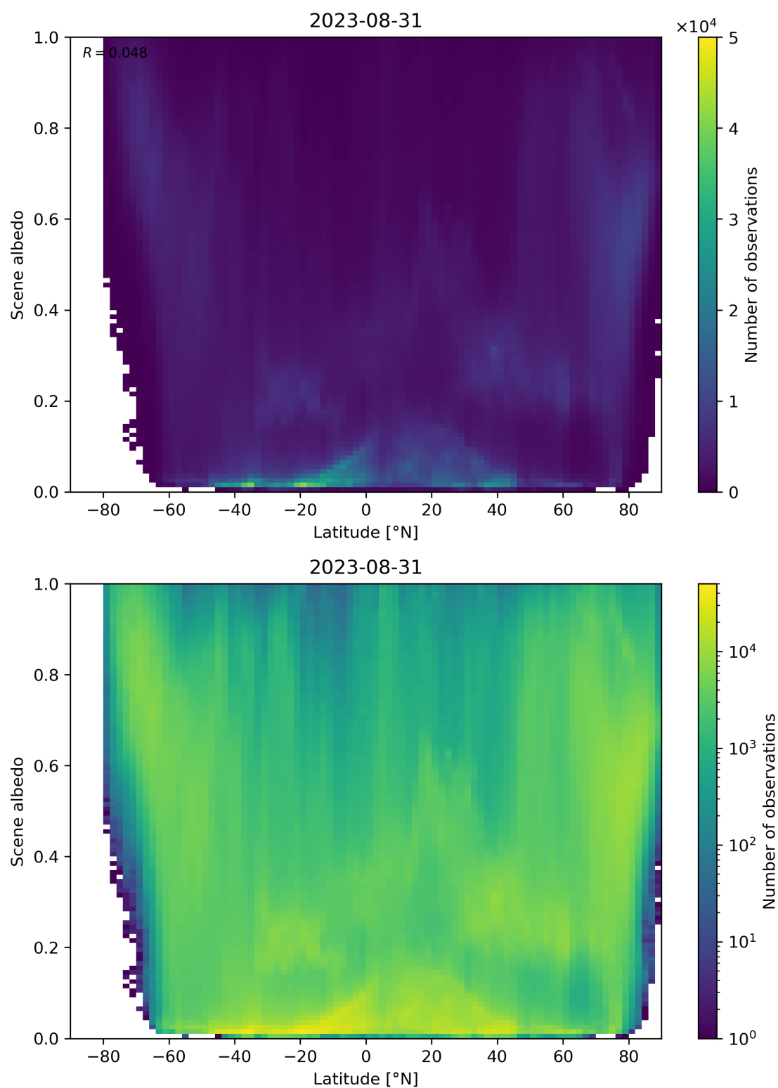
Figure 104: Scatter density plot of “Latitude” against “Scene albedo” for 2023-08-30 to 2023-09-01.
