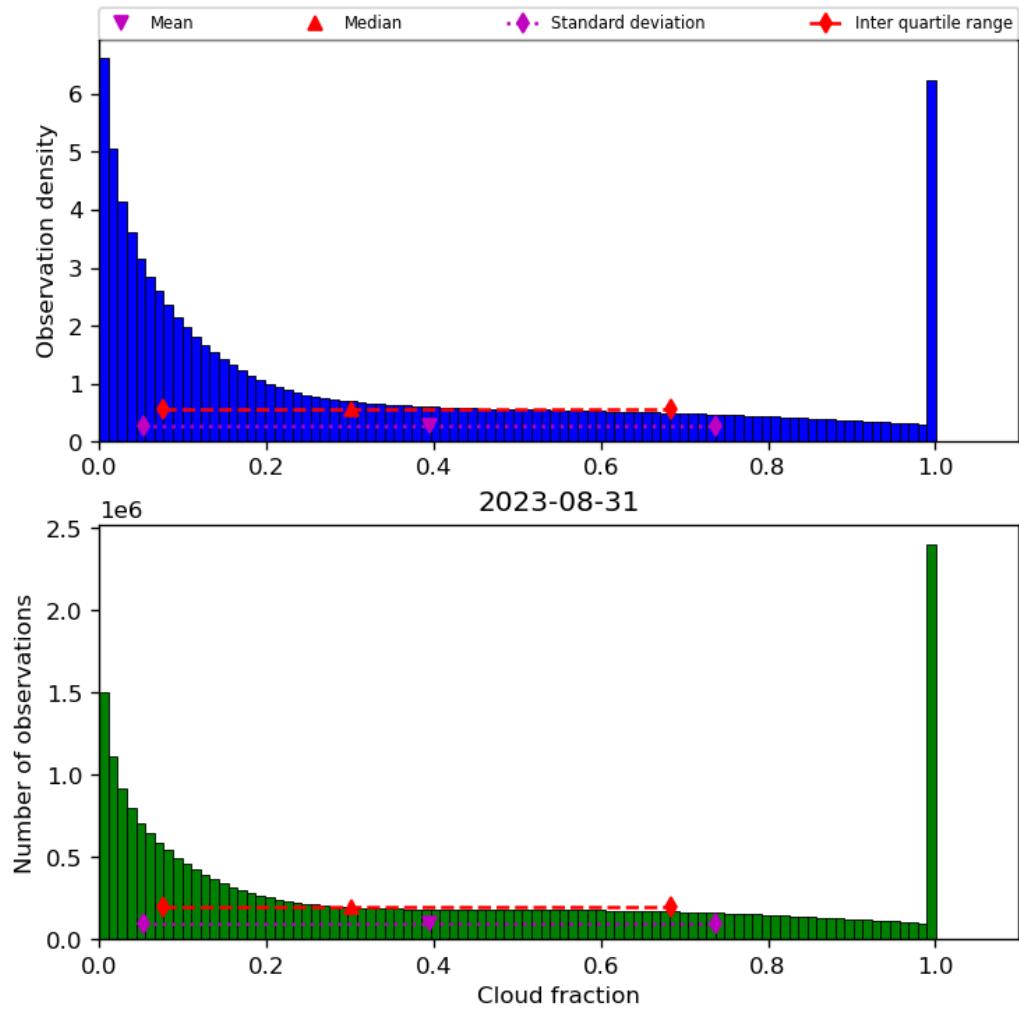
Figure 32: Histogram of “Cloud fraction” for 2023-08-30 to 2023-09-01
