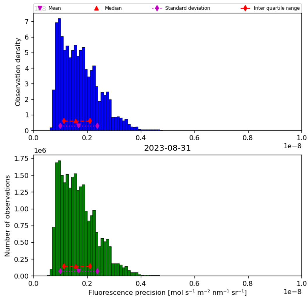
Figure 41: Histogram of “Fluorescence precision” for 2023-08-30 to 2023-09-01
