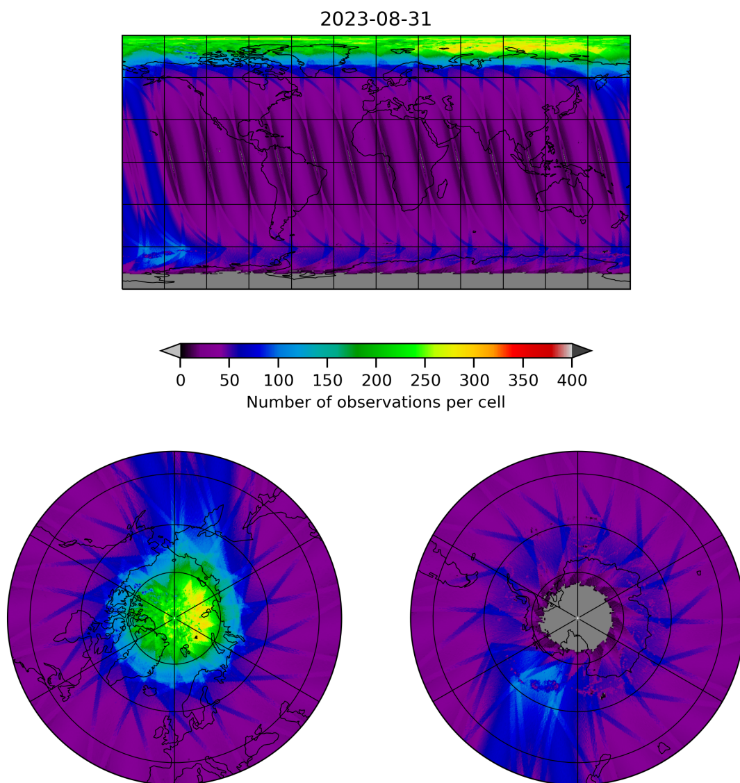
Figure 11: Map of the number of observations for 2023-08-30 to 2023-09-01
