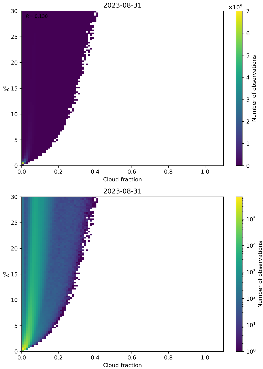
Figure 77: Scatter density plot of “Cloud fraction” against “ \chi^2 ” for 2023-08-30 to 2023-09-01.
