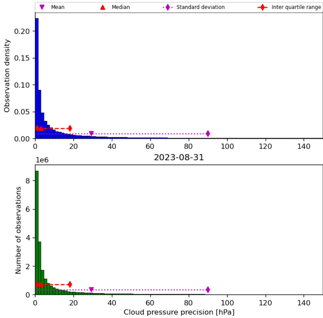
Figure 31: Histogram of “Cloud pressure precision” for 2023-08-30 to 2023-09-01
