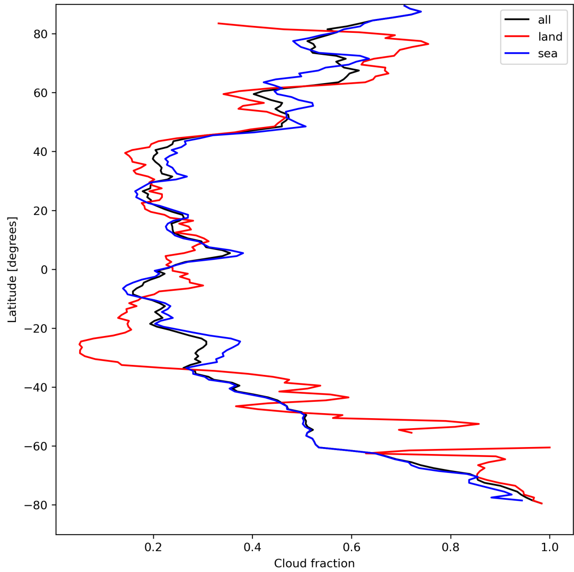
Figure 15: Zonal average of “Cloud fraction” for 2023-08-30 to 2023-09-01.
