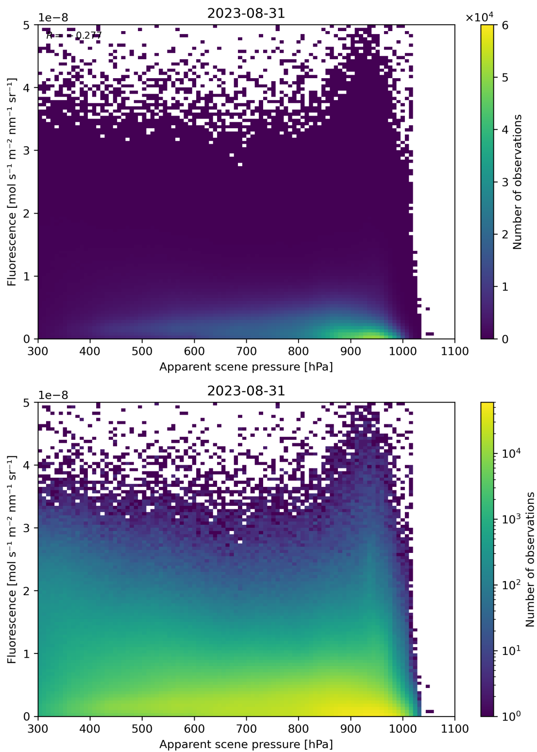
Figure 65: Scatter density plot of “Apparent scene pressure” against “Fluorescence” for 2023-08-30 to 2023-09-01.
