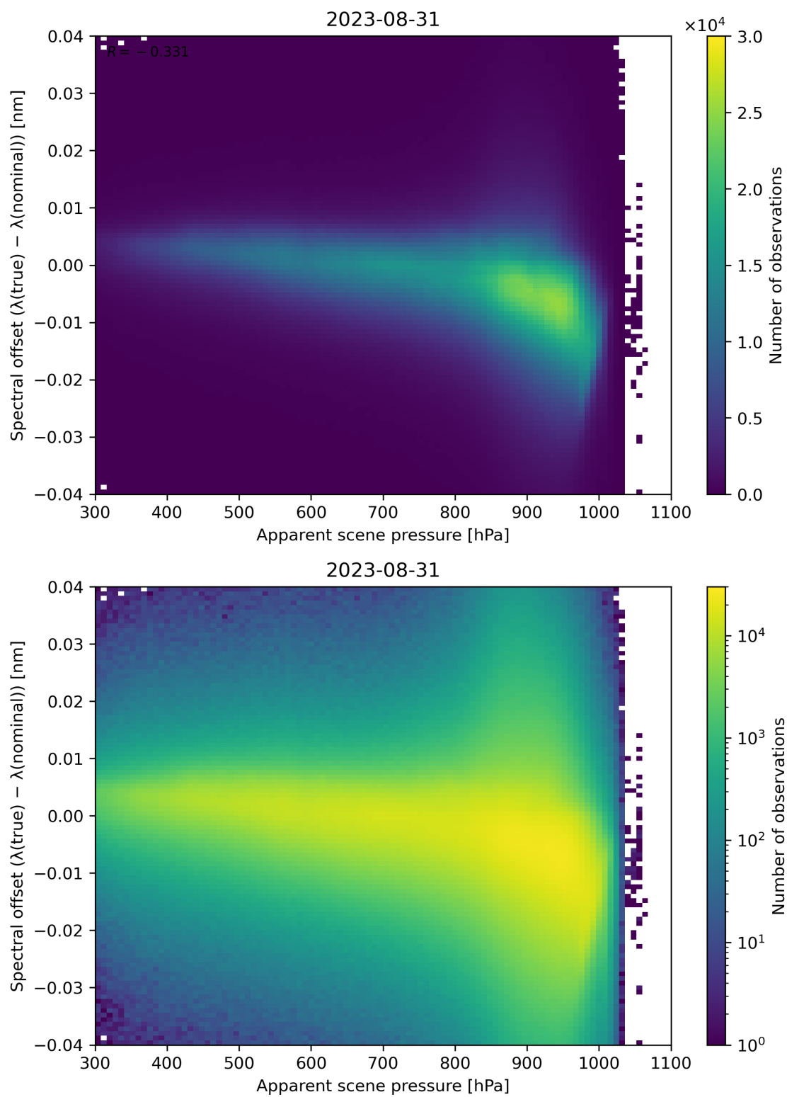
Figure 68: Scatter density plot of “Apparent scene pressure” against “Spectral offset ( \lambda(\text{true}) - \lambda(\text{nominal}) )” for 2023-08-30 to 2023-09-01.
