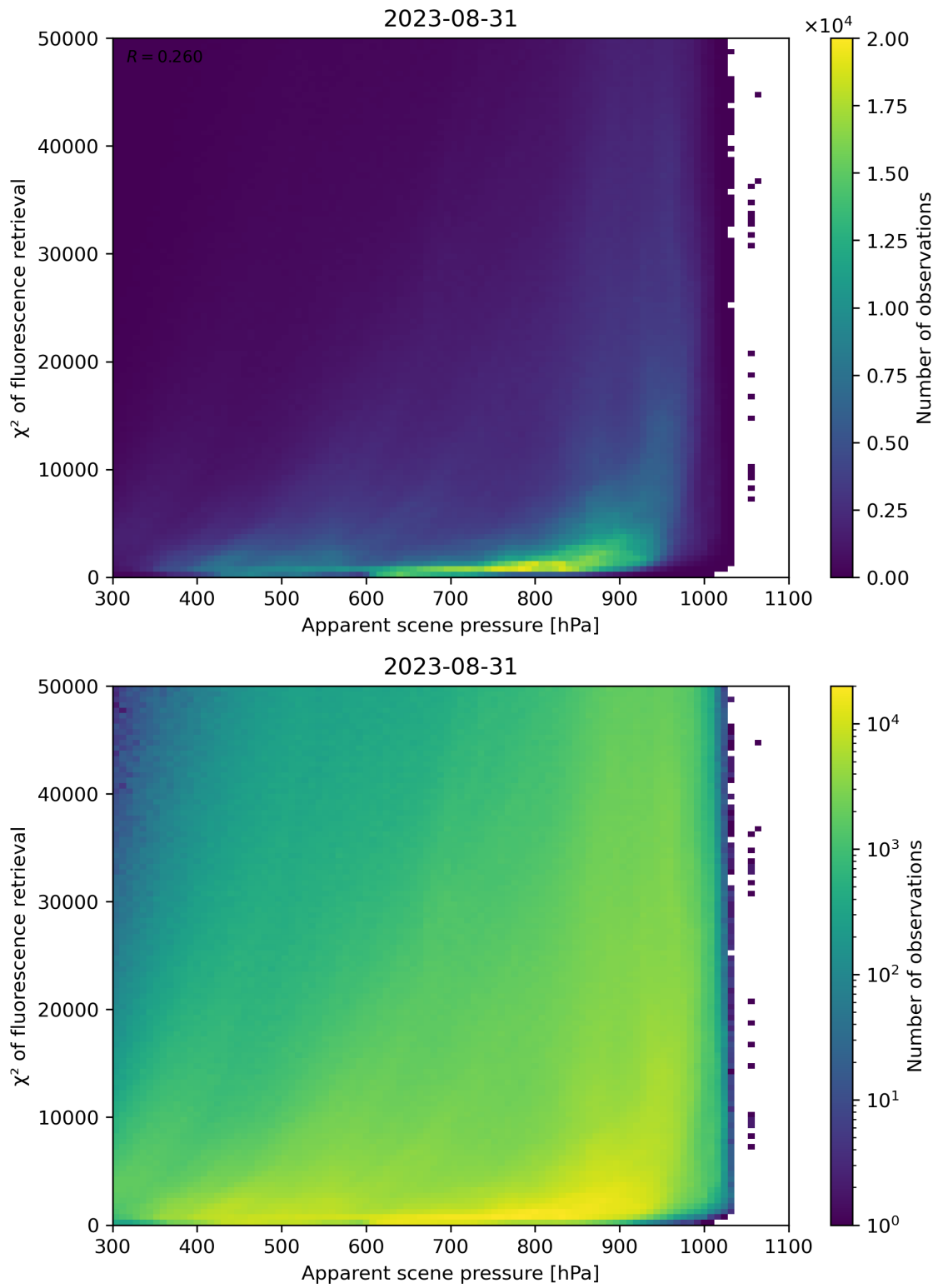
Figure 64: Scatter density plot of “Apparent scene pressure” against “ \chi^2 of fluorescence retrieval” for 2023-08-30 to 2023-09-01.
