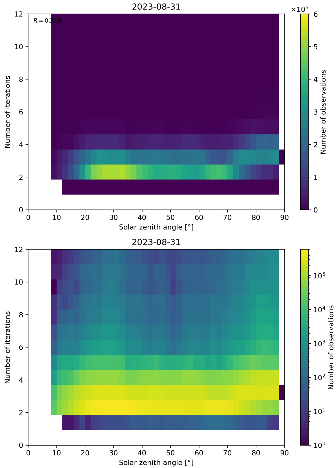
Figure 125: Scatter density plot of “Solar zenith angle” against “Number of iterations” for 2023-08-30 to 2023-09-01.
