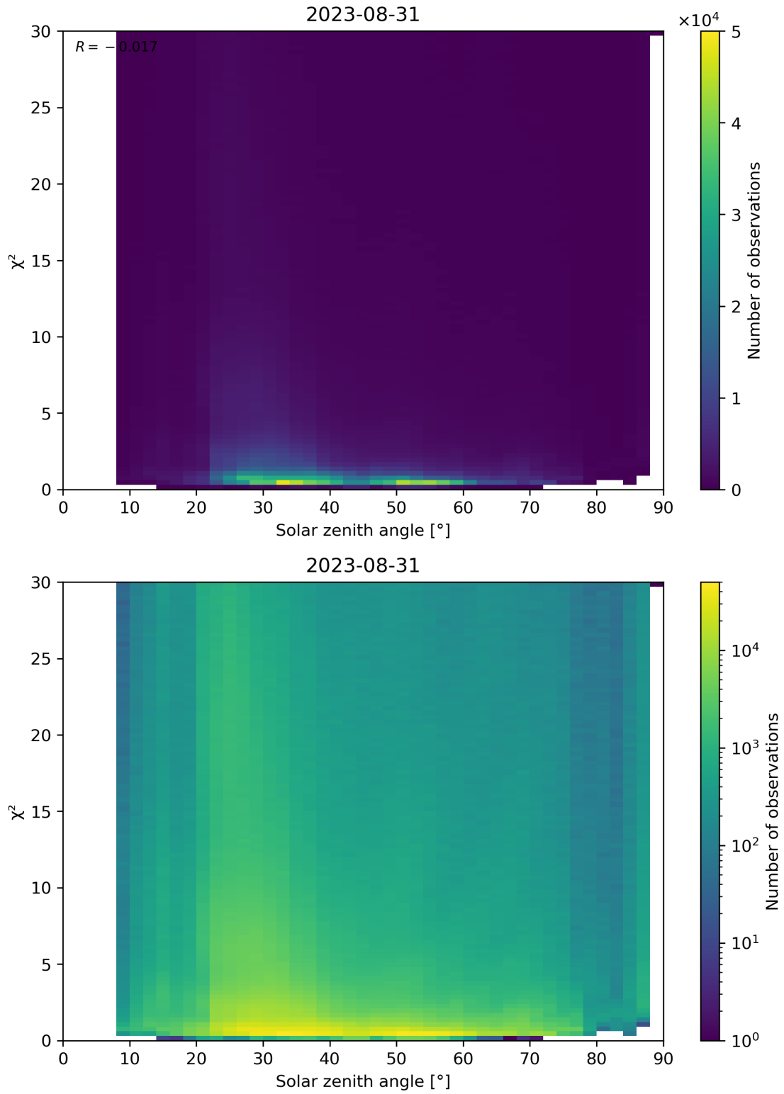
Figure 119: Scatter density plot of “Solar zenith angle” against “ \chi^2 ” for 2023-08-30 to 2023-09-01.
