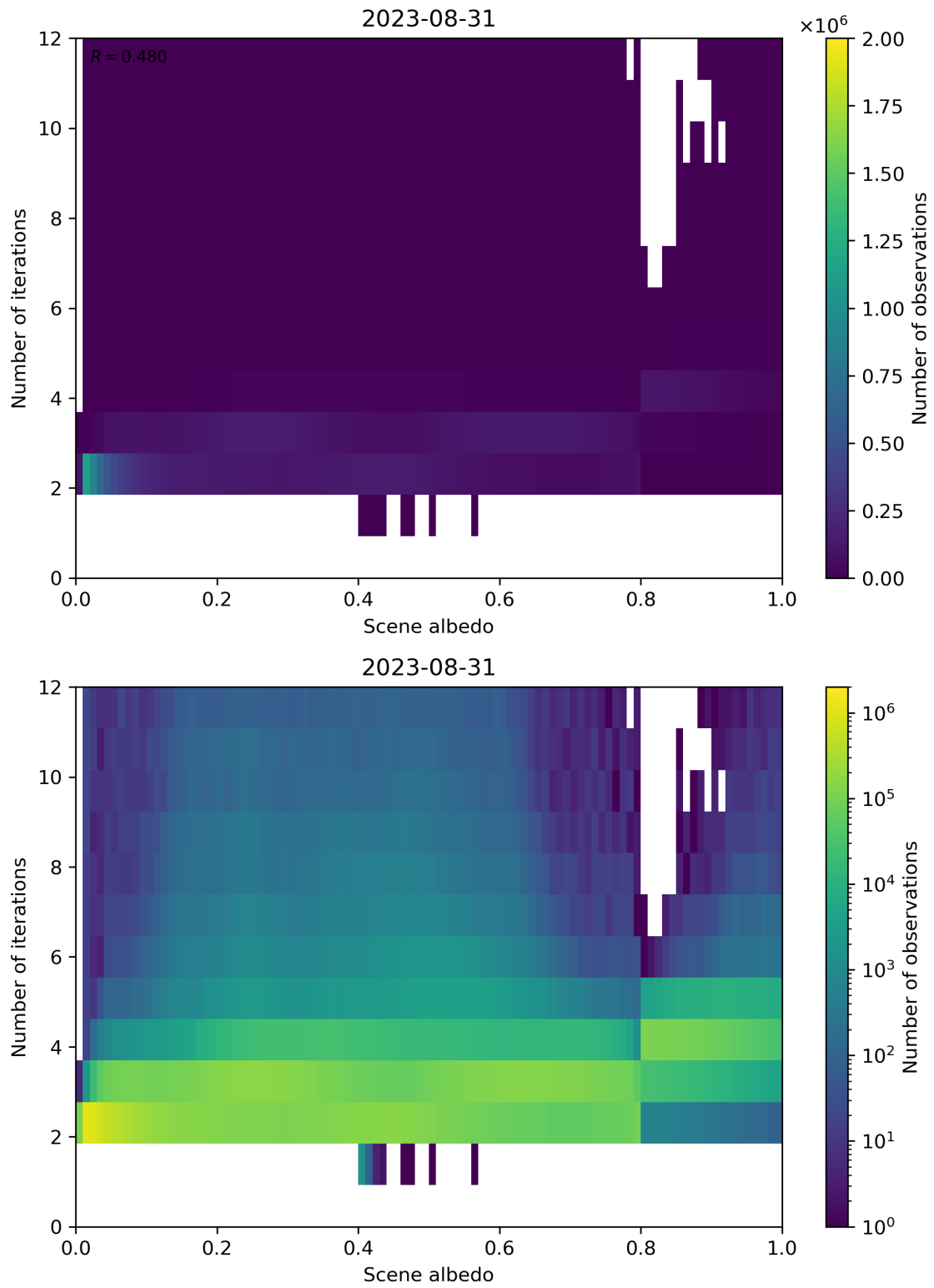
Figure 115: Scatter density plot of “Scene albedo” against “Number of iterations” for 2023-08-30 to 2023-09-01.
