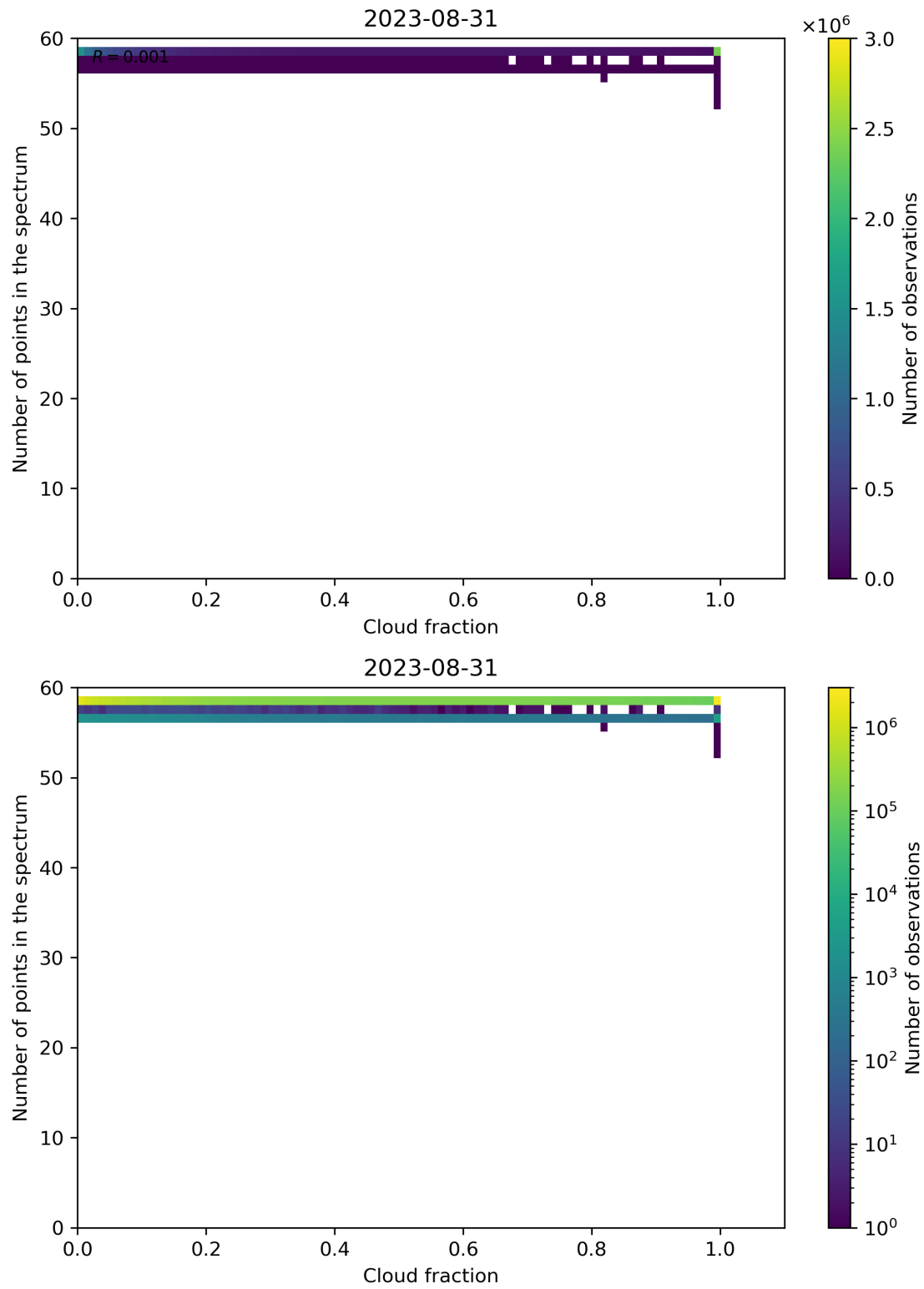
Figure 81: Scatter density plot of “Cloud fraction” against “Number of points in the spectrum” for 2023-08-30 to 2023-09-01.
