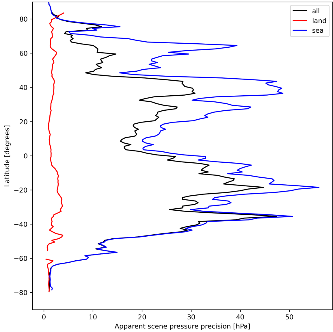
Figure 20: Zonal average of “Apparent scene pressure precision” for 2023-08-30 to 2023-09-01.
