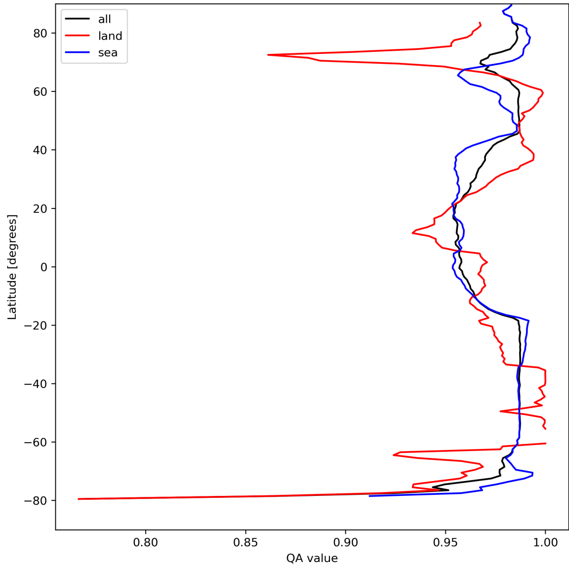
Figure 12: Zonal average of “QA value” for 2023-08-30 to 2023-09-01.
