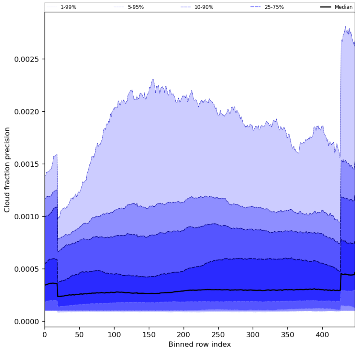
Figure 50: Along track statistics of “Cloud fraction precision” for 2023-08-30 to 2023-09-01
