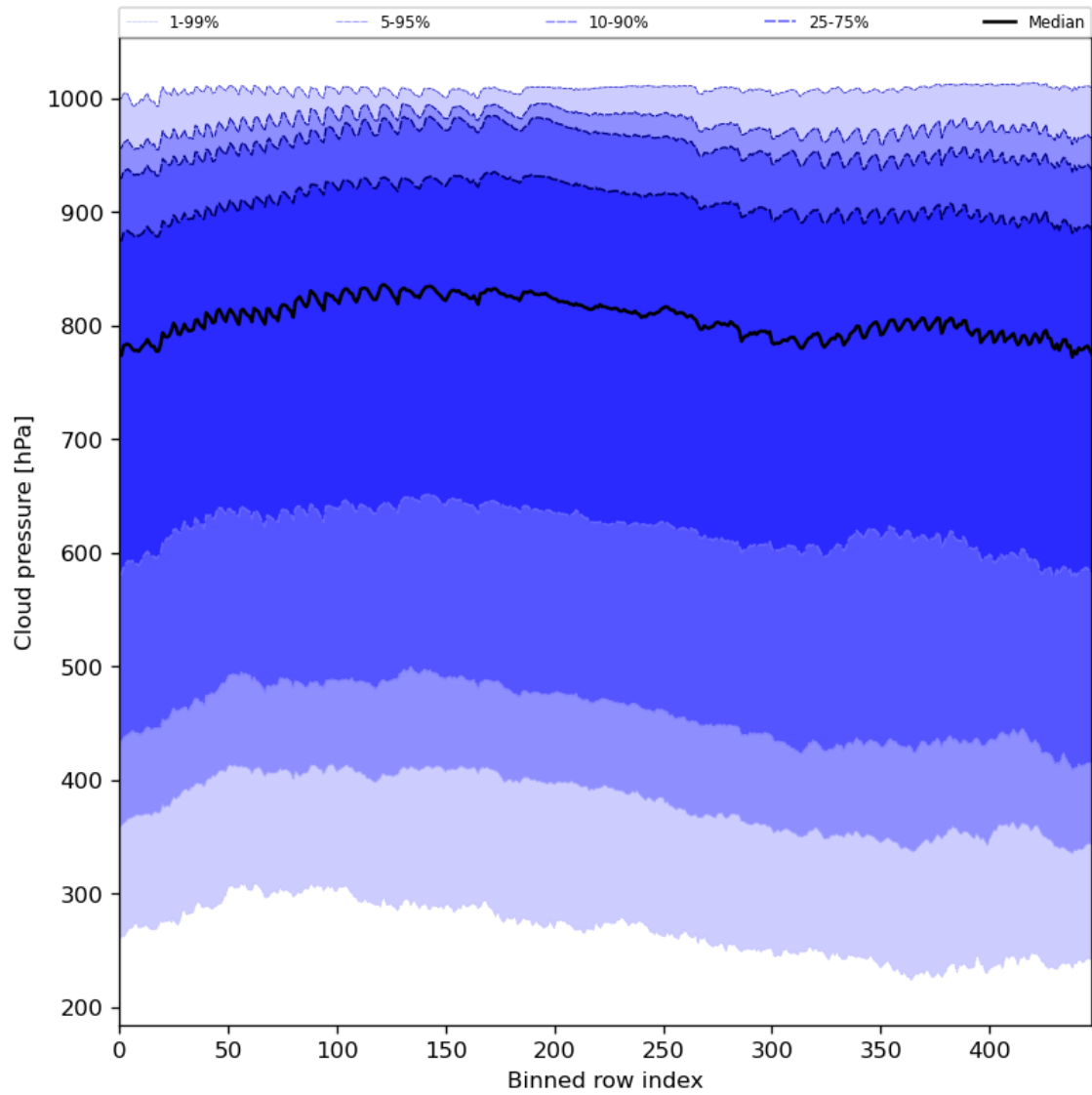
Figure 47: Along track statistics of "Cloud pressure" for 2023-08-30 to 2023-09-01
