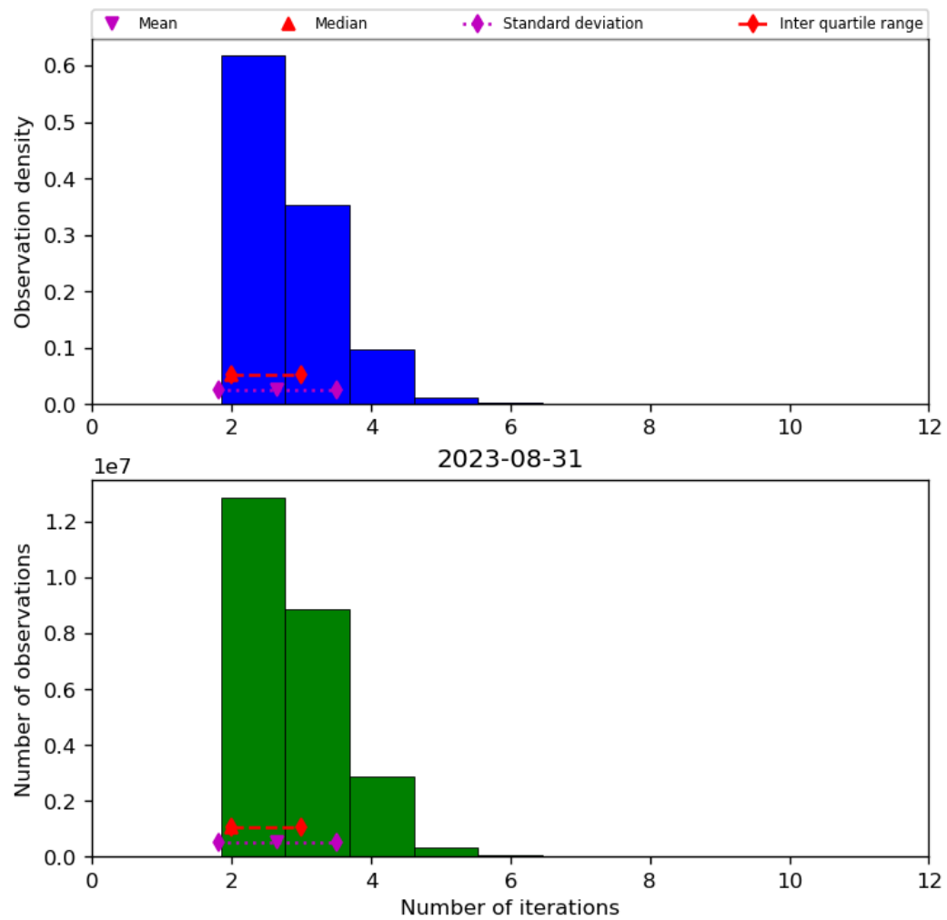
Figure 39: Histogram of “Number of iterations” for 2023-08-30 to 2023-09-01
