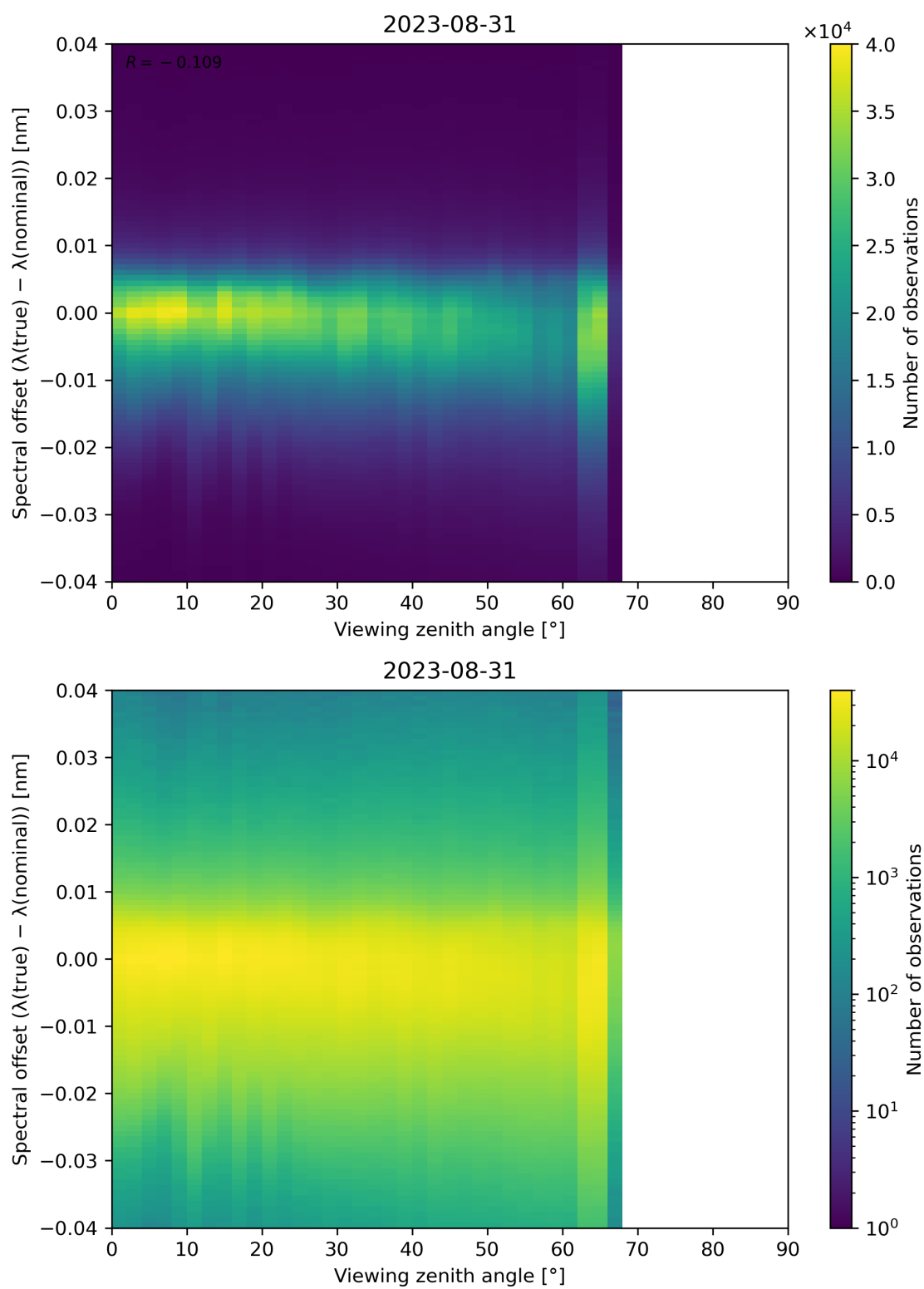
Figure 140: Scatter density plot of “Viewing zenith angle” against “Spectral offset ( \lambda(\text{true}) - \lambda(\text{nominal}) )” for 2023-08-30 to 2023-09-01.
