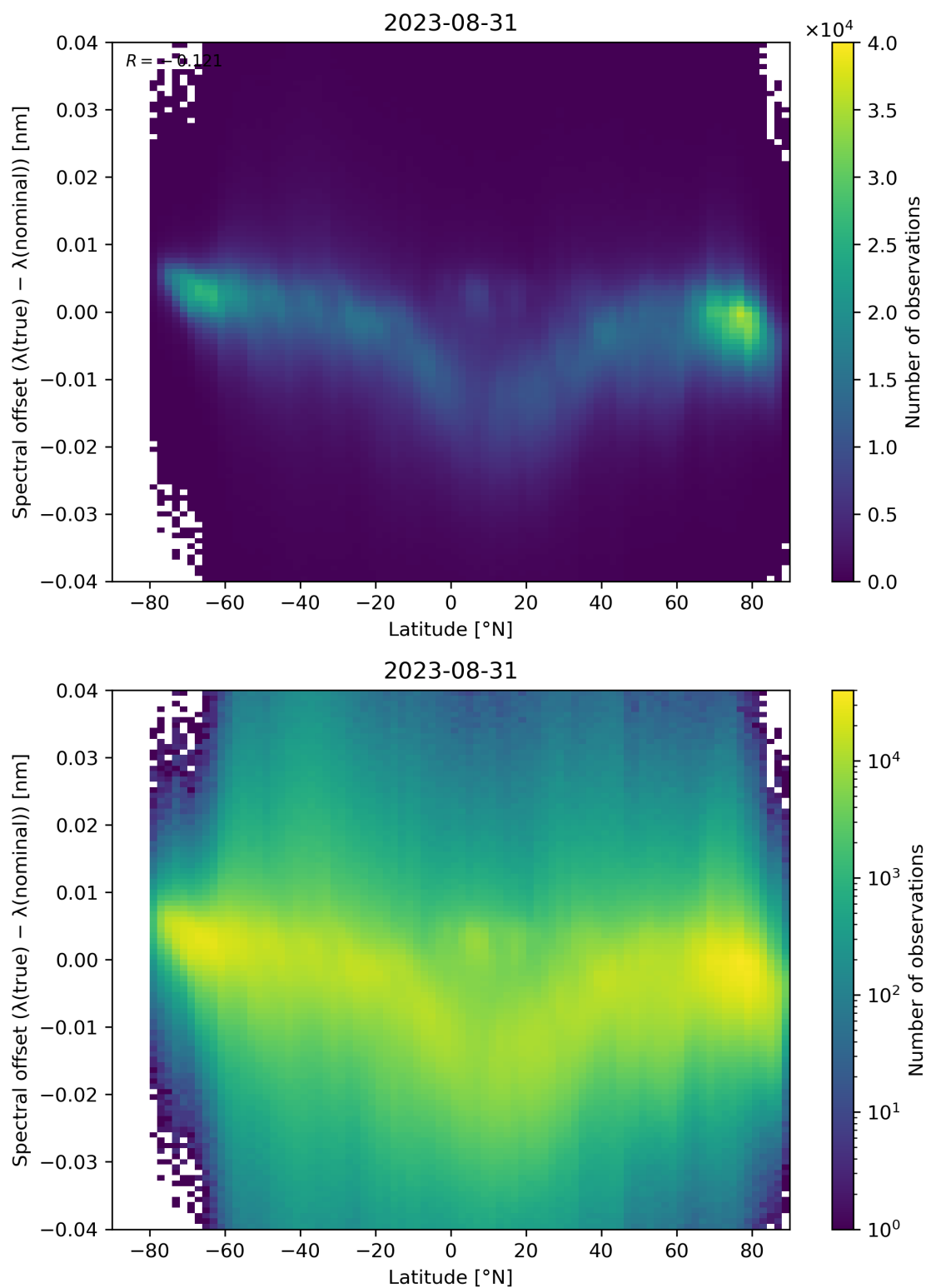
Figure 105: Scatter density plot of “Latitude” against “Spectral offset ( \lambda(\text{true}) - \lambda(\text{nominal}) )” for 2023-08-30 to 2023-09-01.
