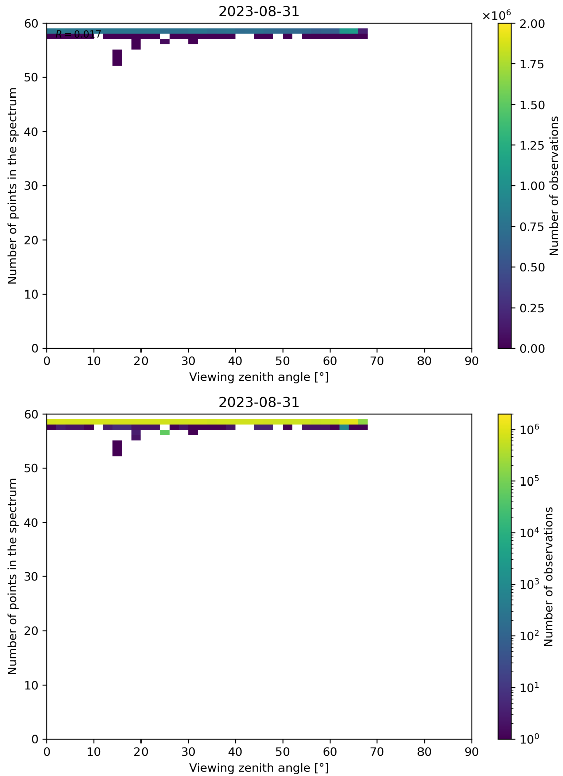
Figure 137: Scatter density plot of “Viewing zenith angle” against “Number of points in the spectrum” for 2023-08-30 to 2023-09-01.
