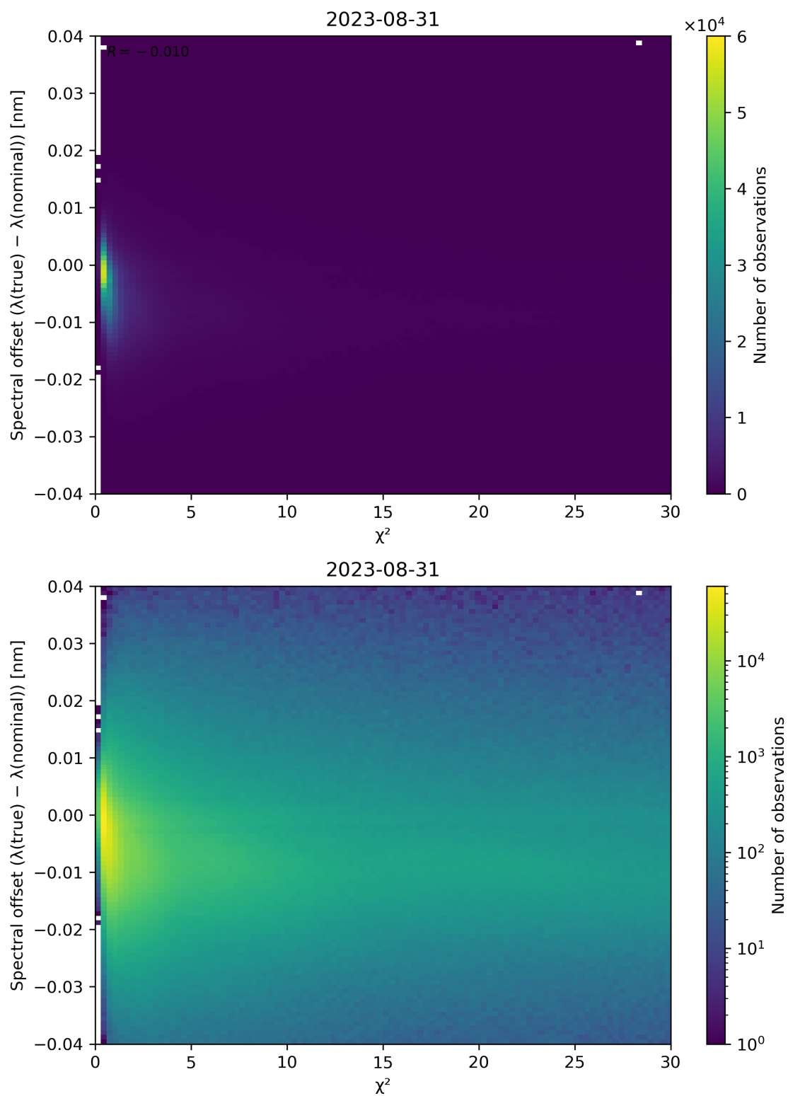
Figure 75: Scatter density plot of “ \chi^2 ” against “Spectral offset ( \lambda(\text{true}) - \lambda(\text{nominal}) )” for 2023-08-30 to 2023-09-01.
