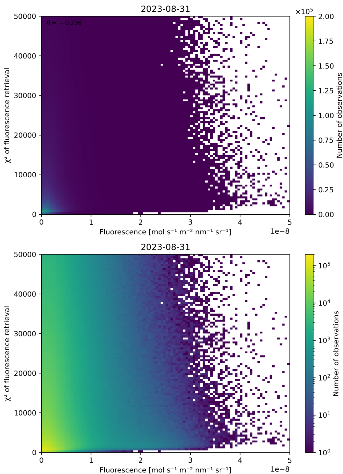
Figure 93: Scatter density plot of “Fluorescence” against “ \chi^2 of fluorescence retrieval” for 2023-08-30 to 2023-09-01.
