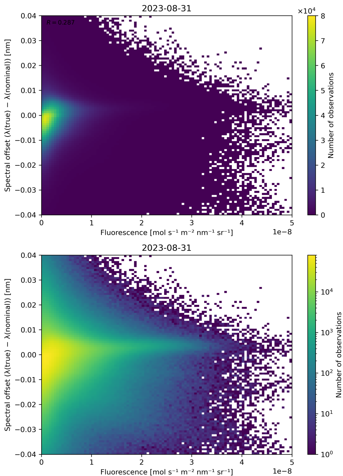
Figure 95: Scatter density plot of “Fluorescence” against “Spectral offset ( \lambda(\text{true}) - \lambda(\text{nominal}) )” for 2023-08-30 to 2023-09-01.
