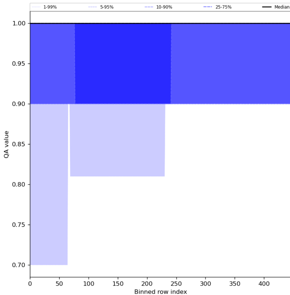
Figure 46: Along track statistics of “QA value” for 2023-08-30 to 2023-09-01
