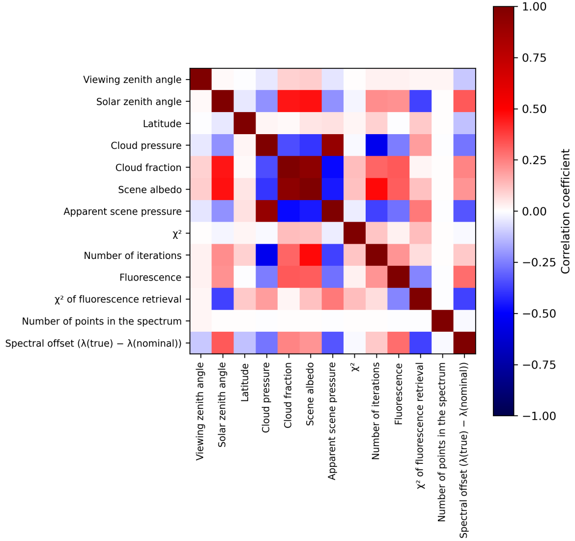
Figure 2: Map of correlation matrix for 2023-08-30 to 2023-09-01.
