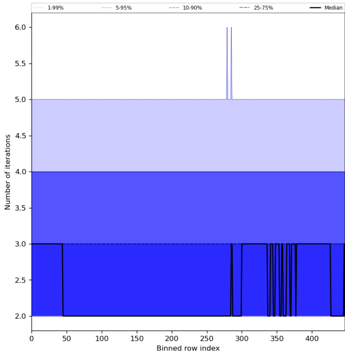
Figure 56: Along track statistics of “Number of iterations” for 2023-08-30 to 2023-09-01
