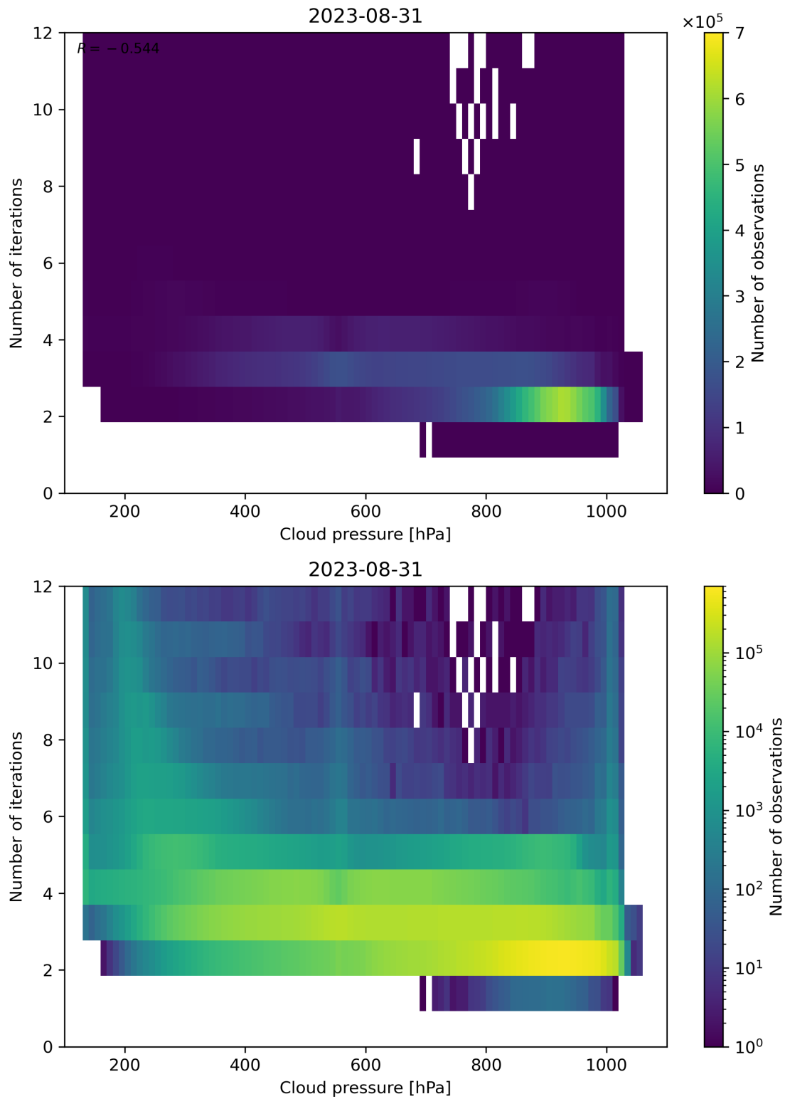
Figure 89: Scatter density plot of “Cloud pressure” against “Number of iterations” for 2023-08-30 to 2023-09-01.
