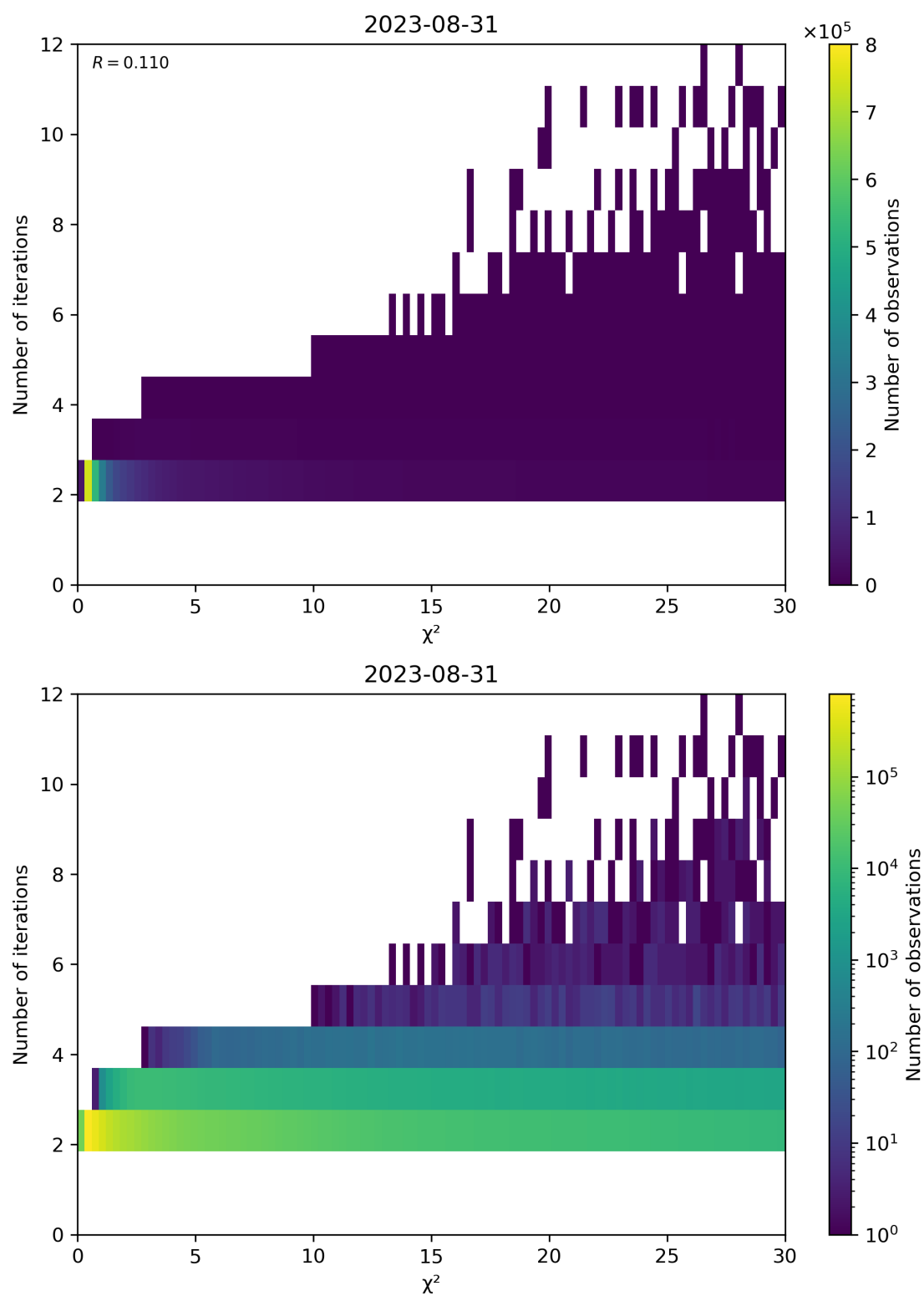
Figure 73: Scatter density plot of “ \chi^2 ” against “Number of iterations” for 2023-08-30 to 2023-09-01.
