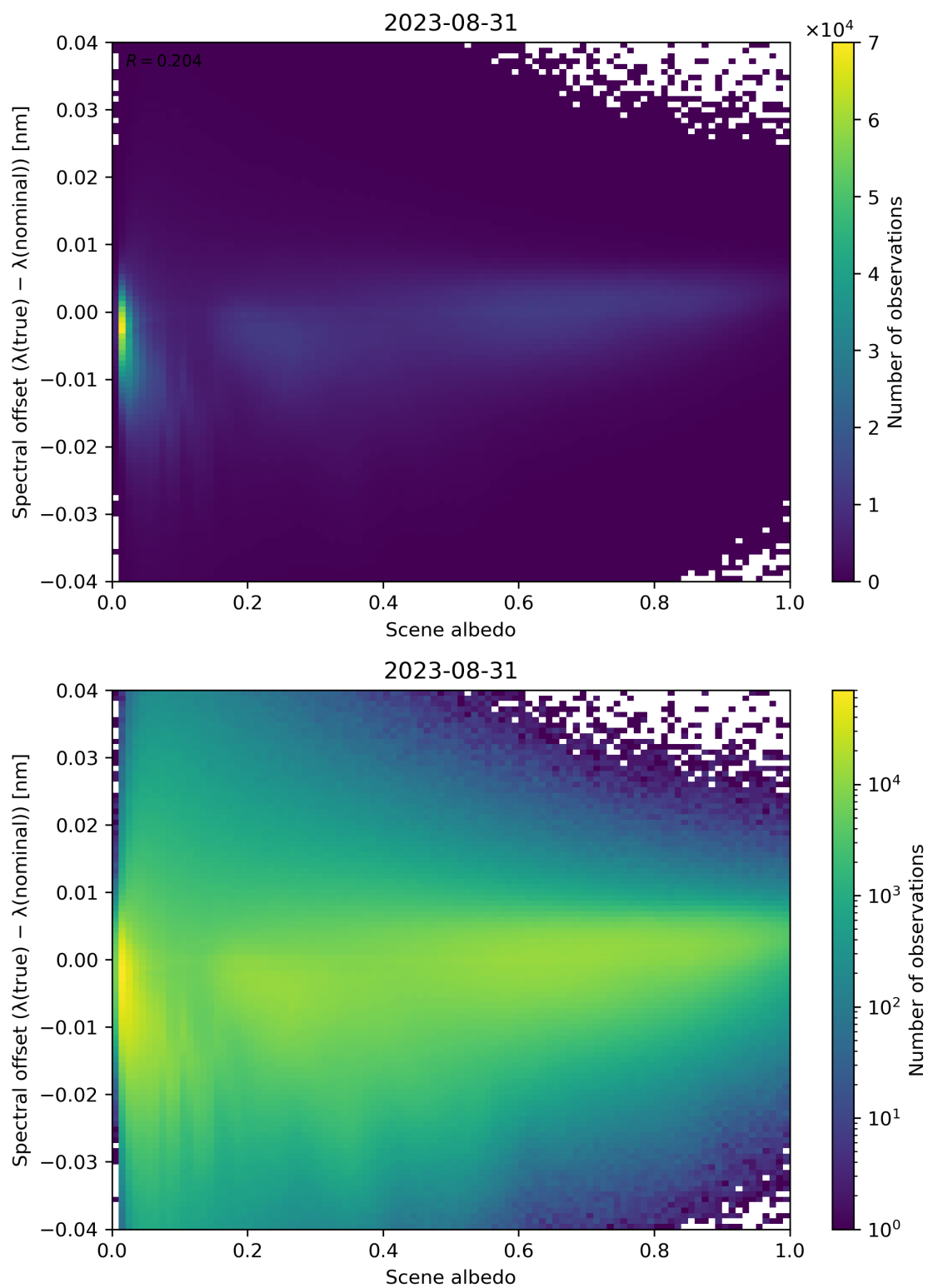
Figure 117: Scatter density plot of “Scene albedo” against “Spectral offset ( \lambda(\text{true}) - \lambda(\text{nominal}) )” for 2023-08-30 to 2023-09-01.
