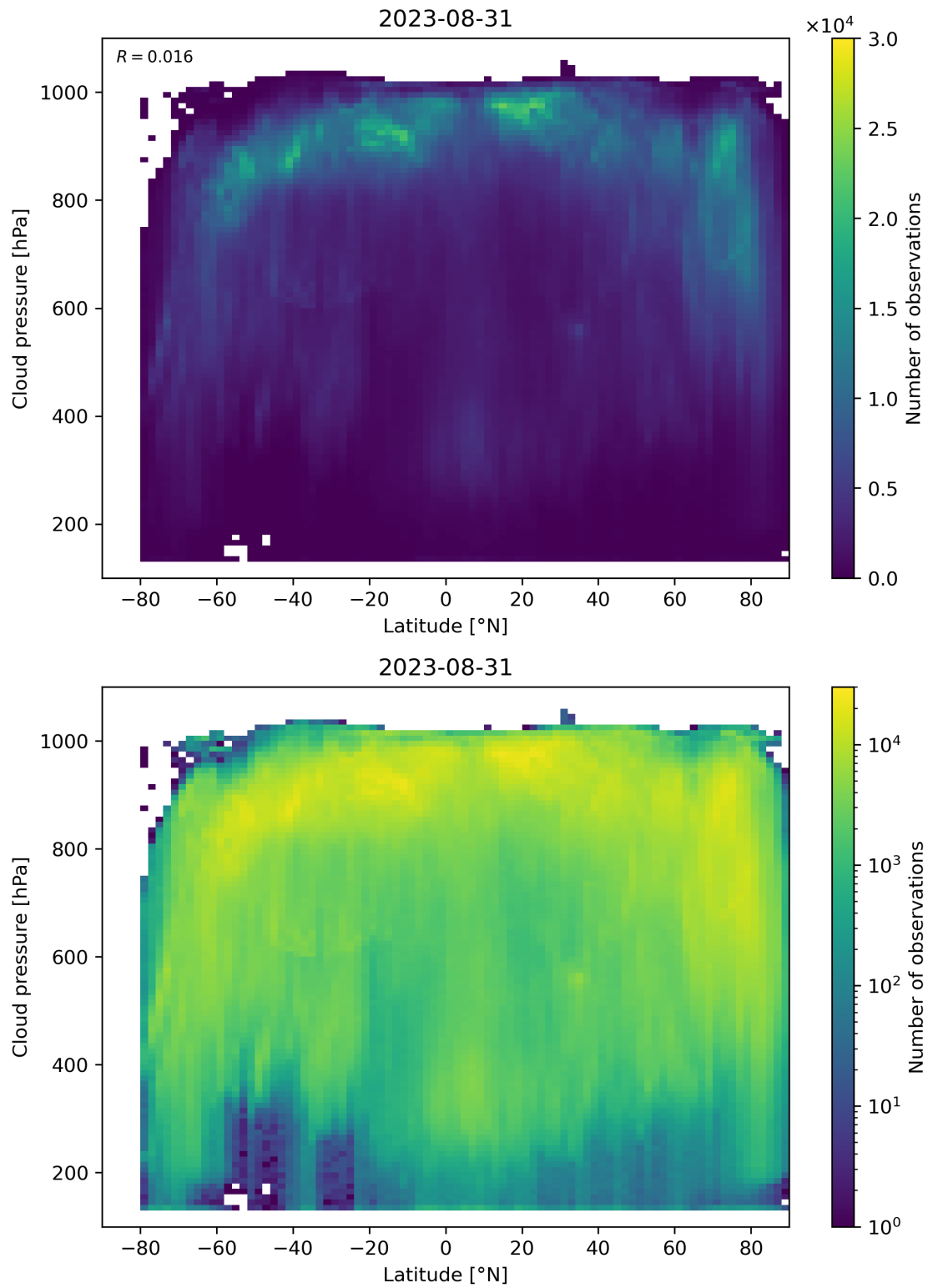
Figure 100: Scatter density plot of “Latitude” against “Cloud pressure” for 2023-08-30 to 2023-09-01.
