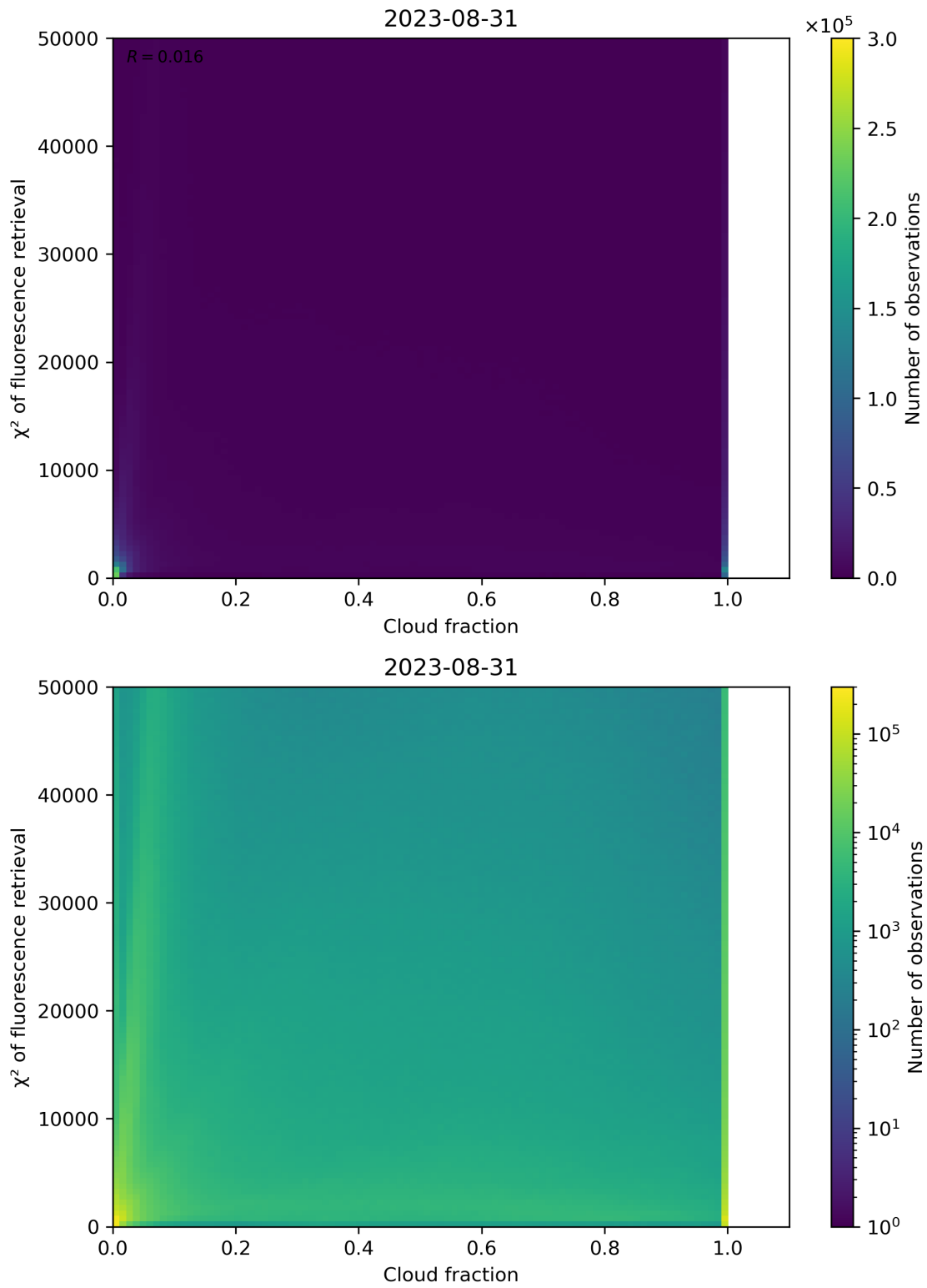
Figure 78: Scatter density plot of “Cloud fraction” against “ \chi^2 of fluorescence retrieval” for 2023-08-30 to 2023-09-01.
