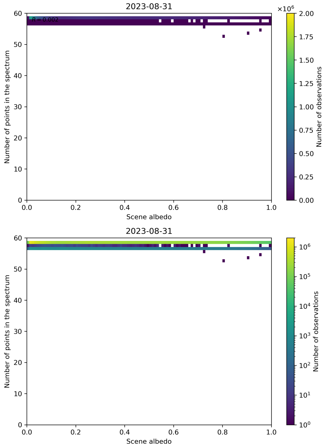
Figure 116: Scatter density plot of “Scene albedo” against “Number of points in the spectrum” for 2023-08-30 to 2023-09-01.
