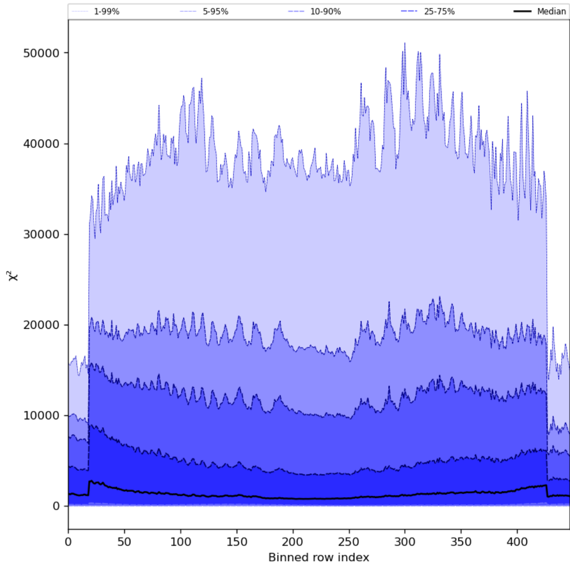
Figure 55: Along track statistics of “ \chi^2 ” for 2023-08-30 to 2023-09-01
