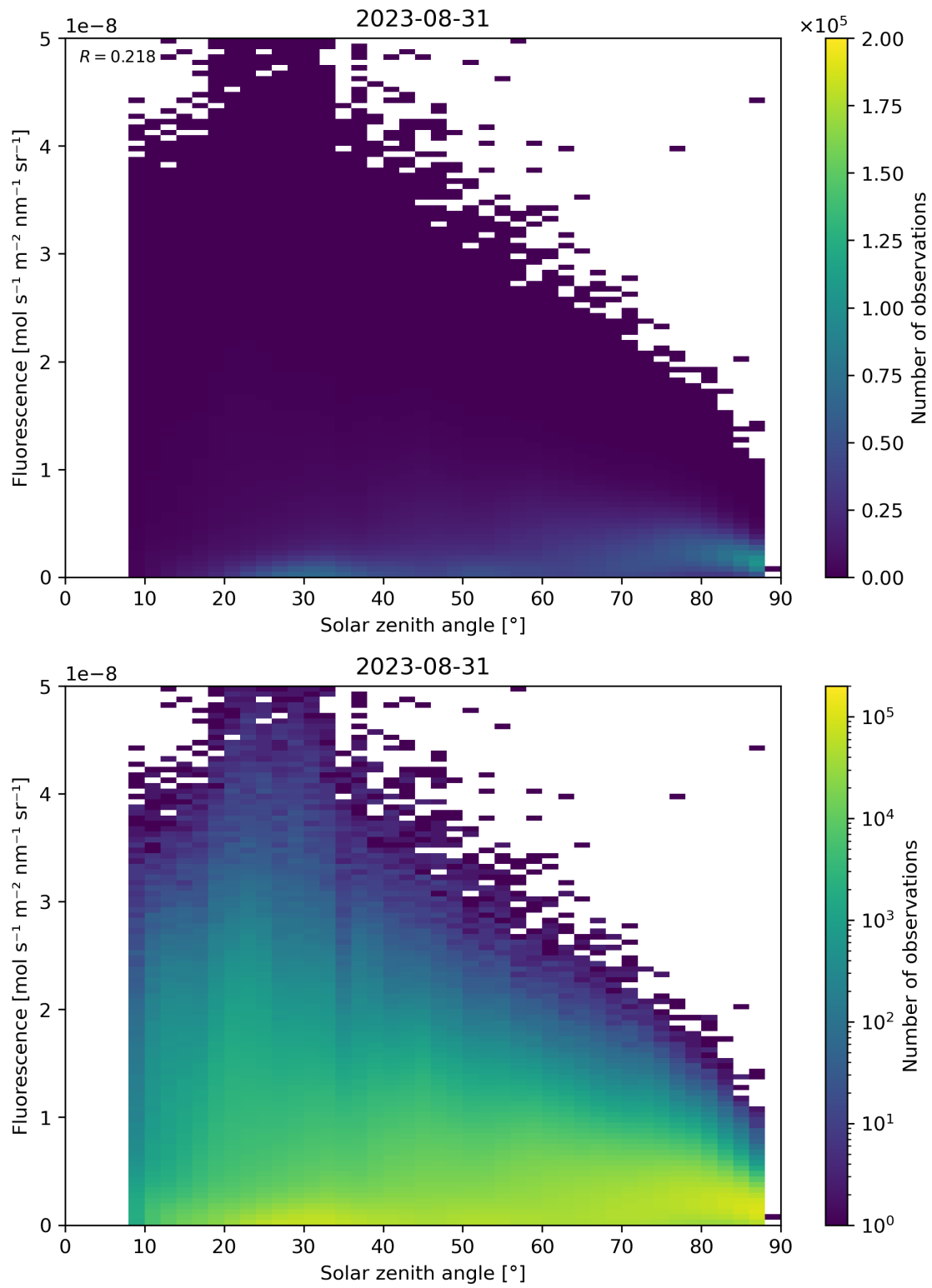
Figure 123: Scatter density plot of “Solar zenith angle” against “Fluorescence” for 2023-08-30 to 2023-09-01.
