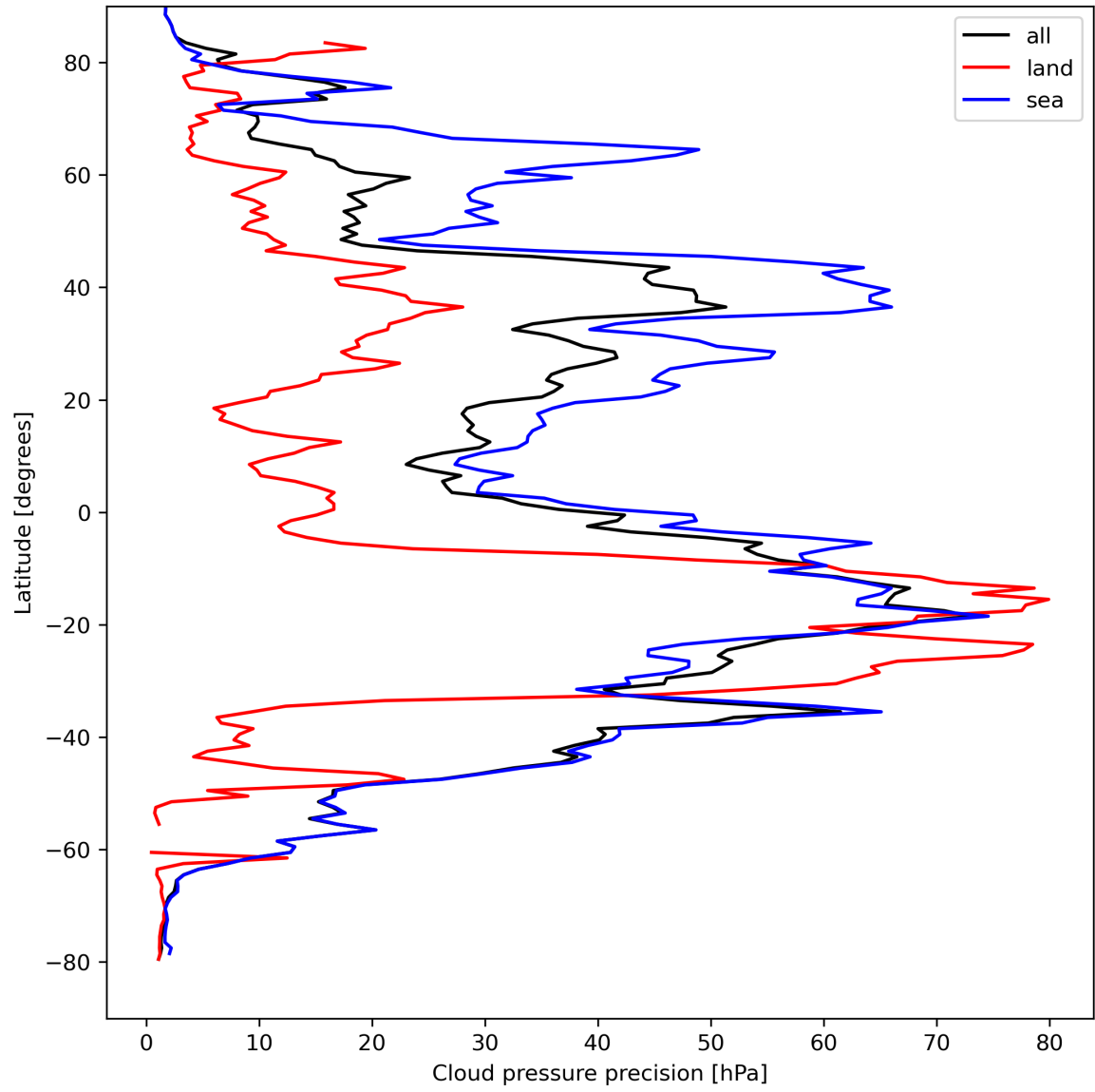
Figure 14: Zonal average of “Cloud pressure precision” for 2023-08-30 to 2023-09-01.
