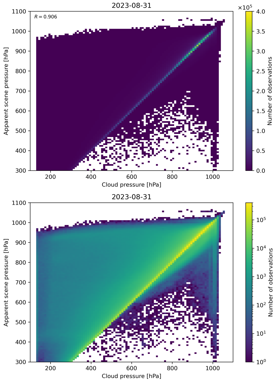
Figure 84: Scatter density plot of “Cloud pressure” against “Apparent scene pressure” for 2023-08-30 to 2023-09-01.
