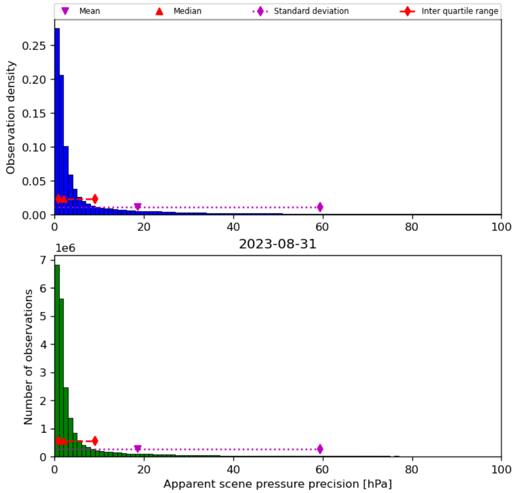
Figure 37: Histogram of “Apparent scene pressure precision” for 2023-08-30 to 2023-09-01
