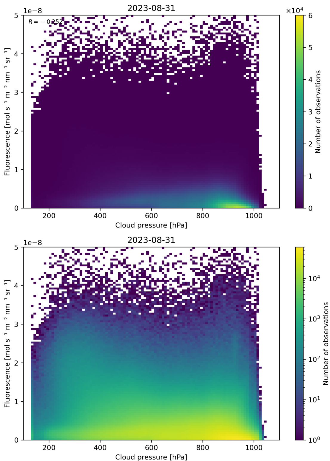
Figure 88: Scatter density plot of “Cloud pressure” against “Fluorescence” for 2023-08-30 to 2023-09-01.
