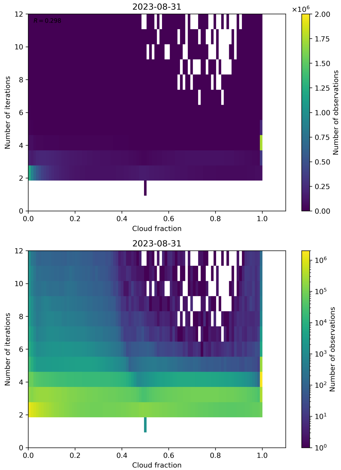
Figure 80: Scatter density plot of “Cloud fraction” against “Number of iterations” for 2023-08-30 to 2023-09-01.
