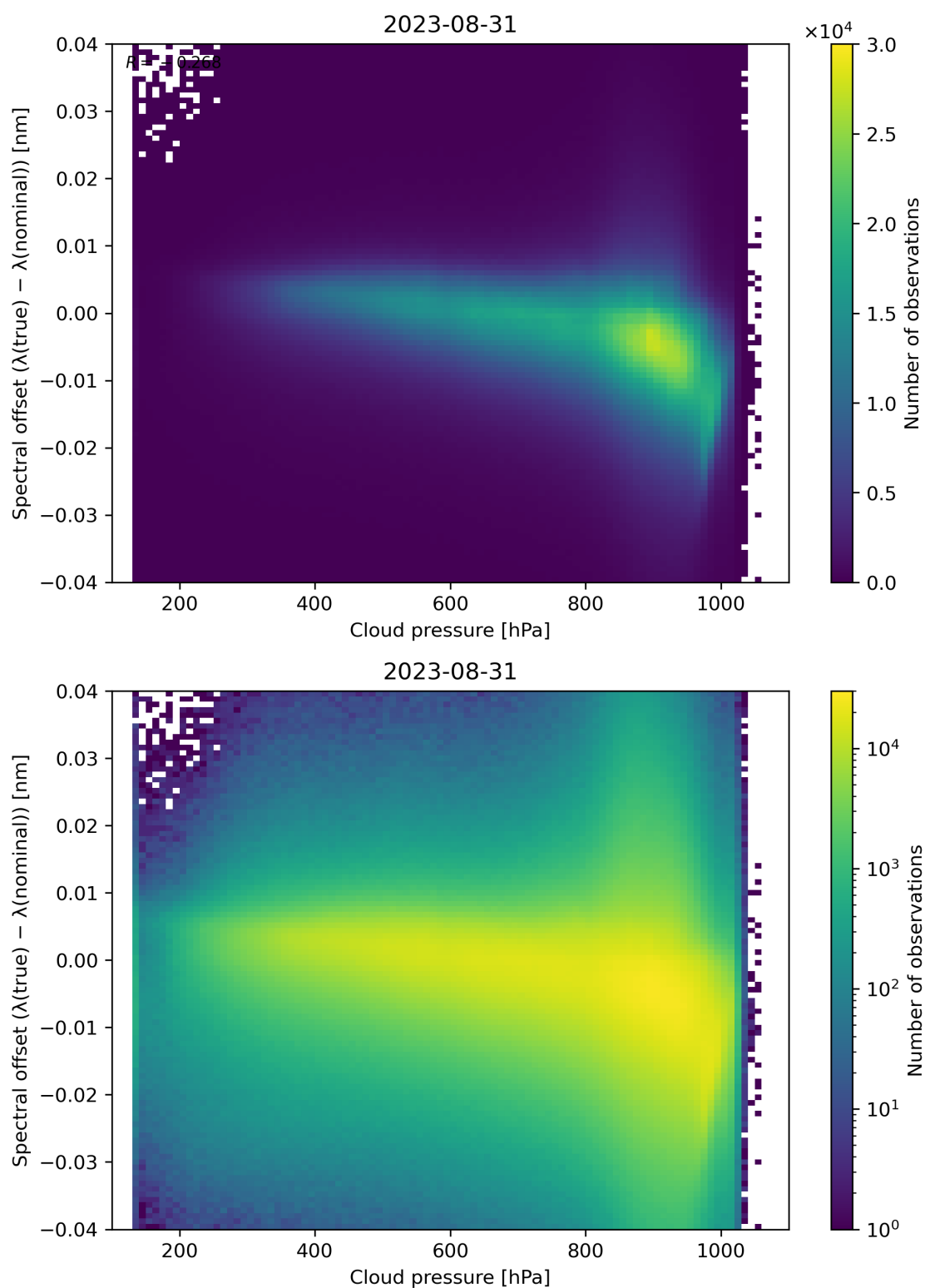
Figure 92: Scatter density plot of “Cloud pressure” against “Spectral offset ( \lambda(\text{true}) - \lambda(\text{nominal}) )” for 2023-08-30 to 2023-09-01.
