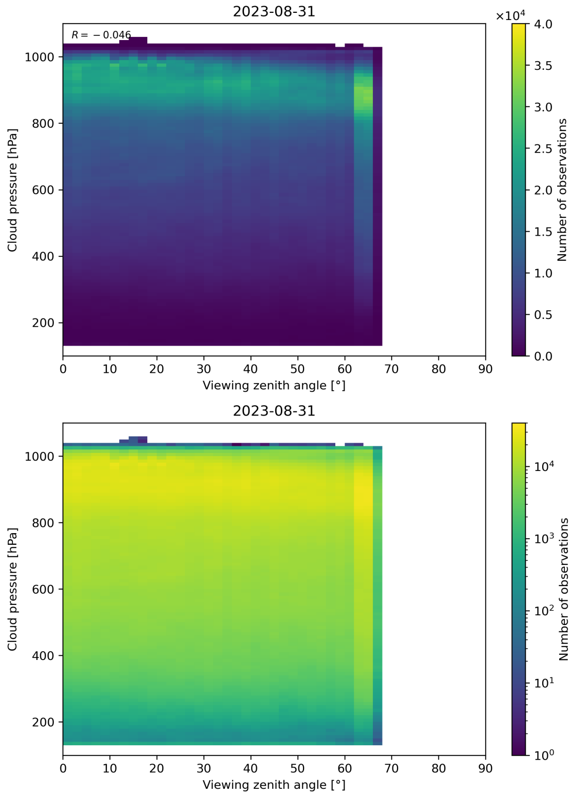
Figure 133: Scatter density plot of “Viewing zenith angle” against “Cloud pressure” for 2023-08-30 to 2023-09-01.
