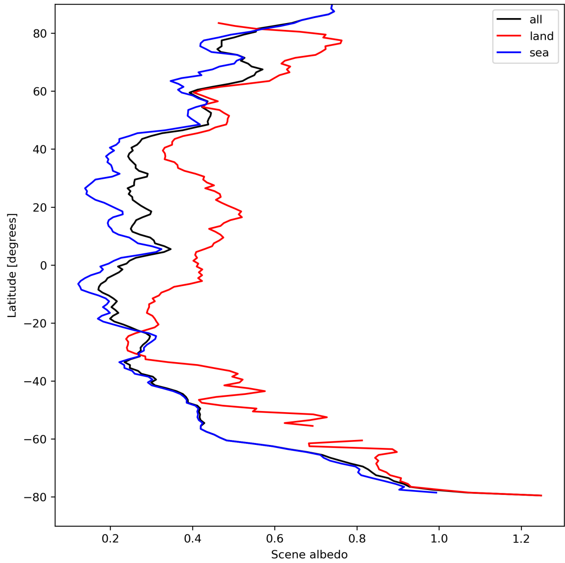
Figure 17: Zonal average of “Scene albedo” for 2023-08-30 to 2023-09-01.
