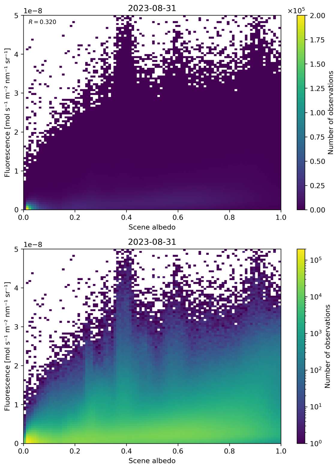
Figure 114: Scatter density plot of "Scene albedo" against "Fluorescence" for 2023-08-30 to 2023-09-01.
