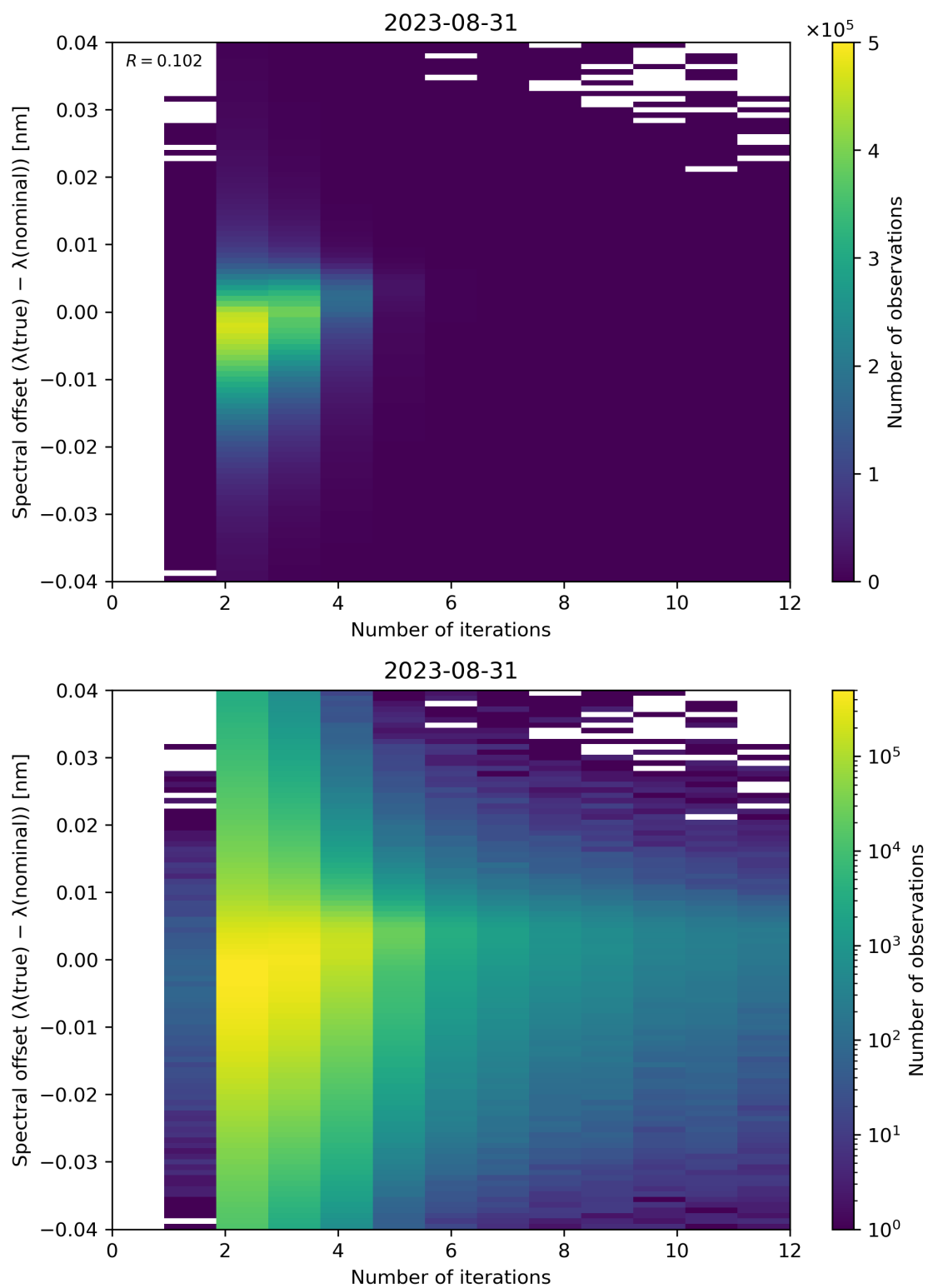
Figure 109: Scatter density plot of “Number of iterations” against “Spectral offset ( \lambda(\text{true}) - \lambda(\text{nominal}) )” for 2023-08-30 to 2023-09-01.
