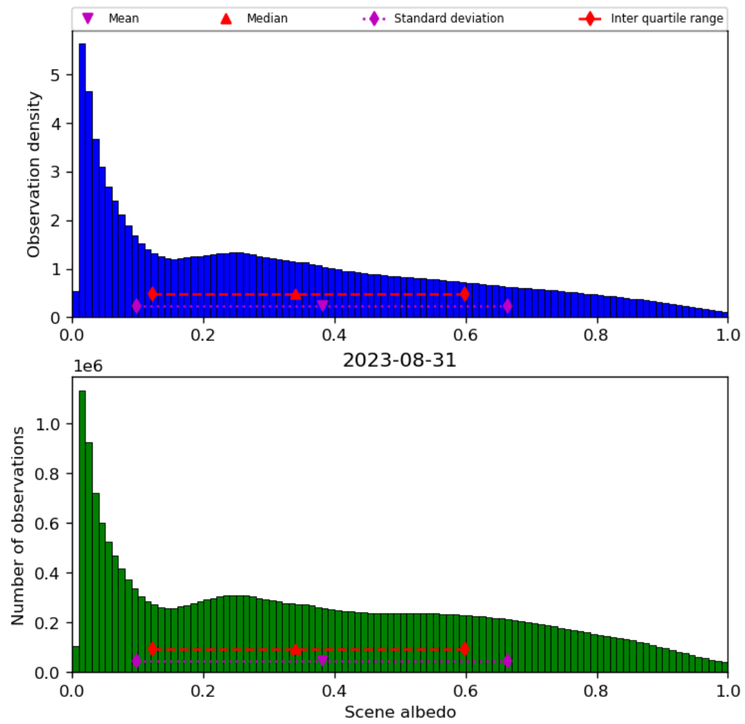
Figure 34: Histogram of “Scene albedo” for 2023-08-30 to 2023-09-01
