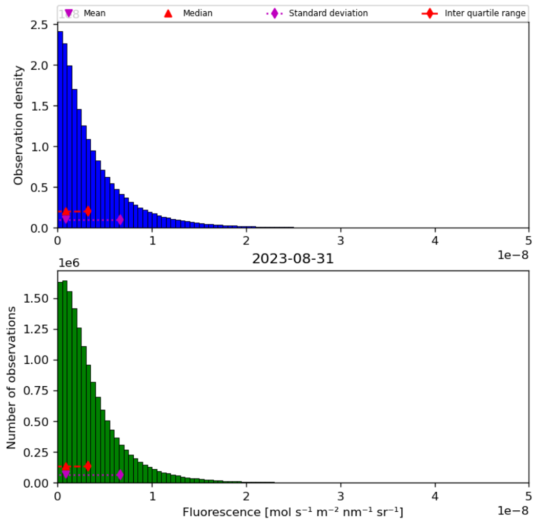
Figure 40: Histogram of “Fluorescence” for 2023-08-30 to 2023-09-01
