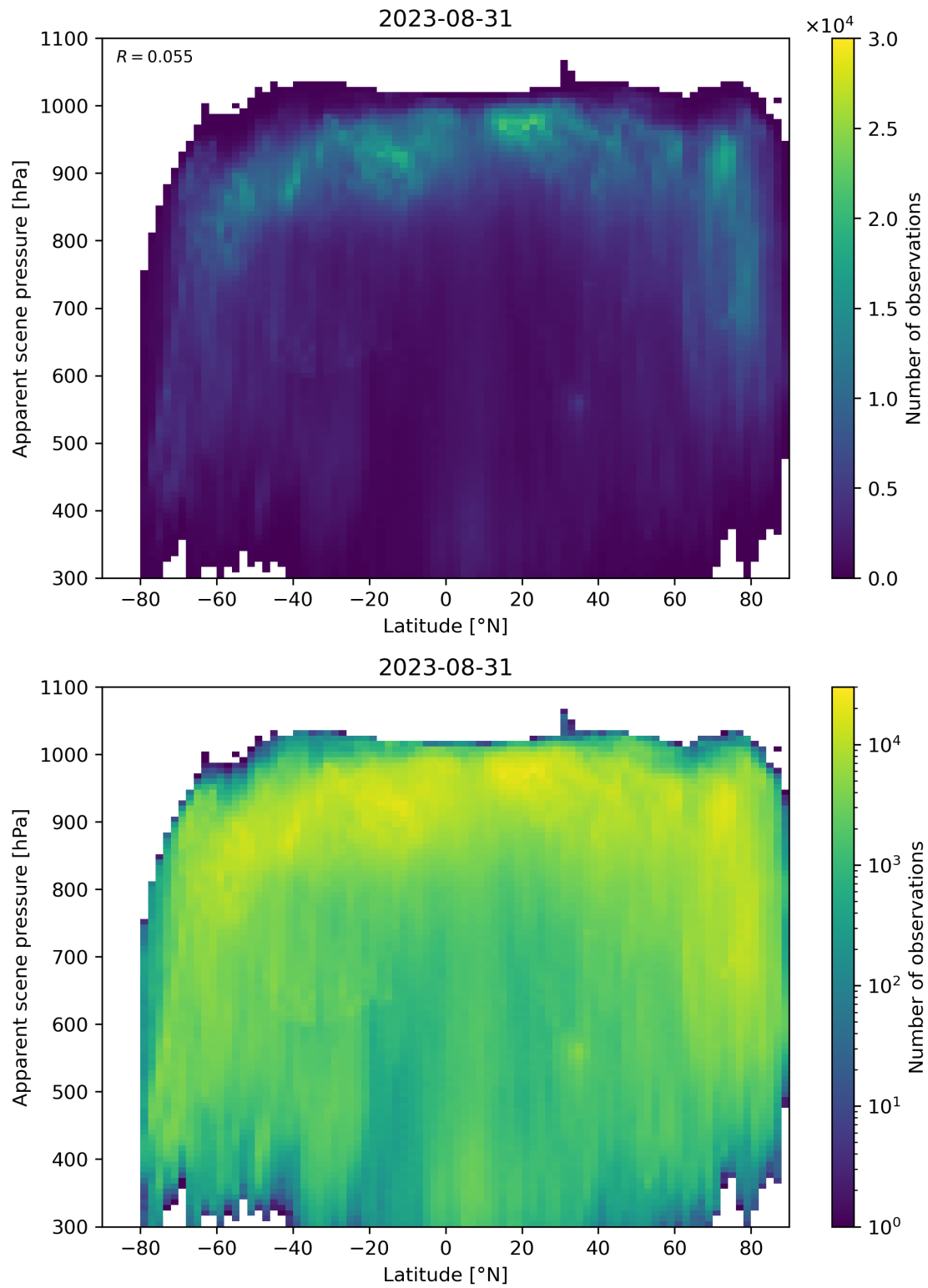
Figure 96: Scatter density plot of “Latitude” against “Apparent scene pressure” for 2023-08-30 to 2023-09-01.
