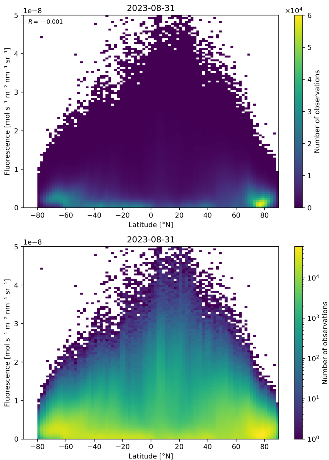
Figure 101: Scatter density plot of “Latitude” against “Fluorescence” for 2023-08-30 to 2023-09-01.
