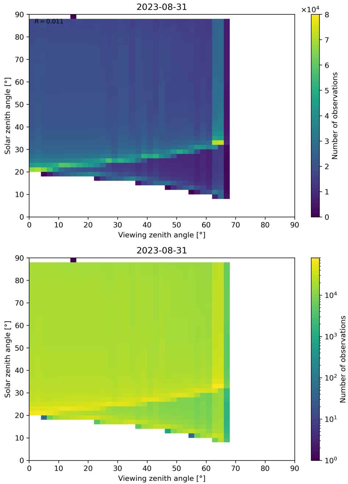
Figure 139: Scatter density plot of “Viewing zenith angle” against “Solar zenith angle” for 2023-08-30 to 2023-09-01.
