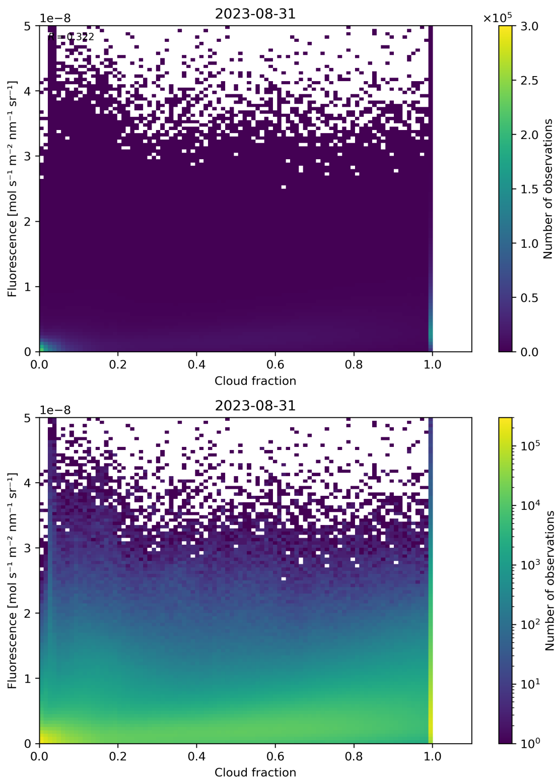
Figure 79: Scatter density plot of “Cloud fraction” against “Fluorescence” for 2023-08-30 to 2023-09-01.
