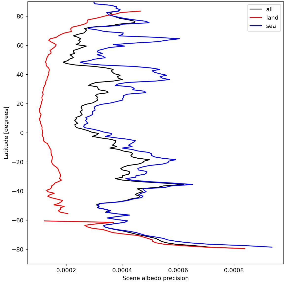
Figure 18: Zonal average of “Scene albedo precision” for 2023-08-30 to 2023-09-01.
