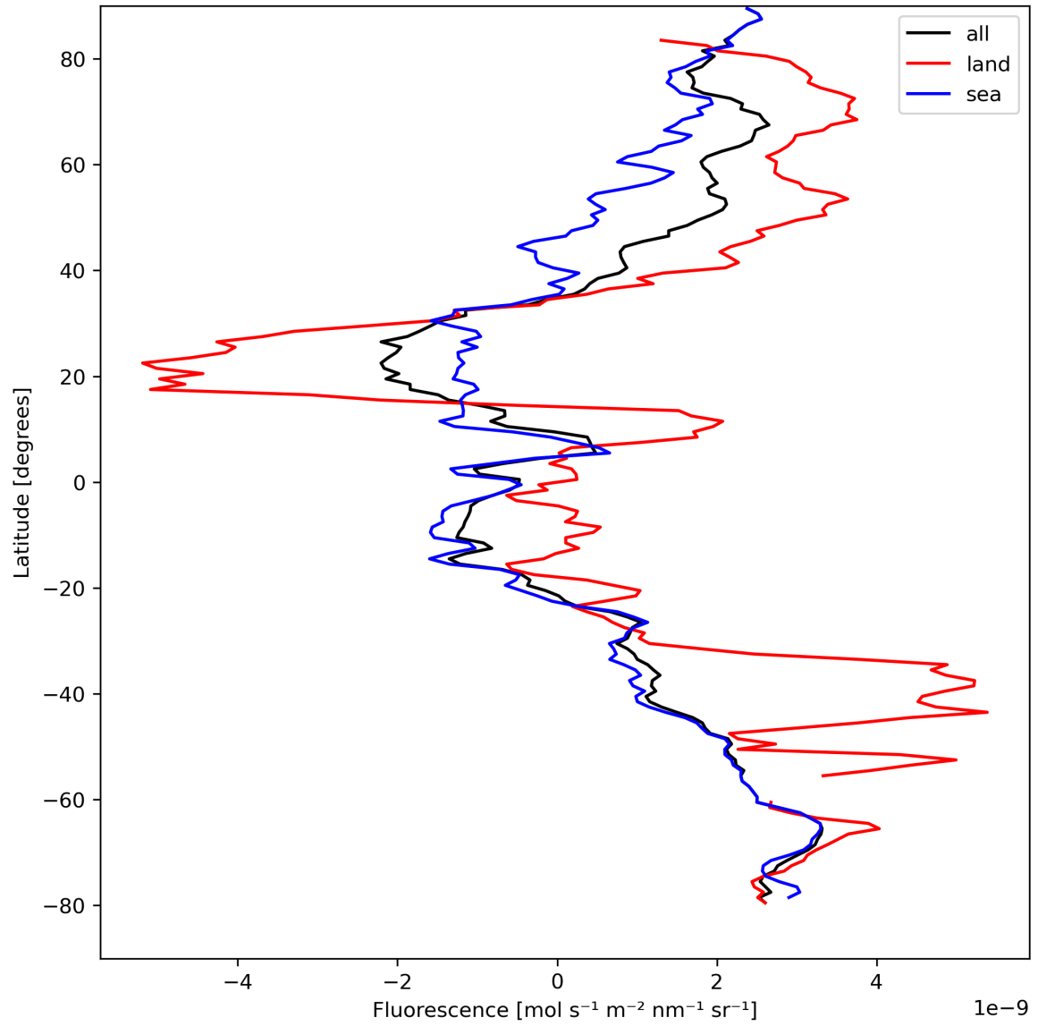
Figure 23: Zonal average of “Fluorescence” for 2023-08-30 to 2023-09-01.
