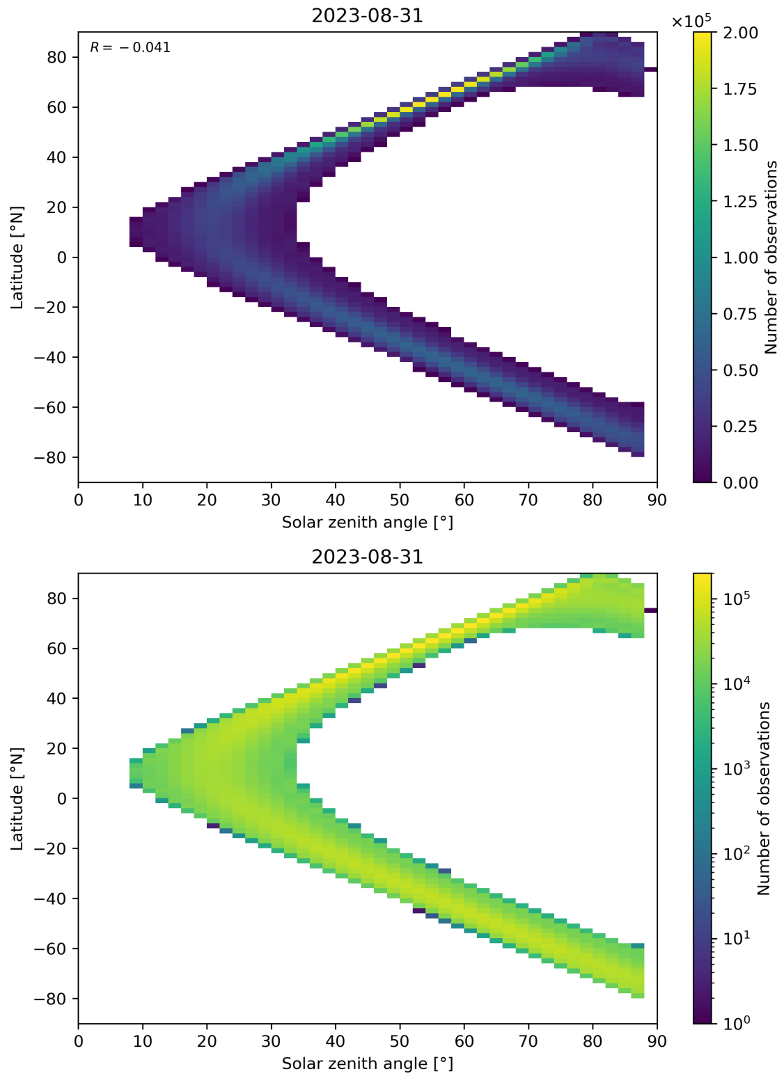
Figure 124: Scatter density plot of “Solar zenith angle” against “Latitude” for 2023-08-30 to 2023-09-01.
