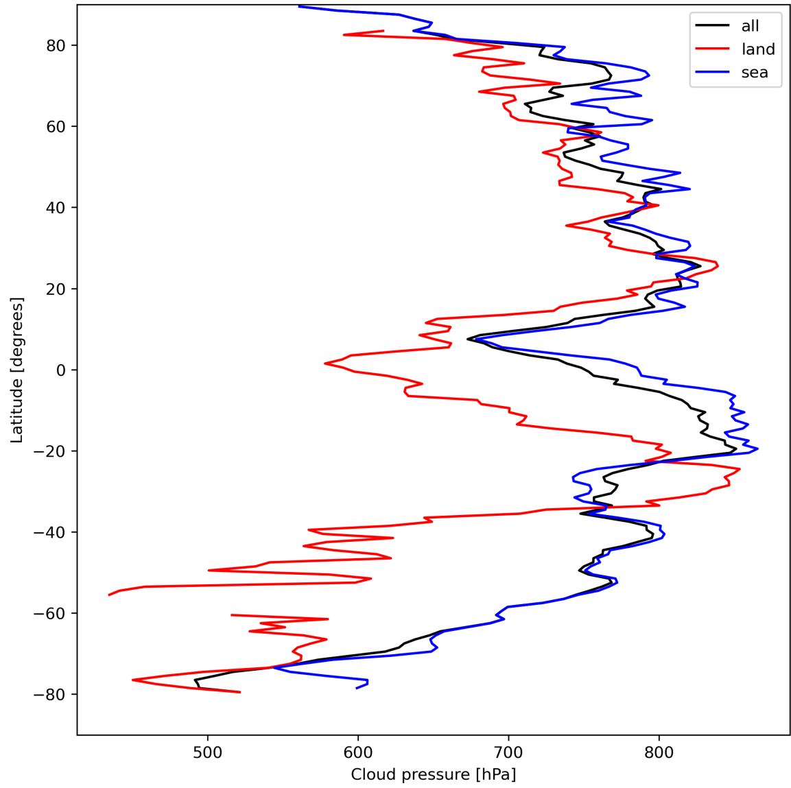
Figure 13: Zonal average of “Cloud pressure” for 2023-08-30 to 2023-09-01.
