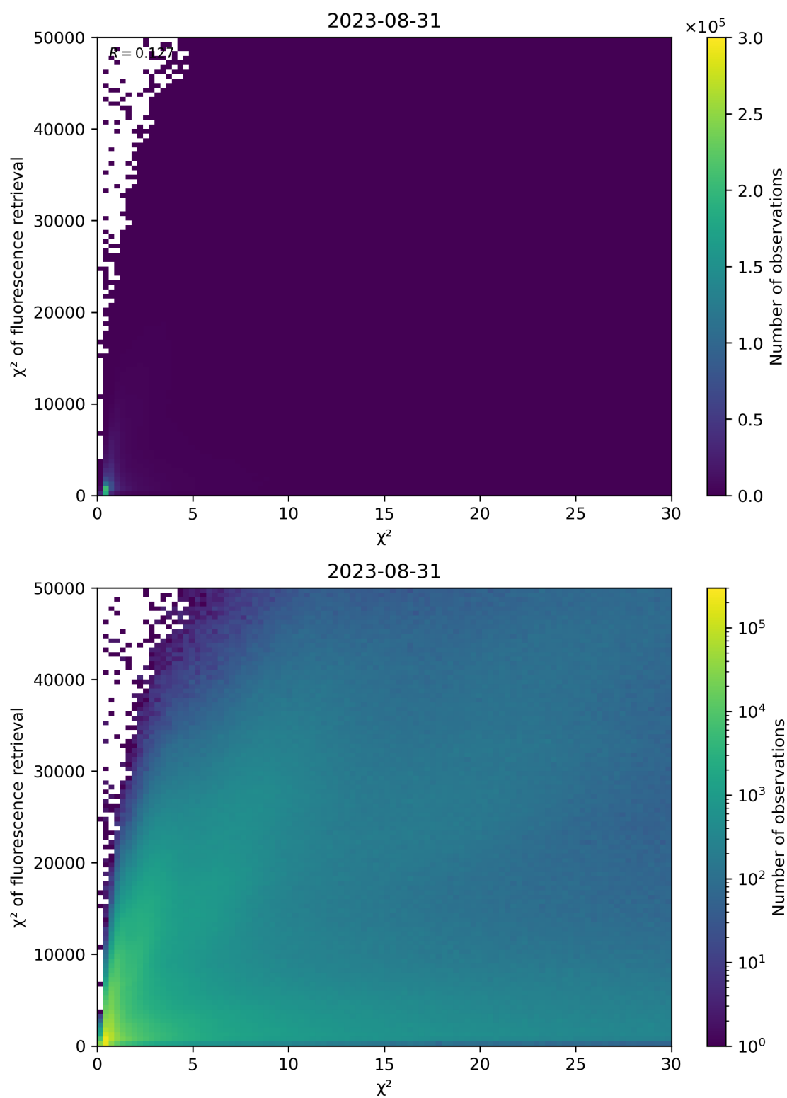
Figure 69: Scatter density plot of “ \chi^2 ” against “ \chi^2 of fluorescence retrieval” for 2023-08-30 to 2023-09-01.
