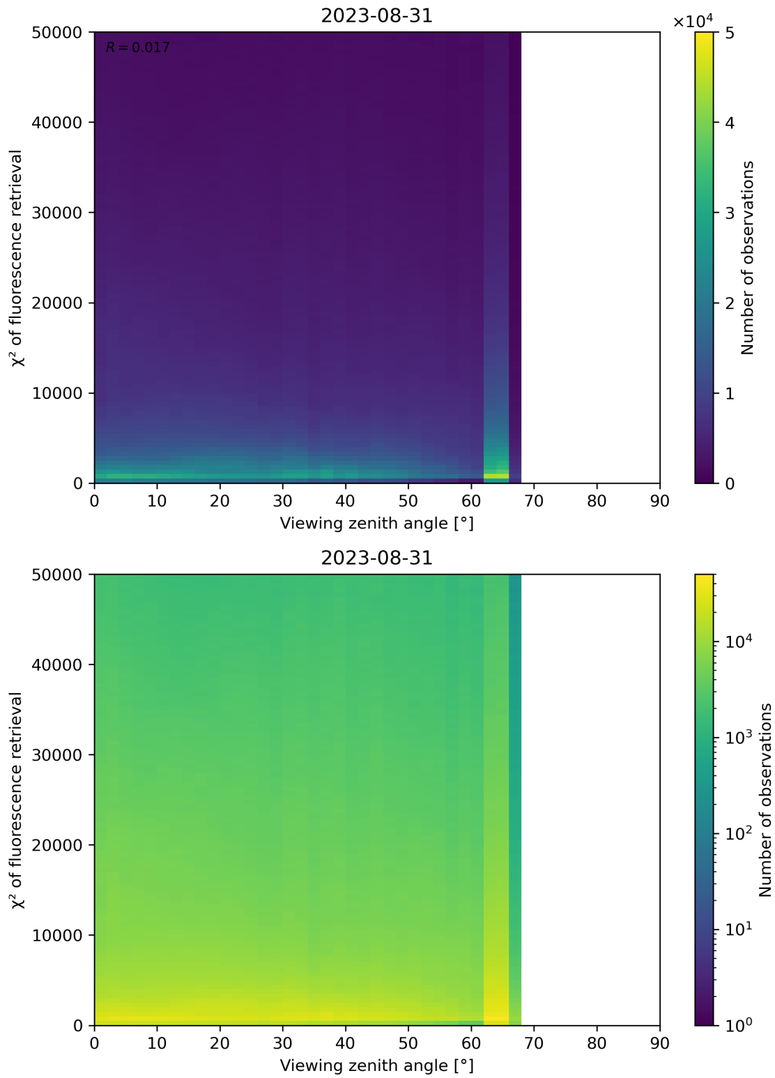
Figure 131: Scatter density plot of “Viewing zenith angle” against “ \chi^2 of fluorescence retrieval” for 2023-08-30 to 2023-09-01.
