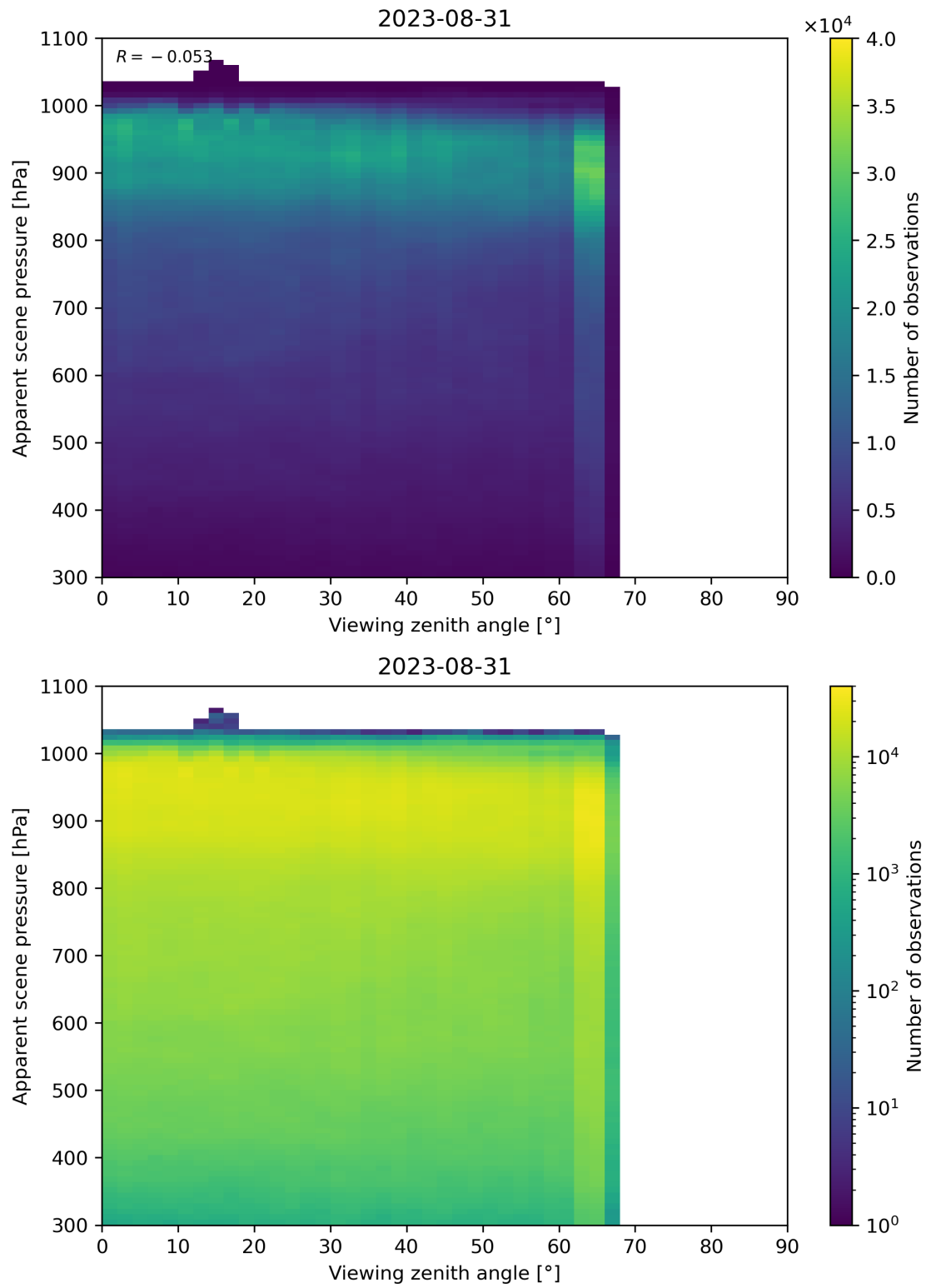
Figure 129: Scatter density plot of “Viewing zenith angle” against “Apparent scene pressure” for 2023-08-30 to 2023-09-01.
