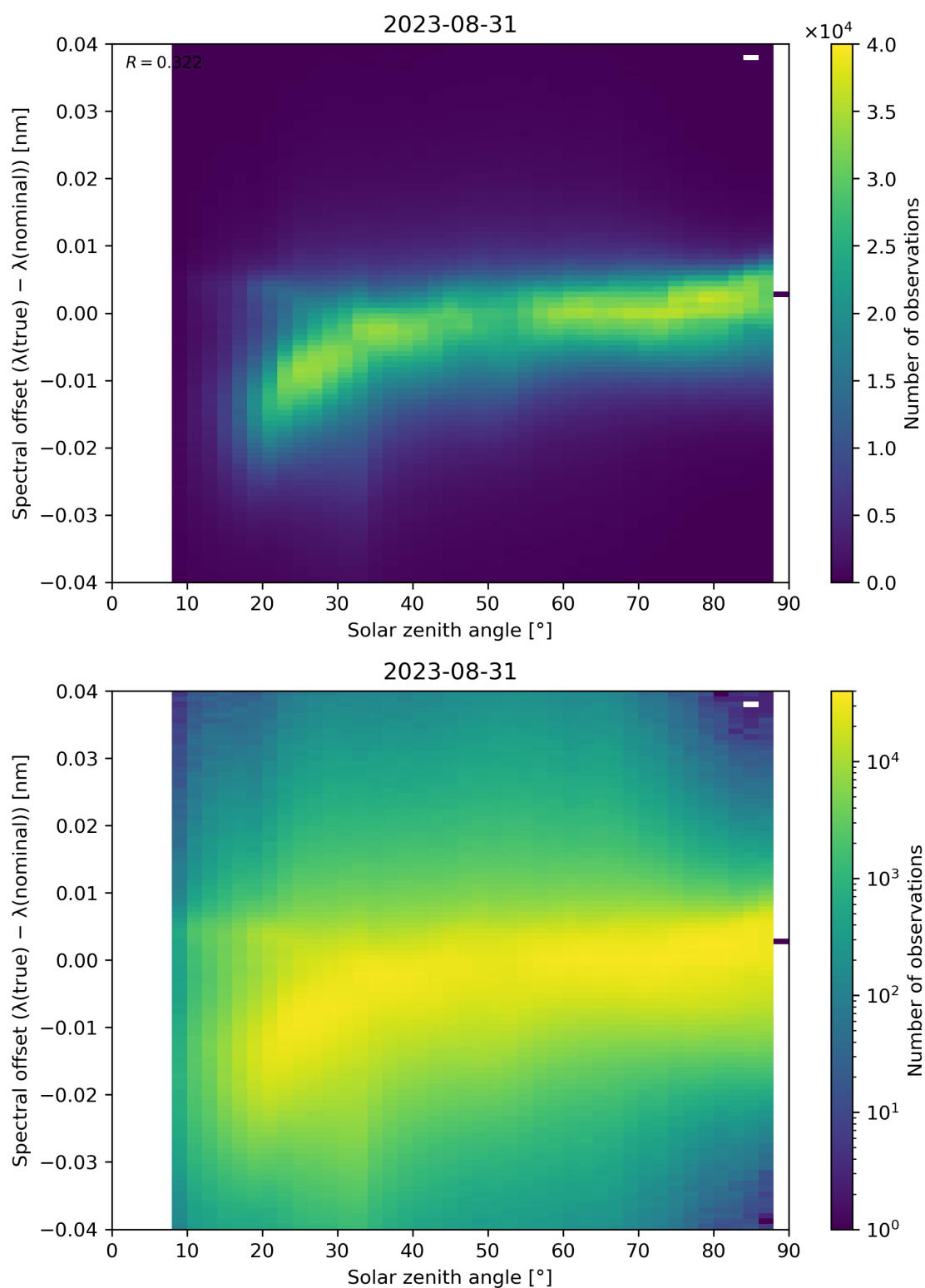
Figure 128: Scatter density plot of “Solar zenith angle” against “Spectral offset ( \lambda(\text{true}) - \lambda(\text{nominal}) )” for 2023-08-30 to 2023-09-01.
