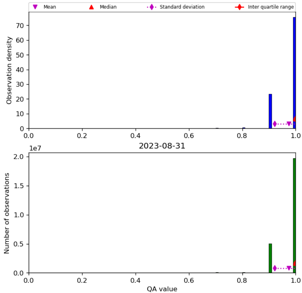
Figure 29: Histogram of “QA value” for 2023-08-30 to 2023-09-01
