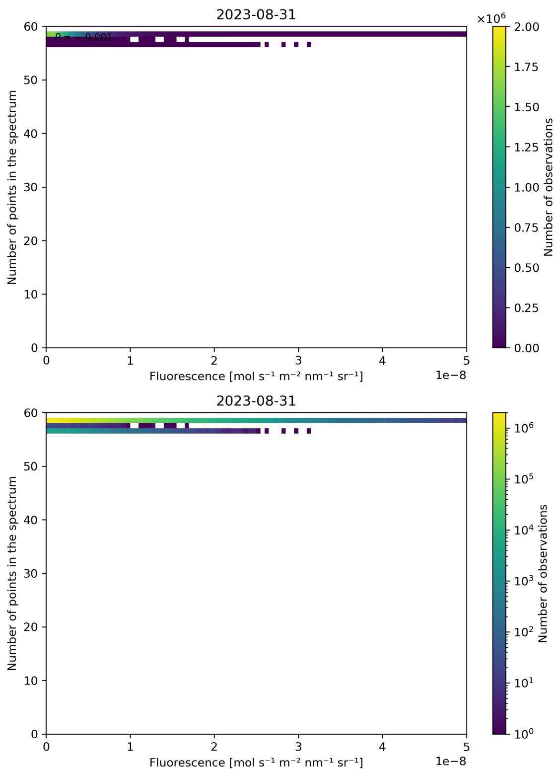
Figure 94: Scatter density plot of “Fluorescence” against “Number of points in the spectrum” for 2023-08-30 to 2023-09-01.
