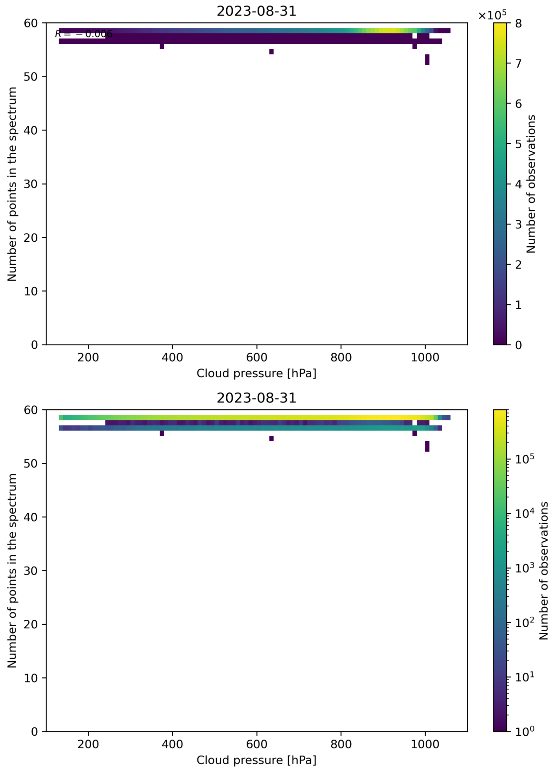
Figure 90: Scatter density plot of “Cloud pressure” against “Number of points in the spectrum” for 2023-08-30 to 2023-09-01.
