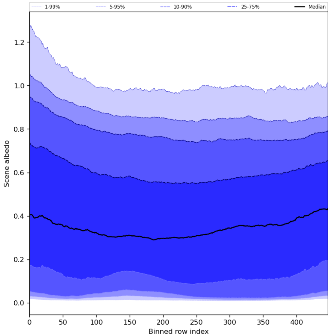
Figure 51: Along track statistics of "Scene albedo" for 2023-08-30 to 2023-09-01
