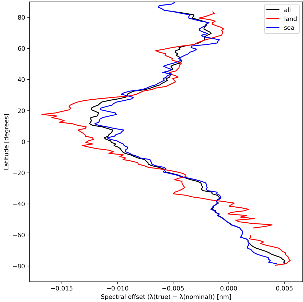
Figure 28: Zonal average of “Spectral offset ( \lambda(\text{true}) - \lambda(\text{nominal}) )” for 2023-08-30 to 2023-09-01.
