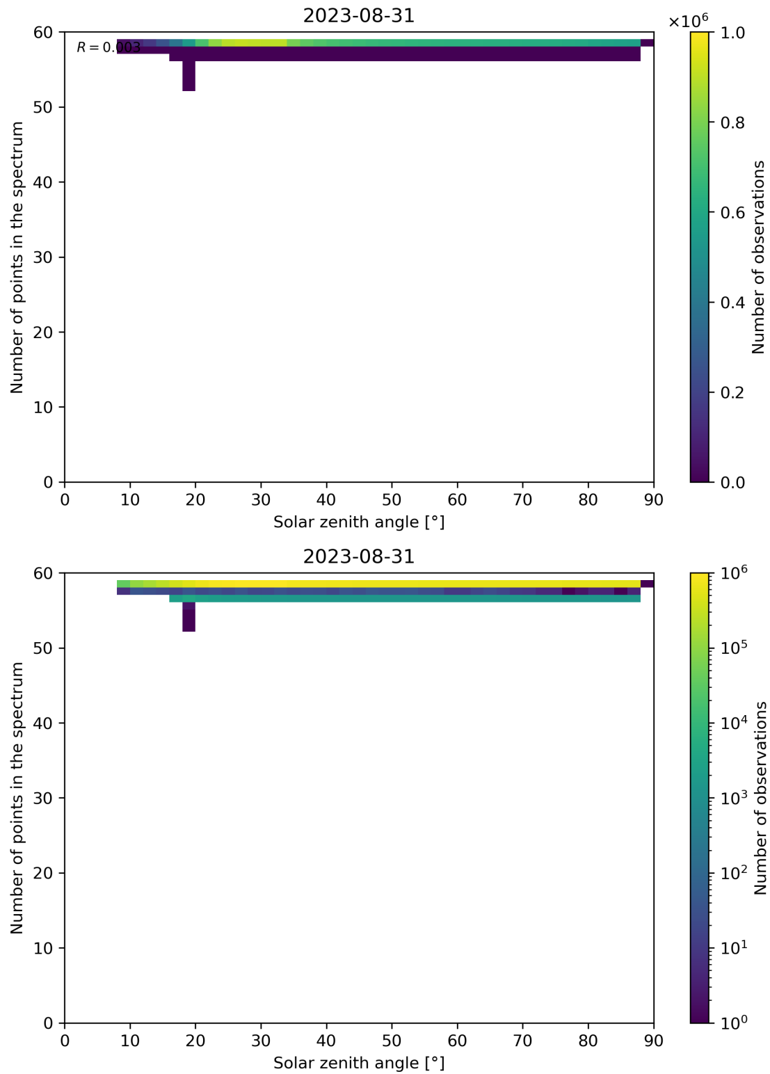
Figure 126: Scatter density plot of “Solar zenith angle” against “Number of points in the spectrum” for 2023-08-30 to 2023-09-01.
