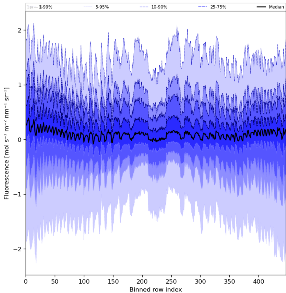
Figure 57: Along track statistics of “Fluorescence” for 2023-08-30 to 2023-09-01
