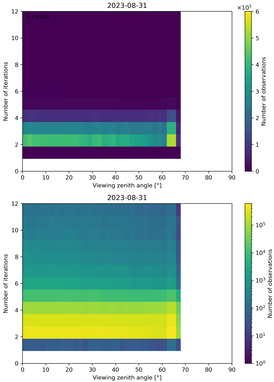
Figure 136: Scatter density plot of “Viewing zenith angle” against “Number of iterations” for 2023-08-30 to 2023-09-01.
