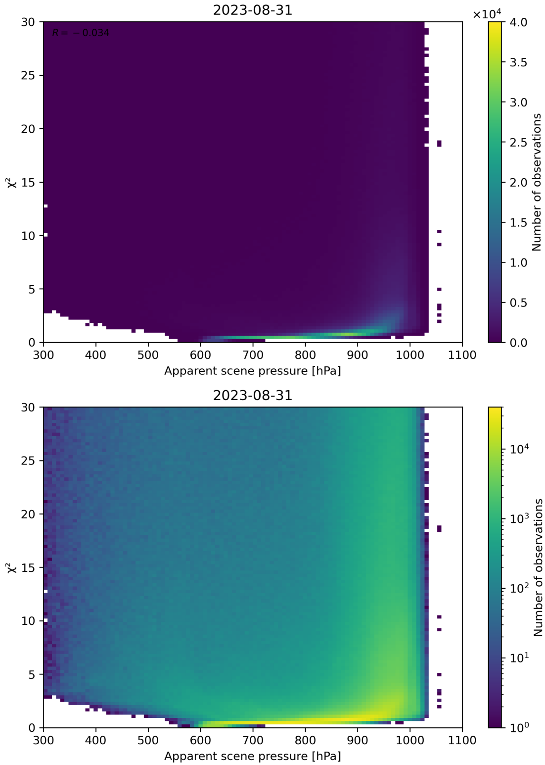
Figure 63: Scatter density plot of “Apparent scene pressure” against “ \chi^2 ” for 2023-08-30 to 2023-09-01.
