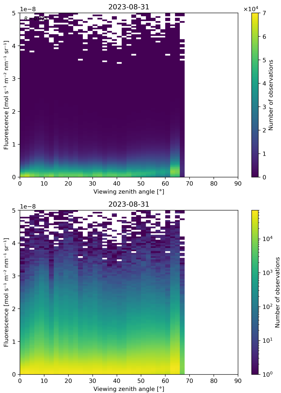
Figure 134: Scatter density plot of “Viewing zenith angle” against “Fluorescence” for 2023-08-30 to 2023-09-01.
