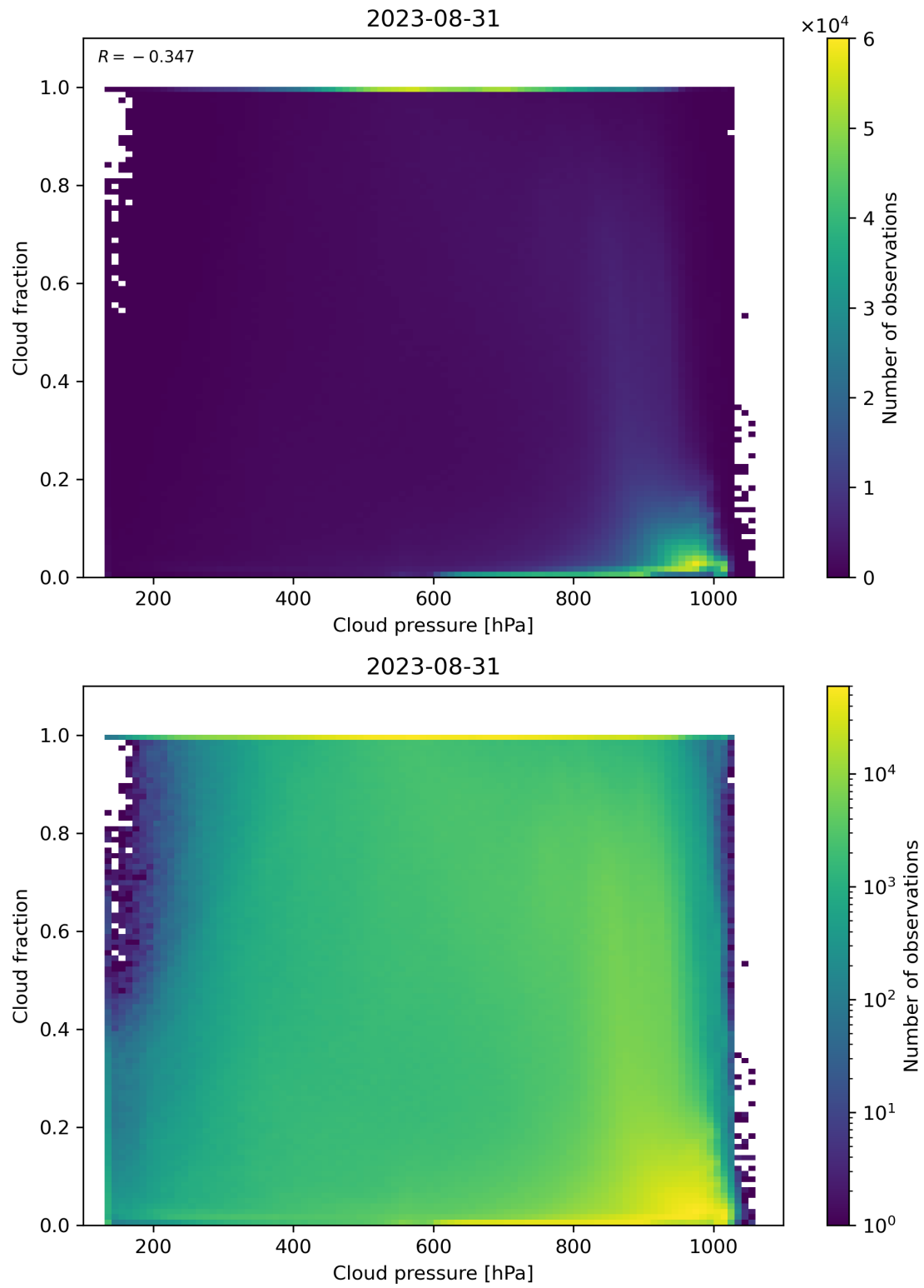
Figure 87: Scatter density plot of “Cloud pressure” against “Cloud fraction” for 2023-08-30 to 2023-09-01.
