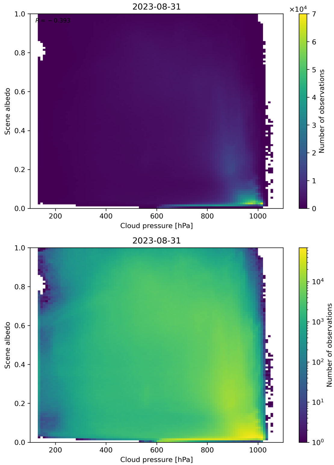
Figure 91: Scatter density plot of “Cloud pressure” against “Scene albedo” for 2023-08-30 to 2023-09-01.
