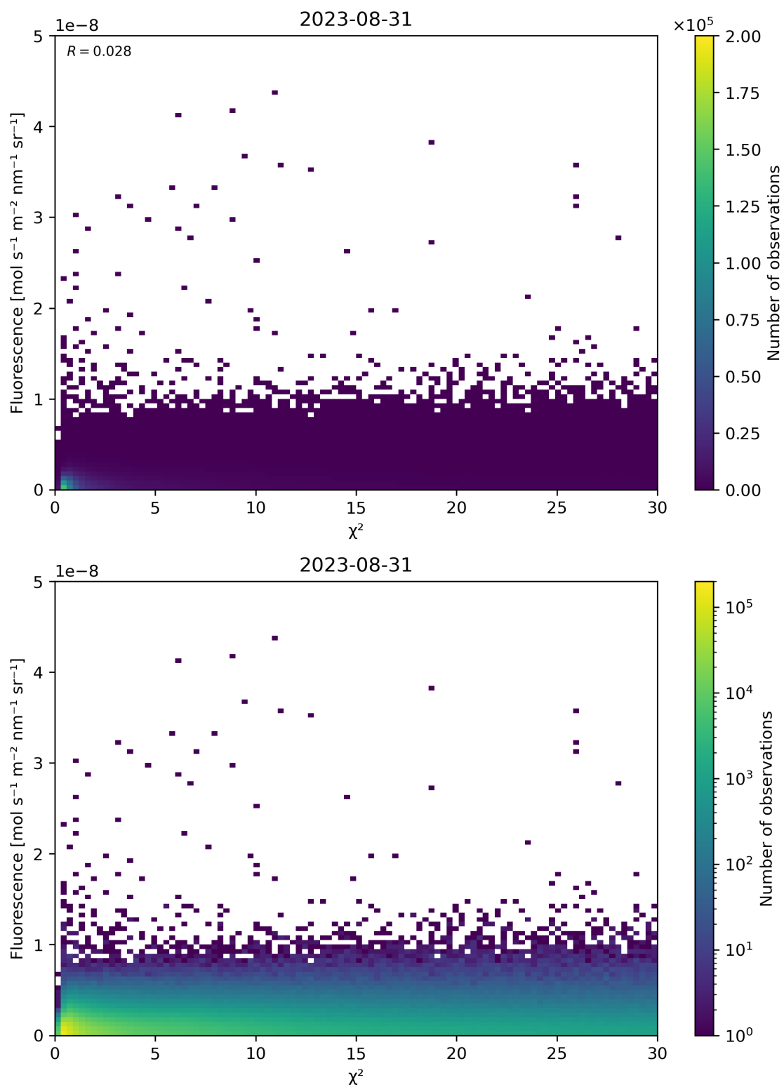
Figure 70: Scatter density plot of “ \chi^2 ” against “Fluorescence” for 2023-08-30 to 2023-09-01.
