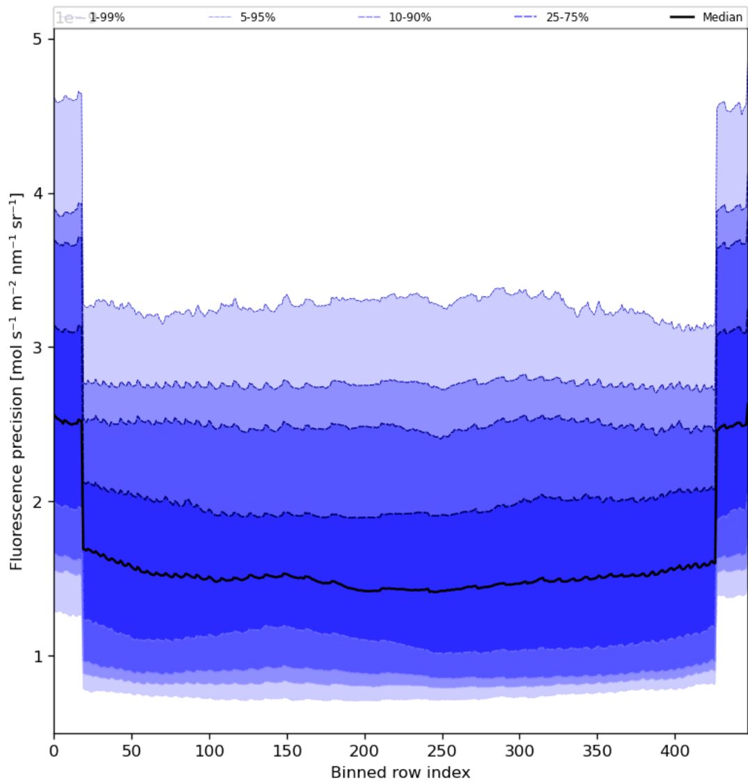
Figure 58: Along track statistics of "Fluorescence precision" for 2023-08-30 to 2023-09-01
