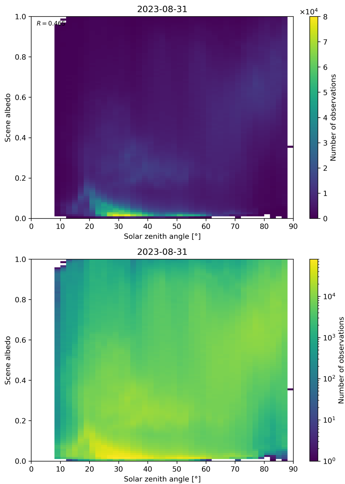
Figure 127: Scatter density plot of “Solar zenith angle” against “Scene albedo” for 2023-08-30 to 2023-09-01.
