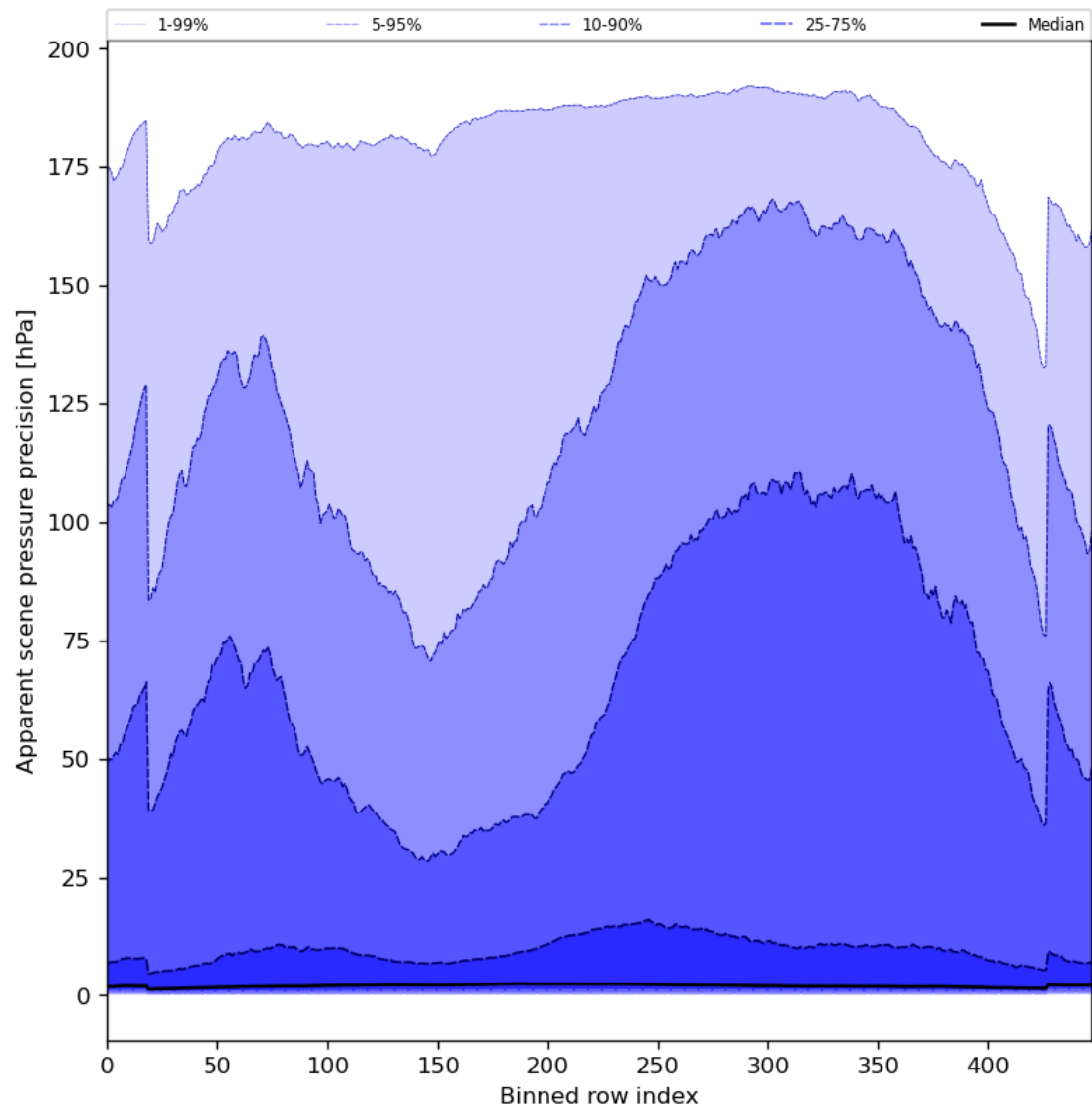
Figure 54: Along track statistics of “Apparent scene pressure precision” for 2023-08-30 to 2023-09-01
