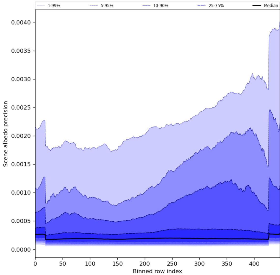
Figure 52: Along track statistics of “Scene albedo precision” for 2023-08-30 to 2023-09-01
