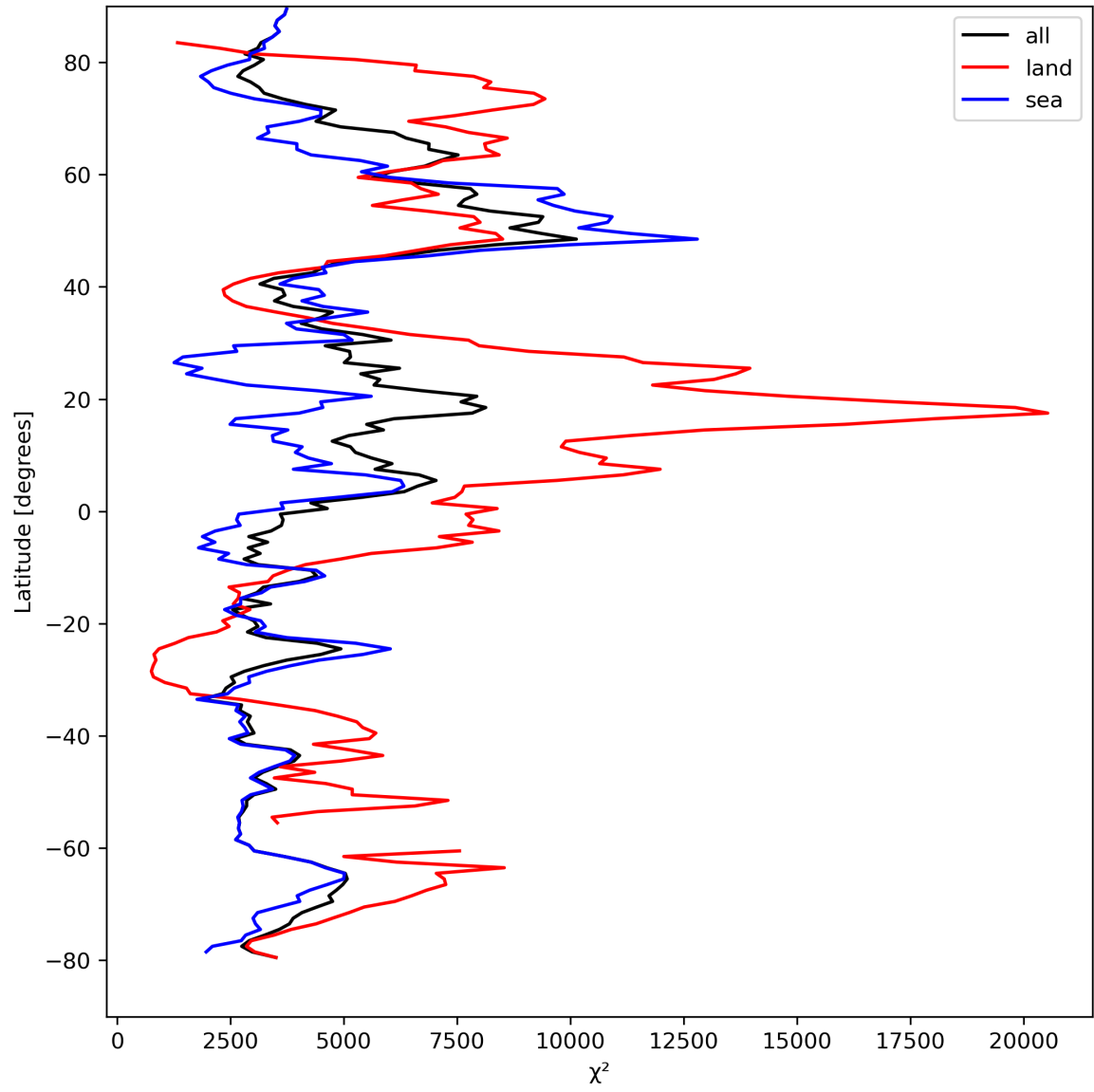
Figure 21: Zonal average of “ \chi^2 ” for 2023-08-30 to 2023-09-01.
