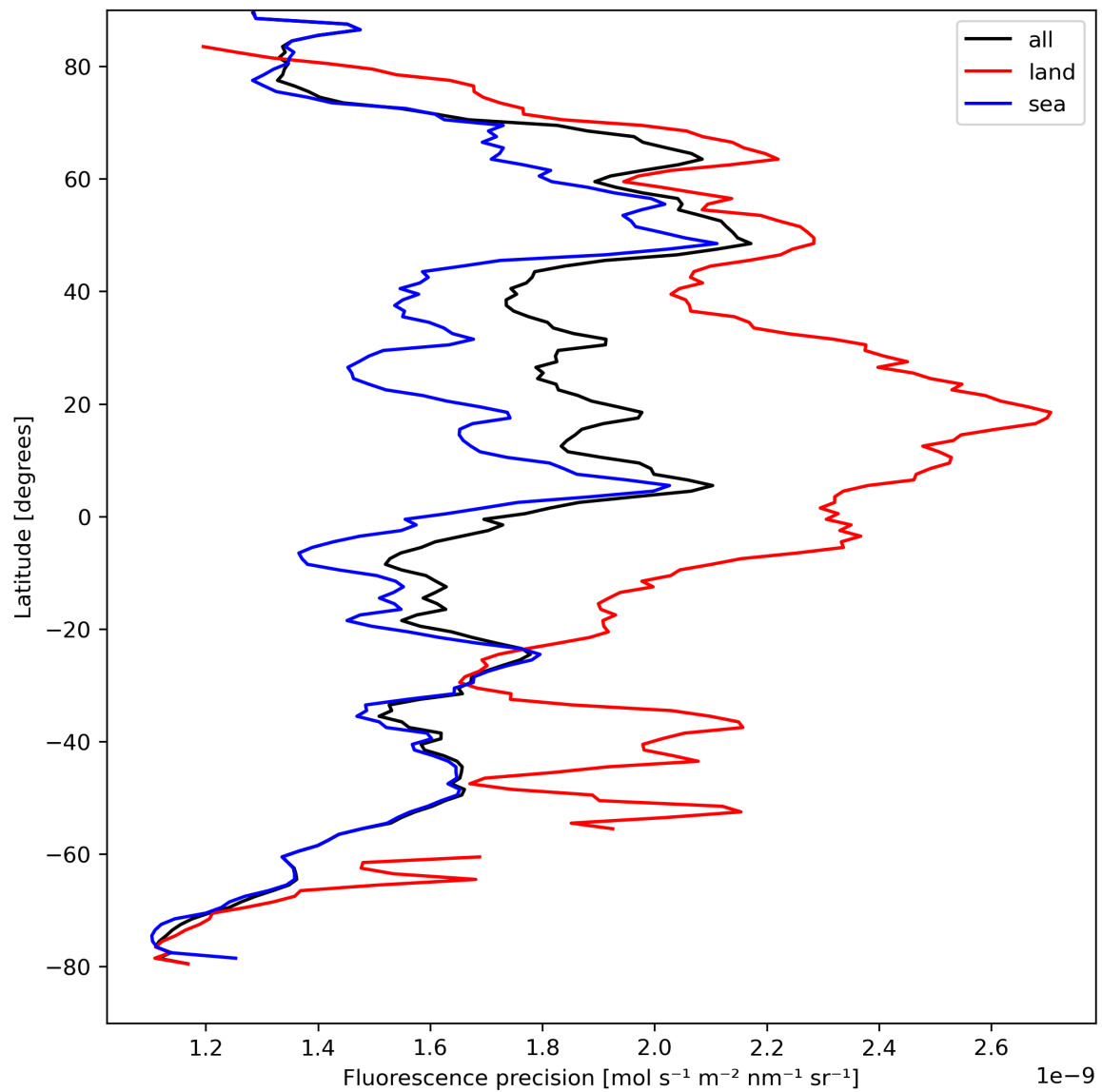
Figure 24: Zonal average of “Fluorescence precision” for 2023-08-30 to 2023-09-01.
