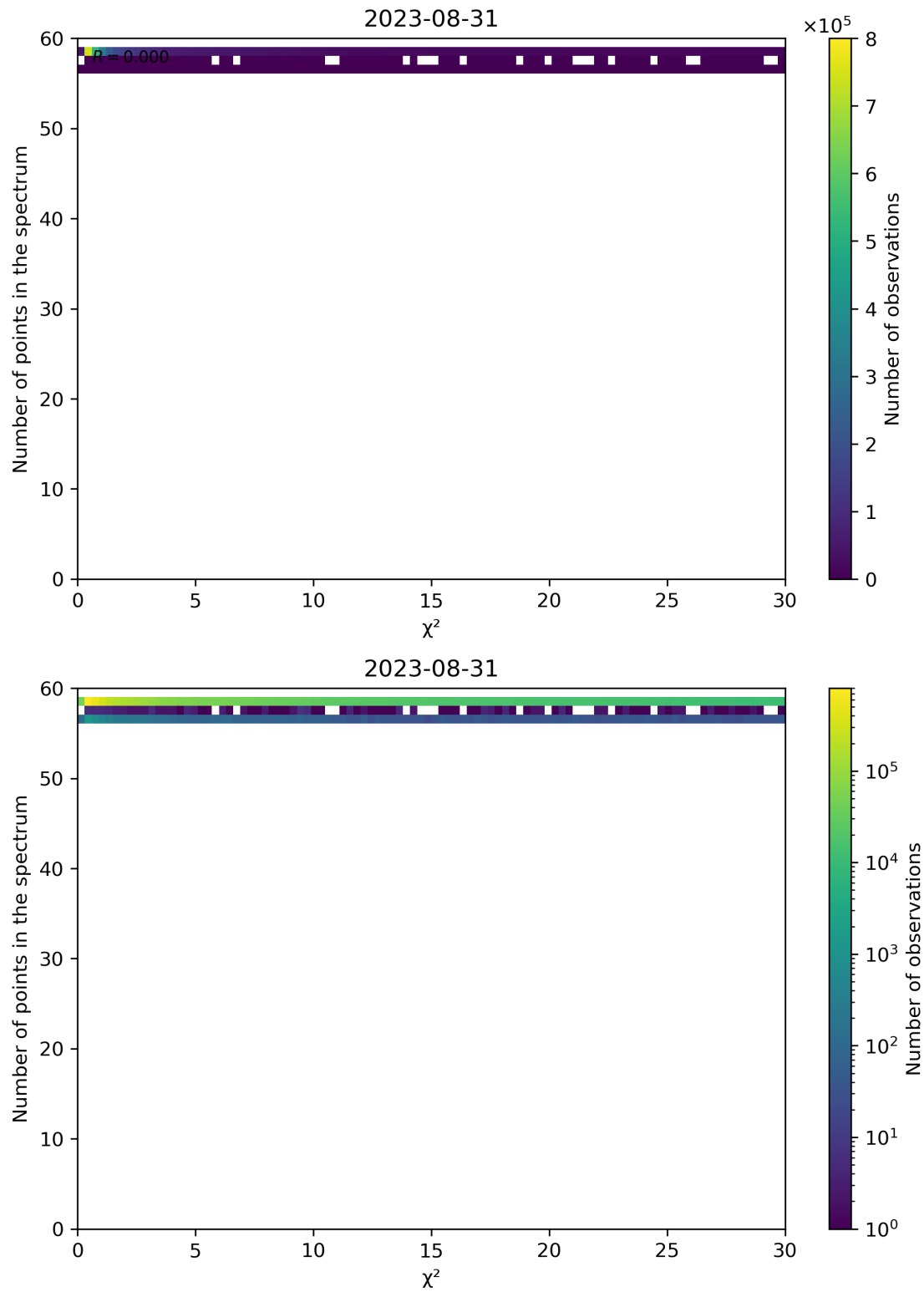
Figure 74: Scatter density plot of “ \chi^2 ” against “Number of points in the spectrum” for 2023-08-30 to 2023-09-01.
