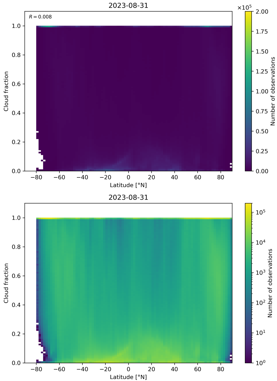
Figure 99: Scatter density plot of “Latitude” against “Cloud fraction” for 2023-08-30 to 2023-09-01.
