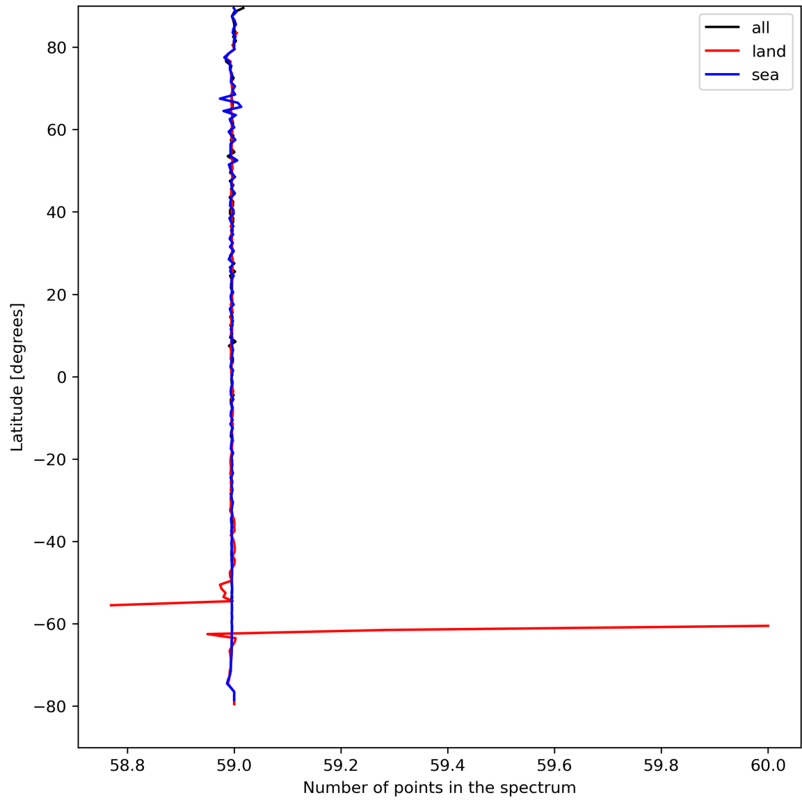
Figure 27: Zonal average of “Number of points in the spectrum” for 2023-08-30 to 2023-09-01.
