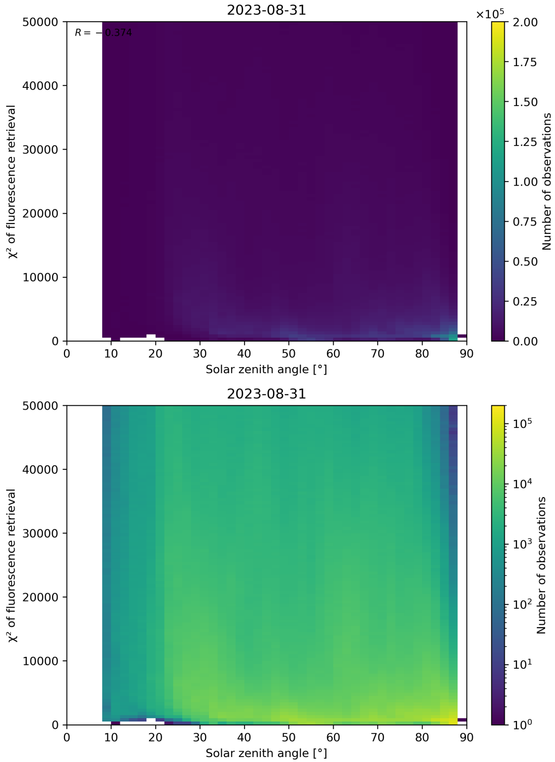
Figure 120: Scatter density plot of “Solar zenith angle” against “ \chi^2 of fluorescence retrieval” for 2023-08-30 to 2023-09-01.
