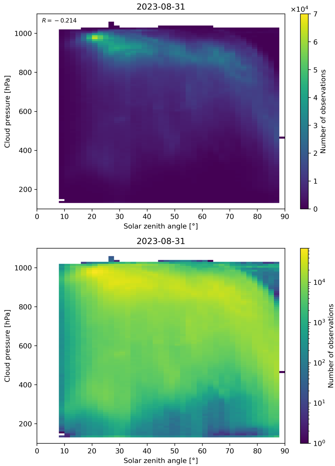
Figure 122: Scatter density plot of “Solar zenith angle” against “Cloud pressure” for 2023-08-30 to 2023-09-01.
