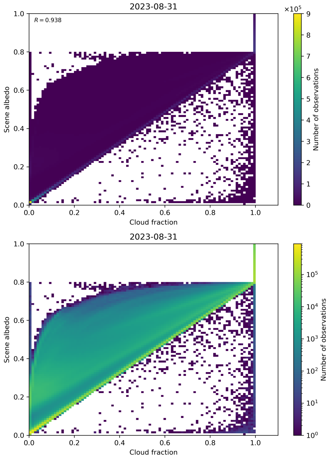
Figure 82: Scatter density plot of “Cloud fraction” against “Scene albedo” for 2023-08-30 to 2023-09-01.
