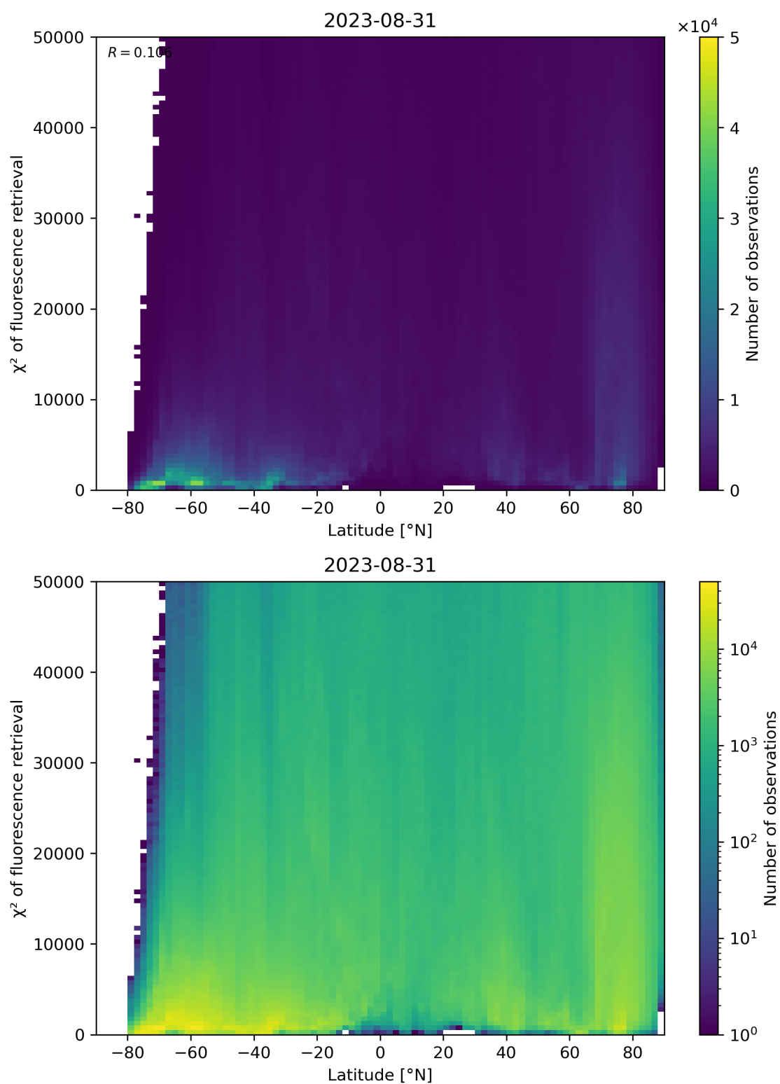
Figure 98: Scatter density plot of “Latitude” against “ \chi^2 of fluorescence retrieval” for 2023-08-30 to 2023-09-01.
