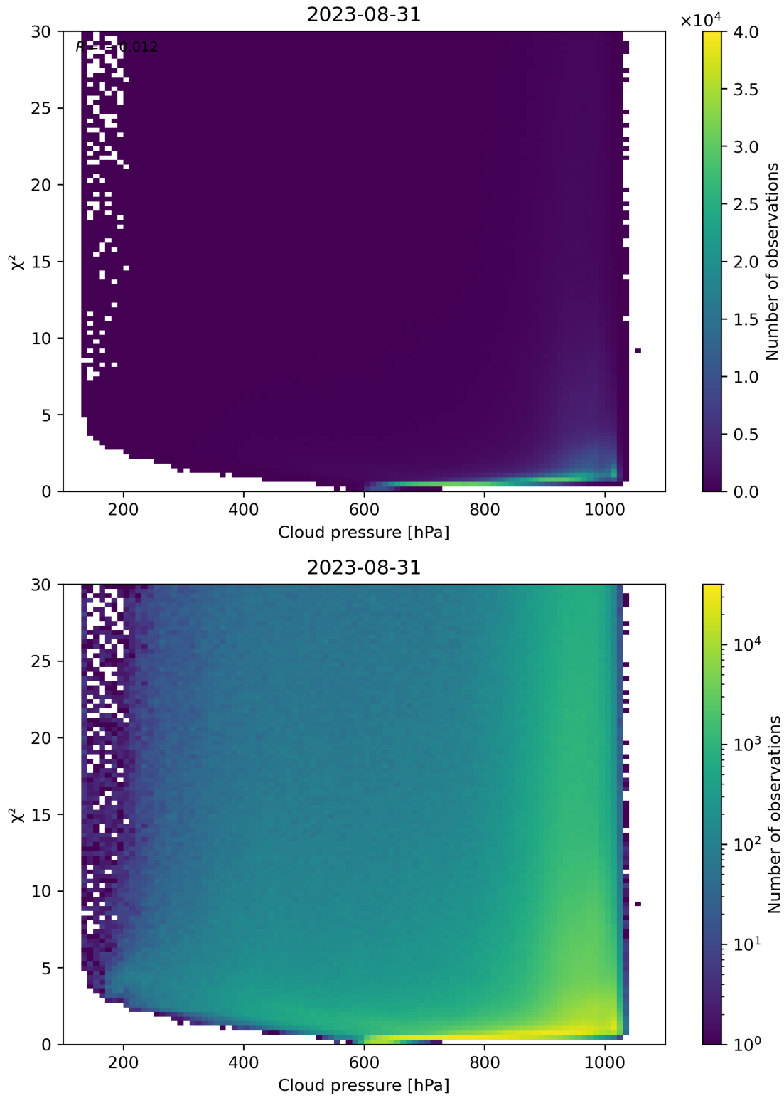
Figure 85: Scatter density plot of “Cloud pressure” against “ \chi^2 ” for 2023-08-30 to 2023-09-01.
