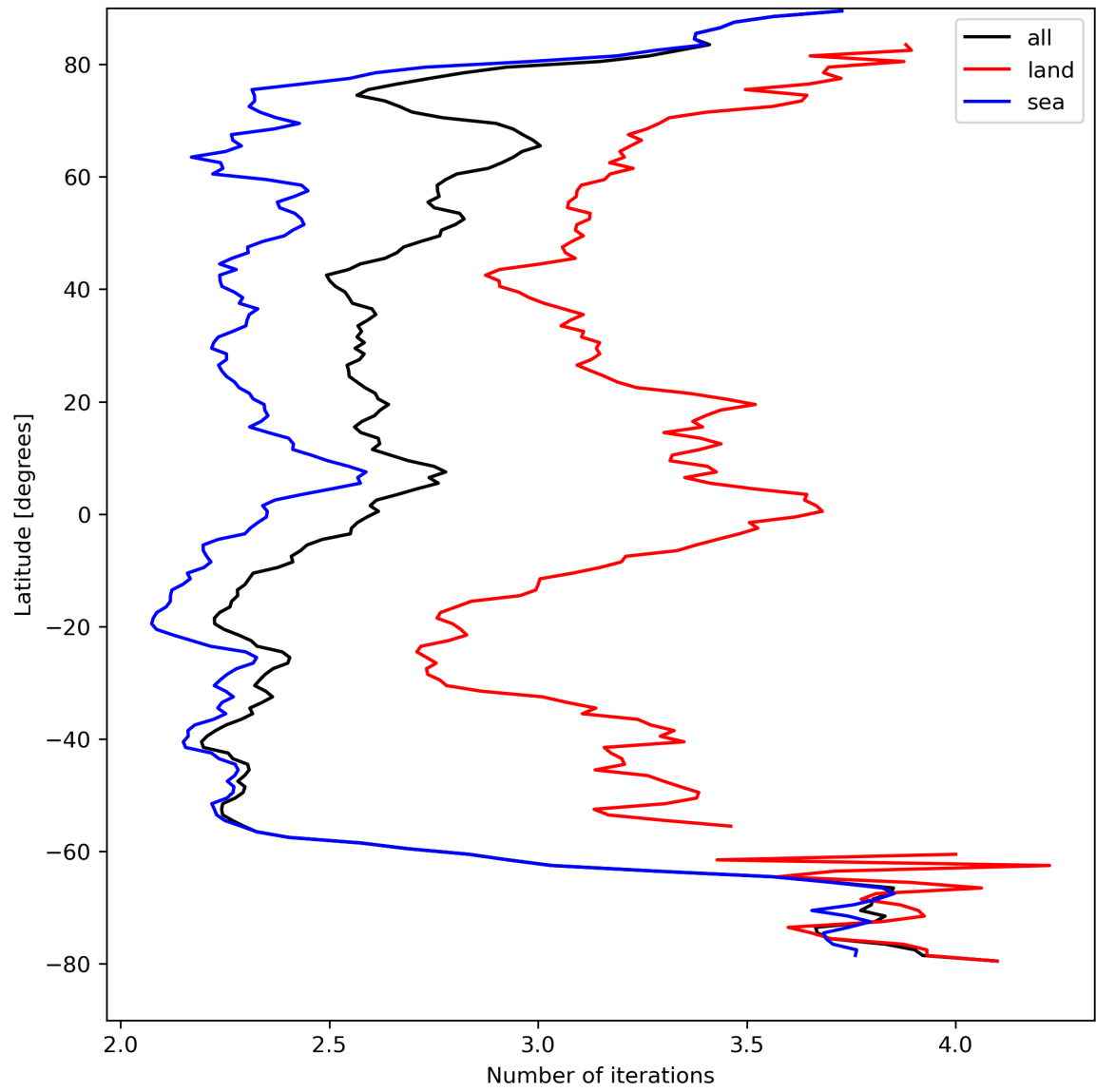
Figure 22: Zonal average of “Number of iterations” for 2023-08-30 to 2023-09-01.
