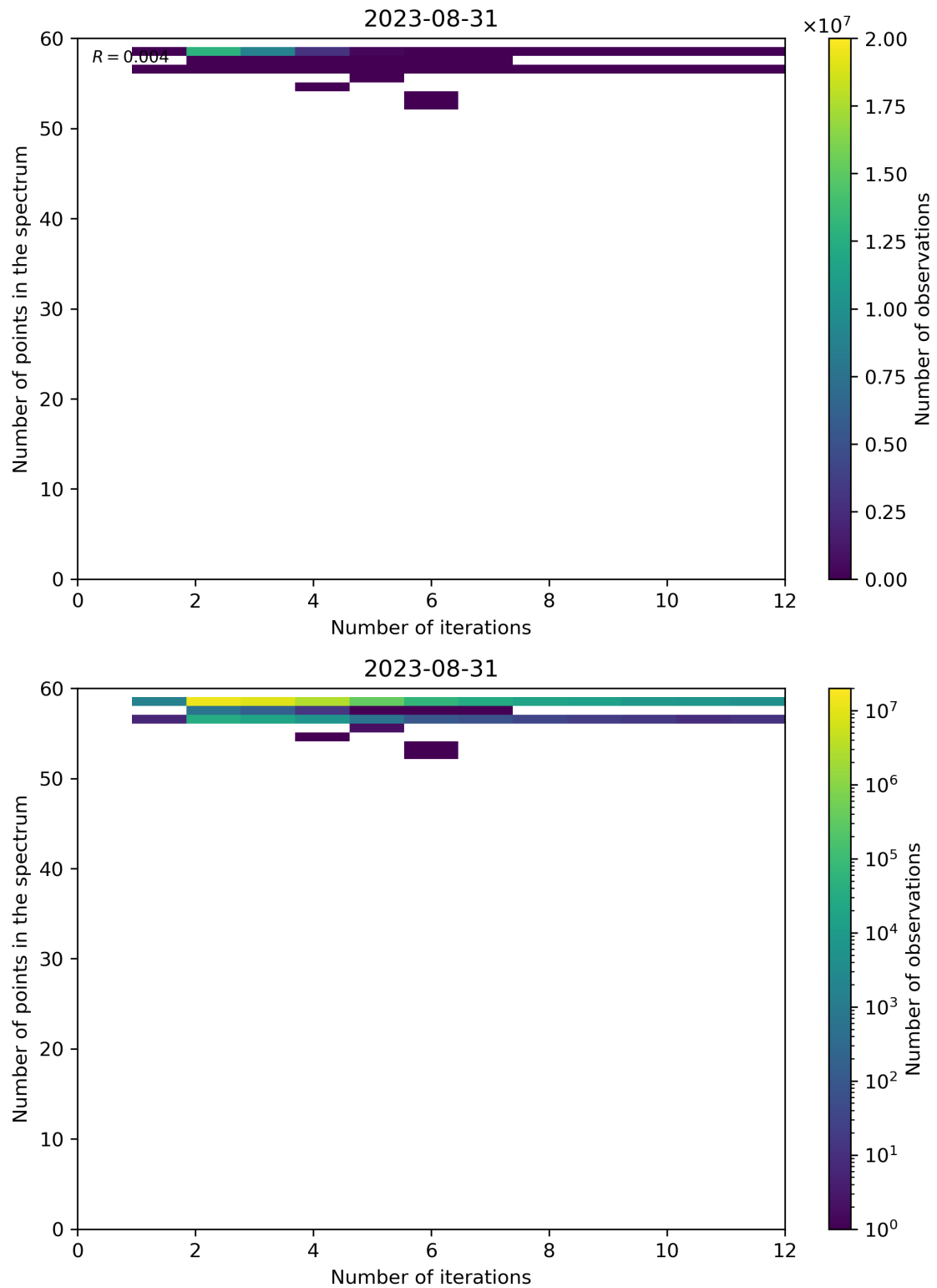
Figure 108: Scatter density plot of “Number of iterations” against “Number of points in the spectrum” for 2023-08-30 to 2023-09-01.
