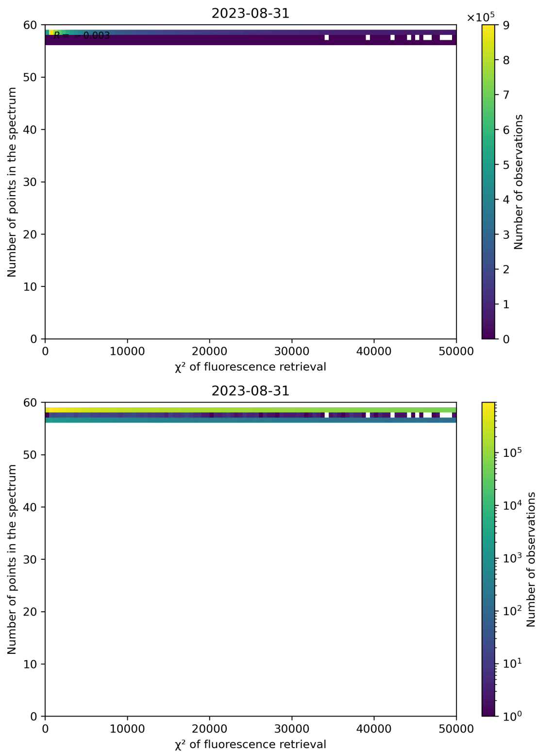
Figure 71: Scatter density plot of " \chi^2 of fluorescence retrieval" against "Number of points in the spectrum" for 2023-08-30 to 2023-09-01.
