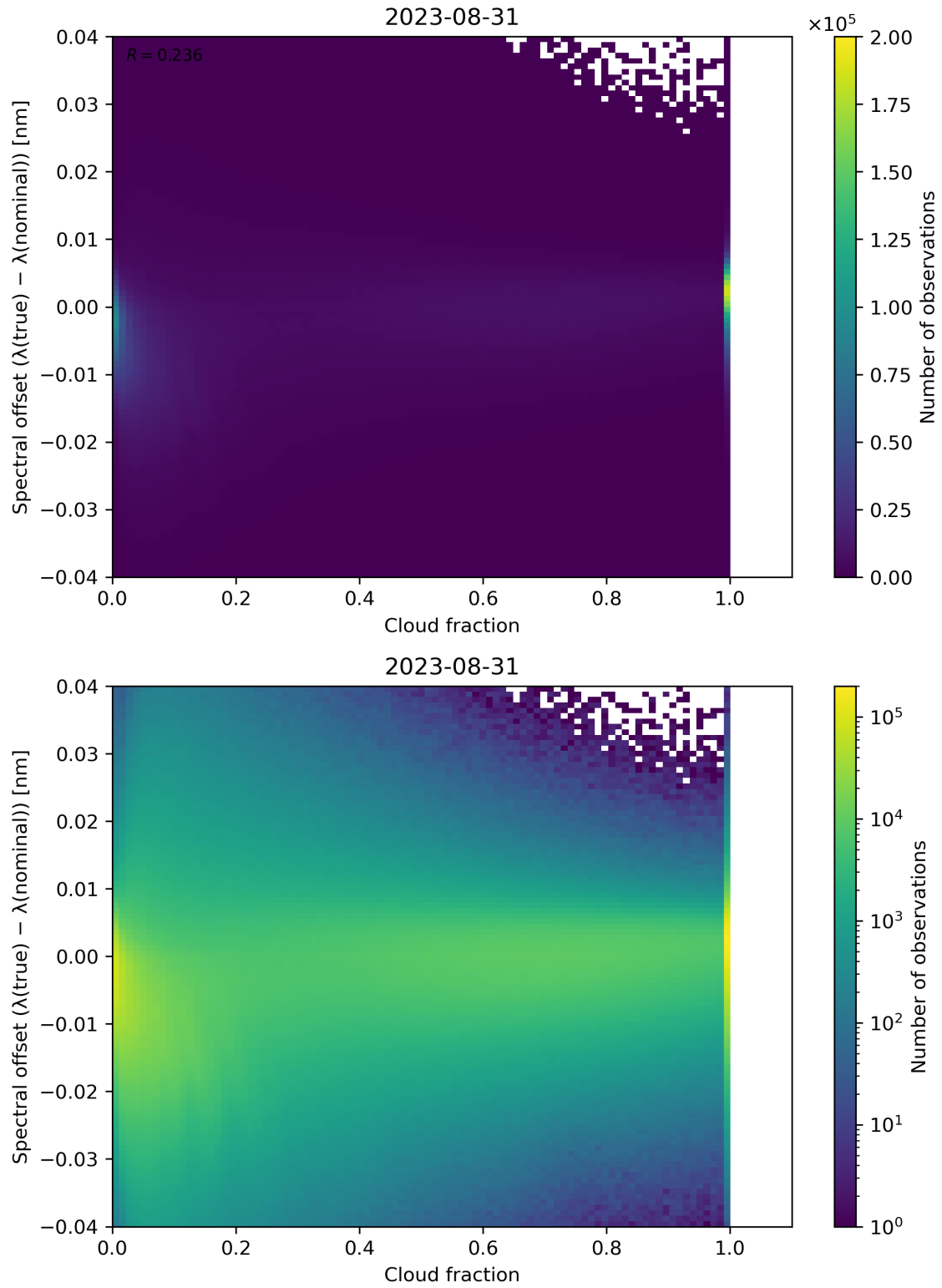
Figure 83: Scatter density plot of “Cloud fraction” against “Spectral offset ( \lambda(\text{true}) - \lambda(\text{nominal}) )” for 2023-08-30 to 2023-09-01.
