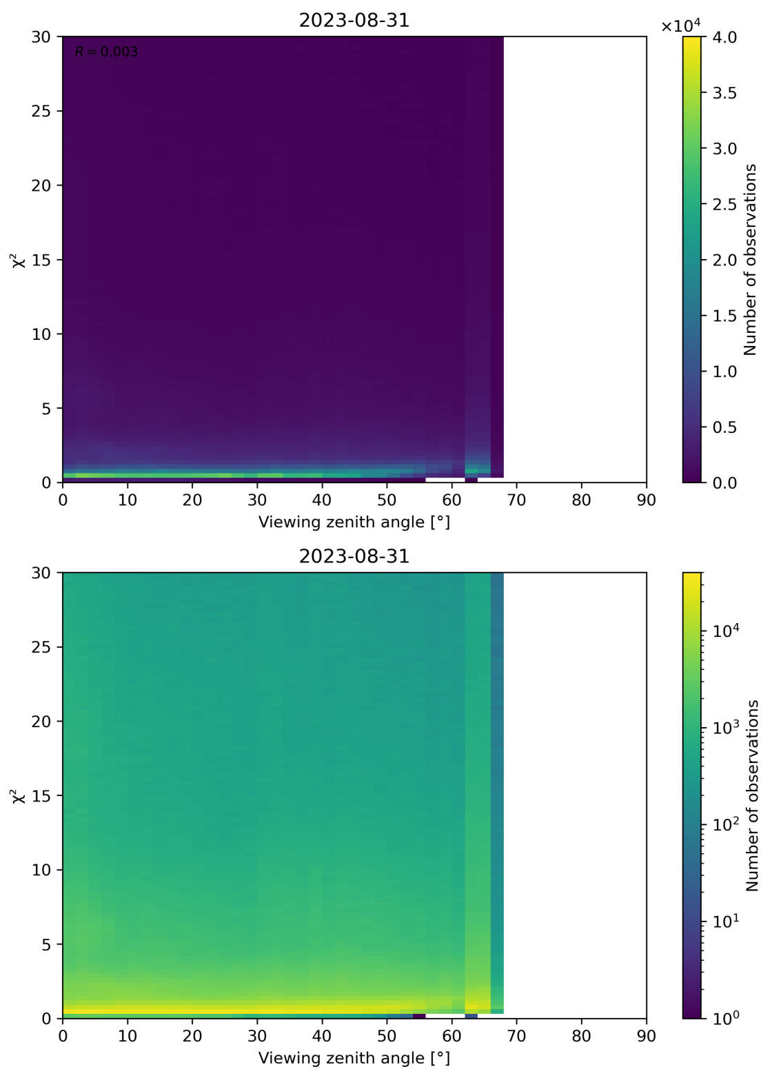
Figure 130: Scatter density plot of “Viewing zenith angle” against “ \chi^2 ” for 2023-08-30 to 2023-09-01.
