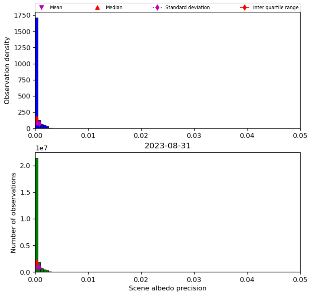
Figure 35: Histogram of “Scene albedo precision” for 2023-08-30 to 2023-09-01
