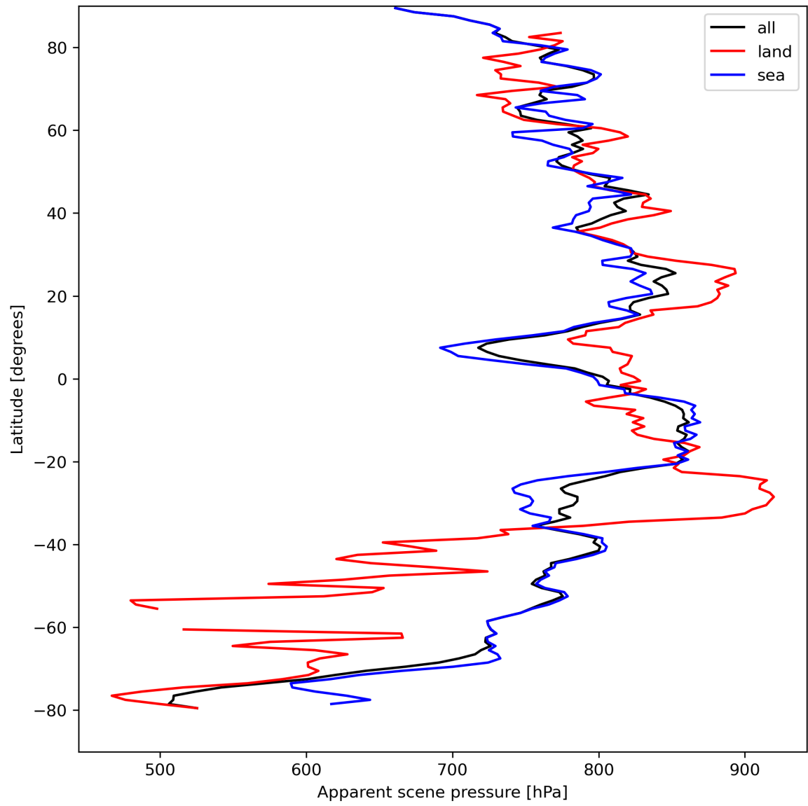
Figure 19: Zonal average of “Apparent scene pressure” for 2023-08-30 to 2023-09-01.
