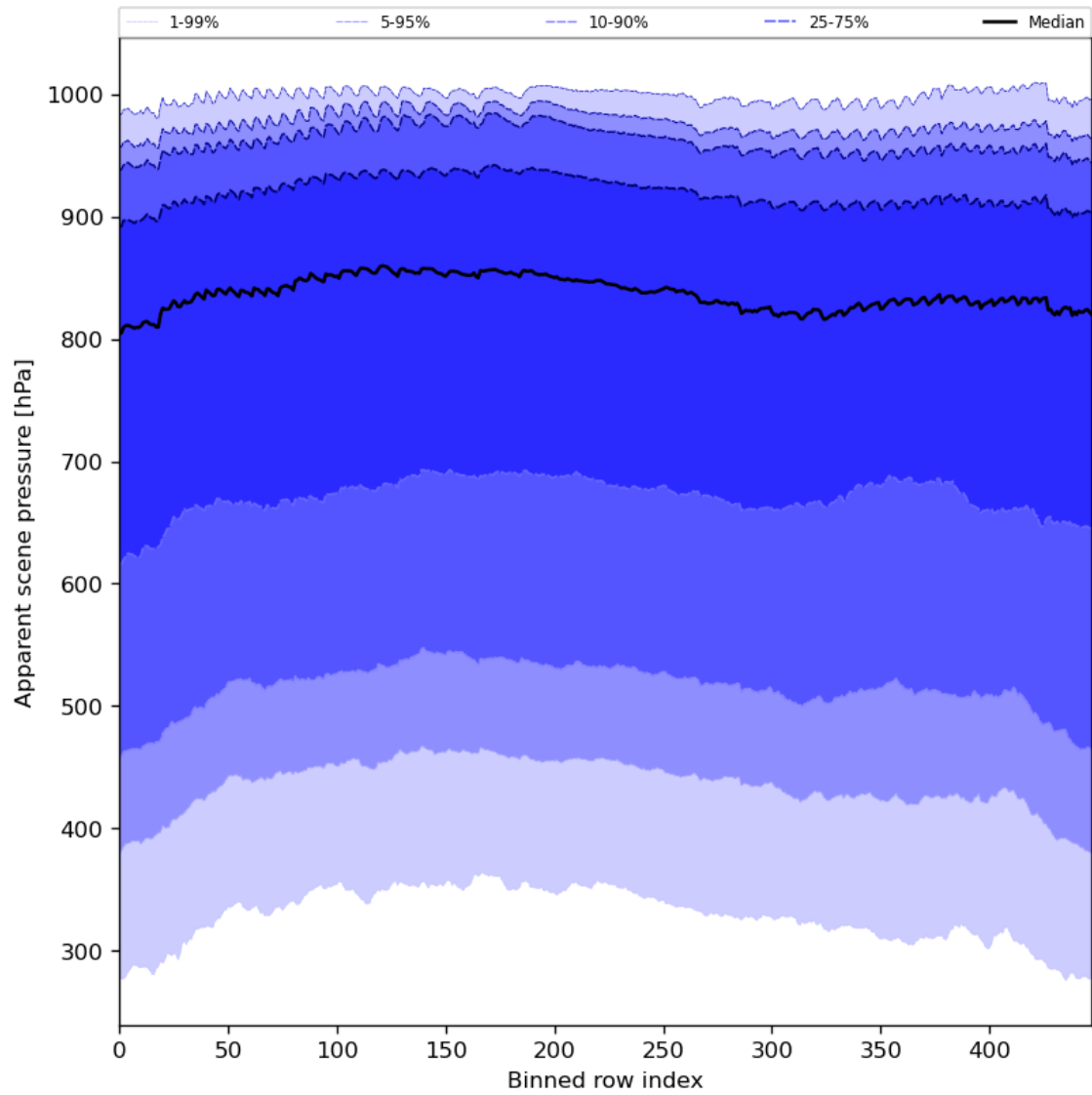
Figure 53: Along track statistics of “Apparent scene pressure” for 2023-08-30 to 2023-09-01
