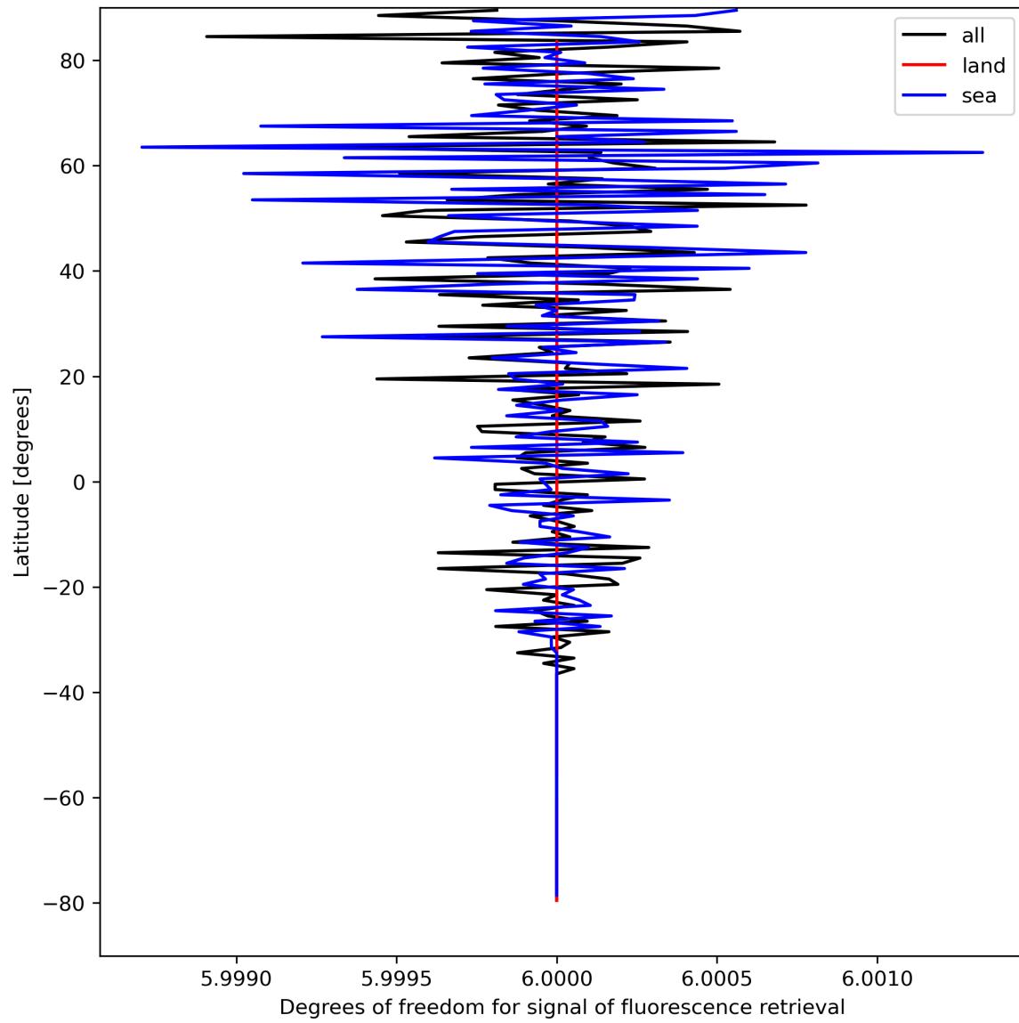
Figure 26: Zonal average of “Degrees of freedom for signal of fluorescence retrieval” for 2023-08-30 to 2023-09-01.
