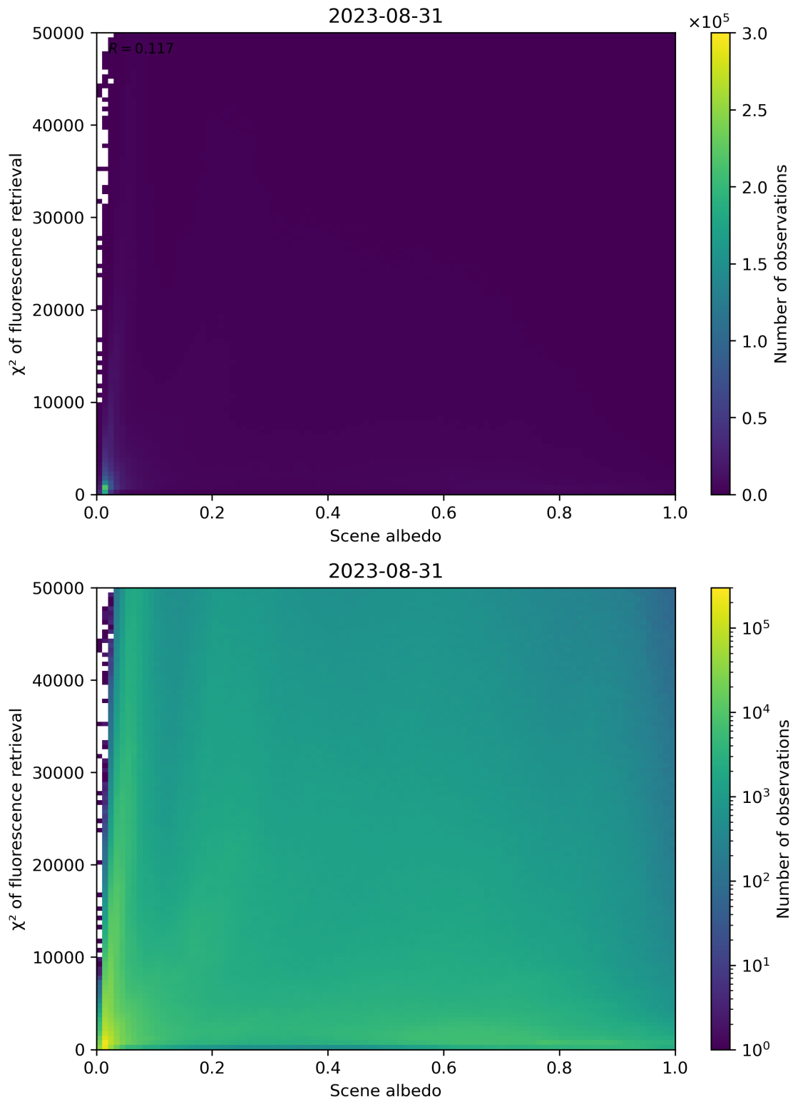
Figure 113: Scatter density plot of “Scene albedo” against “ \chi^2 of fluorescence retrieval” for 2023-08-30 to 2023-09-01.
