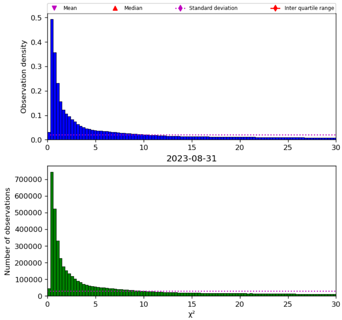
Figure 38: Histogram of " \chi^2 " for 2023-08-30 to 2023-09-01
