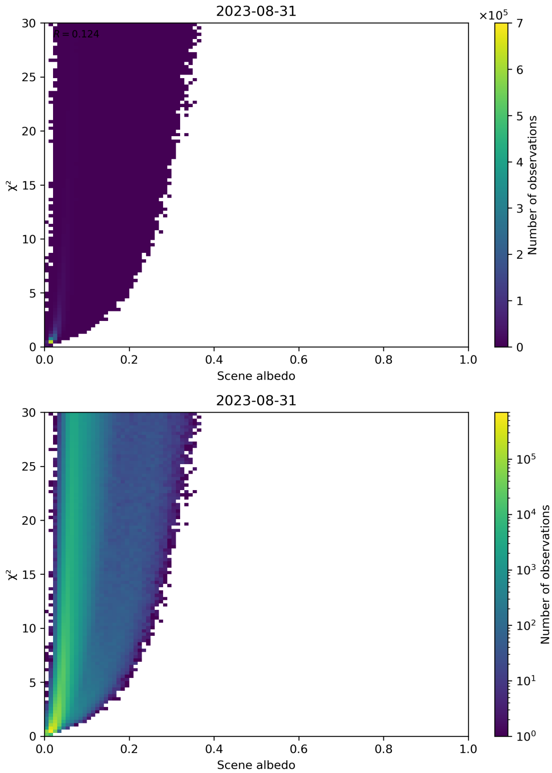
Figure 112: Scatter density plot of “Scene albedo” against “ \chi^2 ” for 2023-08-30 to 2023-09-01.
