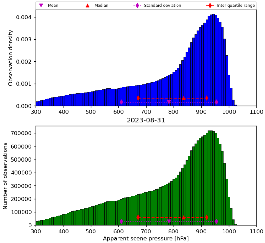
Figure 36: Histogram of “Apparent scene pressure” for 2023-08-30 to 2023-09-01
