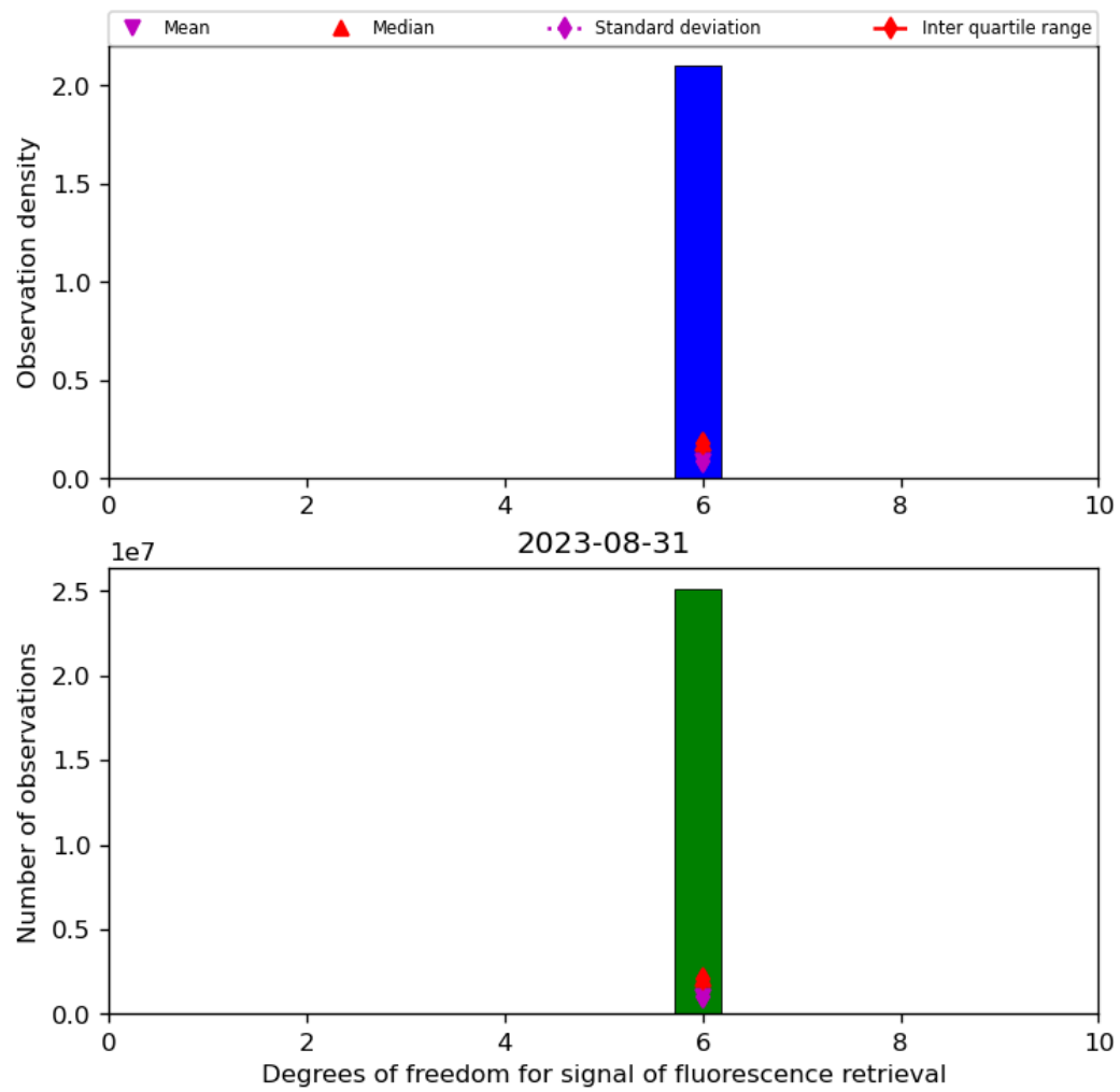
Figure 43: Histogram of “Degrees of freedom for signal of fluorescence retrieval” for 2023-08-30 to 2023-09-01
