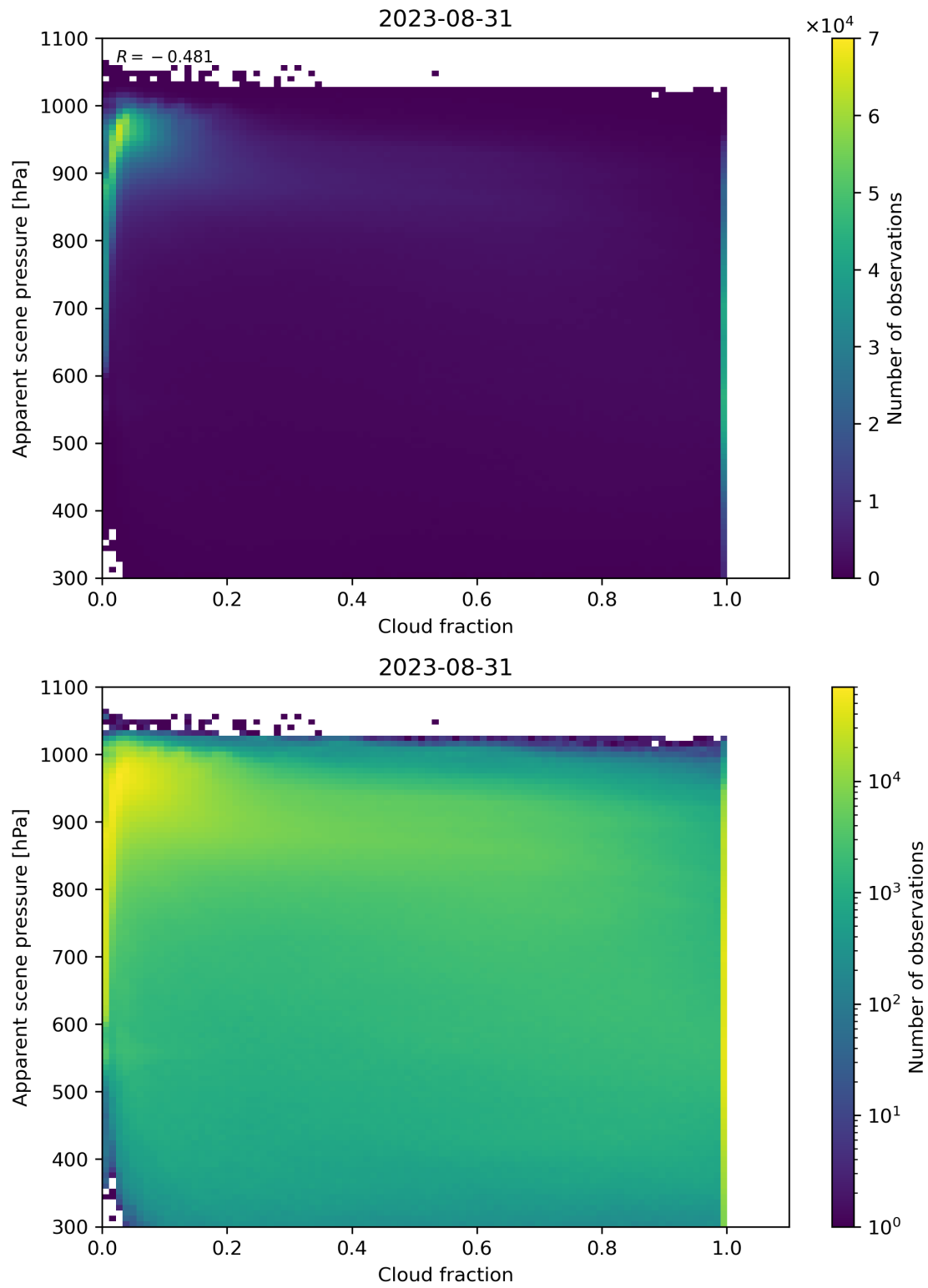
Figure 76: Scatter density plot of “Cloud fraction” against “Apparent scene pressure” for 2023-08-30 to 2023-09-01.
