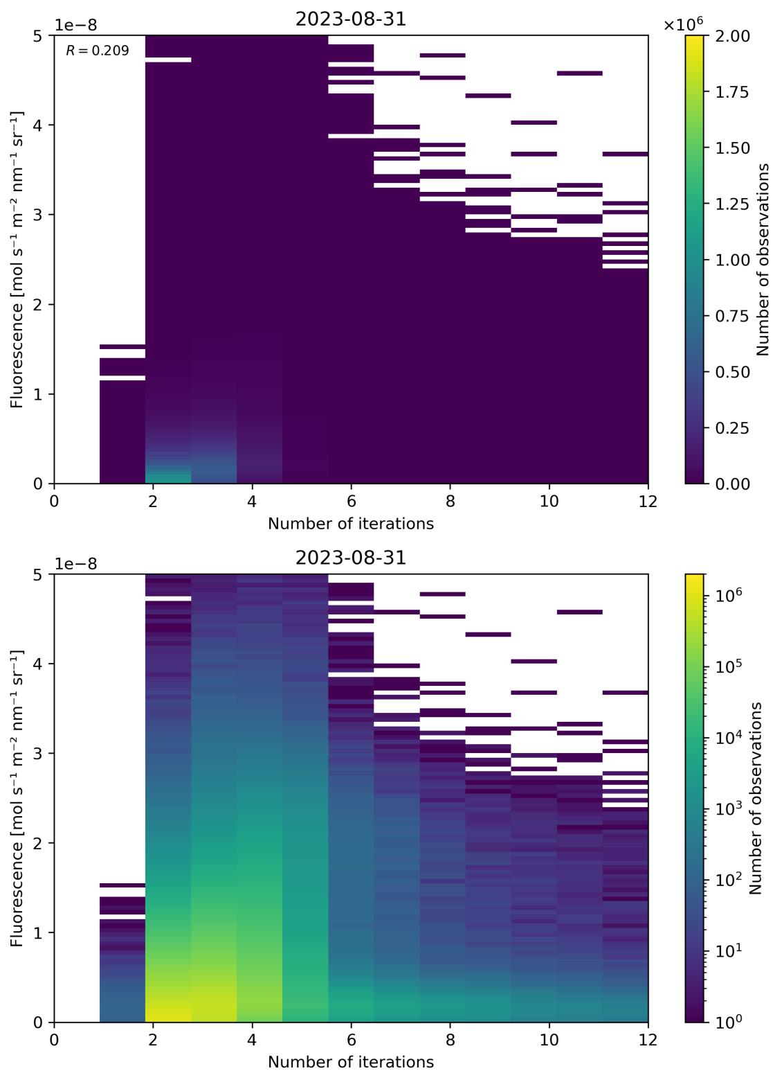
Figure 107: Scatter density plot of “Number of iterations” against “Fluorescence” for 2023-08-30 to 2023-09-01.
