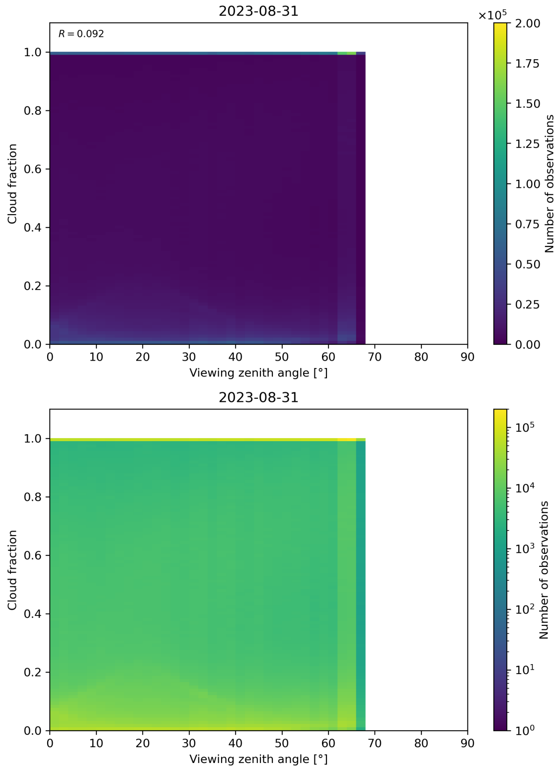
Figure 132: Scatter density plot of “Viewing zenith angle” against “Cloud fraction” for 2023-08-30 to 2023-09-01.
