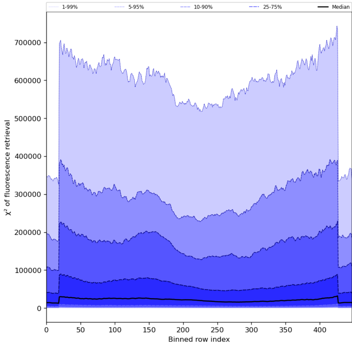
Figure 59: Along track statistics of “ \chi^2 of fluorescence retrieval” for 2023-08-30 to 2023-09-01
