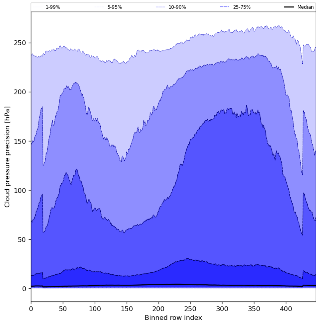
Figure 48: Along track statistics of “Cloud pressure precision” for 2023-08-30 to 2023-09-01
