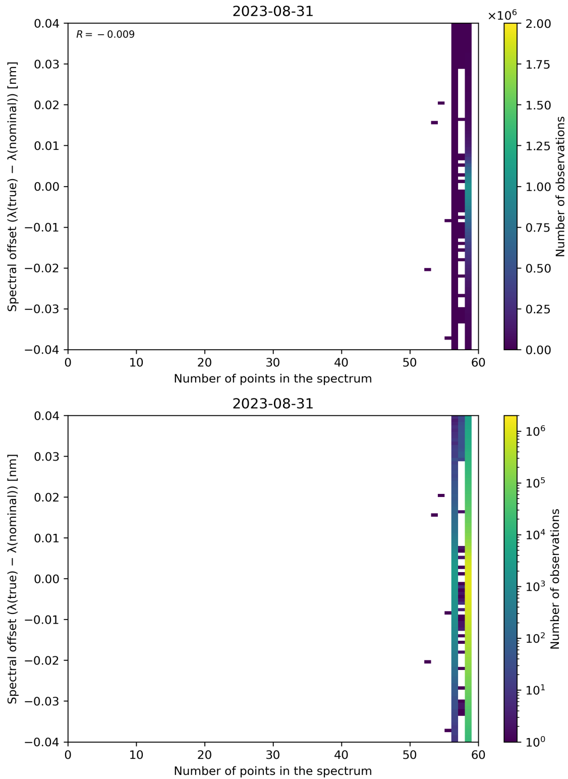
Figure 110: Scatter density plot of “Number of points in the spectrum” against “Spectral offset ( \lambda(\text{true}) - \lambda(\text{nominal}) )” for 2023-08-30 to 2023-09-01.
