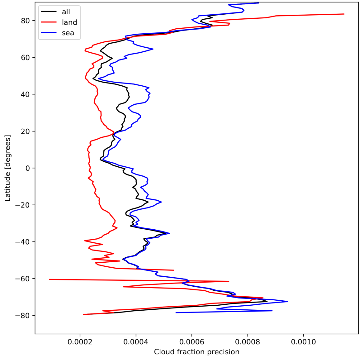
Figure 16: Zonal average of “Cloud fraction precision” for 2023-08-30 to 2023-09-01.
