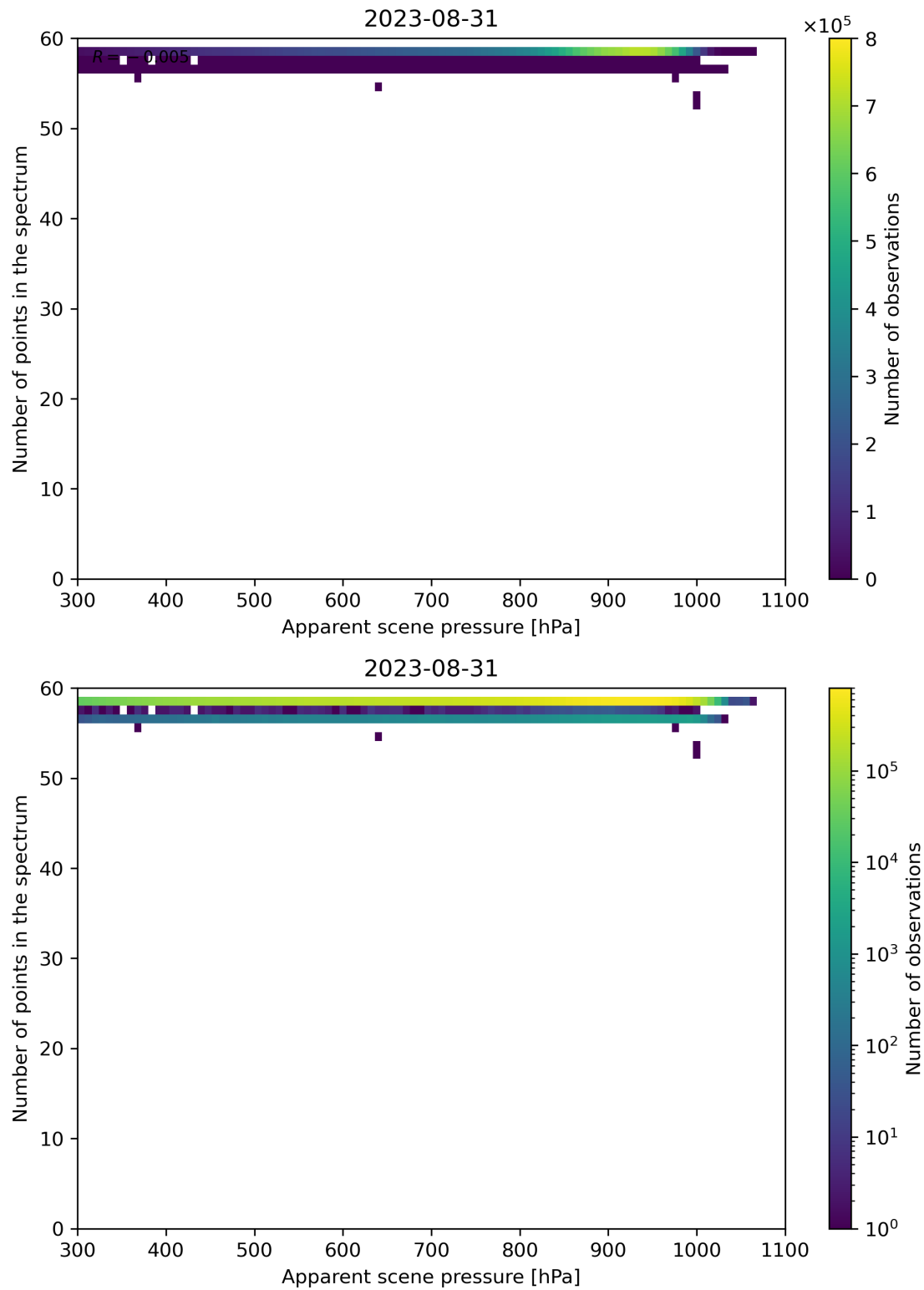
Figure 67: Scatter density plot of “Apparent scene pressure” against “Number of points in the spectrum” for 2023-08-30 to 2023-09-01.
