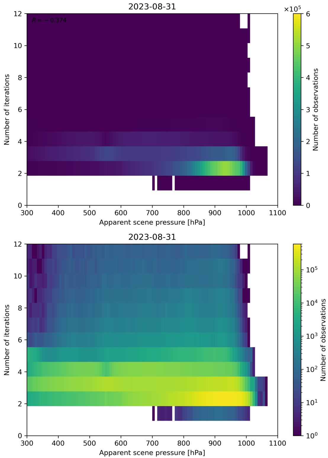
Figure 66: Scatter density plot of “Apparent scene pressure” against “Number of iterations” for 2023-08-30 to 2023-09-01.
