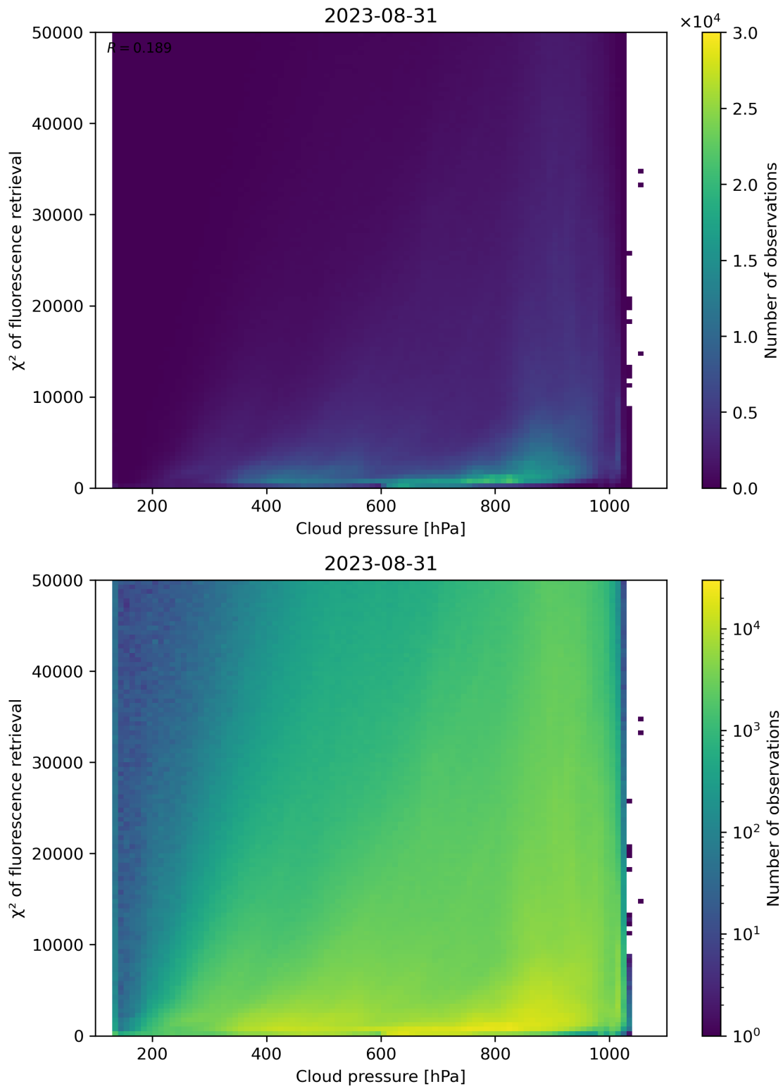
Figure 86: Scatter density plot of “Cloud pressure” against “ \chi^2 of fluorescence retrieval” for 2023-08-30 to 2023-09-01.
