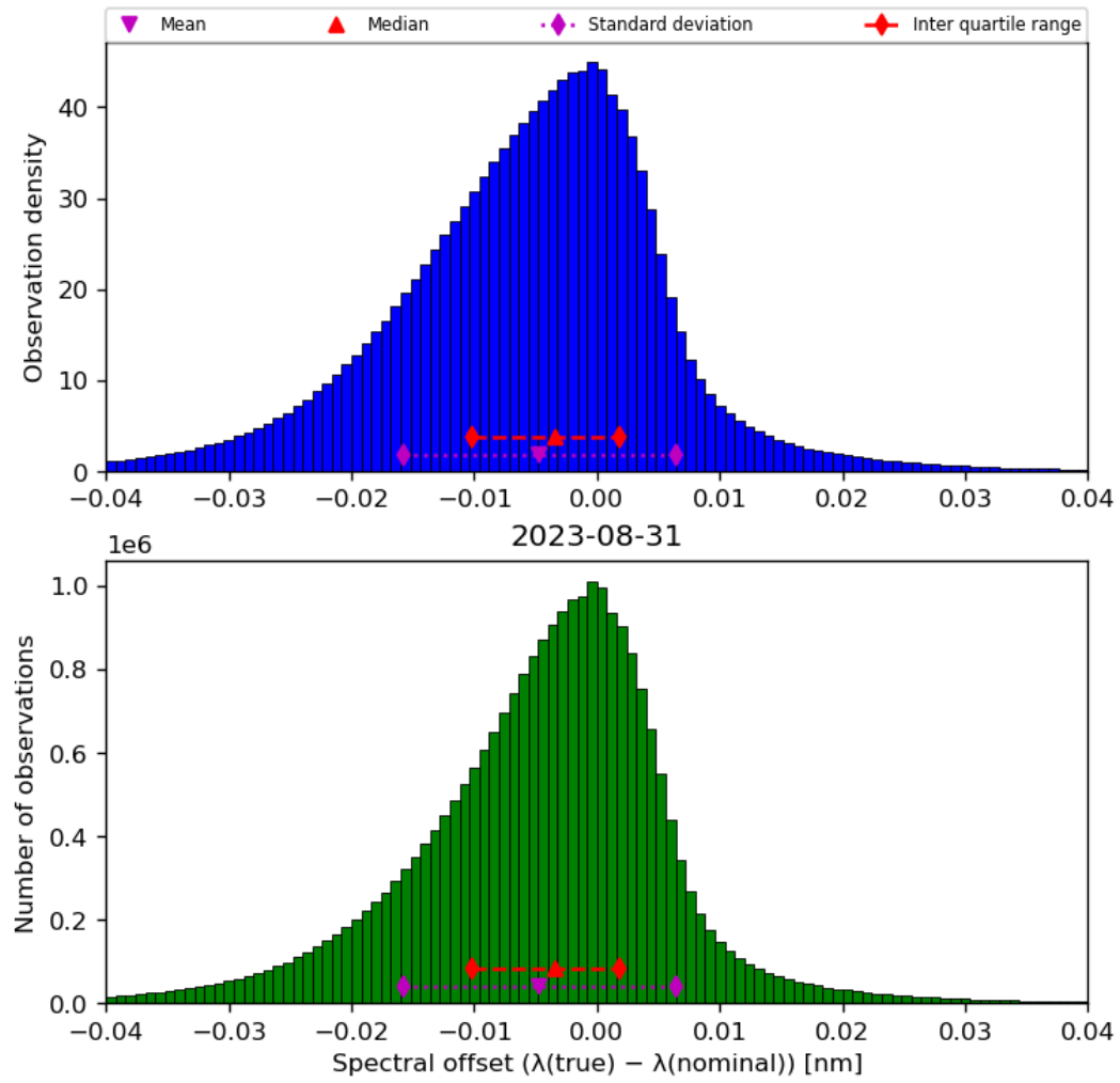
Figure 45: Histogram of “Spectral offset ( \lambda(\text{true}) - \lambda(\text{nominal}) )” for 2023-08-30 to 2023-09-01
