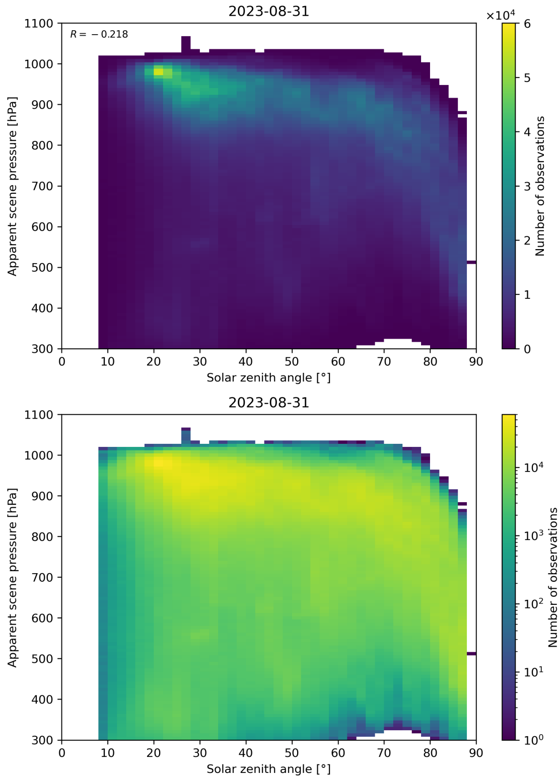
Figure 118: Scatter density plot of “Solar zenith angle” against “Apparent scene pressure” for 2023-08-30 to 2023-09-01.
