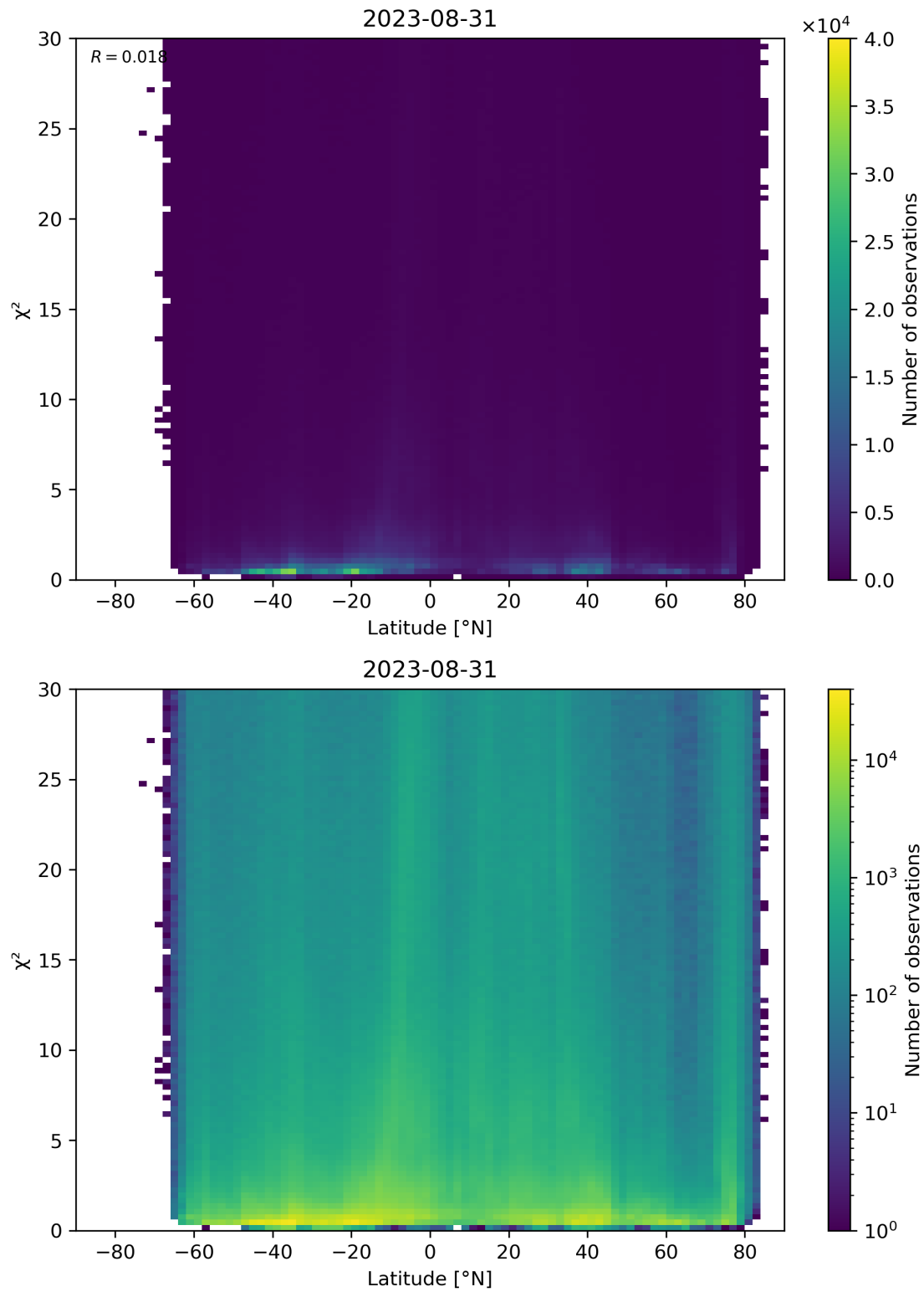
Figure 97: Scatter density plot of “Latitude” against “ \chi^2 ” for 2023-08-30 to 2023-09-01.
