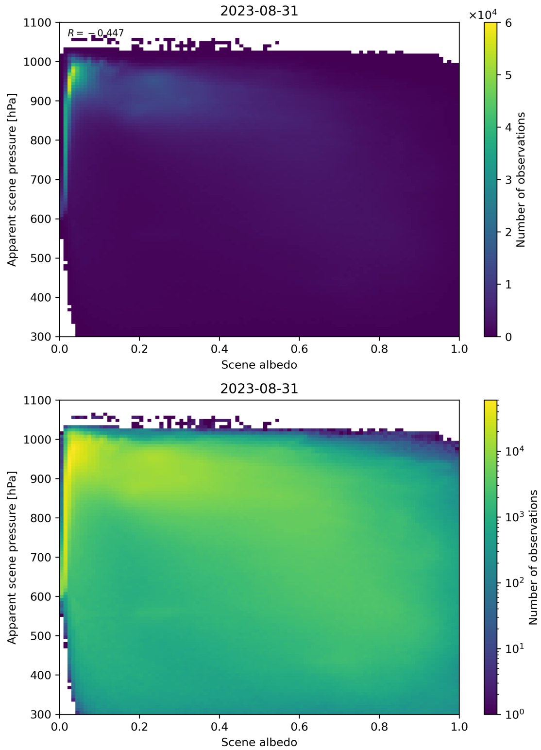
Figure 111: Scatter density plot of “Scene albedo” against “Apparent scene pressure” for 2023-08-30 to 2023-09-01.
