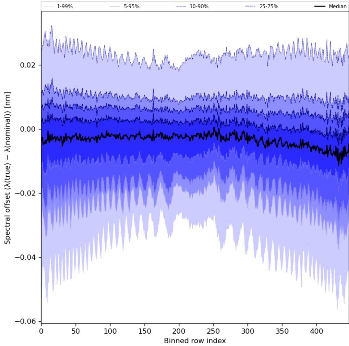
Figure 62: Along track statistics of “Spectral offset ( \lambda(\text{true}) - \lambda(\text{nominal}) )” for 2023-08-30 to 2023-09-01
