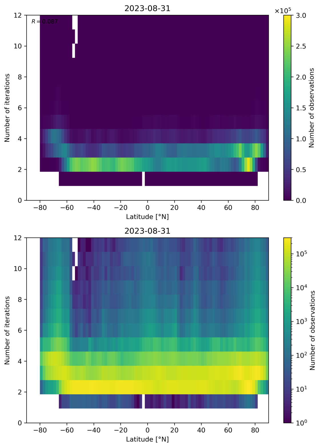
Figure 102: Scatter density plot of “Latitude” against “Number of iterations” for 2023-08-30 to 2023-09-01.
