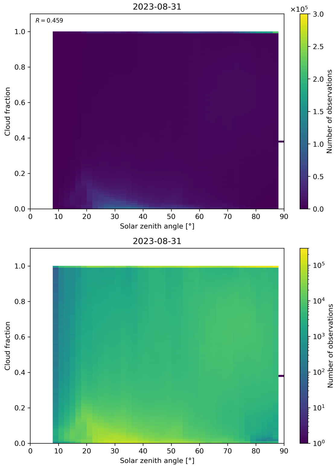
Figure 121: Scatter density plot of “Solar zenith angle” against “Cloud fraction” for 2023-08-30 to 2023-09-01.
