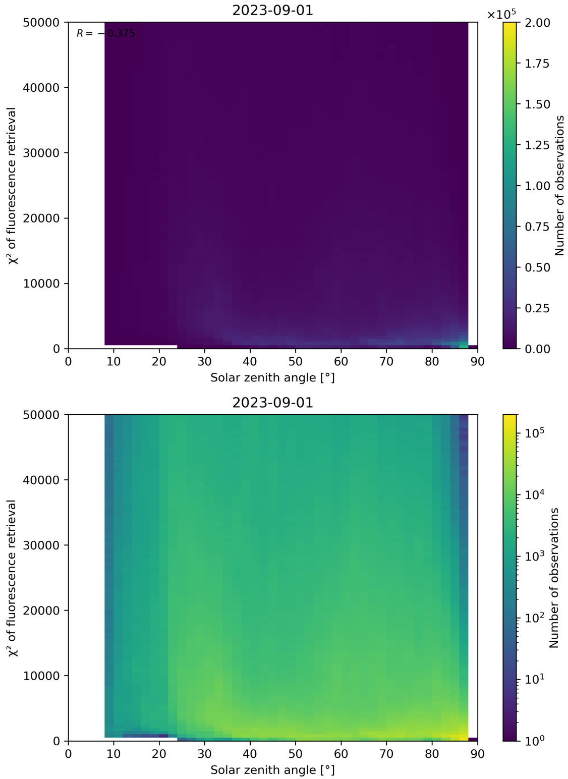
Figure 120: Scatter density plot of “Solar zenith angle” against “ \chi^2 of fluorescence retrieval” for 2023-08-31 to 2023-09-02.
