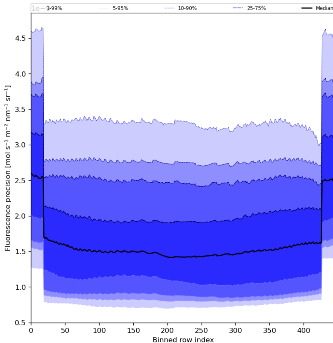
Figure 58: Along track statistics of “Fluorescence precision” for 2023-08-31 to 2023-09-02
