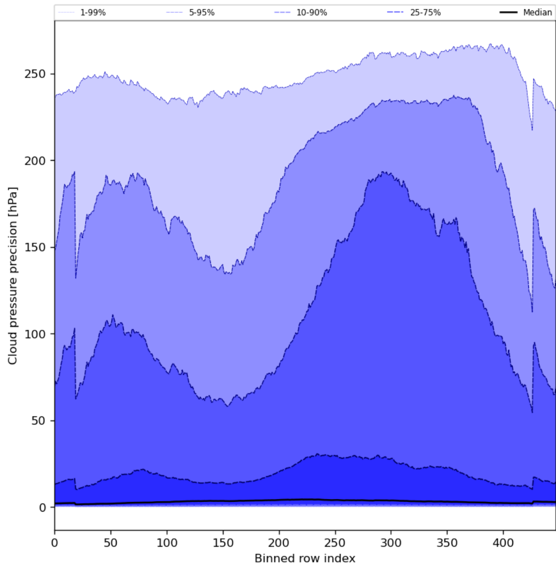
Figure 48: Along track statistics of “Cloud pressure precision” for 2023-08-31 to 2023-09-02
