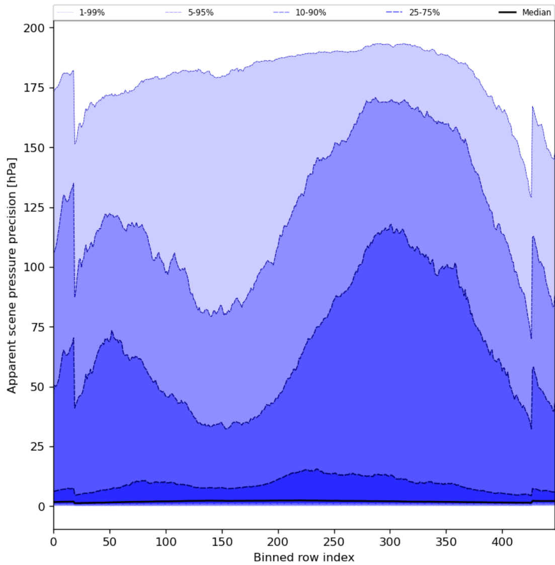
Figure 54: Along track statistics of “Apparent scene pressure precision” for 2023-08-31 to 2023-09-02
