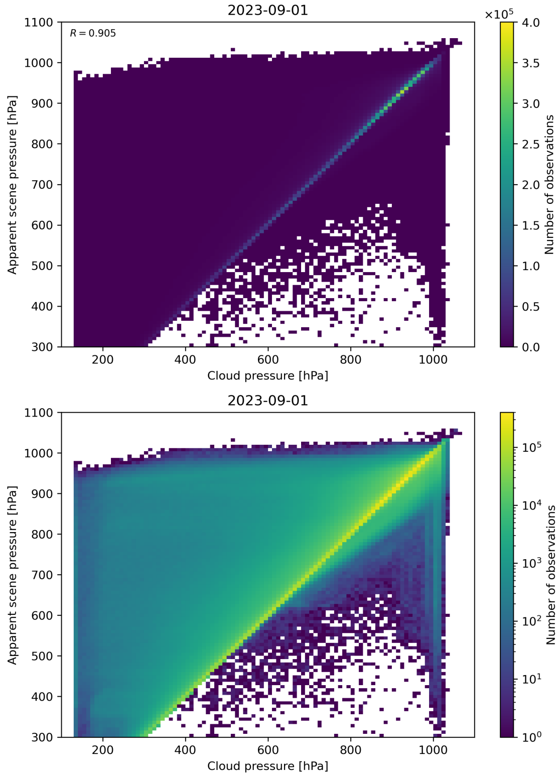
Figure 84: Scatter density plot of “Cloud pressure” against “Apparent scene pressure” for 2023-08-31 to 2023-09-02.
