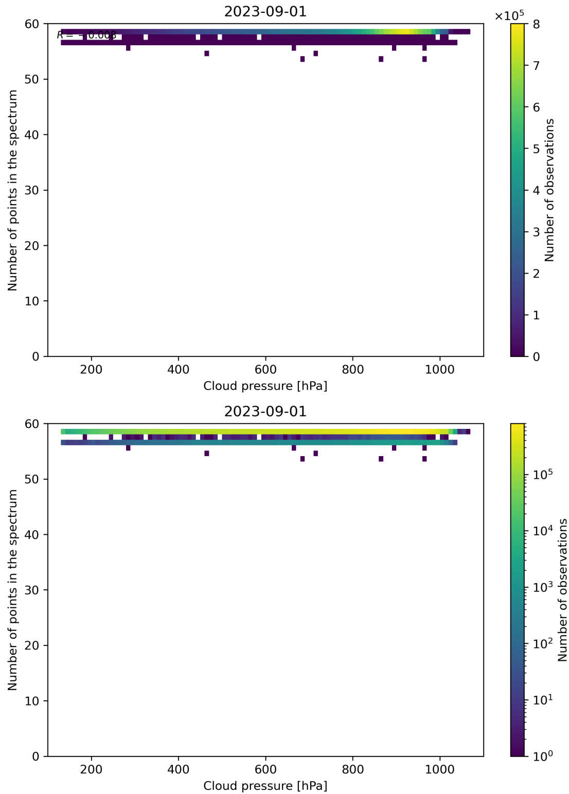
Figure 90: Scatter density plot of “Cloud pressure” against “Number of points in the spectrum” for 2023-08-31 to 2023-09-02.
