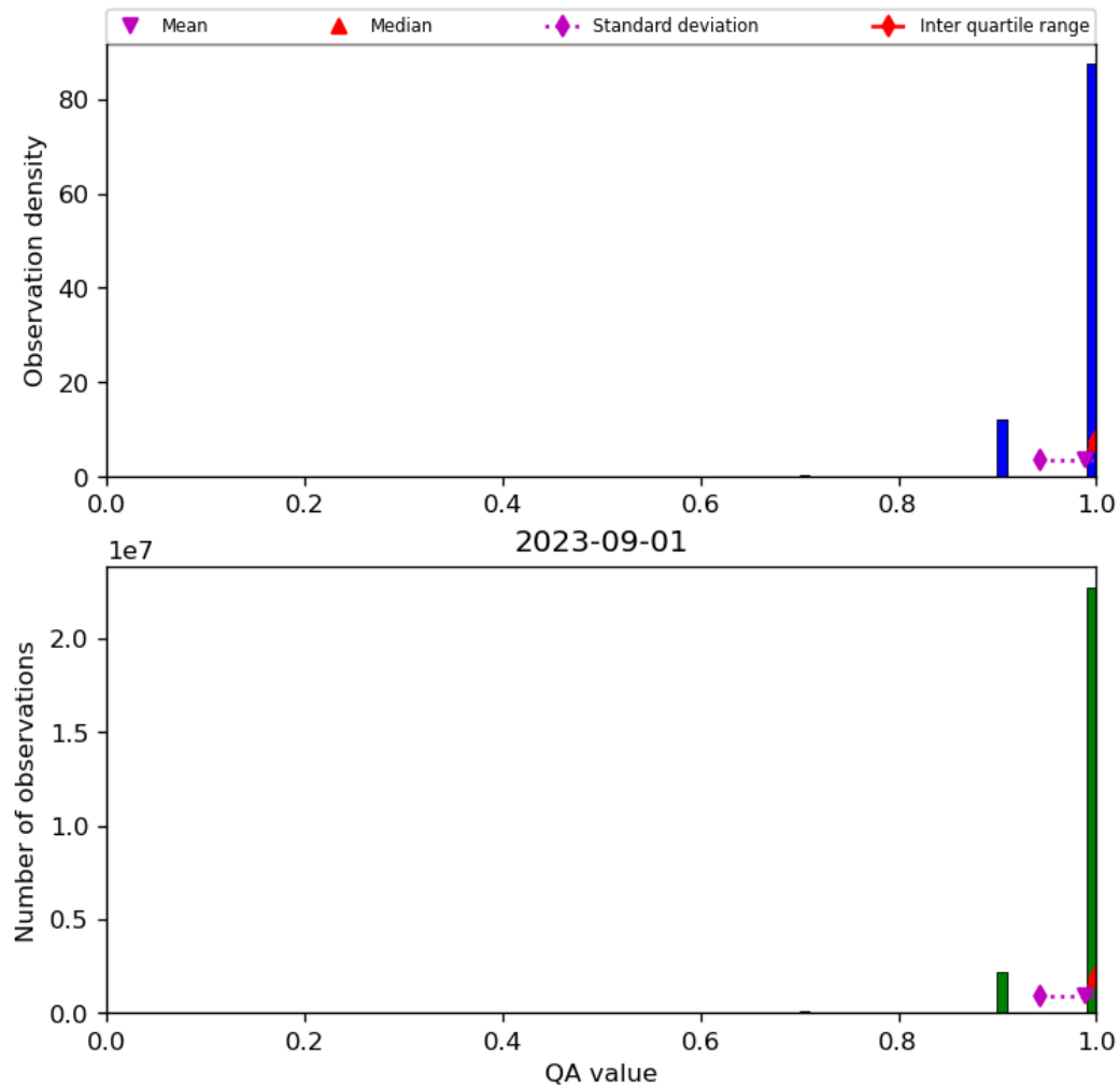
Figure 29: Histogram of “QA value” for 2023-08-31 to 2023-09-02
