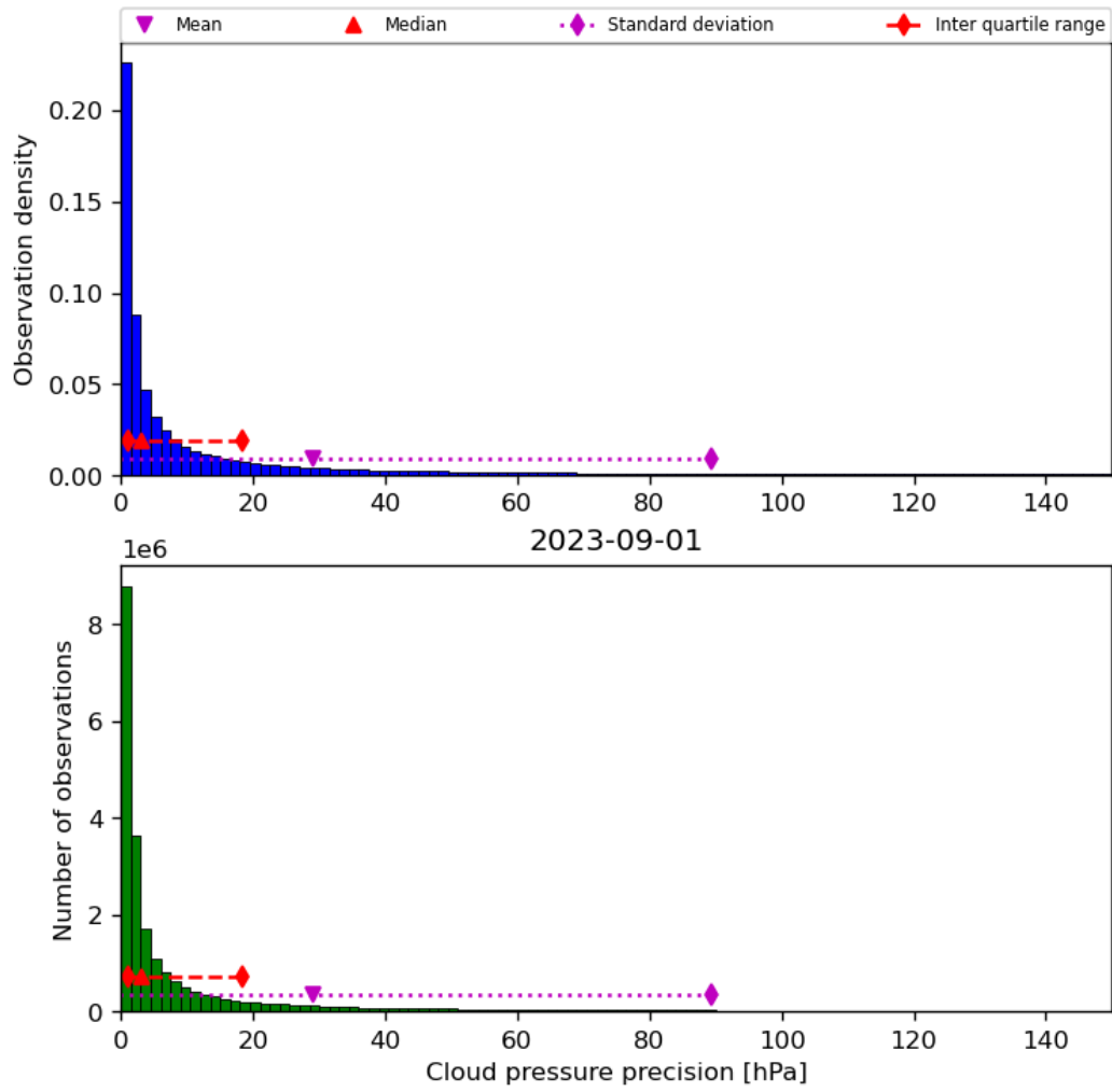
Figure 31: Histogram of “Cloud pressure precision” for 2023-08-31 to 2023-09-02
