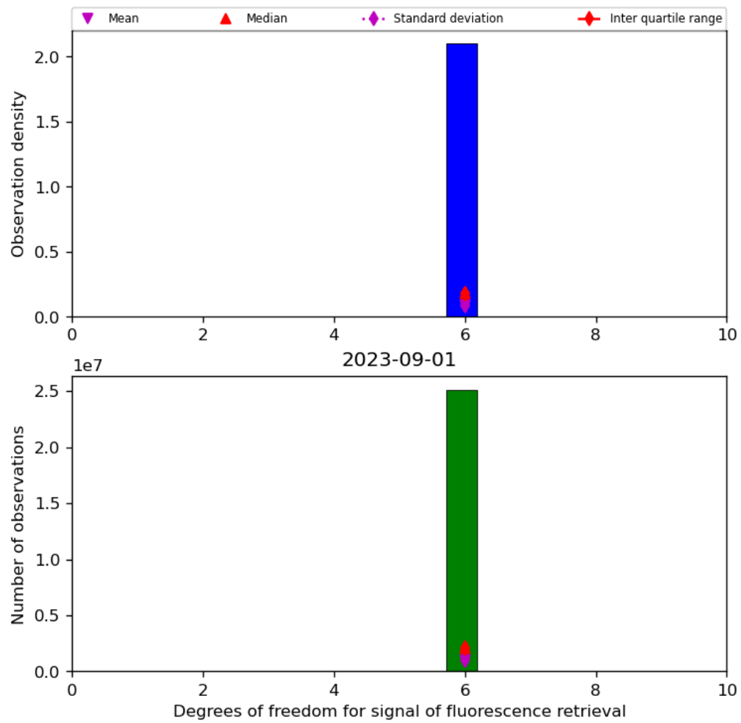
Figure 43: Histogram of “Degrees of freedom for signal of fluorescence retrieval” for 2023-08-31 to 2023-09-02
