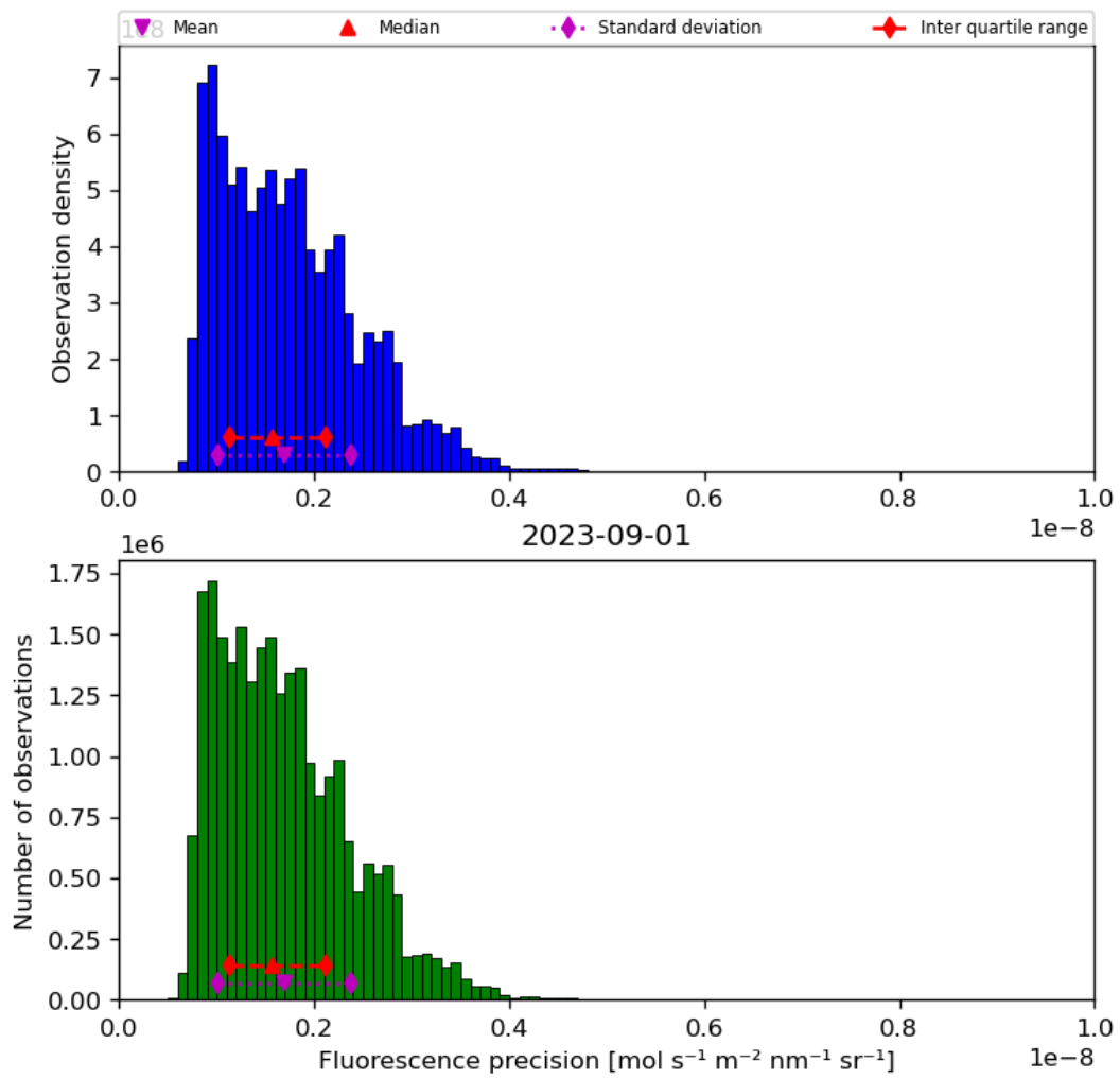
Figure 41: Histogram of “Fluorescence precision” for 2023-08-31 to 2023-09-02
