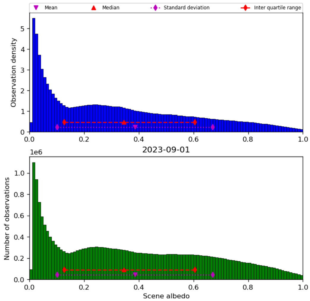
Figure 34: Histogram of “Scene albedo” for 2023-08-31 to 2023-09-02
