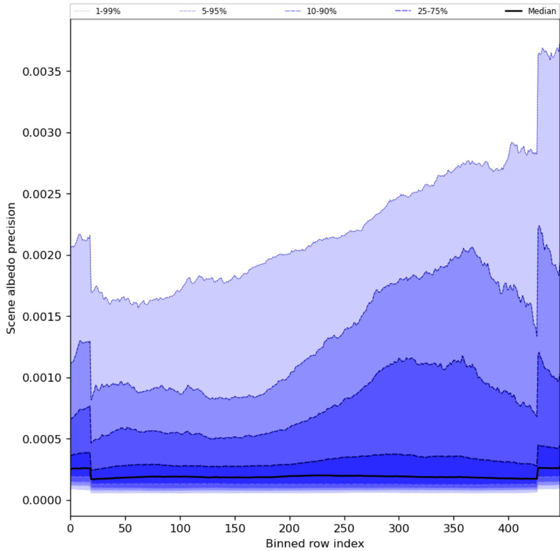
Figure 52: Along track statistics of “Scene albedo precision” for 2023-08-31 to 2023-09-02
