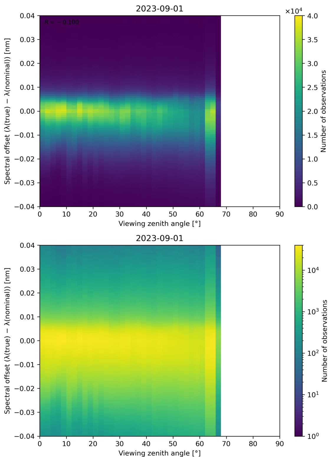
Figure 140: Scatter density plot of “Viewing zenith angle” against “Spectral offset ( \lambda(\text{true}) - \lambda(\text{nominal}) )” for 2023-08-31 to 2023-09-02.
