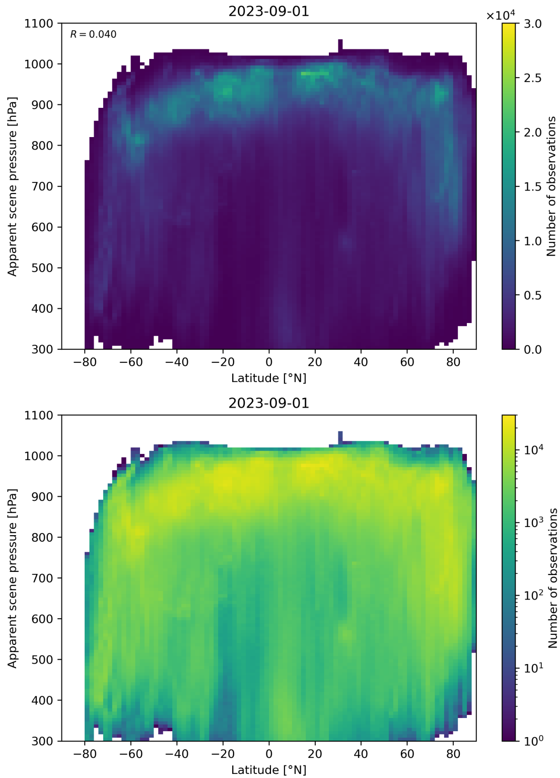
Figure 96: Scatter density plot of “Latitude” against “Apparent scene pressure” for 2023-08-31 to 2023-09-02.
