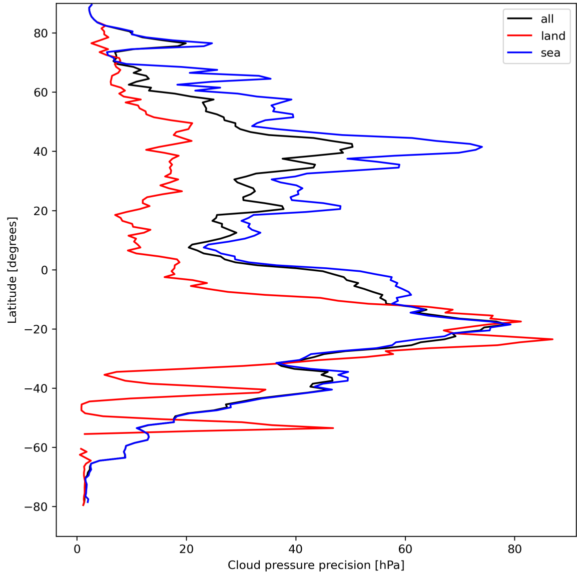
Figure 14: Zonal average of “Cloud pressure precision” for 2023-08-31 to 2023-09-02.
