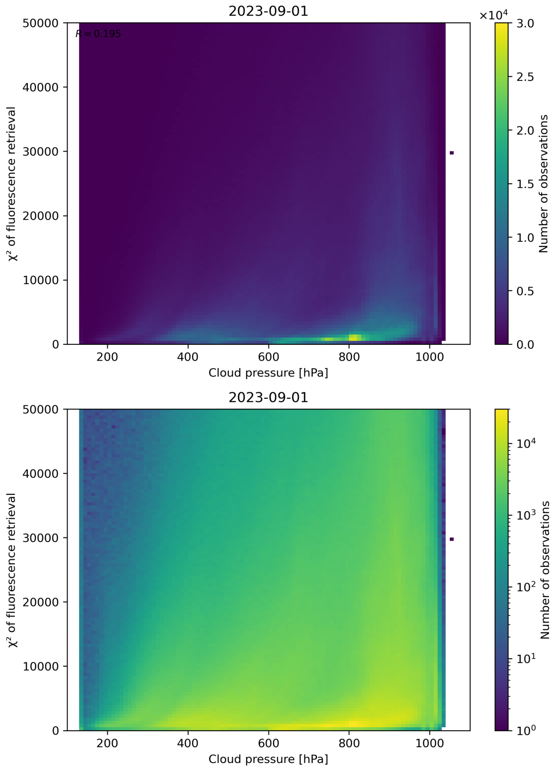
Figure 86: Scatter density plot of “Cloud pressure” against “ \chi^2 of fluorescence retrieval” for 2023-08-31 to 2023-09-02.
