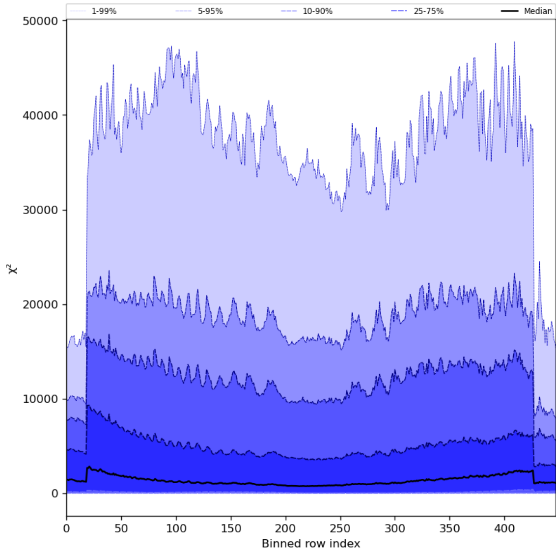
Figure 55: Along track statistics of “ \chi^2 ” for 2023-08-31 to 2023-09-02
