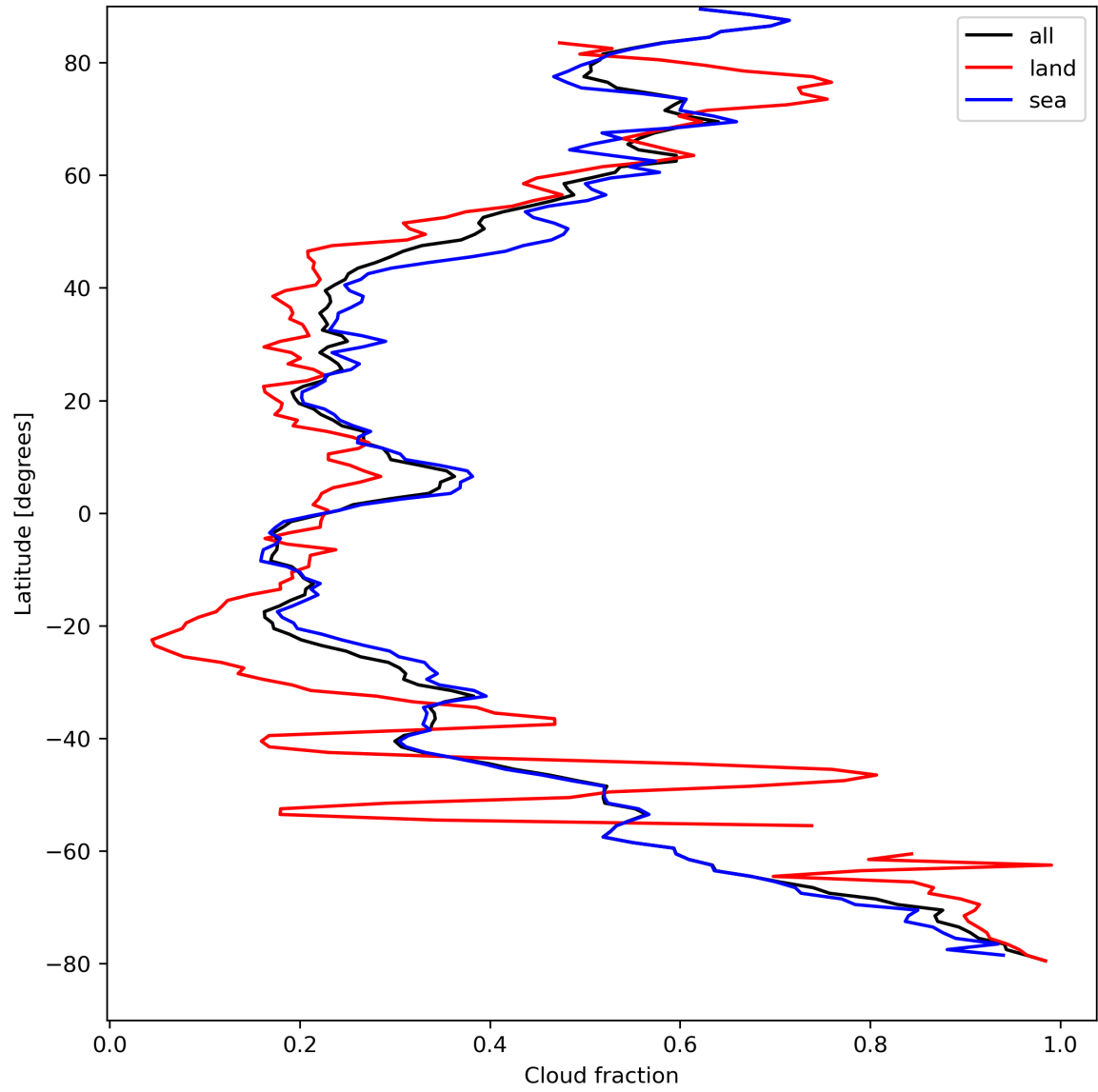
Figure 15: Zonal average of “Cloud fraction” for 2023-08-31 to 2023-09-02.
