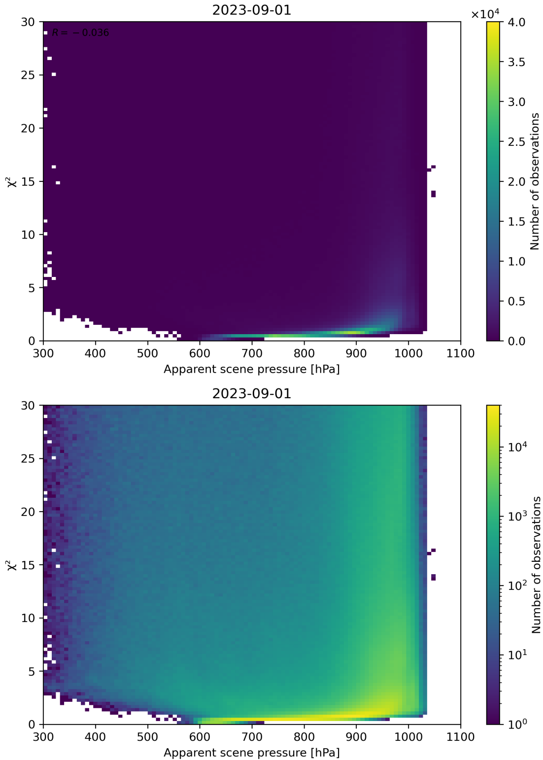
Figure 63: Scatter density plot of “Apparent scene pressure” against “ \chi^2 ” for 2023-08-31 to 2023-09-02.
