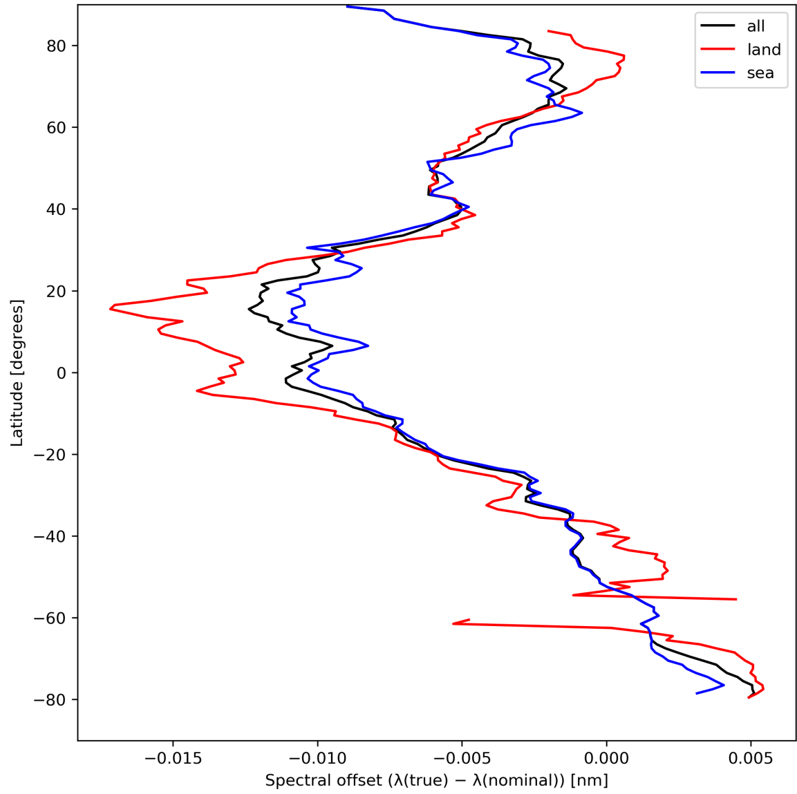
Figure 28: Zonal average of “Spectral offset ( \lambda(\text{true}) - \lambda(\text{nominal}) )” for 2023-08-31 to 2023-09-02.
