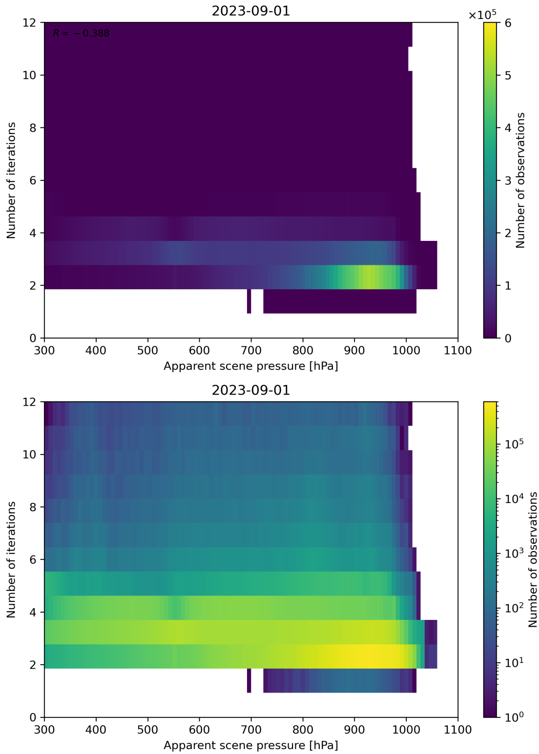
Figure 66: Scatter density plot of “Apparent scene pressure” against “Number of iterations” for 2023-08-31 to 2023-09-02.
