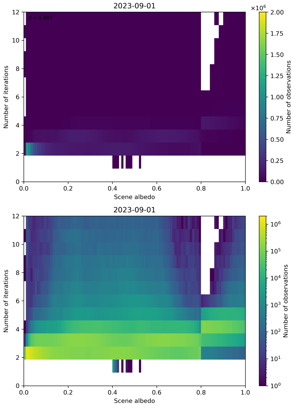
Figure 115: Scatter density plot of “Scene albedo” against “Number of iterations” for 2023-08-31 to 2023-09-02.
