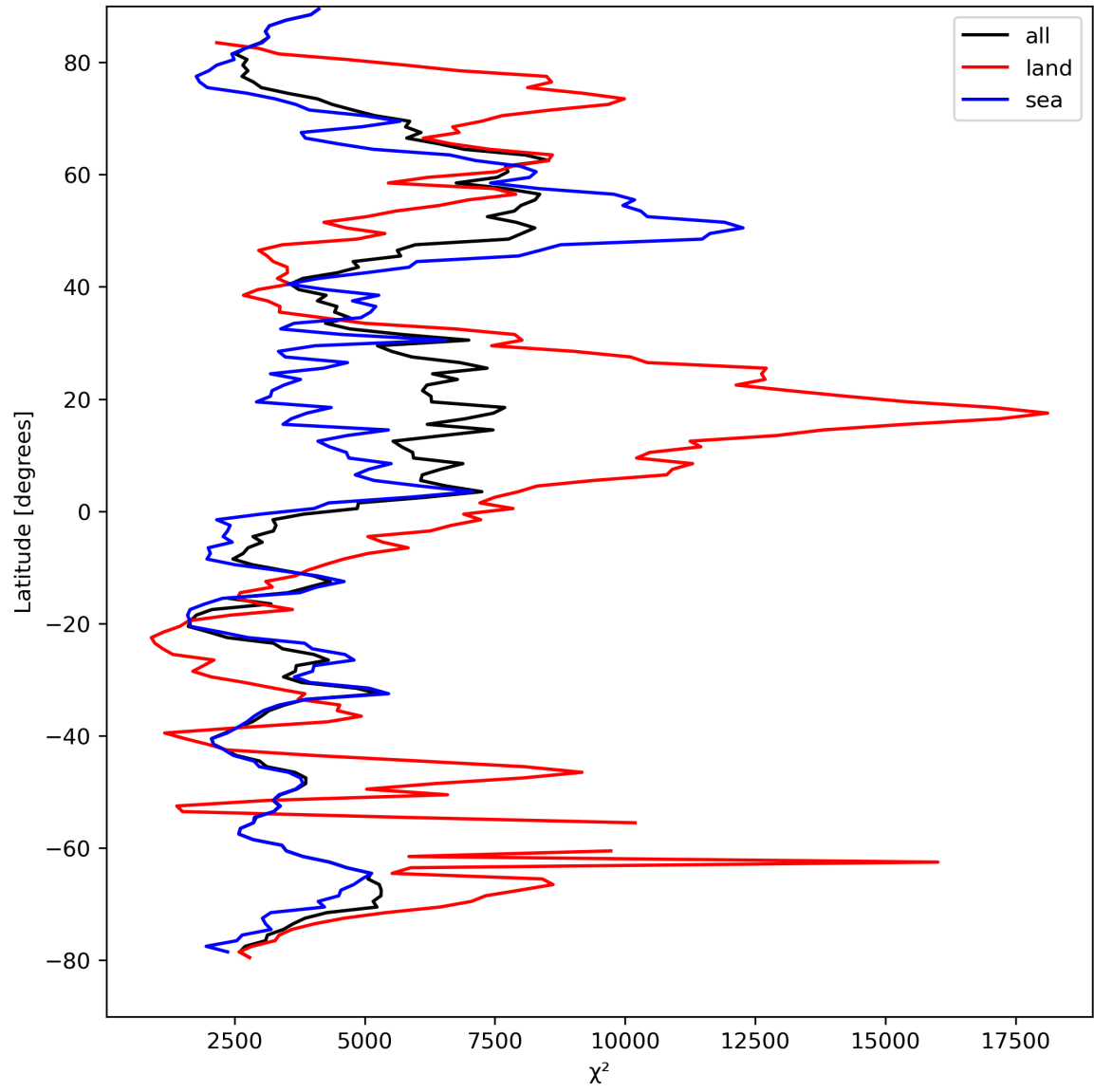
Figure 21: Zonal average of “ \chi^2 ” for 2023-08-31 to 2023-09-02.
