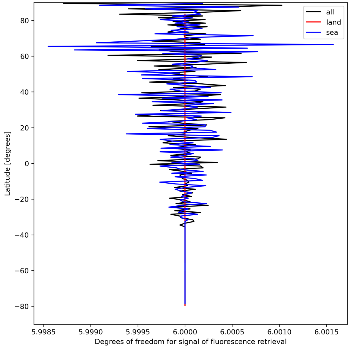
Figure 26: Zonal average of “Degrees of freedom for signal of fluorescence retrieval” for 2023-08-31 to 2023-09-02.
