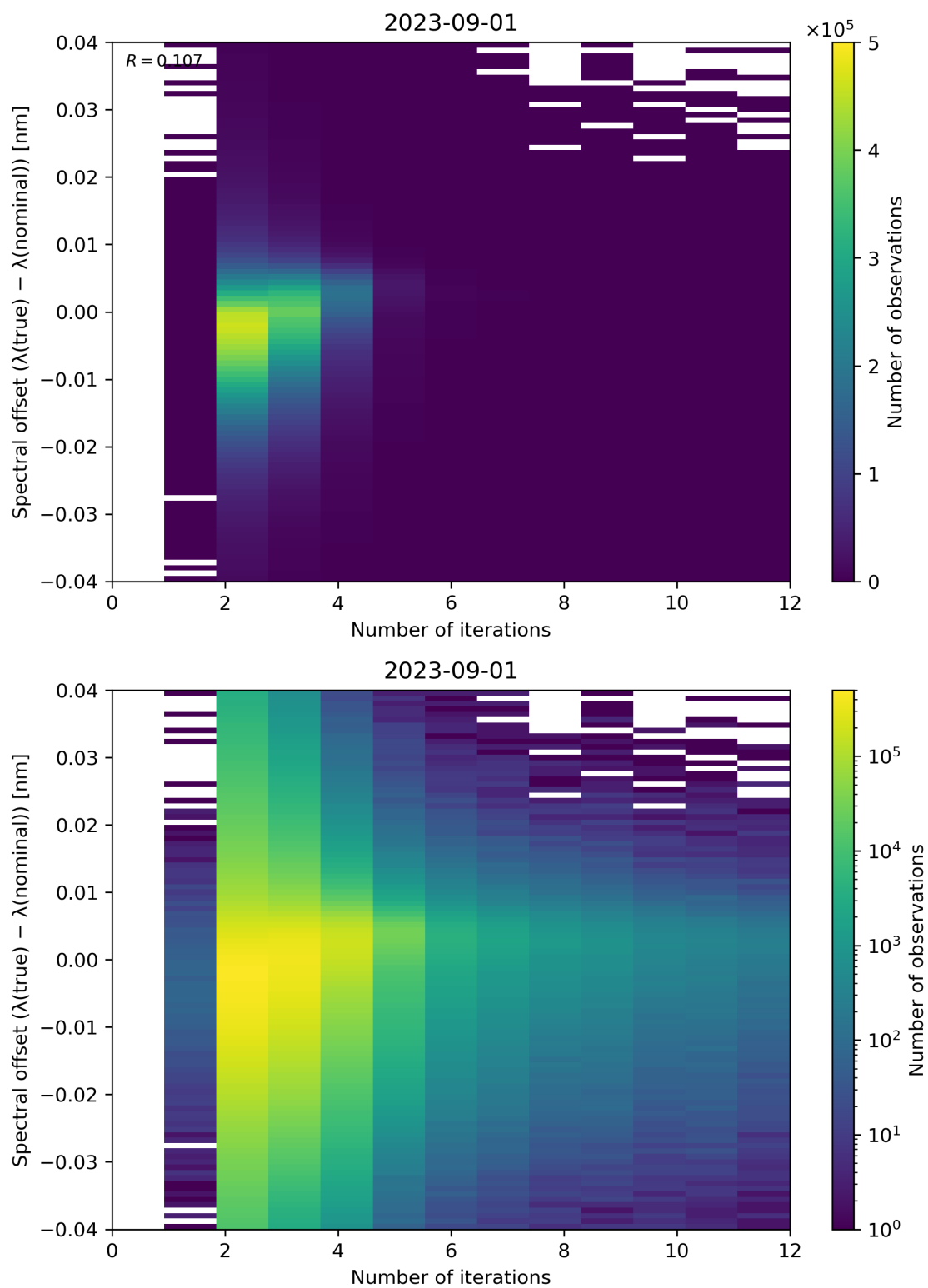
Figure 109: Scatter density plot of “Number of iterations” against “Spectral offset ( \lambda(\text{true}) - \lambda(\text{nominal}) )” for 2023-08-31 to 2023-09-02.
