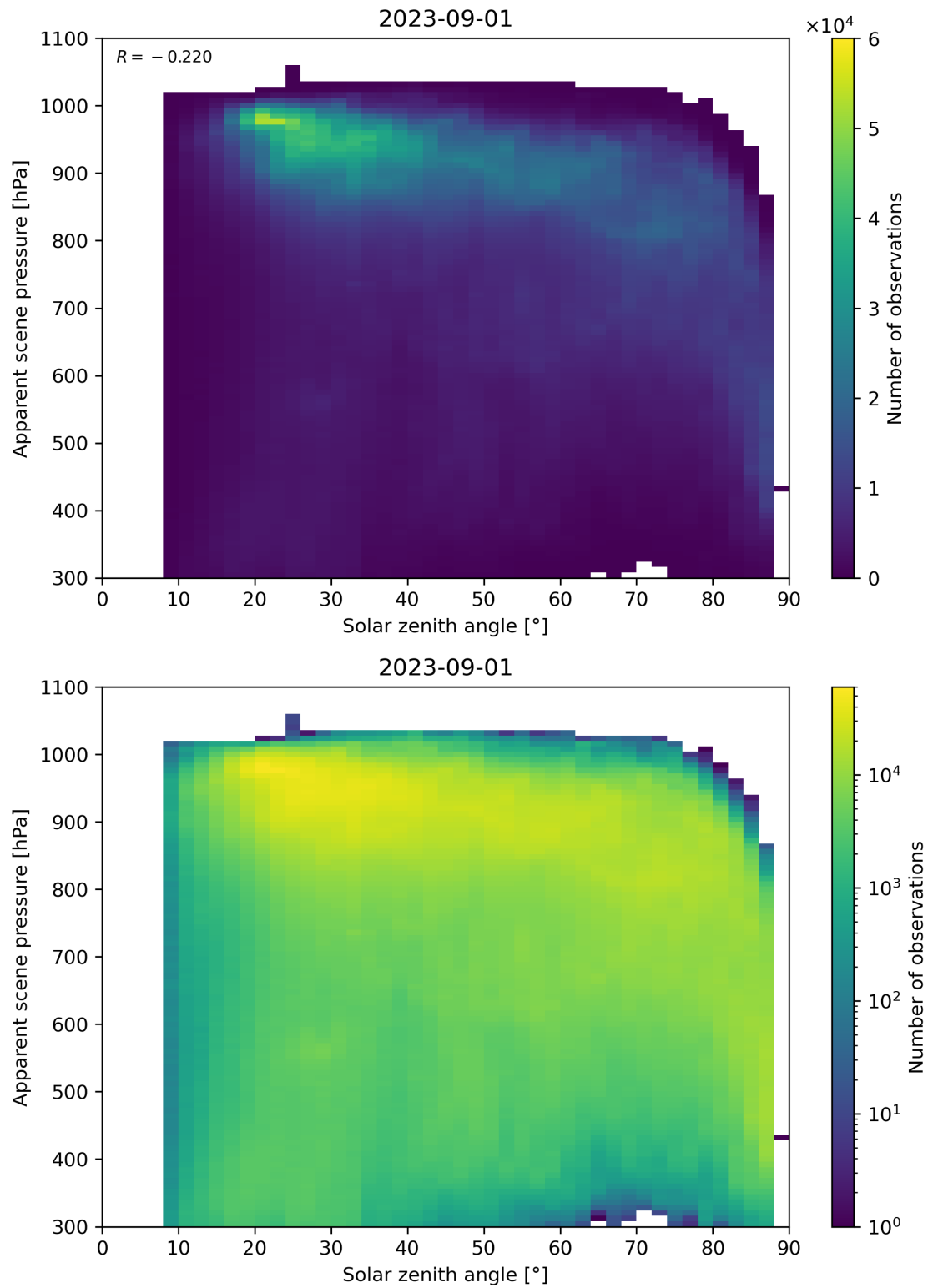
Figure 118: Scatter density plot of “Solar zenith angle” against “Apparent scene pressure” for 2023-08-31 to 2023-09-02.
