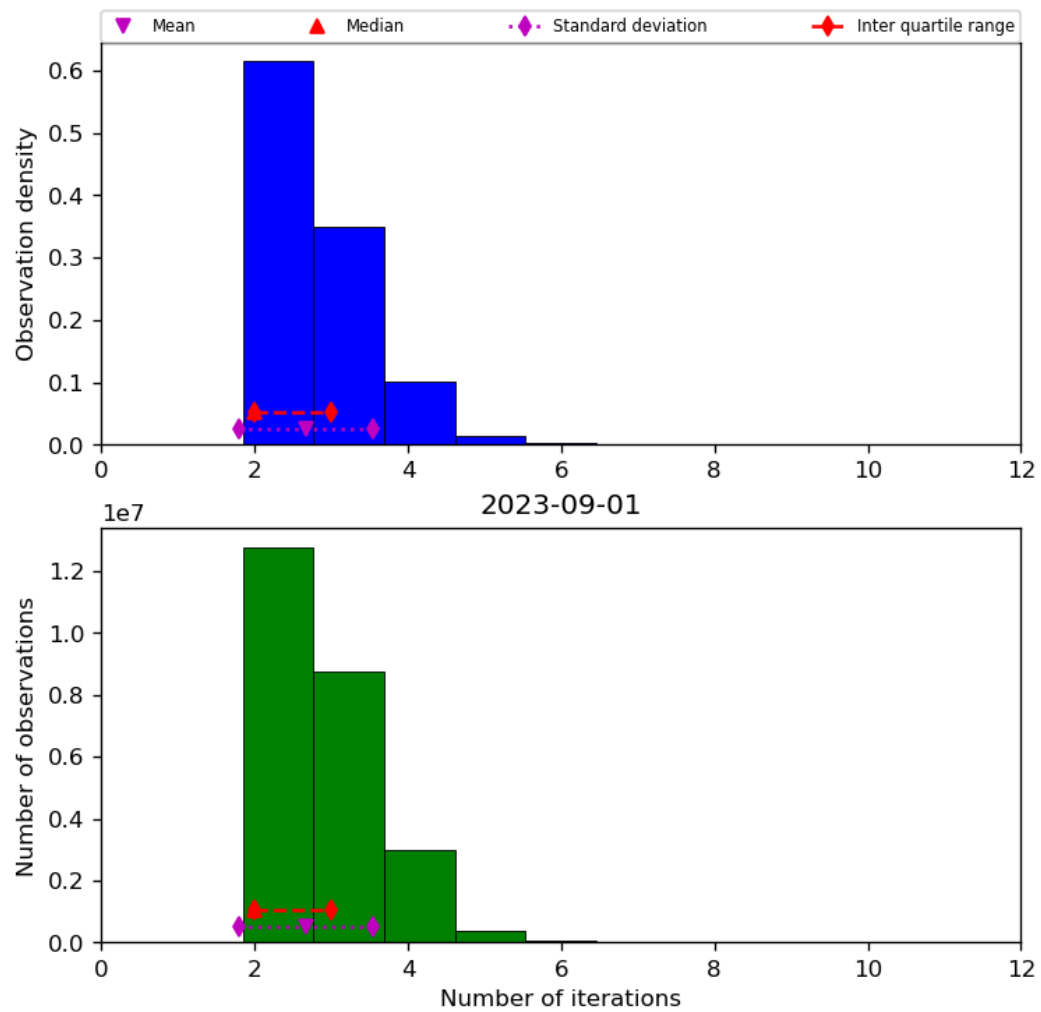
Figure 39: Histogram of “Number of iterations” for 2023-08-31 to 2023-09-02
