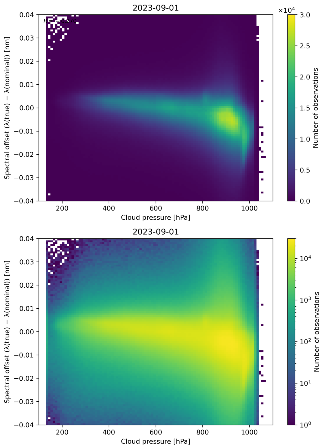
Figure 92: Scatter density plot of “Cloud pressure” against “Spectral offset ( \lambda(\text{true}) - \lambda(\text{nominal}) )” for 2023-08-31 to 2023-09-02.
