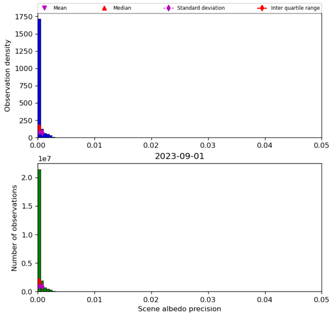
Figure 35: Histogram of “Scene albedo precision” for 2023-08-31 to 2023-09-02
