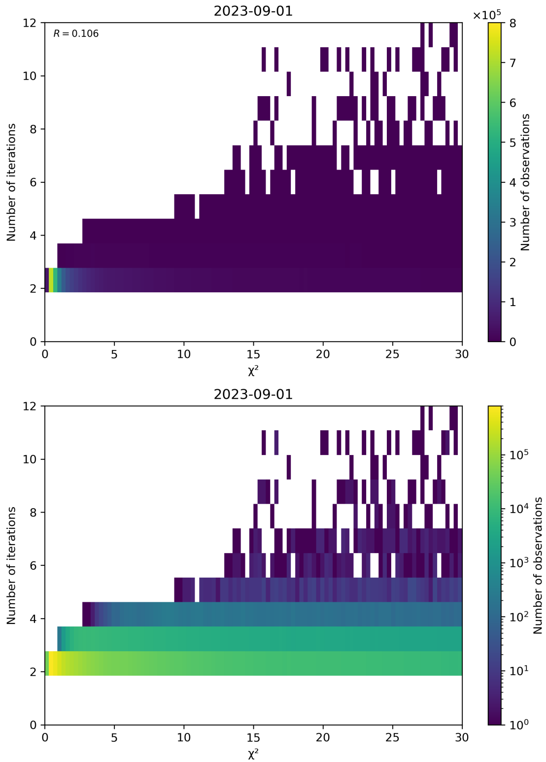
Figure 73: Scatter density plot of “ \chi^2 ” against “Number of iterations” for 2023-08-31 to 2023-09-02.
