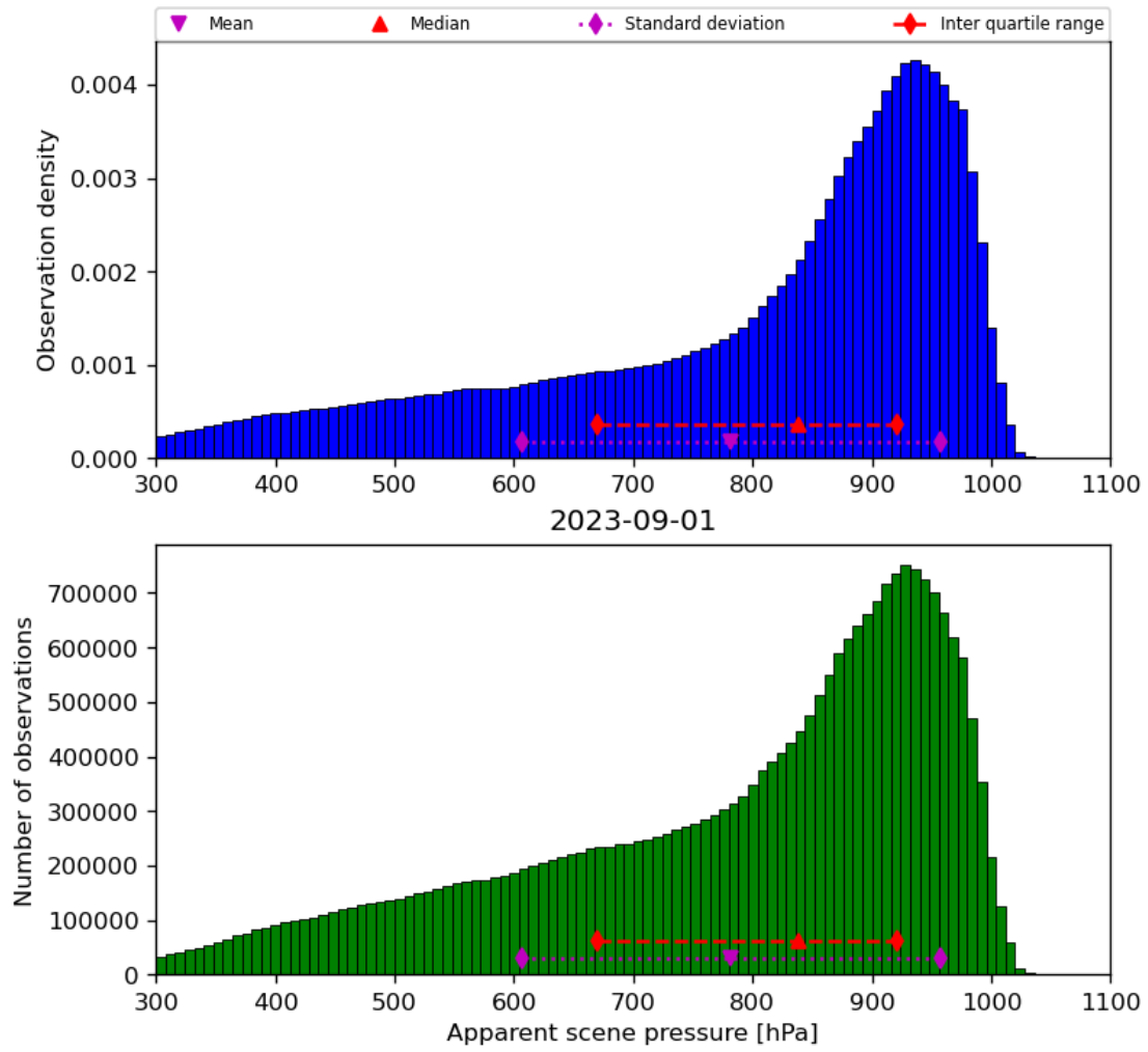
Figure 36: Histogram of “Apparent scene pressure” for 2023-08-31 to 2023-09-02
