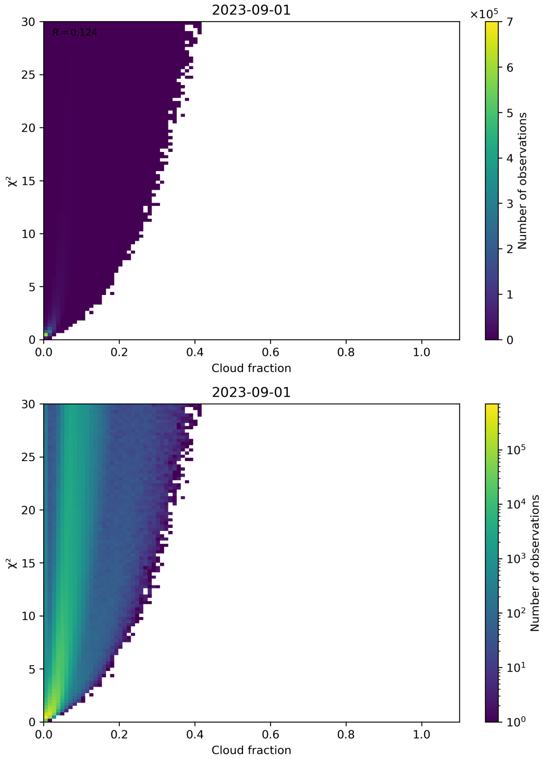
Figure 77: Scatter density plot of “Cloud fraction” against “ \chi^2 ” for 2023-08-31 to 2023-09-02.
