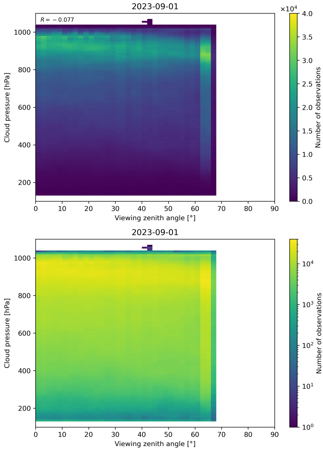
Figure 133: Scatter density plot of “Viewing zenith angle” against “Cloud pressure” for 2023-08-31 to 2023-09-02.
