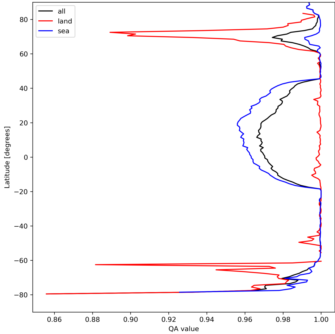
Figure 12: Zonal average of “QA value” for 2023-08-31 to 2023-09-02.
