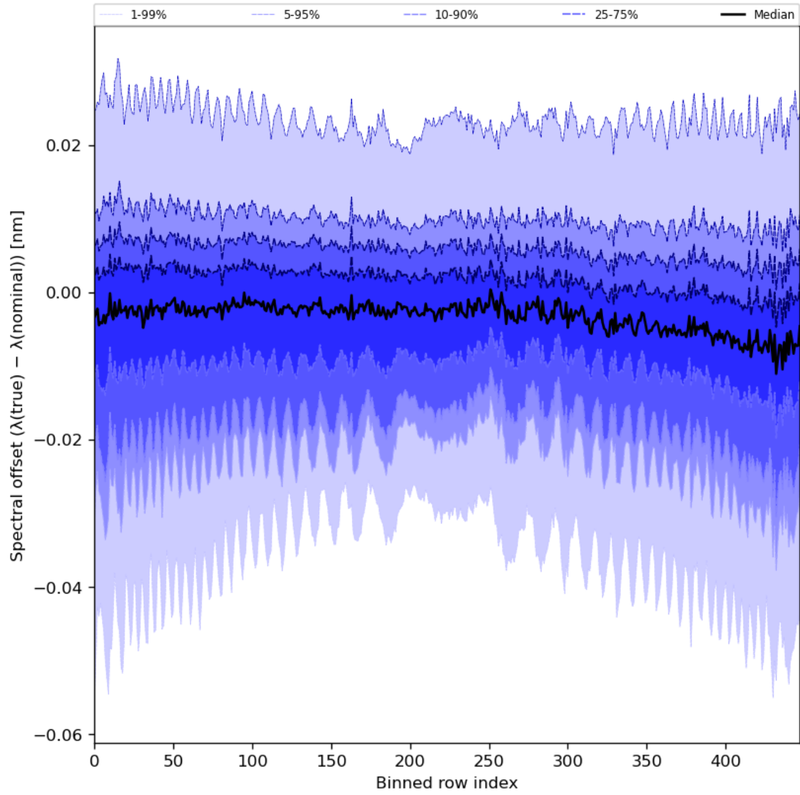
Figure 62: Along track statistics of “Spectral offset ( \lambda(\text{true}) - \lambda(\text{nominal}) )” for 2023-08-31 to 2023-09-02
