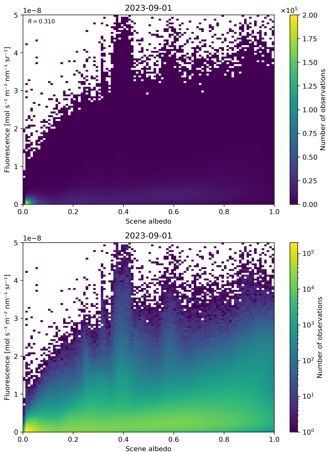
Figure 114: Scatter density plot of “Scene albedo” against “Fluorescence” for 2023-08-31 to 2023-09-02.
