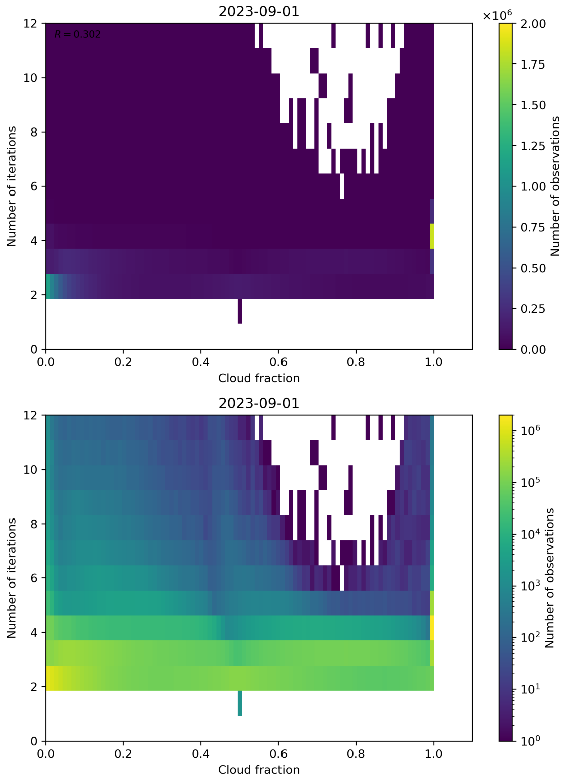
Figure 80: Scatter density plot of “Cloud fraction” against “Number of iterations” for 2023-08-31 to 2023-09-02.
