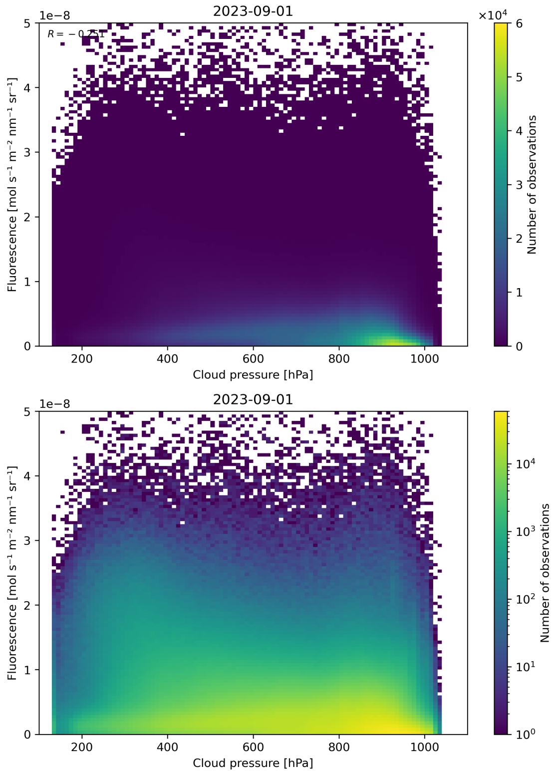
Figure 88: Scatter density plot of “Cloud pressure” against “Fluorescence” for 2023-08-31 to 2023-09-02.
