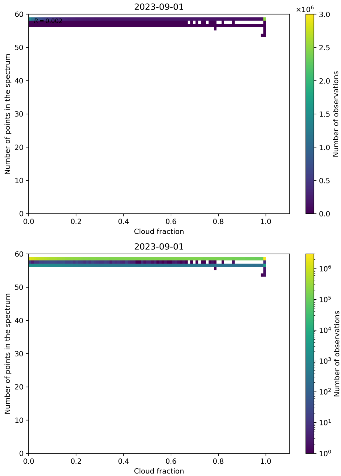
Figure 81: Scatter density plot of “Cloud fraction” against “Number of points in the spectrum” for 2023-08-31 to 2023-09-02.
