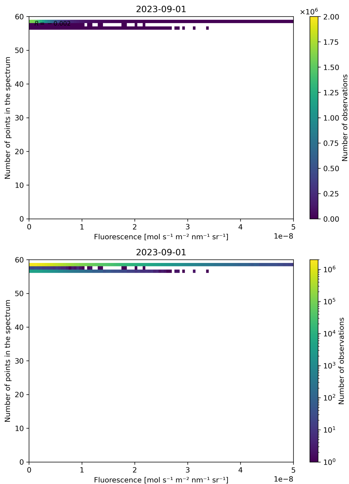
Figure 94: Scatter density plot of “Fluorescence” against “Number of points in the spectrum” for 2023-08-31 to 2023-09-02.
