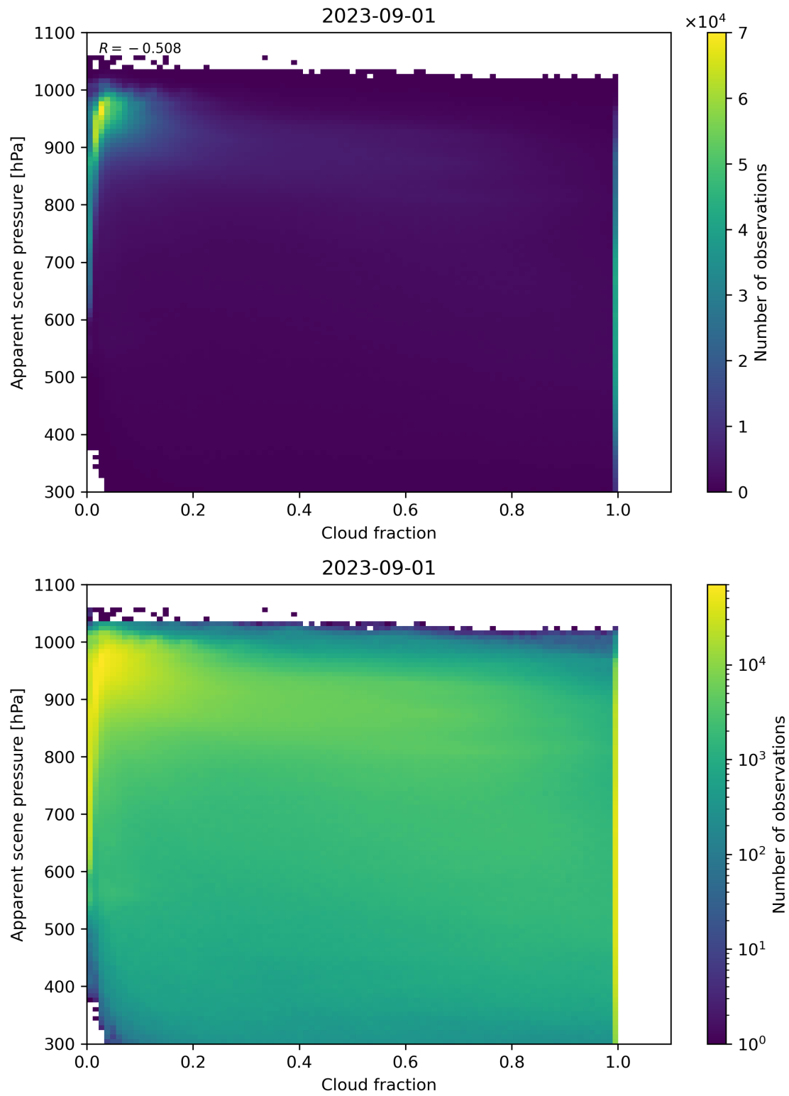
Figure 76: Scatter density plot of “Cloud fraction” against “Apparent scene pressure” for 2023-08-31 to 2023-09-02.
