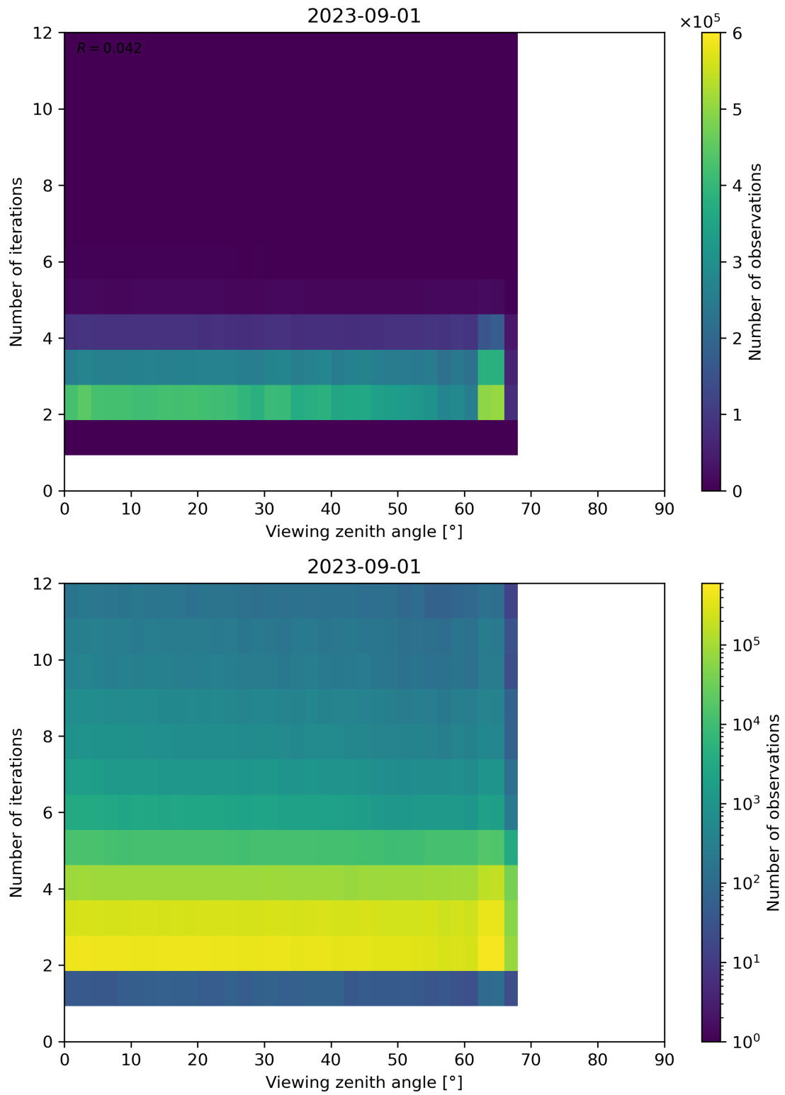
Figure 136: Scatter density plot of “Viewing zenith angle” against “Number of iterations” for 2023-08-31 to 2023-09-02.
