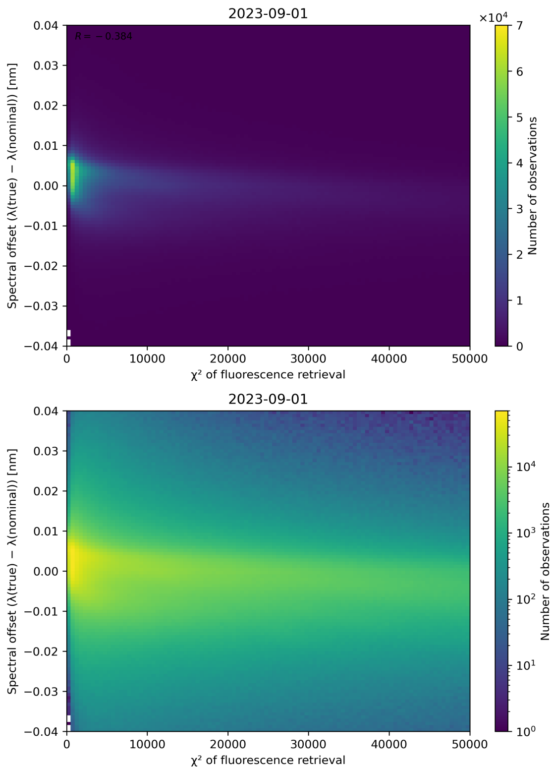
Figure 72: Scatter density plot of " \chi^2 of fluorescence retrieval" against "Spectral offset ( \lambda(\text{true}) - \lambda(\text{nominal}) )" for 2023-08-31 to 2023-09-02.
