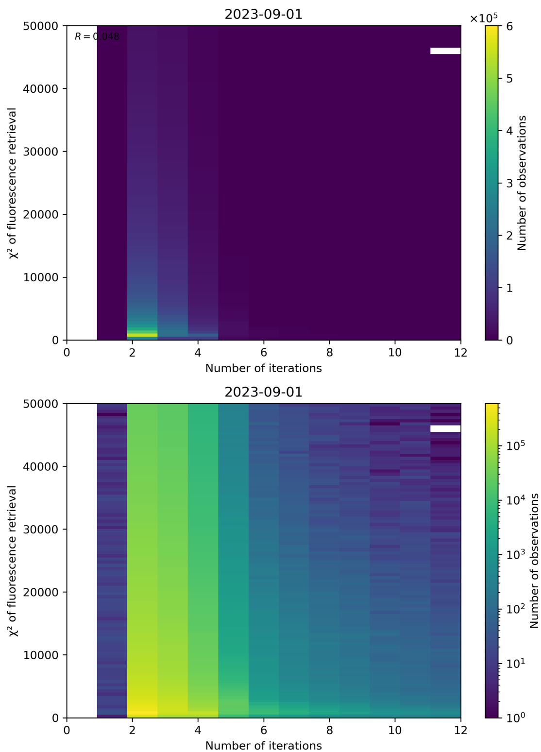
Figure 106: Scatter density plot of “Number of iterations” against “ \chi^2 of fluorescence retrieval” for 2023-08-31 to 2023-09-02.
