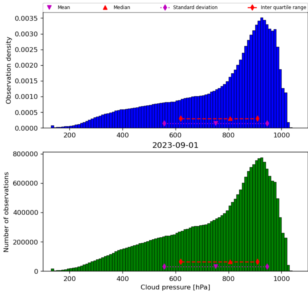
Figure 30: Histogram of “Cloud pressure” for 2023-08-31 to 2023-09-02
