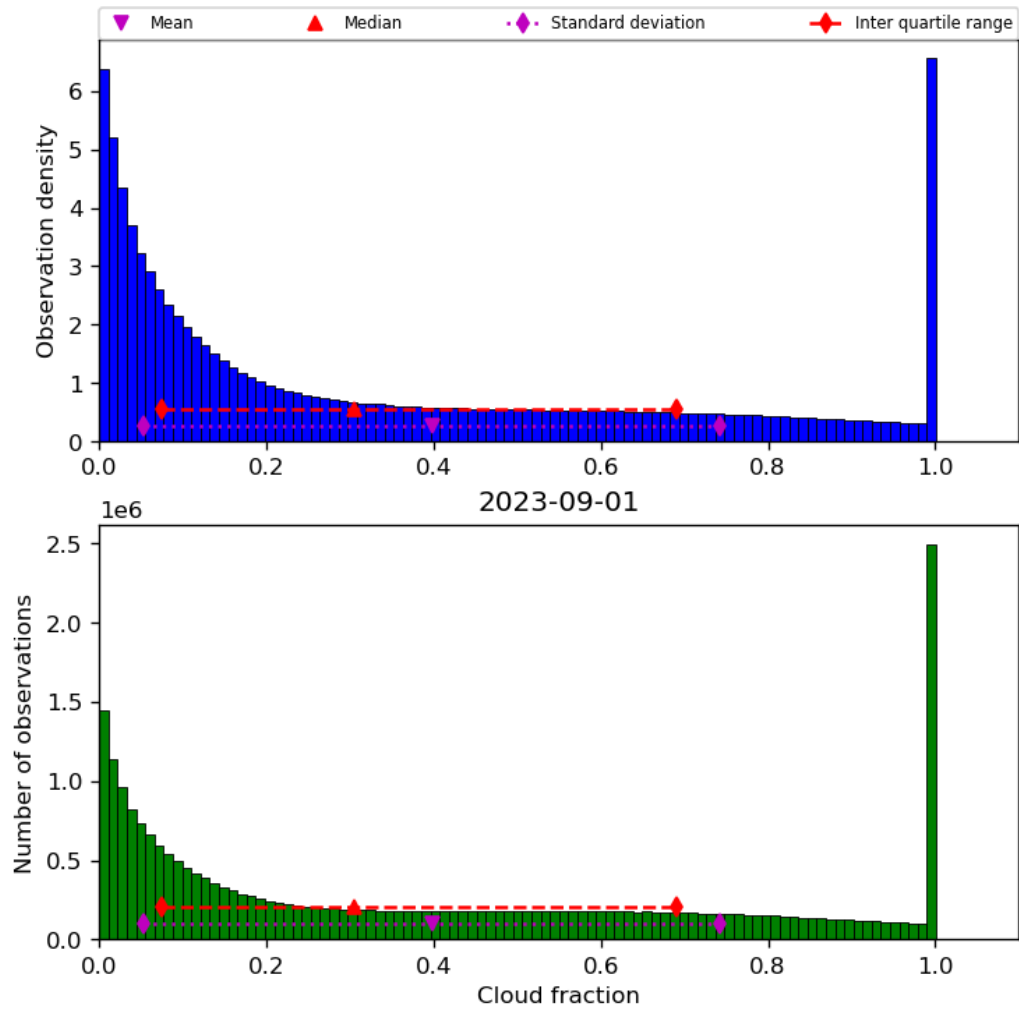
Figure 32: Histogram of “Cloud fraction” for 2023-08-31 to 2023-09-02
