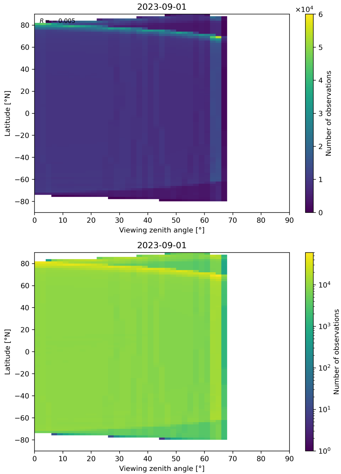
Figure 135: Scatter density plot of “Viewing zenith angle” against “Latitude” for 2023-08-31 to 2023-09-02.
