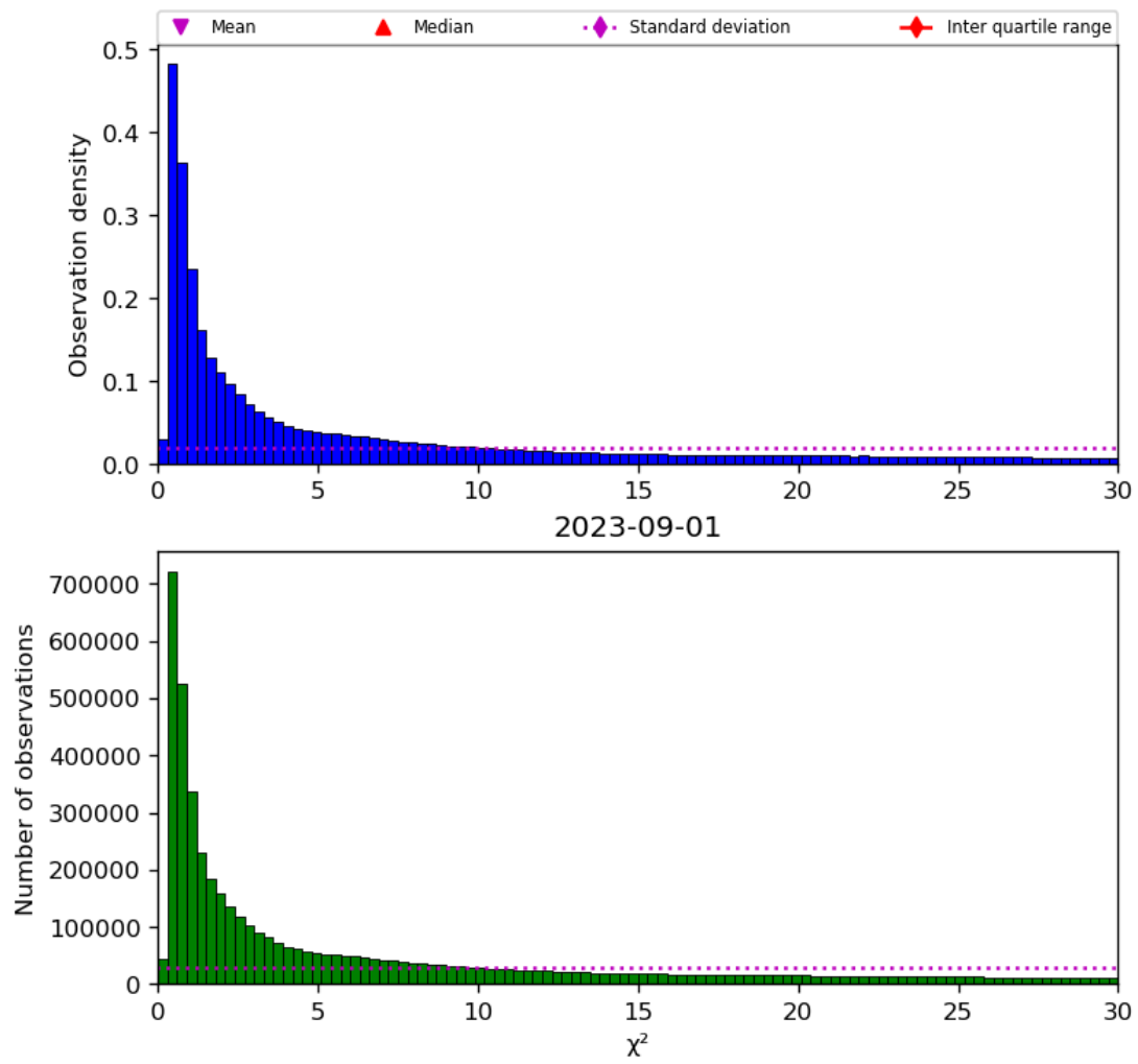
Figure 38: Histogram of “ \chi^2 ” for 2023-08-31 to 2023-09-02
