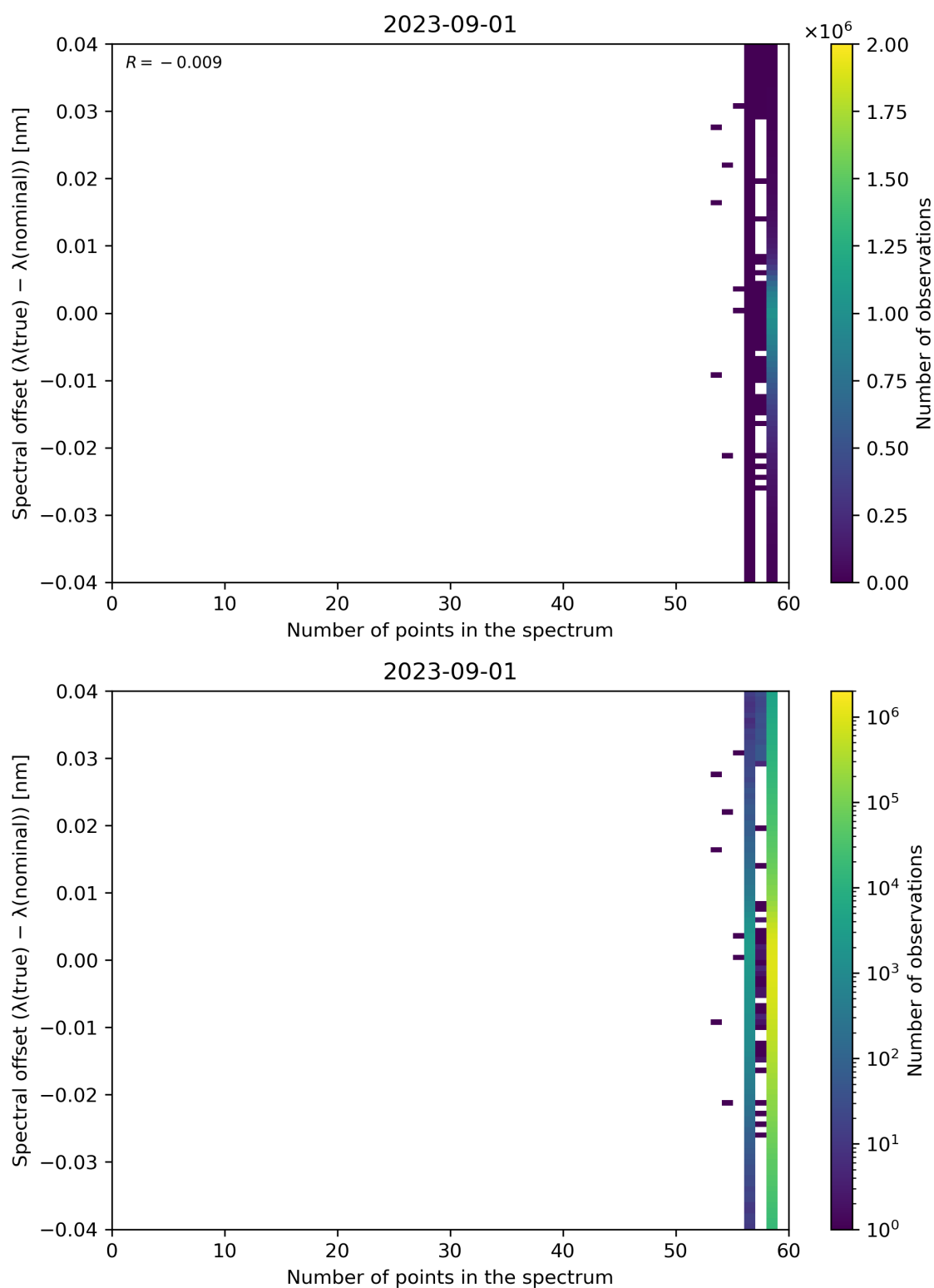
Figure 110: Scatter density plot of “Number of points in the spectrum” against “Spectral offset ( \lambda(\text{true}) - \lambda(\text{nominal}) )” for 2023-08-31 to 2023-09-02.
