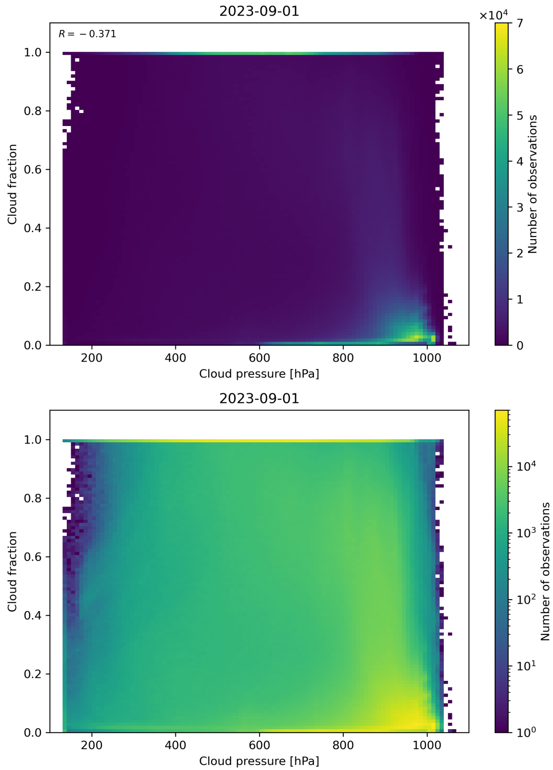
Figure 87: Scatter density plot of “Cloud pressure” against “Cloud fraction” for 2023-08-31 to 2023-09-02.
