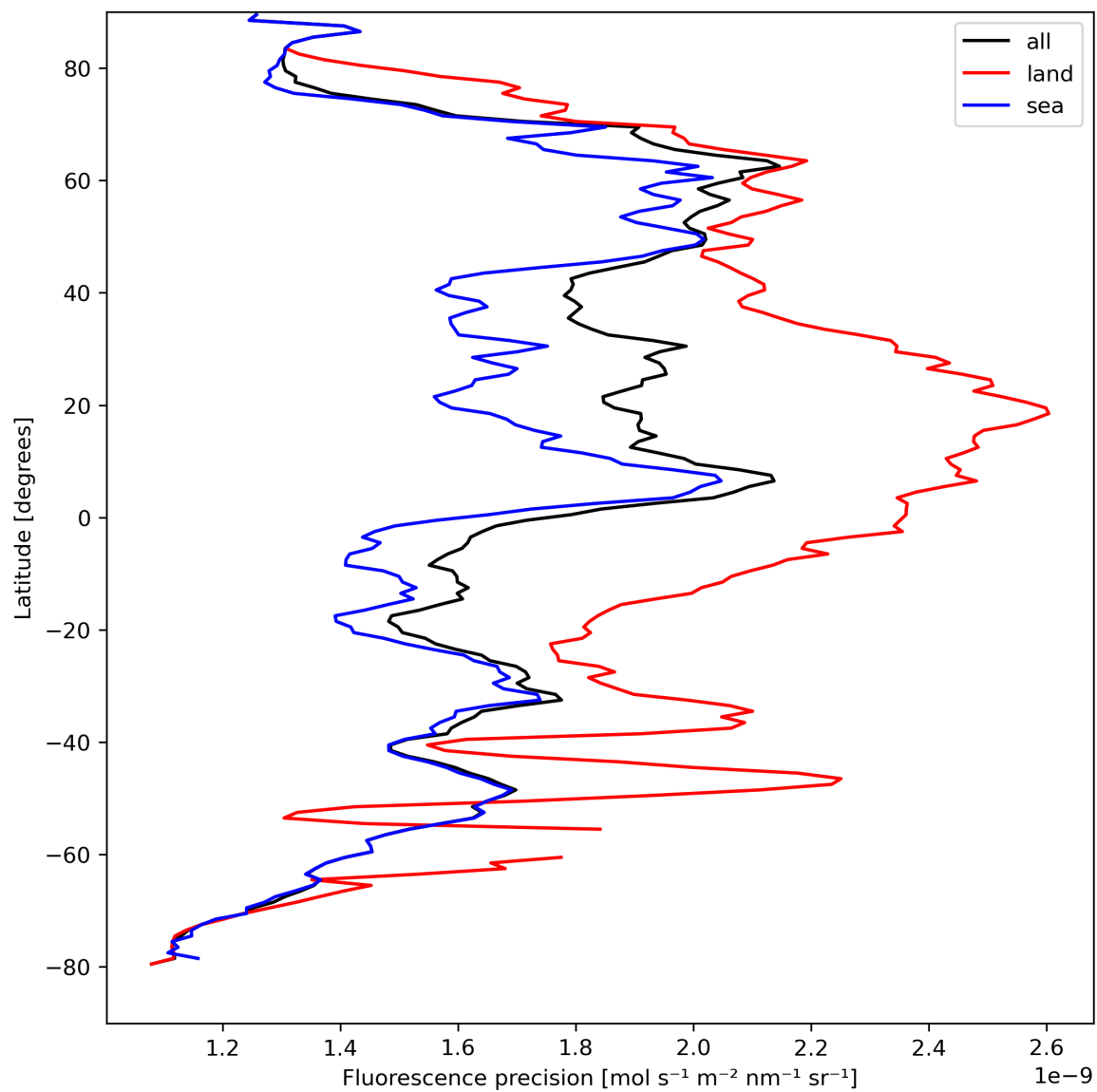
Figure 24: Zonal average of “Fluorescence precision” for 2023-08-31 to 2023-09-02.
