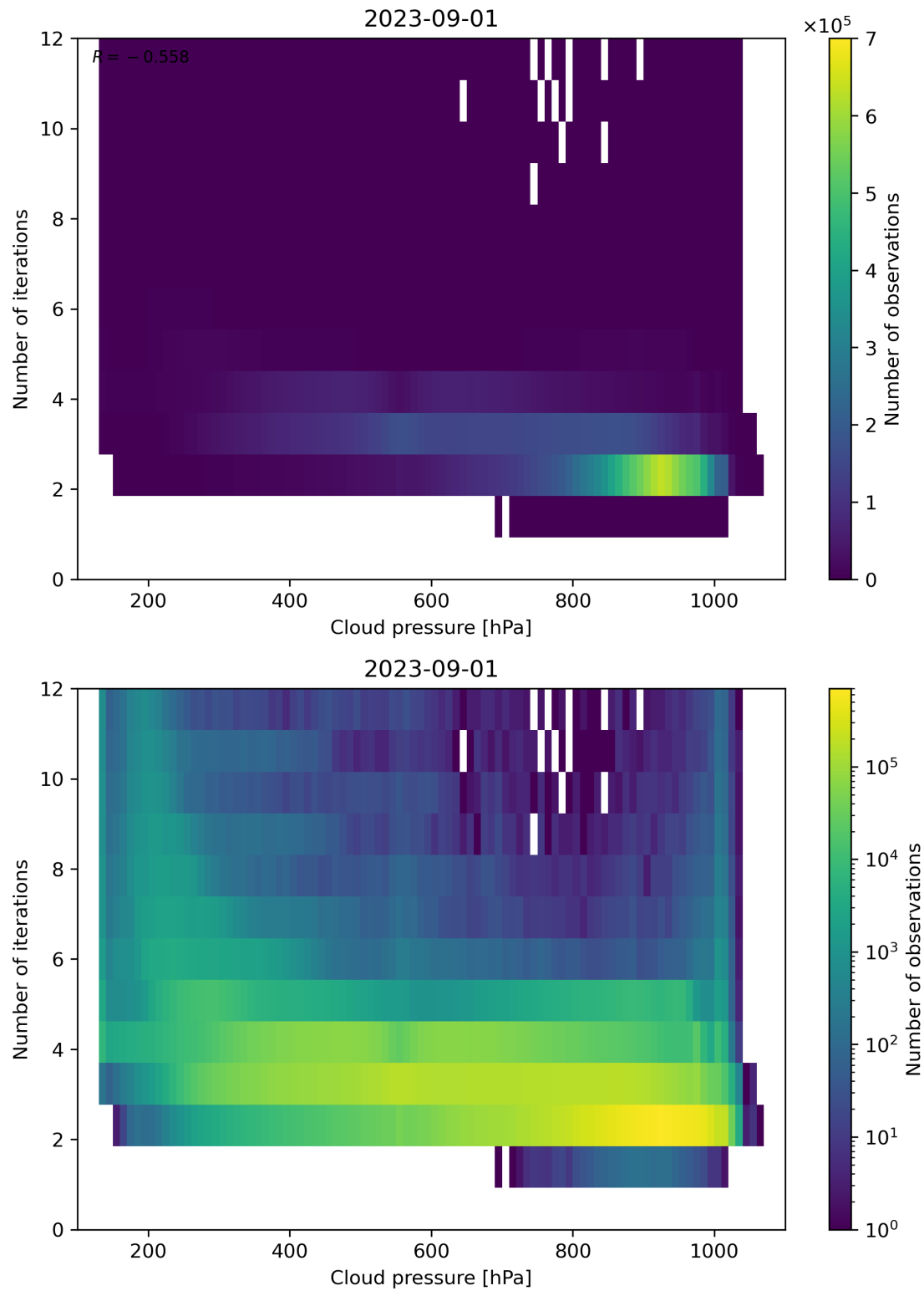
Figure 89: Scatter density plot of “Cloud pressure” against “Number of iterations” for 2023-08-31 to 2023-09-02.
