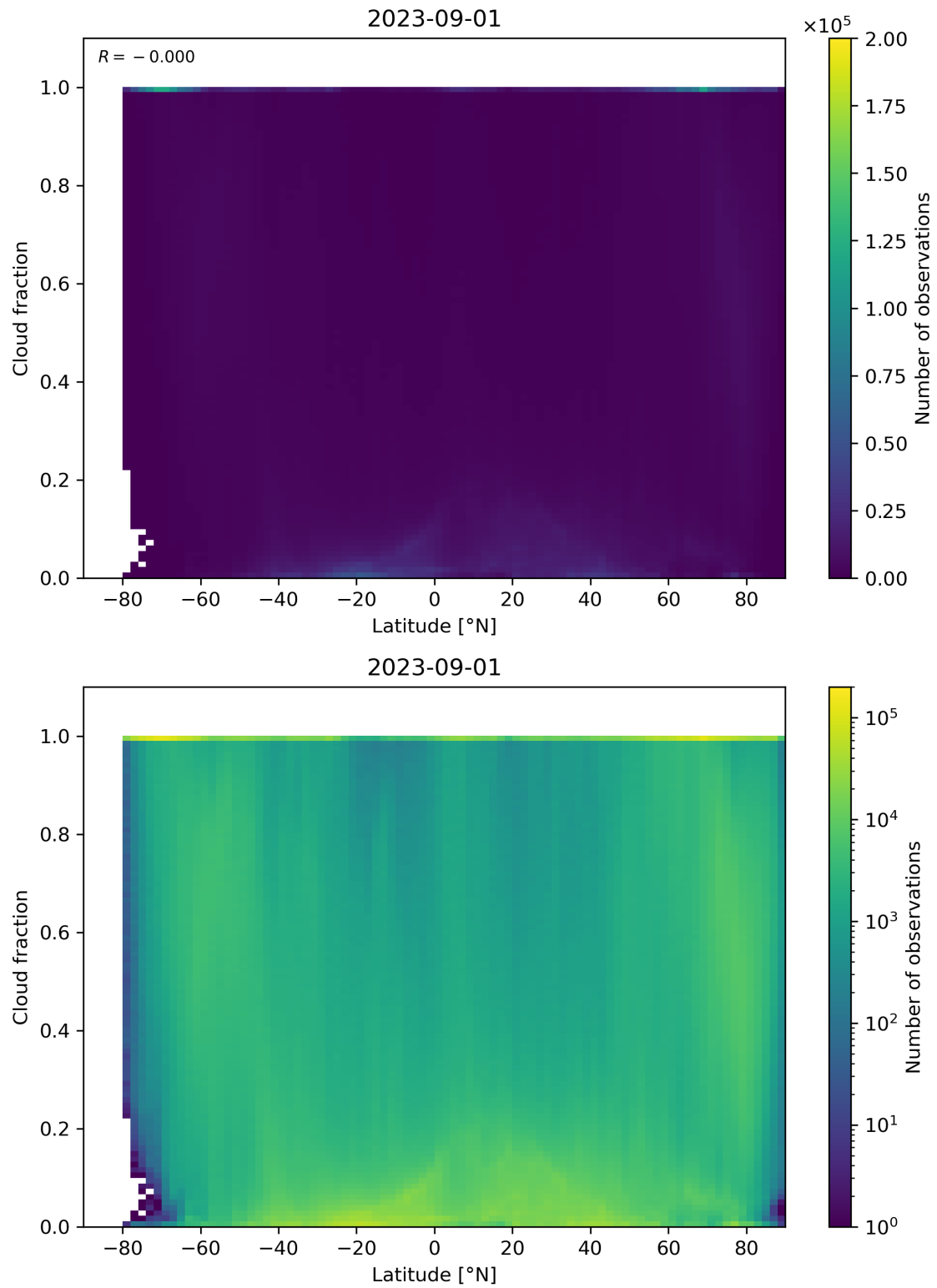
Figure 99: Scatter density plot of “Latitude” against “Cloud fraction” for 2023-08-31 to 2023-09-02.
