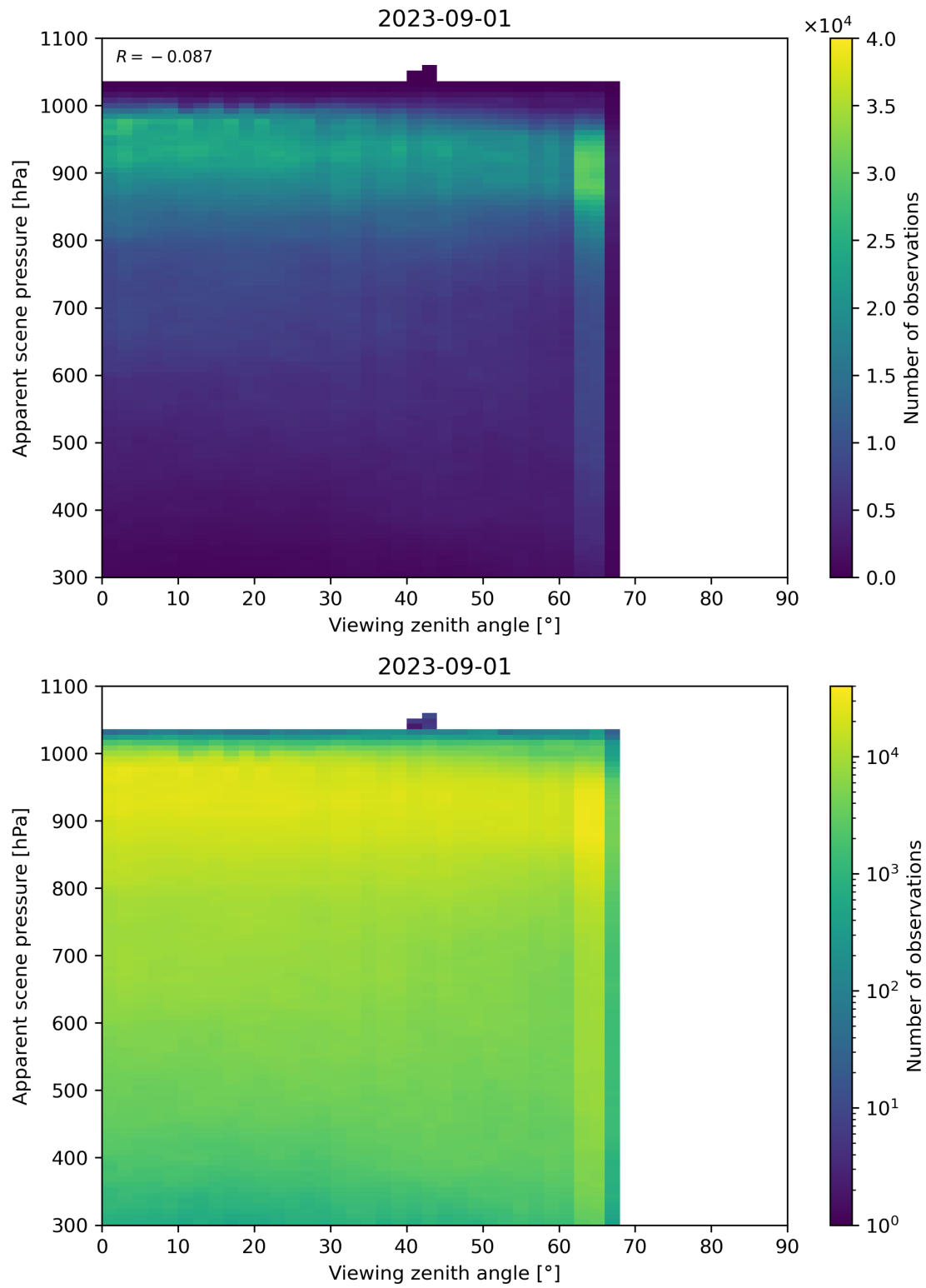
Figure 129: Scatter density plot of “Viewing zenith angle” against “Apparent scene pressure” for 2023-08-31 to 2023-09-02.
