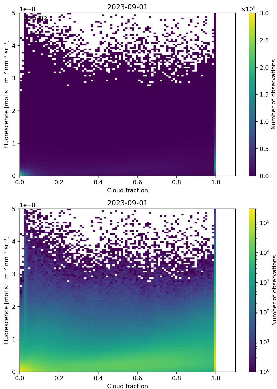
Figure 79: Scatter density plot of “Cloud fraction” against “Fluorescence” for 2023-08-31 to 2023-09-02.
