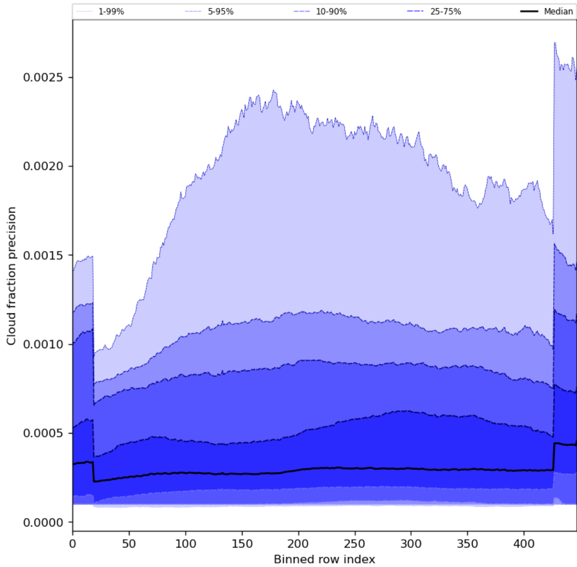
Figure 50: Along track statistics of “Cloud fraction precision” for 2023-08-31 to 2023-09-02
