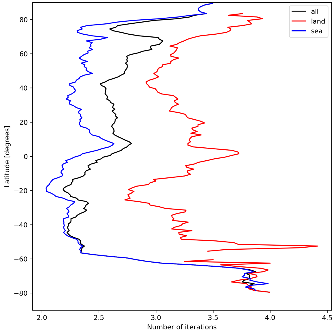
Figure 22: Zonal average of “Number of iterations” for 2023-08-31 to 2023-09-02.
