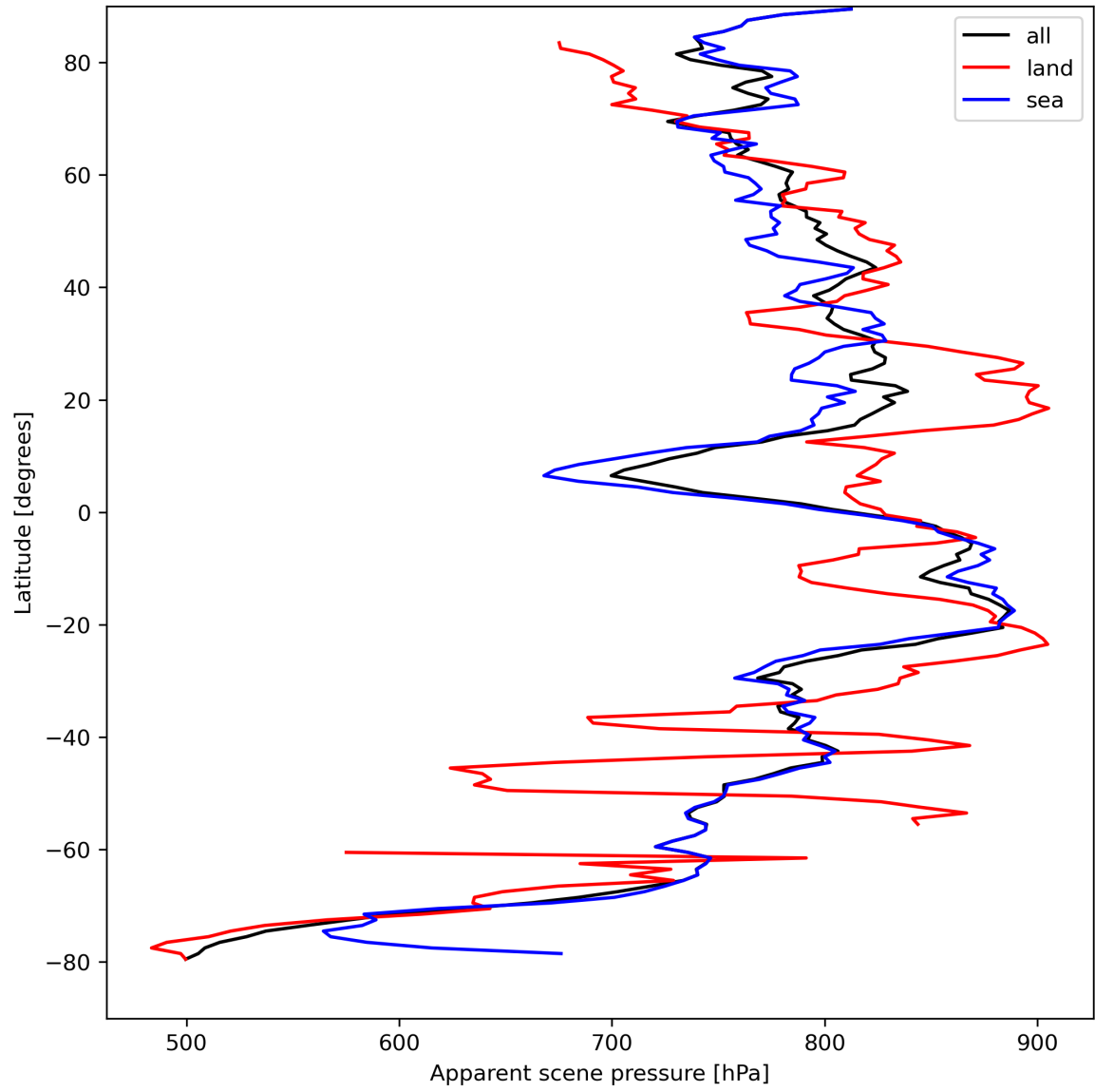
Figure 19: Zonal average of “Apparent scene pressure” for 2023-08-31 to 2023-09-02.
