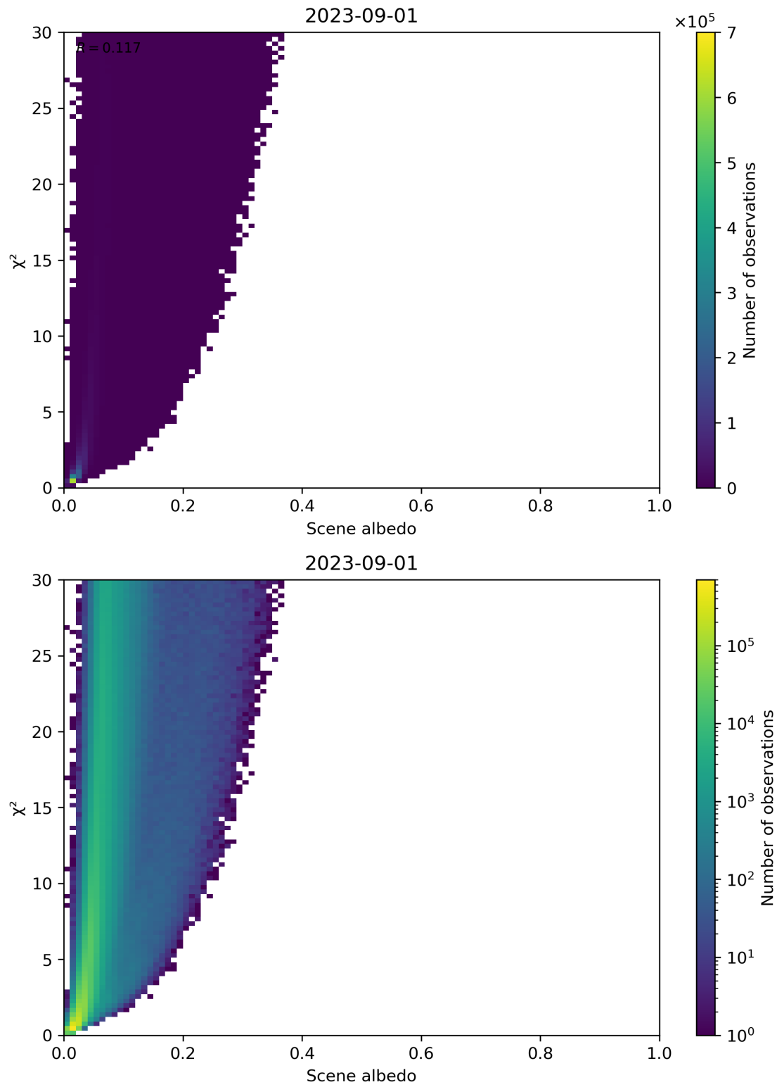
Figure 112: Scatter density plot of “Scene albedo” against “ \chi^2 ” for 2023-08-31 to 2023-09-02.
