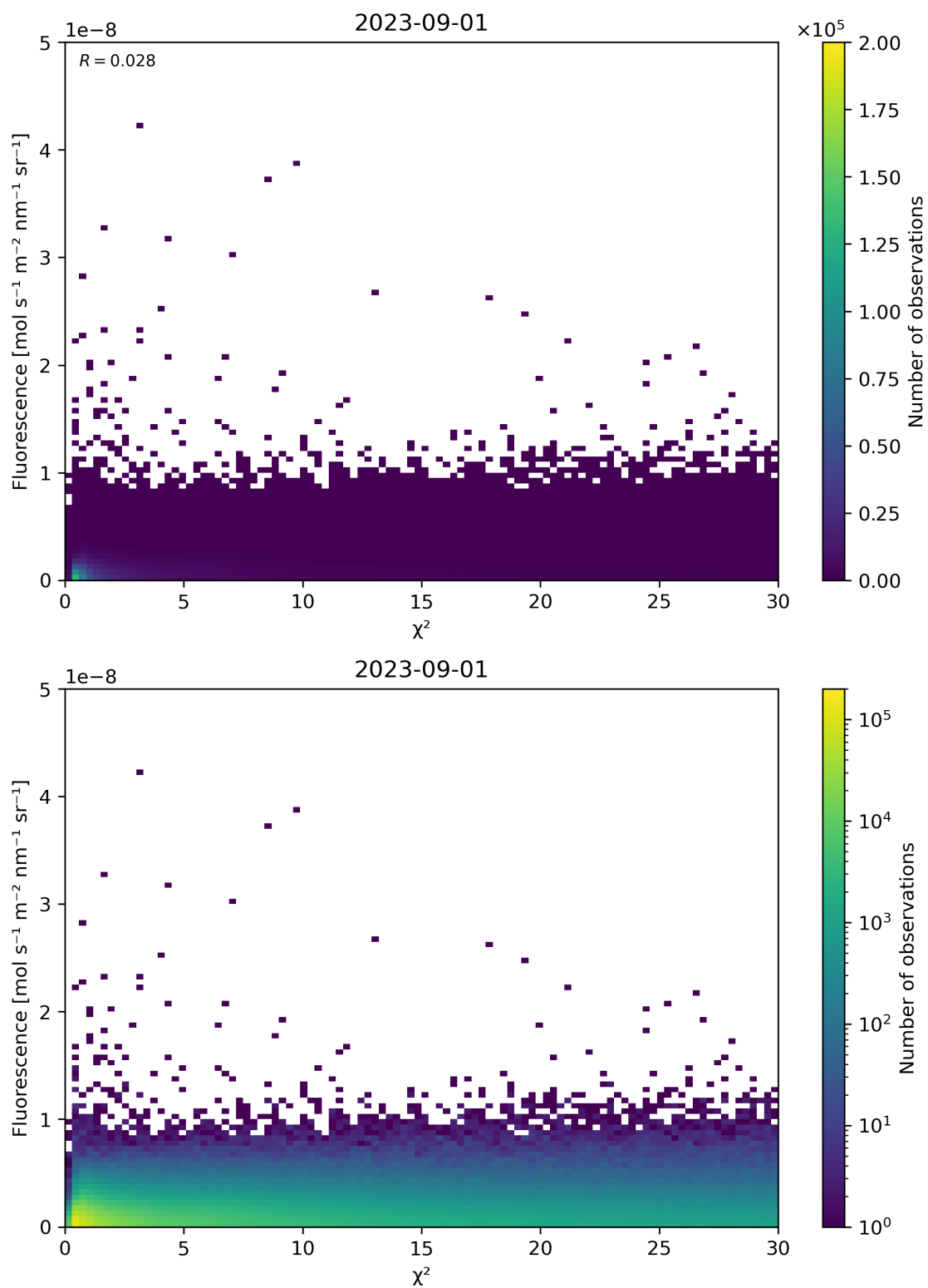
Figure 70: Scatter density plot of “ \chi^2 ” against “Fluorescence” for 2023-08-31 to 2023-09-02.
