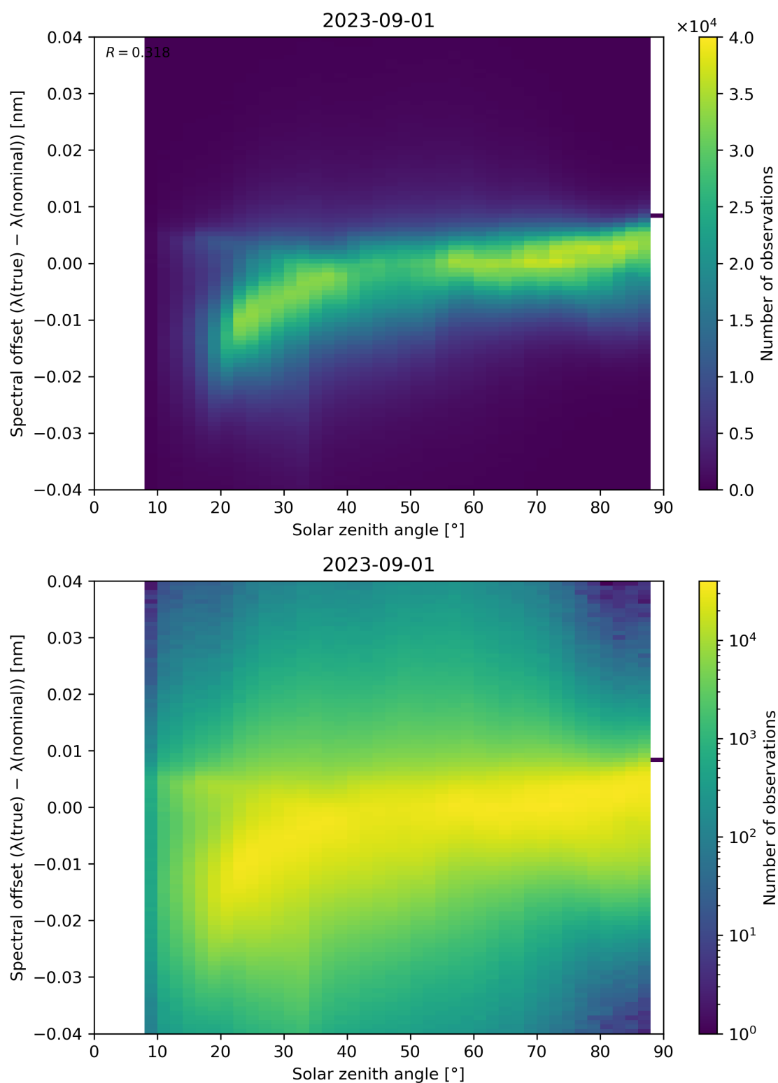
Figure 128: Scatter density plot of “Solar zenith angle” against “Spectral offset ( \lambda(\text{true}) - \lambda(\text{nominal}) )” for 2023-08-31 to 2023-09-02.
