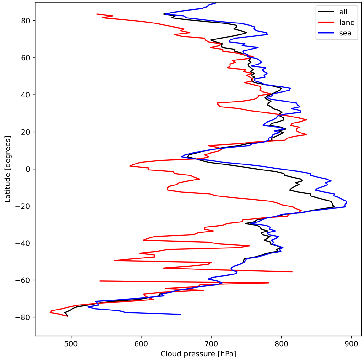
Figure 13: Zonal average of “Cloud pressure” for 2023-08-31 to 2023-09-02.
