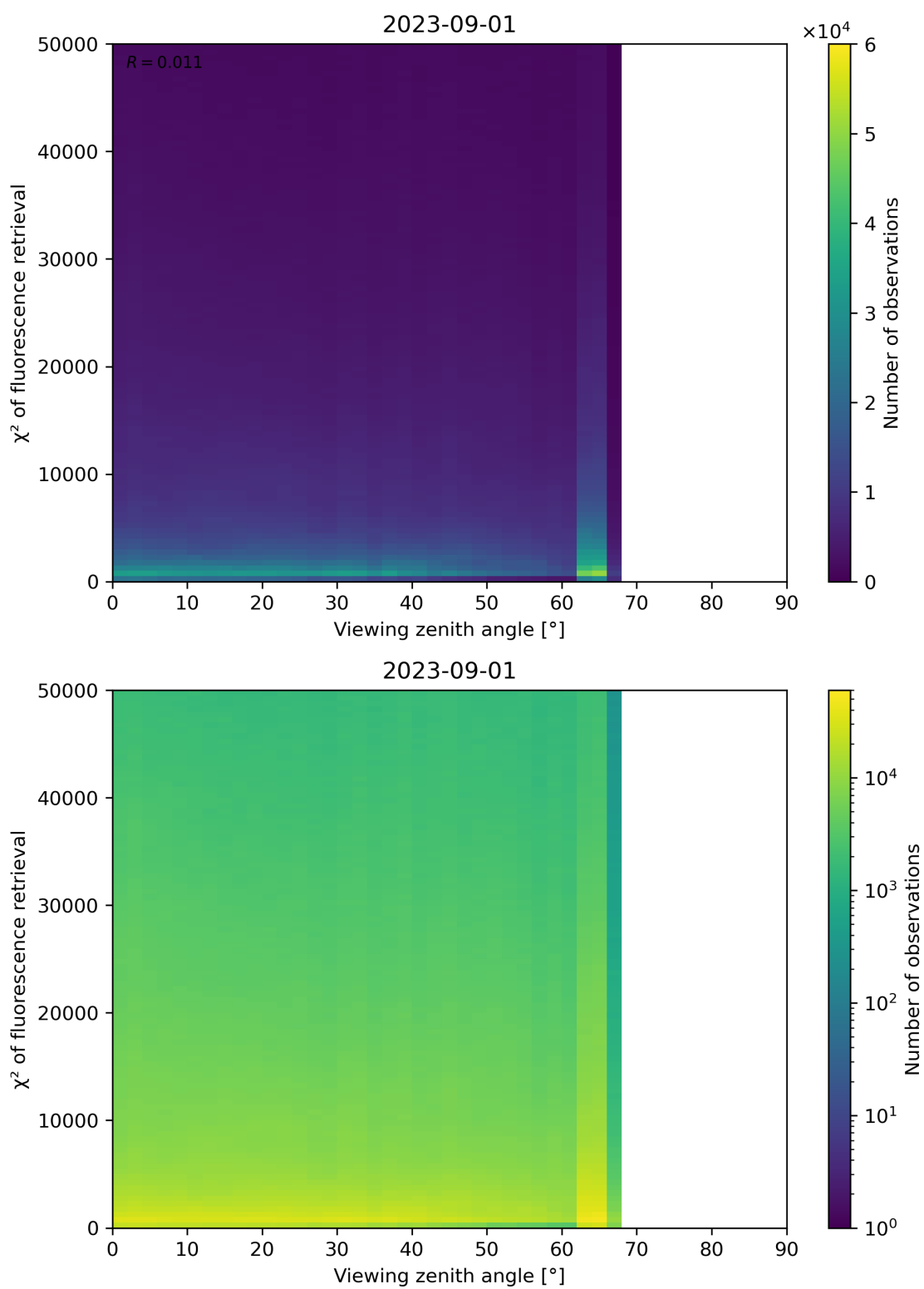
Figure 131: Scatter density plot of “Viewing zenith angle” against “ \chi^2 of fluorescence retrieval” for 2023-08-31 to 2023-09-02.
