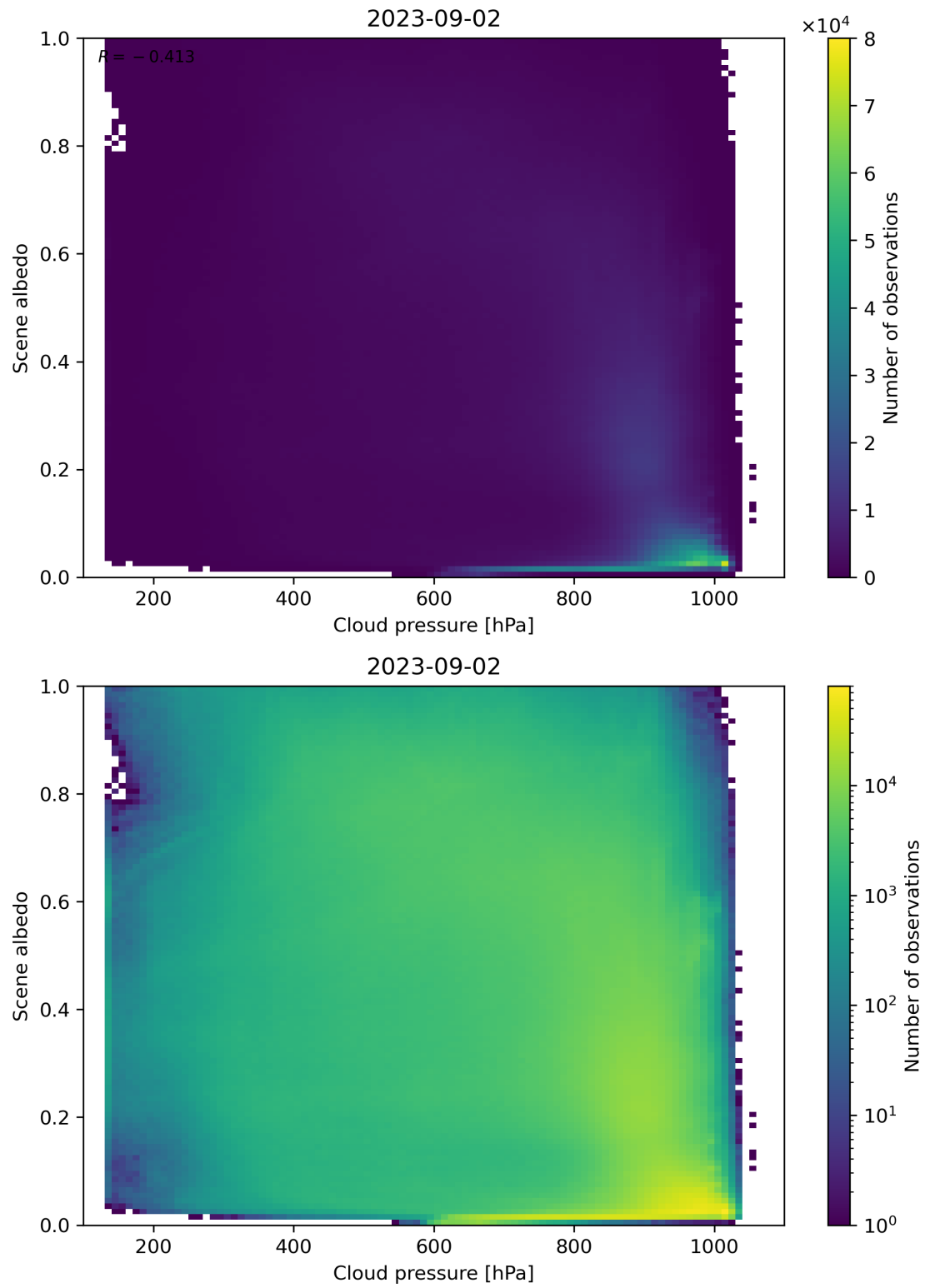
Figure 91: Scatter density plot of “Cloud pressure” against “Scene albedo” for 2023-09-01 to 2023-09-03.
