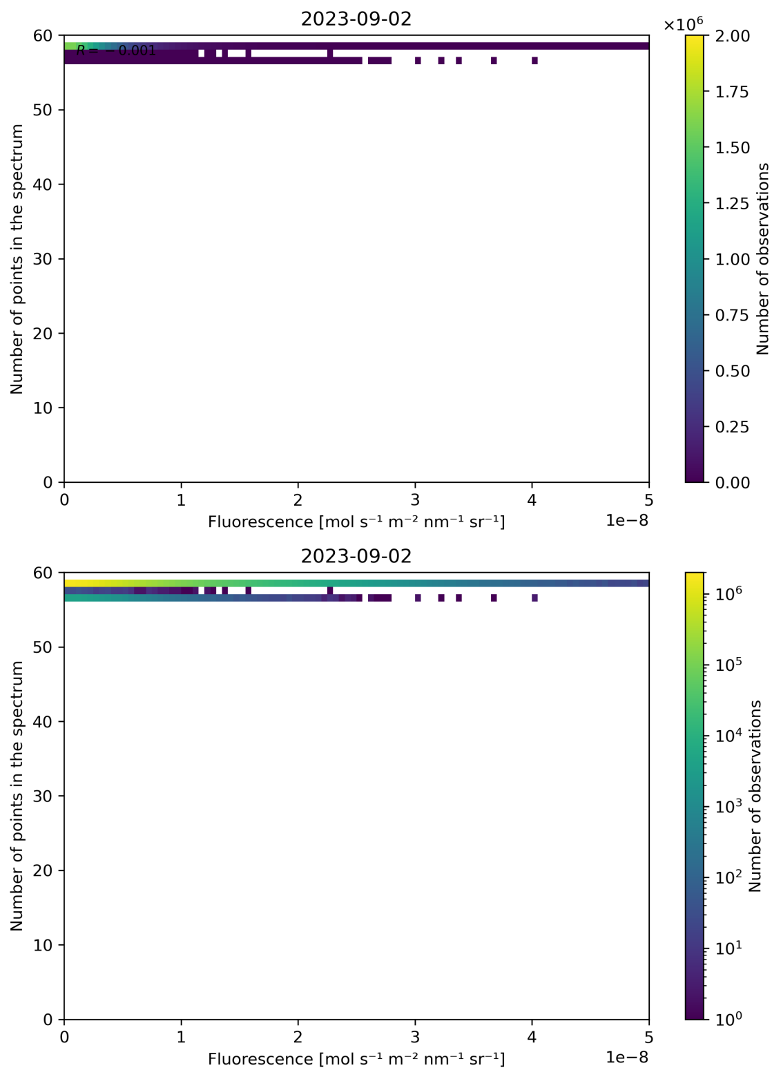
Figure 94: Scatter density plot of “Fluorescence” against “Number of points in the spectrum” for 2023-09-01 to 2023-09-03.
