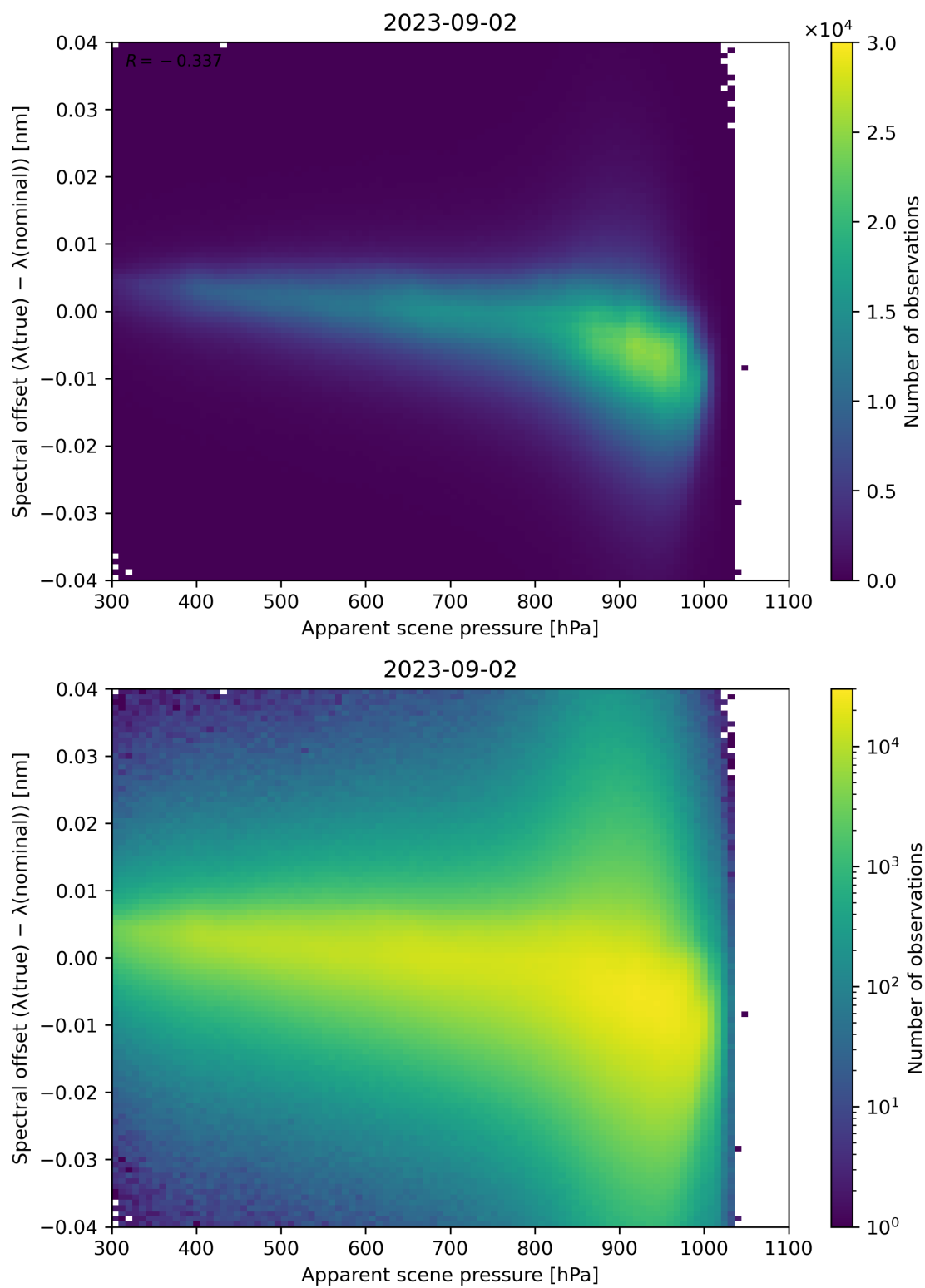
Figure 68: Scatter density plot of “Apparent scene pressure” against “Spectral offset ( \lambda(\text{true}) - \lambda(\text{nominal}) )” for 2023-09-01 to 2023-09-03.
