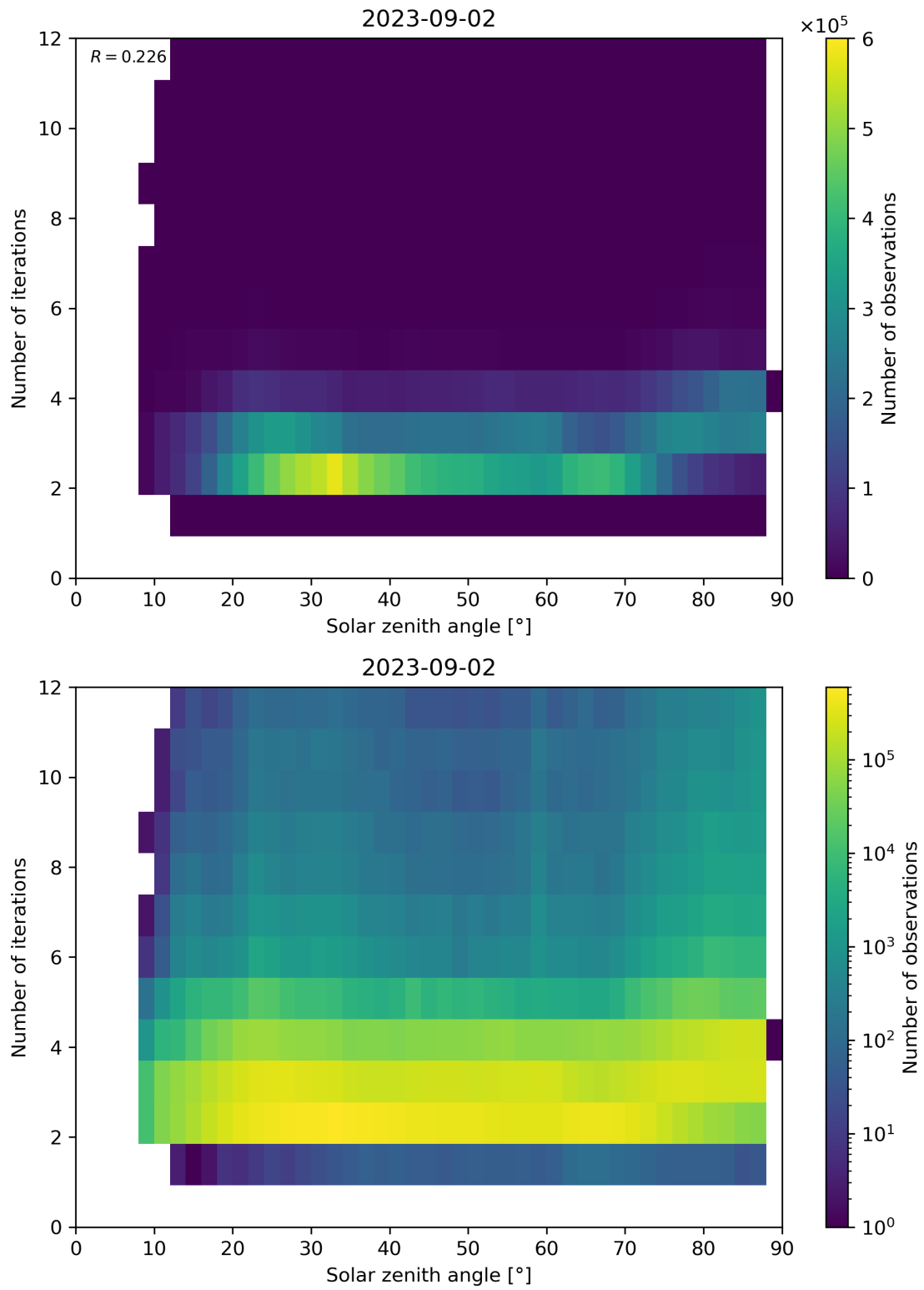
Figure 125: Scatter density plot of “Solar zenith angle” against “Number of iterations” for 2023-09-01 to 2023-09-03.
