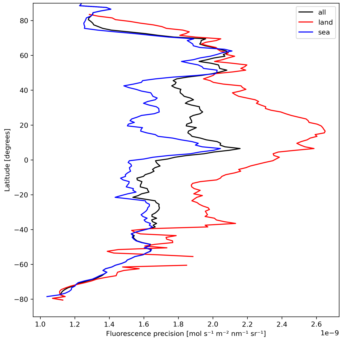
Figure 24: Zonal average of “Fluorescence precision” for 2023-09-01 to 2023-09-03.
