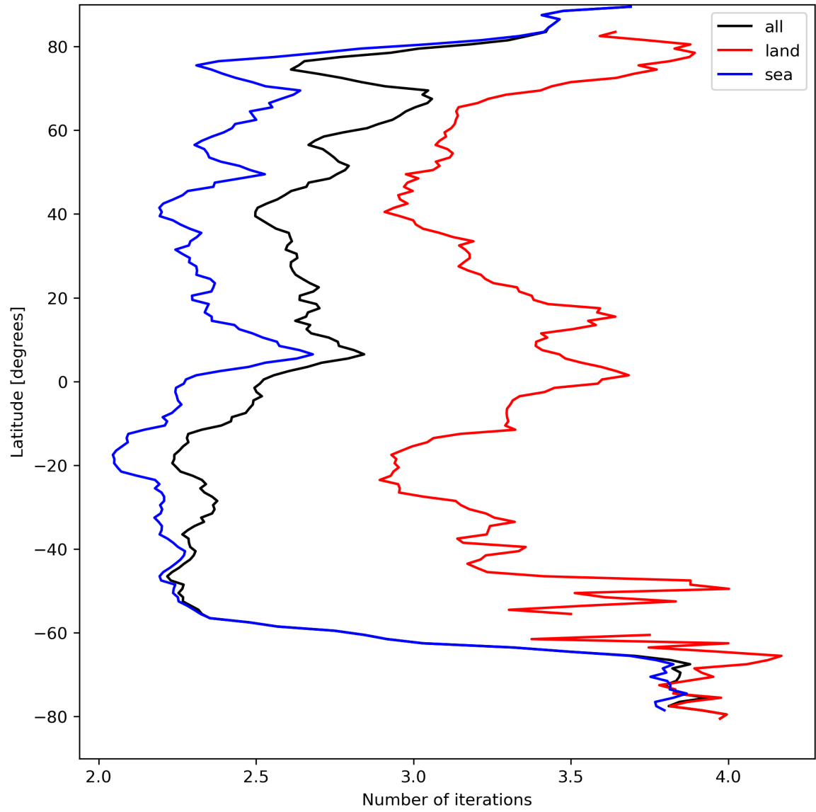
Figure 22: Zonal average of “Number of iterations” for 2023-09-01 to 2023-09-03.
