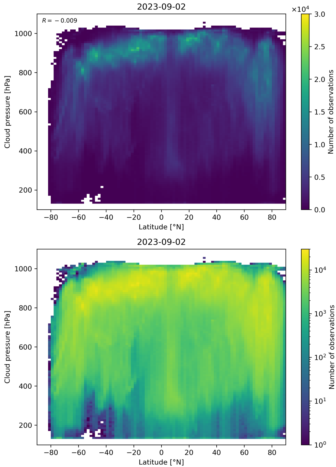
Figure 100: Scatter density plot of “Latitude” against “Cloud pressure” for 2023-09-01 to 2023-09-03.
