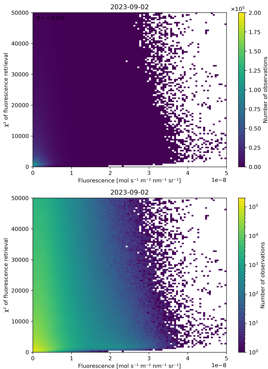
Figure 93: Scatter density plot of “Fluorescence” against “ \chi^2 of fluorescence retrieval” for 2023-09-01 to 2023-09-03.
