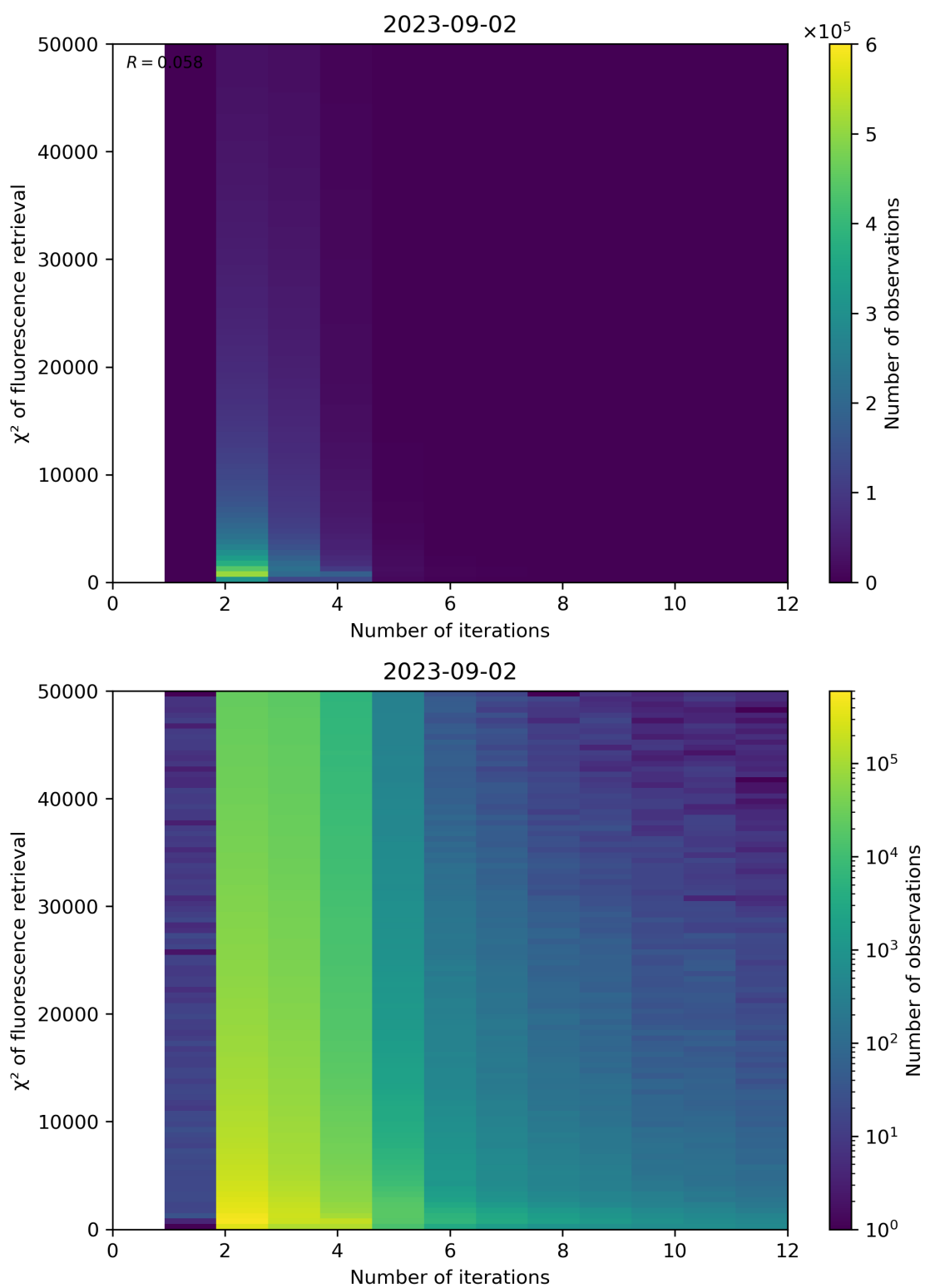
Figure 106: Scatter density plot of “Number of iterations” against “ \chi^2 of fluorescence retrieval” for 2023-09-01 to 2023-09-03.
