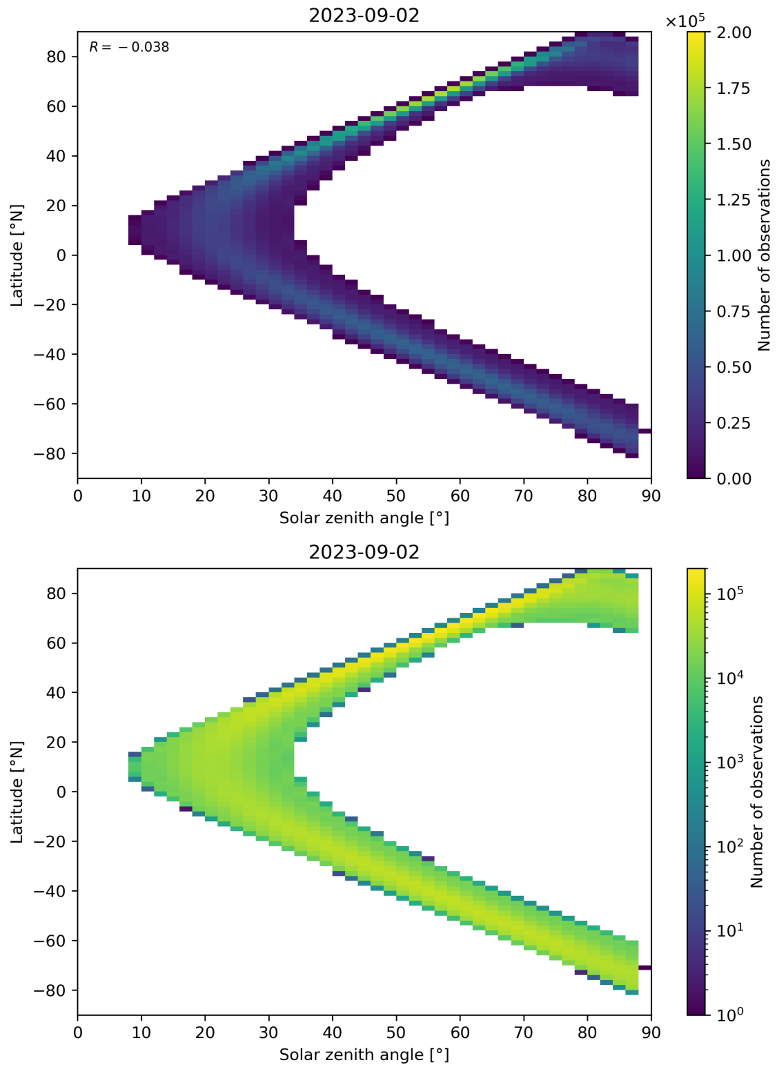
Figure 124: Scatter density plot of “Solar zenith angle” against “Latitude” for 2023-09-01 to 2023-09-03.
