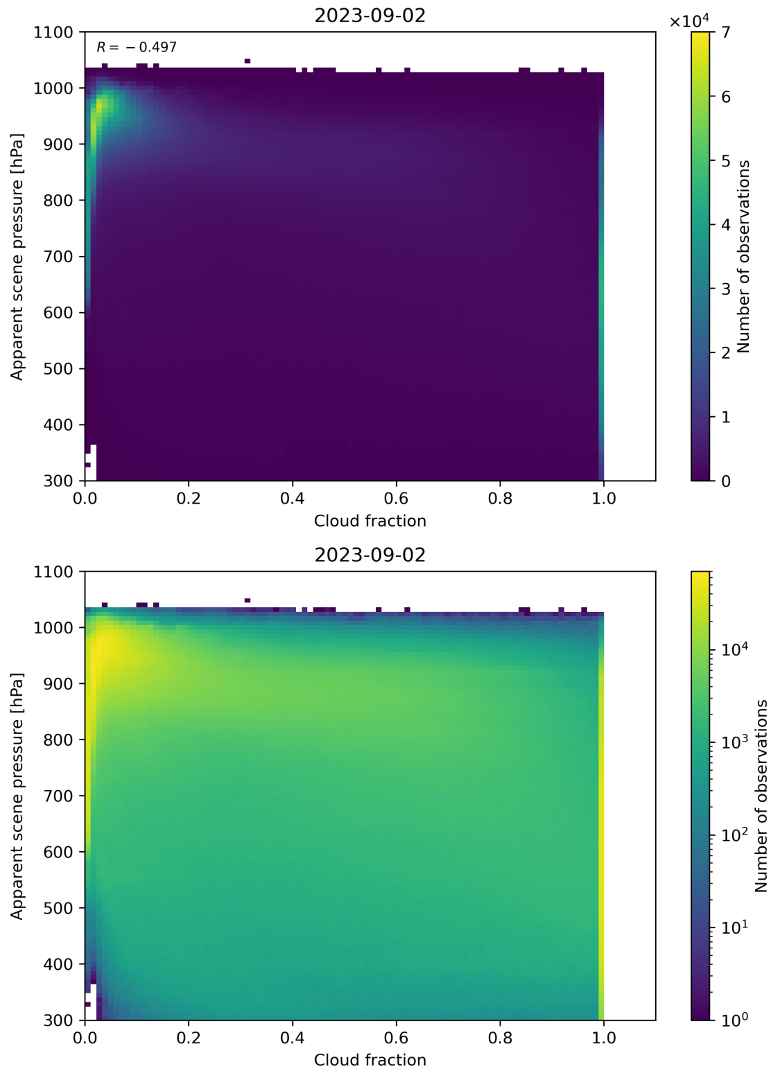
Figure 76: Scatter density plot of “Cloud fraction” against “Apparent scene pressure” for 2023-09-01 to 2023-09-03.
