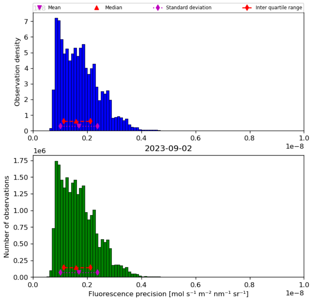
Figure 41: Histogram of “Fluorescence precision” for 2023-09-01 to 2023-09-03
