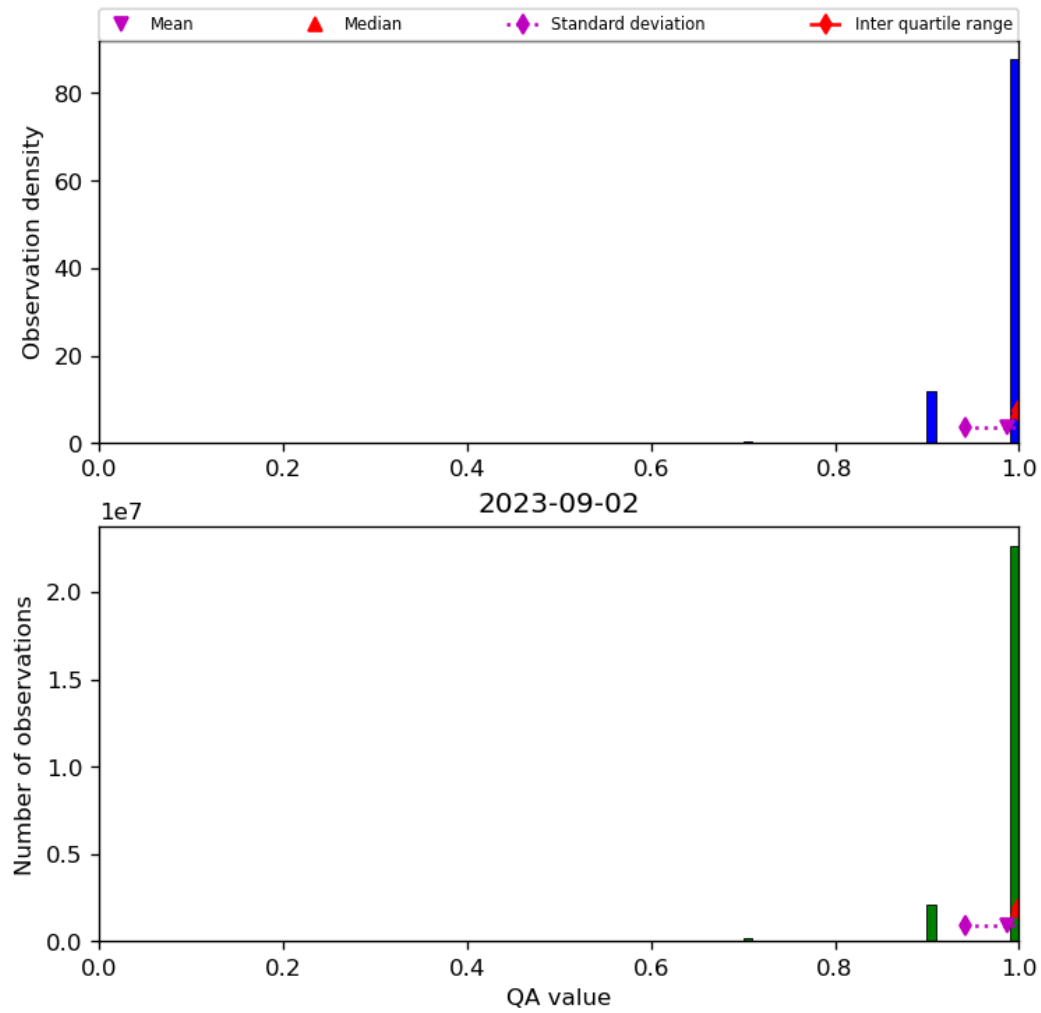
Figure 29: Histogram of “QA value” for 2023-09-01 to 2023-09-03
