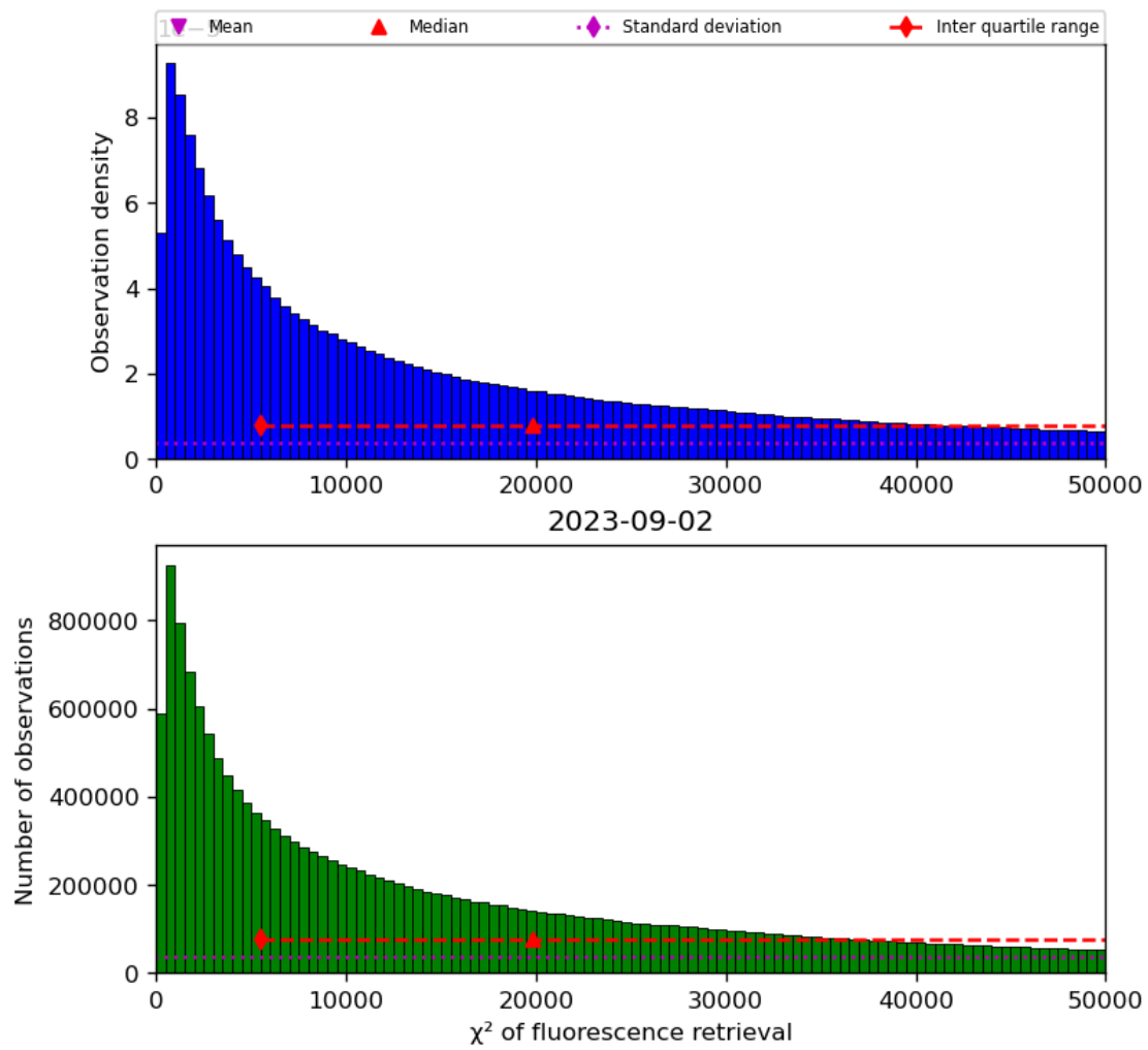
Figure 42: Histogram of “ \chi^2 of fluorescence retrieval” for 2023-09-01 to 2023-09-03
