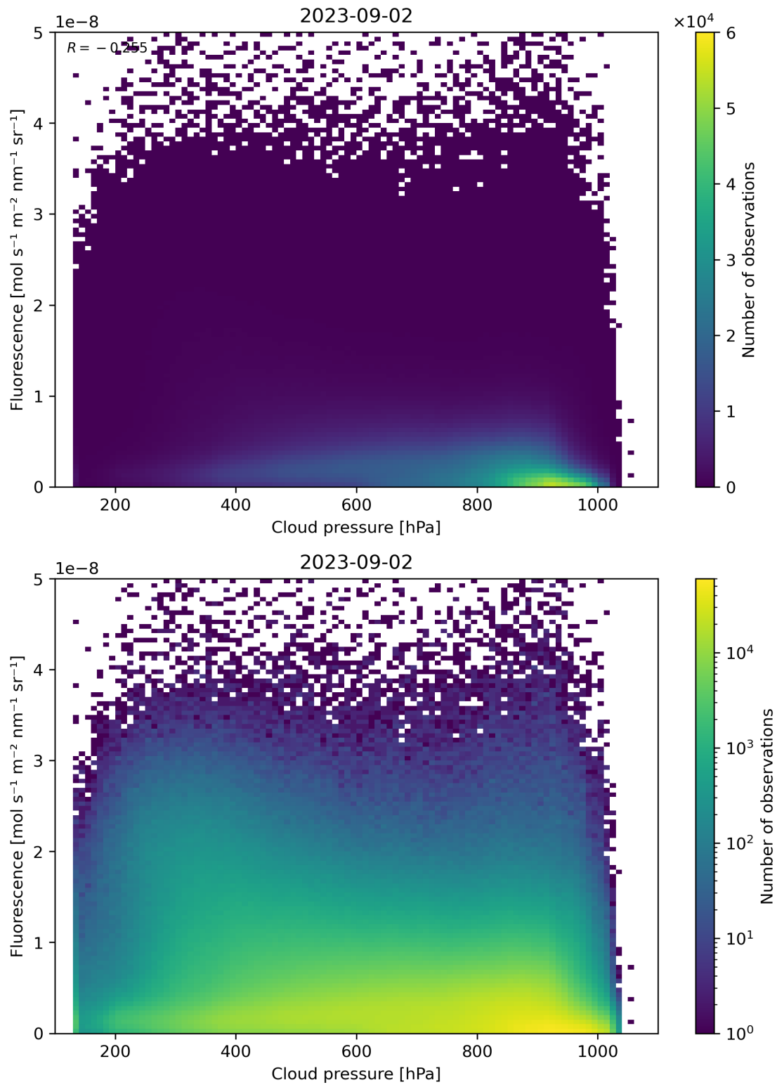
Figure 88: Scatter density plot of “Cloud pressure” against “Fluorescence” for 2023-09-01 to 2023-09-03.
