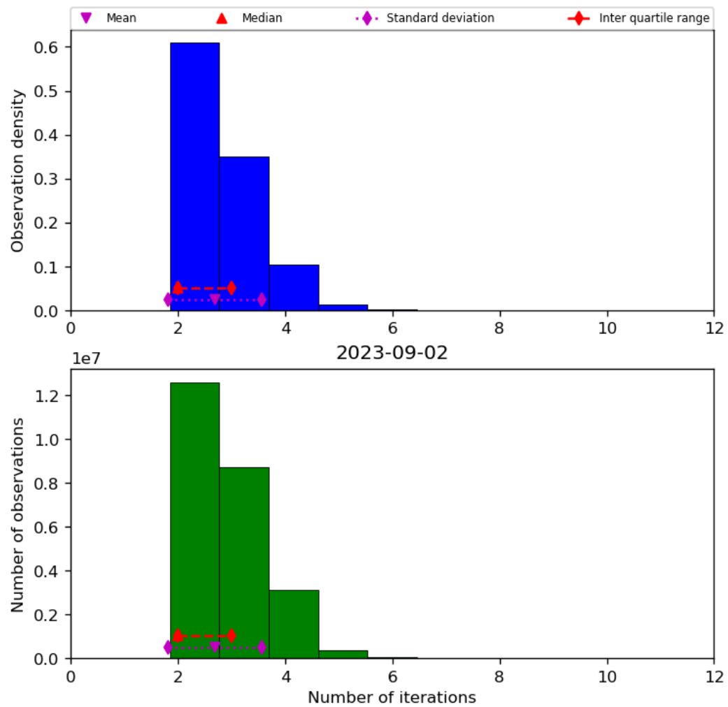
Figure 39: Histogram of “Number of iterations” for 2023-09-01 to 2023-09-03
