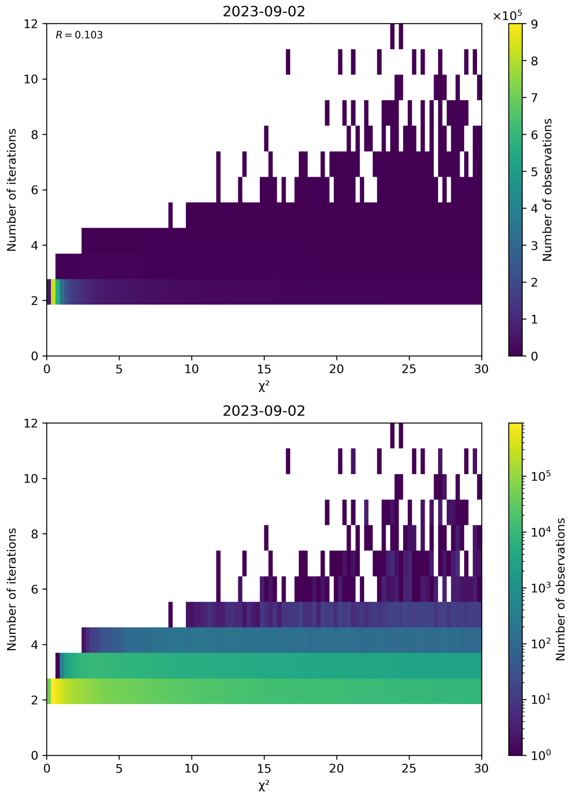
Figure 73: Scatter density plot of " \chi^2 " against "Number of iterations" for 2023-09-01 to 2023-09-03.
