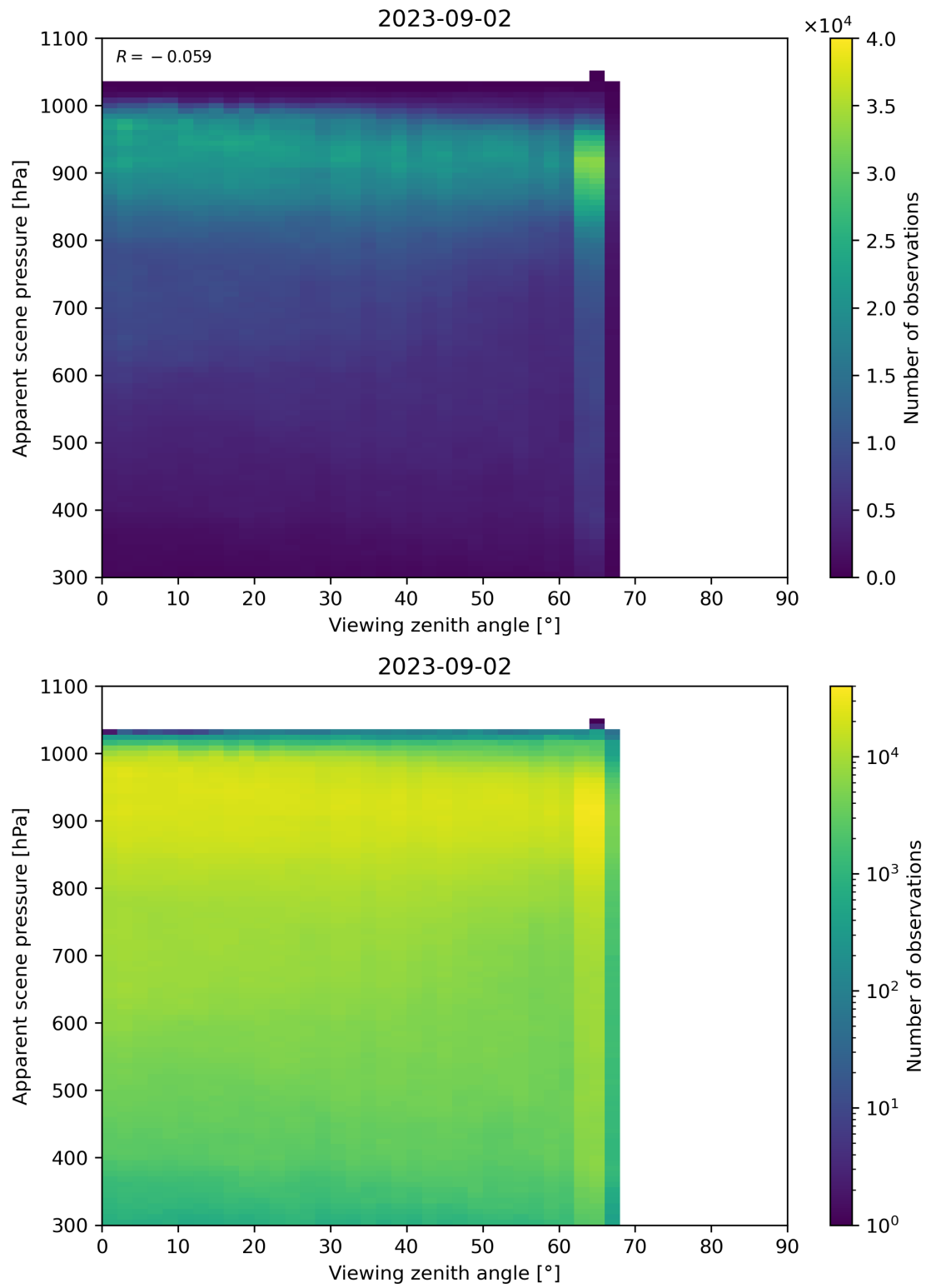
Figure 129: Scatter density plot of “Viewing zenith angle” against “Apparent scene pressure” for 2023-09-01 to 2023-09-03.
