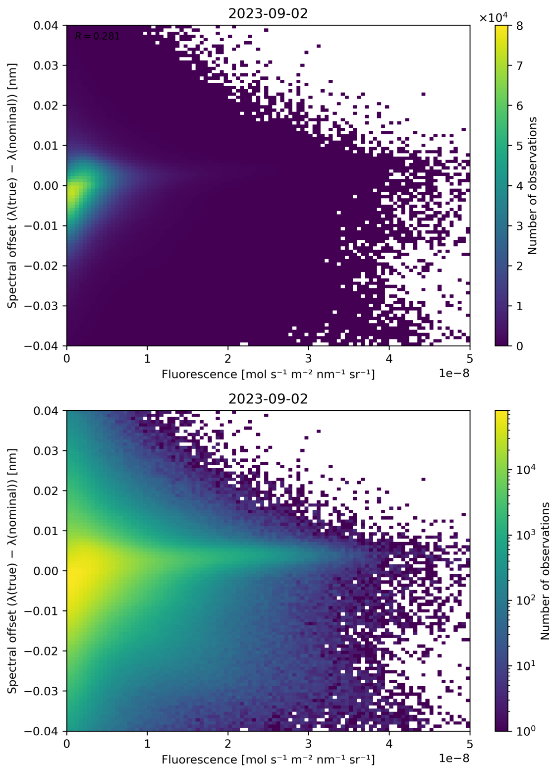
Figure 95: Scatter density plot of “Fluorescence” against “Spectral offset ( \lambda(\text{true}) - \lambda(\text{nominal}) )” for 2023-09-01 to 2023-09-03.
