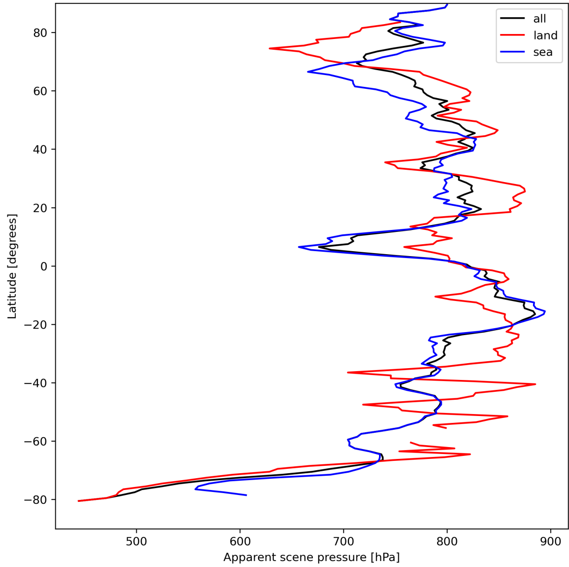
Figure 19: Zonal average of “Apparent scene pressure” for 2023-09-01 to 2023-09-03.
