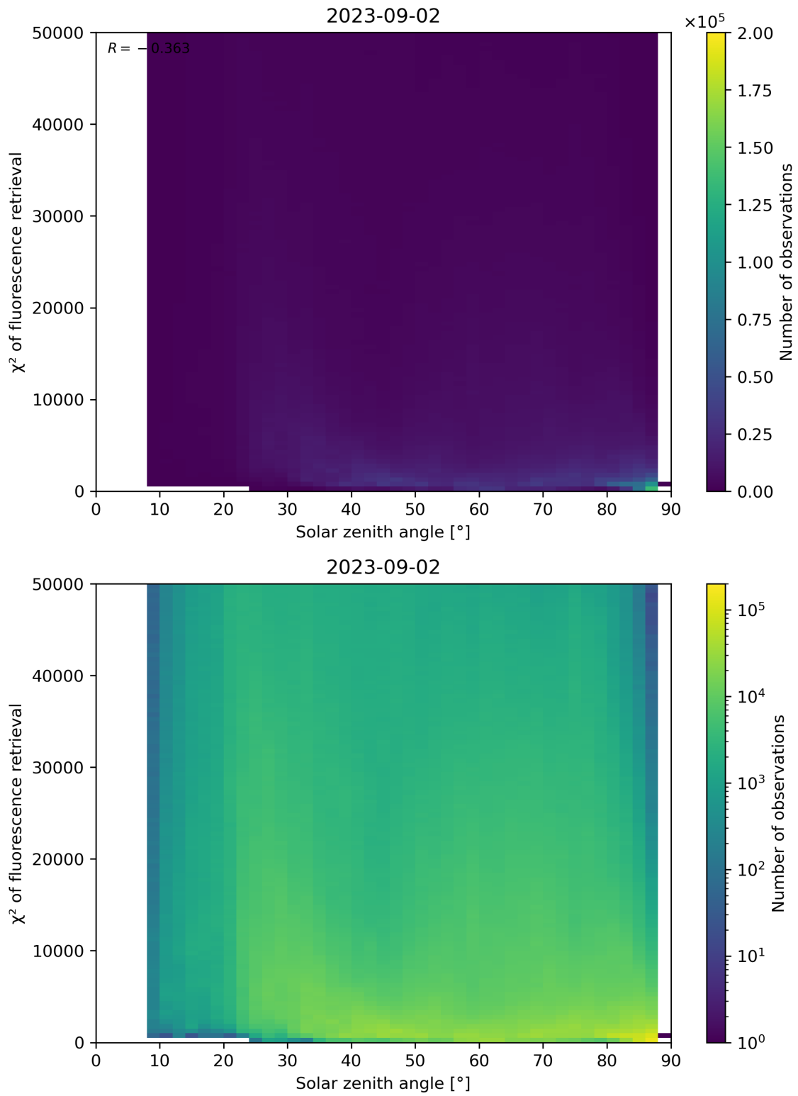
Figure 120: Scatter density plot of “Solar zenith angle” against “ \chi^2 of fluorescence retrieval” for 2023-09-01 to 2023-09-03.
