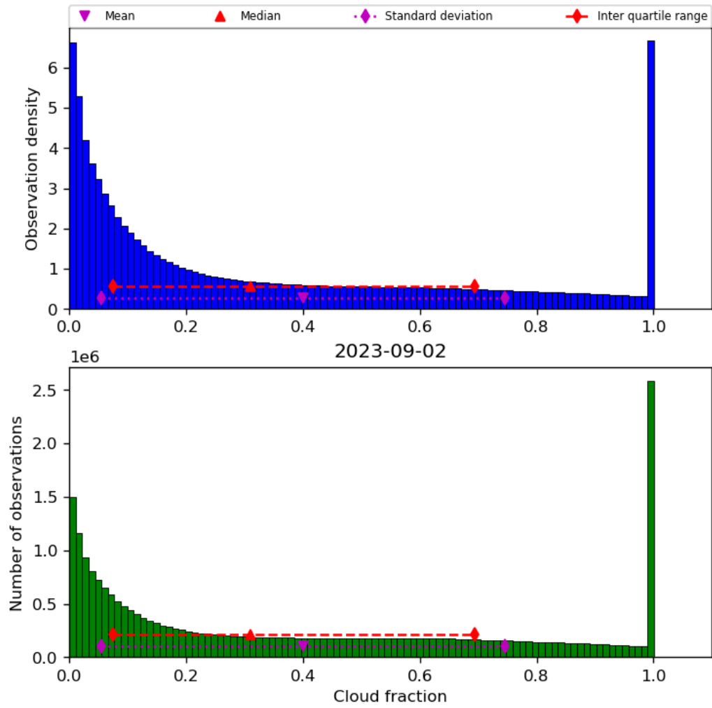
Figure 32: Histogram of “Cloud fraction” for 2023-09-01 to 2023-09-03
