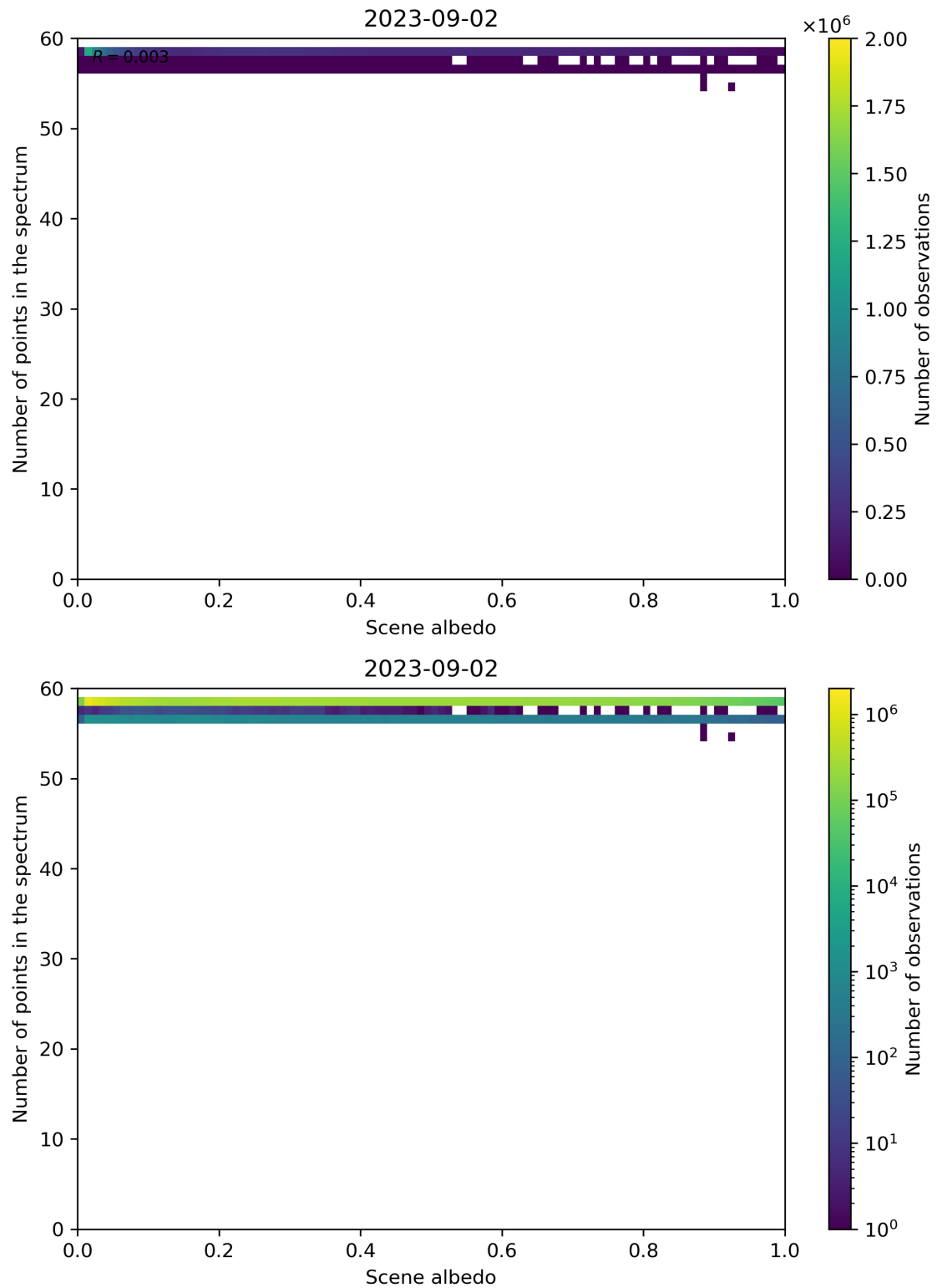
Figure 116: Scatter density plot of “Scene albedo” against “Number of points in the spectrum” for 2023-09-01 to 2023-09-03.
