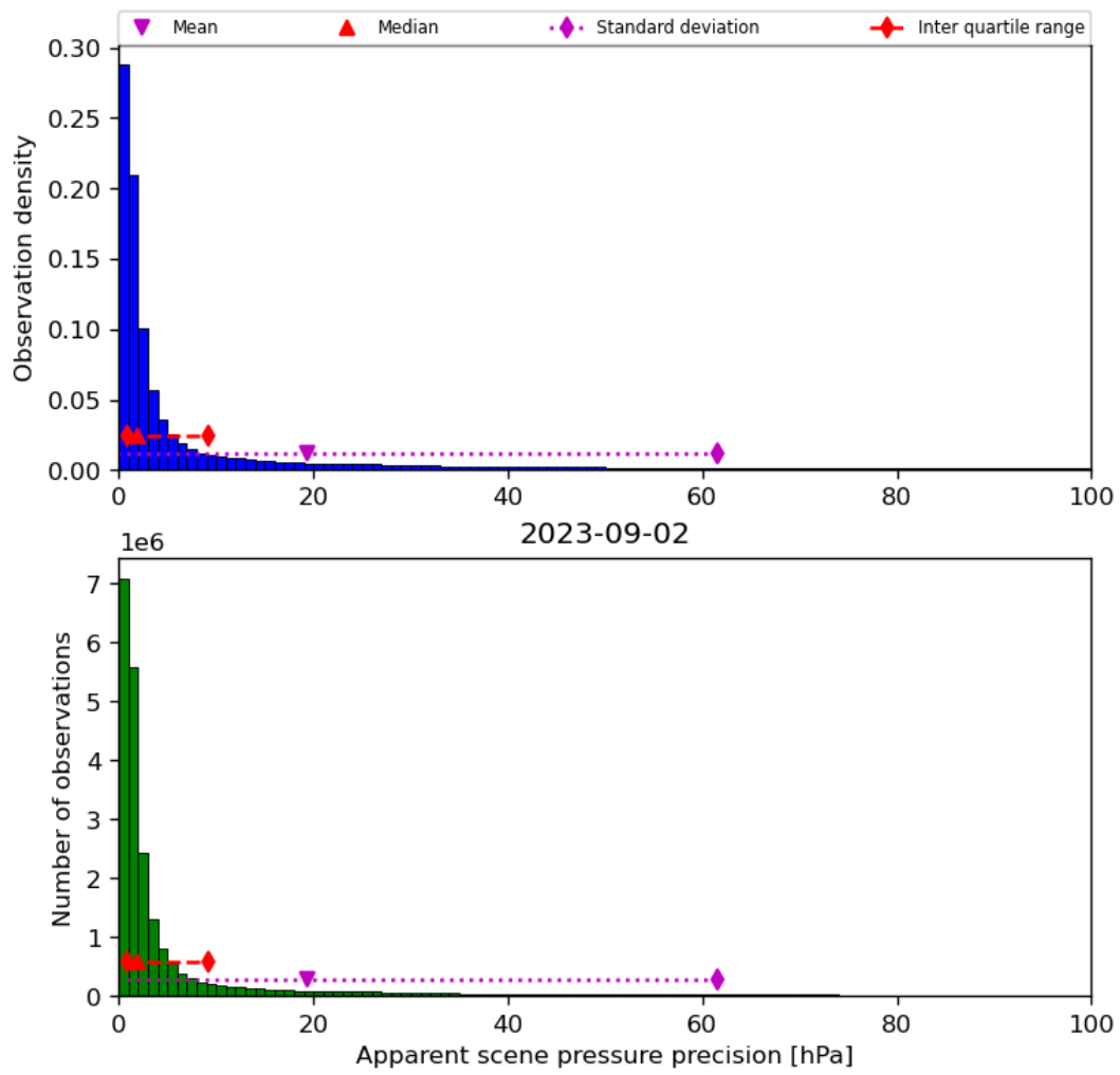
Figure 37: Histogram of “Apparent scene pressure precision” for 2023-09-01 to 2023-09-03
