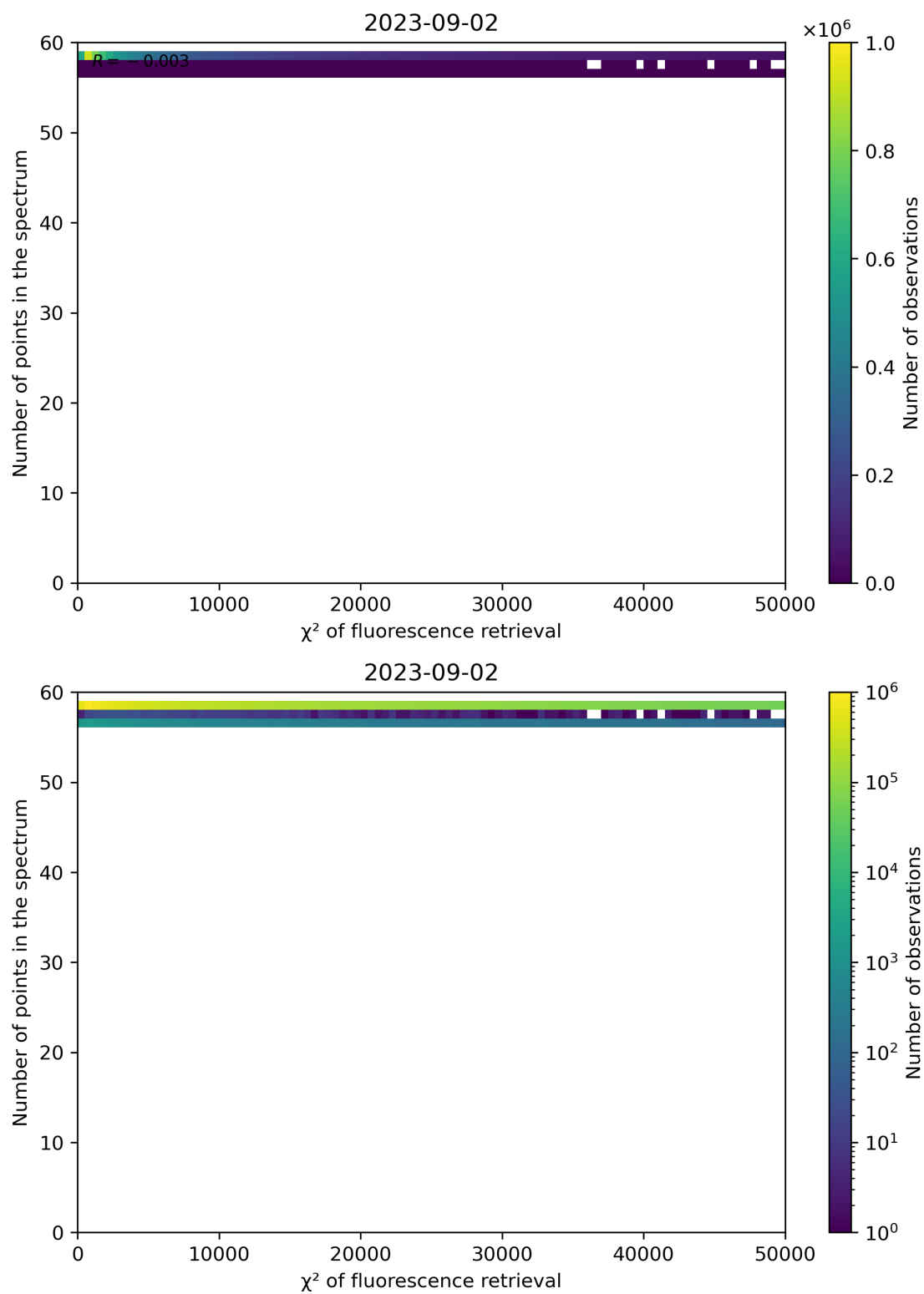
Figure 71: Scatter density plot of “ \chi^2 of fluorescence retrieval” against “Number of points in the spectrum” for 2023-09-01 to 2023-09-03.
