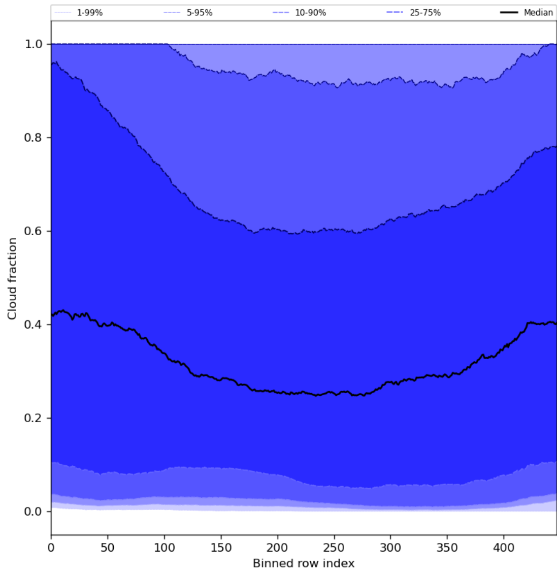
Figure 49: Along track statistics of “Cloud fraction” for 2023-09-01 to 2023-09-03
