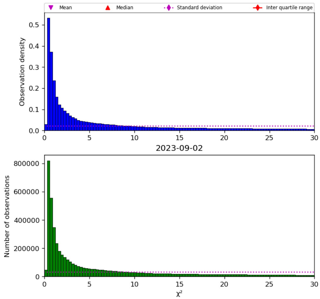
Figure 38: Histogram of " \chi^2 " for 2023-09-01 to 2023-09-03
