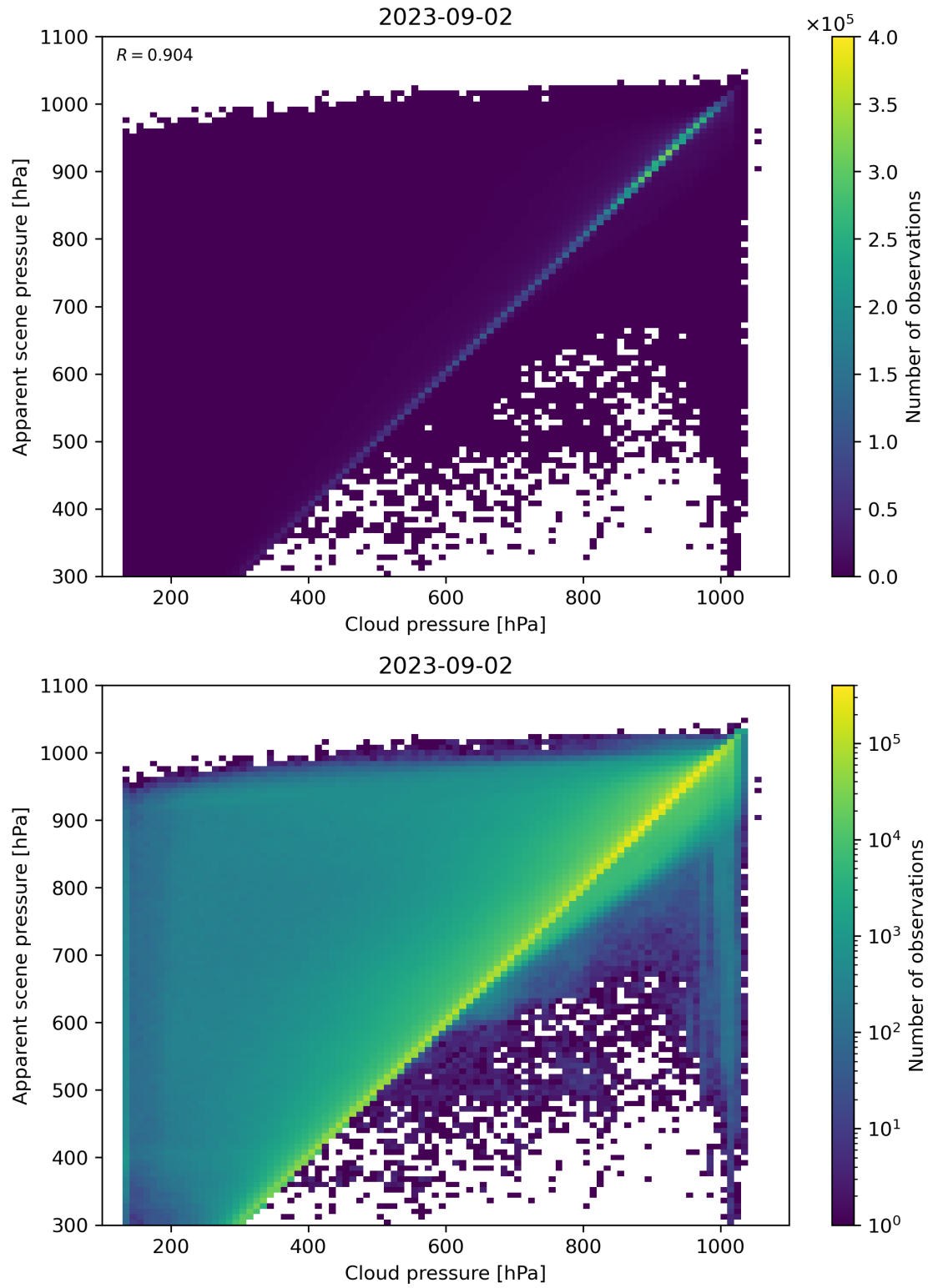
Figure 84: Scatter density plot of “Cloud pressure” against “Apparent scene pressure” for 2023-09-01 to 2023-09-03.
