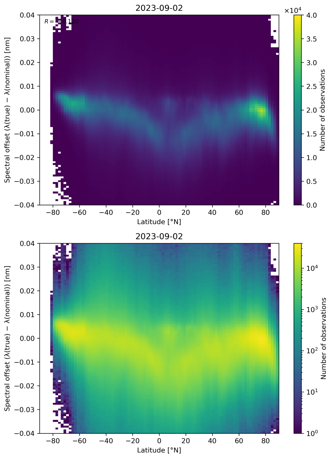
Figure 105: Scatter density plot of “Latitude” against “Spectral offset ( \lambda(\text{true}) - \lambda(\text{nominal}) )” for 2023-09-01 to 2023-09-03.
