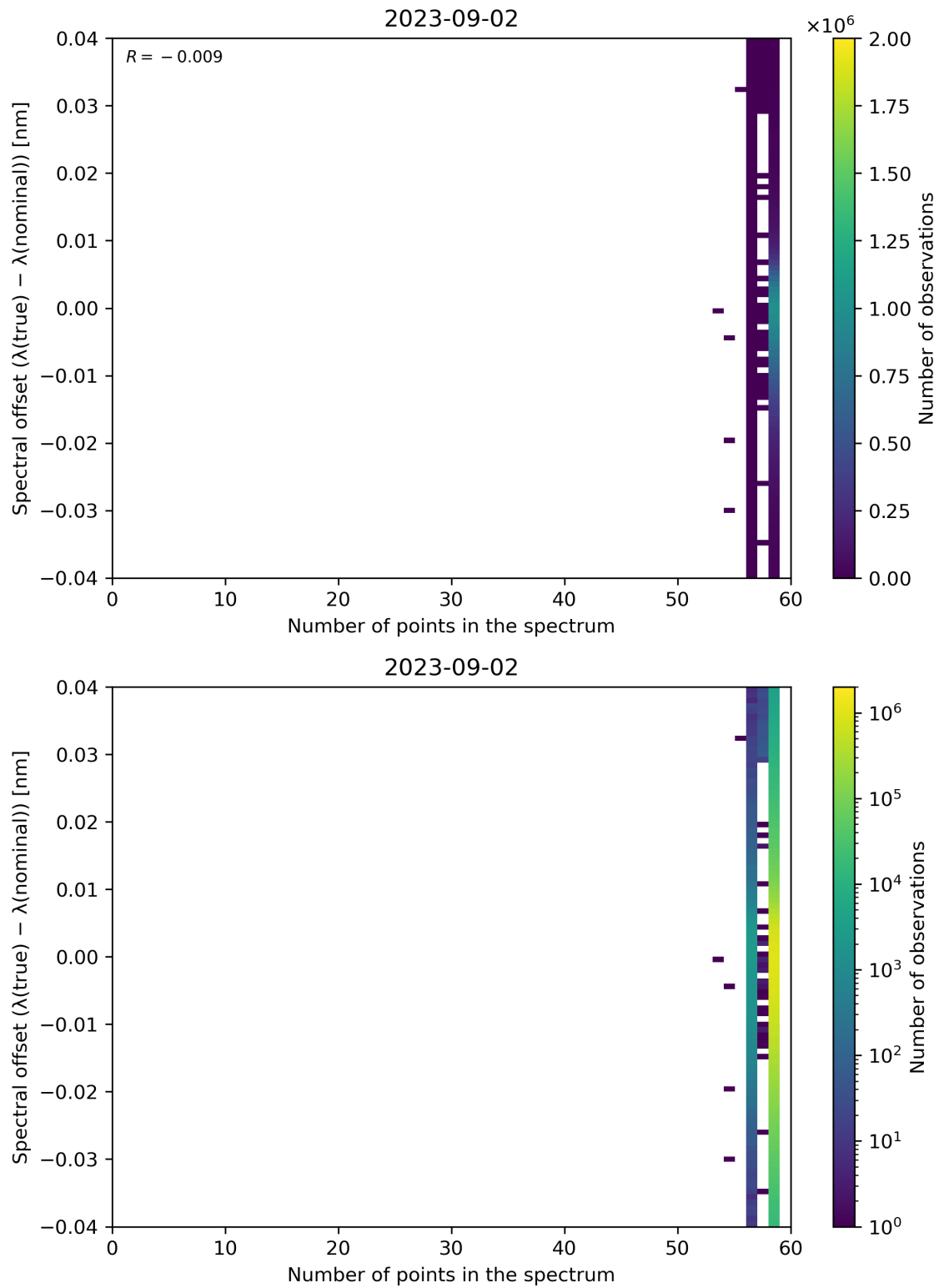
Figure 110: Scatter density plot of “Number of points in the spectrum” against “Spectral offset ( \lambda(\text{true}) - \lambda(\text{nominal}) )” for 2023-09-01 to 2023-09-03.
