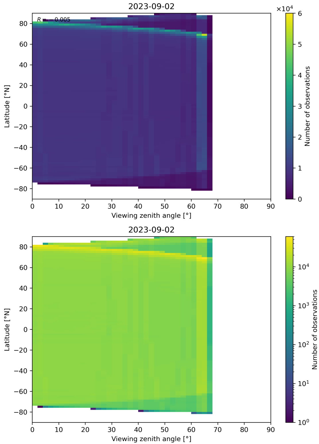
Figure 135: Scatter density plot of “Viewing zenith angle” against “Latitude” for 2023-09-01 to 2023-09-03.
