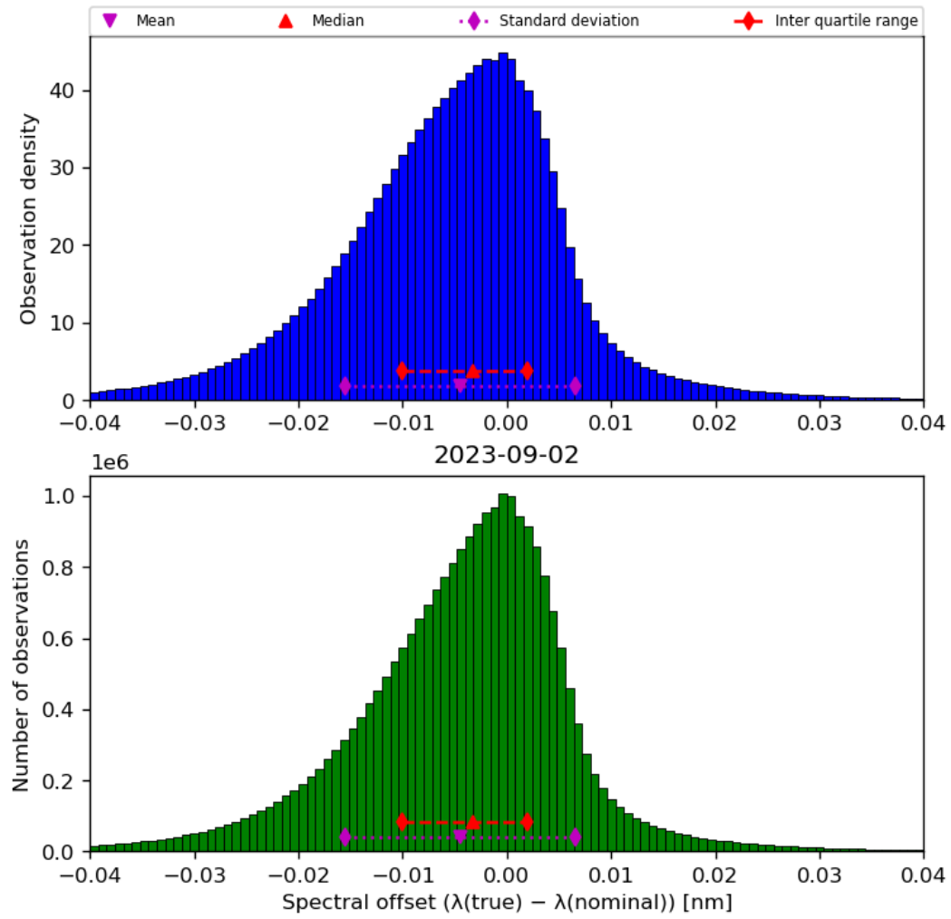
Figure 45: Histogram of “Spectral offset ( \lambda(\text{true}) - \lambda(\text{nominal}) )” for 2023-09-01 to 2023-09-03
