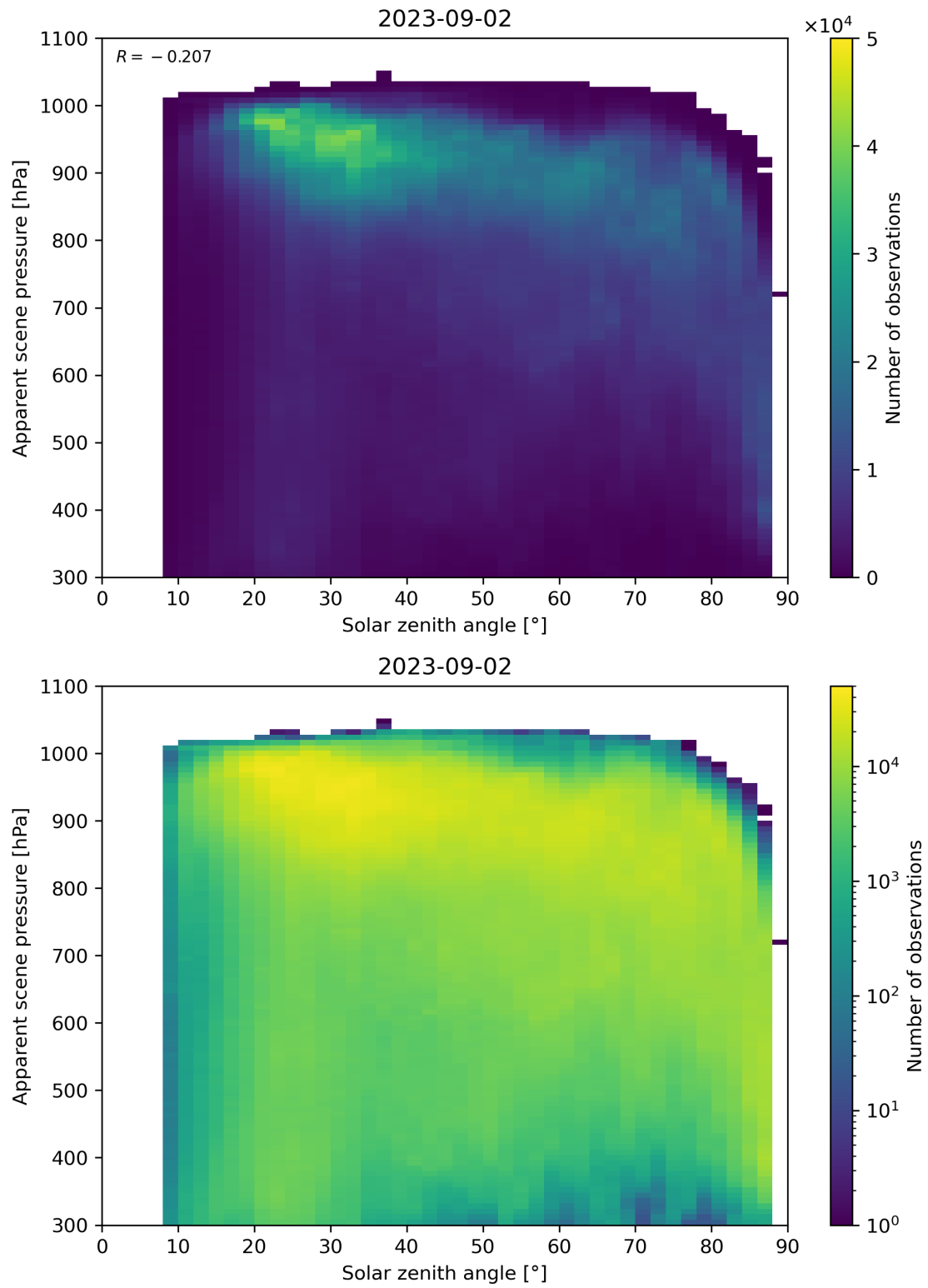
Figure 118: Scatter density plot of “Solar zenith angle” against “Apparent scene pressure” for 2023-09-01 to 2023-09-03.
