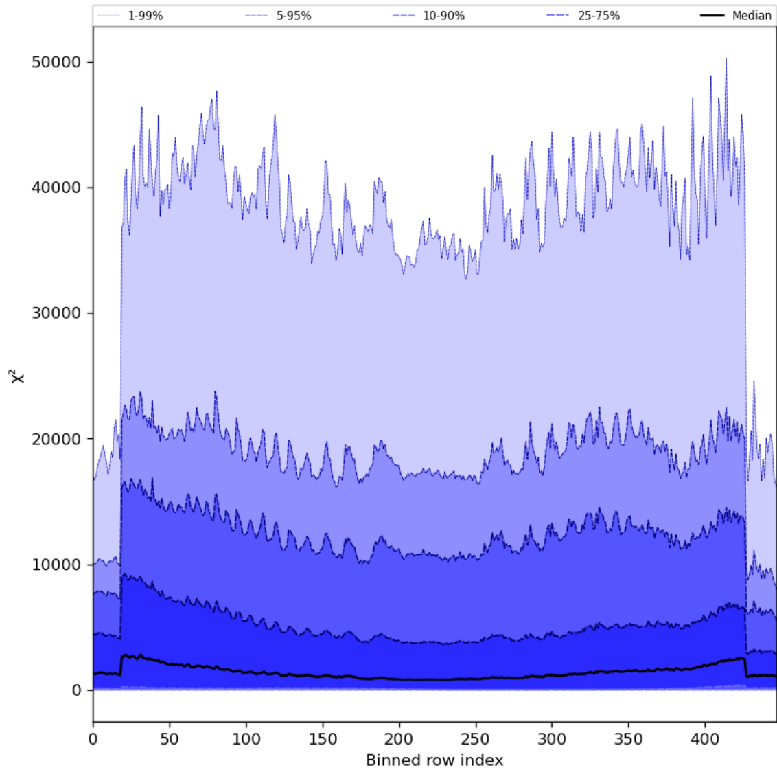
Figure 55: Along track statistics of “ \chi^2 ” for 2023-09-01 to 2023-09-03
