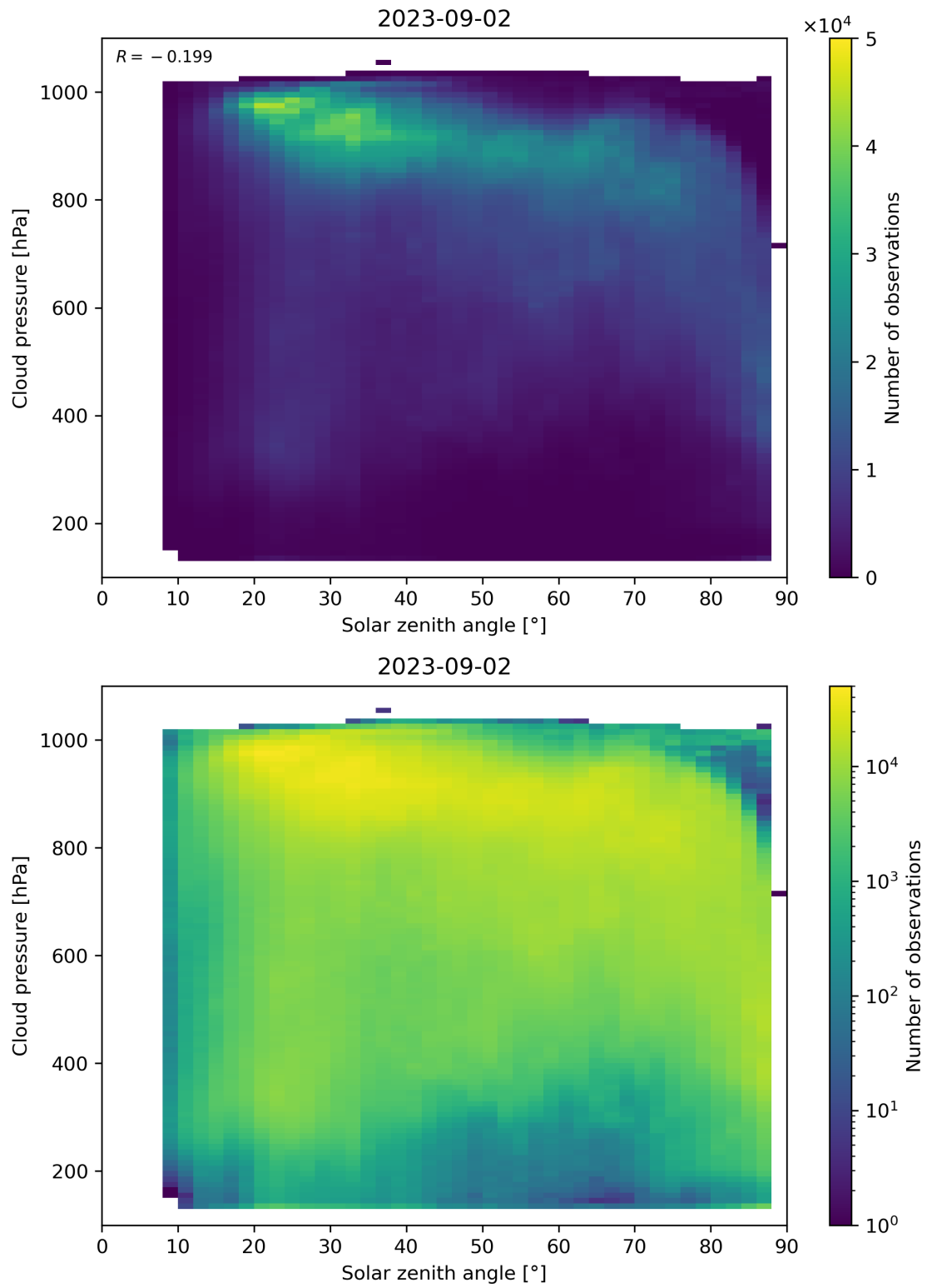
Figure 122: Scatter density plot of “Solar zenith angle” against “Cloud pressure” for 2023-09-01 to 2023-09-03.
