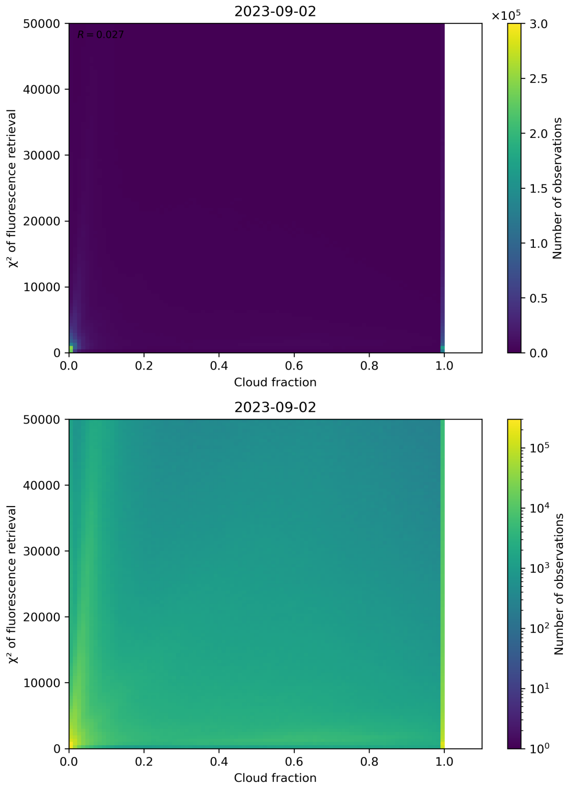
Figure 78: Scatter density plot of “Cloud fraction” against “ \chi^2 of fluorescence retrieval” for 2023-09-01 to 2023-09-03.
