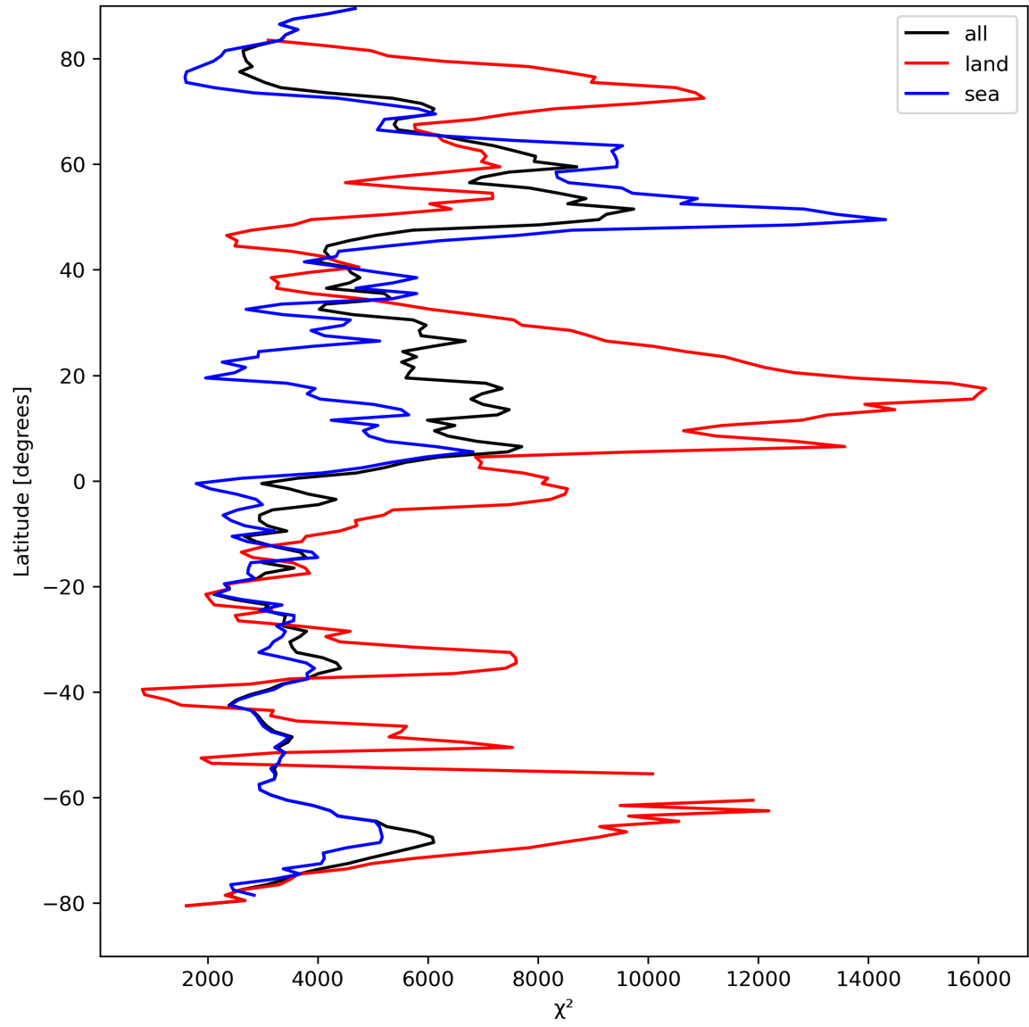
Figure 21: Zonal average of “ \chi^2 ” for 2023-09-01 to 2023-09-03.
