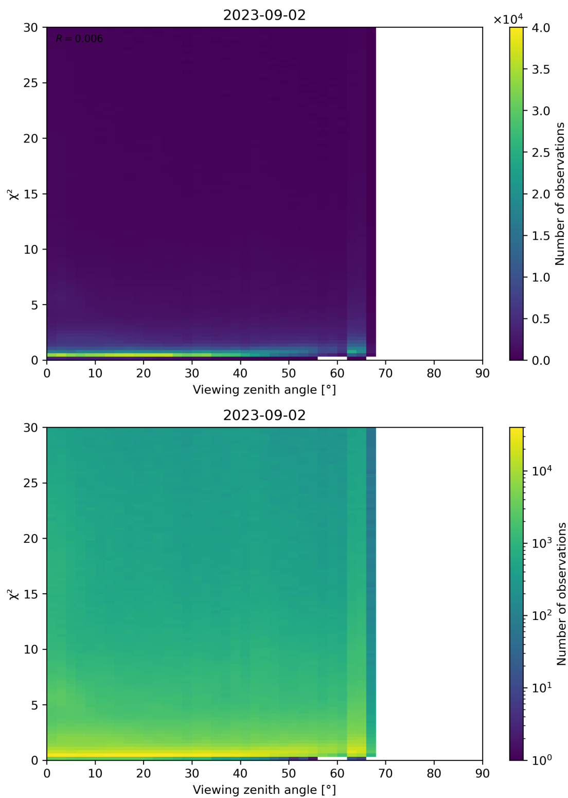
Figure 130: Scatter density plot of “Viewing zenith angle” against “ \chi^2 ” for 2023-09-01 to 2023-09-03.
