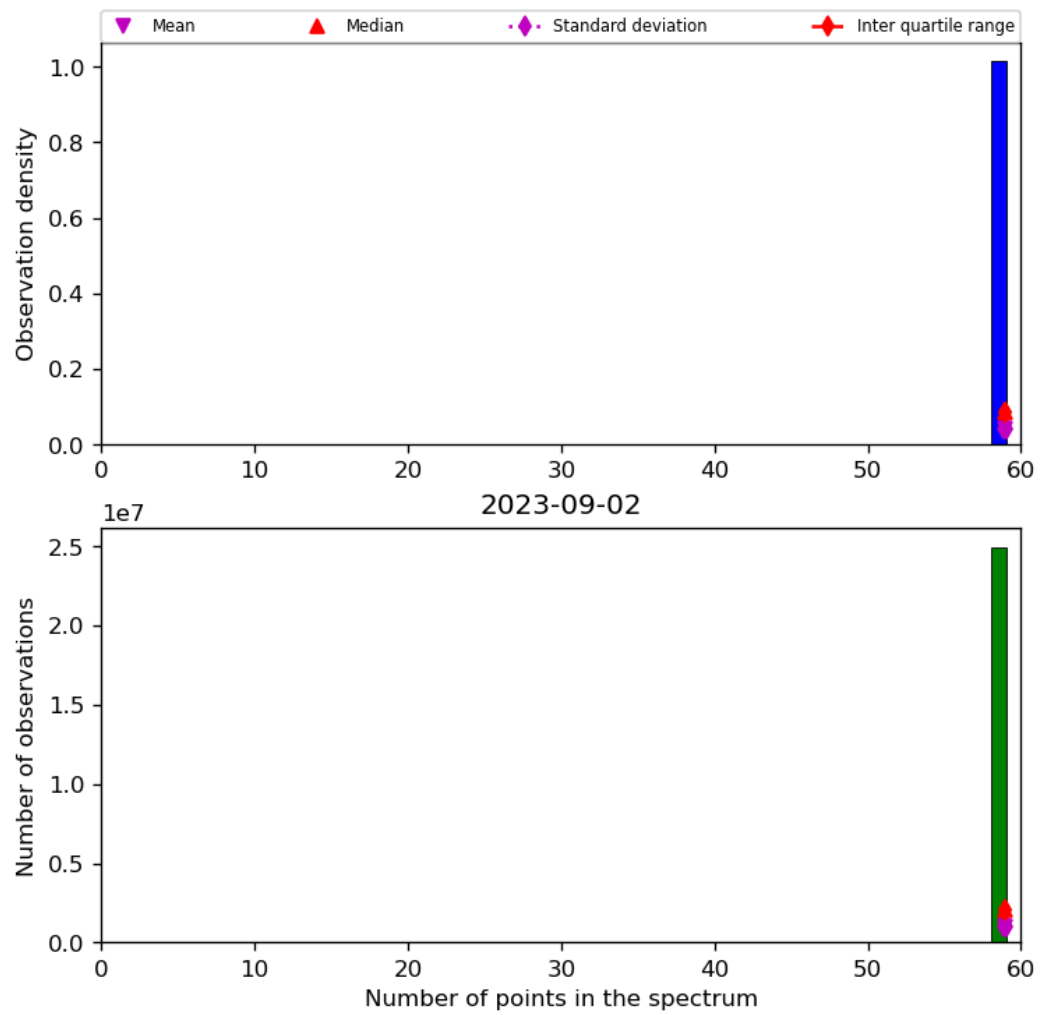
Figure 44: Histogram of “Number of points in the spectrum” for 2023-09-01 to 2023-09-03
