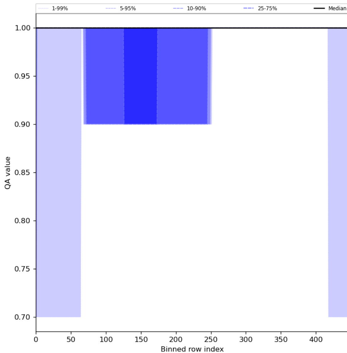
Figure 46: Along track statistics of “QA value” for 2023-09-01 to 2023-09-03
