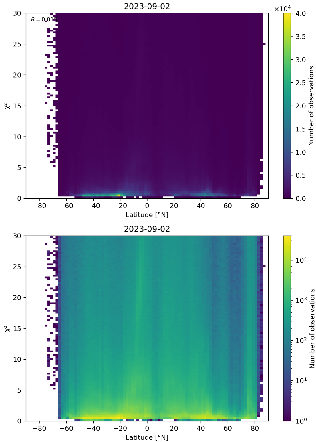
Figure 97: Scatter density plot of “Latitude” against “ \chi^2 ” for 2023-09-01 to 2023-09-03.
