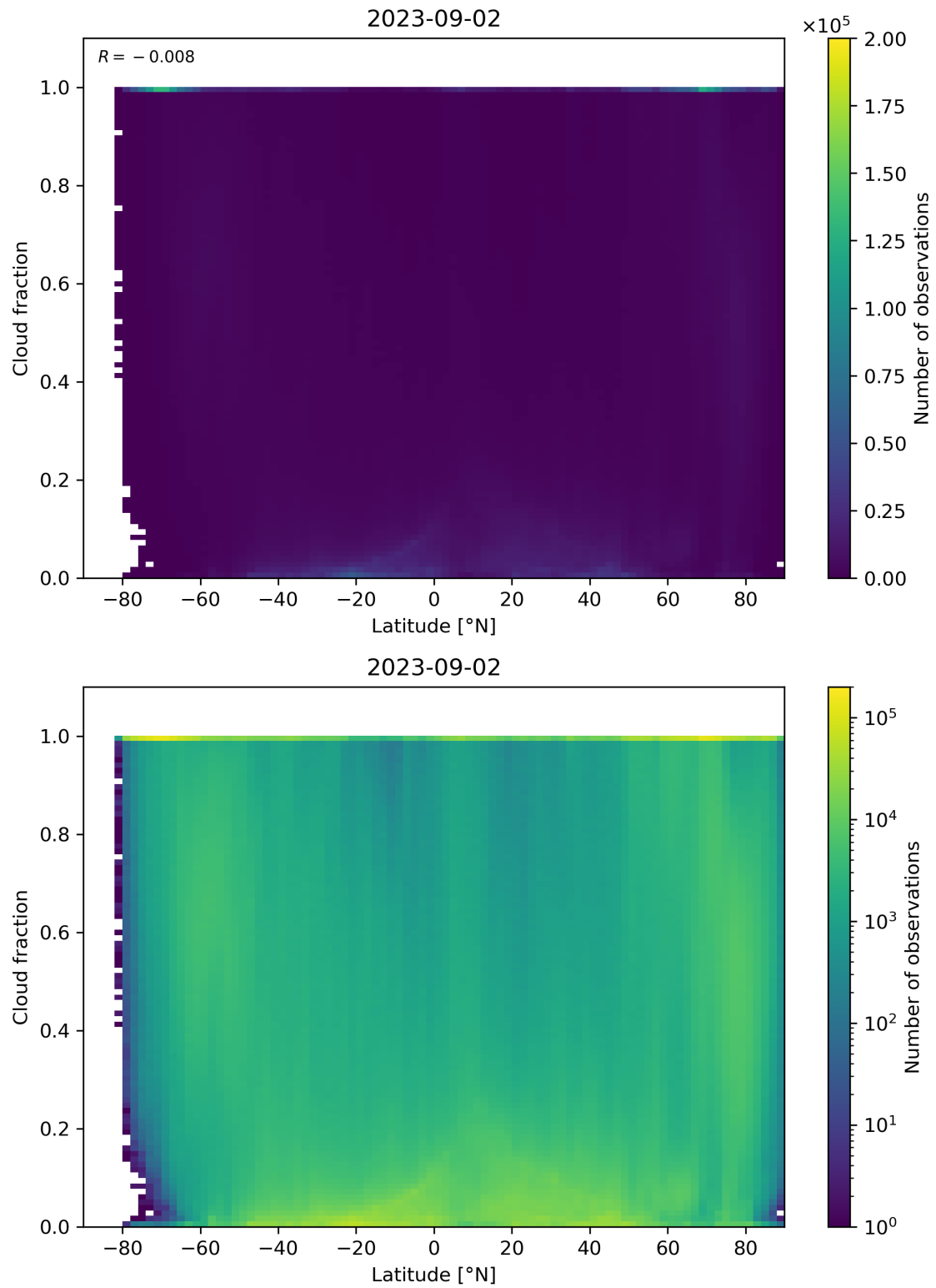
Figure 99: Scatter density plot of “Latitude” against “Cloud fraction” for 2023-09-01 to 2023-09-03.
