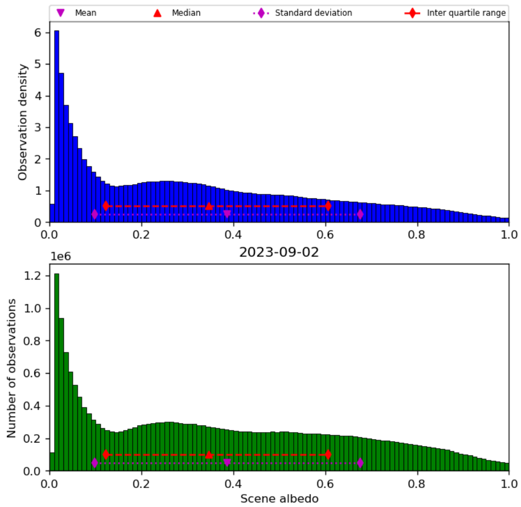
Figure 34: Histogram of “Scene albedo” for 2023-09-01 to 2023-09-03
