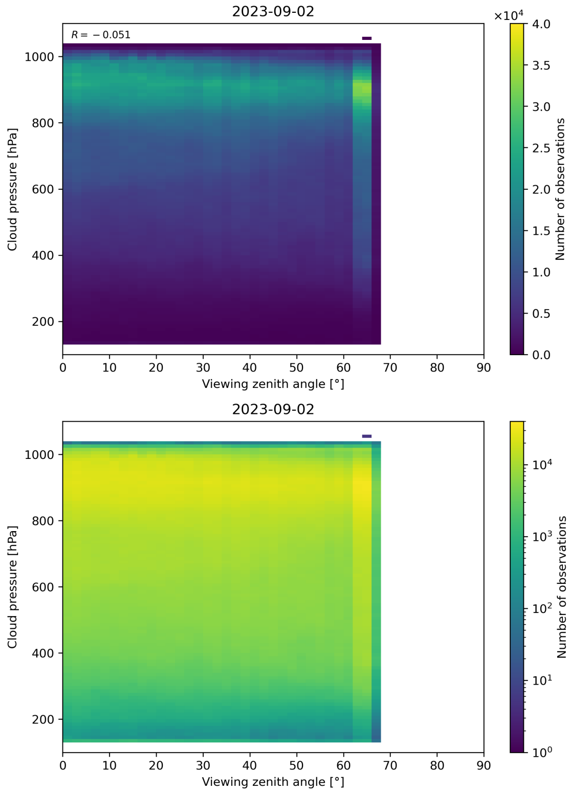
Figure 133: Scatter density plot of “Viewing zenith angle” against “Cloud pressure” for 2023-09-01 to 2023-09-03.
