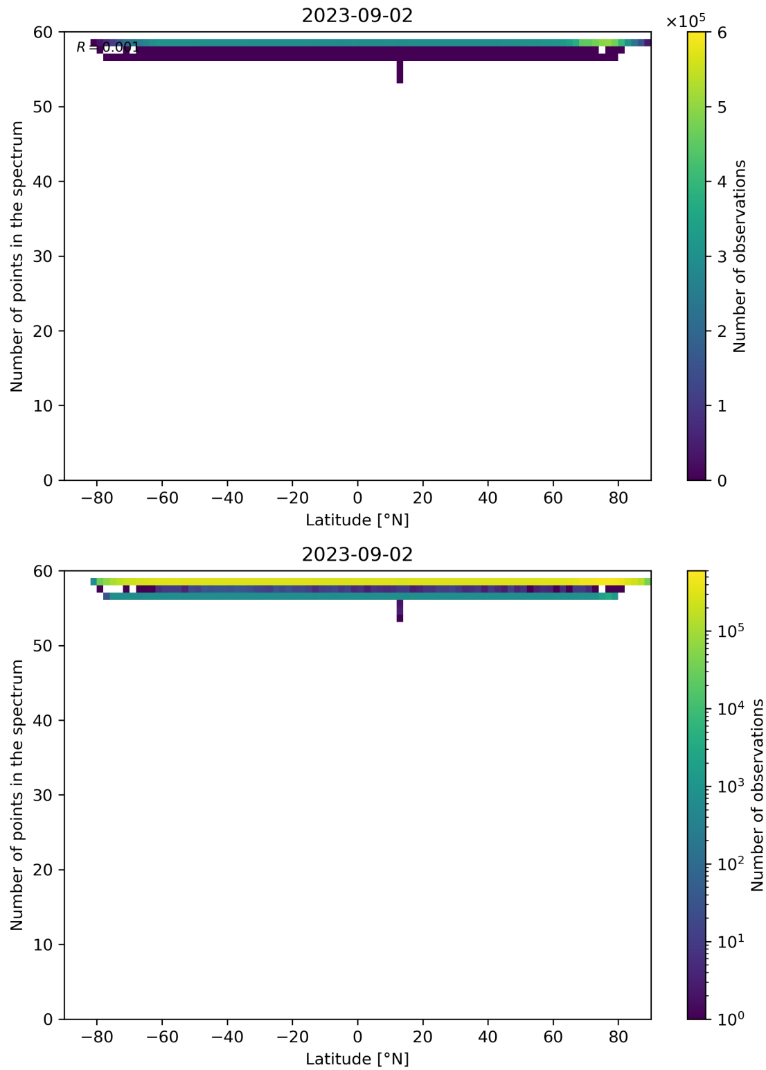
Figure 103: Scatter density plot of “Latitude” against “Number of points in the spectrum” for 2023-09-01 to 2023-09-03.
