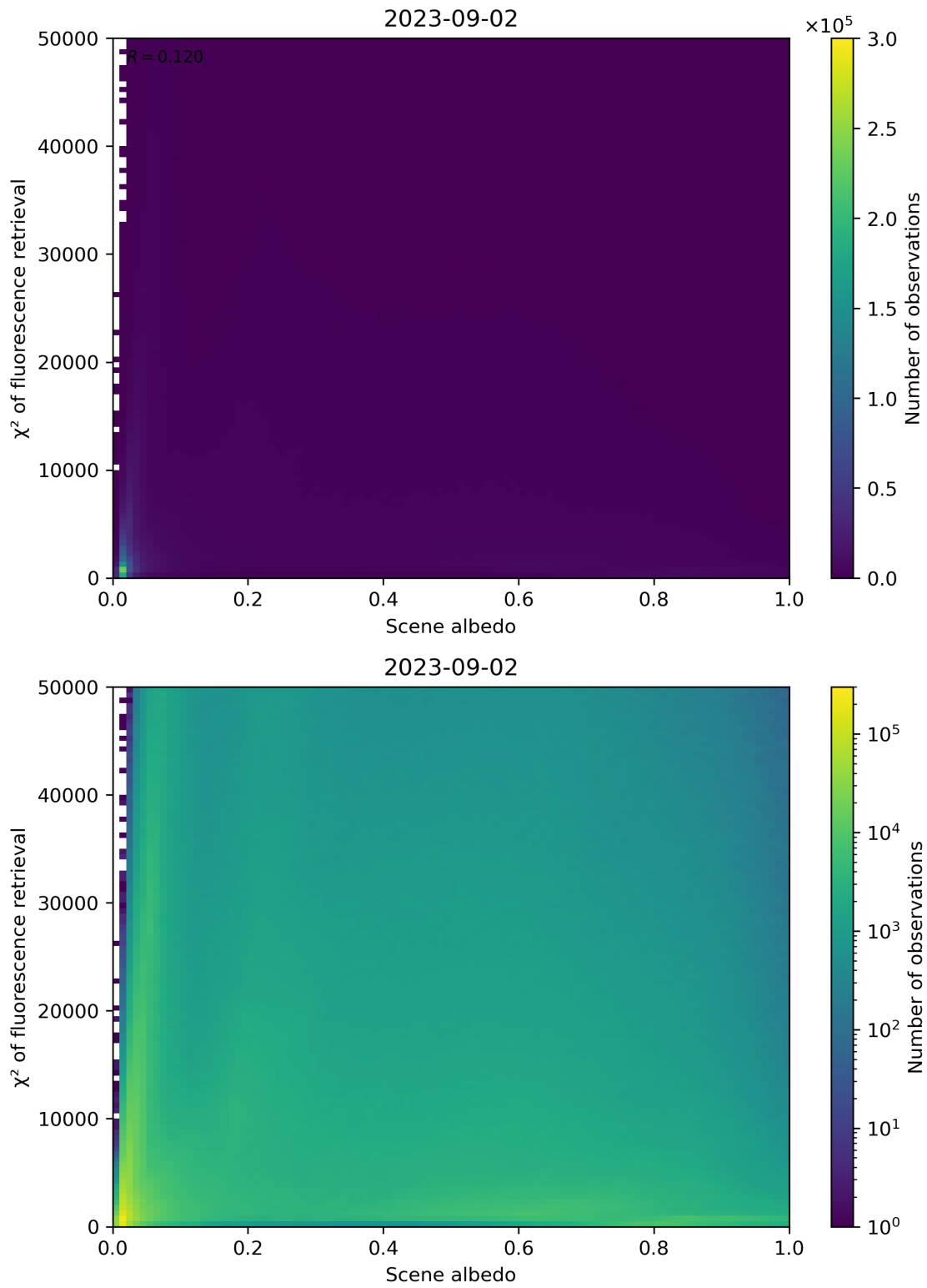
Figure 113: Scatter density plot of “Scene albedo” against “ \chi^2 of fluorescence retrieval” for 2023-09-01 to 2023-09-03.
