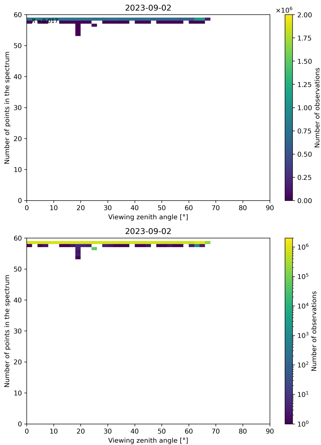
Figure 137: Scatter density plot of “Viewing zenith angle” against “Number of points in the spectrum” for 2023-09-01 to 2023-09-03.
