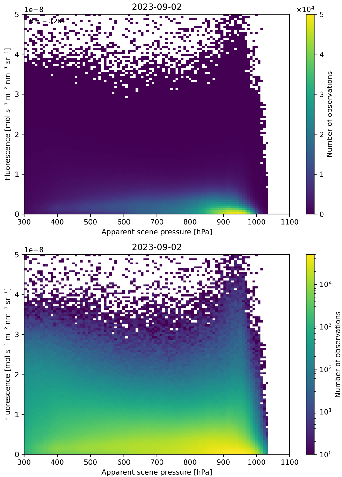
Figure 65: Scatter density plot of “Apparent scene pressure” against “Fluorescence” for 2023-09-01 to 2023-09-03.
