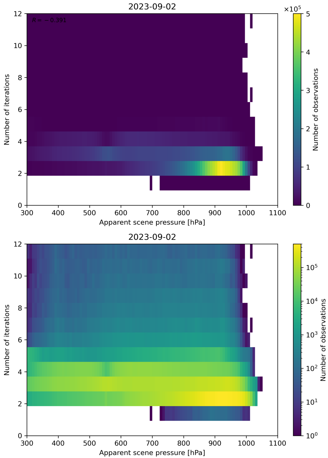
Figure 66: Scatter density plot of “Apparent scene pressure” against “Number of iterations” for 2023-09-01 to 2023-09-03.
