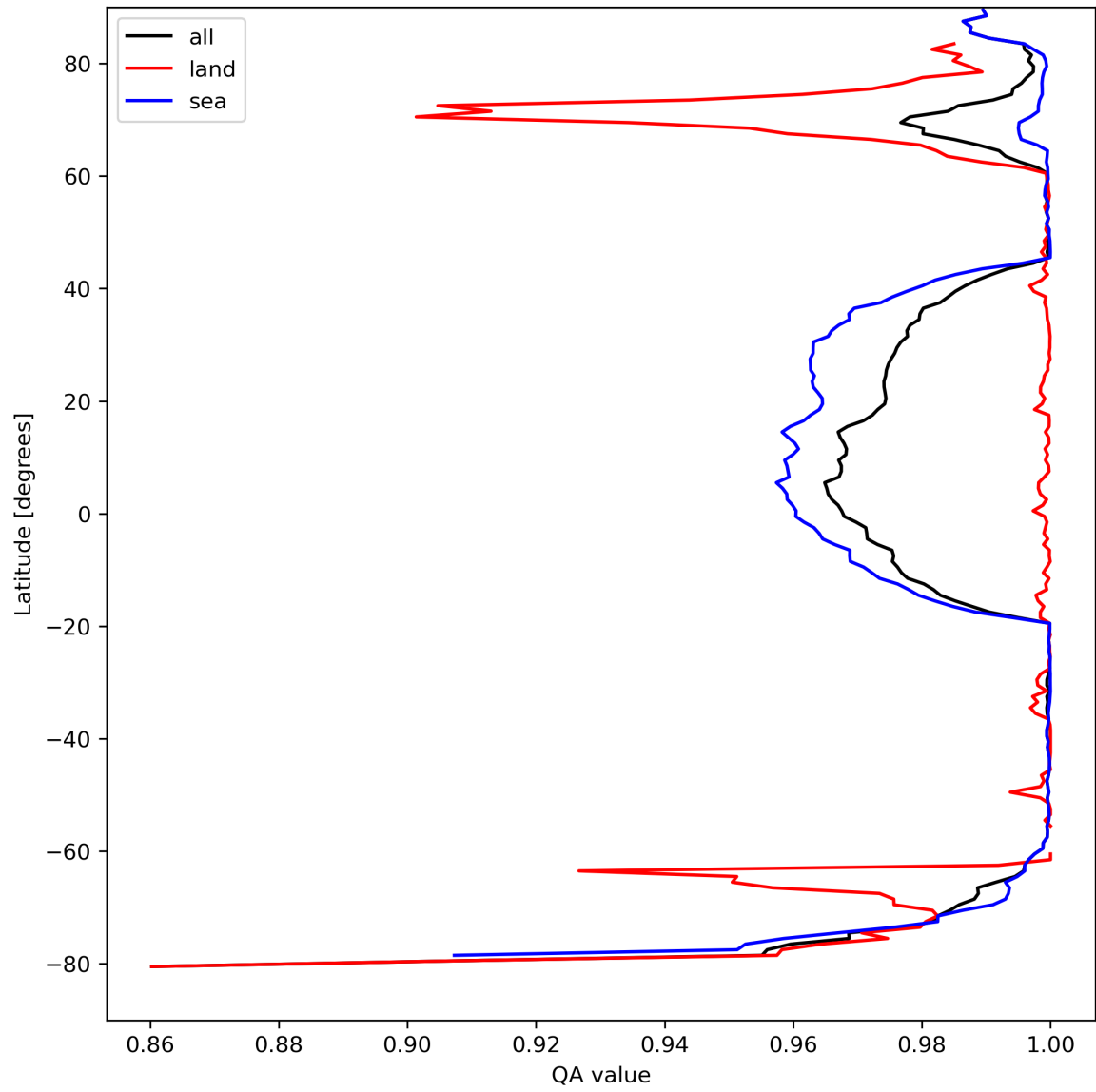
Figure 12: Zonal average of “QA value” for 2023-09-02 to 2023-09-04.
