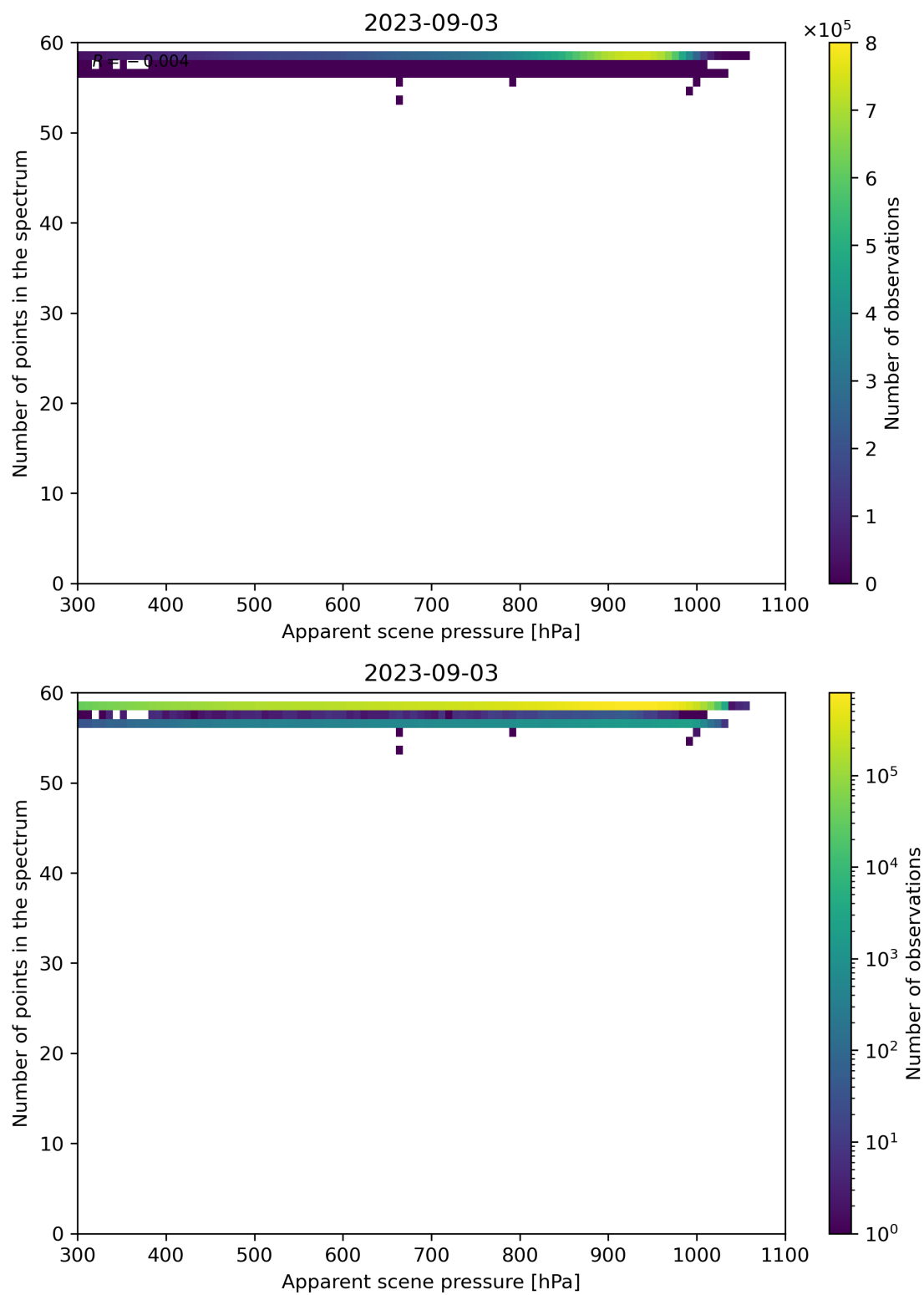
Figure 67: Scatter density plot of “Apparent scene pressure” against “Number of points in the spectrum” for 2023-09-02 to 2023-09-04.
