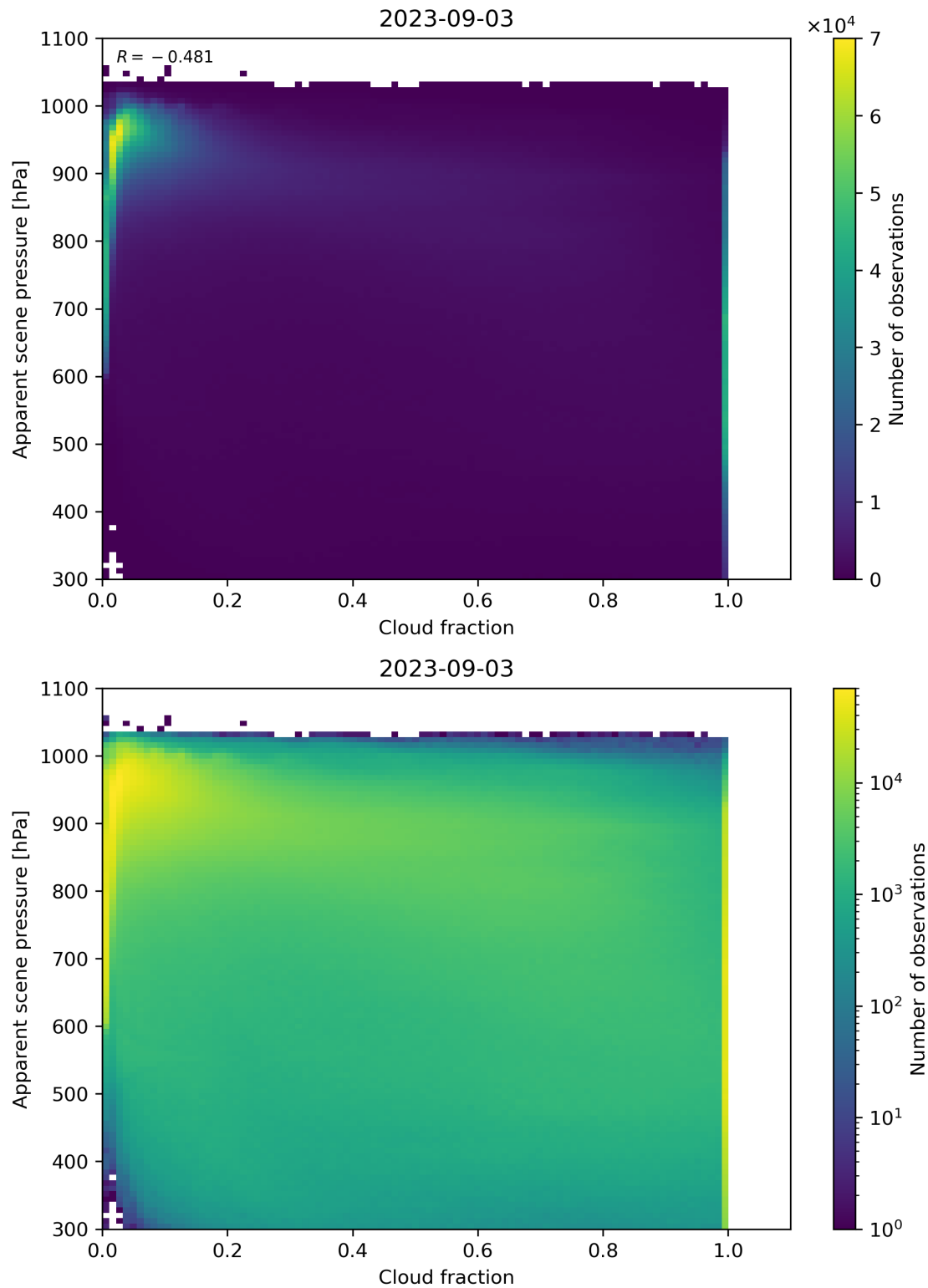
Figure 76: Scatter density plot of “Cloud fraction” against “Apparent scene pressure” for 2023-09-02 to 2023-09-04.
