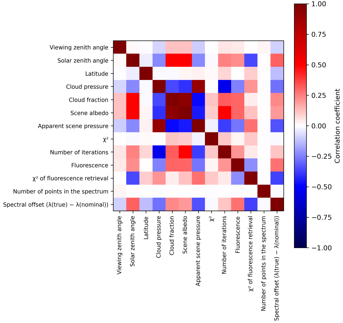
Figure 2: Map of correlation matrix for 2023-09-02 to 2023-09-04.
