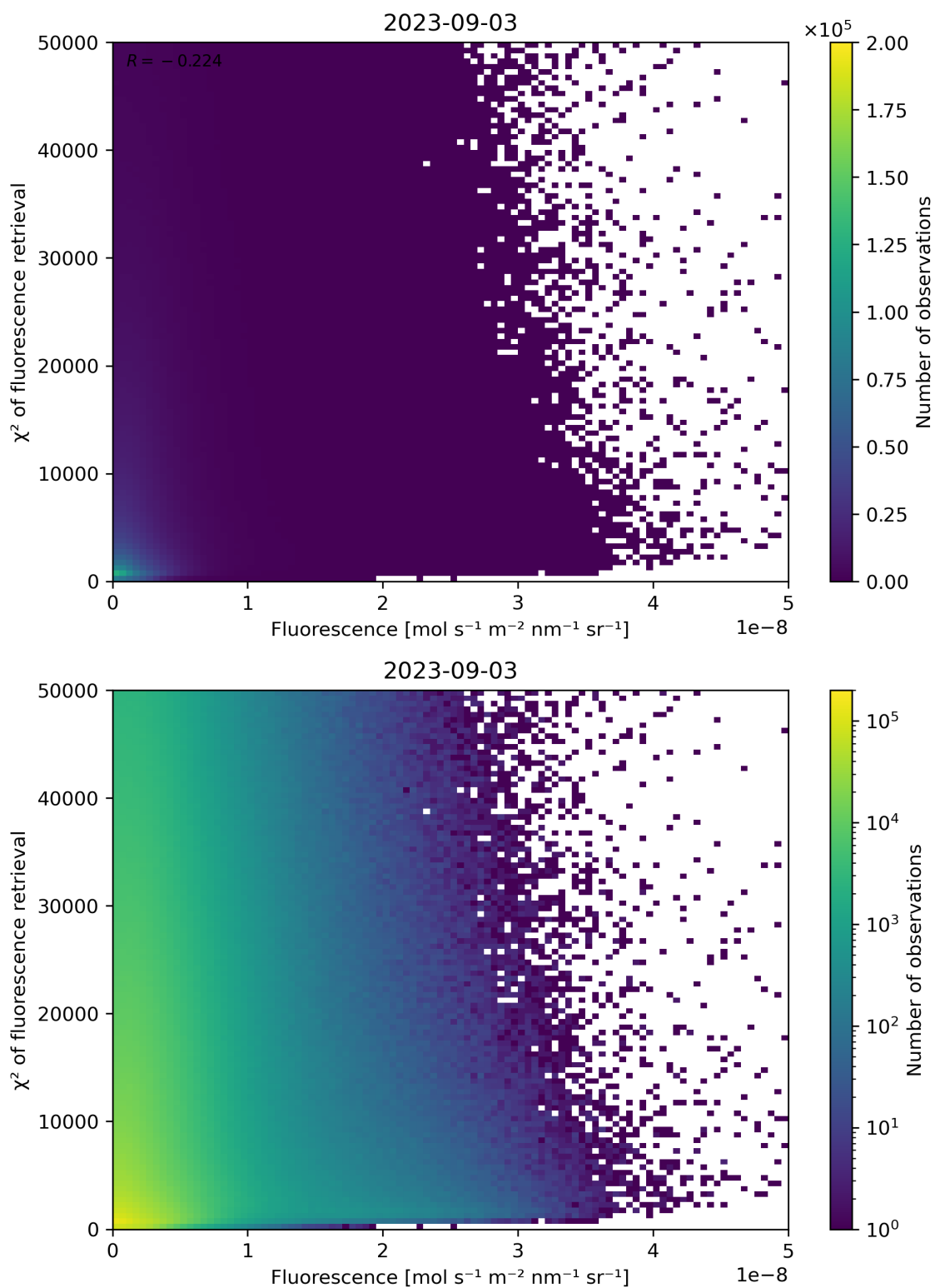
Figure 93: Scatter density plot of “Fluorescence” against “ \chi^2 of fluorescence retrieval” for 2023-09-02 to 2023-09-04.
