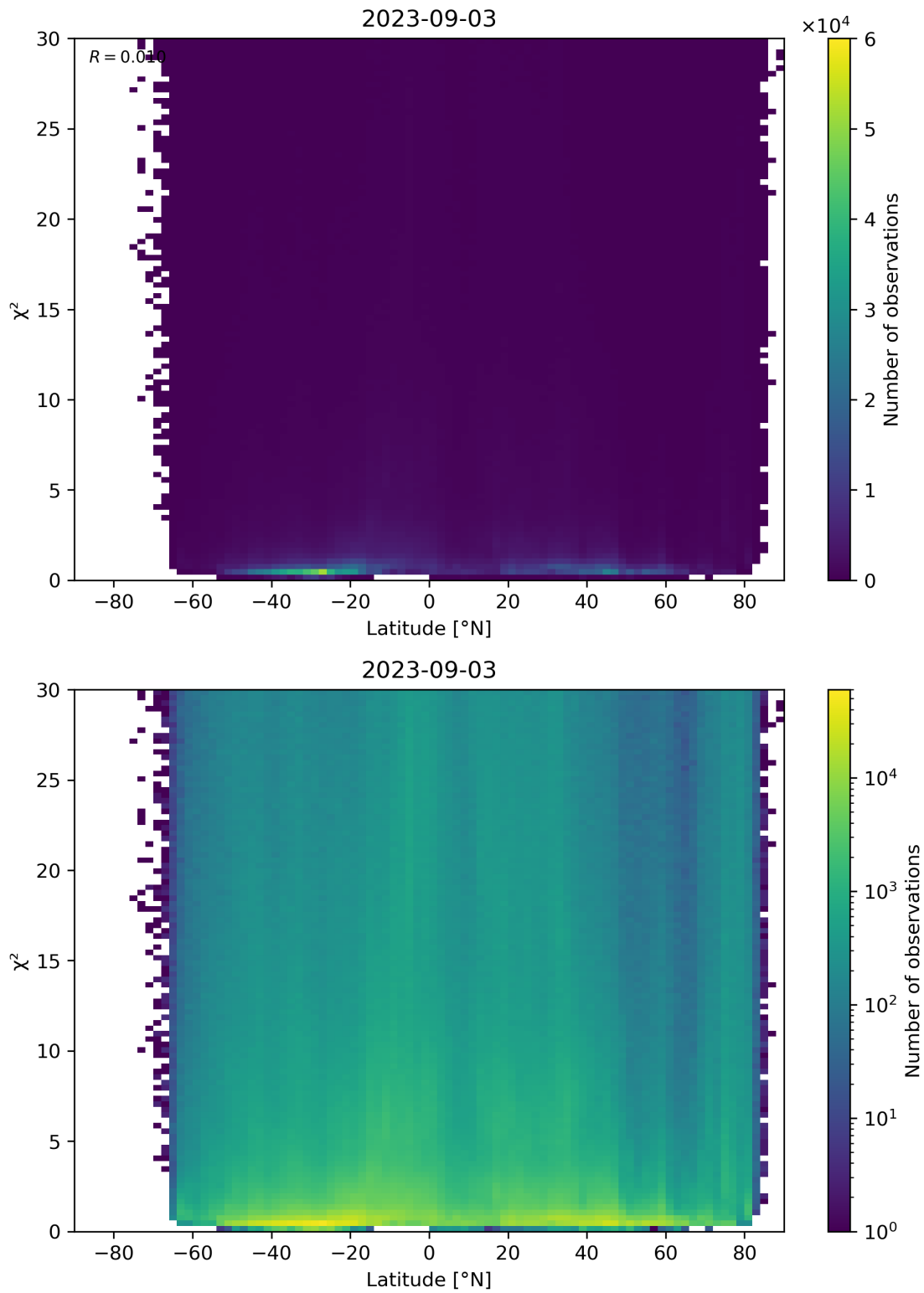
Figure 97: Scatter density plot of “Latitude” against “ \chi^2 ” for 2023-09-02 to 2023-09-04.
