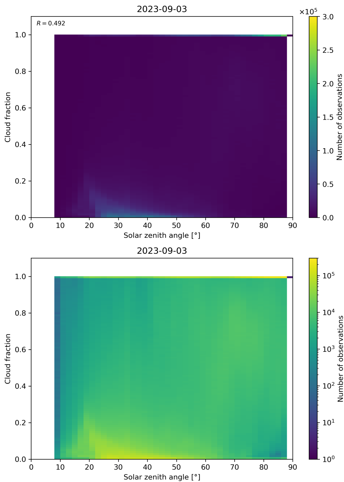
Figure 121: Scatter density plot of “Solar zenith angle” against “Cloud fraction” for 2023-09-02 to 2023-09-04.
