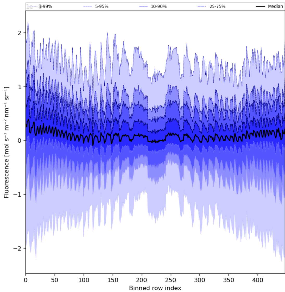
Figure 57: Along track statistics of “Fluorescence” for 2023-09-02 to 2023-09-04
