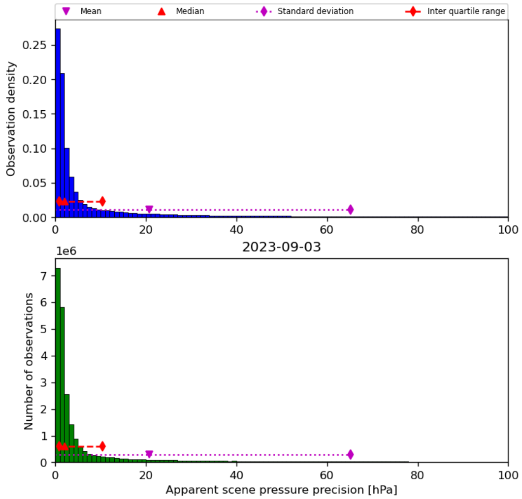
Figure 37: Histogram of “Apparent scene pressure precision” for 2023-09-02 to 2023-09-04
