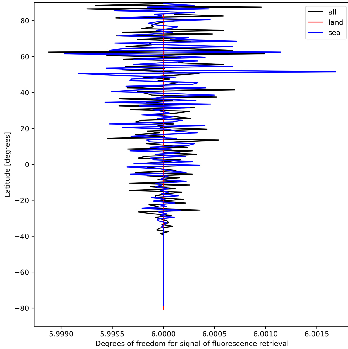
Figure 26: Zonal average of “Degrees of freedom for signal of fluorescence retrieval” for 2023-09-02 to 2023-09-04.
