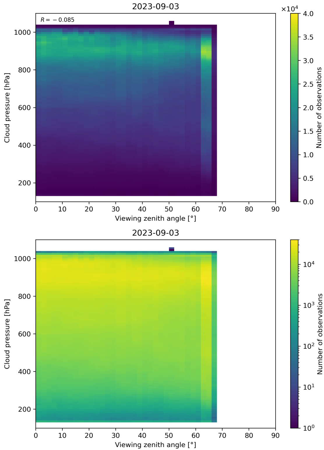
Figure 133: Scatter density plot of “Viewing zenith angle” against “Cloud pressure” for 2023-09-02 to 2023-09-04.
