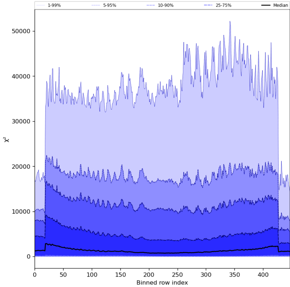
Figure 55: Along track statistics of “ \chi^2 ” for 2023-09-02 to 2023-09-04
