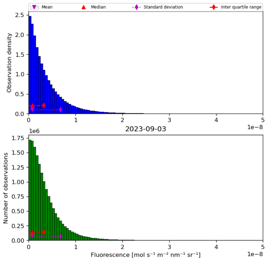
Figure 40: Histogram of “Fluorescence” for 2023-09-02 to 2023-09-04
