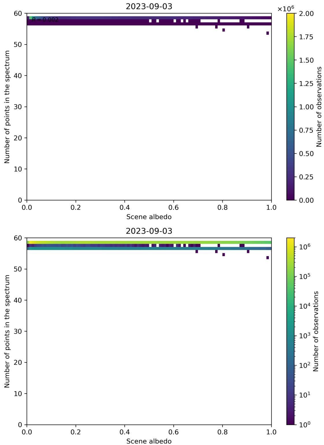
Figure 116: Scatter density plot of “Scene albedo” against “Number of points in the spectrum” for 2023-09-02 to 2023-09-04.
