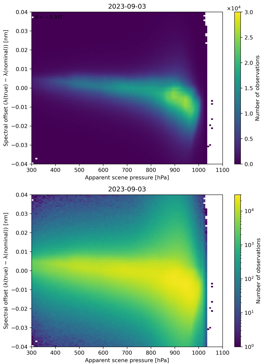
Figure 68: Scatter density plot of “Apparent scene pressure” against “Spectral offset ( \lambda(\text{true}) - \lambda(\text{nominal}) )” for 2023-09-02 to 2023-09-04.
