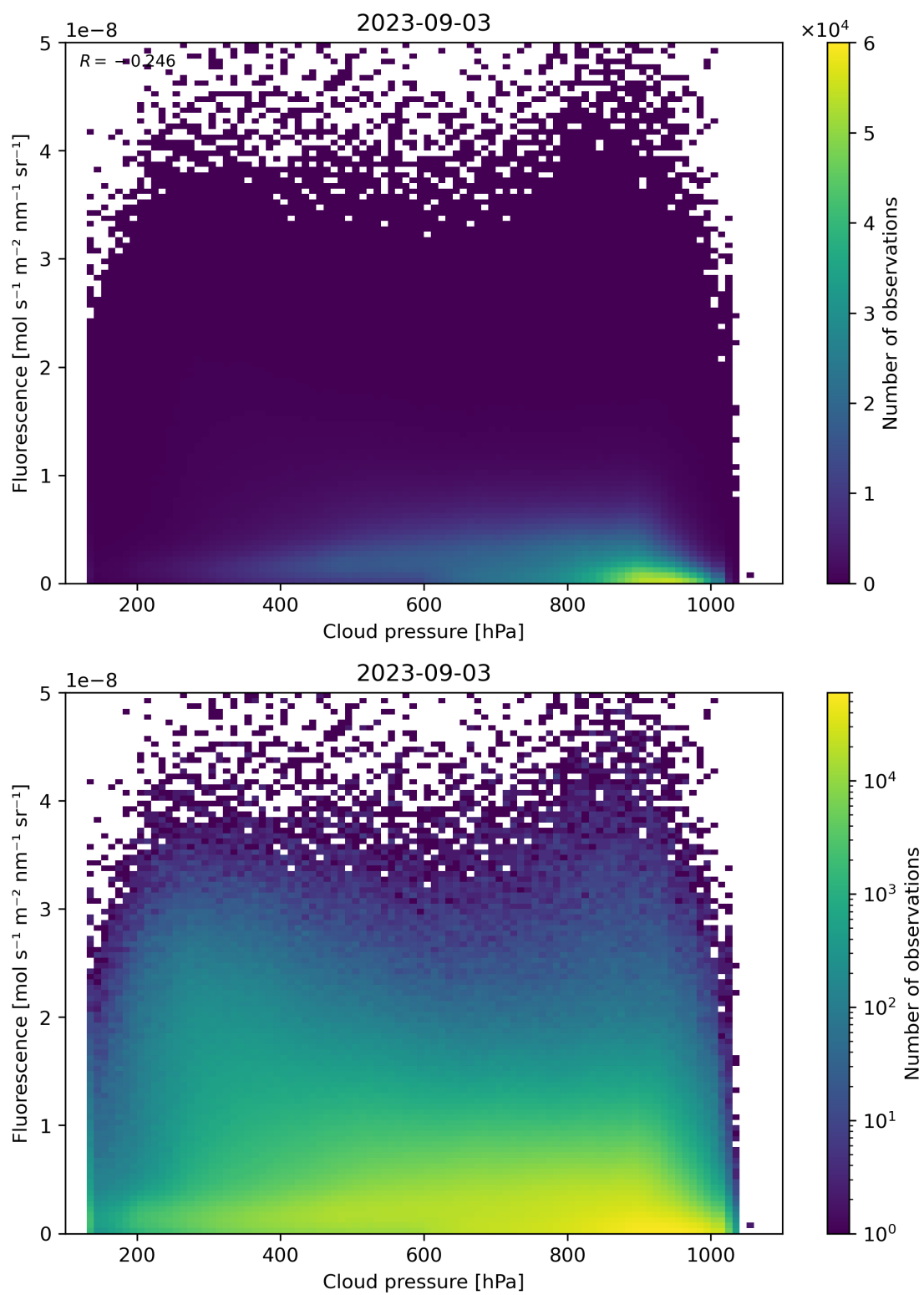
Figure 88: Scatter density plot of “Cloud pressure” against “Fluorescence” for 2023-09-02 to 2023-09-04.
