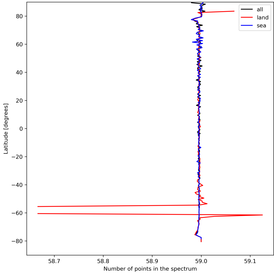
Figure 27: Zonal average of “Number of points in the spectrum” for 2023-09-02 to 2023-09-04.
