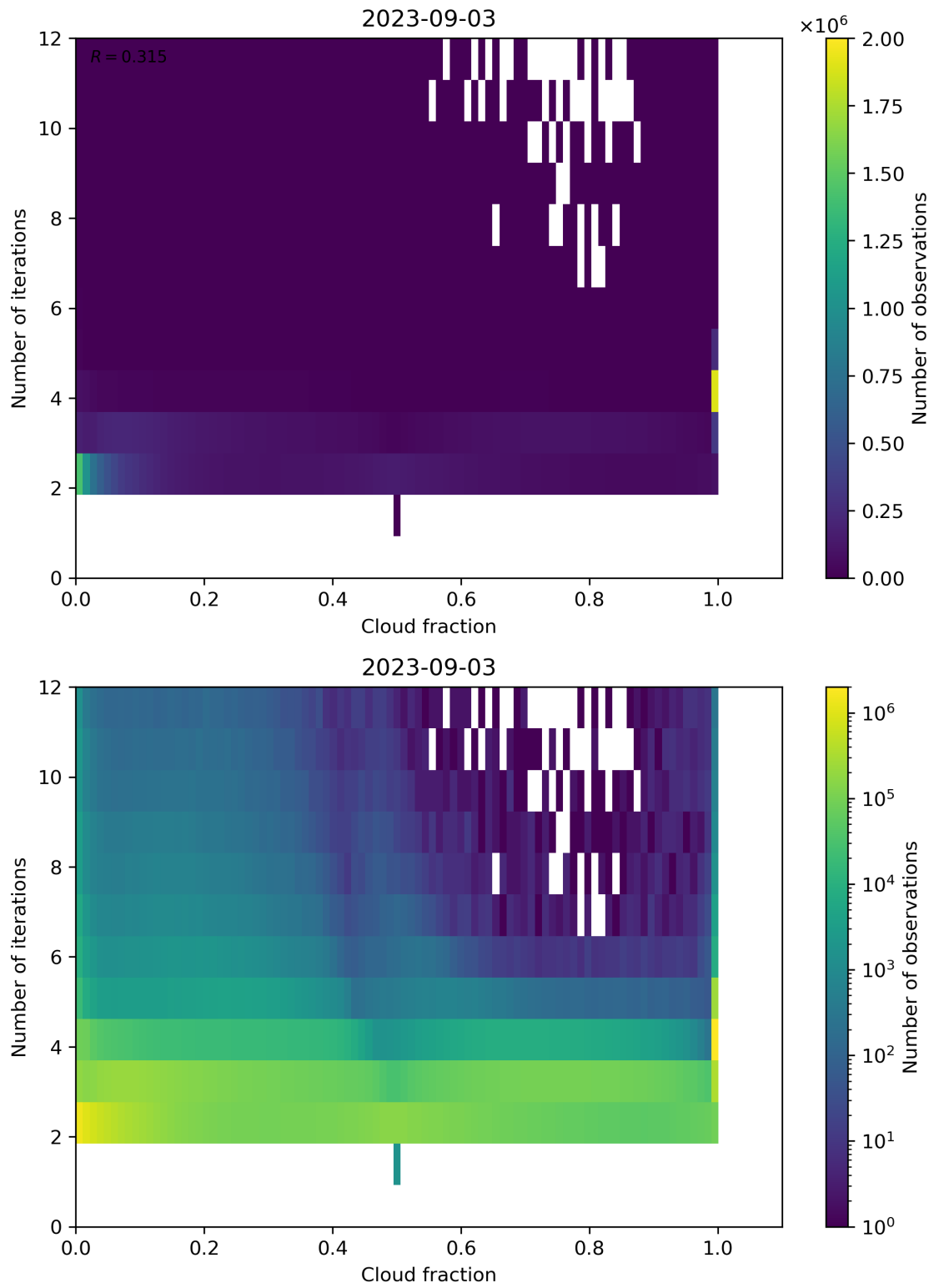
Figure 80: Scatter density plot of “Cloud fraction” against “Number of iterations” for 2023-09-02 to 2023-09-04.
