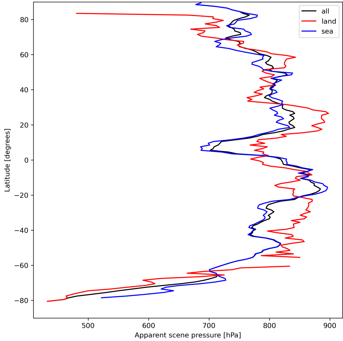
Figure 19: Zonal average of “Apparent scene pressure” for 2023-09-02 to 2023-09-04.
