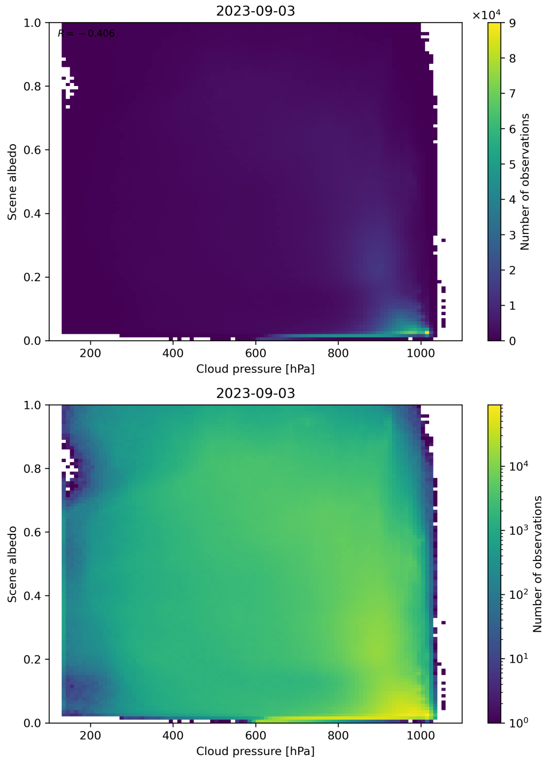
Figure 91: Scatter density plot of “Cloud pressure” against “Scene albedo” for 2023-09-02 to 2023-09-04.
