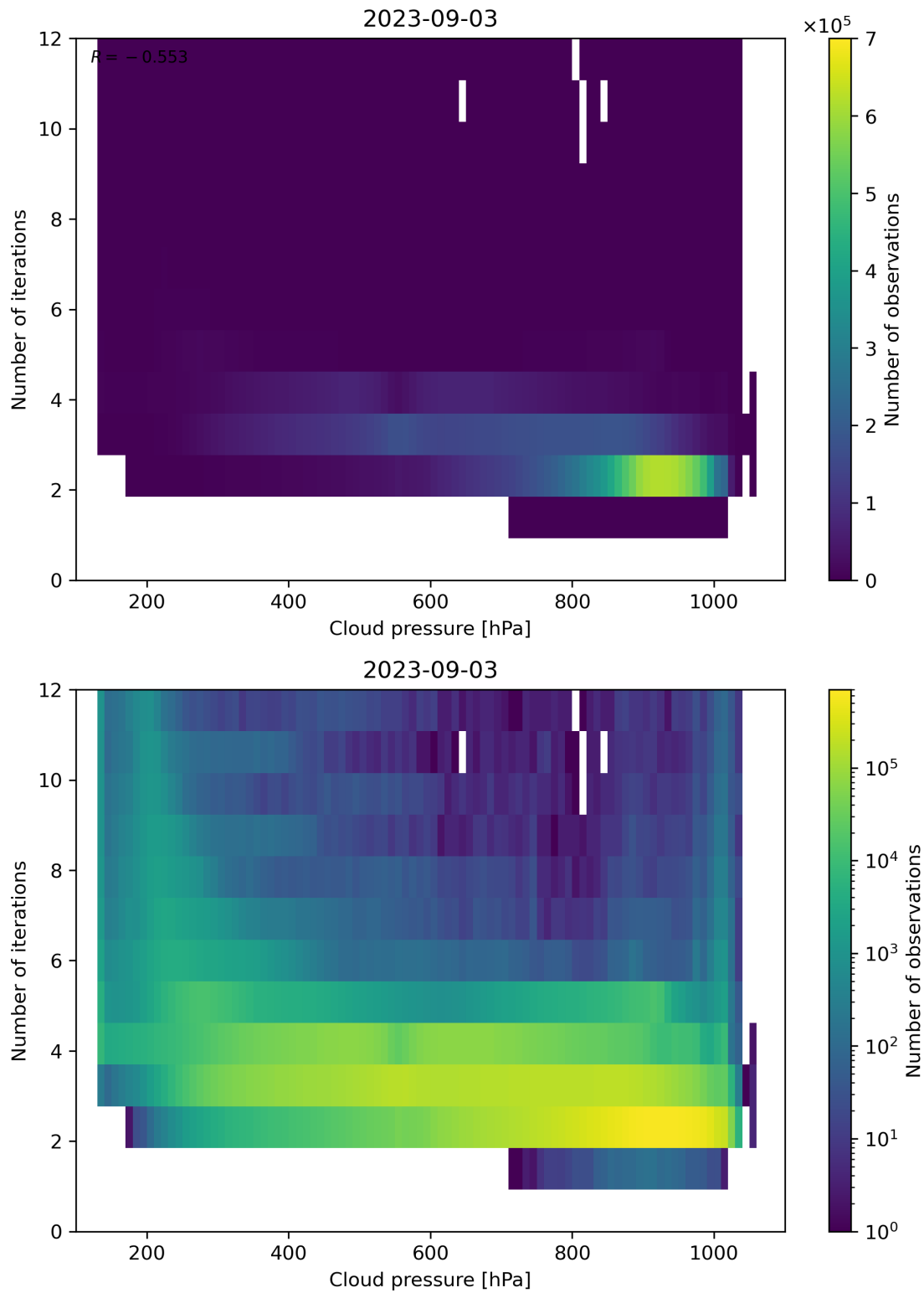
Figure 89: Scatter density plot of “Cloud pressure” against “Number of iterations” for 2023-09-02 to 2023-09-04.
