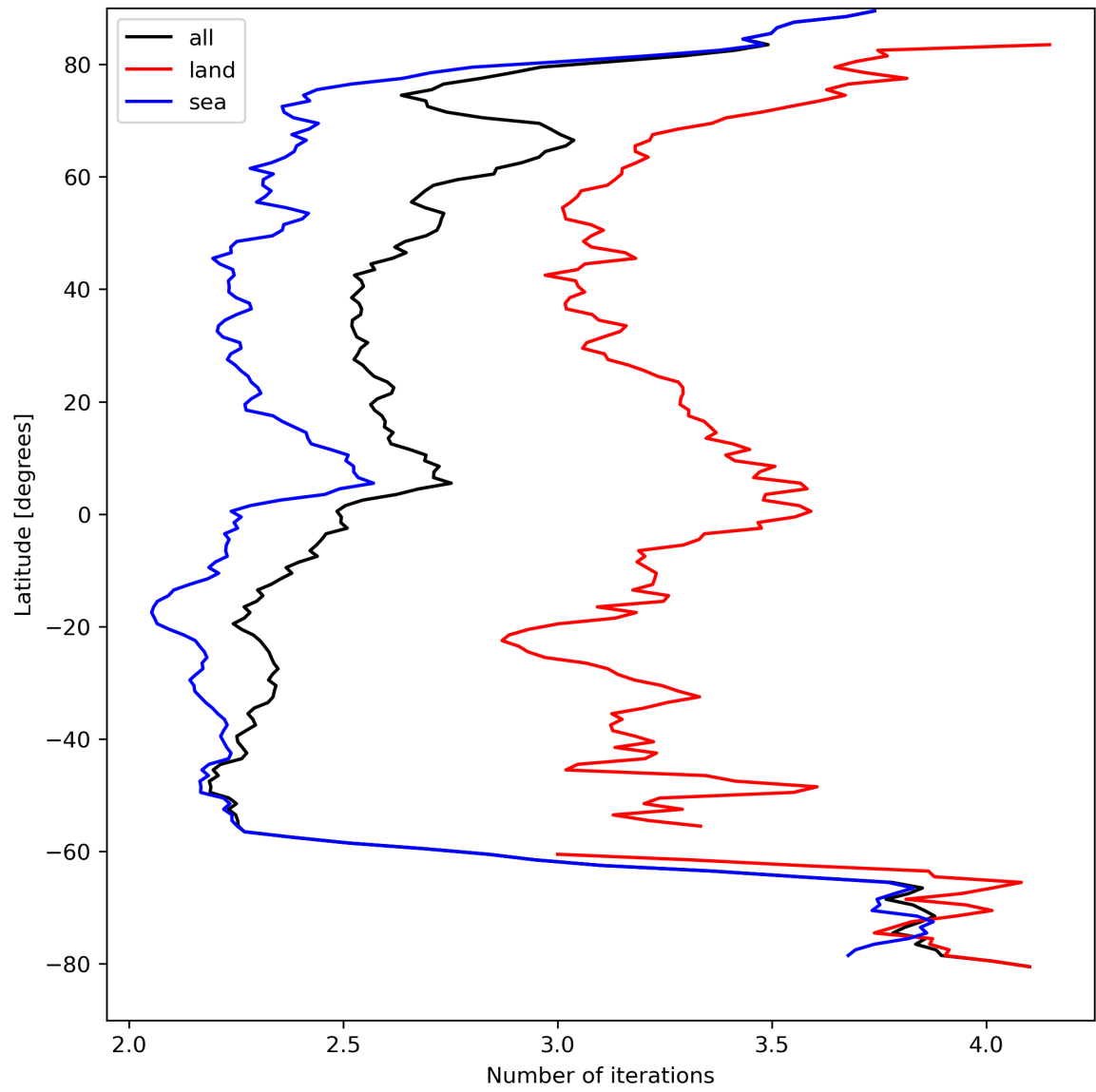
Figure 22: Zonal average of “Number of iterations” for 2023-09-02 to 2023-09-04.
