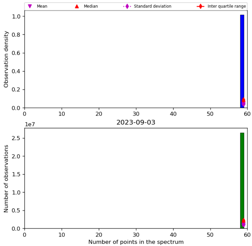
Figure 44: Histogram of “Number of points in the spectrum” for 2023-09-02 to 2023-09-04
