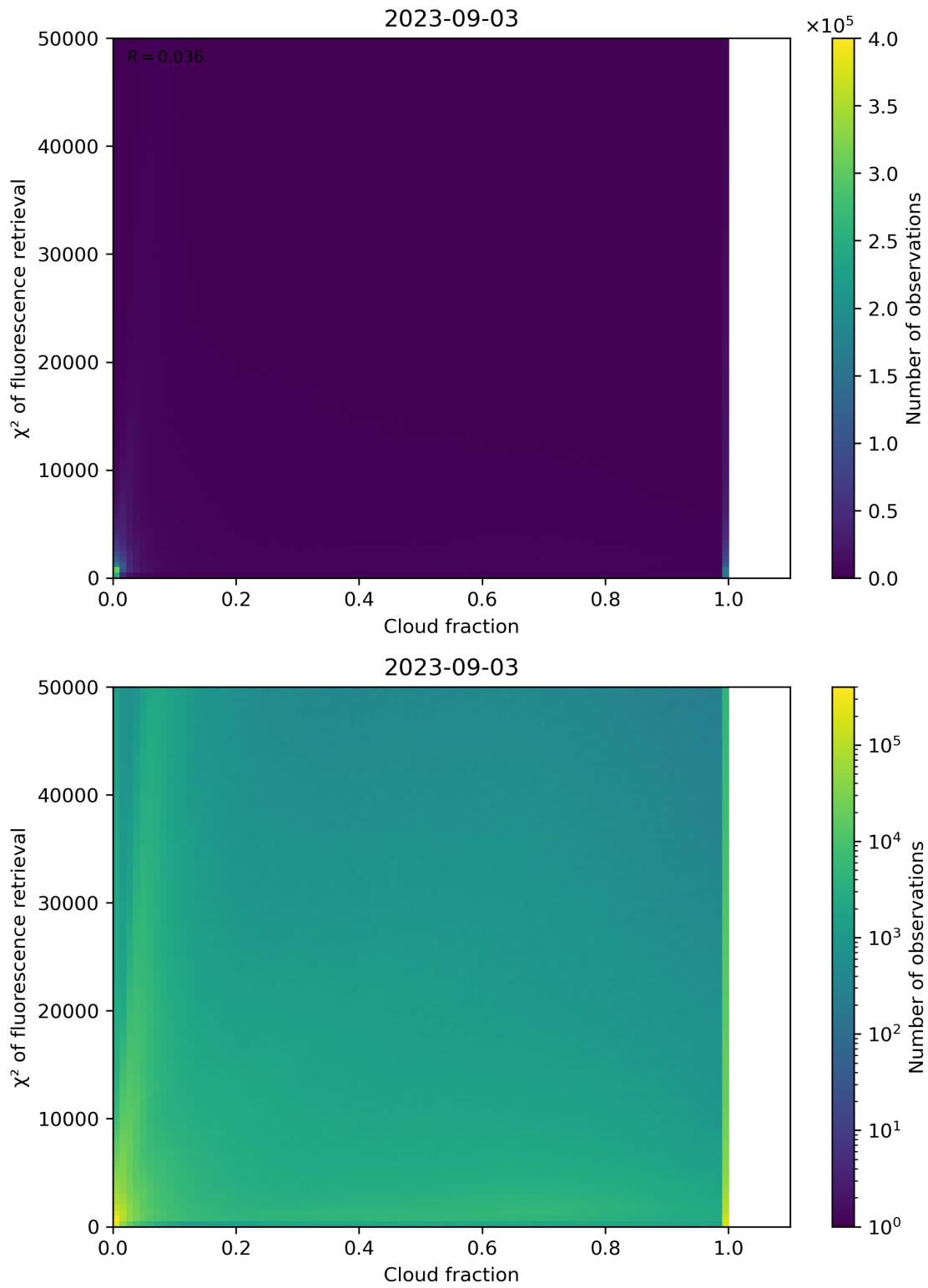
Figure 78: Scatter density plot of “Cloud fraction” against “ \chi^2 of fluorescence retrieval” for 2023-09-02 to 2023-09-04.
