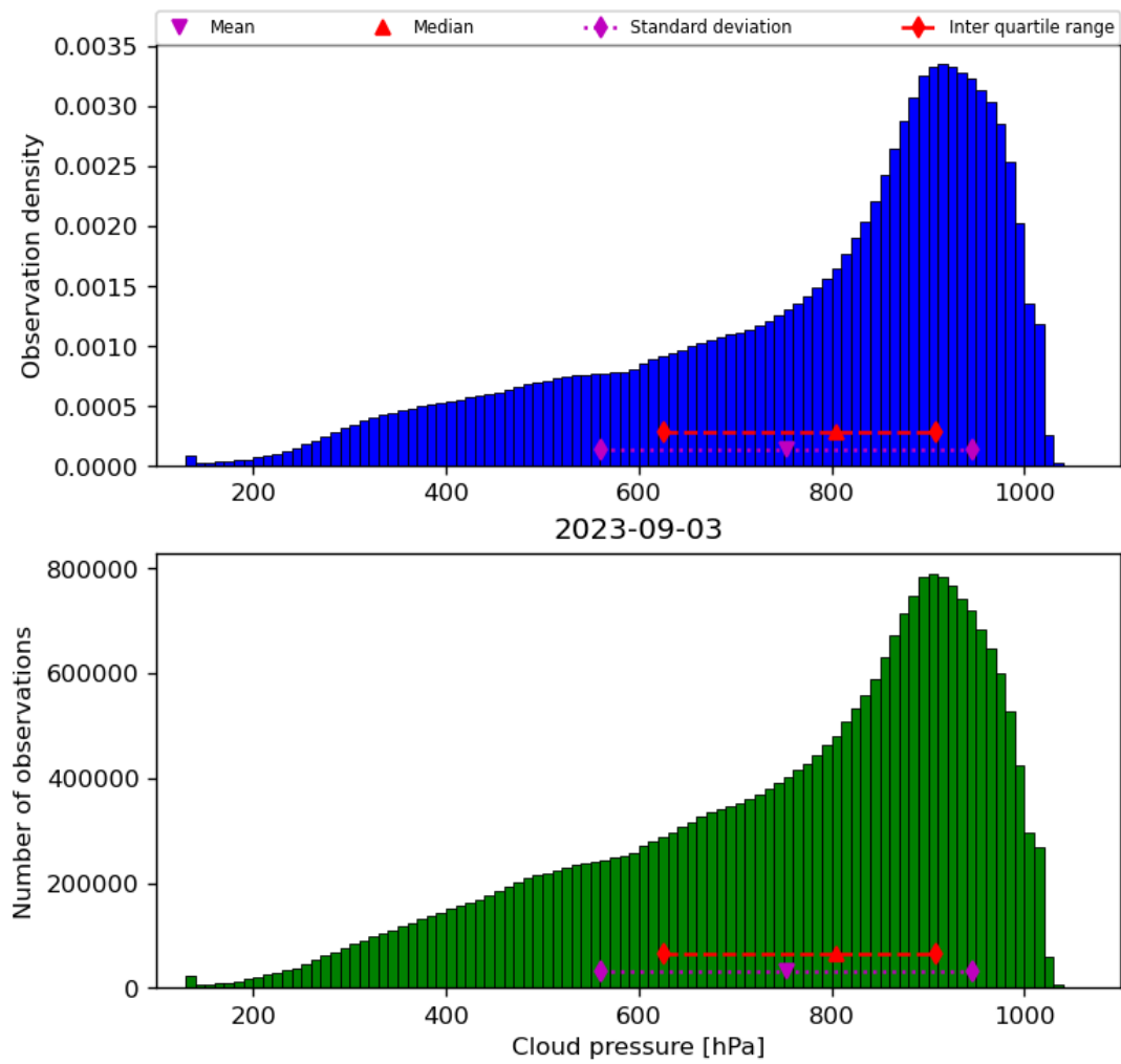
Figure 30: Histogram of “Cloud pressure” for 2023-09-02 to 2023-09-04
