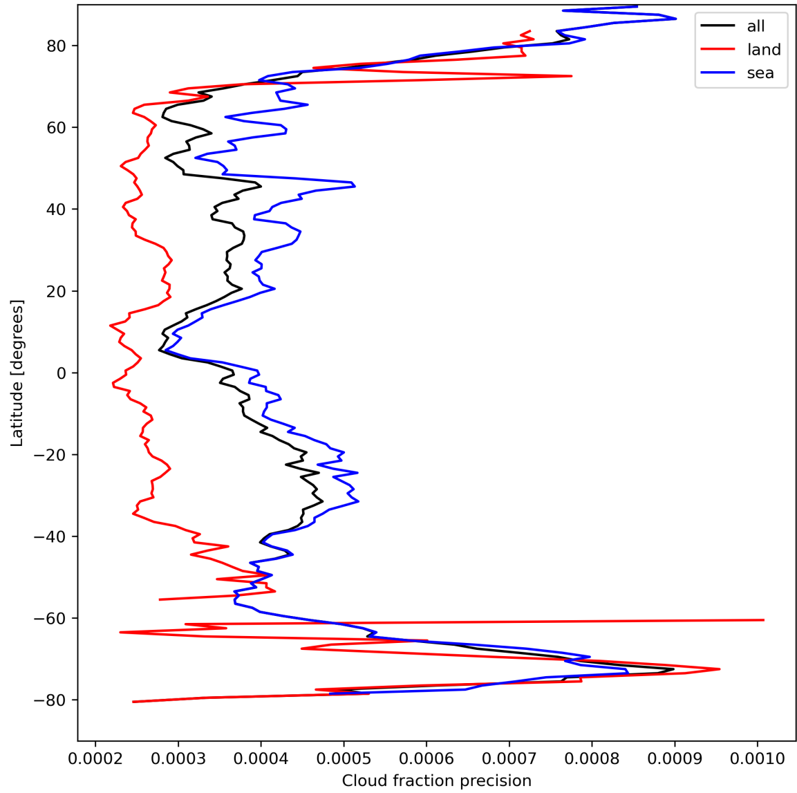
Figure 16: Zonal average of “Cloud fraction precision” for 2023-09-02 to 2023-09-04.
