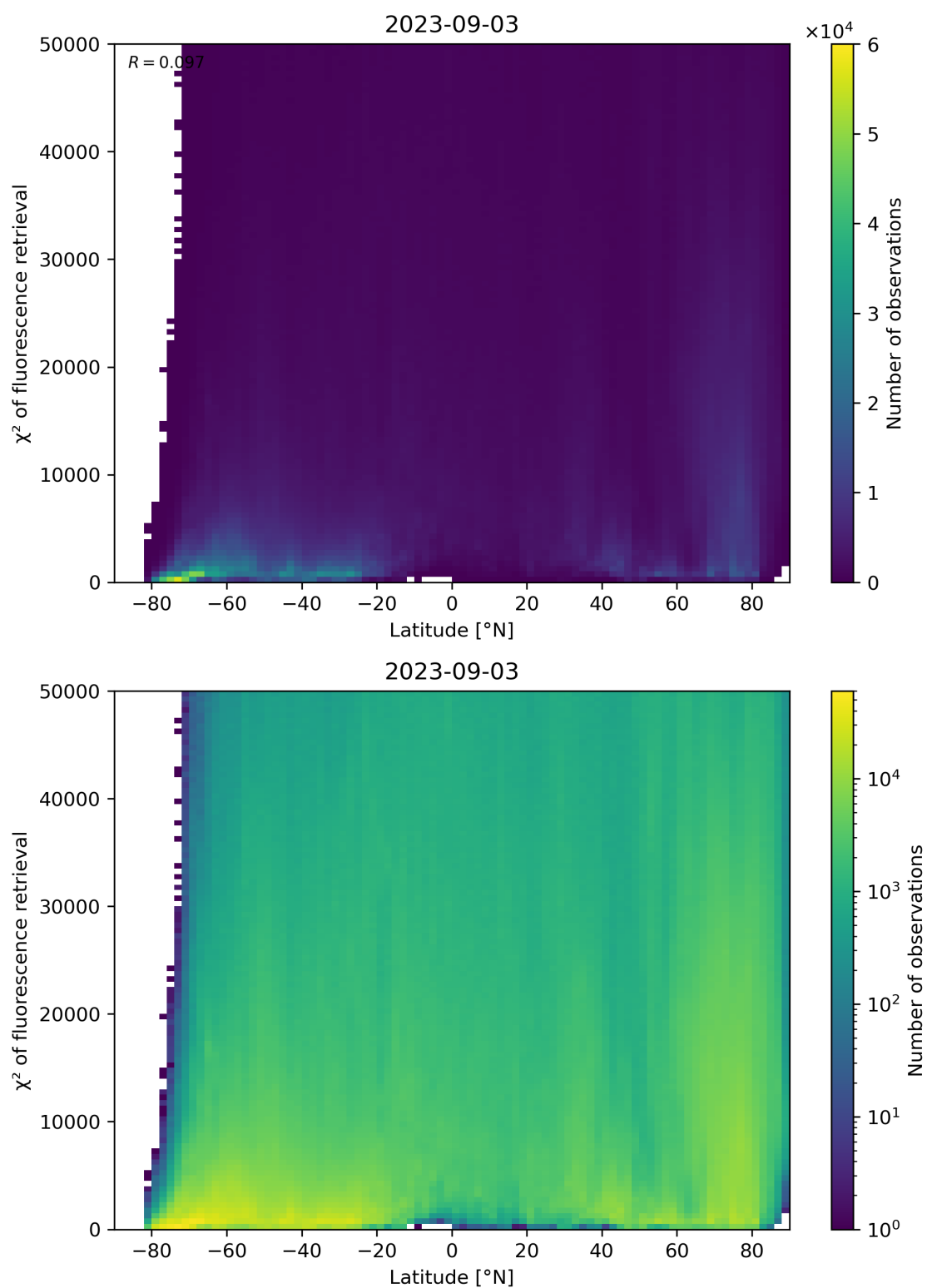
Figure 98: Scatter density plot of “Latitude” against “ \chi^2 of fluorescence retrieval” for 2023-09-02 to 2023-09-04.
