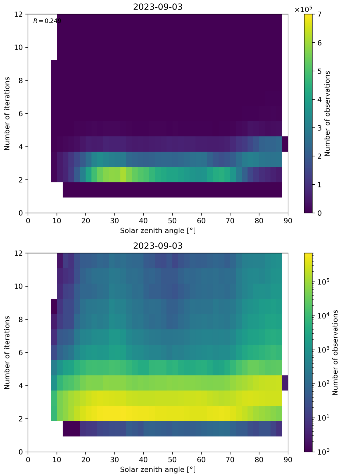
Figure 125: Scatter density plot of “Solar zenith angle” against “Number of iterations” for 2023-09-02 to 2023-09-04.
