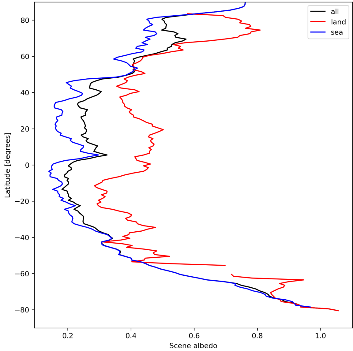
Figure 17: Zonal average of “Scene albedo” for 2023-09-02 to 2023-09-04.
