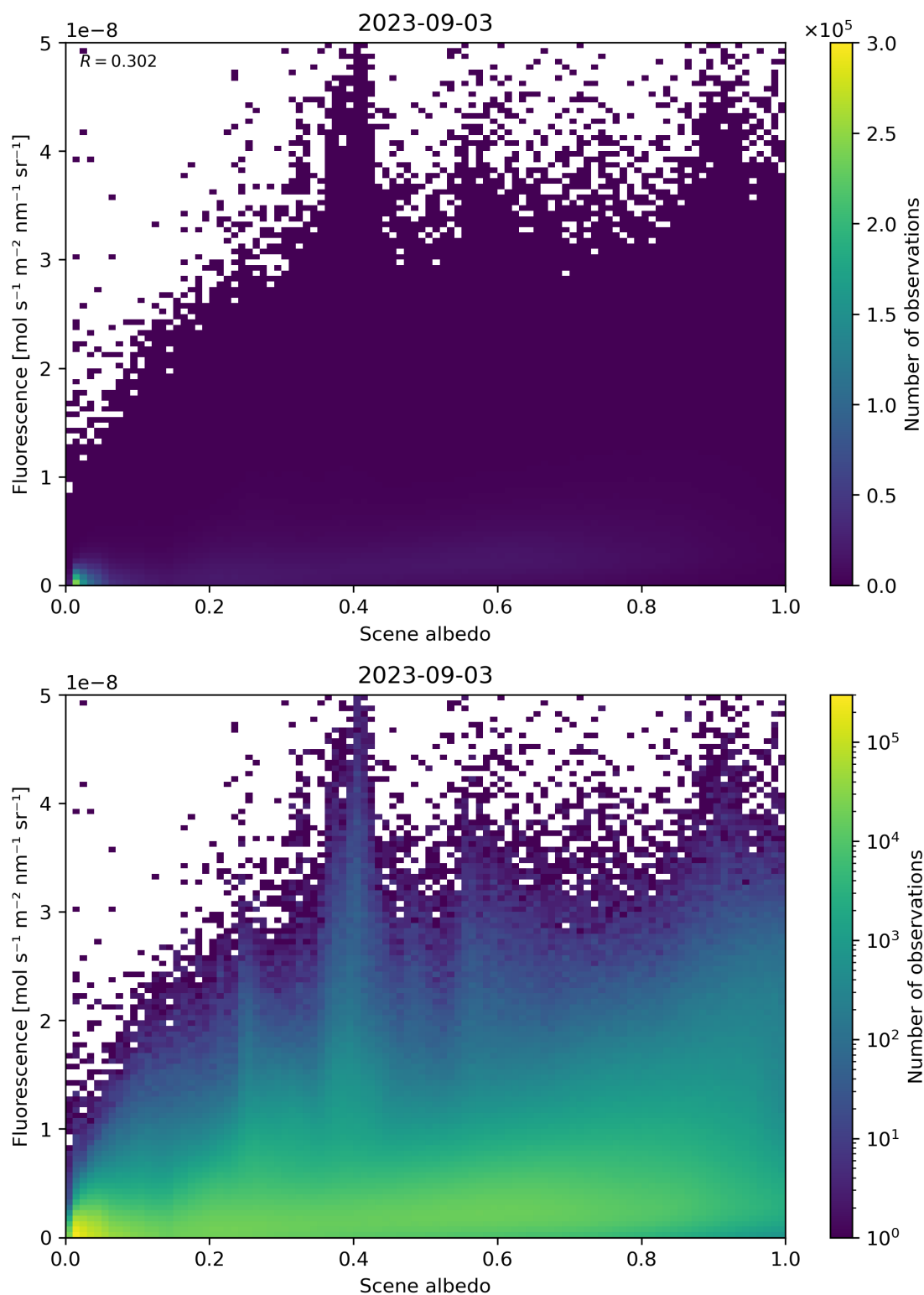
Figure 114: Scatter density plot of “Scene albedo” against “Fluorescence” for 2023-09-02 to 2023-09-04.
