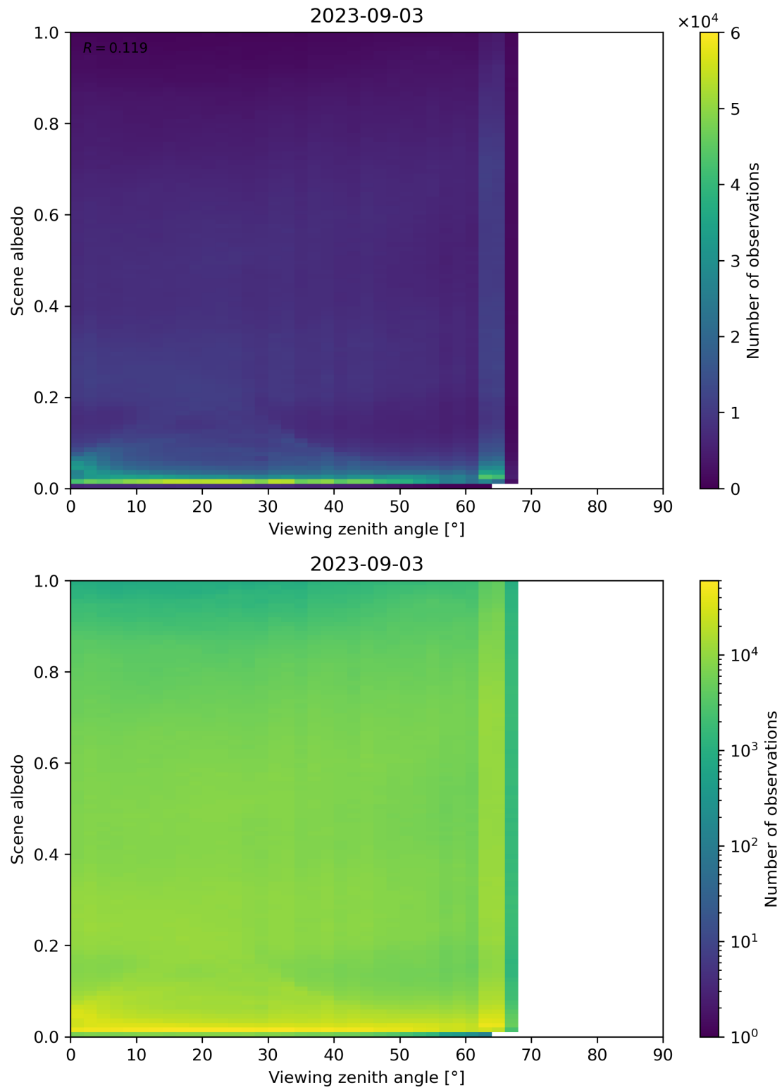
Figure 138: Scatter density plot of “Viewing zenith angle” against “Scene albedo” for 2023-09-02 to 2023-09-04.
