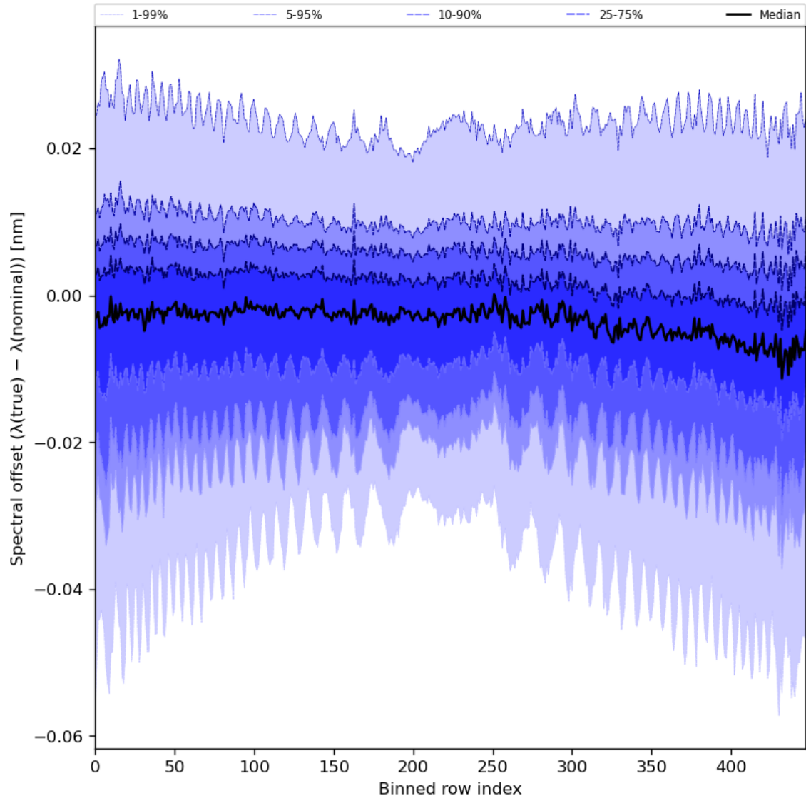
Figure 62: Along track statistics of “Spectral offset ( \lambda(\text{true}) - \lambda(\text{nominal}) )” for 2023-09-02 to 2023-09-04
