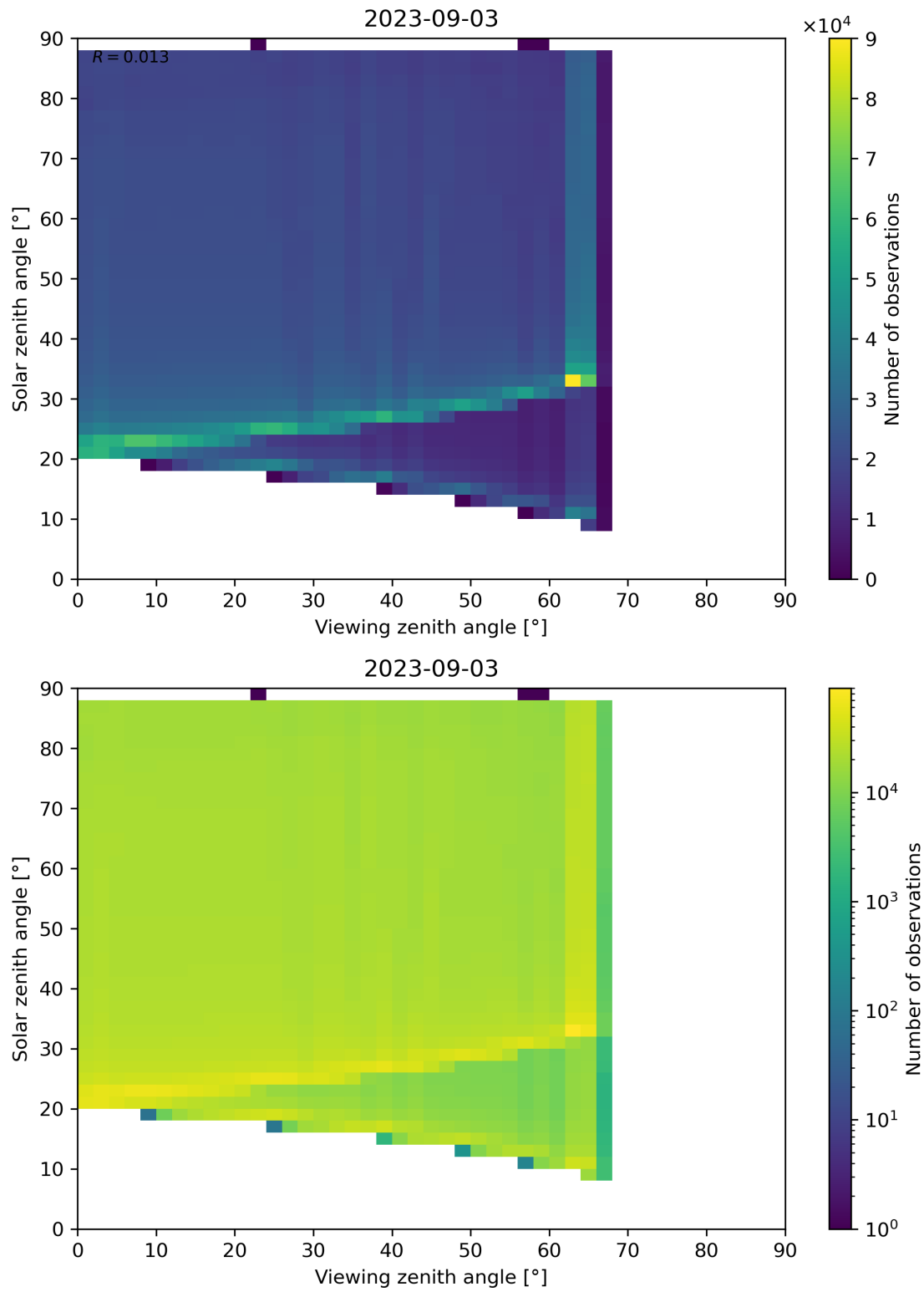
Figure 139: Scatter density plot of “Viewing zenith angle” against “Solar zenith angle” for 2023-09-02 to 2023-09-04.
