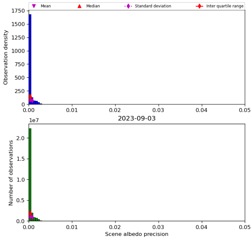
Figure 35: Histogram of “Scene albedo precision” for 2023-09-02 to 2023-09-04
