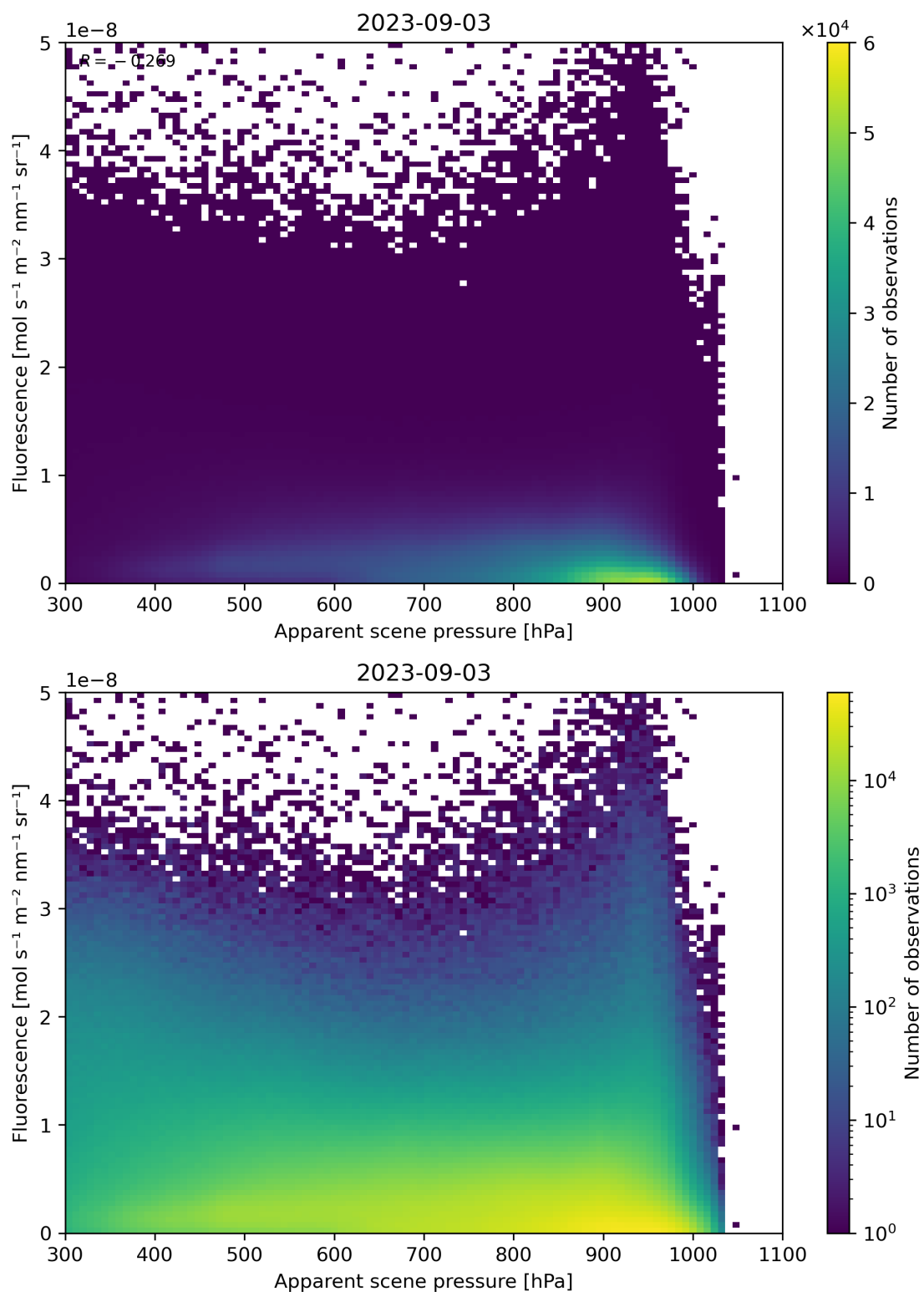
Figure 65: Scatter density plot of “Apparent scene pressure” against “Fluorescence” for 2023-09-02 to 2023-09-04.
