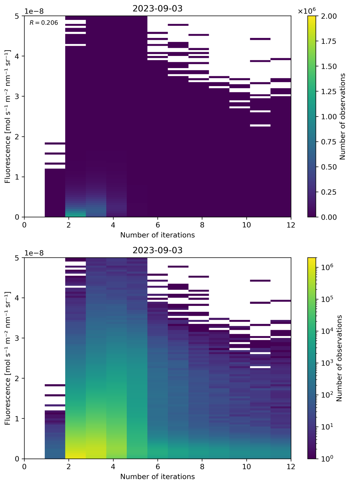
Figure 107: Scatter density plot of “Number of iterations” against “Fluorescence” for 2023-09-02 to 2023-09-04.
