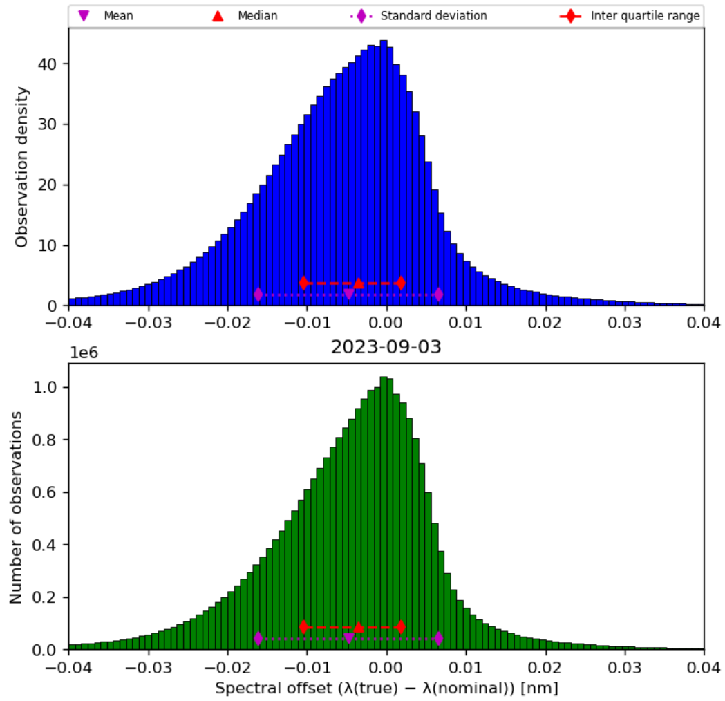
Figure 45: Histogram of “Spectral offset ( \lambda(\text{true}) - \lambda(\text{nominal}) )” for 2023-09-02 to 2023-09-04
