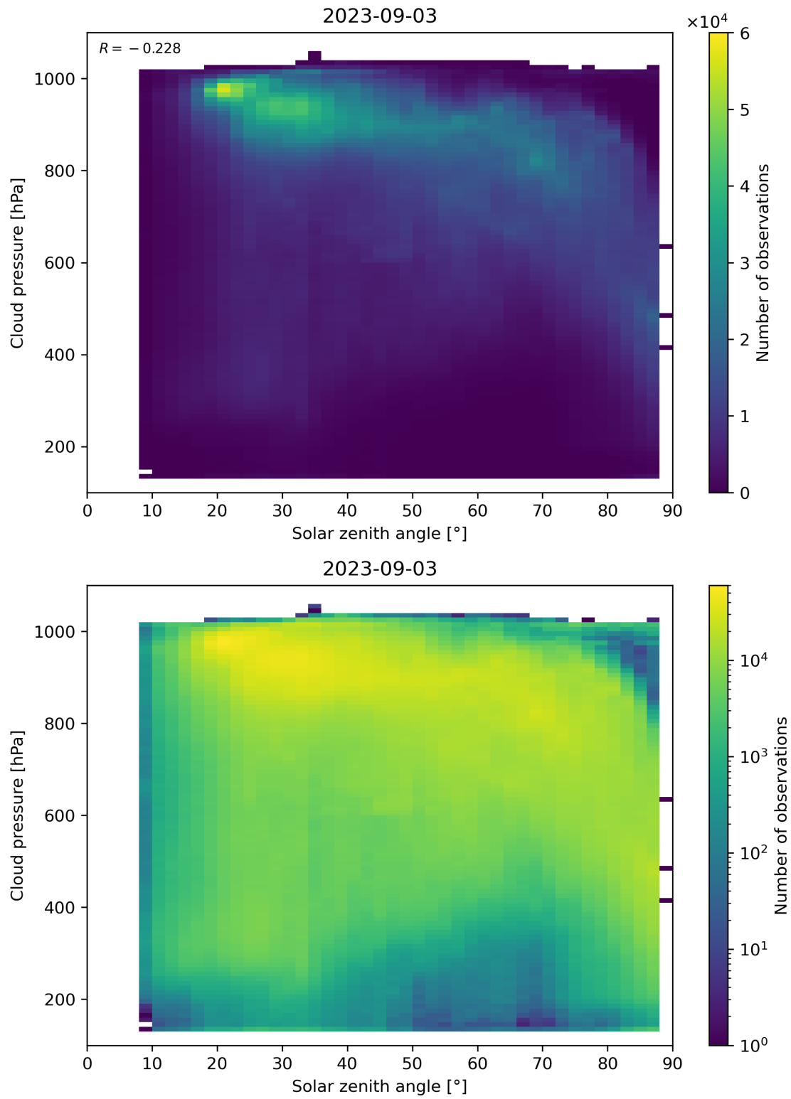
Figure 122: Scatter density plot of “Solar zenith angle” against “Cloud pressure” for 2023-09-02 to 2023-09-04.
