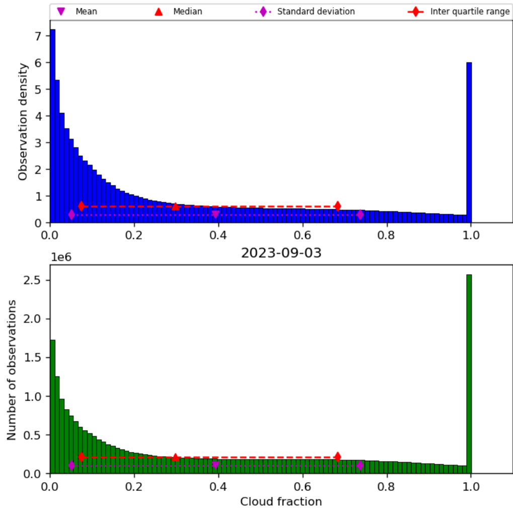
Figure 32: Histogram of “Cloud fraction” for 2023-09-02 to 2023-09-04
