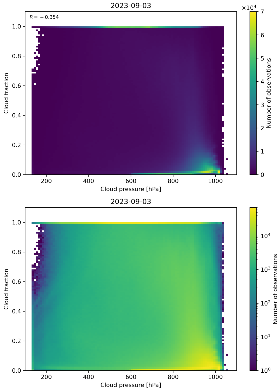
Figure 87: Scatter density plot of “Cloud pressure” against “Cloud fraction” for 2023-09-02 to 2023-09-04.
