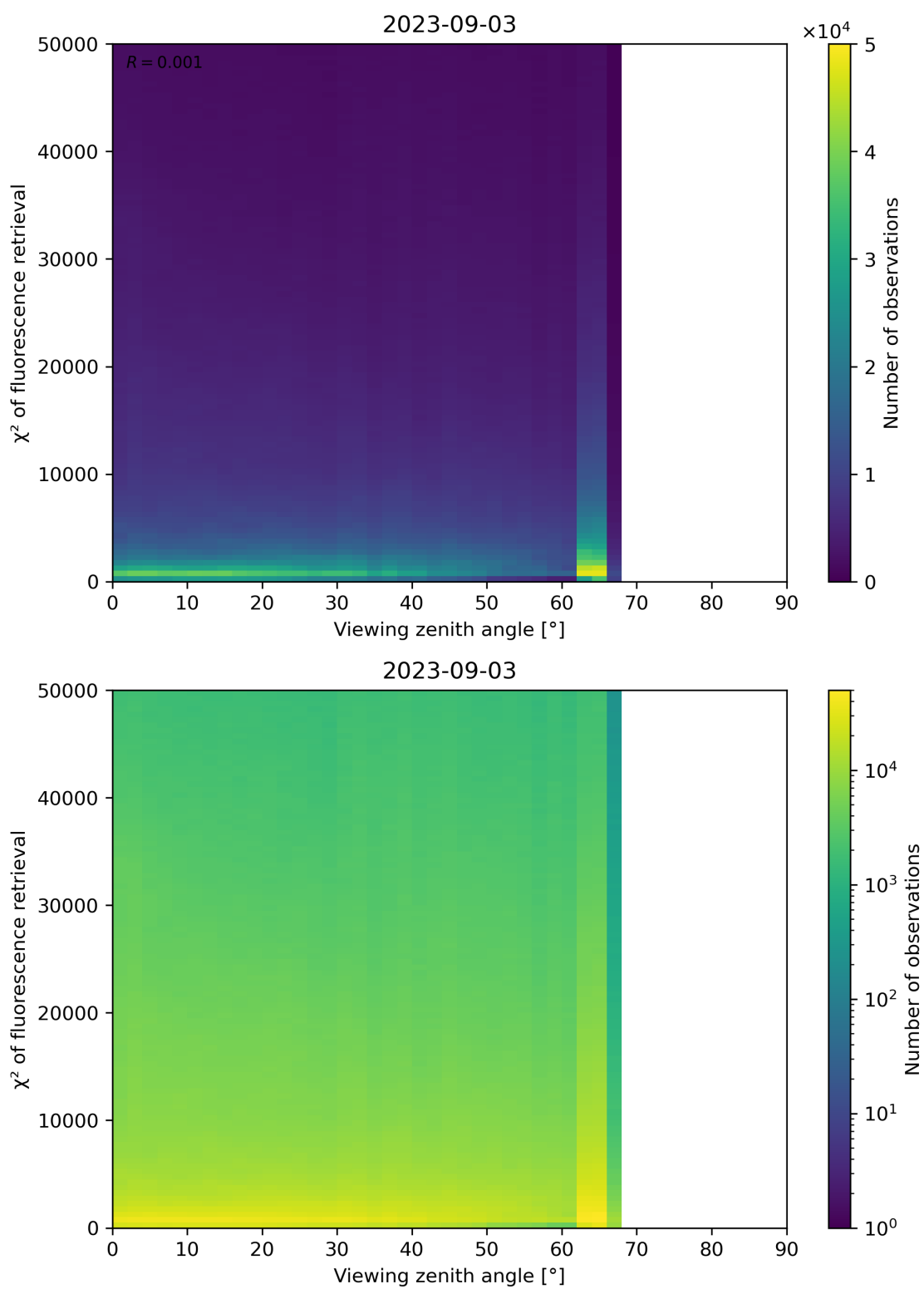
Figure 131: Scatter density plot of “Viewing zenith angle” against “ \chi^2 of fluorescence retrieval” for 2023-09-02 to 2023-09-04.
