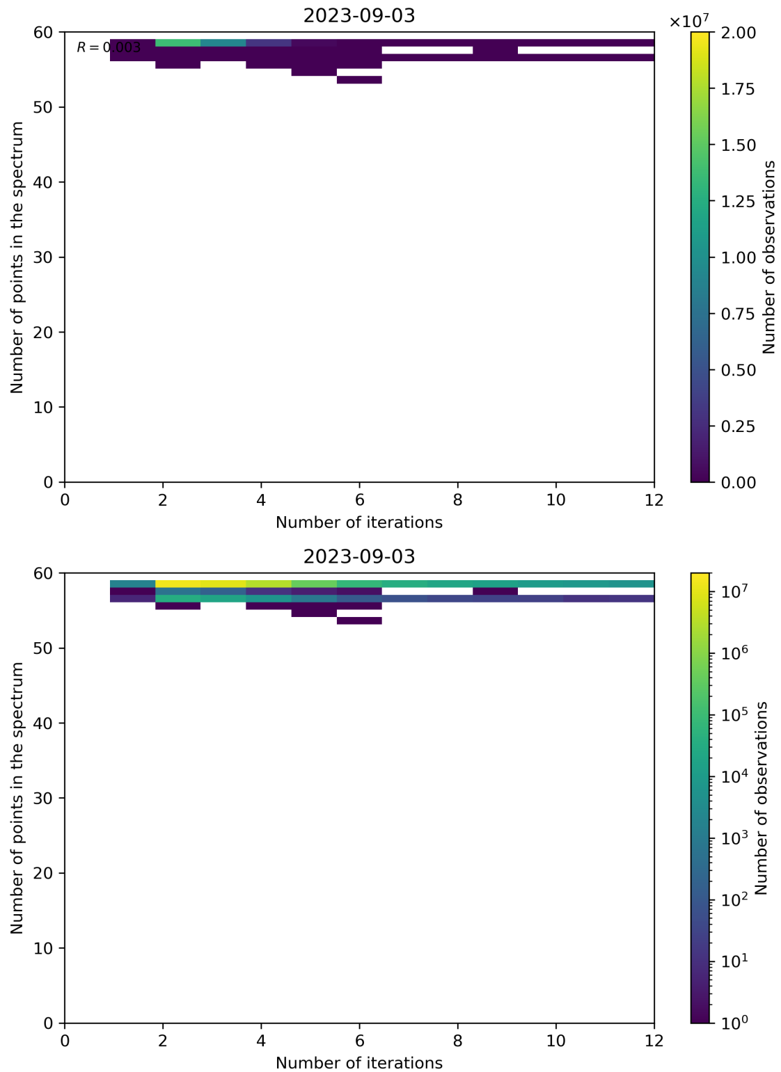
Figure 108: Scatter density plot of “Number of iterations” against “Number of points in the spectrum” for 2023-09-02 to 2023-09-04.
