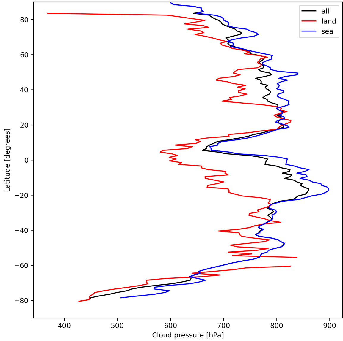
Figure 13: Zonal average of “Cloud pressure” for 2023-09-02 to 2023-09-04.
