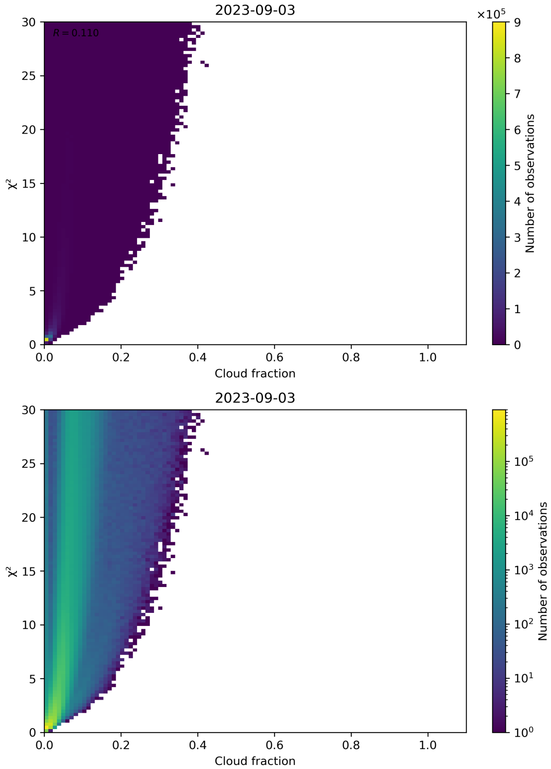
Figure 77: Scatter density plot of “Cloud fraction” against “ \chi^2 ” for 2023-09-02 to 2023-09-04.
