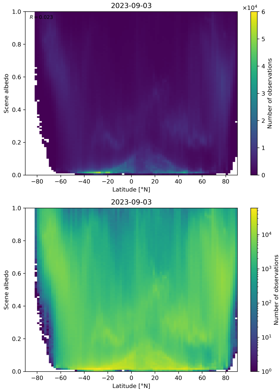
Figure 104: Scatter density plot of “Latitude” against “Scene albedo” for 2023-09-02 to 2023-09-04.
