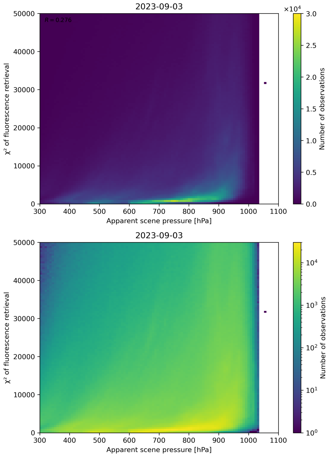
Figure 64: Scatter density plot of “Apparent scene pressure” against “ \chi^2 of fluorescence retrieval” for 2023-09-02 to 2023-09-04.
