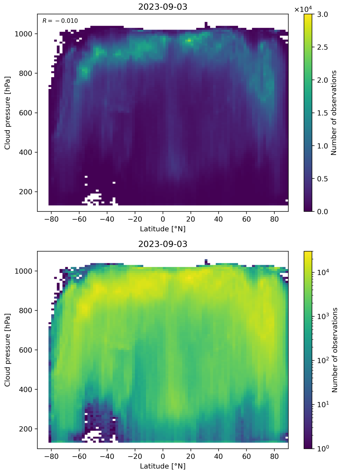
Figure 100: Scatter density plot of “Latitude” against “Cloud pressure” for 2023-09-02 to 2023-09-04.
