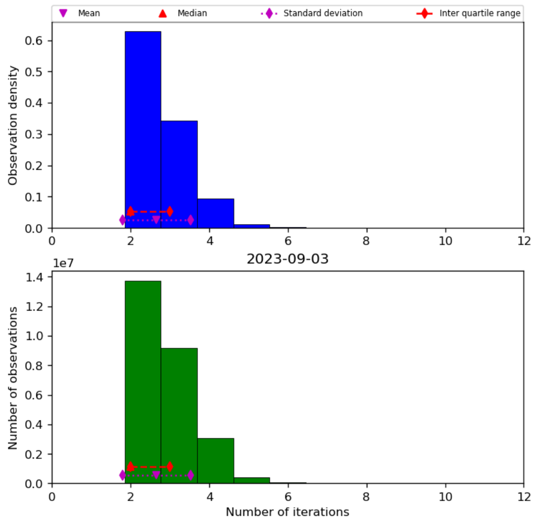
Figure 39: Histogram of “Number of iterations” for 2023-09-02 to 2023-09-04
