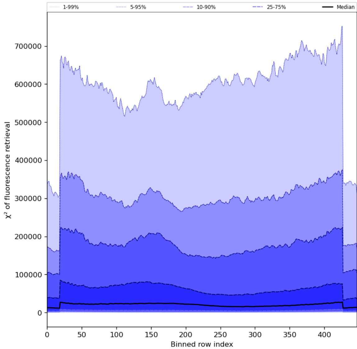
Figure 59: Along track statistics of “ \chi^2 of fluorescence retrieval” for 2023-09-02 to 2023-09-04
