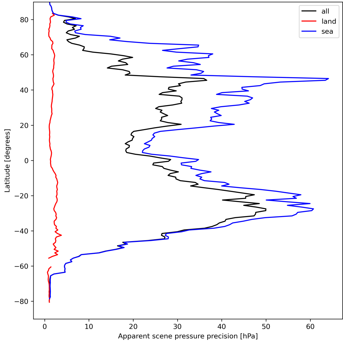
Figure 20: Zonal average of “Apparent scene pressure precision” for 2023-09-02 to 2023-09-04.
