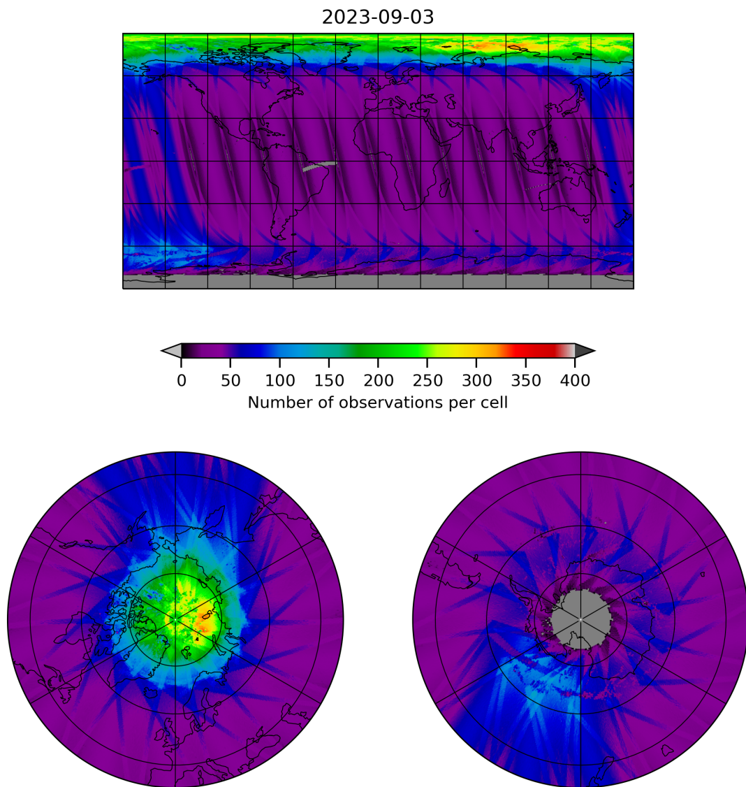
Figure 11: Map of the number of observations for 2023-09-02 to 2023-09-04
