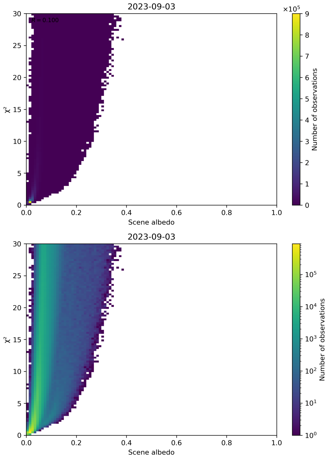
Figure 112: Scatter density plot of “Scene albedo” against “ \chi^2 ” for 2023-09-02 to 2023-09-04.
