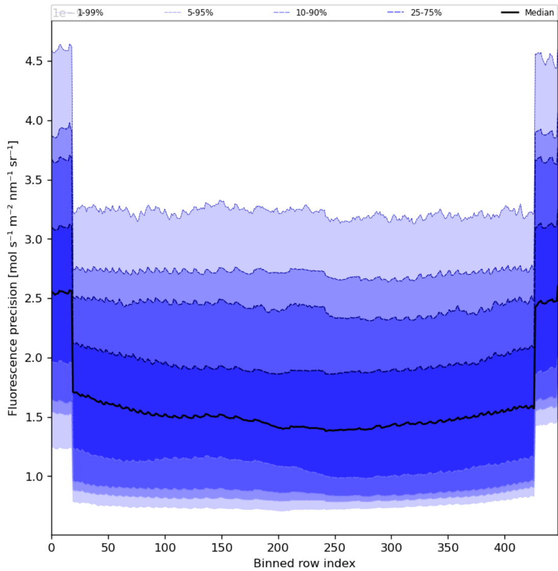
Figure 58: Along track statistics of “Fluorescence precision” for 2023-09-02 to 2023-09-04
