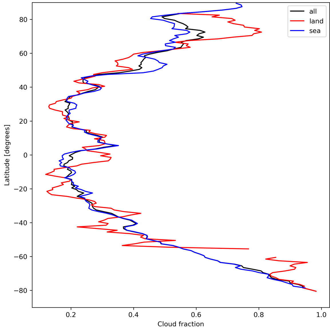
Figure 15: Zonal average of “Cloud fraction” for 2023-09-02 to 2023-09-04.
