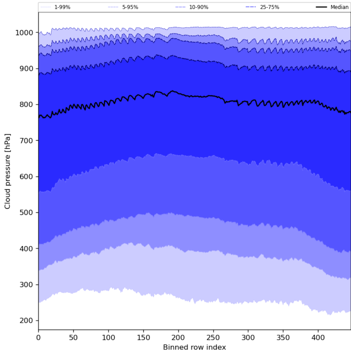
Figure 47: Along track statistics of “Cloud pressure” for 2023-09-02 to 2023-09-04
