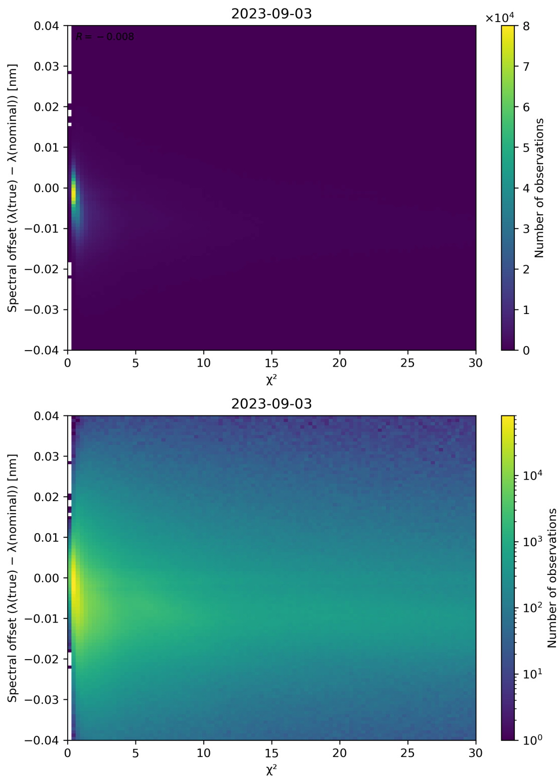
Figure 75: Scatter density plot of “ \chi^2 ” against “Spectral offset ( \lambda(\text{true}) - \lambda(\text{nominal}) )” for 2023-09-02 to 2023-09-04.
