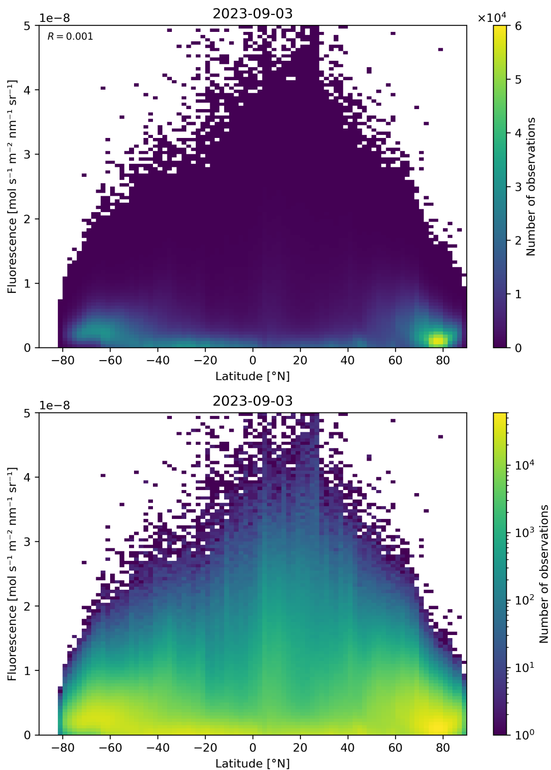
Figure 101: Scatter density plot of “Latitude” against “Fluorescence” for 2023-09-02 to 2023-09-04.
