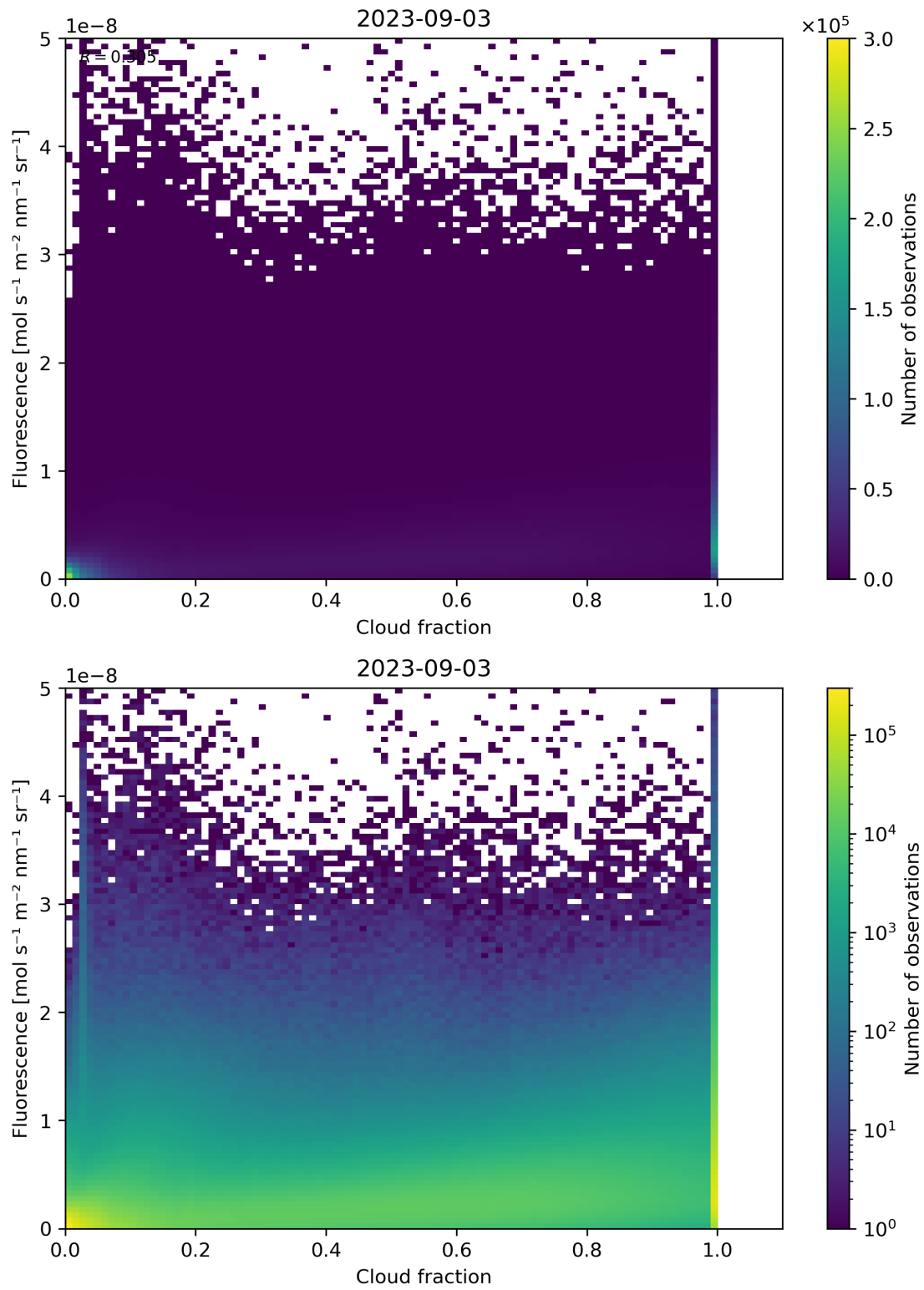
Figure 79: Scatter density plot of “Cloud fraction” against “Fluorescence” for 2023-09-02 to 2023-09-04.
