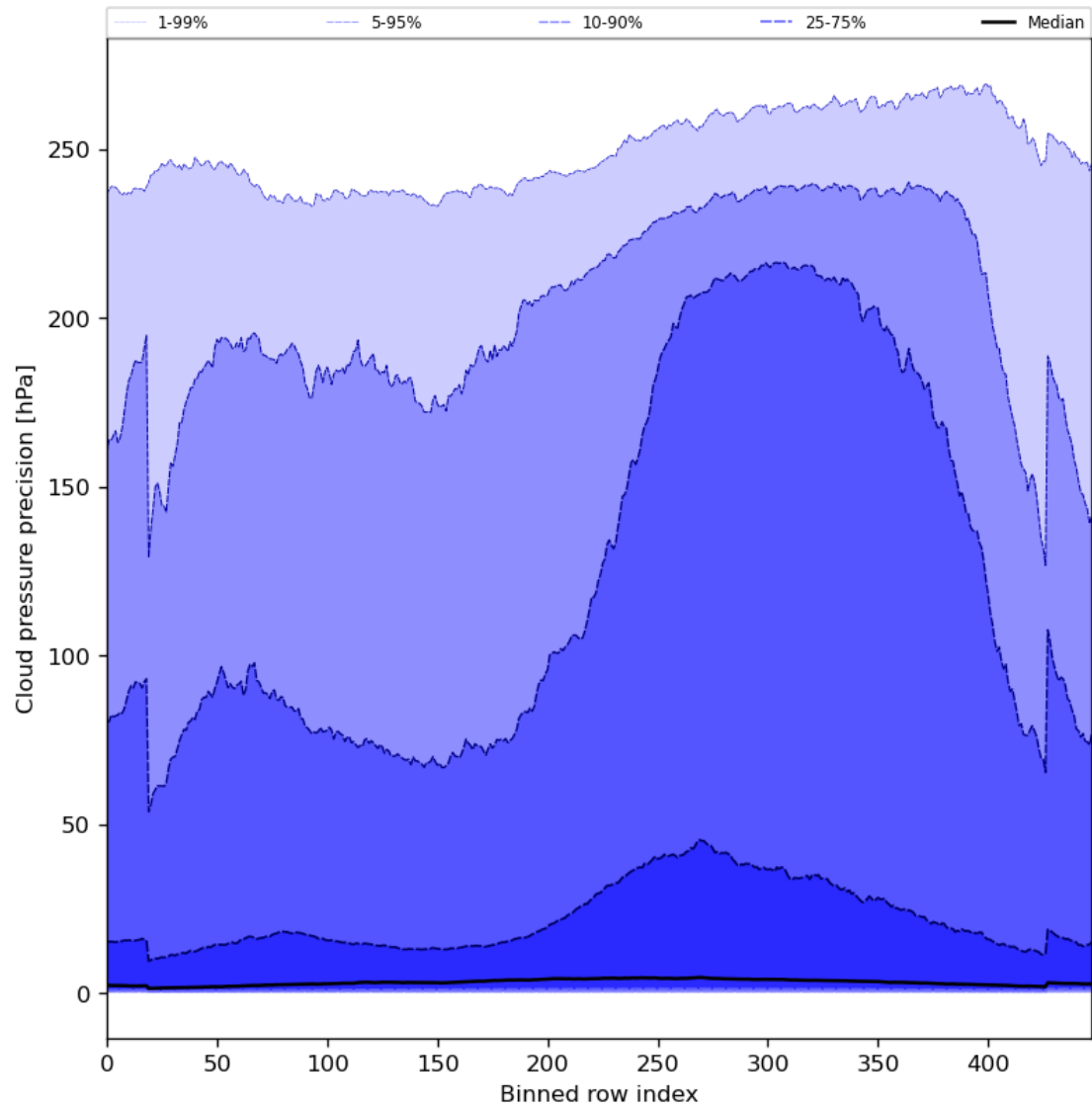
Figure 48: Along track statistics of “Cloud pressure precision” for 2023-09-02 to 2023-09-04
