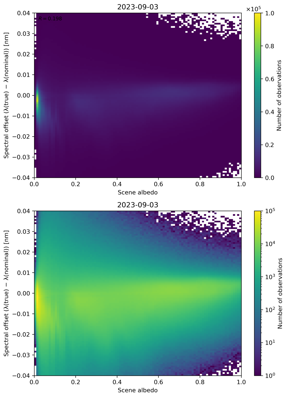
Figure 117: Scatter density plot of “Scene albedo” against “Spectral offset ( \lambda(\text{true}) - \lambda(\text{nominal}) )” for 2023-09-02 to 2023-09-04.
