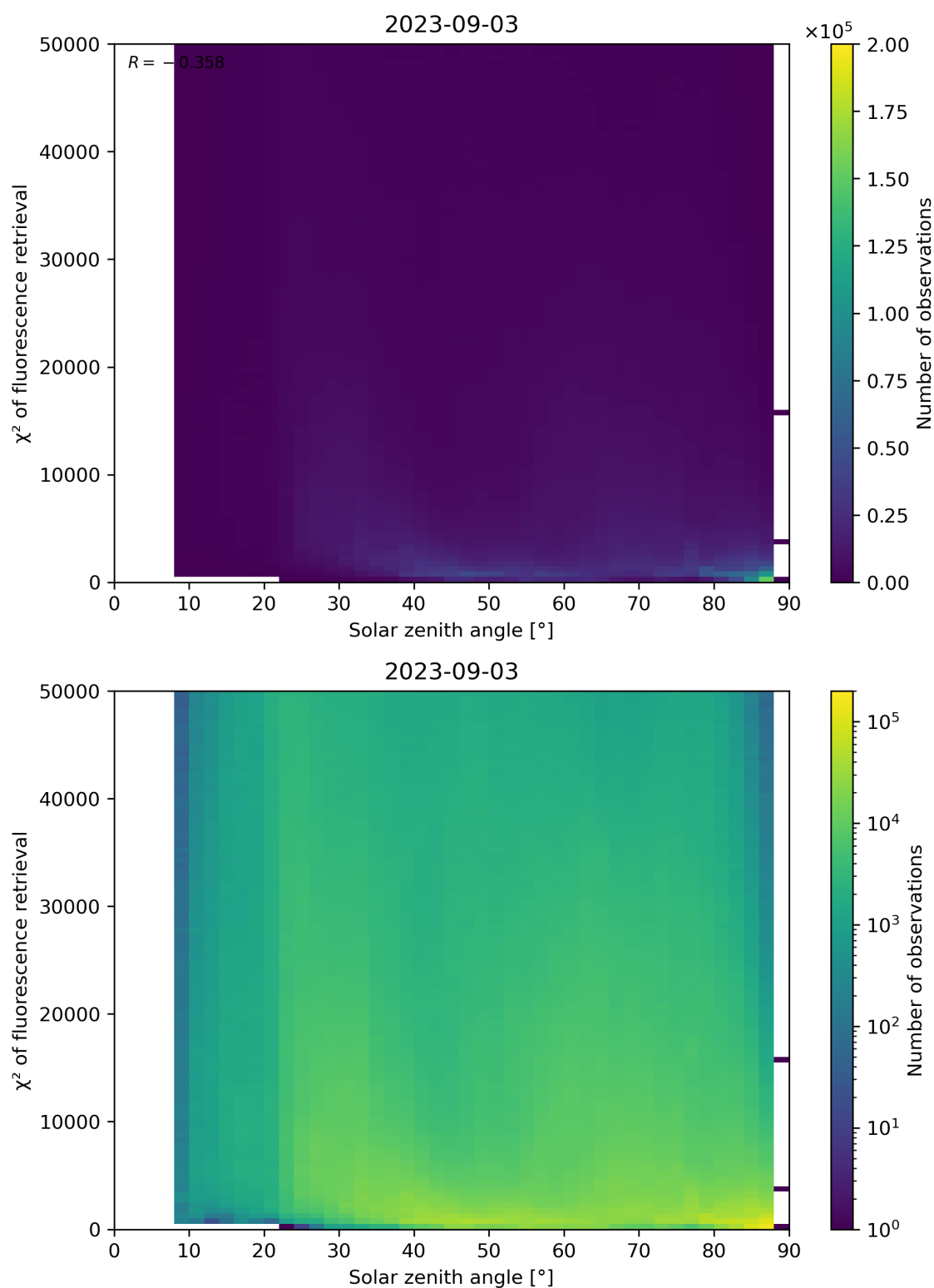
Figure 120: Scatter density plot of “Solar zenith angle” against “ \chi^2 of fluorescence retrieval” for 2023-09-02 to 2023-09-04.
