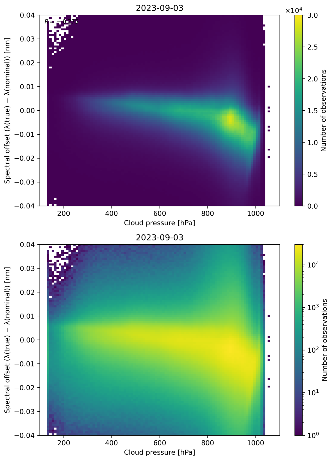
Figure 92: Scatter density plot of “Cloud pressure” against “Spectral offset ( \lambda(\text{true}) - \lambda(\text{nominal}) )” for 2023-09-02 to 2023-09-04.
