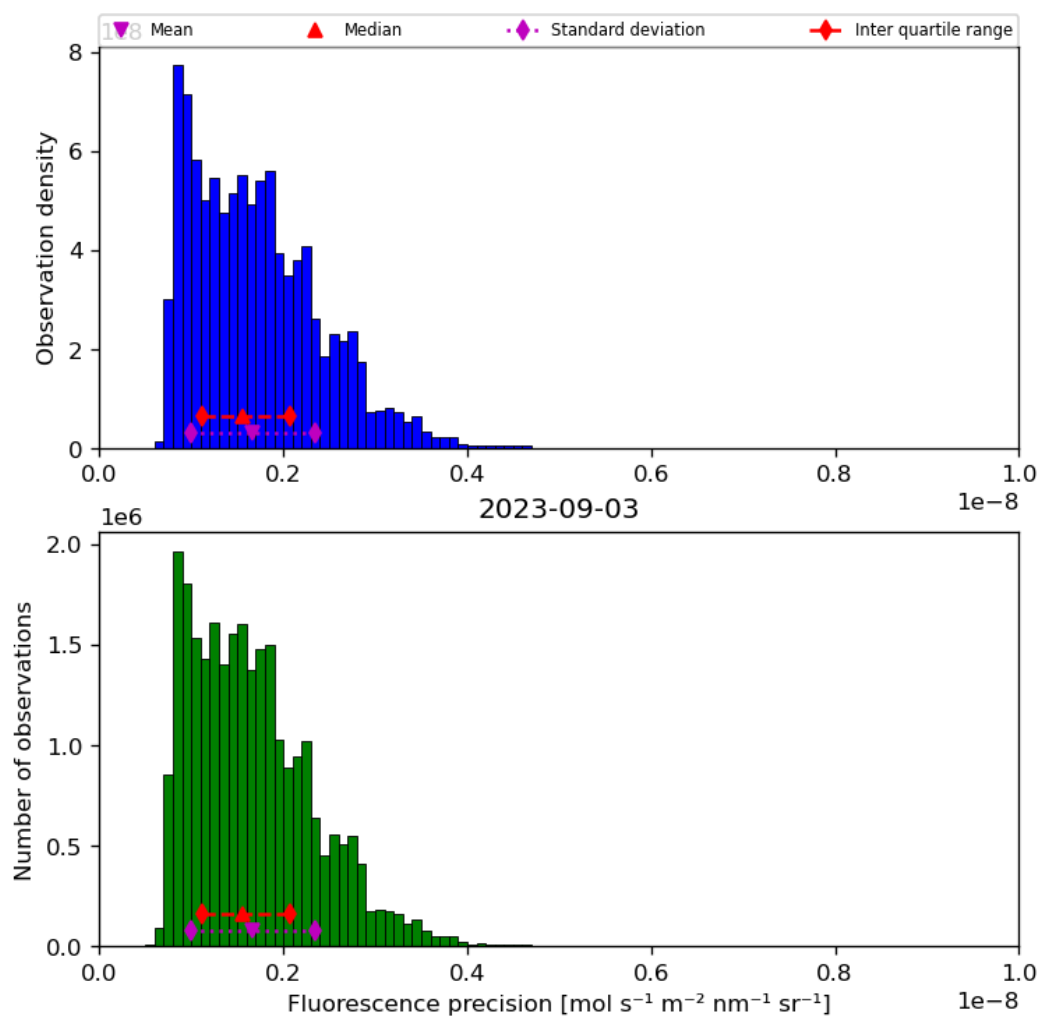
Figure 41: Histogram of “Fluorescence precision” for 2023-09-02 to 2023-09-04
