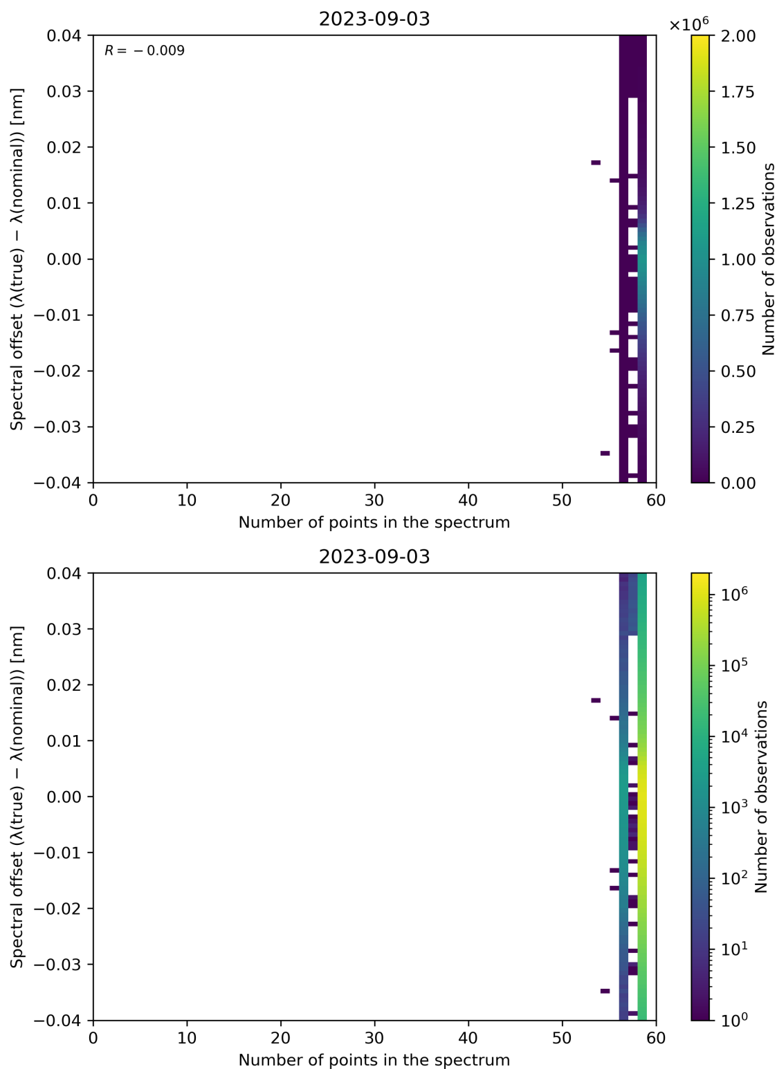
Figure 110: Scatter density plot of “Number of points in the spectrum” against “Spectral offset ( \lambda(\text{true}) - \lambda(\text{nominal}) )” for 2023-09-02 to 2023-09-04.
