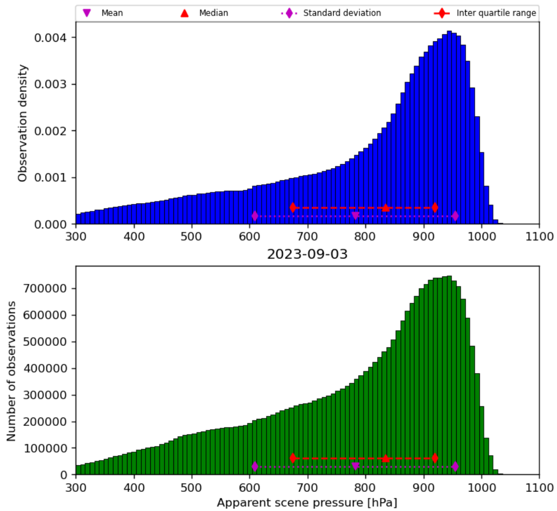
Figure 36: Histogram of “Apparent scene pressure” for 2023-09-02 to 2023-09-04
