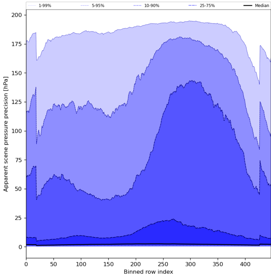
Figure 54: Along track statistics of “Apparent scene pressure precision” for 2023-09-02 to 2023-09-04
