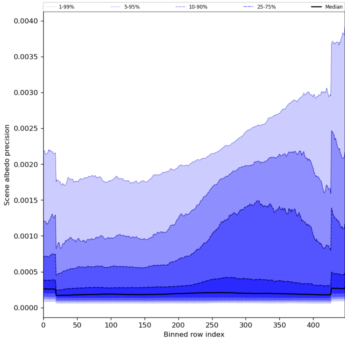
Figure 52: Along track statistics of “Scene albedo precision” for 2023-09-02 to 2023-09-04
