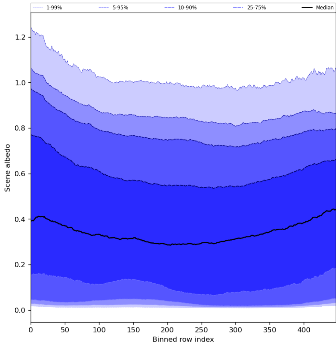
Figure 51: Along track statistics of “Scene albedo” for 2023-09-02 to 2023-09-04
