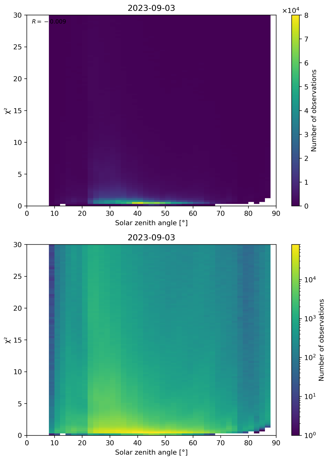
Figure 119: Scatter density plot of “Solar zenith angle” against “ \chi^2 ” for 2023-09-02 to 2023-09-04.
