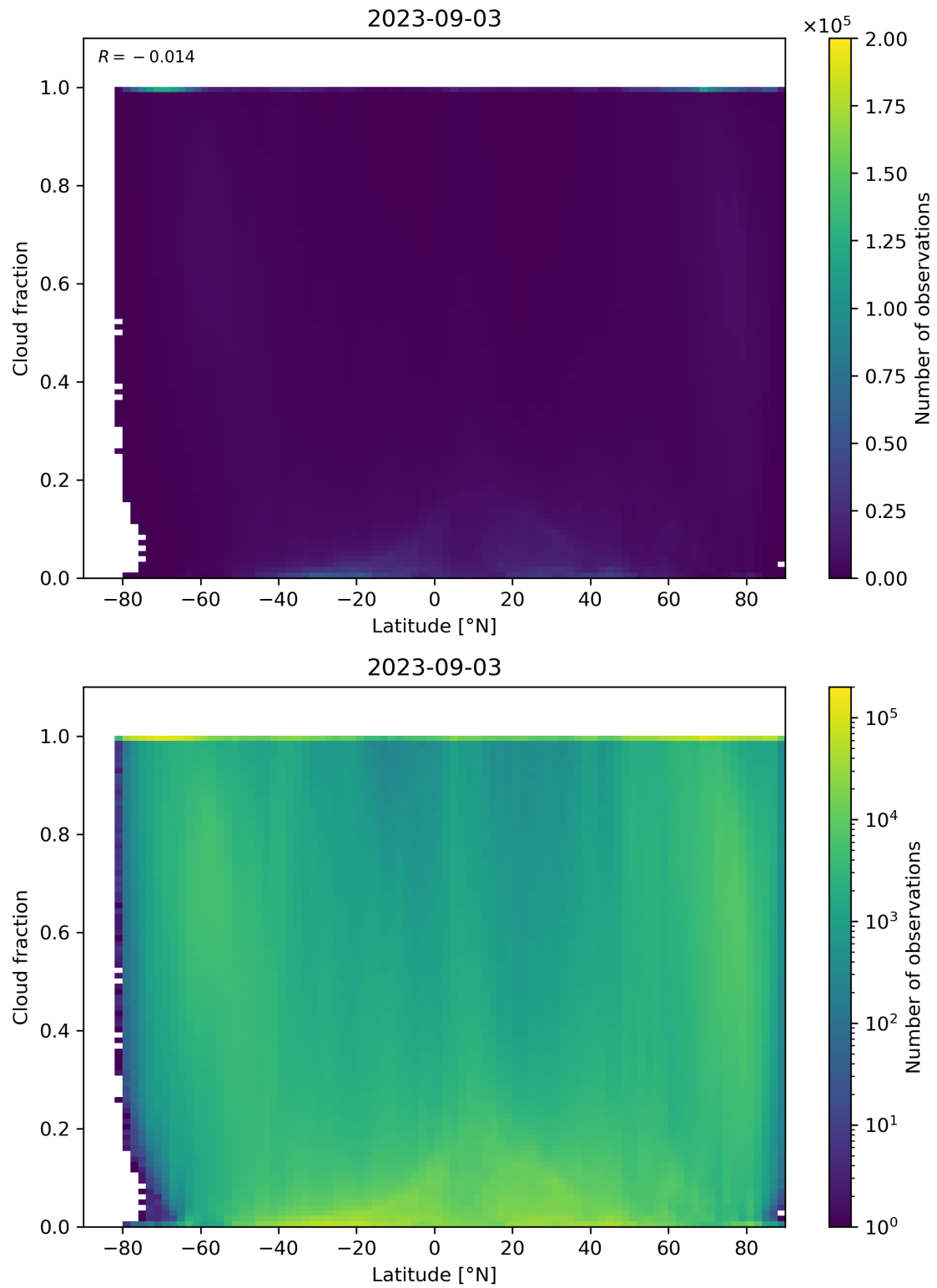
Figure 99: Scatter density plot of “Latitude” against “Cloud fraction” for 2023-09-02 to 2023-09-04.
