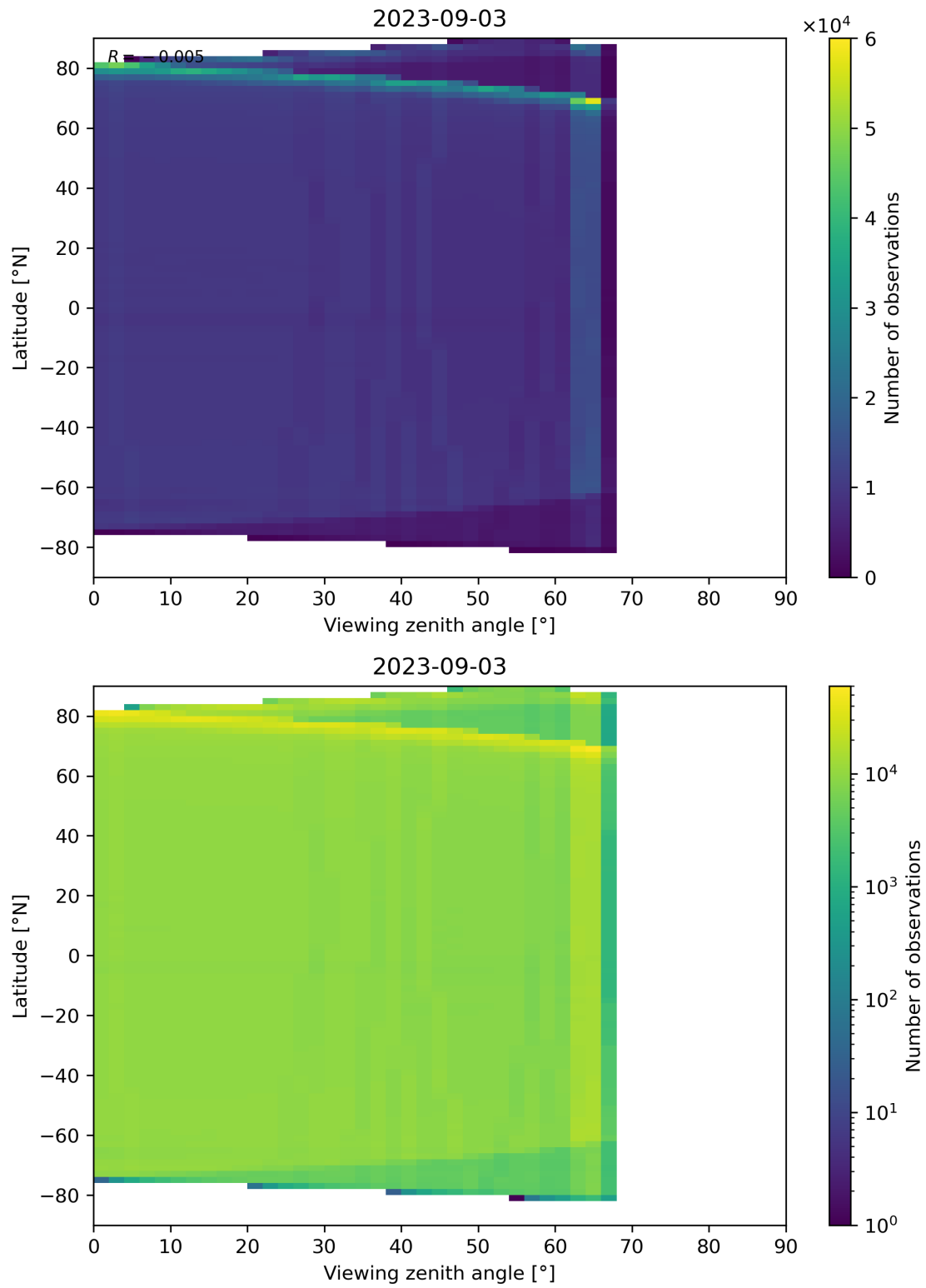
Figure 135: Scatter density plot of “Viewing zenith angle” against “Latitude” for 2023-09-02 to 2023-09-04.
