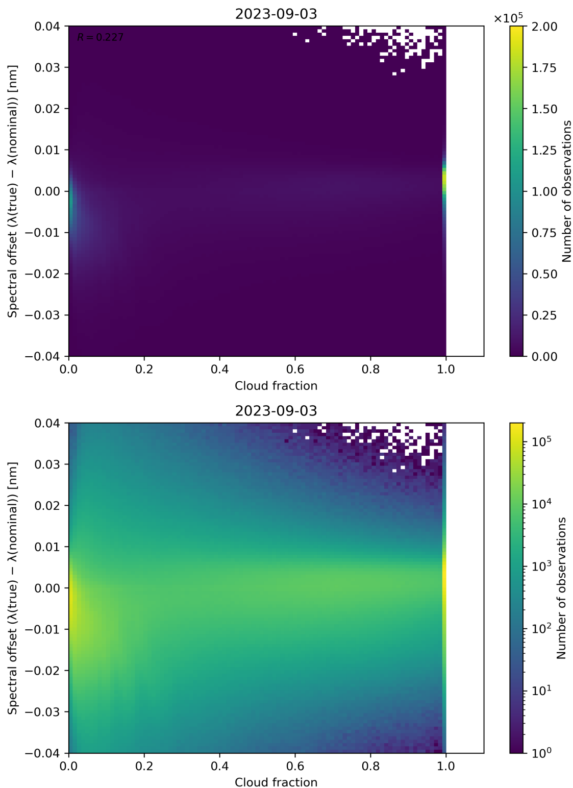
Figure 83: Scatter density plot of “Cloud fraction” against “Spectral offset ( \lambda(\text{true}) - \lambda(\text{nominal}) )” for 2023-09-02 to 2023-09-04.
