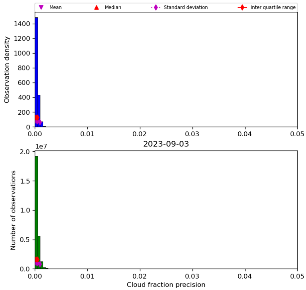
Figure 33: Histogram of “Cloud fraction precision” for 2023-09-02 to 2023-09-04
