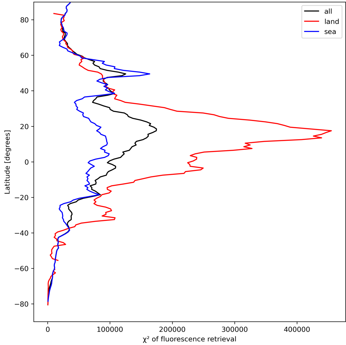
Figure 25: Zonal average of “ \chi^2 of fluorescence retrieval” for 2023-09-02 to 2023-09-04.
