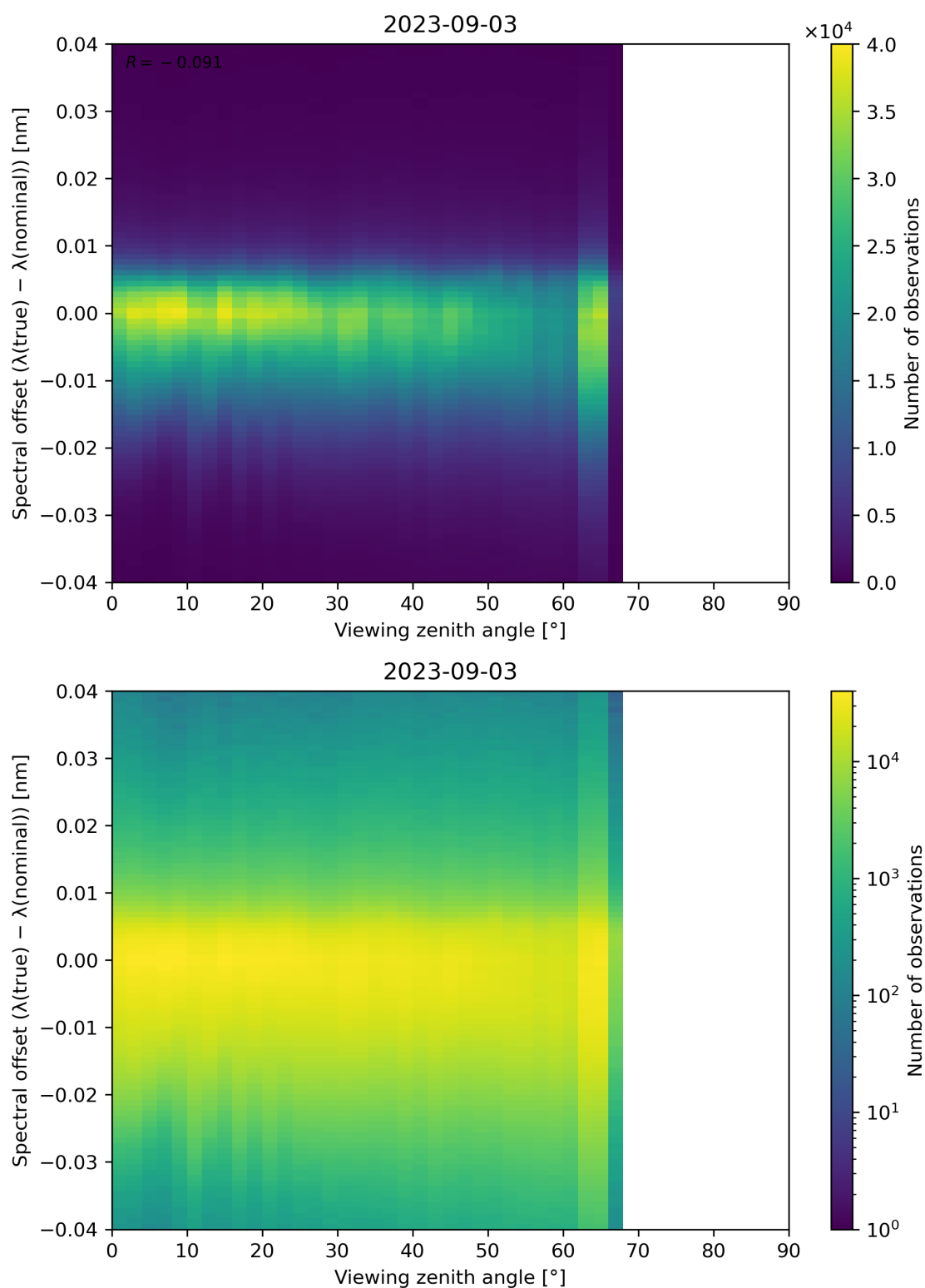
Figure 140: Scatter density plot of “Viewing zenith angle” against “Spectral offset ( \lambda(\text{true}) - \lambda(\text{nominal}) )” for 2023-09-02 to 2023-09-04.
