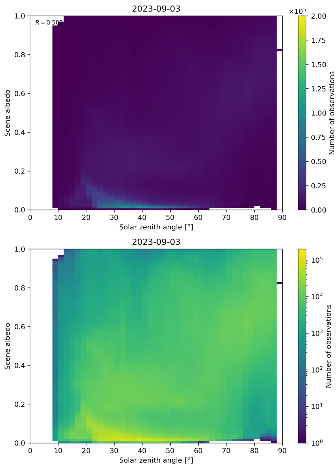
Figure 127: Scatter density plot of “Solar zenith angle” against “Scene albedo” for 2023-09-02 to 2023-09-04.
