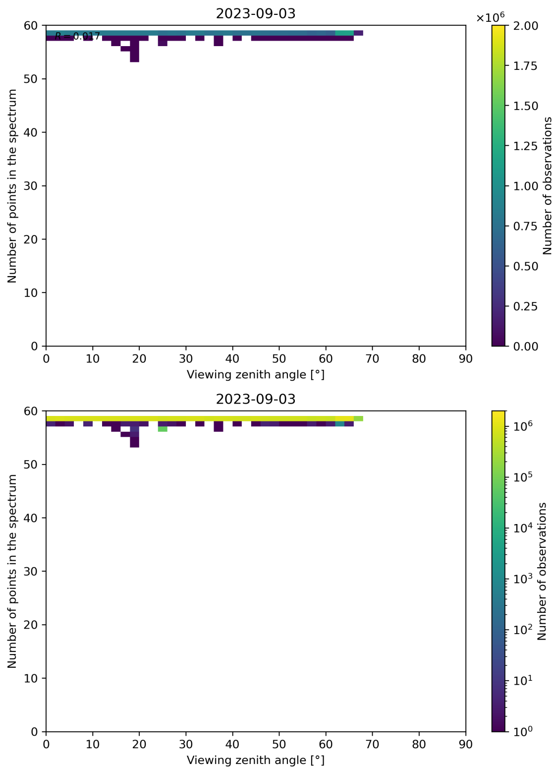
Figure 137: Scatter density plot of “Viewing zenith angle” against “Number of points in the spectrum” for 2023-09-02 to 2023-09-04.
