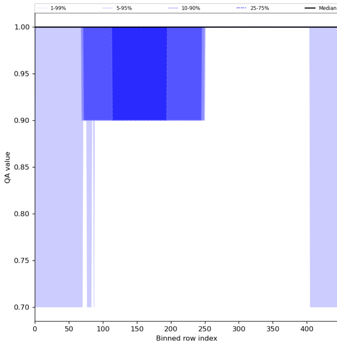
Figure 46: Along track statistics of “QA value” for 2023-09-02 to 2023-09-04
