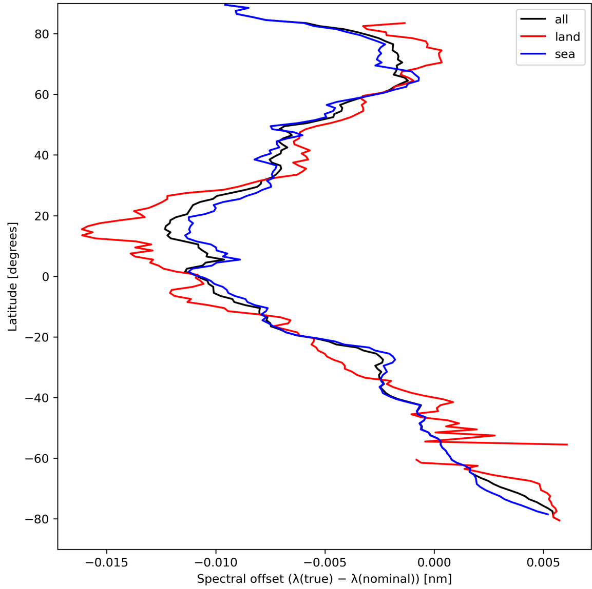
Figure 28: Zonal average of “Spectral offset ( \lambda(\text{true}) - \lambda(\text{nominal}) )” for 2023-09-02 to 2023-09-04.
