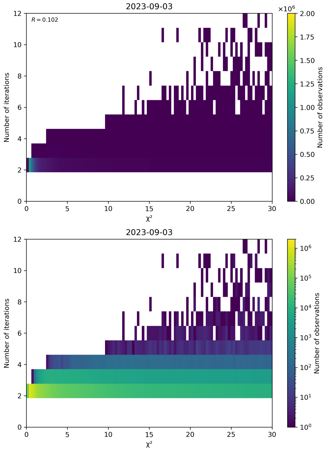
Figure 73: Scatter density plot of “ \chi^2 ” against “Number of iterations” for 2023-09-02 to 2023-09-04.
