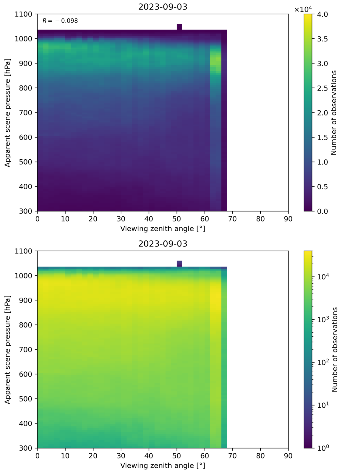
Figure 129: Scatter density plot of “Viewing zenith angle” against “Apparent scene pressure” for 2023-09-02 to 2023-09-04.
