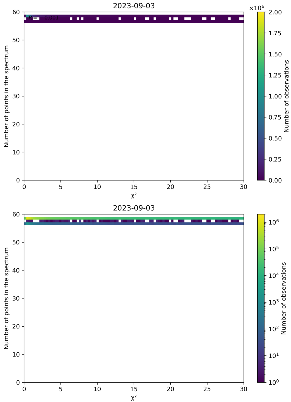
Figure 74: Scatter density plot of " \chi^2 " against "Number of points in the spectrum" for 2023-09-02 to 2023-09-04.
