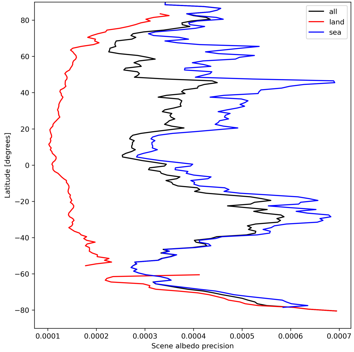
Figure 18: Zonal average of “Scene albedo precision” for 2023-09-02 to 2023-09-04.
