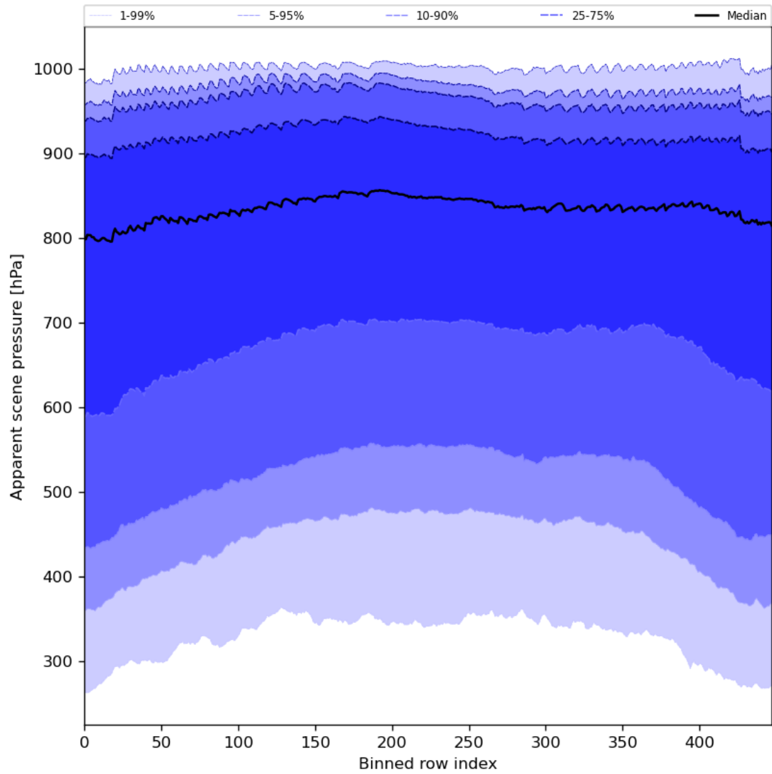
Figure 53: Along track statistics of “Apparent scene pressure” for 2023-09-02 to 2023-09-04
