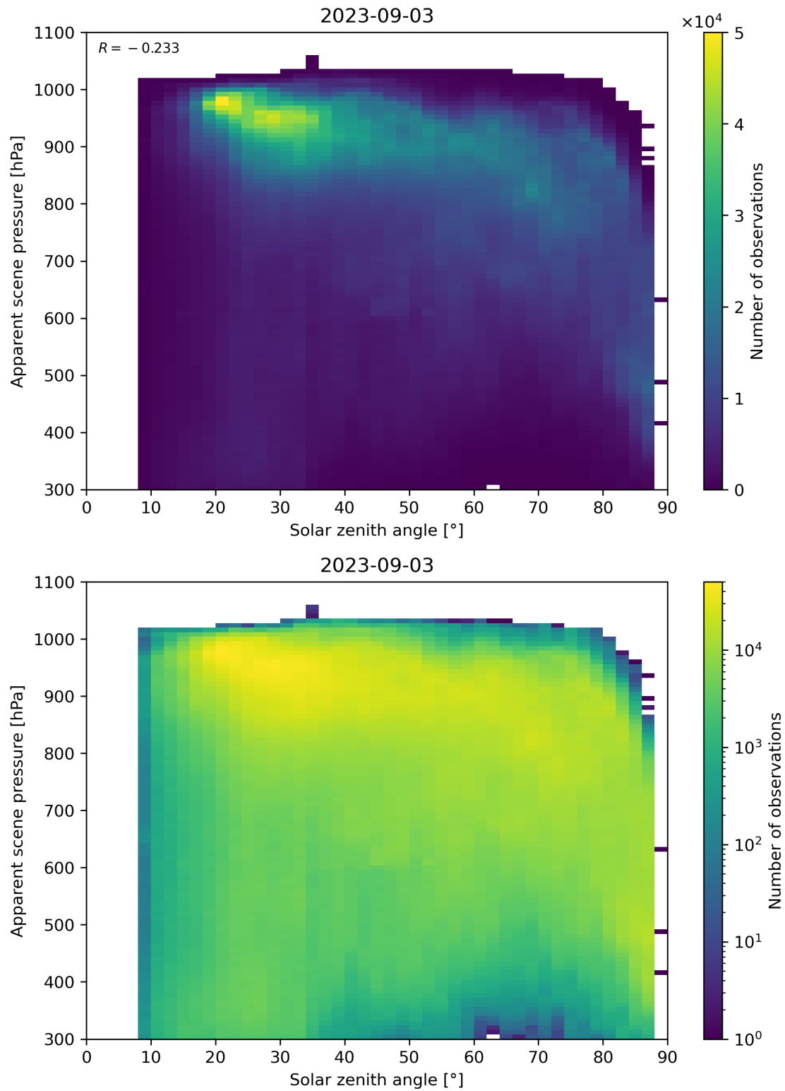
Figure 118: Scatter density plot of “Solar zenith angle” against “Apparent scene pressure” for 2023-09-02 to 2023-09-04.
