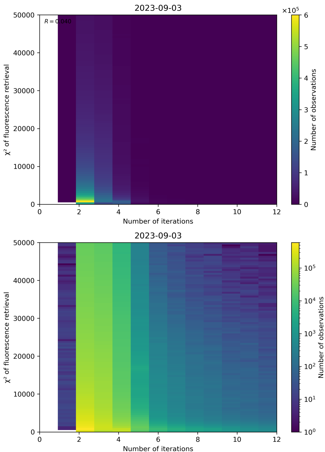
Figure 106: Scatter density plot of “Number of iterations” against “ \chi^2 of fluorescence retrieval” for 2023-09-02 to 2023-09-04.
