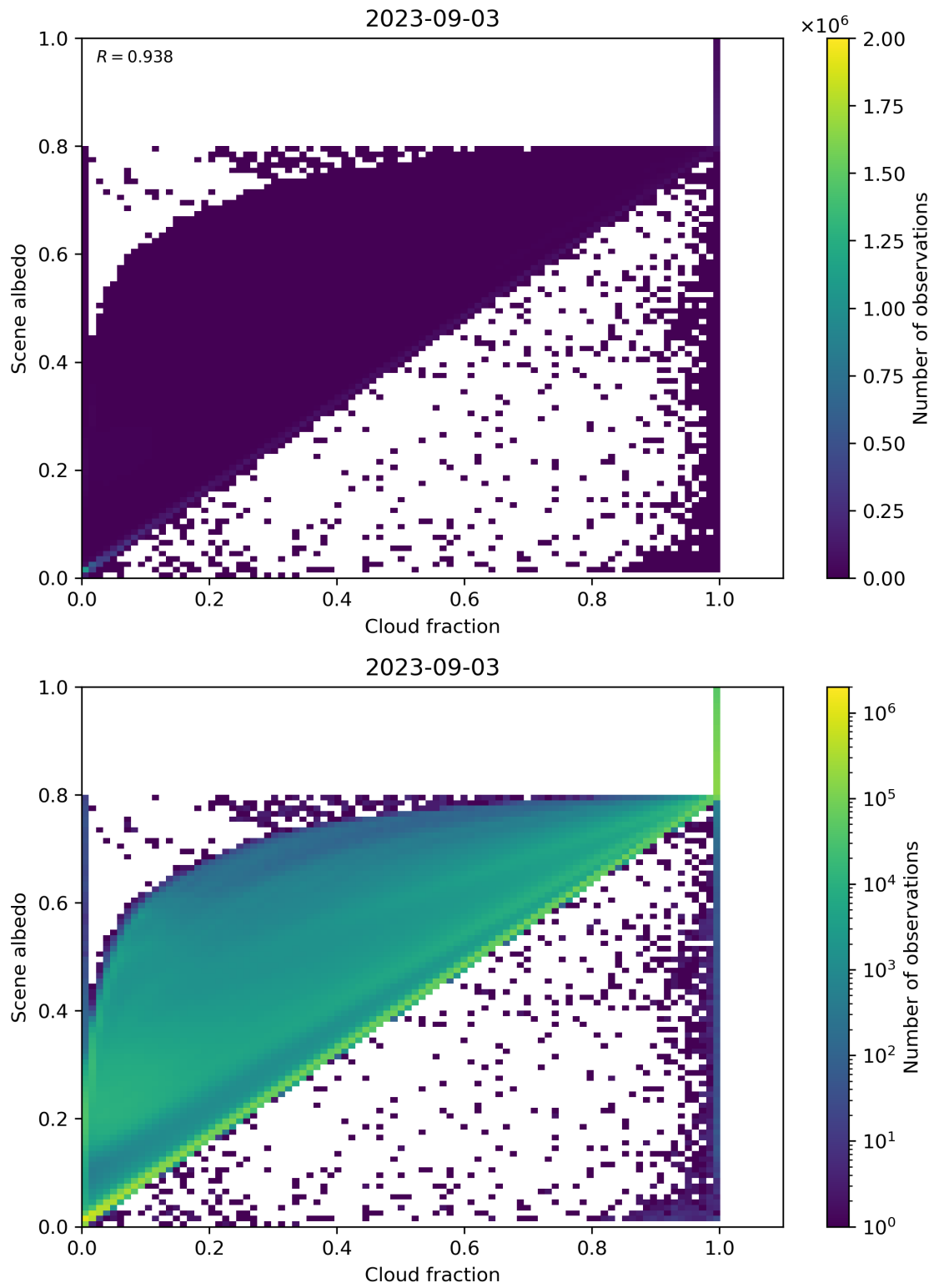
Figure 82: Scatter density plot of “Cloud fraction” against “Scene albedo” for 2023-09-02 to 2023-09-04.
