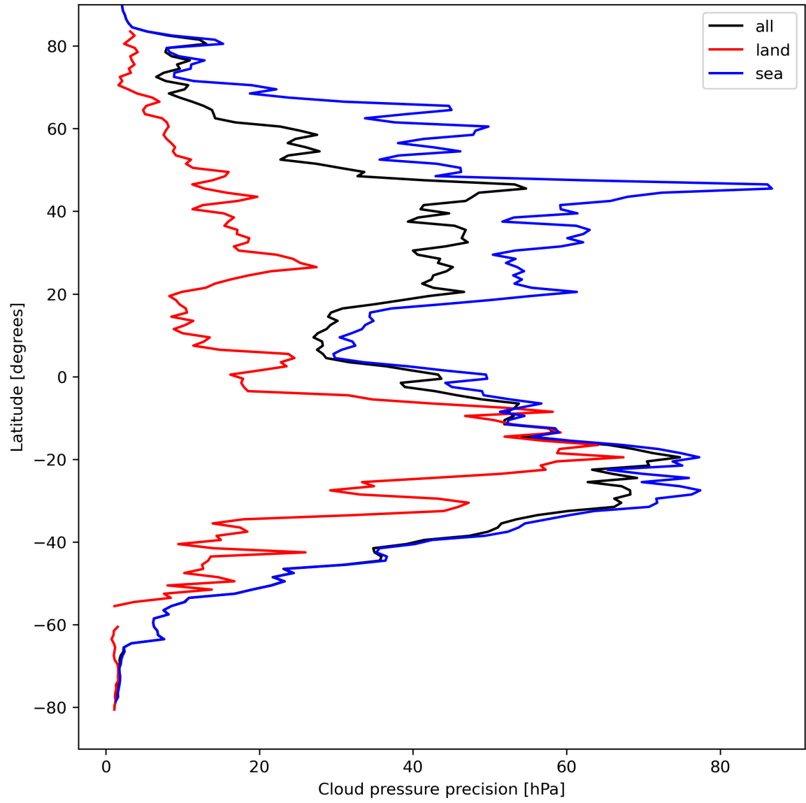
Figure 14: Zonal average of “Cloud pressure precision” for 2023-09-02 to 2023-09-04.
