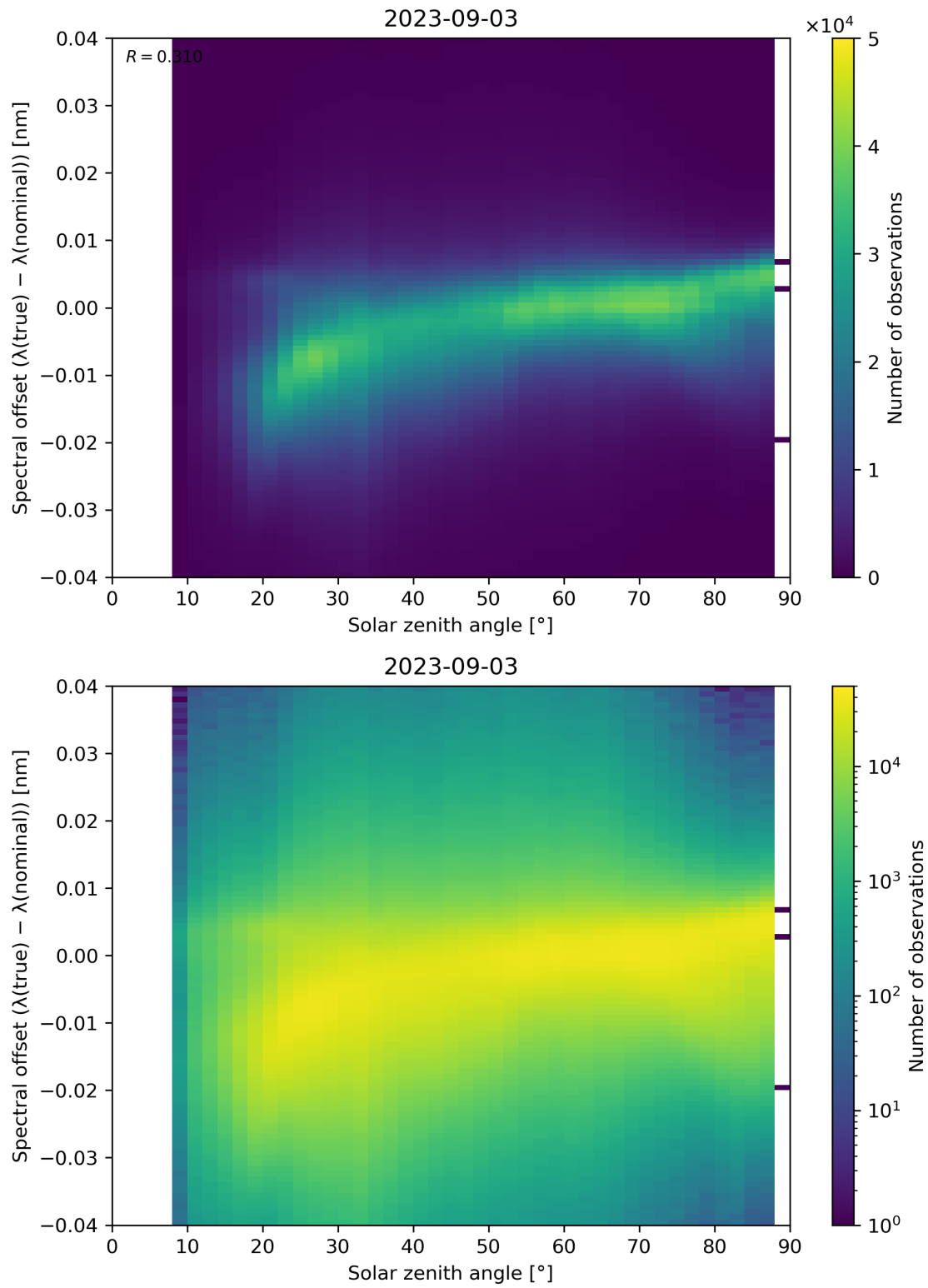
Figure 128: Scatter density plot of “Solar zenith angle” against “Spectral offset ( \lambda(\text{true}) - \lambda(\text{nominal}) )” for 2023-09-02 to 2023-09-04.
