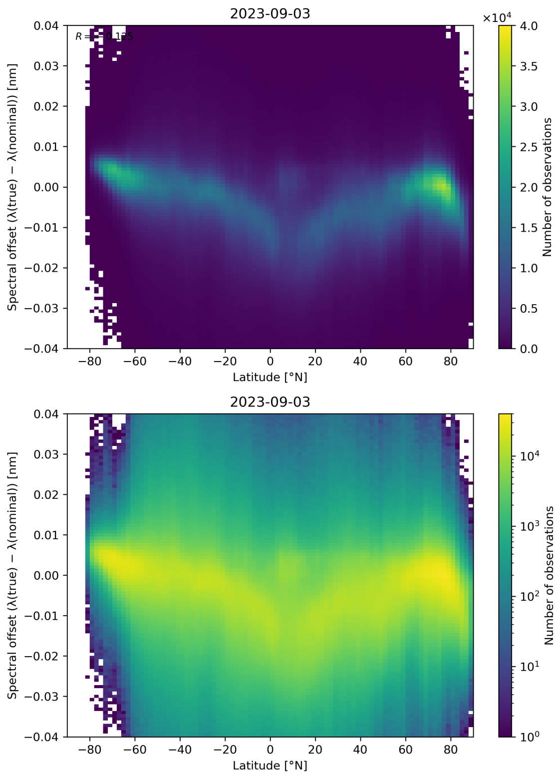
Figure 105: Scatter density plot of “Latitude” against “Spectral offset ( \lambda(\text{true}) - \lambda(\text{nominal}) )” for 2023-09-02 to 2023-09-04.
