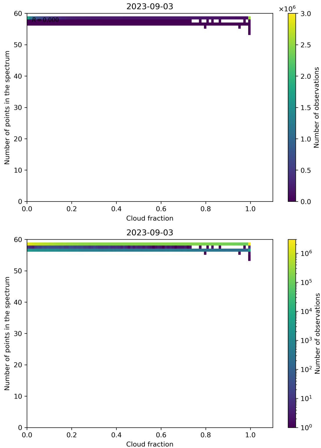
Figure 81: Scatter density plot of “Cloud fraction” against “Number of points in the spectrum” for 2023-09-02 to 2023-09-04.
