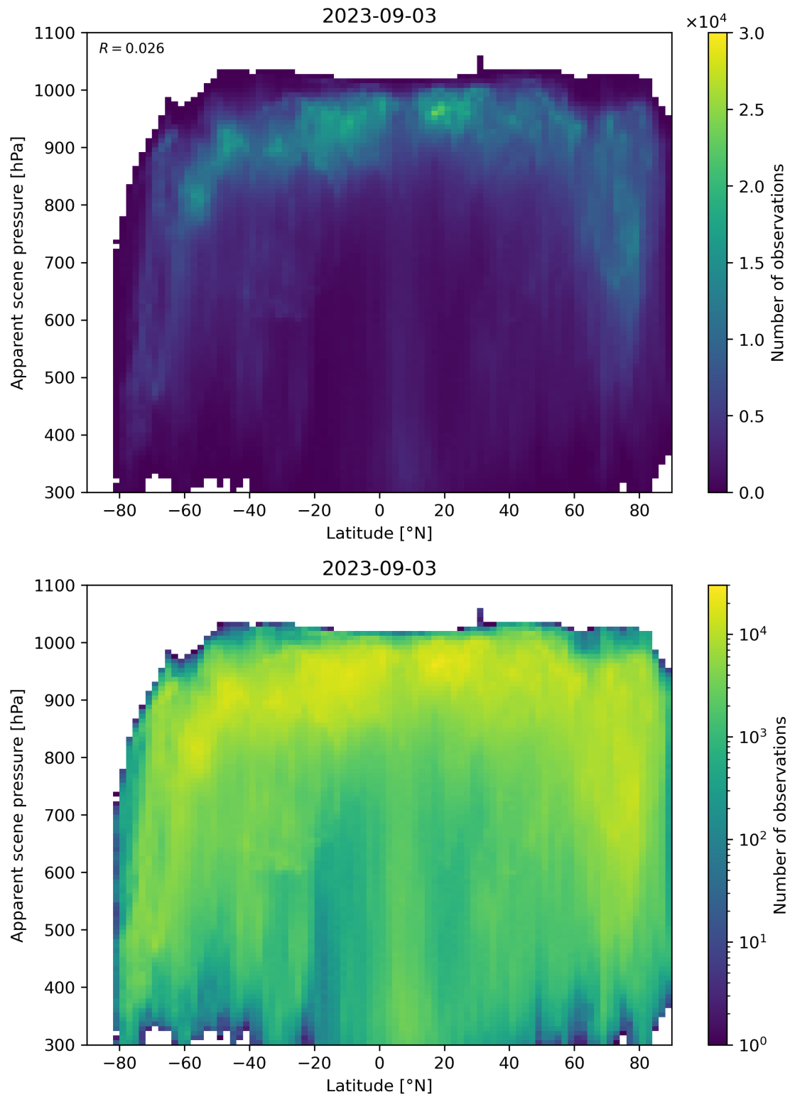
Figure 96: Scatter density plot of “Latitude” against “Apparent scene pressure” for 2023-09-02 to 2023-09-04.
