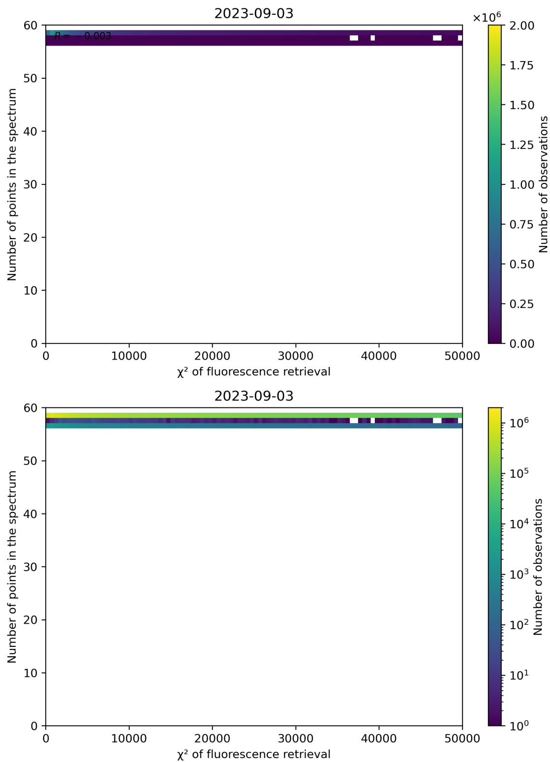
Figure 71: Scatter density plot of " \chi^2 of fluorescence retrieval" against "Number of points in the spectrum" for 2023-09-02 to 2023-09-04.
