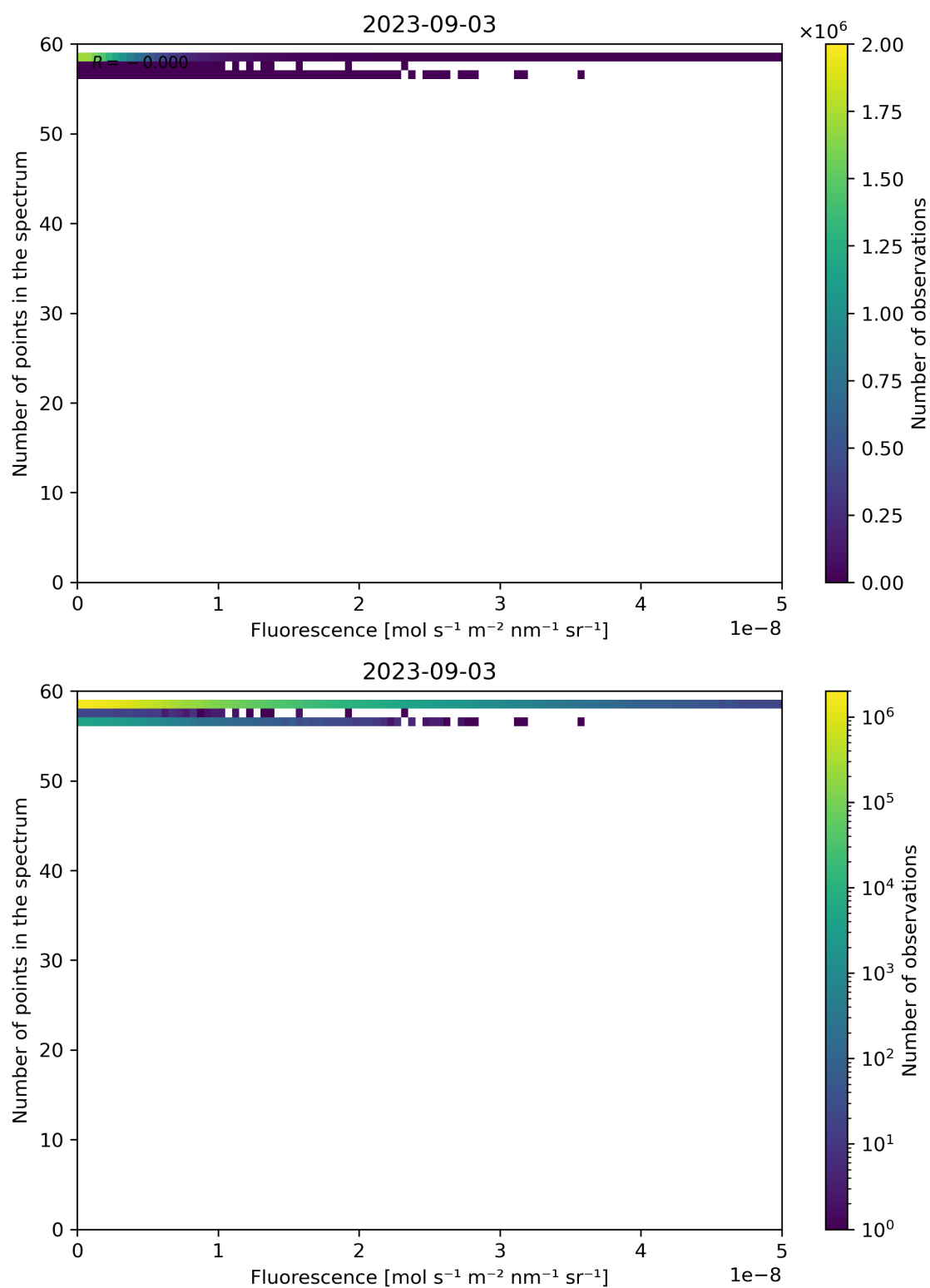
Figure 94: Scatter density plot of “Fluorescence” against “Number of points in the spectrum” for 2023-09-02 to 2023-09-04.
