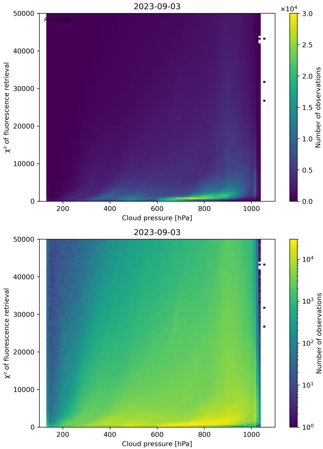
Figure 86: Scatter density plot of “Cloud pressure” against “ \chi^2 of fluorescence retrieval” for 2023-09-02 to 2023-09-04.
