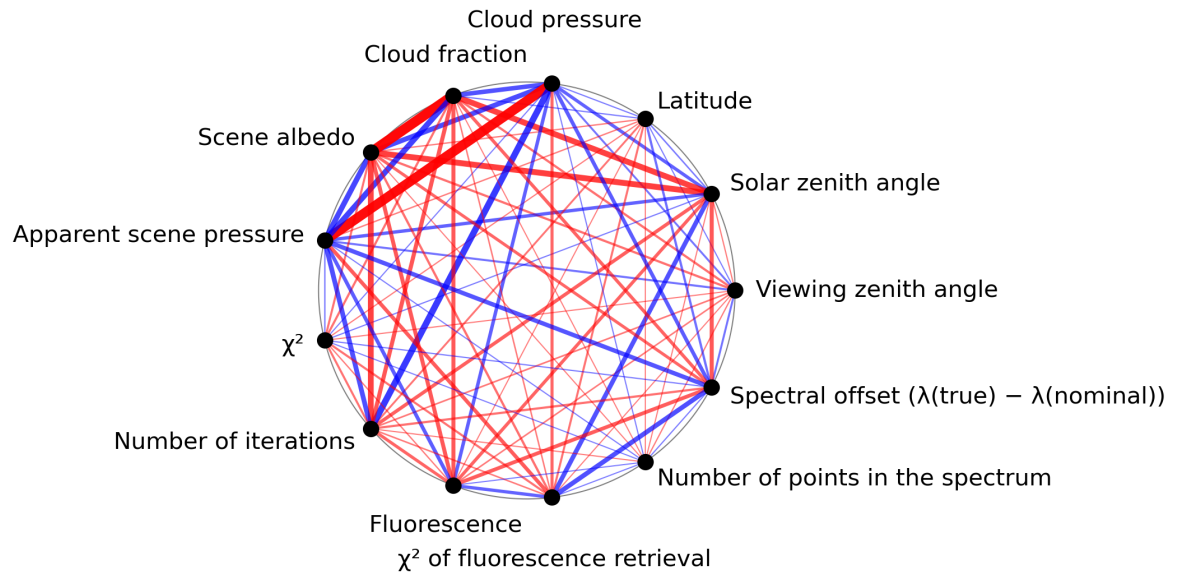
Figure 1: Map of correlation graph for 2023-09-02 to 2023-09-04.
