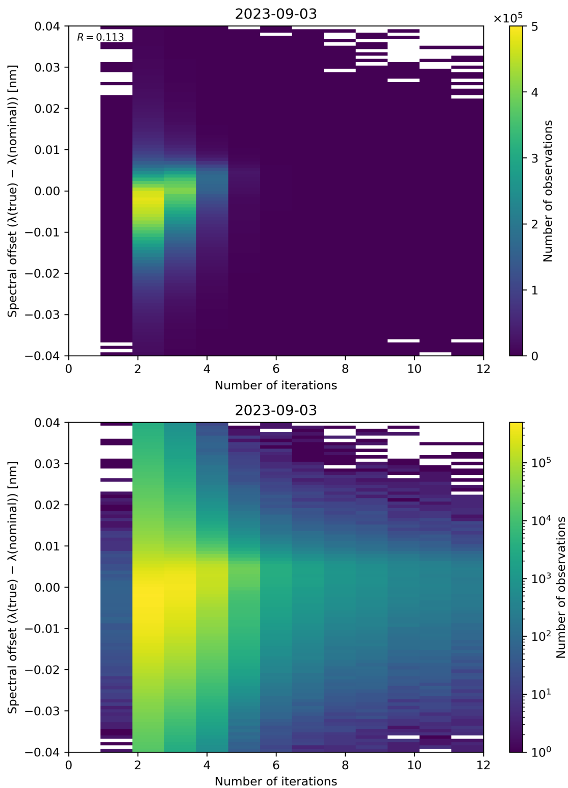
Figure 109: Scatter density plot of “Number of iterations” against “Spectral offset ( \lambda(\text{true}) - \lambda(\text{nominal}) )” for 2023-09-02 to 2023-09-04.
