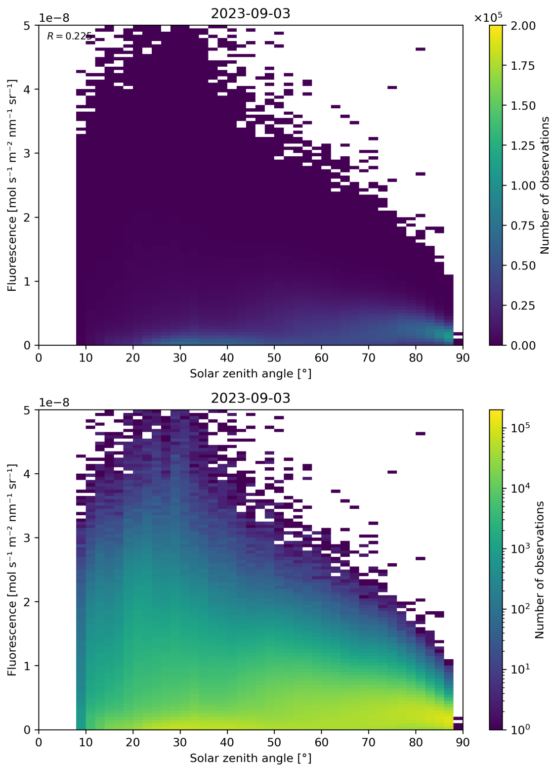
Figure 123: Scatter density plot of “Solar zenith angle” against “Fluorescence” for 2023-09-02 to 2023-09-04.
