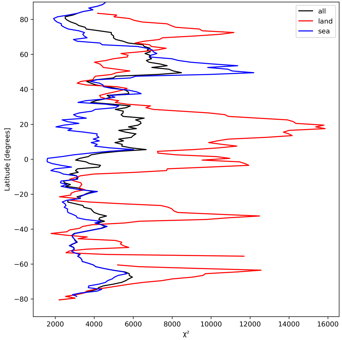
Figure 21: Zonal average of “ \chi^2 ” for 2023-09-02 to 2023-09-04.
