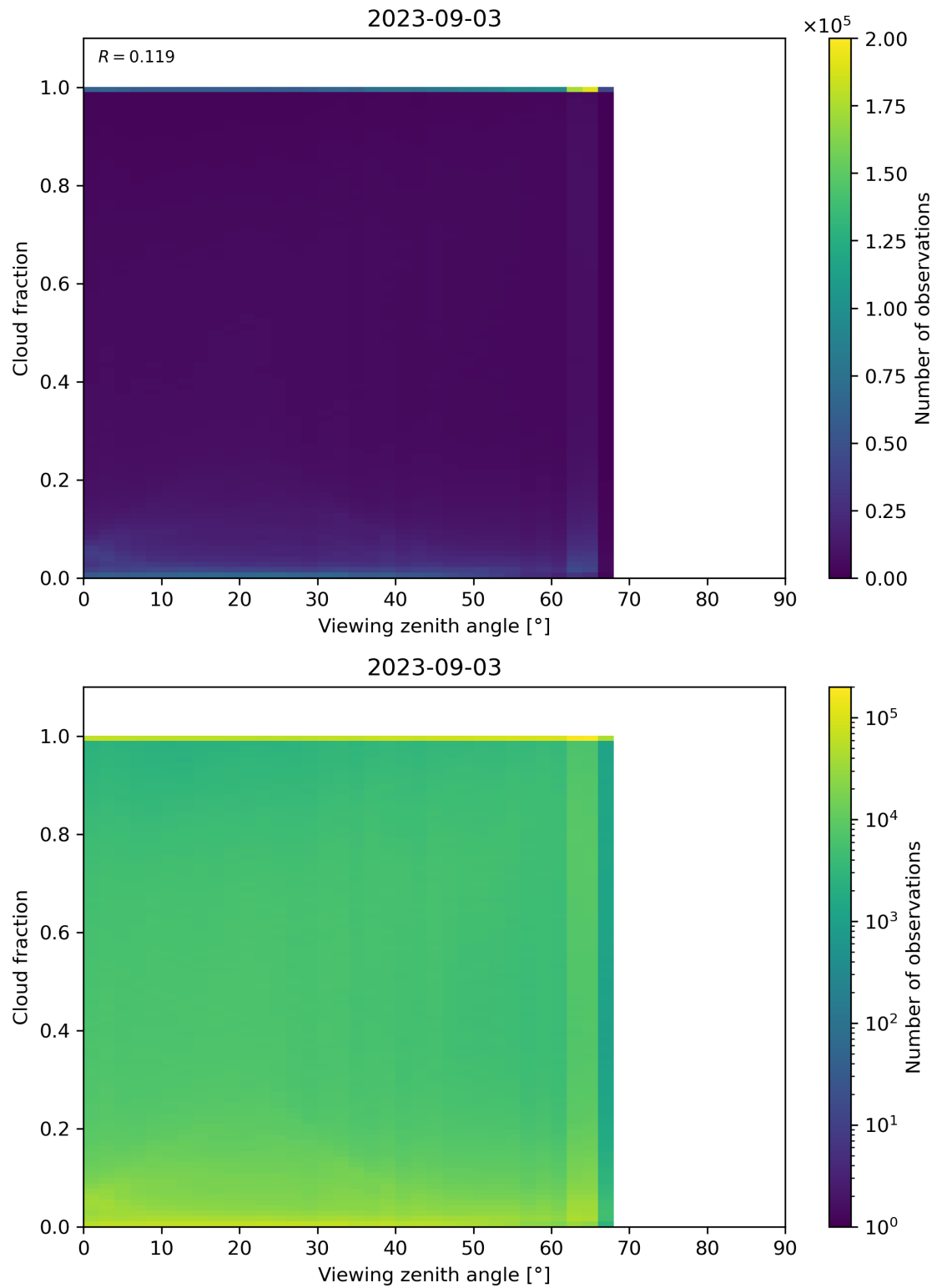
Figure 132: Scatter density plot of “Viewing zenith angle” against “Cloud fraction” for 2023-09-02 to 2023-09-04.
