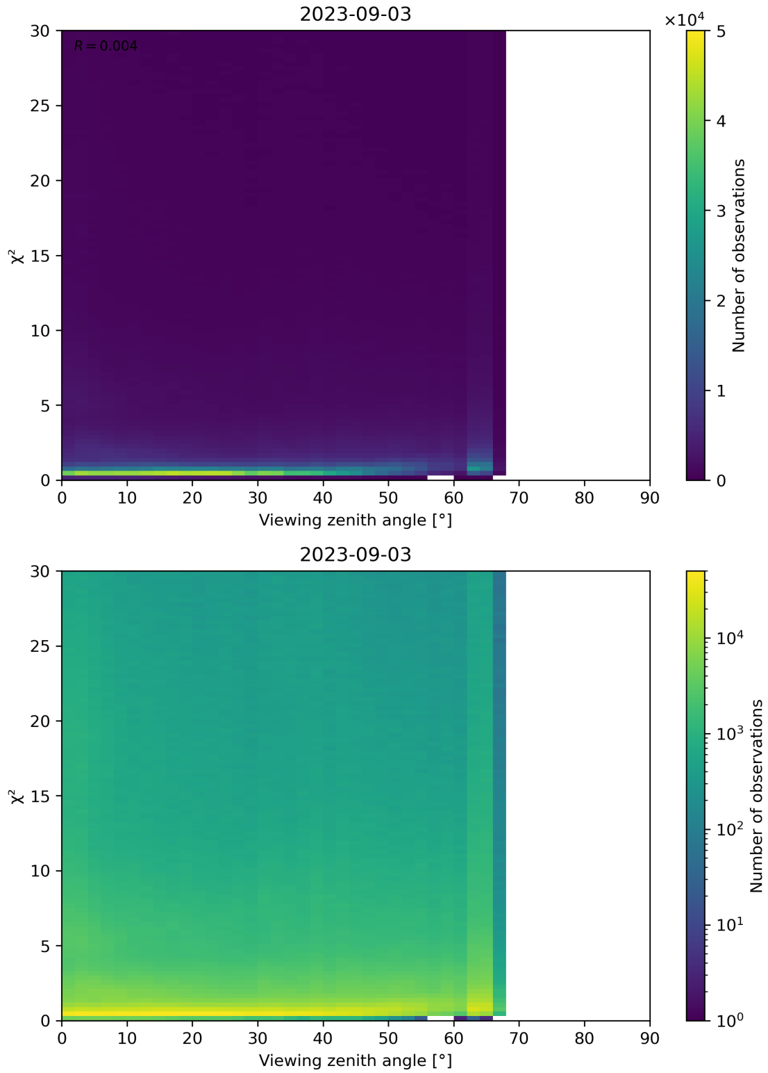
Figure 130: Scatter density plot of “Viewing zenith angle” against “ \chi^2 ” for 2023-09-02 to 2023-09-04.
