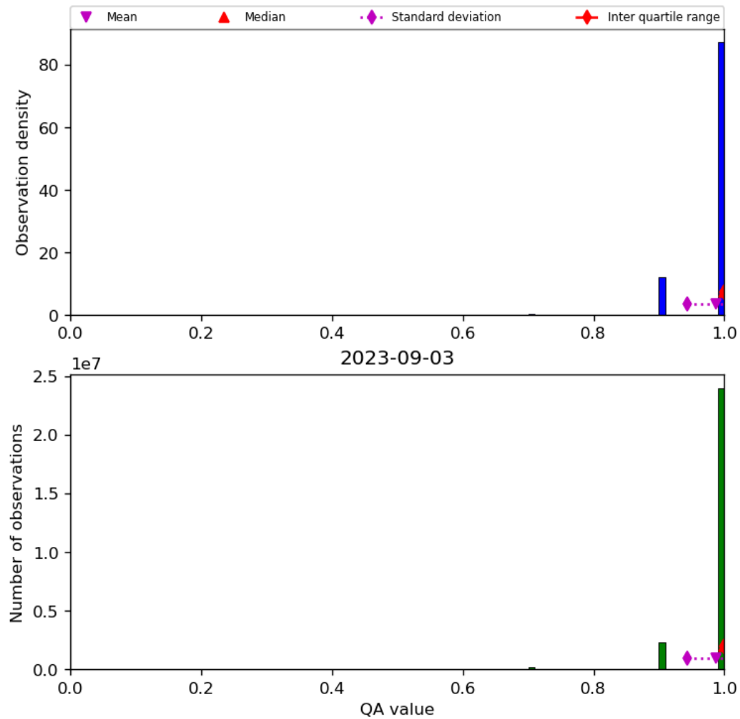
Figure 29: Histogram of “QA value” for 2023-09-02 to 2023-09-04
