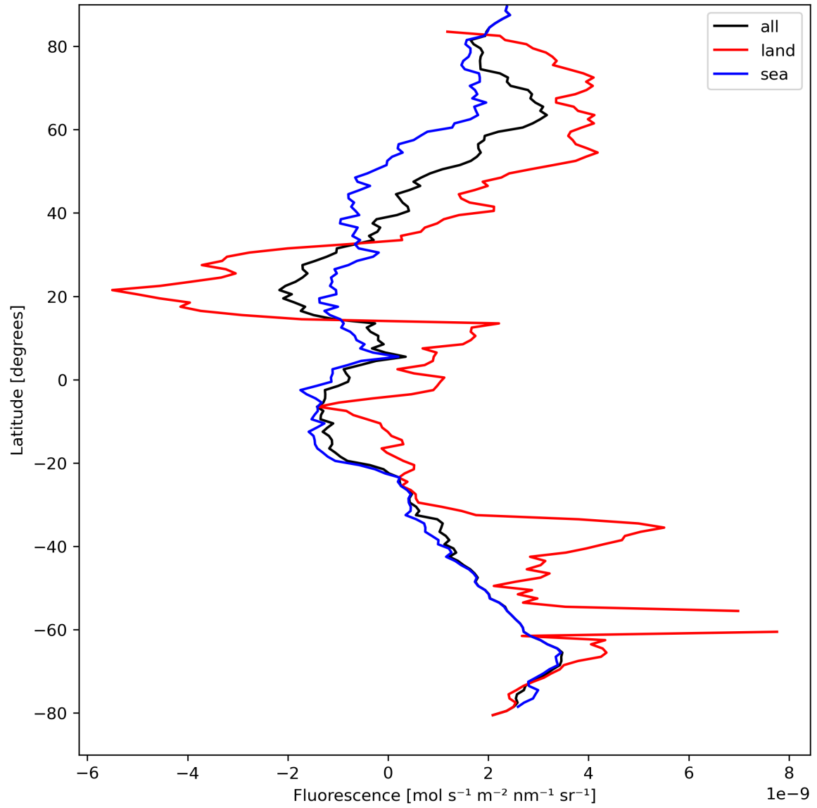
Figure 23: Zonal average of “Fluorescence” for 2023-09-02 to 2023-09-04.
