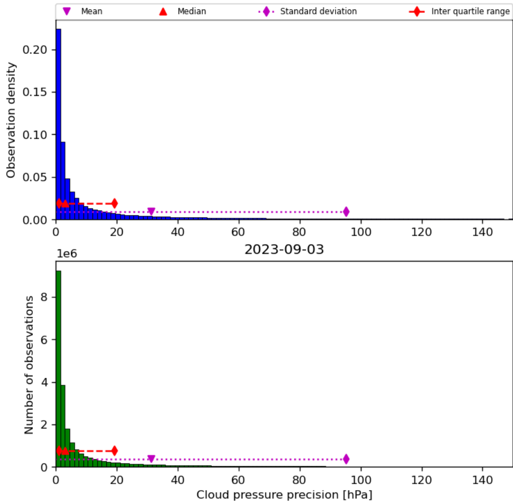
Figure 31: Histogram of “Cloud pressure precision” for 2023-09-02 to 2023-09-04
