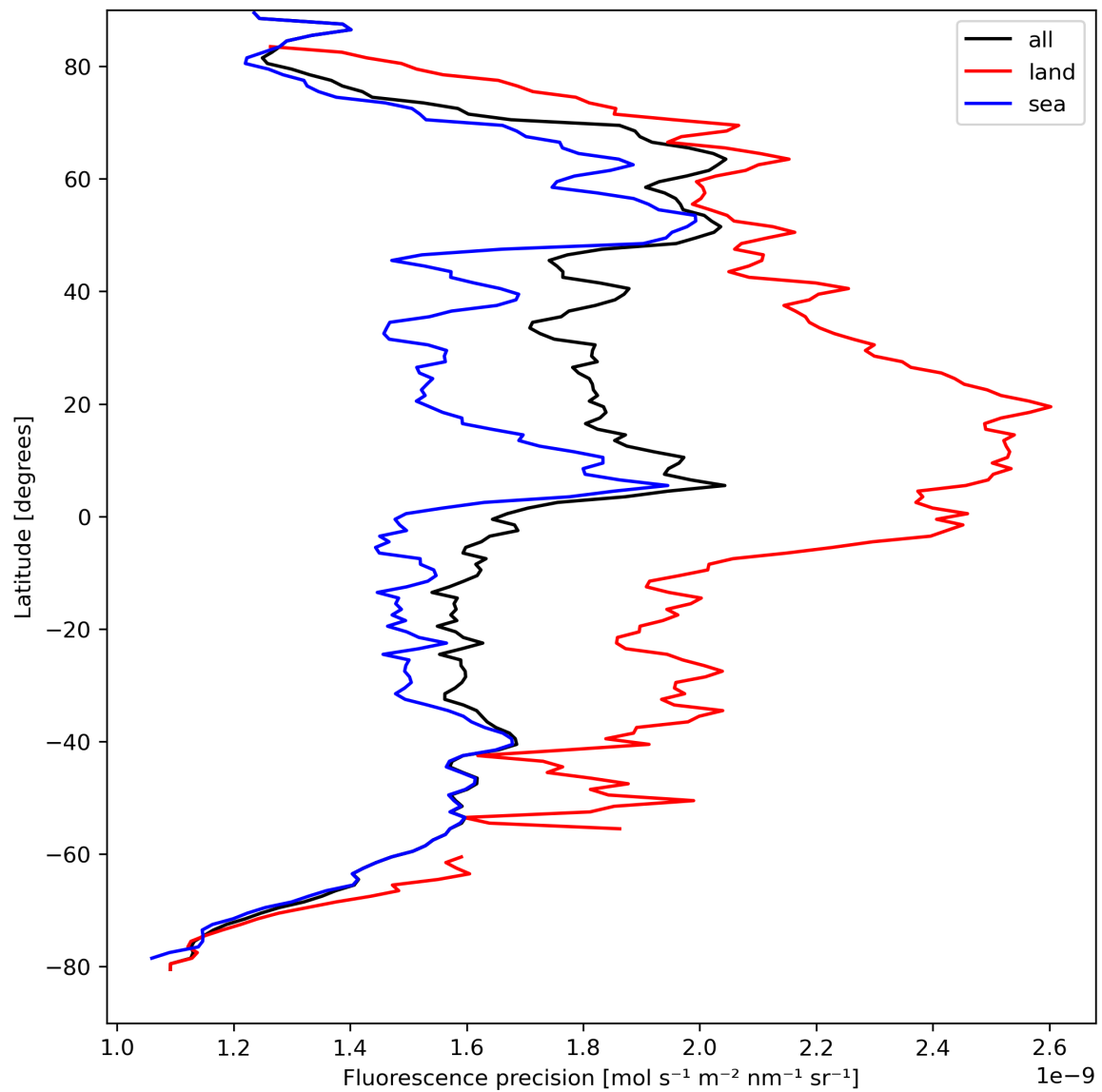
Figure 24: Zonal average of “Fluorescence precision” for 2023-09-02 to 2023-09-04.
