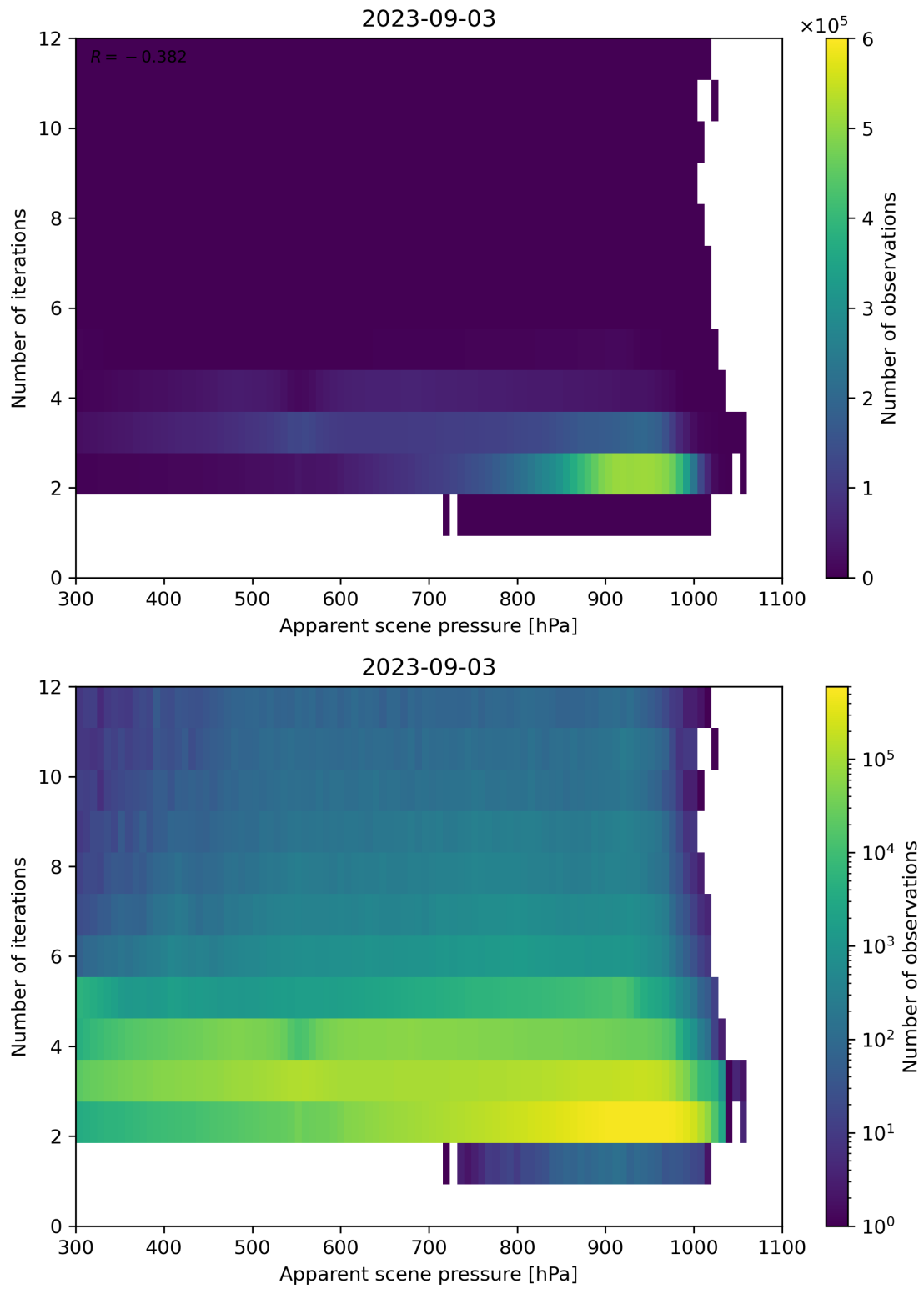
Figure 66: Scatter density plot of “Apparent scene pressure” against “Number of iterations” for 2023-09-02 to 2023-09-04.
