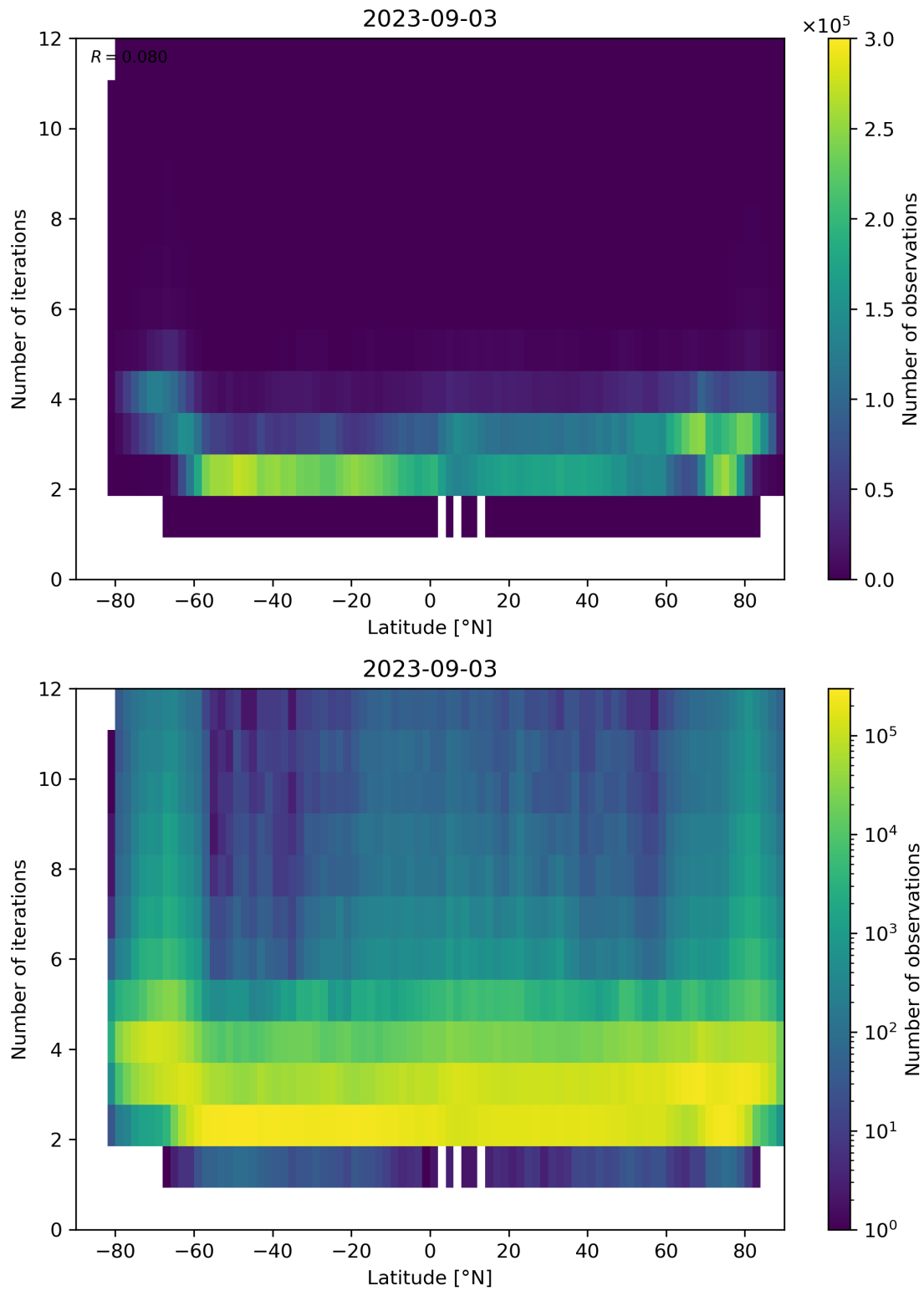
Figure 102: Scatter density plot of “Latitude” against “Number of iterations” for 2023-09-02 to 2023-09-04.
