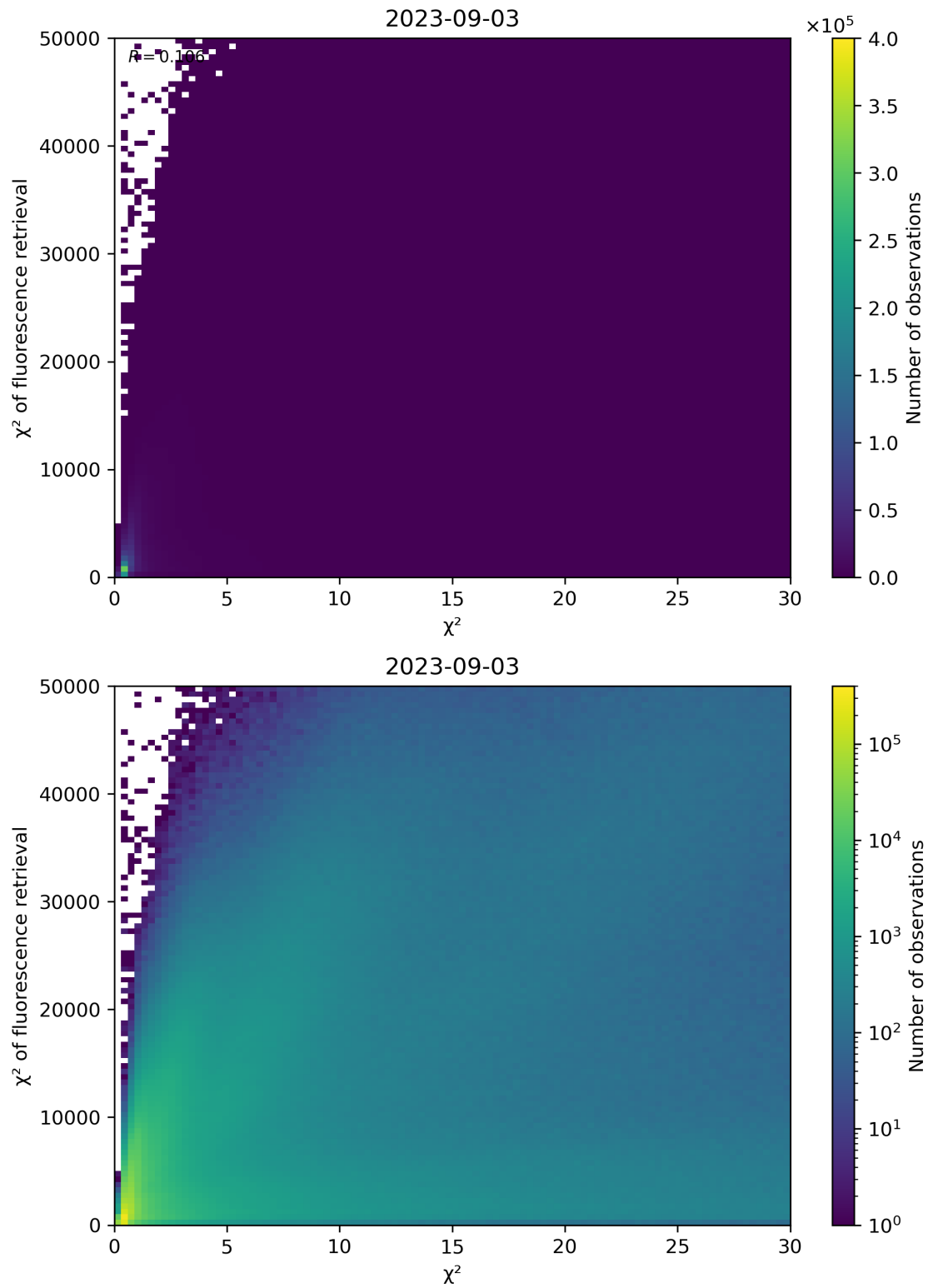
Figure 69: Scatter density plot of “ \chi^2 ” against “ \chi^2 of fluorescence retrieval” for 2023-09-02 to 2023-09-04.
