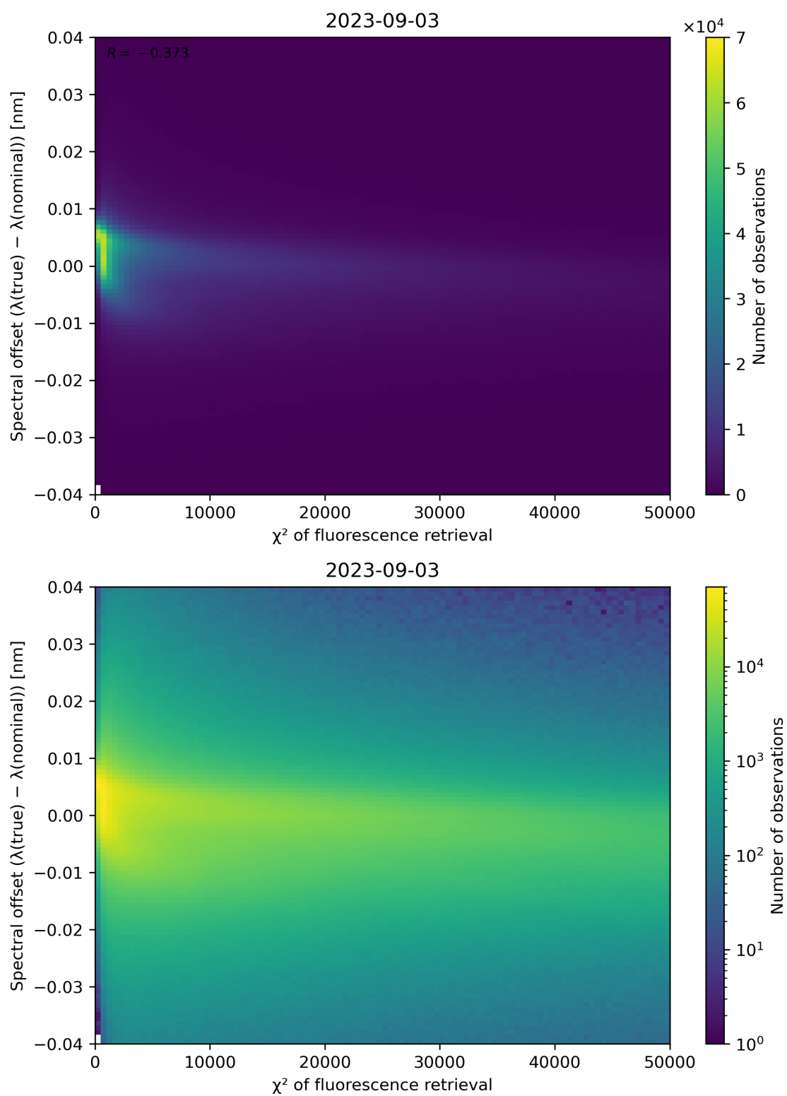
Figure 72: Scatter density plot of " \chi^2 of fluorescence retrieval" against "Spectral offset ( \lambda(\text{true}) - \lambda(\text{nominal}) )" for 2023-09-02 to 2023-09-04.
