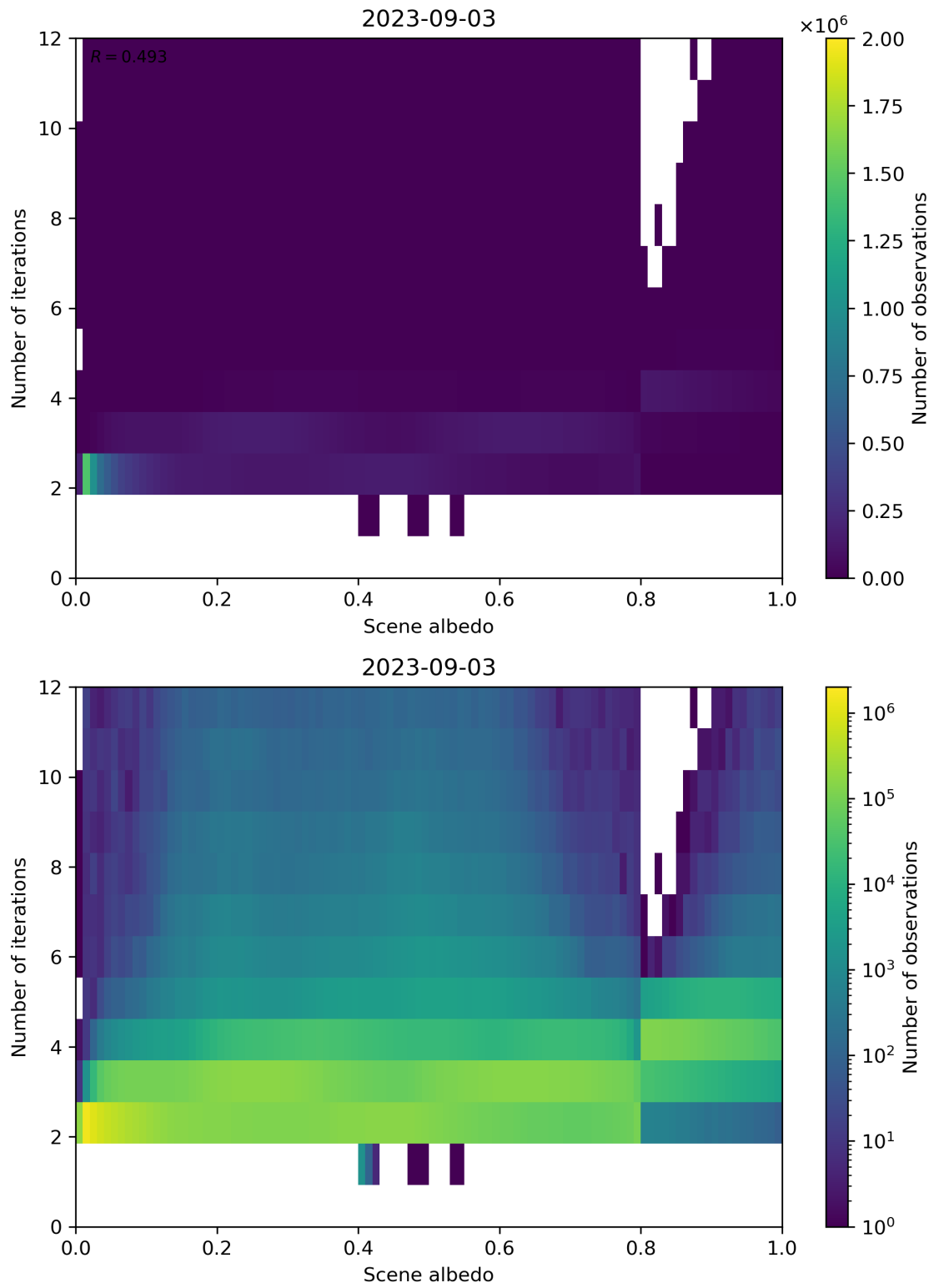
Figure 115: Scatter density plot of “Scene albedo” against “Number of iterations” for 2023-09-02 to 2023-09-04.
