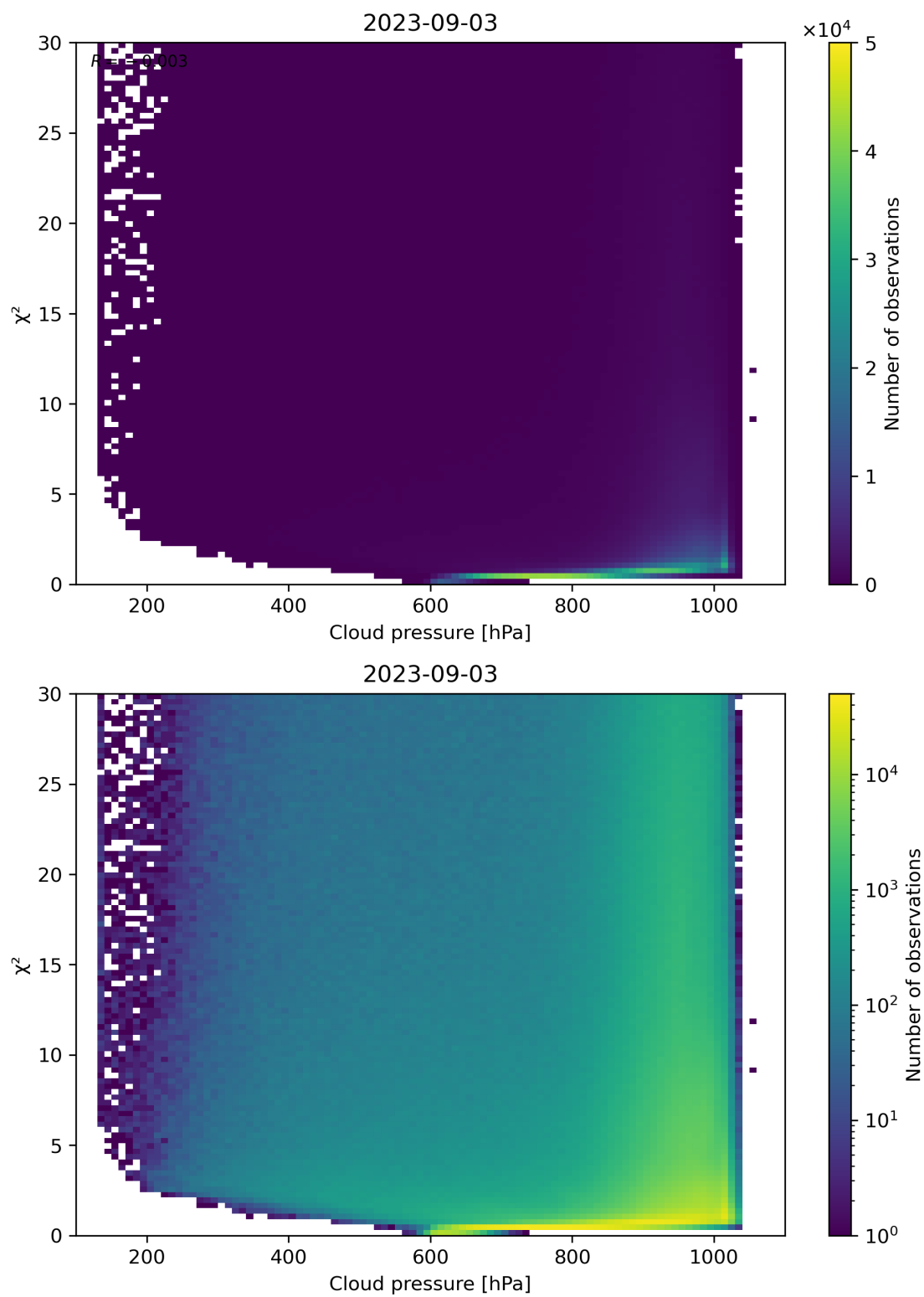
Figure 85: Scatter density plot of “Cloud pressure” against “ \chi^2 ” for 2023-09-02 to 2023-09-04.
