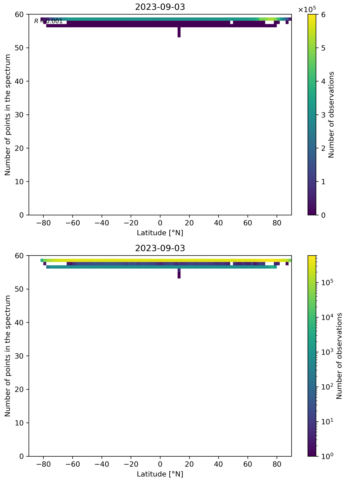
Figure 103: Scatter density plot of “Latitude” against “Number of points in the spectrum” for 2023-09-02 to 2023-09-04.
