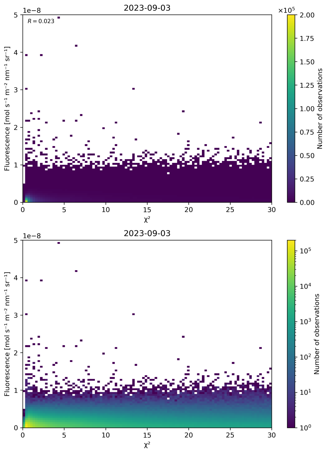
Figure 70: Scatter density plot of “ \chi^2 ” against “Fluorescence” for 2023-09-02 to 2023-09-04.
