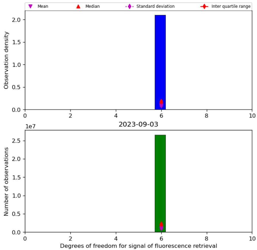
Figure 43: Histogram of “Degrees of freedom for signal of fluorescence retrieval” for 2023-09-02 to 2023-09-04
