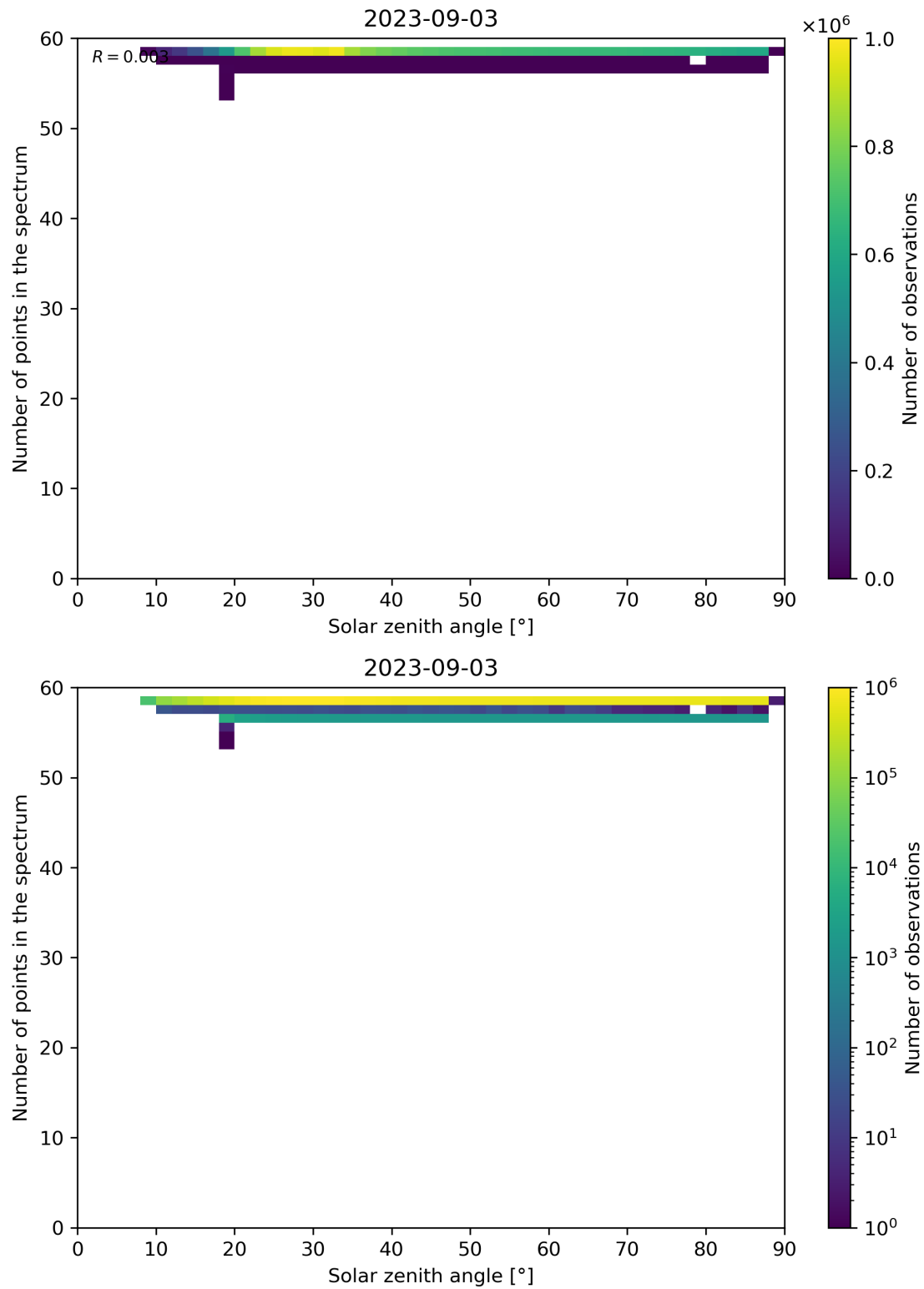
Figure 126: Scatter density plot of “Solar zenith angle” against “Number of points in the spectrum” for 2023-09-02 to 2023-09-04.
