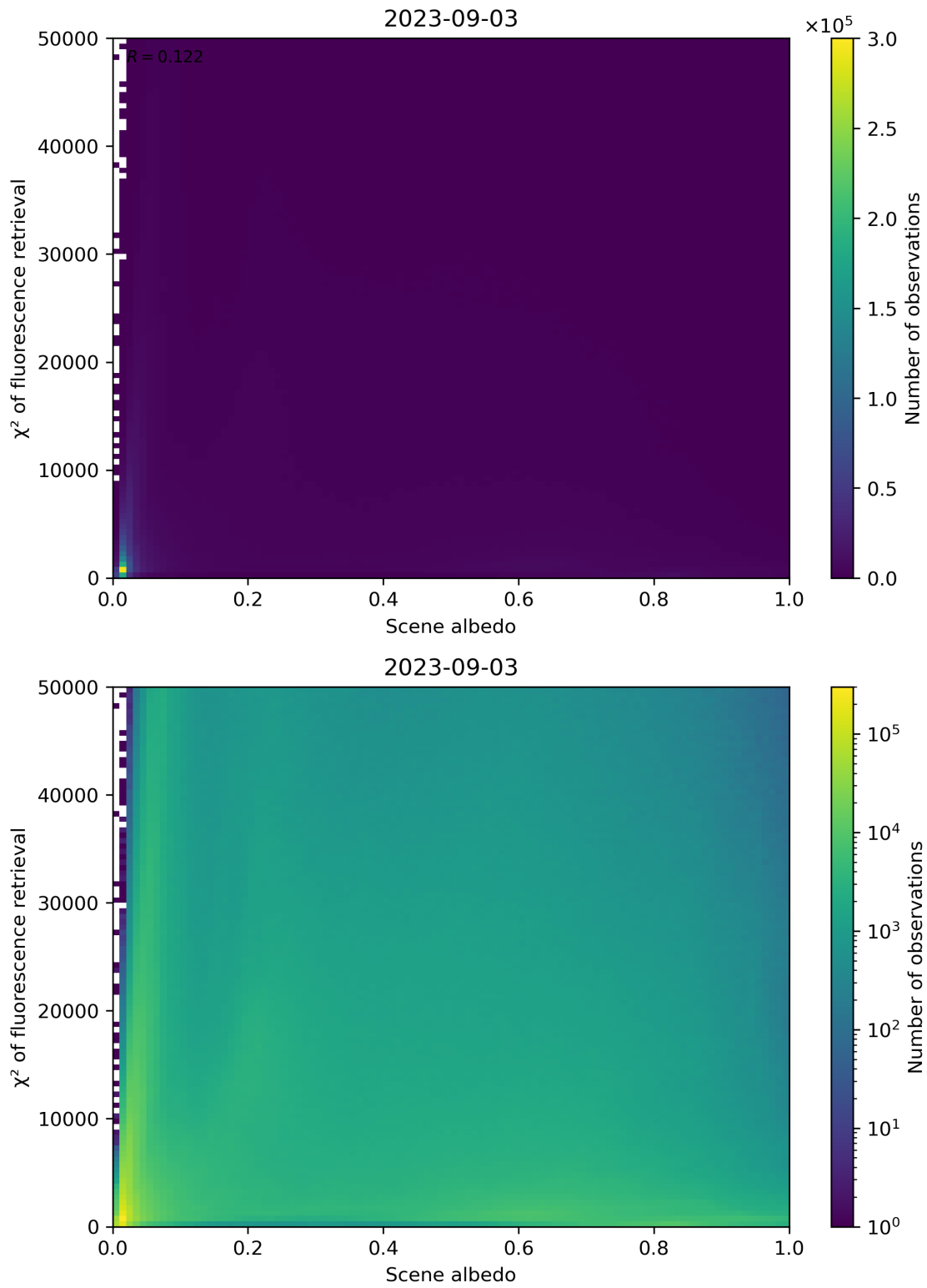
Figure 113: Scatter density plot of “Scene albedo” against “ \chi^2 of fluorescence retrieval” for 2023-09-02 to 2023-09-04.
