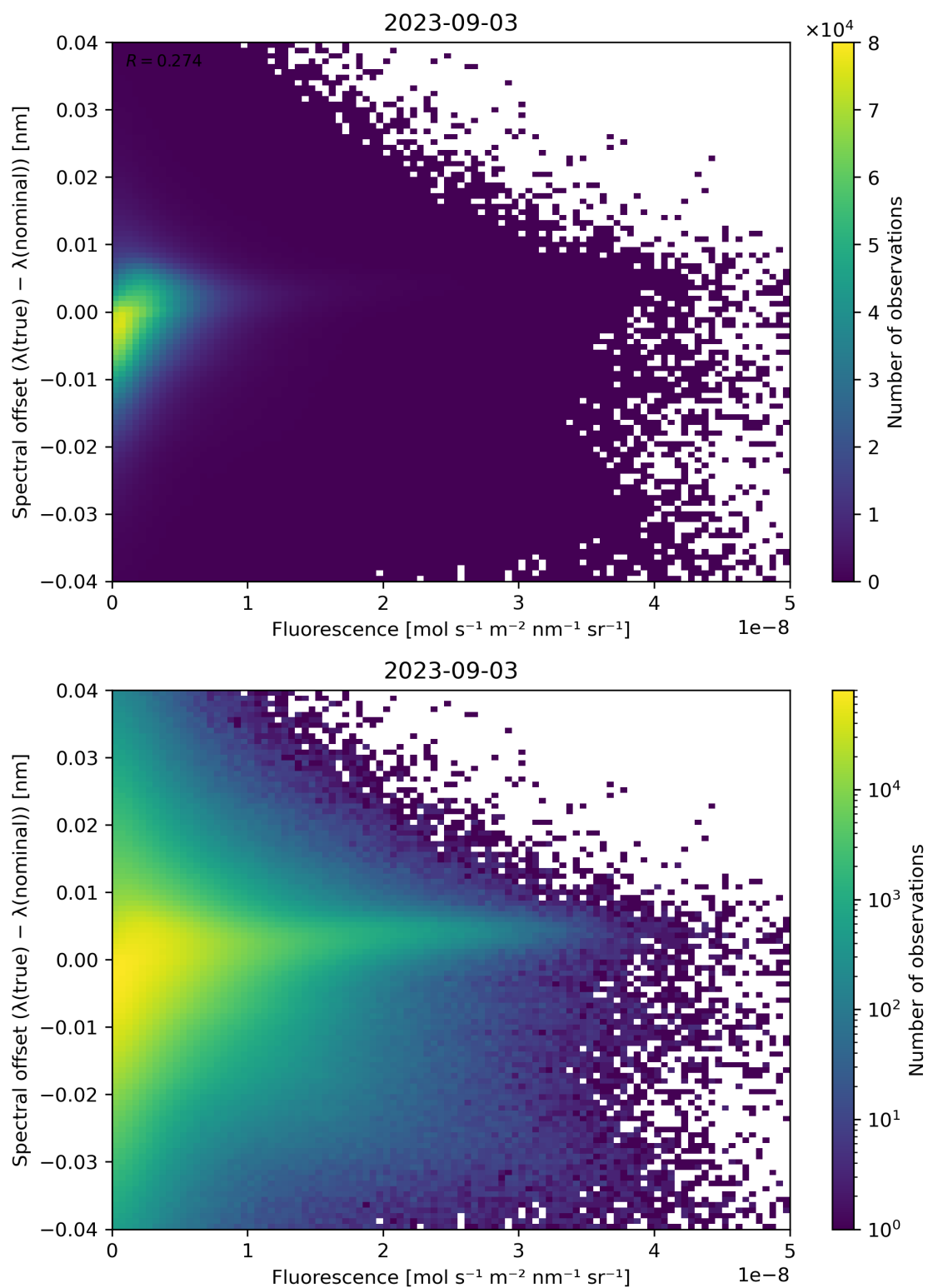
Figure 95: Scatter density plot of “Fluorescence” against “Spectral offset ( \lambda(\text{true}) - \lambda(\text{nominal}) )” for 2023-09-02 to 2023-09-04.
