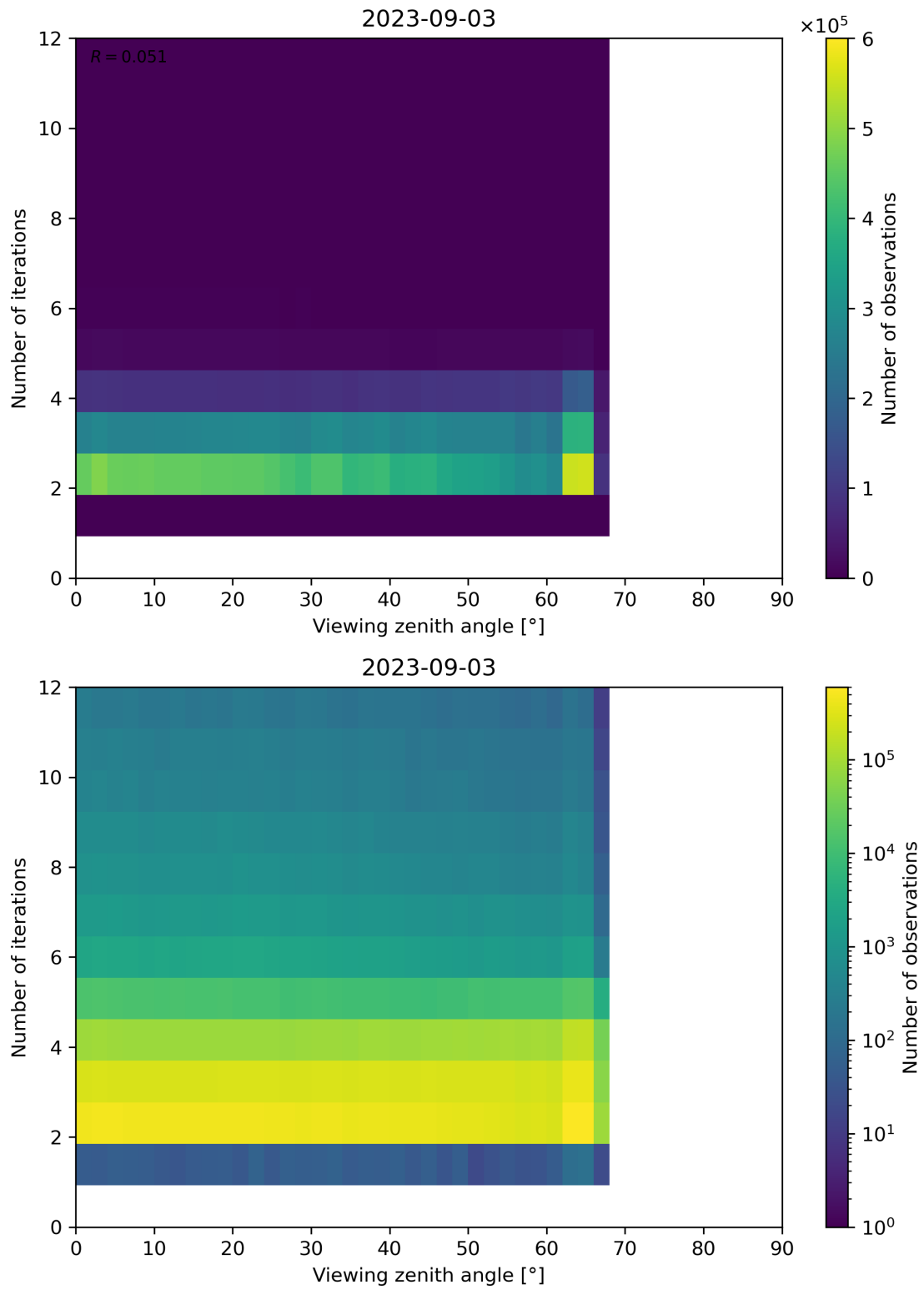
Figure 136: Scatter density plot of “Viewing zenith angle” against “Number of iterations” for 2023-09-02 to 2023-09-04.
