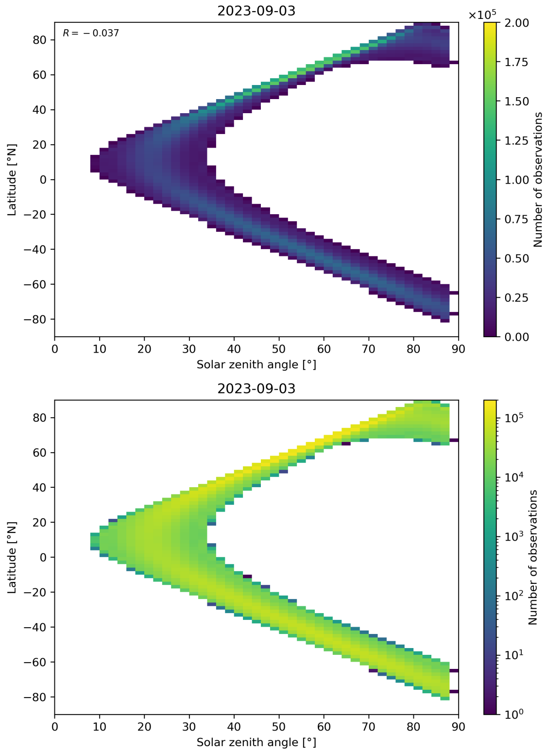
Figure 124: Scatter density plot of “Solar zenith angle” against “Latitude” for 2023-09-02 to 2023-09-04.
