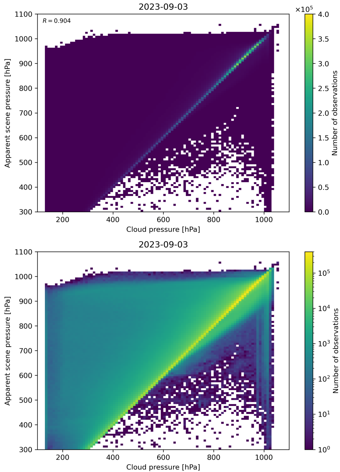
Figure 84: Scatter density plot of “Cloud pressure” against “Apparent scene pressure” for 2023-09-02 to 2023-09-04.
