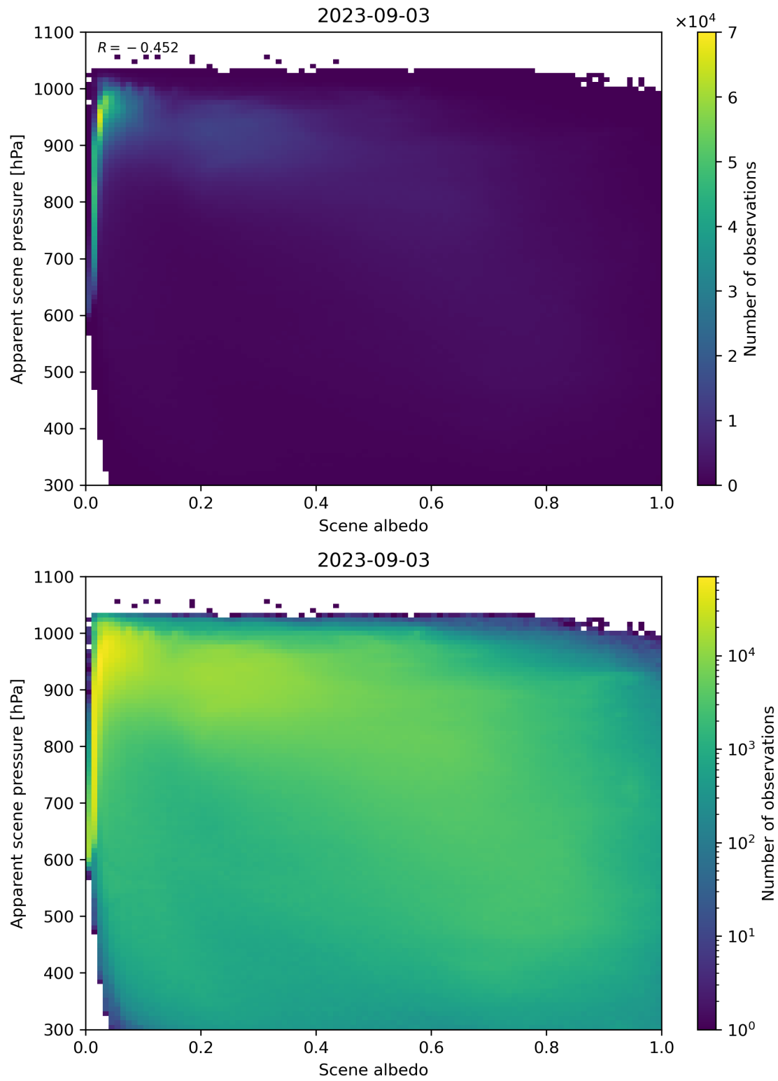
Figure 111: Scatter density plot of “Scene albedo” against “Apparent scene pressure” for 2023-09-02 to 2023-09-04.
