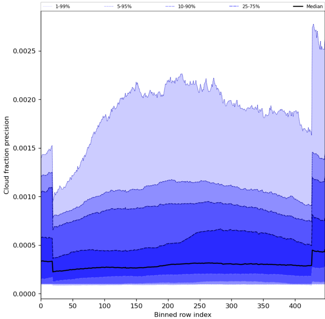
Figure 50: Along track statistics of “Cloud fraction precision” for 2023-09-02 to 2023-09-04
