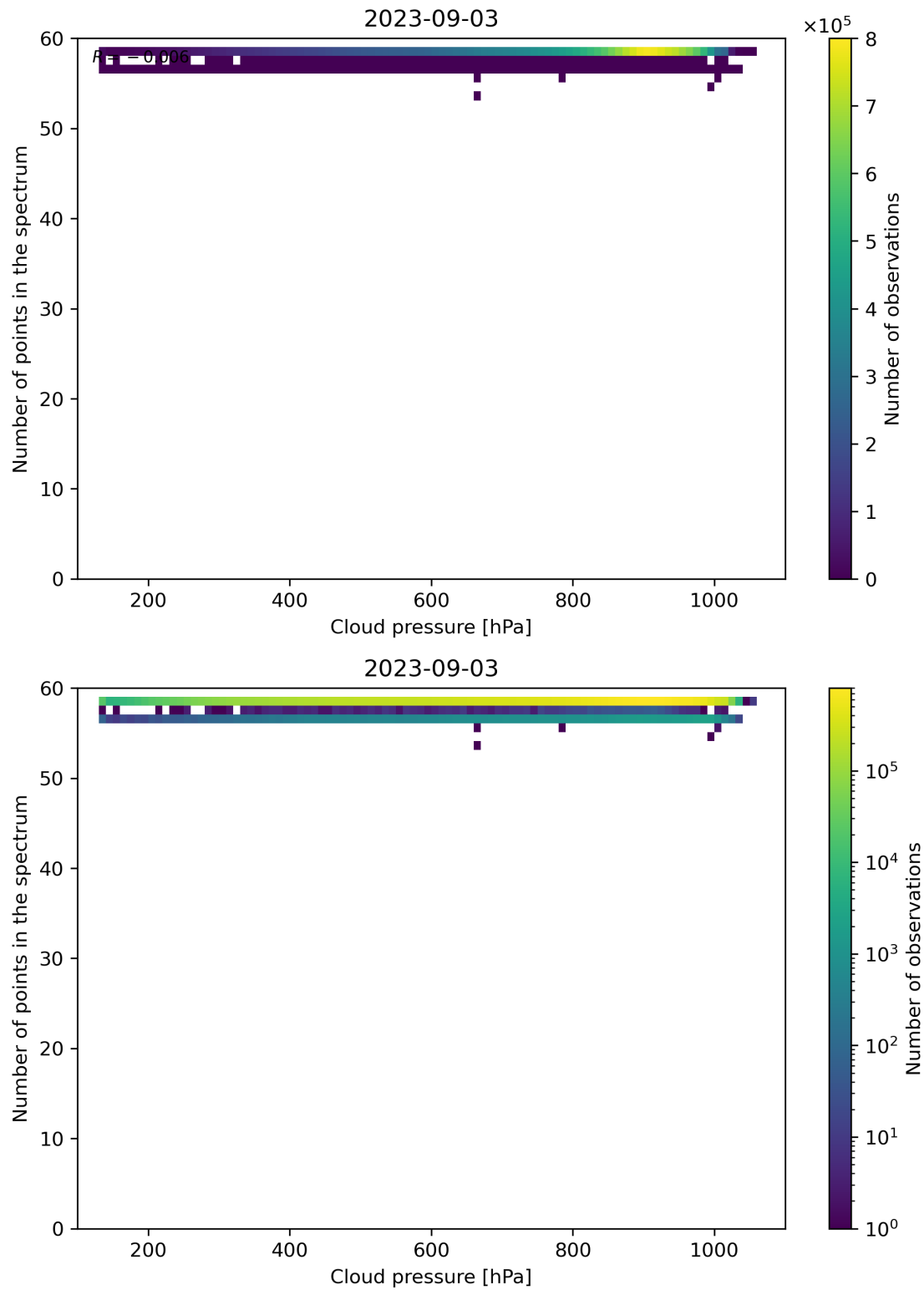
Figure 90: Scatter density plot of “Cloud pressure” against “Number of points in the spectrum” for 2023-09-02 to 2023-09-04.
