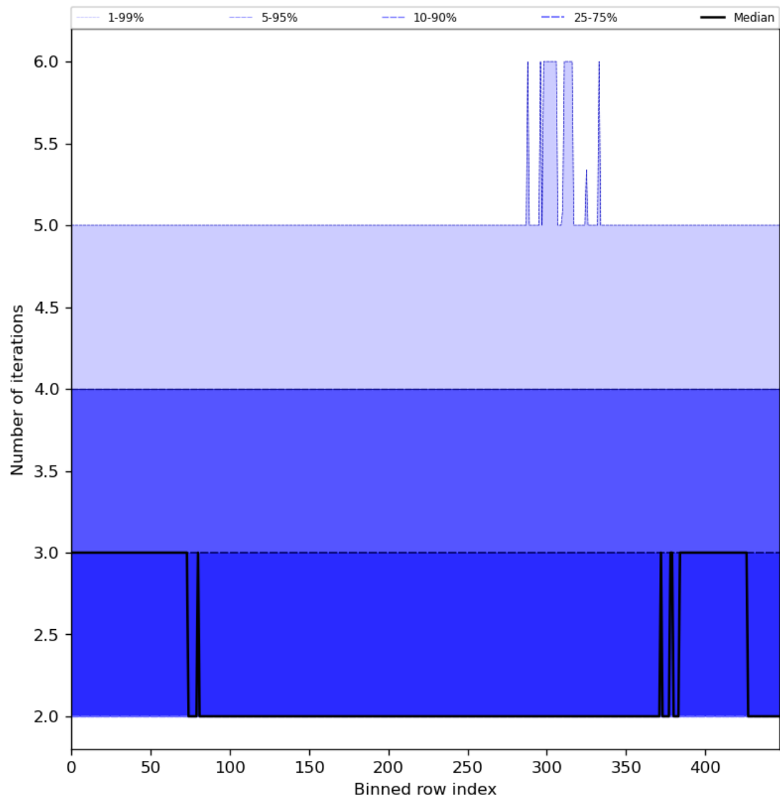
Figure 56: Along track statistics of "Number of iterations" for 2023-09-02 to 2023-09-04
