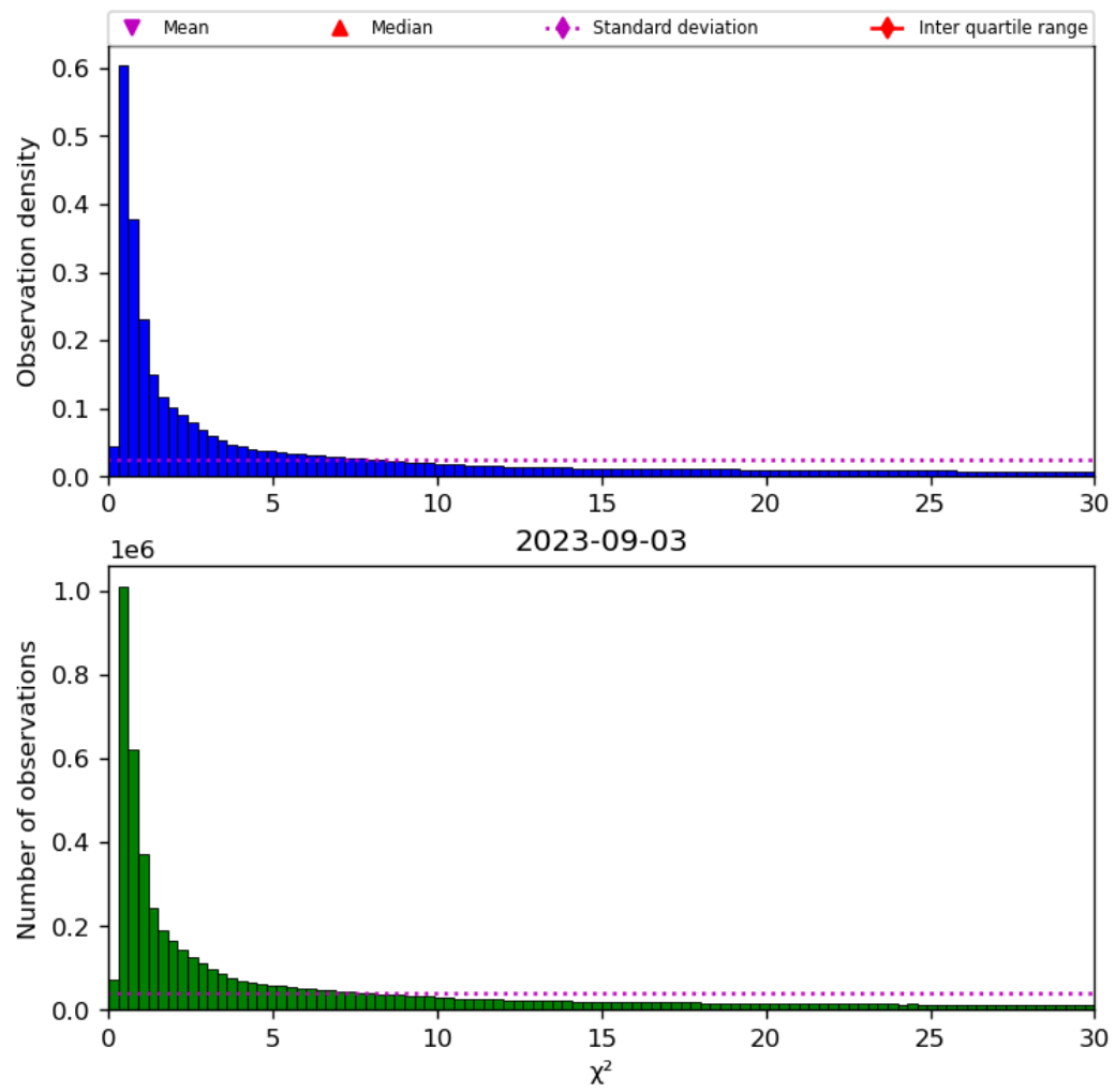
Figure 38: Histogram of “ \chi^2 ” for 2023-09-02 to 2023-09-04
