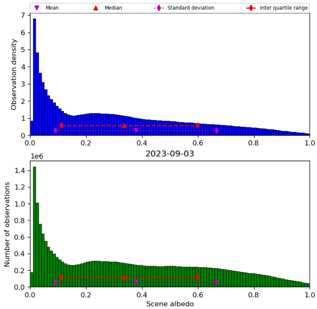
Figure 34: Histogram of “Scene albedo” for 2023-09-02 to 2023-09-04
