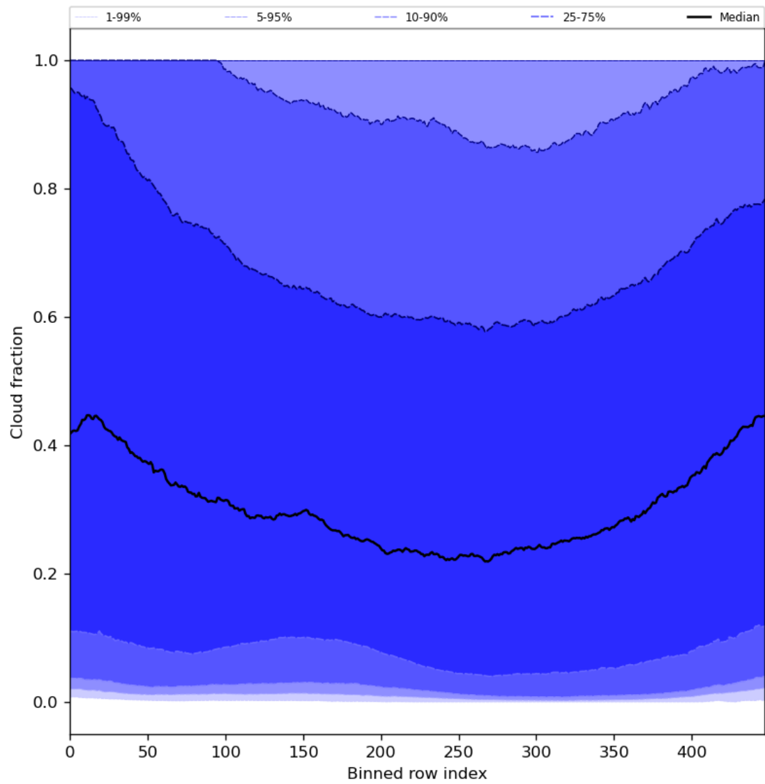
Figure 49: Along track statistics of “Cloud fraction” for 2023-09-02 to 2023-09-04
