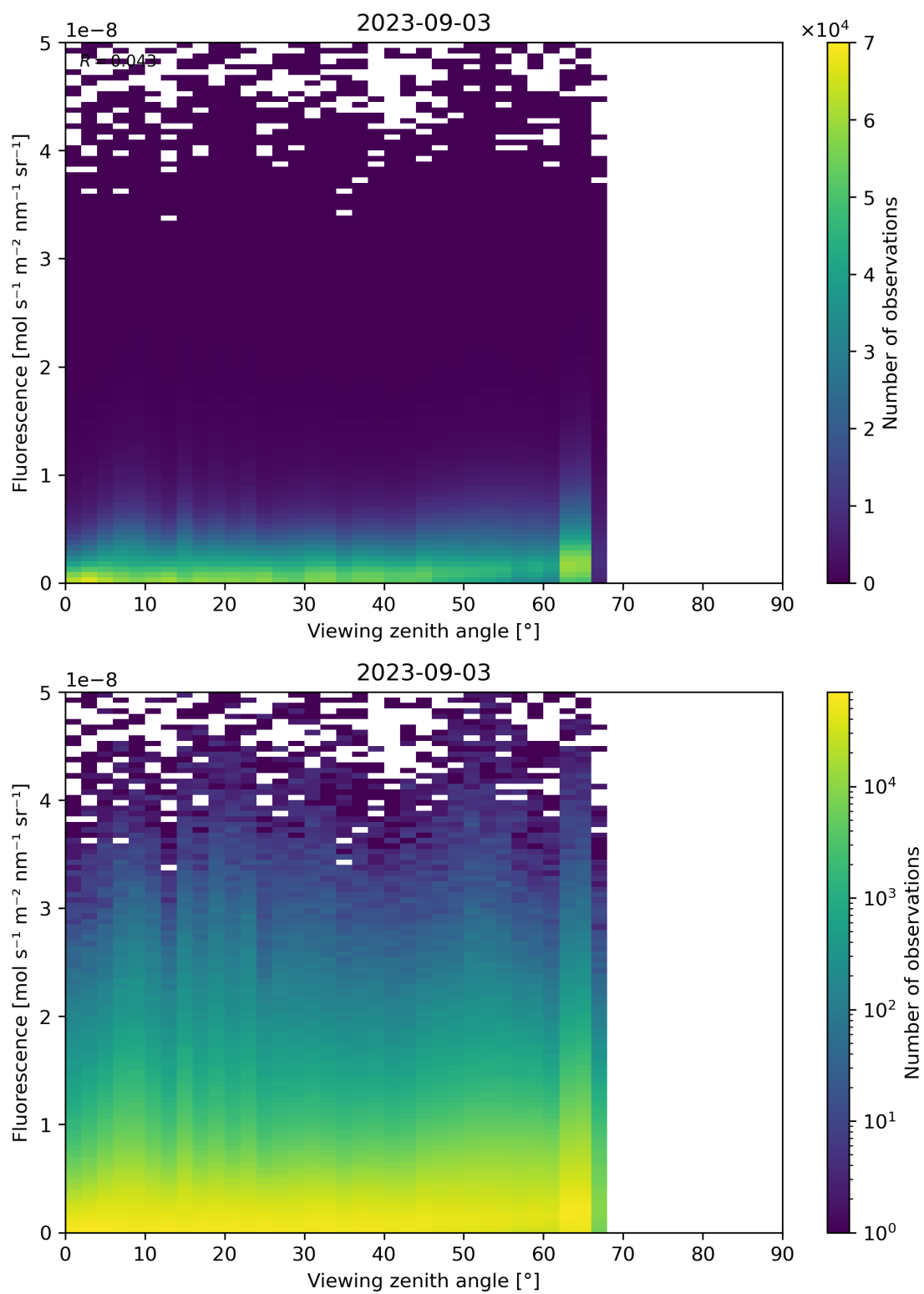
Figure 134: Scatter density plot of “Viewing zenith angle” against “Fluorescence” for 2023-09-02 to 2023-09-04.
