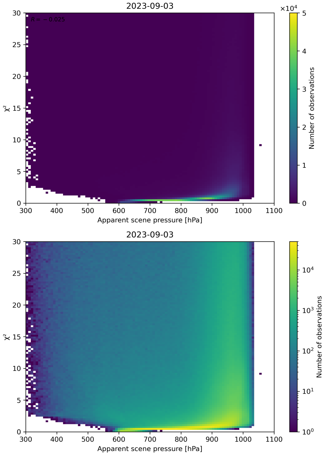
Figure 63: Scatter density plot of “Apparent scene pressure” against “ \chi^2 ” for 2023-09-02 to 2023-09-04.
