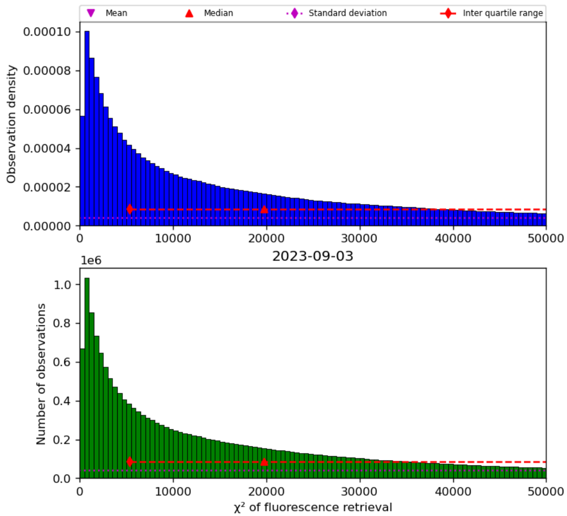
Figure 42: Histogram of “ \chi^2 of fluorescence retrieval” for 2023-09-02 to 2023-09-04
