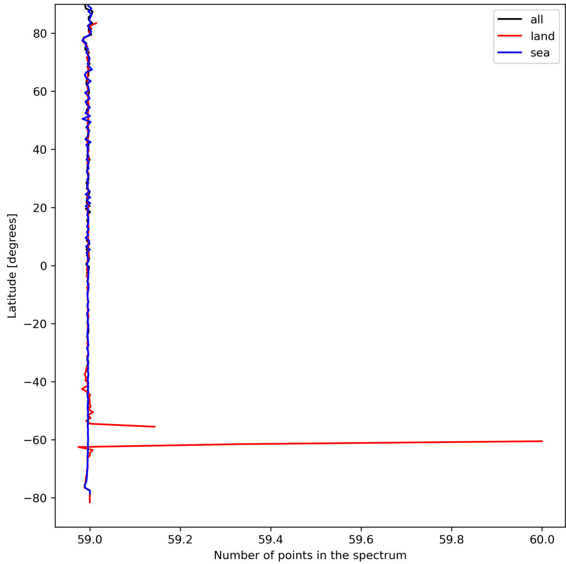
Figure 27: Zonal average of “Number of points in the spectrum” for 2023-09-04 to 2023-09-05.
