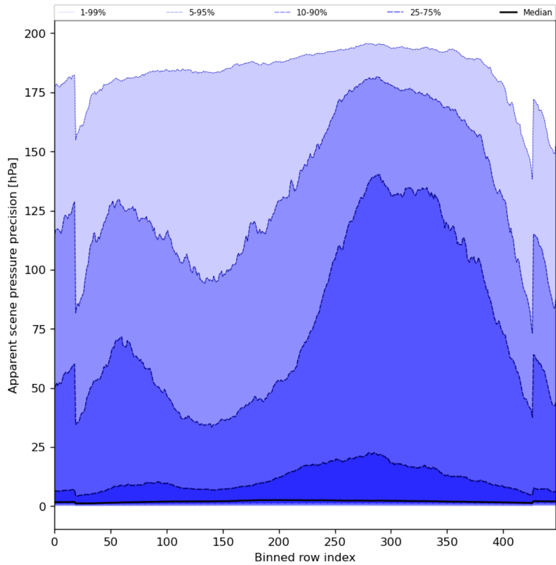
Figure 54: Along track statistics of “Apparent scene pressure precision” for 2023-09-04 to 2023-09-05
