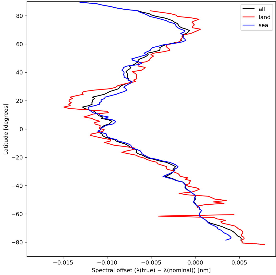
Figure 28: Zonal average of “Spectral offset ( \lambda(\text{true}) - \lambda(\text{nominal}) )” for 2023-09-04 to 2023-09-05.
