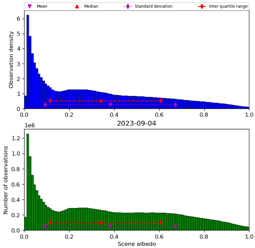
Figure 34: Histogram of “Scene albedo” for 2023-09-04 to 2023-09-05
