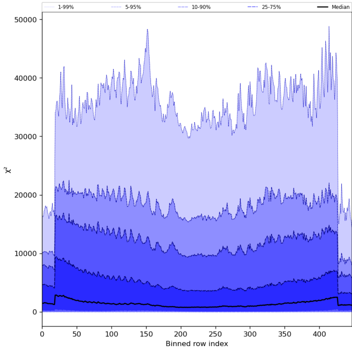
Figure 55: Along track statistics of “ \chi^2 ” for 2023-09-04 to 2023-09-05
