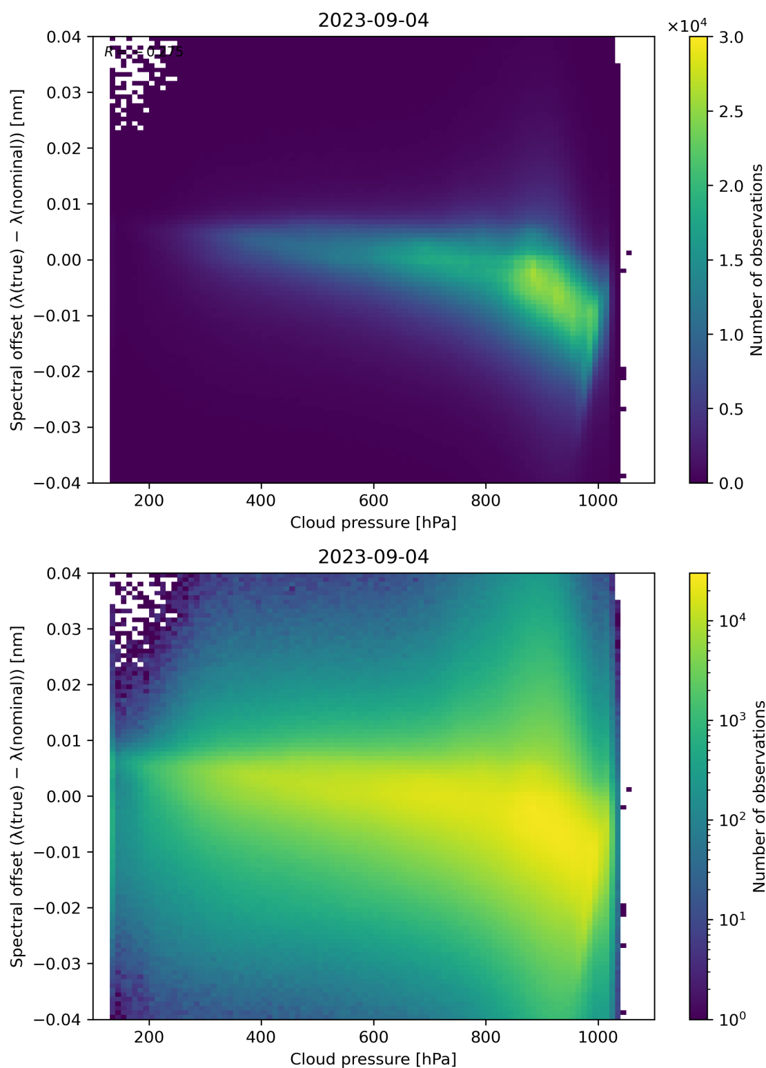
Figure 92: Scatter density plot of “Cloud pressure” against “Spectral offset ( \lambda(\text{true}) - \lambda(\text{nominal}) )” for 2023-09-04 to 2023-09-05.
