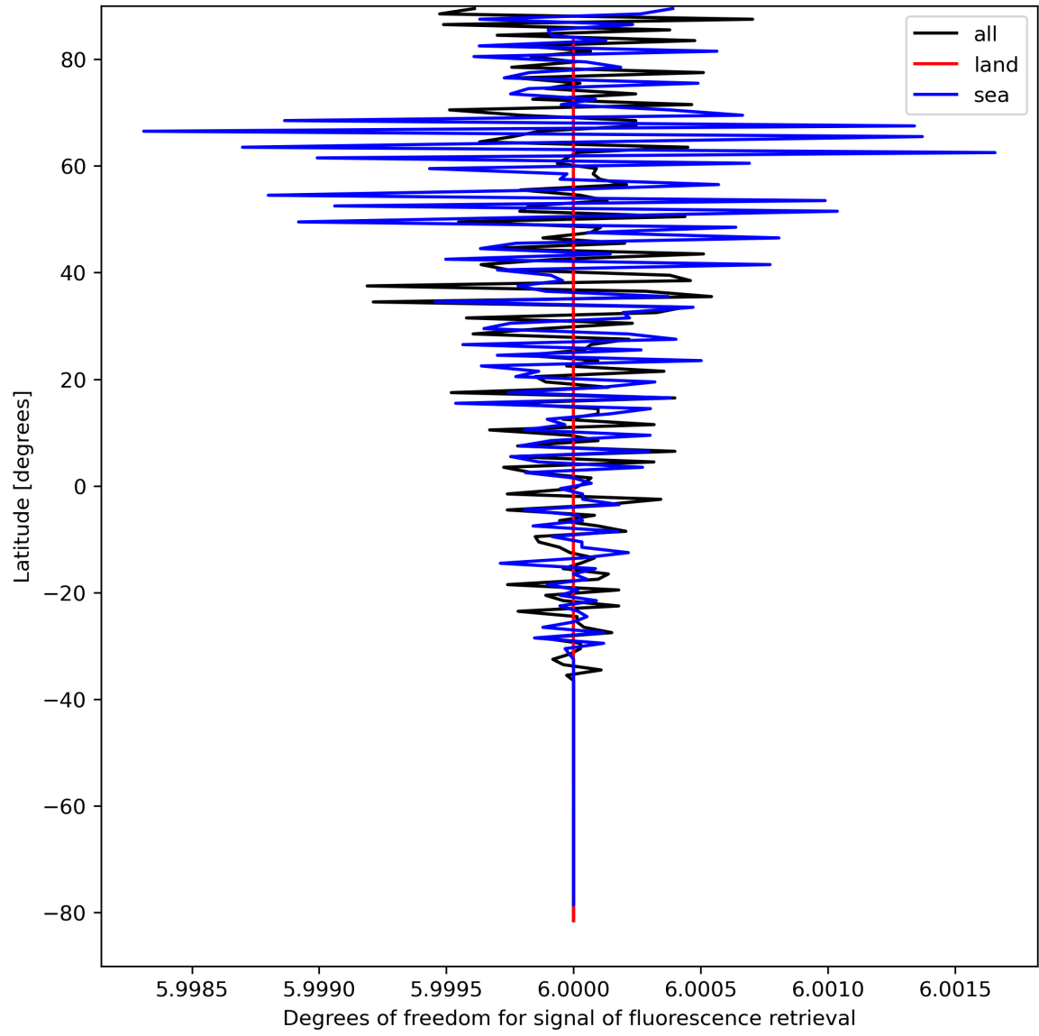
Figure 26: Zonal average of “Degrees of freedom for signal of fluorescence retrieval” for 2023-09-04 to 2023-09-05.
