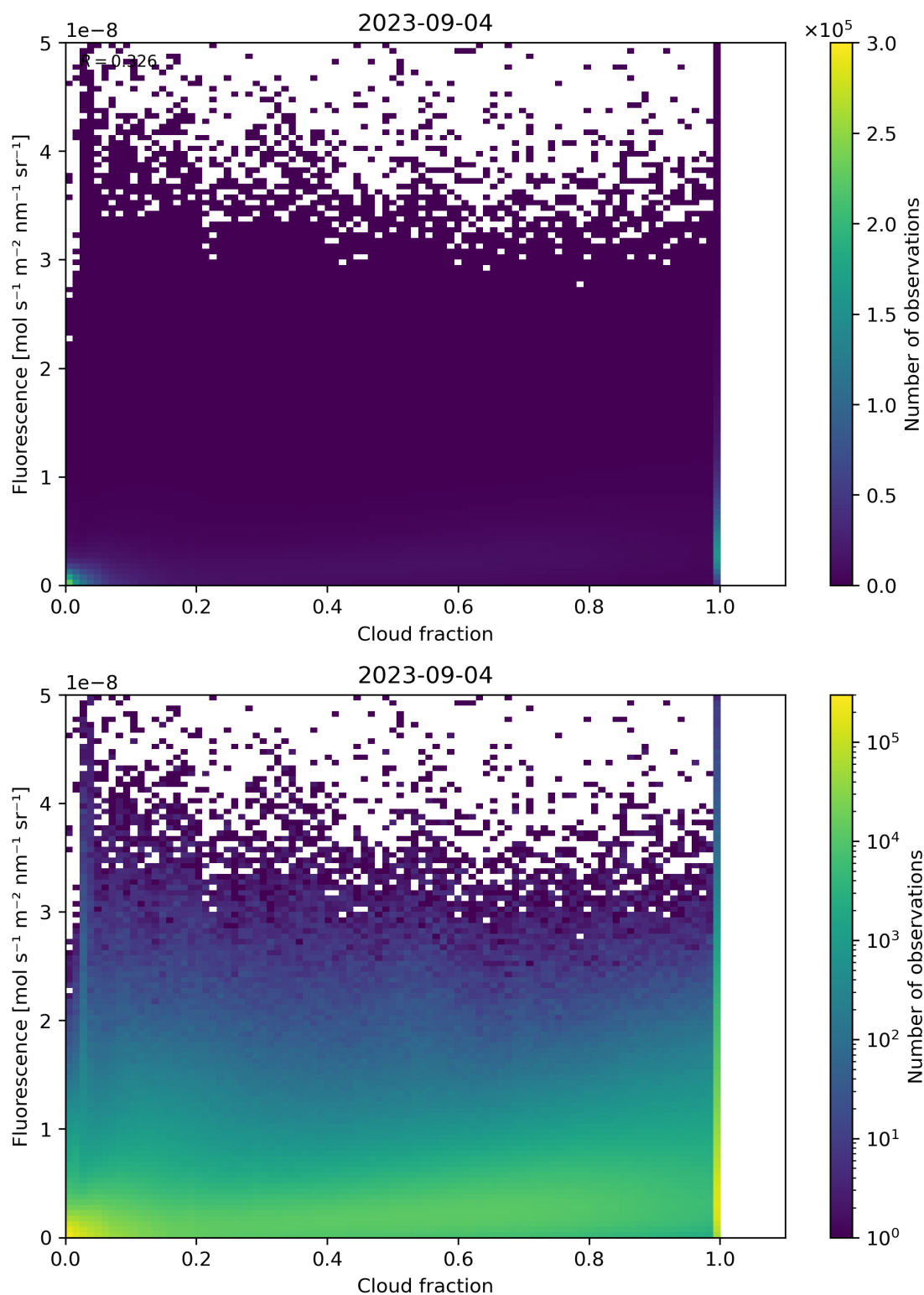
Figure 79: Scatter density plot of “Cloud fraction” against “Fluorescence” for 2023-09-04 to 2023-09-05.
