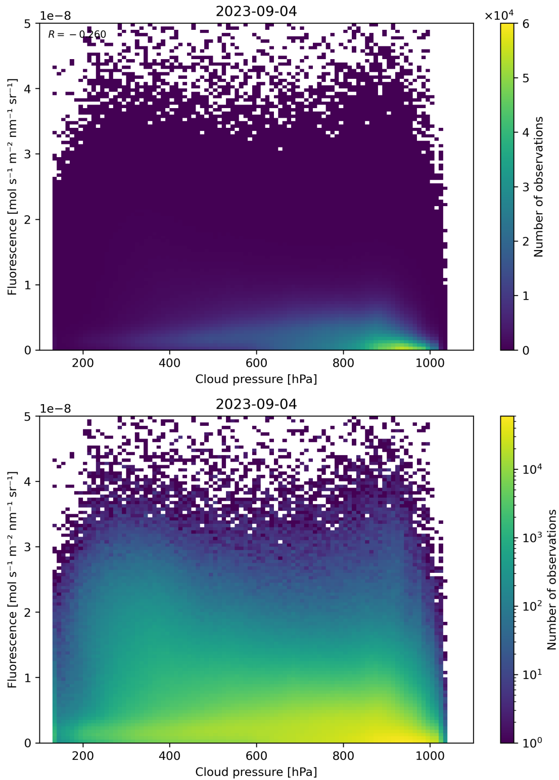
Figure 88: Scatter density plot of “Cloud pressure” against “Fluorescence” for 2023-09-04 to 2023-09-05.
