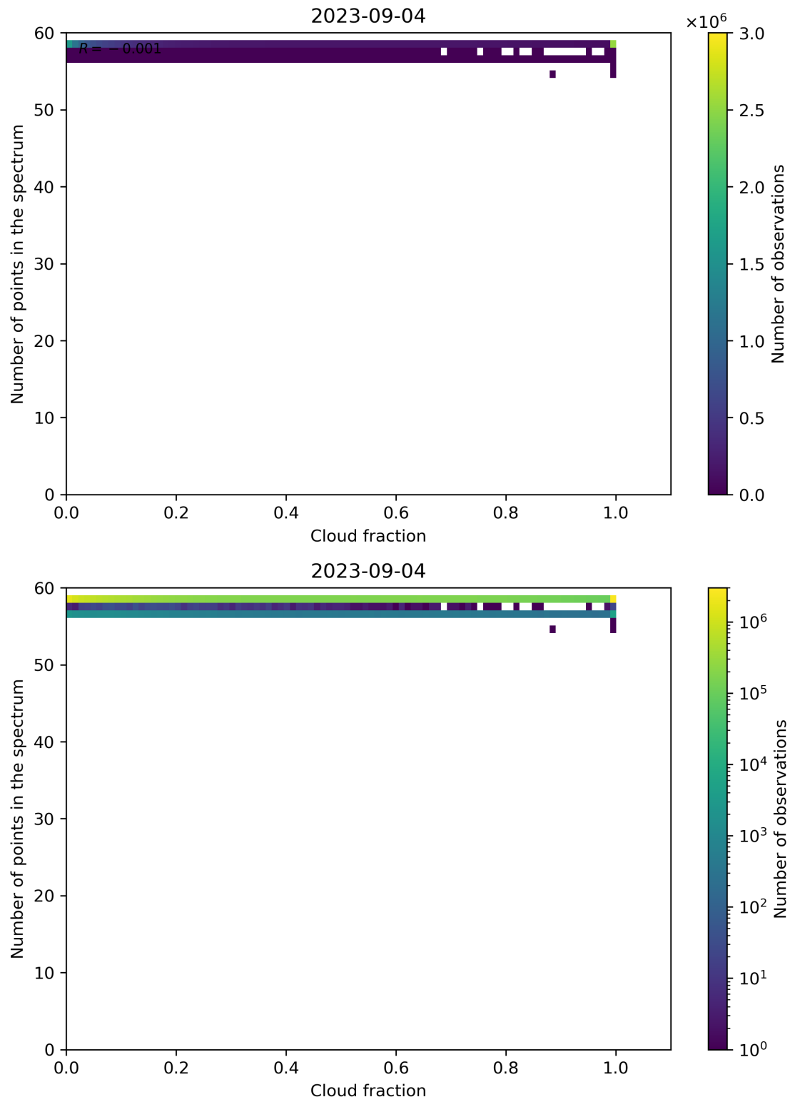
Figure 81: Scatter density plot of “Cloud fraction” against “Number of points in the spectrum” for 2023-09-04 to 2023-09-05.
