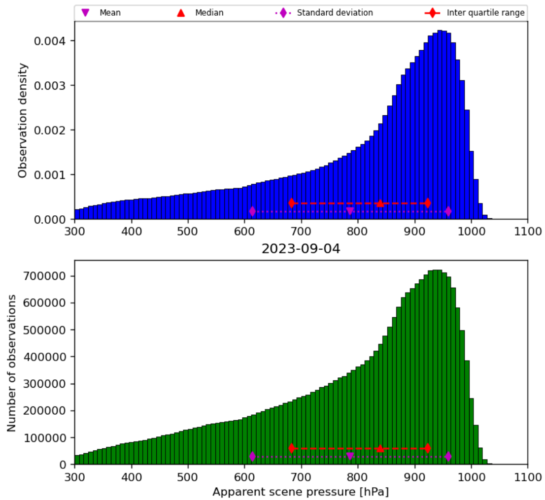
Figure 36: Histogram of “Apparent scene pressure” for 2023-09-04 to 2023-09-05
