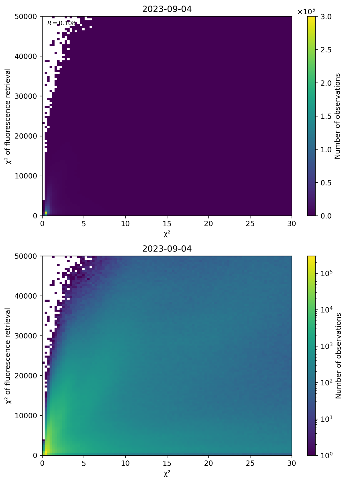
Figure 69: Scatter density plot of “ \chi^2 ” against “ \chi^2 of fluorescence retrieval” for 2023-09-04 to 2023-09-05.
