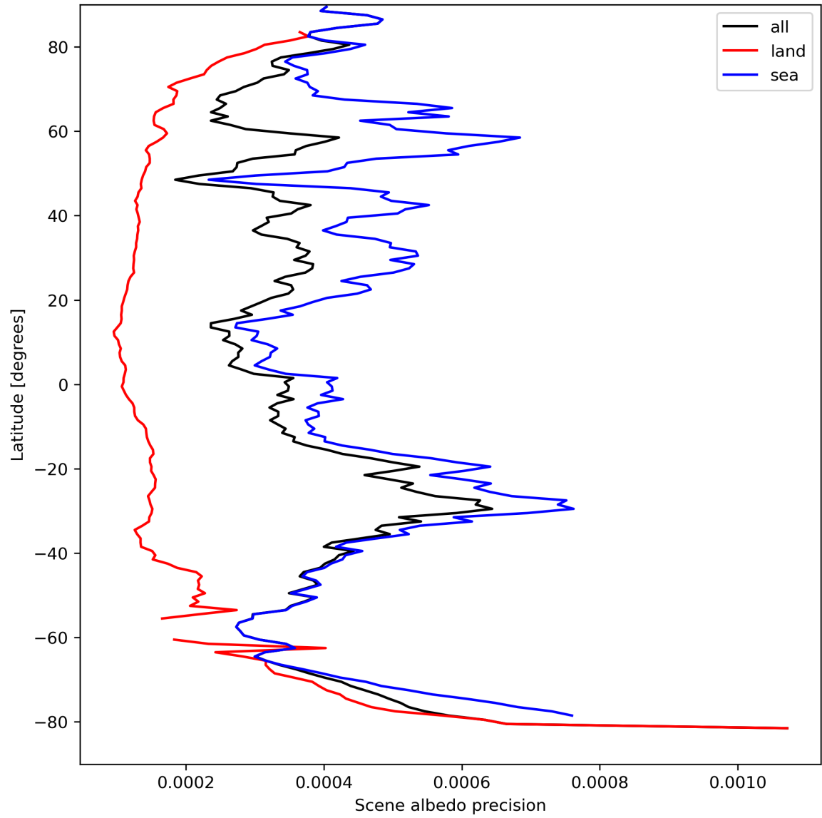
Figure 18: Zonal average of “Scene albedo precision” for 2023-09-04 to 2023-09-05.
