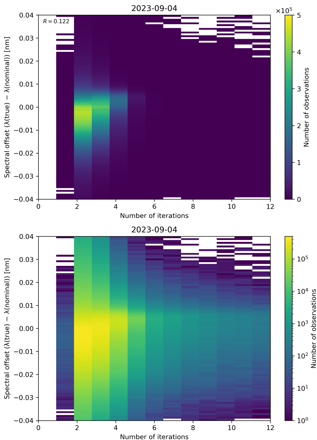
Figure 109: Scatter density plot of “Number of iterations” against “Spectral offset ( \lambda(\text{true}) - \lambda(\text{nominal}) )” for 2023-09-04 to 2023-09-05.
