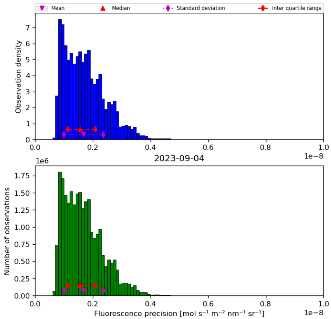
Figure 41: Histogram of “Fluorescence precision” for 2023-09-04 to 2023-09-05
