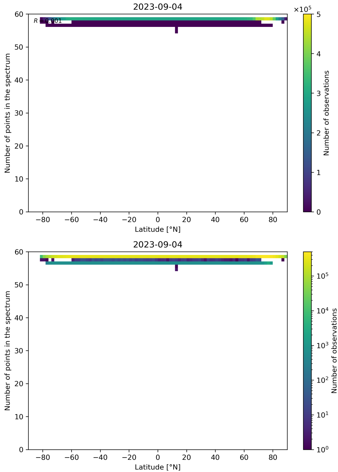
Figure 103: Scatter density plot of “Latitude” against “Number of points in the spectrum” for 2023-09-04 to 2023-09-05.
