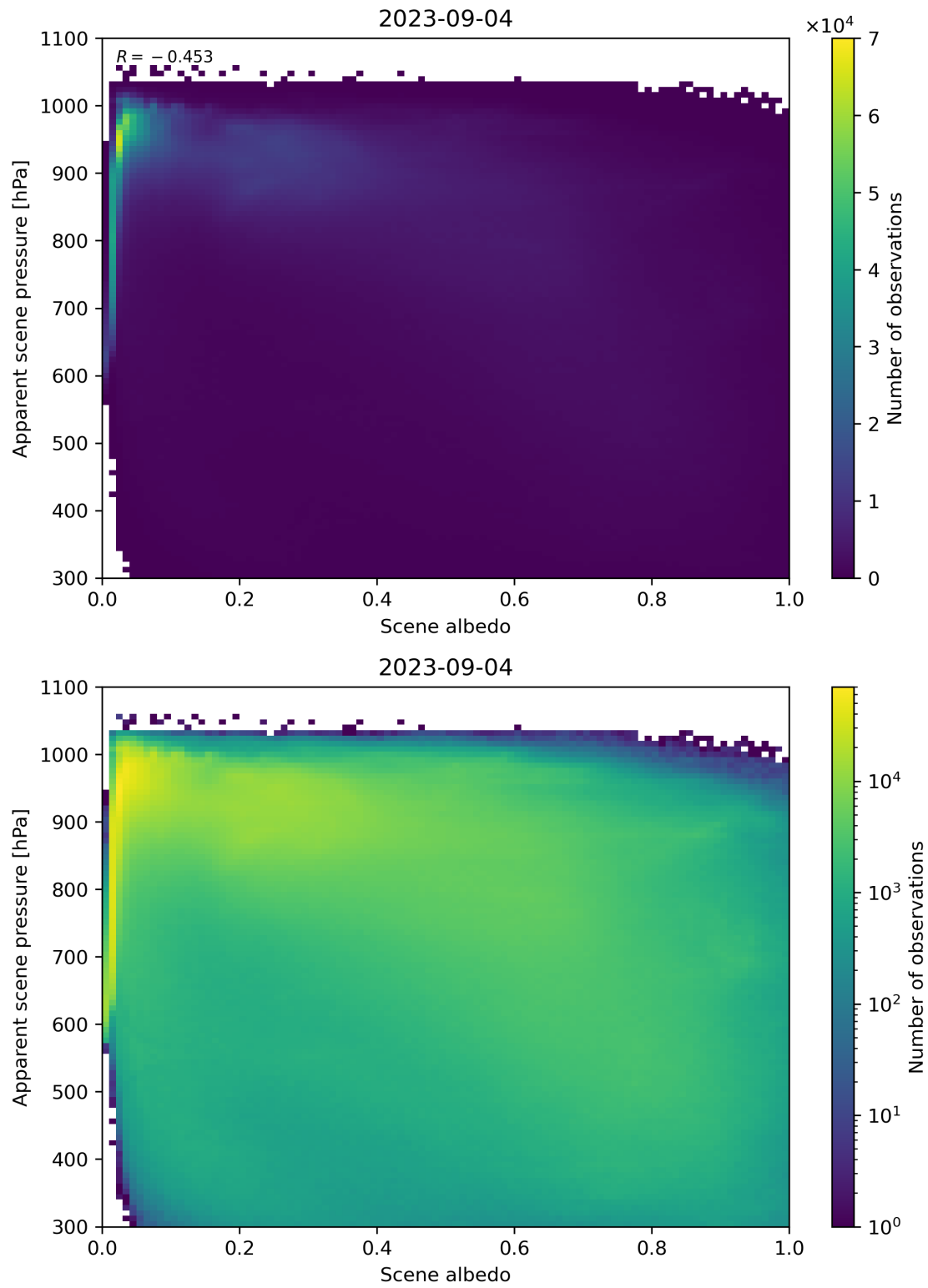
Figure 111: Scatter density plot of “Scene albedo” against “Apparent scene pressure” for 2023-09-04 to 2023-09-05.
