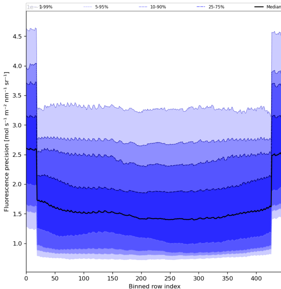
Figure 58: Along track statistics of “Fluorescence precision” for 2023-09-04 to 2023-09-05
