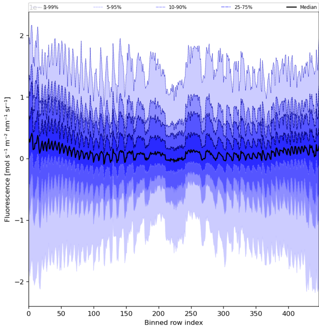
Figure 57: Along track statistics of “Fluorescence” for 2023-09-04 to 2023-09-05
