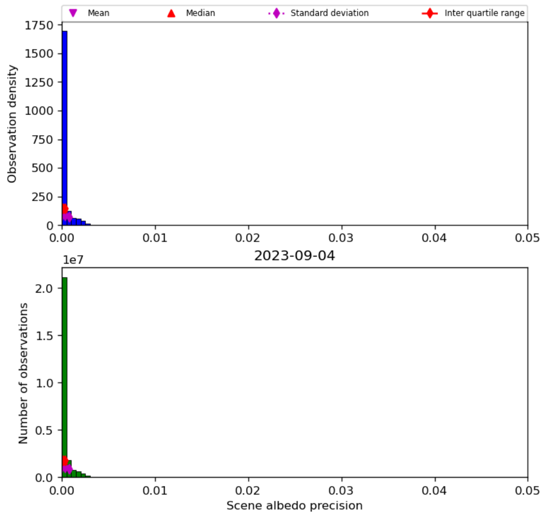
Figure 35: Histogram of “Scene albedo precision” for 2023-09-04 to 2023-09-05
