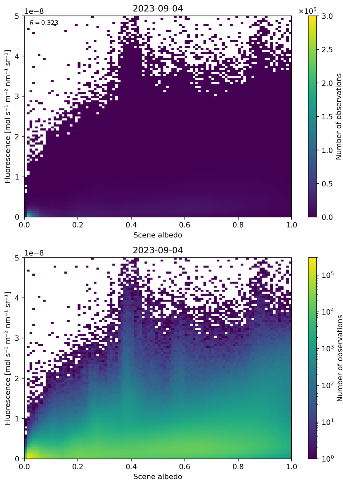
Figure 114: Scatter density plot of “Scene albedo” against “Fluorescence” for 2023-09-04 to 2023-09-05.
