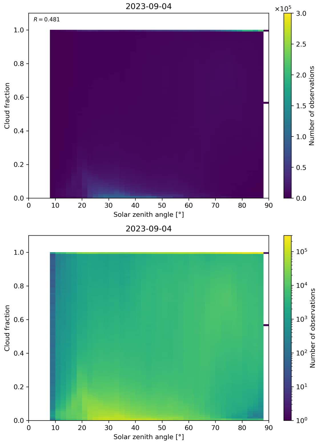
Figure 121: Scatter density plot of “Solar zenith angle” against “Cloud fraction” for 2023-09-04 to 2023-09-05.
