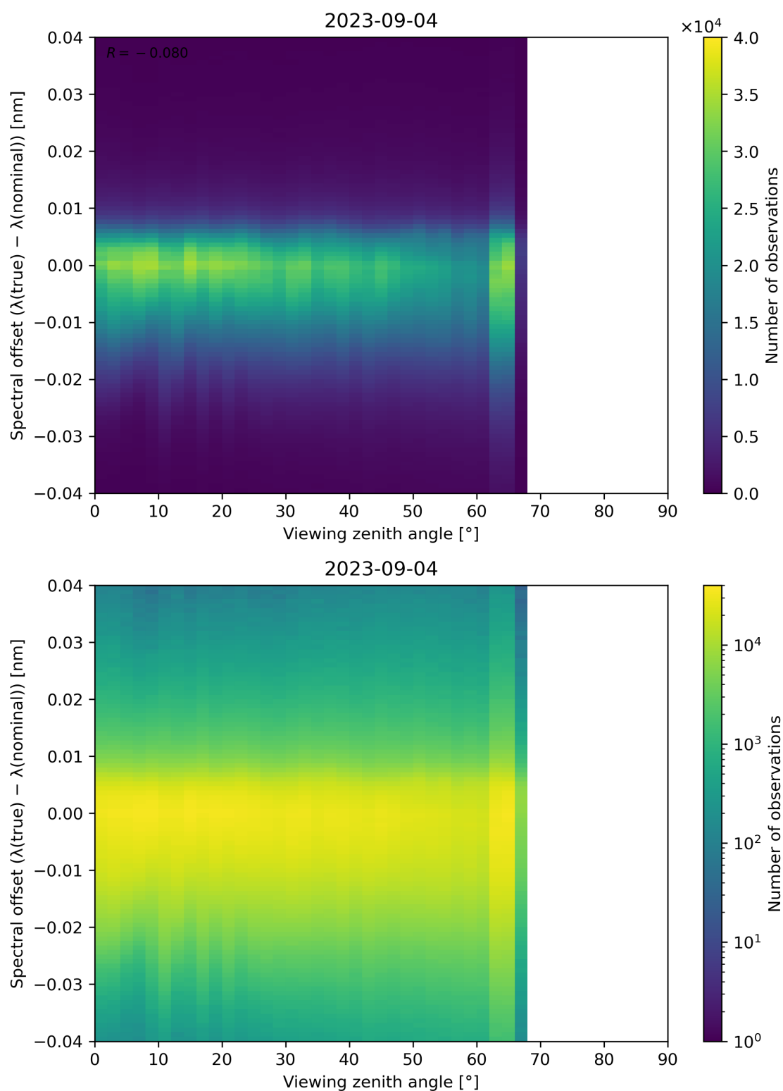
Figure 140: Scatter density plot of “Viewing zenith angle” against “Spectral offset ( \lambda(\text{true}) - \lambda(\text{nominal}) )” for 2023-09-04 to 2023-09-05.
