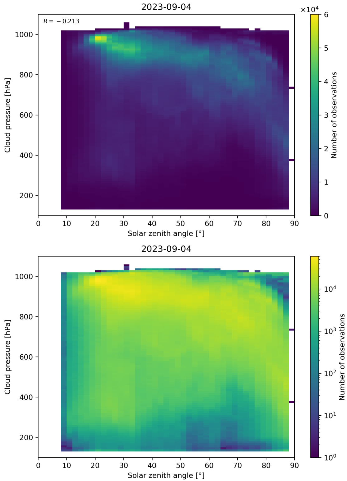
Figure 122: Scatter density plot of “Solar zenith angle” against “Cloud pressure” for 2023-09-04 to 2023-09-05.
