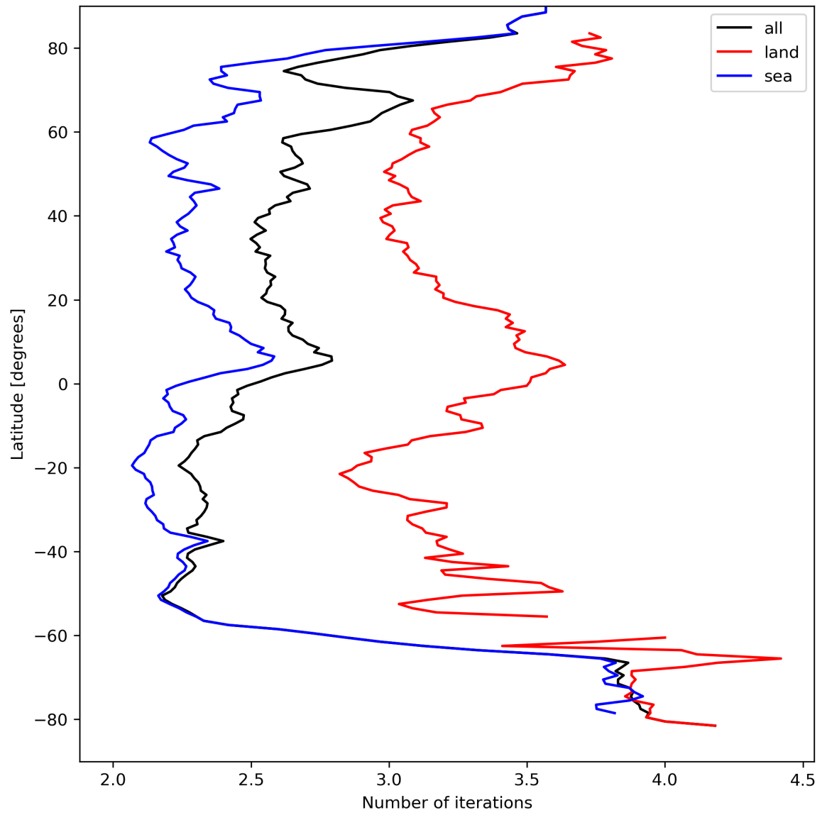
Figure 22: Zonal average of “Number of iterations” for 2023-09-04 to 2023-09-05.
