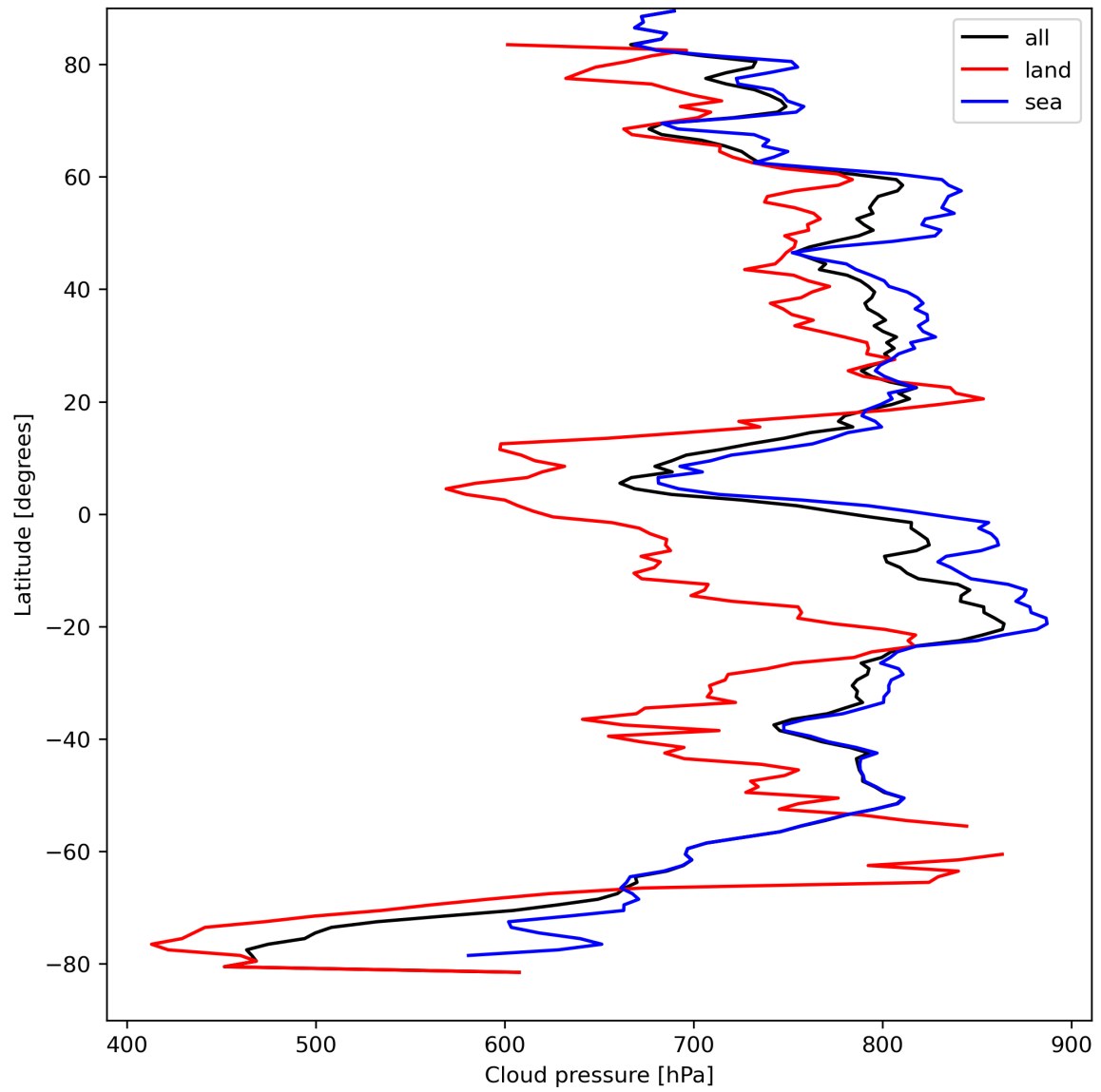
Figure 13: Zonal average of “Cloud pressure” for 2023-09-04 to 2023-09-05.
