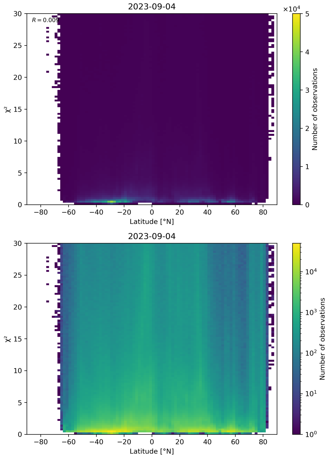
Figure 97: Scatter density plot of “Latitude” against “ \chi^2 ” for 2023-09-04 to 2023-09-05.
