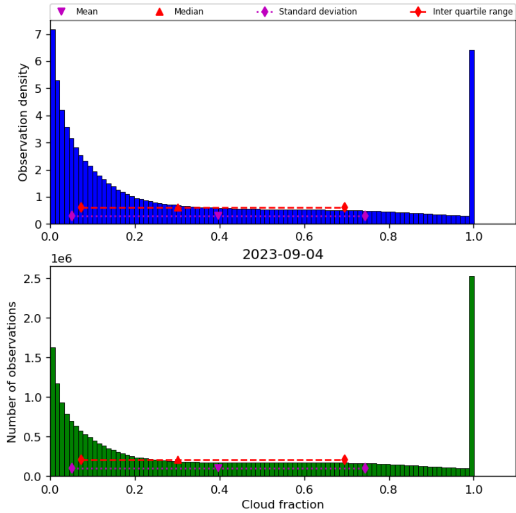
Figure 32: Histogram of “Cloud fraction” for 2023-09-04 to 2023-09-05
