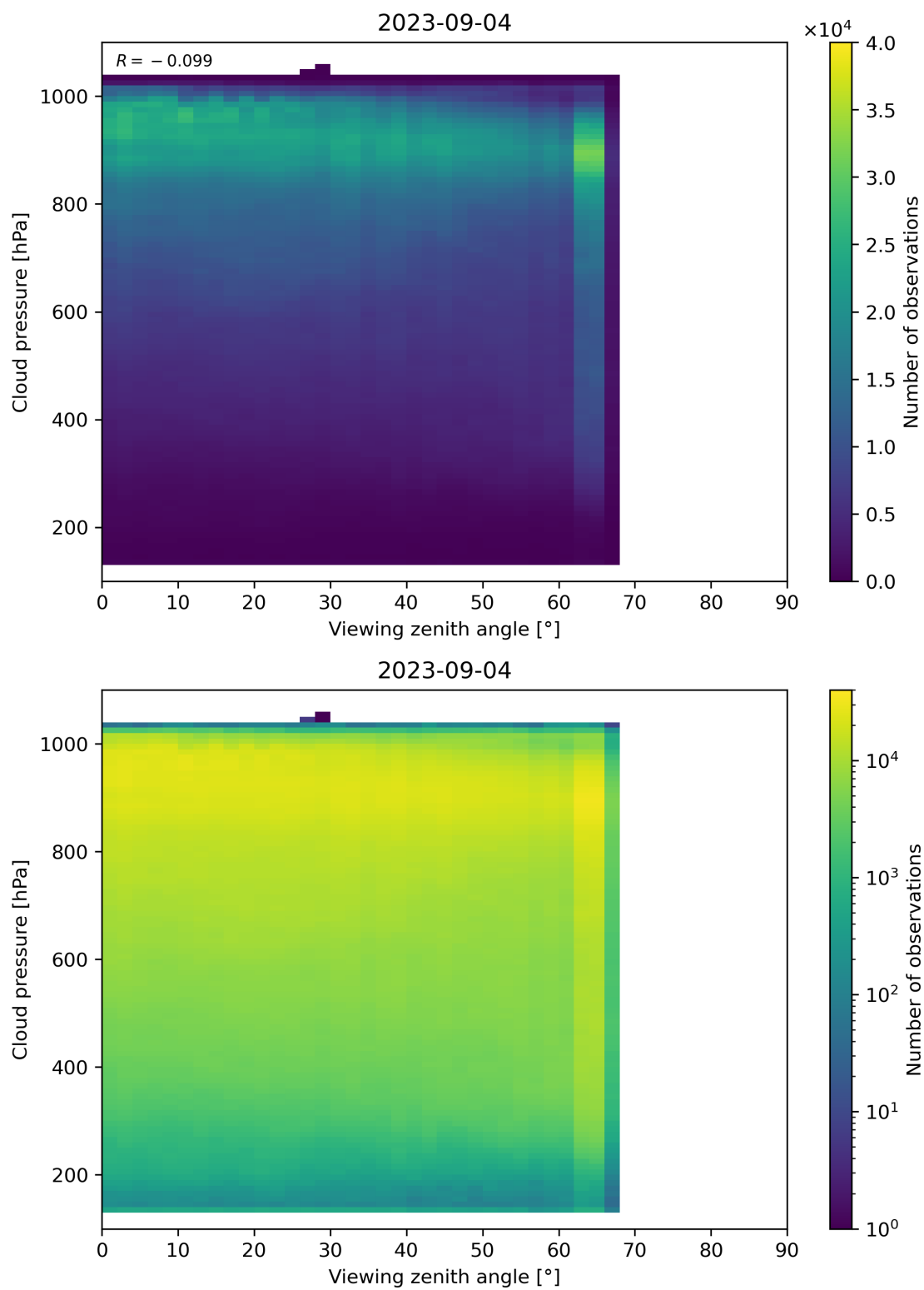
Figure 133: Scatter density plot of “Viewing zenith angle” against “Cloud pressure” for 2023-09-04 to 2023-09-05.
