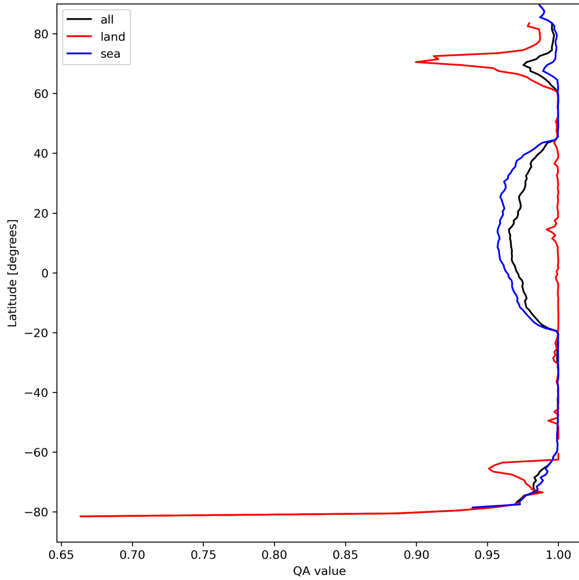
Figure 12: Zonal average of “QA value” for 2023-09-04 to 2023-09-05.
