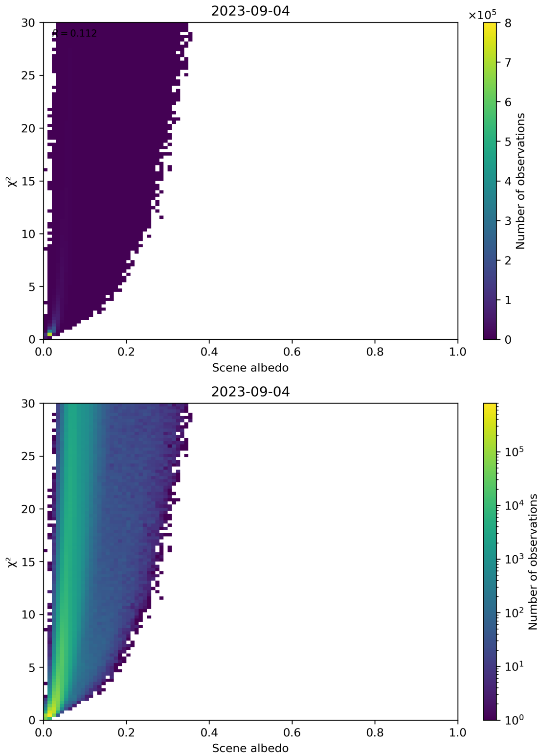
Figure 112: Scatter density plot of “Scene albedo” against “ \chi^2 ” for 2023-09-04 to 2023-09-05.
