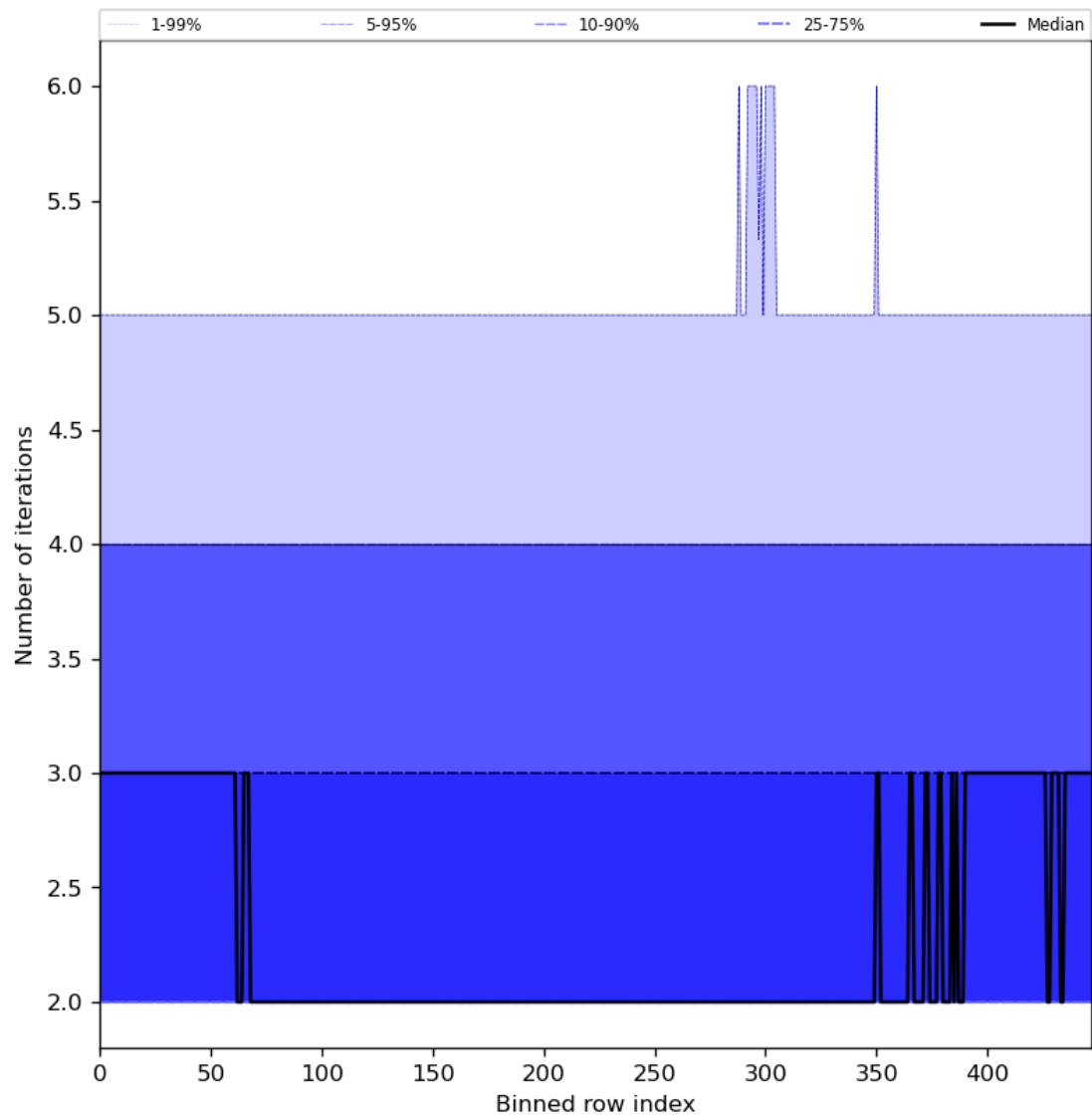
Figure 56: Along track statistics of “Number of iterations” for 2023-09-04 to 2023-09-05
