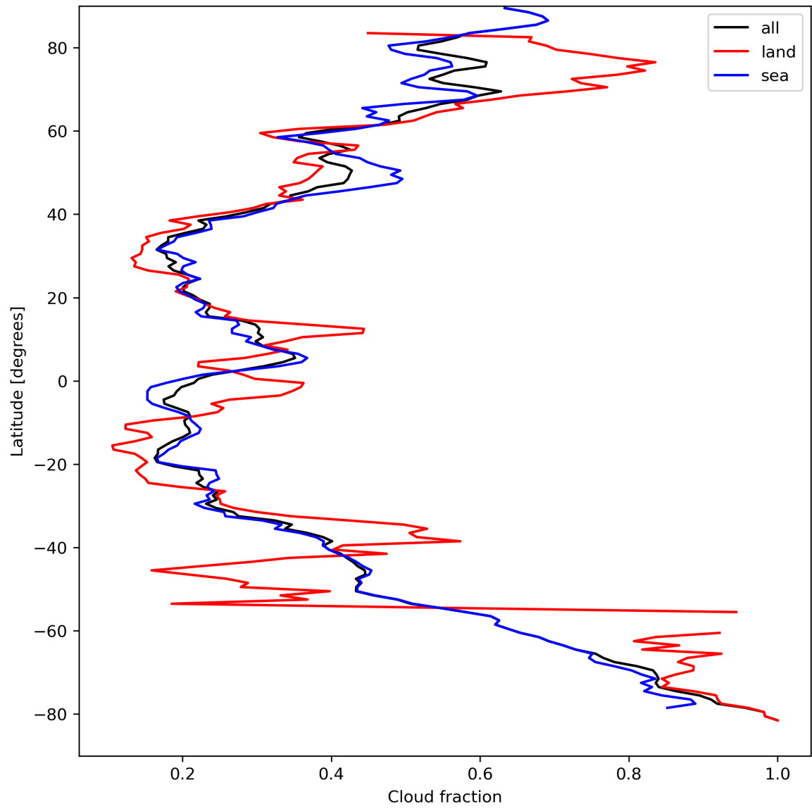
Figure 15: Zonal average of “Cloud fraction” for 2023-09-04 to 2023-09-05.
