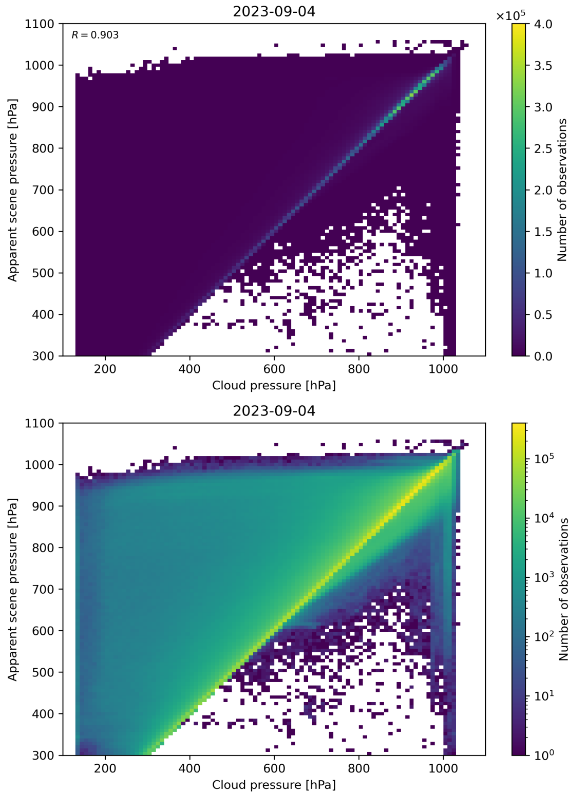
Figure 84: Scatter density plot of “Cloud pressure” against “Apparent scene pressure” for 2023-09-04 to 2023-09-05.
