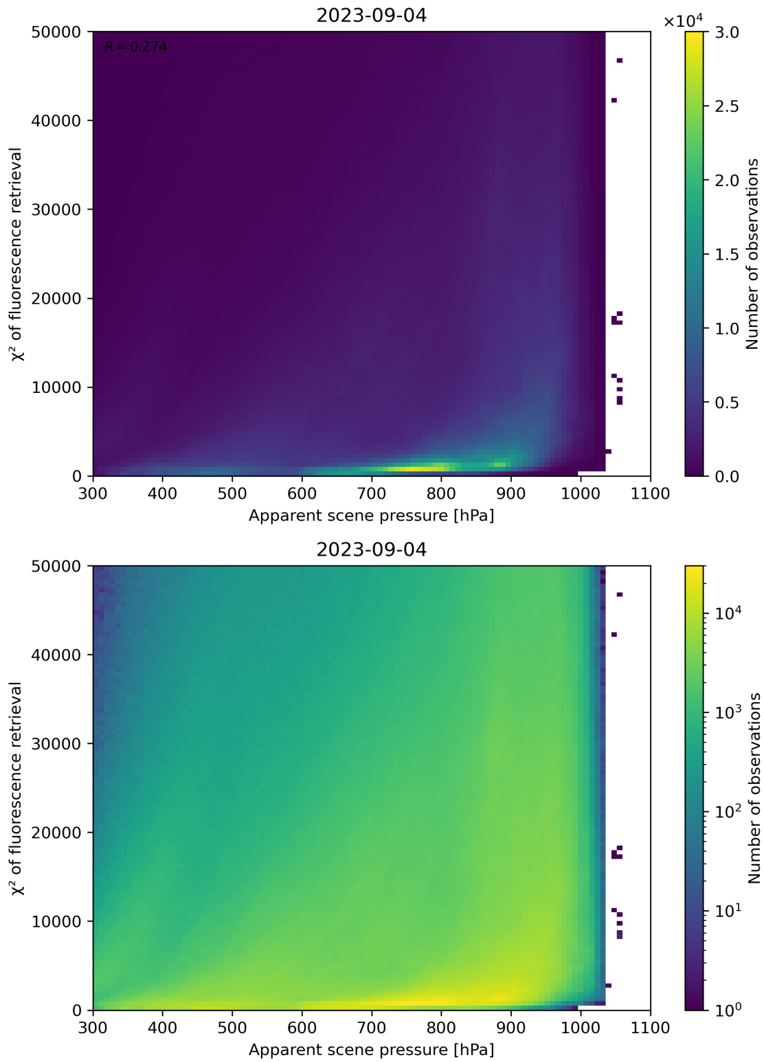
Figure 64: Scatter density plot of “Apparent scene pressure” against “ \chi^2 of fluorescence retrieval” for 2023-09-04 to 2023-09-05.
