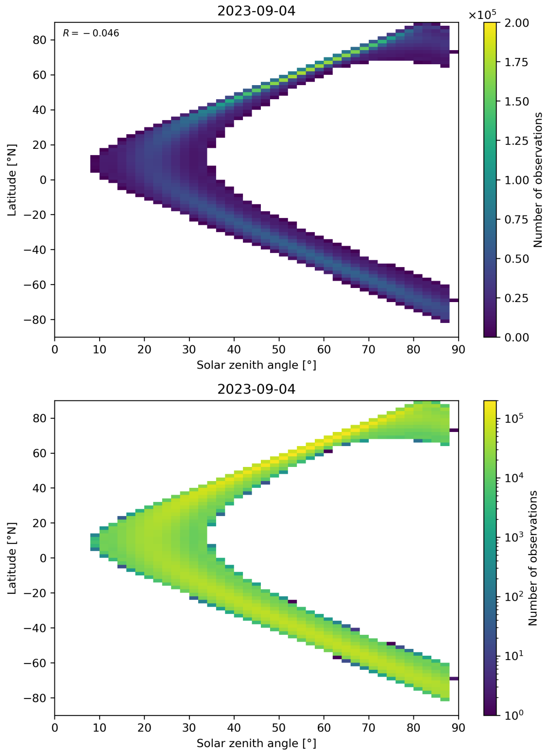
Figure 124: Scatter density plot of “Solar zenith angle” against “Latitude” for 2023-09-04 to 2023-09-05.
