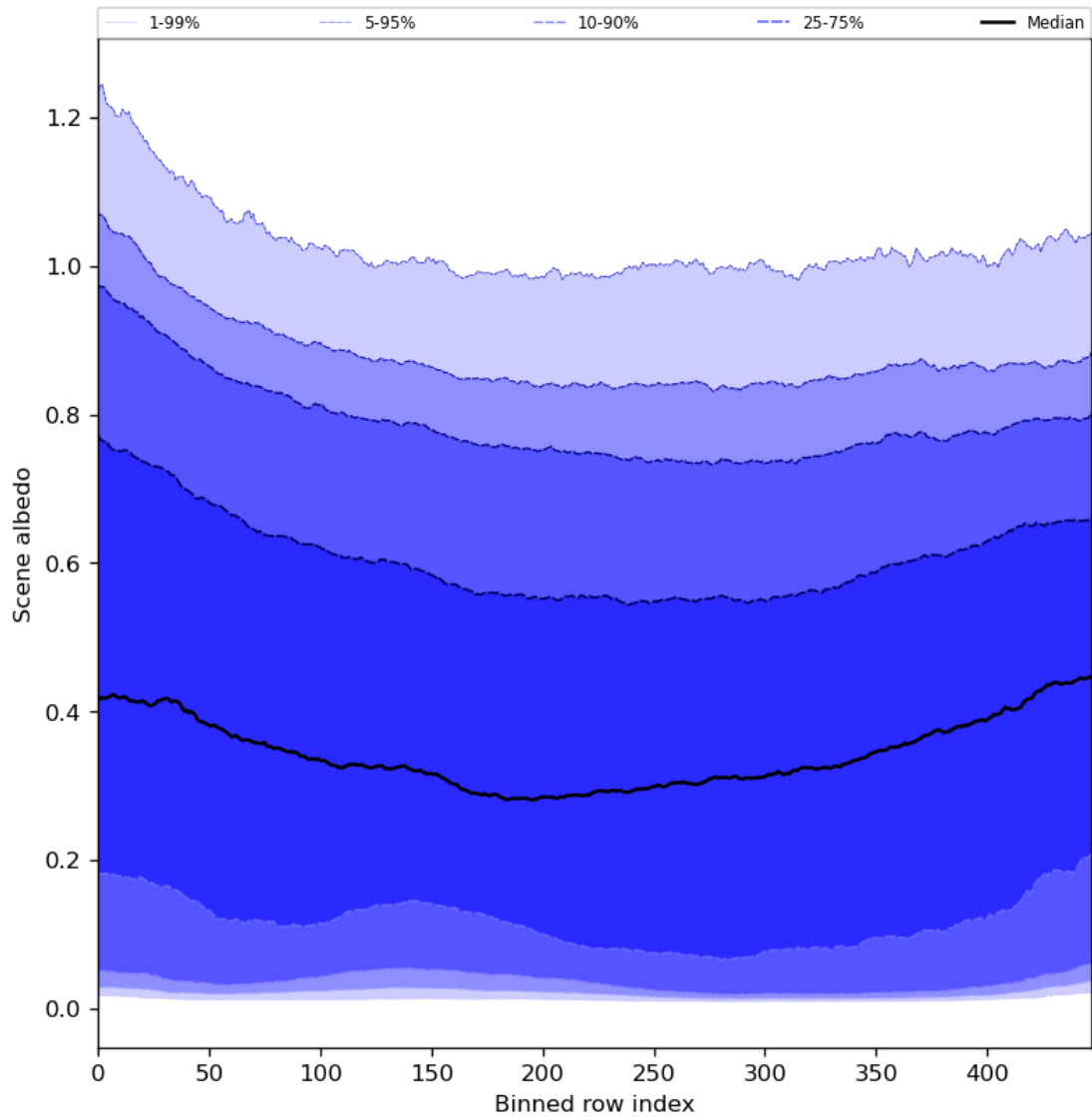
Figure 51: Along track statistics of “Scene albedo” for 2023-09-04 to 2023-09-05
