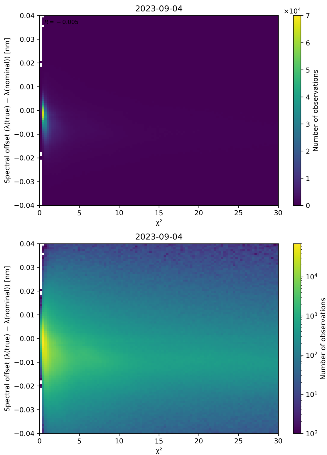
Figure 75: Scatter density plot of “ \chi^2 ” against “Spectral offset ( \lambda(\text{true}) - \lambda(\text{nominal}) )” for 2023-09-04 to 2023-09-05.
