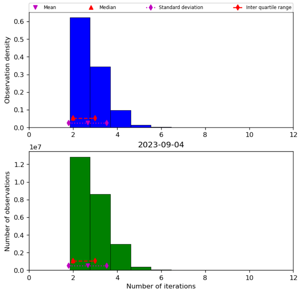
Figure 39: Histogram of “Number of iterations” for 2023-09-04 to 2023-09-05
