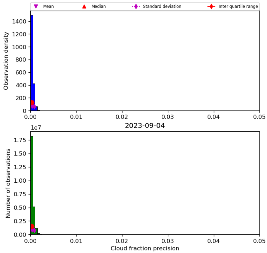
Figure 33: Histogram of “Cloud fraction precision” for 2023-09-04 to 2023-09-05
