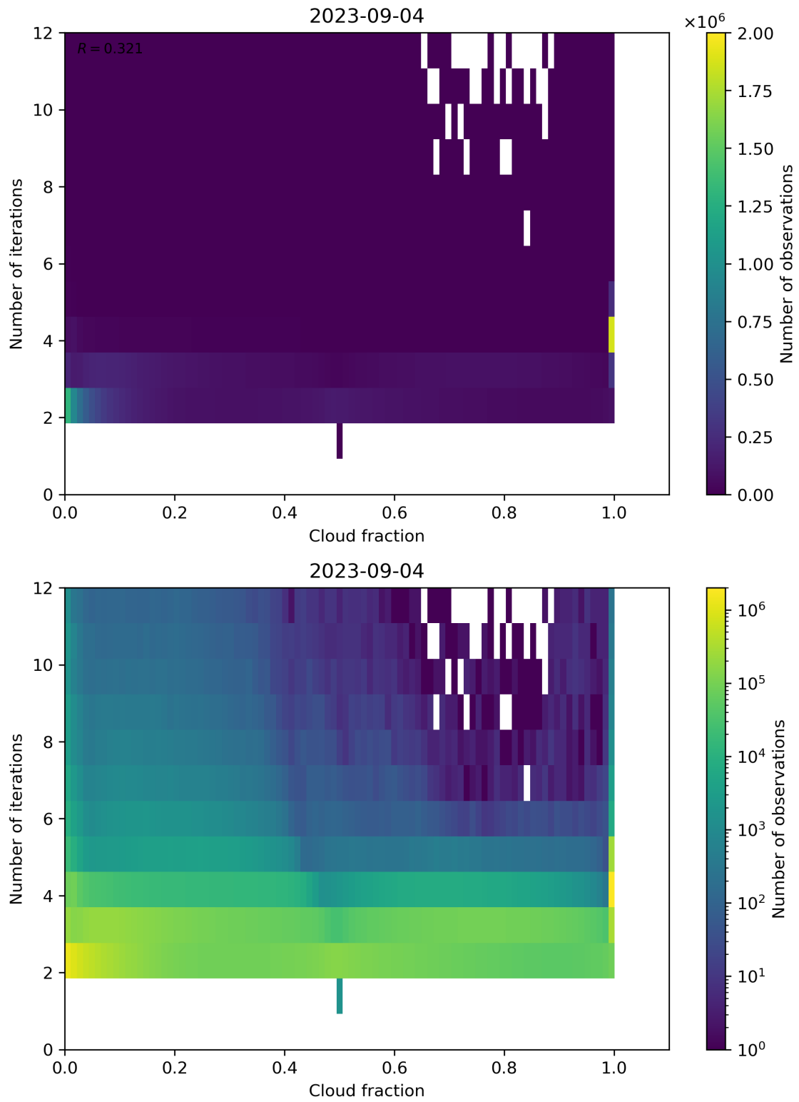
Figure 80: Scatter density plot of “Cloud fraction” against “Number of iterations” for 2023-09-04 to 2023-09-05.
