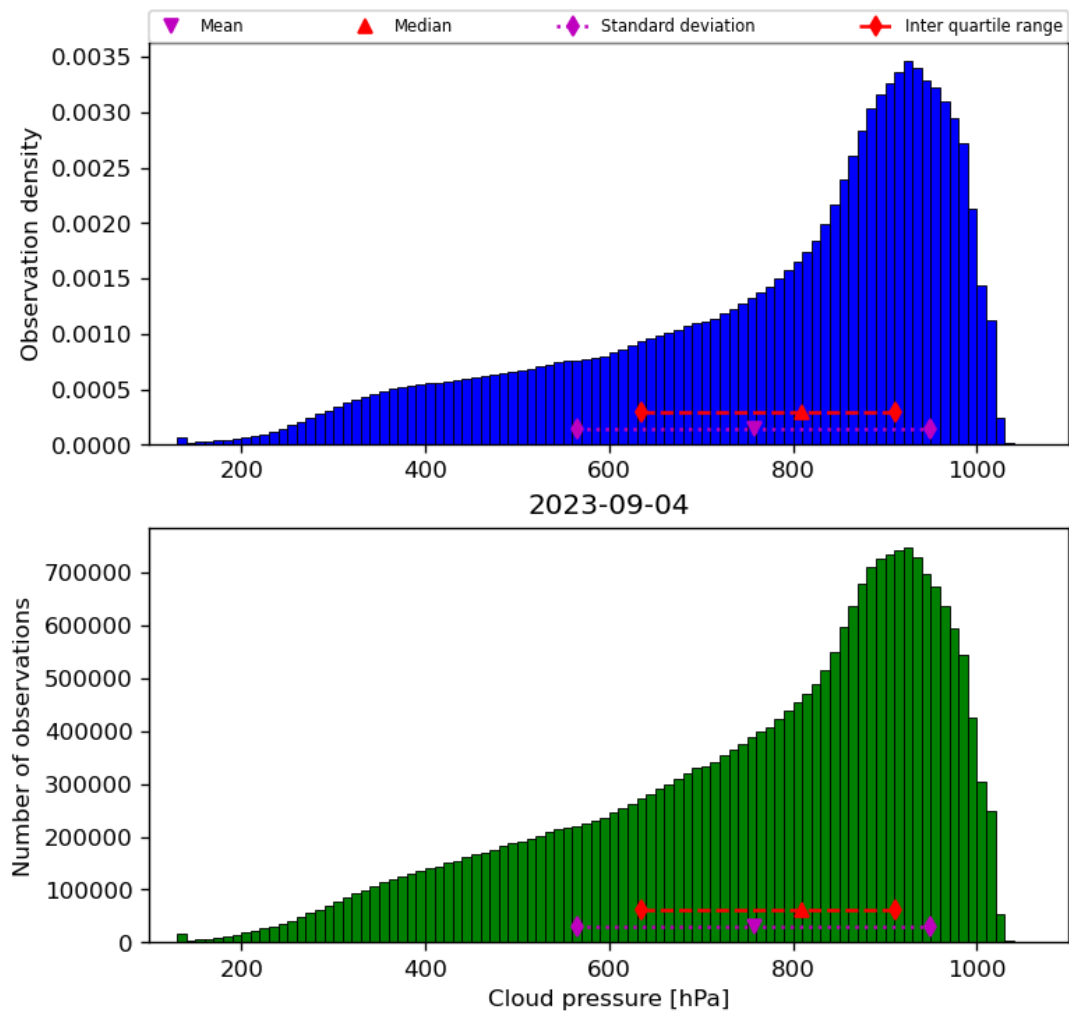
Figure 30: Histogram of “Cloud pressure” for 2023-09-04 to 2023-09-05
