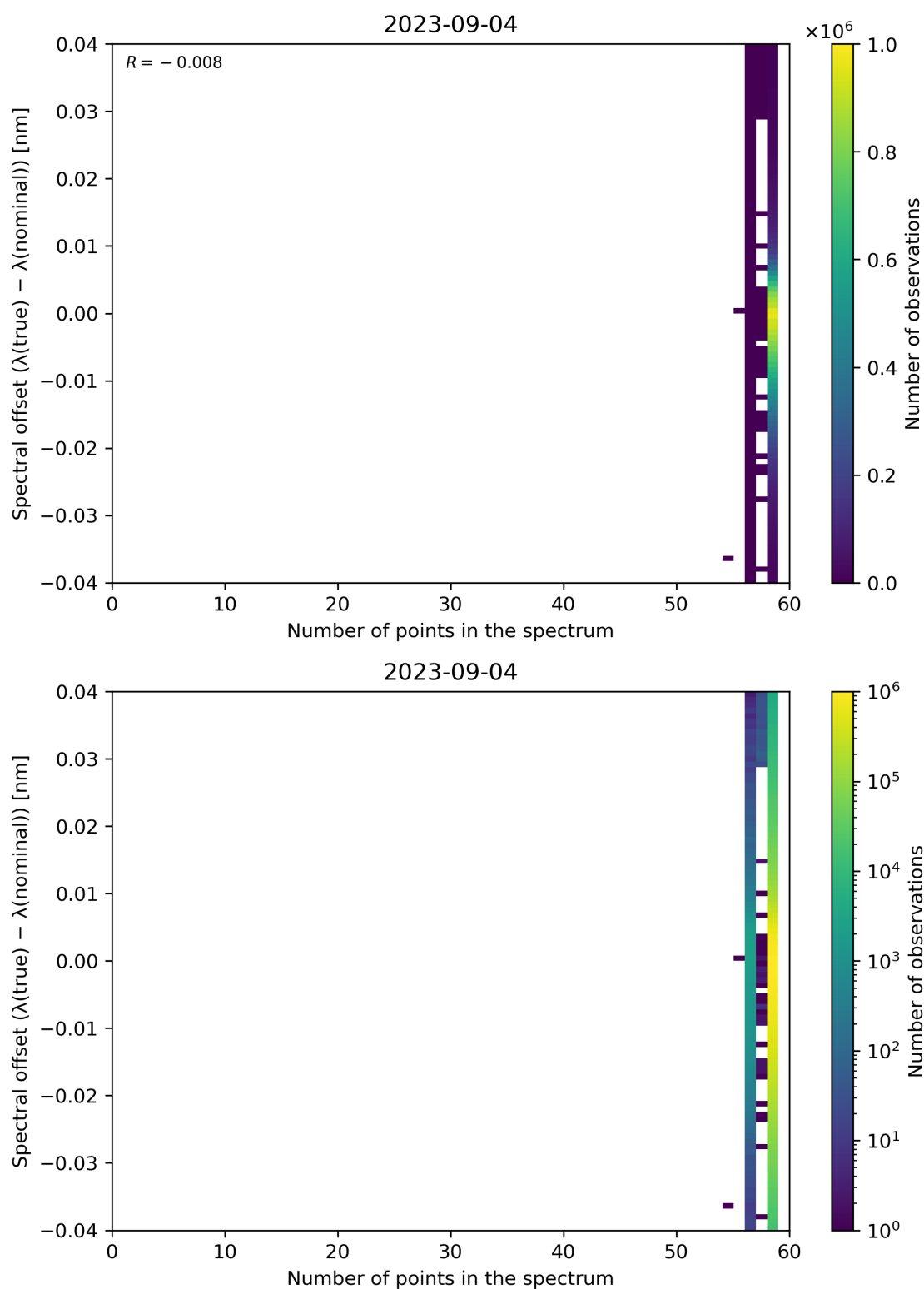
Figure 110: Scatter density plot of “Number of points in the spectrum” against “Spectral offset ( \lambda(\text{true}) - \lambda(\text{nominal}) )” for 2023-09-04 to 2023-09-05.
