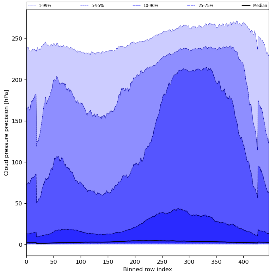
Figure 48: Along track statistics of “Cloud pressure precision” for 2023-09-04 to 2023-09-05
