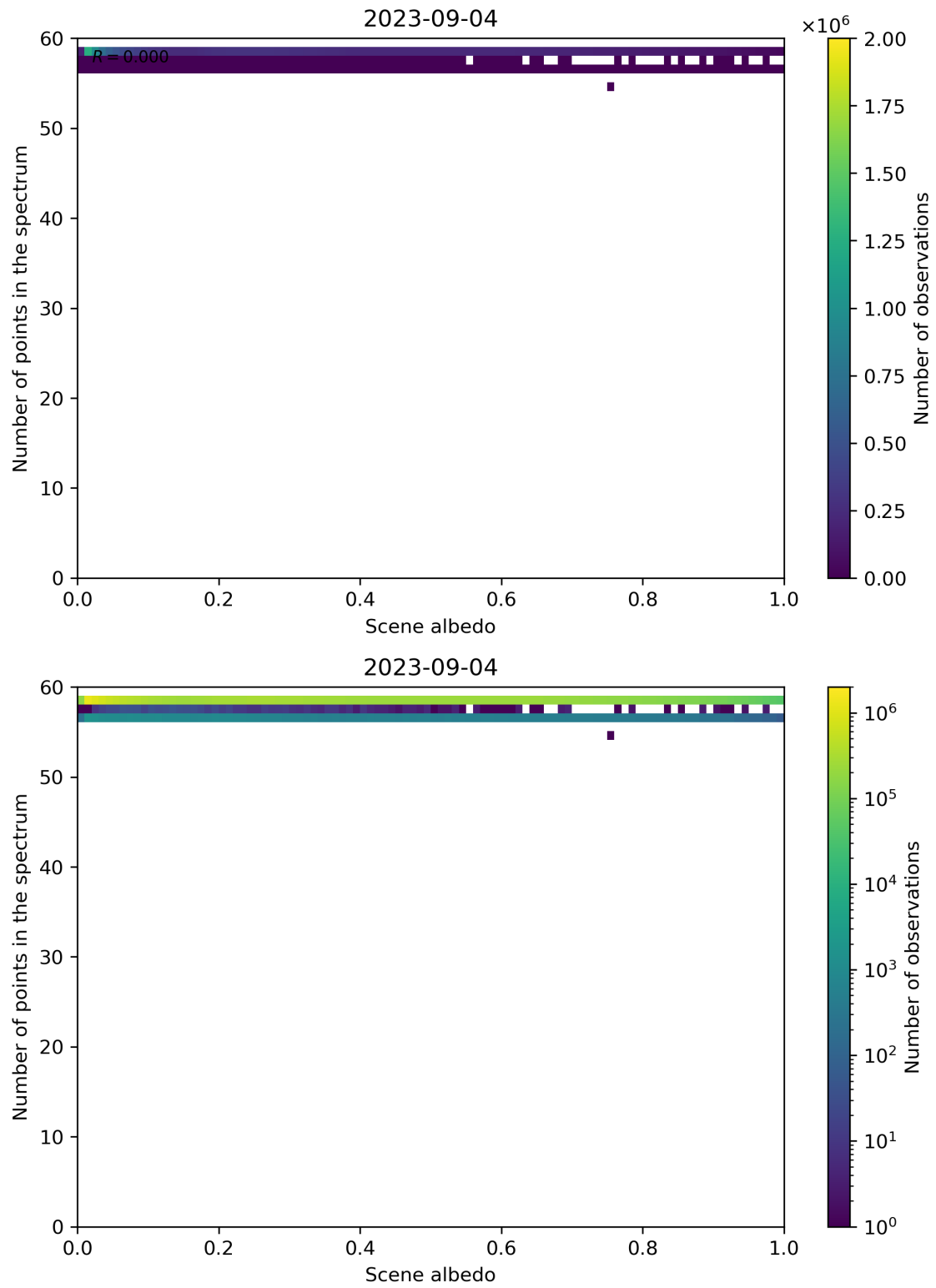
Figure 116: Scatter density plot of “Scene albedo” against “Number of points in the spectrum” for 2023-09-04 to 2023-09-05.
