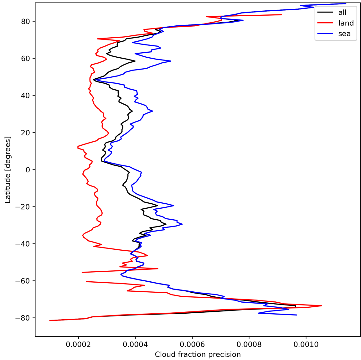
Figure 16: Zonal average of “Cloud fraction precision” for 2023-09-04 to 2023-09-05.
