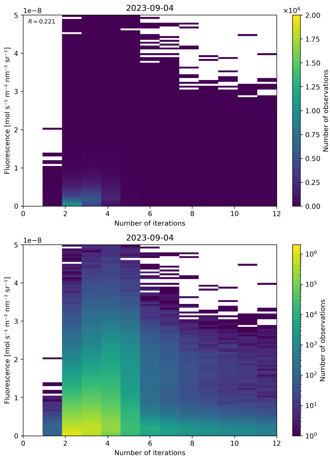
Figure 107: Scatter density plot of “Number of iterations” against “Fluorescence” for 2023-09-04 to 2023-09-05.
