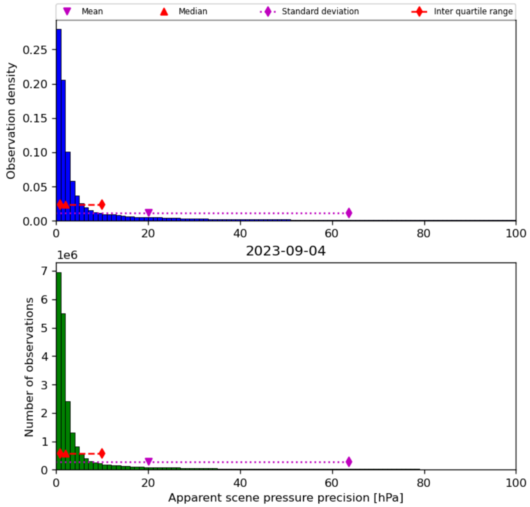
Figure 37: Histogram of “Apparent scene pressure precision” for 2023-09-04 to 2023-09-05
