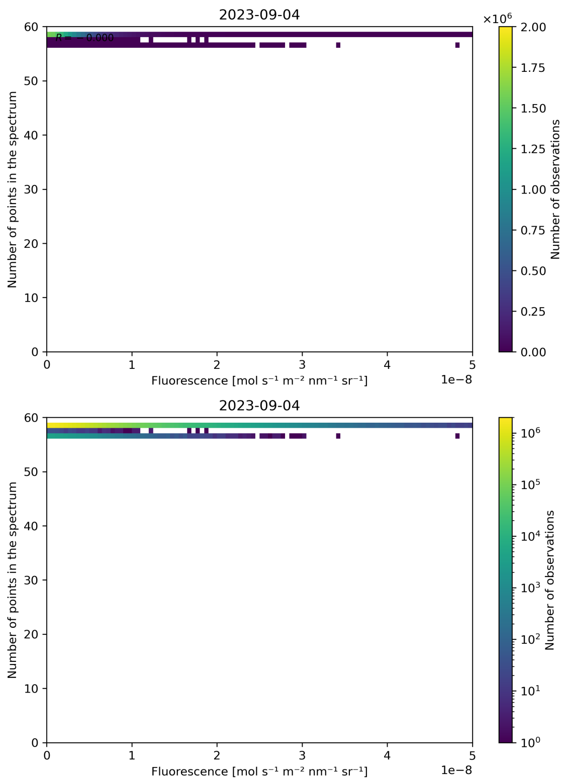
Figure 94: Scatter density plot of “Fluorescence” against “Number of points in the spectrum” for 2023-09-04 to 2023-09-05.
