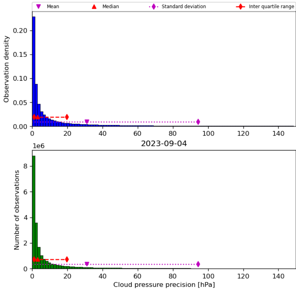
Figure 31: Histogram of “Cloud pressure precision” for 2023-09-04 to 2023-09-05
