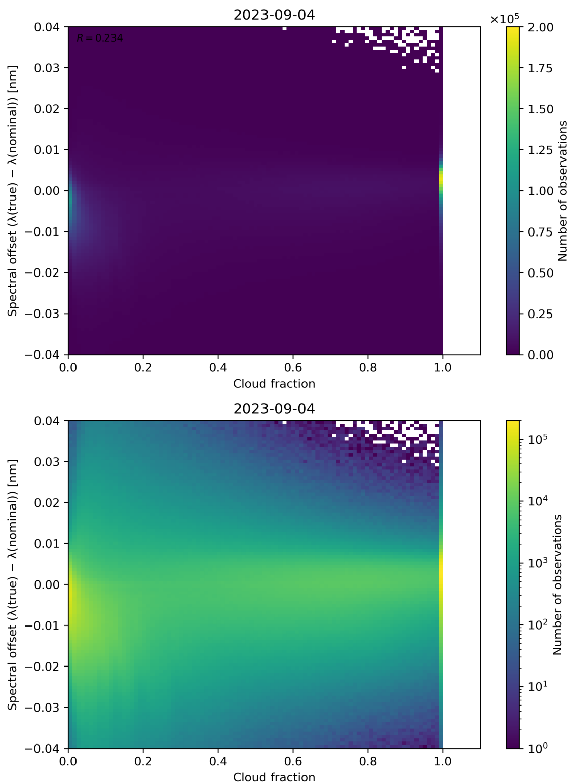
Figure 83: Scatter density plot of “Cloud fraction” against “Spectral offset ( \lambda(\text{true}) - \lambda(\text{nominal}) )” for 2023-09-04 to 2023-09-05.
