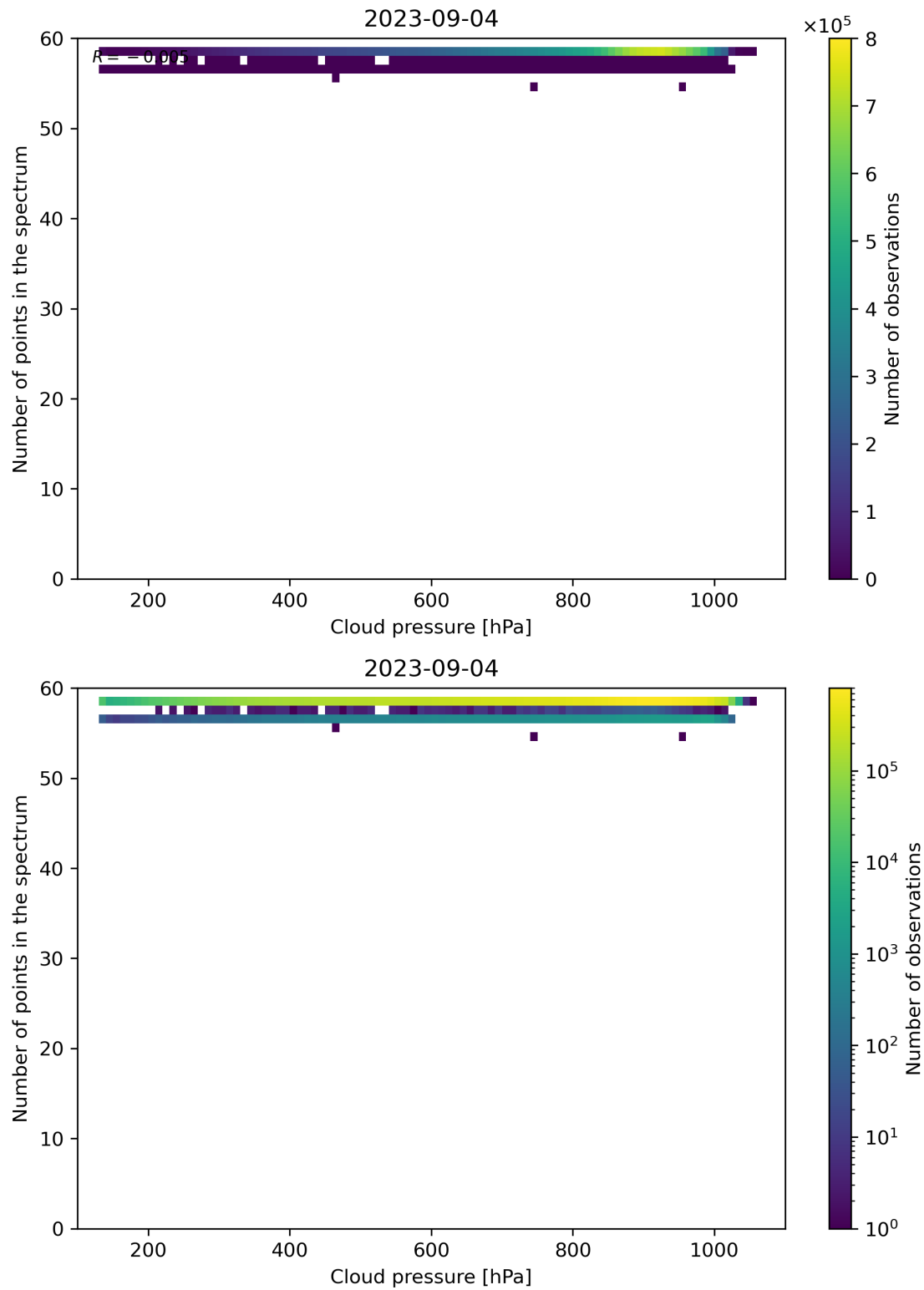
Figure 90: Scatter density plot of “Cloud pressure” against “Number of points in the spectrum” for 2023-09-04 to 2023-09-05.
