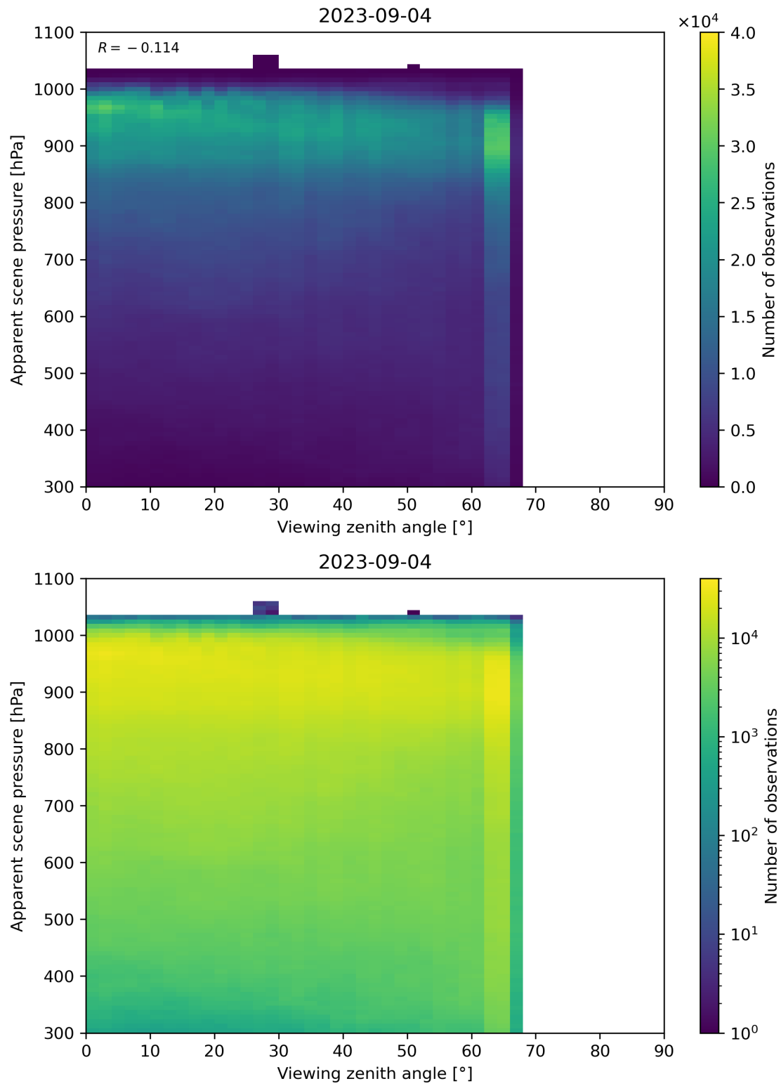
Figure 129: Scatter density plot of “Viewing zenith angle” against “Apparent scene pressure” for 2023-09-04 to 2023-09-05.
