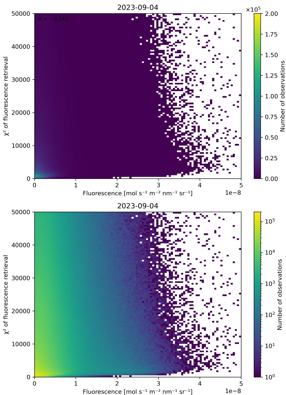
Figure 93: Scatter density plot of “Fluorescence” against “ \chi^2 of fluorescence retrieval” for 2023-09-04 to 2023-09-05.
