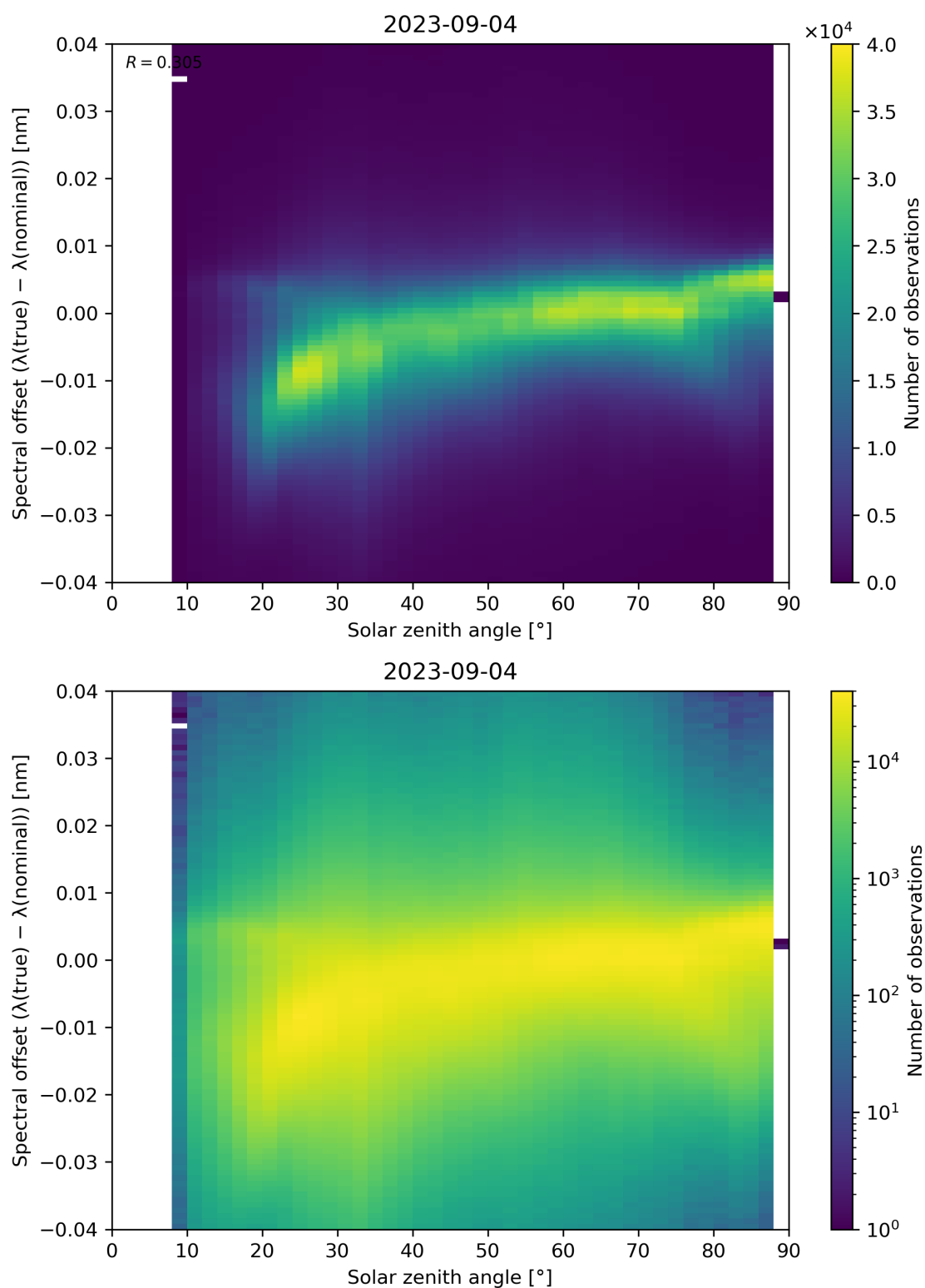
Figure 128: Scatter density plot of “Solar zenith angle” against “Spectral offset ( \lambda(\text{true}) - \lambda(\text{nominal}) )” for 2023-09-04 to 2023-09-05.
