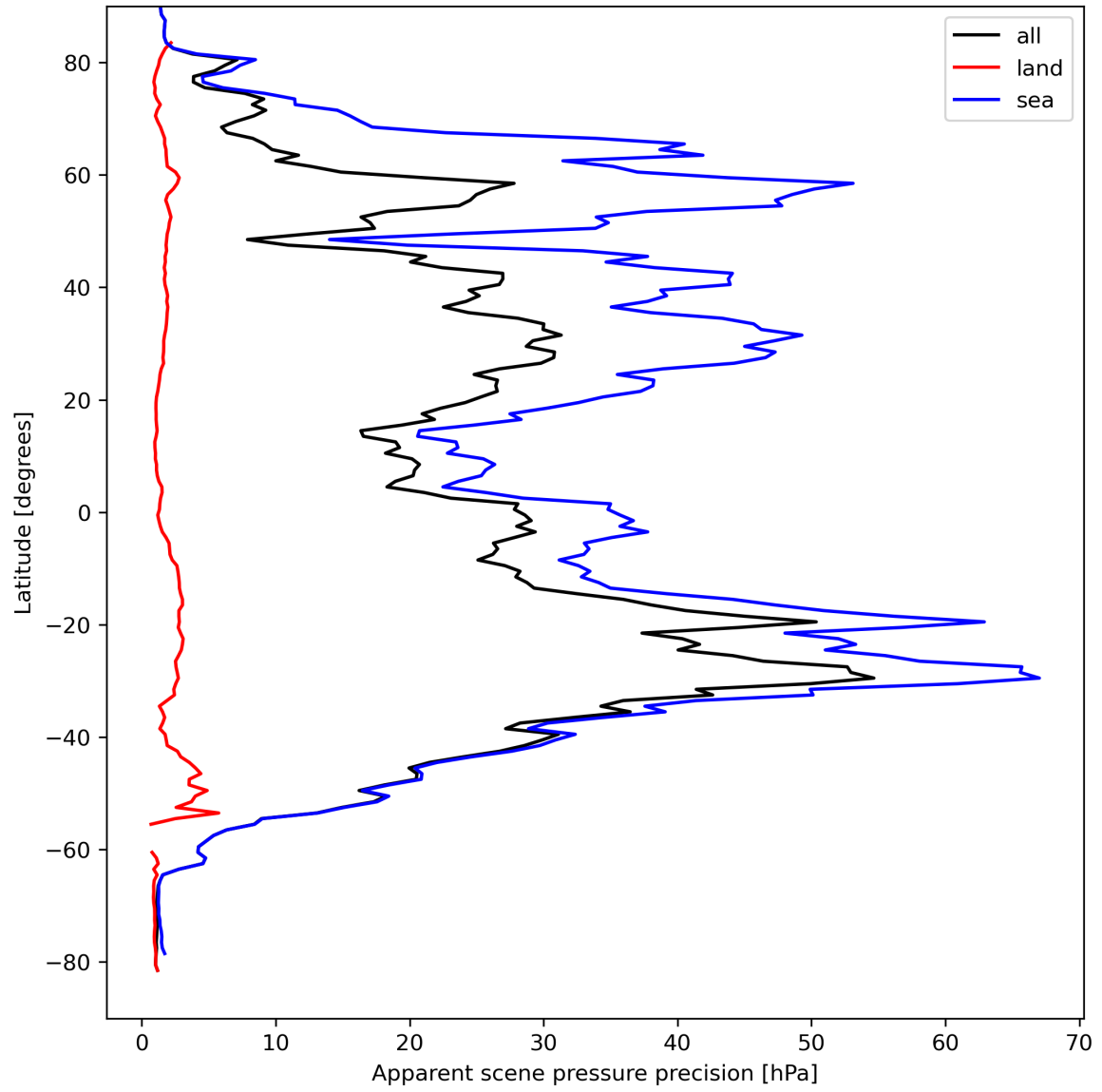
Figure 20: Zonal average of “Apparent scene pressure precision” for 2023-09-04 to 2023-09-05.
