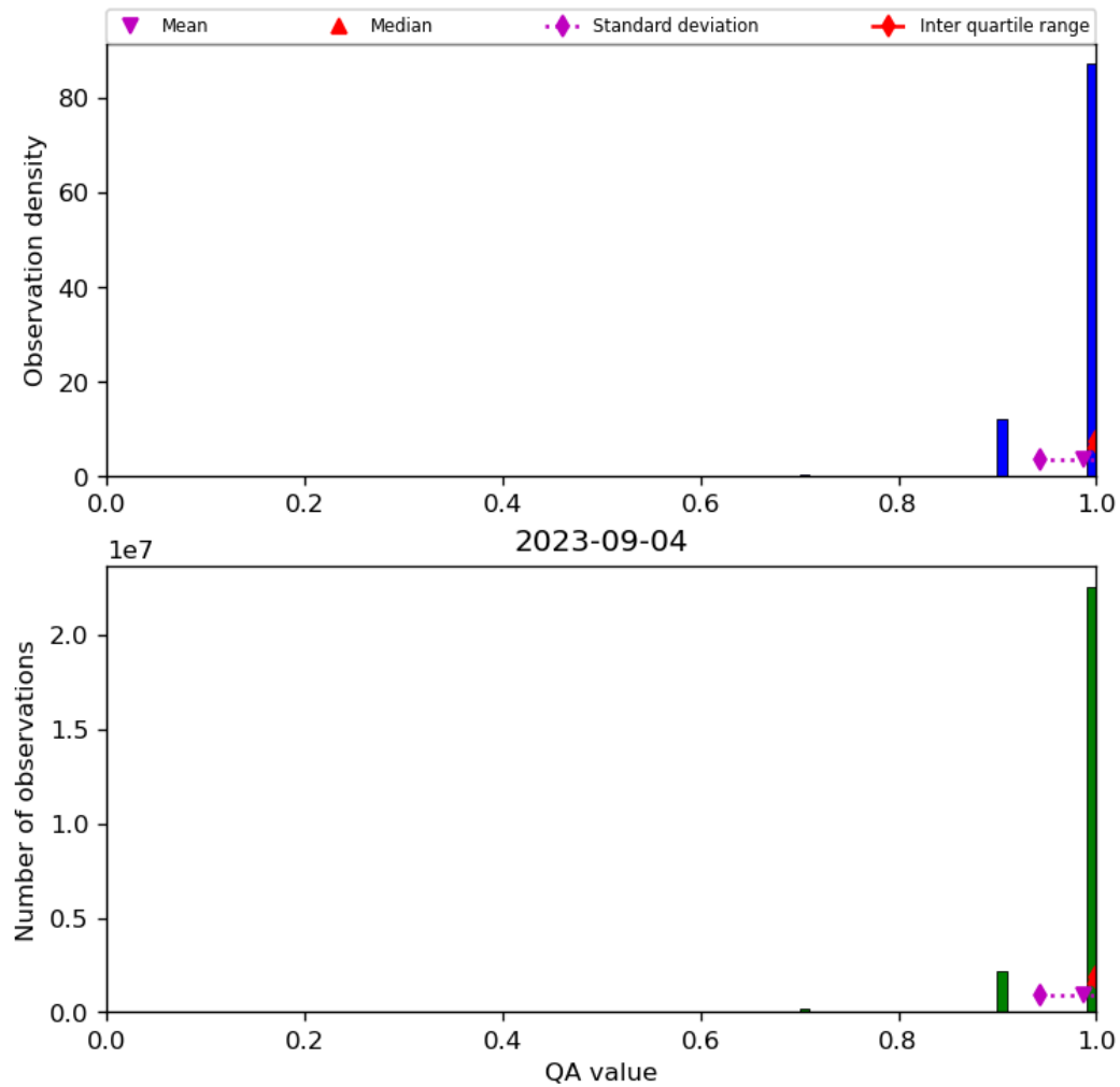
Figure 29: Histogram of “QA value” for 2023-09-04 to 2023-09-05
