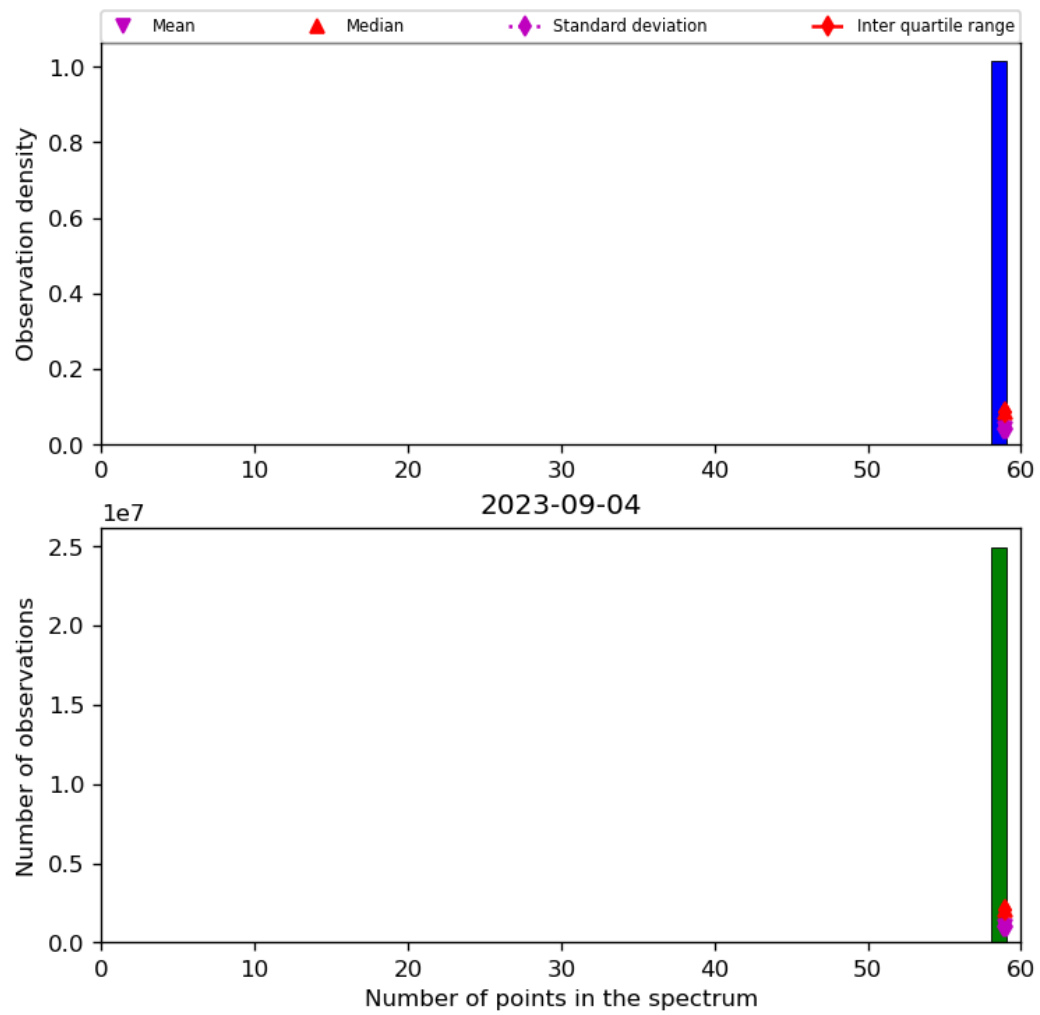
Figure 44: Histogram of “Number of points in the spectrum” for 2023-09-04 to 2023-09-05
