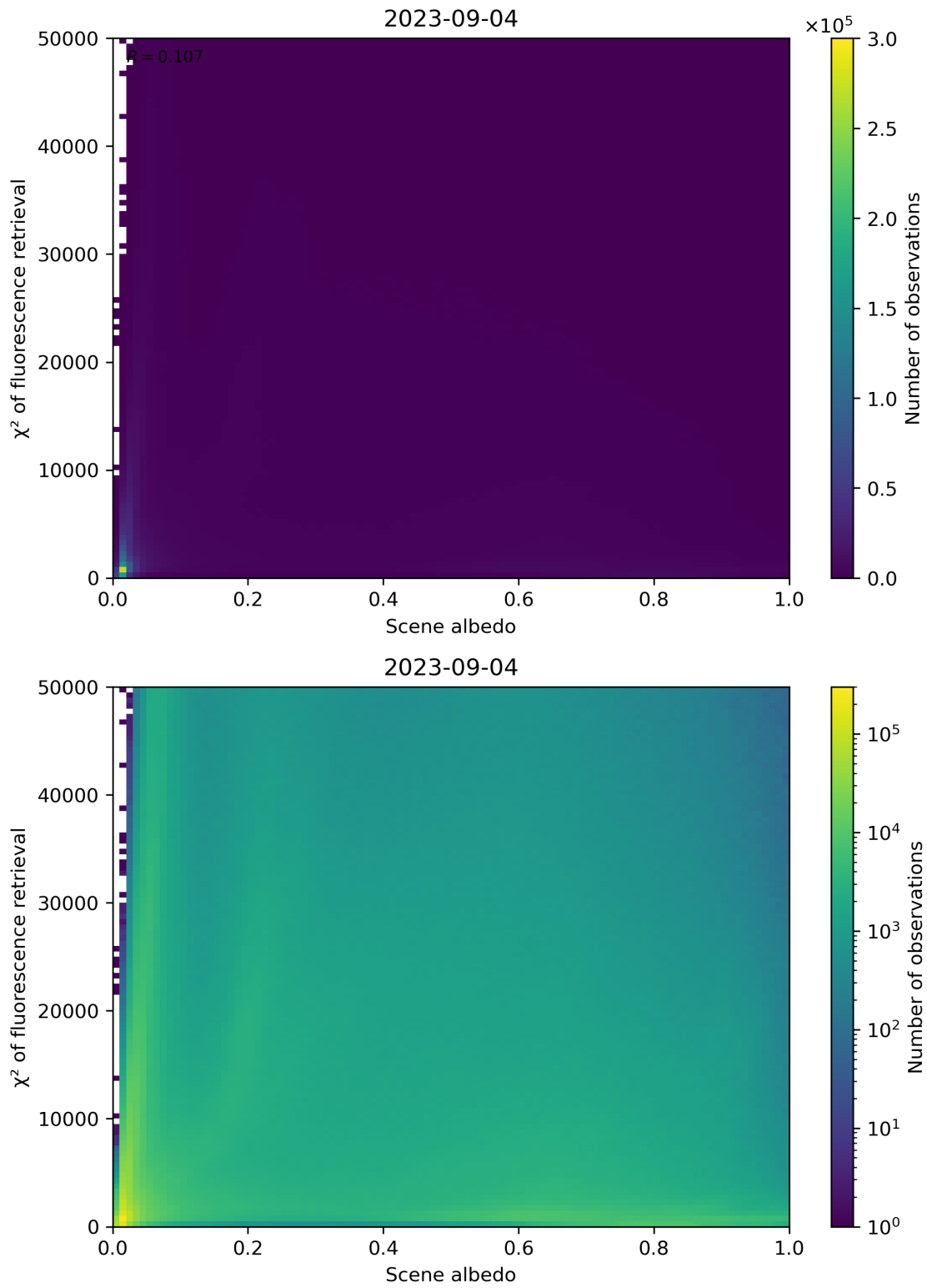
Figure 113: Scatter density plot of “Scene albedo” against “ \chi^2 of fluorescence retrieval” for 2023-09-04 to 2023-09-05.
