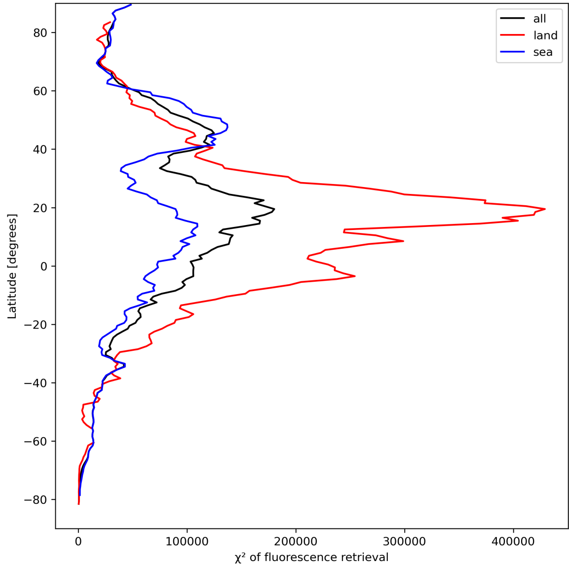
Figure 25: Zonal average of “ \chi^2 of fluorescence retrieval” for 2023-09-04 to 2023-09-05.
