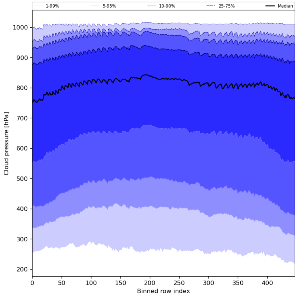
Figure 47: Along track statistics of “Cloud pressure” for 2023-09-04 to 2023-09-05
