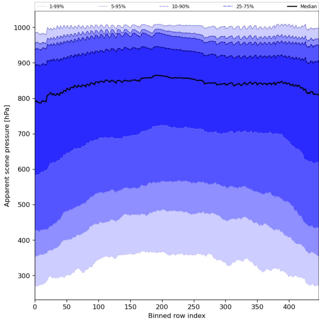
Figure 53: Along track statistics of “Apparent scene pressure” for 2023-09-04 to 2023-09-05
