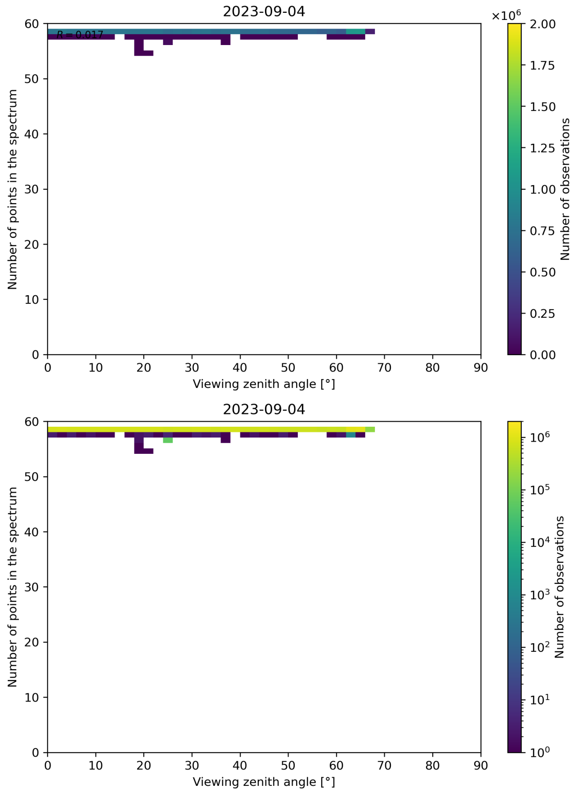
Figure 137: Scatter density plot of “Viewing zenith angle” against “Number of points in the spectrum” for 2023-09-04 to 2023-09-05.
