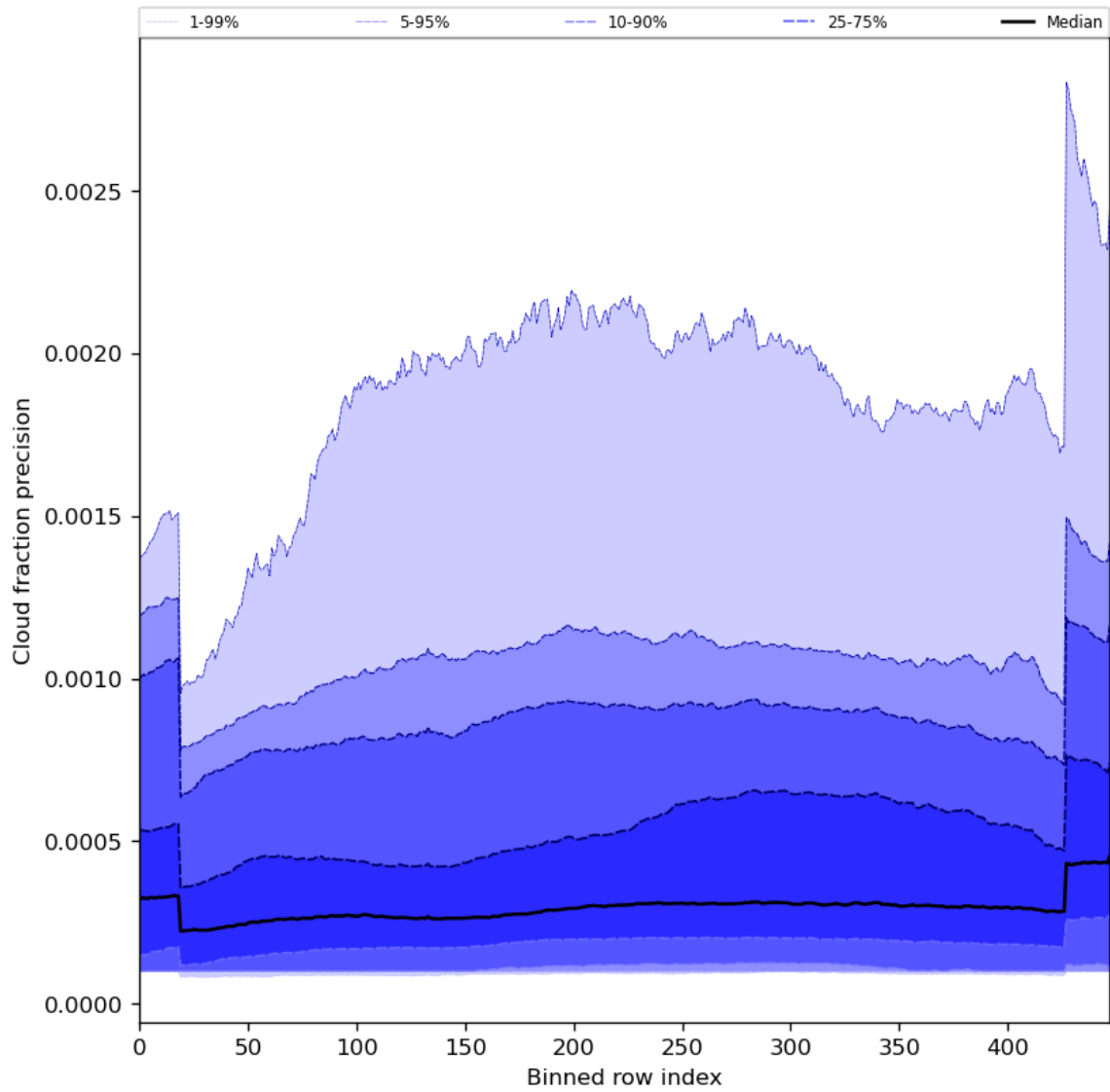
Figure 50: Along track statistics of “Cloud fraction precision” for 2023-09-04 to 2023-09-05
