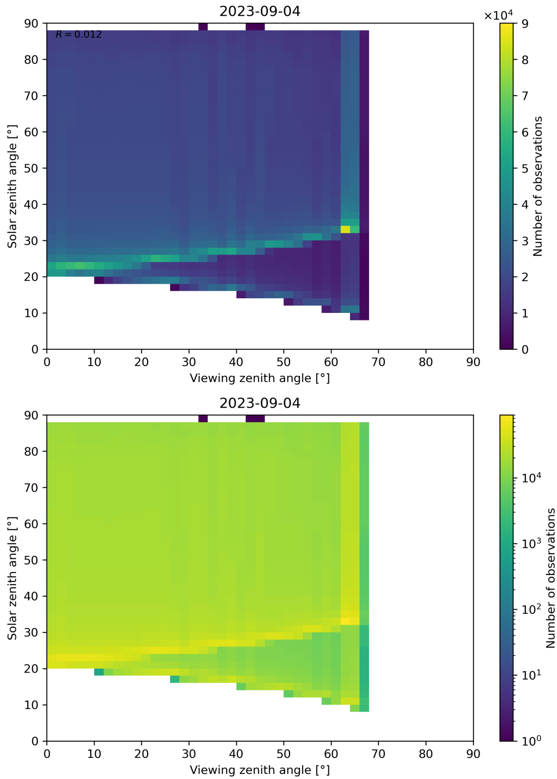
Figure 139: Scatter density plot of “Viewing zenith angle” against “Solar zenith angle” for 2023-09-04 to 2023-09-05.
