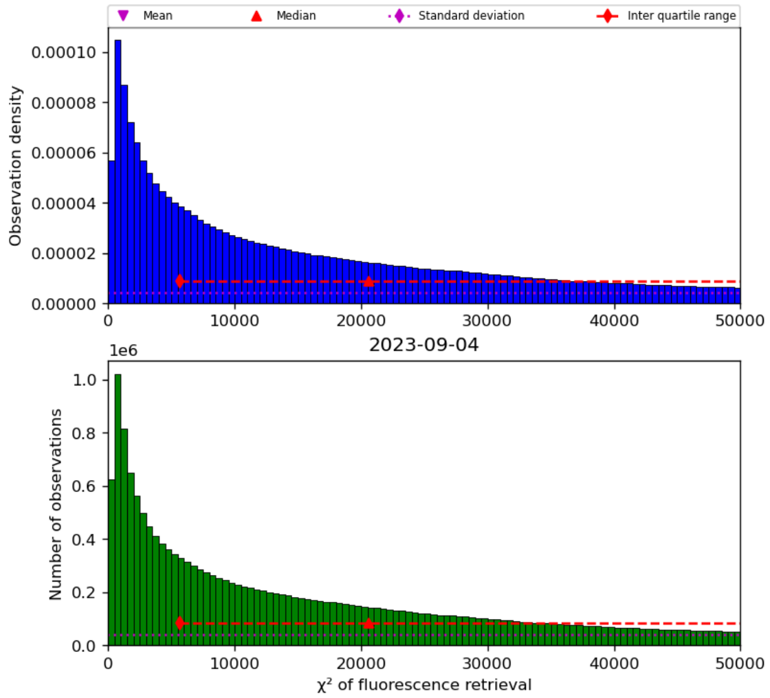
Figure 42: Histogram of “ \chi^2 of fluorescence retrieval” for 2023-09-04 to 2023-09-05
