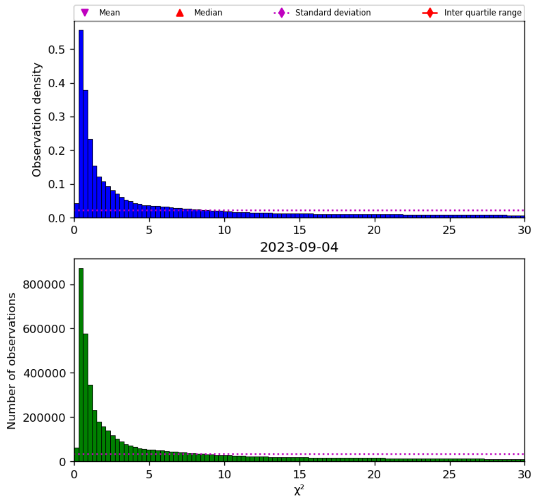
Figure 38: Histogram of " \chi^2 " for 2023-09-04 to 2023-09-05
