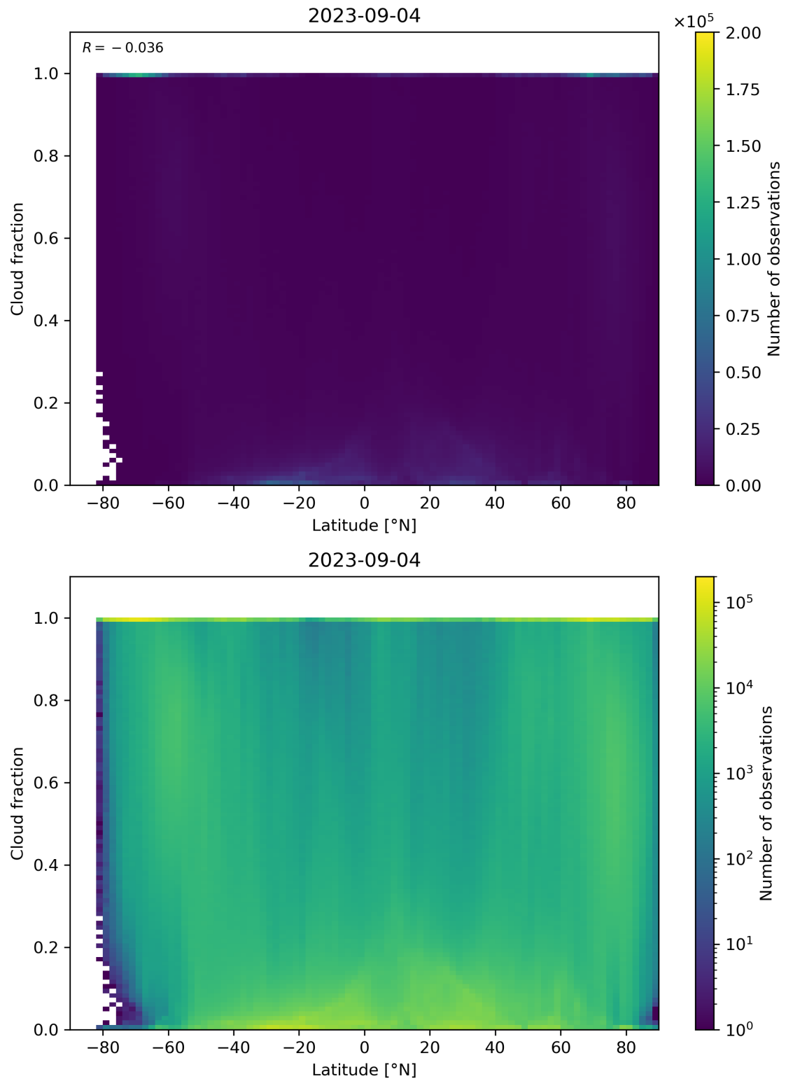
Figure 99: Scatter density plot of “Latitude” against “Cloud fraction” for 2023-09-04 to 2023-09-05.
