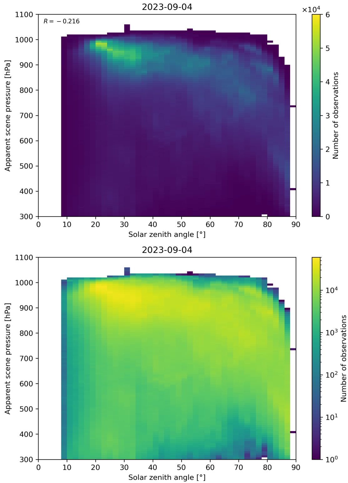
Figure 118: Scatter density plot of “Solar zenith angle” against “Apparent scene pressure” for 2023-09-04 to 2023-09-05.
