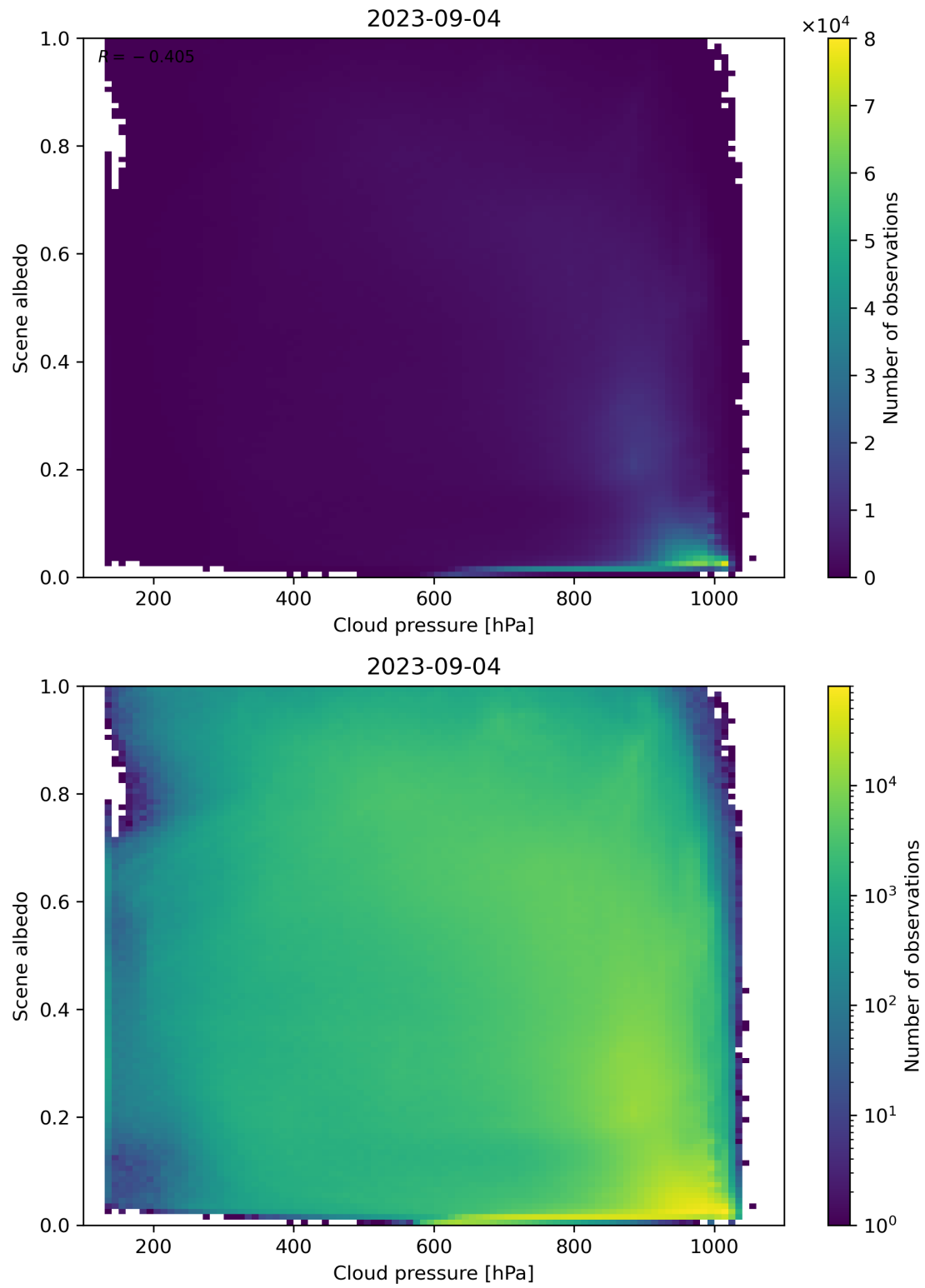
Figure 91: Scatter density plot of “Cloud pressure” against “Scene albedo” for 2023-09-04 to 2023-09-05.
