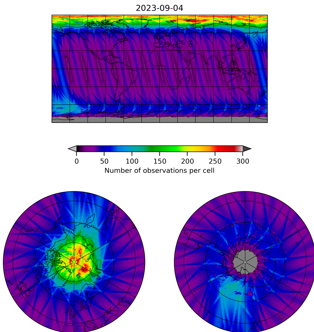
Figure 11: Map of the number of observations for 2023-09-04 to 2023-09-05
