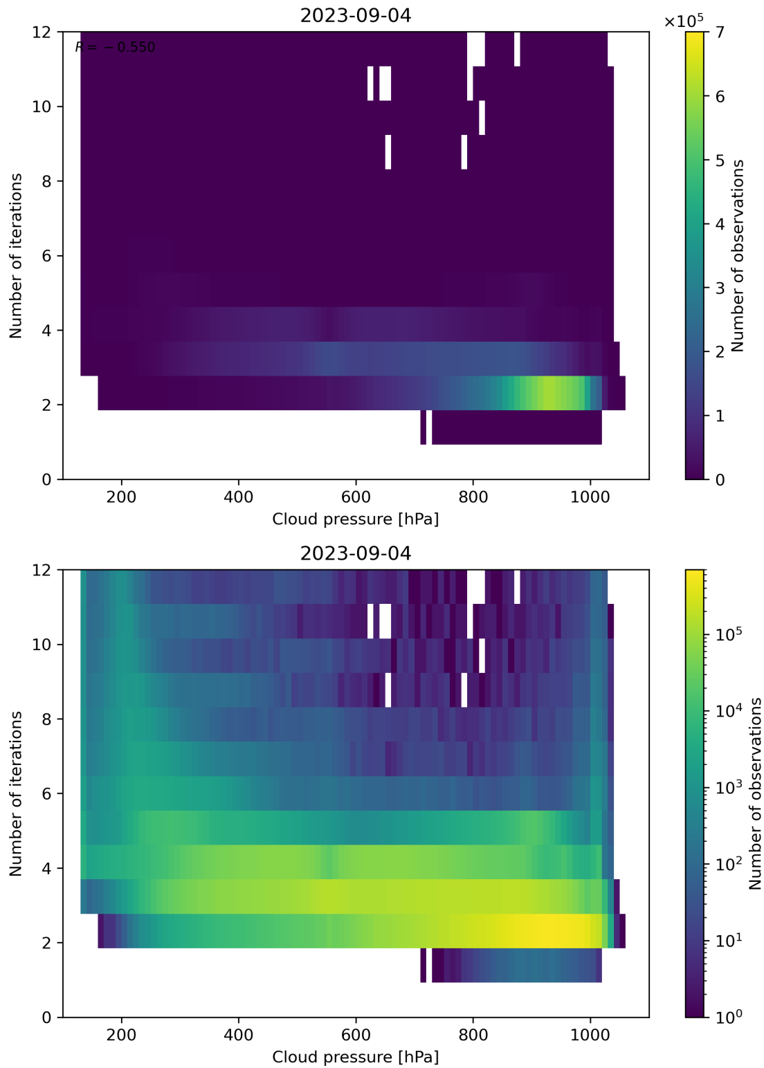
Figure 89: Scatter density plot of “Cloud pressure” against “Number of iterations” for 2023-09-04 to 2023-09-05.
