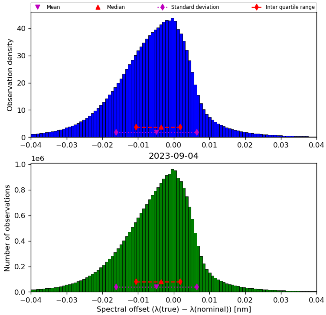
Figure 45: Histogram of “Spectral offset ( \lambda(\text{true}) - \lambda(\text{nominal}) )” for 2023-09-04 to 2023-09-05
