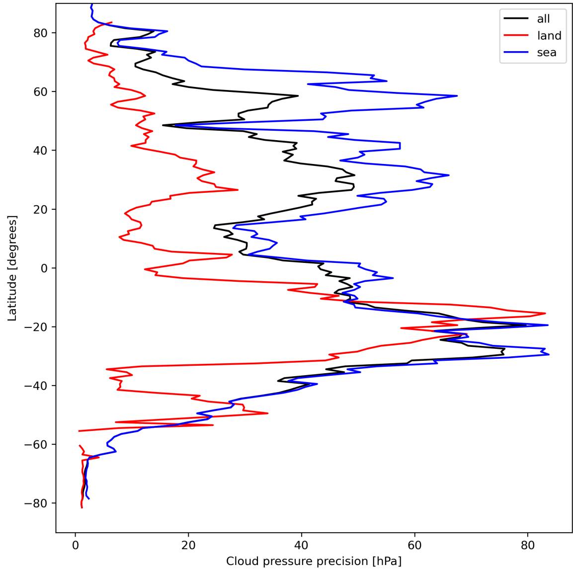
Figure 14: Zonal average of “Cloud pressure precision” for 2023-09-04 to 2023-09-05.
