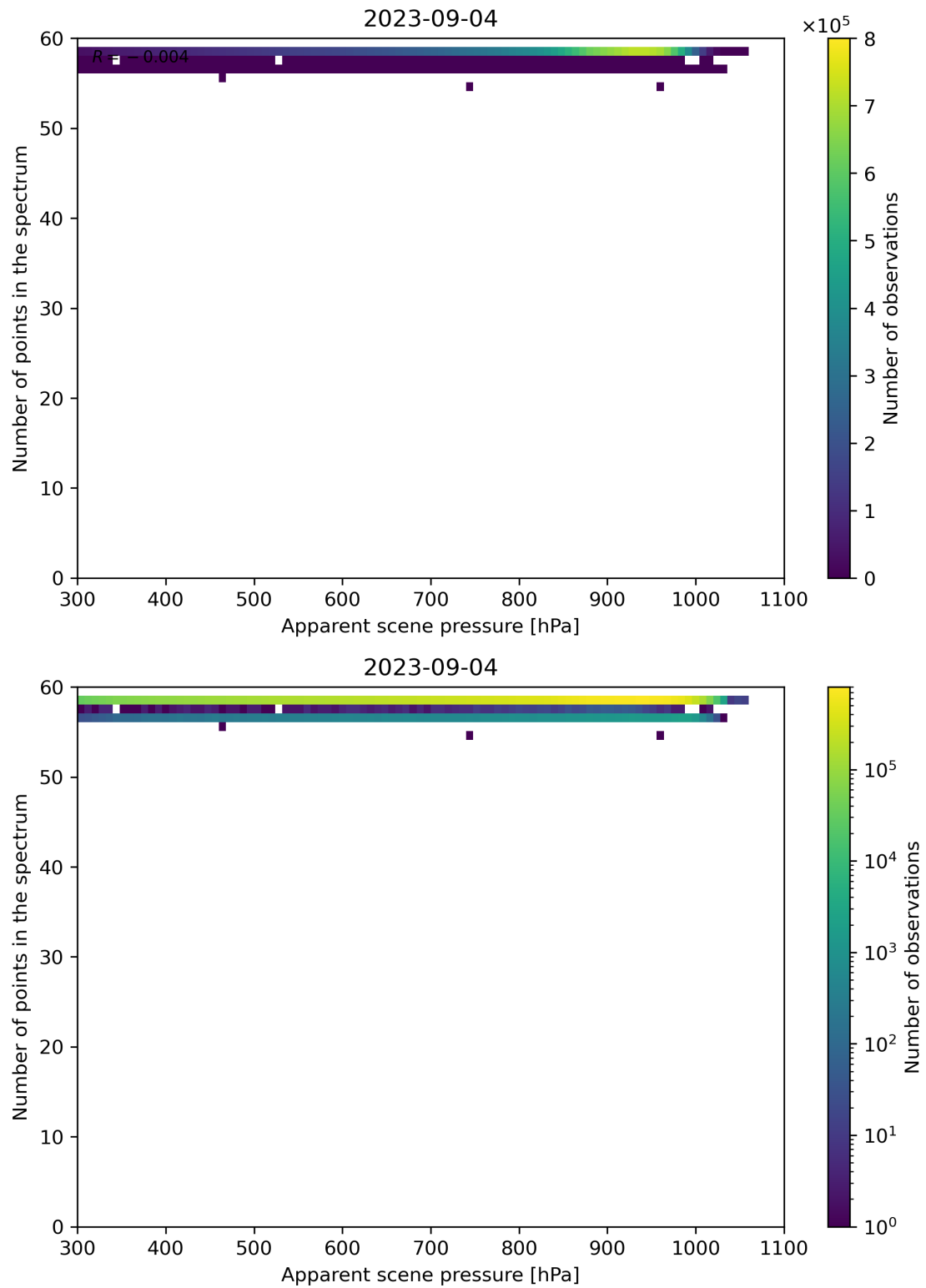
Figure 67: Scatter density plot of “Apparent scene pressure” against “Number of points in the spectrum” for 2023-09-04 to 2023-09-05.
