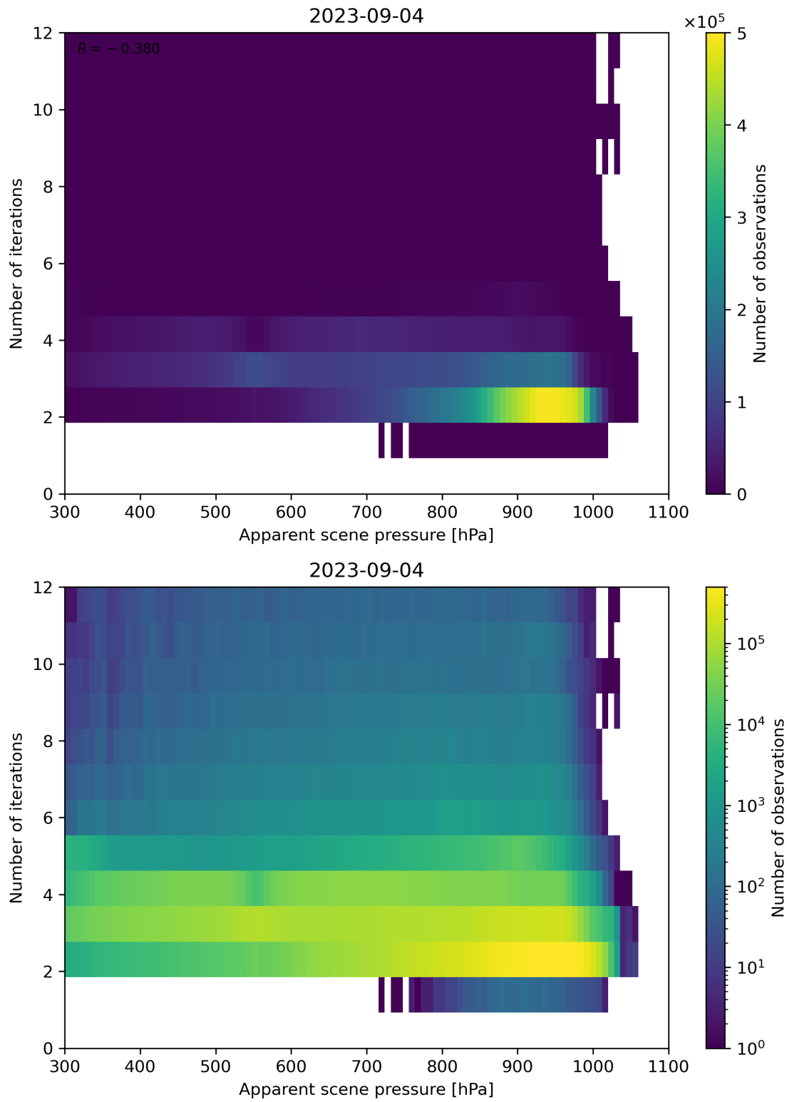
Figure 66: Scatter density plot of “Apparent scene pressure” against “Number of iterations” for 2023-09-04 to 2023-09-05.
