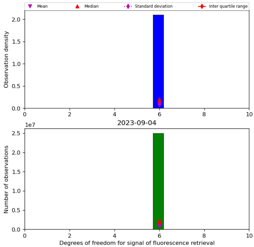
Figure 43: Histogram of “Degrees of freedom for signal of fluorescence retrieval” for 2023-09-04 to 2023-09-05
