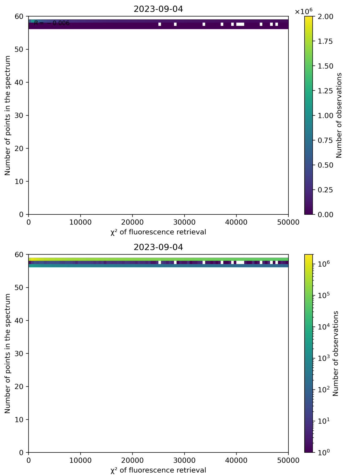
Figure 71: Scatter density plot of “ \chi^2 of fluorescence retrieval” against “Number of points in the spectrum” for 2023-09-04 to 2023-09-05.
