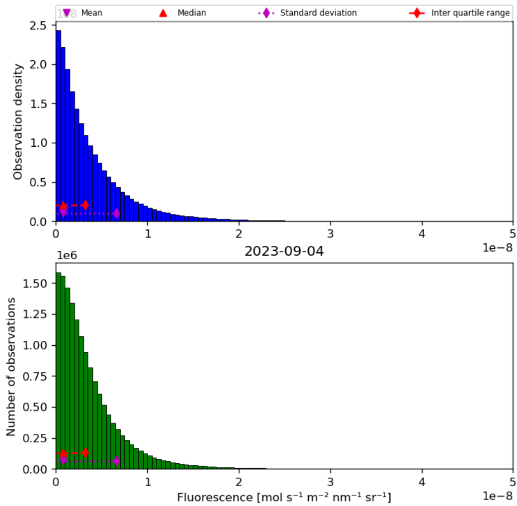
Figure 40: Histogram of “Fluorescence” for 2023-09-04 to 2023-09-05
