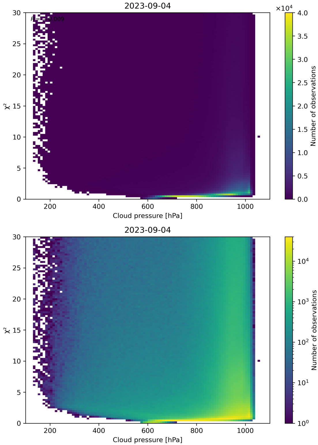
Figure 85: Scatter density plot of “Cloud pressure” against “ \chi^2 ” for 2023-09-04 to 2023-09-05.
