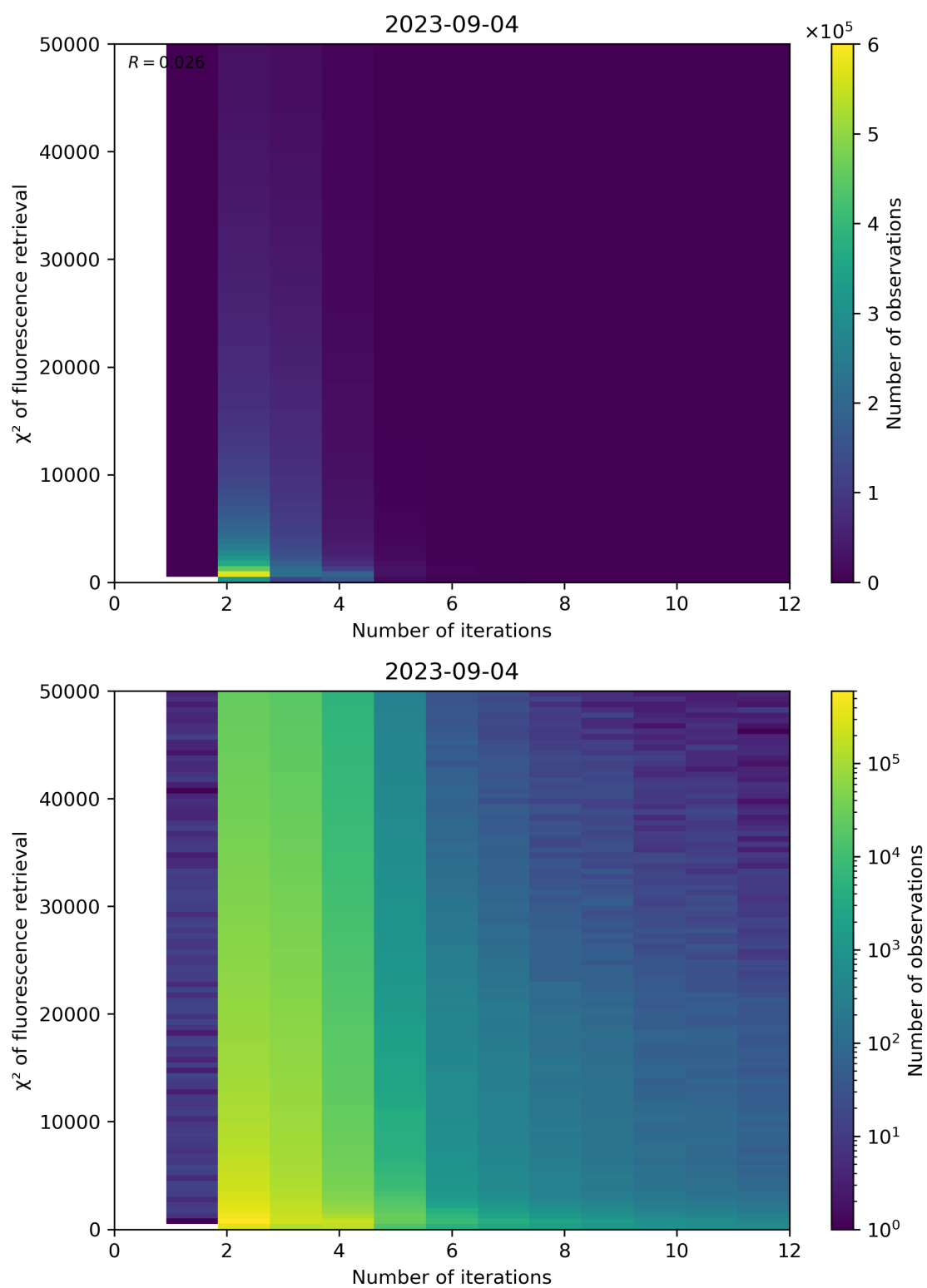
Figure 106: Scatter density plot of “Number of iterations” against “ \chi^2 of fluorescence retrieval” for 2023-09-04 to 2023-09-05.
