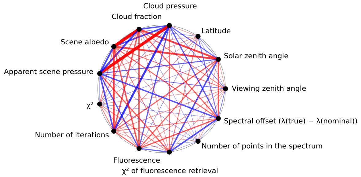
Figure 1: Map of correlation graph for 2023-09-04 to 2023-09-05.
