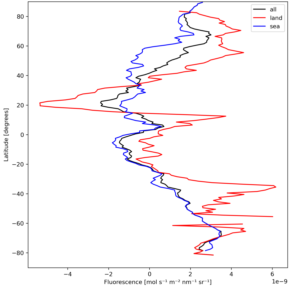
Figure 23: Zonal average of “Fluorescence” for 2023-09-04 to 2023-09-05.
