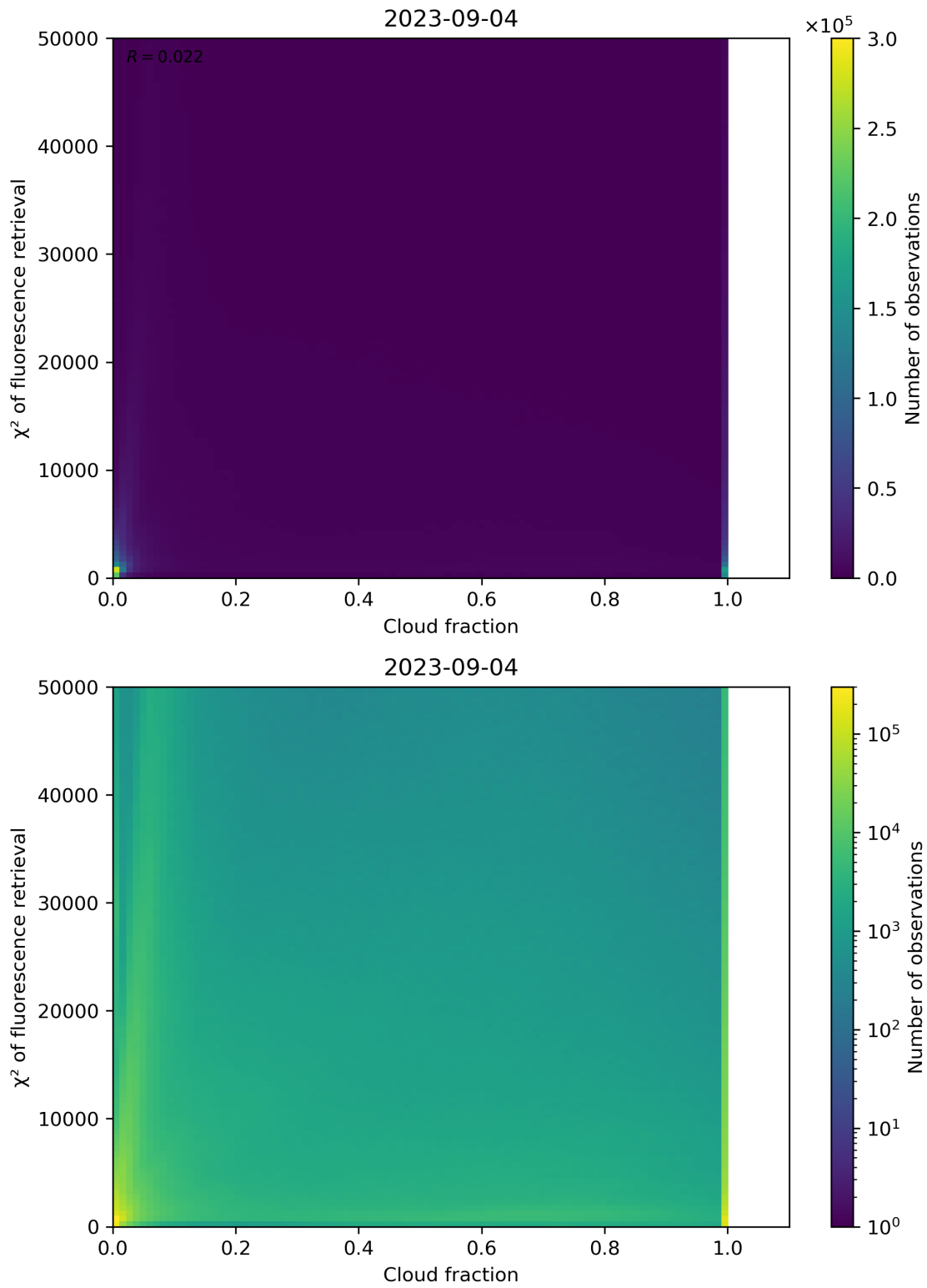
Figure 78: Scatter density plot of “Cloud fraction” against “ \chi^2 of fluorescence retrieval” for 2023-09-04 to 2023-09-05.
