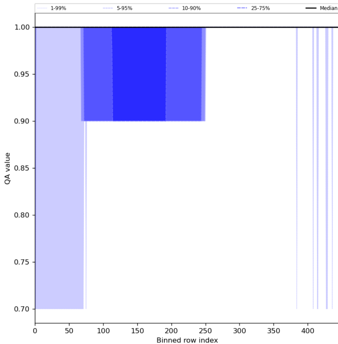
Figure 46: Along track statistics of “QA value” for 2023-09-04 to 2023-09-05
