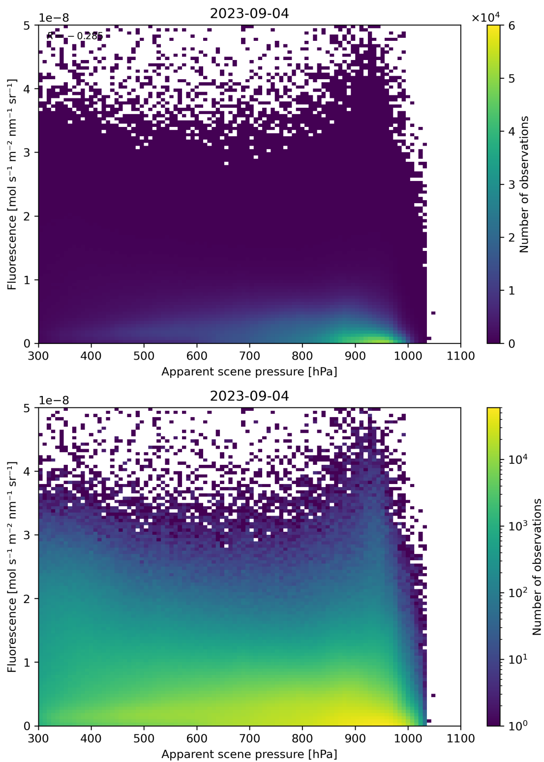
Figure 65: Scatter density plot of “Apparent scene pressure” against “Fluorescence” for 2023-09-04 to 2023-09-05.
