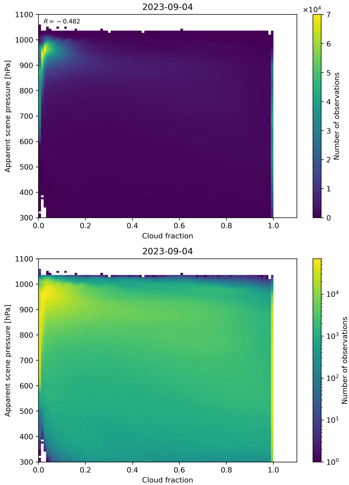
Figure 76: Scatter density plot of “Cloud fraction” against “Apparent scene pressure” for 2023-09-04 to 2023-09-05.
