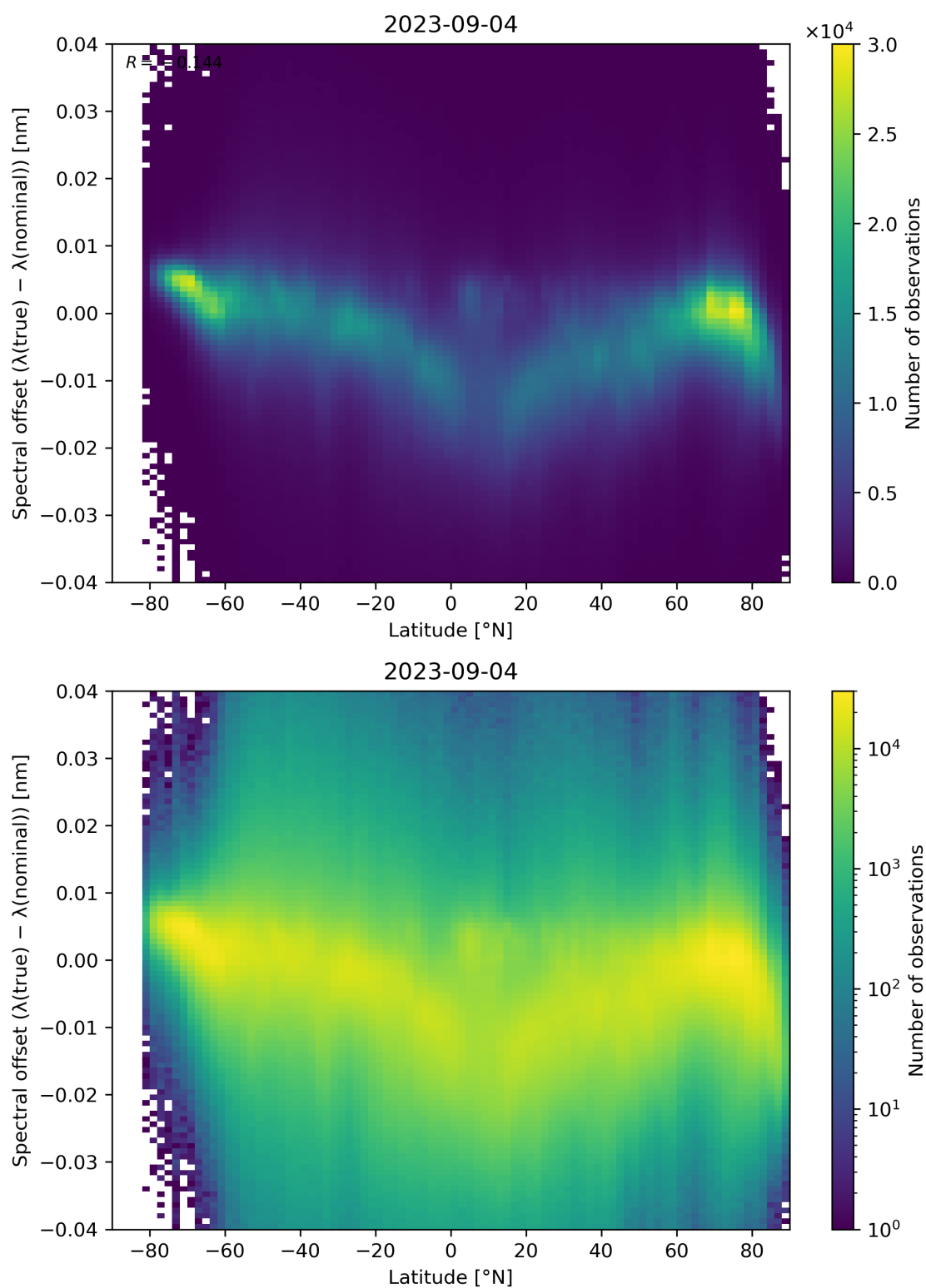
Figure 105: Scatter density plot of “Latitude” against “Spectral offset ( \lambda(\text{true}) - \lambda(\text{nominal}) )” for 2023-09-04 to 2023-09-05.
