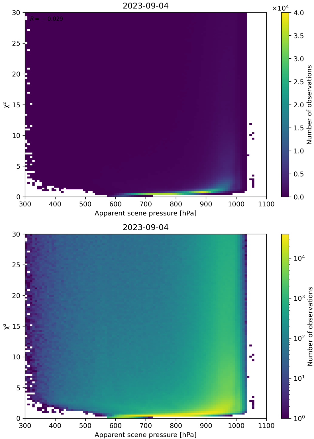
Figure 63: Scatter density plot of “Apparent scene pressure” against “ \chi^2 ” for 2023-09-04 to 2023-09-05.
