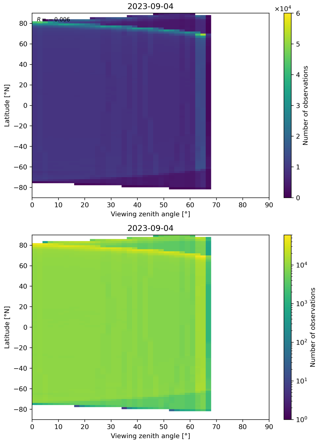
Figure 135: Scatter density plot of “Viewing zenith angle” against “Latitude” for 2023-09-04 to 2023-09-05.
