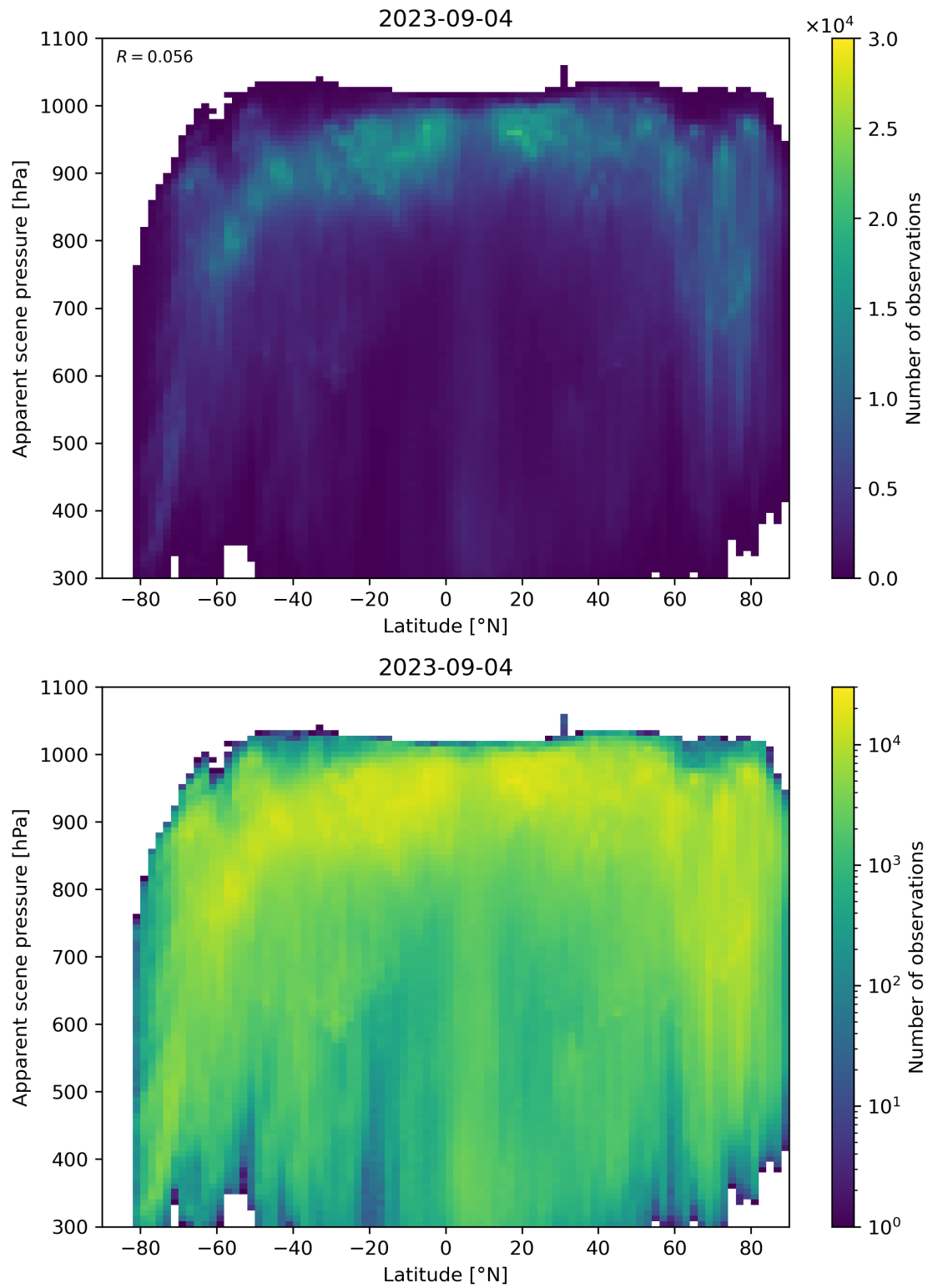
Figure 96: Scatter density plot of “Latitude” against “Apparent scene pressure” for 2023-09-04 to 2023-09-05.
