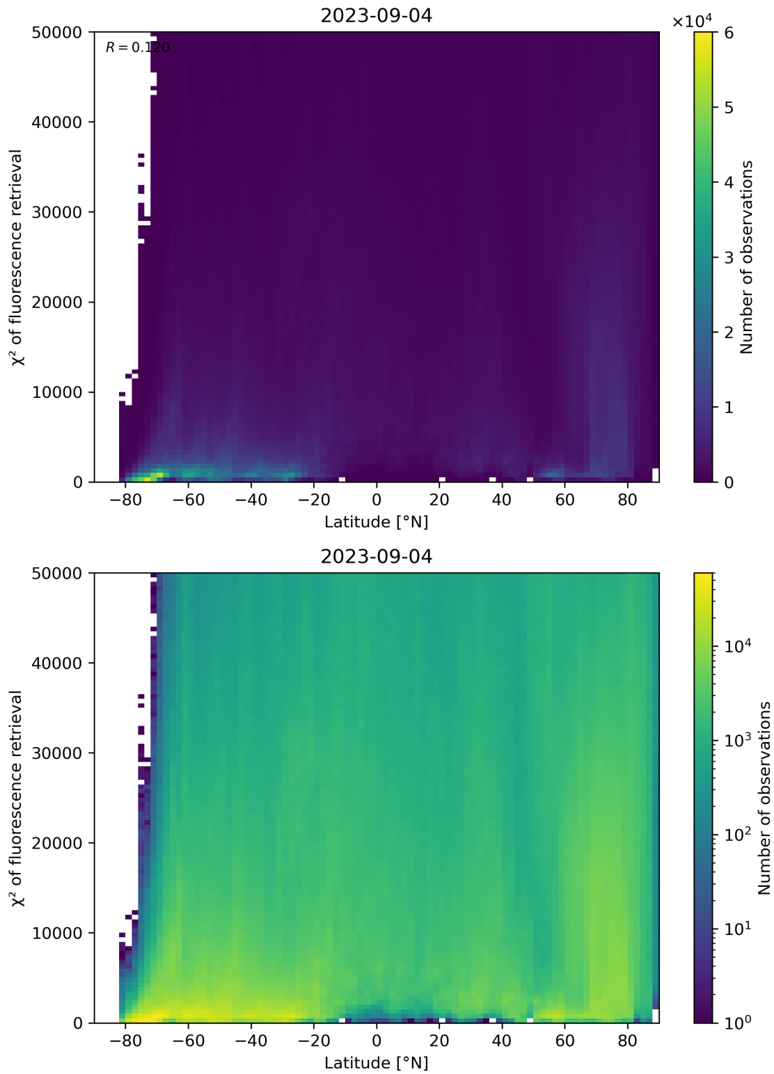
Figure 98: Scatter density plot of “Latitude” against “ \chi^2 of fluorescence retrieval” for 2023-09-04 to 2023-09-05.
