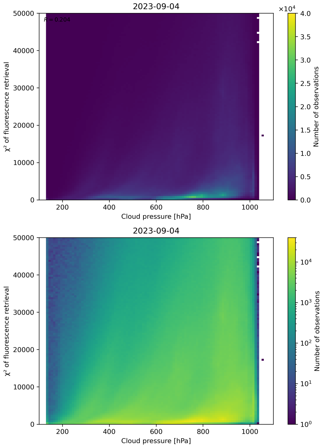
Figure 86: Scatter density plot of “Cloud pressure” against “ \chi^2 of fluorescence retrieval” for 2023-09-04 to 2023-09-05.
