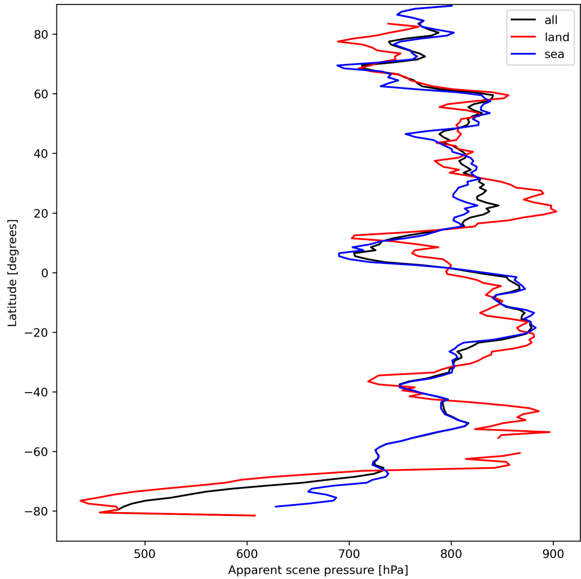
Figure 19: Zonal average of “Apparent scene pressure” for 2023-09-04 to 2023-09-05.
