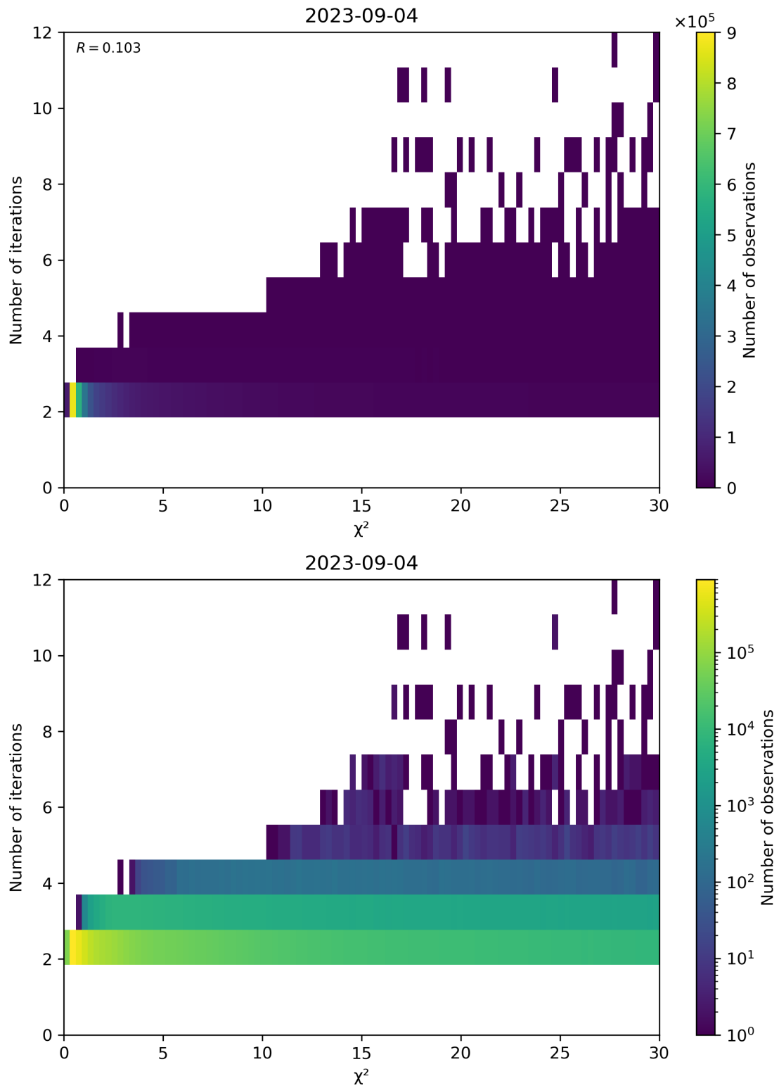
Figure 73: Scatter density plot of “ \chi^2 ” against “Number of iterations” for 2023-09-04 to 2023-09-05.
