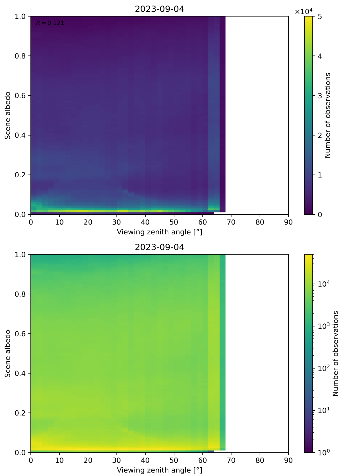
Figure 138: Scatter density plot of “Viewing zenith angle” against “Scene albedo” for 2023-09-04 to 2023-09-05.
