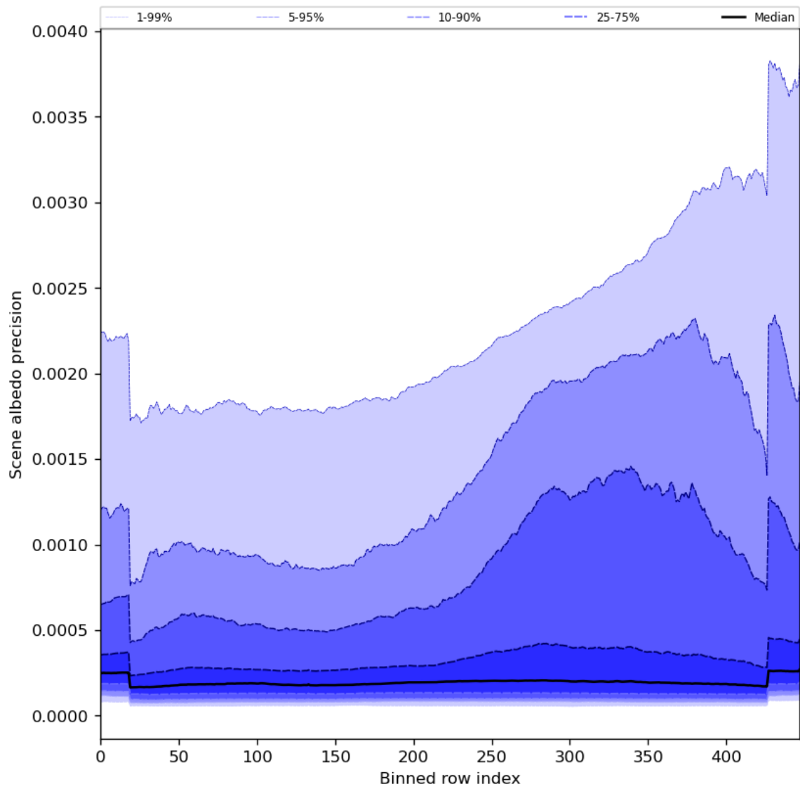
Figure 52: Along track statistics of “Scene albedo precision” for 2023-09-04 to 2023-09-05
