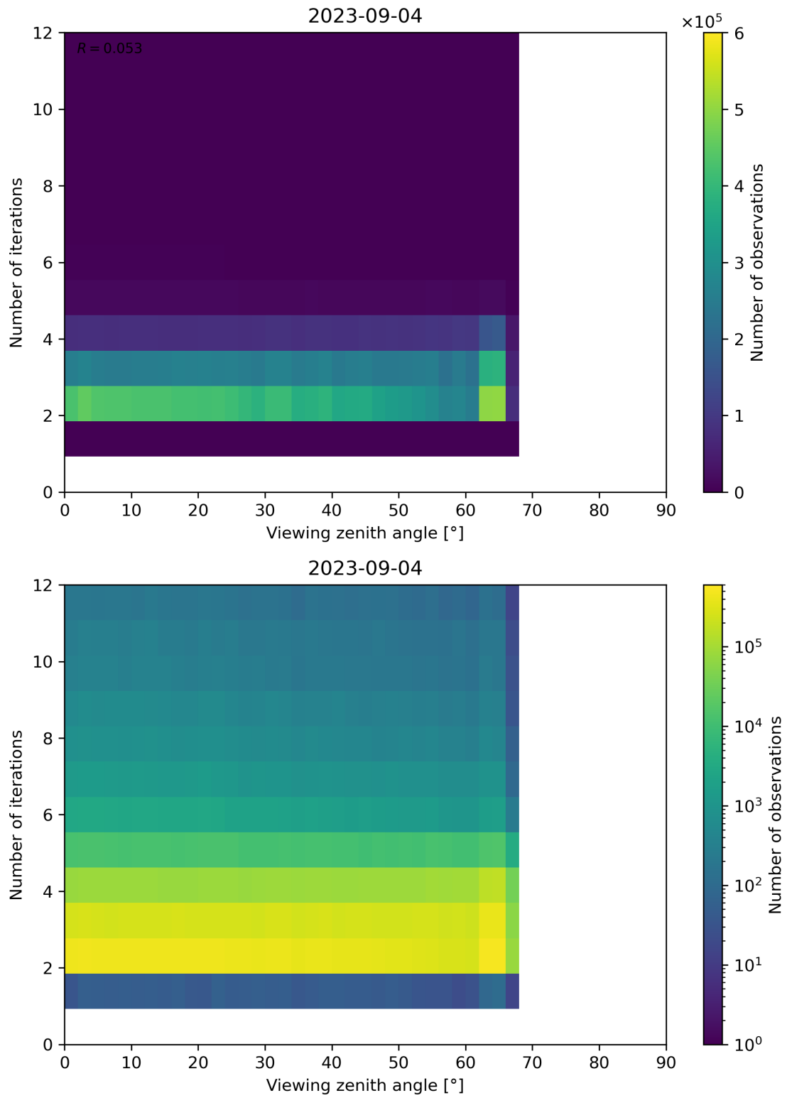
Figure 136: Scatter density plot of “Viewing zenith angle” against “Number of iterations” for 2023-09-04 to 2023-09-05.
