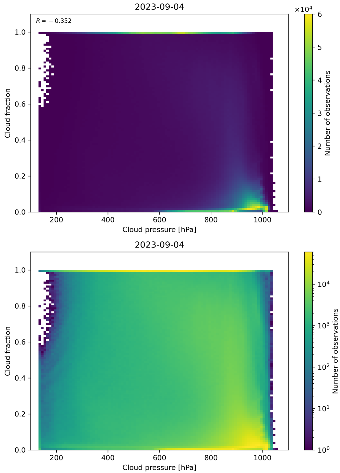
Figure 87: Scatter density plot of “Cloud pressure” against “Cloud fraction” for 2023-09-04 to 2023-09-05.
