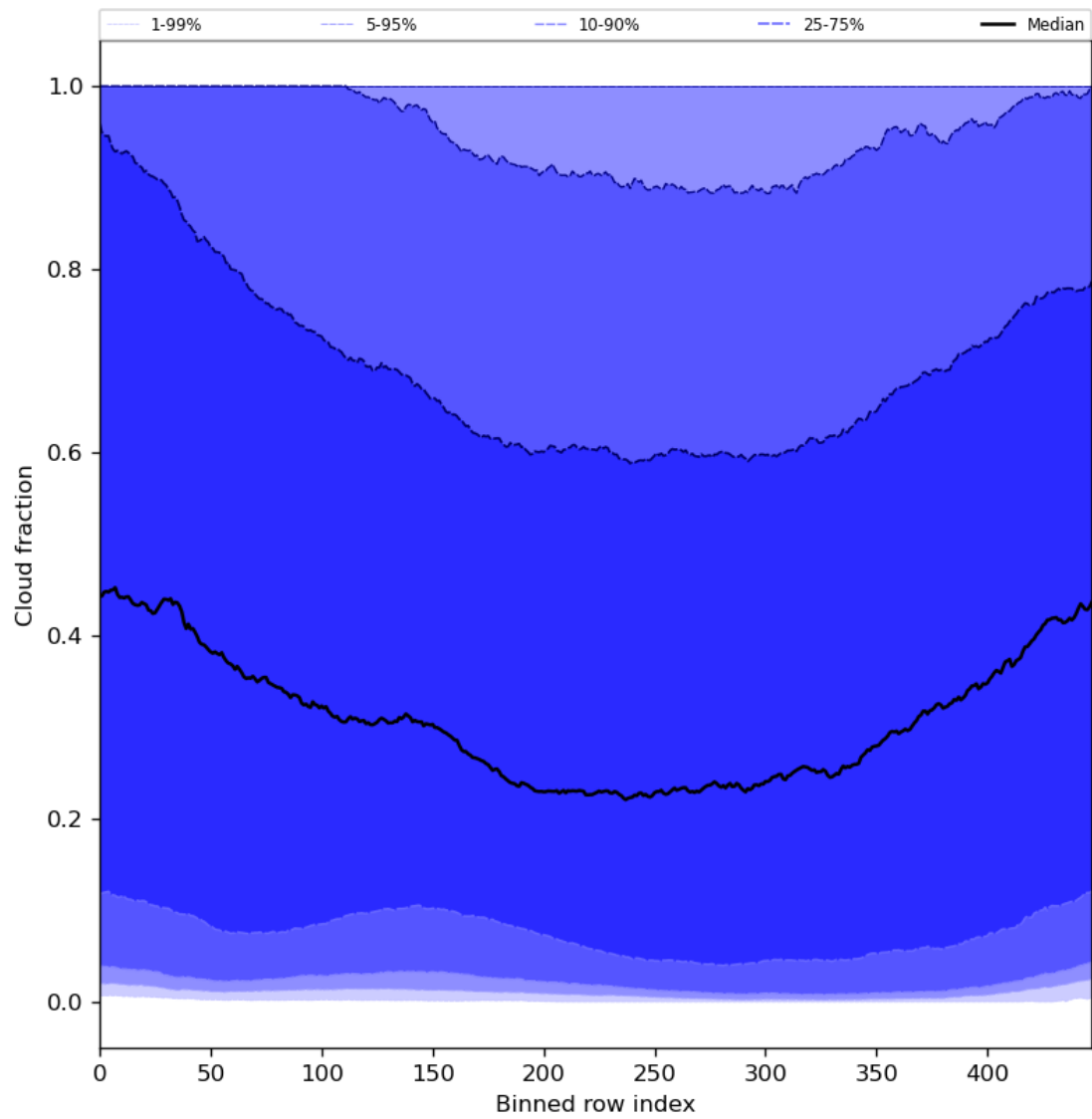
Figure 49: Along track statistics of “Cloud fraction” for 2023-09-04 to 2023-09-05
