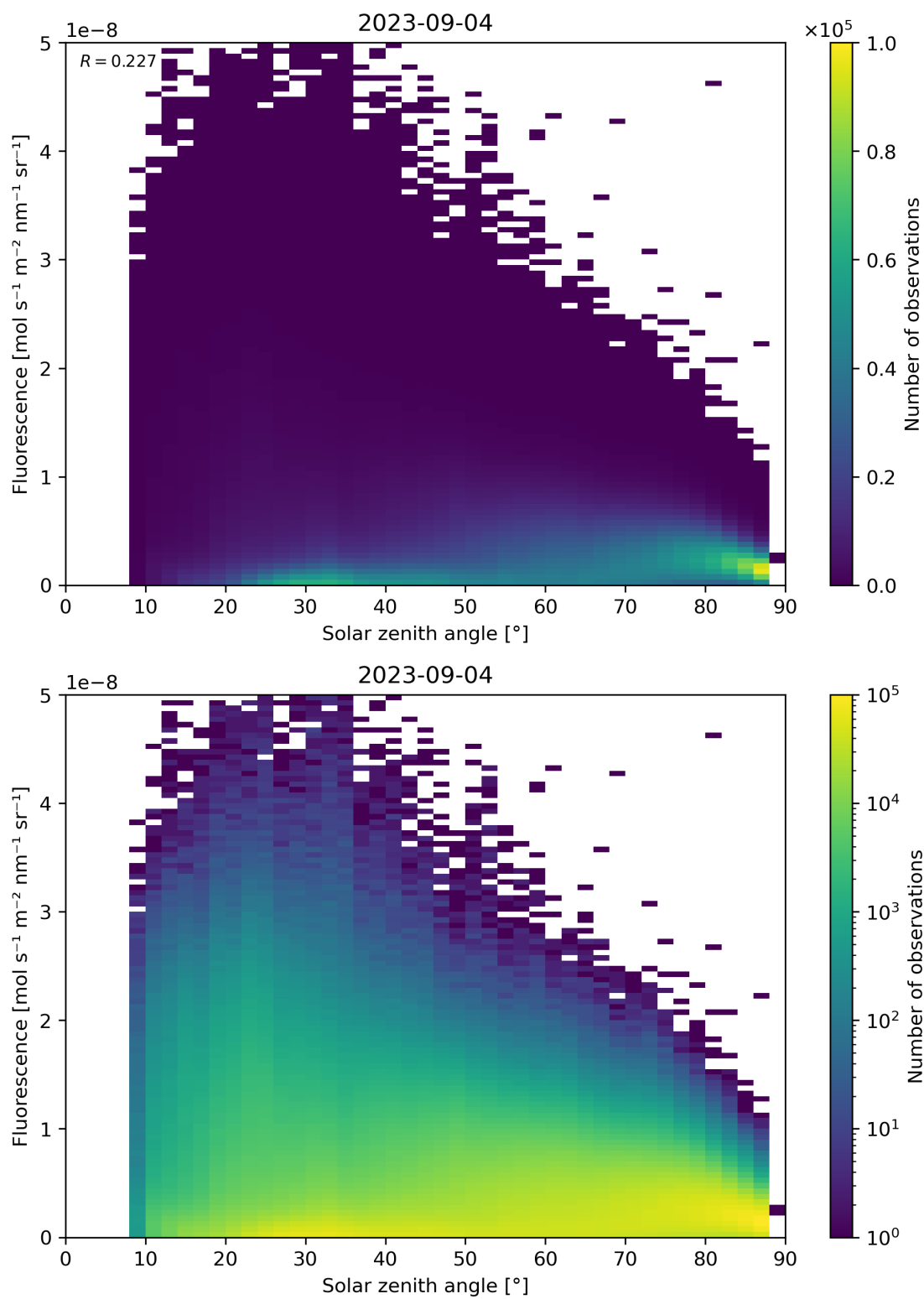
Figure 123: Scatter density plot of “Solar zenith angle” against “Fluorescence” for 2023-09-04 to 2023-09-05.
