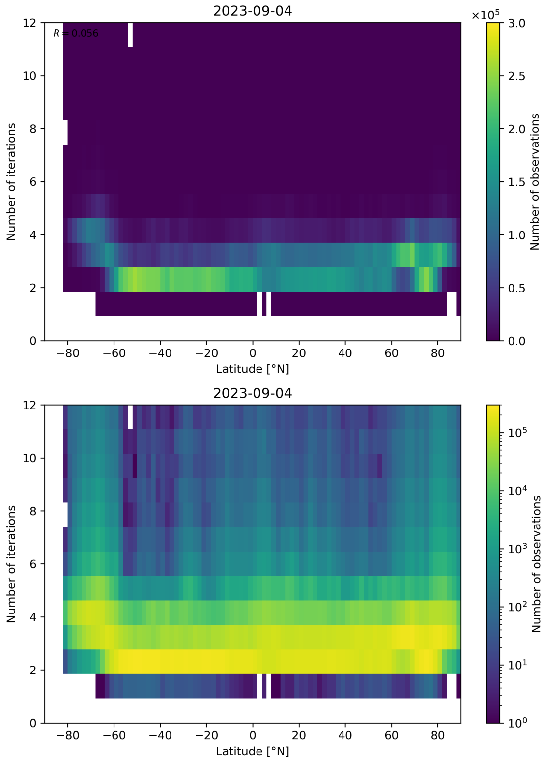
Figure 102: Scatter density plot of “Latitude” against “Number of iterations” for 2023-09-04 to 2023-09-05.
