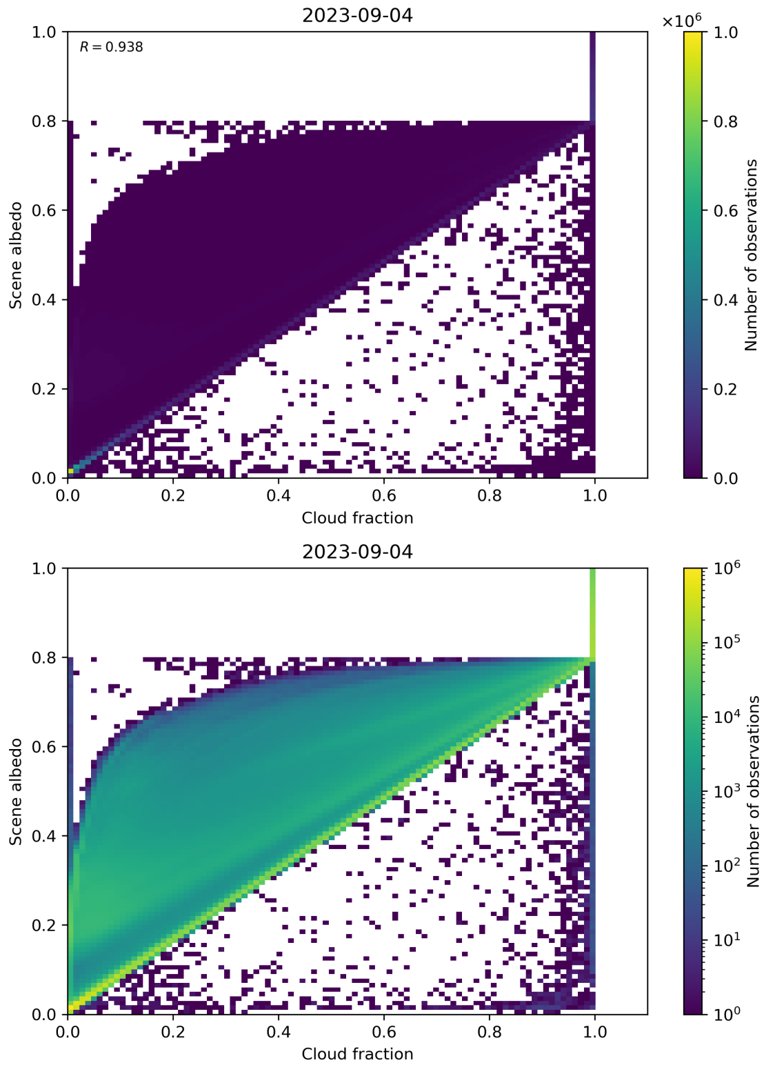
Figure 82: Scatter density plot of “Cloud fraction” against “Scene albedo” for 2023-09-04 to 2023-09-05.
