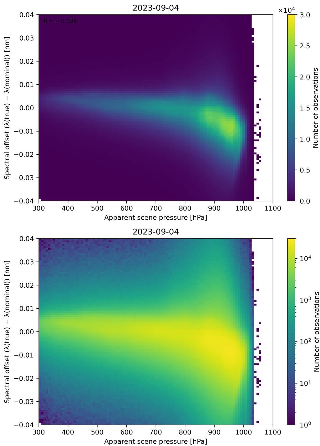
Figure 68: Scatter density plot of “Apparent scene pressure” against “Spectral offset ( \lambda(\text{true}) - \lambda(\text{nominal}) )” for 2023-09-04 to 2023-09-05.
