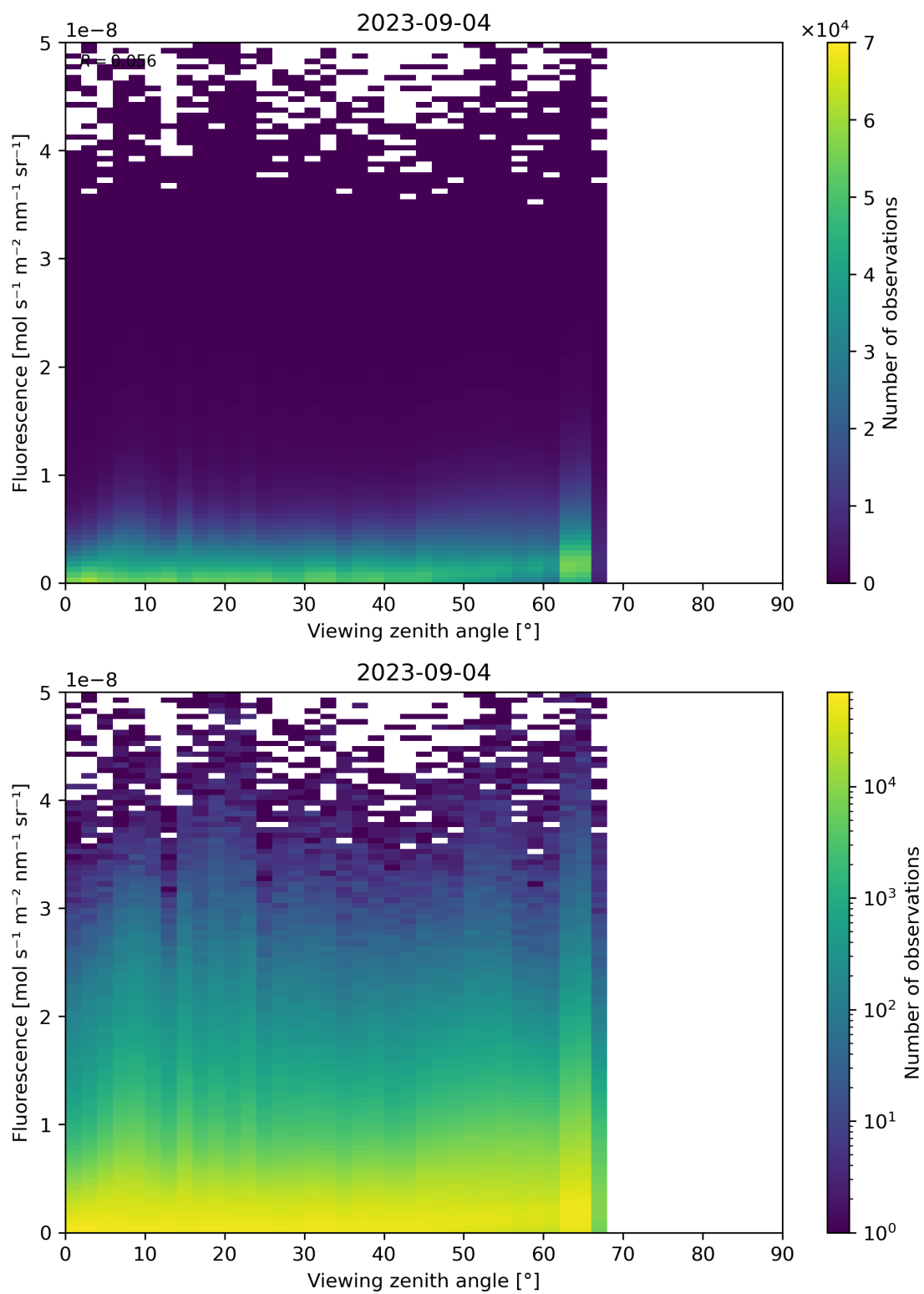
Figure 134: Scatter density plot of “Viewing zenith angle” against “Fluorescence” for 2023-09-04 to 2023-09-05.
