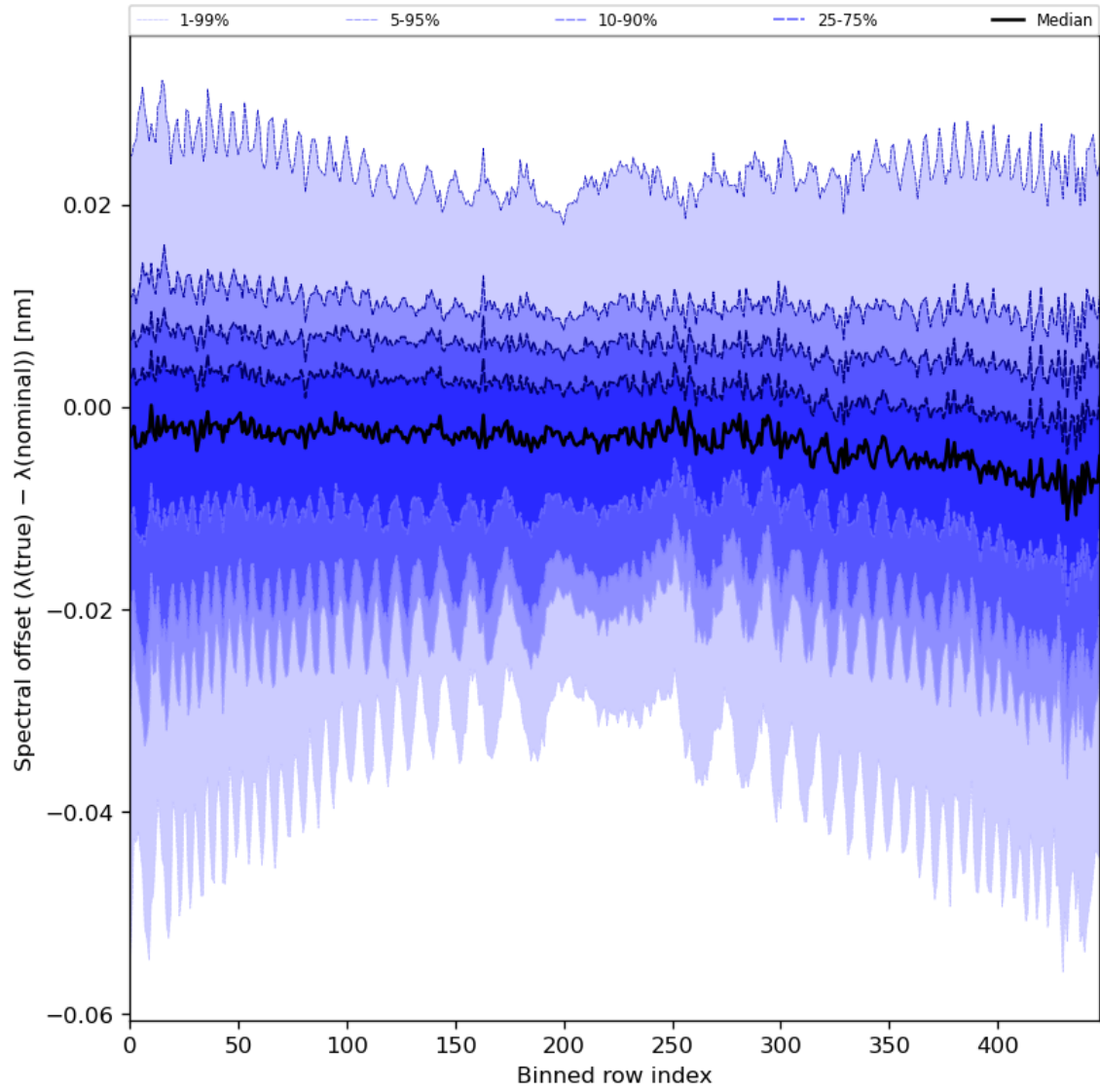
Figure 62: Along track statistics of “Spectral offset ( \lambda(\text{true}) - \lambda(\text{nominal}) )” for 2023-09-04 to 2023-09-05
