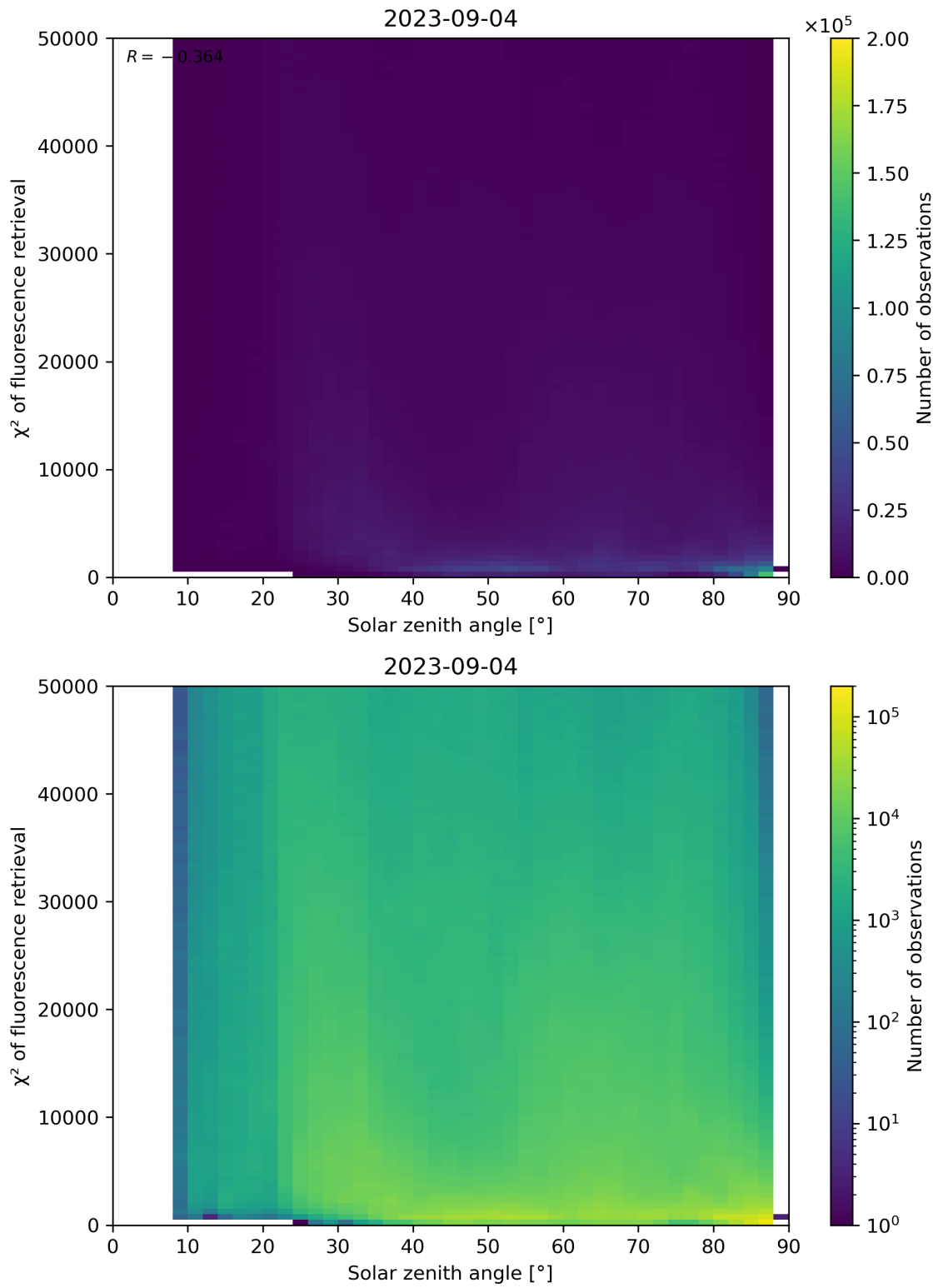
Figure 120: Scatter density plot of “Solar zenith angle” against “ \chi^2 of fluorescence retrieval” for 2023-09-04 to 2023-09-05.
