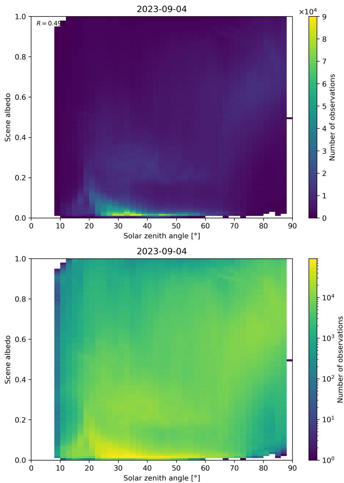
Figure 127: Scatter density plot of “Solar zenith angle” against “Scene albedo” for 2023-09-04 to 2023-09-05.
