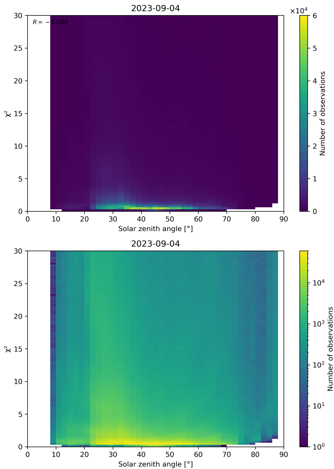
Figure 119: Scatter density plot of “Solar zenith angle” against “ \chi^2 ” for 2023-09-04 to 2023-09-05.
