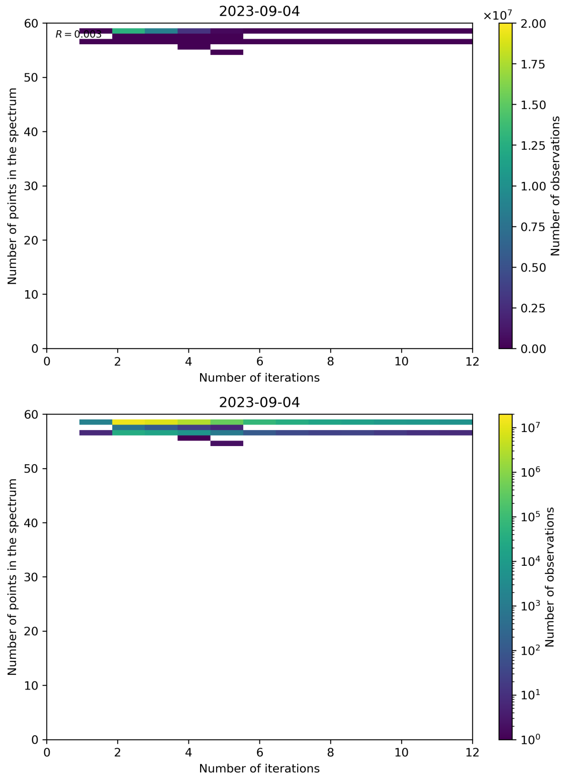
Figure 108: Scatter density plot of “Number of iterations” against “Number of points in the spectrum” for 2023-09-04 to 2023-09-05.
