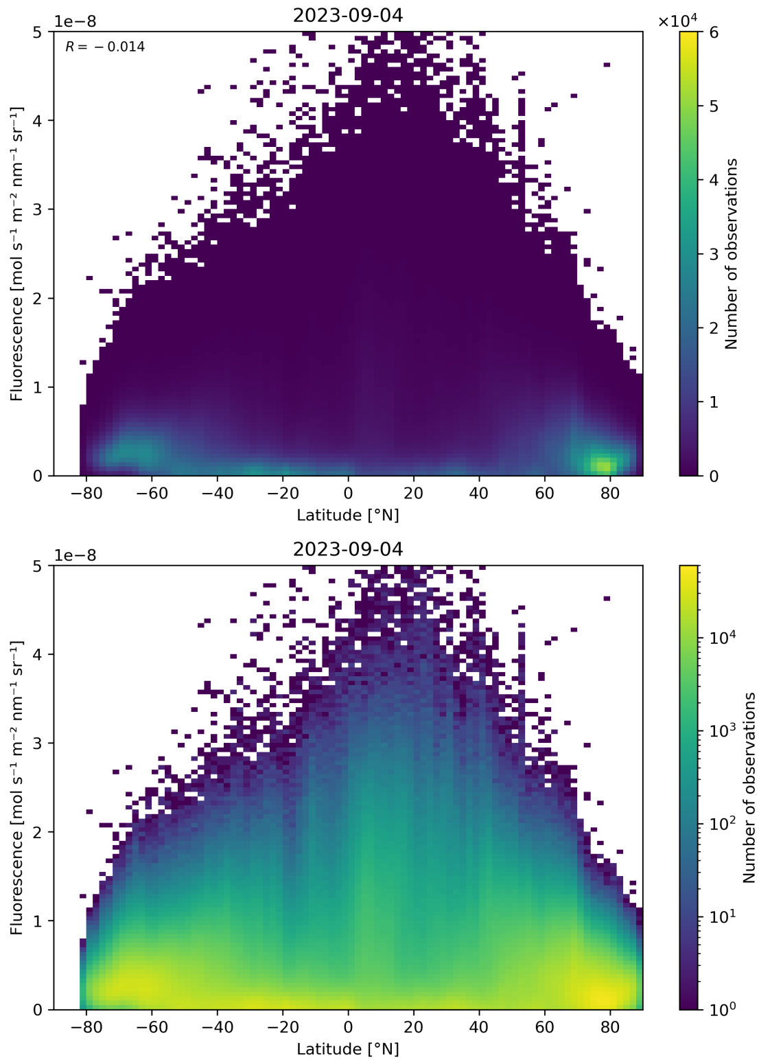
Figure 101: Scatter density plot of “Latitude” against “Fluorescence” for 2023-09-04 to 2023-09-05.
