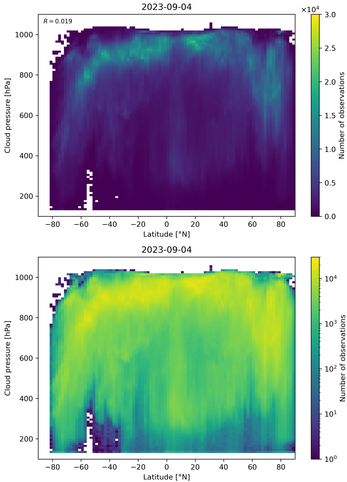
Figure 100: Scatter density plot of “Latitude” against “Cloud pressure” for 2023-09-04 to 2023-09-05.
