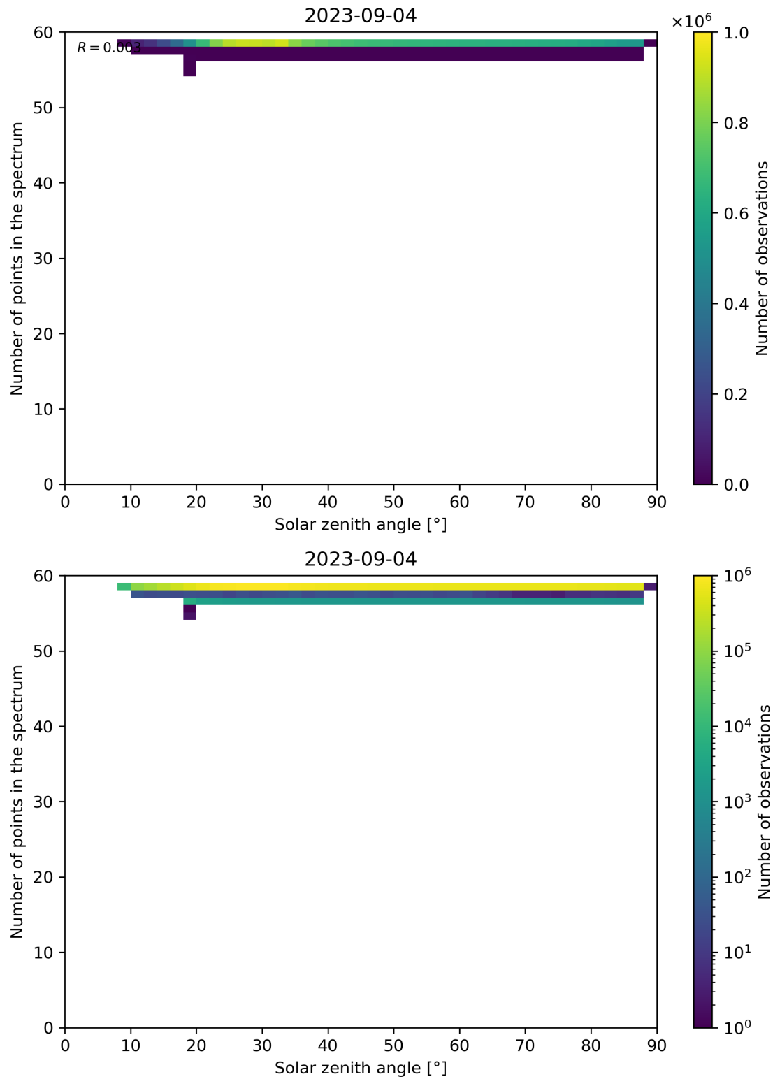
Figure 126: Scatter density plot of “Solar zenith angle” against “Number of points in the spectrum” for 2023-09-04 to 2023-09-05.
