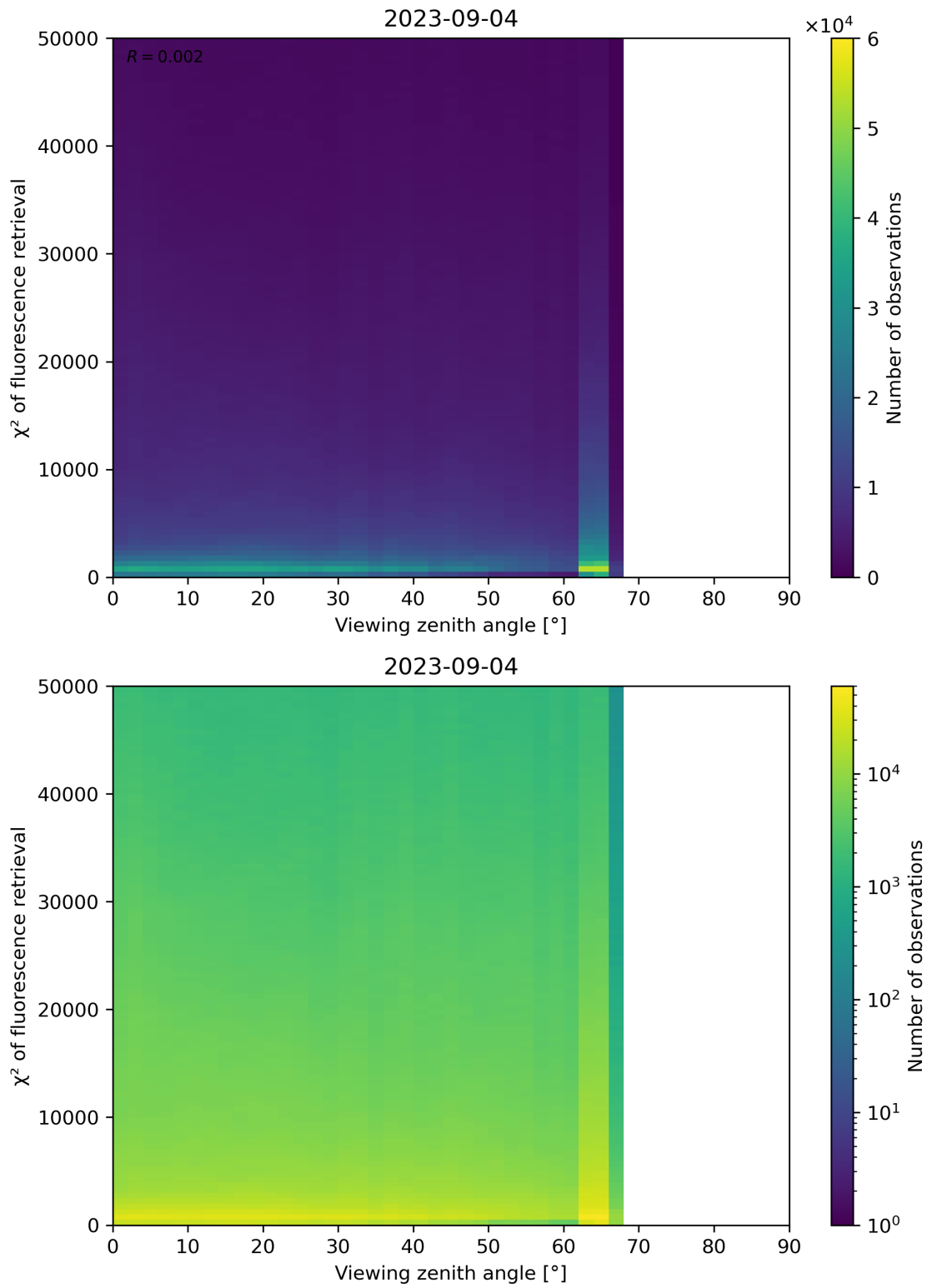
Figure 131: Scatter density plot of “Viewing zenith angle” against “ \chi^2 of fluorescence retrieval” for 2023-09-04 to 2023-09-05.
