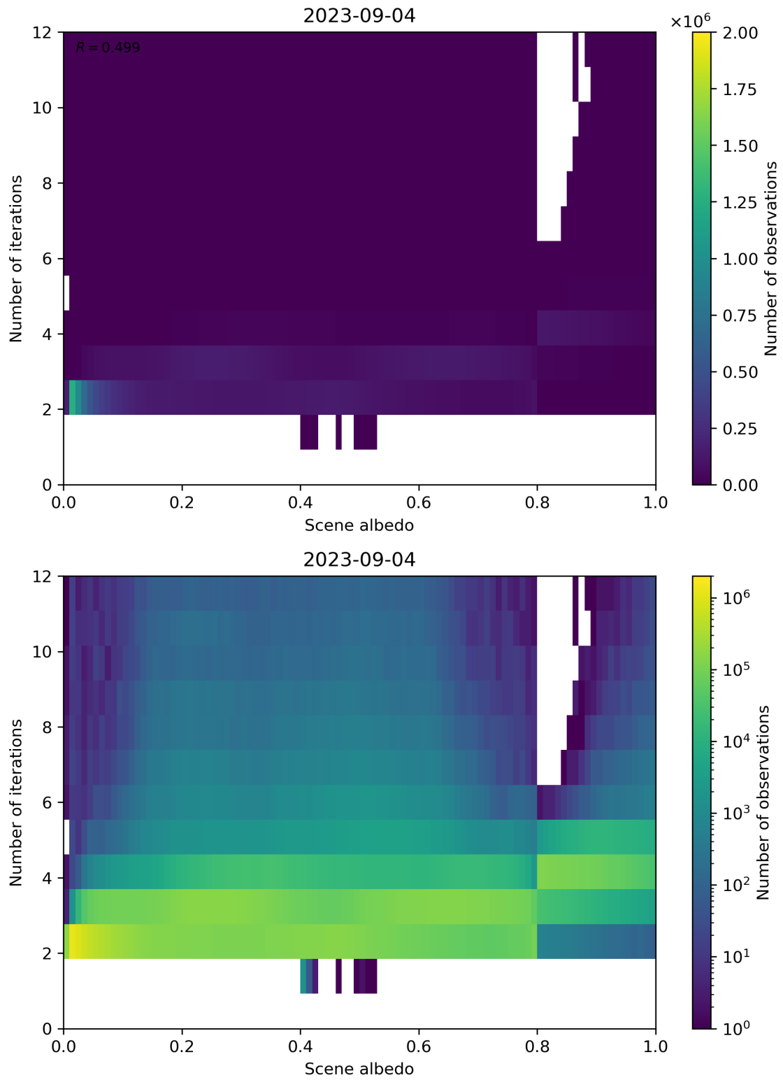
Figure 115: Scatter density plot of “Scene albedo” against “Number of iterations” for 2023-09-04 to 2023-09-05.
