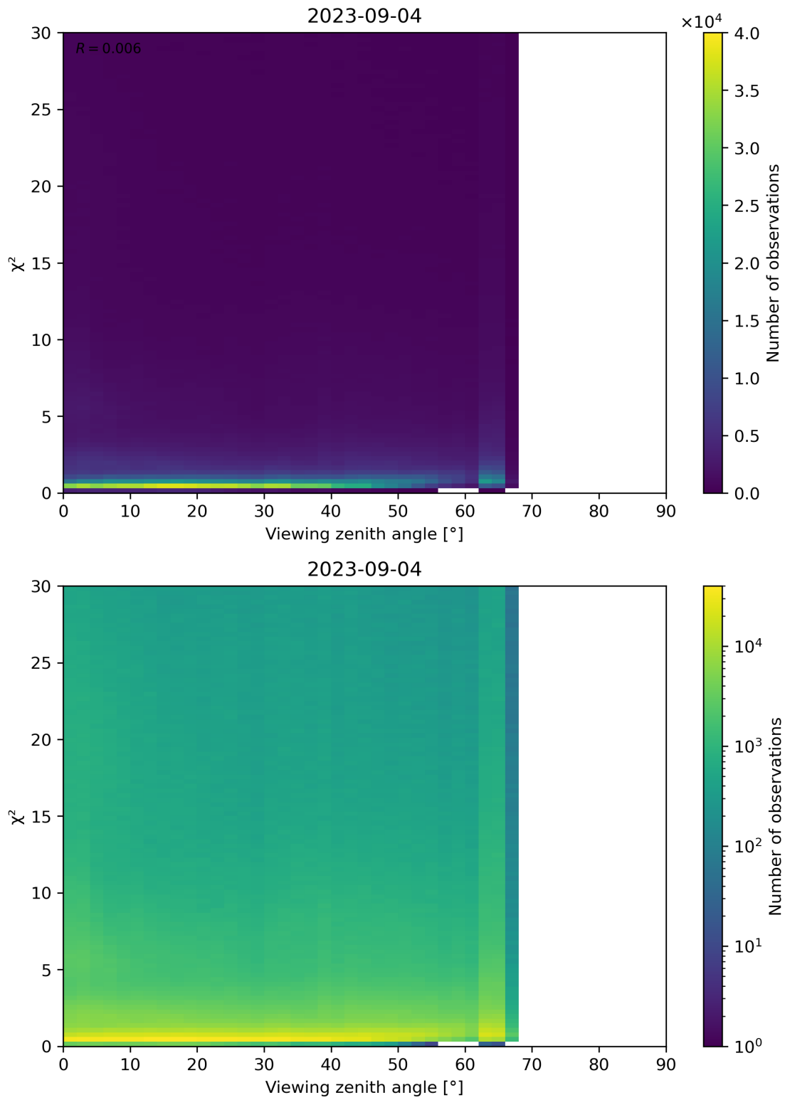
Figure 130: Scatter density plot of “Viewing zenith angle” against “ \chi^2 ” for 2023-09-04 to 2023-09-05.
