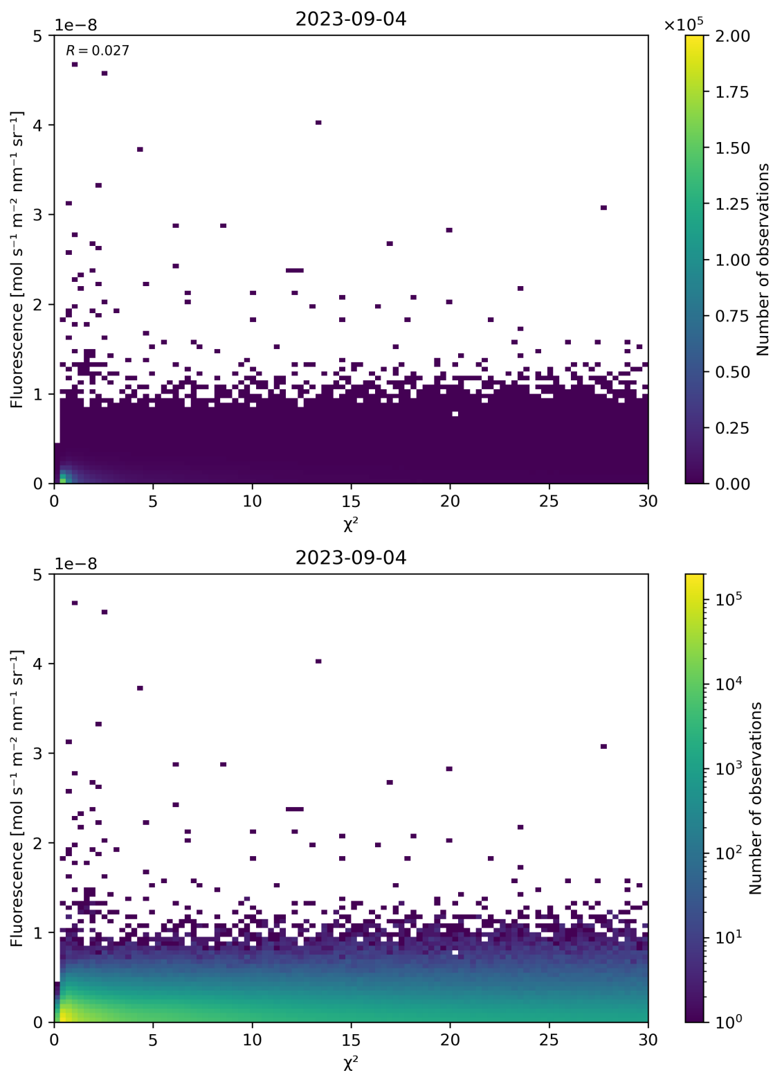
Figure 70: Scatter density plot of “ \chi^2 ” against “Fluorescence” for 2023-09-04 to 2023-09-05.
