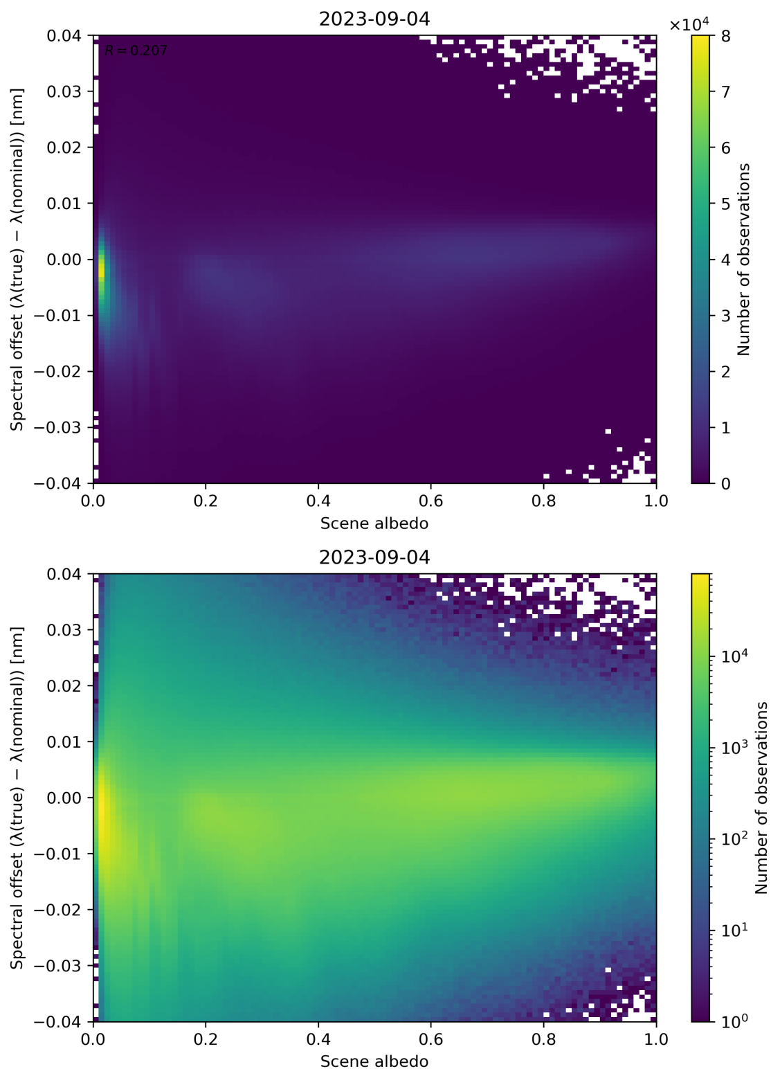
Figure 117: Scatter density plot of “Scene albedo” against “Spectral offset ( \lambda(\text{true}) - \lambda(\text{nominal}) )” for 2023-09-04 to 2023-09-05.
