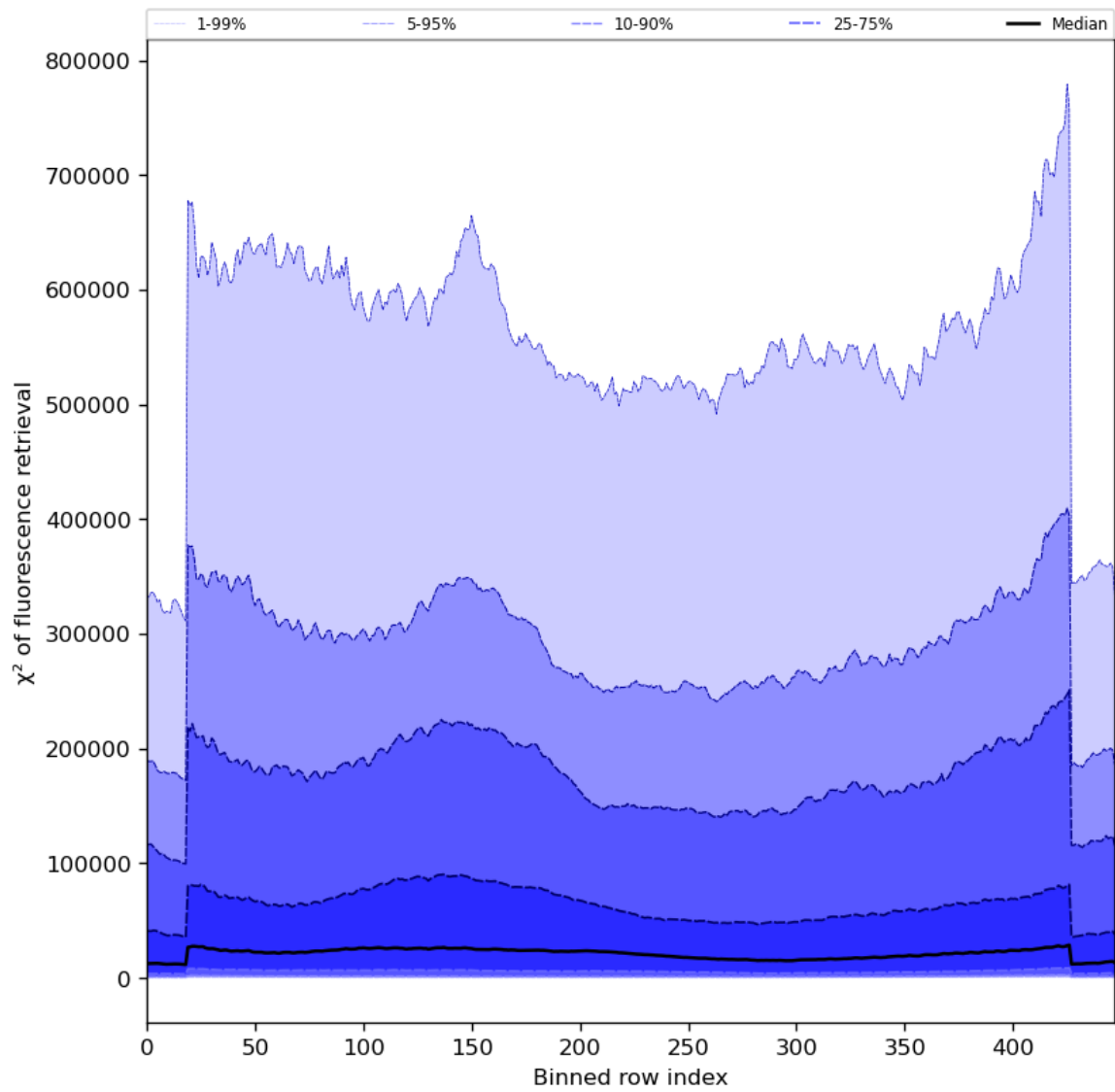
Figure 59: Along track statistics of “ \chi^2 of fluorescence retrieval” for 2023-09-04 to 2023-09-05
