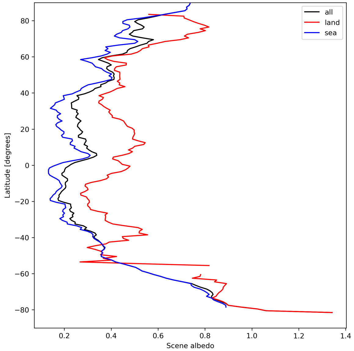
Figure 17: Zonal average of “Scene albedo” for 2023-09-04 to 2023-09-05.
