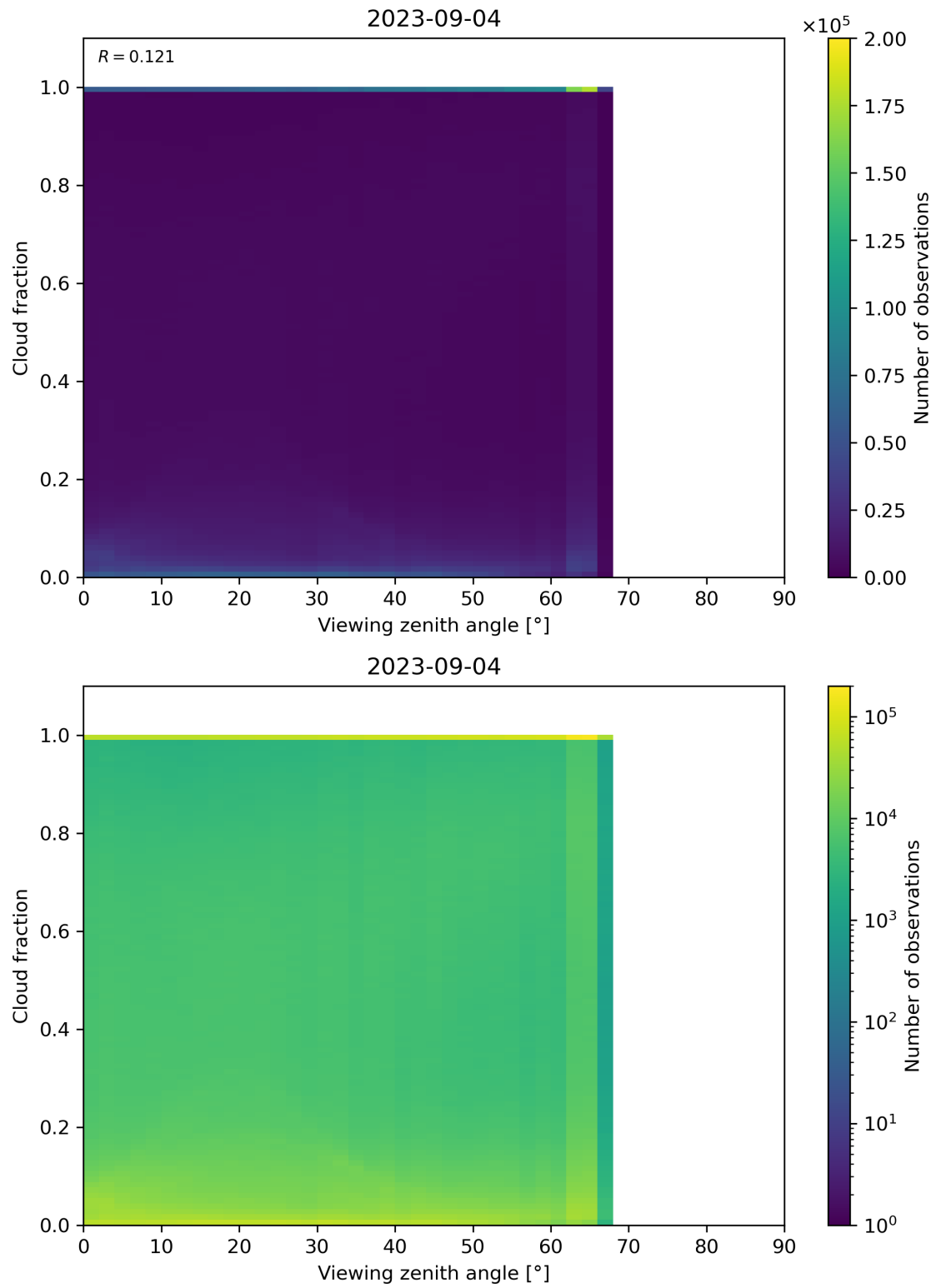
Figure 132: Scatter density plot of “Viewing zenith angle” against “Cloud fraction” for 2023-09-04 to 2023-09-05.
