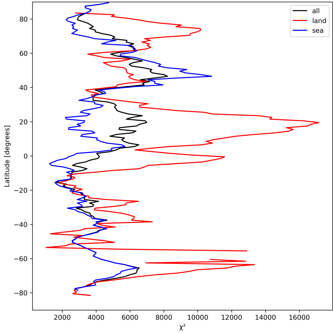
Figure 21: Zonal average of “ \chi^2 ” for 2023-09-04 to 2023-09-05.
