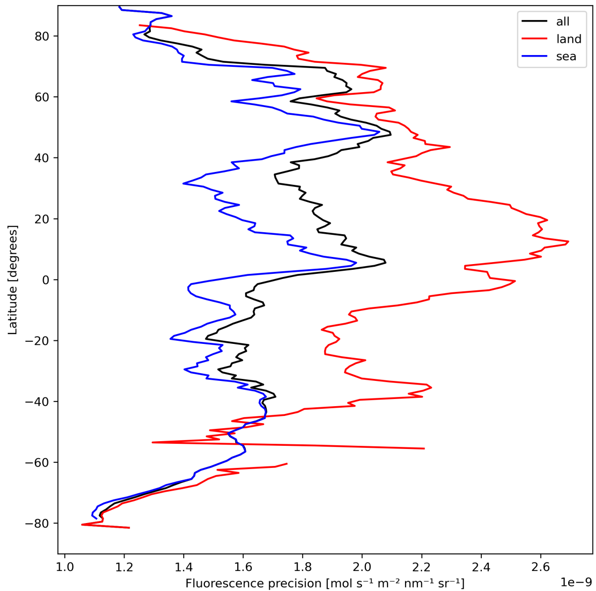
Figure 24: Zonal average of “Fluorescence precision” for 2023-09-04 to 2023-09-05.
