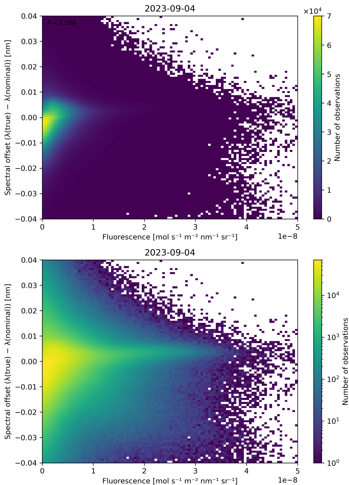
Figure 95: Scatter density plot of “Fluorescence” against “Spectral offset ( \lambda(\text{true}) - \lambda(\text{nominal}) )” for 2023-09-04 to 2023-09-05.
