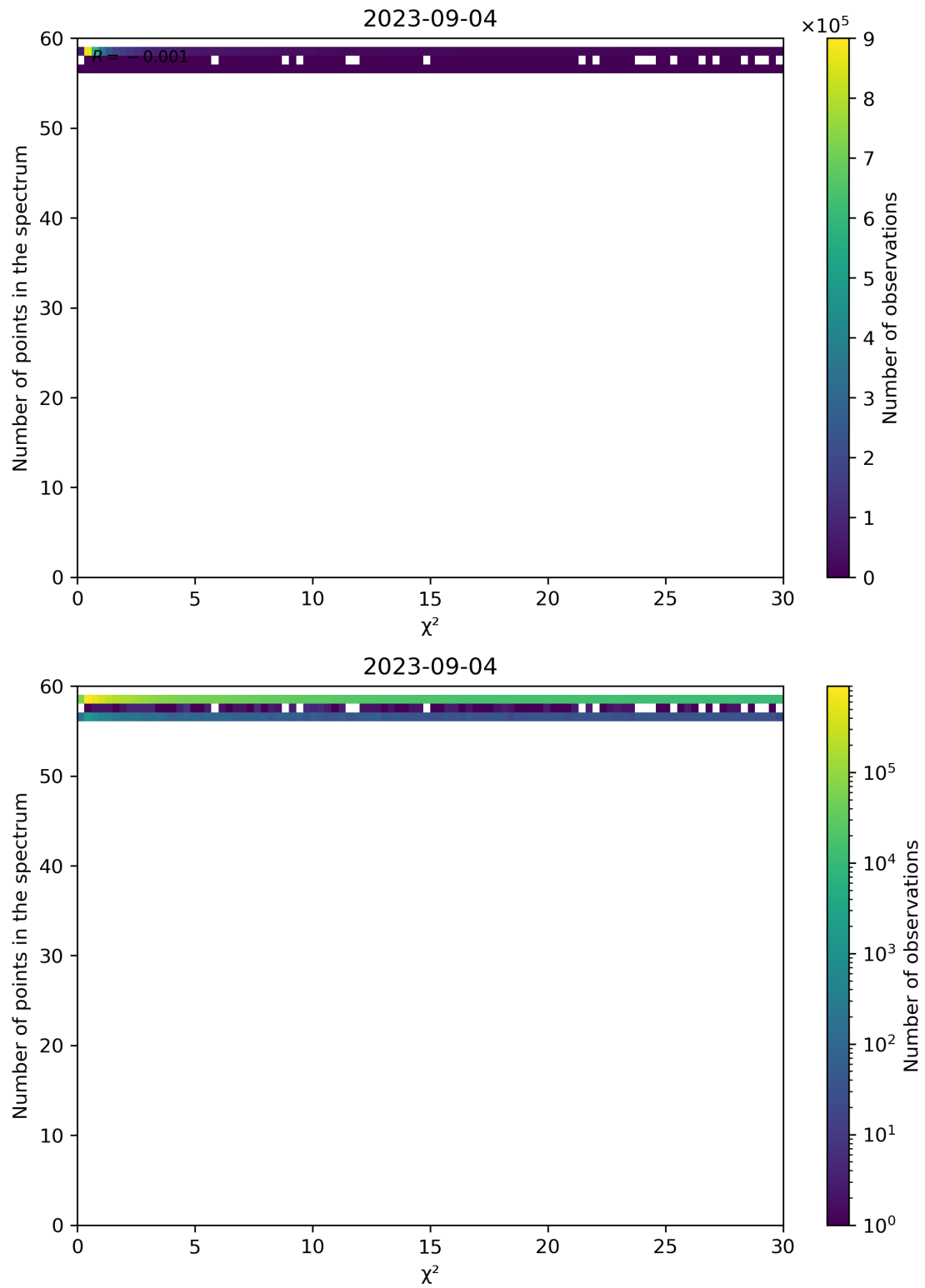
Figure 74: Scatter density plot of “ \chi^2 ” against “Number of points in the spectrum” for 2023-09-04 to 2023-09-05.
