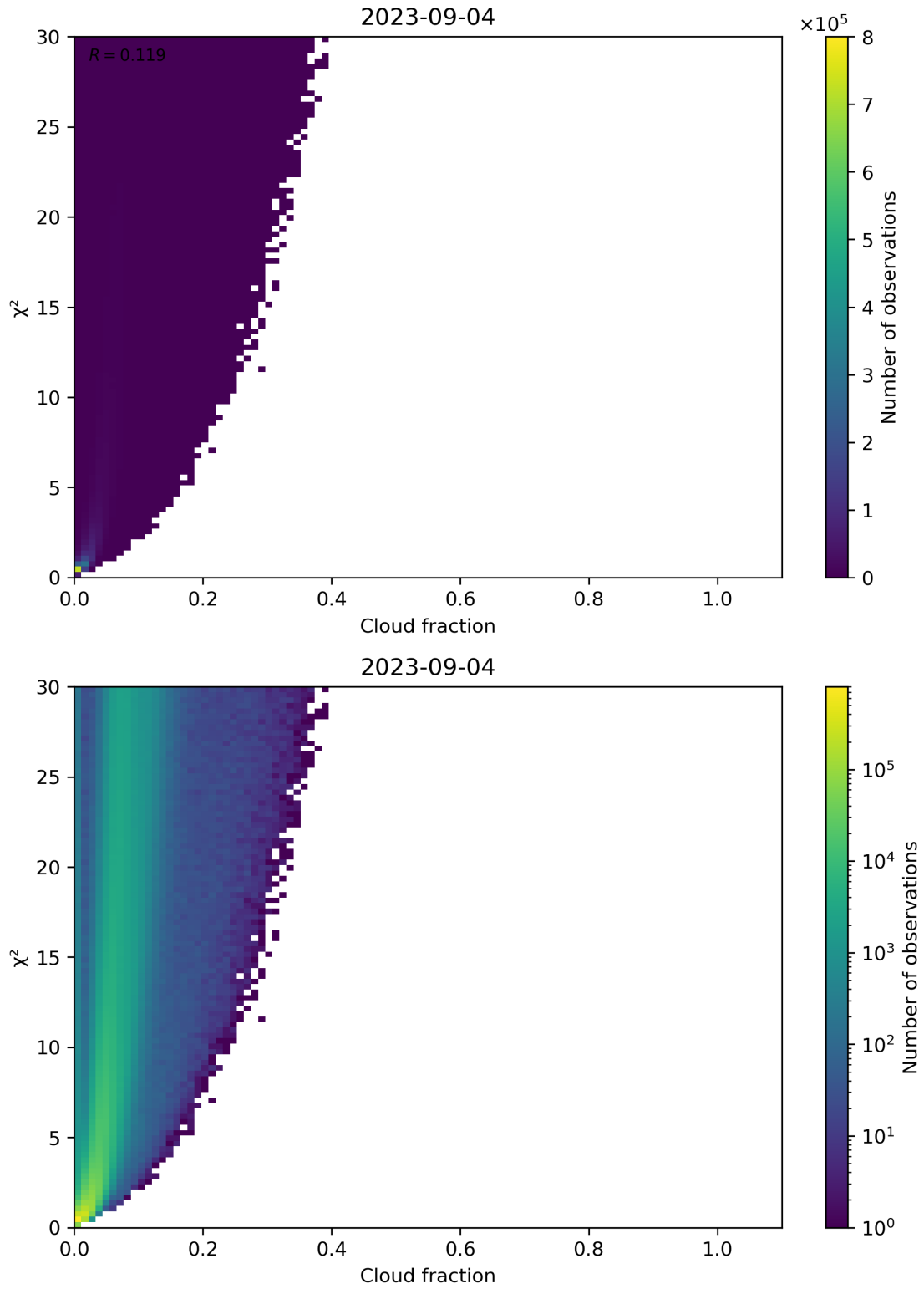
Figure 77: Scatter density plot of “Cloud fraction” against “ \chi^2 ” for 2023-09-04 to 2023-09-05.
