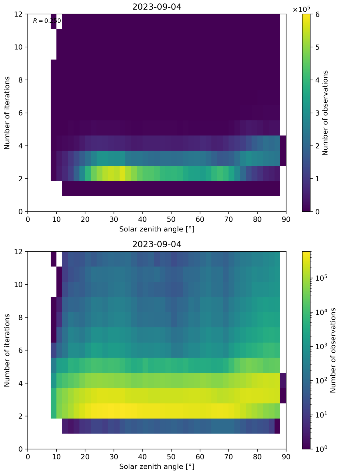
Figure 125: Scatter density plot of “Solar zenith angle” against “Number of iterations” for 2023-09-04 to 2023-09-05.
