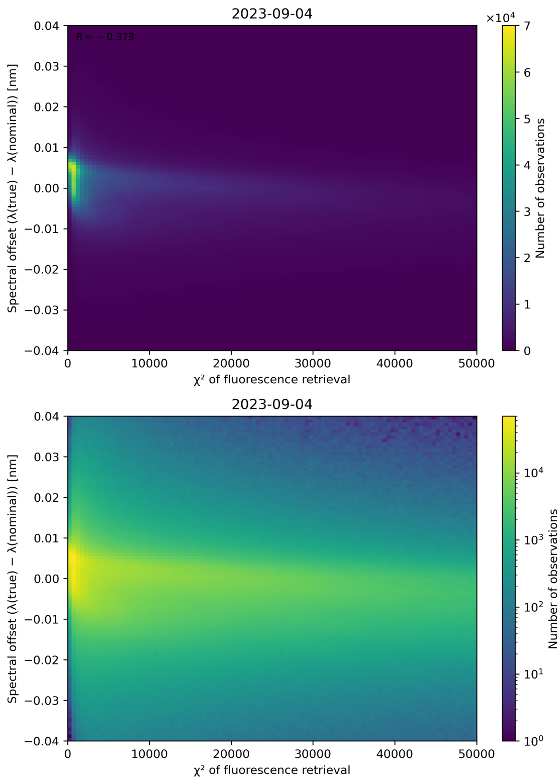
Figure 72: Scatter density plot of " \chi^2 of fluorescence retrieval" against "Spectral offset ( \lambda(\text{true}) - \lambda(\text{nominal}) )" for 2023-09-04 to 2023-09-05.
