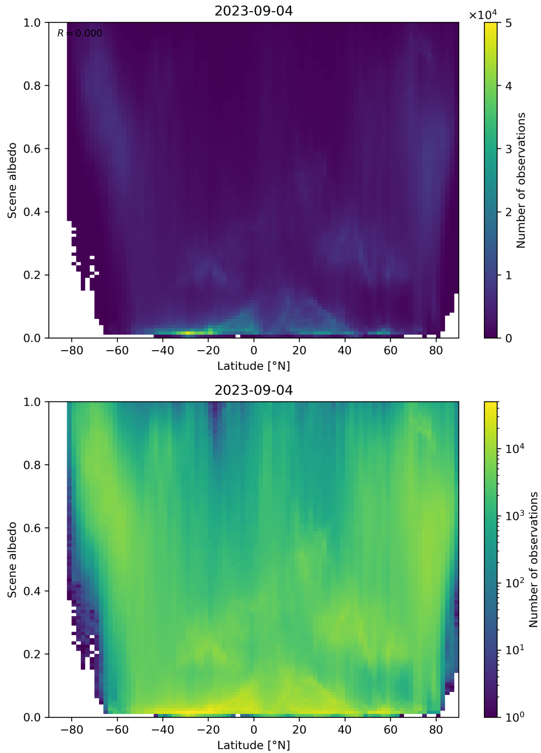
Figure 104: Scatter density plot of “Latitude” against “Scene albedo” for 2023-09-04 to 2023-09-05.
