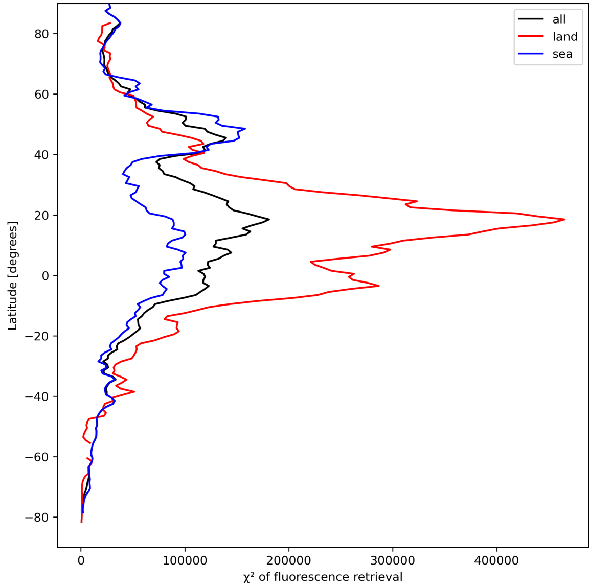
Figure 25: Zonal average of “ \chi^2 of fluorescence retrieval” for 2023-09-05 to 2023-09-06.
