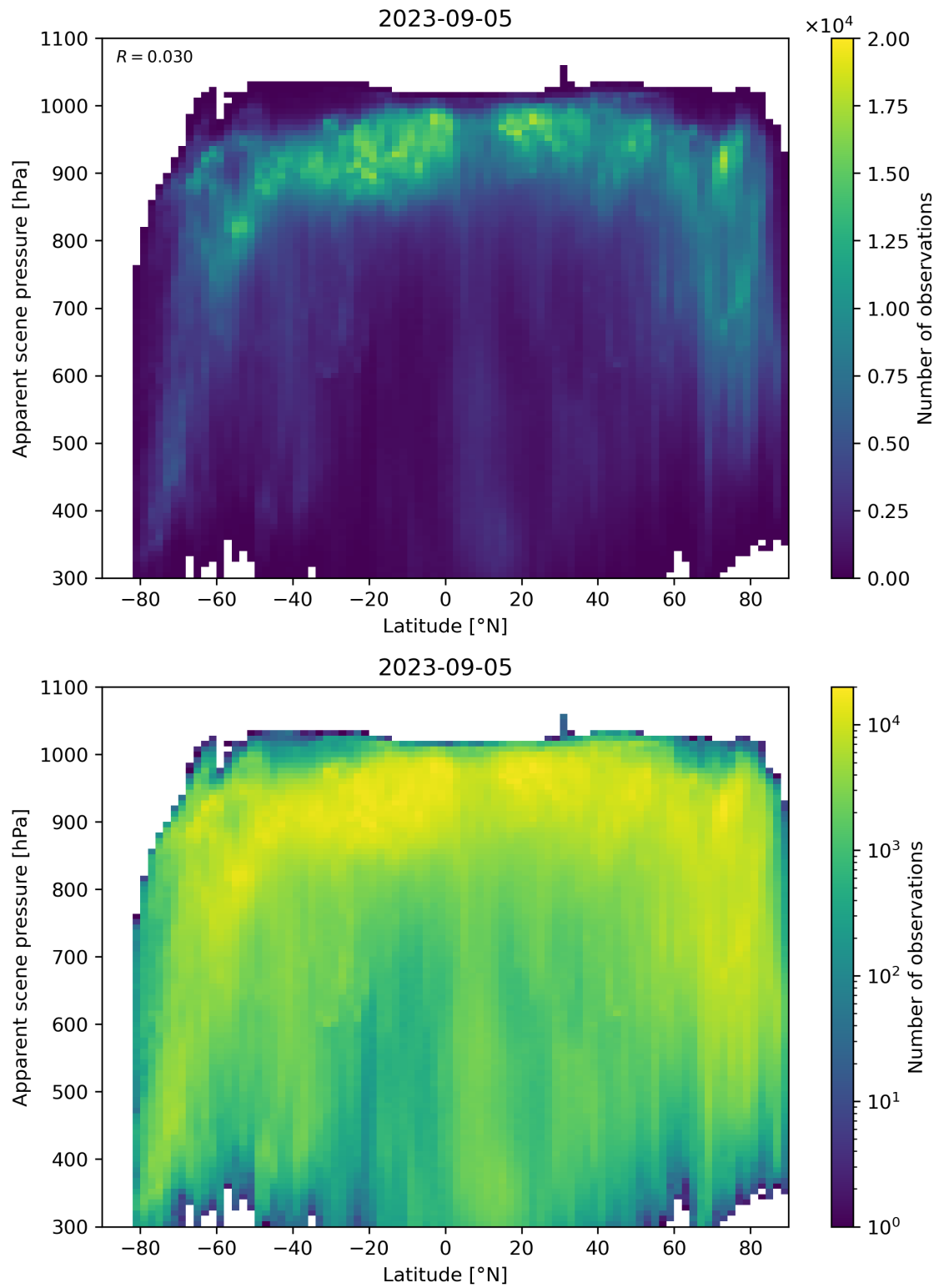
Figure 96: Scatter density plot of “Latitude” against “Apparent scene pressure” for 2023-09-05 to 2023-09-06.
