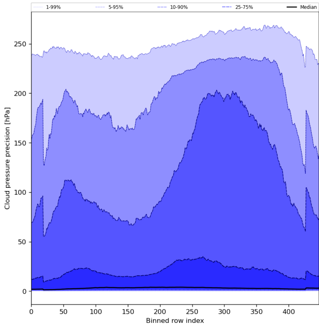
Figure 48: Along track statistics of “Cloud pressure precision” for 2023-09-05 to 2023-09-06
