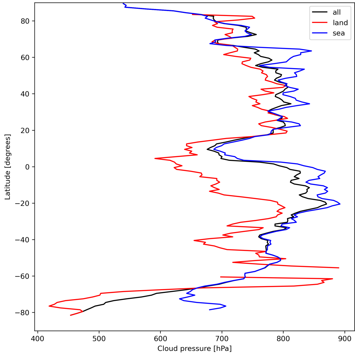
Figure 13: Zonal average of “Cloud pressure” for 2023-09-05 to 2023-09-06.
