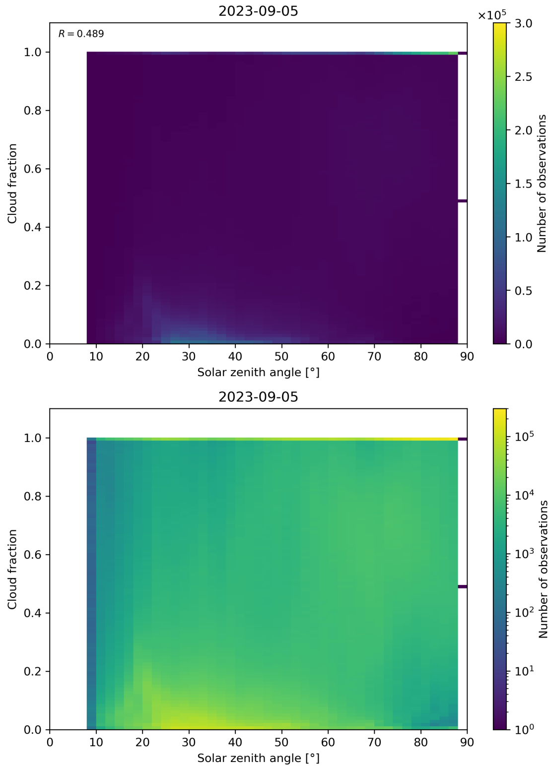
Figure 121: Scatter density plot of “Solar zenith angle” against “Cloud fraction” for 2023-09-05 to 2023-09-06.
