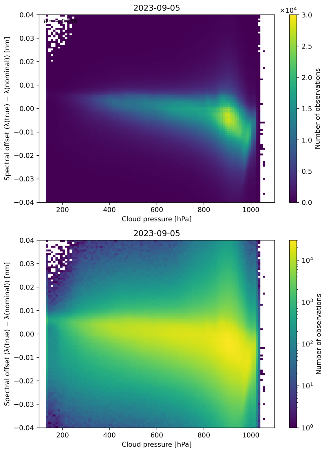
Figure 92: Scatter density plot of “Cloud pressure” against “Spectral offset ( \lambda(\text{true}) - \lambda(\text{nominal}) )” for 2023-09-05 to 2023-09-06.
