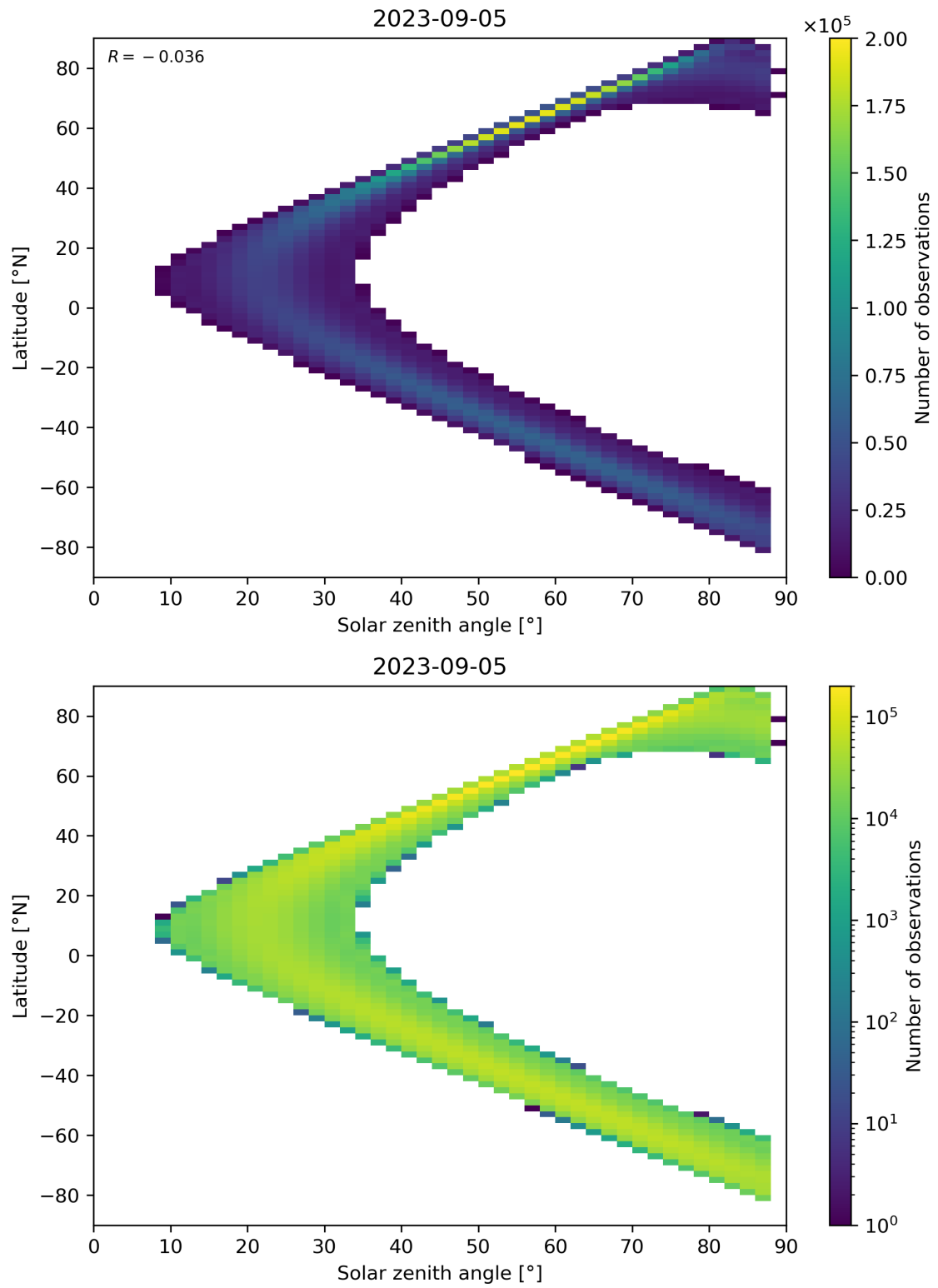
Figure 124: Scatter density plot of “Solar zenith angle” against “Latitude” for 2023-09-05 to 2023-09-06.
