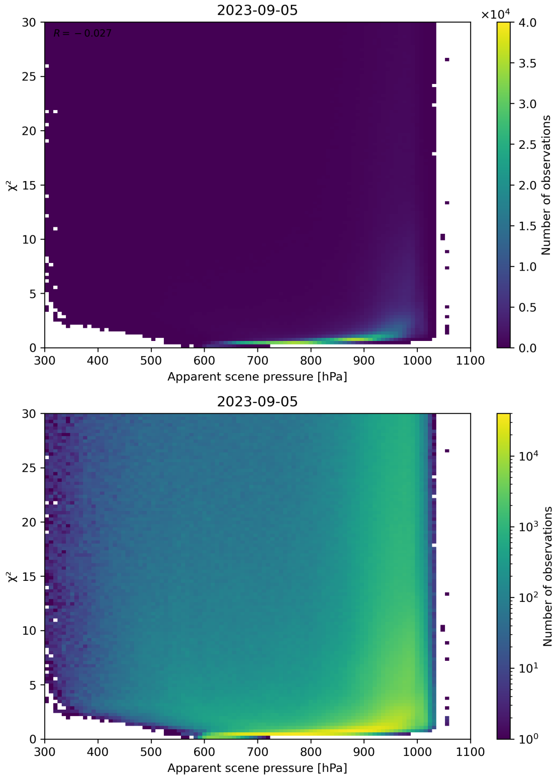
Figure 63: Scatter density plot of “Apparent scene pressure” against “ \chi^2 ” for 2023-09-05 to 2023-09-06.
