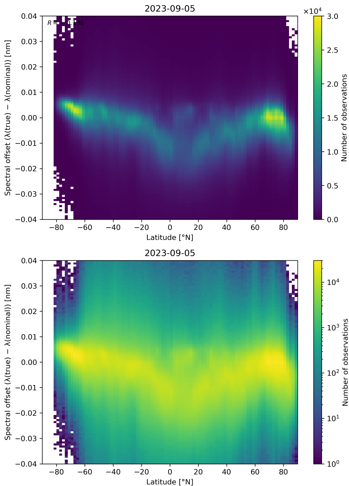
Figure 105: Scatter density plot of “Latitude” against “Spectral offset ( \lambda(\text{true}) - \lambda(\text{nominal}) )” for 2023-09-05 to 2023-09-06.
