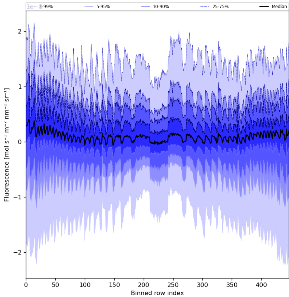
Figure 57: Along track statistics of “Fluorescence” for 2023-09-05 to 2023-09-06
