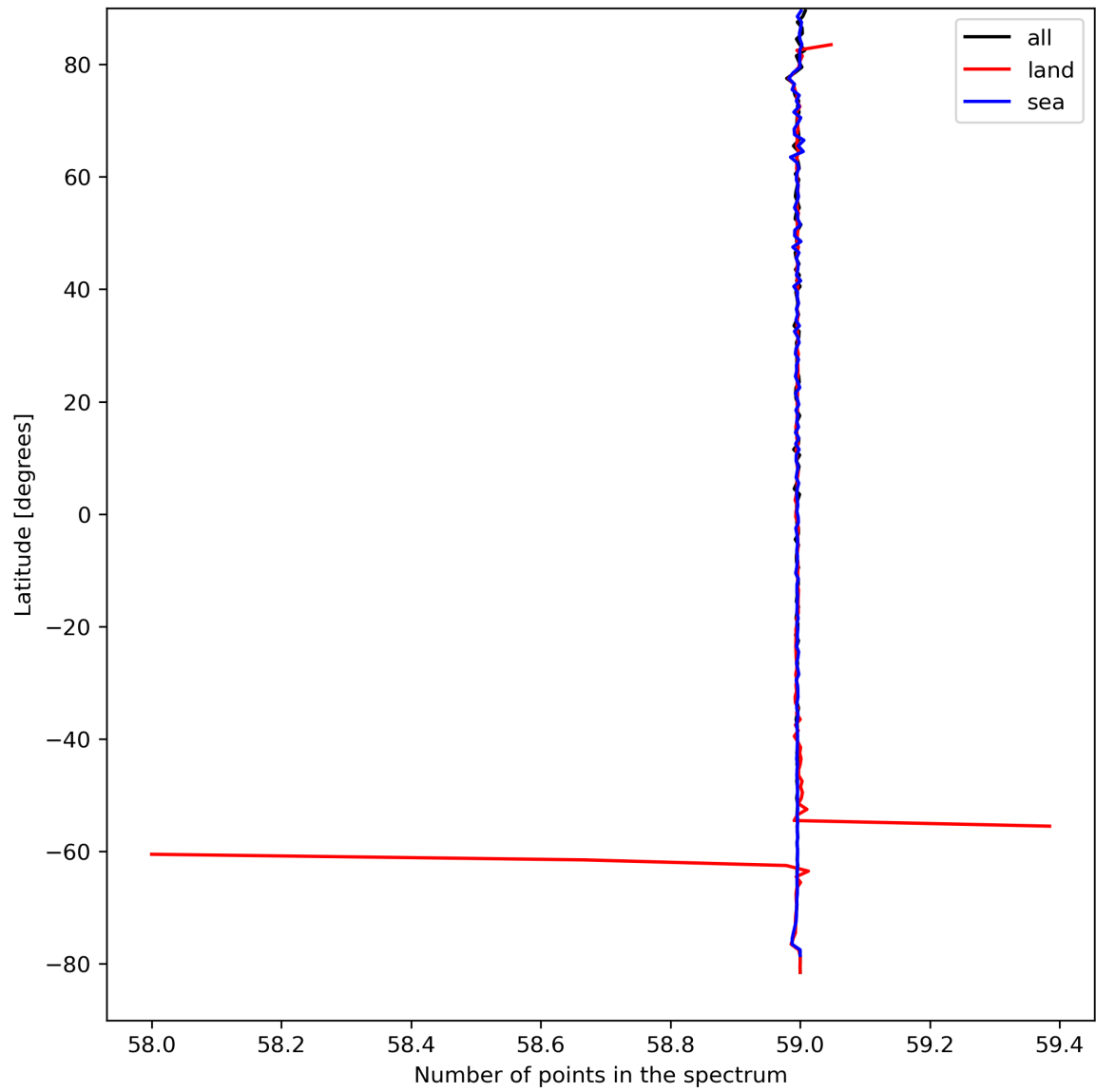
Figure 27: Zonal average of “Number of points in the spectrum” for 2023-09-05 to 2023-09-06.
