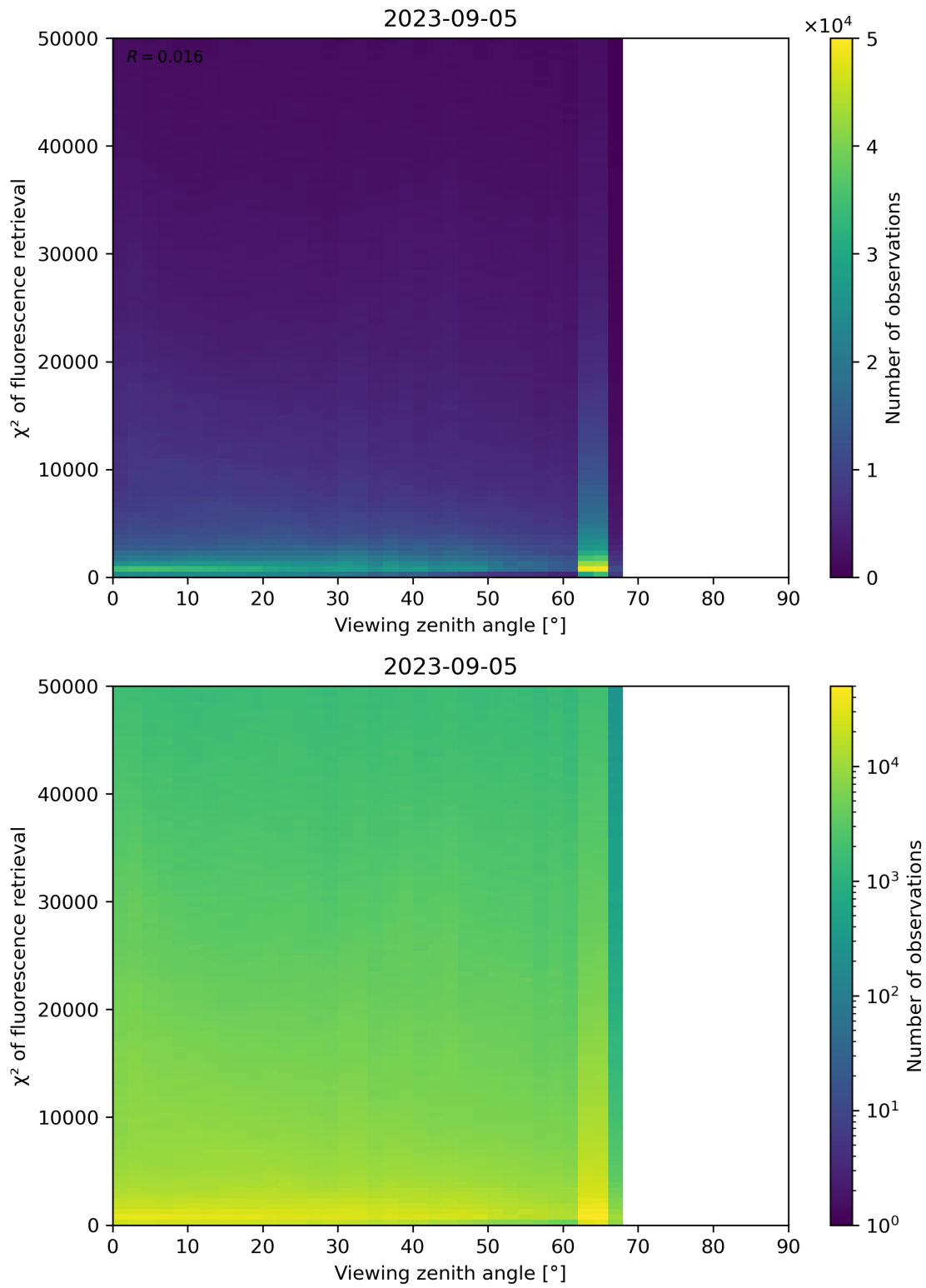
Figure 131: Scatter density plot of “Viewing zenith angle” against “ \chi^2 of fluorescence retrieval” for 2023-09-05 to 2023-09-06.
