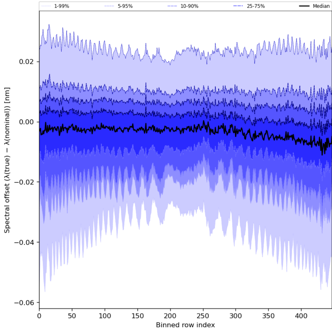
Figure 62: Along track statistics of “Spectral offset ( \lambda(\text{true}) - \lambda(\text{nominal}) )” for 2023-09-05 to 2023-09-06
