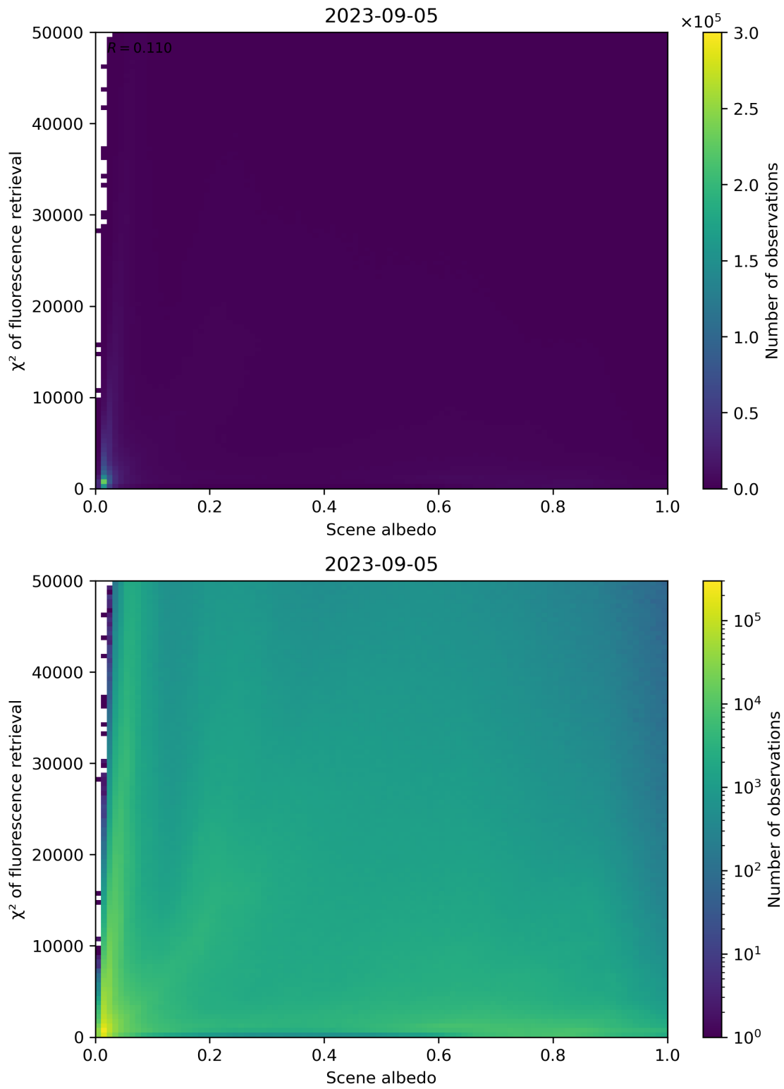
Figure 113: Scatter density plot of “Scene albedo” against “ \chi^2 of fluorescence retrieval” for 2023-09-05 to 2023-09-06.
