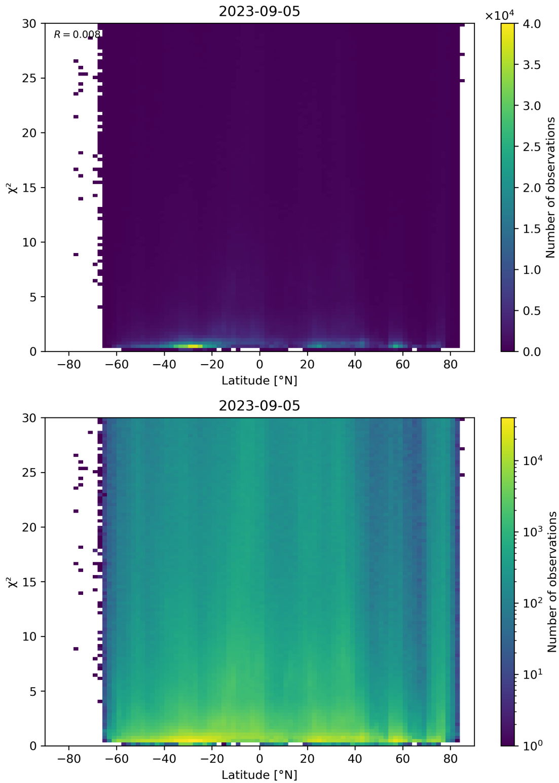
Figure 97: Scatter density plot of “Latitude” against “ \chi^2 ” for 2023-09-05 to 2023-09-06.
