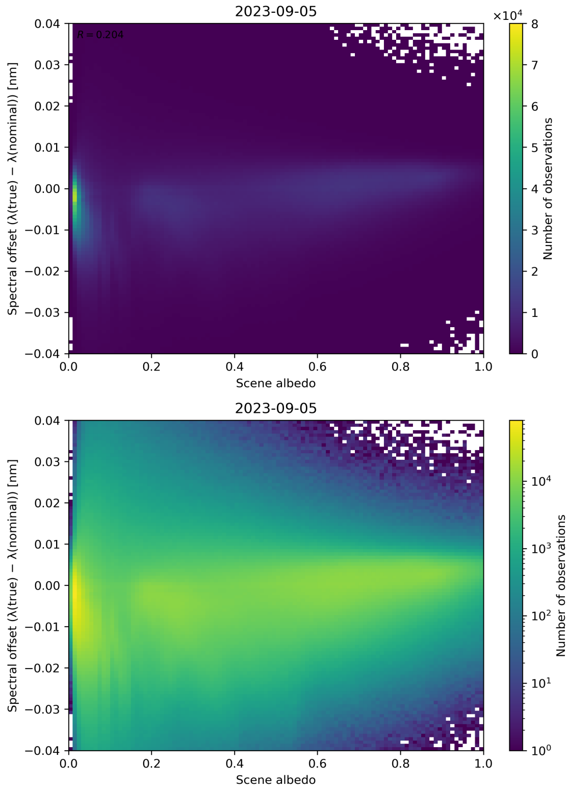
Figure 117: Scatter density plot of “Scene albedo” against “Spectral offset ( \lambda(\text{true}) - \lambda(\text{nominal}) )” for 2023-09-05 to 2023-09-06.
