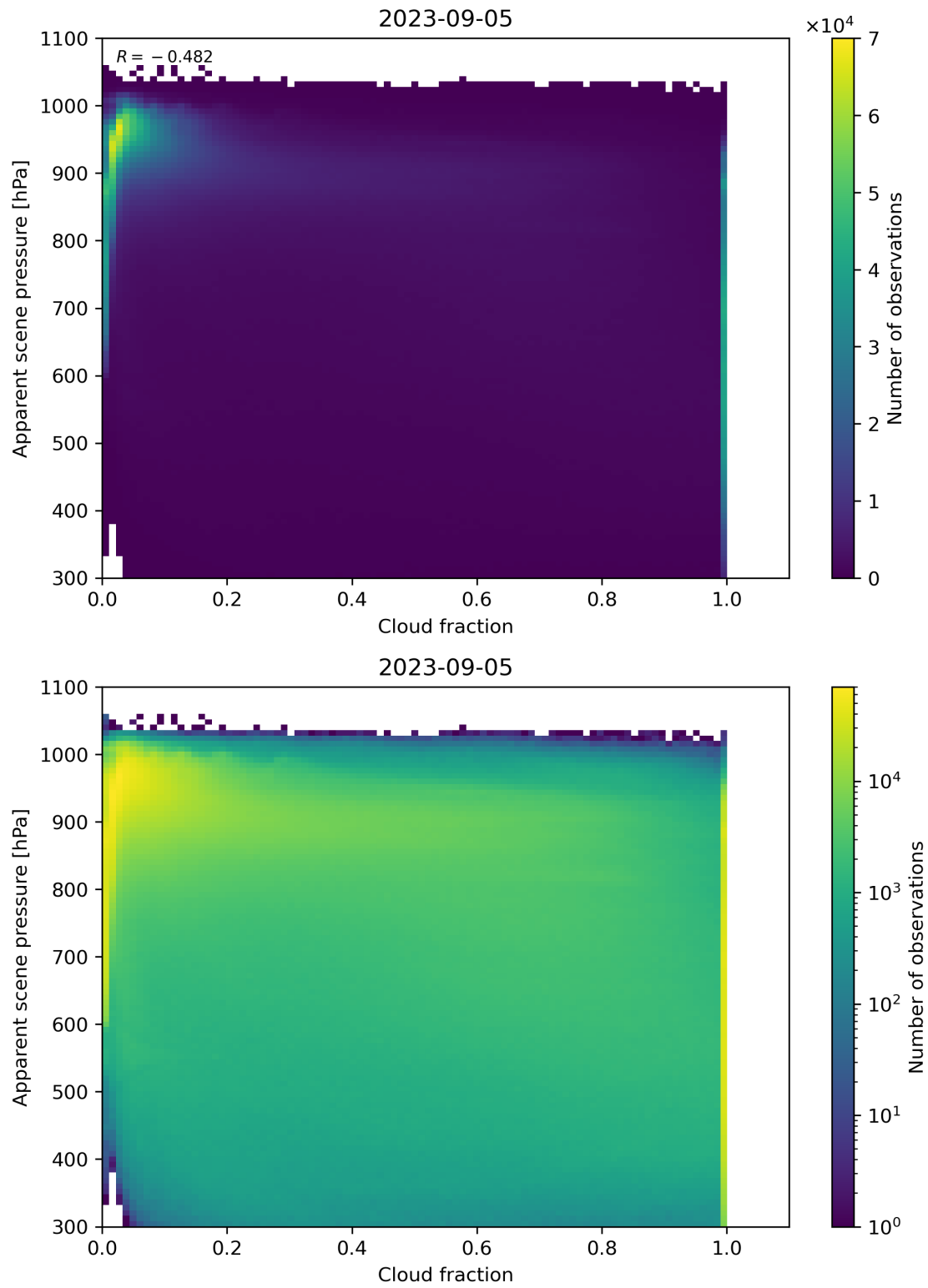
Figure 76: Scatter density plot of “Cloud fraction” against “Apparent scene pressure” for 2023-09-05 to 2023-09-06.
