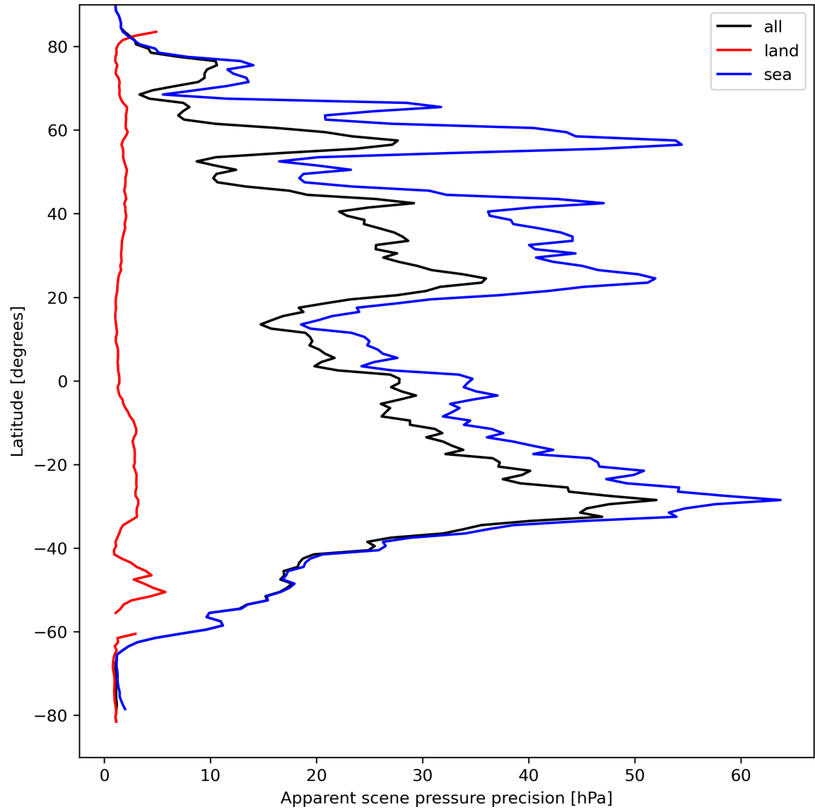
Figure 20: Zonal average of “Apparent scene pressure precision” for 2023-09-05 to 2023-09-06.
