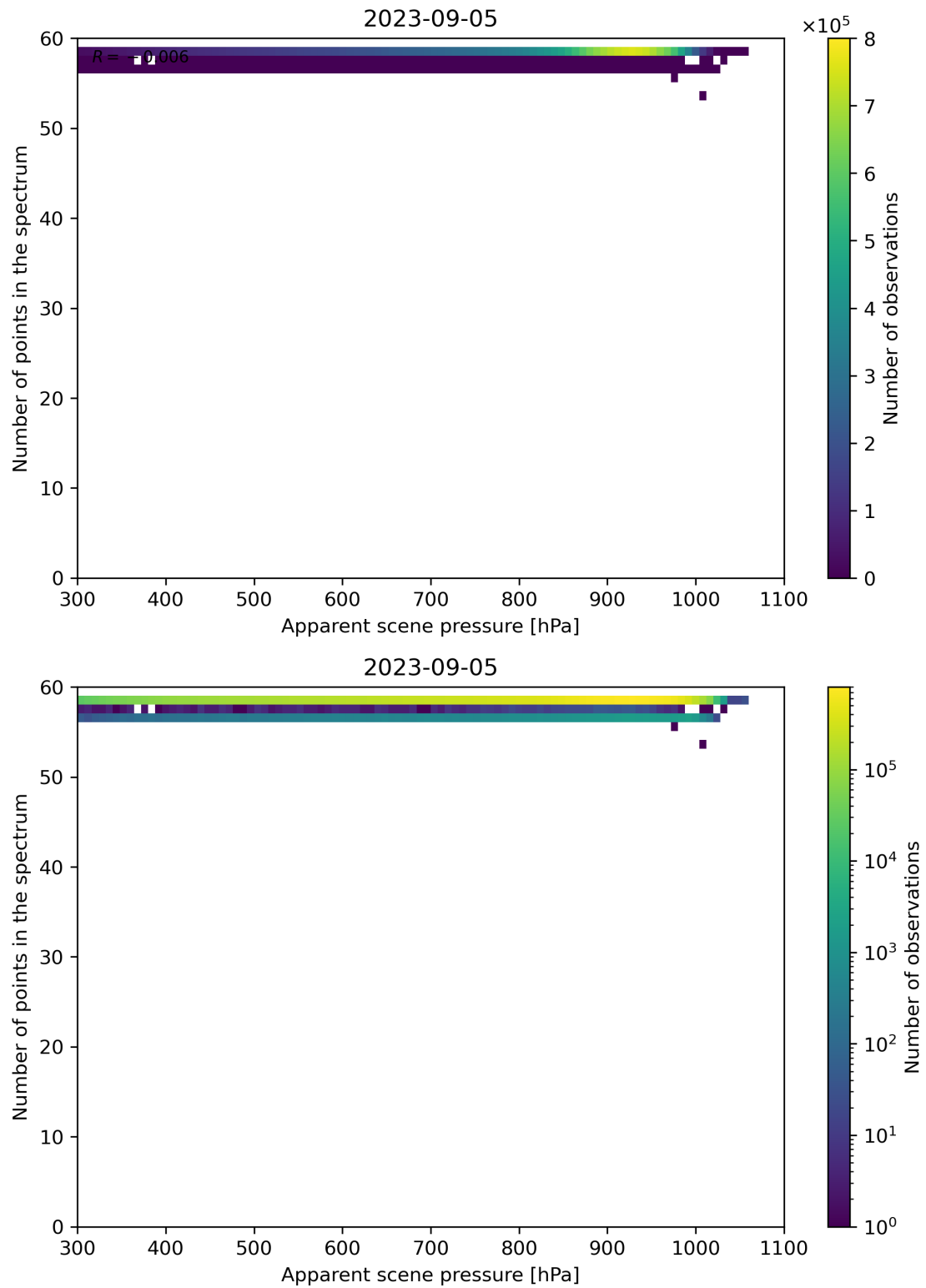
Figure 67: Scatter density plot of “Apparent scene pressure” against “Number of points in the spectrum” for 2023-09-05 to 2023-09-06.
