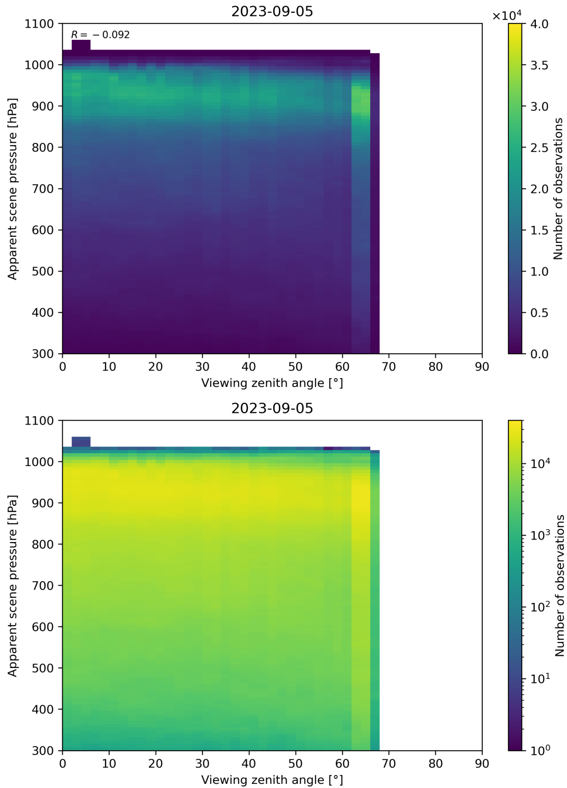
Figure 129: Scatter density plot of “Viewing zenith angle” against “Apparent scene pressure” for 2023-09-05 to 2023-09-06.
