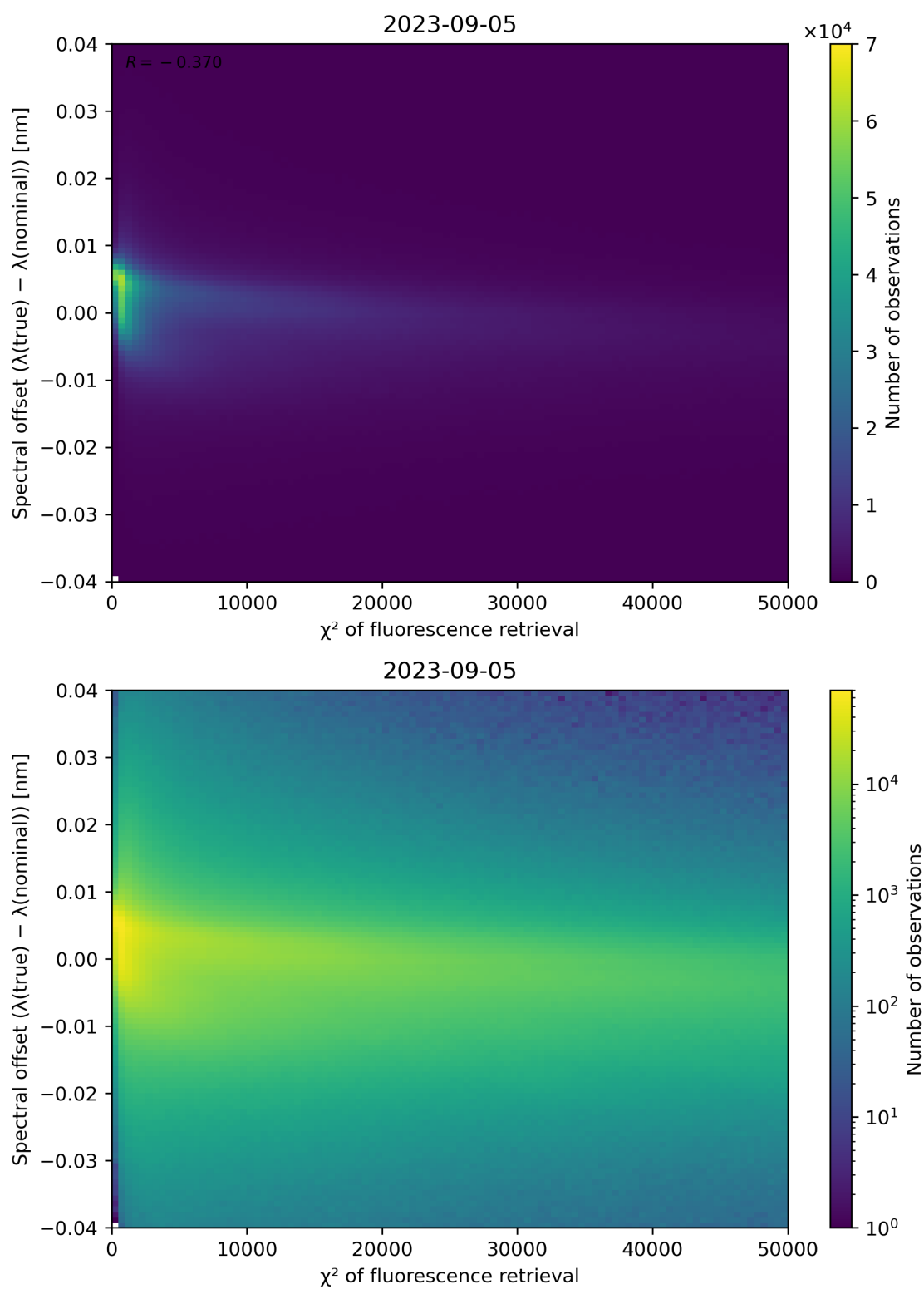
Figure 72: Scatter density plot of " \chi^2 of fluorescence retrieval" against "Spectral offset ( \lambda(\text{true}) - \lambda(\text{nominal})) " for 2023-09-05 to 2023-09-06.
