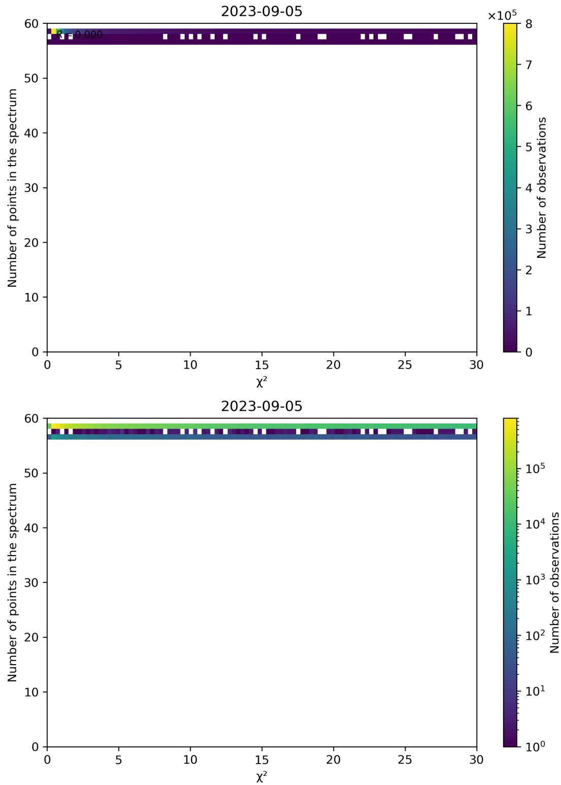
Figure 74: Scatter density plot of “ \chi^2 ” against “Number of points in the spectrum” for 2023-09-05 to 2023-09-06.
