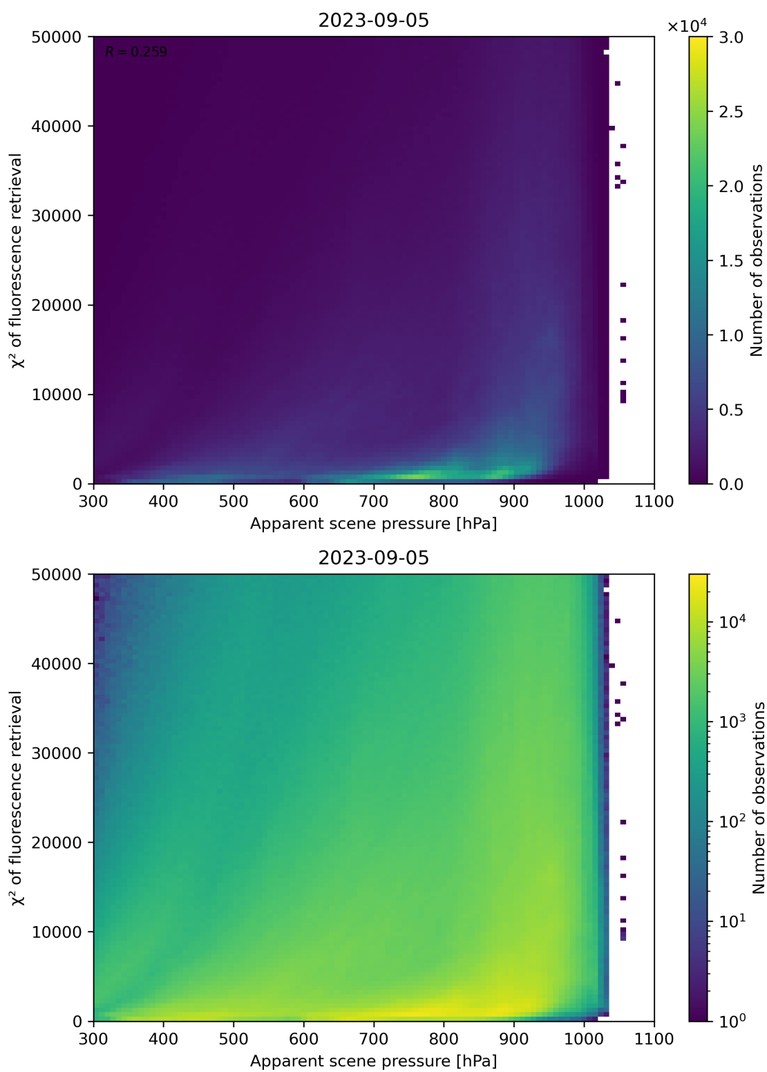
Figure 64: Scatter density plot of “Apparent scene pressure” against “ \chi^2 of fluorescence retrieval” for 2023-09-05 to 2023-09-06.
