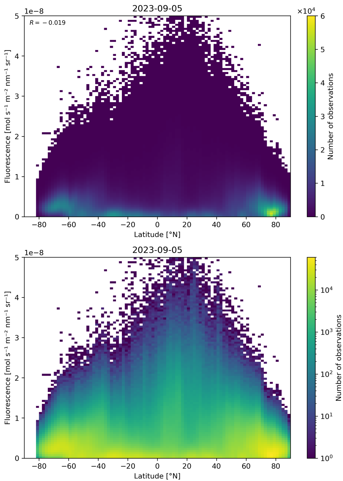
Figure 101: Scatter density plot of “Latitude” against “Fluorescence” for 2023-09-05 to 2023-09-06.
