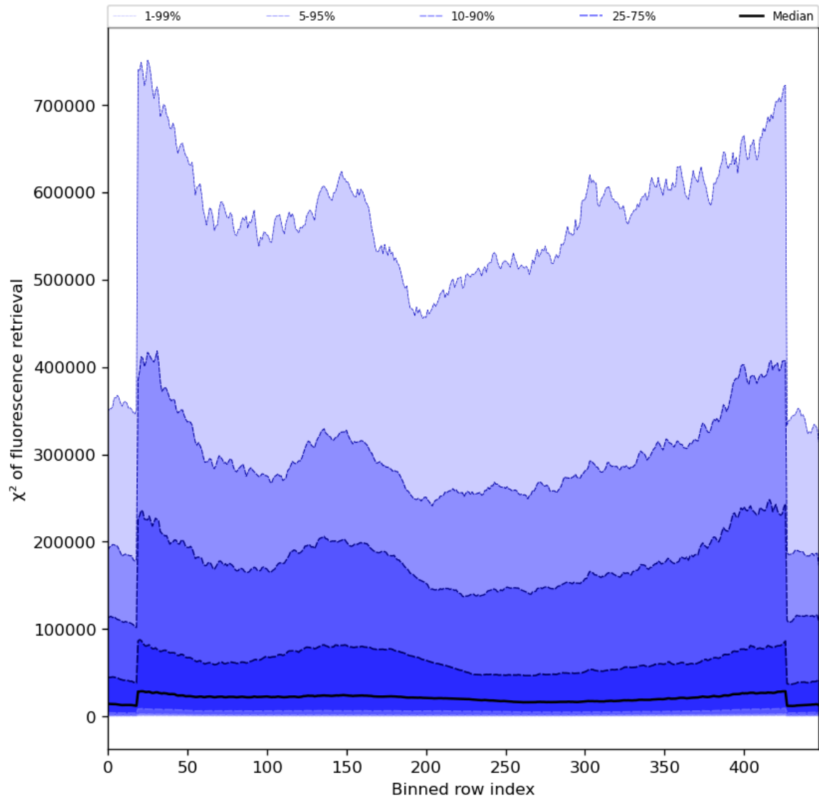
Figure 59: Along track statistics of “ \chi^2 of fluorescence retrieval” for 2023-09-05 to 2023-09-06
