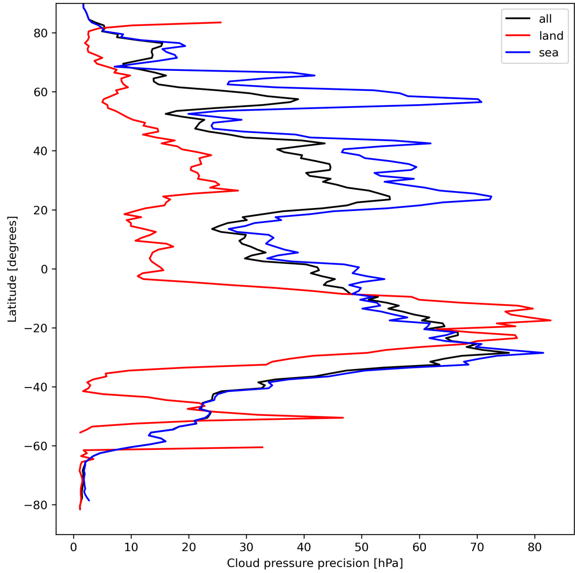
Figure 14: Zonal average of “Cloud pressure precision” for 2023-09-05 to 2023-09-06.
