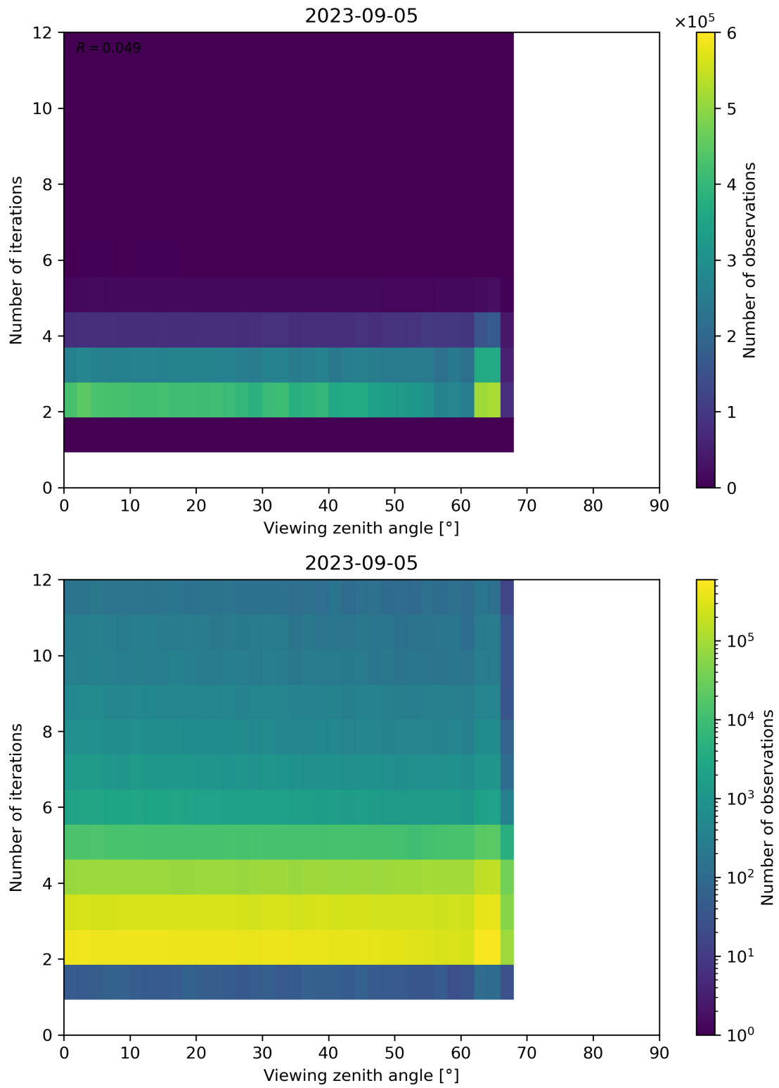
Figure 136: Scatter density plot of “Viewing zenith angle” against “Number of iterations” for 2023-09-05 to 2023-09-06.
