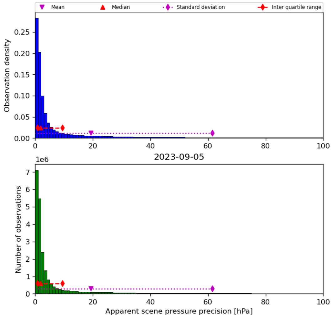
Figure 37: Histogram of “Apparent scene pressure precision” for 2023-09-05 to 2023-09-06
