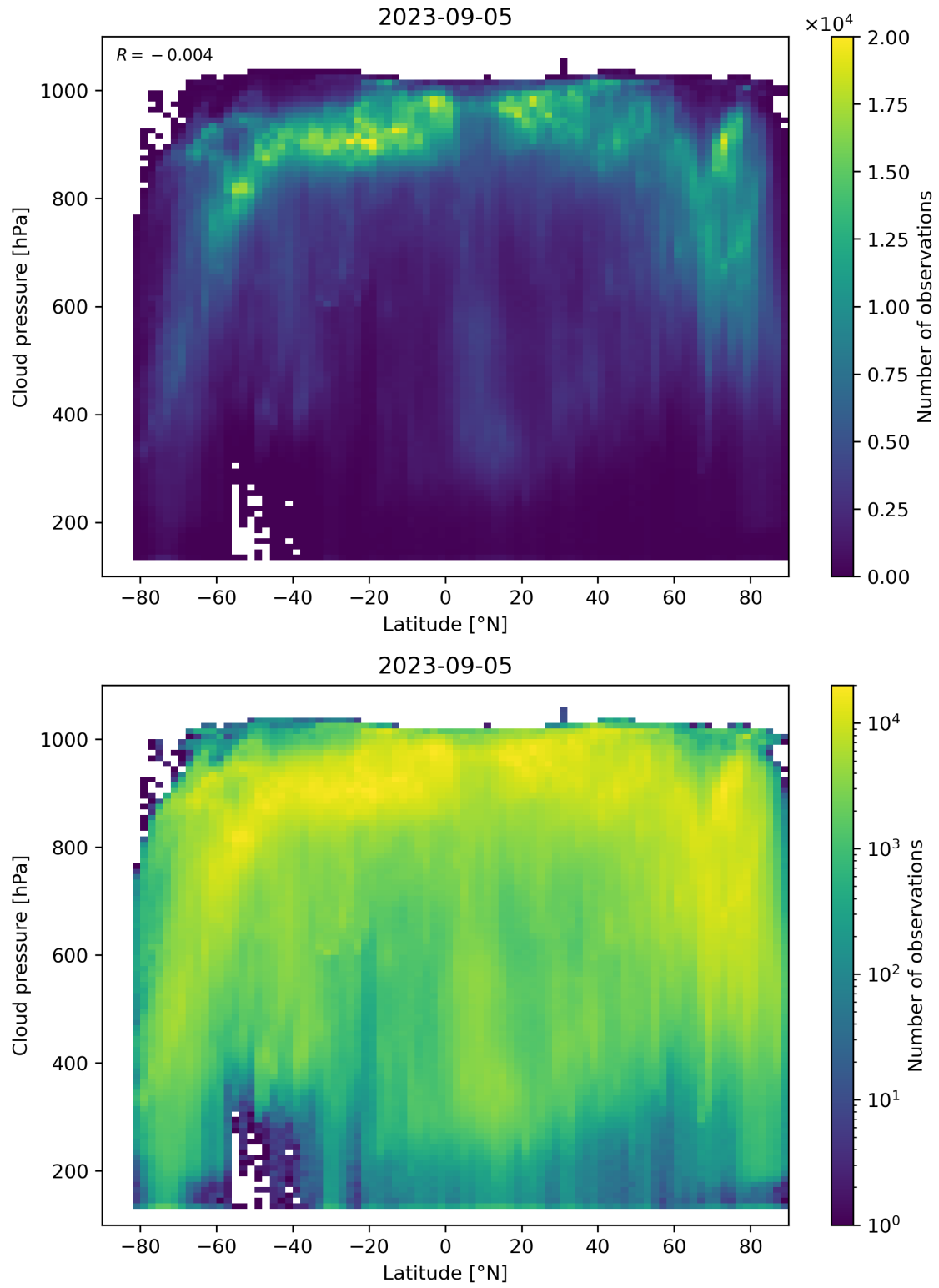
Figure 100: Scatter density plot of “Latitude” against “Cloud pressure” for 2023-09-05 to 2023-09-06.
