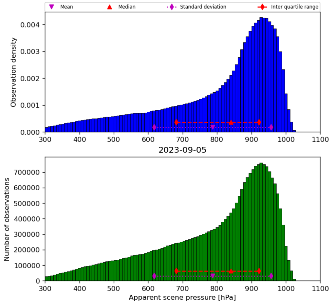
Figure 36: Histogram of “Apparent scene pressure” for 2023-09-05 to 2023-09-06
