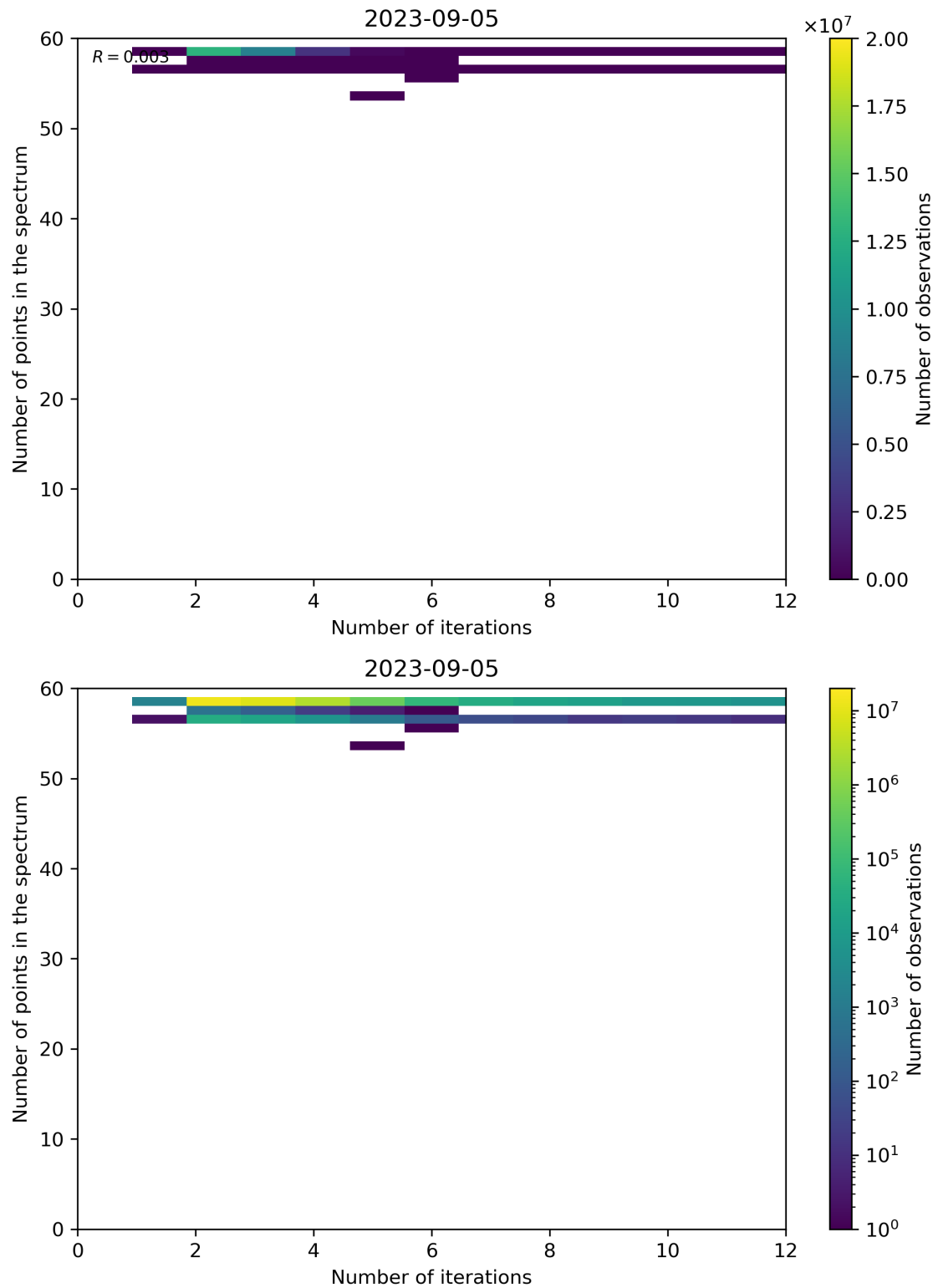
Figure 108: Scatter density plot of “Number of iterations” against “Number of points in the spectrum” for 2023-09-05 to 2023-09-06.
