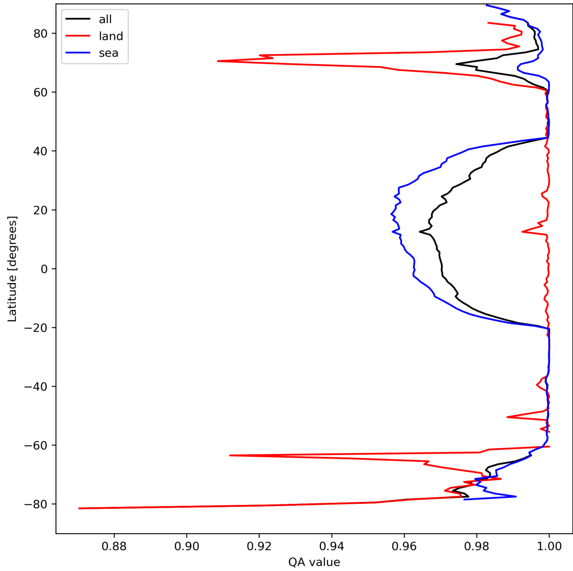
Figure 12: Zonal average of "QA value" for 2023-09-05 to 2023-09-06.
