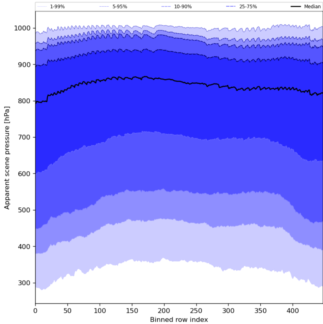
Figure 53: Along track statistics of “Apparent scene pressure” for 2023-09-05 to 2023-09-06
