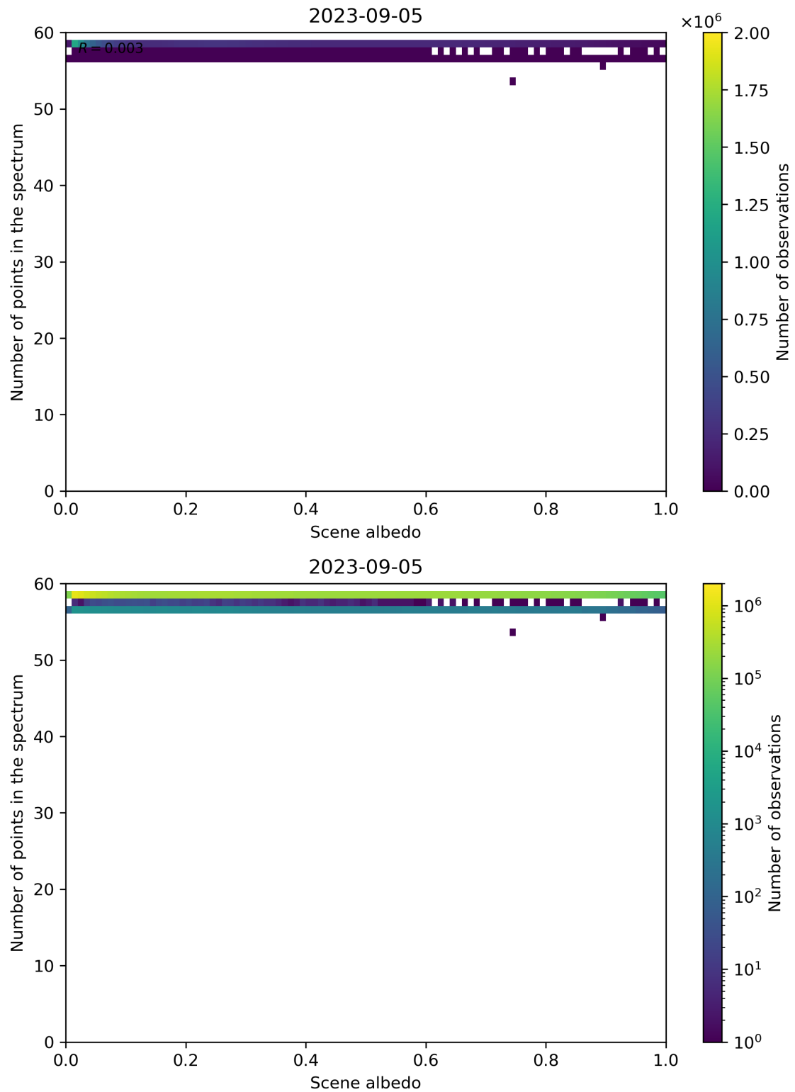
Figure 116: Scatter density plot of “Scene albedo” against “Number of points in the spectrum” for 2023-09-05 to 2023-09-06.
