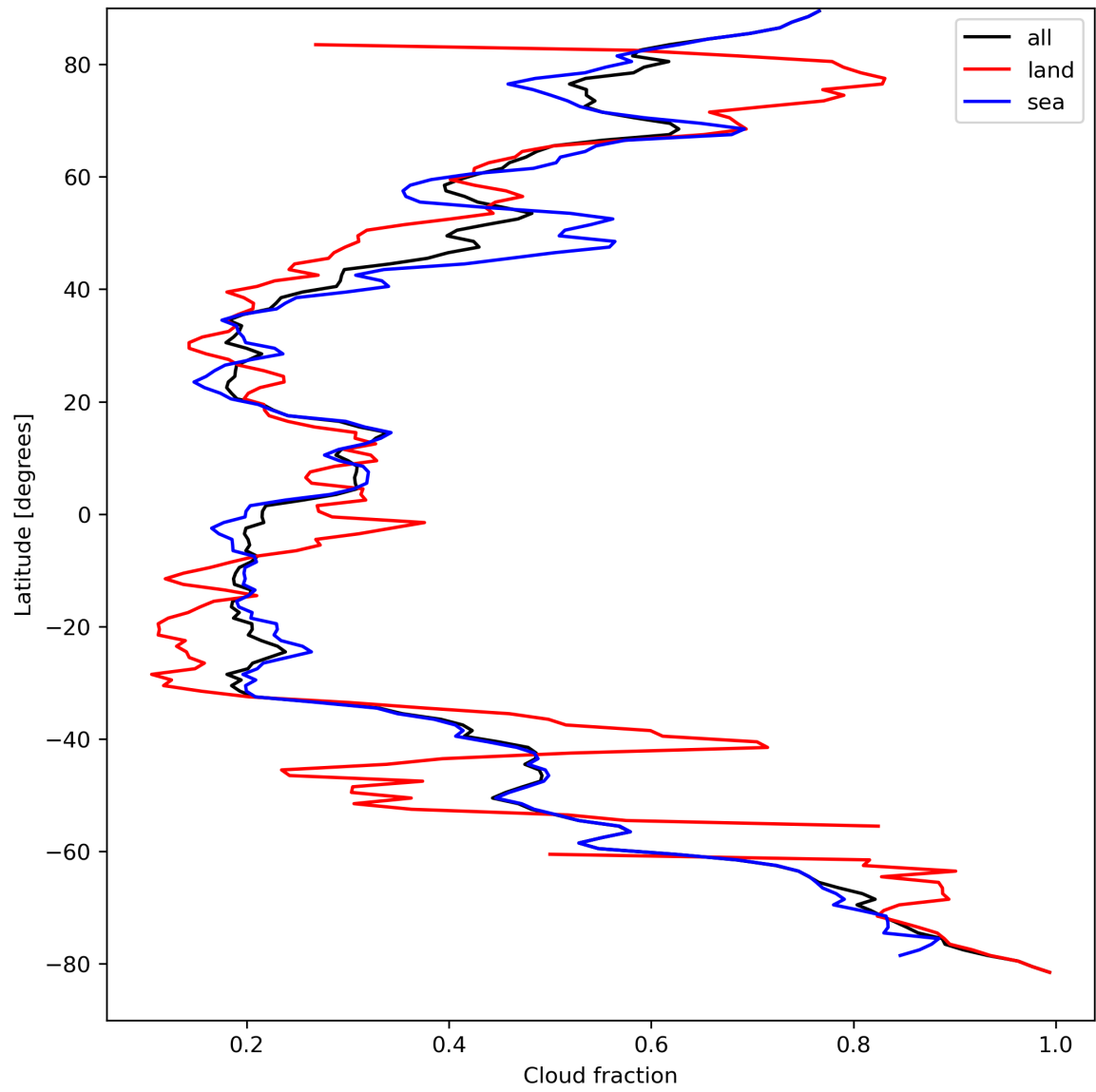
Figure 15: Zonal average of “Cloud fraction” for 2023-09-05 to 2023-09-06.
