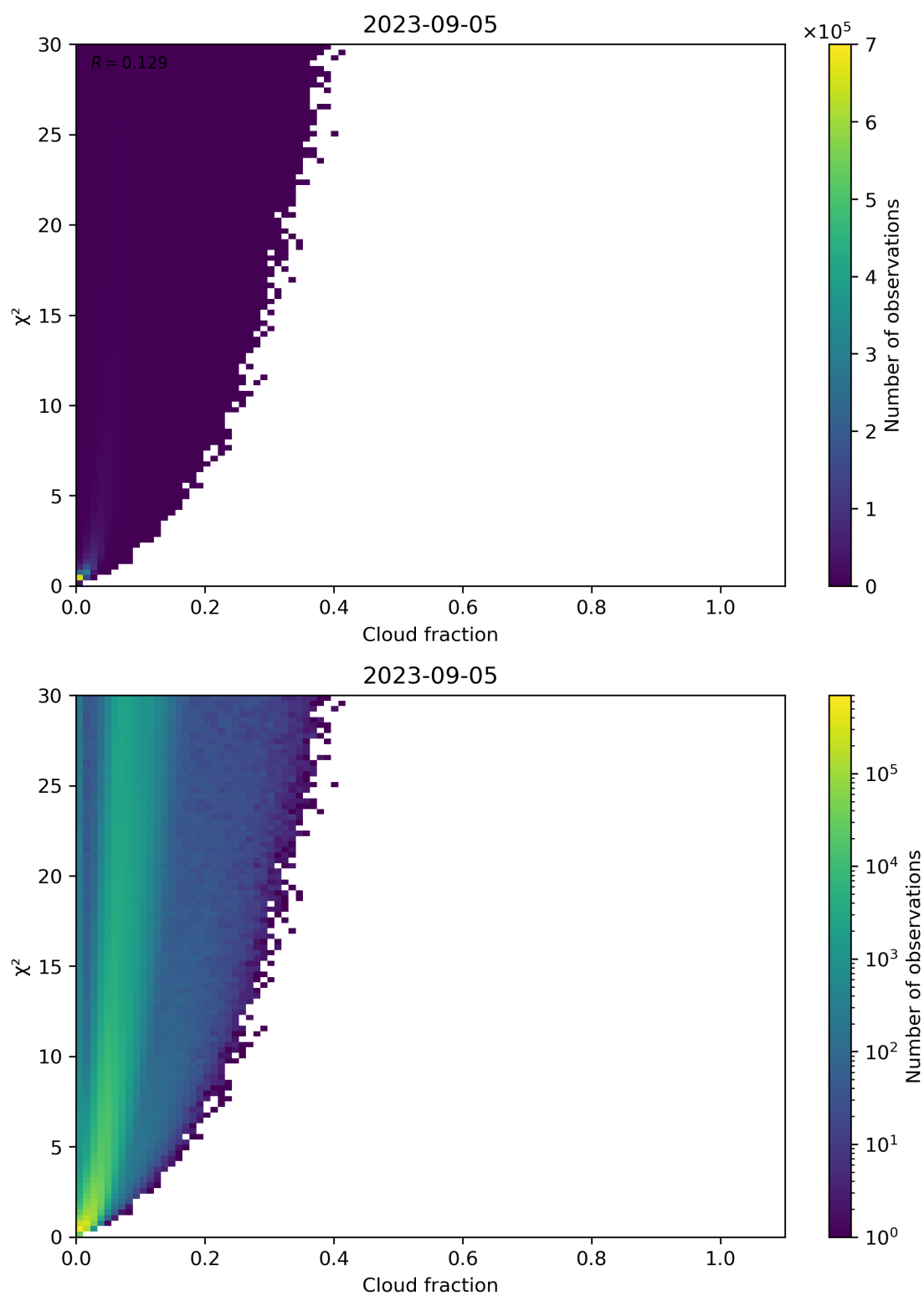
Figure 77: Scatter density plot of “Cloud fraction” against “ \chi^2 ” for 2023-09-05 to 2023-09-06.
