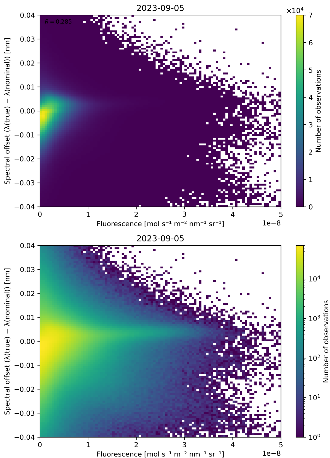
Figure 95: Scatter density plot of “Fluorescence” against “Spectral offset ( \lambda(\text{true}) - \lambda(\text{nominal}) )” for 2023-09-05 to 2023-09-06.
