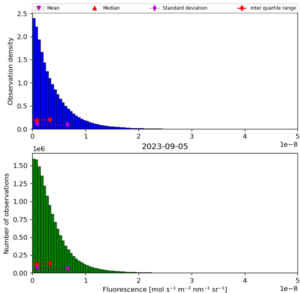
Figure 40: Histogram of “Fluorescence” for 2023-09-05 to 2023-09-06
