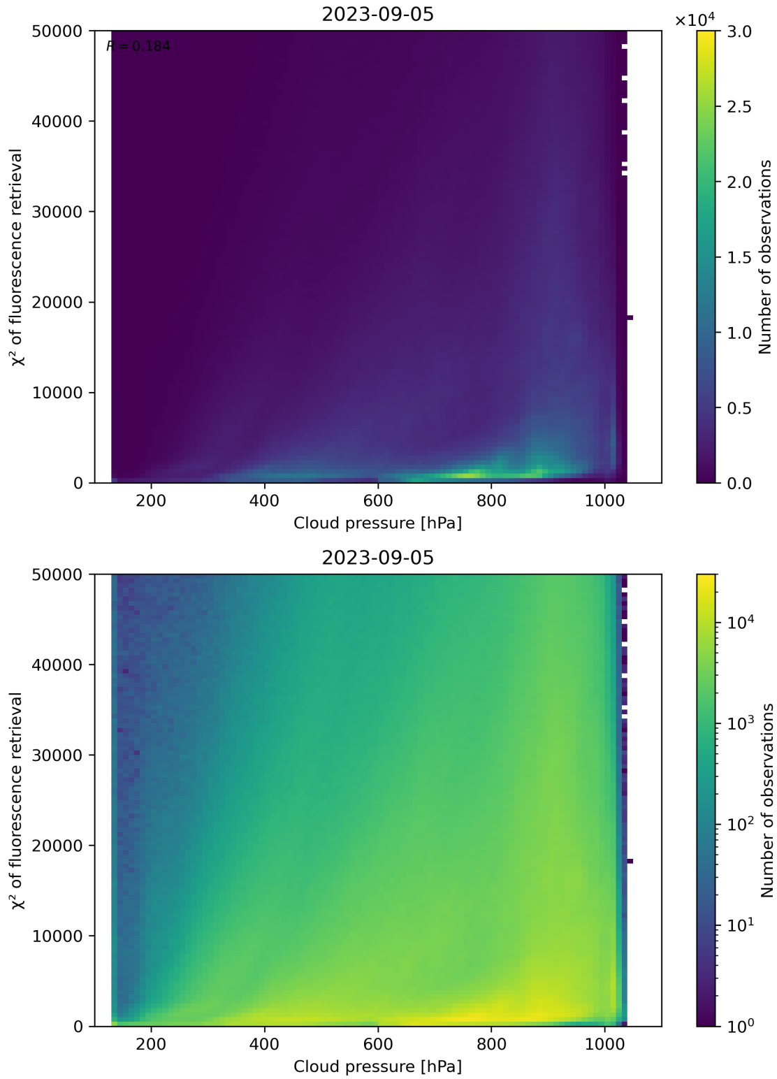
Figure 86: Scatter density plot of “Cloud pressure” against “ \chi^2 of fluorescence retrieval” for 2023-09-05 to 2023-09-06.
