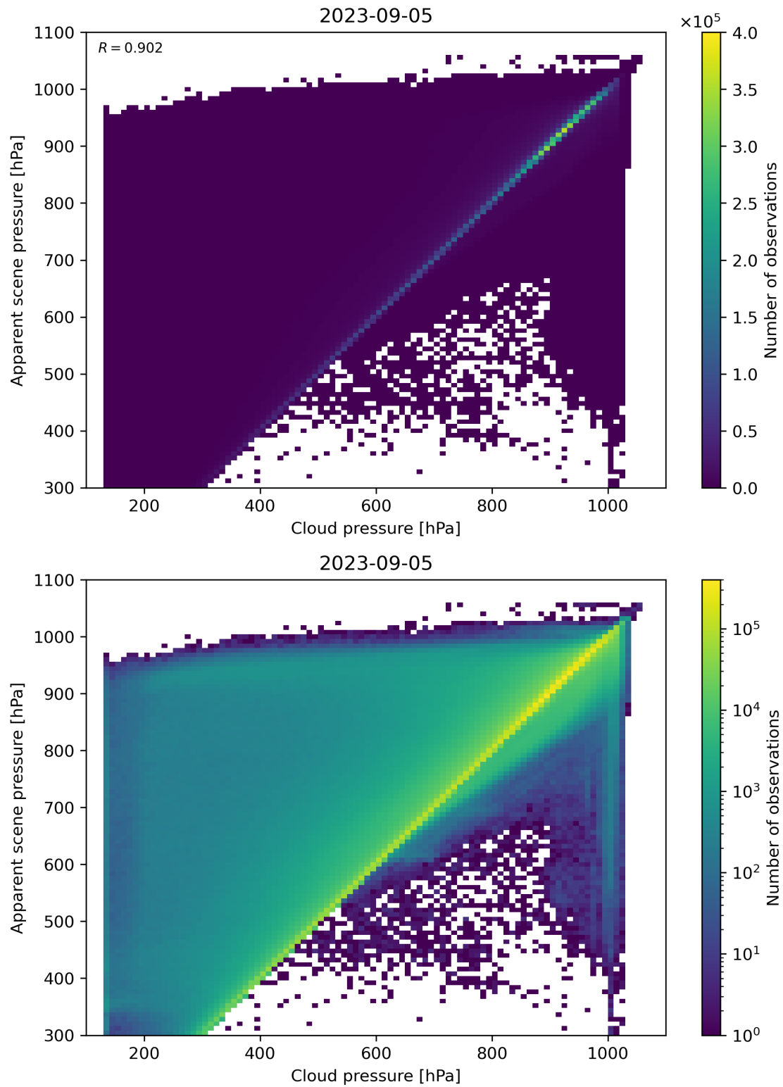
Figure 84: Scatter density plot of “Cloud pressure” against “Apparent scene pressure” for 2023-09-05 to 2023-09-06.
