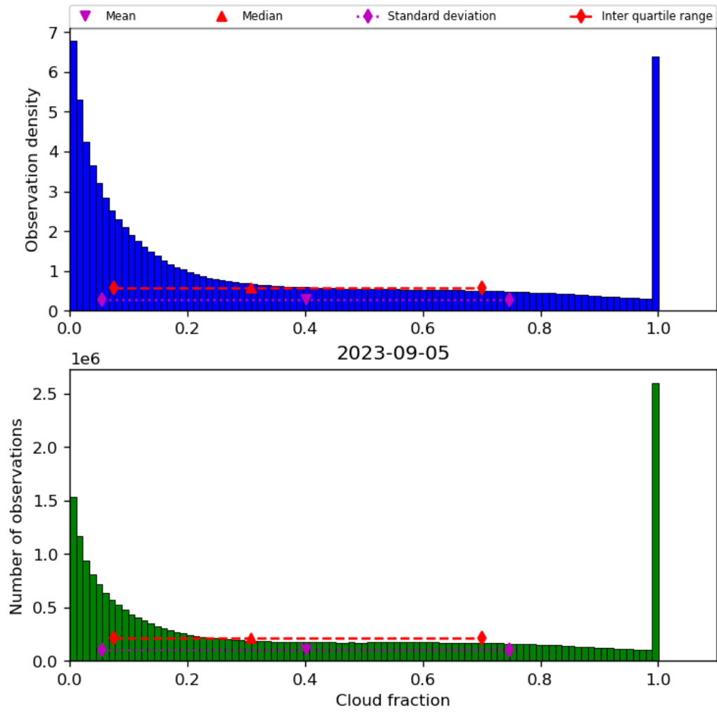
Figure 32: Histogram of “Cloud fraction” for 2023-09-05 to 2023-09-06
