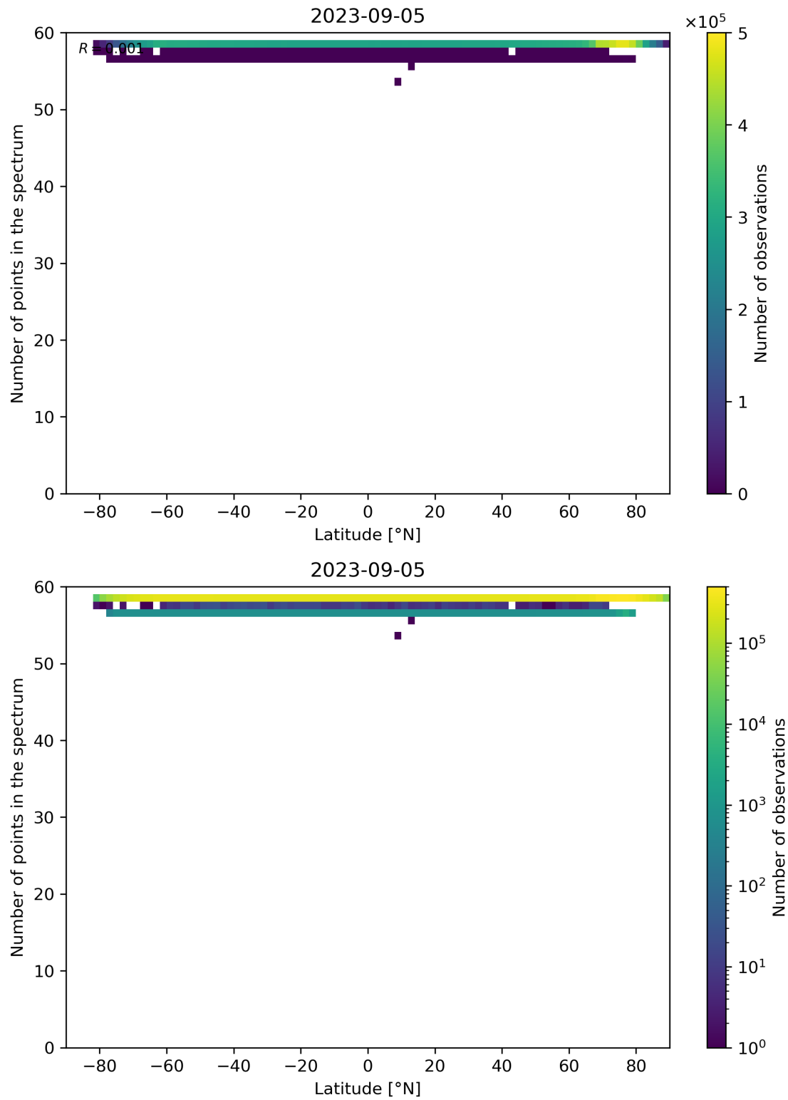
Figure 103: Scatter density plot of “Latitude” against “Number of points in the spectrum” for 2023-09-05 to 2023-09-06.
