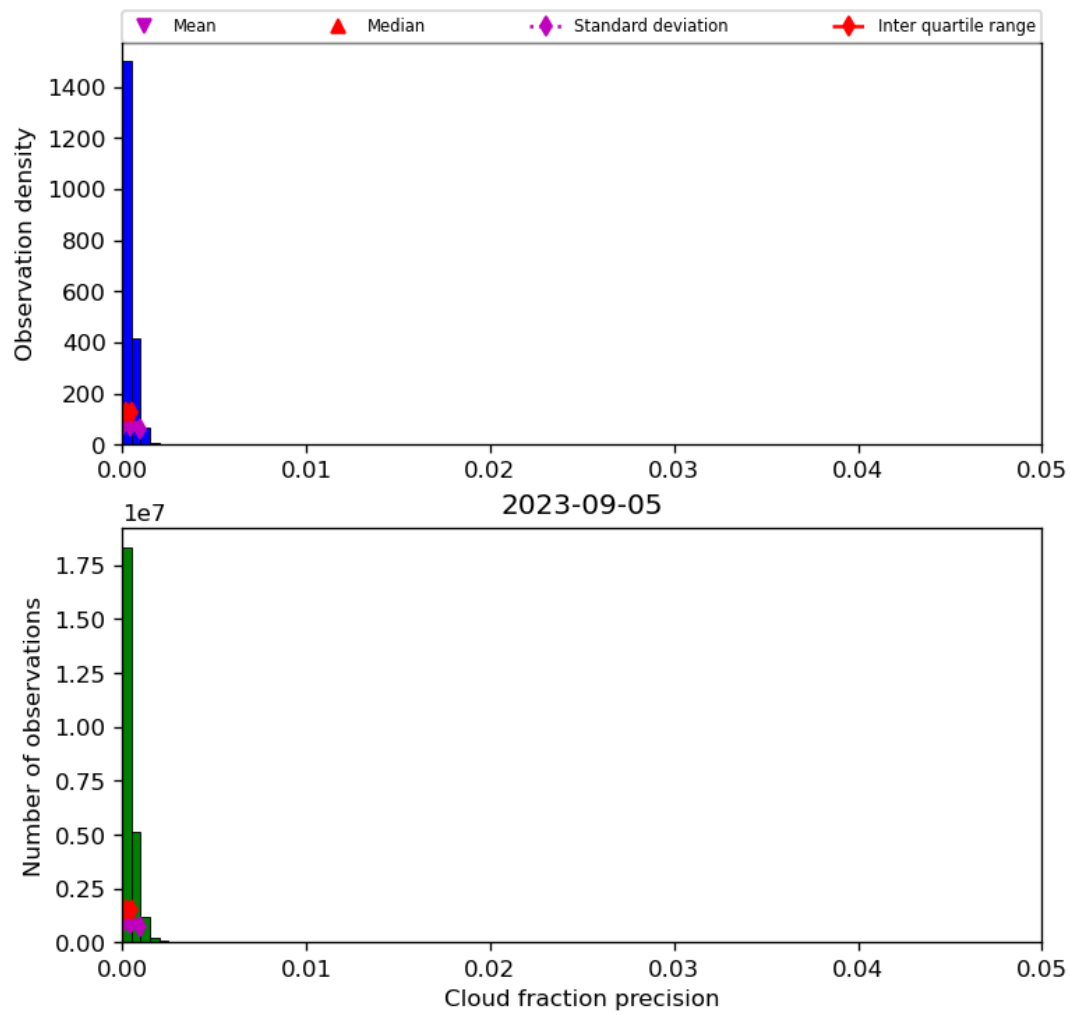
Figure 33: Histogram of “Cloud fraction precision” for 2023-09-05 to 2023-09-06
