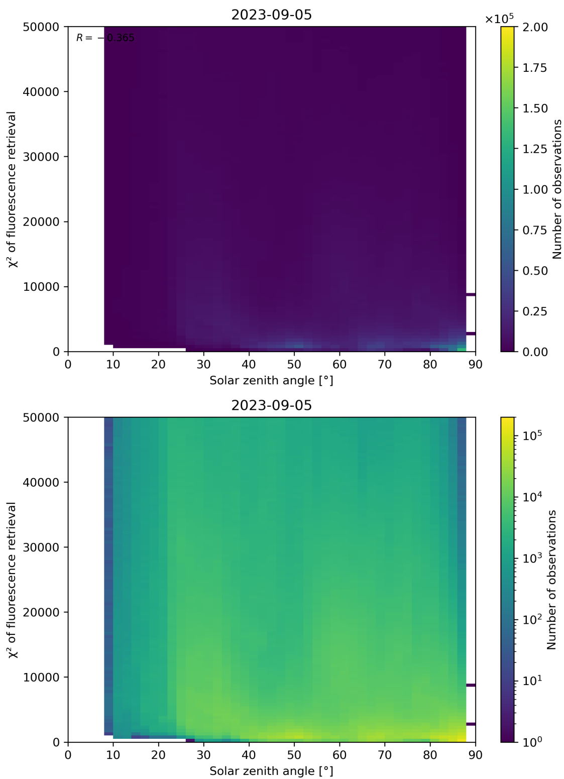
Figure 120: Scatter density plot of “Solar zenith angle” against “ \chi^2 of fluorescence retrieval” for 2023-09-05 to 2023-09-06.
