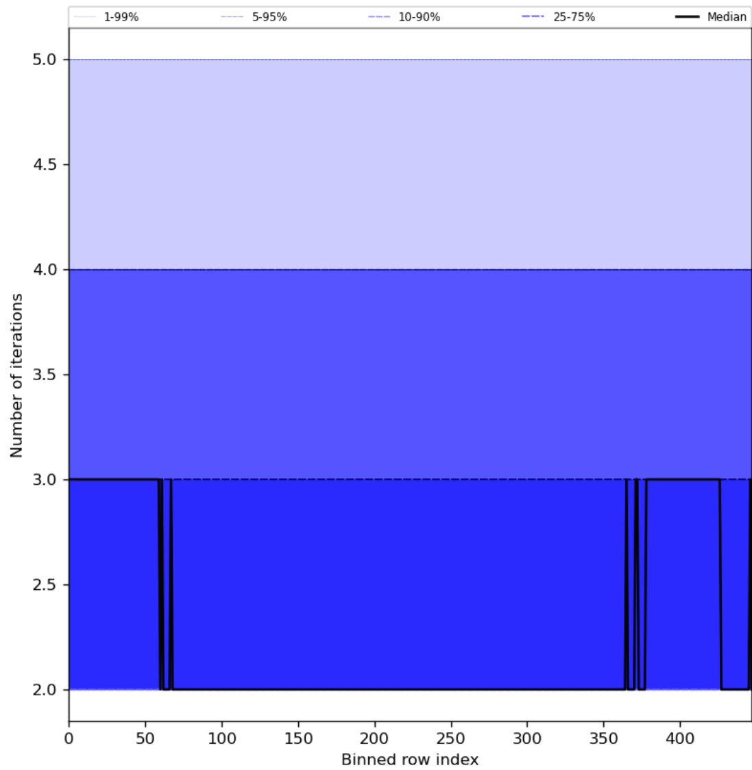
Figure 56: Along track statistics of “Number of iterations” for 2023-09-05 to 2023-09-06
