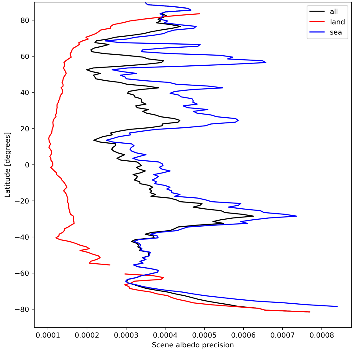
Figure 18: Zonal average of “Scene albedo precision” for 2023-09-05 to 2023-09-06.
