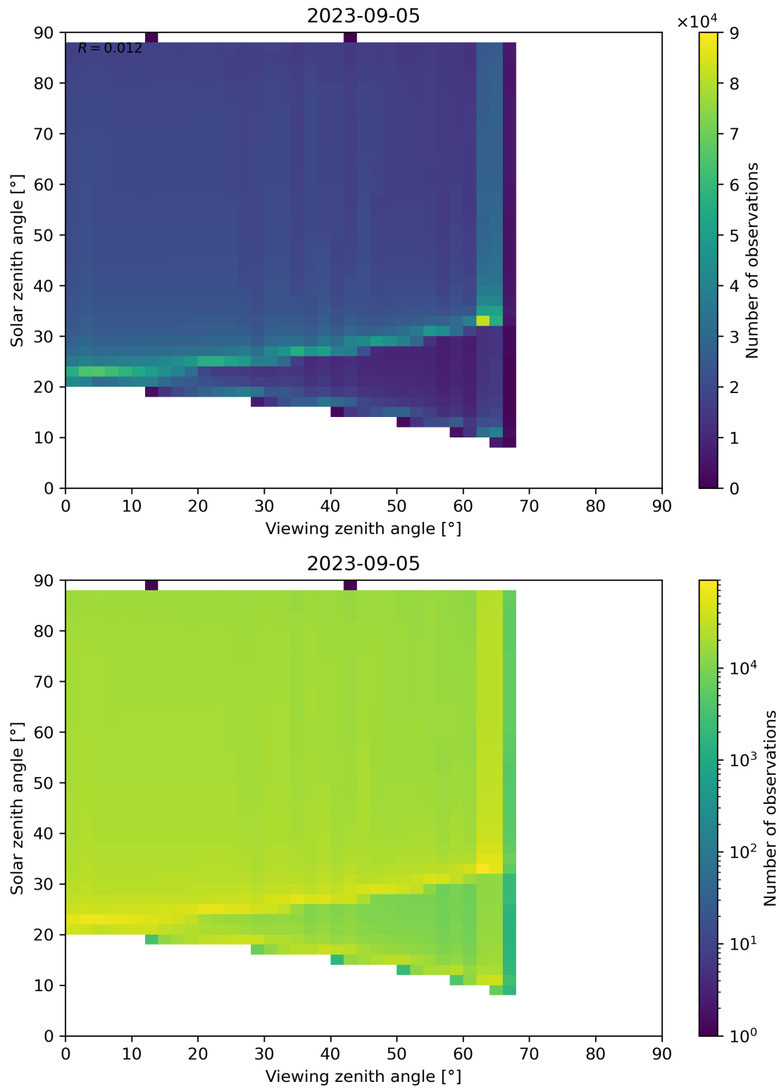
Figure 139: Scatter density plot of “Viewing zenith angle” against “Solar zenith angle” for 2023-09-05 to 2023-09-06.
