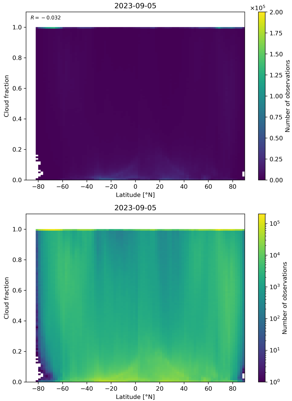
Figure 99: Scatter density plot of “Latitude” against “Cloud fraction” for 2023-09-05 to 2023-09-06.
