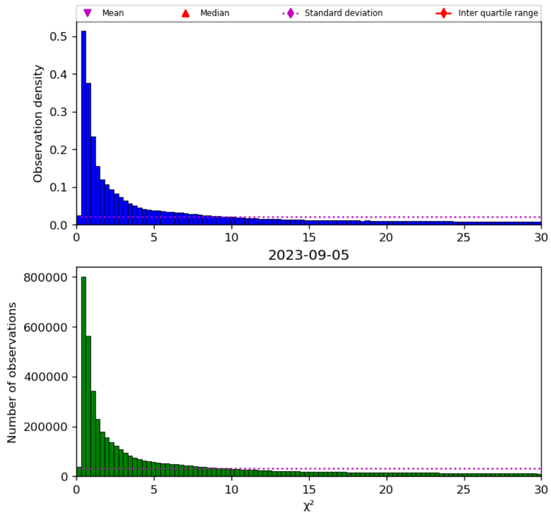
Figure 38: Histogram of " \chi^2 " for 2023-09-05 to 2023-09-06
