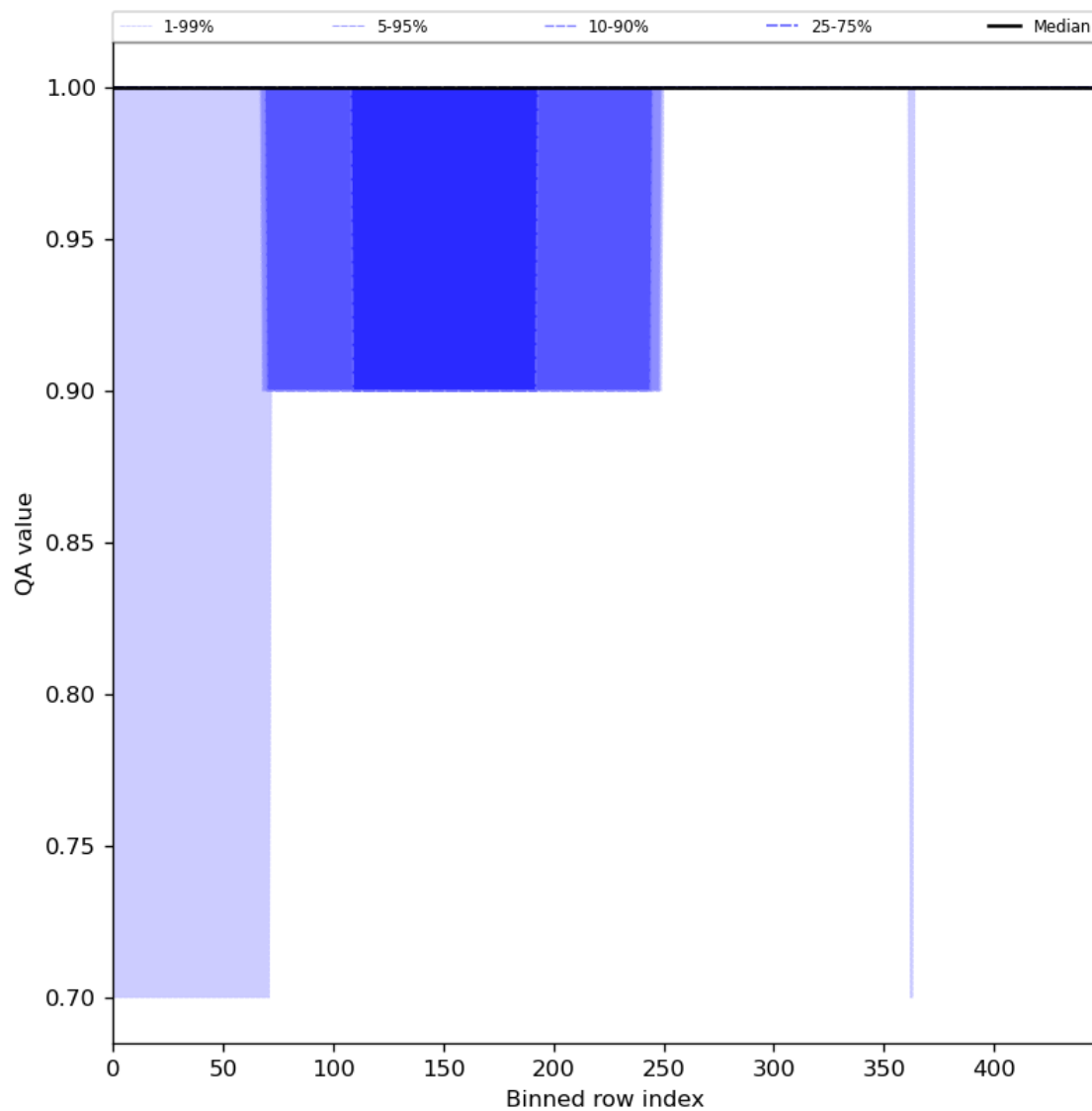
Figure 46: Along track statistics of “QA value” for 2023-09-05 to 2023-09-06
