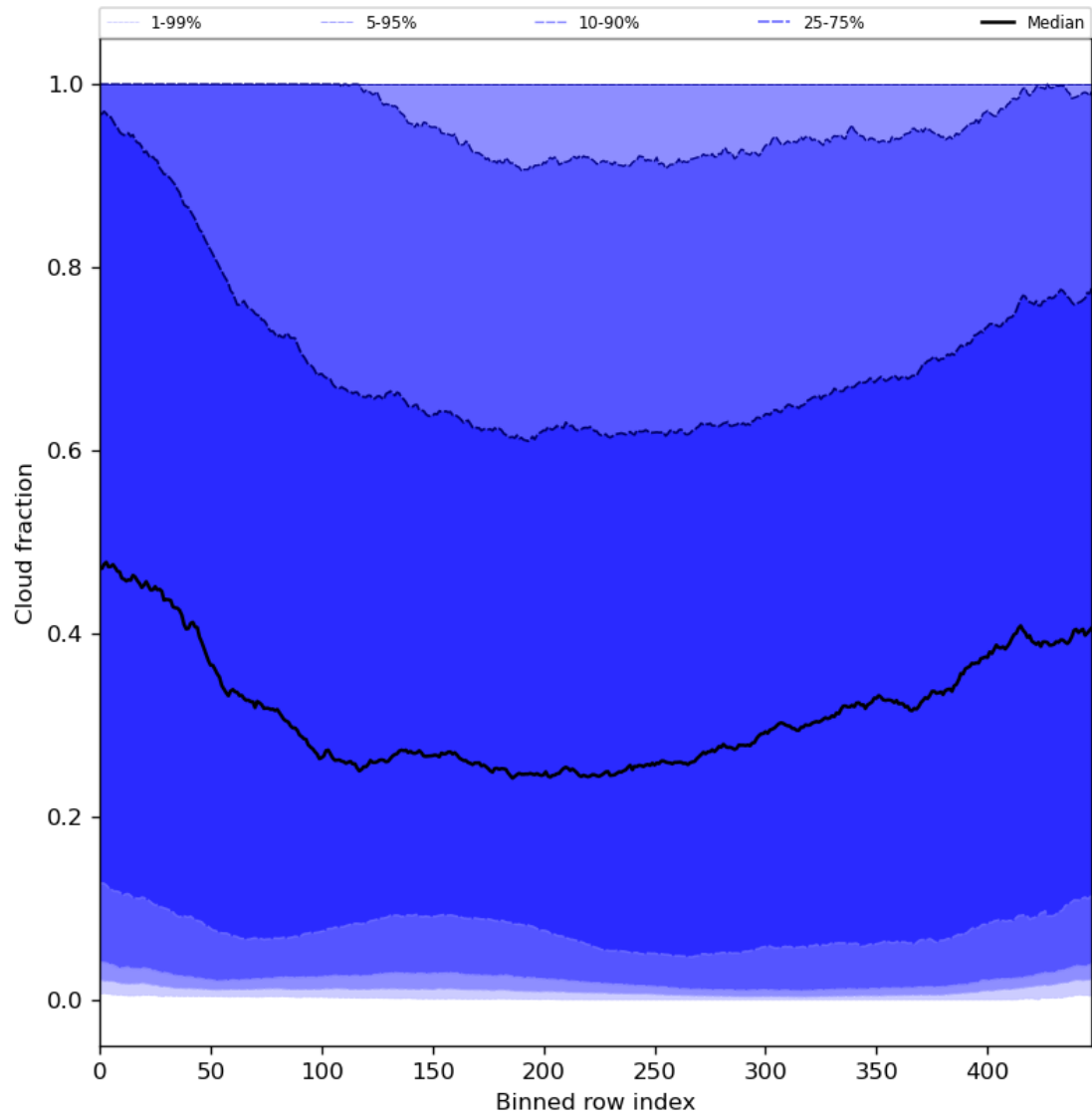
Figure 49: Along track statistics of “Cloud fraction” for 2023-09-05 to 2023-09-06
