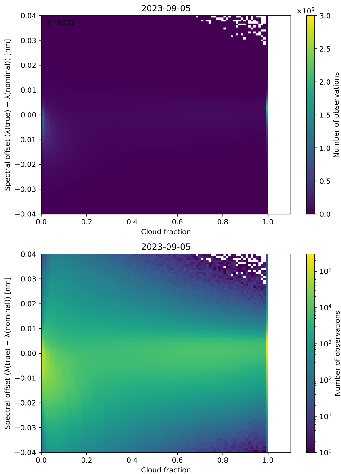
Figure 83: Scatter density plot of “Cloud fraction” against “Spectral offset ( \lambda(\text{true}) - \lambda(\text{nominal}) )” for 2023-09-05 to 2023-09-06.
