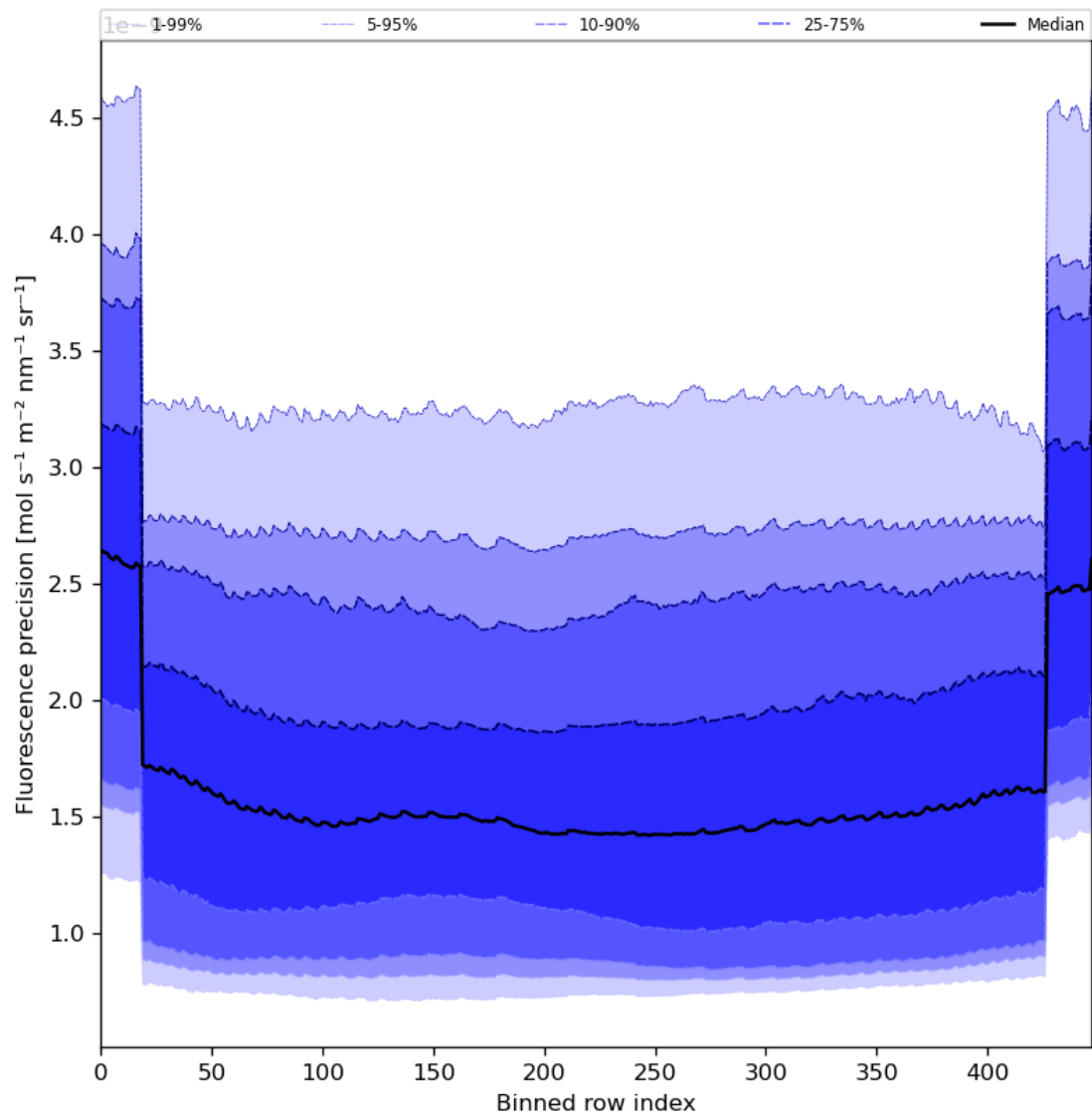
Figure 58: Along track statistics of “Fluorescence precision” for 2023-09-05 to 2023-09-06
