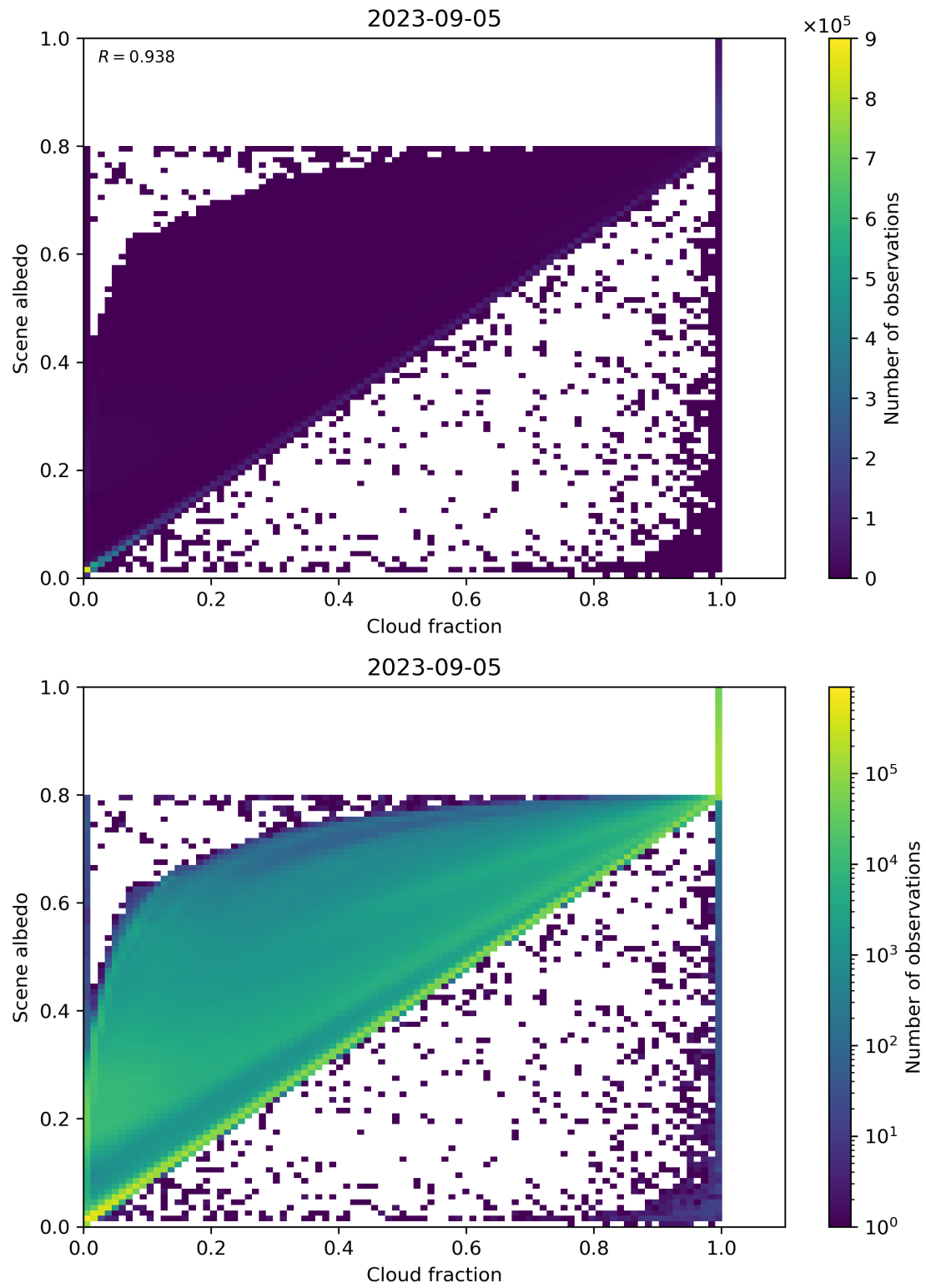
Figure 82: Scatter density plot of “Cloud fraction” against “Scene albedo” for 2023-09-05 to 2023-09-06.
