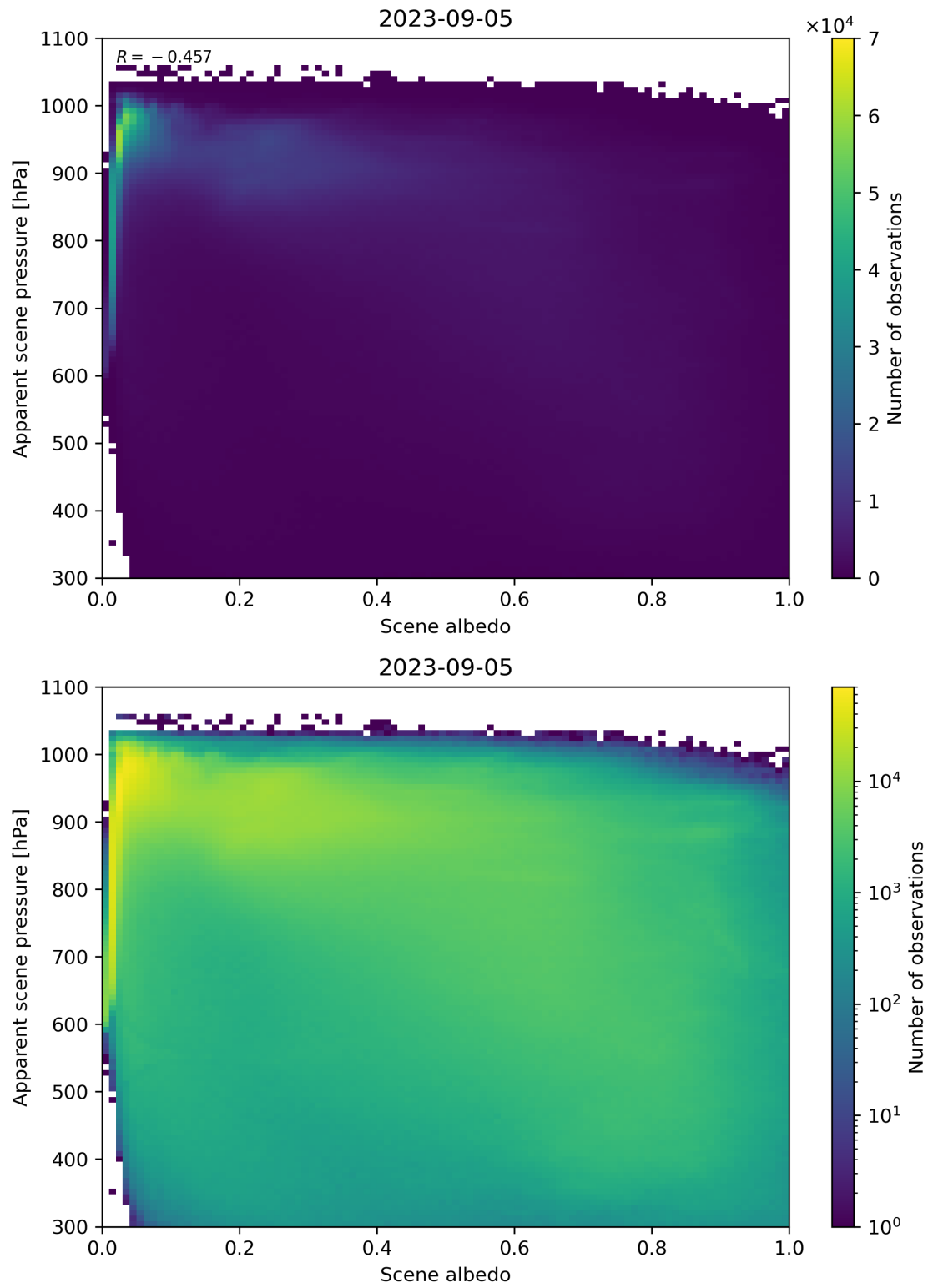
Figure 111: Scatter density plot of “Scene albedo” against “Apparent scene pressure” for 2023-09-05 to 2023-09-06.
