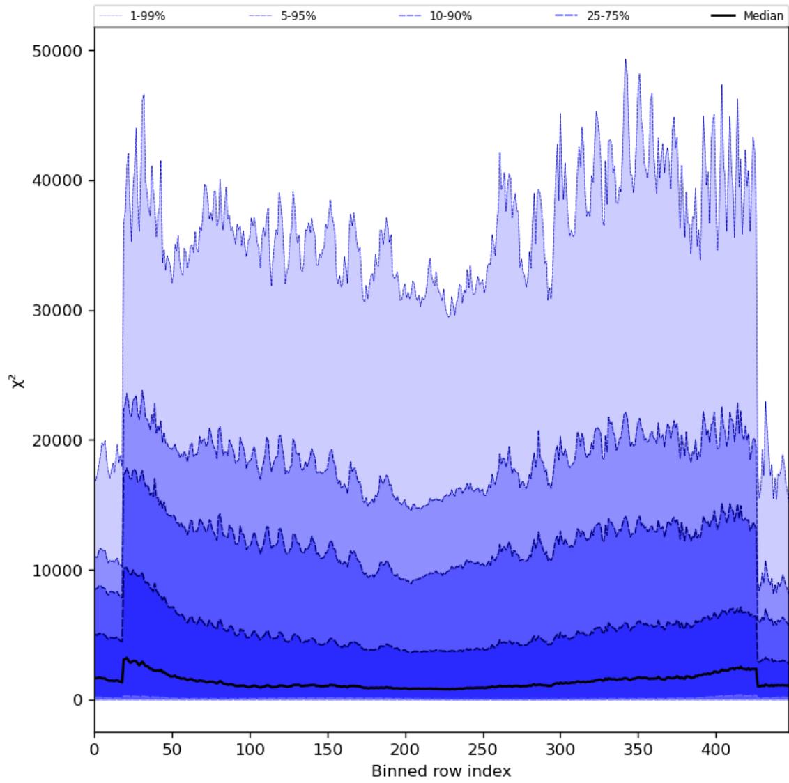
Figure 55: Along track statistics of “ \chi^2 ” for 2023-09-05 to 2023-09-06
