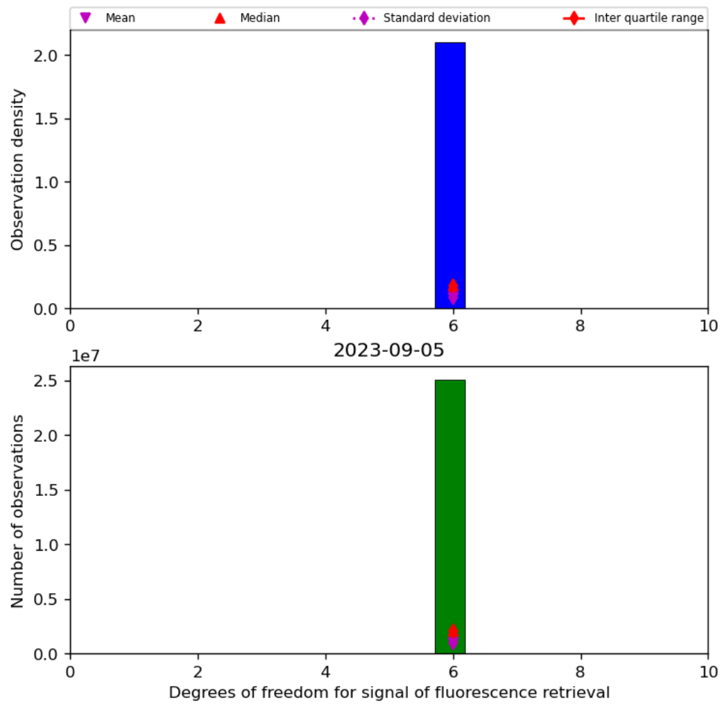
Figure 43: Histogram of “Degrees of freedom for signal of fluorescence retrieval” for 2023-09-05 to 2023-09-06
