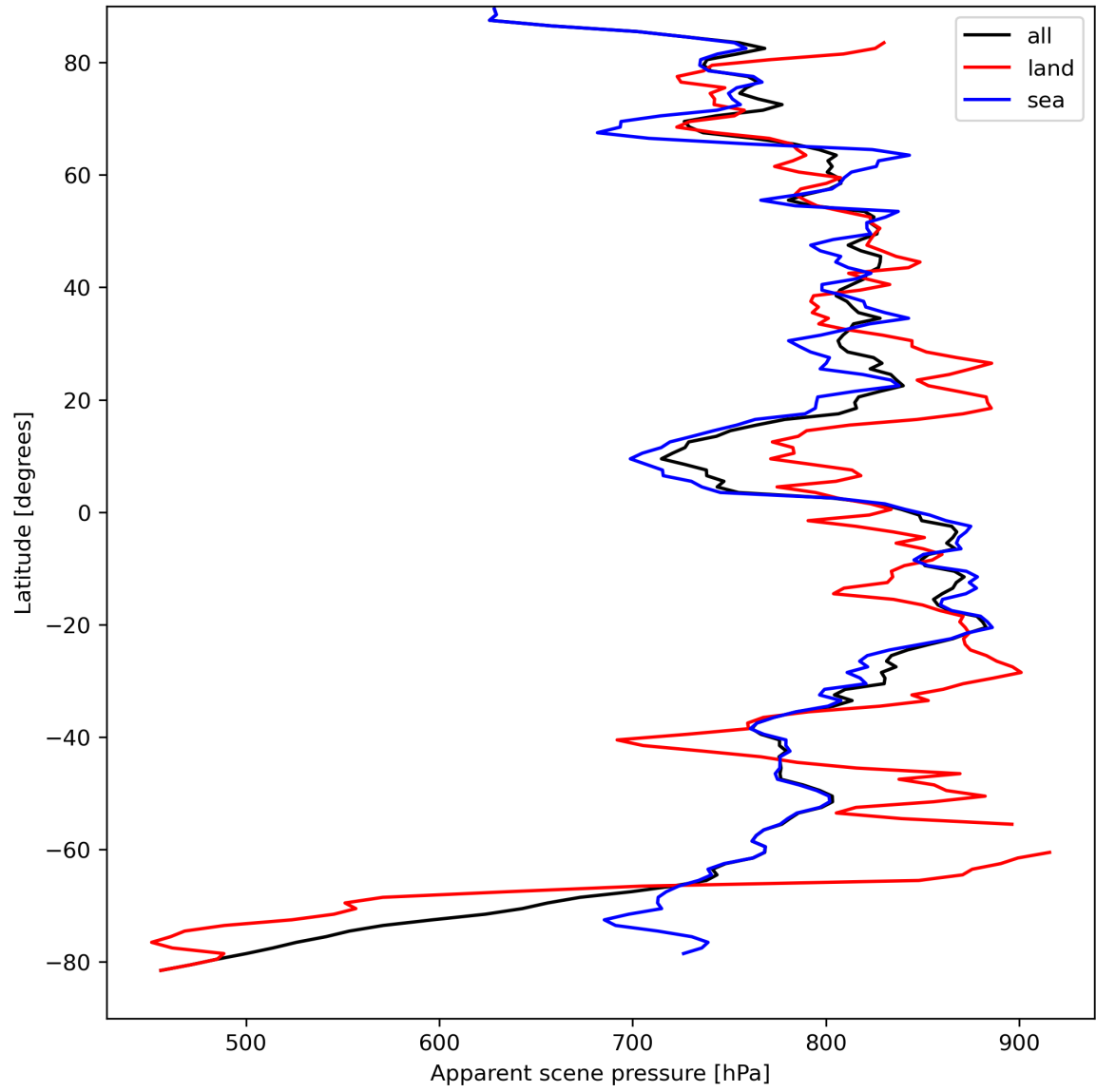
Figure 19: Zonal average of “Apparent scene pressure” for 2023-09-05 to 2023-09-06.
