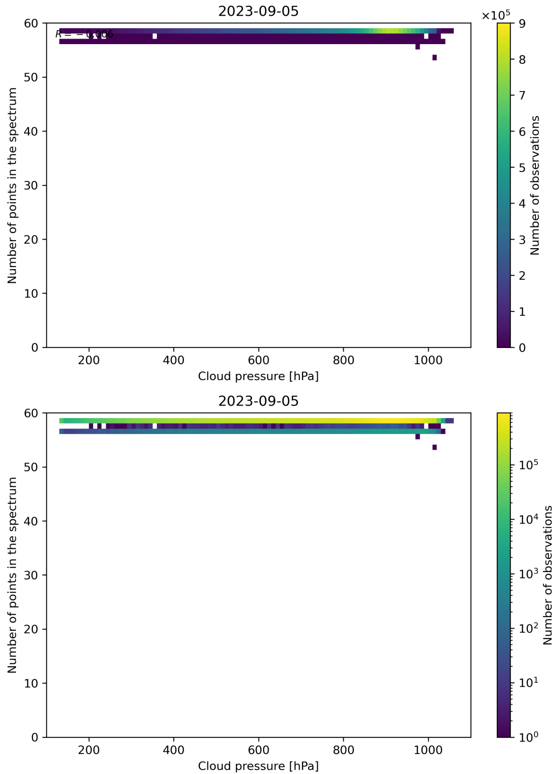
Figure 90: Scatter density plot of “Cloud pressure” against “Number of points in the spectrum” for 2023-09-05 to 2023-09-06.
