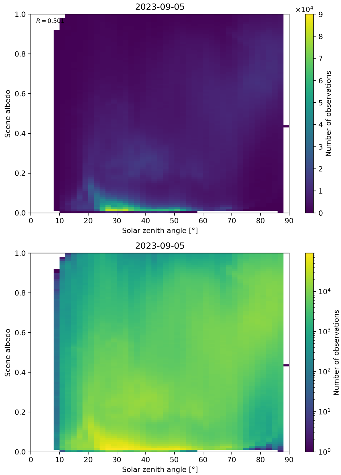
Figure 127: Scatter density plot of “Solar zenith angle” against “Scene albedo” for 2023-09-05 to 2023-09-06.
