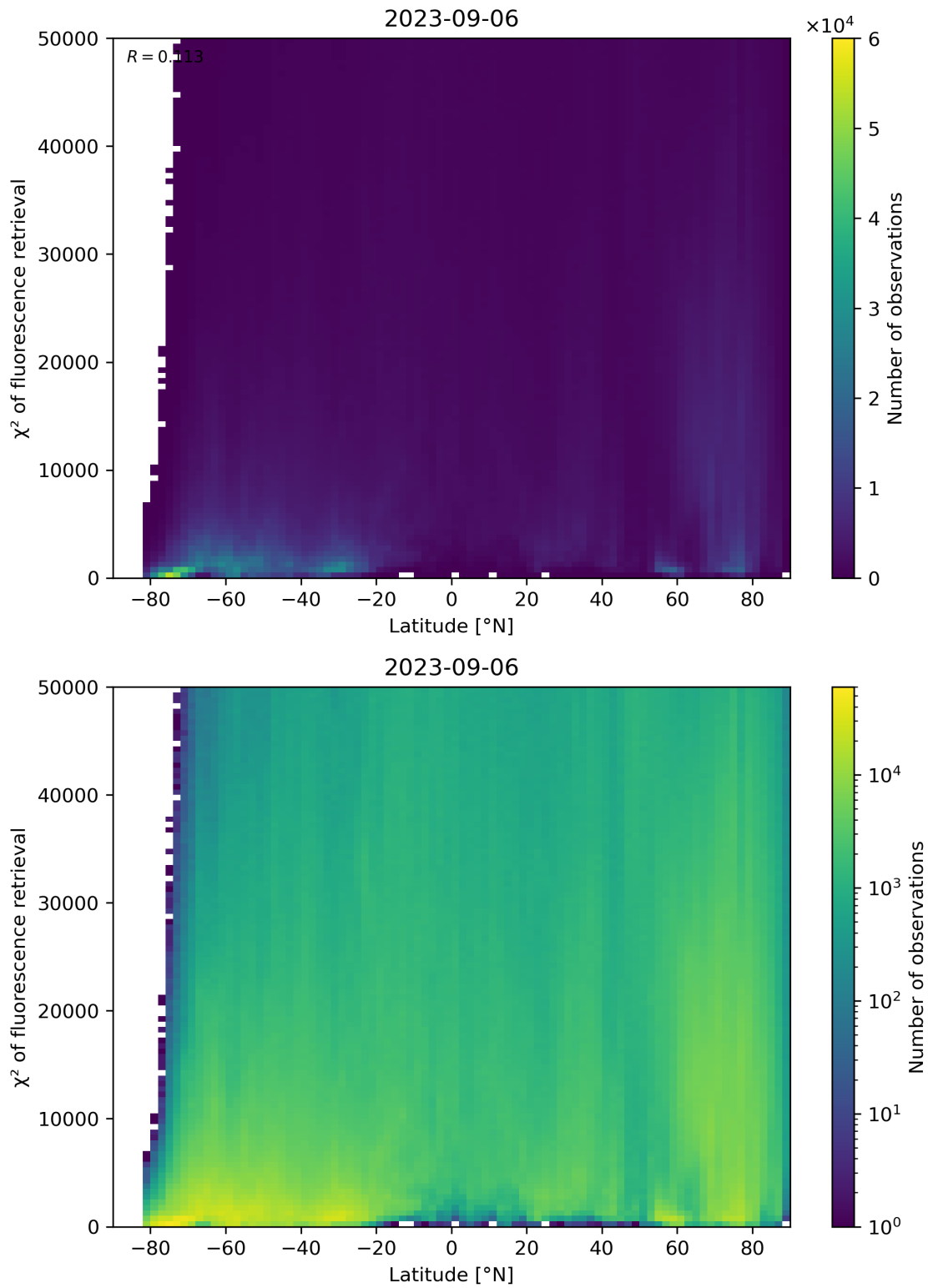
Figure 98: Scatter density plot of “Latitude” against “ \chi^2 of fluorescence retrieval” for 2023-09-05 to 2023-09-07.
