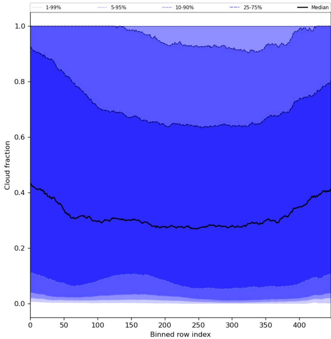
Figure 49: Along track statistics of “Cloud fraction” for 2023-09-05 to 2023-09-07
