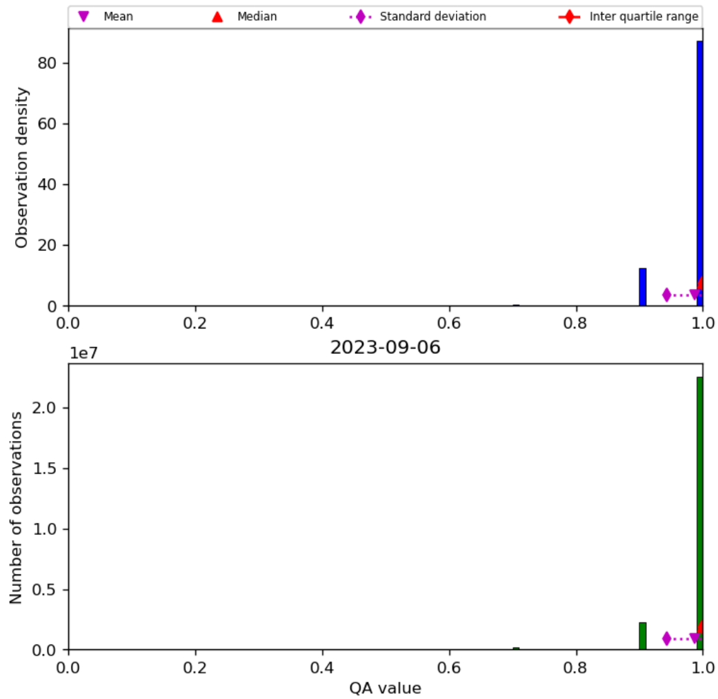
Figure 29: Histogram of “QA value” for 2023-09-05 to 2023-09-07
