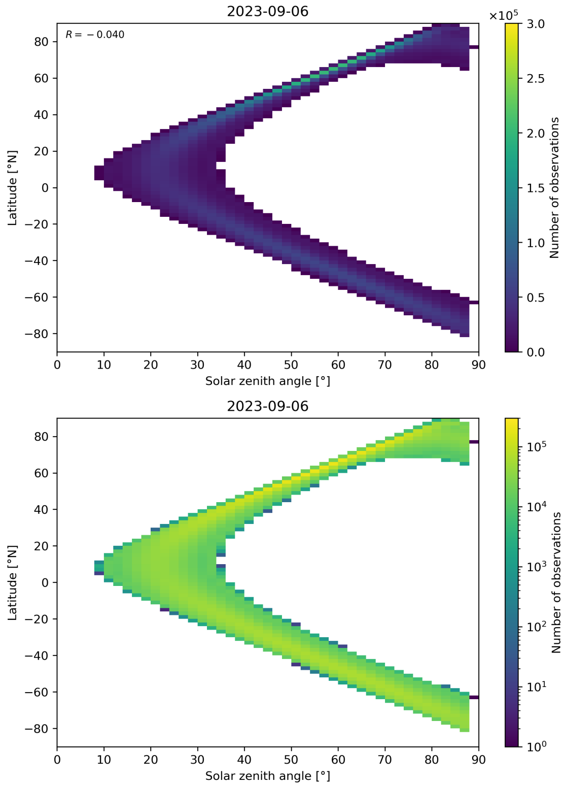
Figure 124: Scatter density plot of “Solar zenith angle” against “Latitude” for 2023-09-05 to 2023-09-07.
