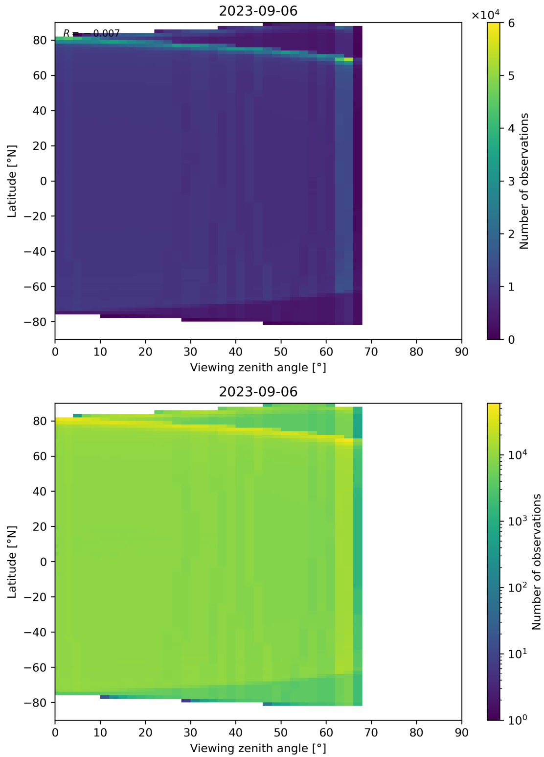
Figure 135: Scatter density plot of “Viewing zenith angle” against “Latitude” for 2023-09-05 to 2023-09-07.
