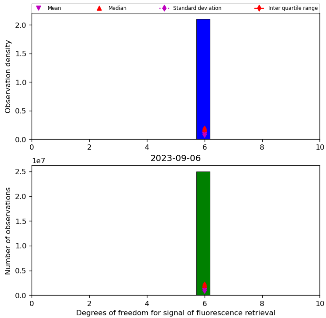
Figure 43: Histogram of "Degrees of freedom for signal of fluorescence retrieval" for 2023-09-05 to 2023-09-07
