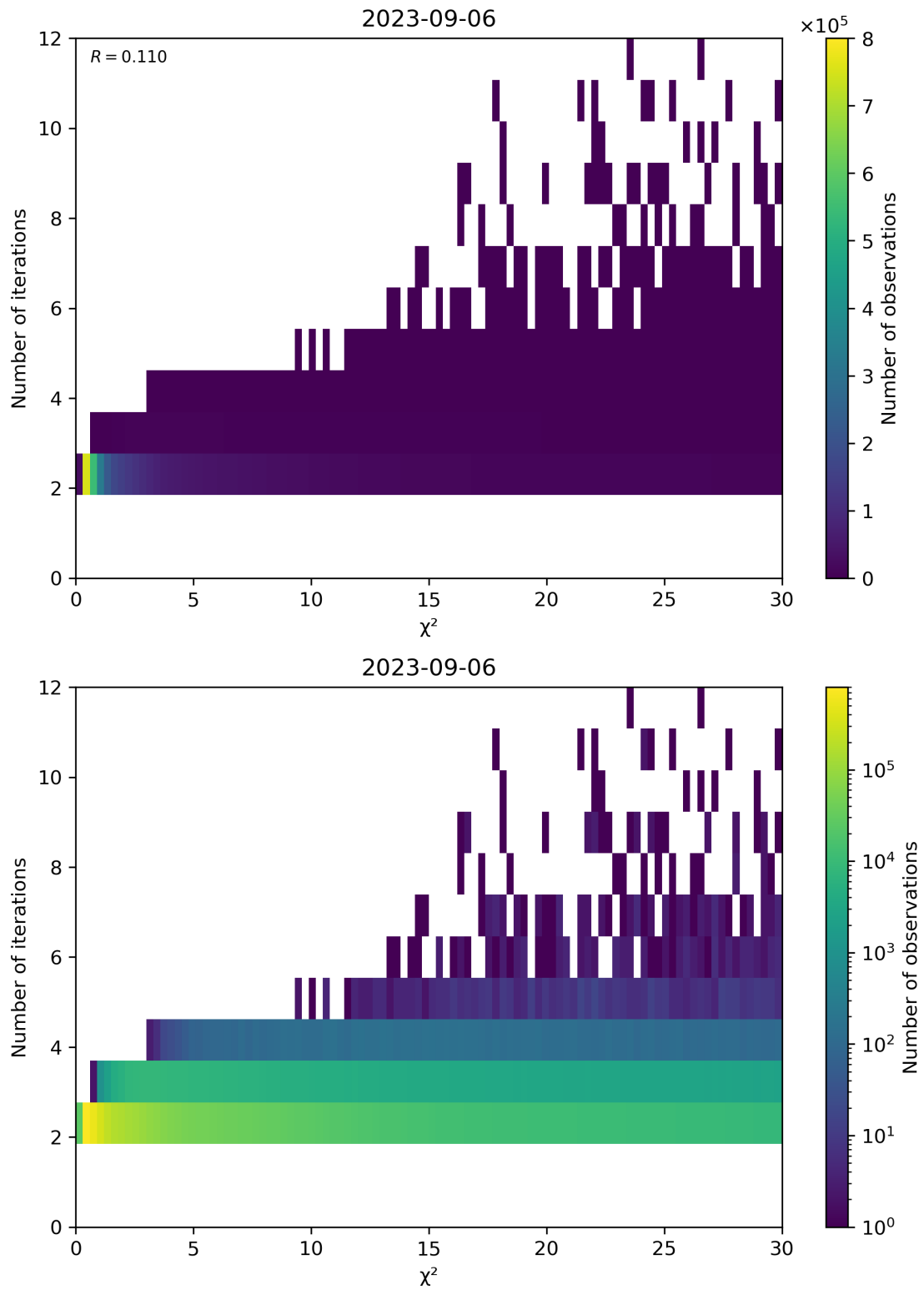
Figure 73: Scatter density plot of “ \chi^2 ” against “Number of iterations” for 2023-09-05 to 2023-09-07.
