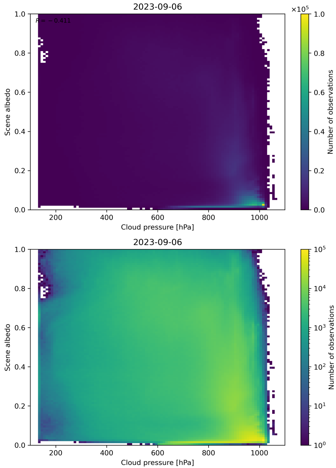
Figure 91: Scatter density plot of “Cloud pressure” against “Scene albedo” for 2023-09-05 to 2023-09-07.
