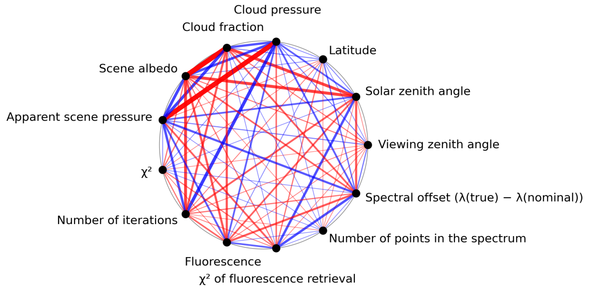
Figure 1: Map of correlation graph for 2023-09-05 to 2023-09-07.
