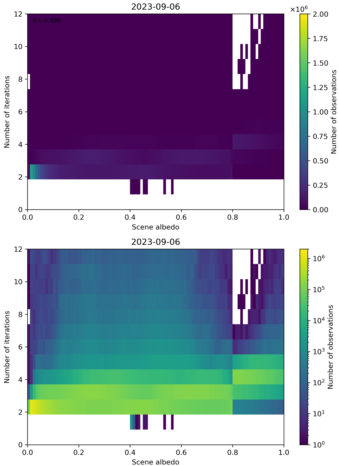
Figure 115: Scatter density plot of “Scene albedo” against “Number of iterations” for 2023-09-05 to 2023-09-07.
