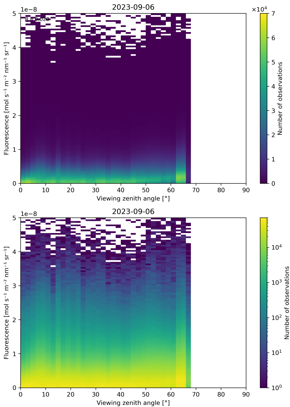
Figure 134: Scatter density plot of “Viewing zenith angle” against “Fluorescence” for 2023-09-05 to 2023-09-07.
