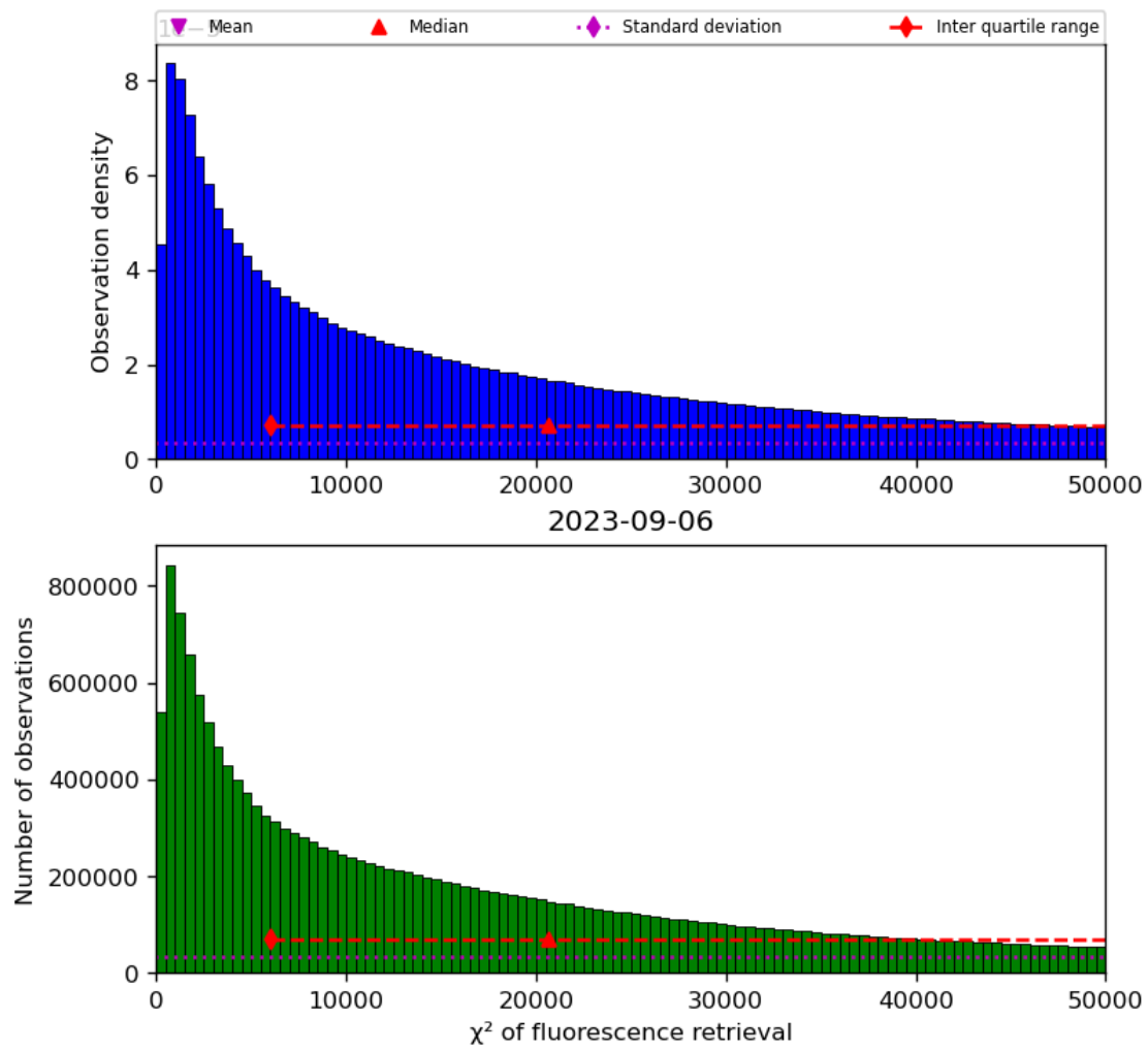
Figure 42: Histogram of “ \chi^2 of fluorescence retrieval” for 2023-09-05 to 2023-09-07
