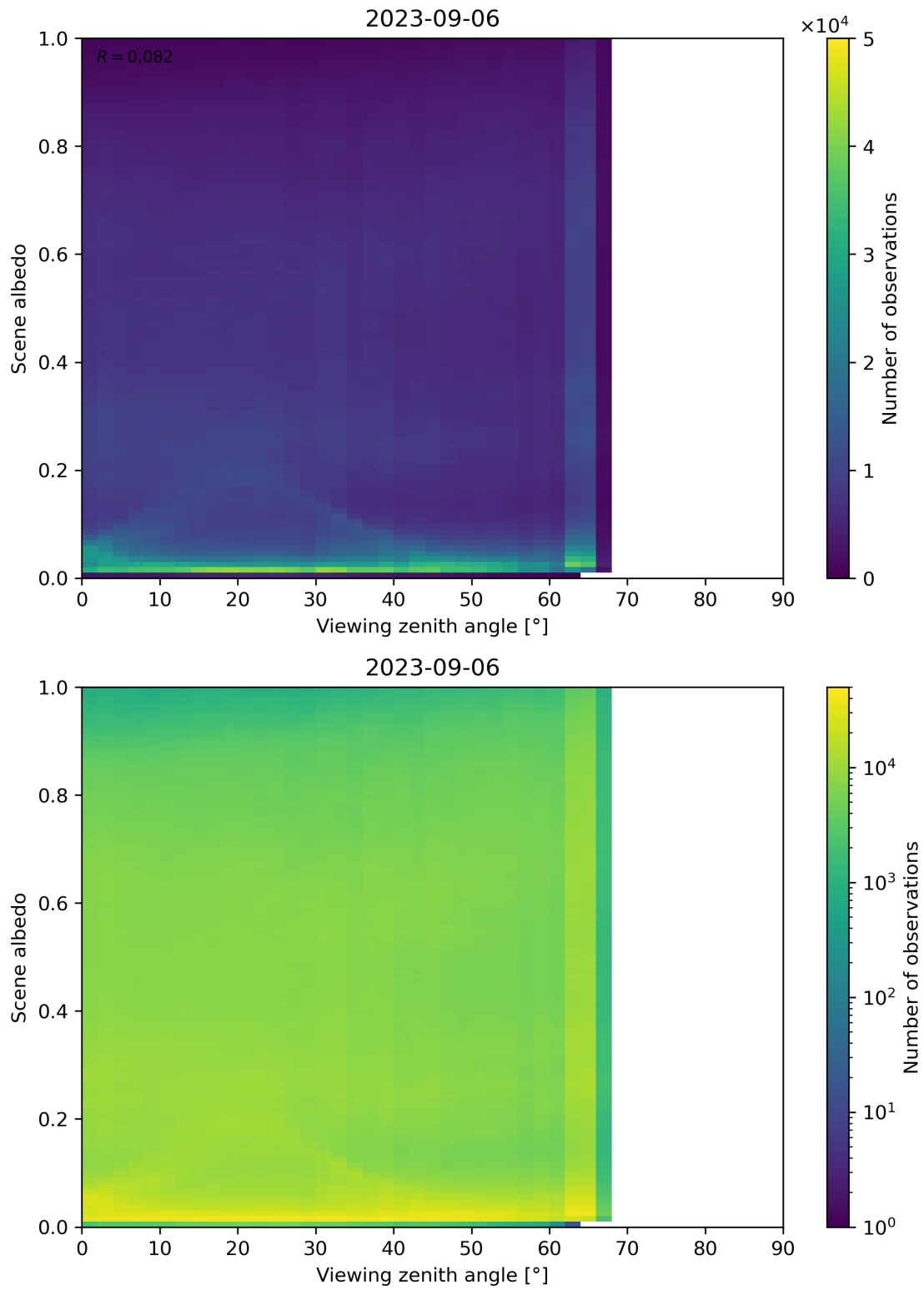
Figure 138: Scatter density plot of “Viewing zenith angle” against “Scene albedo” for 2023-09-05 to 2023-09-07.
