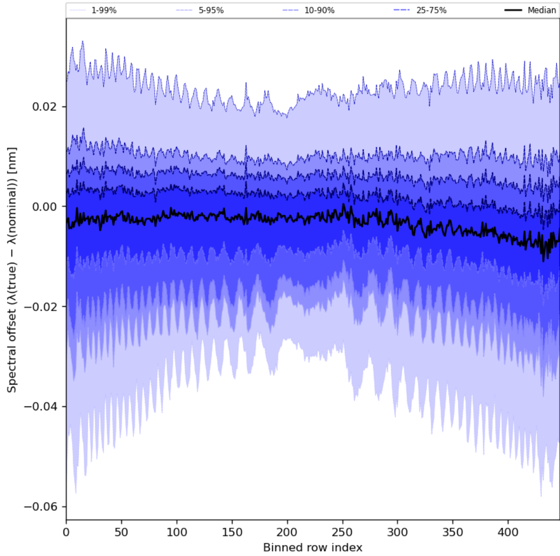
Figure 62: Along track statistics of “Spectral offset ( \lambda(\text{true}) - \lambda(\text{nominal}) )” for 2023-09-05 to 2023-09-07
