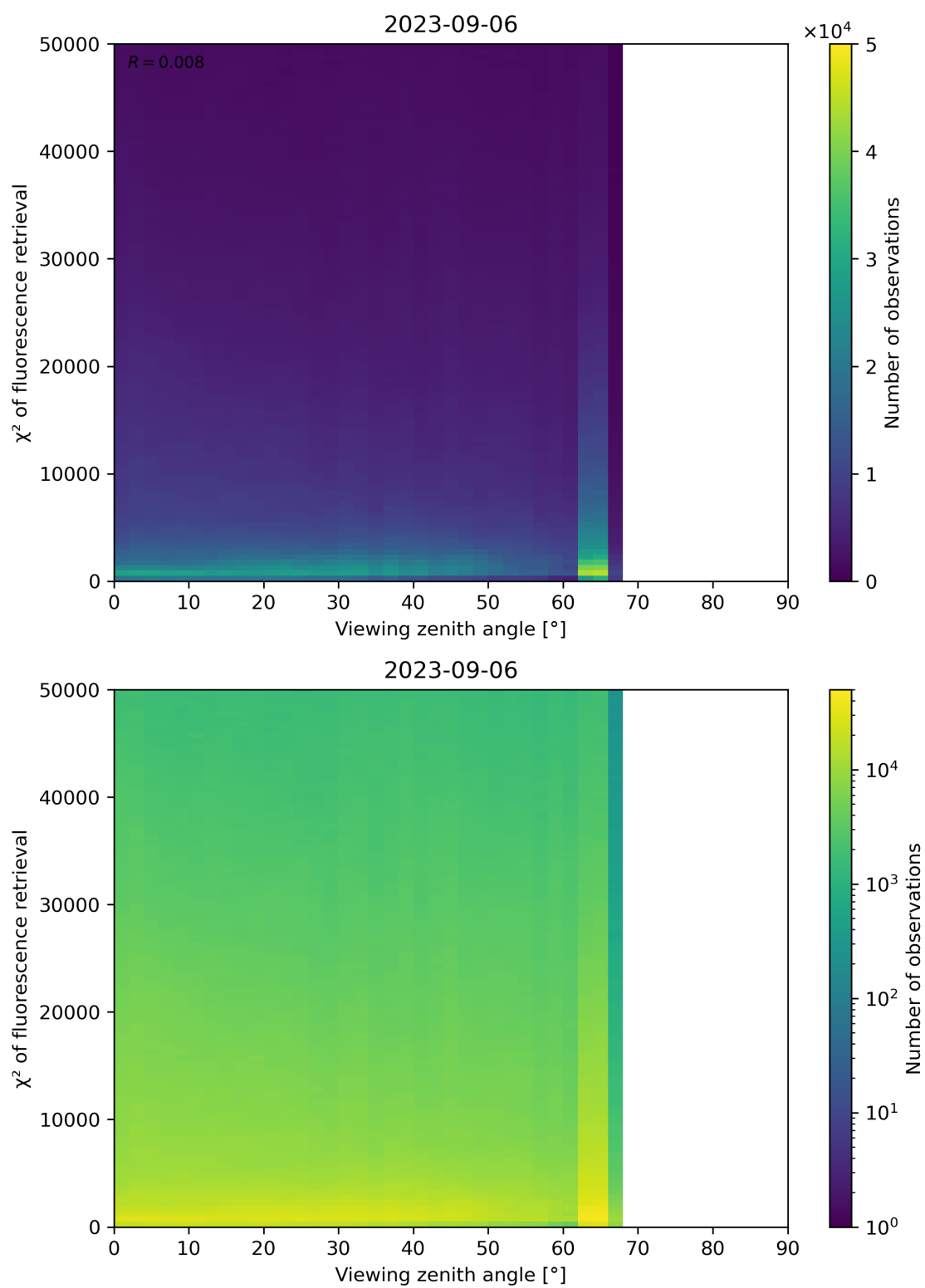
Figure 131: Scatter density plot of “Viewing zenith angle” against “ \chi^2 of fluorescence retrieval” for 2023-09-05 to 2023-09-07.
