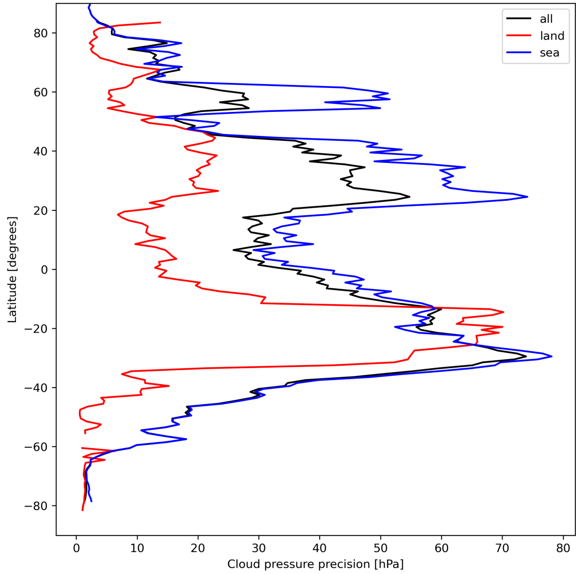
Figure 14: Zonal average of “Cloud pressure precision” for 2023-09-05 to 2023-09-07.
