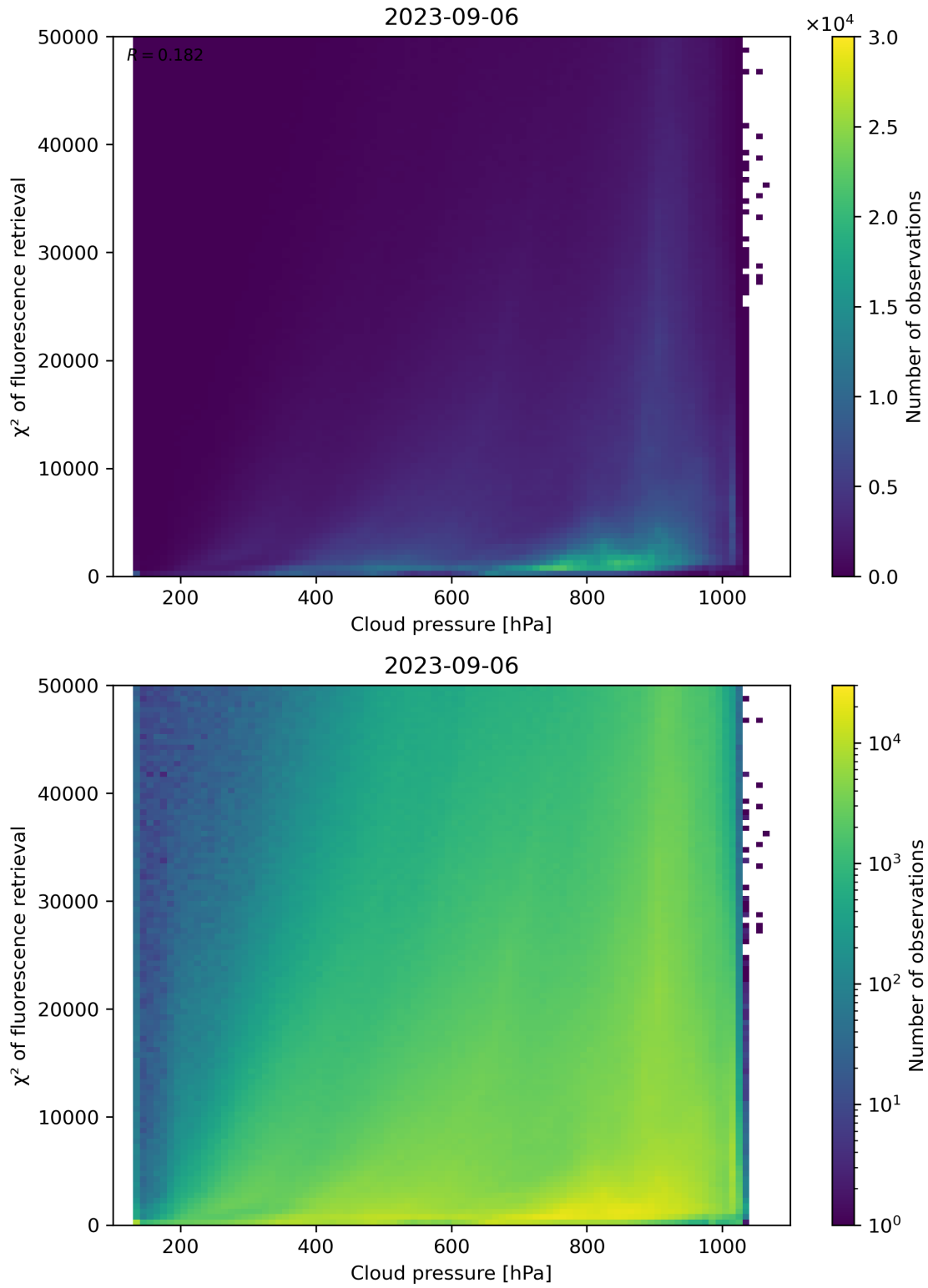
Figure 86: Scatter density plot of “Cloud pressure” against “ \chi^2 of fluorescence retrieval” for 2023-09-05 to 2023-09-07.
