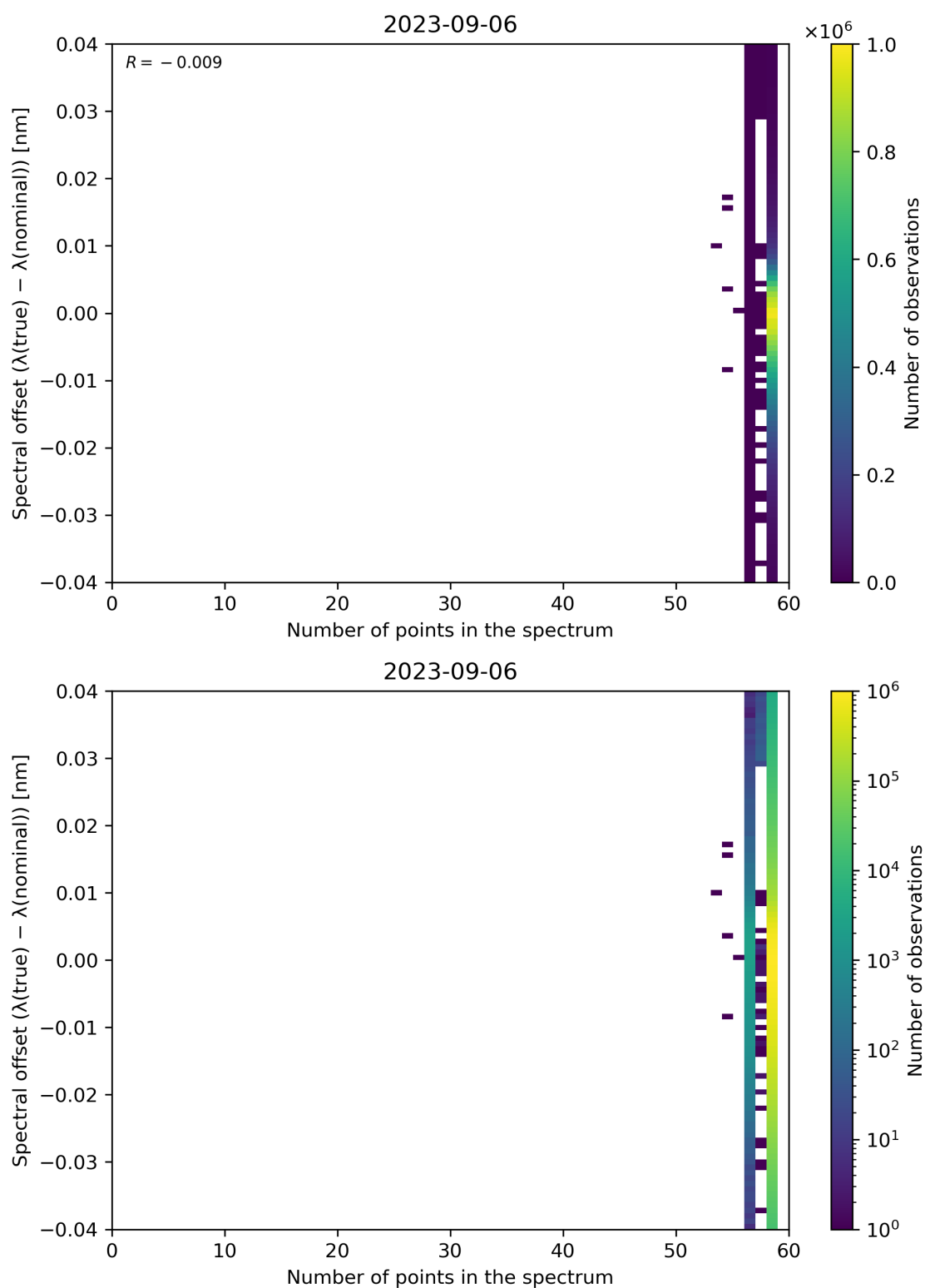
Figure 110: Scatter density plot of “Number of points in the spectrum” against “Spectral offset ( \lambda(\text{true}) - \lambda(\text{nominal}) )” for 2023-09-05 to 2023-09-07.
