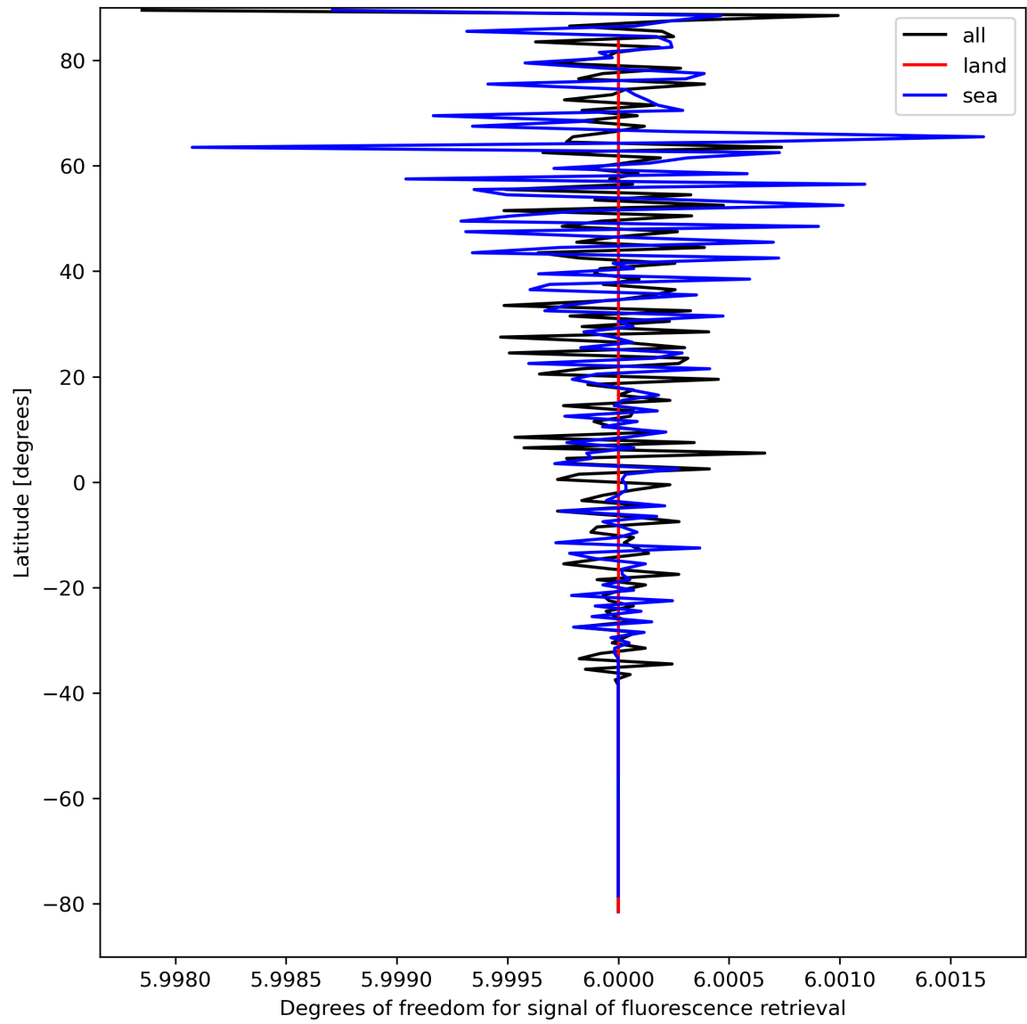
Figure 26: Zonal average of “Degrees of freedom for signal of fluorescence retrieval” for 2023-09-05 to 2023-09-07.
