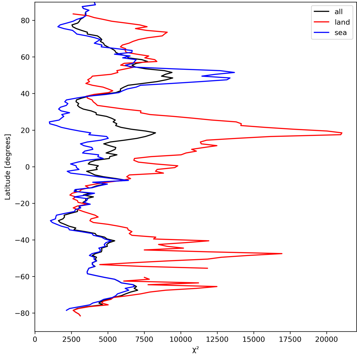
Figure 21: Zonal average of “ \chi^2 ” for 2023-09-05 to 2023-09-07.
