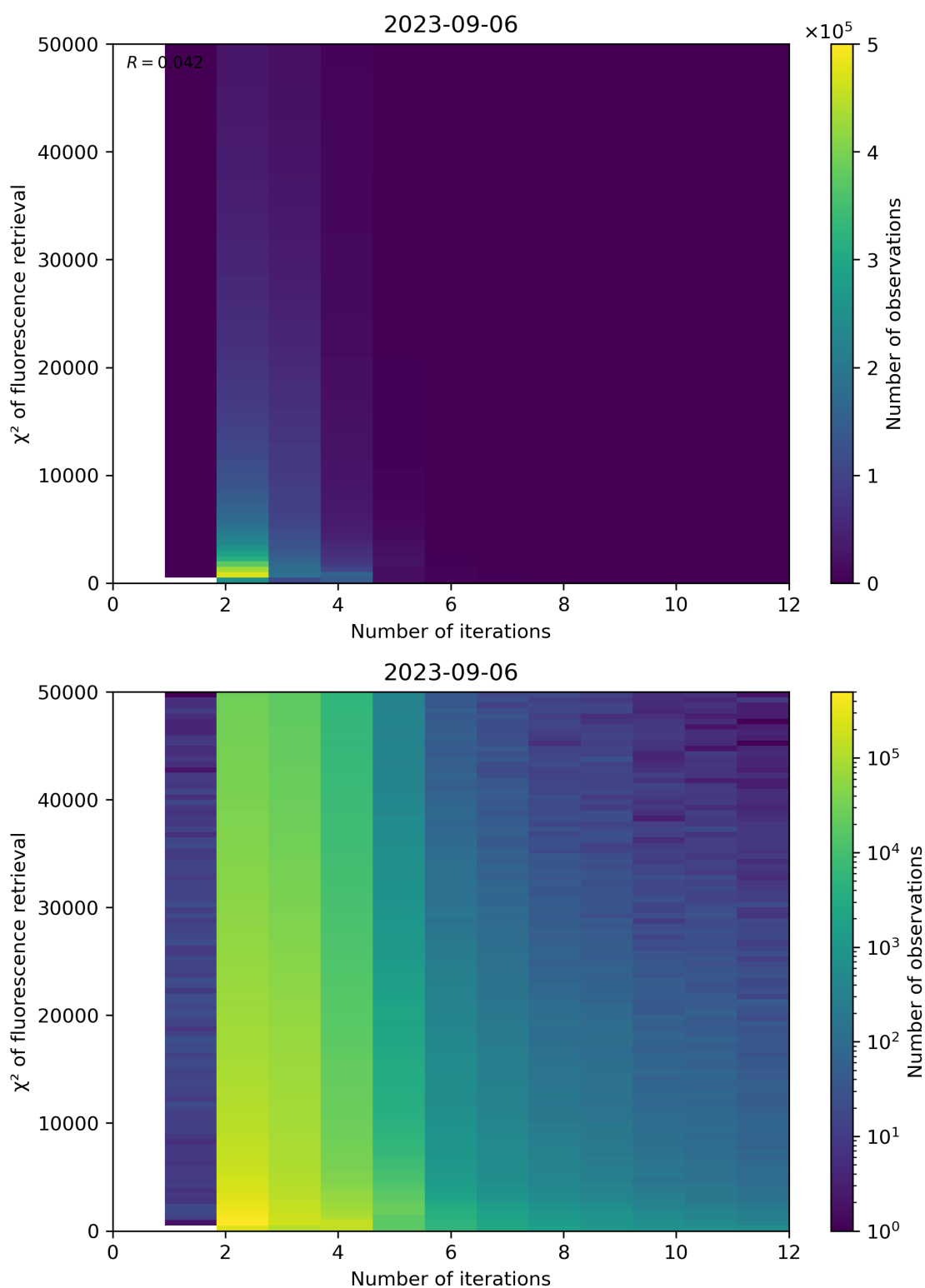
Figure 106: Scatter density plot of “Number of iterations” against “ \chi^2 of fluorescence retrieval” for 2023-09-05 to 2023-09-07.
