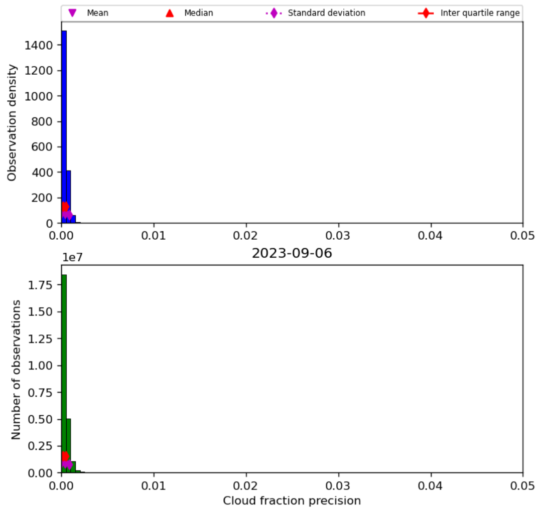
Figure 33: Histogram of “Cloud fraction precision” for 2023-09-05 to 2023-09-07
