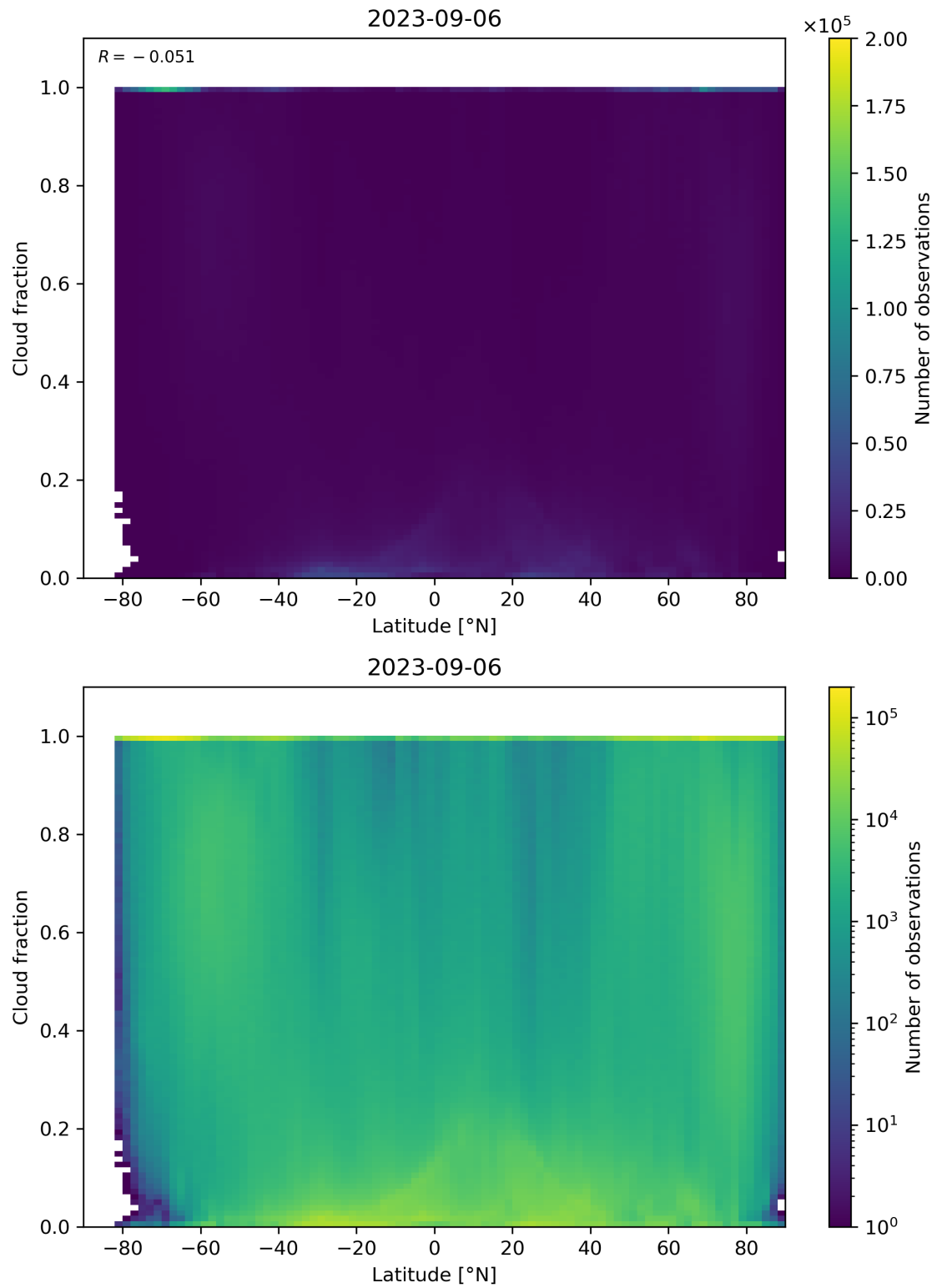
Figure 99: Scatter density plot of “Latitude” against “Cloud fraction” for 2023-09-05 to 2023-09-07.
