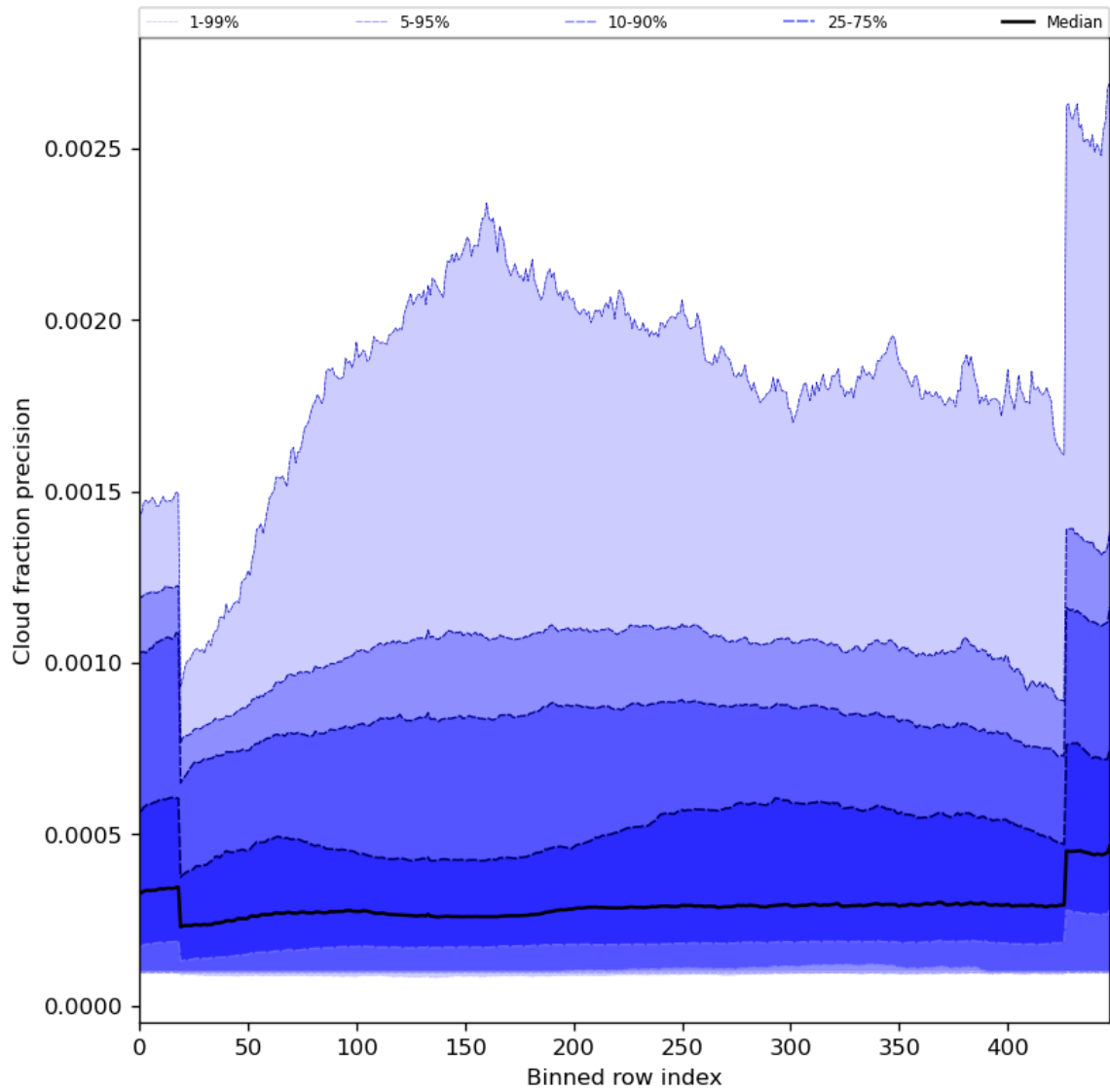
Figure 50: Along track statistics of “Cloud fraction precision” for 2023-09-05 to 2023-09-07
