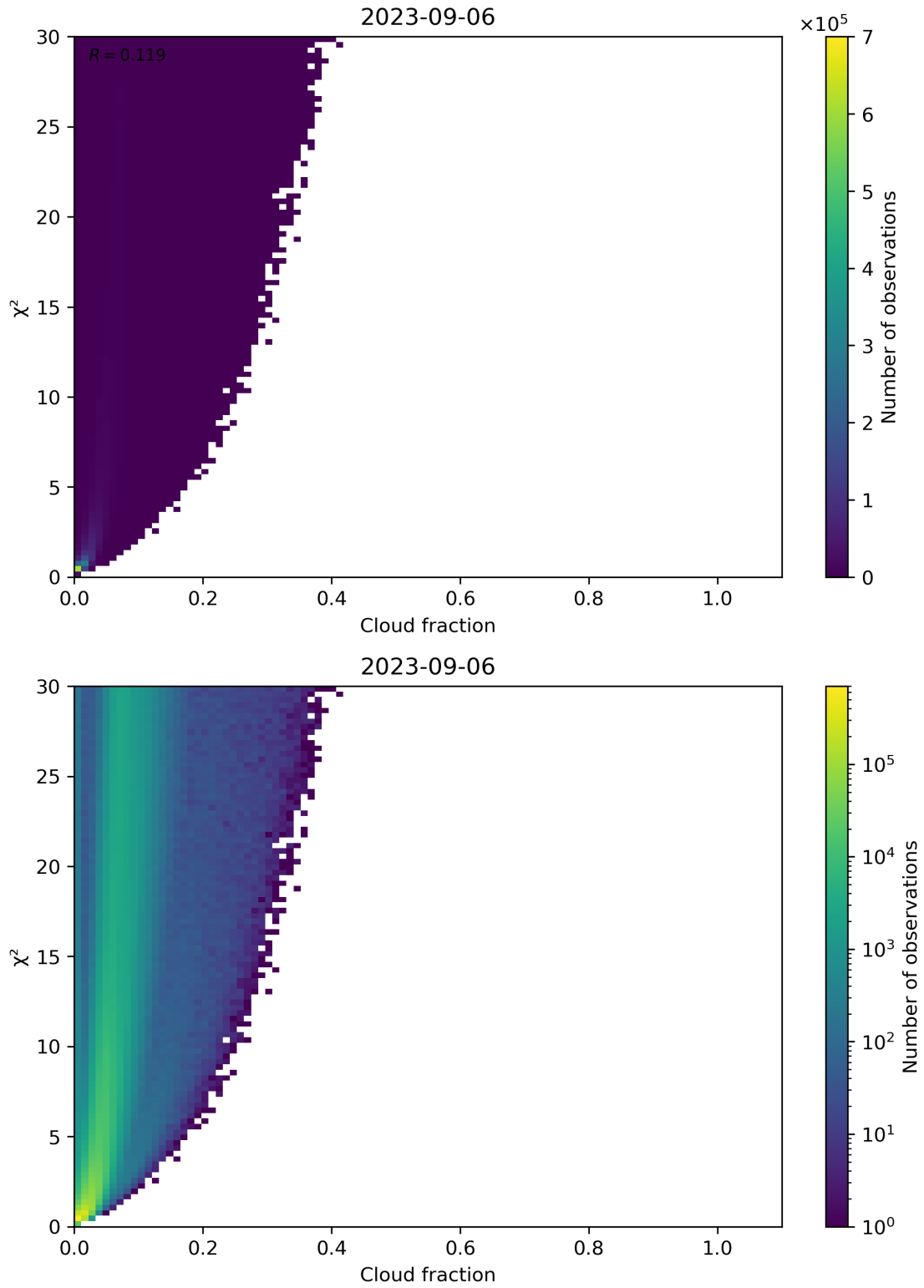
Figure 77: Scatter density plot of “Cloud fraction” against “ \chi^2 ” for 2023-09-05 to 2023-09-07.
