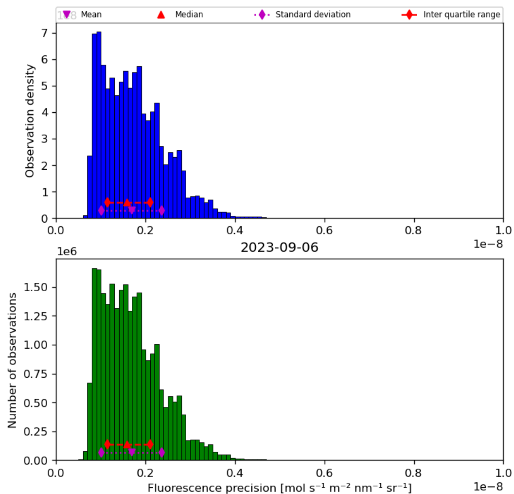
Figure 41: Histogram of “Fluorescence precision” for 2023-09-05 to 2023-09-07
