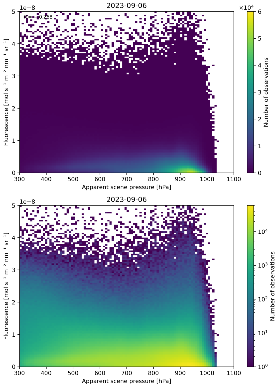
Figure 65: Scatter density plot of “Apparent scene pressure” against “Fluorescence” for 2023-09-05 to 2023-09-07.
