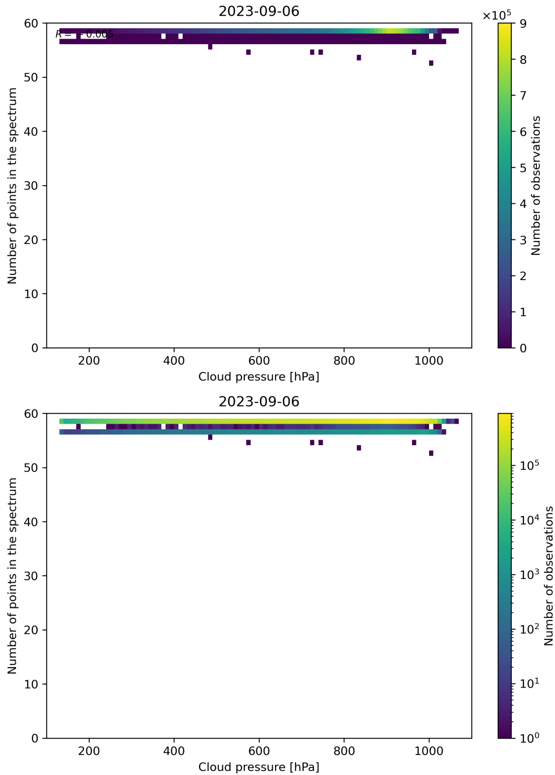
Figure 90: Scatter density plot of “Cloud pressure” against “Number of points in the spectrum” for 2023-09-05 to 2023-09-07.
