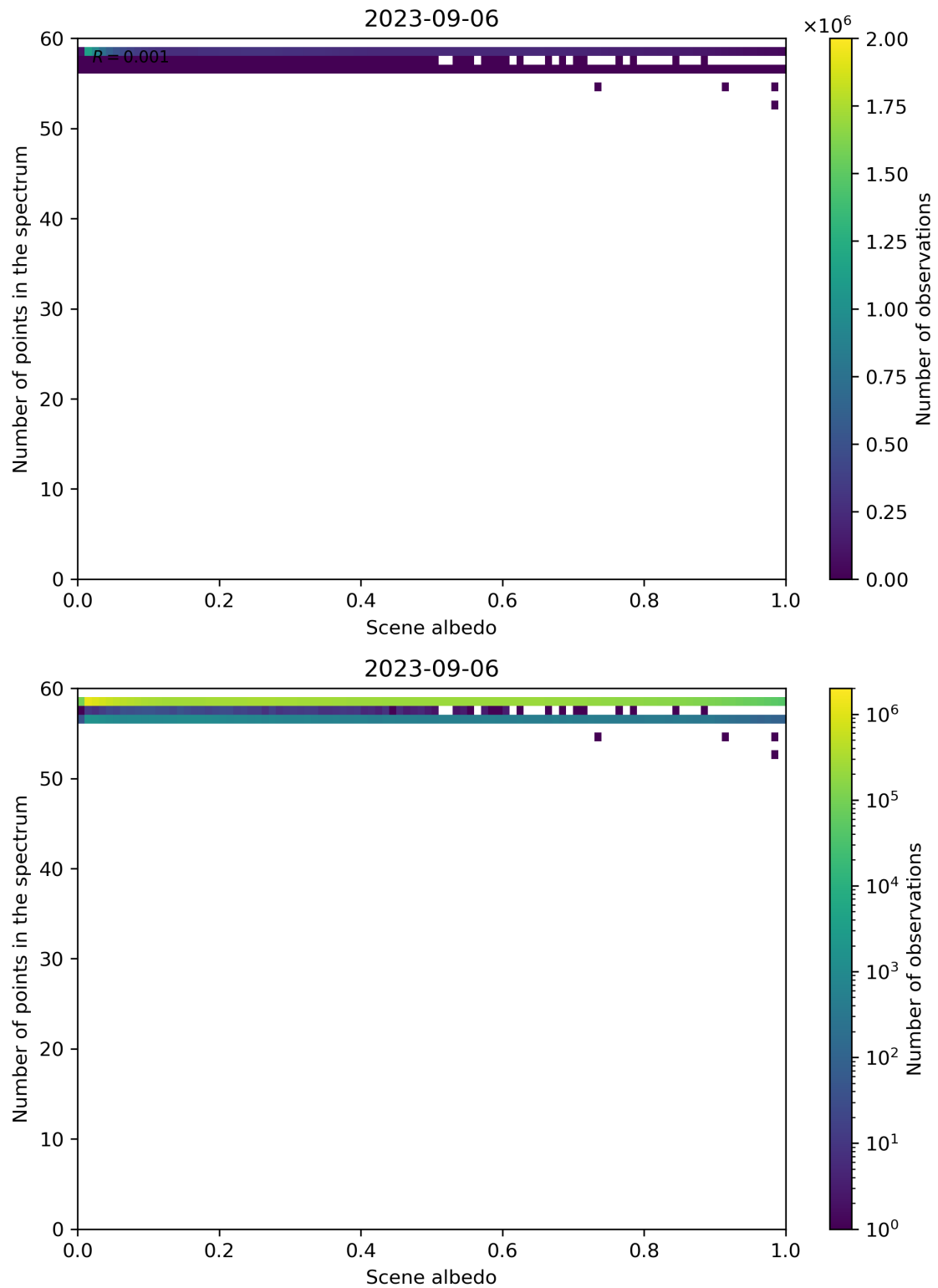
Figure 116: Scatter density plot of “Scene albedo” against “Number of points in the spectrum” for 2023-09-05 to 2023-09-07.
