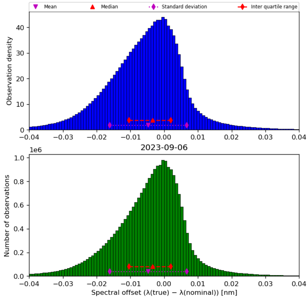
Figure 45: Histogram of “Spectral offset ( \lambda(\text{true}) - \lambda(\text{nominal}) )” for 2023-09-05 to 2023-09-07
