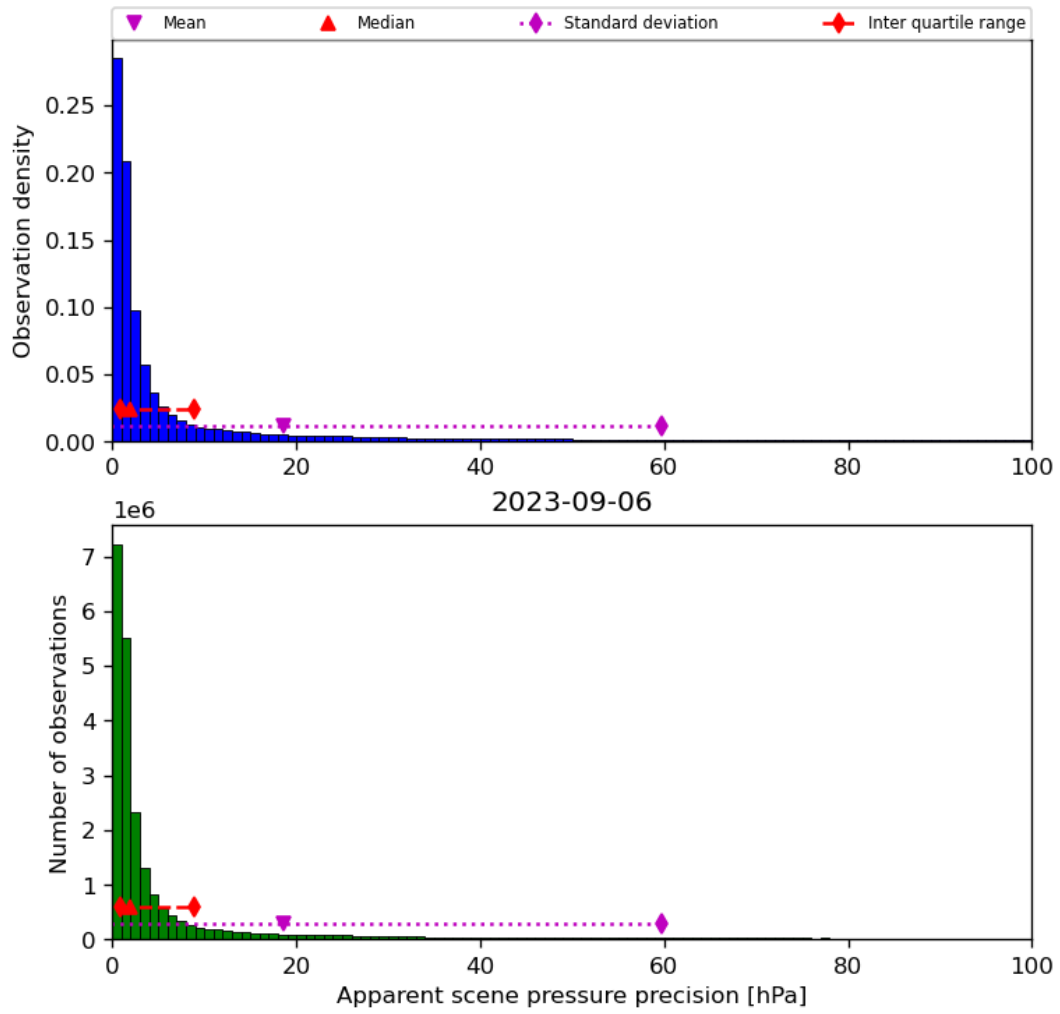
Figure 37: Histogram of “Apparent scene pressure precision” for 2023-09-05 to 2023-09-07
