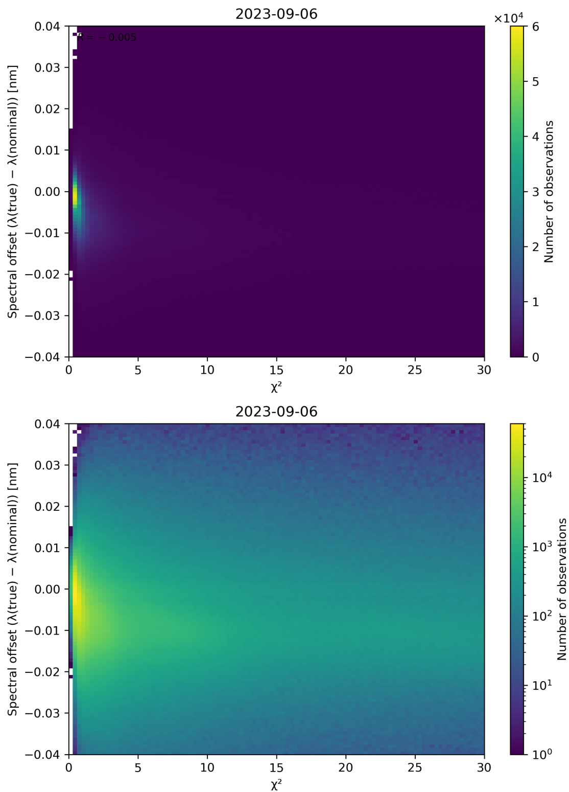
Figure 75: Scatter density plot of “ \chi^2 ” against “Spectral offset ( \lambda(\text{true}) - \lambda(\text{nominal}) )” for 2023-09-05 to 2023-09-07.
