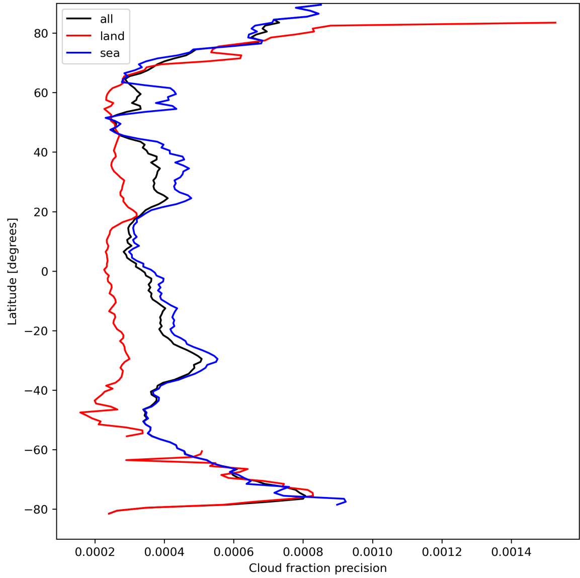
Figure 16: Zonal average of “Cloud fraction precision” for 2023-09-05 to 2023-09-07.
