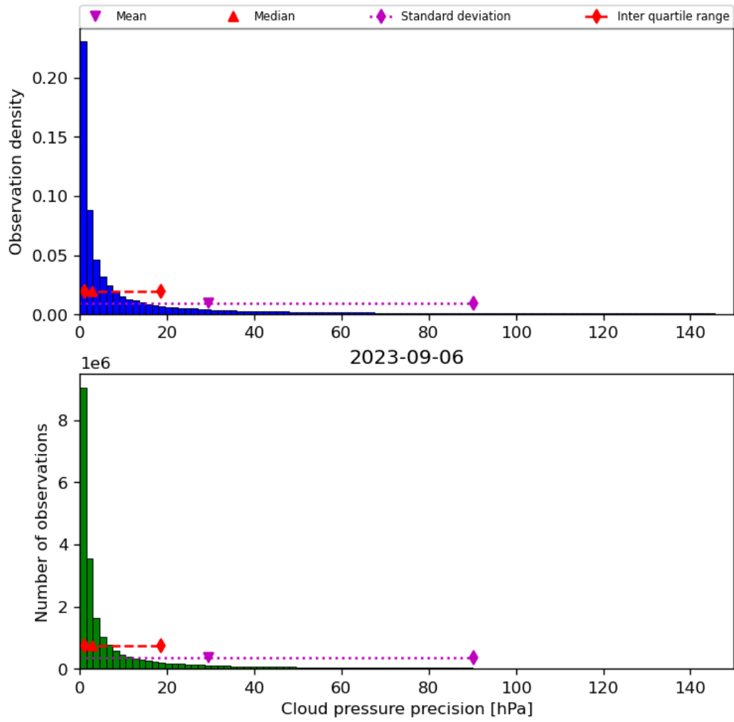
Figure 31: Histogram of “Cloud pressure precision” for 2023-09-05 to 2023-09-07
