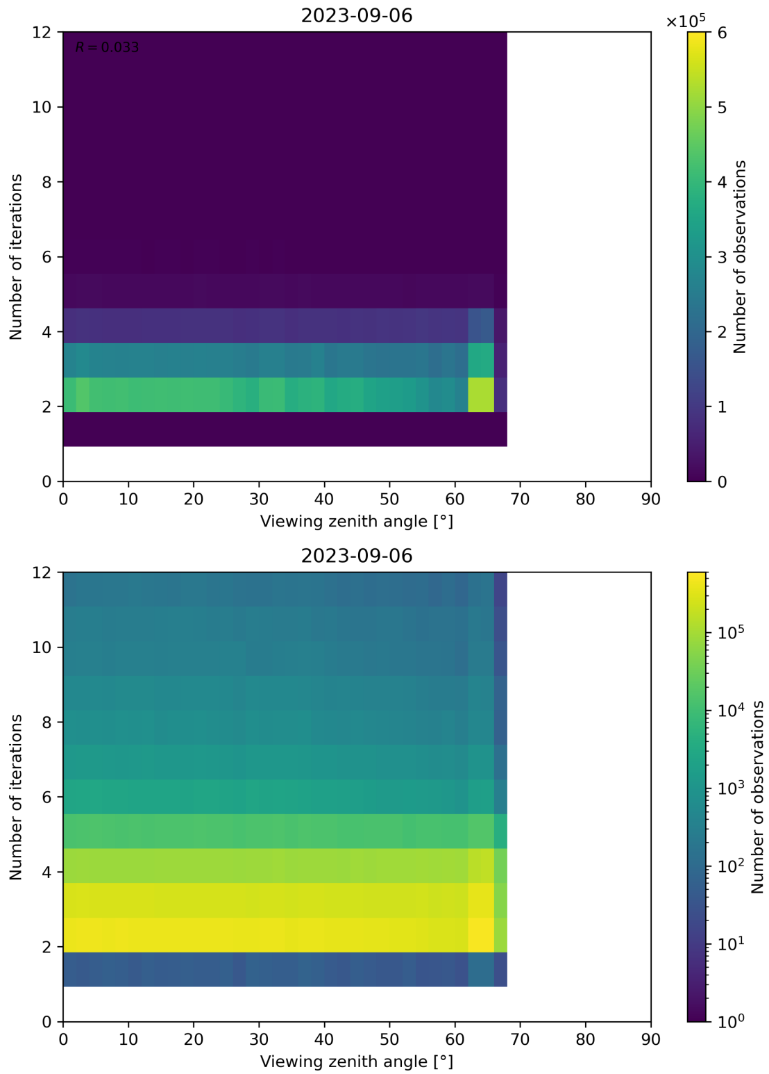
Figure 136: Scatter density plot of “Viewing zenith angle” against “Number of iterations” for 2023-09-05 to 2023-09-07.
