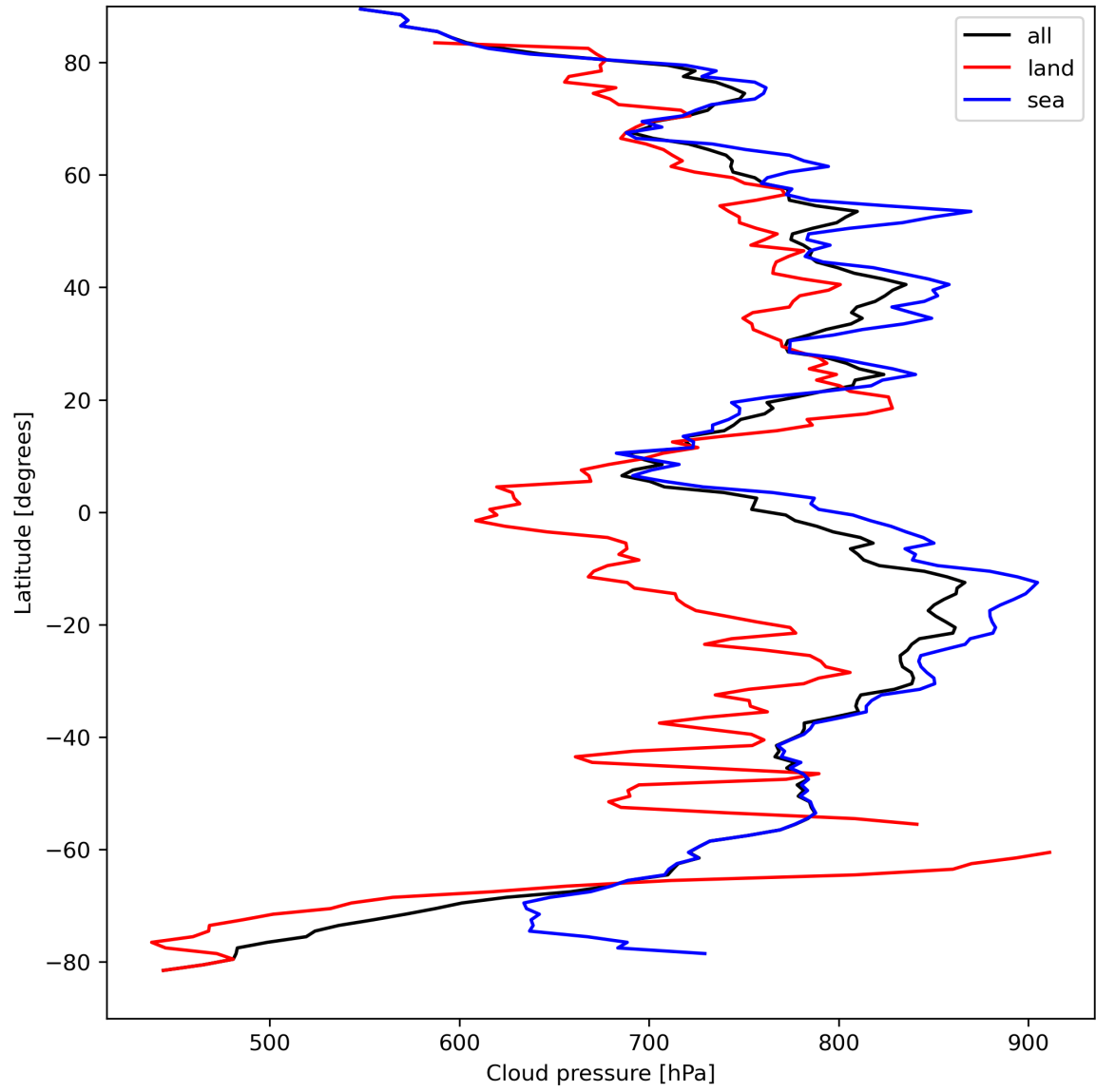
Figure 13: Zonal average of “Cloud pressure” for 2023-09-05 to 2023-09-07.
