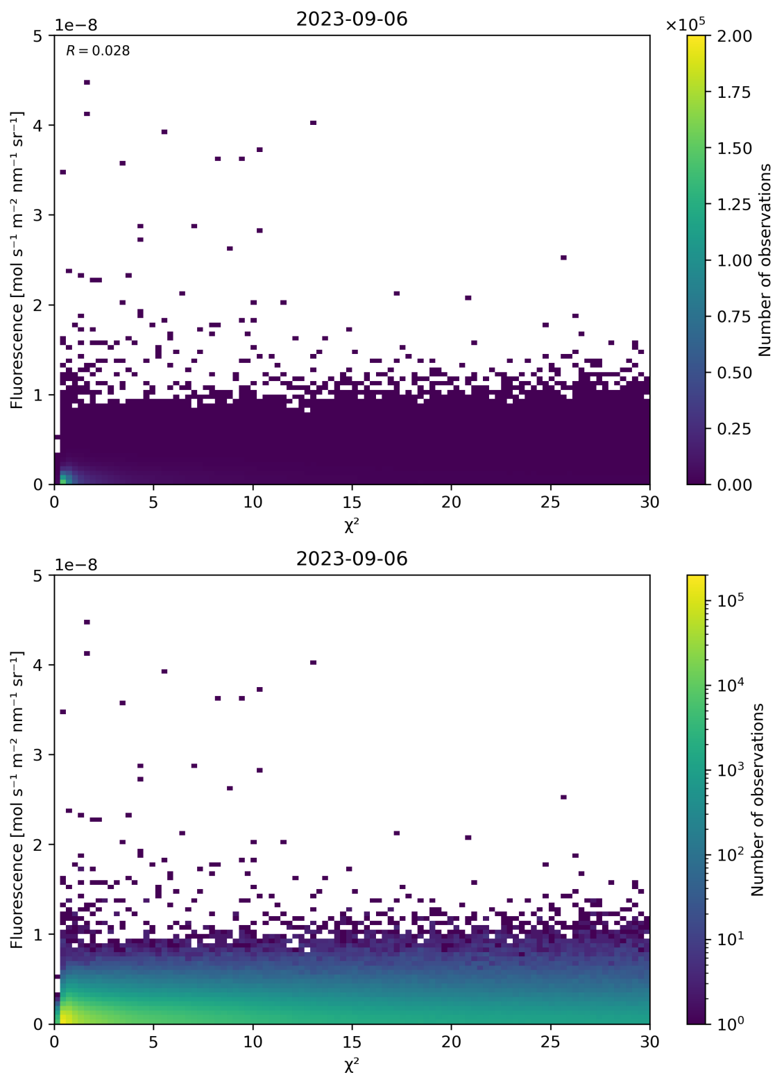
Figure 70: Scatter density plot of “ \chi^2 ” against “Fluorescence” for 2023-09-05 to 2023-09-07.
