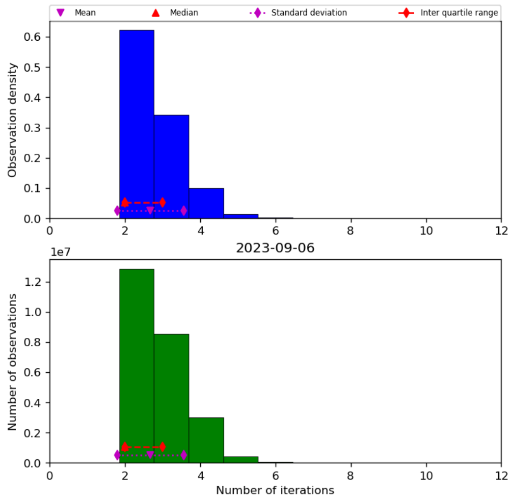
Figure 39: Histogram of “Number of iterations” for 2023-09-05 to 2023-09-07
