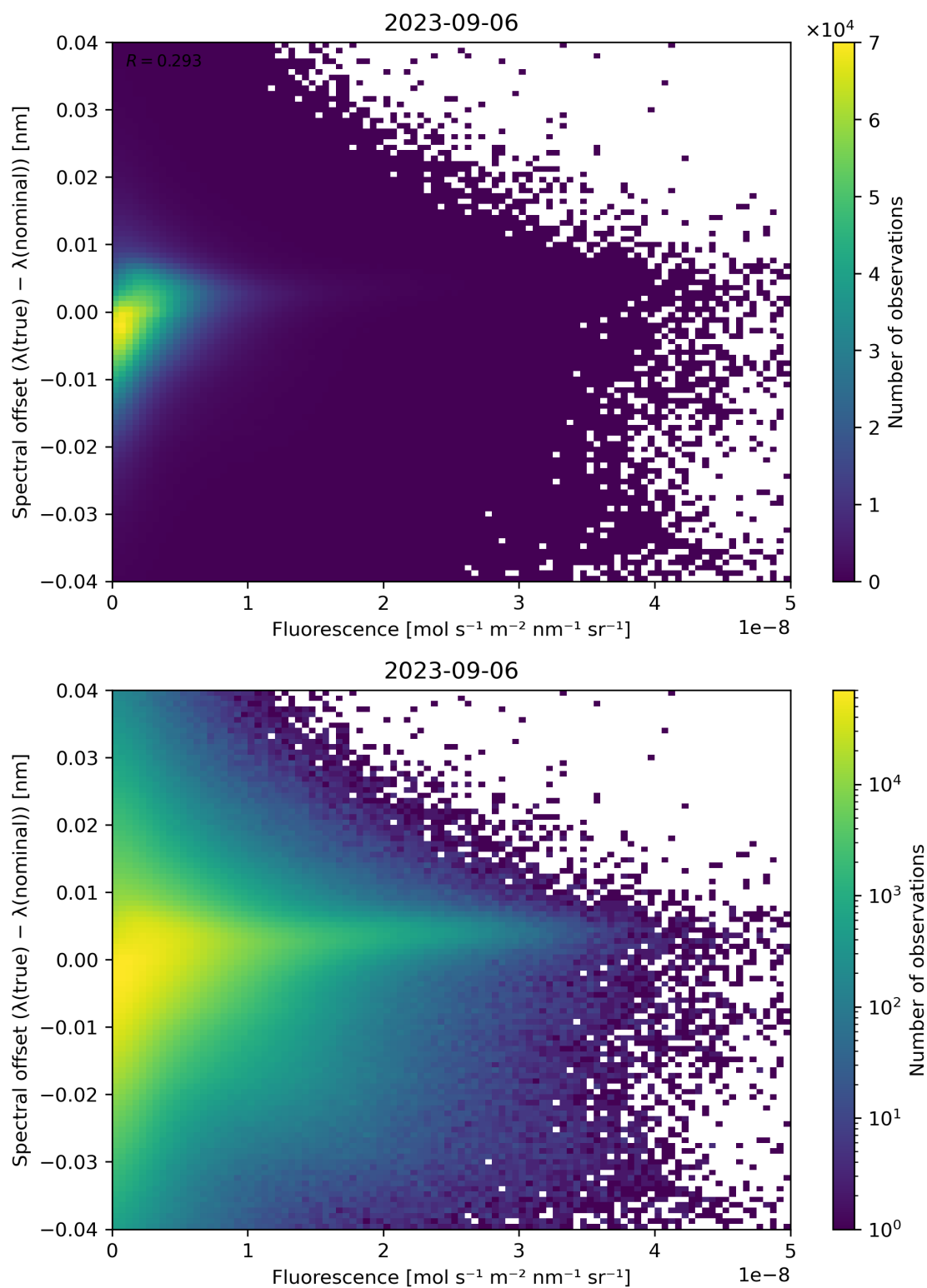
Figure 95: Scatter density plot of “Fluorescence” against “Spectral offset ( \lambda(\text{true}) - \lambda(\text{nominal}) )” for 2023-09-05 to 2023-09-07.
