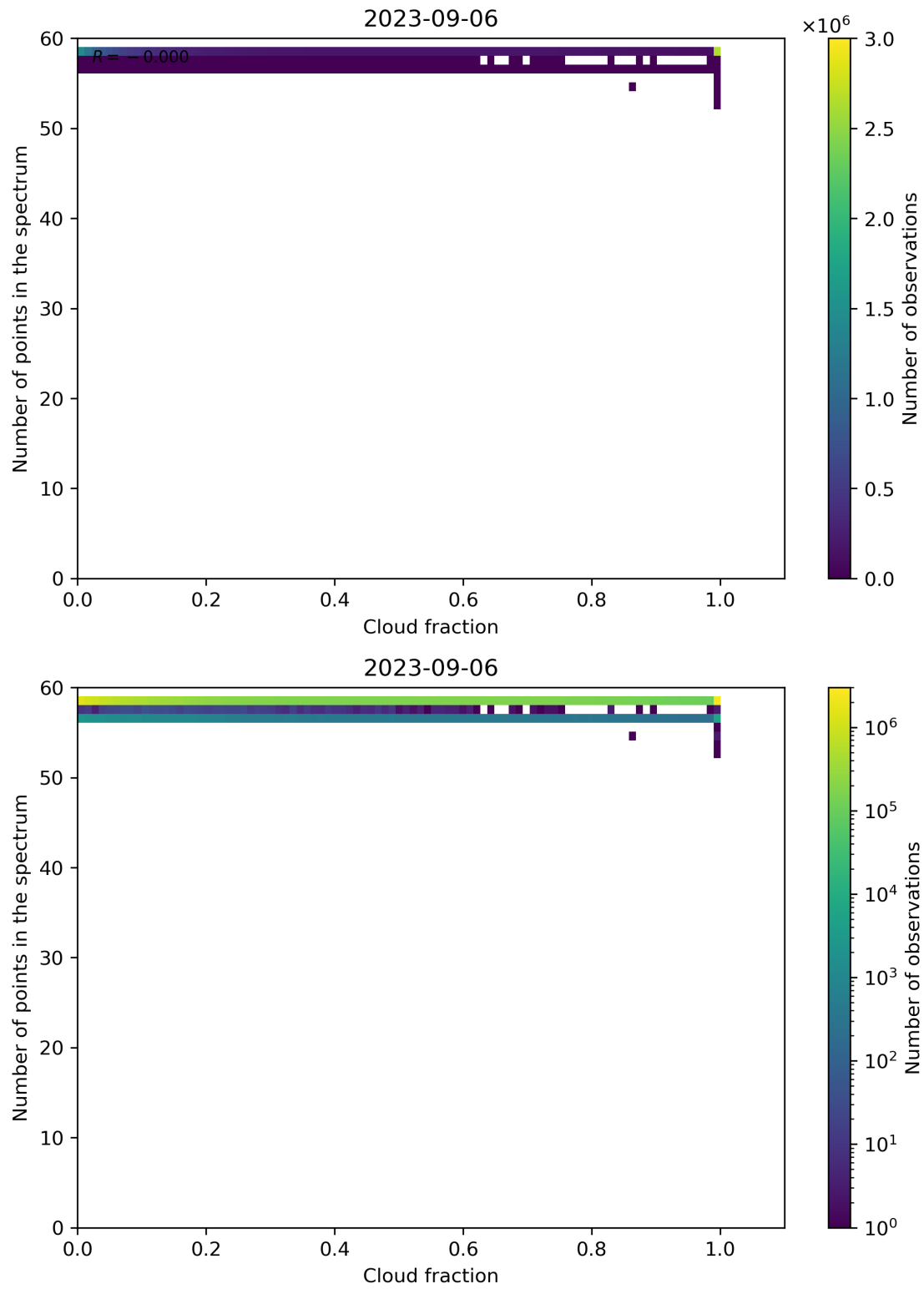
Figure 81: Scatter density plot of “Cloud fraction” against “Number of points in the spectrum” for 2023-09-05 to 2023-09-07.
