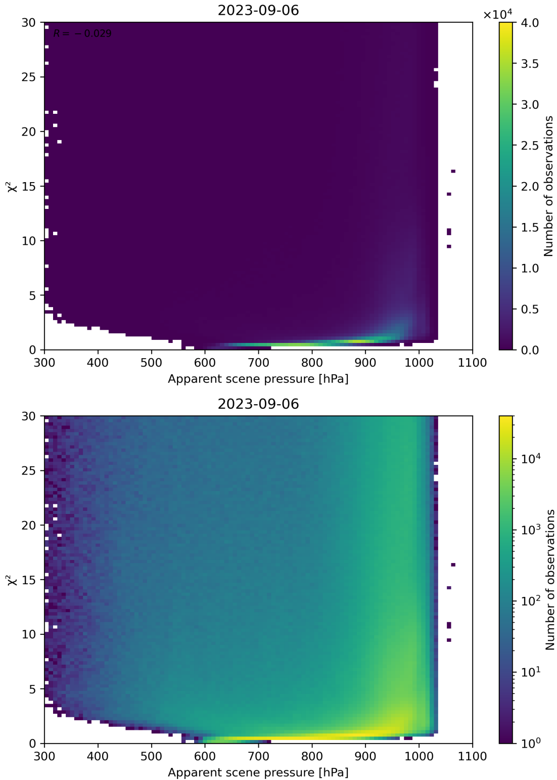
Figure 63: Scatter density plot of “Apparent scene pressure” against “ \chi^2 ” for 2023-09-05 to 2023-09-07.
