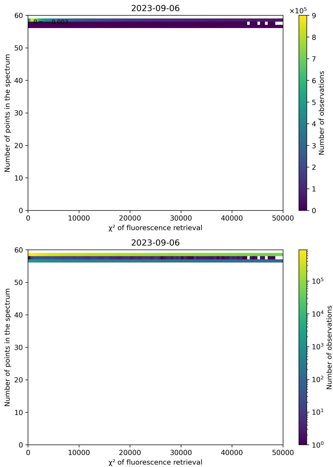
Figure 71: Scatter density plot of " \chi^2 of fluorescence retrieval" against "Number of points in the spectrum" for 2023-09-05 to 2023-09-07.
