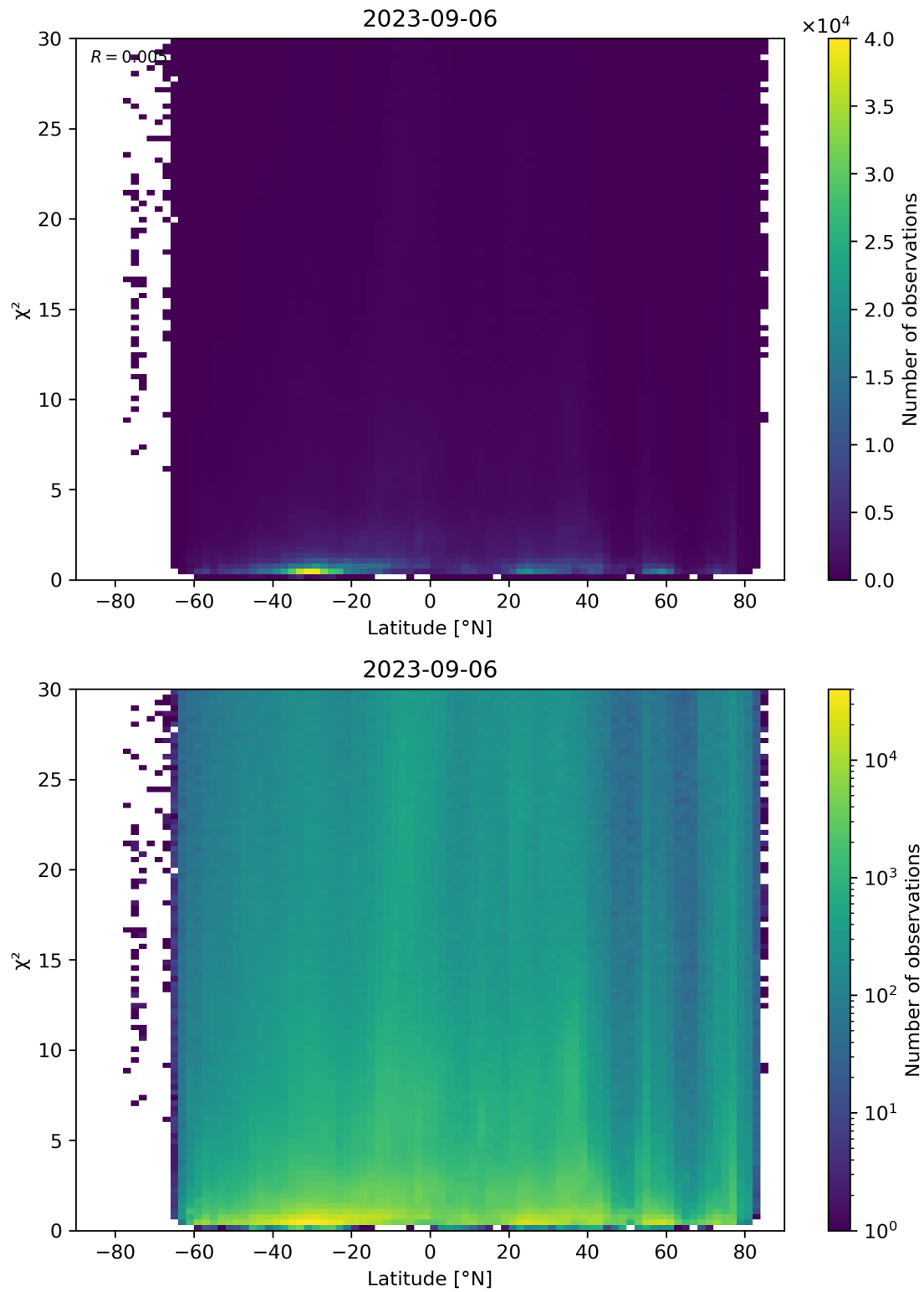
Figure 97: Scatter density plot of “Latitude” against “ \chi^2 ” for 2023-09-05 to 2023-09-07.
