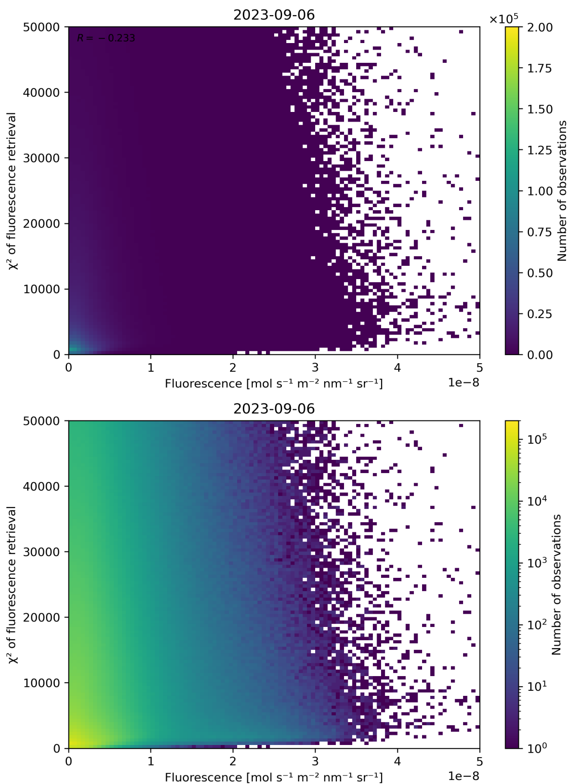
Figure 93: Scatter density plot of “Fluorescence” against “ \chi^2 of fluorescence retrieval” for 2023-09-05 to 2023-09-07.
