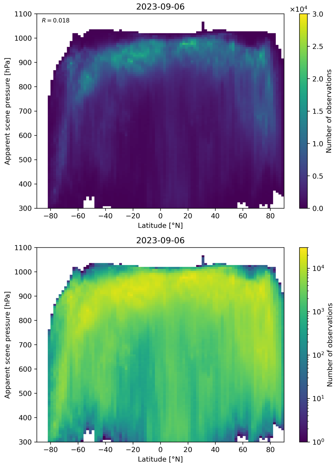
Figure 96: Scatter density plot of “Latitude” against “Apparent scene pressure” for 2023-09-05 to 2023-09-07.
