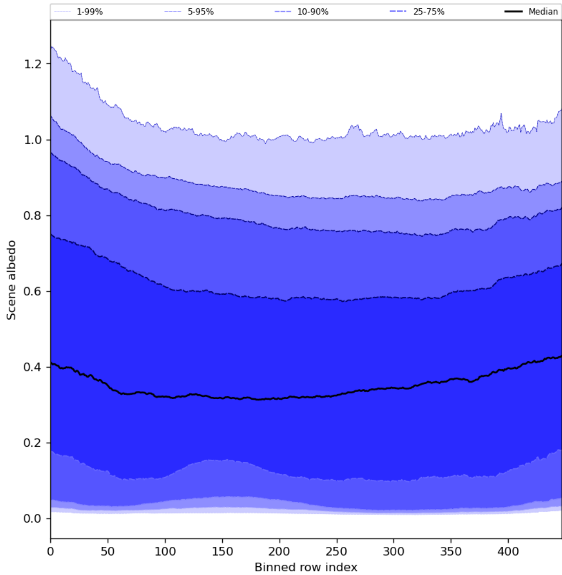
Figure 51: Along track statistics of “Scene albedo” for 2023-09-05 to 2023-09-07
