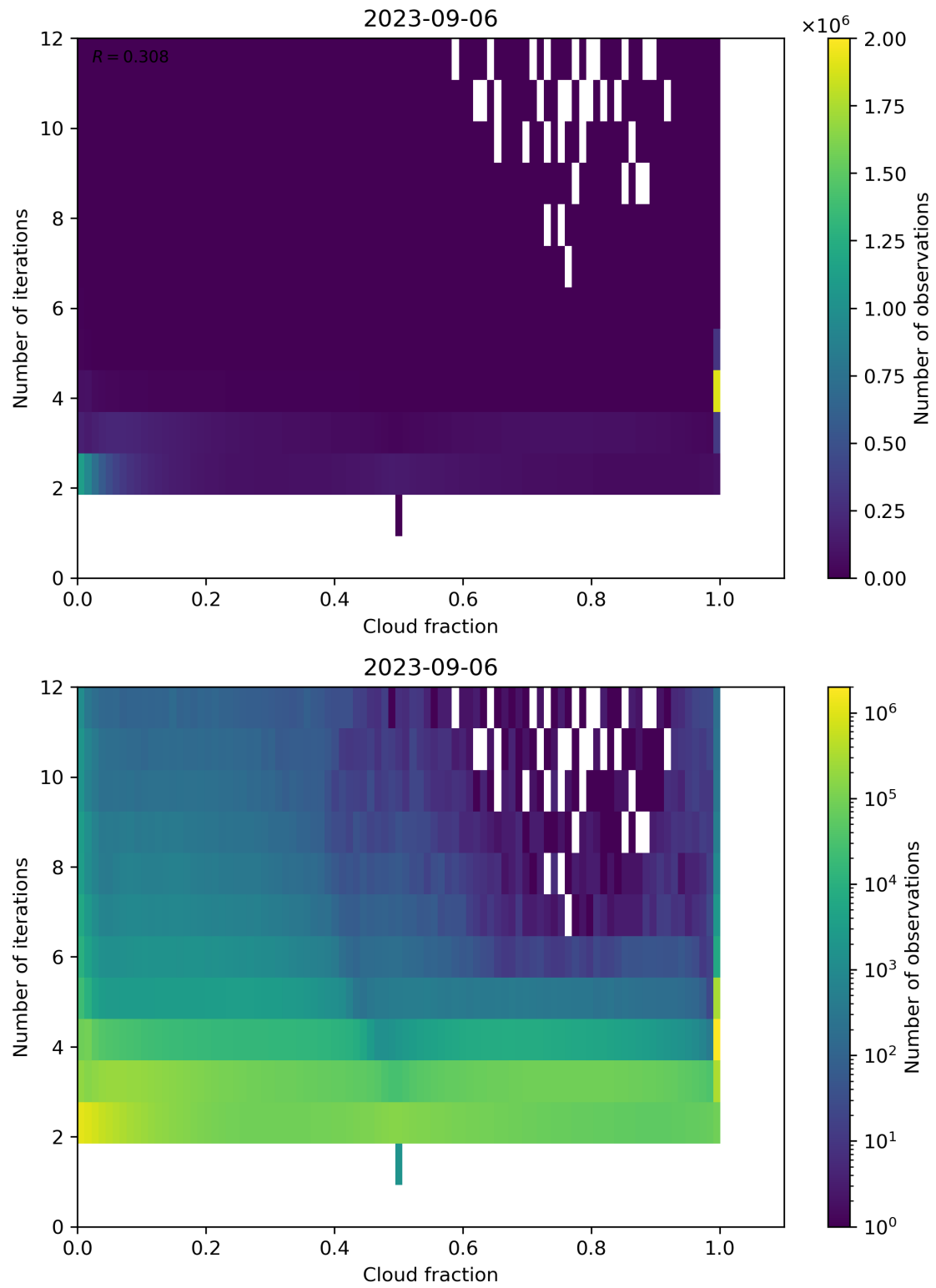
Figure 80: Scatter density plot of “Cloud fraction” against “Number of iterations” for 2023-09-05 to 2023-09-07.
