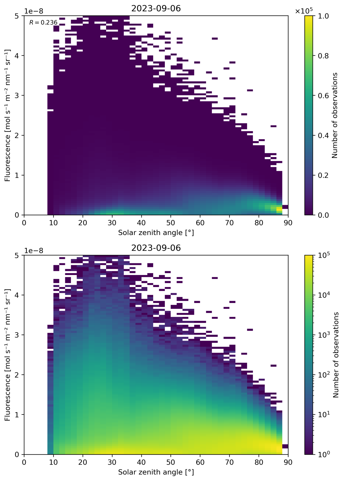
Figure 123: Scatter density plot of “Solar zenith angle” against “Fluorescence” for 2023-09-05 to 2023-09-07.
