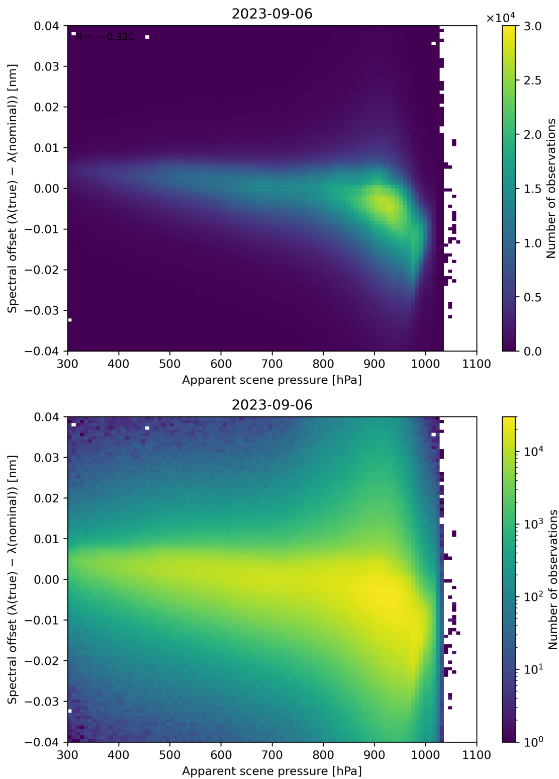
Figure 68: Scatter density plot of “Apparent scene pressure” against “Spectral offset ( \lambda(\text{true}) - \lambda(\text{nominal}) )” for 2023-09-05 to 2023-09-07.
