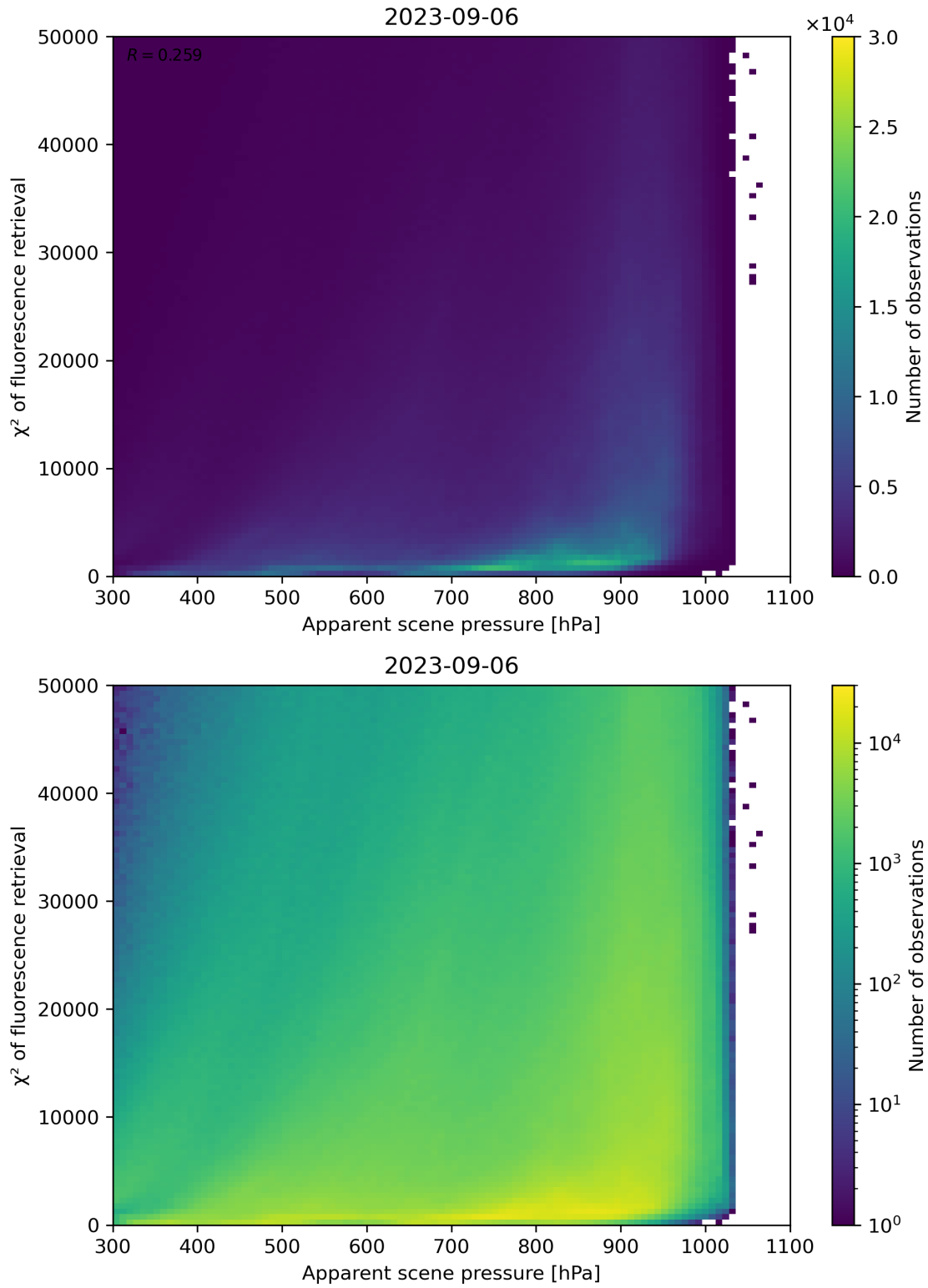
Figure 64: Scatter density plot of “Apparent scene pressure” against “ \chi^2 of fluorescence retrieval” for 2023-09-05 to 2023-09-07.
