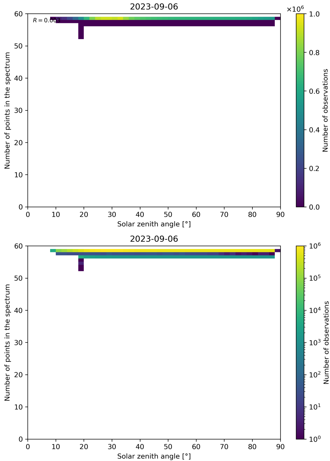
Figure 126: Scatter density plot of “Solar zenith angle” against “Number of points in the spectrum” for 2023-09-05 to 2023-09-07.
