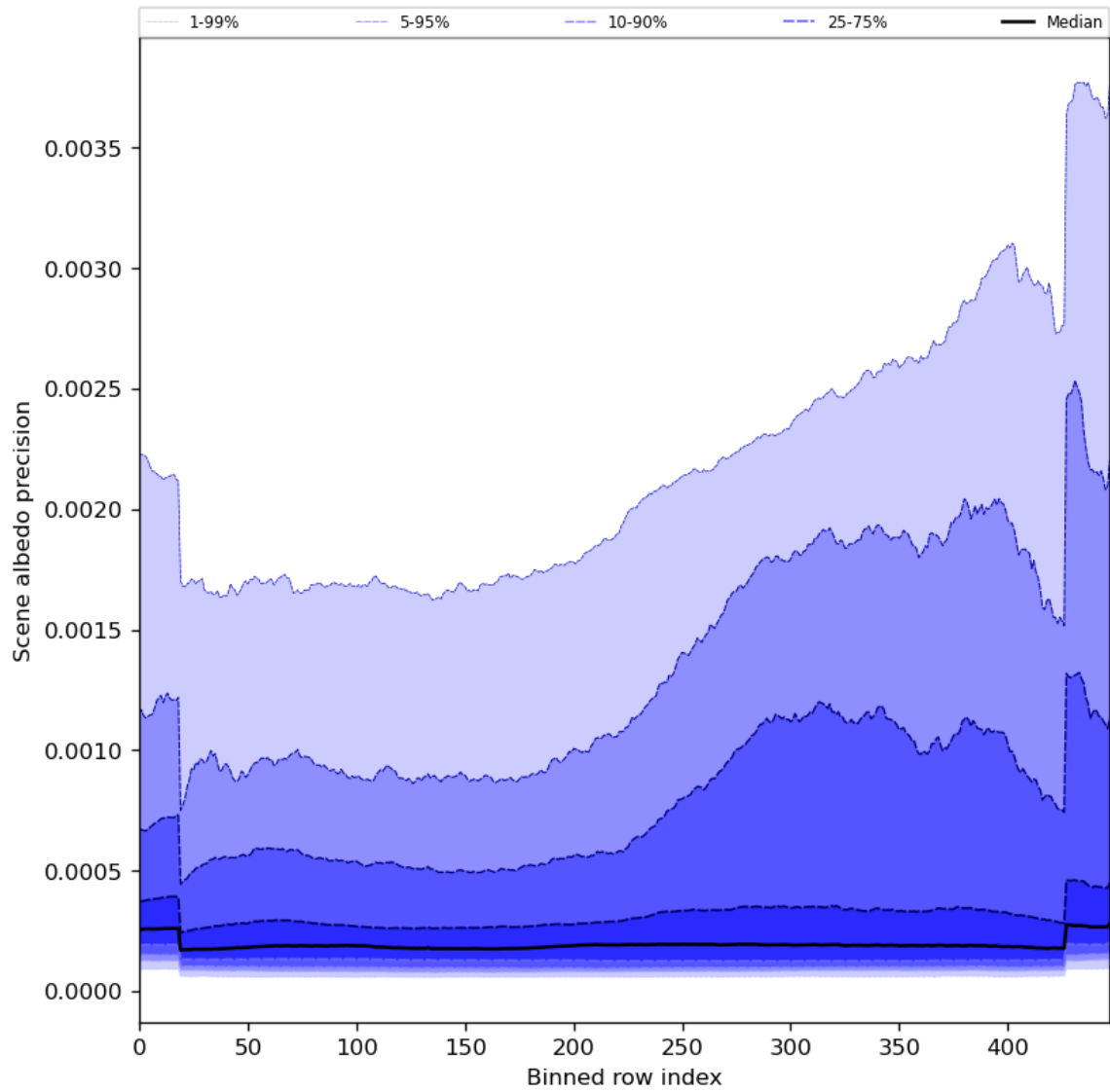
Figure 52: Along track statistics of “Scene albedo precision” for 2023-09-05 to 2023-09-07
