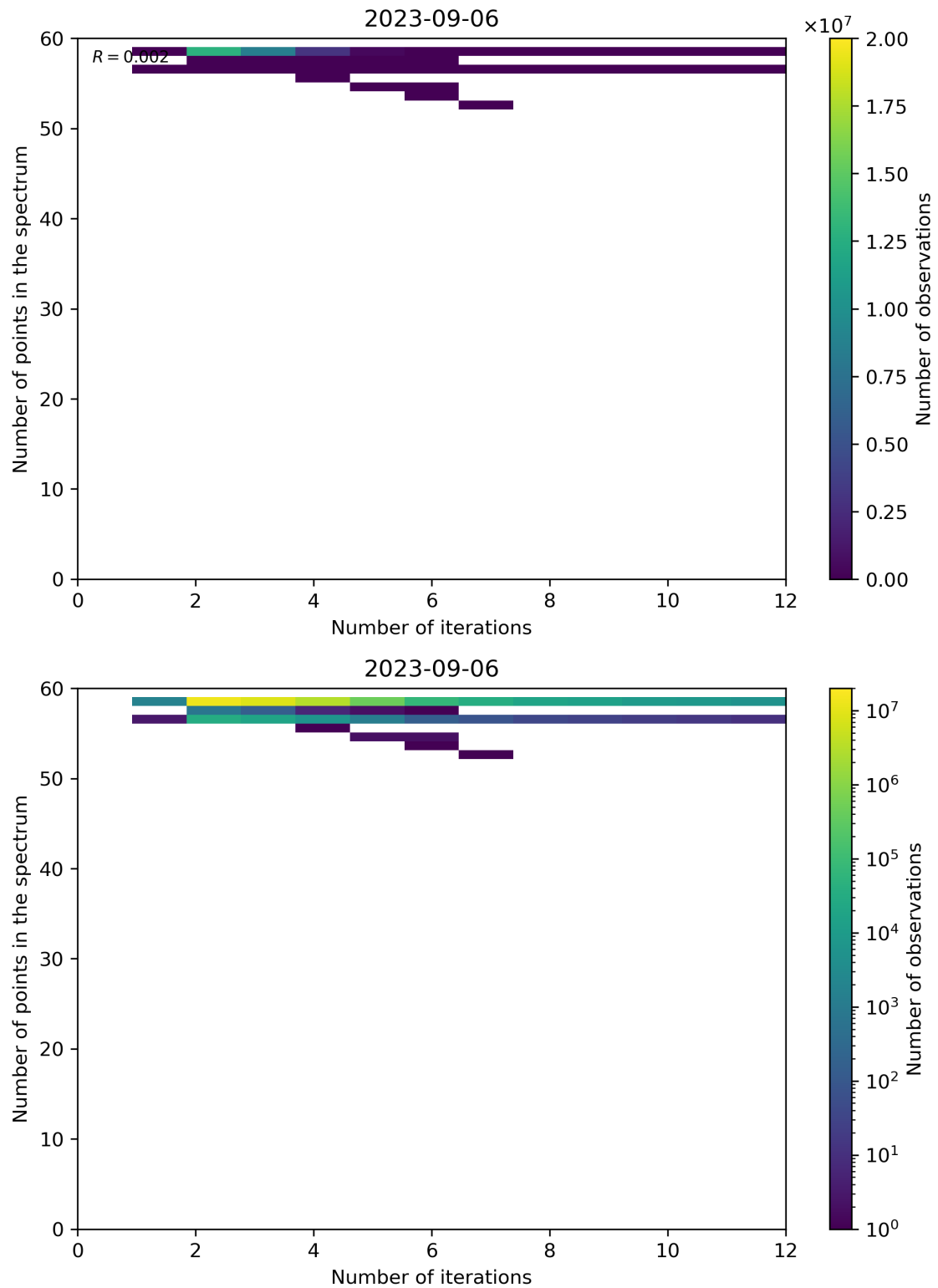
Figure 108: Scatter density plot of “Number of iterations” against “Number of points in the spectrum” for 2023-09-05 to 2023-09-07.
