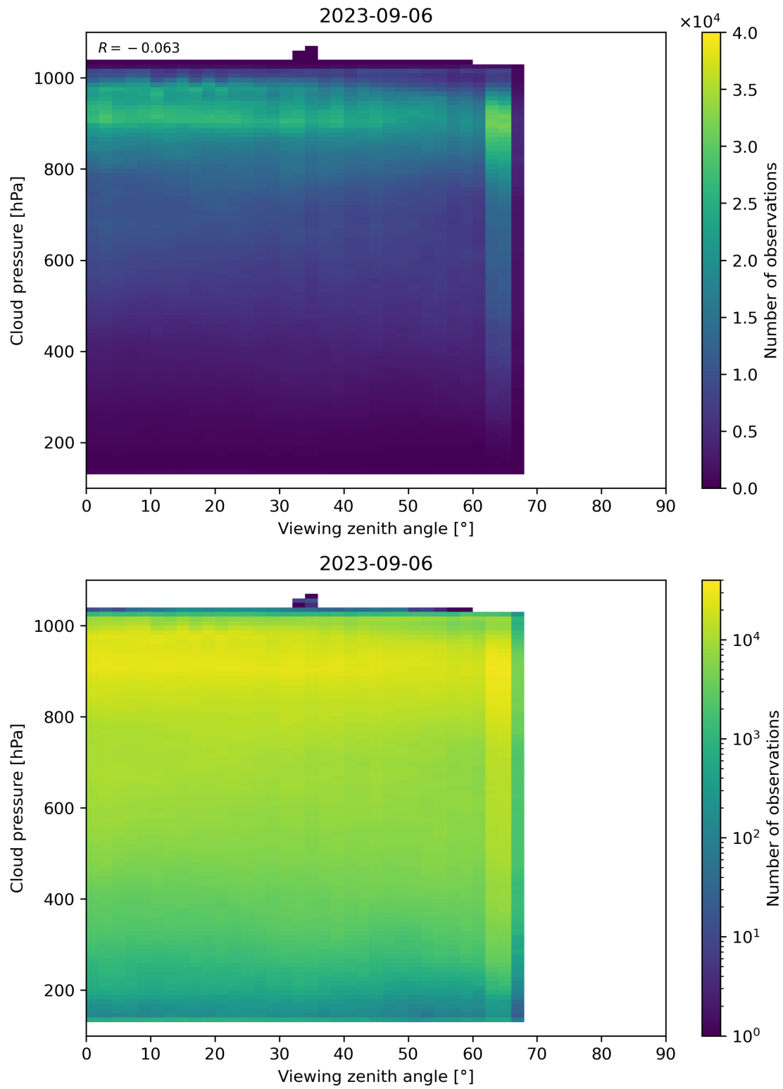
Figure 133: Scatter density plot of “Viewing zenith angle” against “Cloud pressure” for 2023-09-05 to 2023-09-07.
