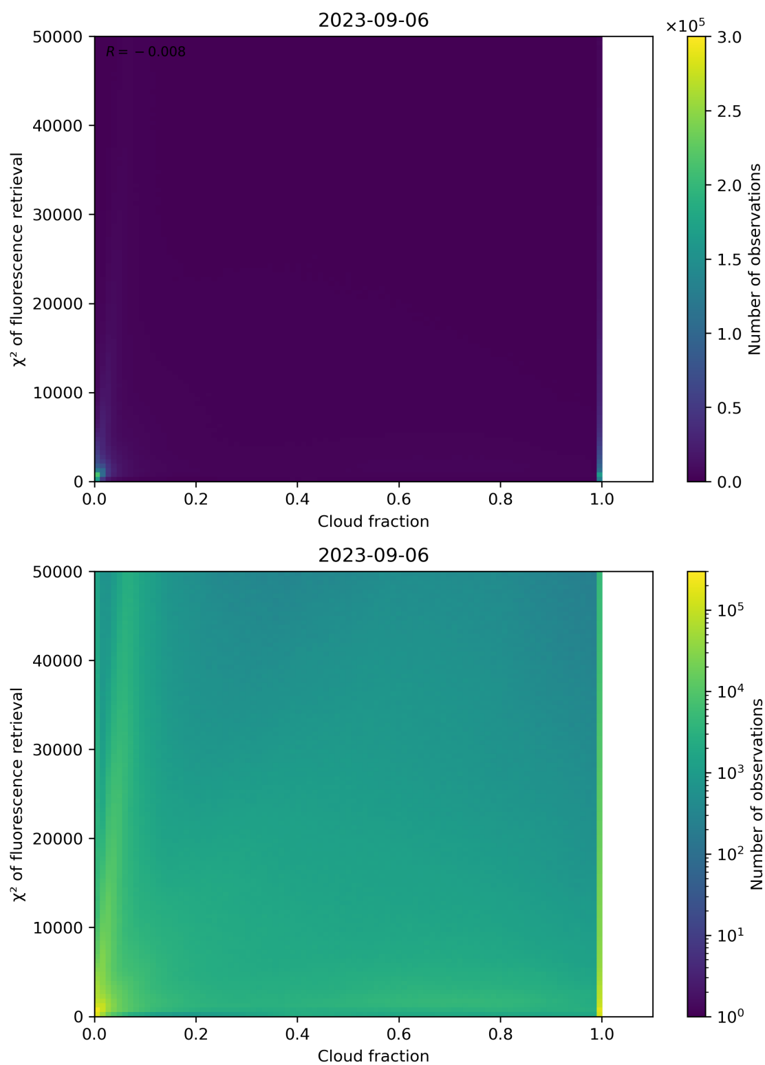
Figure 78: Scatter density plot of “Cloud fraction” against “ \chi^2 of fluorescence retrieval” for 2023-09-05 to 2023-09-07.
