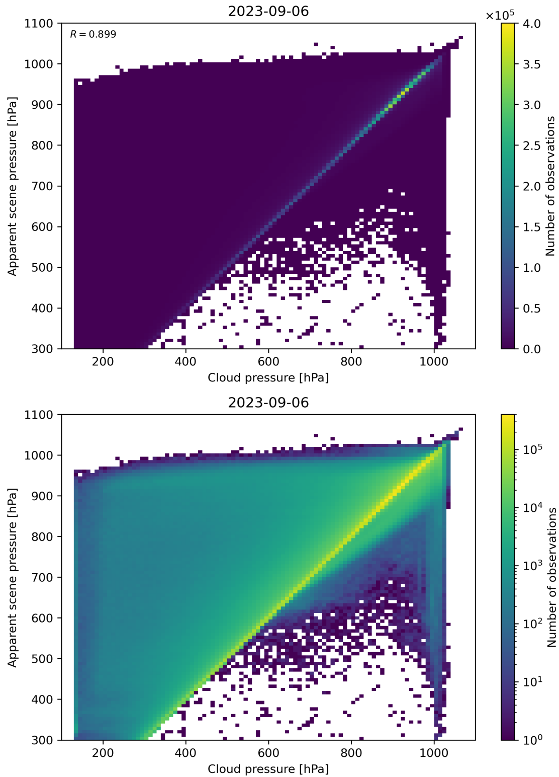
Figure 84: Scatter density plot of “Cloud pressure” against “Apparent scene pressure” for 2023-09-05 to 2023-09-07.
