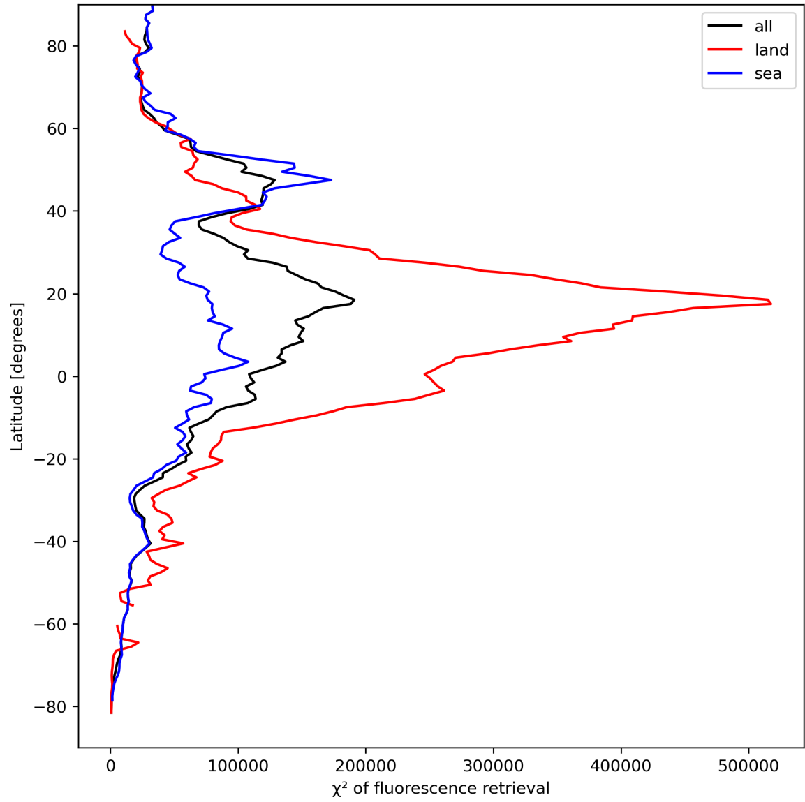
Figure 25: Zonal average of “ \chi^2 of fluorescence retrieval” for 2023-09-05 to 2023-09-07.
