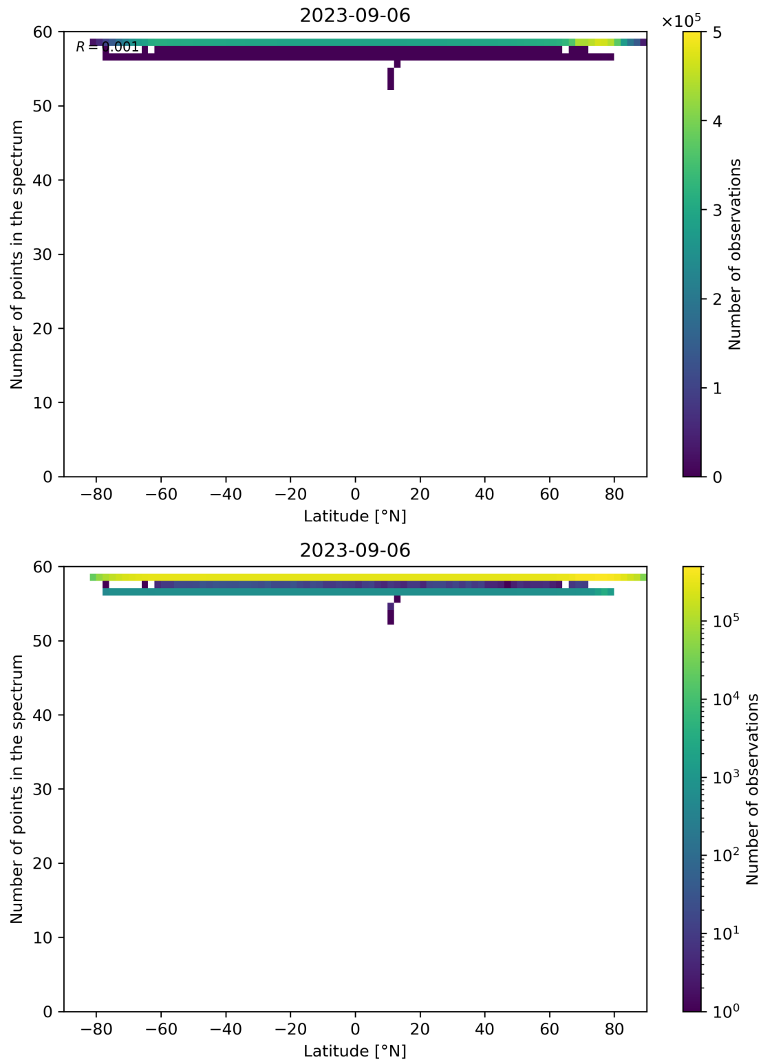
Figure 103: Scatter density plot of “Latitude” against “Number of points in the spectrum” for 2023-09-05 to 2023-09-07.
