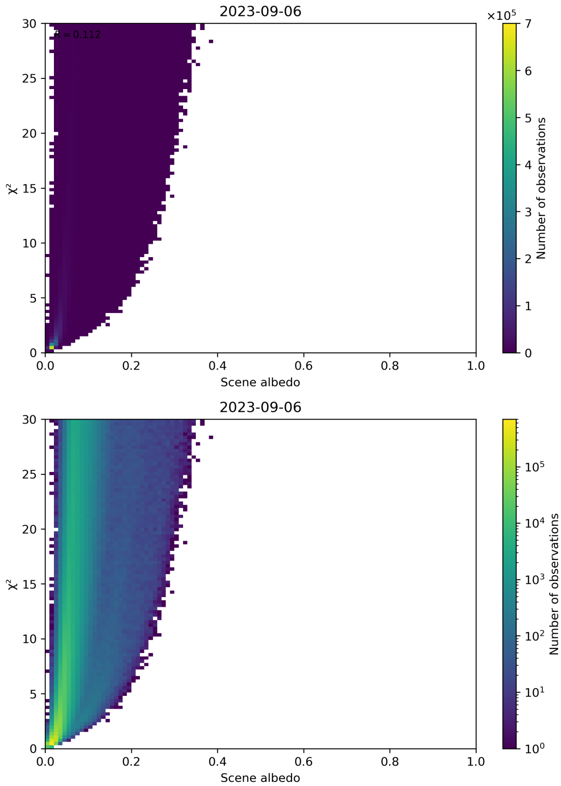
Figure 112: Scatter density plot of “Scene albedo” against “ \chi^2 ” for 2023-09-05 to 2023-09-07.
