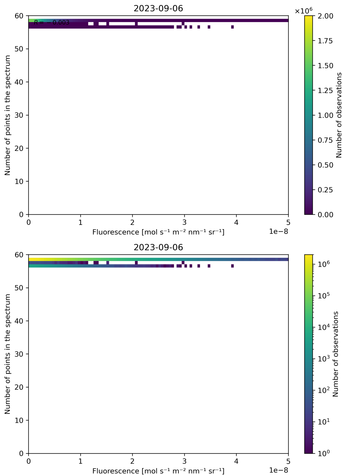
Figure 94: Scatter density plot of “Fluorescence” against “Number of points in the spectrum” for 2023-09-05 to 2023-09-07.
