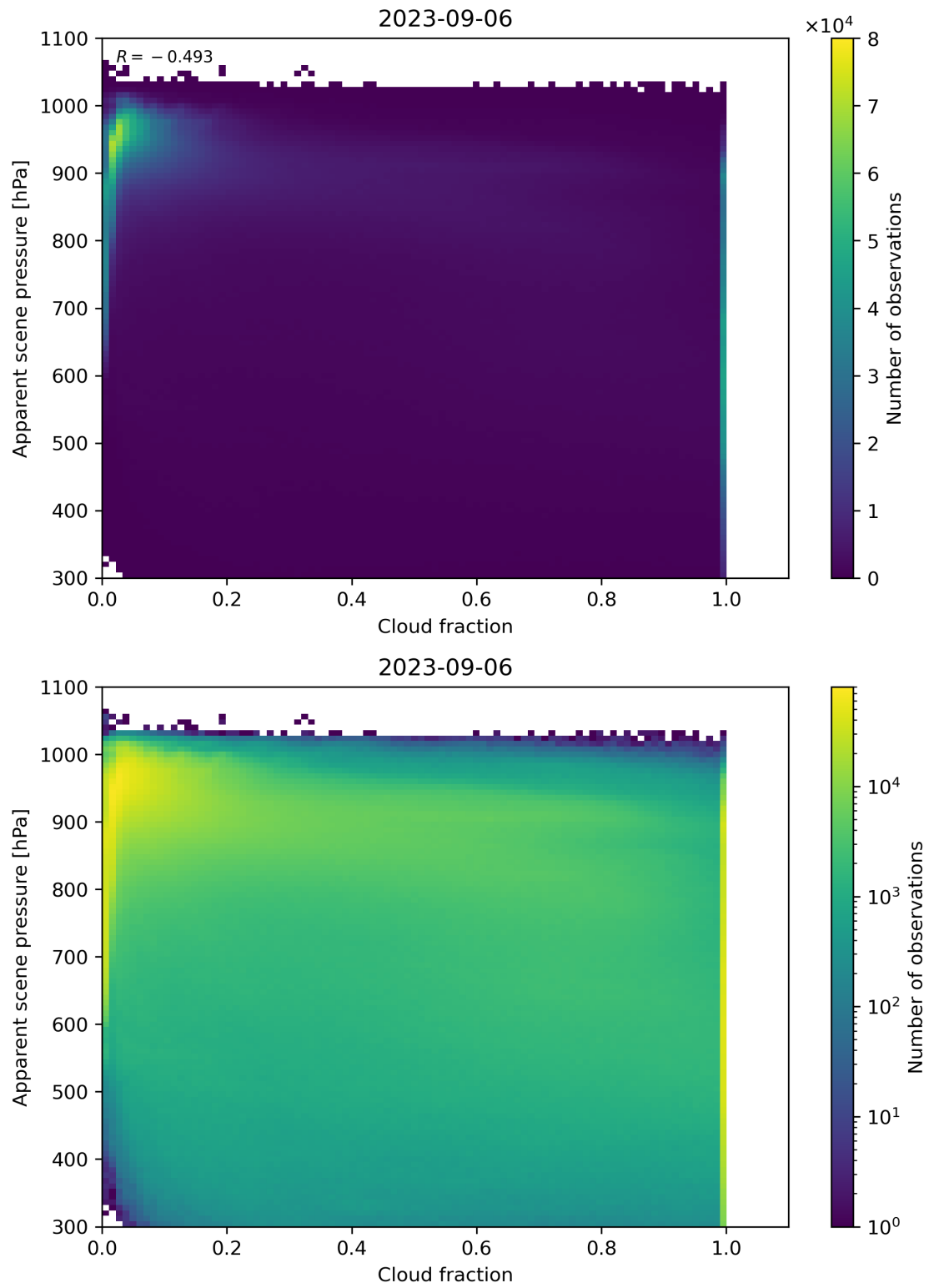
Figure 76: Scatter density plot of “Cloud fraction” against “Apparent scene pressure” for 2023-09-05 to 2023-09-07.
