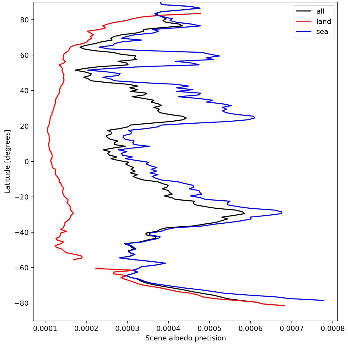
Figure 18: Zonal average of “Scene albedo precision” for 2023-09-05 to 2023-09-07.
