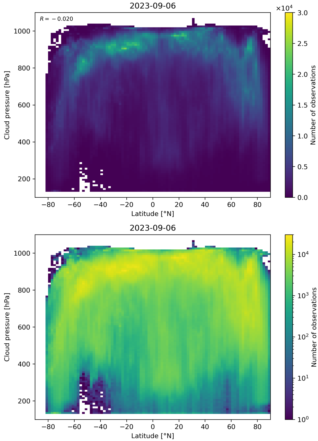
Figure 100: Scatter density plot of “Latitude” against “Cloud pressure” for 2023-09-05 to 2023-09-07.
