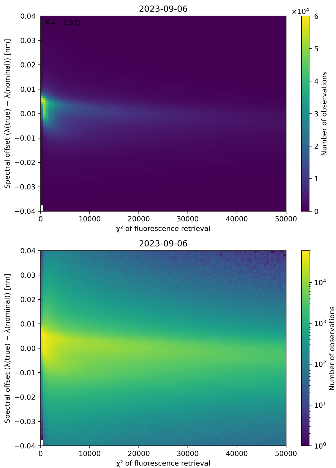
Figure 72: Scatter density plot of " \chi^2 of fluorescence retrieval" against "Spectral offset ( \lambda(\text{true}) - \lambda(\text{nominal})) " for 2023-09-05 to 2023-09-07.
