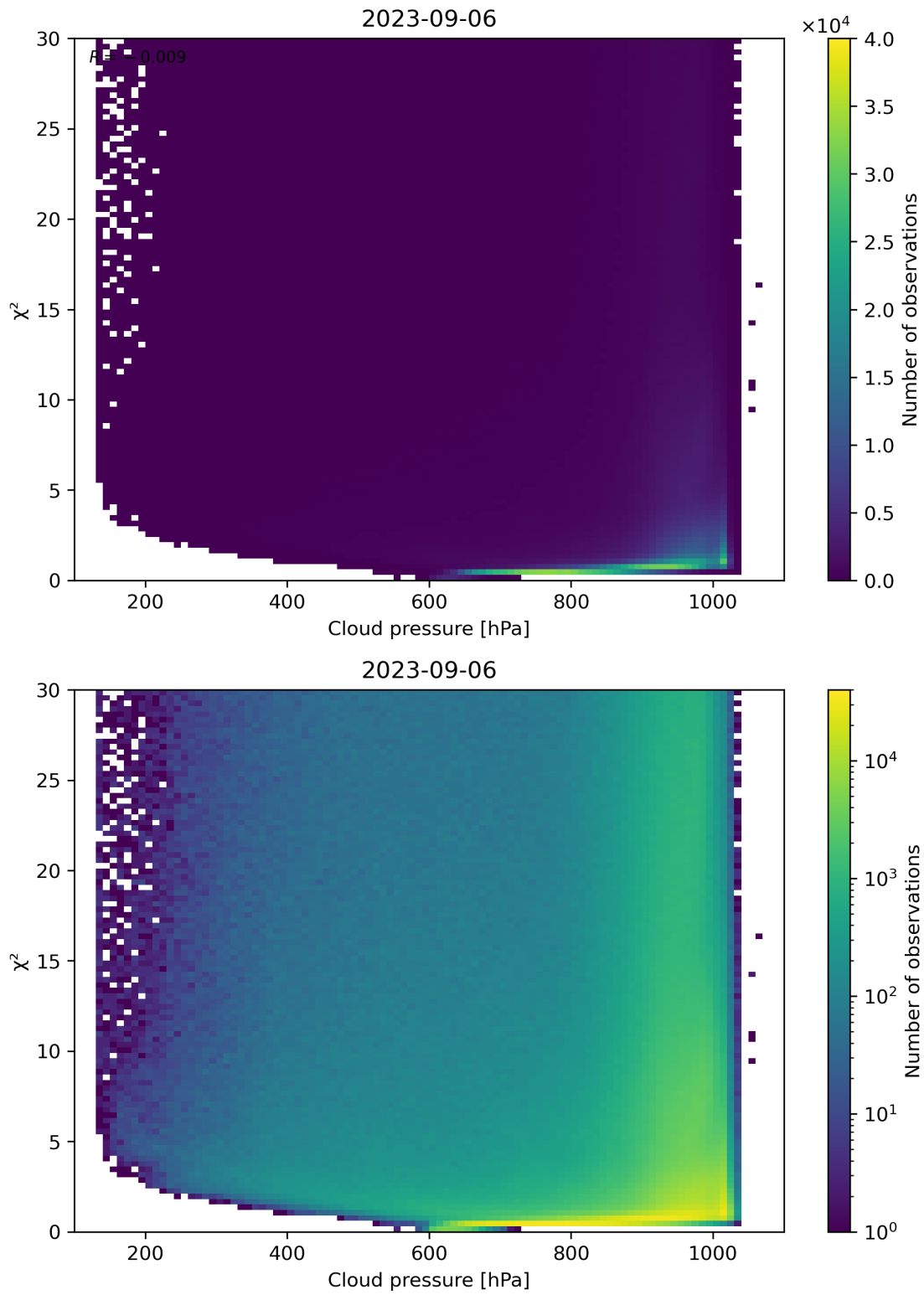
Figure 85: Scatter density plot of “Cloud pressure” against “ \chi^2 ” for 2023-09-05 to 2023-09-07.
