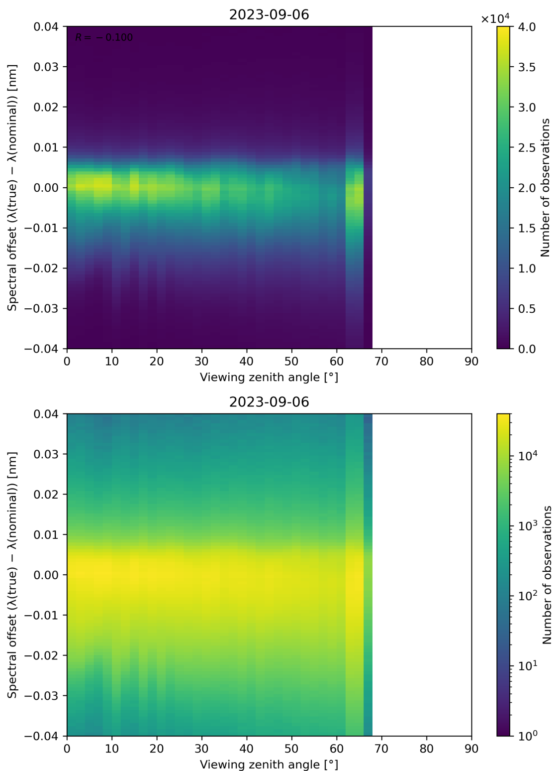
Figure 140: Scatter density plot of “Viewing zenith angle” against “Spectral offset ( \lambda(\text{true}) - \lambda(\text{nominal}) )” for 2023-09-05 to 2023-09-07.
