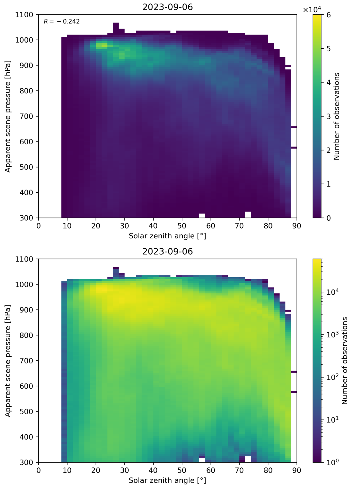
Figure 118: Scatter density plot of “Solar zenith angle” against “Apparent scene pressure” for 2023-09-05 to 2023-09-07.
