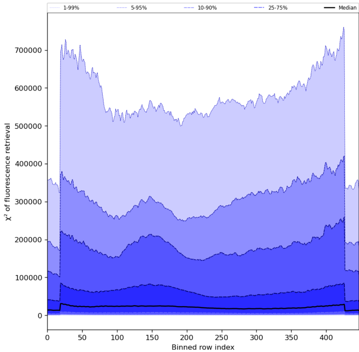
Figure 59: Along track statistics of “ \chi^2 of fluorescence retrieval” for 2023-09-05 to 2023-09-07
