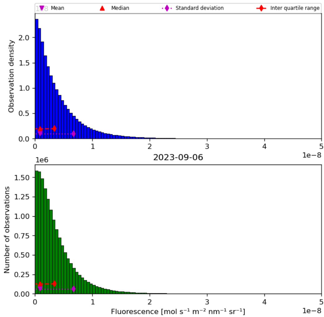
Figure 40: Histogram of “Fluorescence” for 2023-09-05 to 2023-09-07
