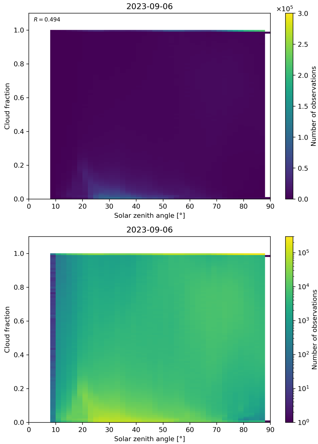
Figure 121: Scatter density plot of “Solar zenith angle” against “Cloud fraction” for 2023-09-05 to 2023-09-07.
