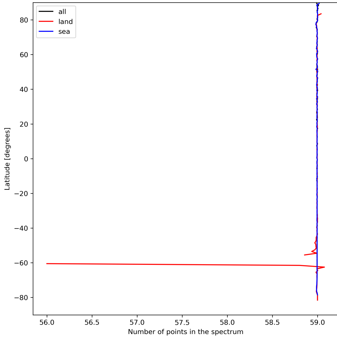
Figure 27: Zonal average of “Number of points in the spectrum” for 2023-09-05 to 2023-09-07.
