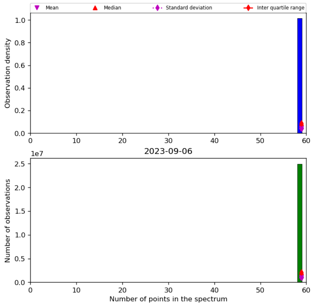
Figure 44: Histogram of “Number of points in the spectrum” for 2023-09-05 to 2023-09-07
