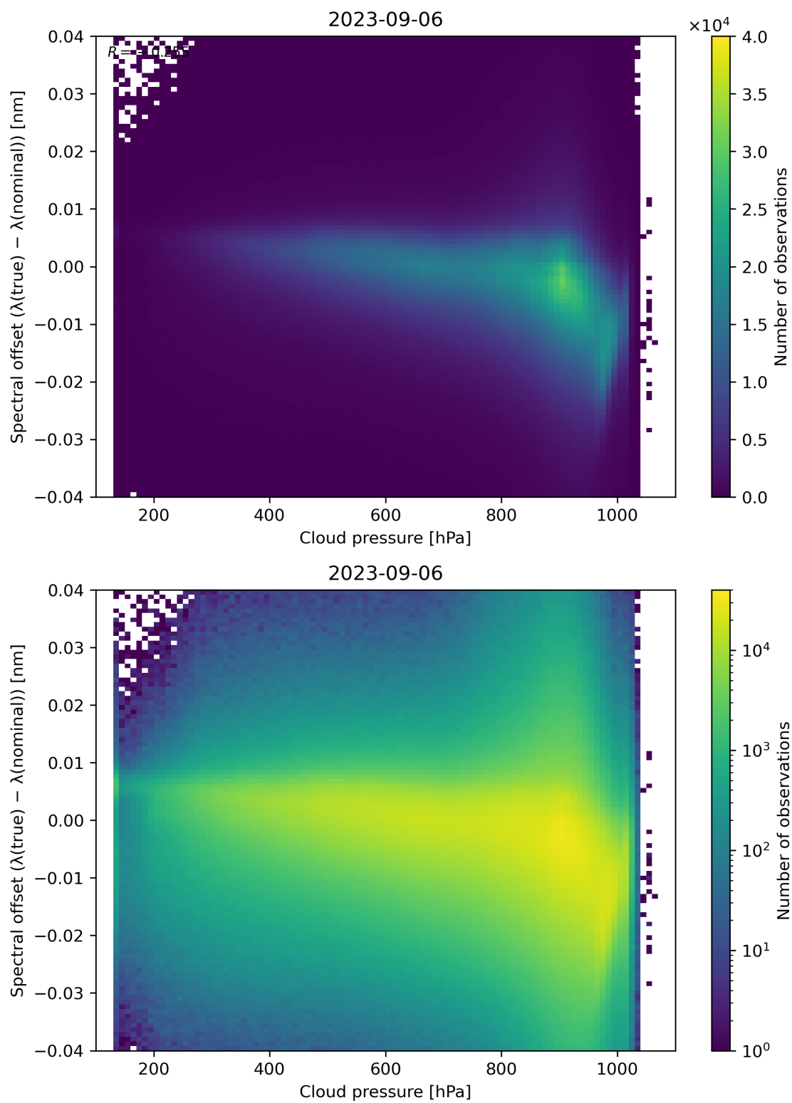
Figure 92: Scatter density plot of “Cloud pressure” against “Spectral offset ( \lambda(\text{true}) - \lambda(\text{nominal}) )” for 2023-09-05 to 2023-09-07.
