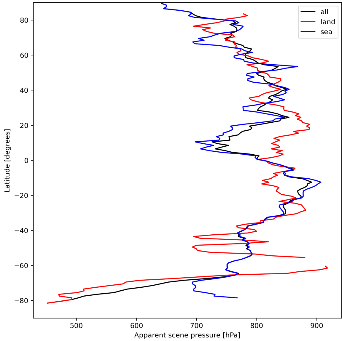
Figure 19: Zonal average of “Apparent scene pressure” for 2023-09-05 to 2023-09-07.
