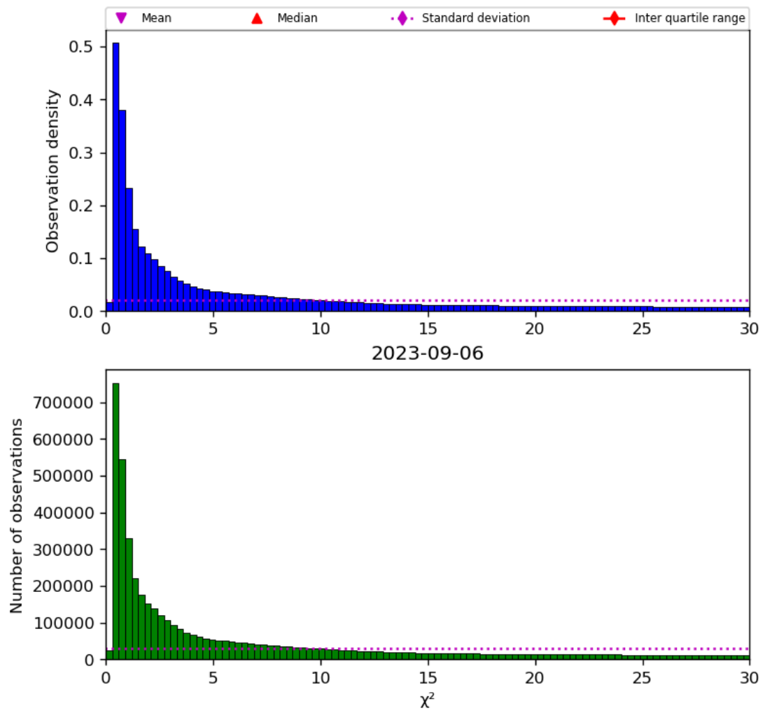
Figure 38: Histogram of “ \chi^2 ” for 2023-09-05 to 2023-09-07
