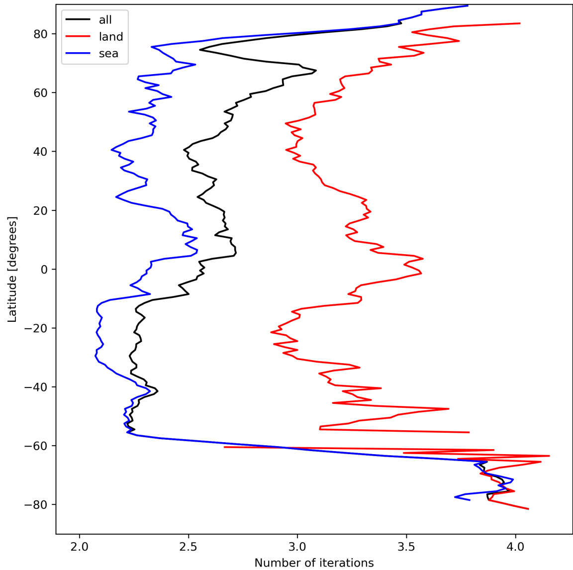
Figure 22: Zonal average of “Number of iterations” for 2023-09-05 to 2023-09-07.
