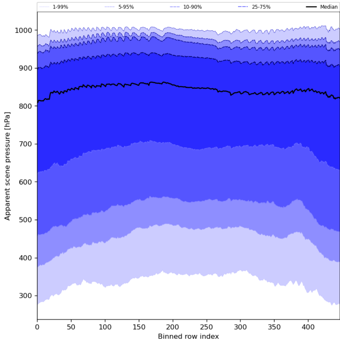
Figure 53: Along track statistics of “Apparent scene pressure” for 2023-09-05 to 2023-09-07
