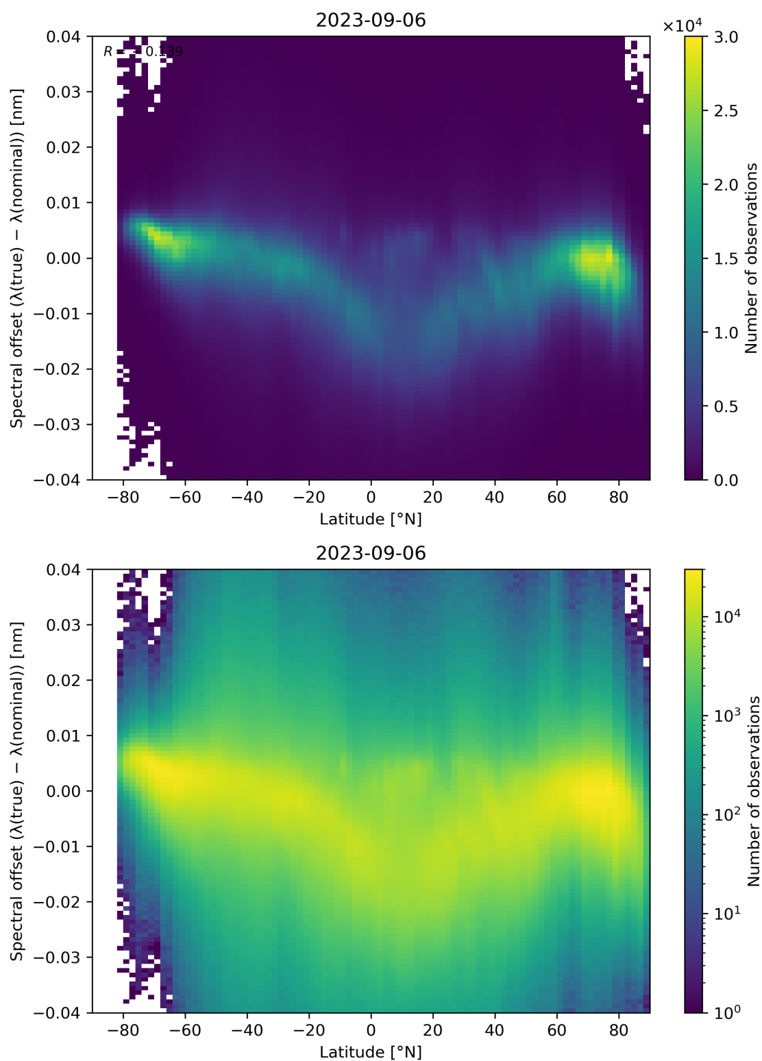
Figure 105: Scatter density plot of “Latitude” against “Spectral offset ( \lambda(\text{true}) - \lambda(\text{nominal}) )” for 2023-09-05 to 2023-09-07.
