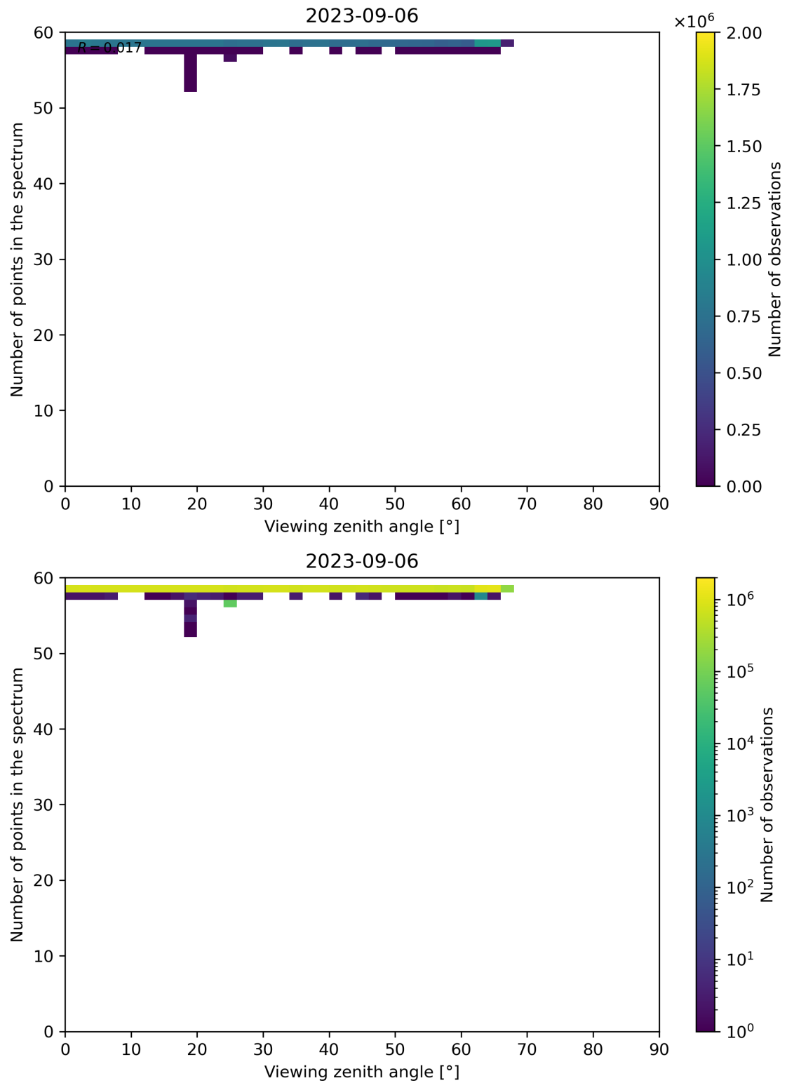
Figure 137: Scatter density plot of “Viewing zenith angle” against “Number of points in the spectrum” for 2023-09-05 to 2023-09-07.
