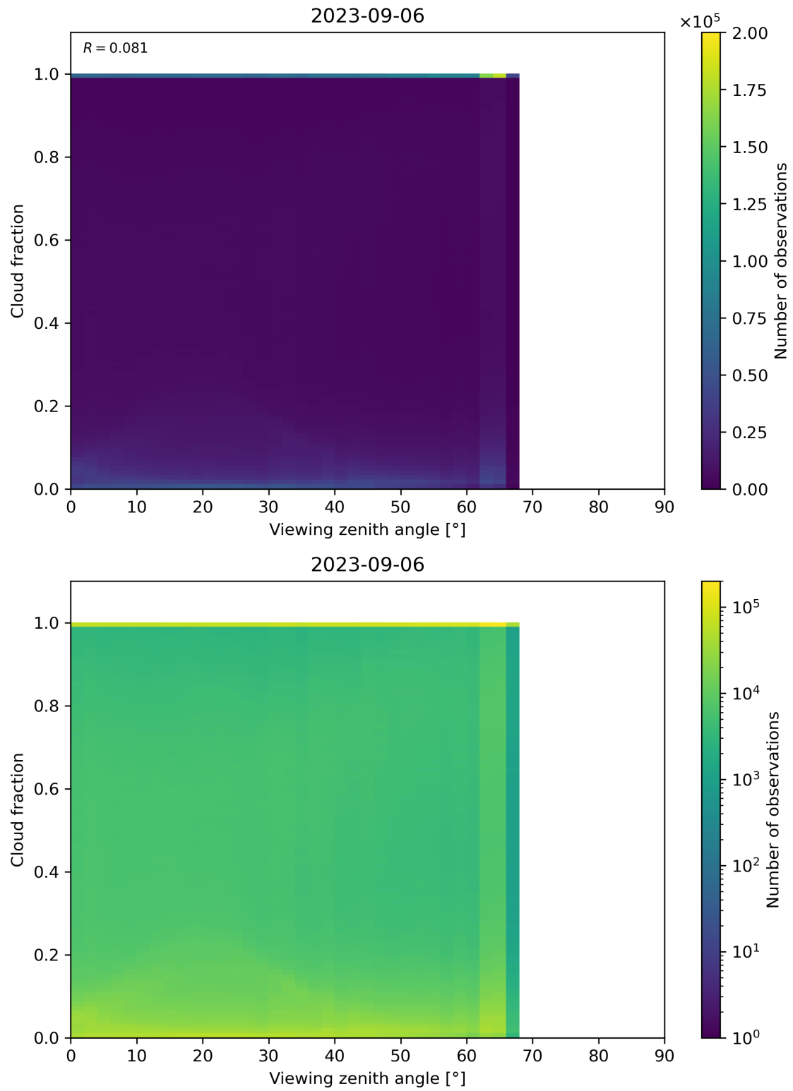
Figure 132: Scatter density plot of “Viewing zenith angle” against “Cloud fraction” for 2023-09-05 to 2023-09-07.
