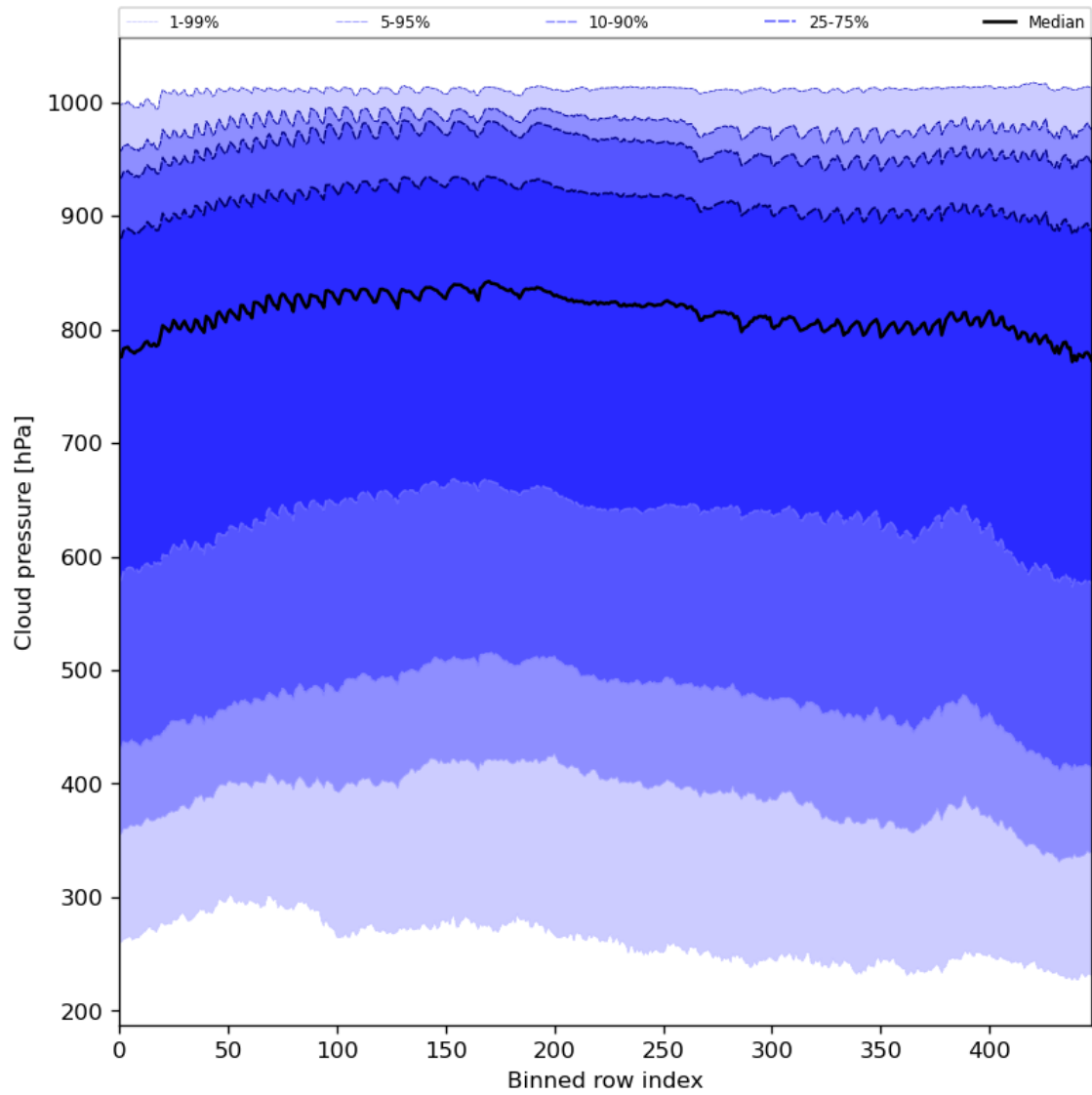
Figure 47: Along track statistics of “Cloud pressure” for 2023-09-05 to 2023-09-07
