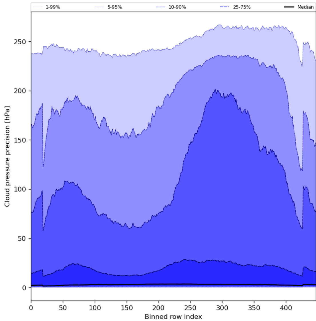
Figure 48: Along track statistics of “Cloud pressure precision” for 2023-09-05 to 2023-09-07
