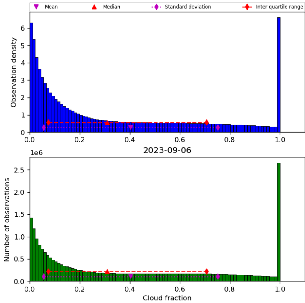
Figure 32: Histogram of “Cloud fraction” for 2023-09-05 to 2023-09-07
