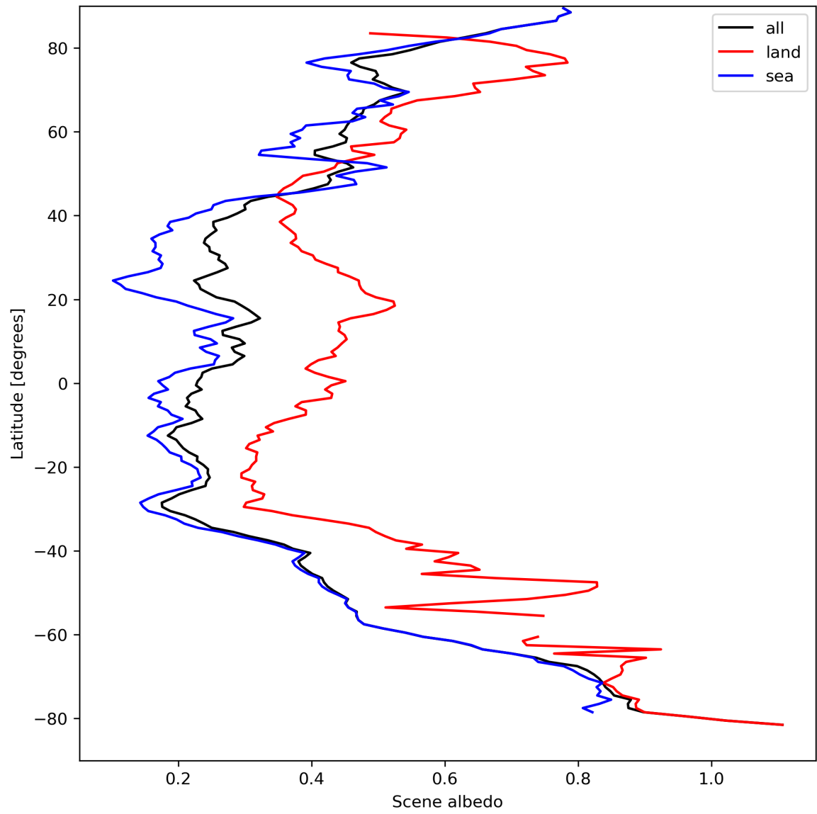
Figure 17: Zonal average of “Scene albedo” for 2023-09-05 to 2023-09-07.
