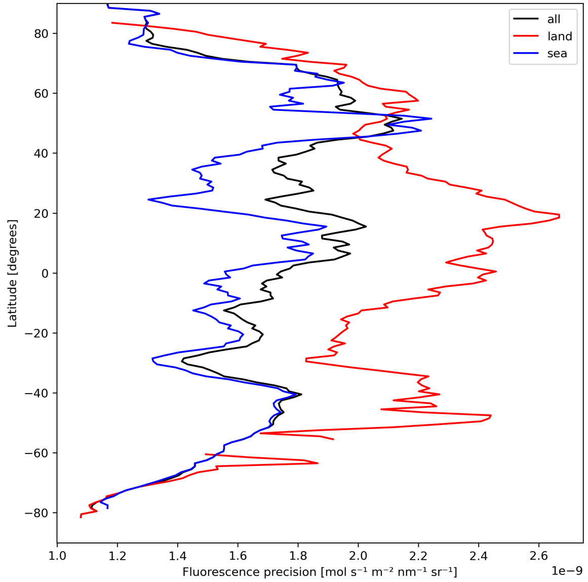
Figure 24: Zonal average of “Fluorescence precision” for 2023-09-05 to 2023-09-07.
