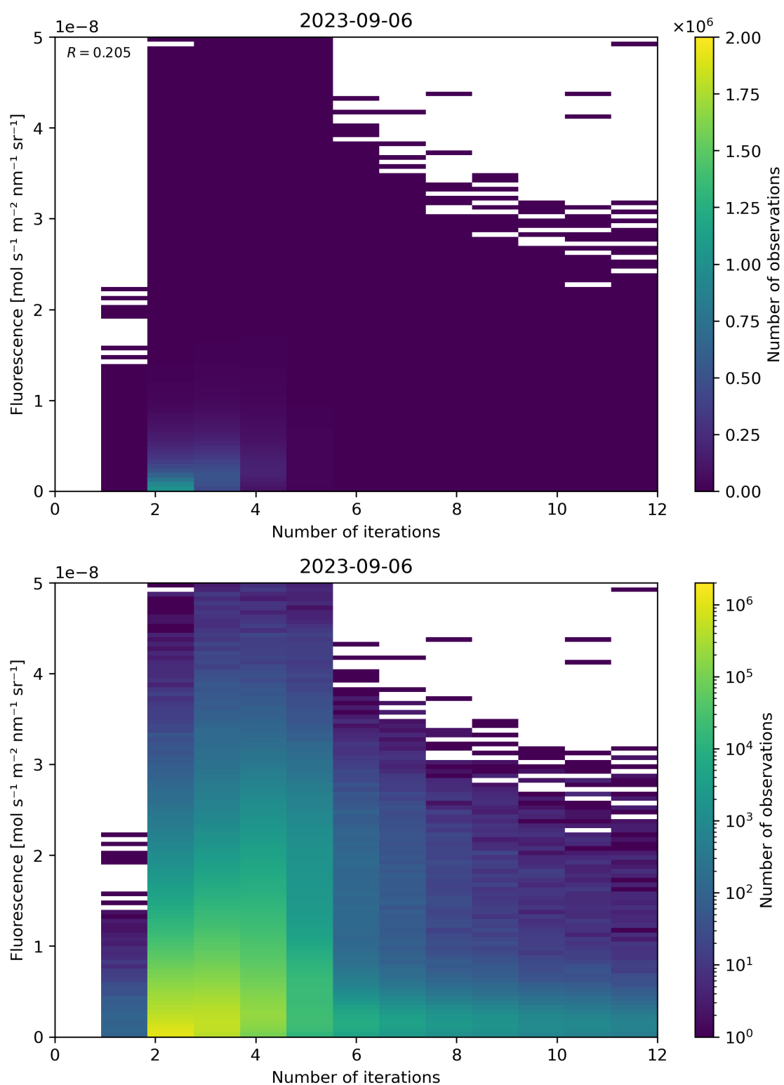
Figure 107: Scatter density plot of “Number of iterations” against “Fluorescence” for 2023-09-05 to 2023-09-07.
