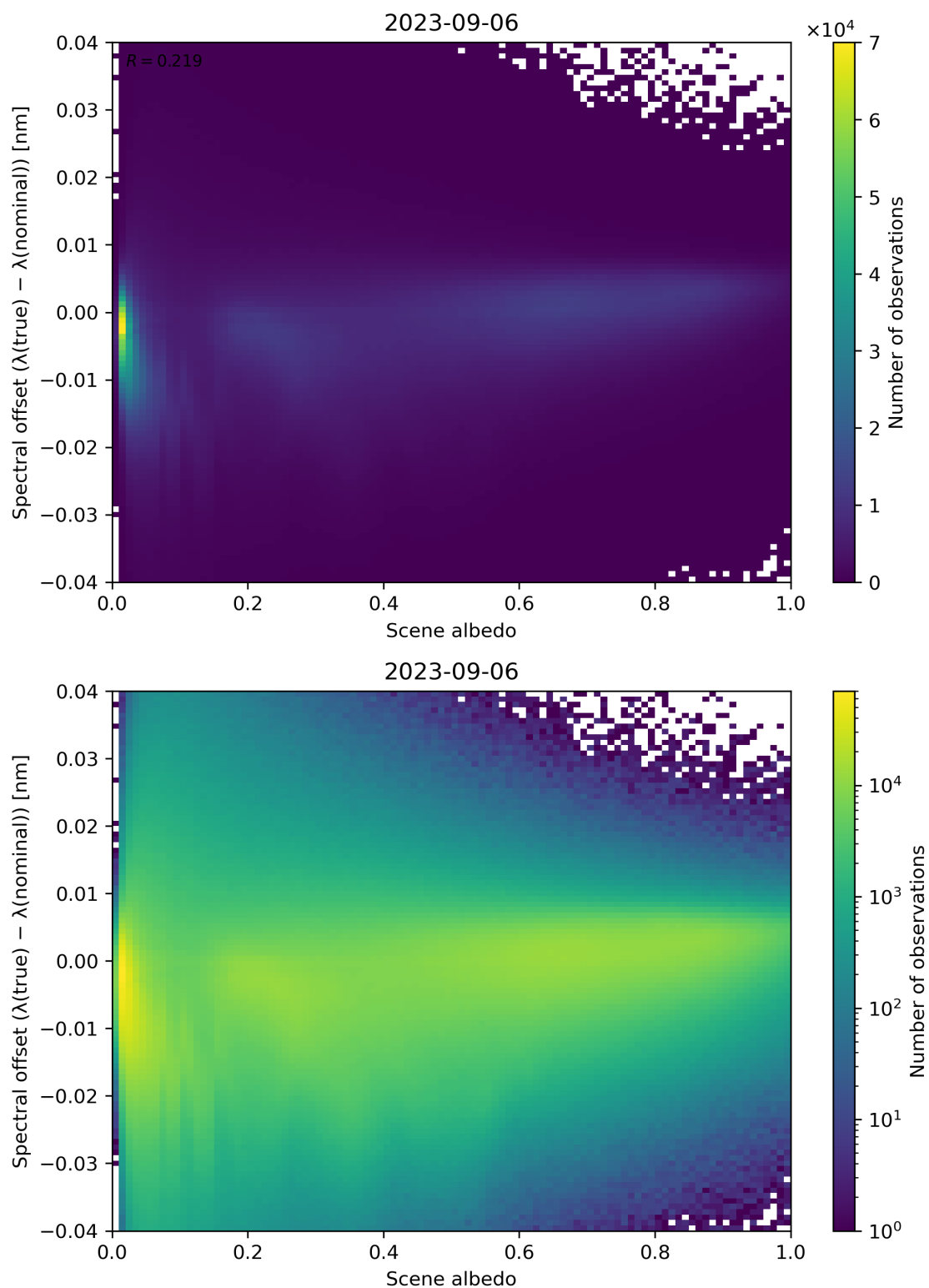
Figure 117: Scatter density plot of “Scene albedo” against “Spectral offset ( \lambda(\text{true}) - \lambda(\text{nominal}) )” for 2023-09-05 to 2023-09-07.
