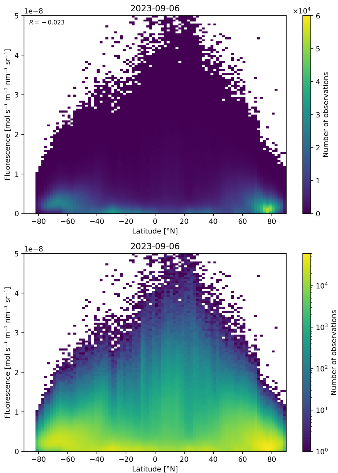
Figure 101: Scatter density plot of “Latitude” against “Fluorescence” for 2023-09-05 to 2023-09-07.
