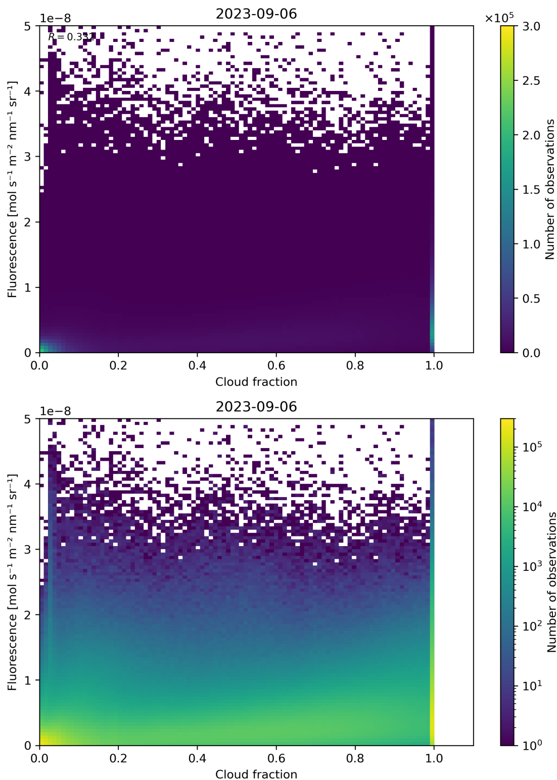
Figure 79: Scatter density plot of “Cloud fraction” against “Fluorescence” for 2023-09-05 to 2023-09-07.
