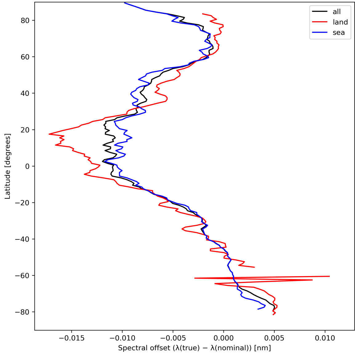
Figure 28: Zonal average of “Spectral offset ( \lambda(\text{true}) - \lambda(\text{nominal}) )” for 2023-09-05 to 2023-09-07.
