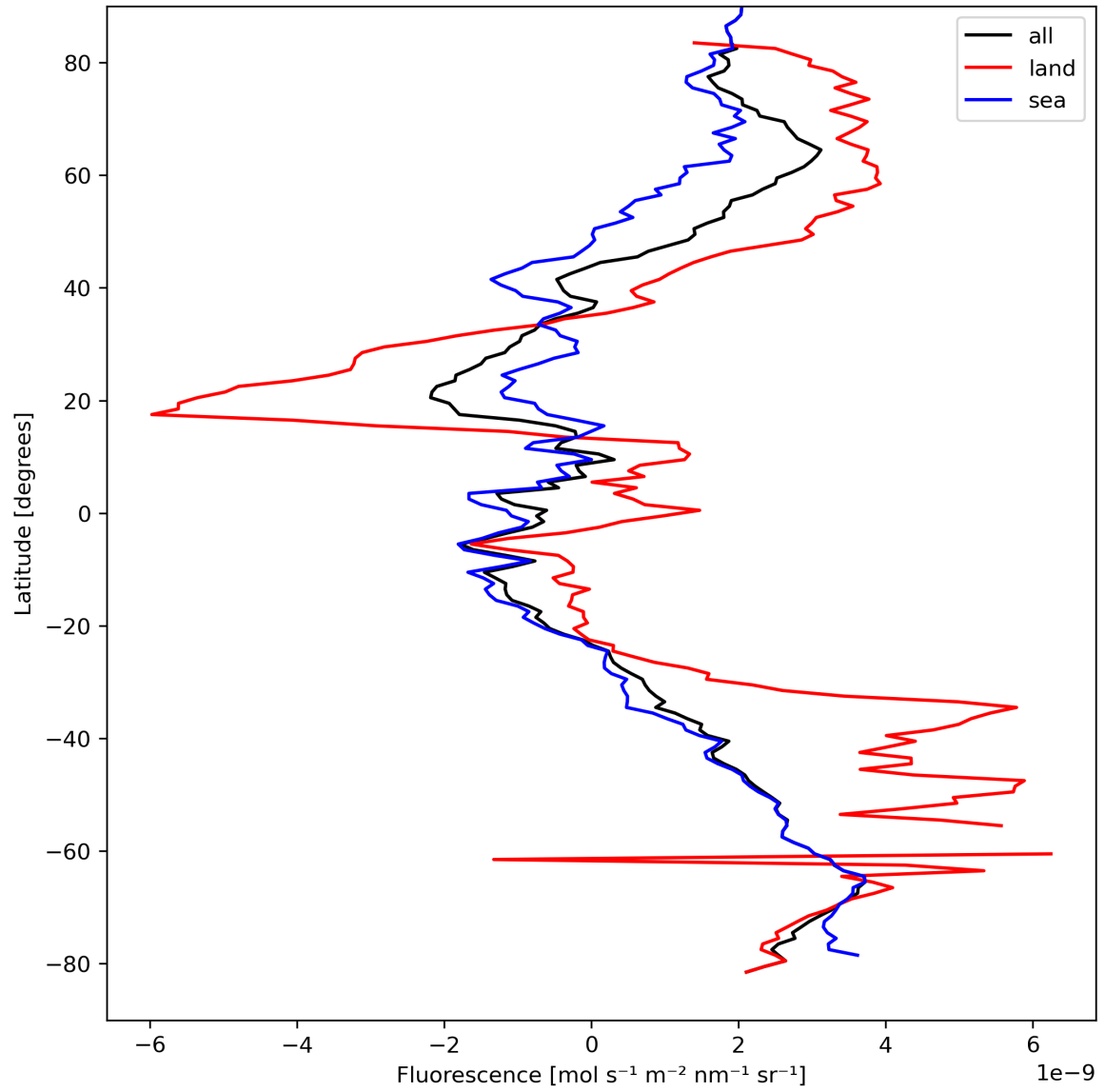
Figure 23: Zonal average of “Fluorescence” for 2023-09-05 to 2023-09-07.
