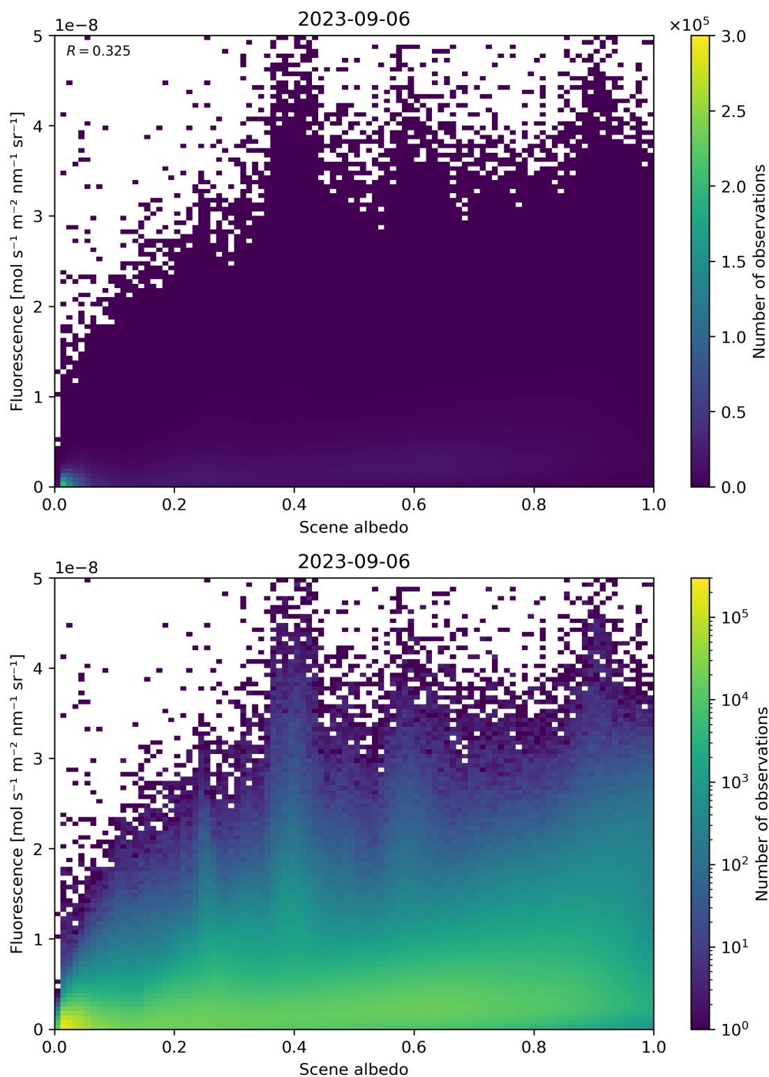
Figure 114: Scatter density plot of “Scene albedo” against “Fluorescence” for 2023-09-05 to 2023-09-07.
