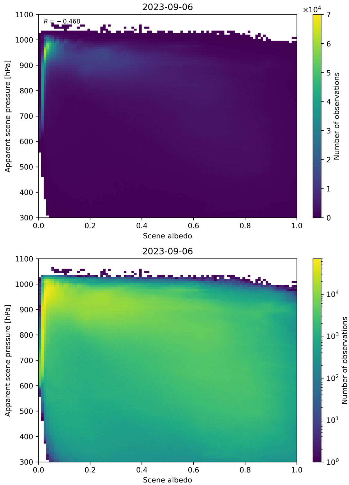
Figure 111: Scatter density plot of “Scene albedo” against “Apparent scene pressure” for 2023-09-05 to 2023-09-07.
