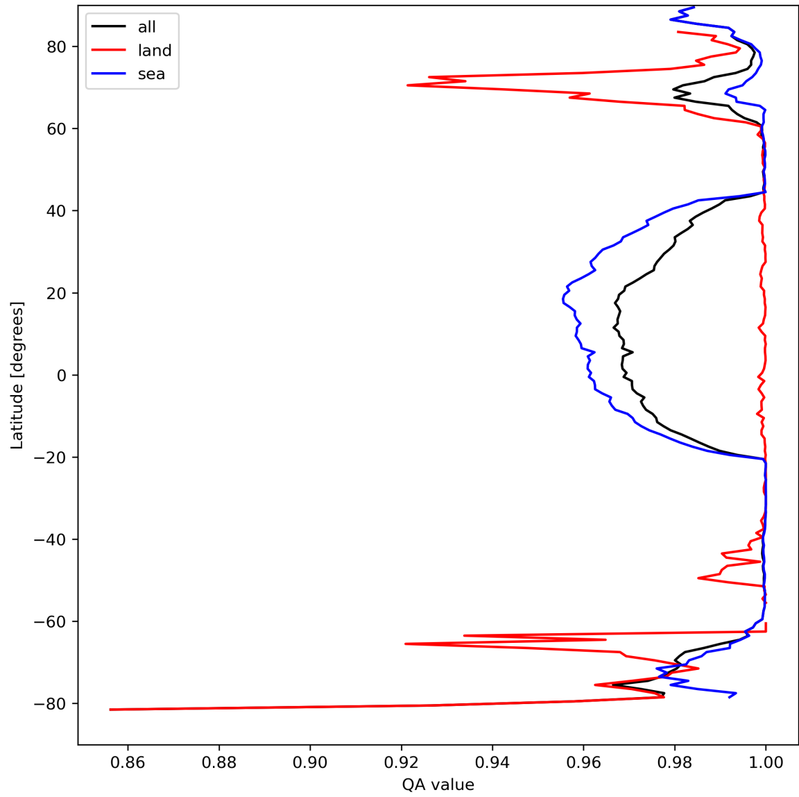
Figure 12: Zonal average of “QA value” for 2023-09-05 to 2023-09-07.
