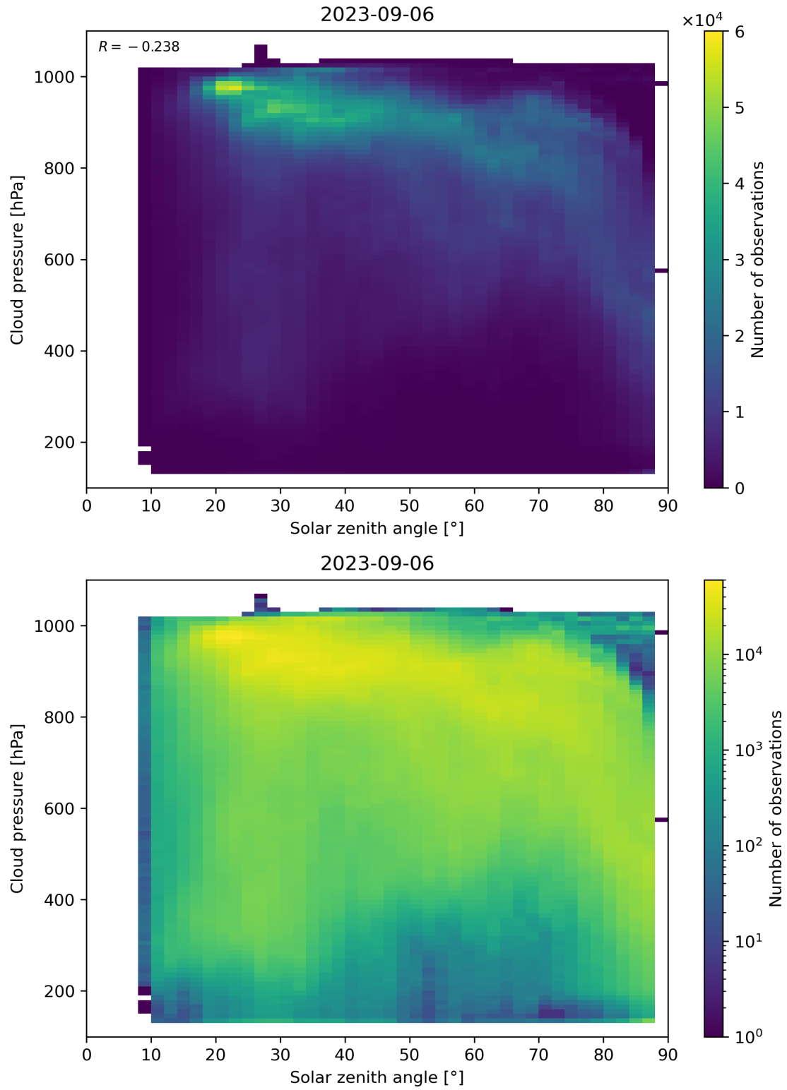
Figure 122: Scatter density plot of “Solar zenith angle” against “Cloud pressure” for 2023-09-05 to 2023-09-07.
