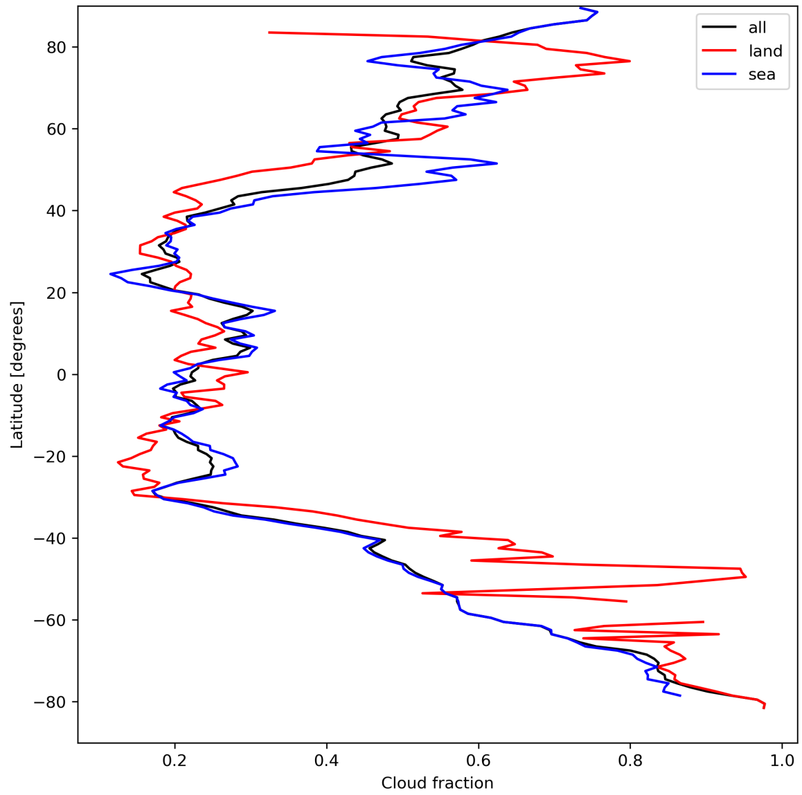
Figure 15: Zonal average of “Cloud fraction” for 2023-09-05 to 2023-09-07.
