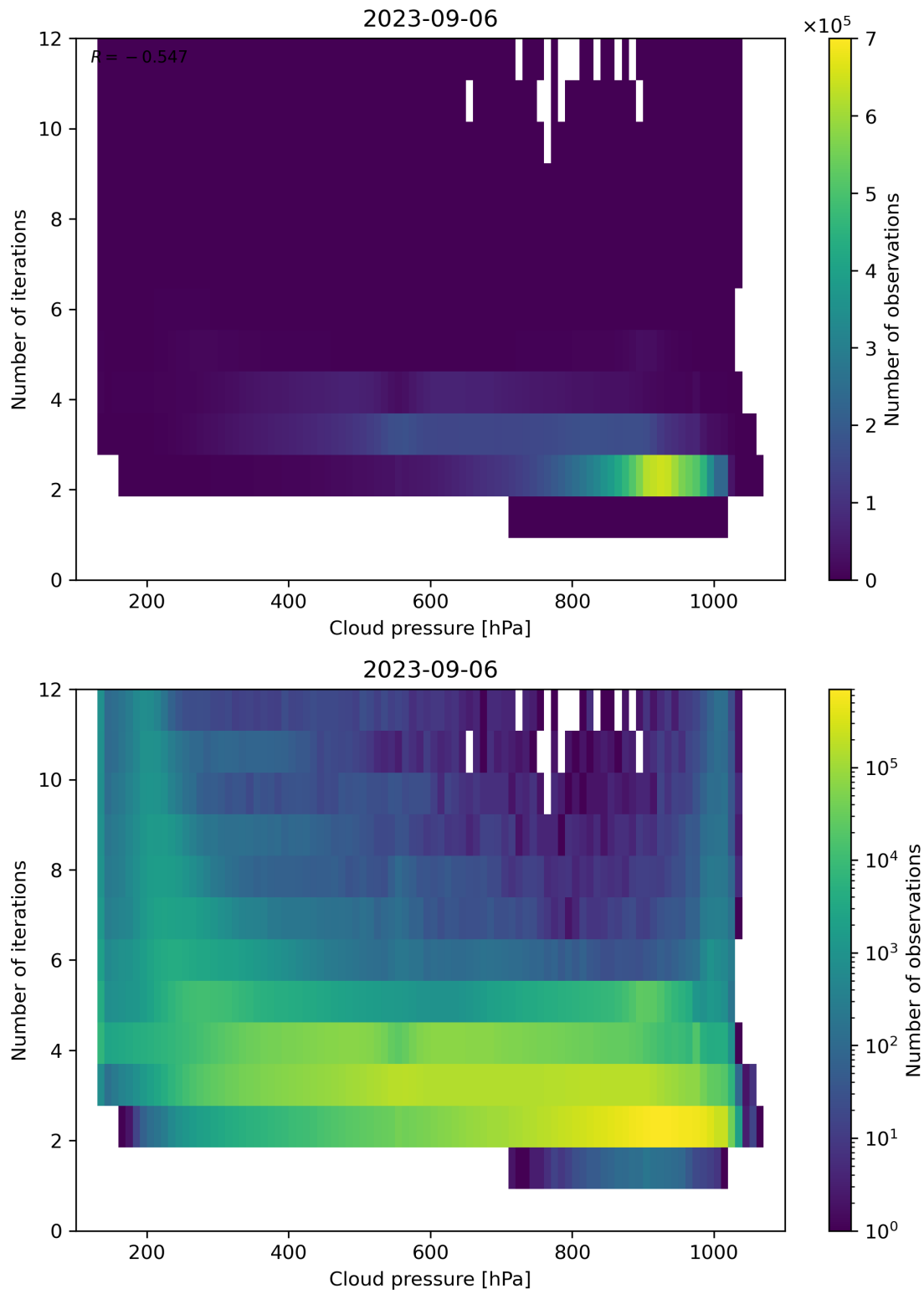
Figure 89: Scatter density plot of “Cloud pressure” against “Number of iterations” for 2023-09-05 to 2023-09-07.
