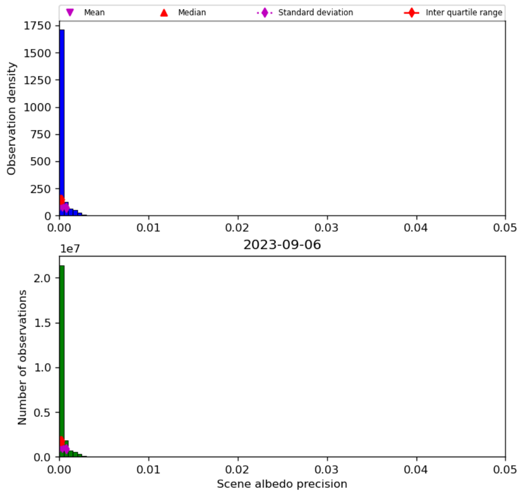
Figure 35: Histogram of “Scene albedo precision” for 2023-09-05 to 2023-09-07
