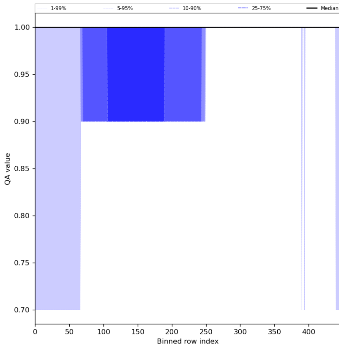
Figure 46: Along track statistics of “QA value” for 2023-09-05 to 2023-09-07
