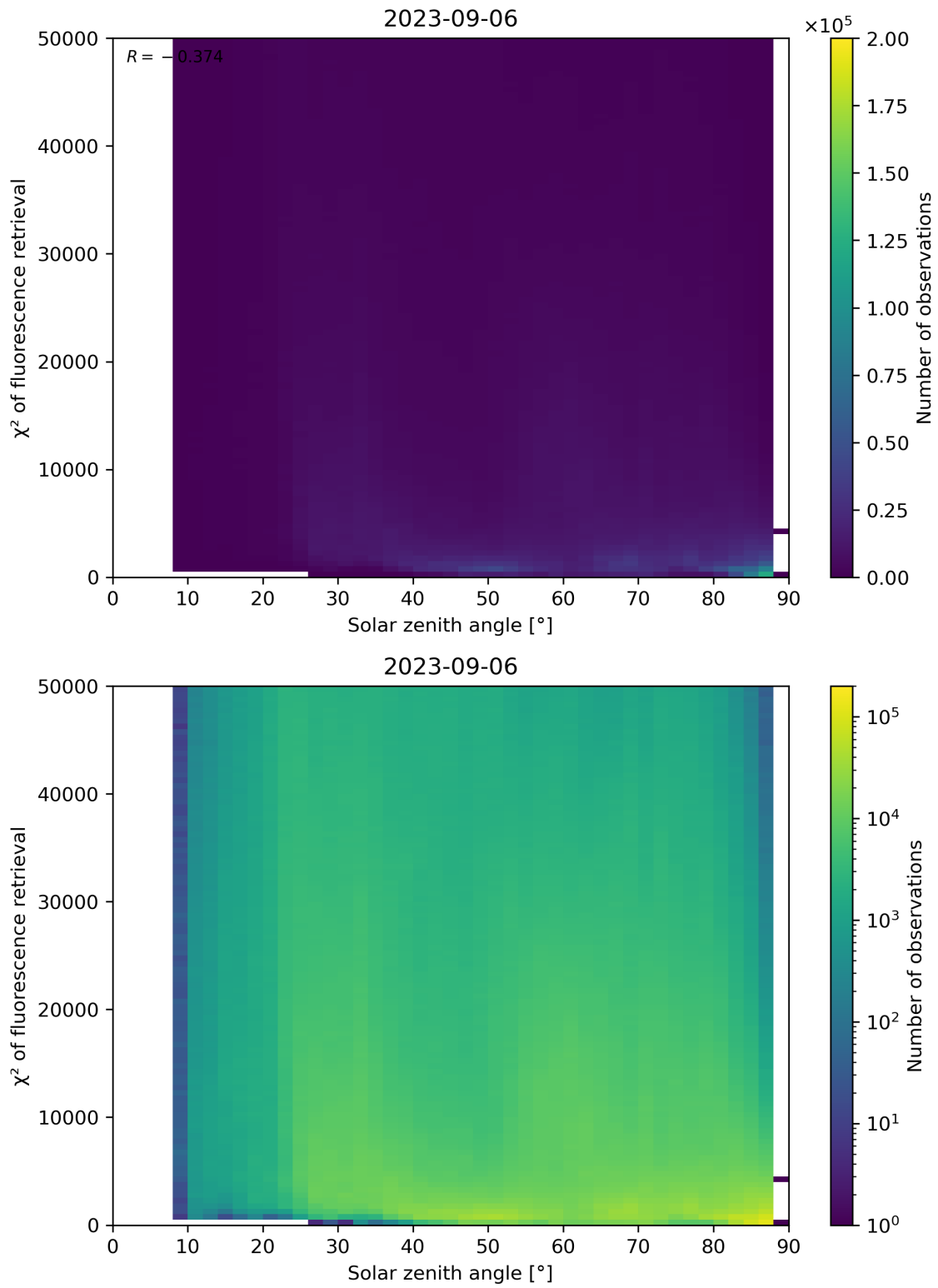
Figure 120: Scatter density plot of “Solar zenith angle” against “ \chi^2 of fluorescence retrieval” for 2023-09-05 to 2023-09-07.
