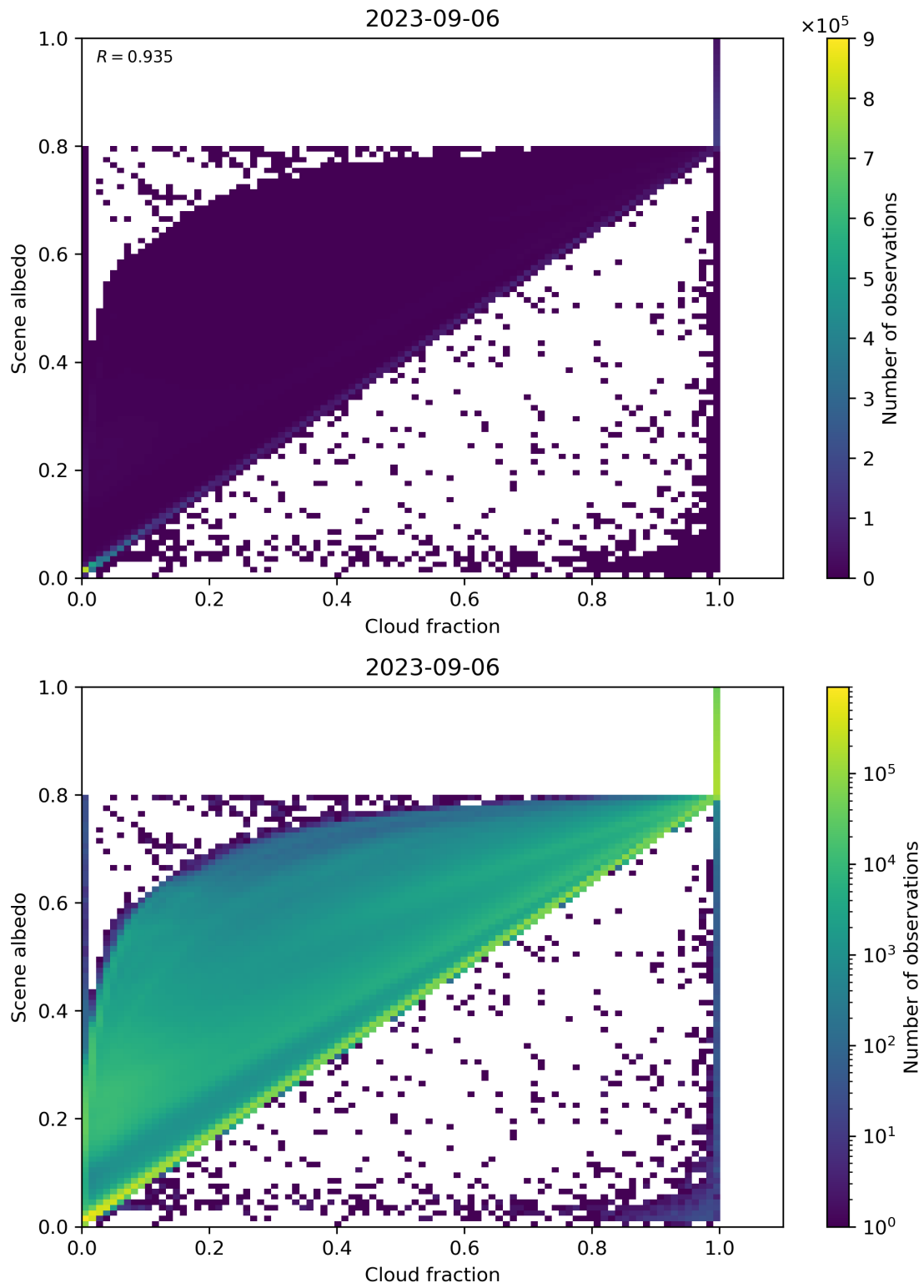
Figure 82: Scatter density plot of “Cloud fraction” against “Scene albedo” for 2023-09-05 to 2023-09-07.
