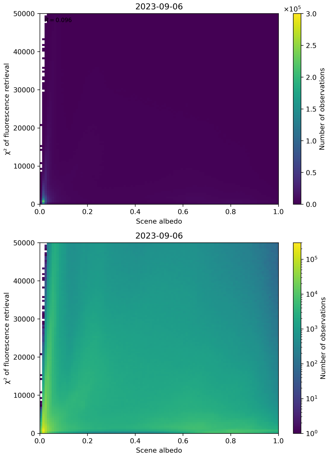
Figure 113: Scatter density plot of “Scene albedo” against “ \chi^2 of fluorescence retrieval” for 2023-09-05 to 2023-09-07.
