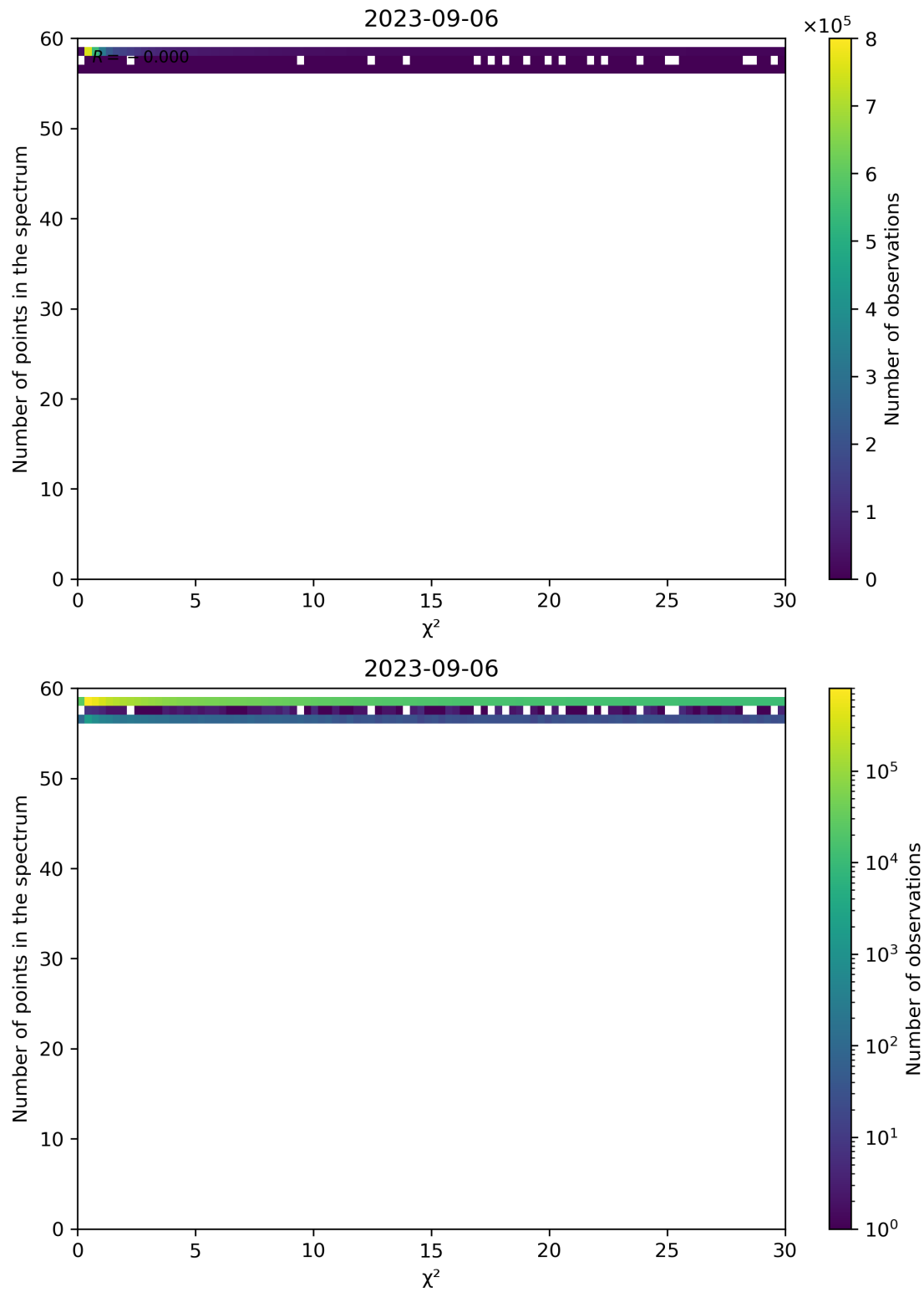
Figure 74: Scatter density plot of " \chi^2 " against "Number of points in the spectrum" for 2023-09-05 to 2023-09-07.
