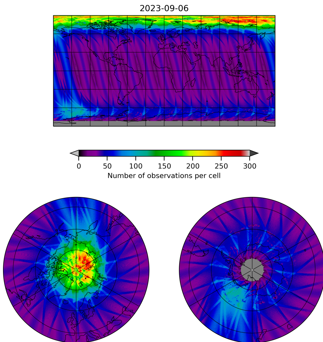
Figure 11: Map of the number of observations for 2023-09-05 to 2023-09-07
