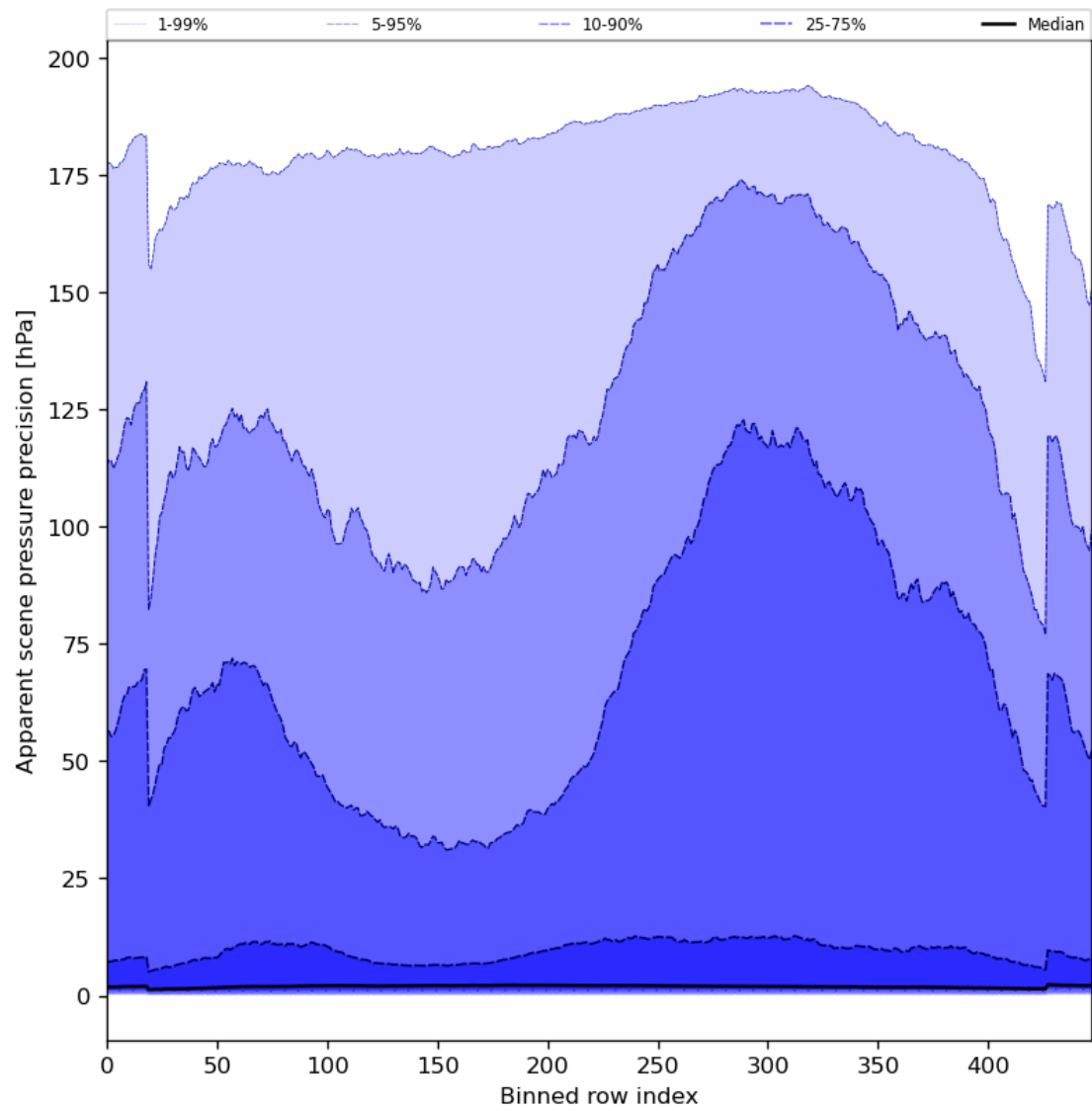
Figure 54: Along track statistics of “Apparent scene pressure precision” for 2023-09-05 to 2023-09-07
