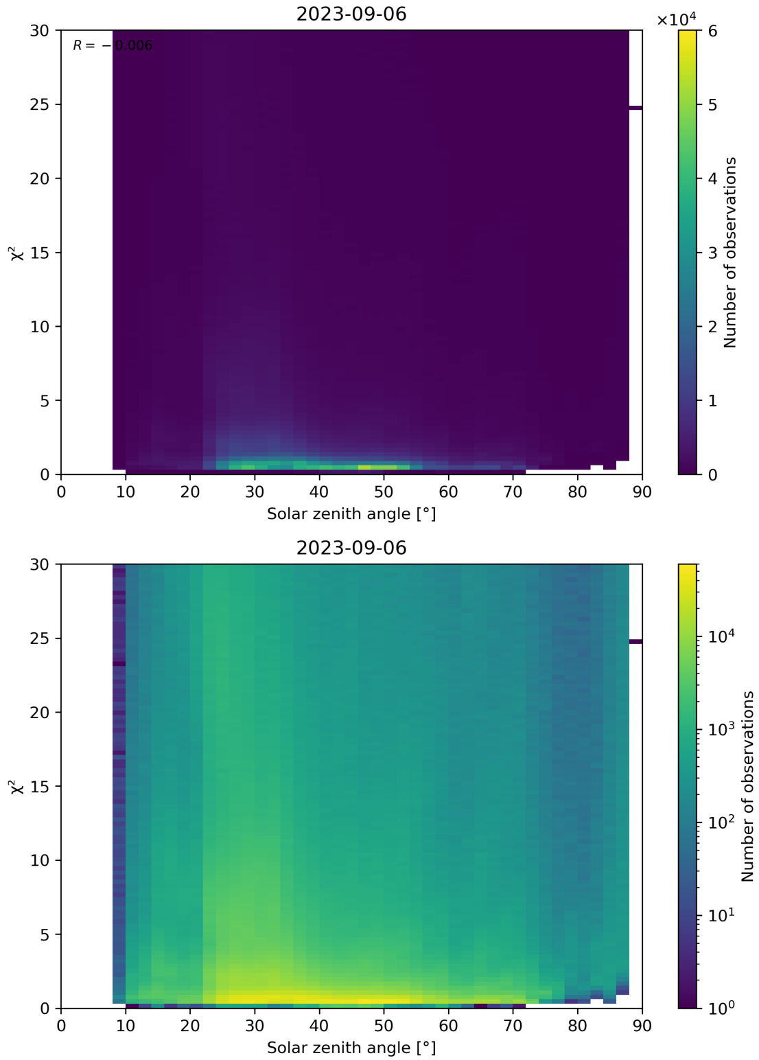
Figure 119: Scatter density plot of “Solar zenith angle” against “ \chi^2 ” for 2023-09-05 to 2023-09-07.
