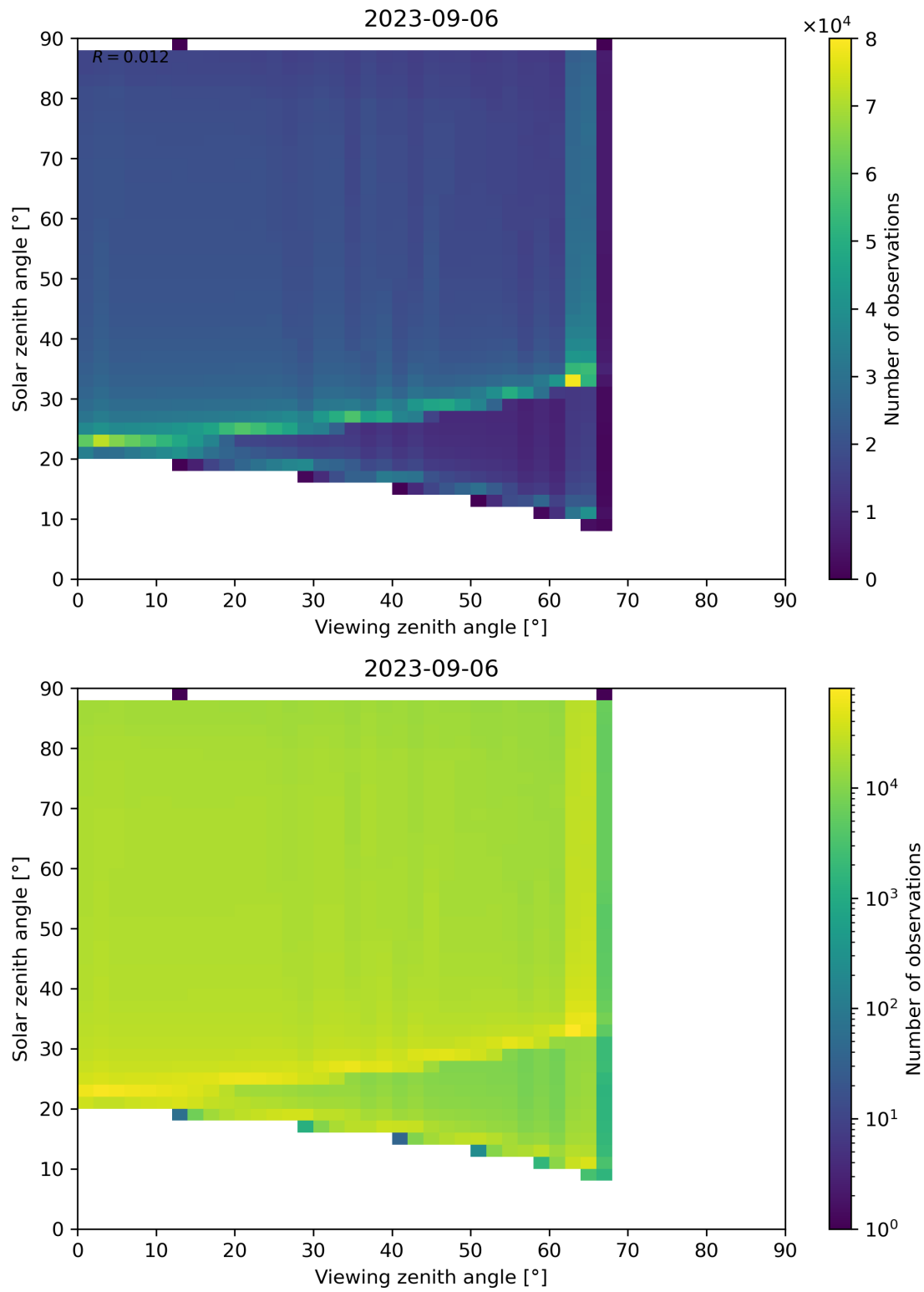
Figure 139: Scatter density plot of “Viewing zenith angle” against “Solar zenith angle” for 2023-09-05 to 2023-09-07.
