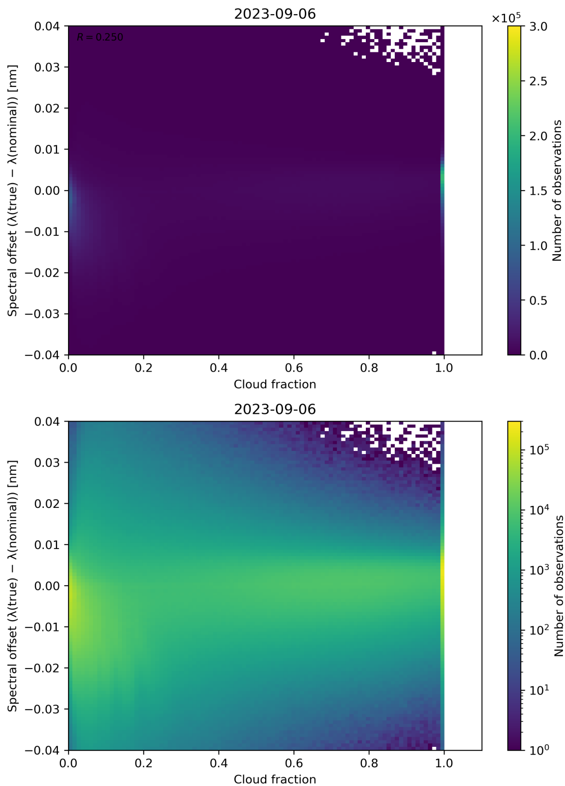
Figure 83: Scatter density plot of “Cloud fraction” against “Spectral offset ( \lambda(\text{true}) - \lambda(\text{nominal}) )” for 2023-09-05 to 2023-09-07.
