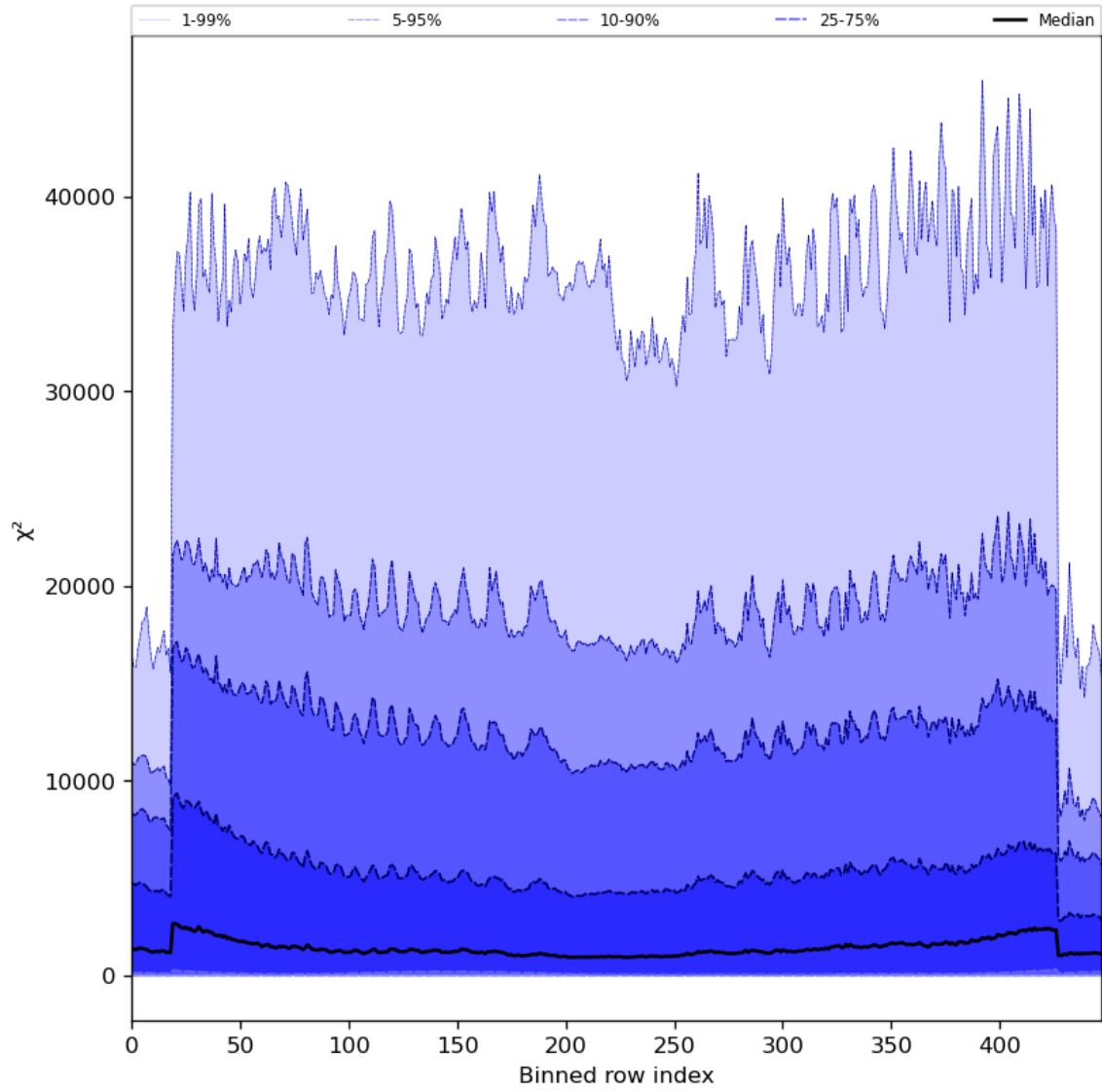
Figure 55: Along track statistics of “ \chi^2 ” for 2023-09-05 to 2023-09-07
