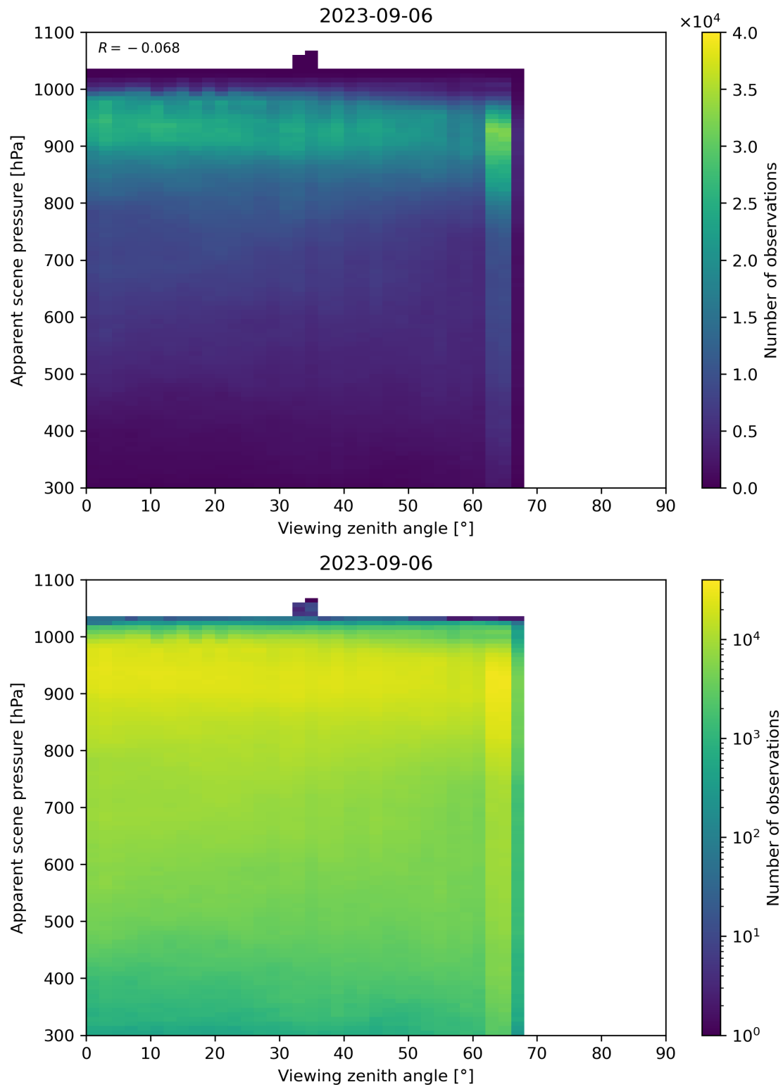
Figure 129: Scatter density plot of “Viewing zenith angle” against “Apparent scene pressure” for 2023-09-05 to 2023-09-07.
