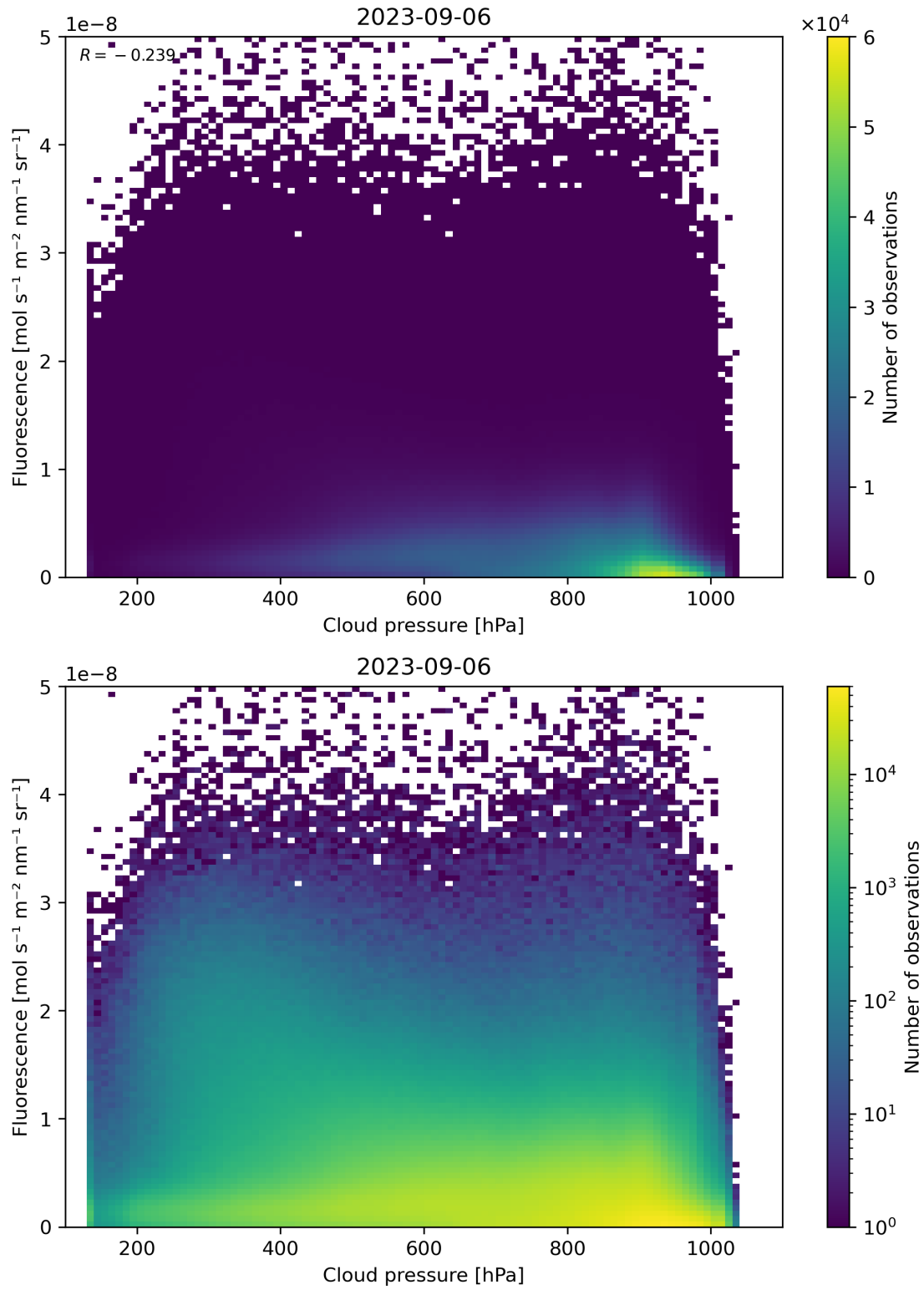
Figure 88: Scatter density plot of “Cloud pressure” against “Fluorescence” for 2023-09-05 to 2023-09-07.
