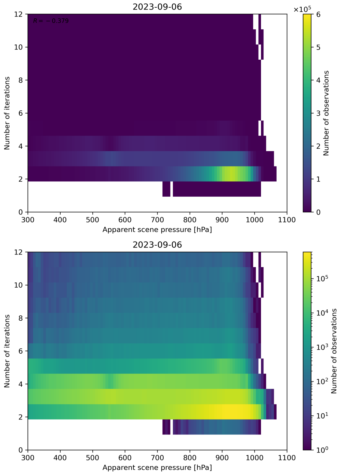
Figure 66: Scatter density plot of “Apparent scene pressure” against “Number of iterations” for 2023-09-05 to 2023-09-07.
