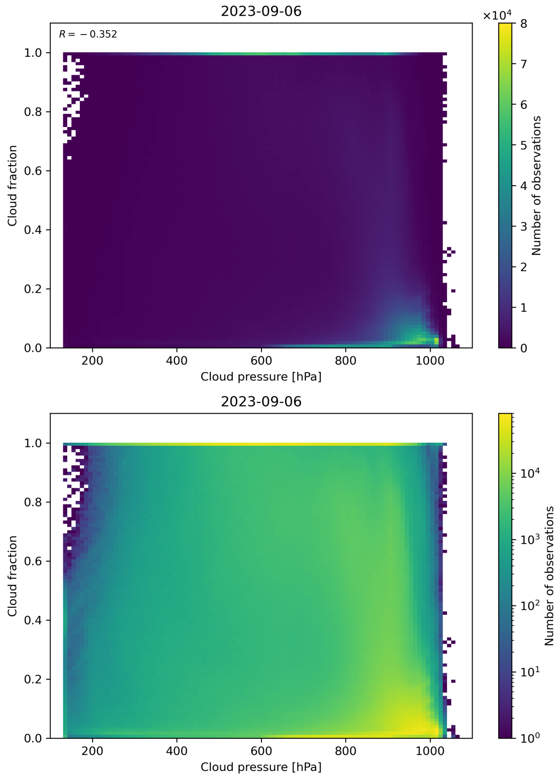
Figure 87: Scatter density plot of “Cloud pressure” against “Cloud fraction” for 2023-09-05 to 2023-09-07.
