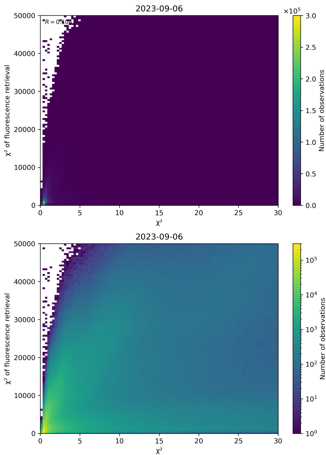
Figure 69: Scatter density plot of “ \chi^2 ” against “ \chi^2 of fluorescence retrieval” for 2023-09-05 to 2023-09-07.
