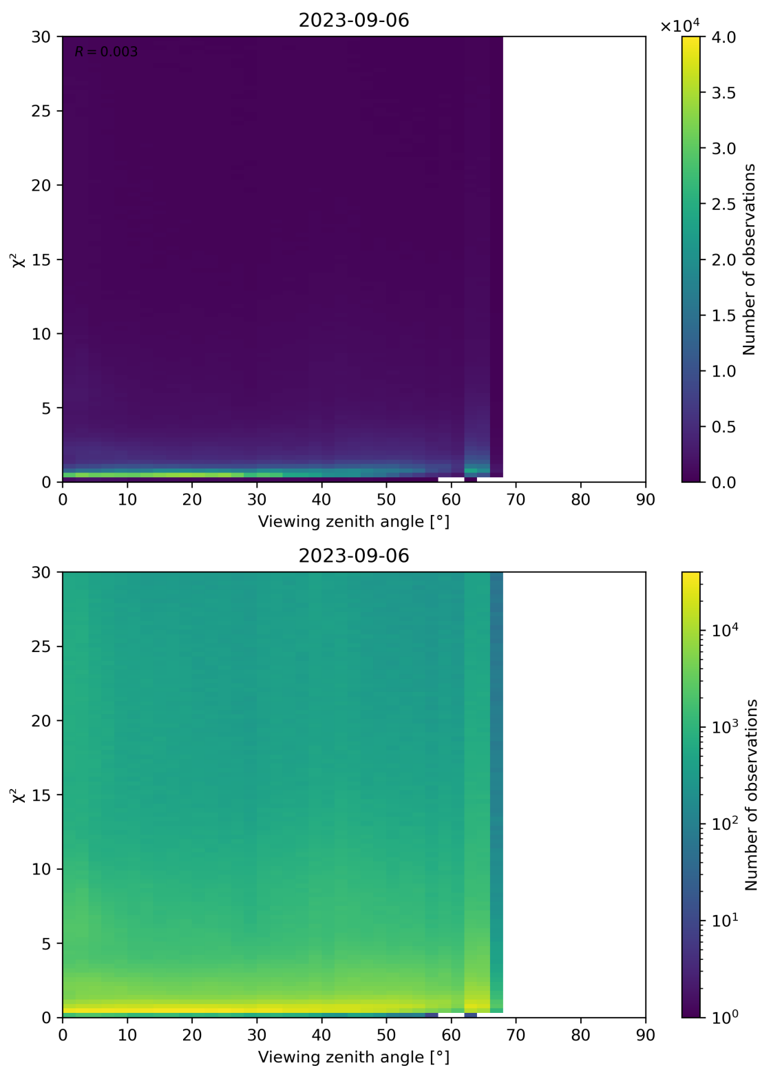
Figure 130: Scatter density plot of “Viewing zenith angle” against “ \chi^2 ” for 2023-09-05 to 2023-09-07.
