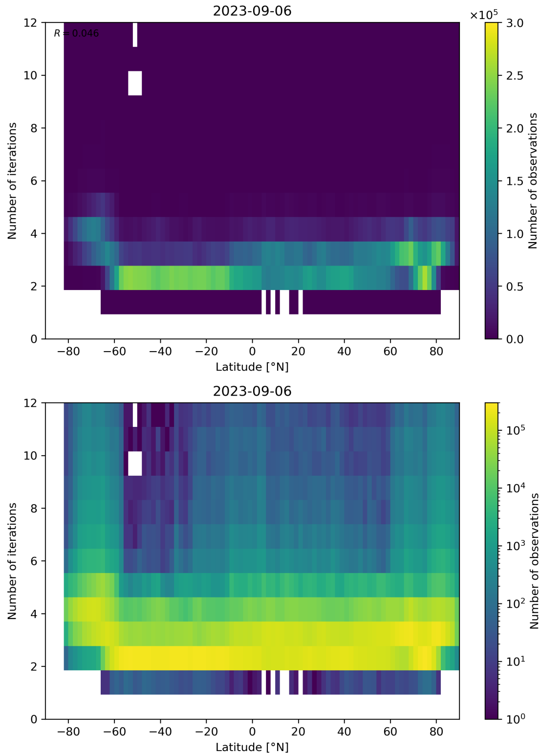
Figure 102: Scatter density plot of “Latitude” against “Number of iterations” for 2023-09-05 to 2023-09-07.
