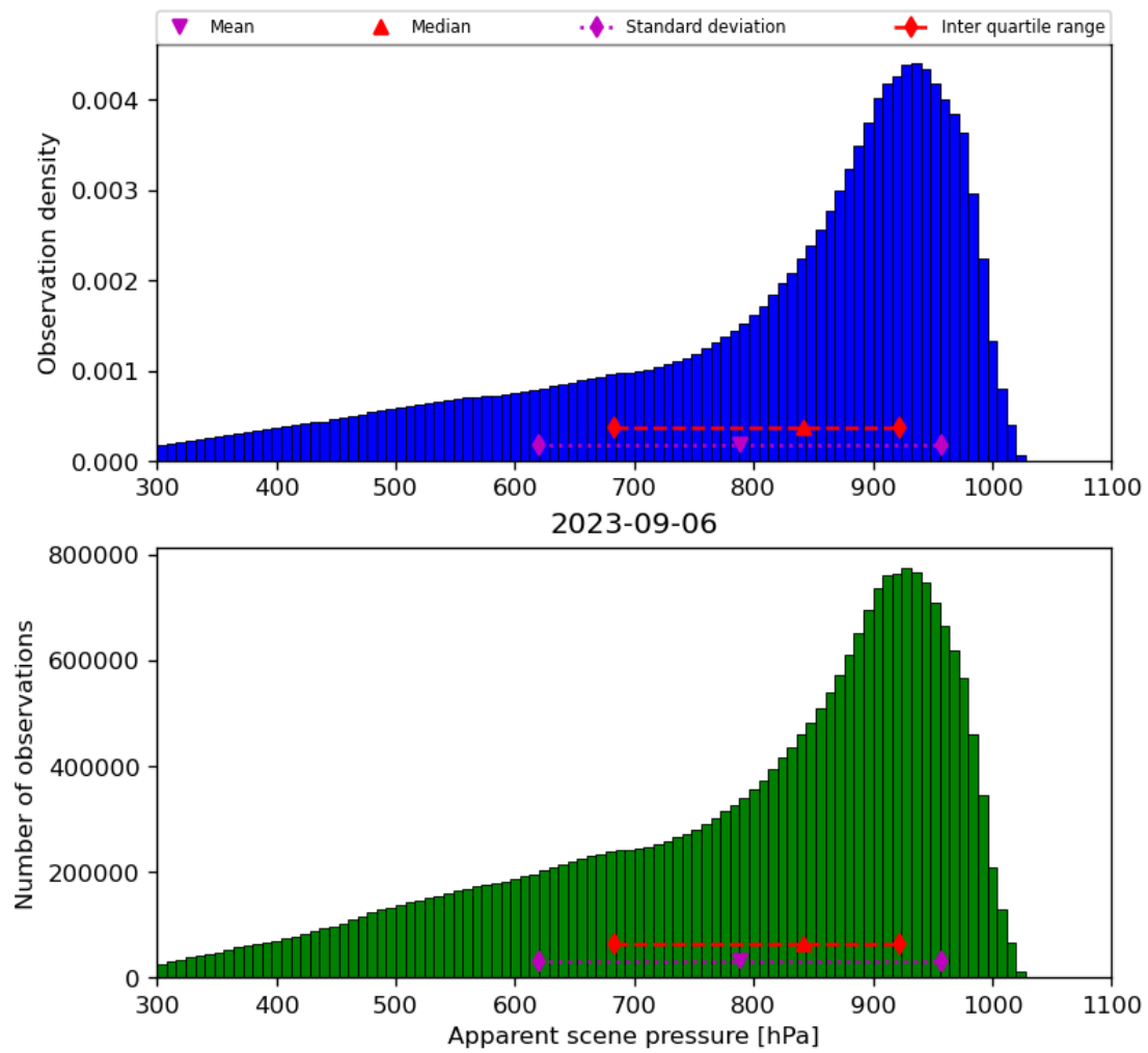
Figure 36: Histogram of “Apparent scene pressure” for 2023-09-05 to 2023-09-07
