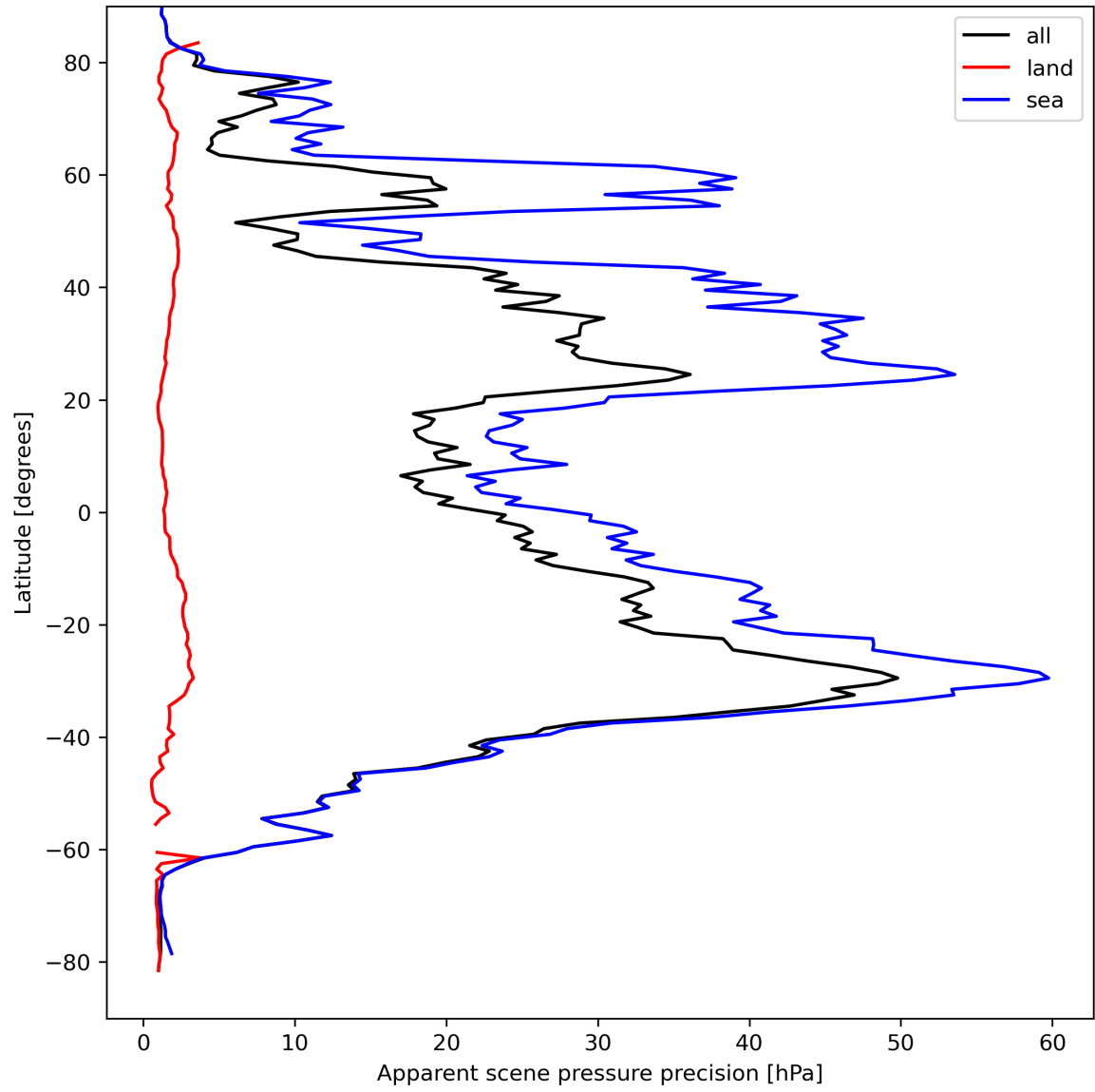
Figure 20: Zonal average of “Apparent scene pressure precision” for 2023-09-05 to 2023-09-07.
