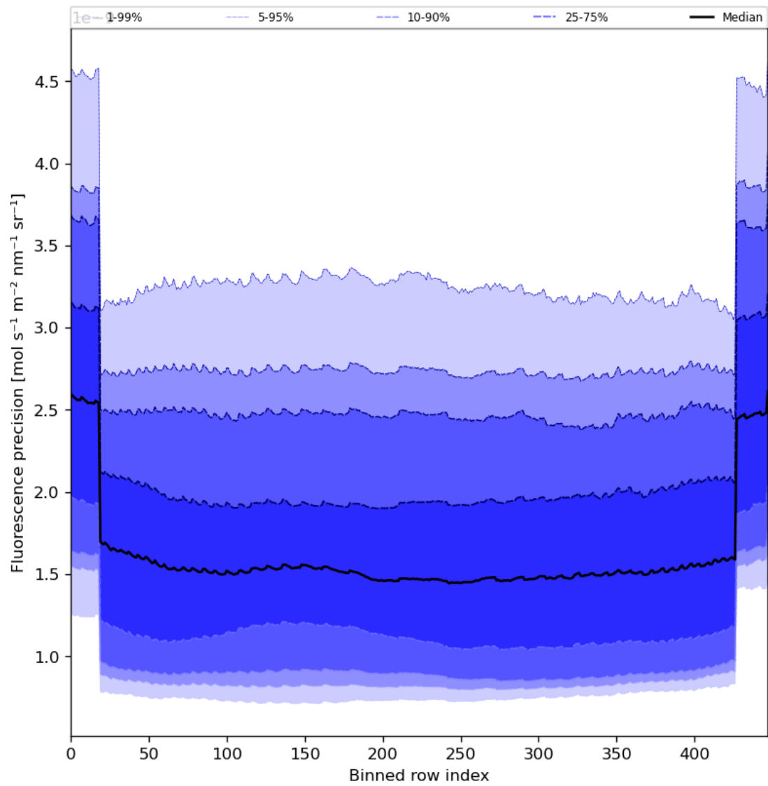
Figure 58: Along track statistics of “Fluorescence precision” for 2023-09-05 to 2023-09-07
