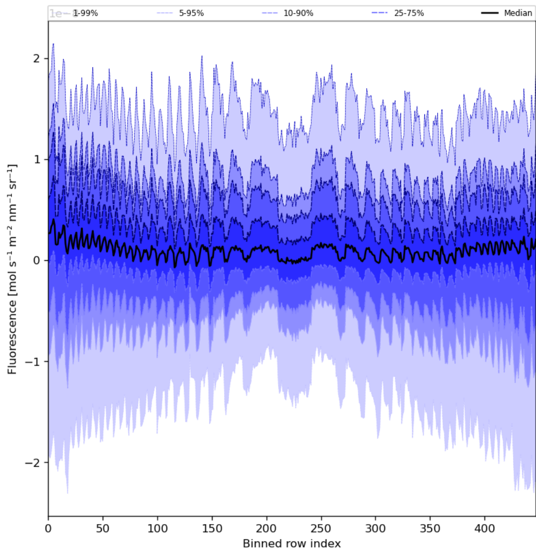
Figure 57: Along track statistics of “Fluorescence” for 2023-09-05 to 2023-09-07
