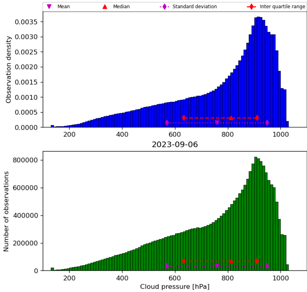
Figure 30: Histogram of “Cloud pressure” for 2023-09-05 to 2023-09-07
