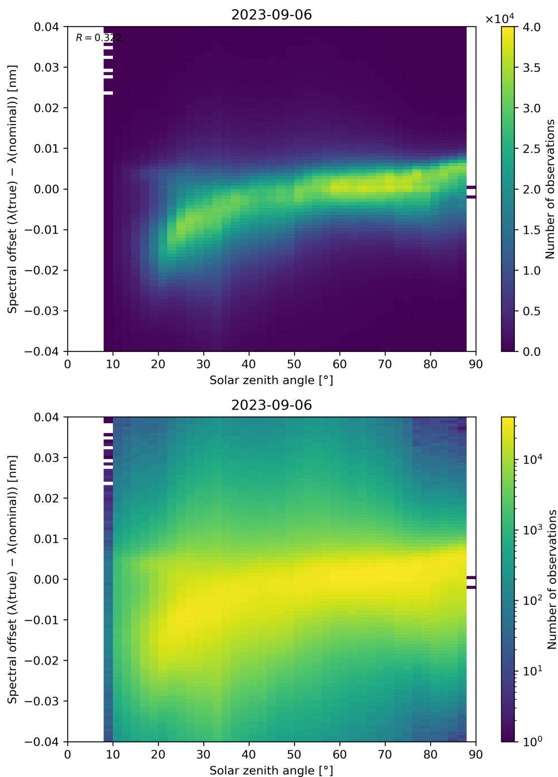
Figure 128: Scatter density plot of “Solar zenith angle” against “Spectral offset ( \lambda(\text{true}) - \lambda(\text{nominal}) )” for 2023-09-05 to 2023-09-07.
