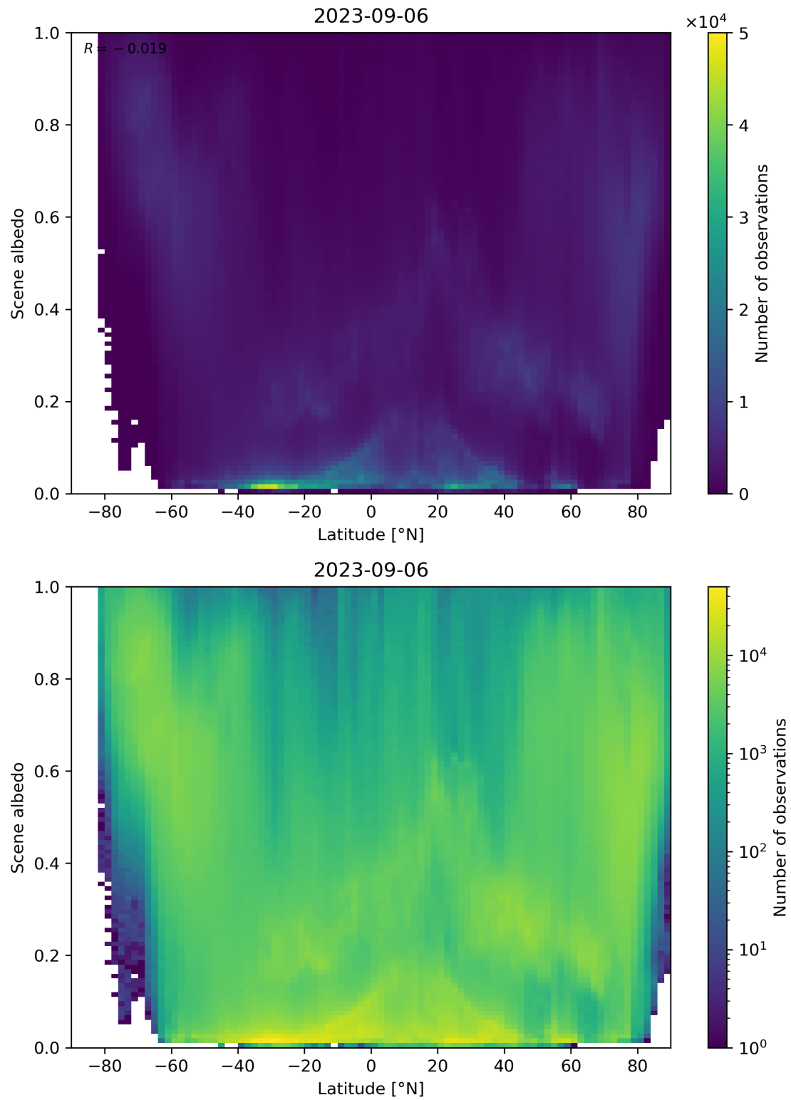
Figure 104: Scatter density plot of “Latitude” against “Scene albedo” for 2023-09-05 to 2023-09-07.
