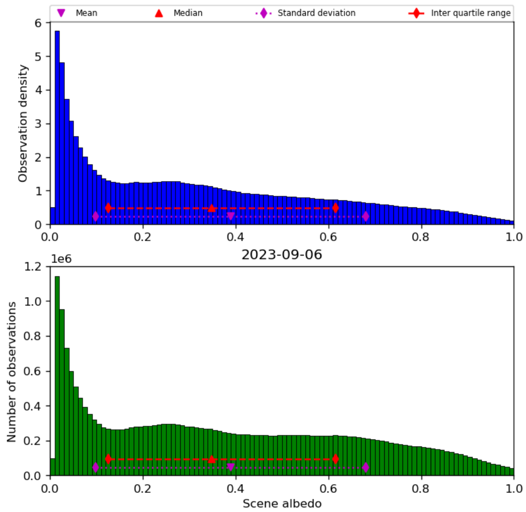
Figure 34: Histogram of “Scene albedo” for 2023-09-05 to 2023-09-07
