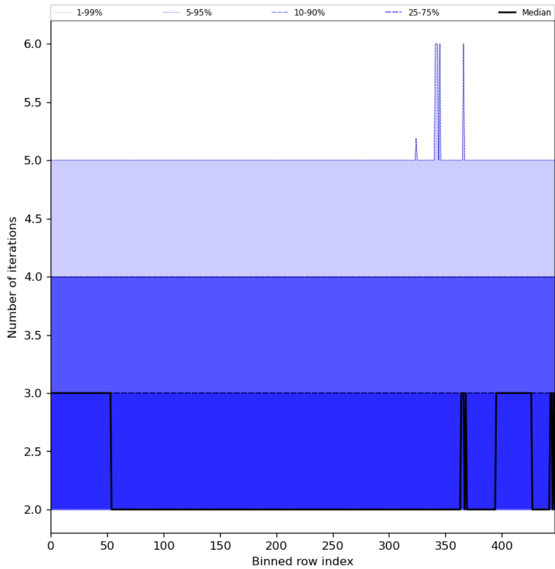
Figure 56: Along track statistics of “Number of iterations” for 2023-09-05 to 2023-09-07
