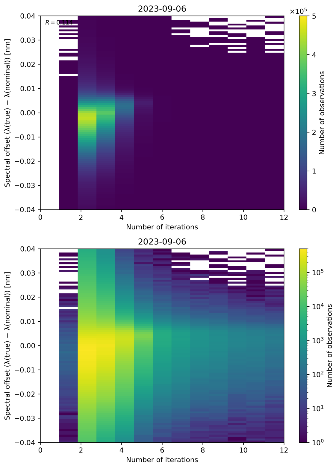
Figure 109: Scatter density plot of “Number of iterations” against “Spectral offset ( \lambda(\text{true}) - \lambda(\text{nominal}) )” for 2023-09-05 to 2023-09-07.
