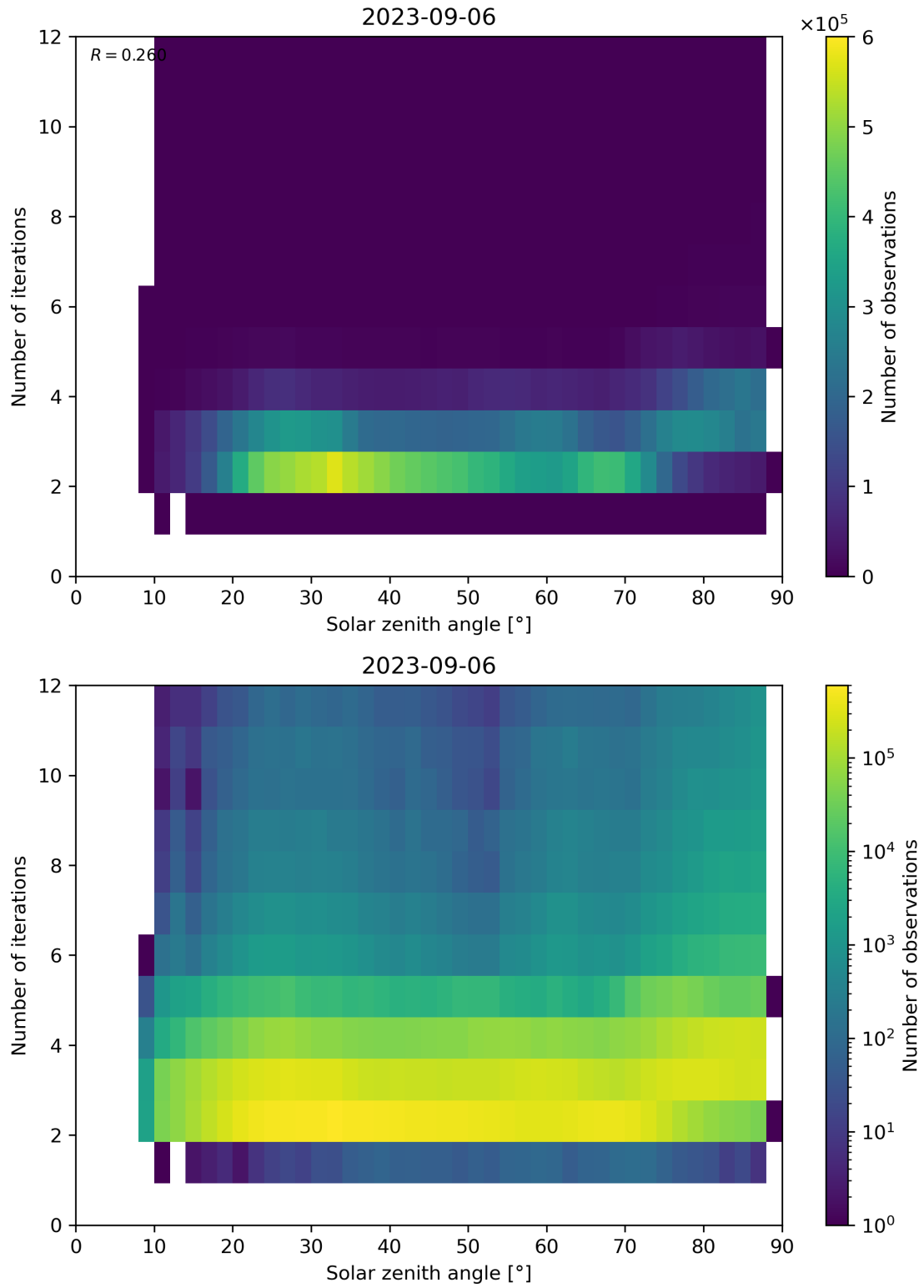
Figure 125: Scatter density plot of “Solar zenith angle” against “Number of iterations” for 2023-09-05 to 2023-09-07.
