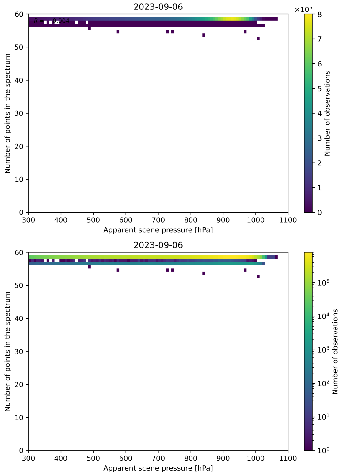
Figure 67: Scatter density plot of “Apparent scene pressure” against “Number of points in the spectrum” for 2023-09-05 to 2023-09-07.
