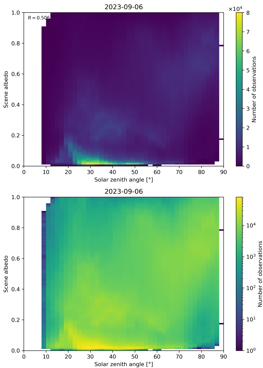
Figure 127: Scatter density plot of “Solar zenith angle” against “Scene albedo” for 2023-09-05 to 2023-09-07.
