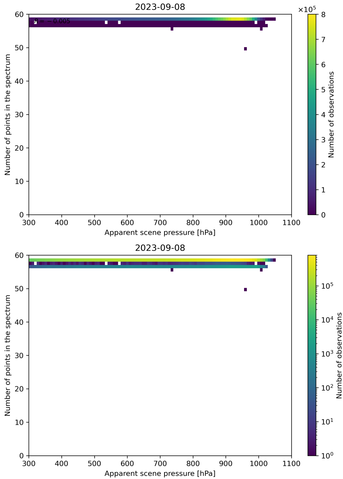
Figure 67: Scatter density plot of “Apparent scene pressure” against “Number of points in the spectrum” for 2023-09-07 to 2023-09-09.
