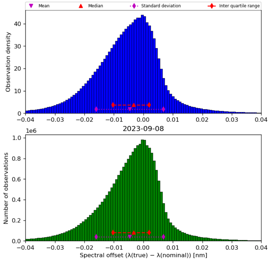
Figure 45: Histogram of “Spectral offset ( \lambda(\text{true}) - \lambda(\text{nominal}) )” for 2023-09-07 to 2023-09-09
