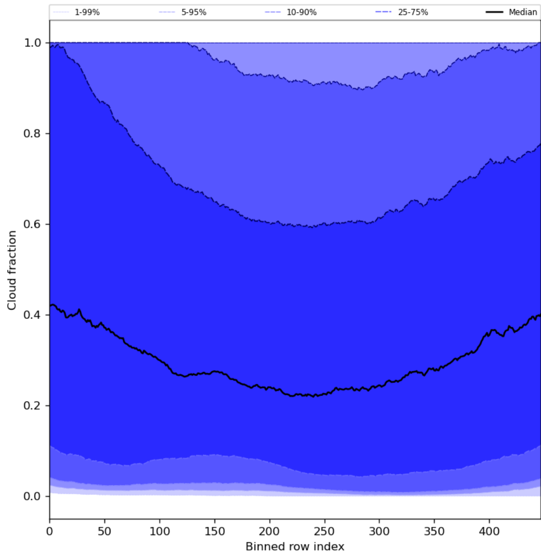
Figure 49: Along track statistics of “Cloud fraction” for 2023-09-07 to 2023-09-09
