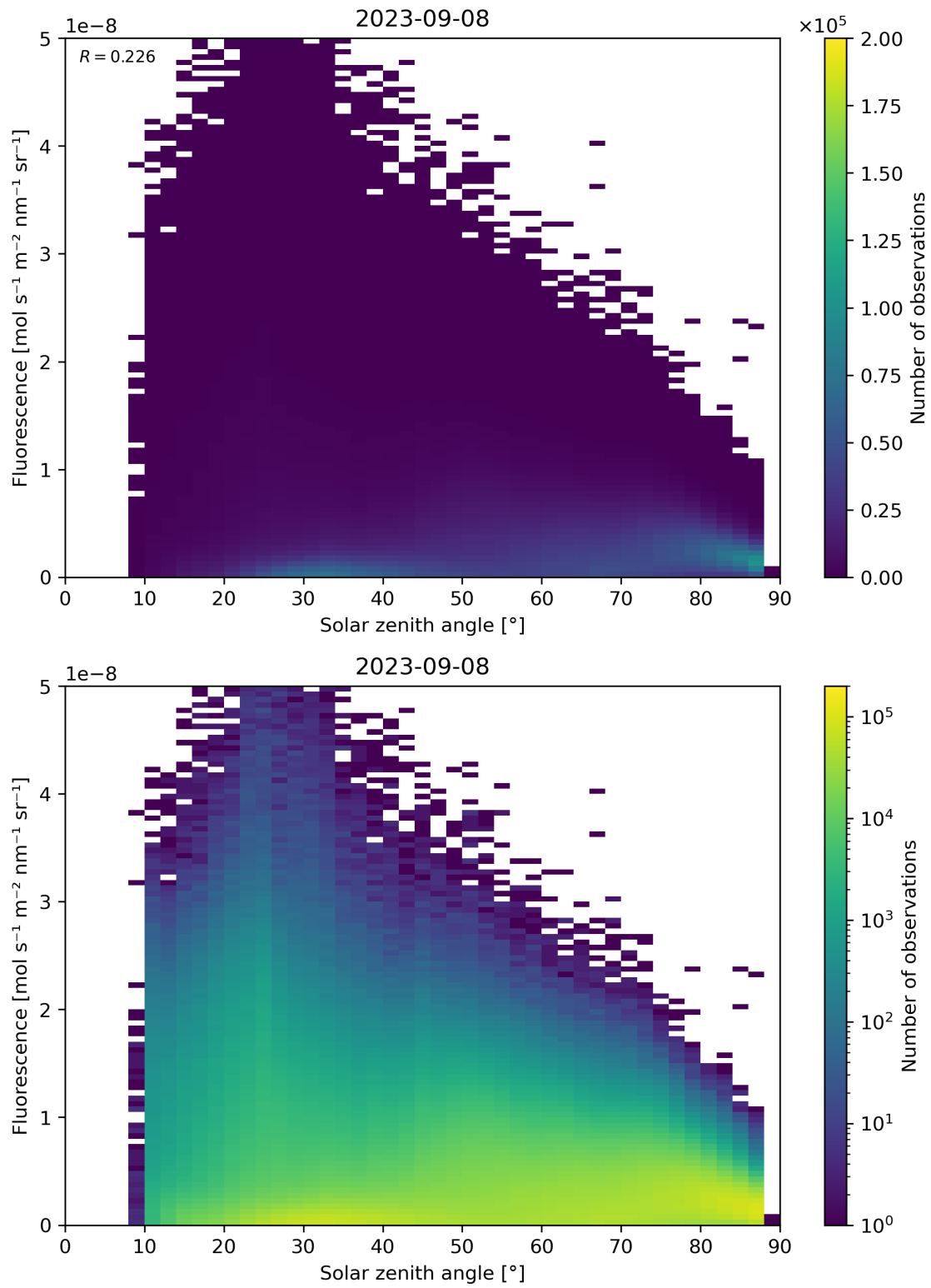
Figure 123: Scatter density plot of “Solar zenith angle” against “Fluorescence” for 2023-09-07 to 2023-09-09.
