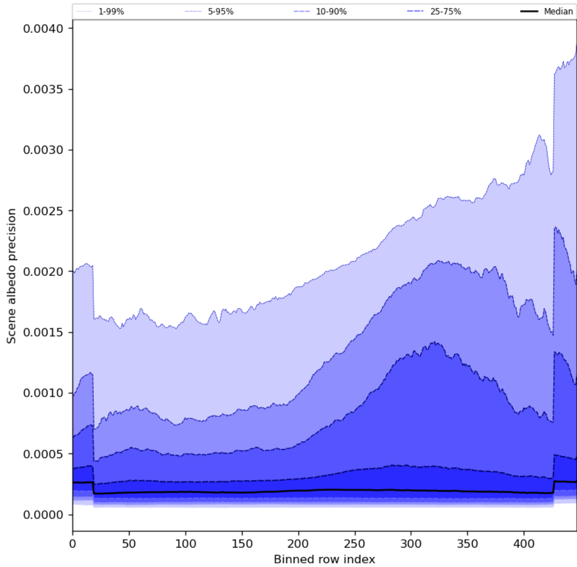
Figure 52: Along track statistics of “Scene albedo precision” for 2023-09-07 to 2023-09-09
