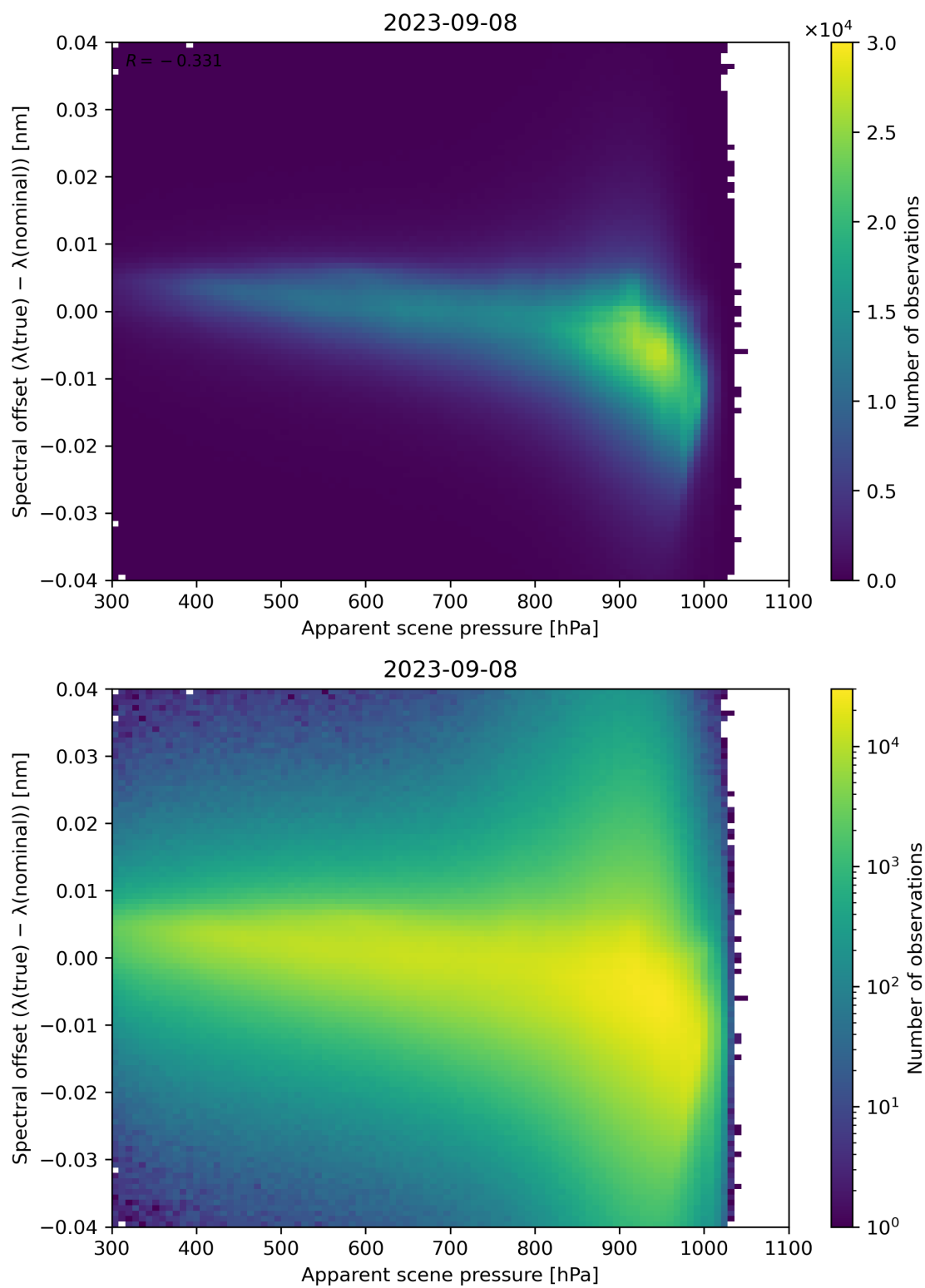
Figure 68: Scatter density plot of “Apparent scene pressure” against “Spectral offset ( \lambda(\text{true}) - \lambda(\text{nominal}) )” for 2023-09-07 to 2023-09-09.
