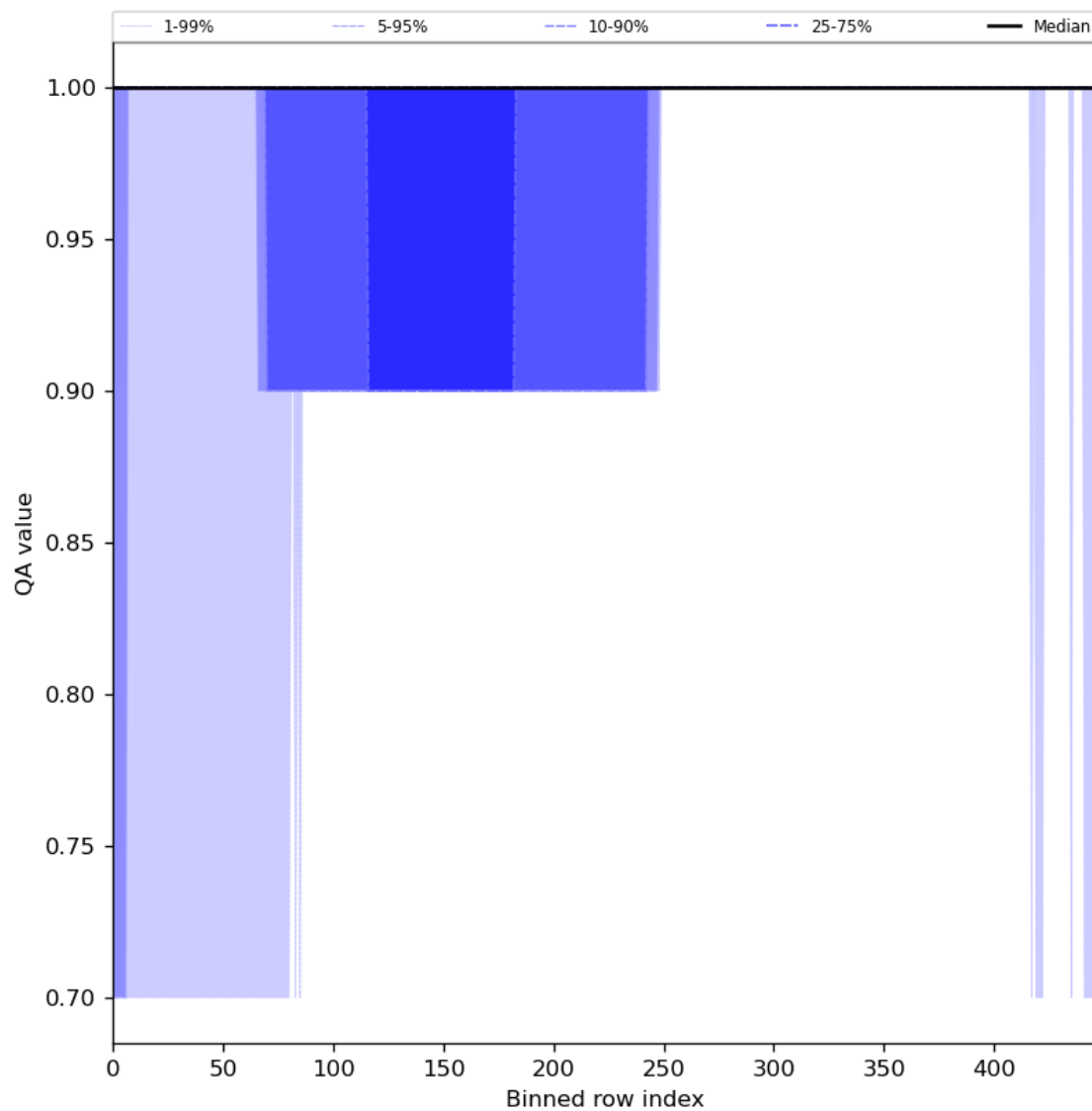
Figure 46: Along track statistics of “QA value” for 2023-09-07 to 2023-09-09
