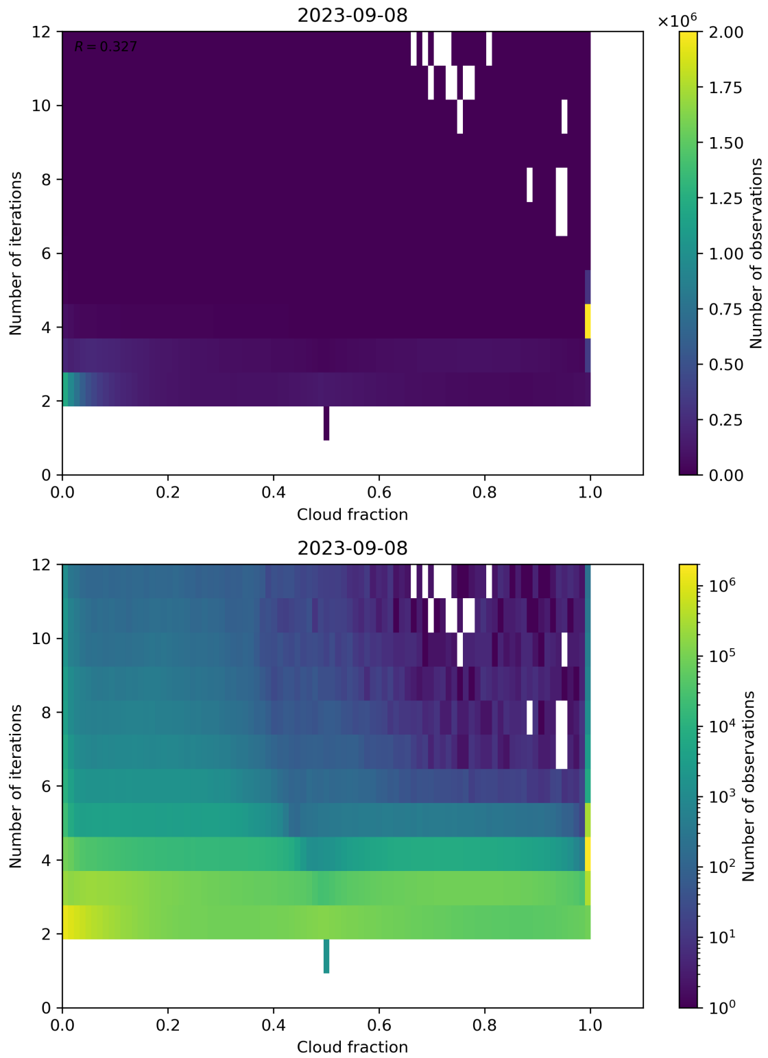
Figure 80: Scatter density plot of “Cloud fraction” against “Number of iterations” for 2023-09-07 to 2023-09-09.
