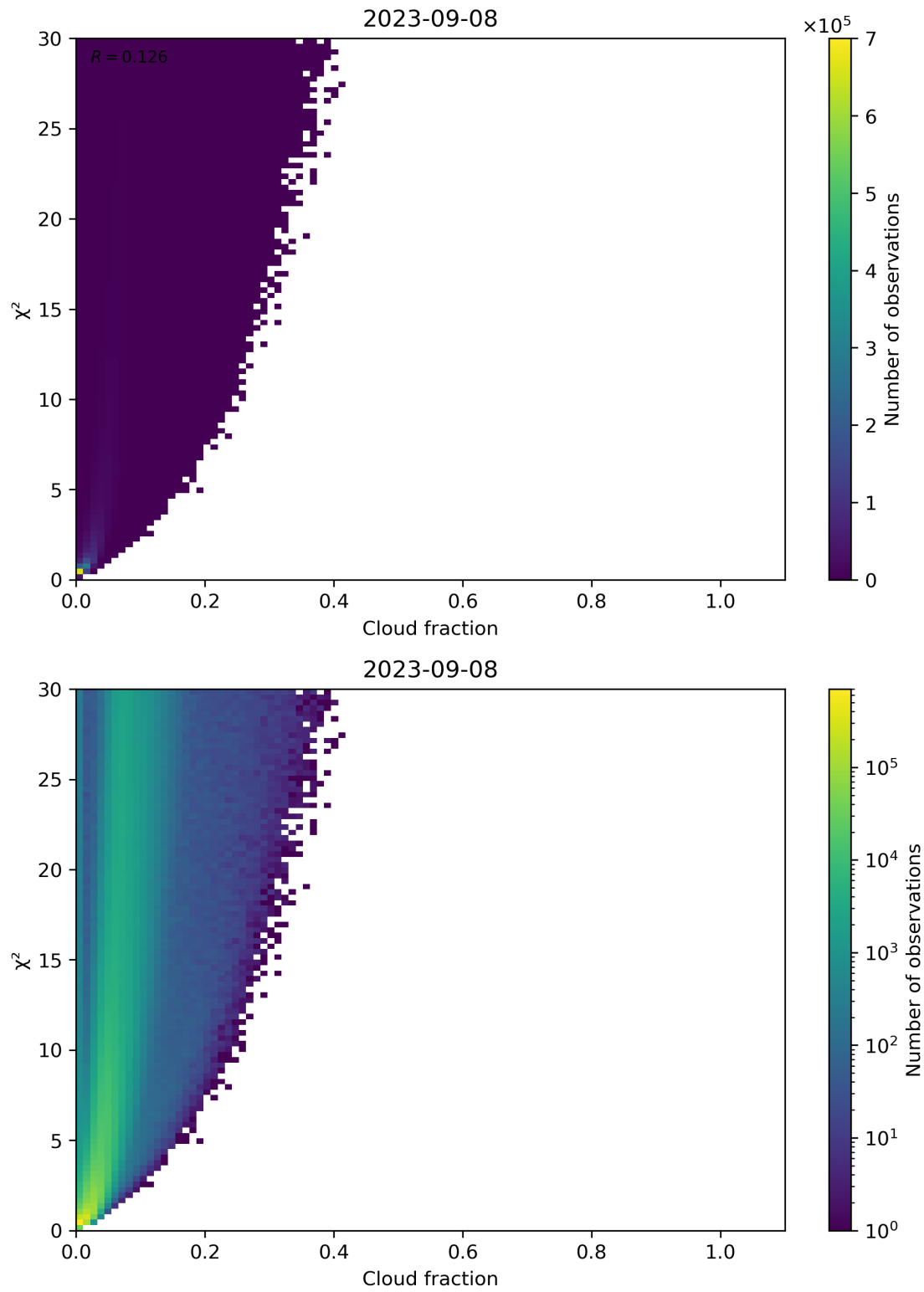
Figure 77: Scatter density plot of “Cloud fraction” against “ \chi^2 ” for 2023-09-07 to 2023-09-09.
