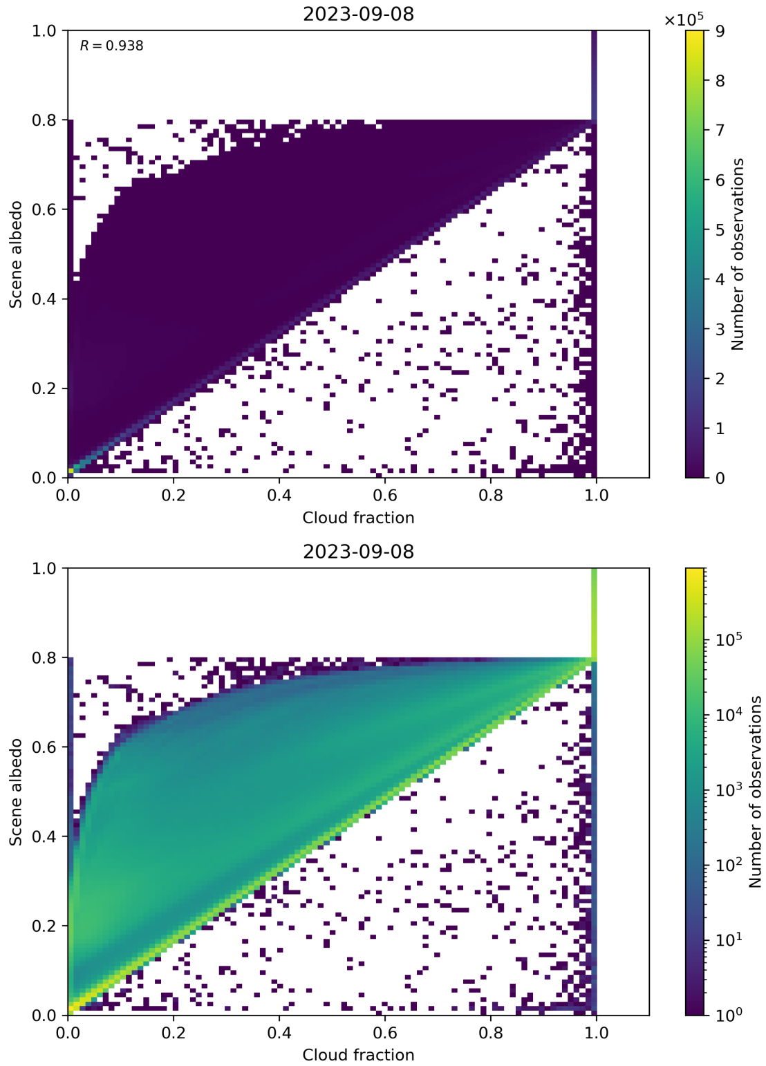
Figure 82: Scatter density plot of “Cloud fraction” against “Scene albedo” for 2023-09-07 to 2023-09-09.
