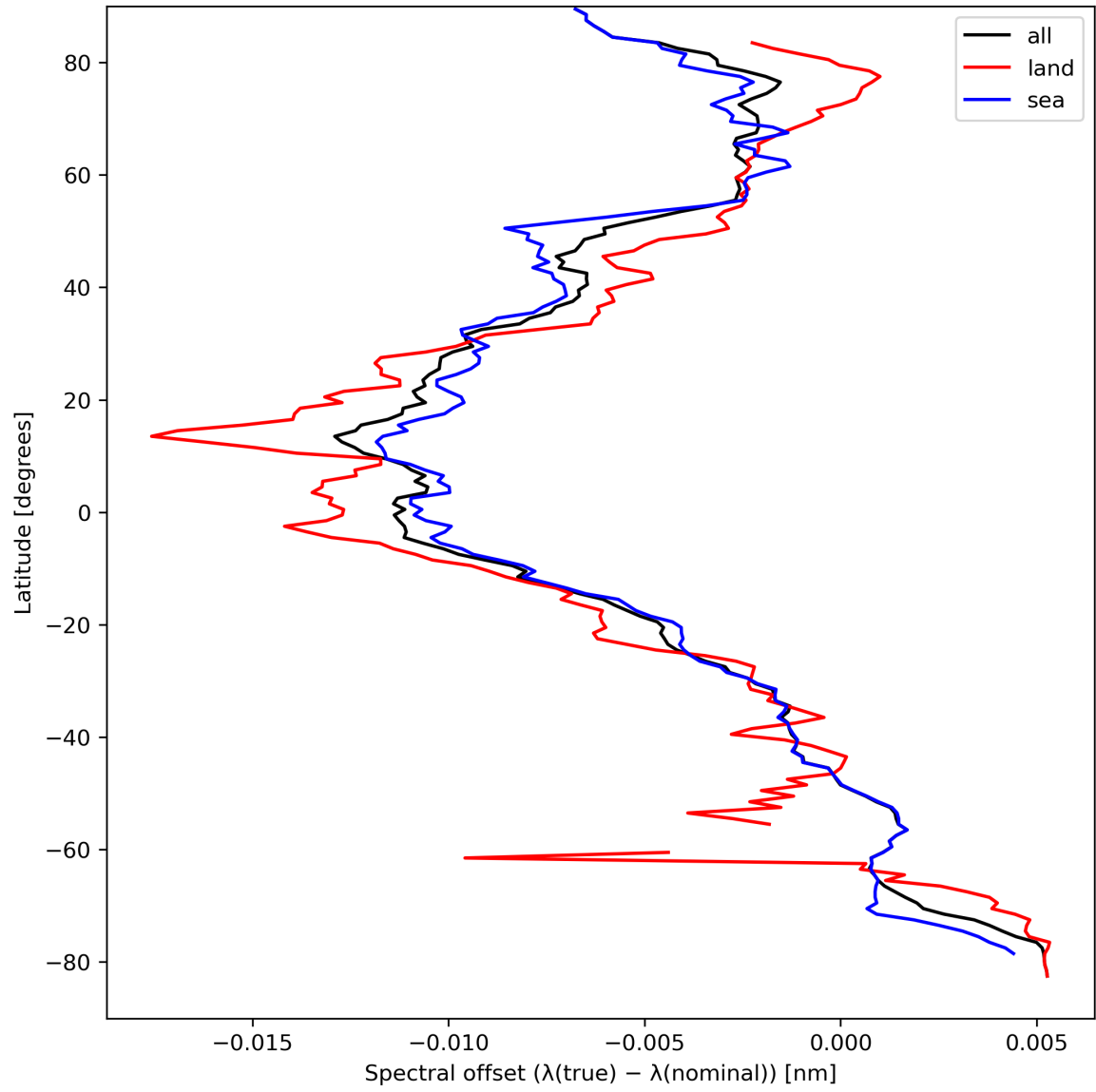
Figure 28: Zonal average of “Spectral offset ( \lambda(\text{true}) - \lambda(\text{nominal}) )” for 2023-09-07 to 2023-09-09.
