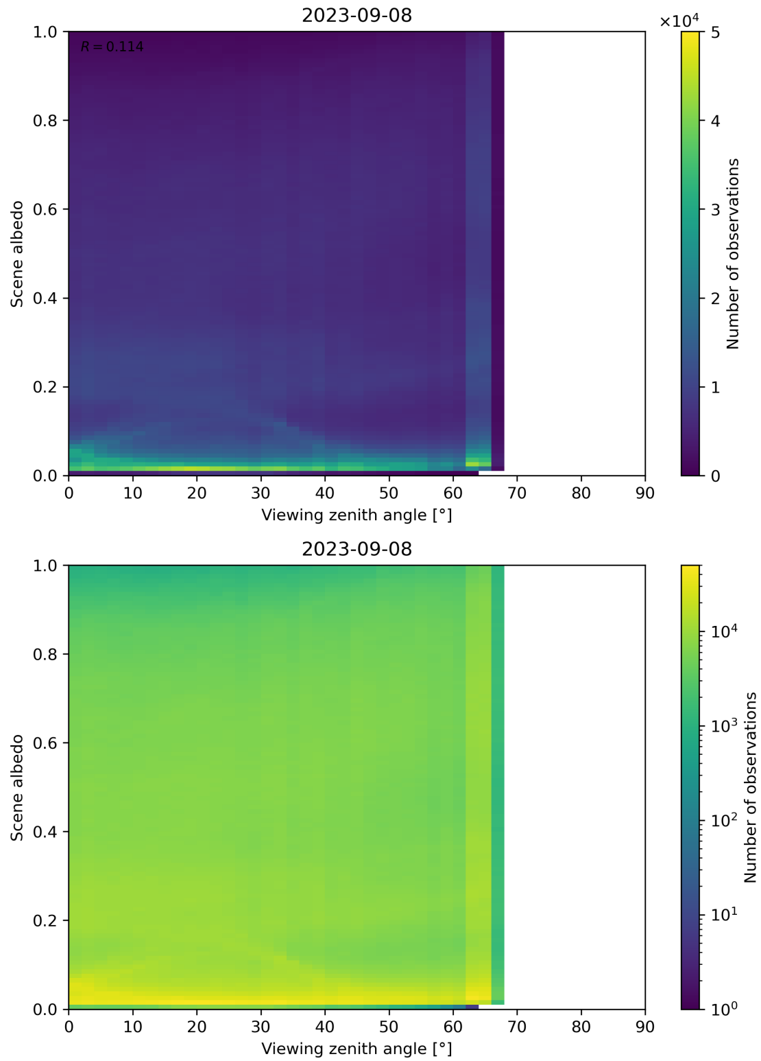
Figure 138: Scatter density plot of “Viewing zenith angle” against “Scene albedo” for 2023-09-07 to 2023-09-09.
