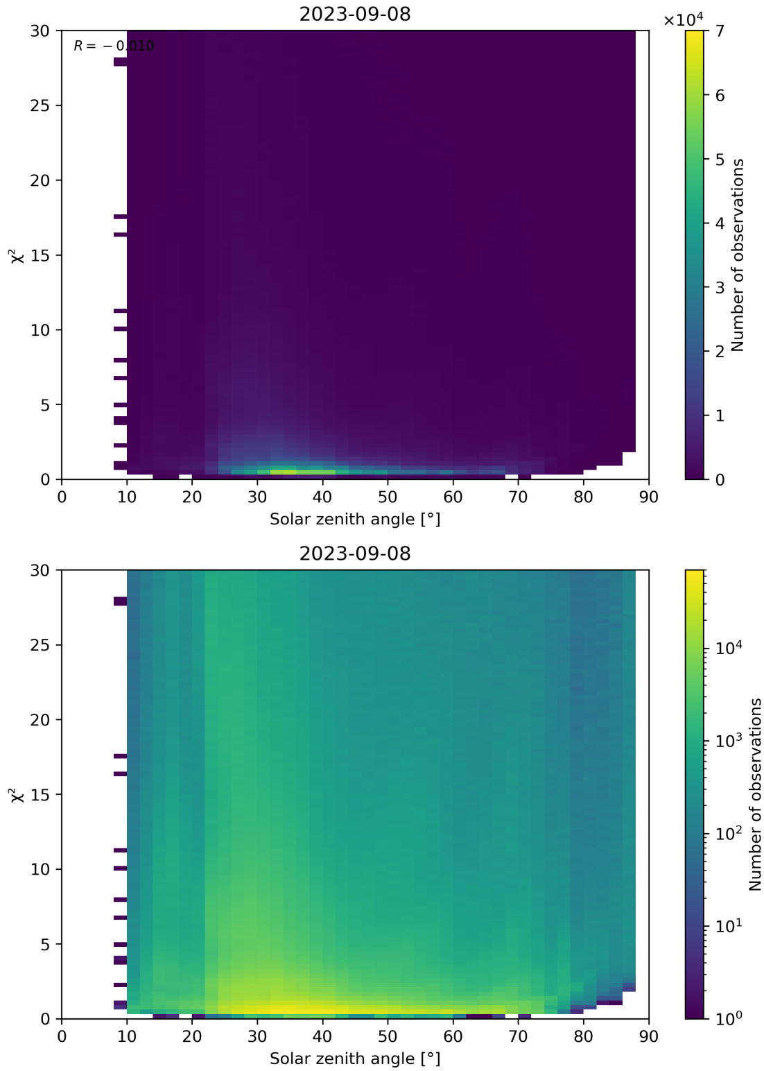
Figure 119: Scatter density plot of “Solar zenith angle” against “ \chi^2 ” for 2023-09-07 to 2023-09-09.
