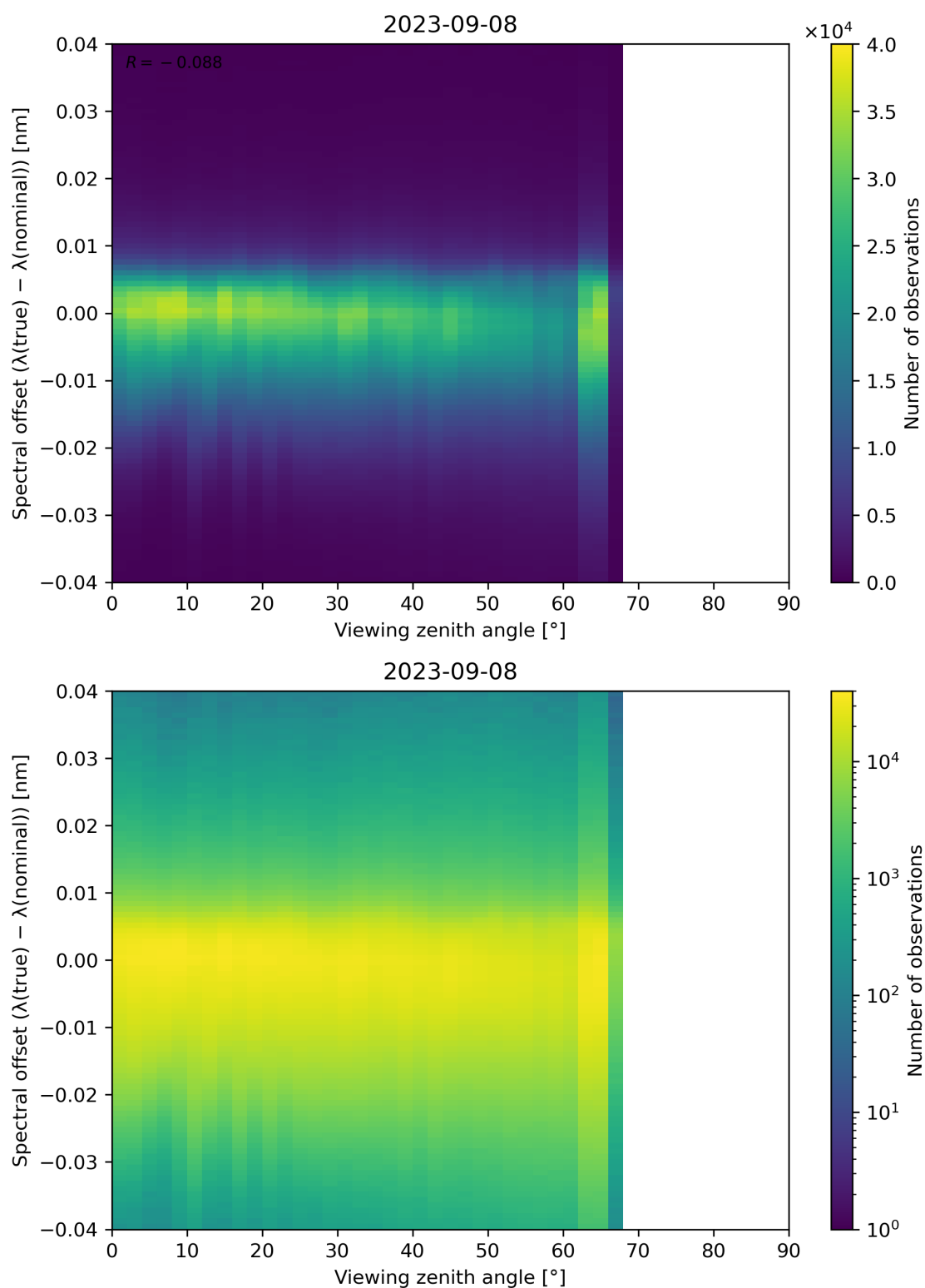
Figure 140: Scatter density plot of “Viewing zenith angle” against “Spectral offset ( \lambda(\text{true}) - \lambda(\text{nominal}) )” for 2023-09-07 to 2023-09-09.
