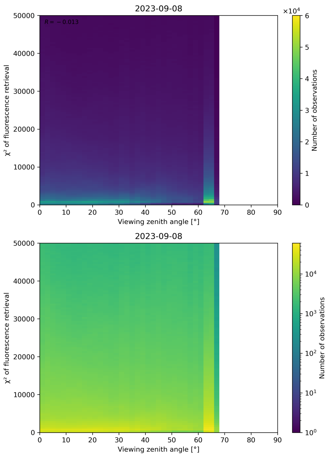
Figure 131: Scatter density plot of “Viewing zenith angle” against “ \chi^2 of fluorescence retrieval” for 2023-09-07 to 2023-09-09.
