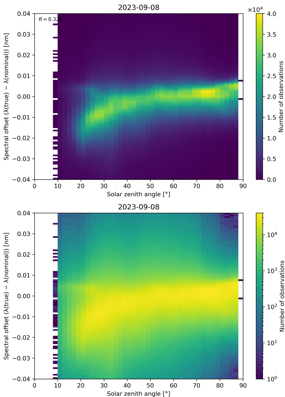
Figure 128: Scatter density plot of “Solar zenith angle” against “Spectral offset ( \lambda(\text{true}) - \lambda(\text{nominal}) )” for 2023-09-07 to 2023-09-09.
