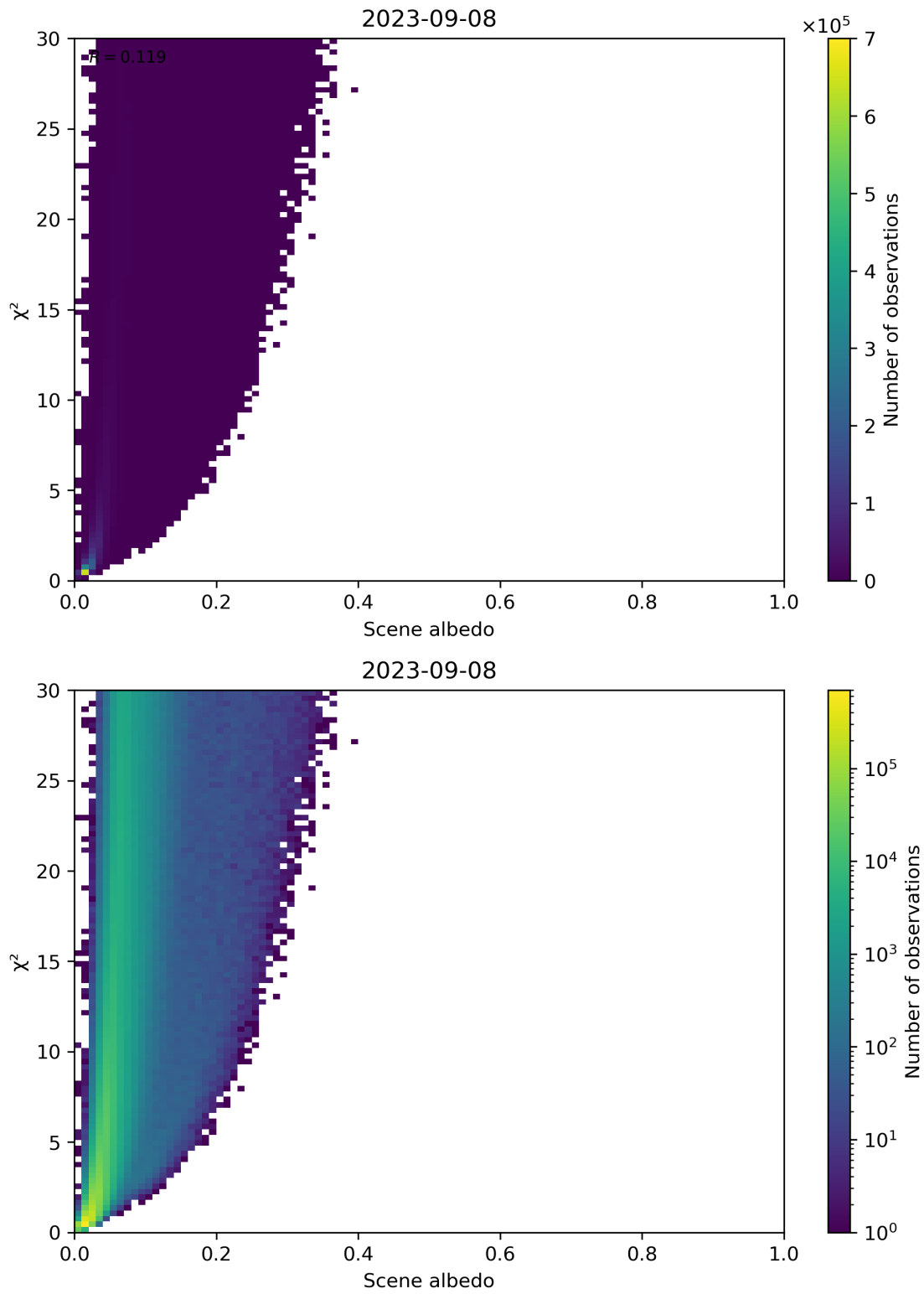
Figure 112: Scatter density plot of “Scene albedo” against “ \chi^2 ” for 2023-09-07 to 2023-09-09.
