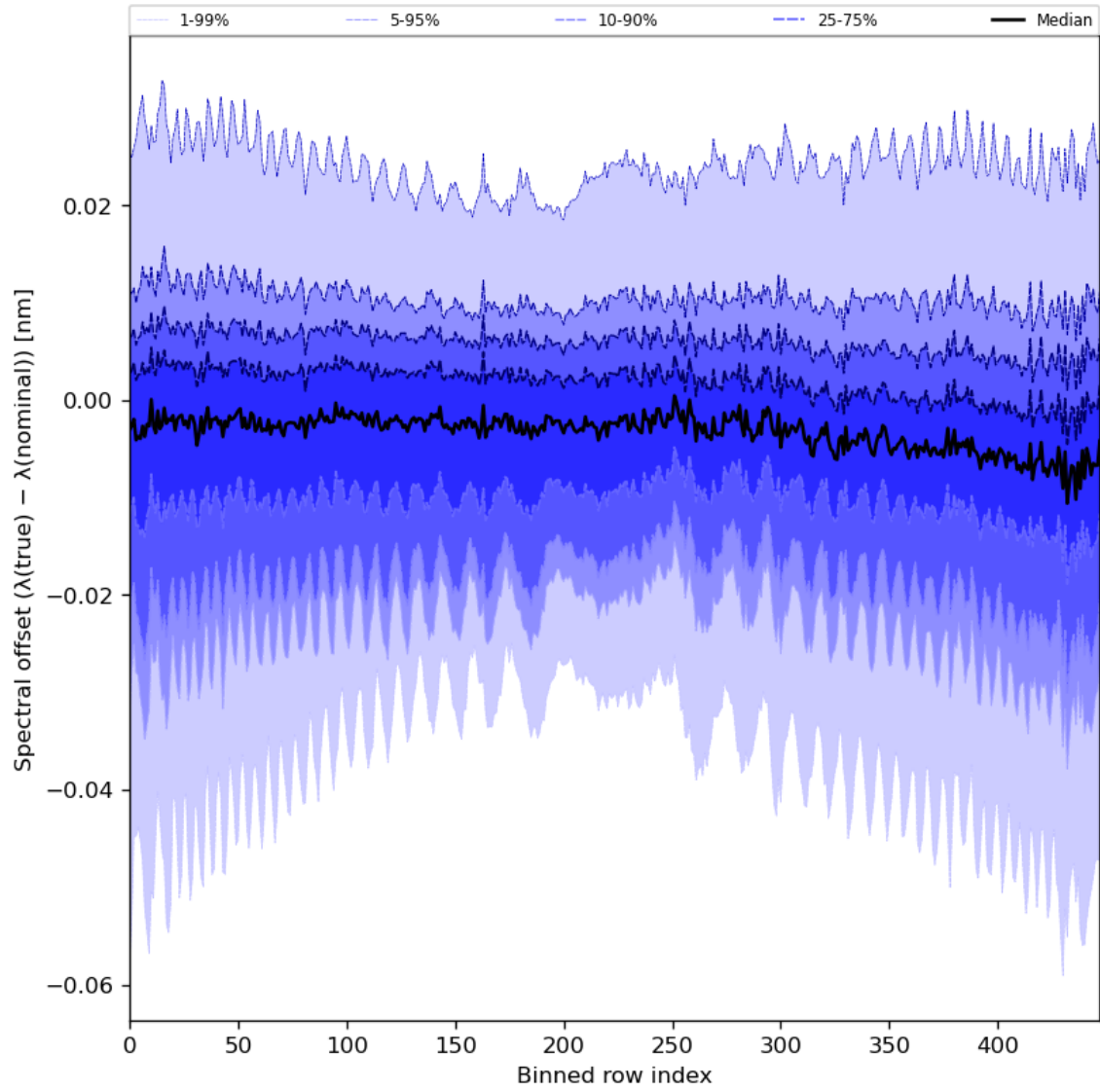
Figure 62: Along track statistics of “Spectral offset ( \lambda(\text{true}) - \lambda(\text{nominal}) )” for 2023-09-07 to 2023-09-09
