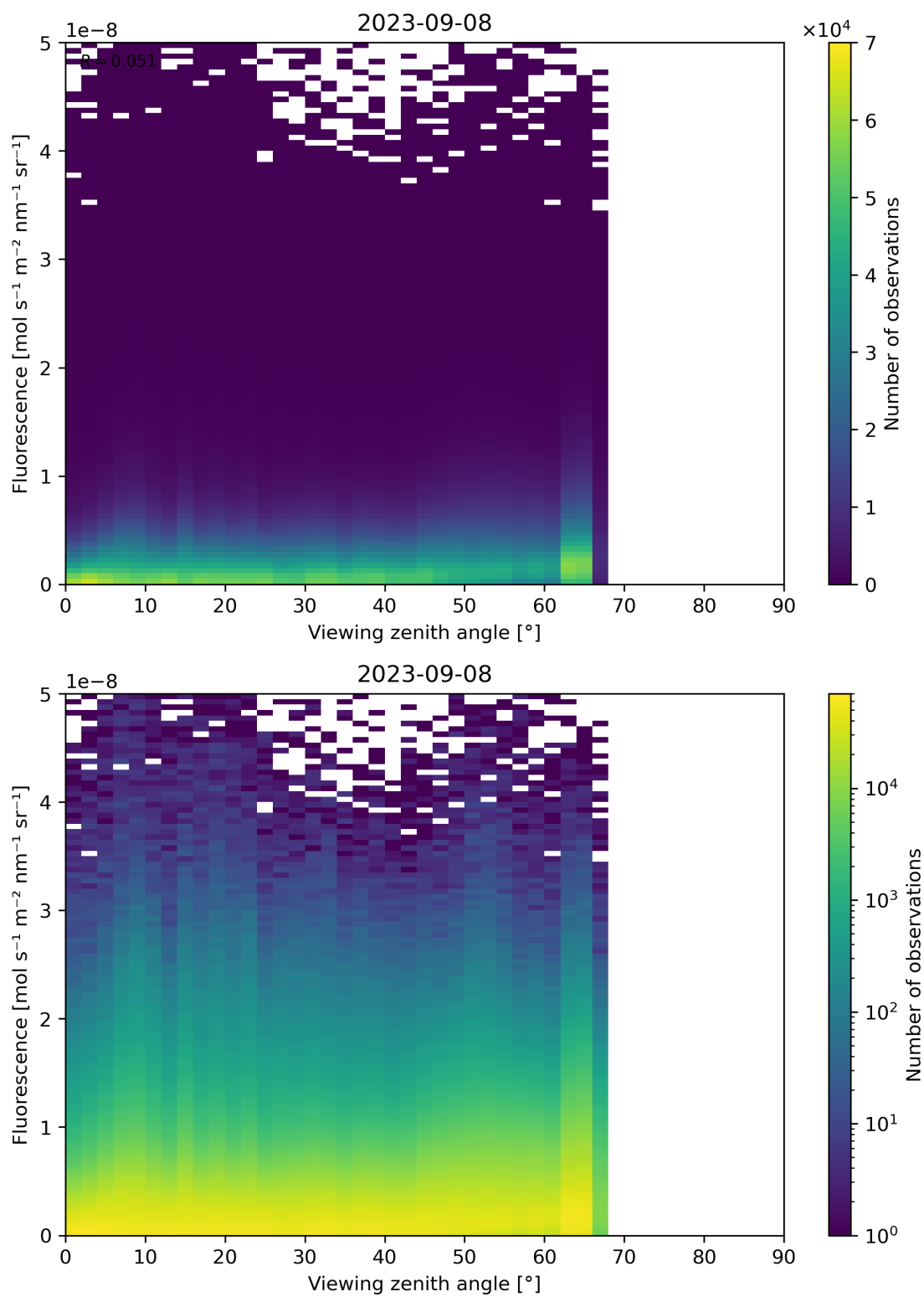
Figure 134: Scatter density plot of “Viewing zenith angle” against “Fluorescence” for 2023-09-07 to 2023-09-09.
