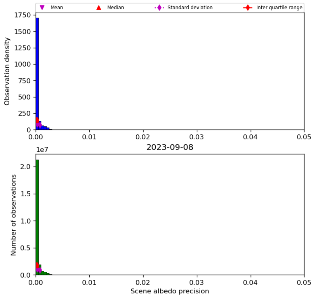
Figure 35: Histogram of “Scene albedo precision” for 2023-09-07 to 2023-09-09
