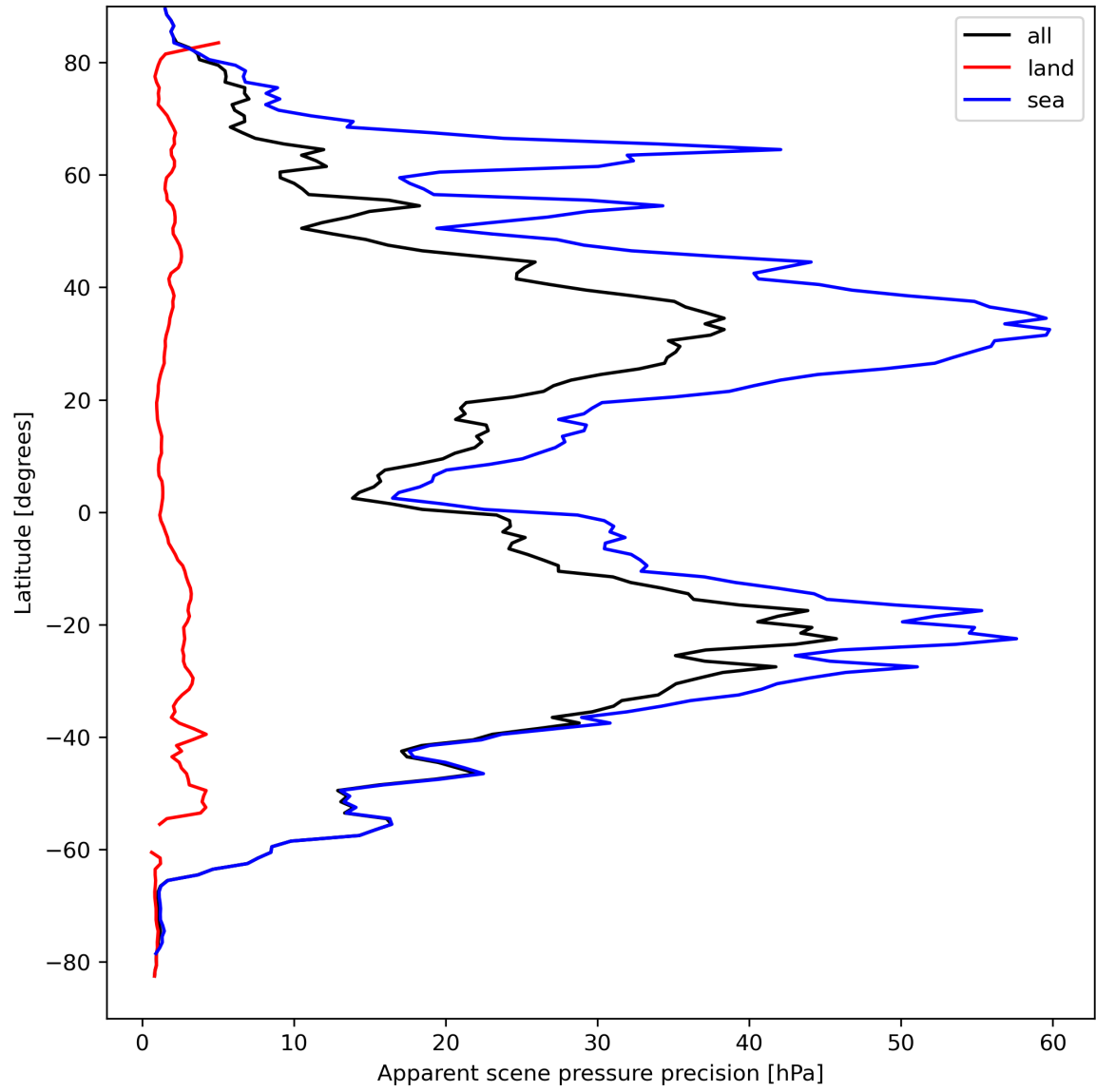
Figure 20: Zonal average of “Apparent scene pressure precision” for 2023-09-07 to 2023-09-09.
