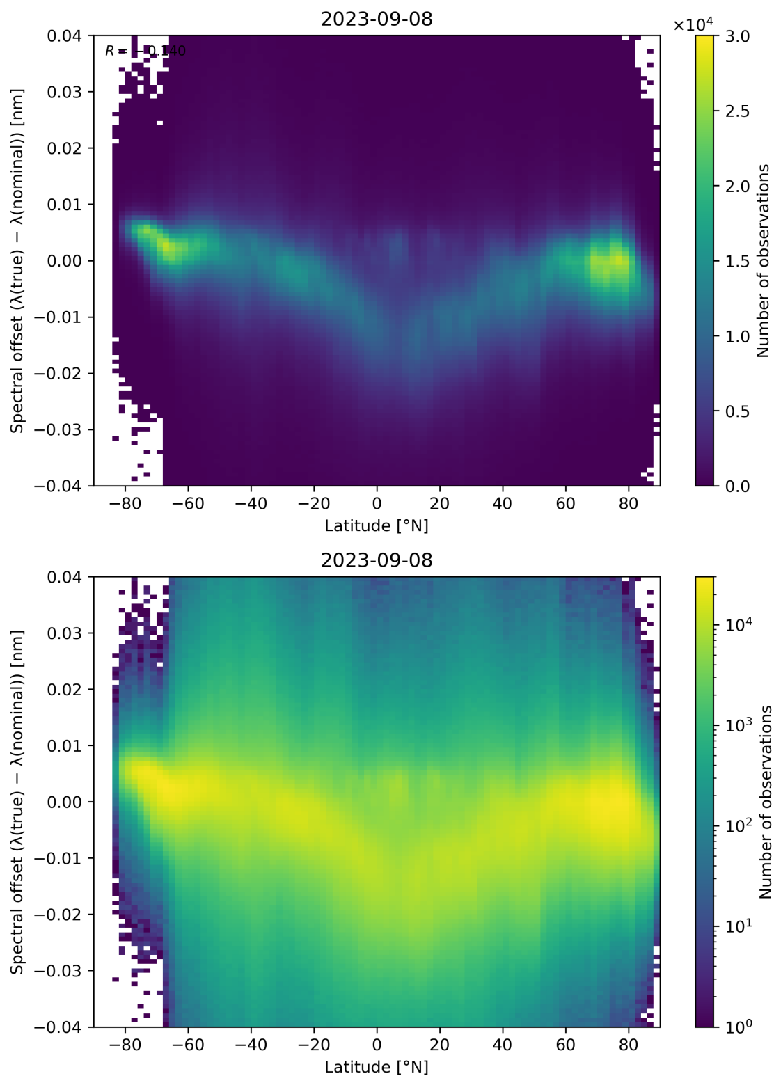
Figure 105: Scatter density plot of “Latitude” against “Spectral offset ( \lambda(\text{true}) - \lambda(\text{nominal}) )” for 2023-09-07 to 2023-09-09.
