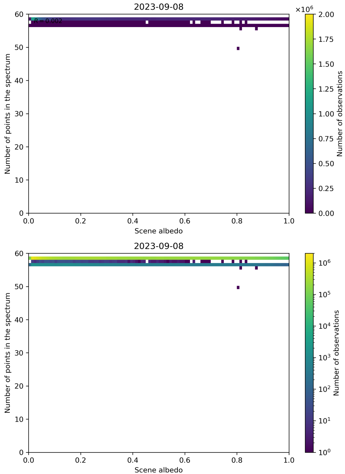
Figure 116: Scatter density plot of “Scene albedo” against “Number of points in the spectrum” for 2023-09-07 to 2023-09-09.
