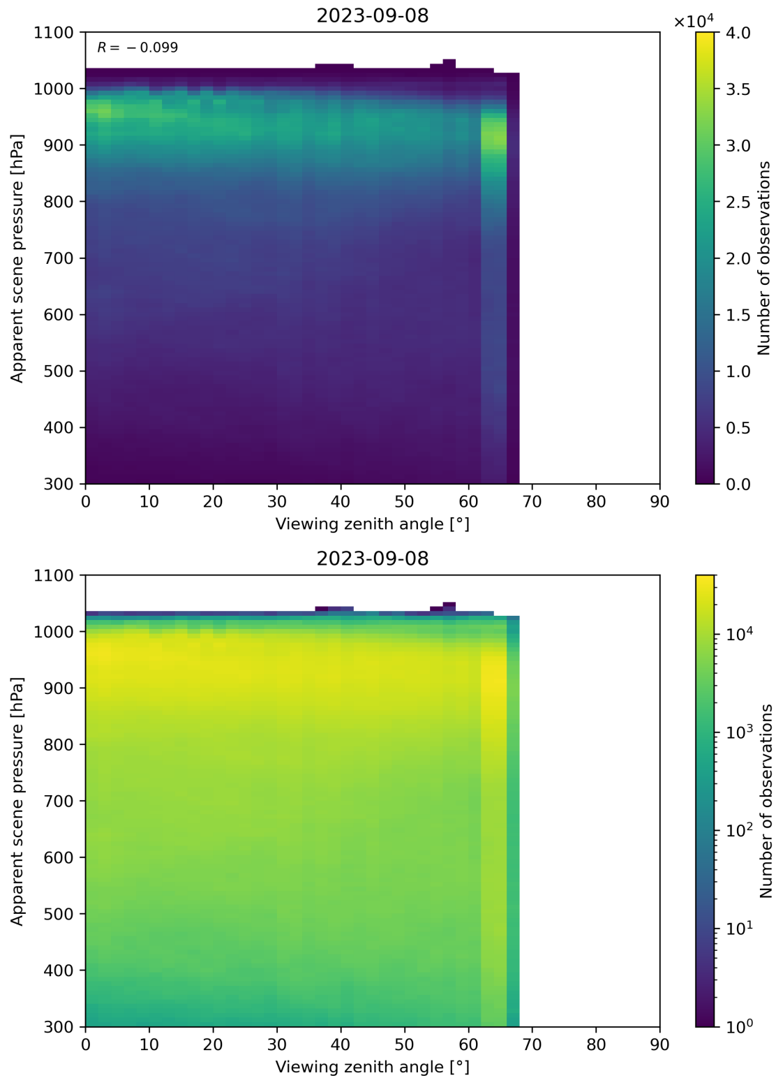
Figure 129: Scatter density plot of “Viewing zenith angle” against “Apparent scene pressure” for 2023-09-07 to 2023-09-09.
