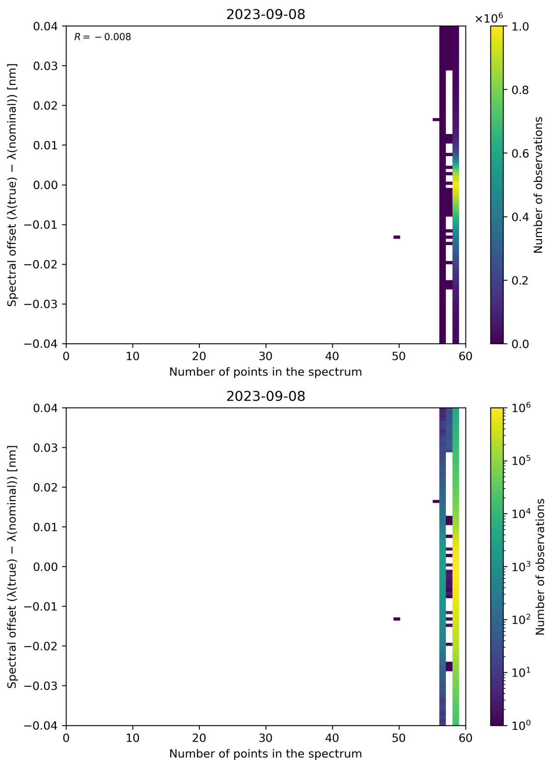
Figure 110: Scatter density plot of “Number of points in the spectrum” against “Spectral offset ( \lambda(\text{true}) - \lambda(\text{nominal}) )” for 2023-09-07 to 2023-09-09.
