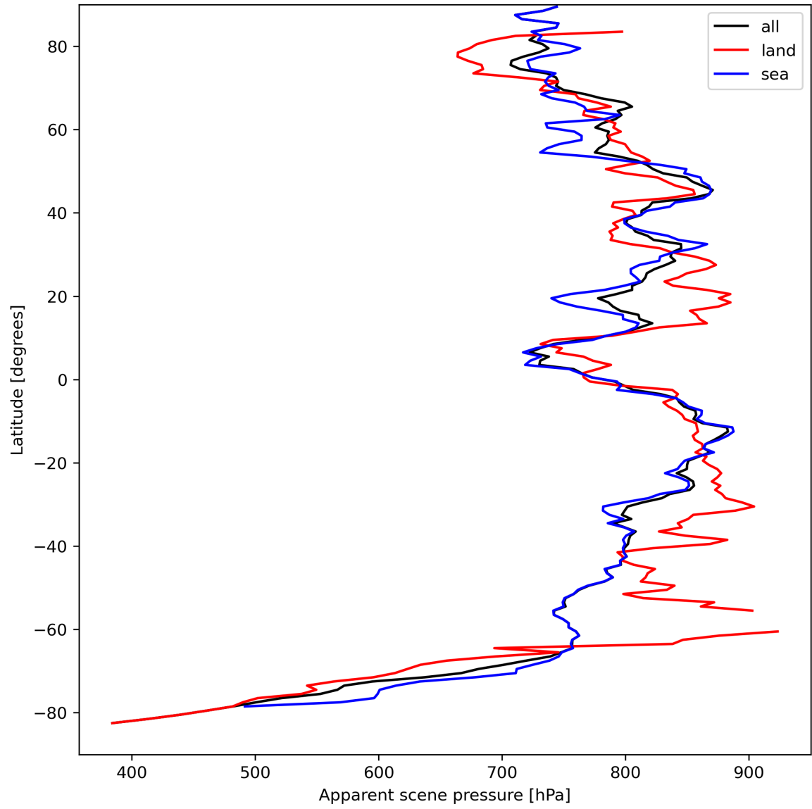
Figure 19: Zonal average of “Apparent scene pressure” for 2023-09-07 to 2023-09-09.
