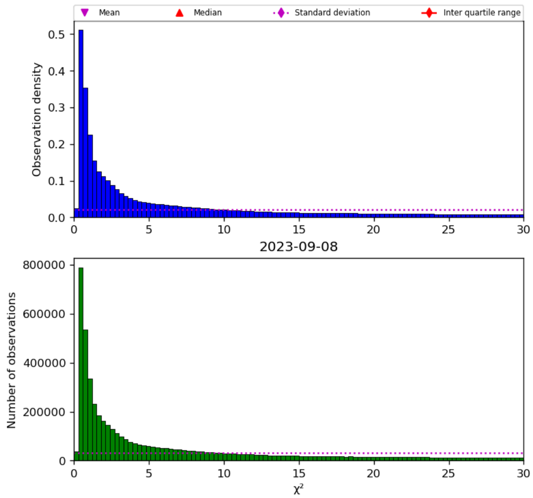
Figure 38: Histogram of “ \chi^2 ” for 2023-09-07 to 2023-09-09
