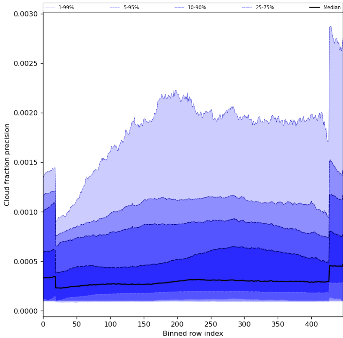
Figure 50: Along track statistics of “Cloud fraction precision” for 2023-09-07 to 2023-09-09
