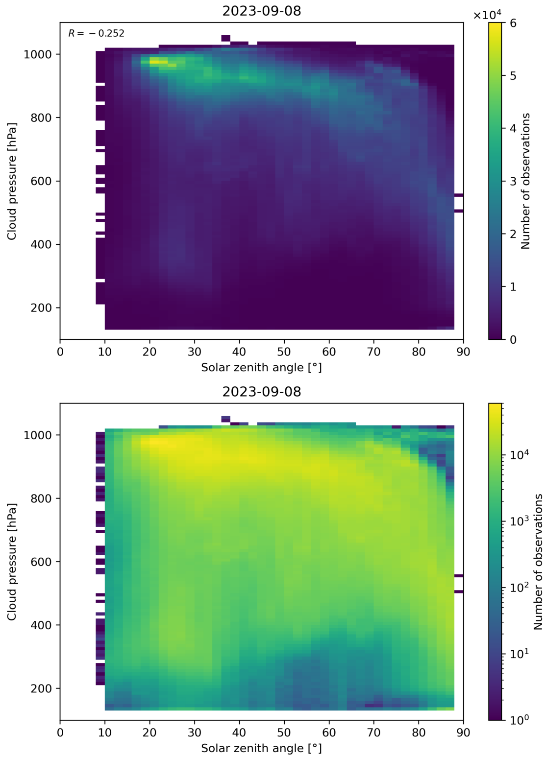
Figure 122: Scatter density plot of “Solar zenith angle” against “Cloud pressure” for 2023-09-07 to 2023-09-09.
