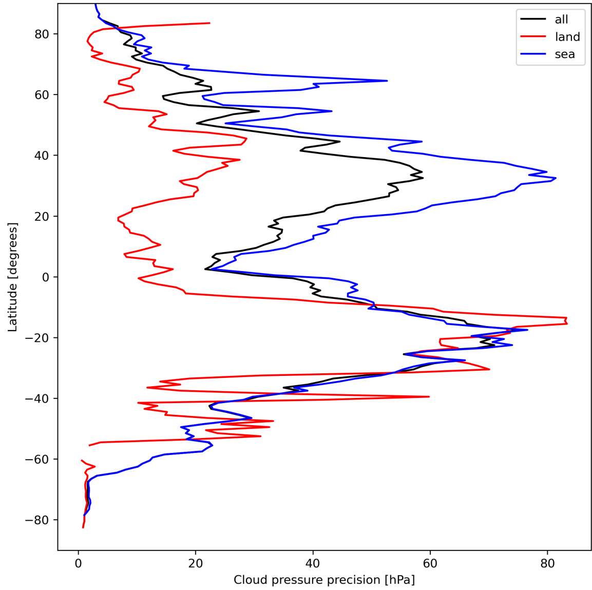
Figure 14: Zonal average of “Cloud pressure precision” for 2023-09-07 to 2023-09-09.
