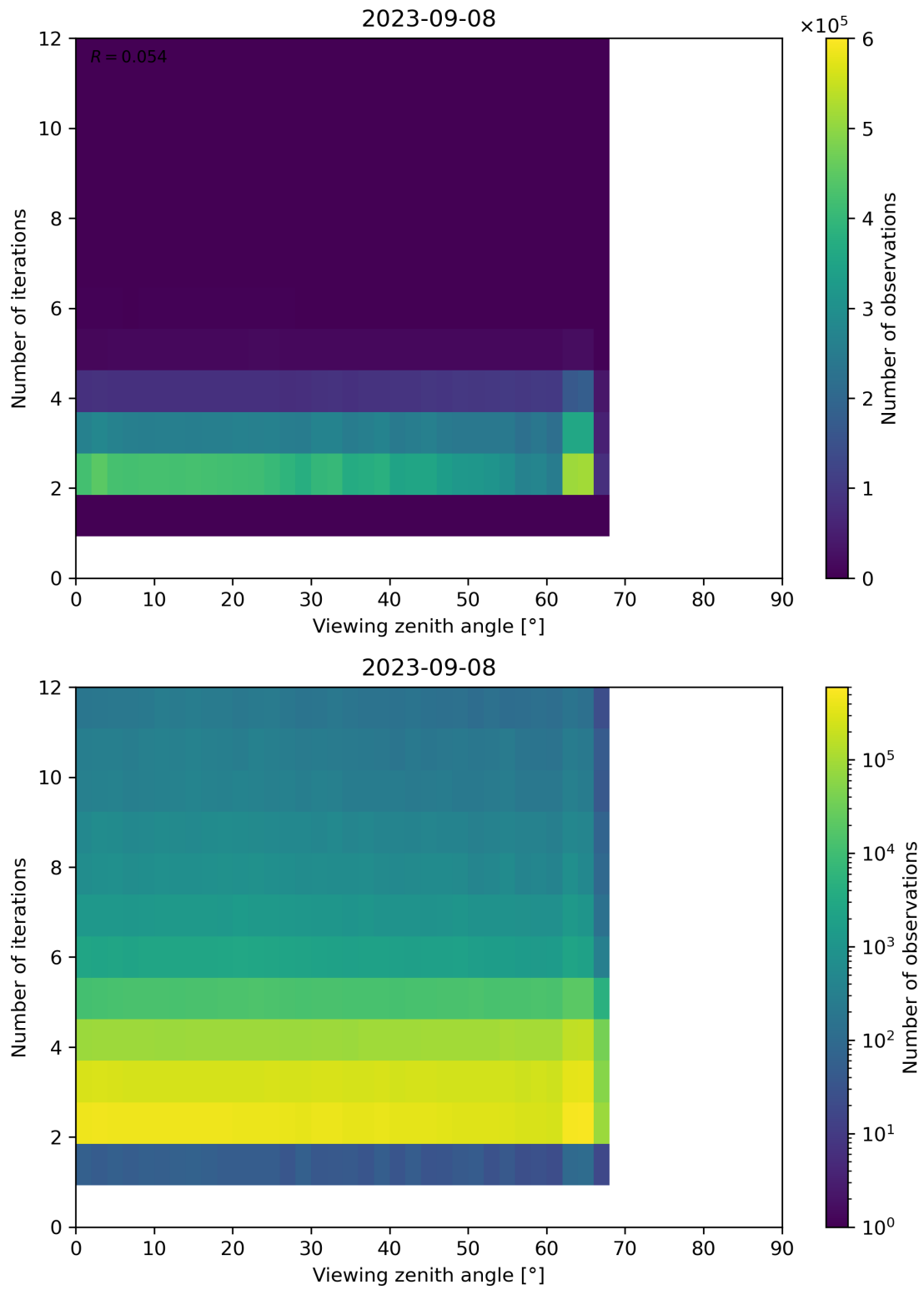
Figure 136: Scatter density plot of “Viewing zenith angle” against “Number of iterations” for 2023-09-07 to 2023-09-09.
