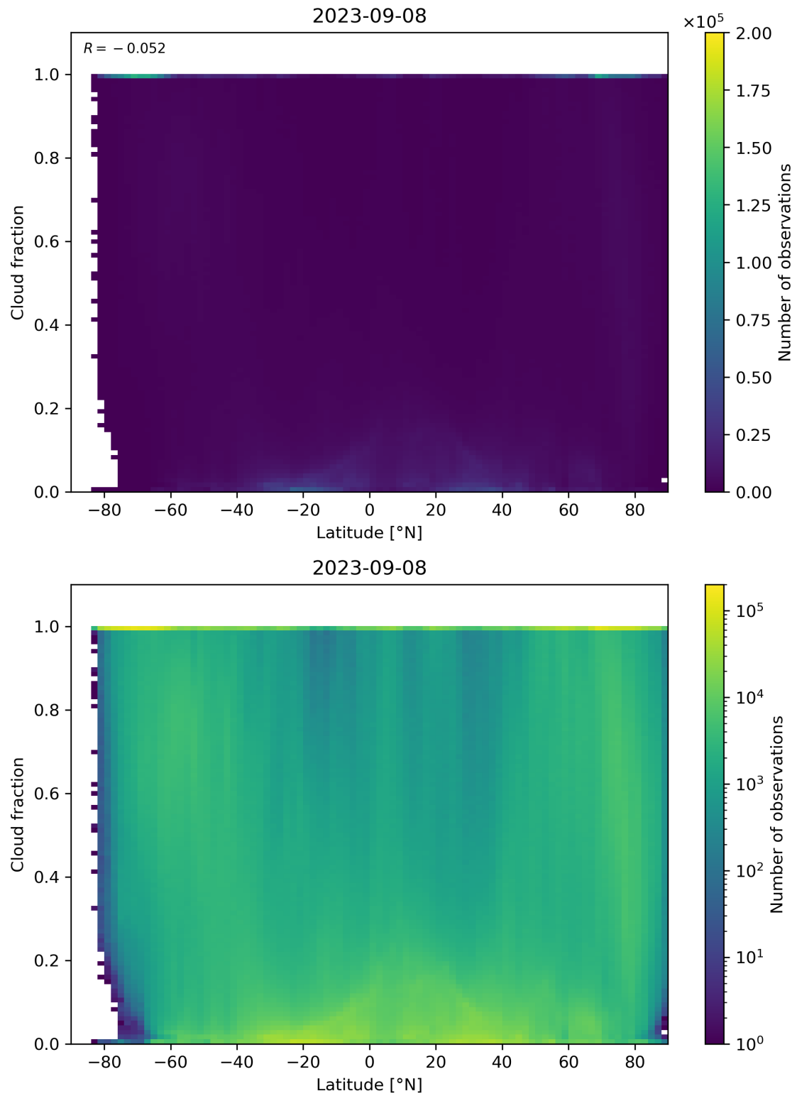
Figure 99: Scatter density plot of “Latitude” against “Cloud fraction” for 2023-09-07 to 2023-09-09.
