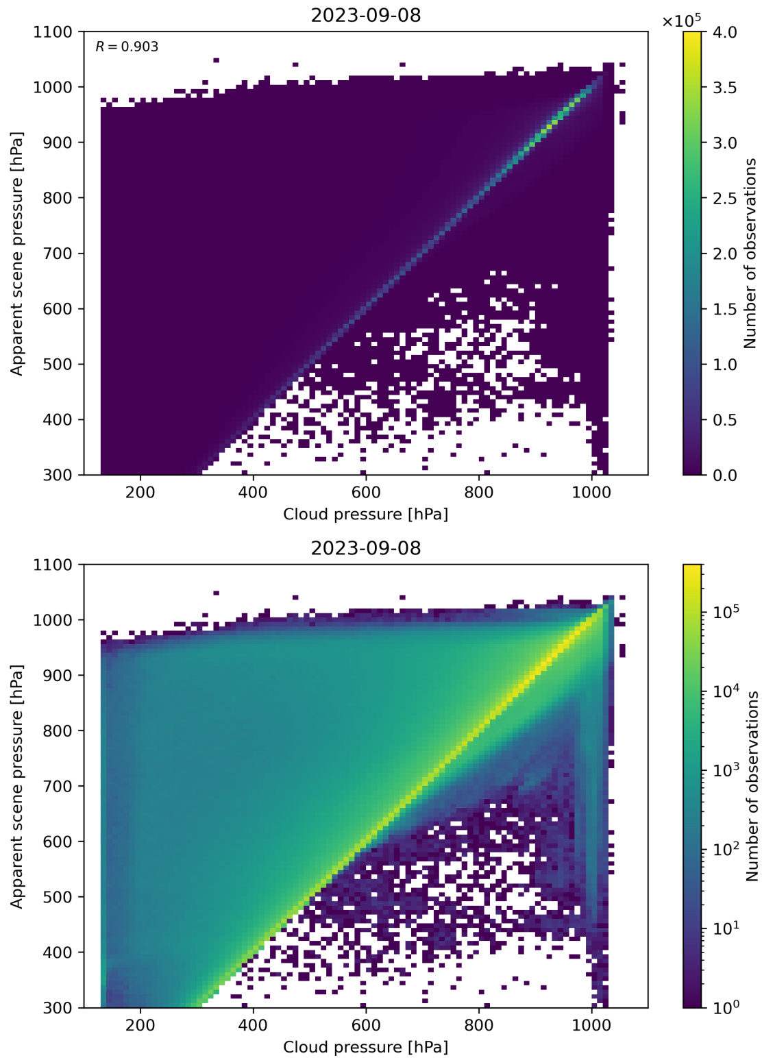
Figure 84: Scatter density plot of “Cloud pressure” against “Apparent scene pressure” for 2023-09-07 to 2023-09-09.
