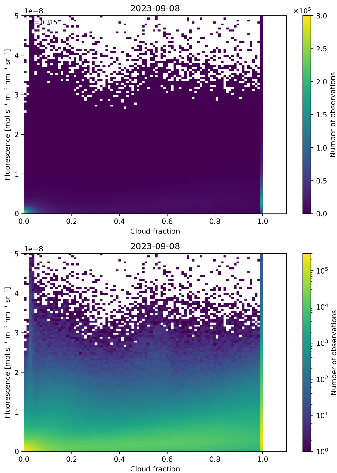
Figure 79: Scatter density plot of “Cloud fraction” against “Fluorescence” for 2023-09-07 to 2023-09-09.
