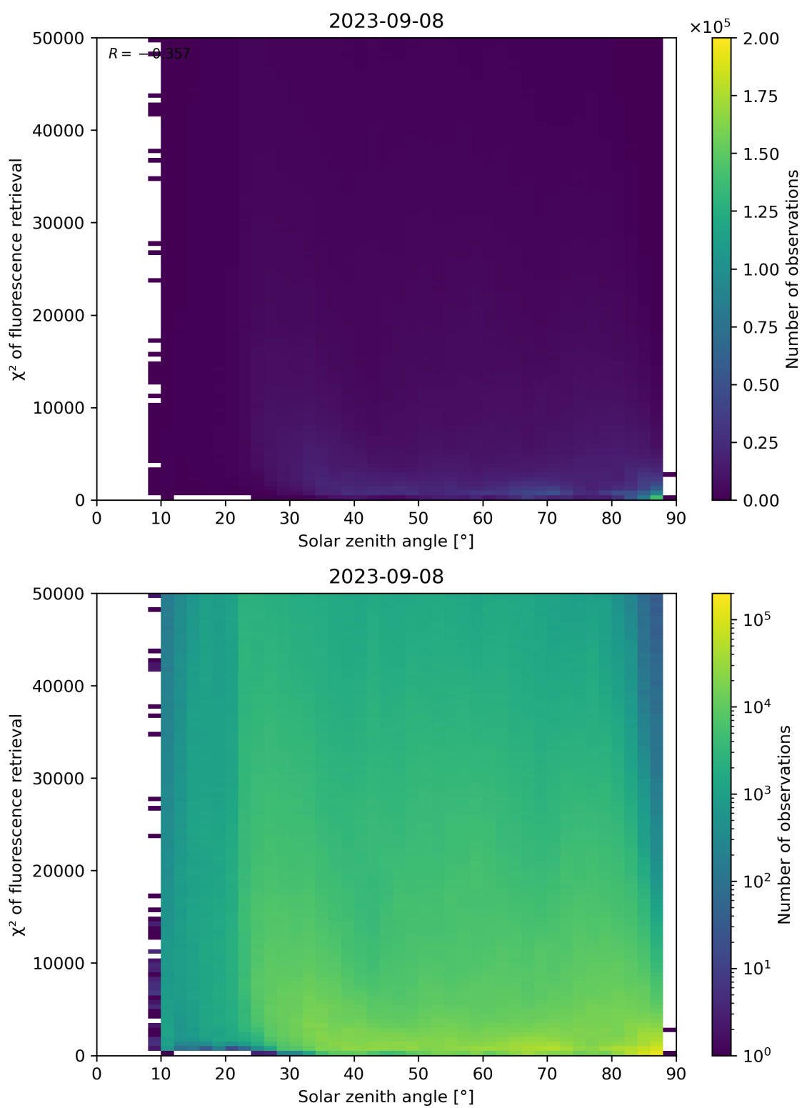
Figure 120: Scatter density plot of “Solar zenith angle” against “ \chi^2 of fluorescence retrieval” for 2023-09-07 to 2023-09-09.
