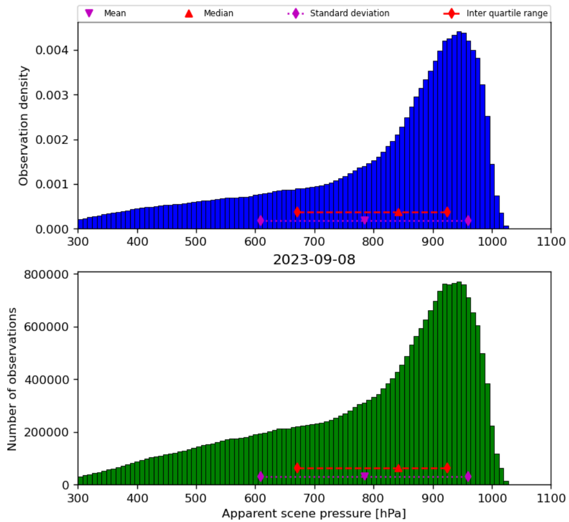
Figure 36: Histogram of “Apparent scene pressure” for 2023-09-07 to 2023-09-09
