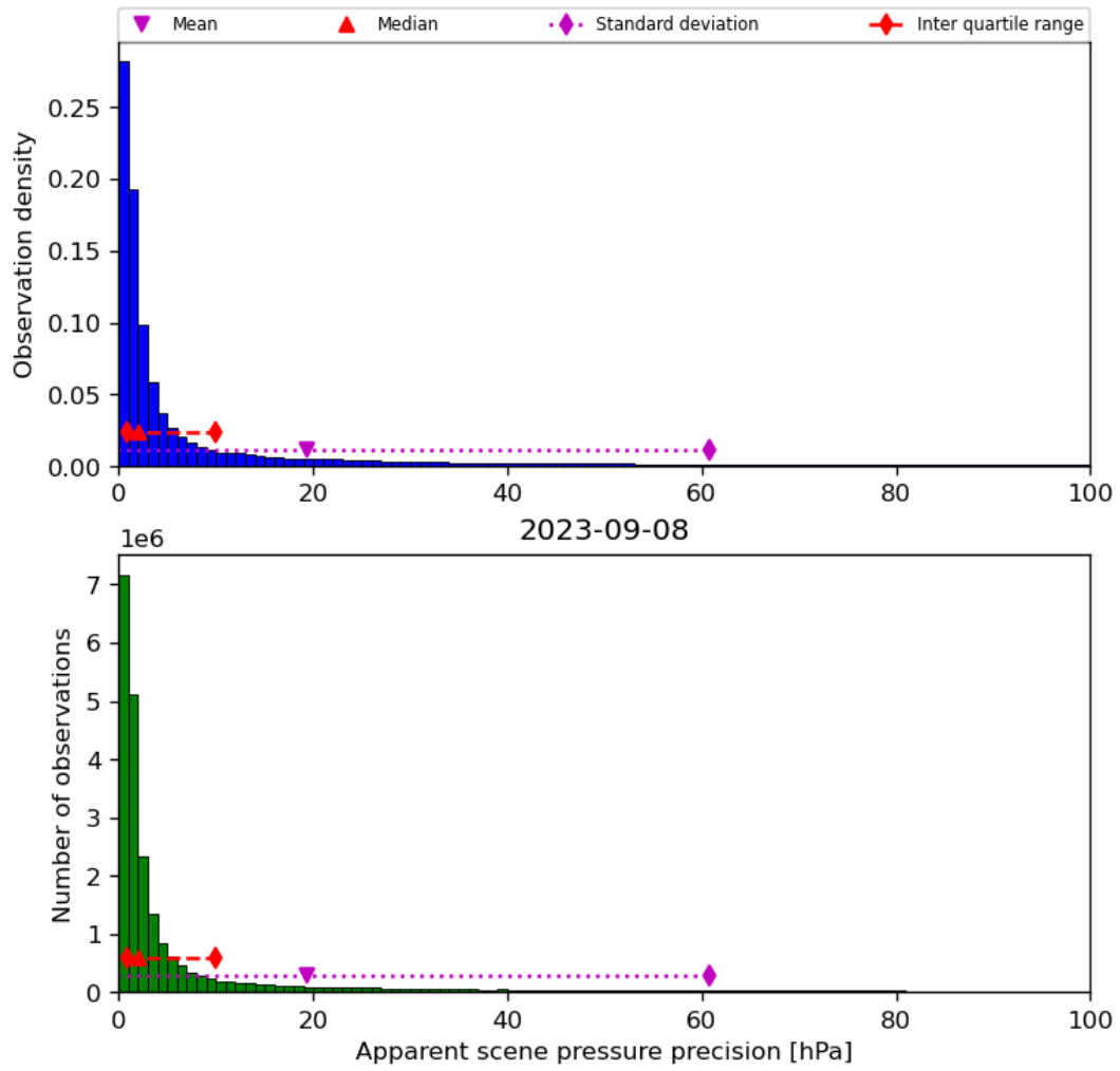
Figure 37: Histogram of “Apparent scene pressure precision” for 2023-09-07 to 2023-09-09
