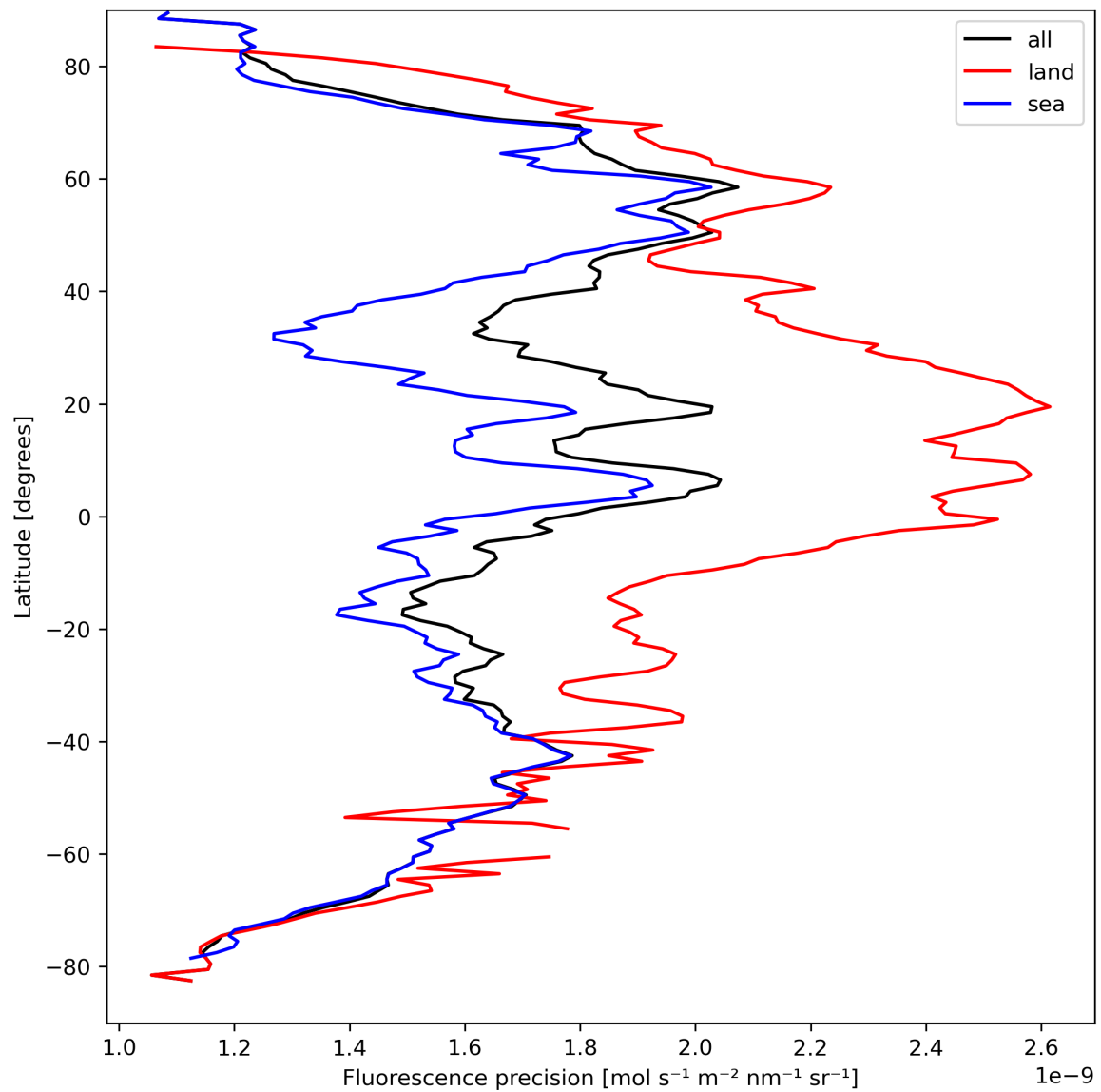
Figure 24: Zonal average of “Fluorescence precision” for 2023-09-07 to 2023-09-09.
