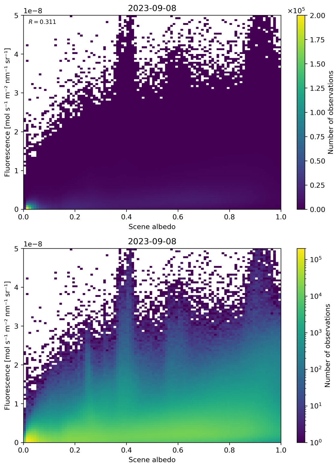
Figure 114: Scatter density plot of “Scene albedo” against “Fluorescence” for 2023-09-07 to 2023-09-09.
