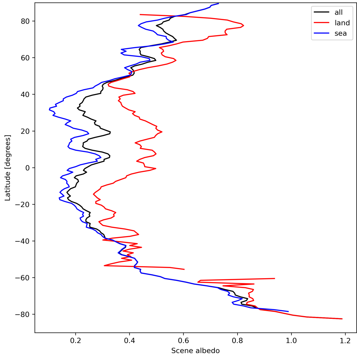
Figure 17: Zonal average of “Scene albedo” for 2023-09-07 to 2023-09-09.
