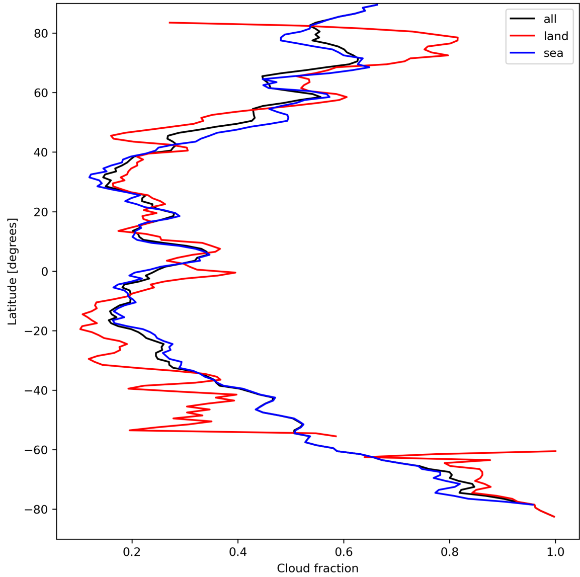
Figure 15: Zonal average of “Cloud fraction” for 2023-09-07 to 2023-09-09.
