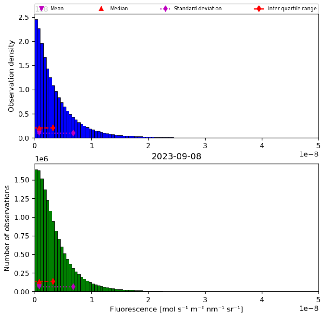
Figure 40: Histogram of “Fluorescence” for 2023-09-07 to 2023-09-09
