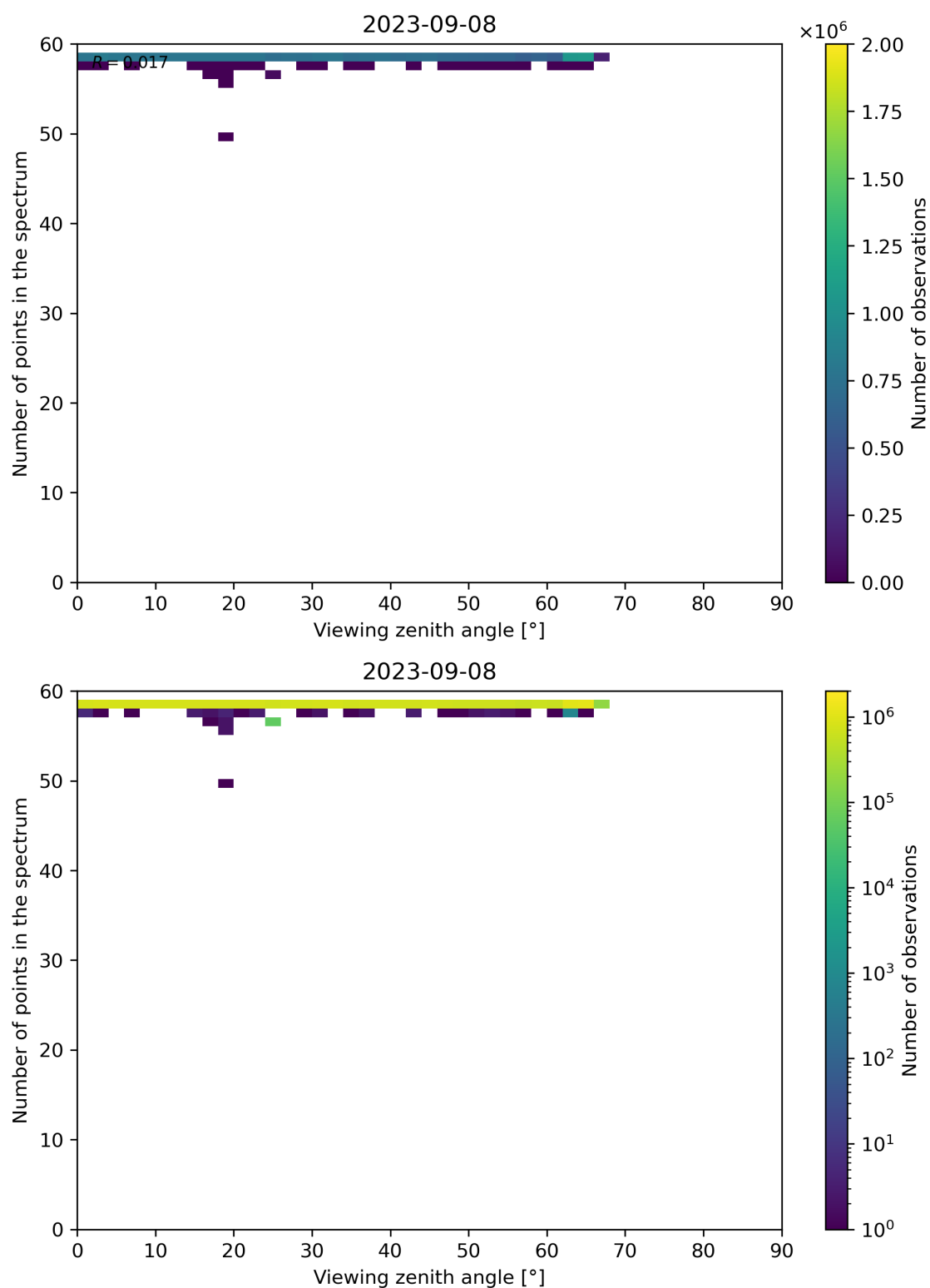
Figure 137: Scatter density plot of “Viewing zenith angle” against “Number of points in the spectrum” for 2023-09-07 to 2023-09-09.
