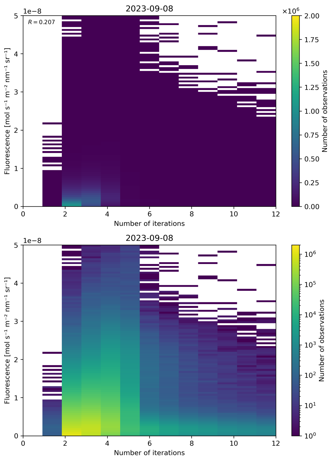
Figure 107: Scatter density plot of “Number of iterations” against “Fluorescence” for 2023-09-07 to 2023-09-09.
