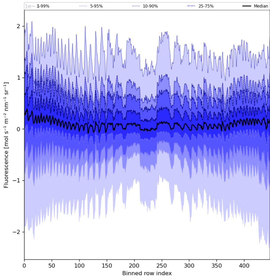
Figure 57: Along track statistics of “Fluorescence” for 2023-09-07 to 2023-09-09
