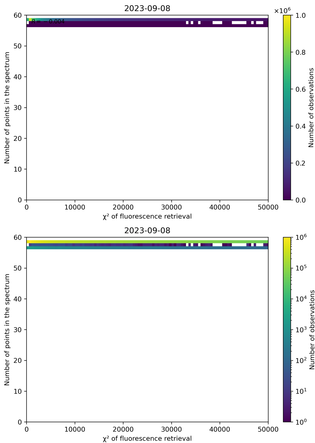
Figure 71: Scatter density plot of “ \chi^2 of fluorescence retrieval” against “Number of points in the spectrum” for 2023-09-07 to 2023-09-09.
