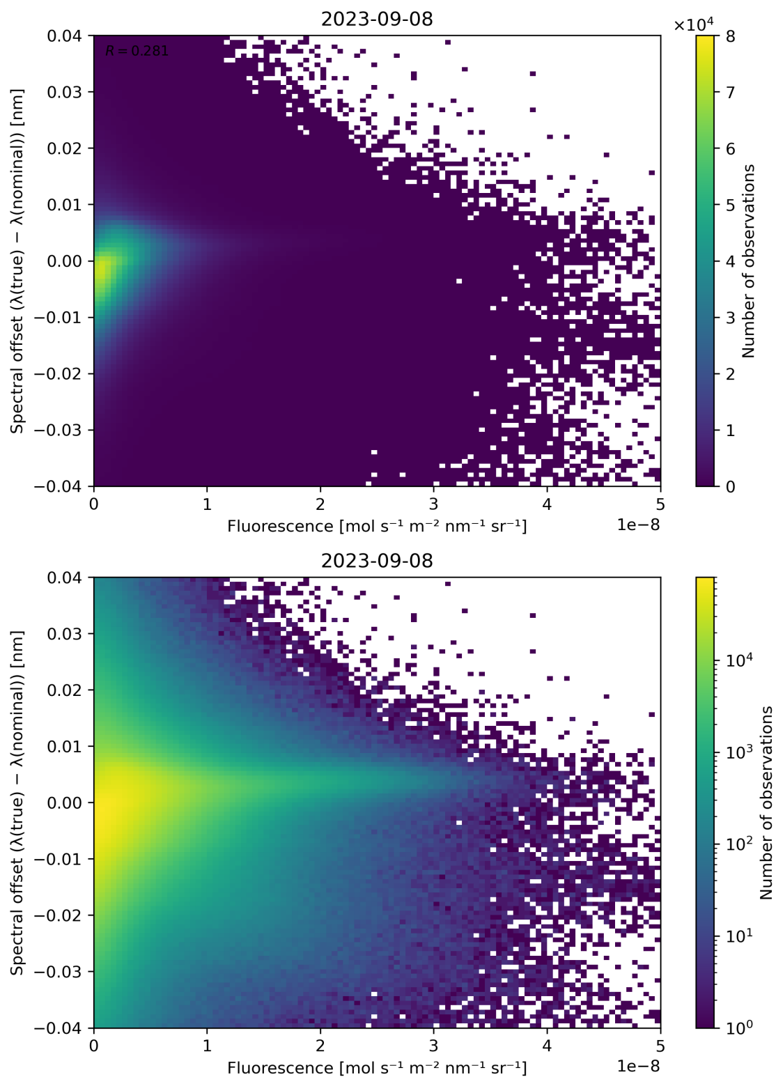
Figure 95: Scatter density plot of “Fluorescence” against “Spectral offset ( \lambda(\text{true}) - \lambda(\text{nominal}) )” for 2023-09-07 to 2023-09-09.
