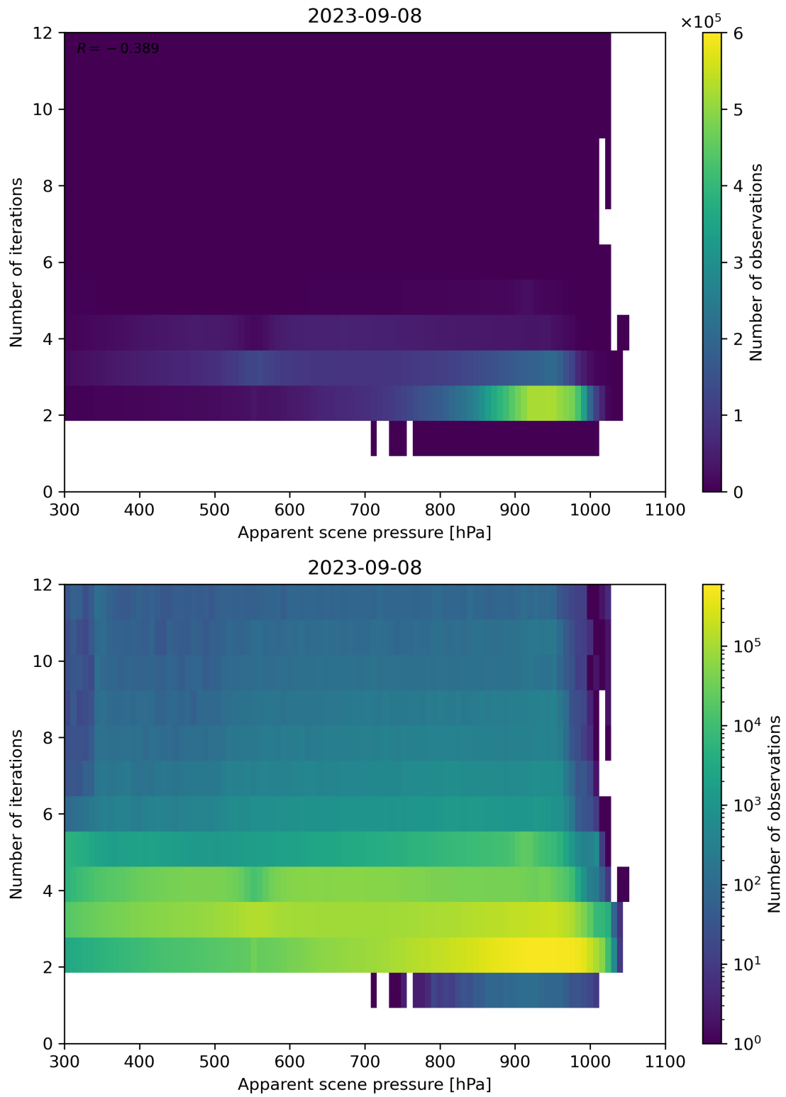
Figure 66: Scatter density plot of “Apparent scene pressure” against “Number of iterations” for 2023-09-07 to 2023-09-09.
