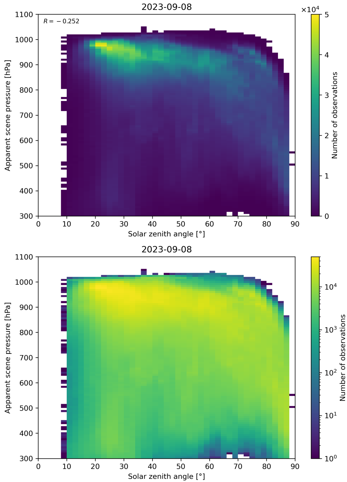
Figure 118: Scatter density plot of “Solar zenith angle” against “Apparent scene pressure” for 2023-09-07 to 2023-09-09.
