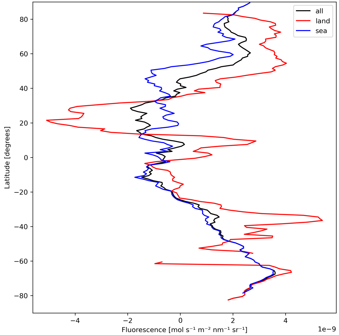
Figure 23: Zonal average of “Fluorescence” for 2023-09-07 to 2023-09-09.
