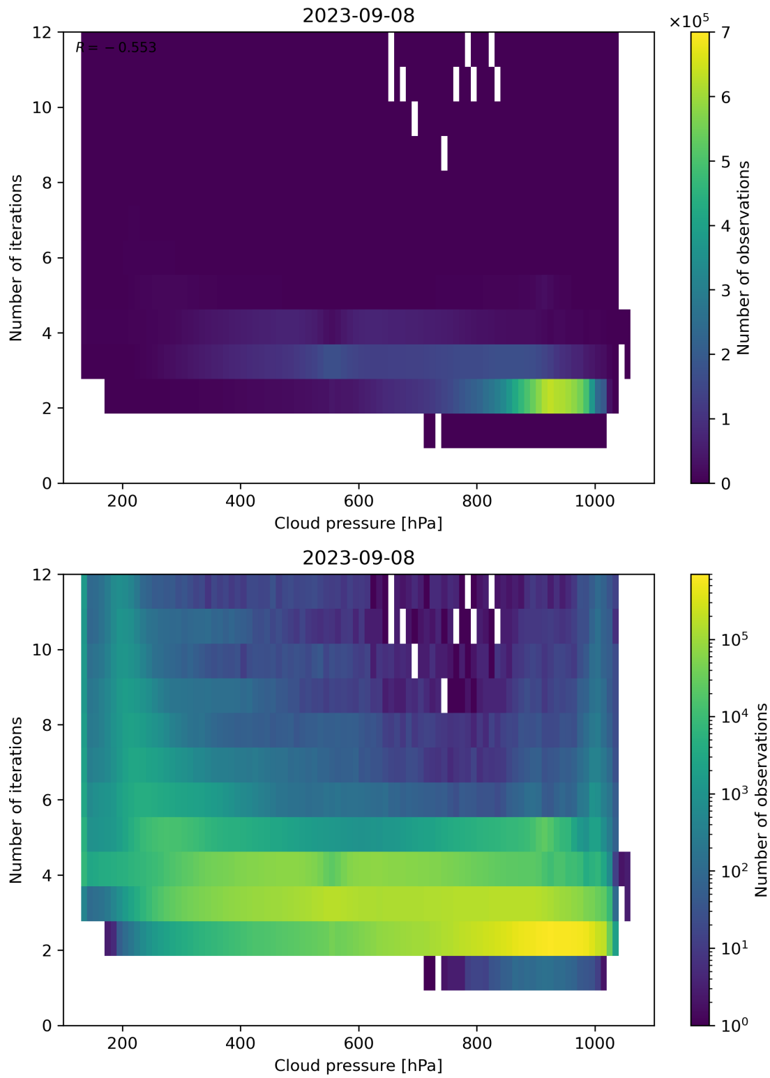
Figure 89: Scatter density plot of “Cloud pressure” against “Number of iterations” for 2023-09-07 to 2023-09-09.
