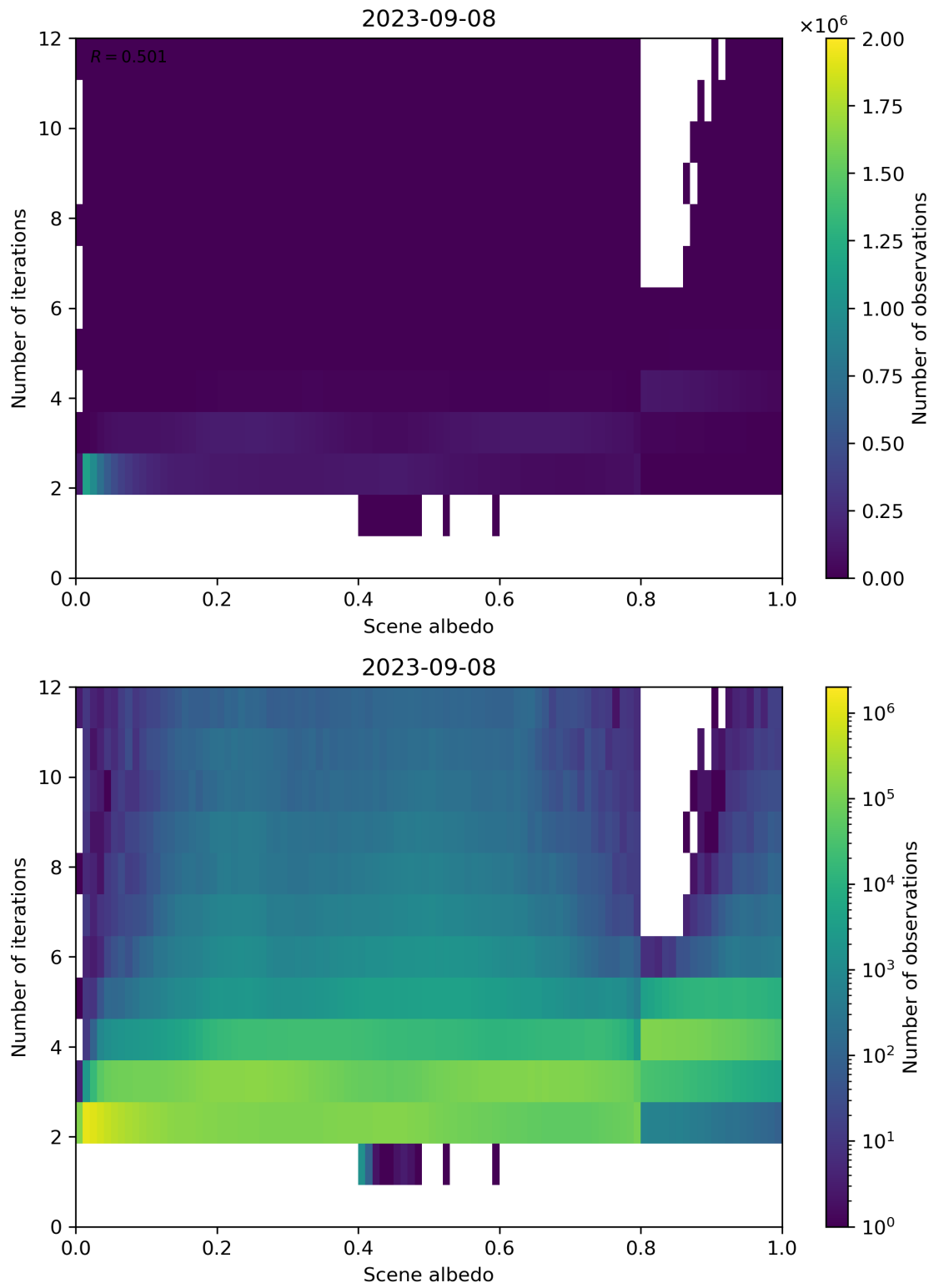
Figure 115: Scatter density plot of “Scene albedo” against “Number of iterations” for 2023-09-07 to 2023-09-09.
