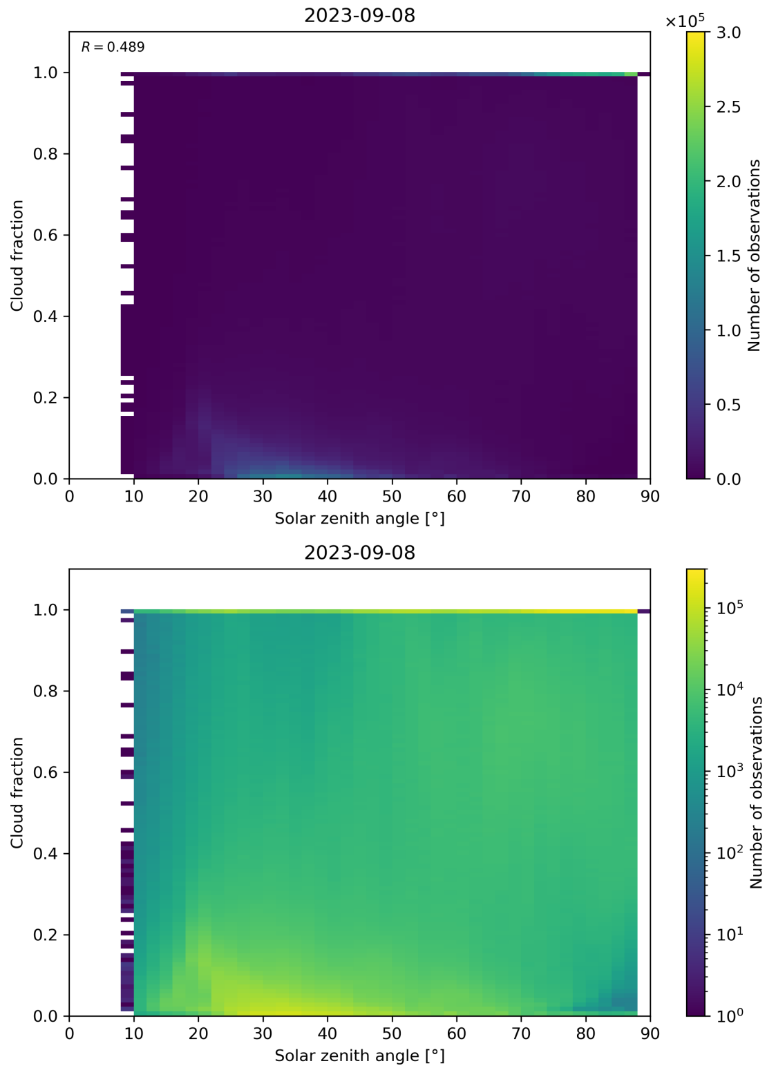
Figure 121: Scatter density plot of “Solar zenith angle” against “Cloud fraction” for 2023-09-07 to 2023-09-09.
