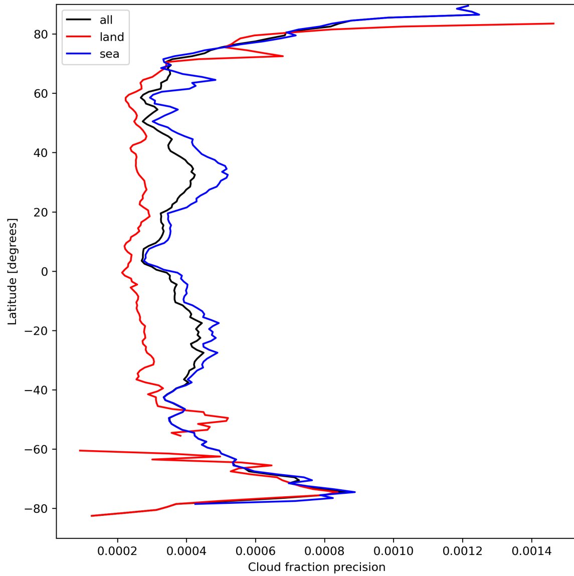
Figure 16: Zonal average of “Cloud fraction precision” for 2023-09-07 to 2023-09-09.
