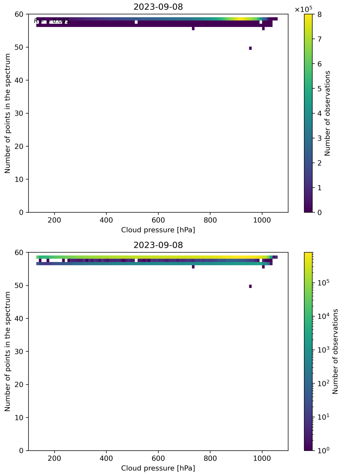
Figure 90: Scatter density plot of “Cloud pressure” against “Number of points in the spectrum” for 2023-09-07 to 2023-09-09.
