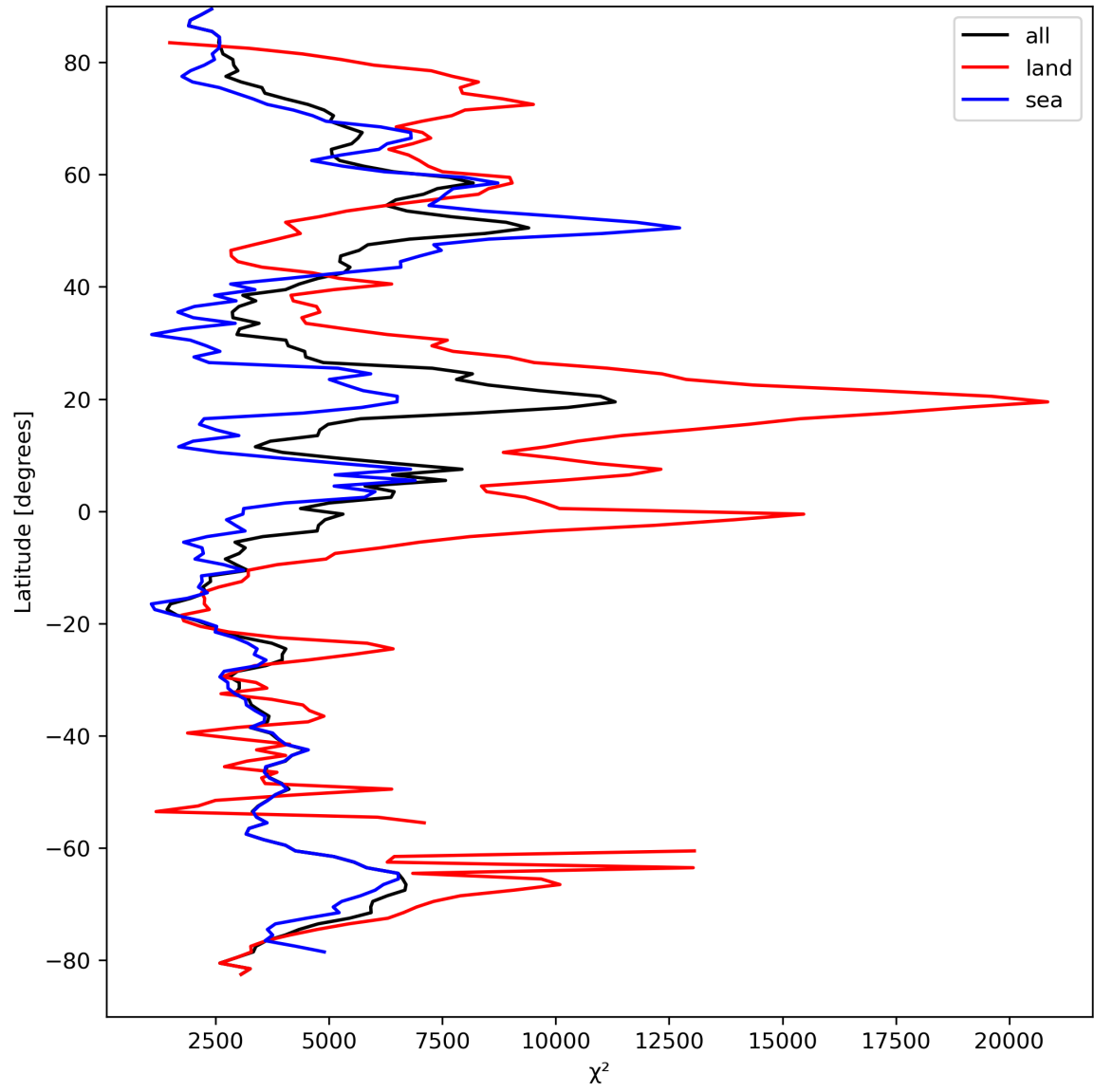
Figure 21: Zonal average of “ \chi^2 ” for 2023-09-07 to 2023-09-09.
