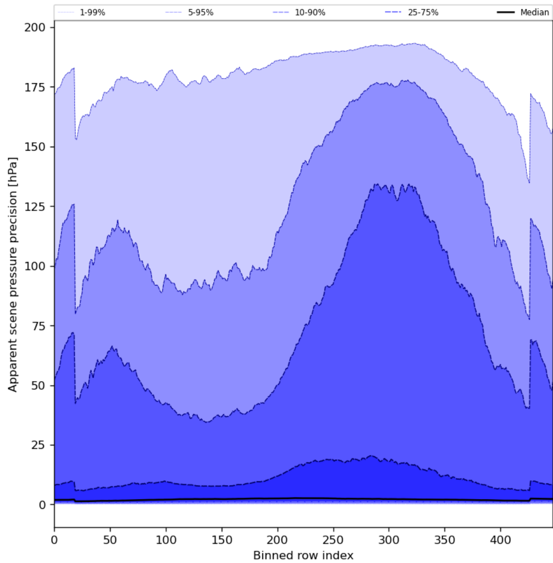
Figure 54: Along track statistics of “Apparent scene pressure precision” for 2023-09-07 to 2023-09-09
