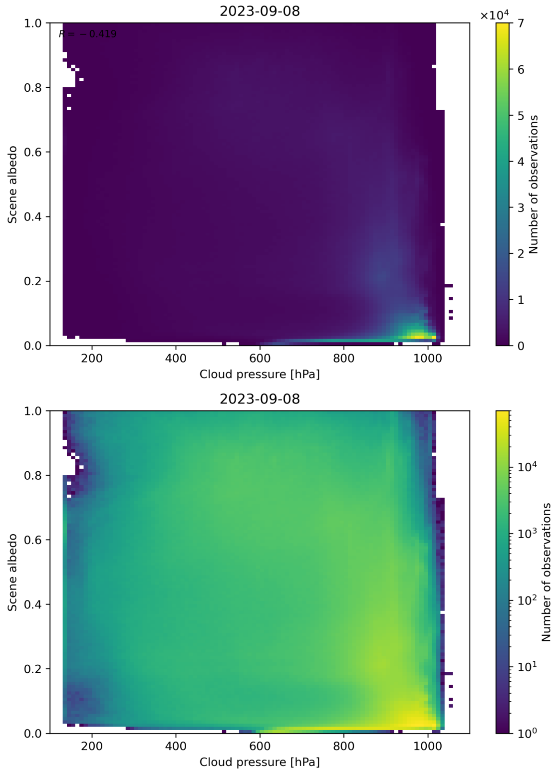
Figure 91: Scatter density plot of “Cloud pressure” against “Scene albedo” for 2023-09-07 to 2023-09-09.
