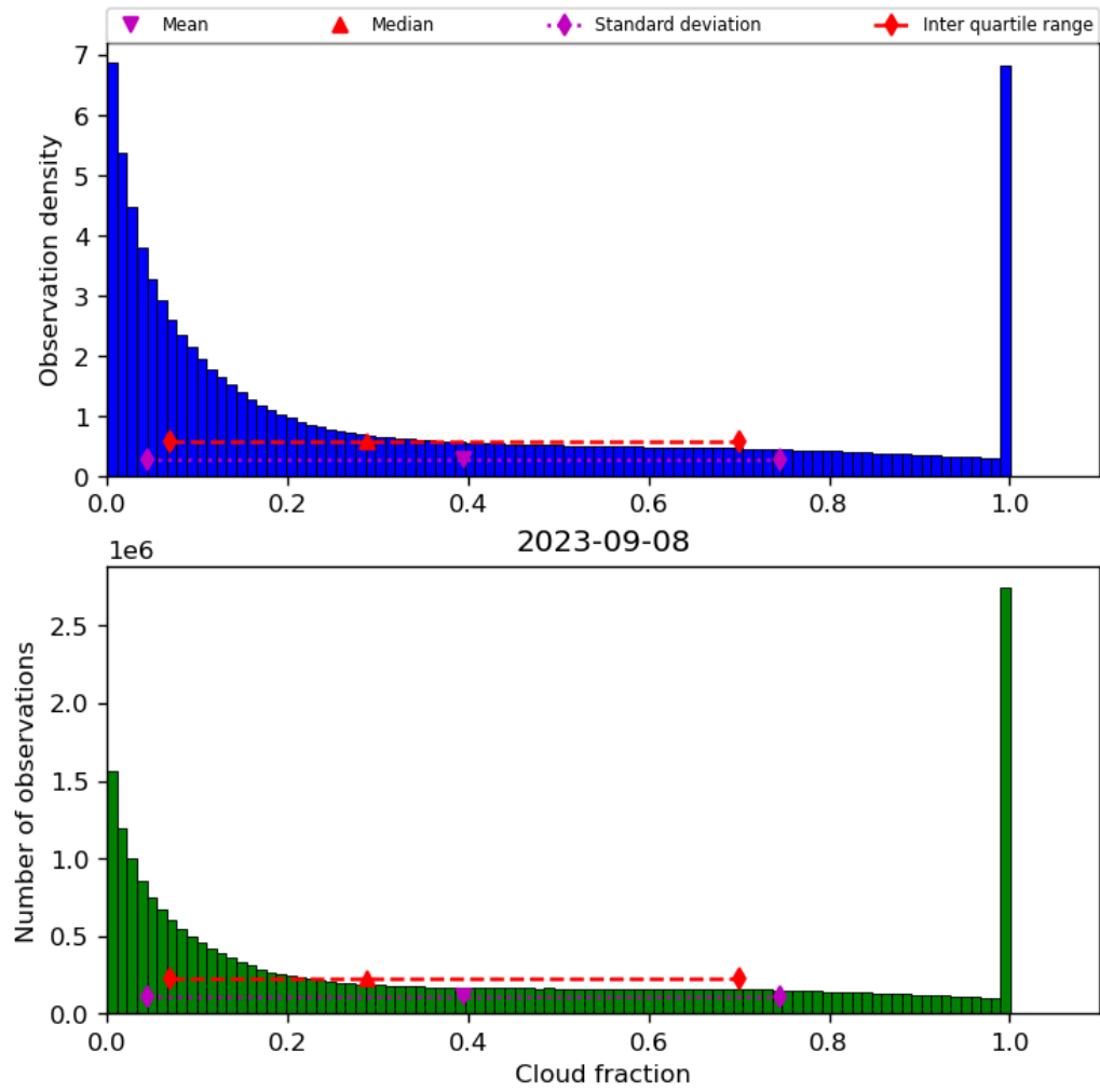
Figure 32: Histogram of “Cloud fraction” for 2023-09-07 to 2023-09-09
