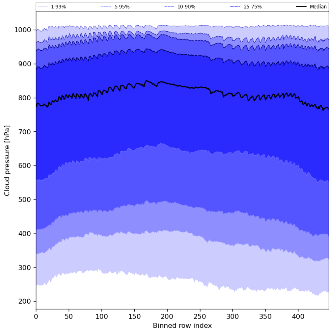
Figure 47: Along track statistics of “Cloud pressure” for 2023-09-07 to 2023-09-09
