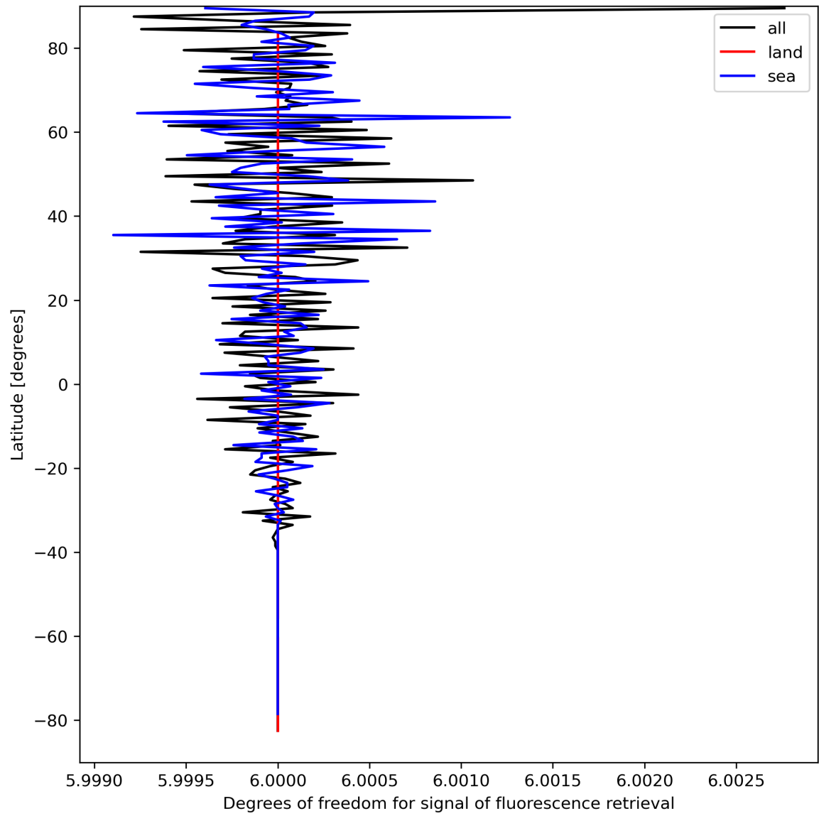
Figure 26: Zonal average of “Degrees of freedom for signal of fluorescence retrieval” for 2023-09-07 to 2023-09-09.
