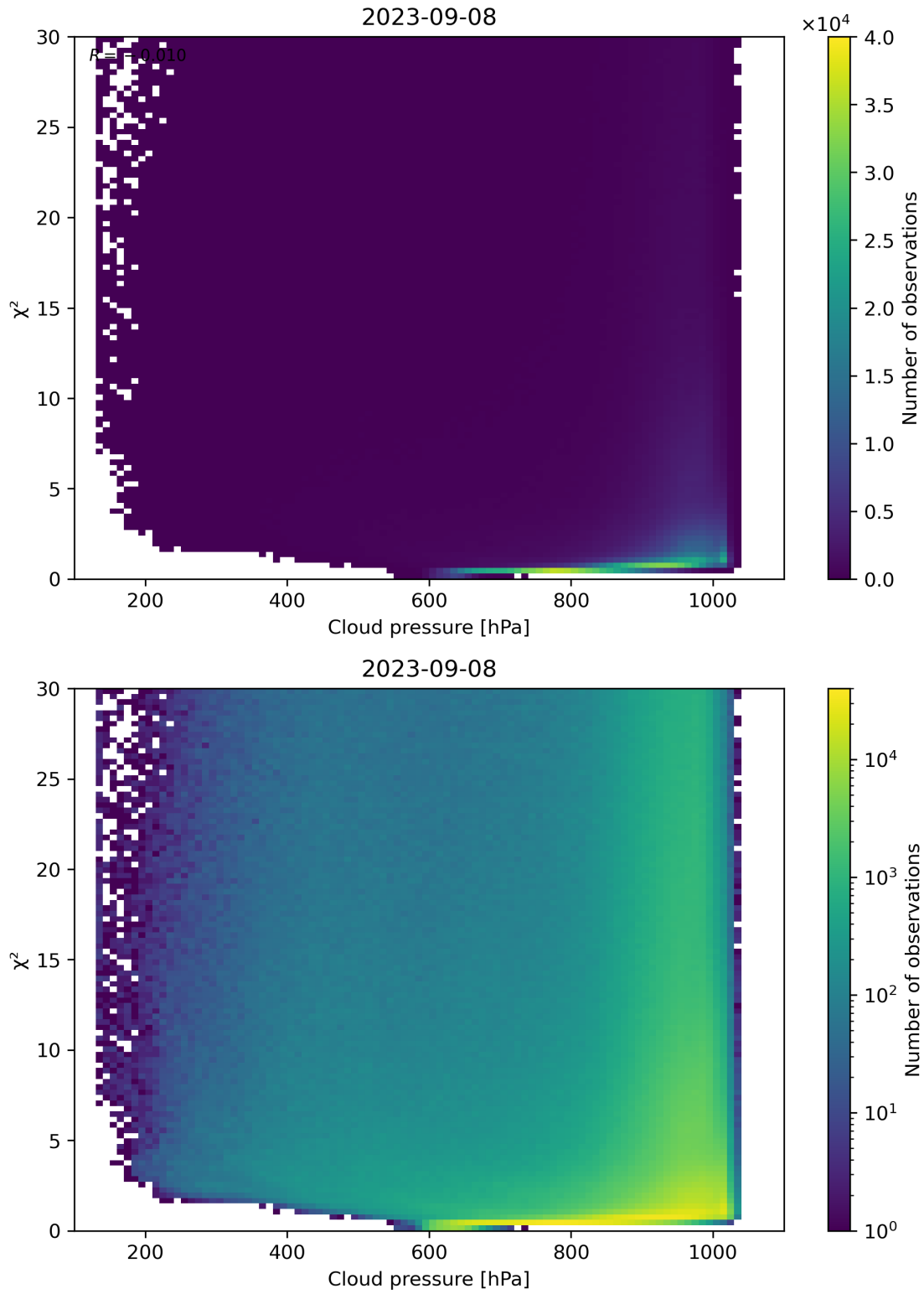
Figure 85: Scatter density plot of “Cloud pressure” against “ \chi^2 ” for 2023-09-07 to 2023-09-09.
