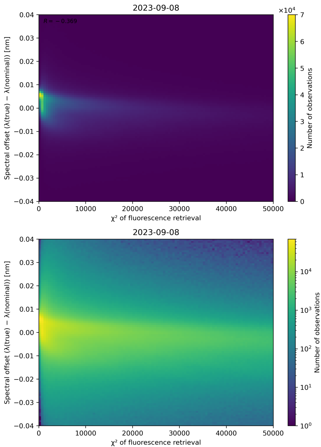
Figure 72: Scatter density plot of " \chi^2 of fluorescence retrieval" against "Spectral offset ( \lambda(\text{true}) - \lambda(\text{nominal}) )" for 2023-09-07 to 2023-09-09.
