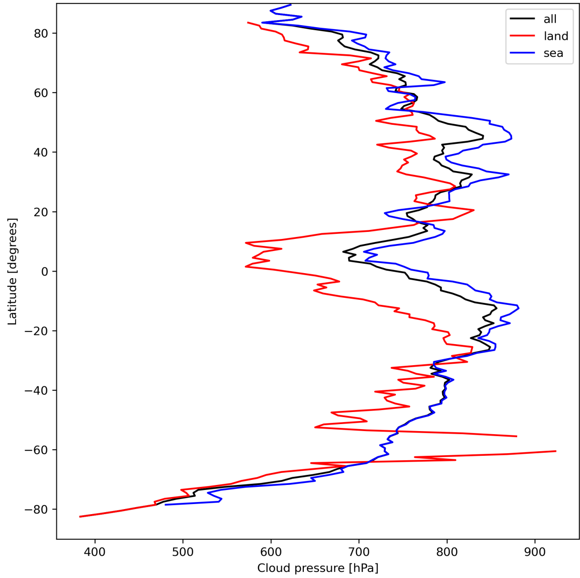
Figure 13: Zonal average of “Cloud pressure” for 2023-09-07 to 2023-09-09.
