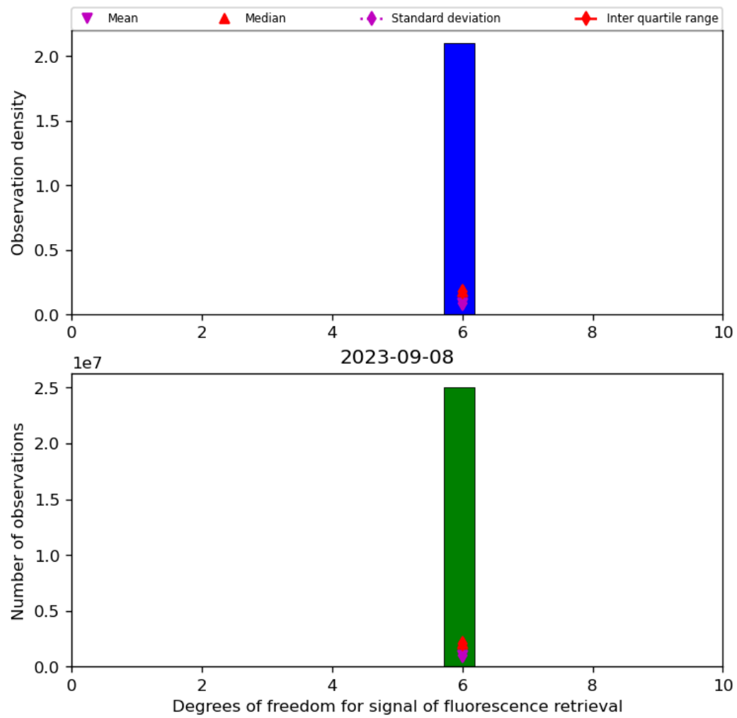
Figure 43: Histogram of “Degrees of freedom for signal of fluorescence retrieval” for 2023-09-07 to 2023-09-09
