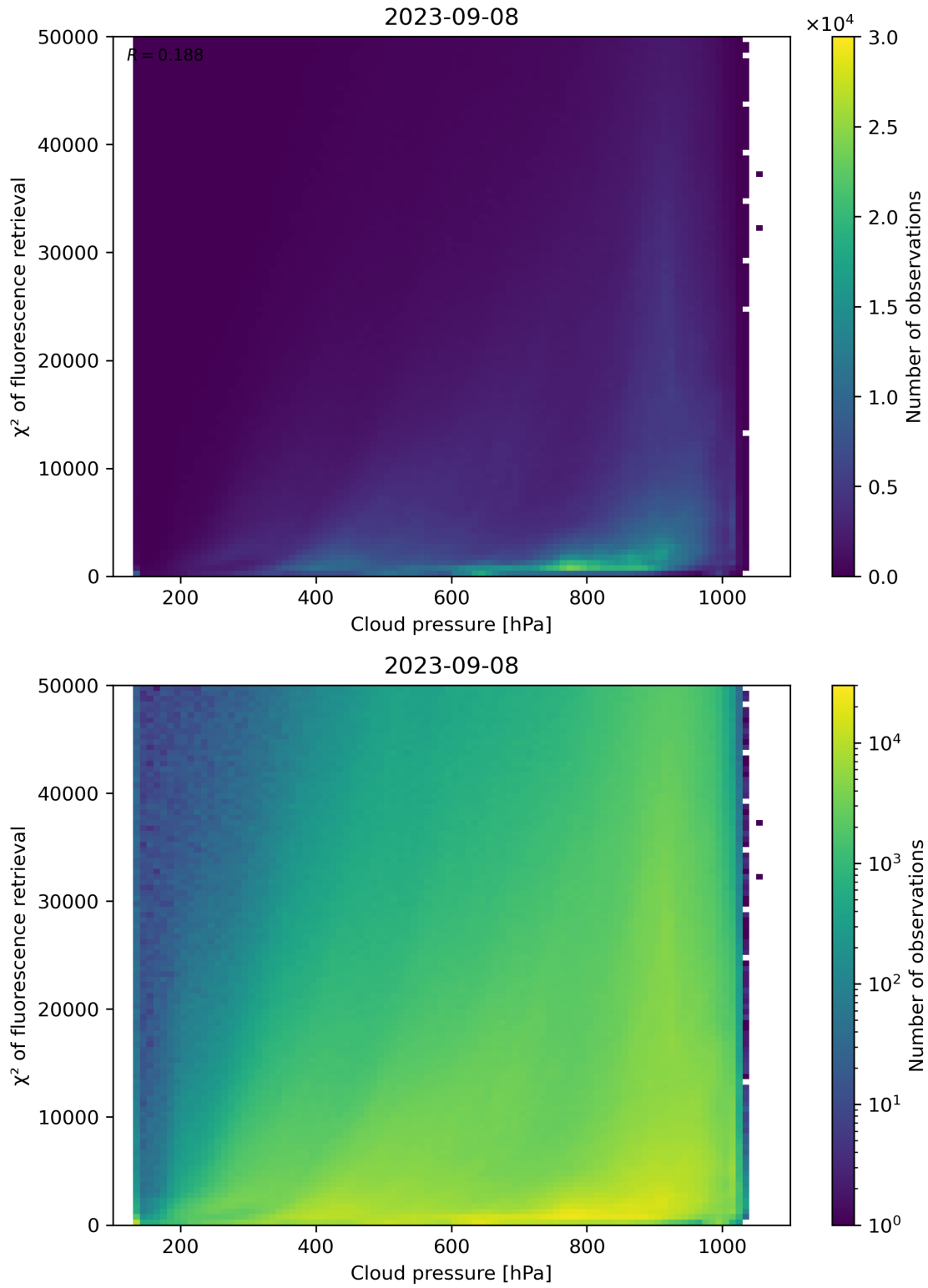
Figure 86: Scatter density plot of “Cloud pressure” against “ \chi^2 of fluorescence retrieval” for 2023-09-07 to 2023-09-09.
