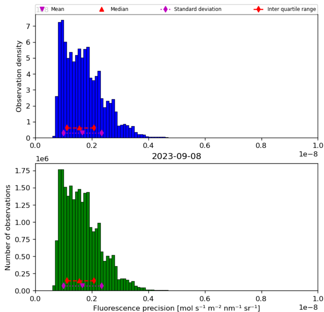
Figure 41: Histogram of “Fluorescence precision” for 2023-09-07 to 2023-09-09
