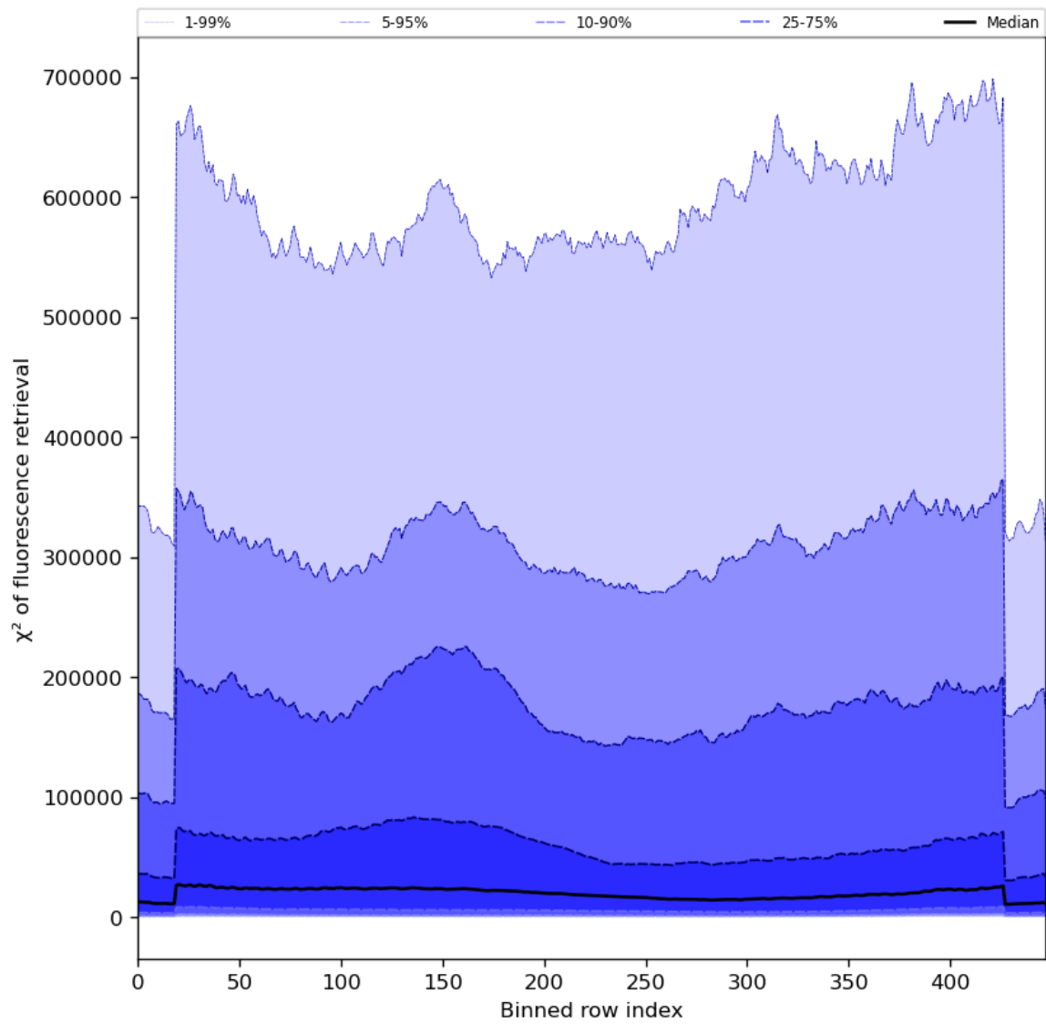
Figure 59: Along track statistics of “ \chi^2 of fluorescence retrieval” for 2023-09-07 to 2023-09-09
