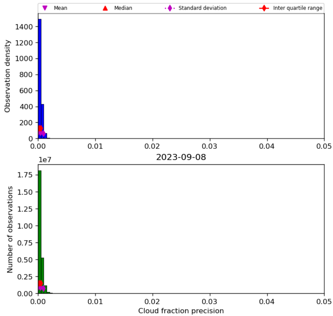
Figure 33: Histogram of “Cloud fraction precision” for 2023-09-07 to 2023-09-09
