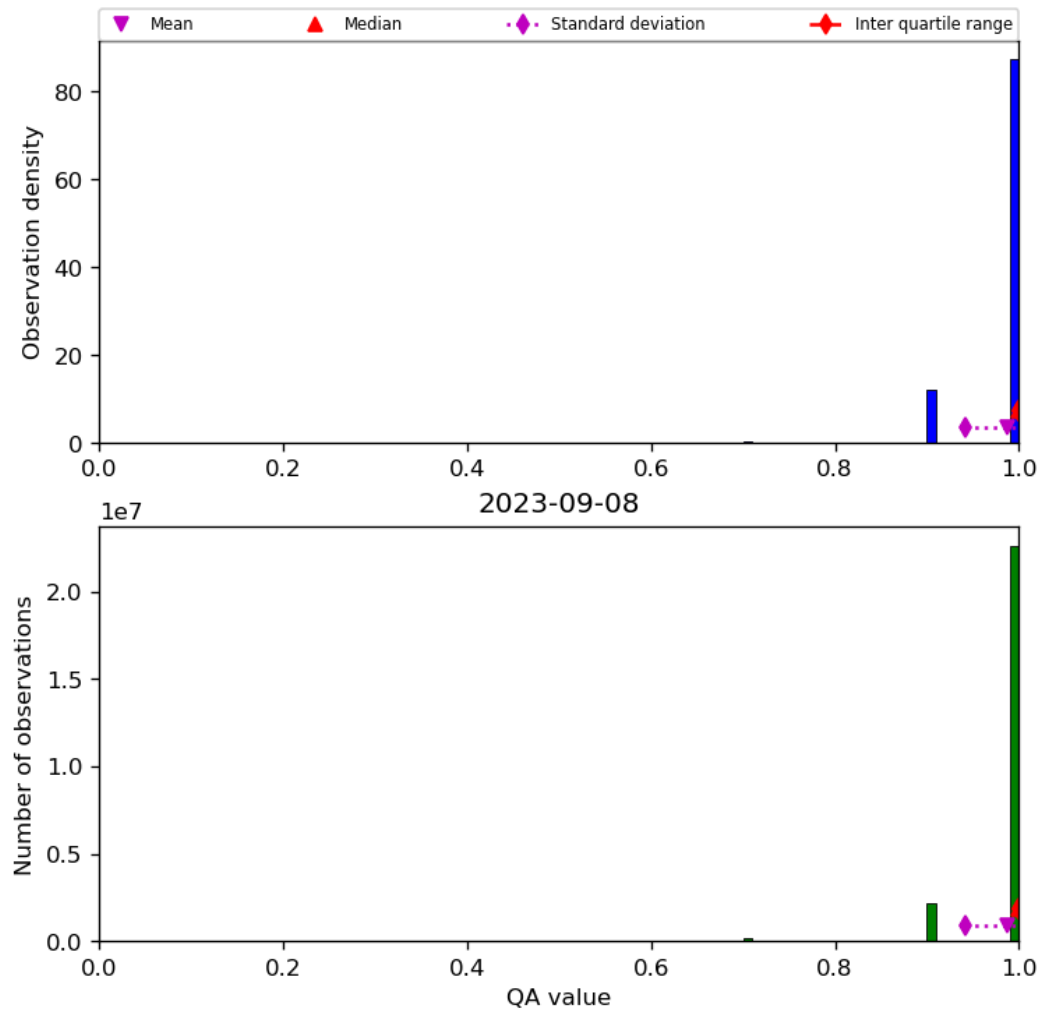
Figure 29: Histogram of “QA value” for 2023-09-07 to 2023-09-09
