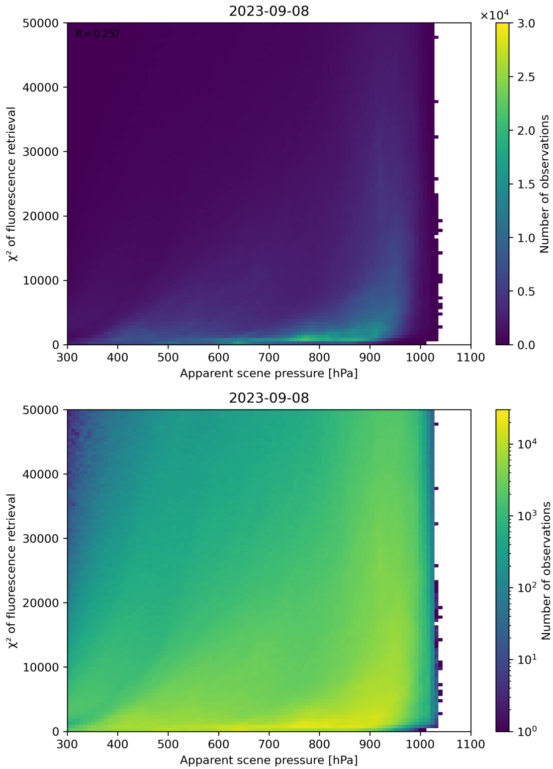
Figure 64: Scatter density plot of “Apparent scene pressure” against “ \chi^2 of fluorescence retrieval” for 2023-09-07 to 2023-09-09.
