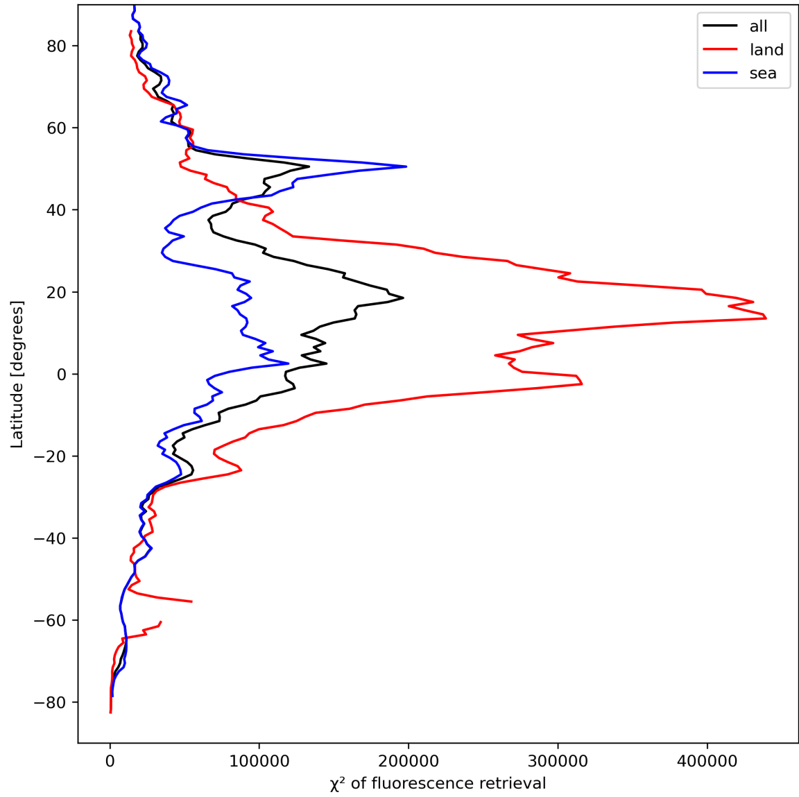
Figure 25: Zonal average of “ \chi^2 of fluorescence retrieval” for 2023-09-07 to 2023-09-09.
