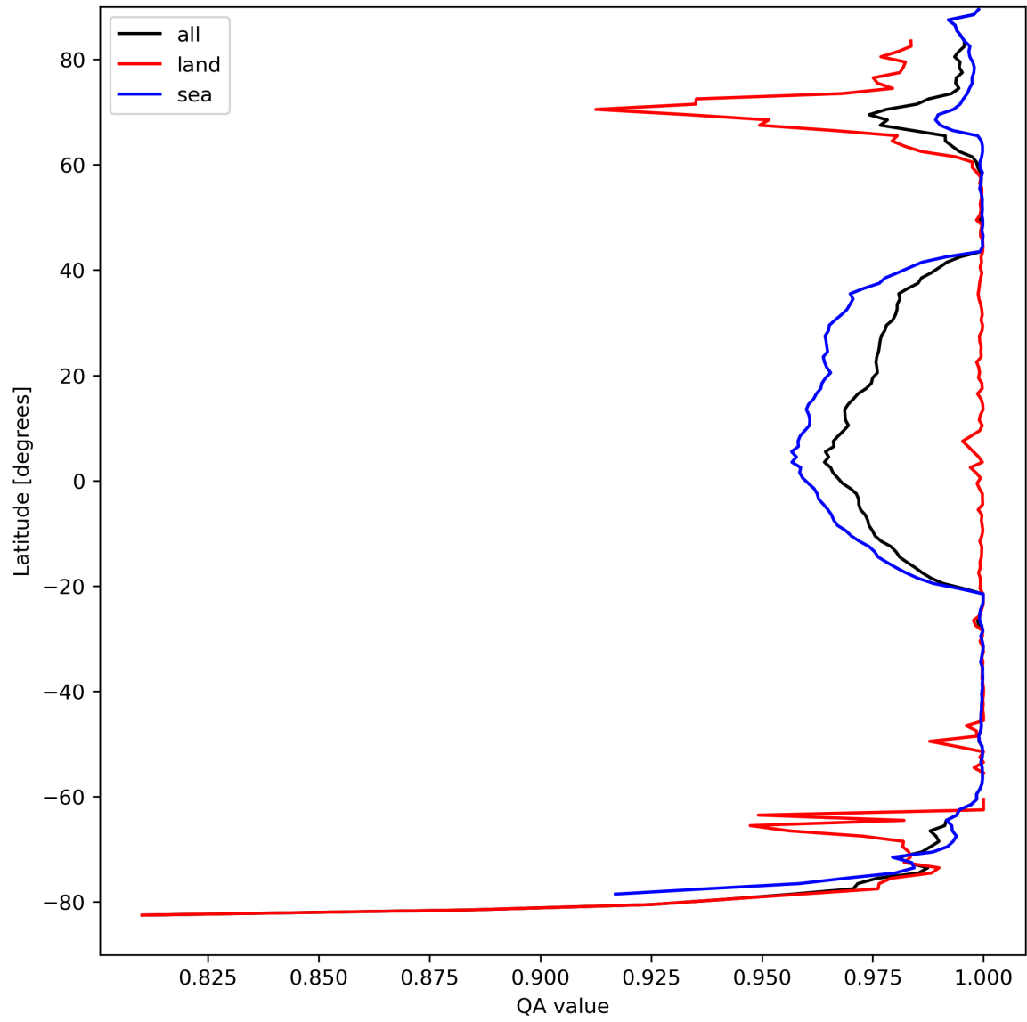
Figure 12: Zonal average of “QA value” for 2023-09-07 to 2023-09-09.
