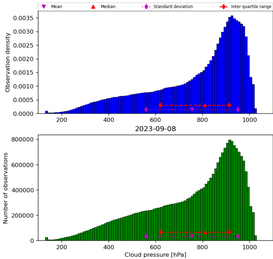
Figure 30: Histogram of “Cloud pressure” for 2023-09-07 to 2023-09-09
