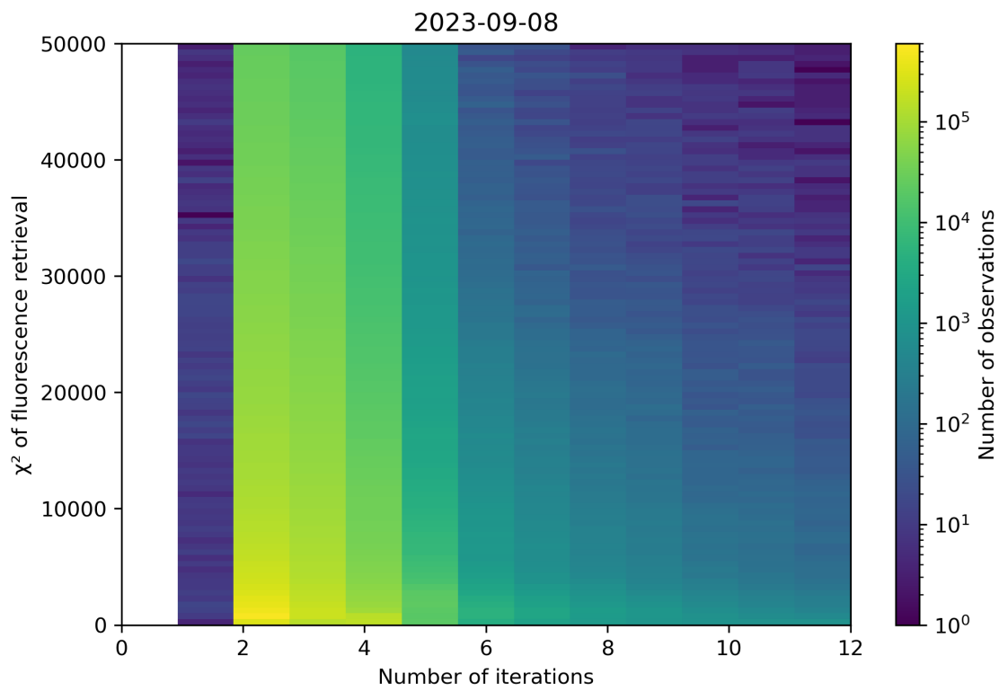
Figure 106: Scatter density plot of “Number of iterations” against “ \chi^2 of fluorescence retrieval” for 2023-09-07 to 2023-09-09.
