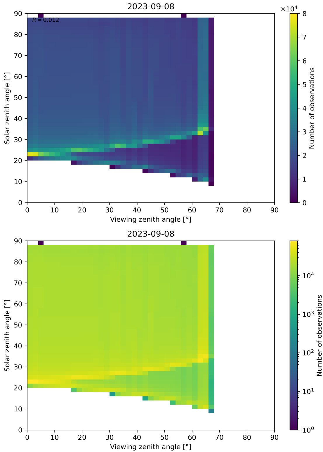
Figure 139: Scatter density plot of “Viewing zenith angle” against “Solar zenith angle” for 2023-09-07 to 2023-09-09.
