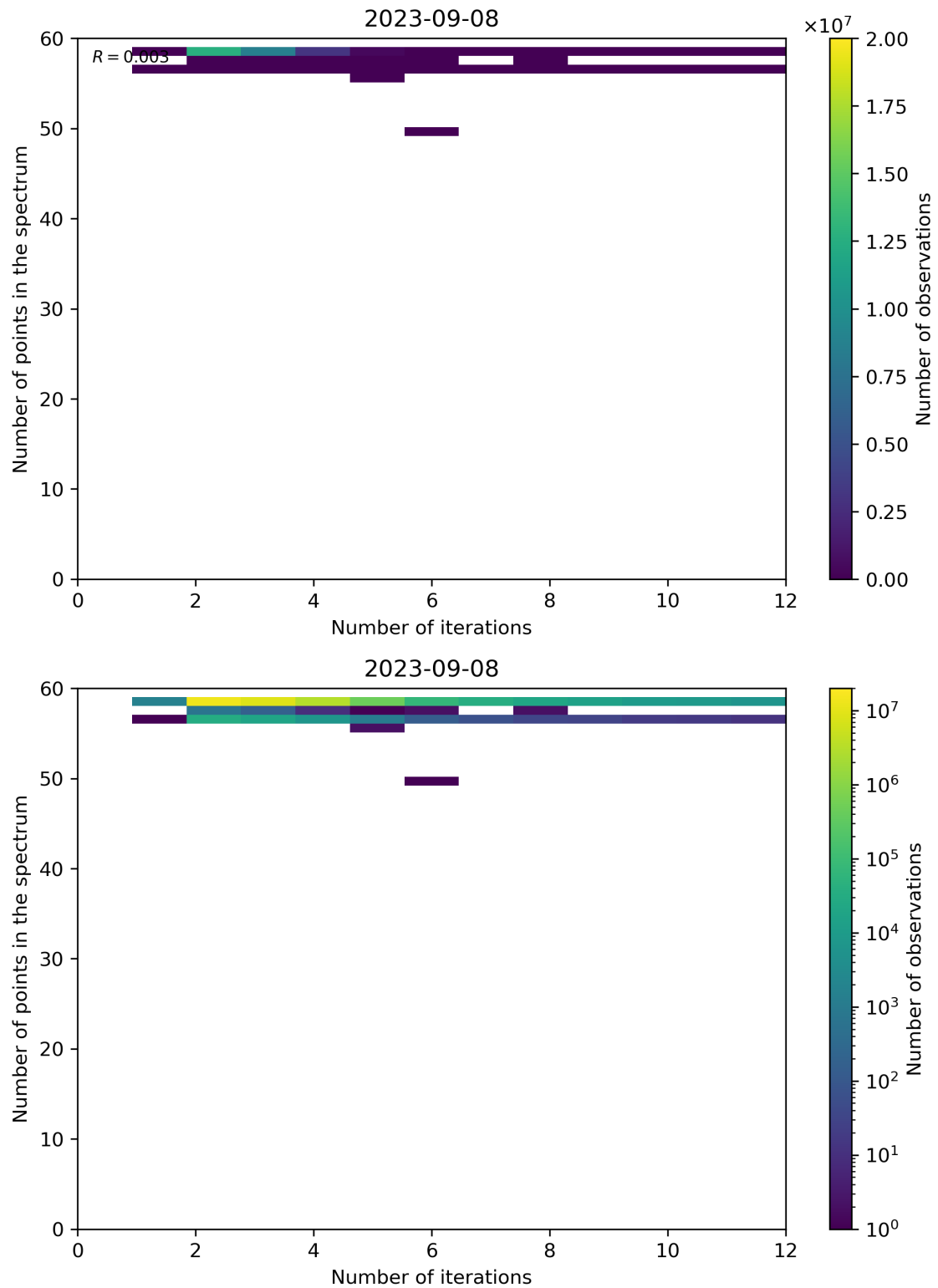
Figure 108: Scatter density plot of “Number of iterations” against “Number of points in the spectrum” for 2023-09-07 to 2023-09-09.
