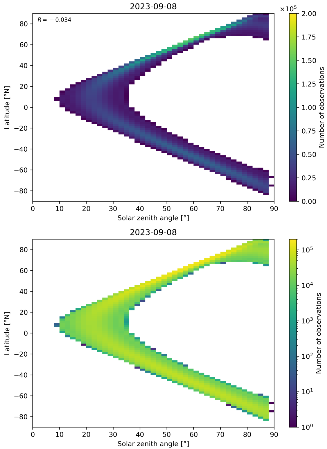
Figure 124: Scatter density plot of “Solar zenith angle” against “Latitude” for 2023-09-07 to 2023-09-09.
