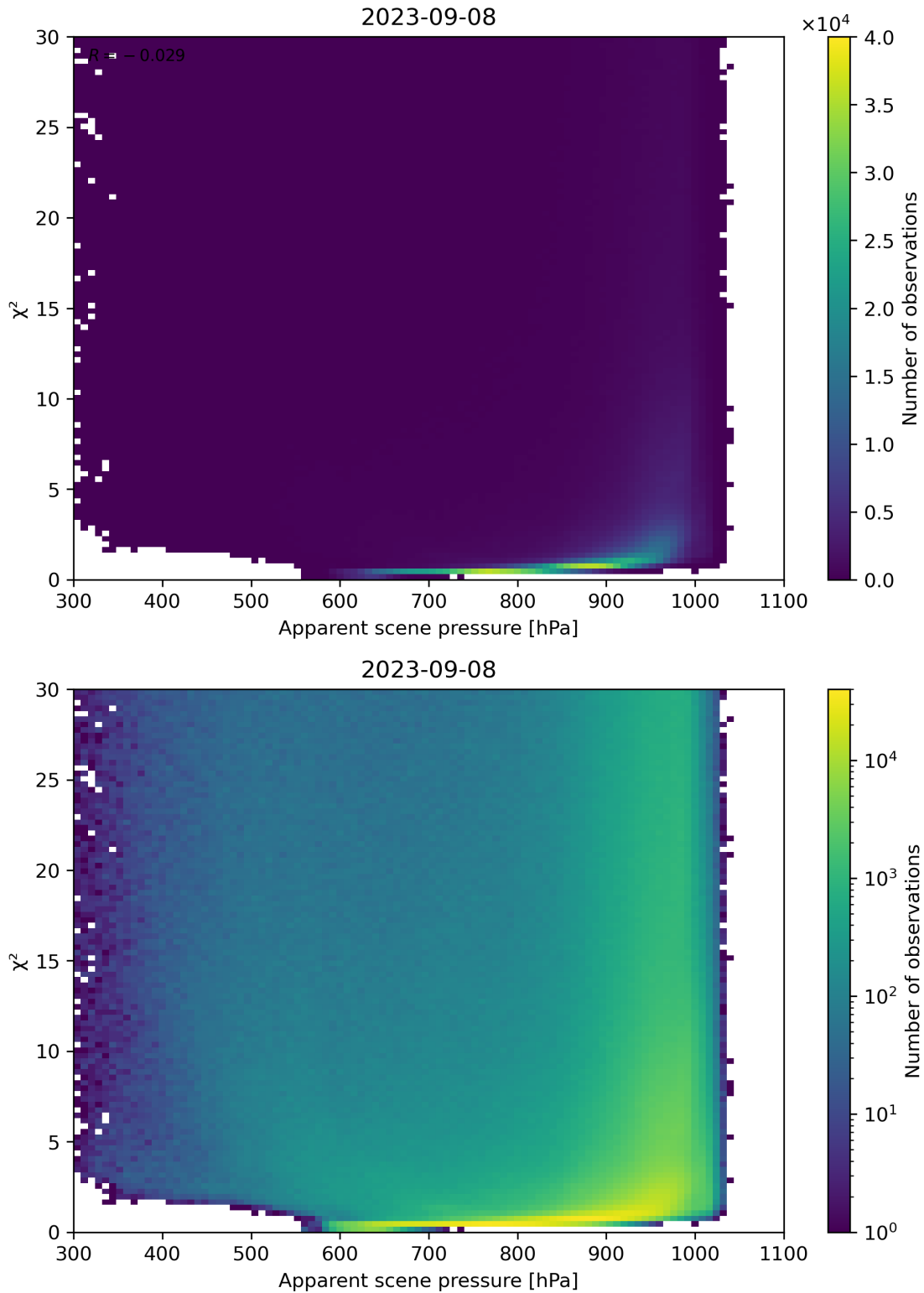
Figure 63: Scatter density plot of “Apparent scene pressure” against “ \chi^2 ” for 2023-09-07 to 2023-09-09.
