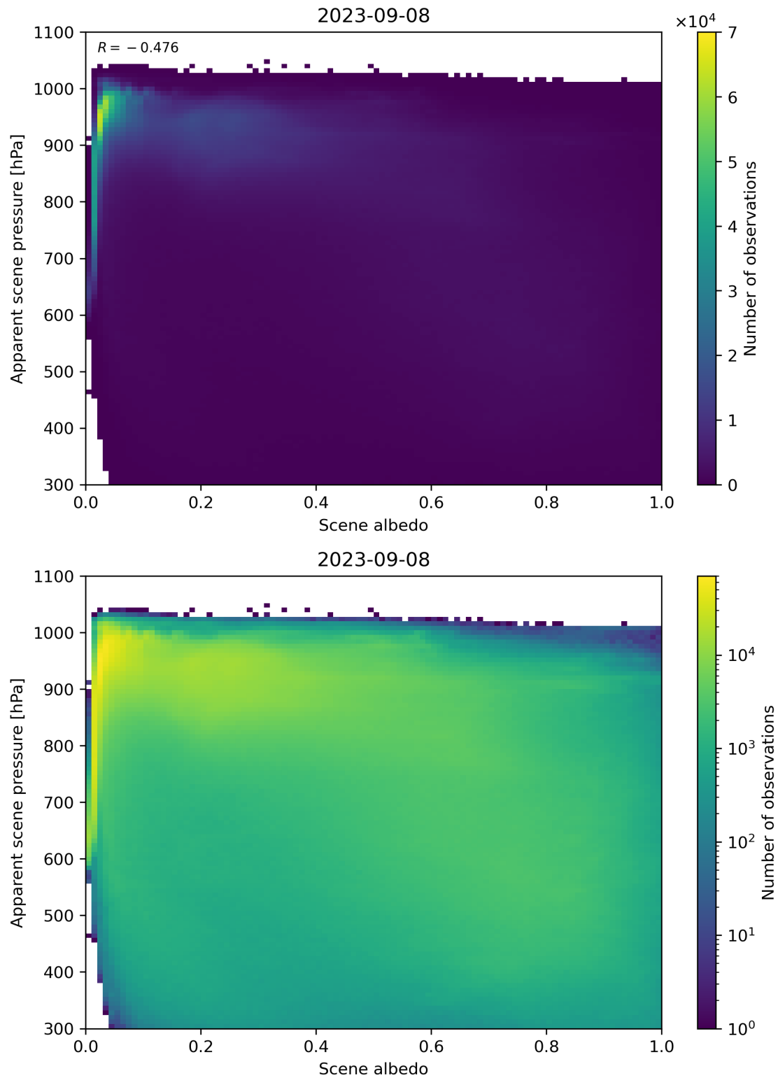
Figure 111: Scatter density plot of “Scene albedo” against “Apparent scene pressure” for 2023-09-07 to 2023-09-09.
