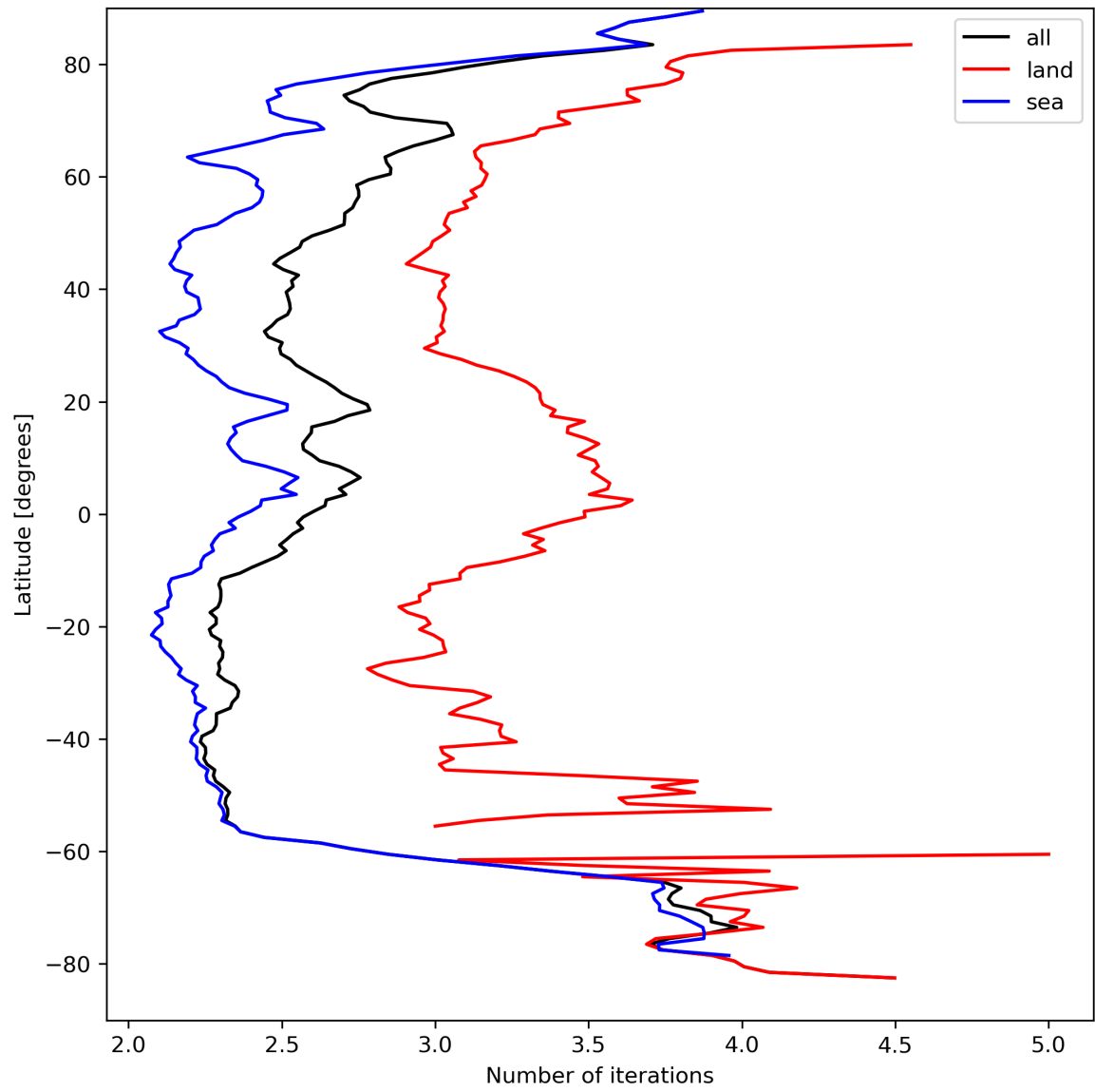
Figure 22: Zonal average of “Number of iterations” for 2023-09-07 to 2023-09-09.
