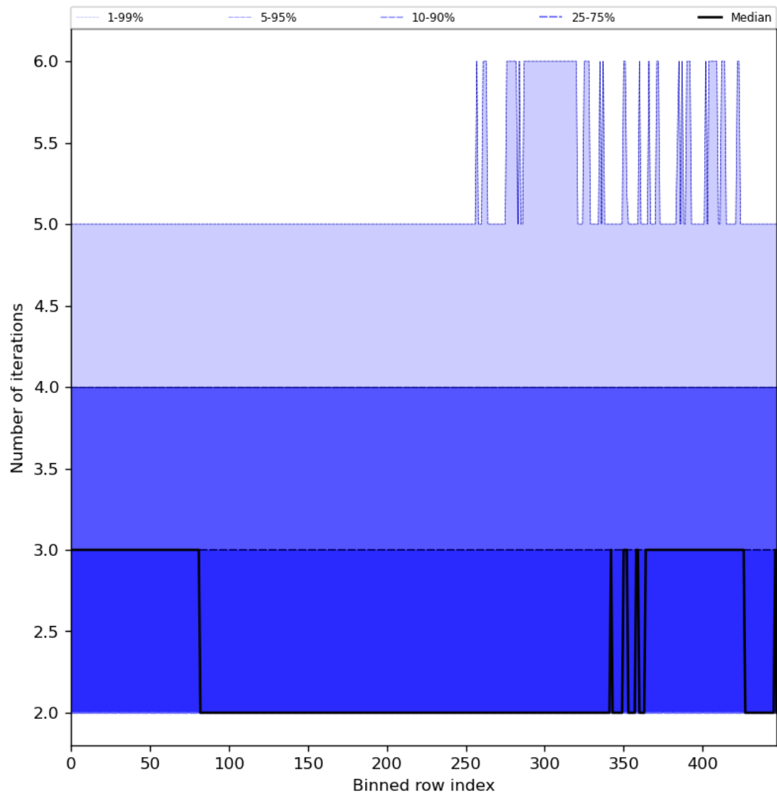
Figure 56: Along track statistics of "Number of iterations" for 2023-09-07 to 2023-09-09
