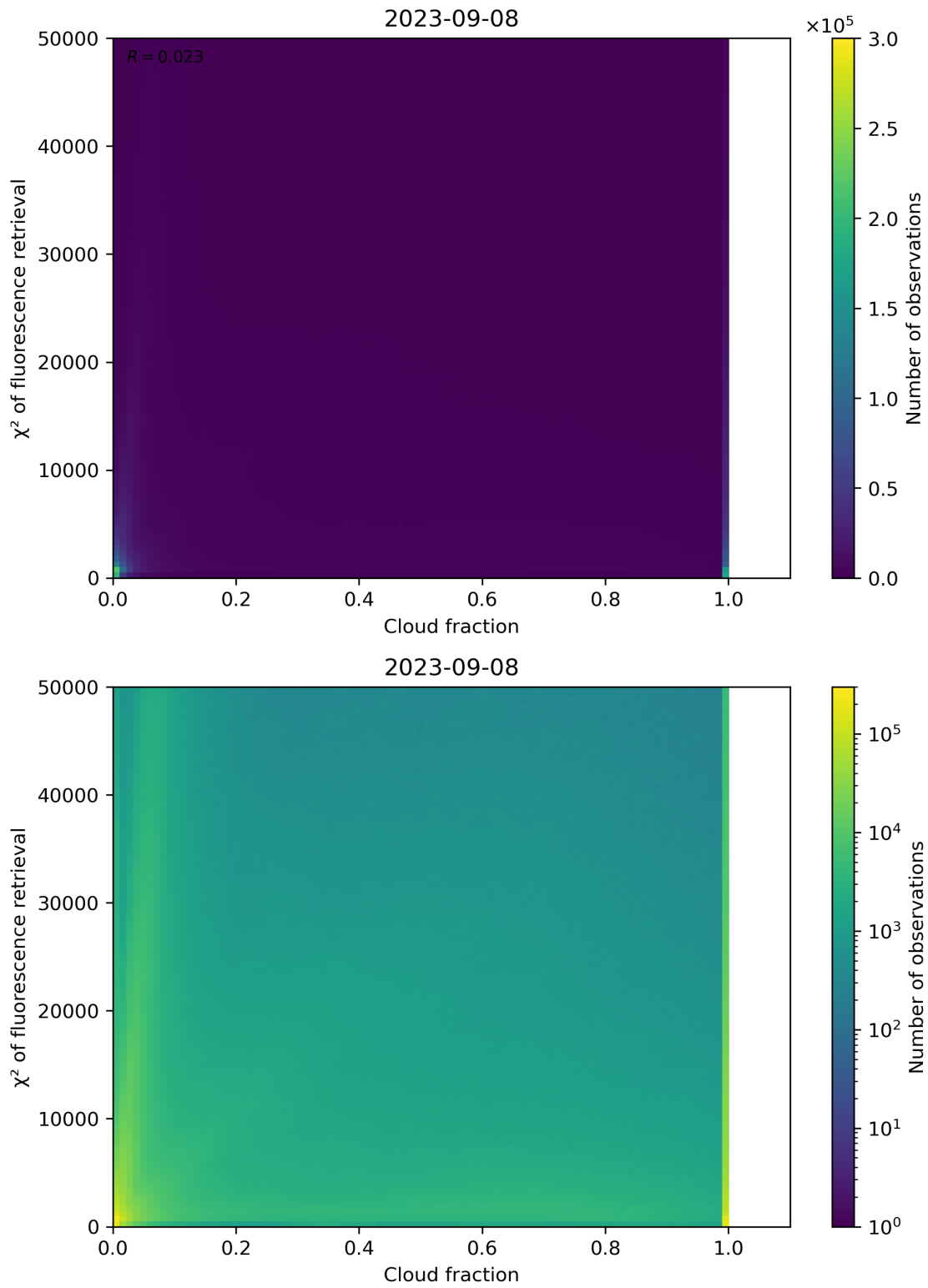
Figure 78: Scatter density plot of “Cloud fraction” against “ \chi^2 of fluorescence retrieval” for 2023-09-07 to 2023-09-09.
