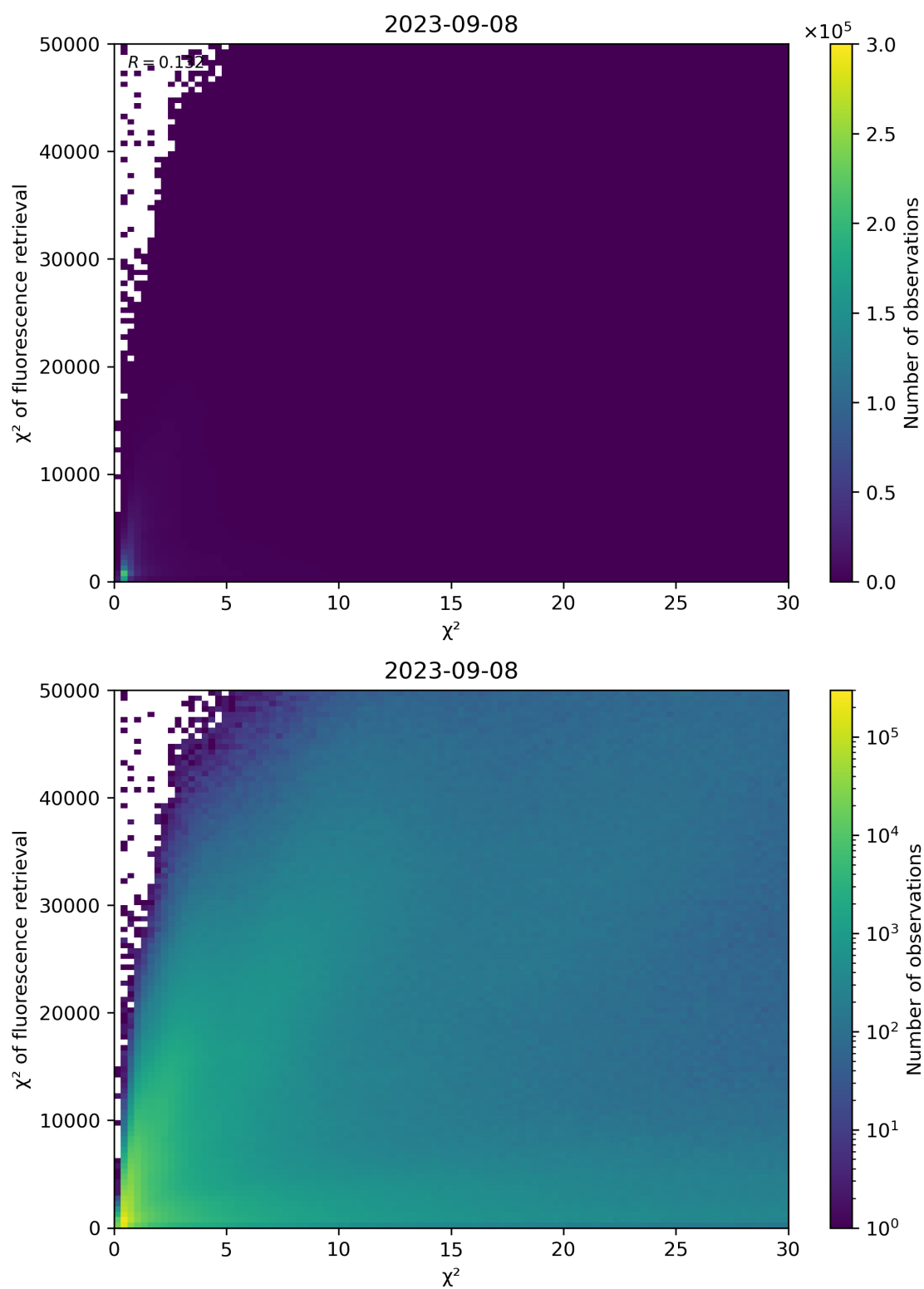
Figure 69: Scatter density plot of “ \chi^2 ” against “ \chi^2 of fluorescence retrieval” for 2023-09-07 to 2023-09-09.
