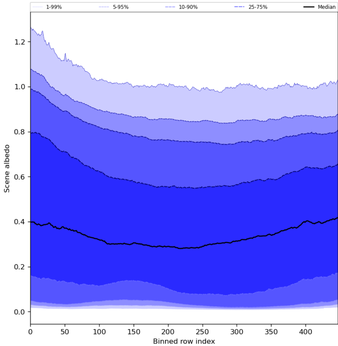
Figure 51: Along track statistics of “Scene albedo” for 2023-09-07 to 2023-09-09
