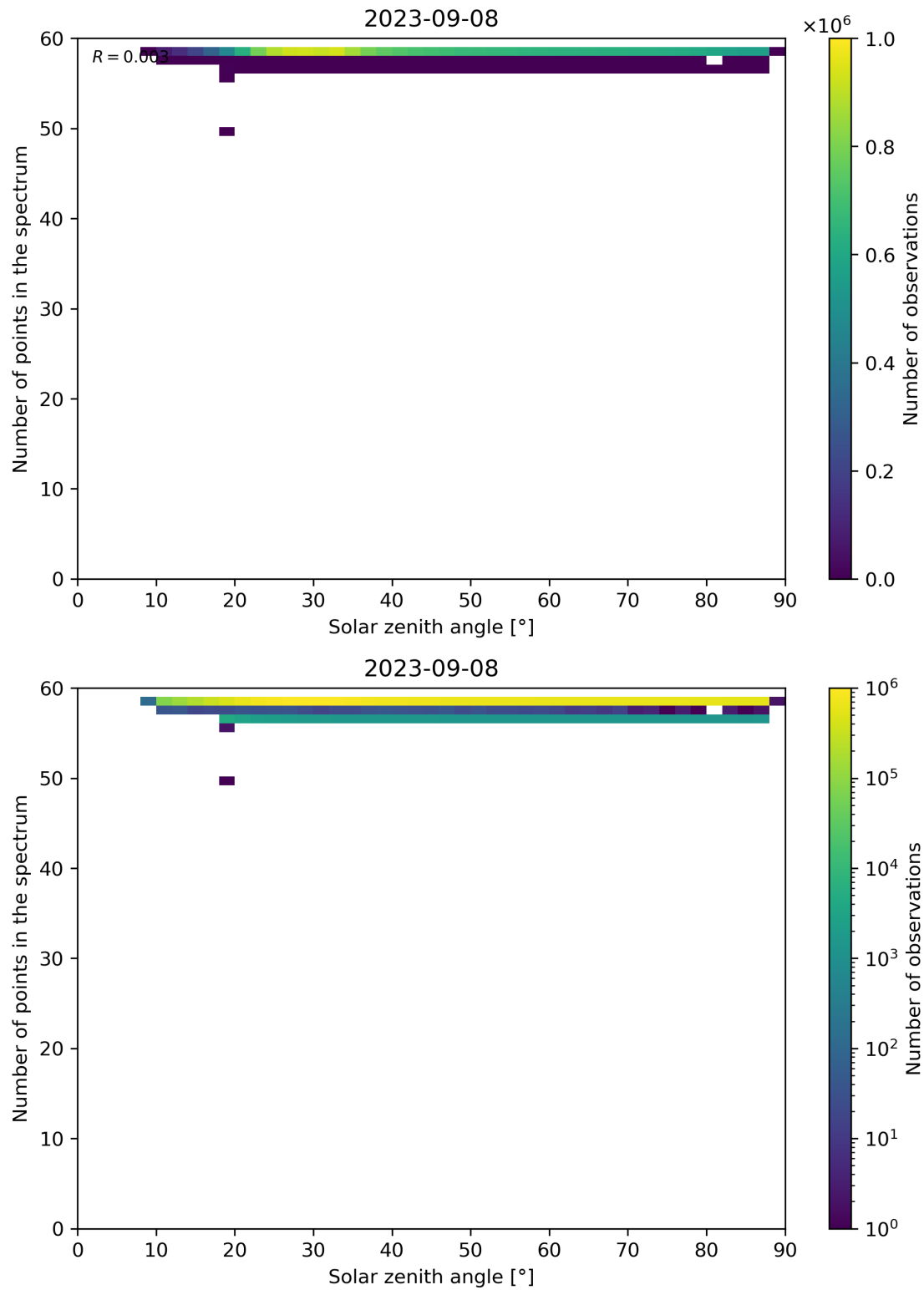
Figure 126: Scatter density plot of “Solar zenith angle” against “Number of points in the spectrum” for 2023-09-07 to 2023-09-09.
