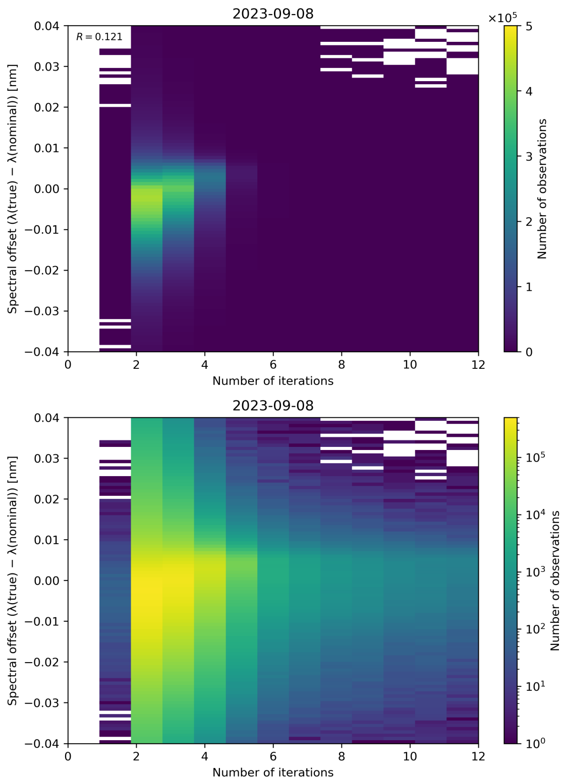
Figure 109: Scatter density plot of “Number of iterations” against “Spectral offset ( \lambda(\text{true}) - \lambda(\text{nominal}) )” for 2023-09-07 to 2023-09-09.
