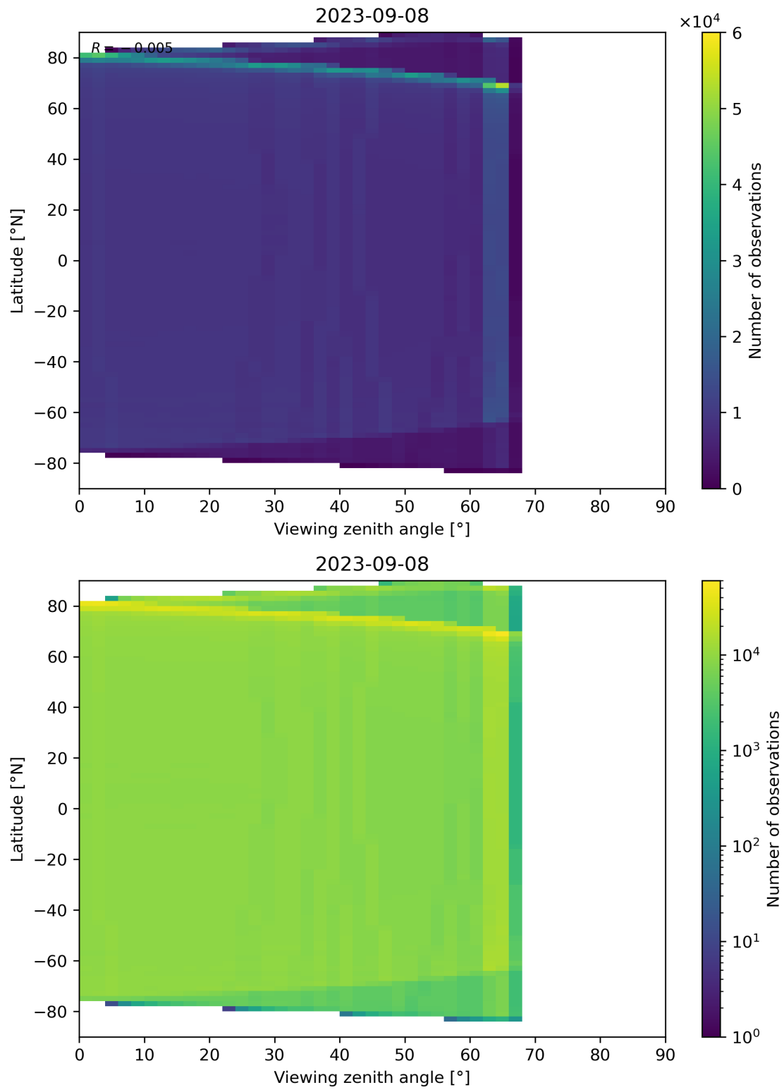
Figure 135: Scatter density plot of “Viewing zenith angle” against “Latitude” for 2023-09-07 to 2023-09-09.
