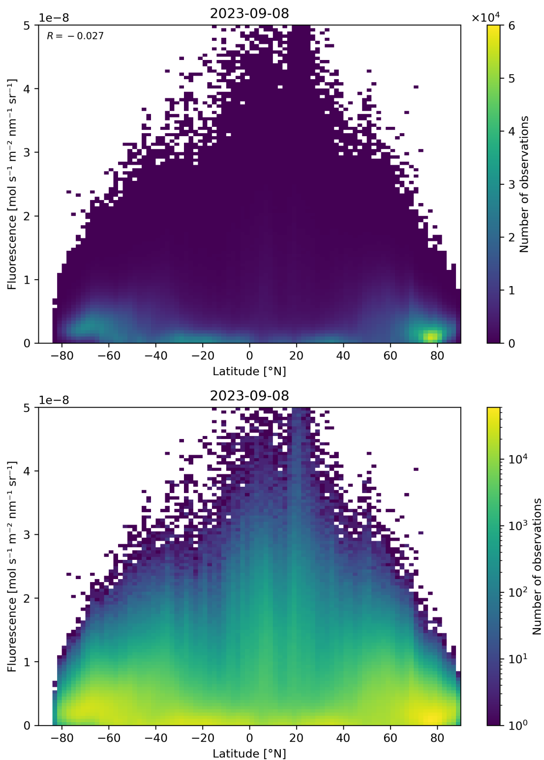
Figure 101: Scatter density plot of “Latitude” against “Fluorescence” for 2023-09-07 to 2023-09-09.
