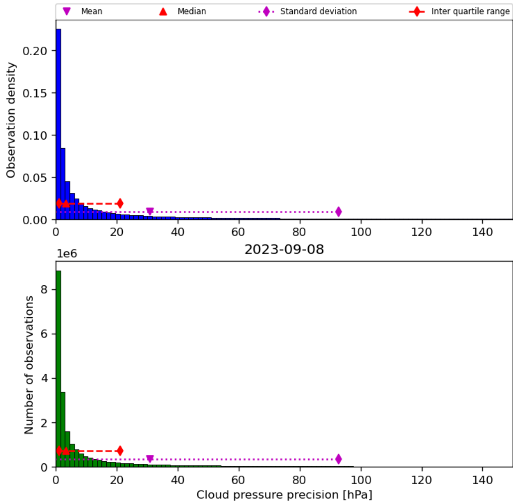
Figure 31: Histogram of “Cloud pressure precision” for 2023-09-07 to 2023-09-09
