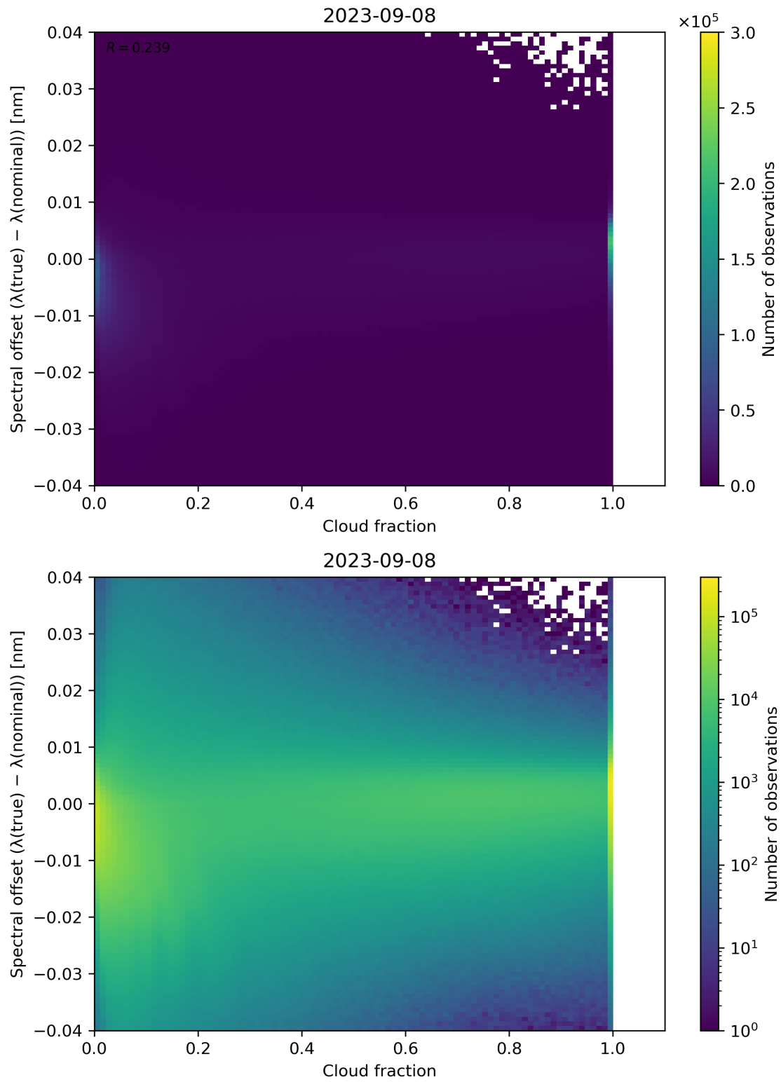
Figure 83: Scatter density plot of “Cloud fraction” against “Spectral offset ( \lambda(\text{true}) - \lambda(\text{nominal}) )” for 2023-09-07 to 2023-09-09.
