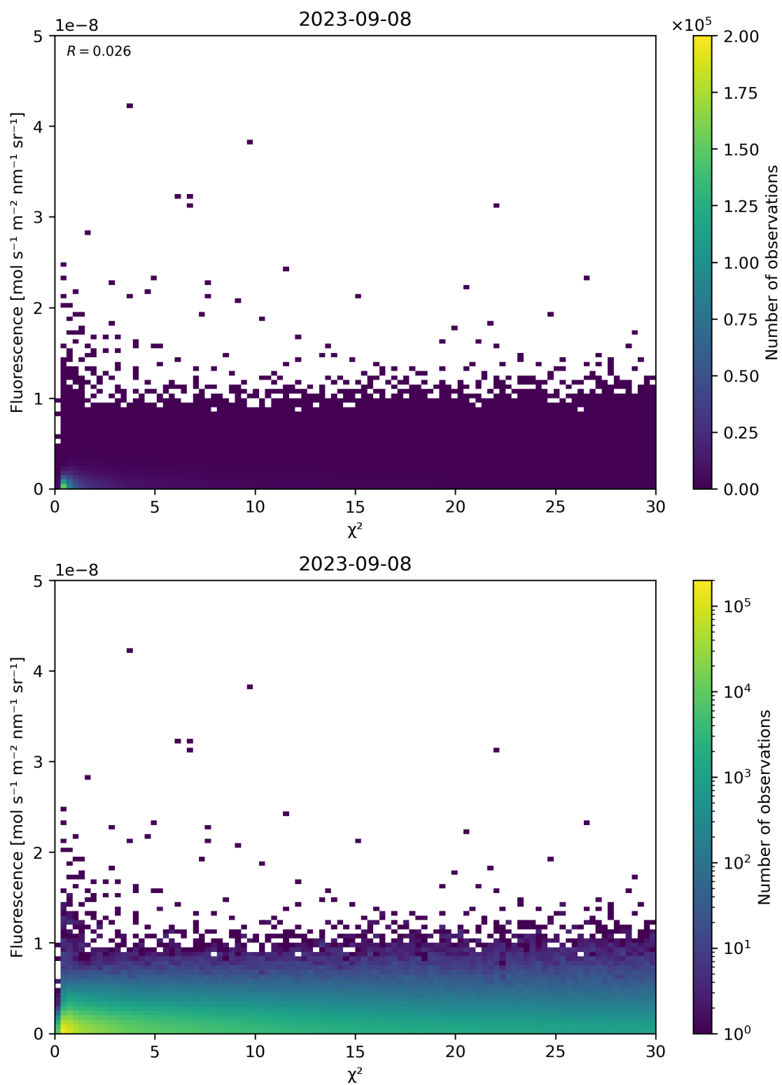
Figure 70: Scatter density plot of “ \chi^2 ” against “Fluorescence” for 2023-09-07 to 2023-09-09.
