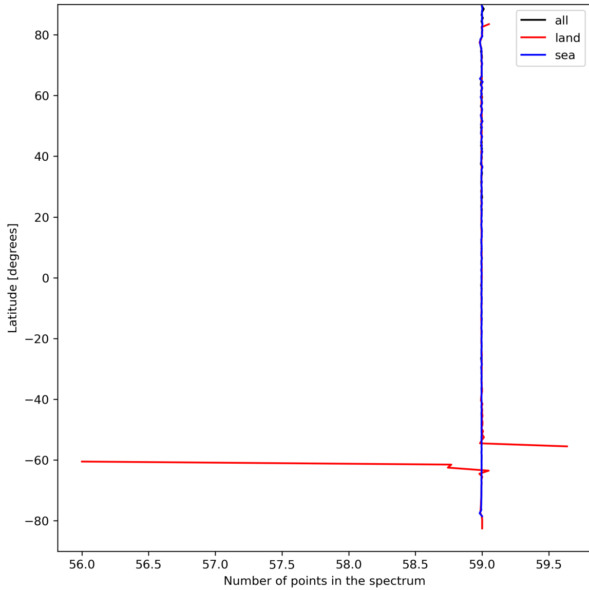
Figure 27: Zonal average of “Number of points in the spectrum” for 2023-09-07 to 2023-09-09.
