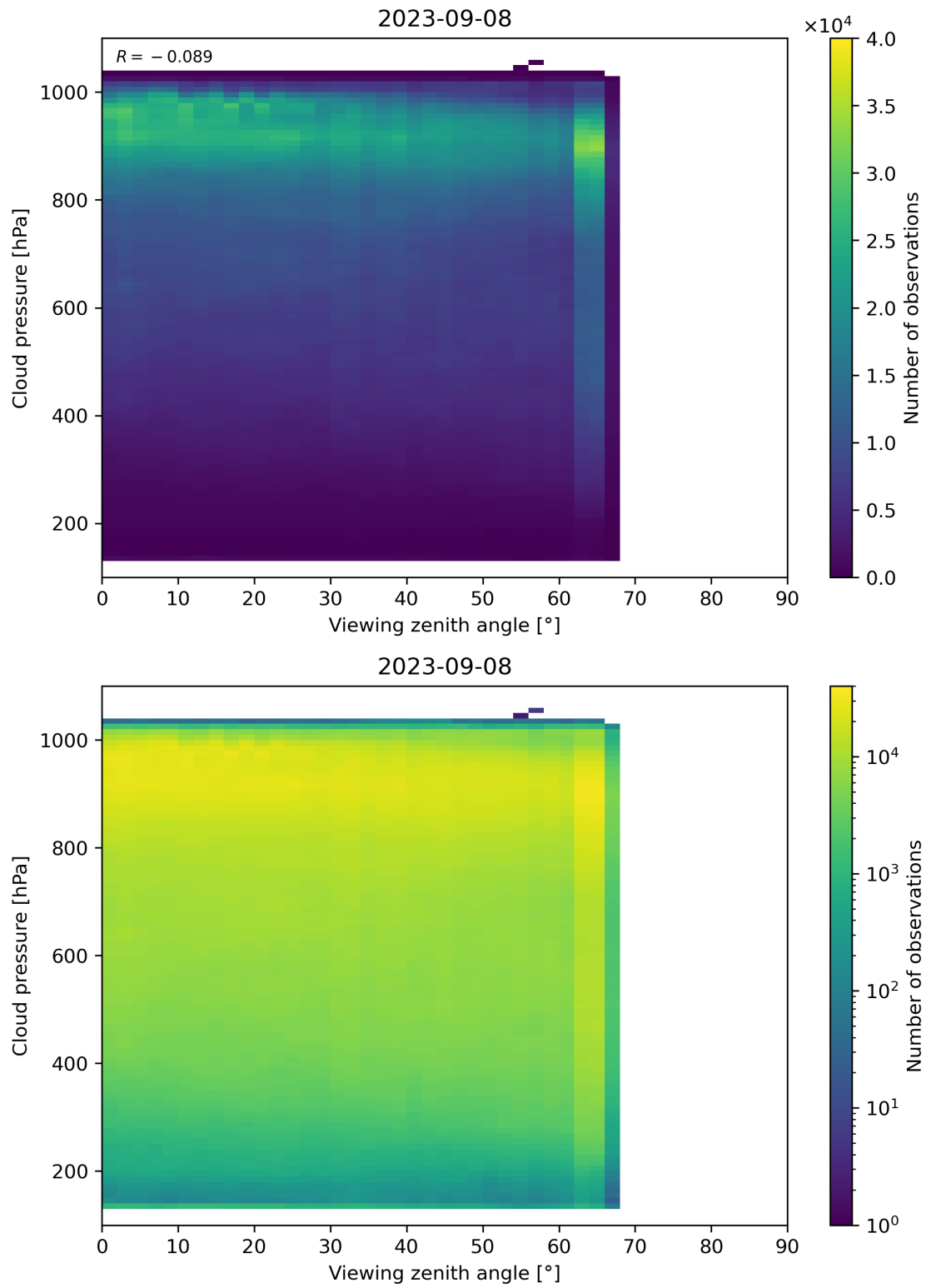
Figure 133: Scatter density plot of “Viewing zenith angle” against “Cloud pressure” for 2023-09-07 to 2023-09-09.
