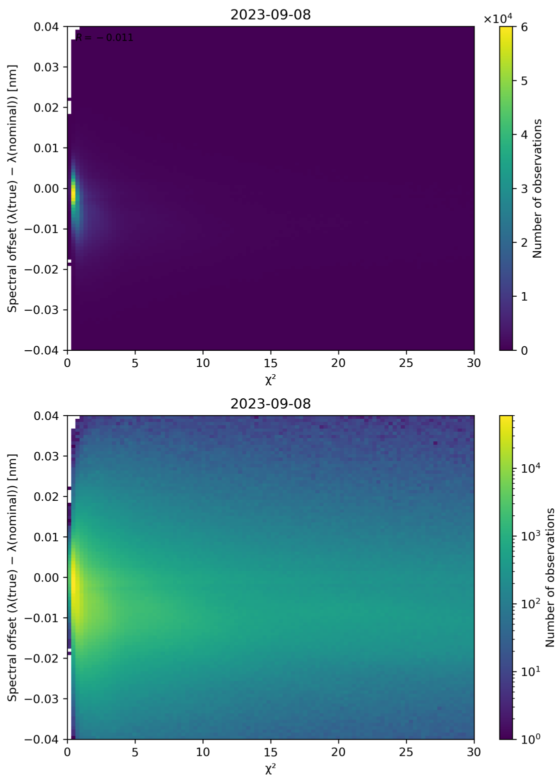
Figure 75: Scatter density plot of “ \chi^2 ” against “Spectral offset ( \lambda(\text{true}) - \lambda(\text{nominal}) )” for 2023-09-07 to 2023-09-09.
