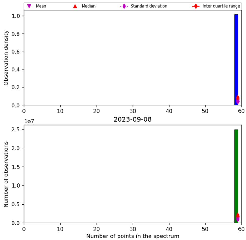
Figure 44: Histogram of “Number of points in the spectrum” for 2023-09-07 to 2023-09-09
