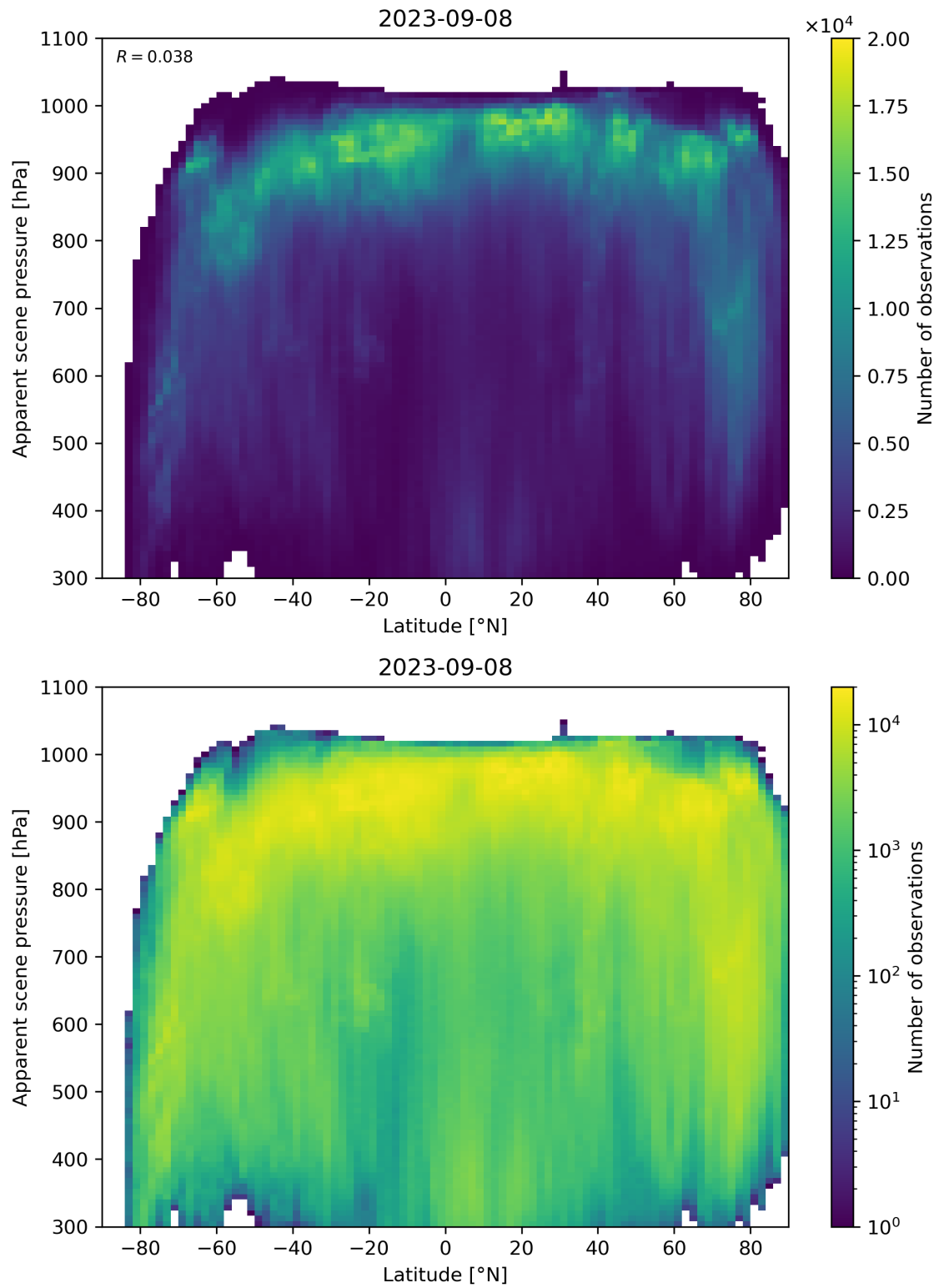
Figure 96: Scatter density plot of “Latitude” against “Apparent scene pressure” for 2023-09-07 to 2023-09-09.
