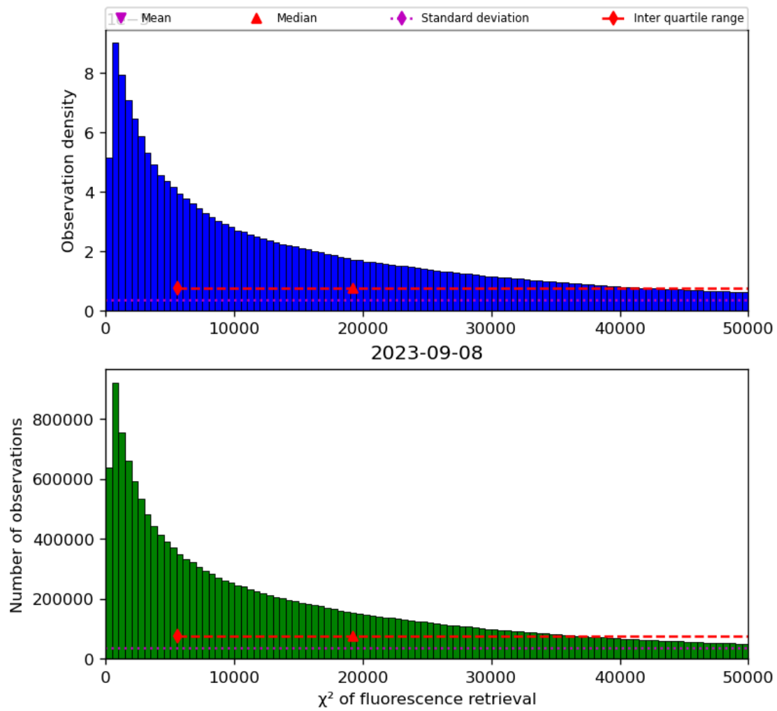
Figure 42: Histogram of “ \chi^2 of fluorescence retrieval” for 2023-09-07 to 2023-09-09
