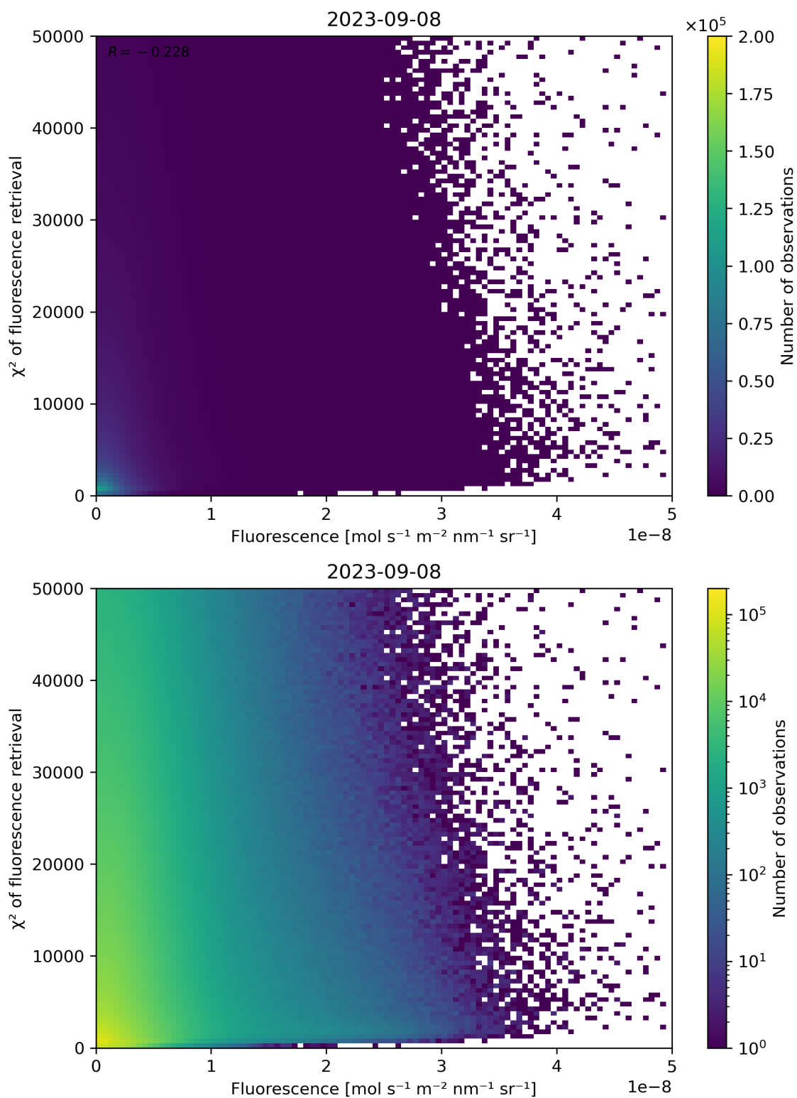
Figure 93: Scatter density plot of “Fluorescence” against “ \chi^2 of fluorescence retrieval” for 2023-09-07 to 2023-09-09.
