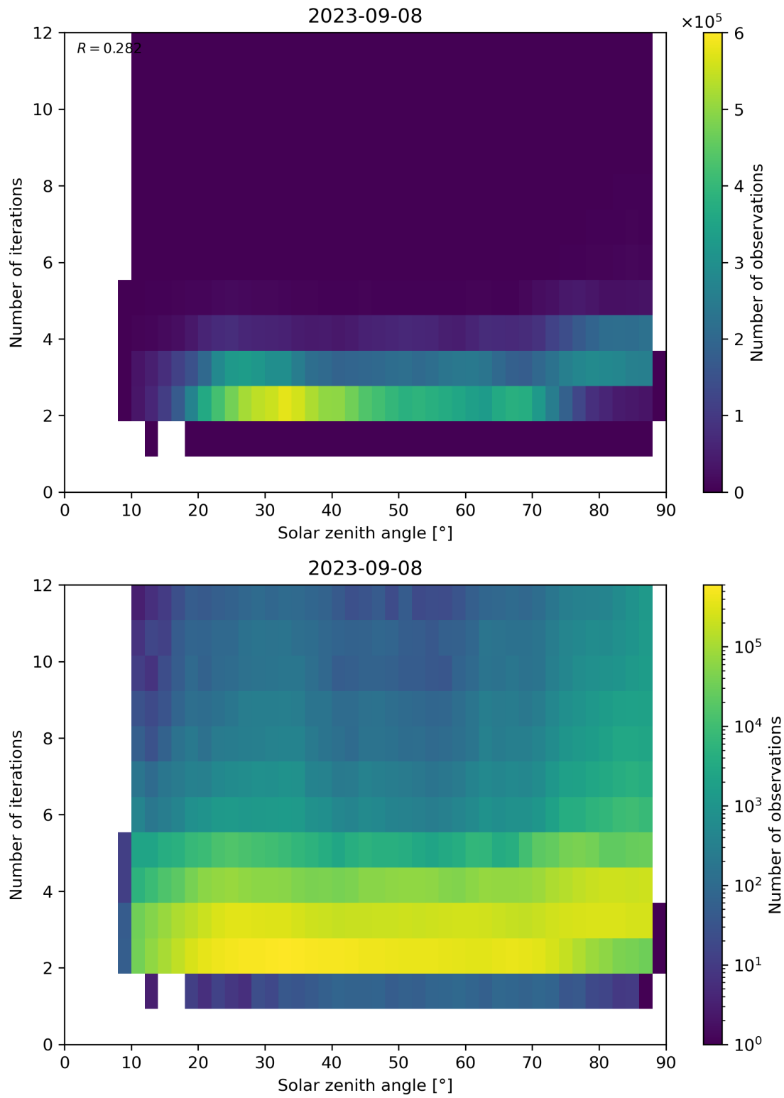
Figure 125: Scatter density plot of “Solar zenith angle” against “Number of iterations” for 2023-09-07 to 2023-09-09.
