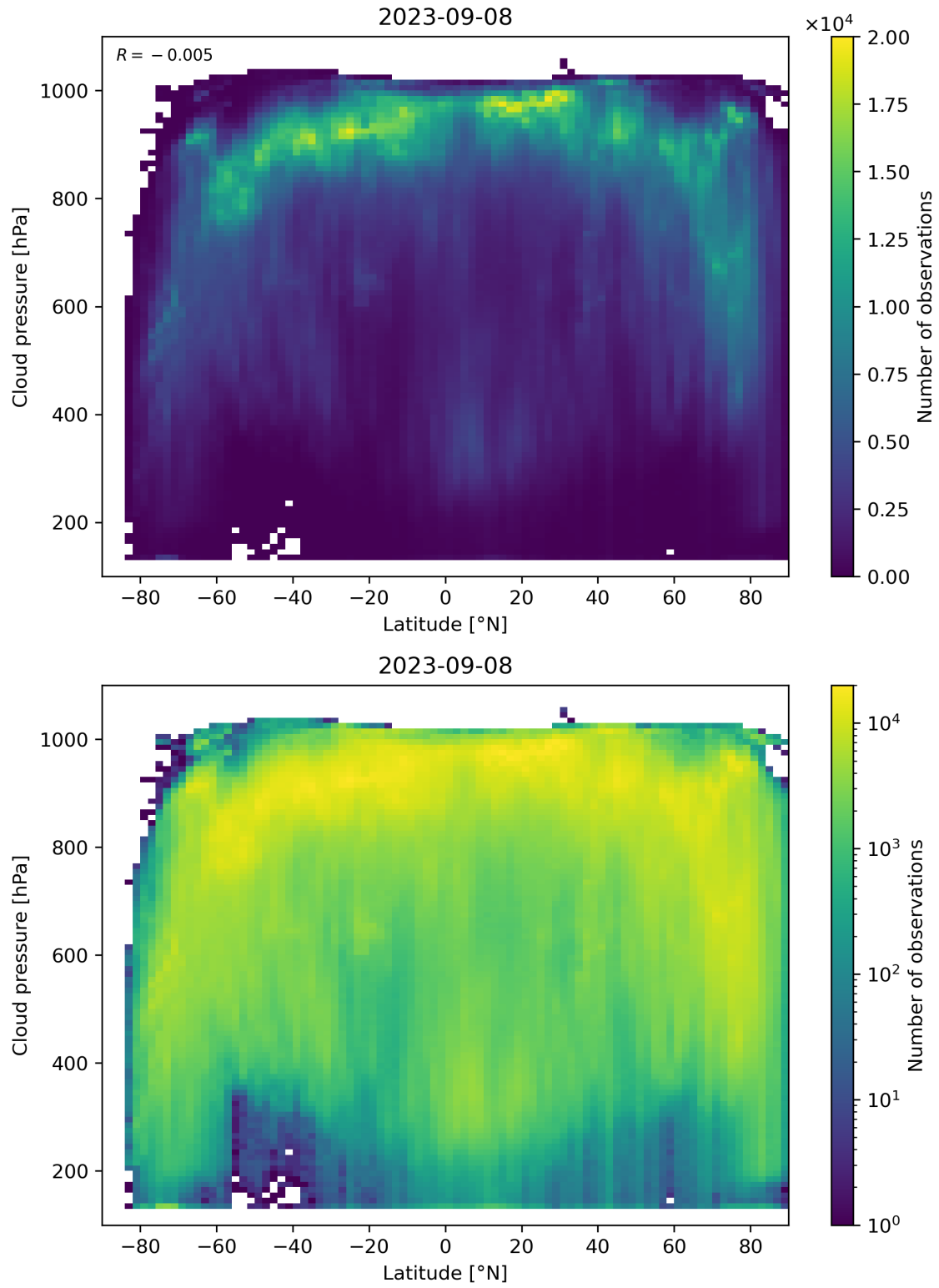
Figure 100: Scatter density plot of “Latitude” against “Cloud pressure” for 2023-09-07 to 2023-09-09.
