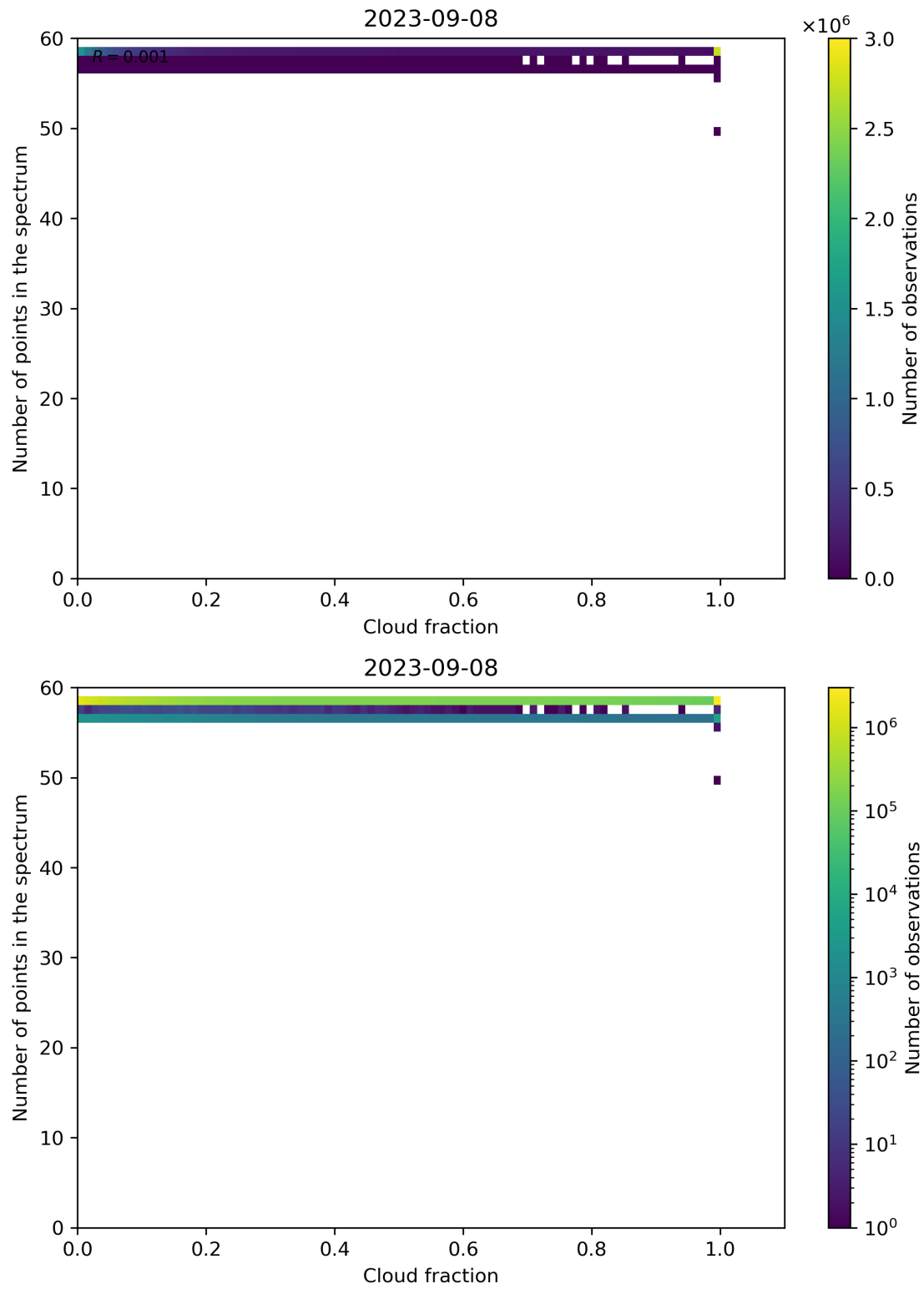
Figure 81: Scatter density plot of “Cloud fraction” against “Number of points in the spectrum” for 2023-09-07 to 2023-09-09.
