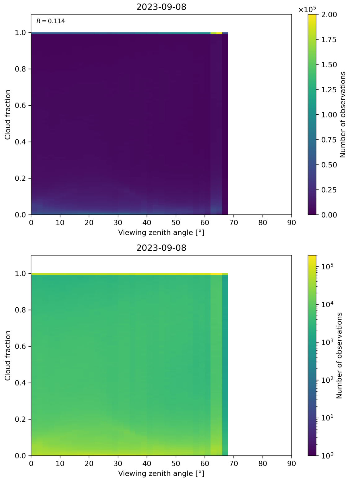
Figure 132: Scatter density plot of “Viewing zenith angle” against “Cloud fraction” for 2023-09-07 to 2023-09-09.
