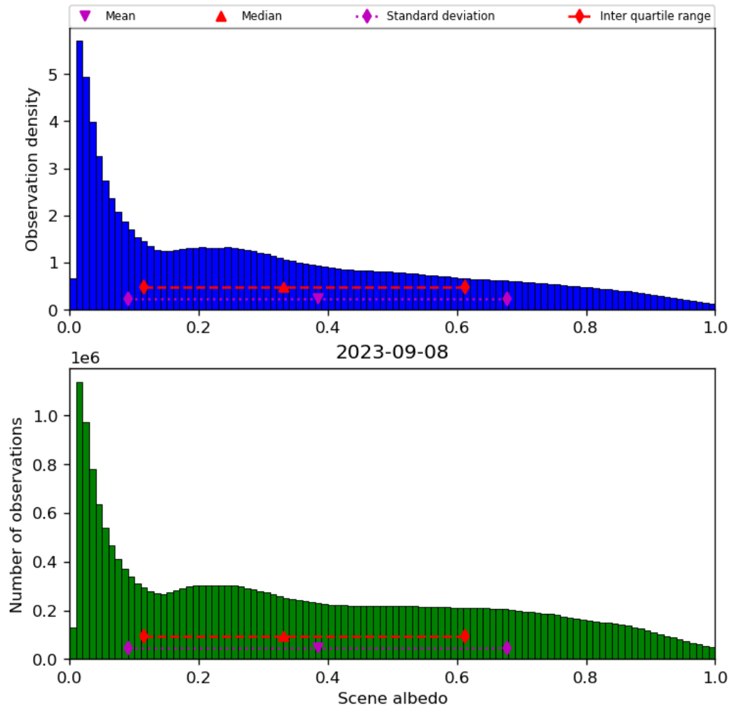
Figure 34: Histogram of “Scene albedo” for 2023-09-07 to 2023-09-09
