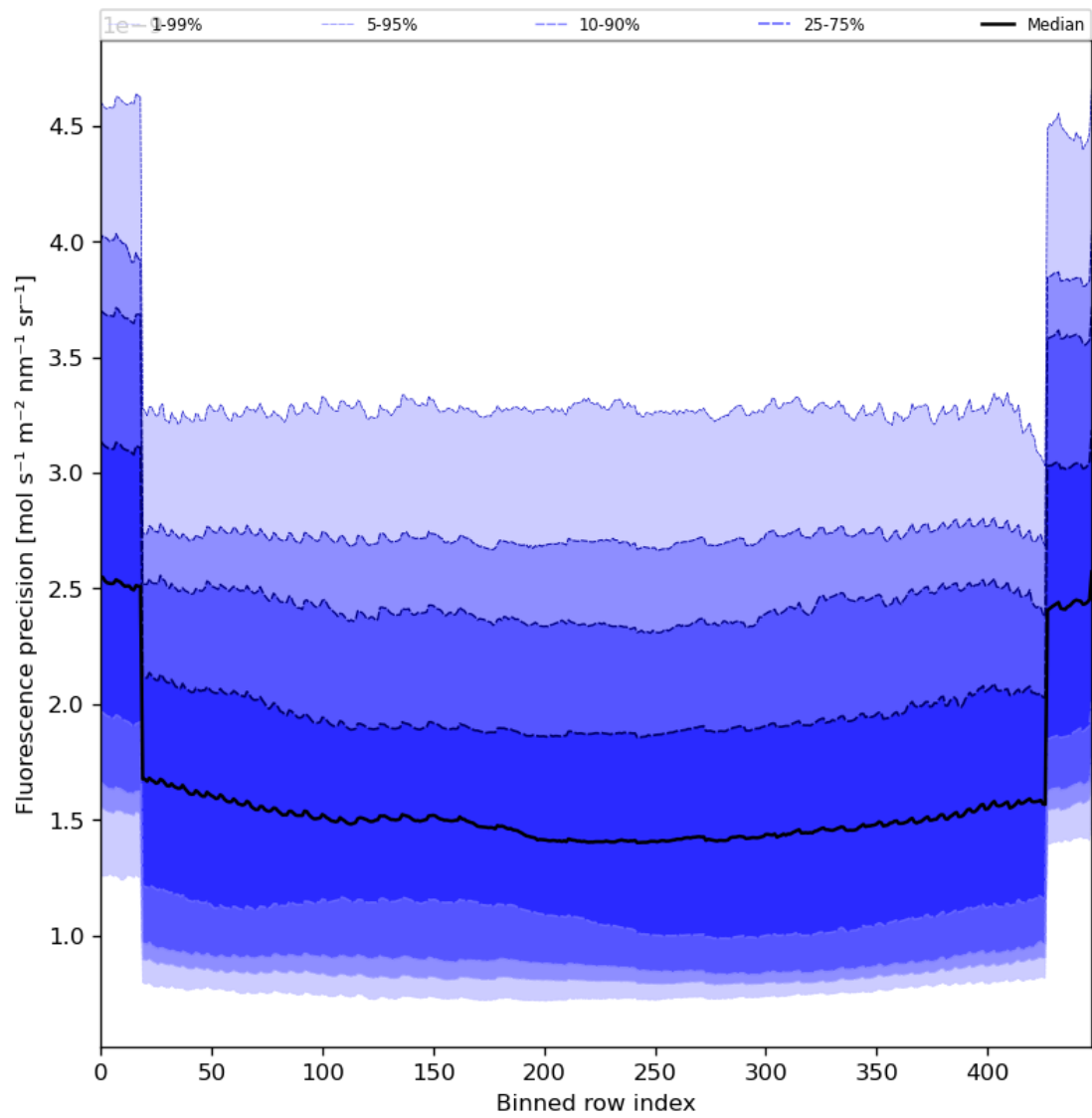
Figure 58: Along track statistics of “Fluorescence precision” for 2023-09-07 to 2023-09-09
