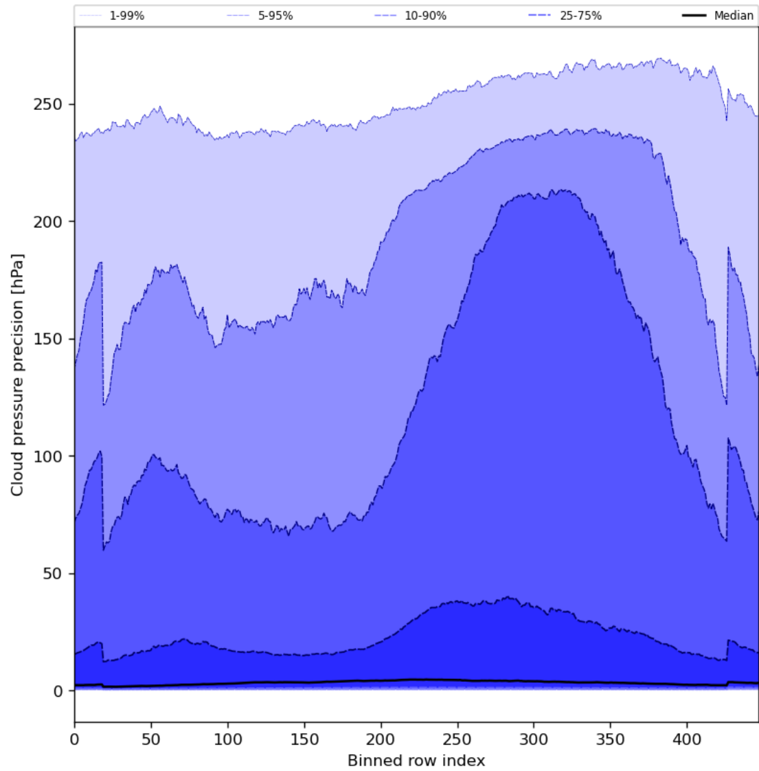
Figure 48: Along track statistics of “Cloud pressure precision” for 2023-09-07 to 2023-09-09
