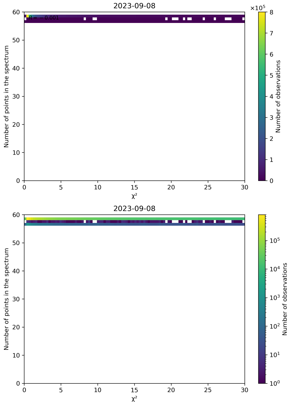
Figure 74: Scatter density plot of “ \chi^2 ” against “Number of points in the spectrum” for 2023-09-07 to 2023-09-09.
