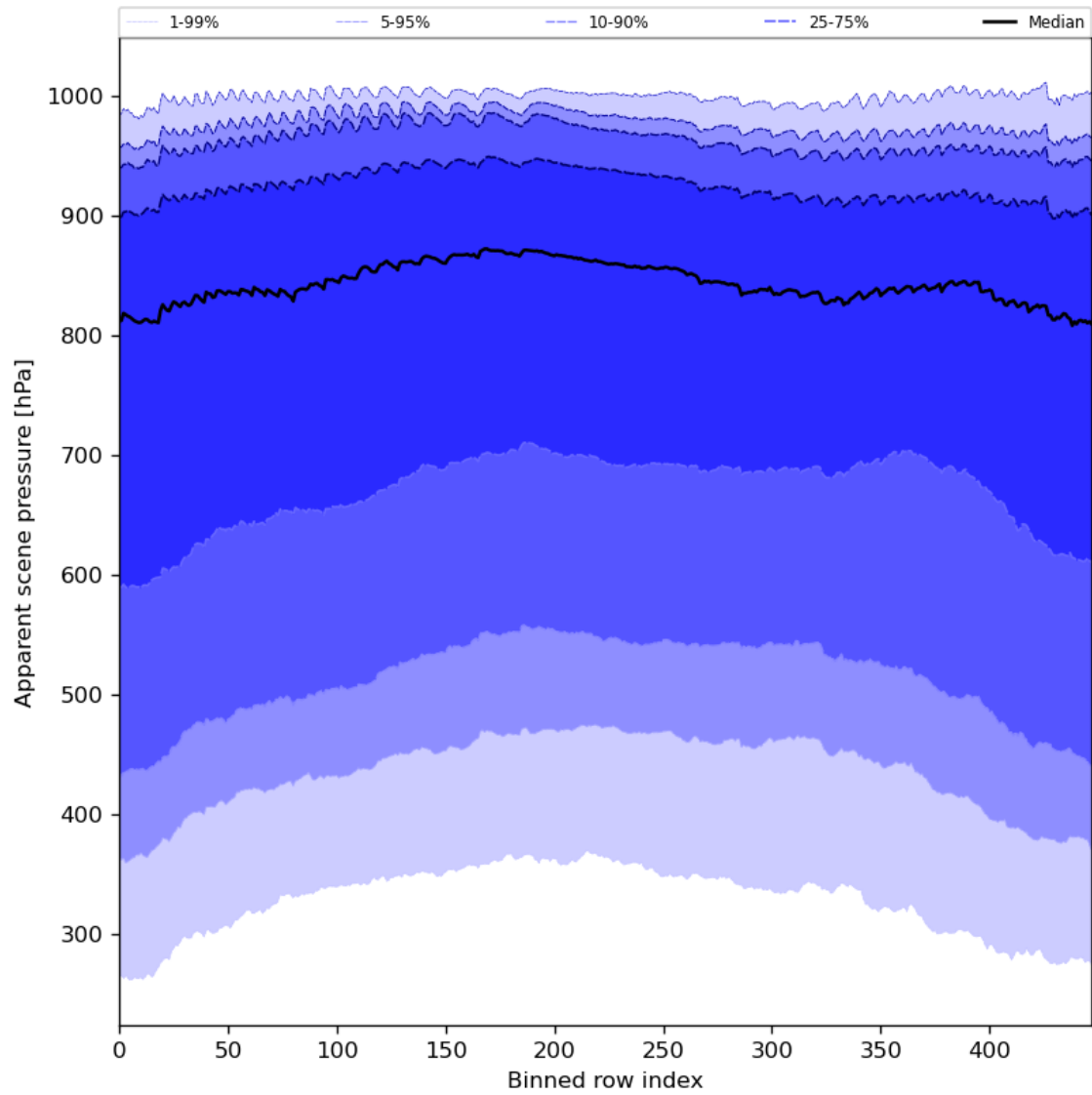
Figure 53: Along track statistics of “Apparent scene pressure” for 2023-09-07 to 2023-09-09
