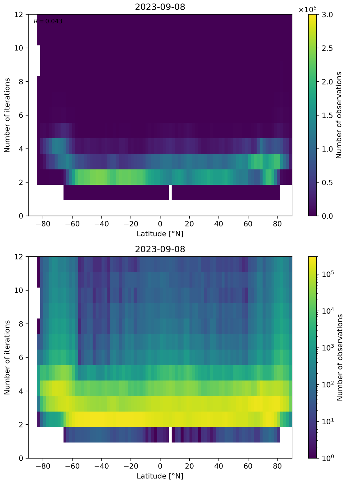
Figure 102: Scatter density plot of “Latitude” against “Number of iterations” for 2023-09-07 to 2023-09-09.
