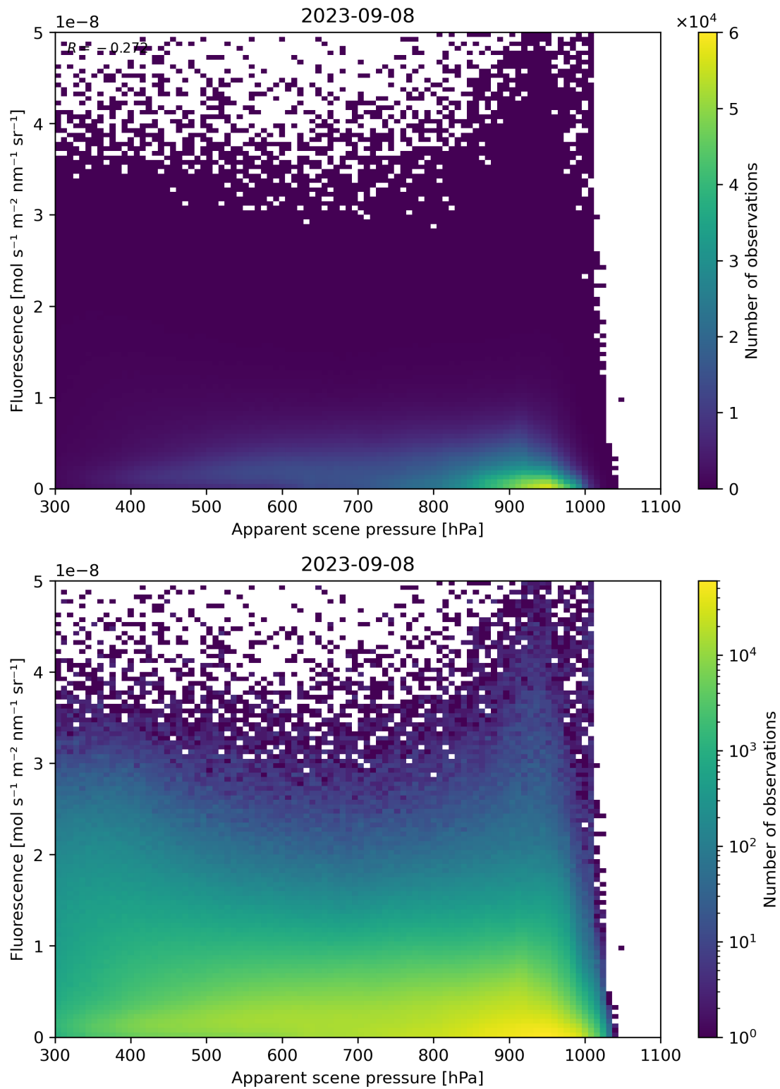
Figure 65: Scatter density plot of “Apparent scene pressure” against “Fluorescence” for 2023-09-07 to 2023-09-09.
