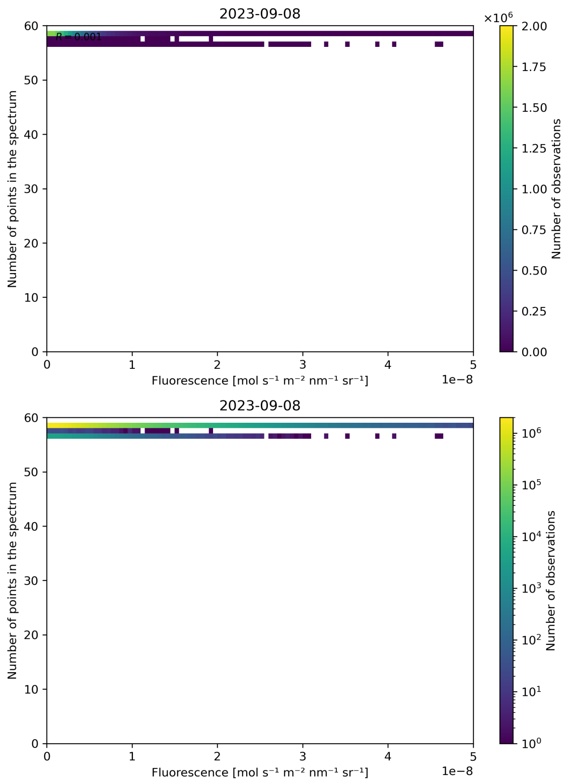
Figure 94: Scatter density plot of “Fluorescence” against “Number of points in the spectrum” for 2023-09-07 to 2023-09-09.
