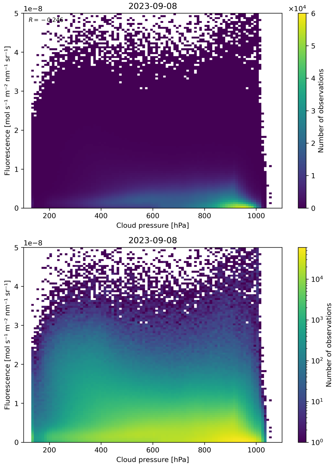
Figure 88: Scatter density plot of “Cloud pressure” against “Fluorescence” for 2023-09-07 to 2023-09-09.
