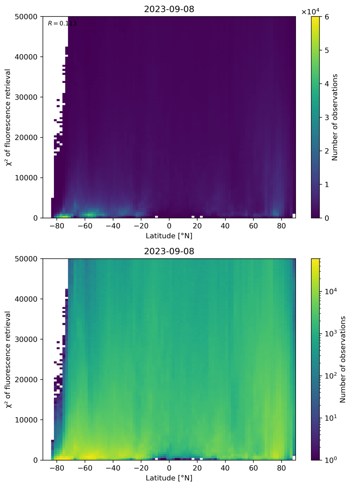
Figure 98: Scatter density plot of “Latitude” against “ \chi^2 of fluorescence retrieval” for 2023-09-07 to 2023-09-09.
