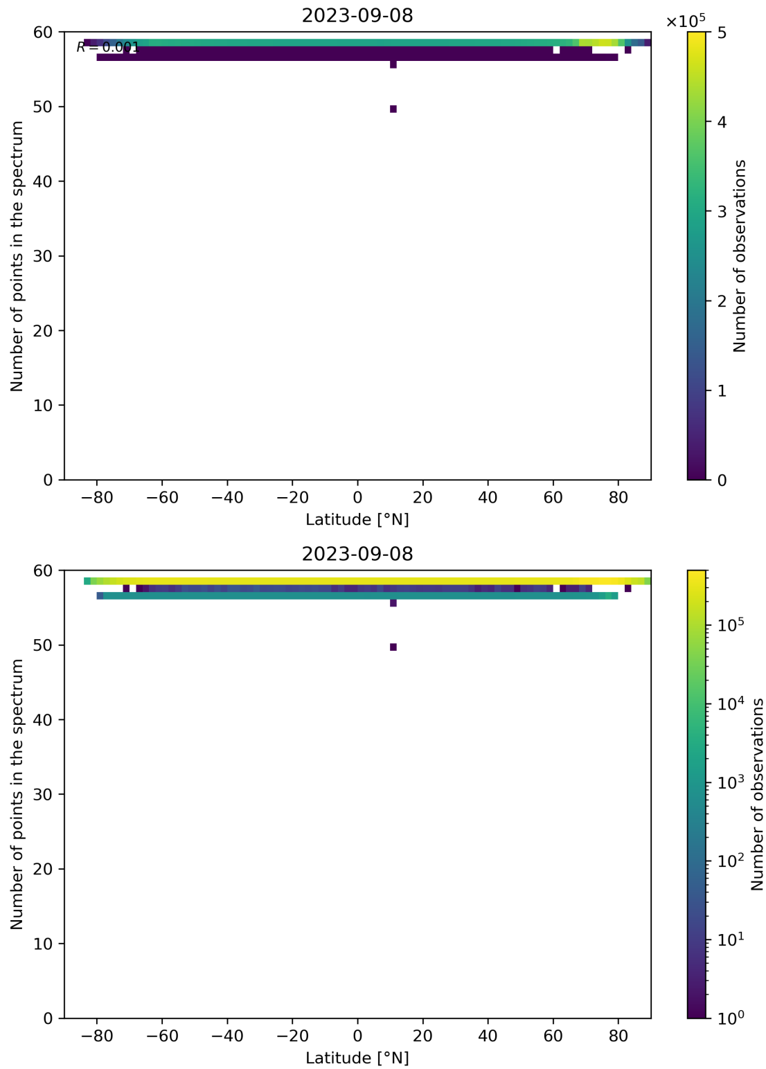
Figure 103: Scatter density plot of “Latitude” against “Number of points in the spectrum” for 2023-09-07 to 2023-09-09.
