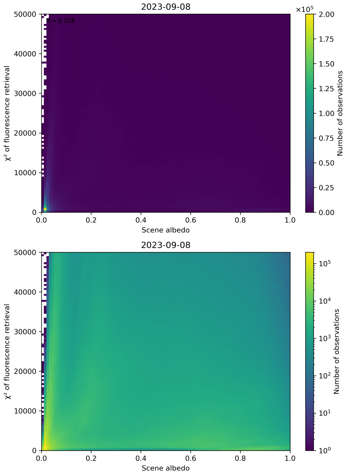
Figure 113: Scatter density plot of “Scene albedo” against “ \chi^2 of fluorescence retrieval” for 2023-09-07 to 2023-09-09.
