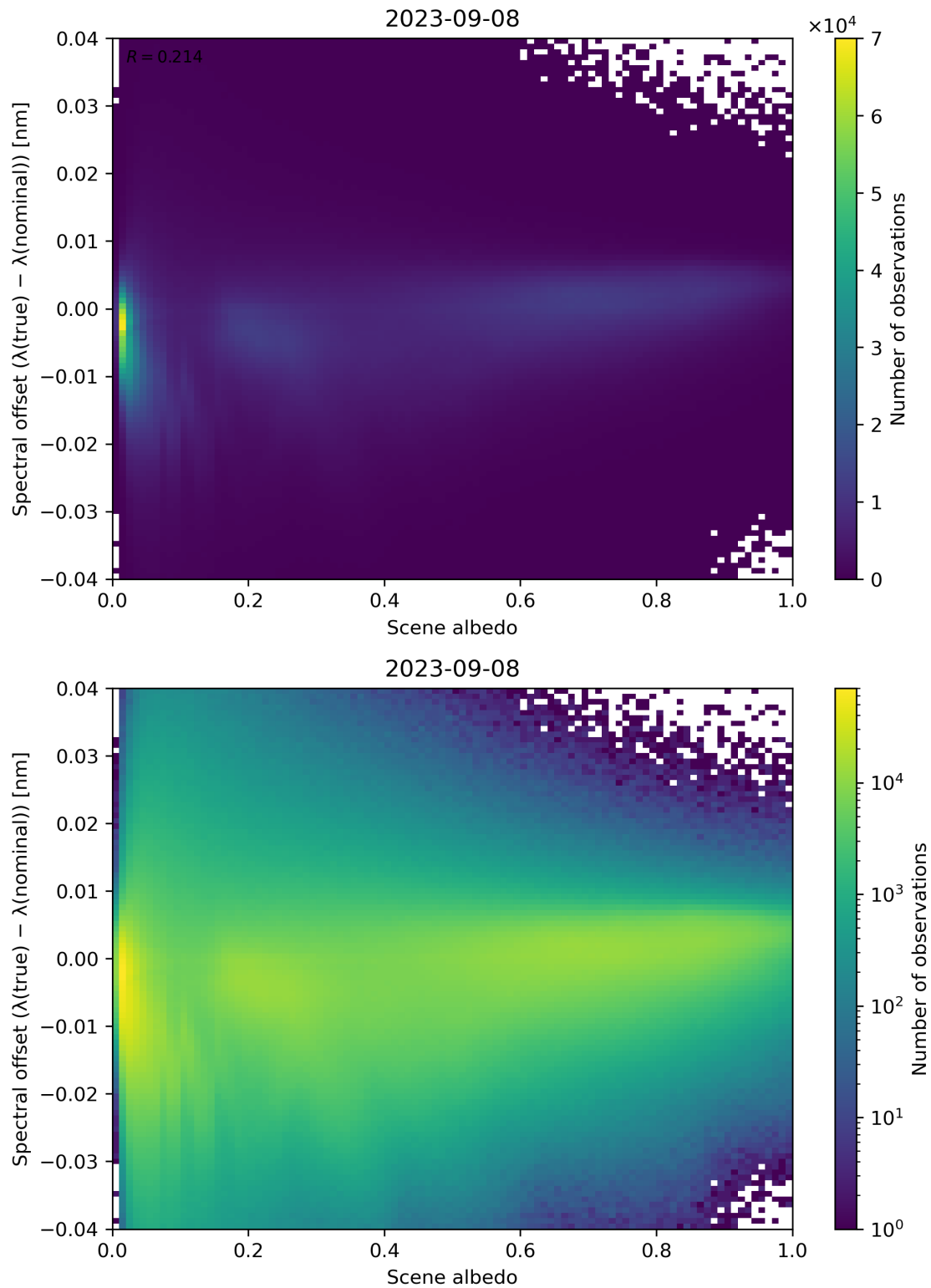
Figure 117: Scatter density plot of “Scene albedo” against “Spectral offset ( \lambda(\text{true}) - \lambda(\text{nominal}) )” for 2023-09-07 to 2023-09-09.
