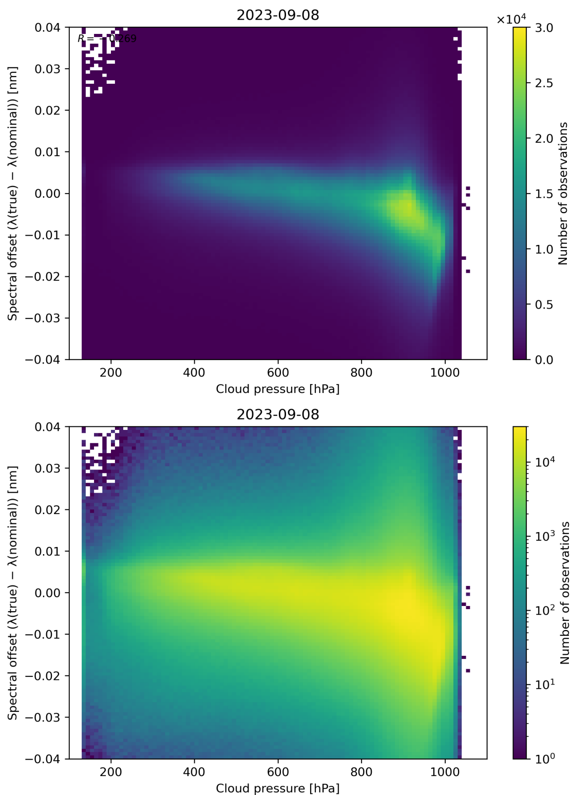
Figure 92: Scatter density plot of “Cloud pressure” against “Spectral offset ( \lambda(\text{true}) - \lambda(\text{nominal}) )” for 2023-09-07 to 2023-09-09.
