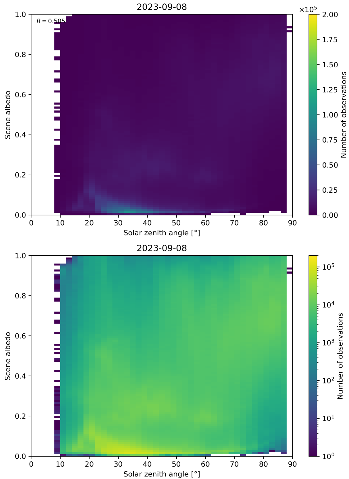
Figure 127: Scatter density plot of “Solar zenith angle” against “Scene albedo” for 2023-09-07 to 2023-09-09.
