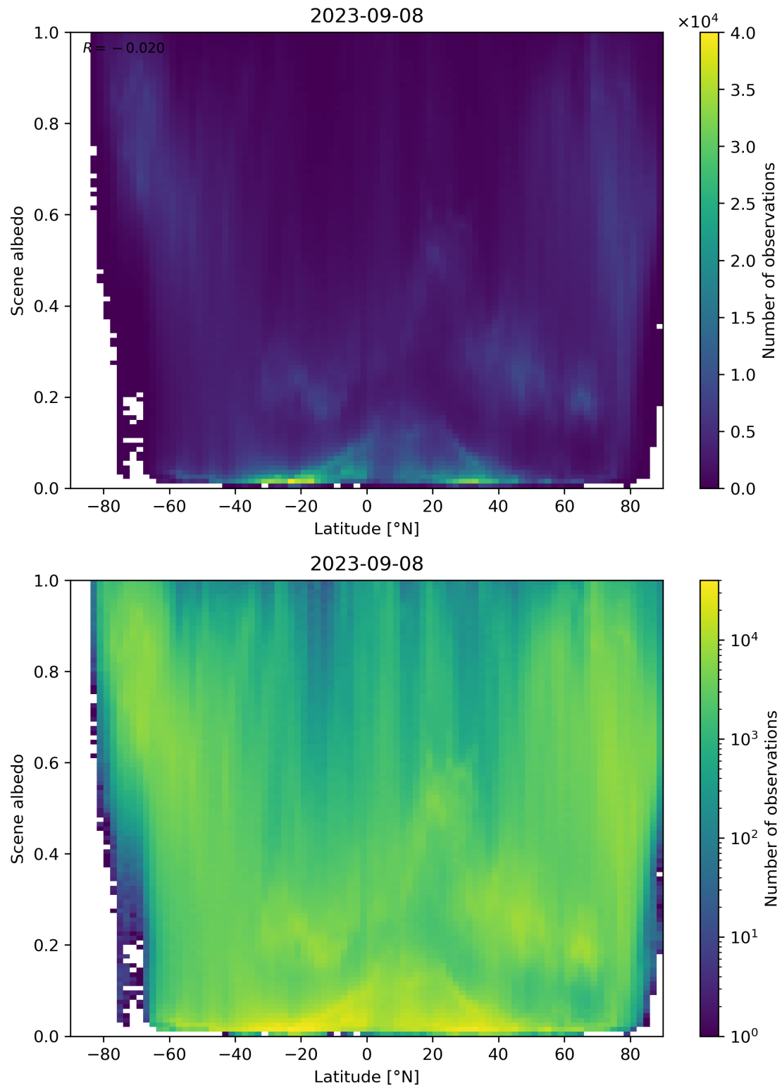
Figure 104: Scatter density plot of “Latitude” against “Scene albedo” for 2023-09-07 to 2023-09-09.
