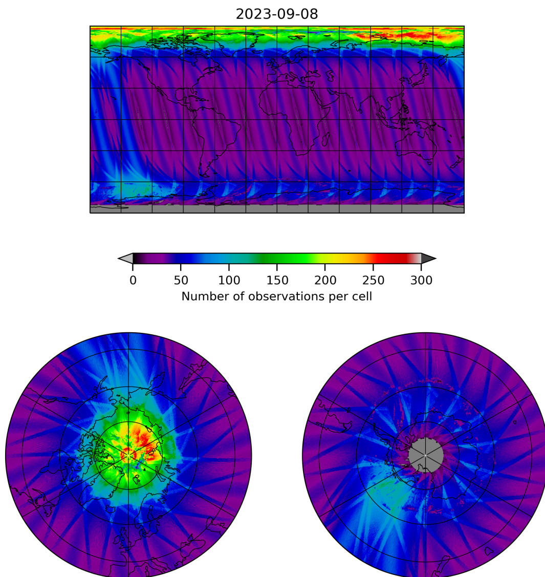
Figure 11: Map of the number of observations for 2023-09-07 to 2023-09-09
