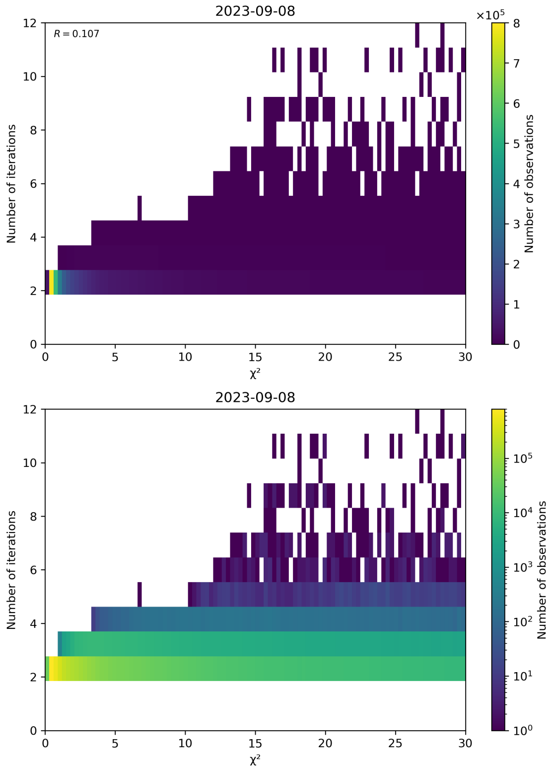
Figure 73: Scatter density plot of “ \chi^2 ” against “Number of iterations” for 2023-09-07 to 2023-09-09.
