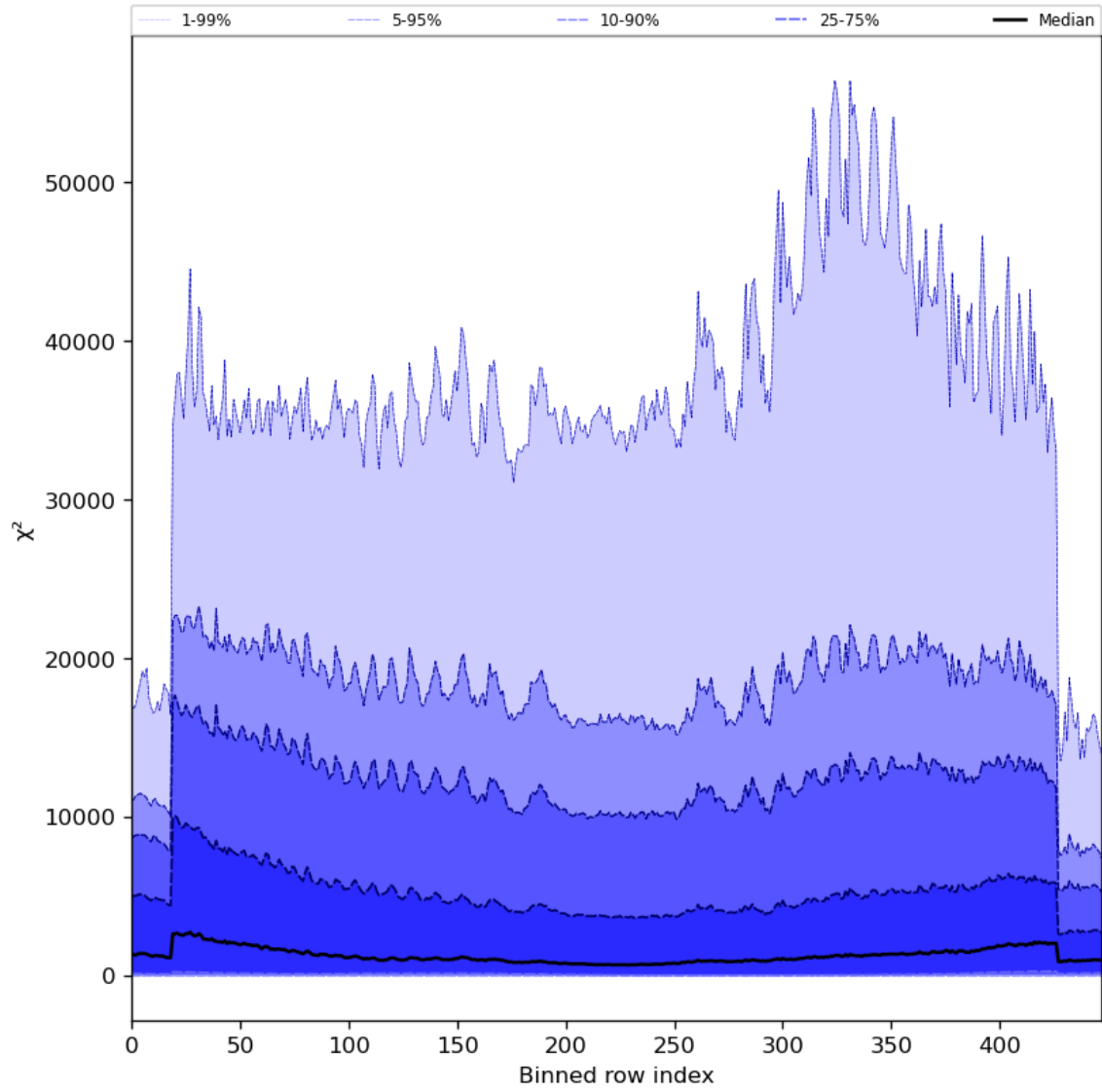
Figure 55: Along track statistics of “ \chi^2 ” for 2023-09-07 to 2023-09-09
