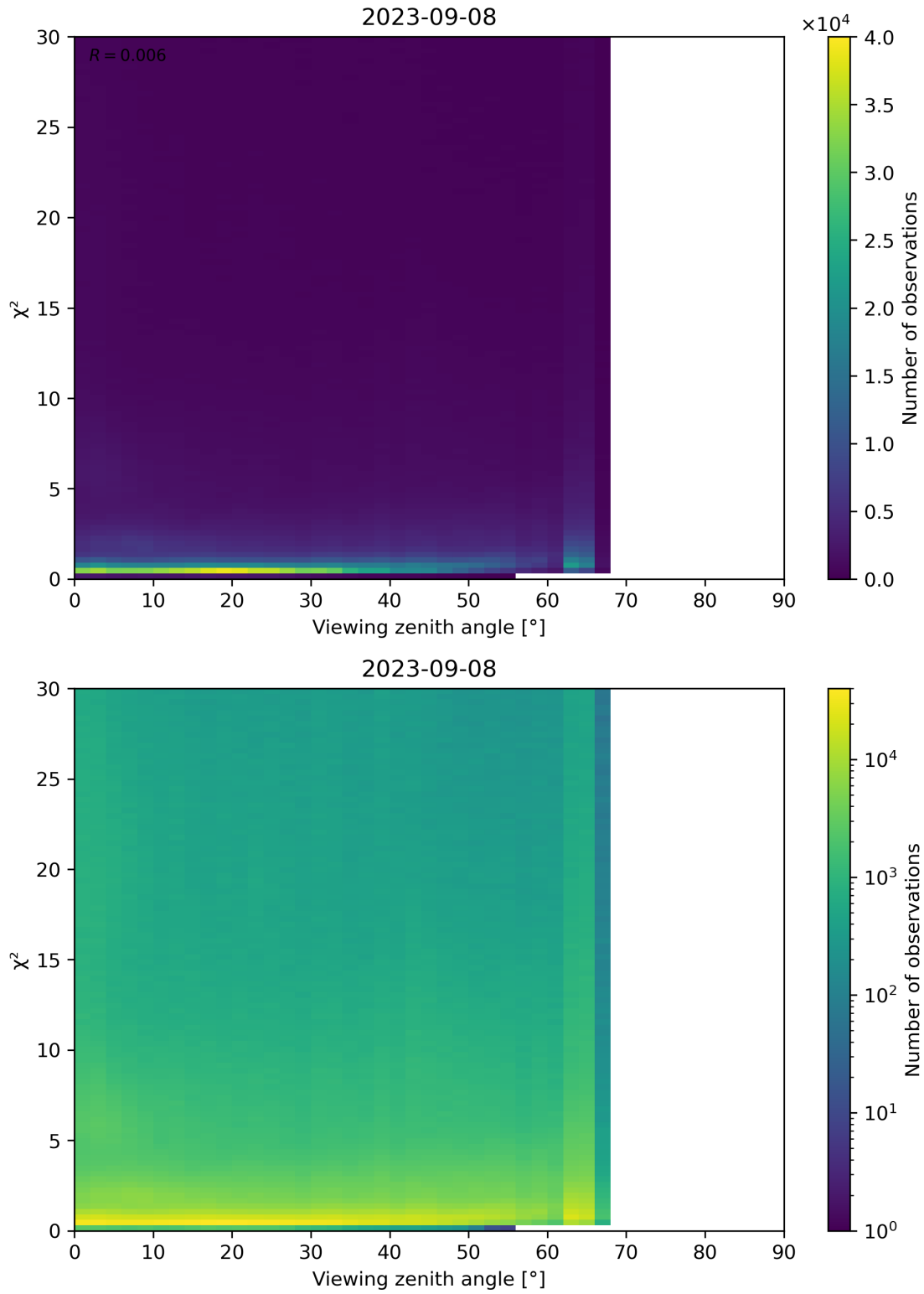
Figure 130: Scatter density plot of “Viewing zenith angle” against “ \chi^2 ” for 2023-09-07 to 2023-09-09.
