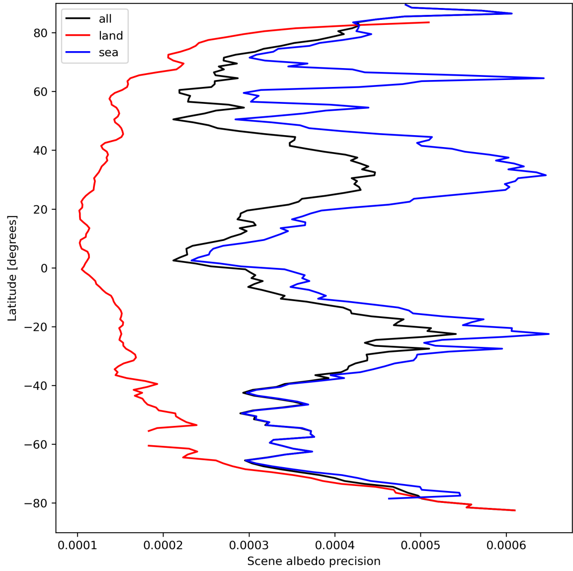
Figure 18: Zonal average of “Scene albedo precision” for 2023-09-07 to 2023-09-09.
