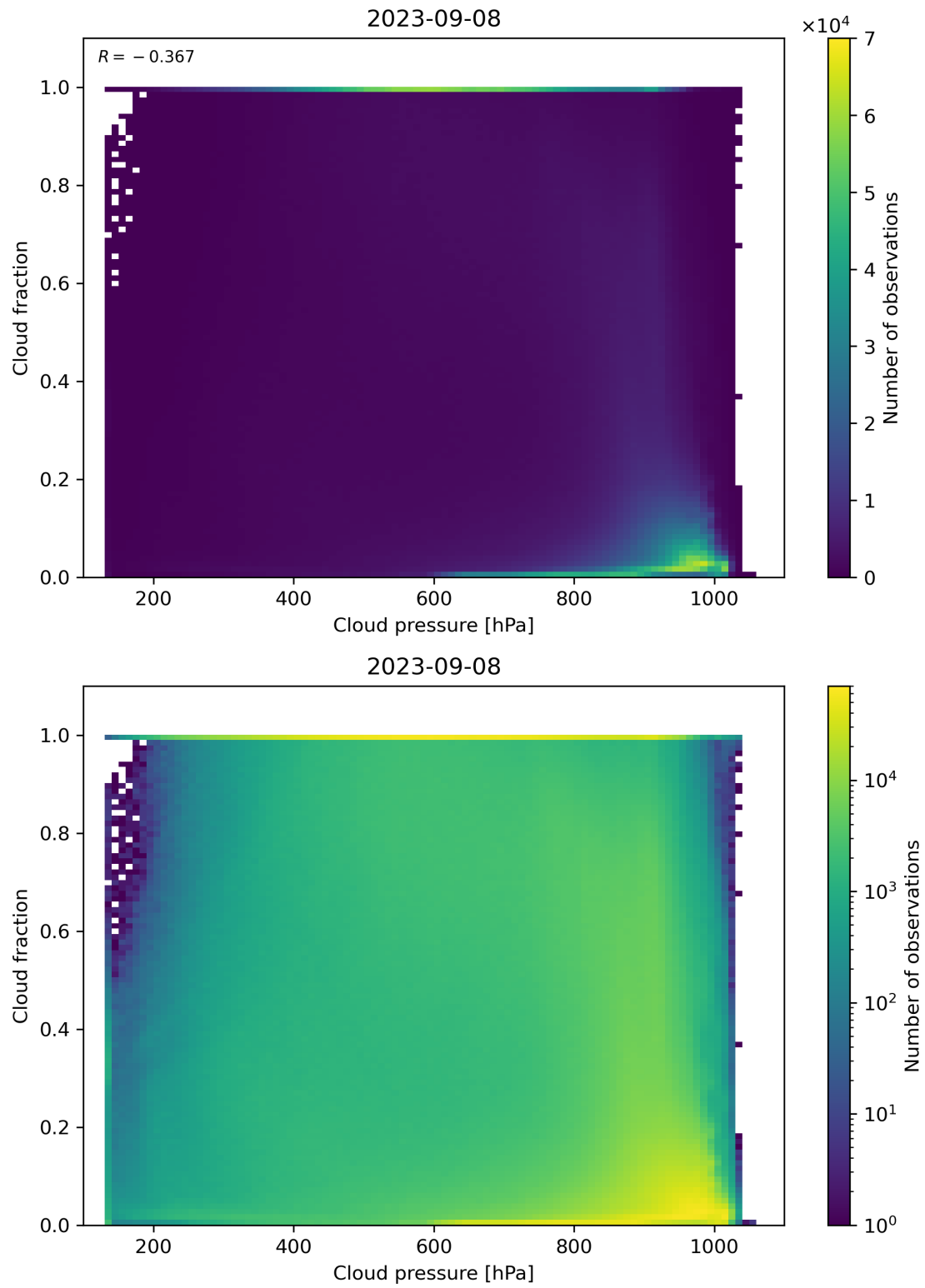
Figure 87: Scatter density plot of “Cloud pressure” against “Cloud fraction” for 2023-09-07 to 2023-09-09.
