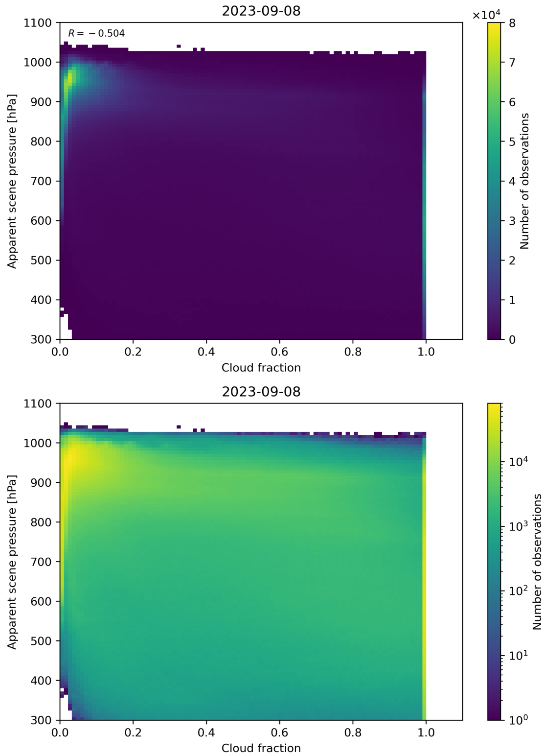
Figure 76: Scatter density plot of “Cloud fraction” against “Apparent scene pressure” for 2023-09-07 to 2023-09-09.
