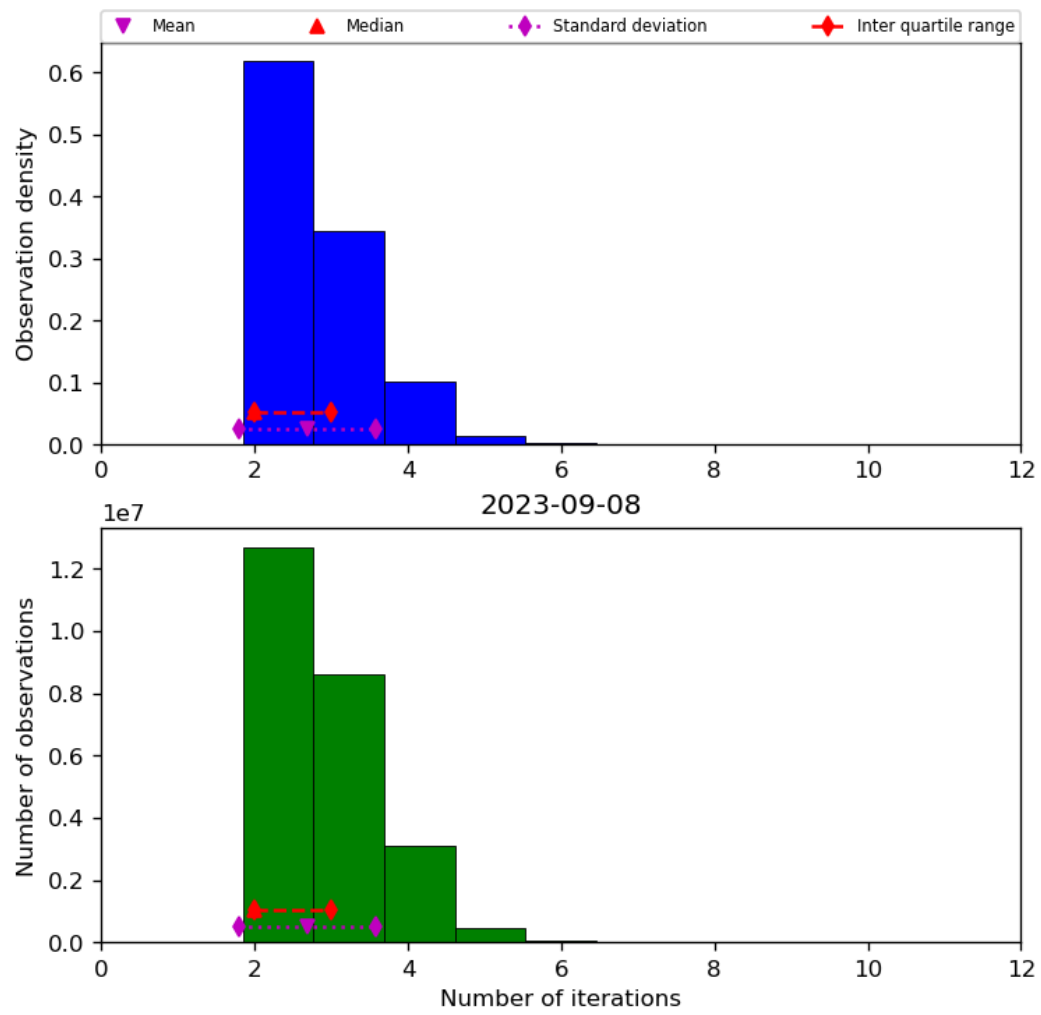
Figure 39: Histogram of “Number of iterations” for 2023-09-07 to 2023-09-09
