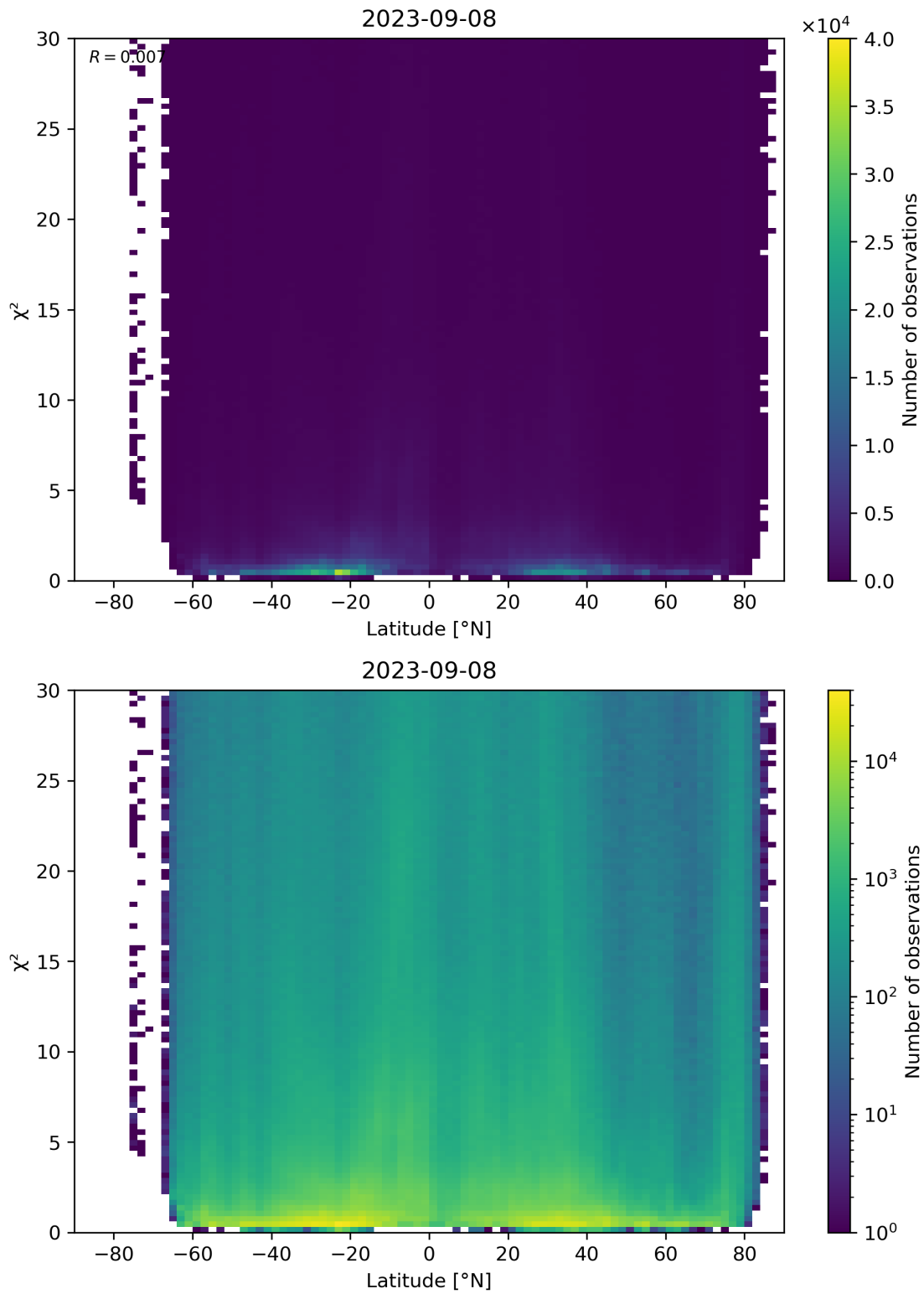
Figure 97: Scatter density plot of “Latitude” against “ \chi^2 ” for 2023-09-07 to 2023-09-09.
