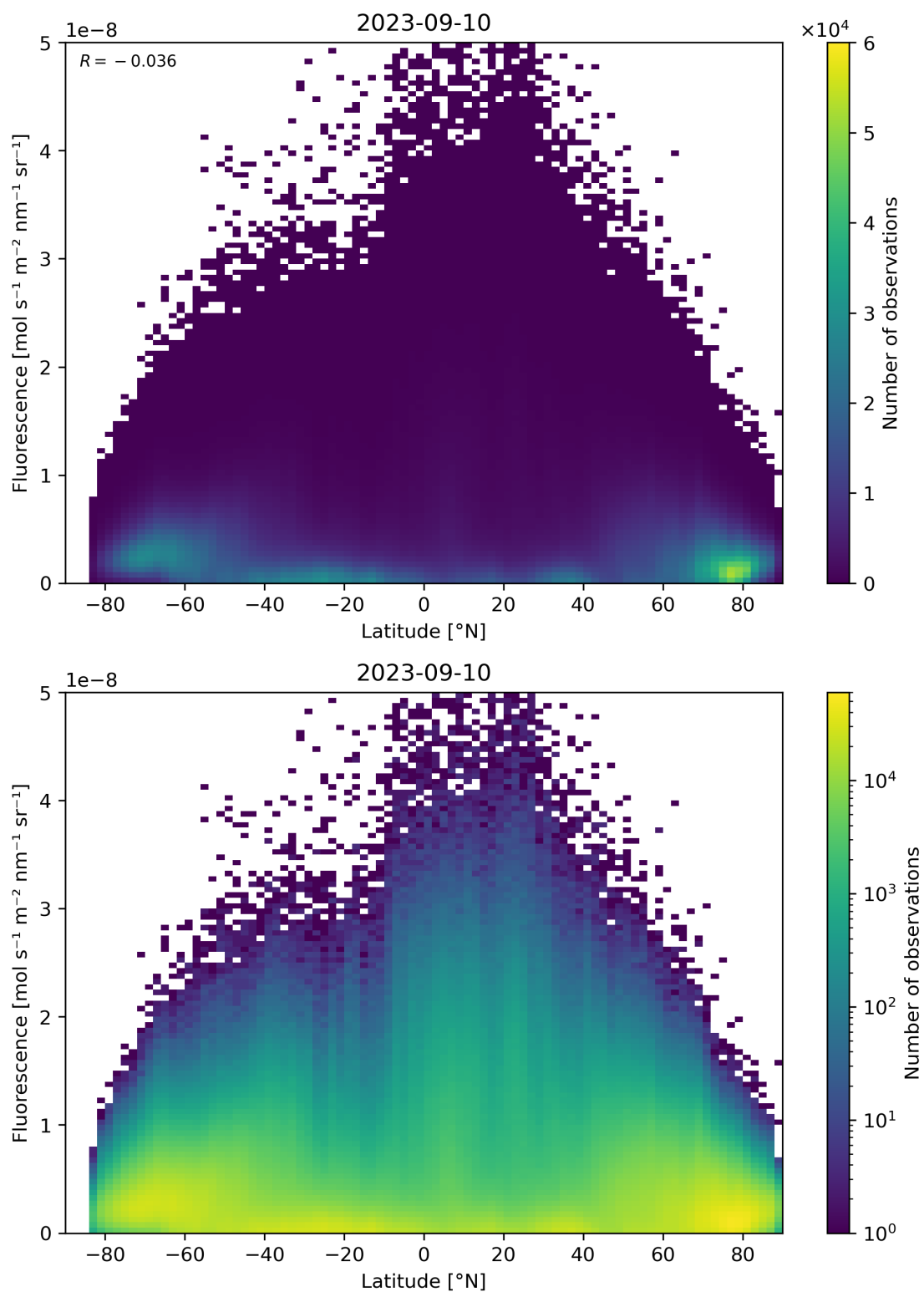
Figure 101: Scatter density plot of “Latitude” against “Fluorescence” for 2023-09-10 to 2023-09-11.
