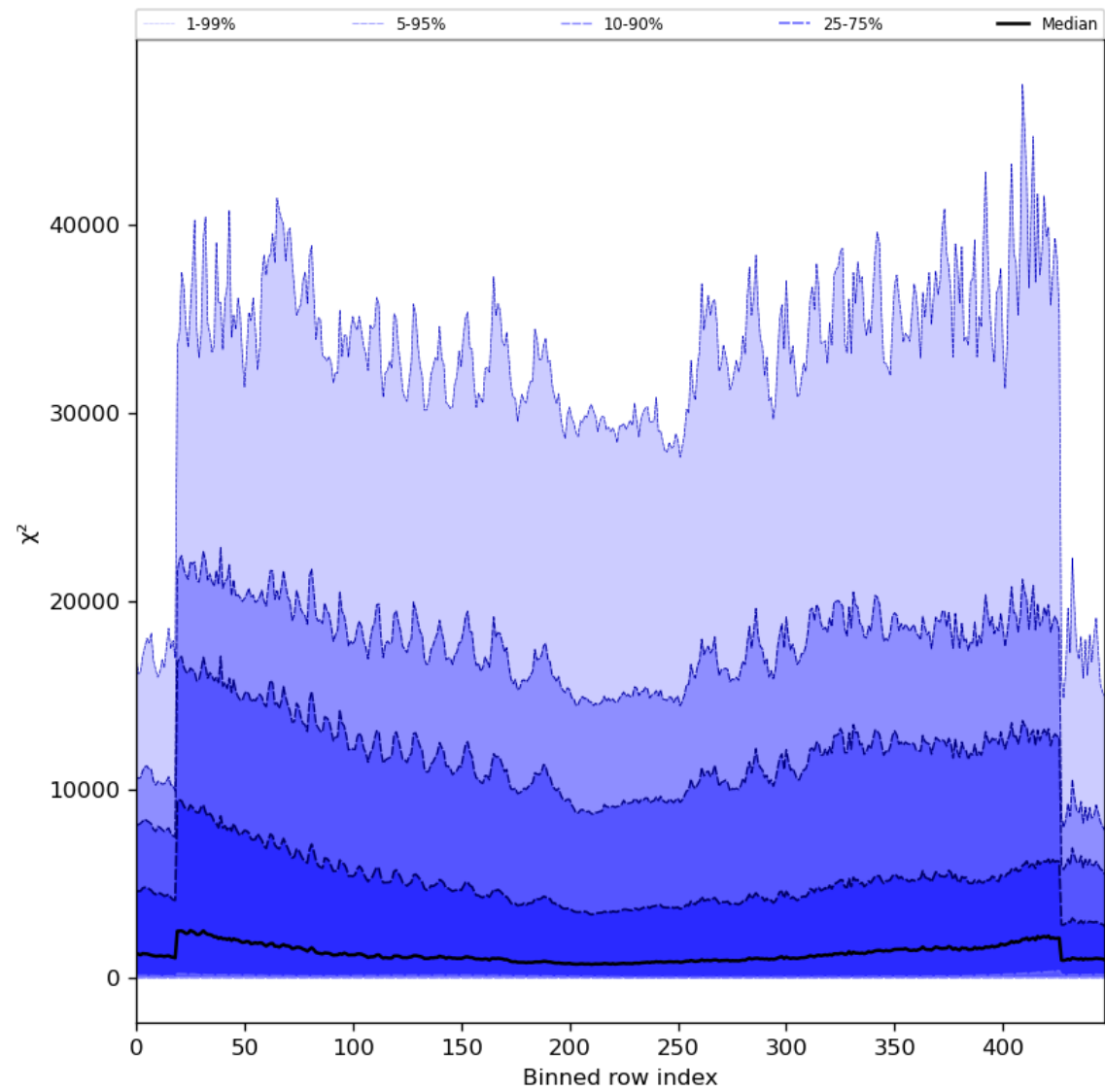
Figure 55: Along track statistics of “ \chi^2 ” for 2023-09-10 to 2023-09-11
