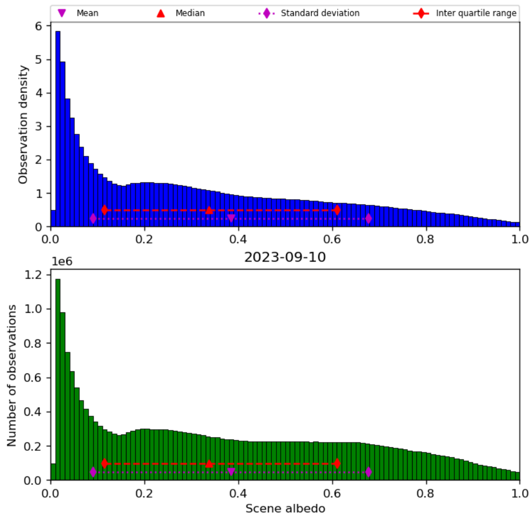
Figure 34: Histogram of “Scene albedo” for 2023-09-10 to 2023-09-11
