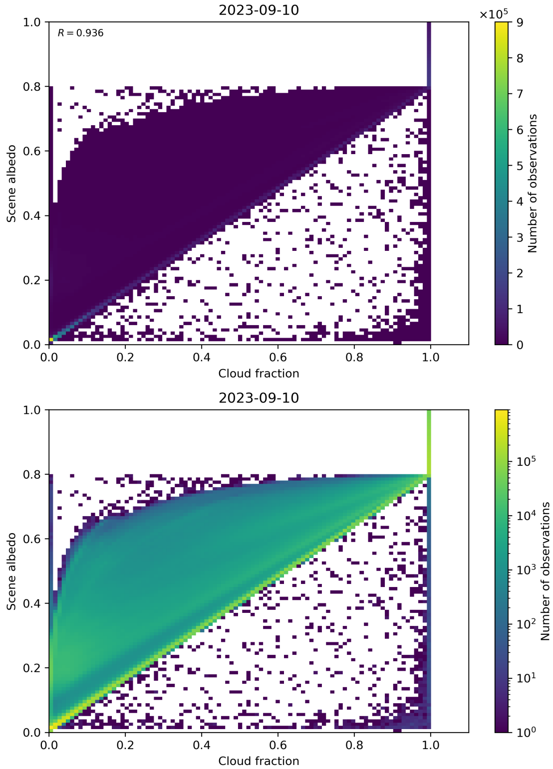
Figure 82: Scatter density plot of “Cloud fraction” against “Scene albedo” for 2023-09-10 to 2023-09-11.
