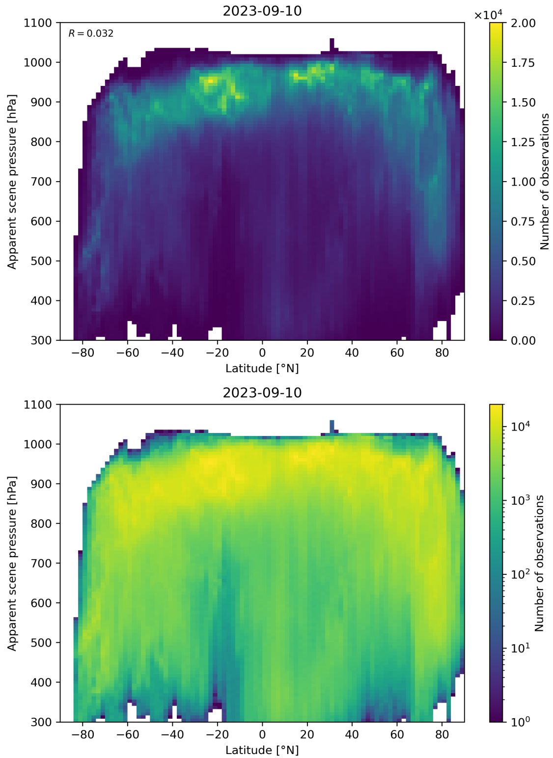
Figure 96: Scatter density plot of “Latitude” against “Apparent scene pressure” for 2023-09-10 to 2023-09-11.
