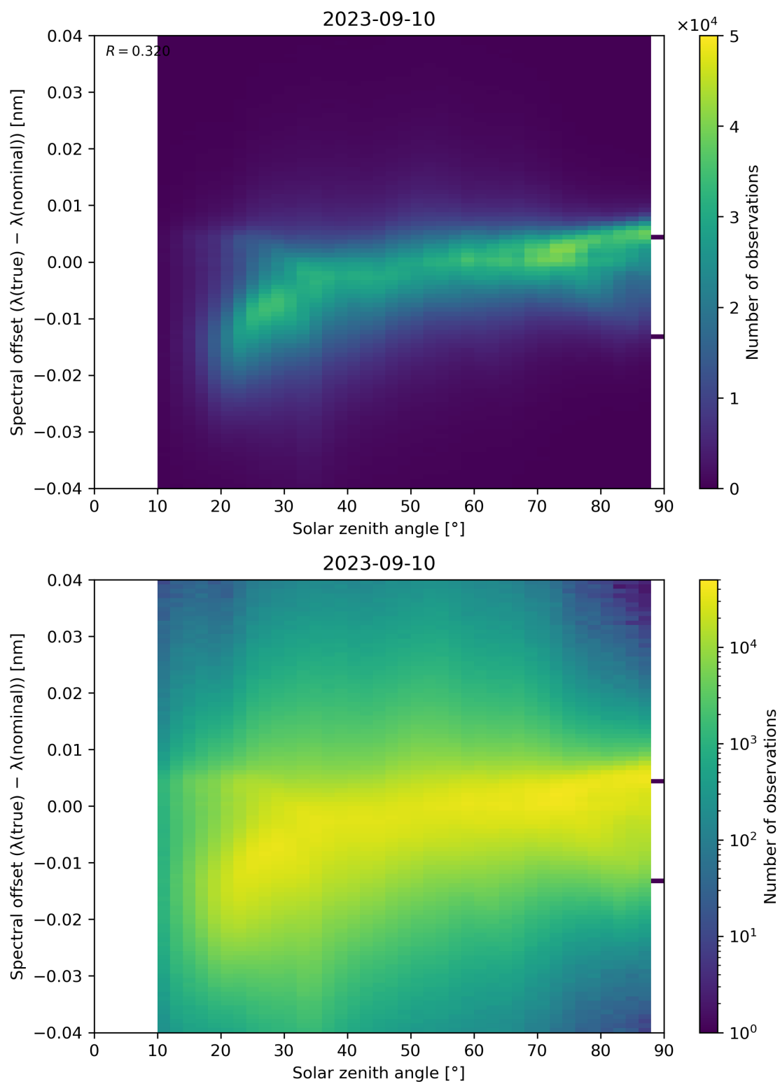
Figure 128: Scatter density plot of “Solar zenith angle” against “Spectral offset ( \lambda(\text{true}) - \lambda(\text{nominal}) )” for 2023-09-10 to 2023-09-11.
