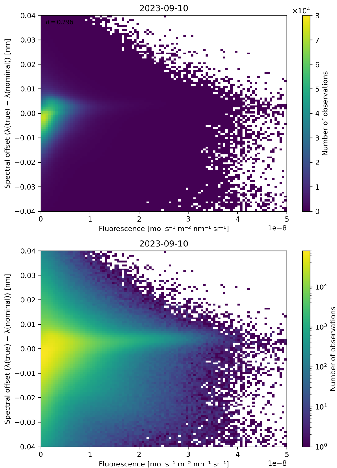
Figure 95: Scatter density plot of “Fluorescence” against “Spectral offset ( \lambda(\text{true}) - \lambda(\text{nominal}) )” for 2023-09-10 to 2023-09-11.
