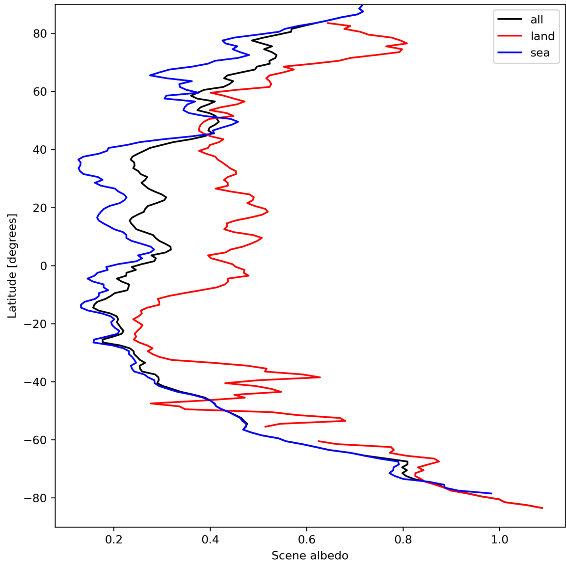
Figure 17: Zonal average of “Scene albedo” for 2023-09-10 to 2023-09-11.
