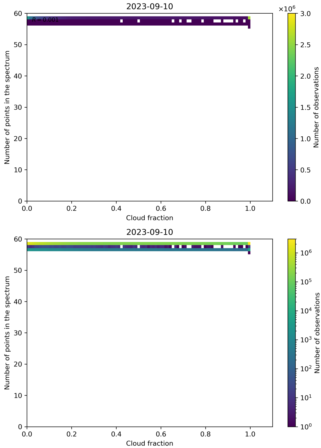
Figure 81: Scatter density plot of “Cloud fraction” against “Number of points in the spectrum” for 2023-09-10 to 2023-09-11.
