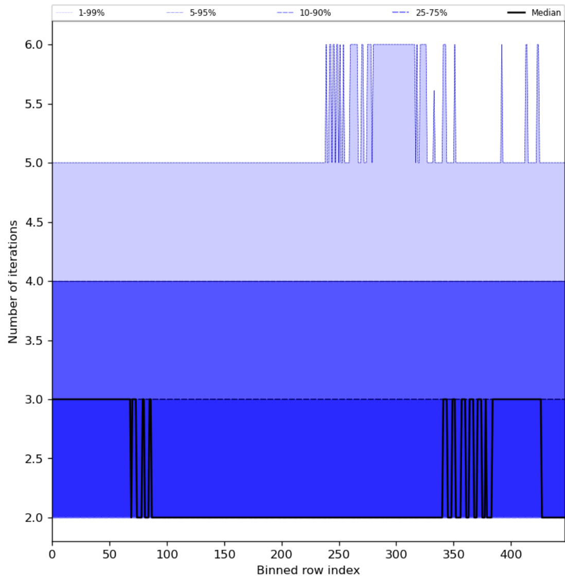
Figure 56: Along track statistics of “Number of iterations” for 2023-09-10 to 2023-09-11
