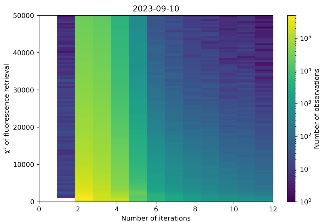
Figure 106: Scatter density plot of “Number of iterations” against “ \chi^2 of fluorescence retrieval” for 2023-09-10 to 2023-09-11.
