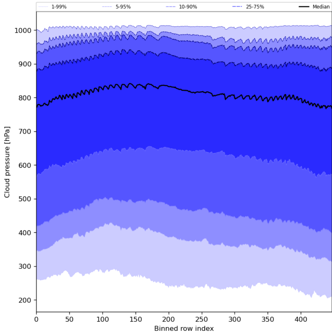
Figure 47: Along track statistics of “Cloud pressure” for 2023-09-10 to 2023-09-11
