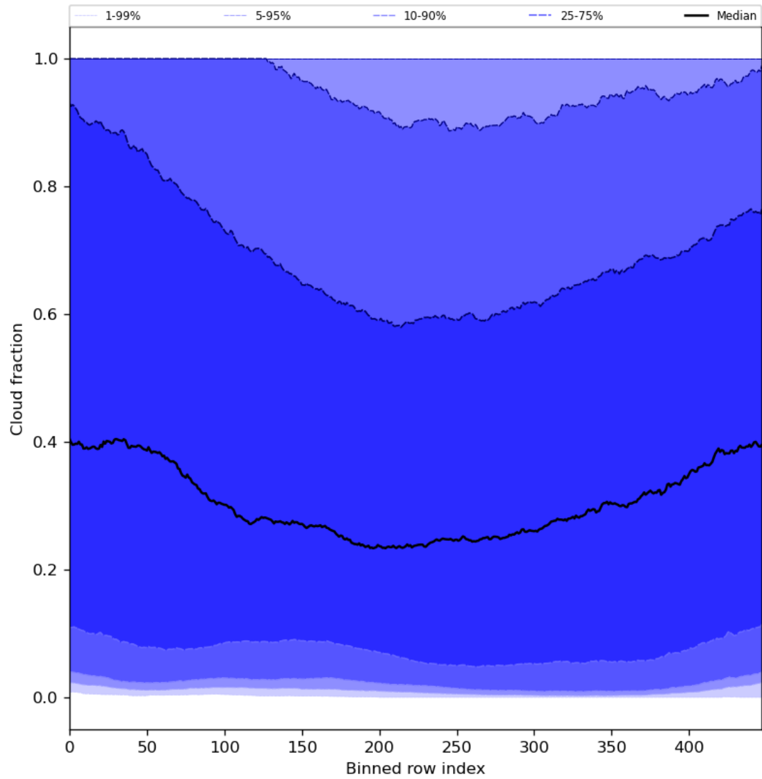
Figure 49: Along track statistics of “Cloud fraction” for 2023-09-10 to 2023-09-11
