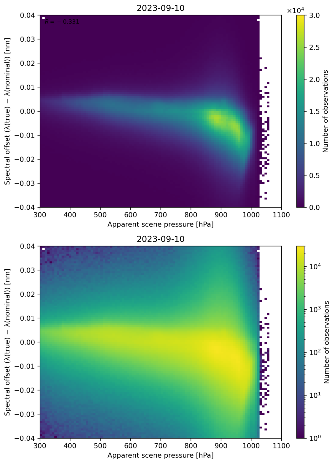
Figure 68: Scatter density plot of “Apparent scene pressure” against “Spectral offset ( \lambda(\text{true}) - \lambda(\text{nominal}) )” for 2023-09-10 to 2023-09-11.
