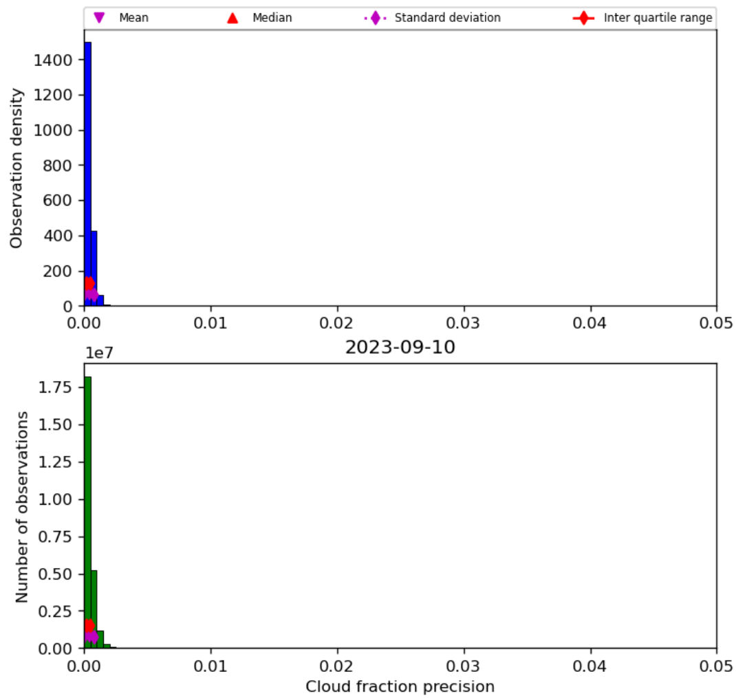
Figure 33: Histogram of “Cloud fraction precision” for 2023-09-10 to 2023-09-11
