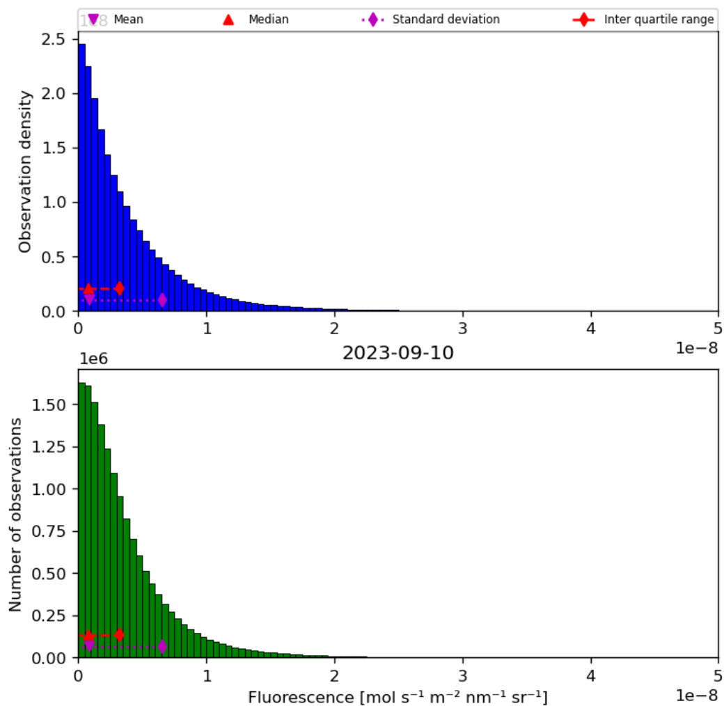
Figure 40: Histogram of “Fluorescence” for 2023-09-10 to 2023-09-11
