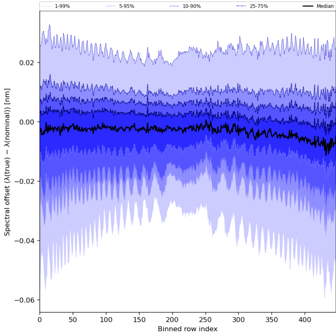
Figure 62: Along track statistics of “Spectral offset ( \lambda(\text{true}) - \lambda(\text{nominal}) )” for 2023-09-10 to 2023-09-11
