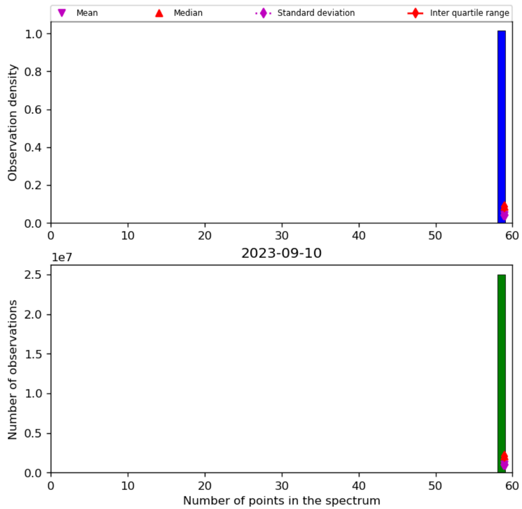
Figure 44: Histogram of “Number of points in the spectrum” for 2023-09-10 to 2023-09-11
