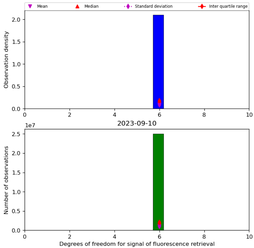
Figure 43: Histogram of “Degrees of freedom for signal of fluorescence retrieval” for 2023-09-10 to 2023-09-11
