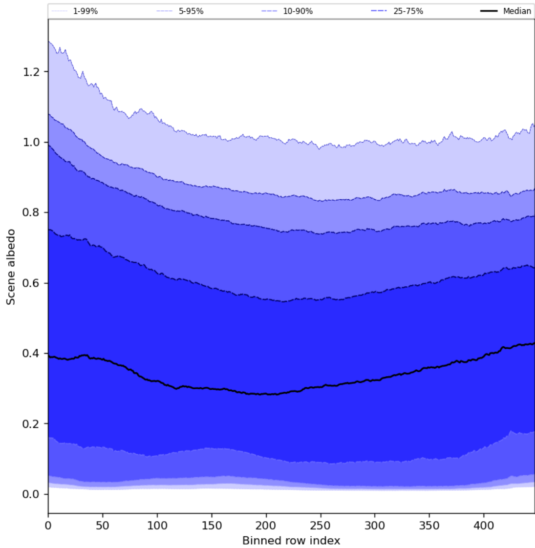
Figure 51: Along track statistics of “Scene albedo” for 2023-09-10 to 2023-09-11
