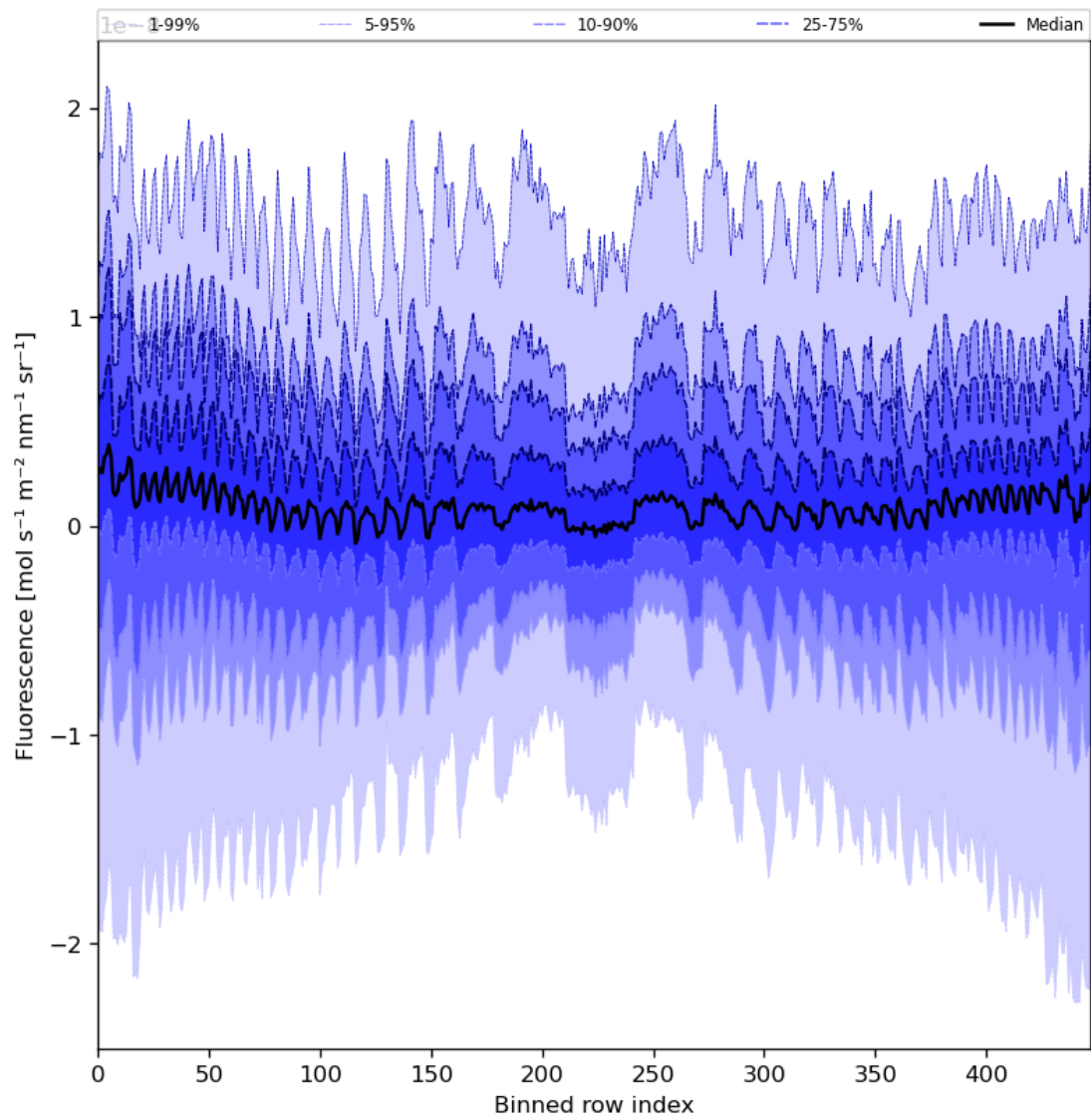
Figure 57: Along track statistics of "Fluorescence" for 2023-09-10 to 2023-09-11
