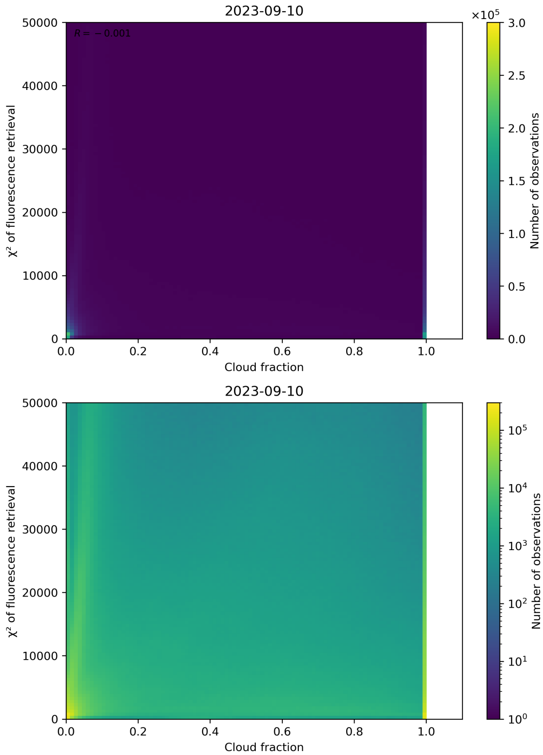
Figure 78: Scatter density plot of “Cloud fraction” against “ \chi^2 of fluorescence retrieval” for 2023-09-10 to 2023-09-11.
