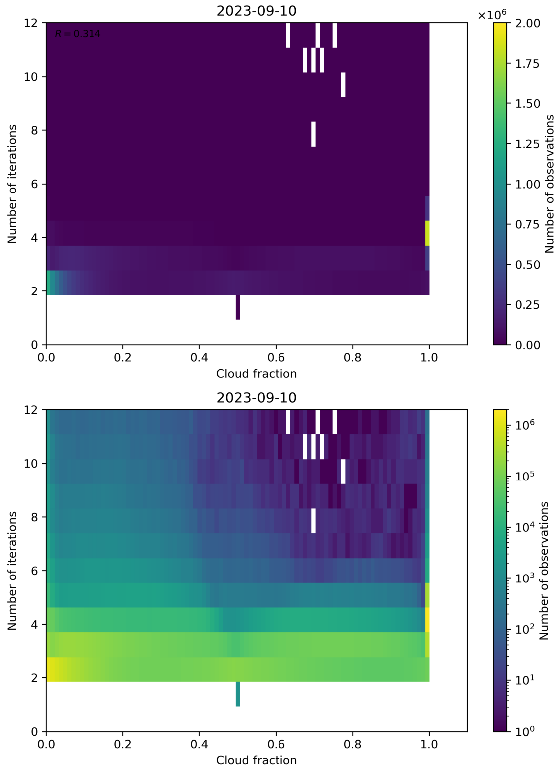
Figure 80: Scatter density plot of “Cloud fraction” against “Number of iterations” for 2023-09-10 to 2023-09-11.
