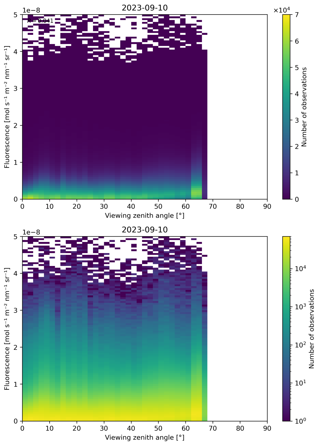
Figure 134: Scatter density plot of “Viewing zenith angle” against “Fluorescence” for 2023-09-10 to 2023-09-11.
