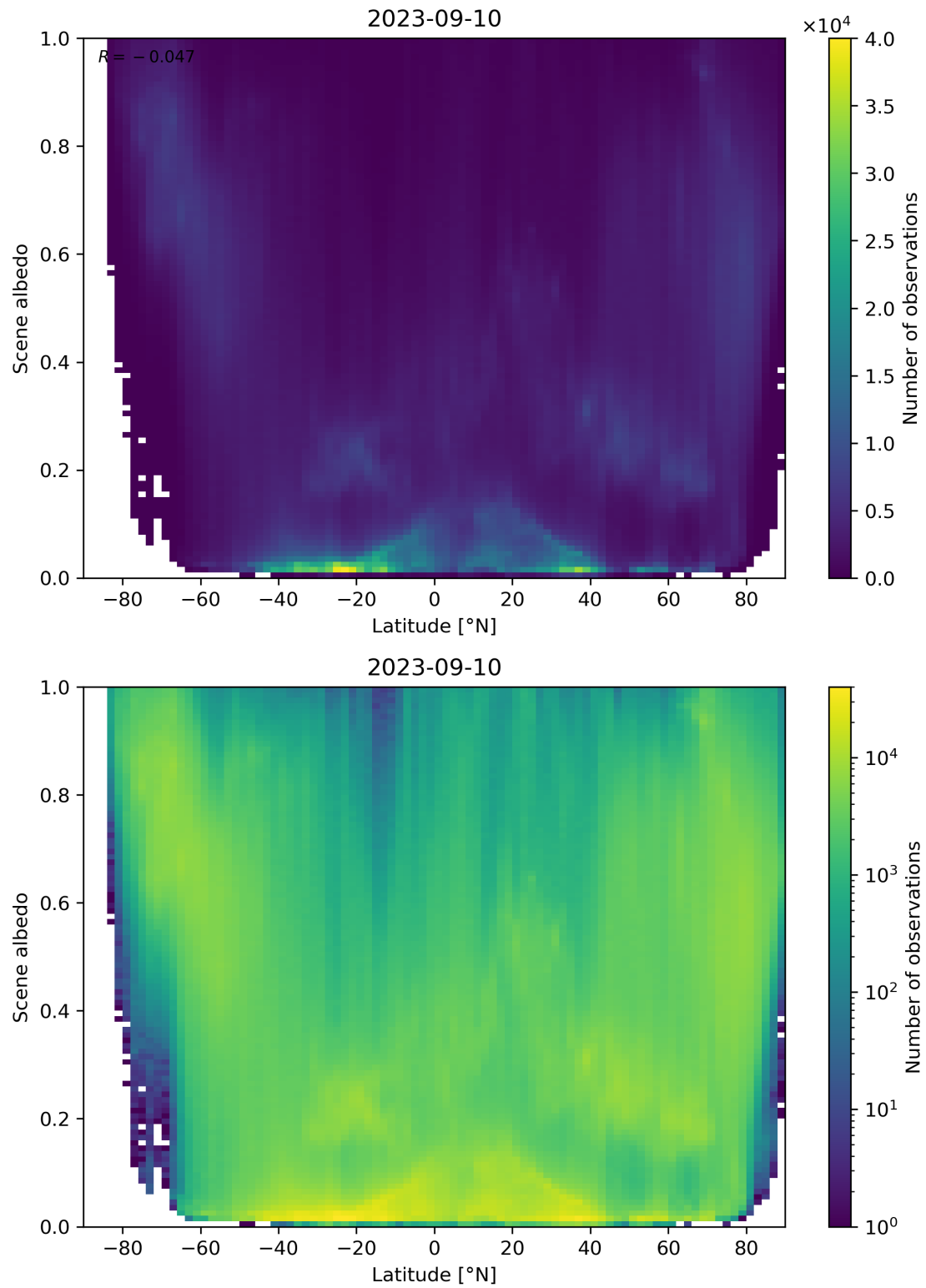
Figure 104: Scatter density plot of “Latitude” against “Scene albedo” for 2023-09-10 to 2023-09-11.
