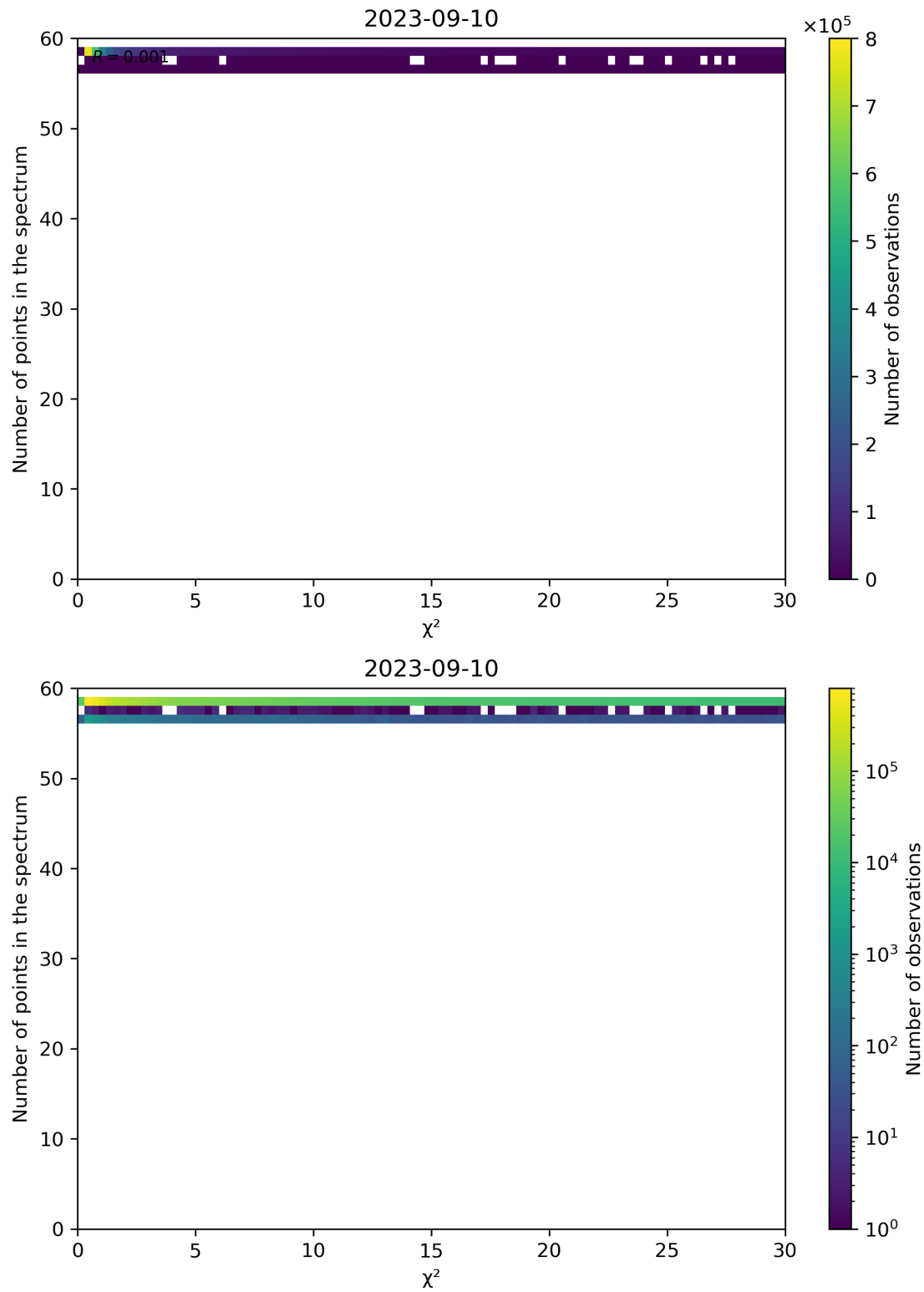
Figure 74: Scatter density plot of " \chi^2 " against "Number of points in the spectrum" for 2023-09-10 to 2023-09-11.
