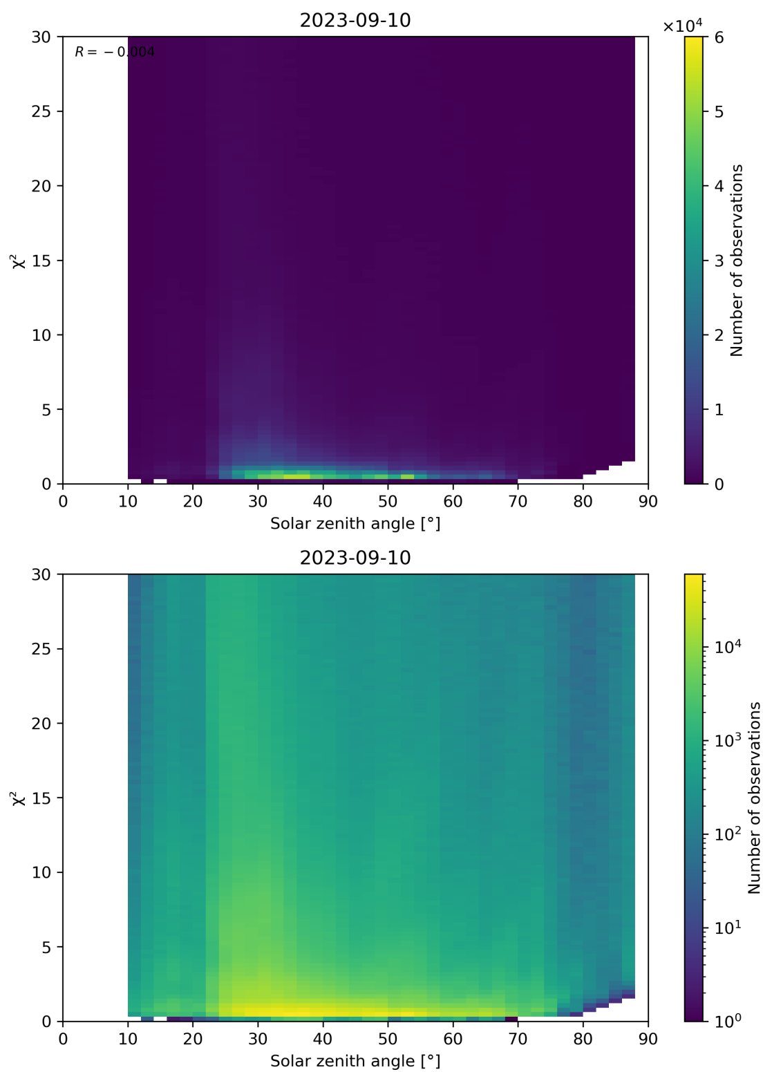
Figure 119: Scatter density plot of “Solar zenith angle” against “ \chi^2 ” for 2023-09-10 to 2023-09-11.
