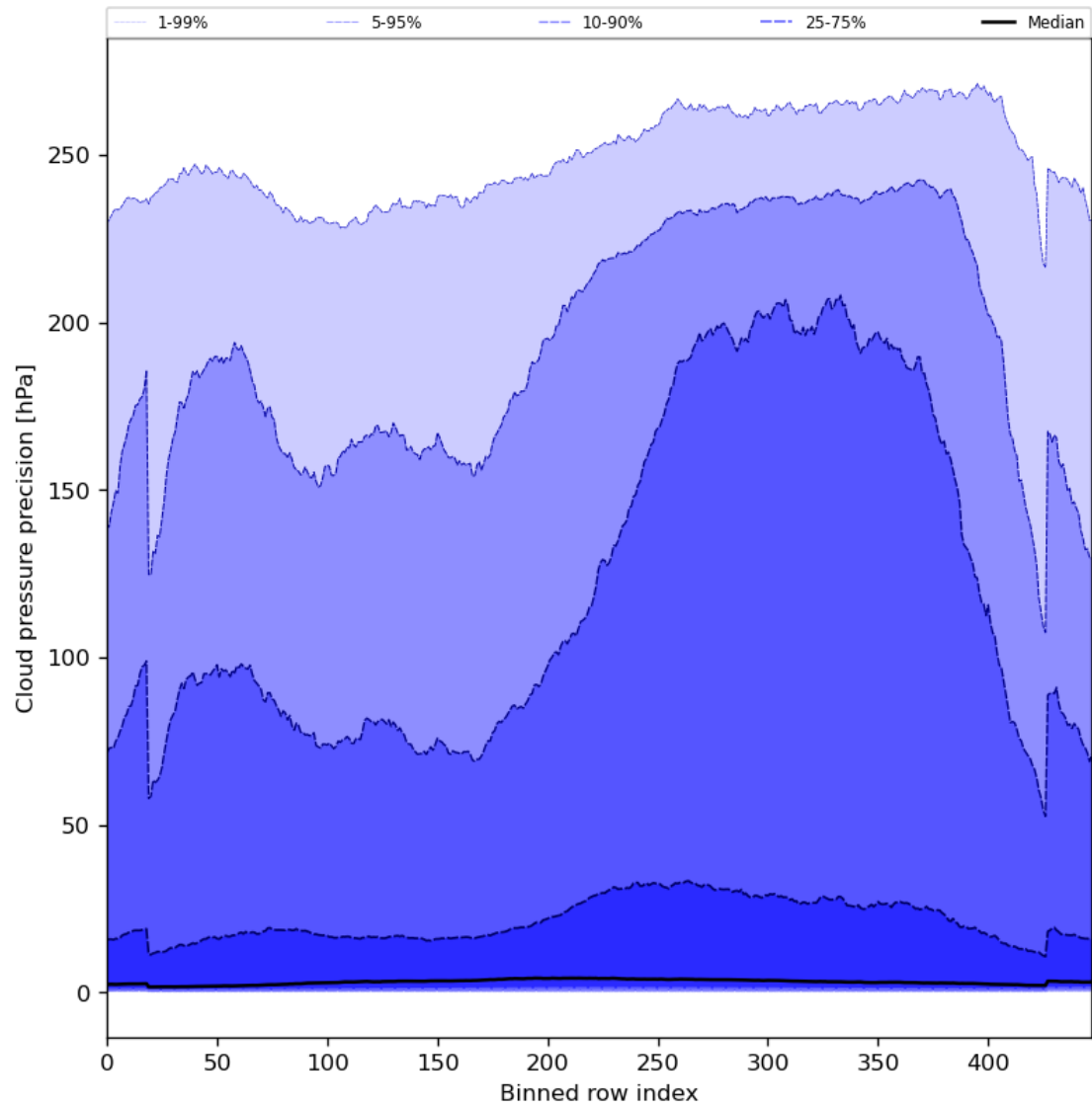
Figure 48: Along track statistics of “Cloud pressure precision” for 2023-09-10 to 2023-09-11
