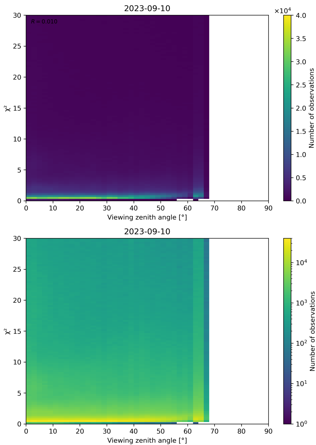
Figure 130: Scatter density plot of “Viewing zenith angle” against “ \chi^2 ” for 2023-09-10 to 2023-09-11.
