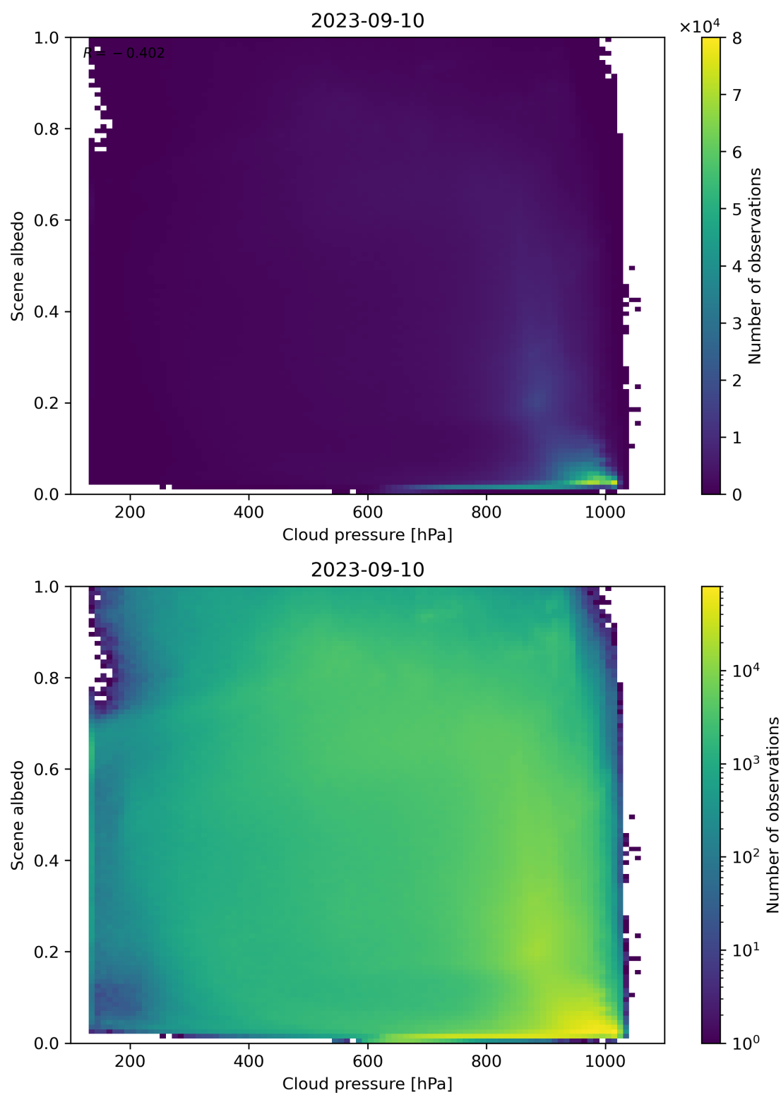
Figure 91: Scatter density plot of “Cloud pressure” against “Scene albedo” for 2023-09-10 to 2023-09-11.
