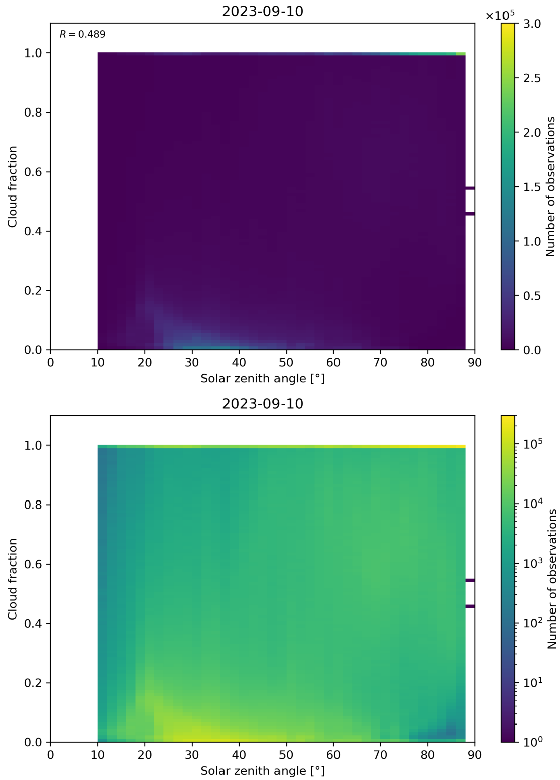
Figure 121: Scatter density plot of “Solar zenith angle” against “Cloud fraction” for 2023-09-10 to 2023-09-11.
