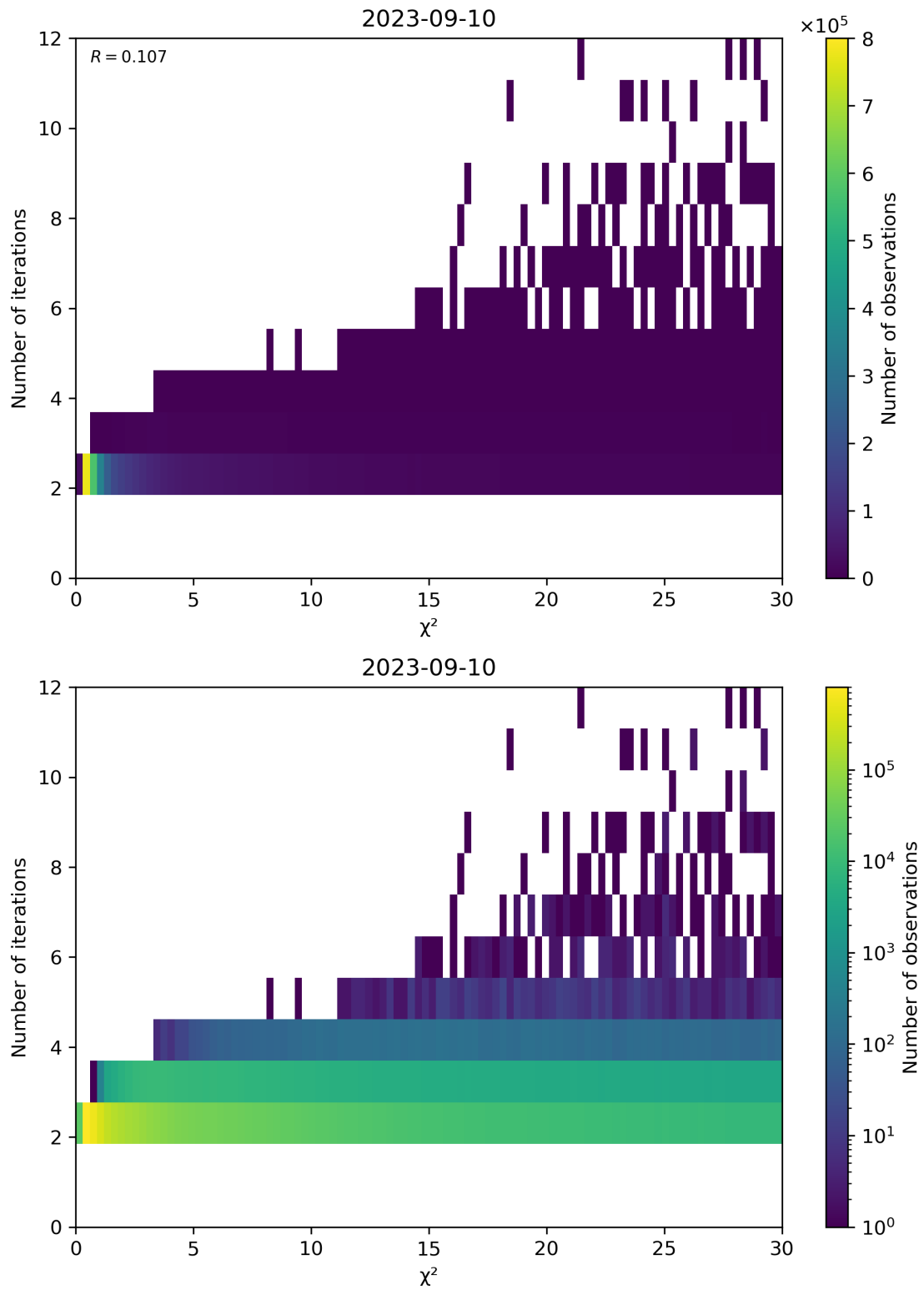
Figure 73: Scatter density plot of " \chi^2 " against "Number of iterations" for 2023-09-10 to 2023-09-11.
