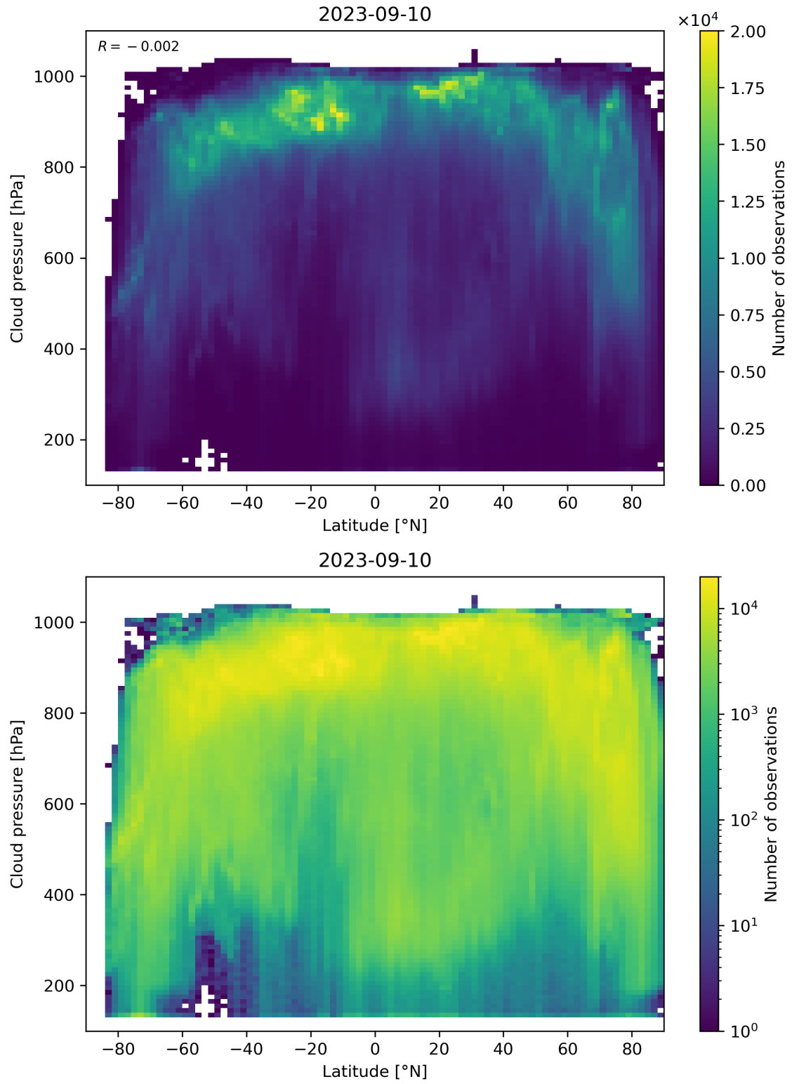
Figure 100: Scatter density plot of “Latitude” against “Cloud pressure” for 2023-09-10 to 2023-09-11.
