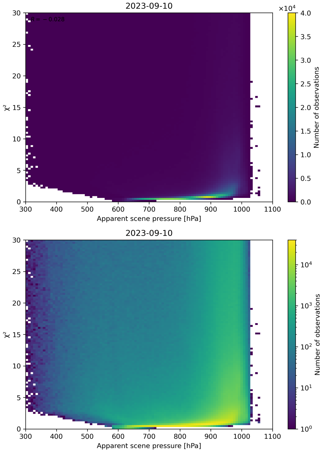
Figure 63: Scatter density plot of “Apparent scene pressure” against “ \chi^2 ” for 2023-09-10 to 2023-09-11.
