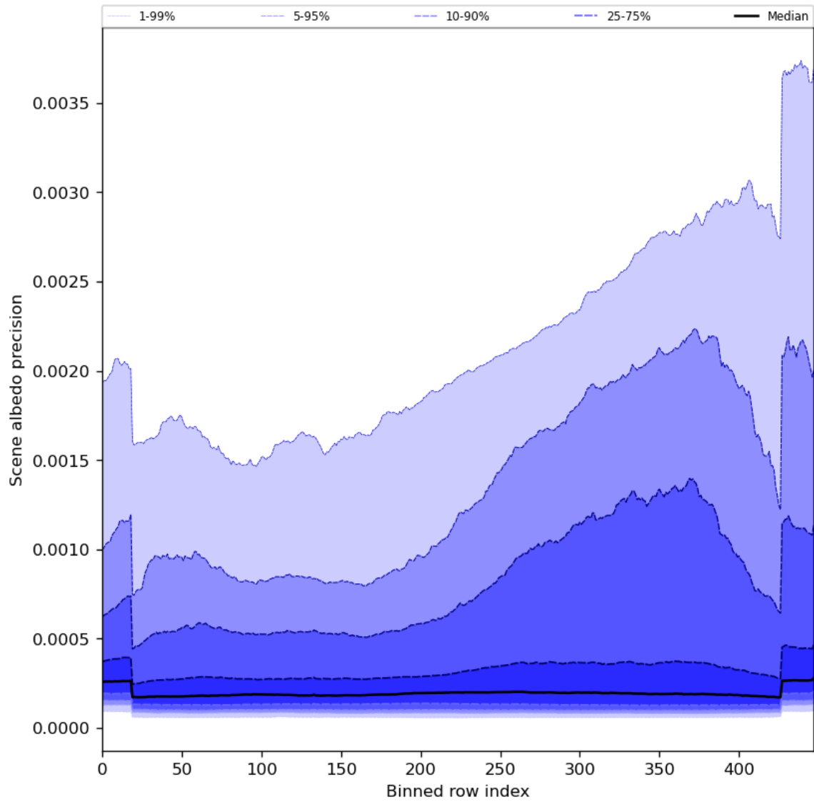
Figure 52: Along track statistics of “Scene albedo precision” for 2023-09-10 to 2023-09-11
