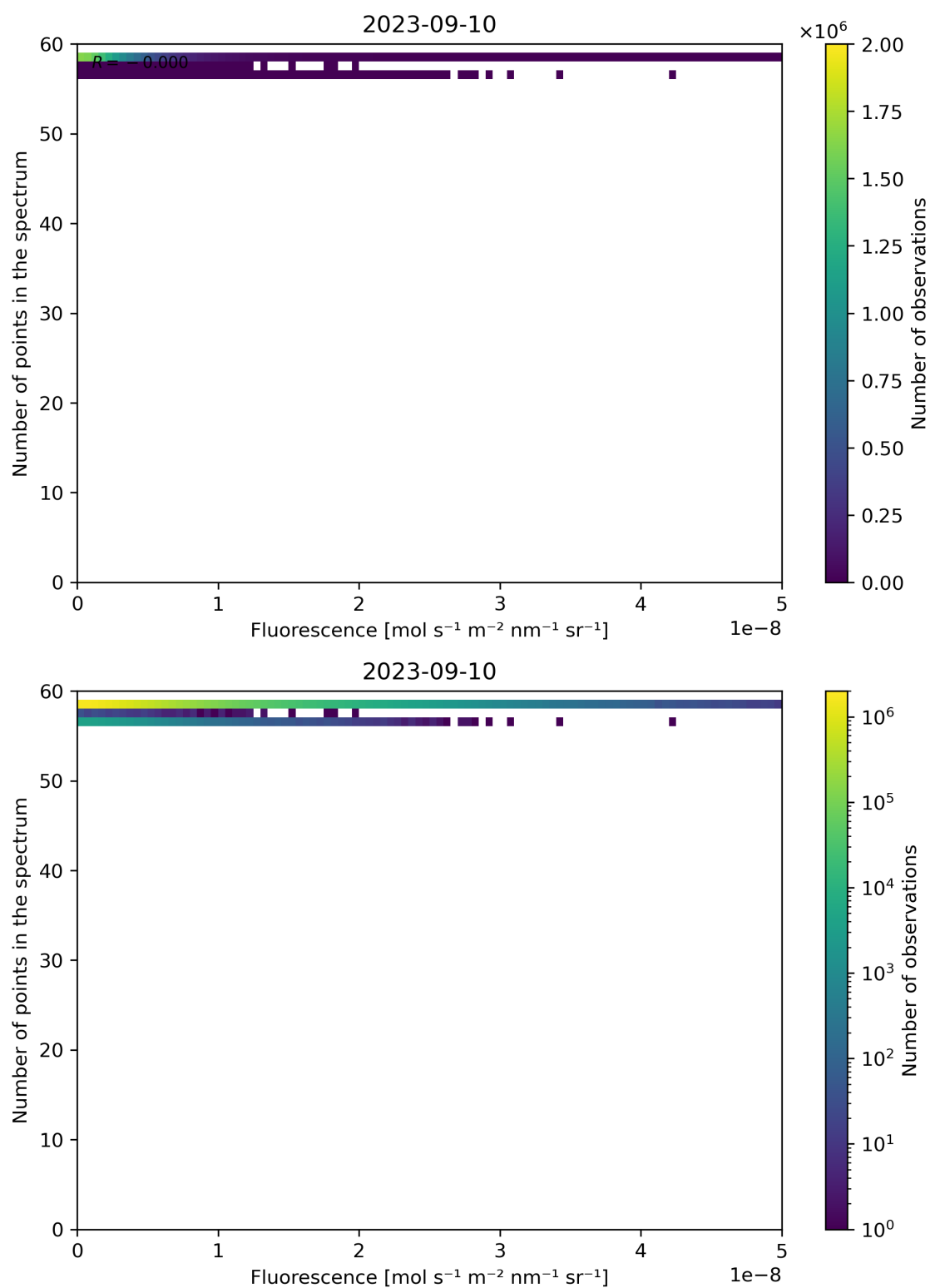
Figure 94: Scatter density plot of “Fluorescence” against “Number of points in the spectrum” for 2023-09-10 to 2023-09-11.
