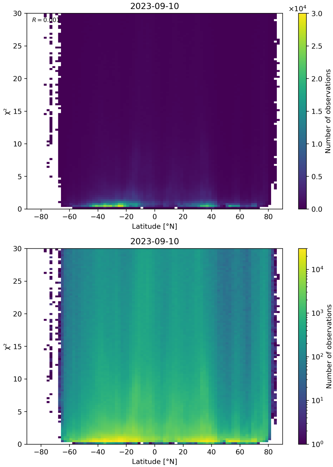
Figure 97: Scatter density plot of “Latitude” against “ \chi^2 ” for 2023-09-10 to 2023-09-11.
