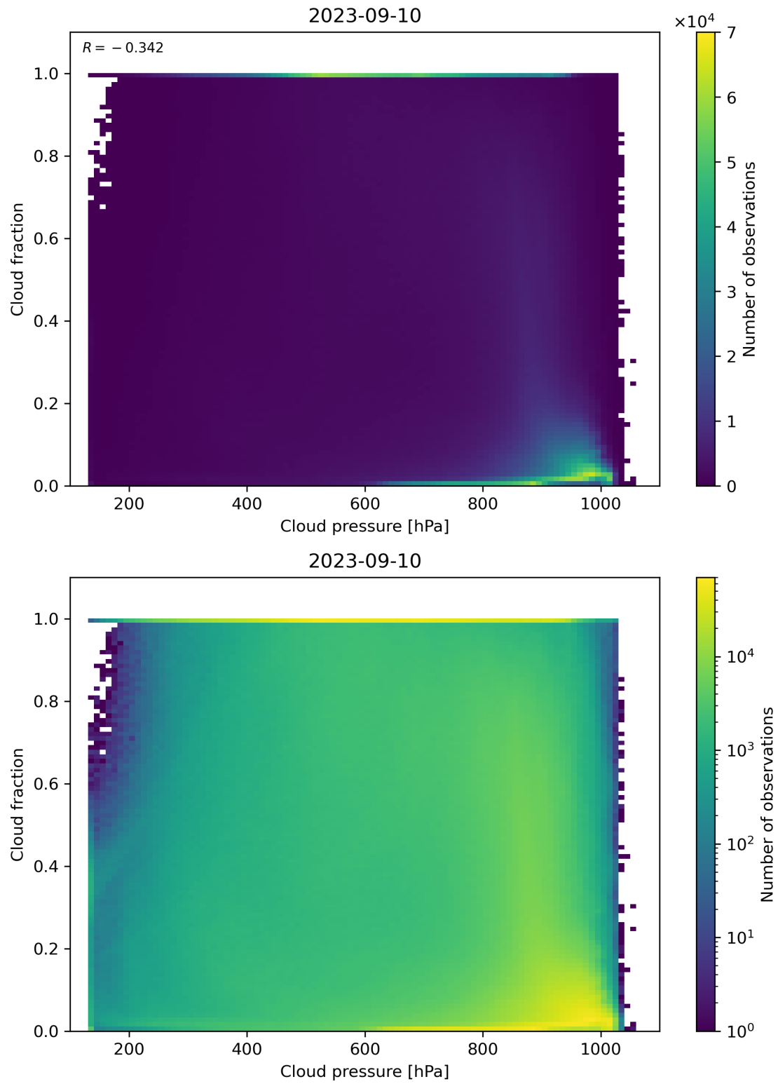
Figure 87: Scatter density plot of “Cloud pressure” against “Cloud fraction” for 2023-09-10 to 2023-09-11.
