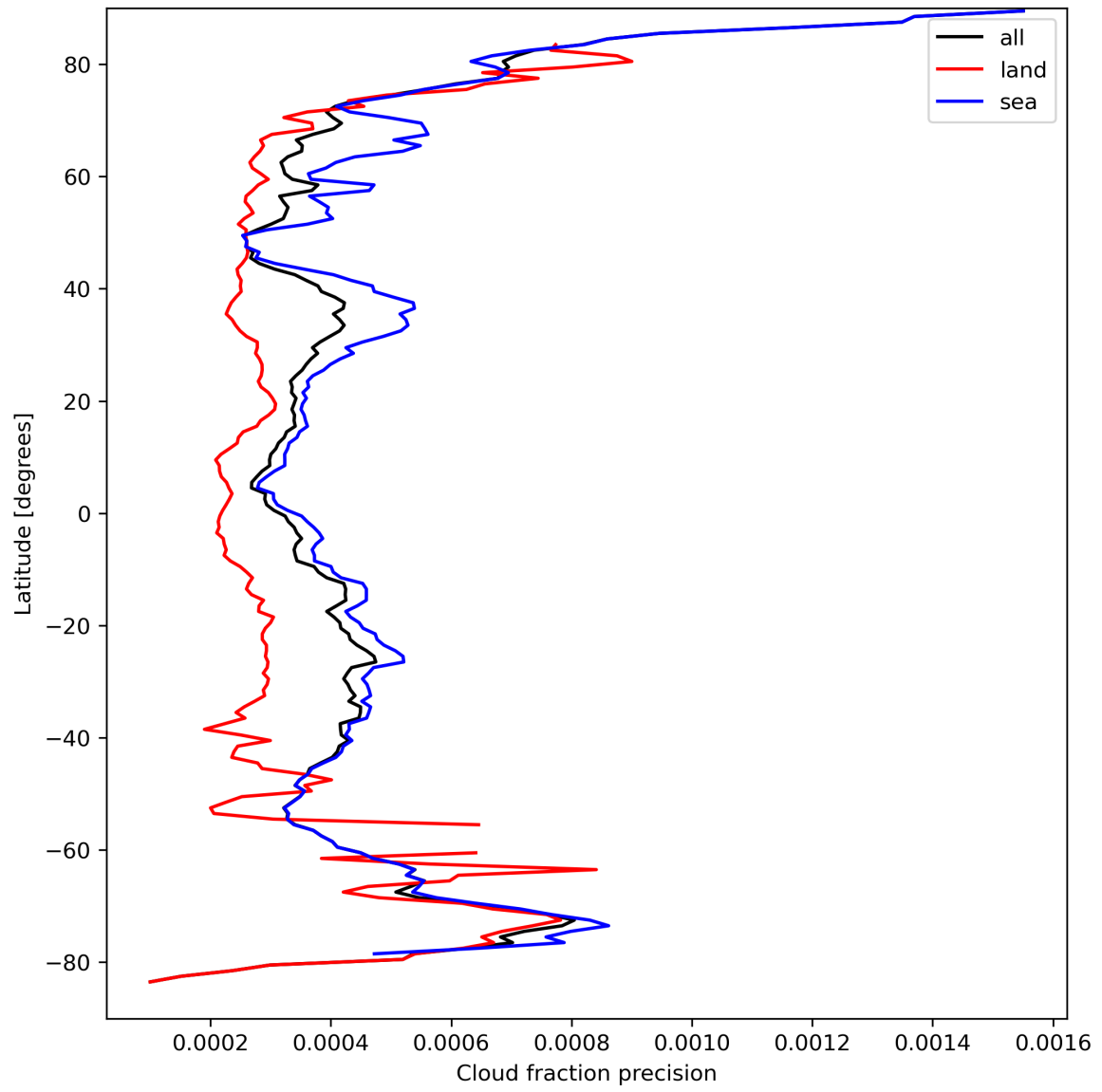
Figure 16: Zonal average of “Cloud fraction precision” for 2023-09-10 to 2023-09-11.
