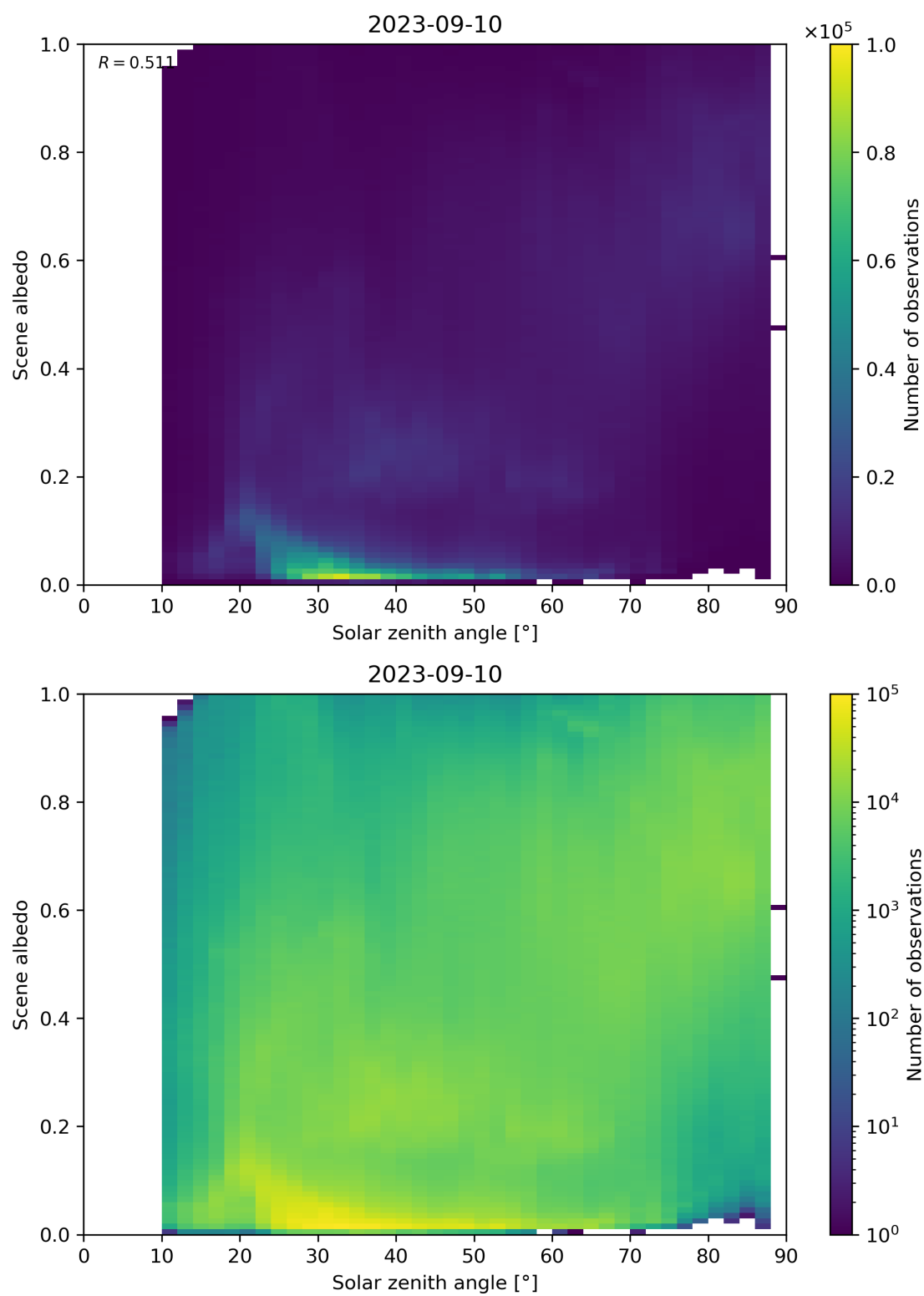
Figure 127: Scatter density plot of “Solar zenith angle” against “Scene albedo” for 2023-09-10 to 2023-09-11.
