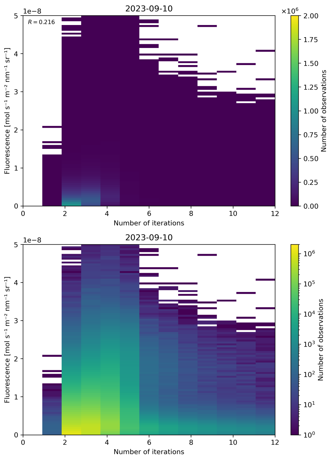
Figure 107: Scatter density plot of “Number of iterations” against “Fluorescence” for 2023-09-10 to 2023-09-11.
