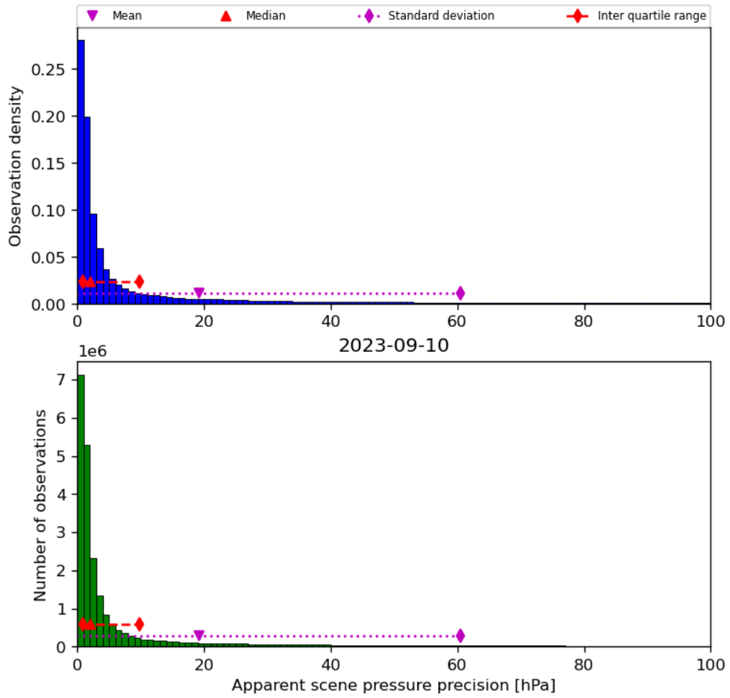
Figure 37: Histogram of “Apparent scene pressure precision” for 2023-09-10 to 2023-09-11
