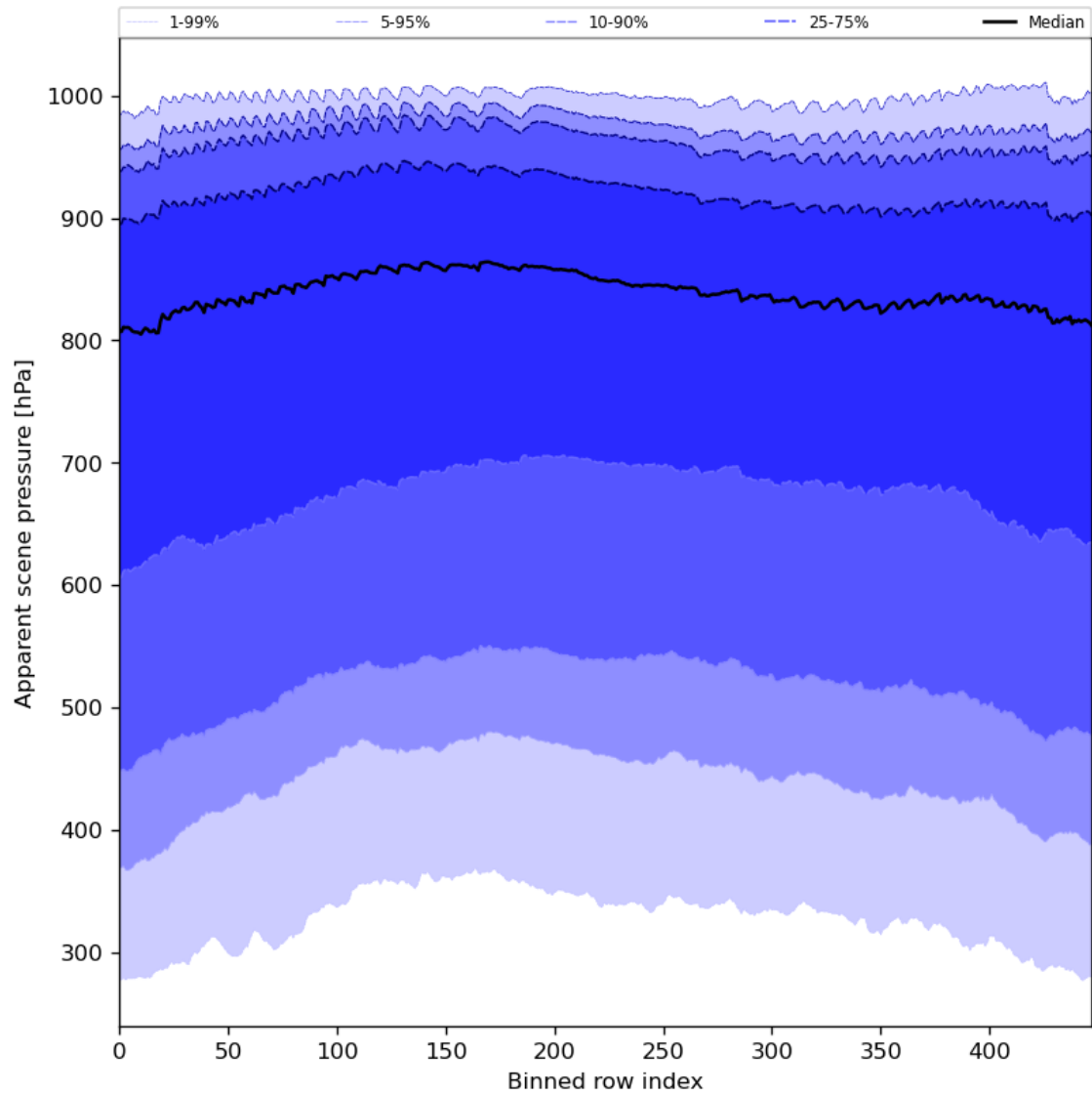
Figure 53: Along track statistics of “Apparent scene pressure” for 2023-09-10 to 2023-09-11
