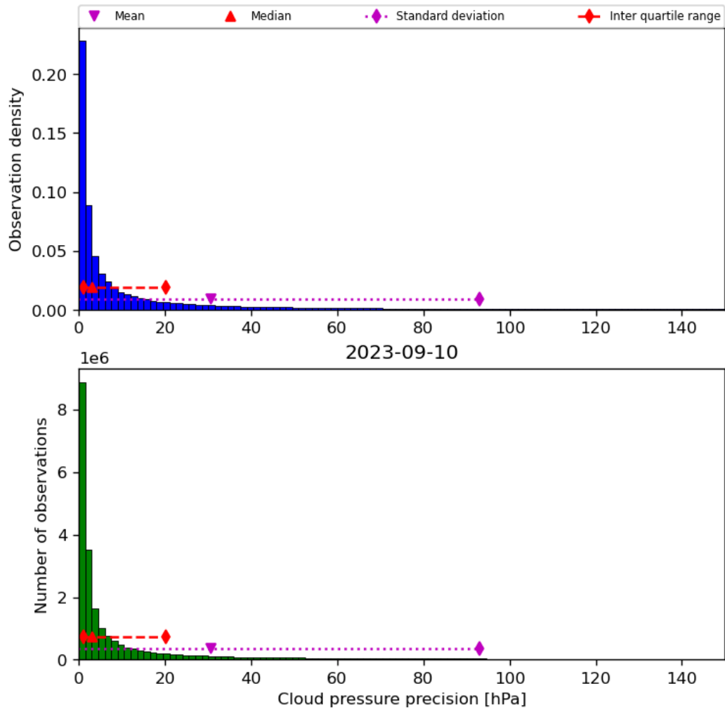
Figure 31: Histogram of “Cloud pressure precision” for 2023-09-10 to 2023-09-11
