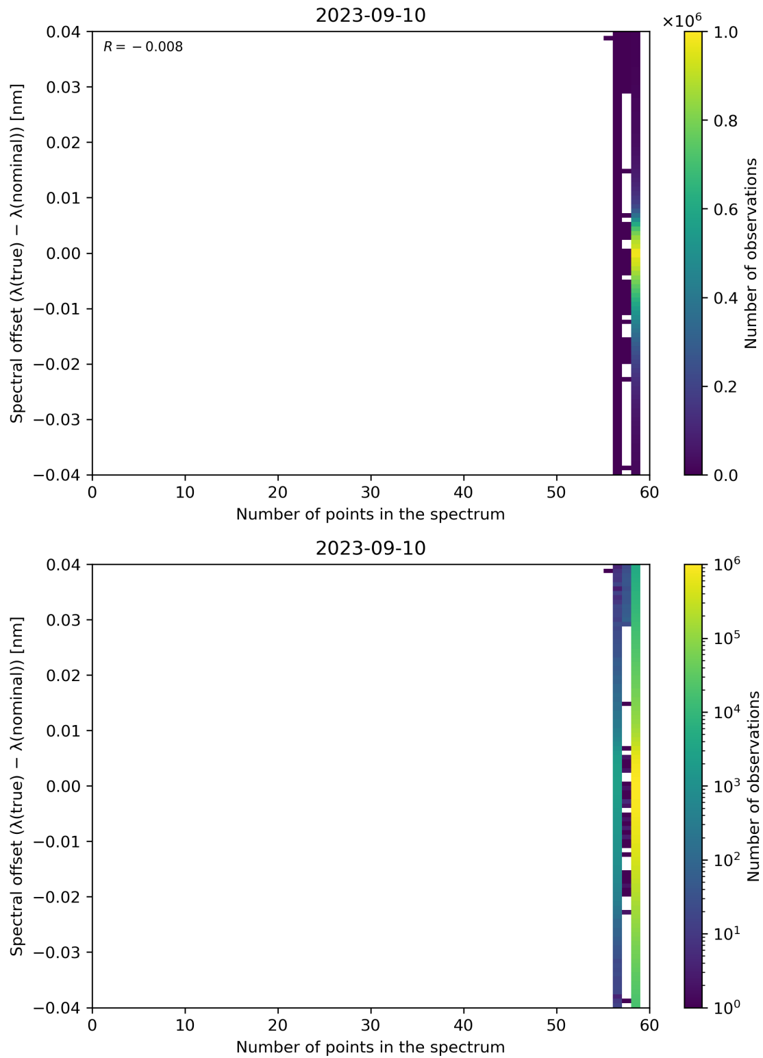
Figure 110: Scatter density plot of “Number of points in the spectrum” against “Spectral offset ( \lambda(\text{true}) - \lambda(\text{nominal}) )” for 2023-09-10 to 2023-09-11.
