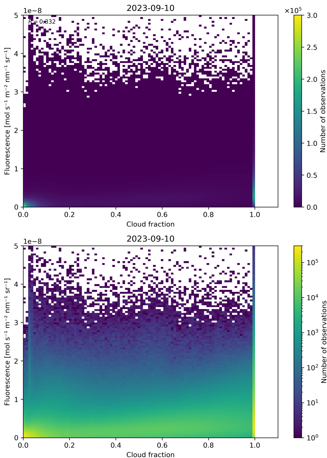
Figure 79: Scatter density plot of “Cloud fraction” against “Fluorescence” for 2023-09-10 to 2023-09-11.
