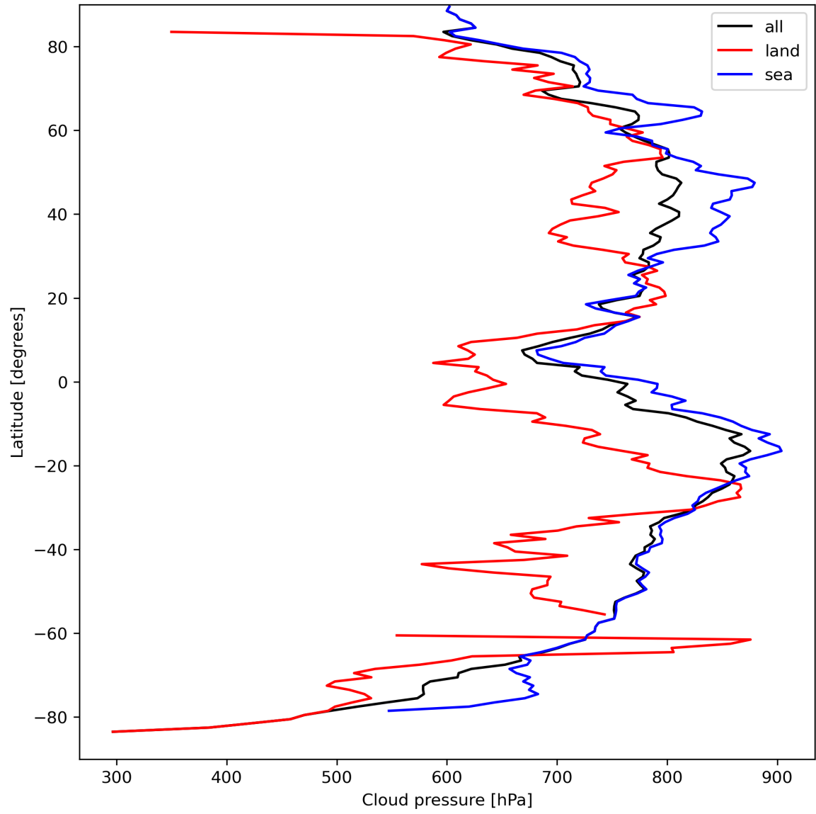
Figure 13: Zonal average of “Cloud pressure” for 2023-09-10 to 2023-09-11.
