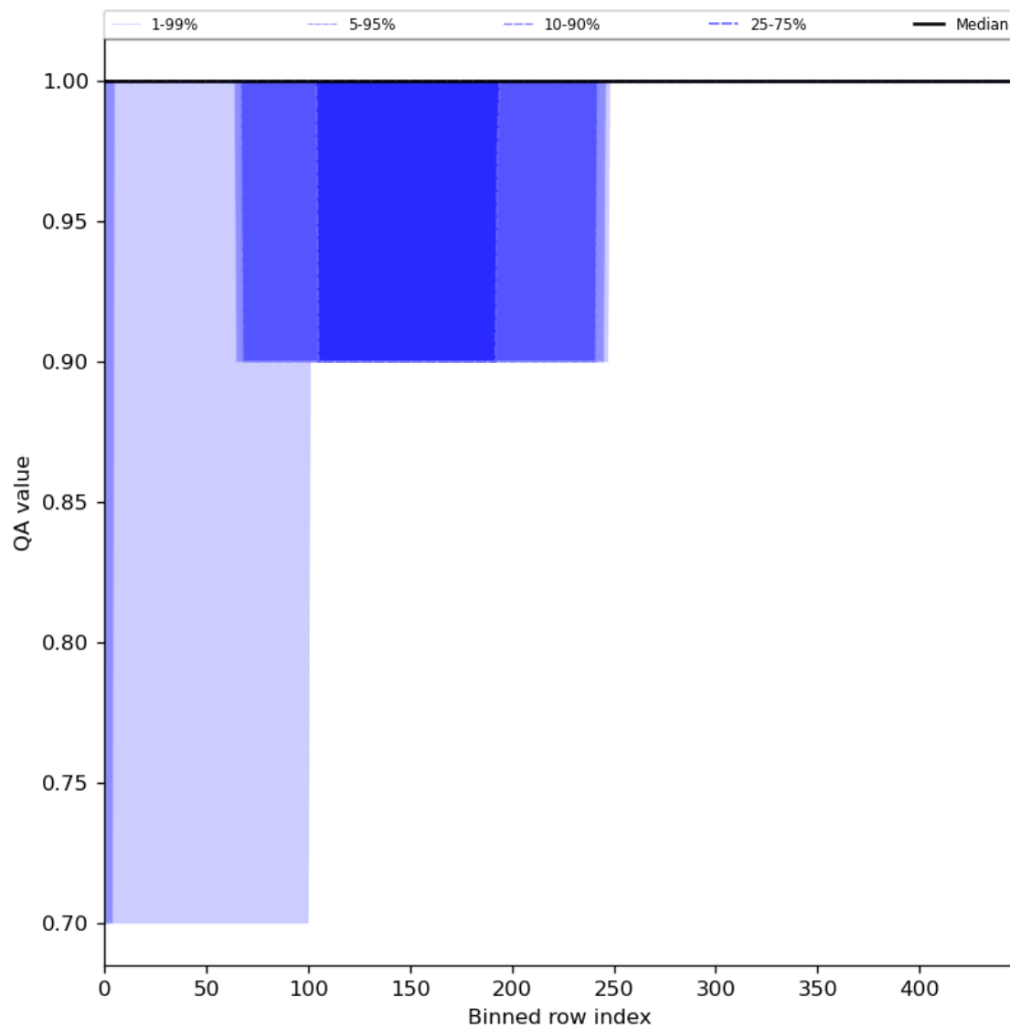
Figure 46: Along track statistics of “QA value” for 2023-09-10 to 2023-09-11
