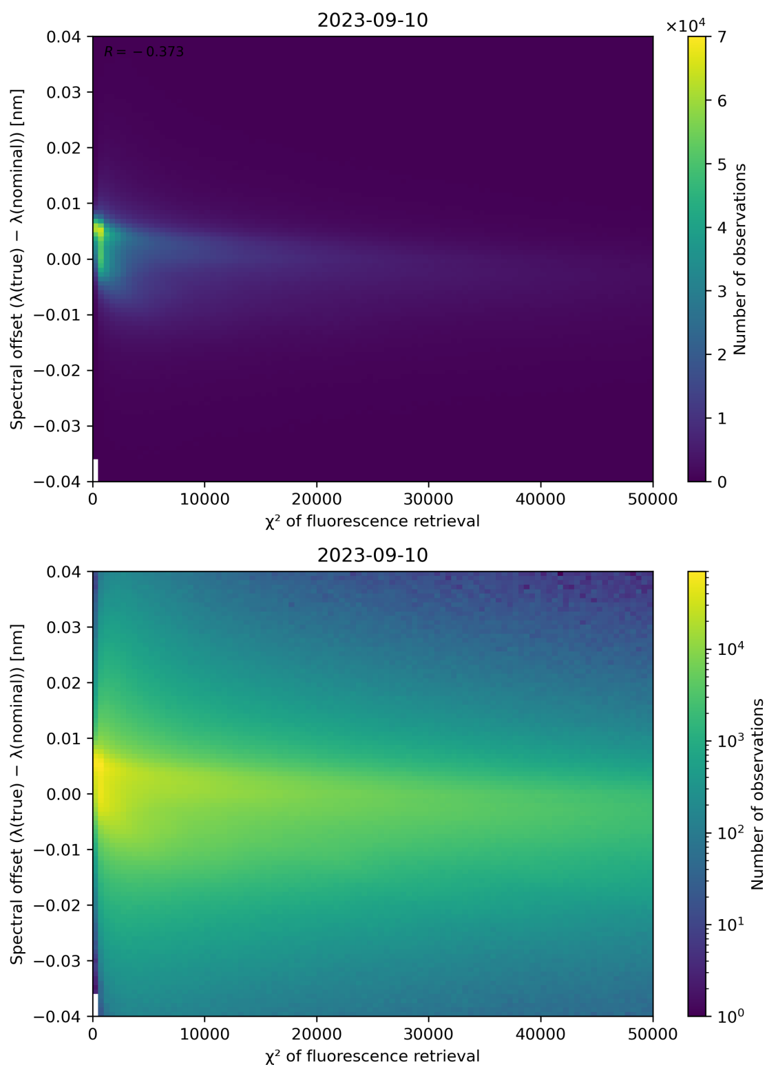
Figure 72: Scatter density plot of " \chi^2 of fluorescence retrieval" against "Spectral offset ( \lambda(\text{true}) - \lambda(\text{nominal}) )" for 2023-09-10 to 2023-09-11.
