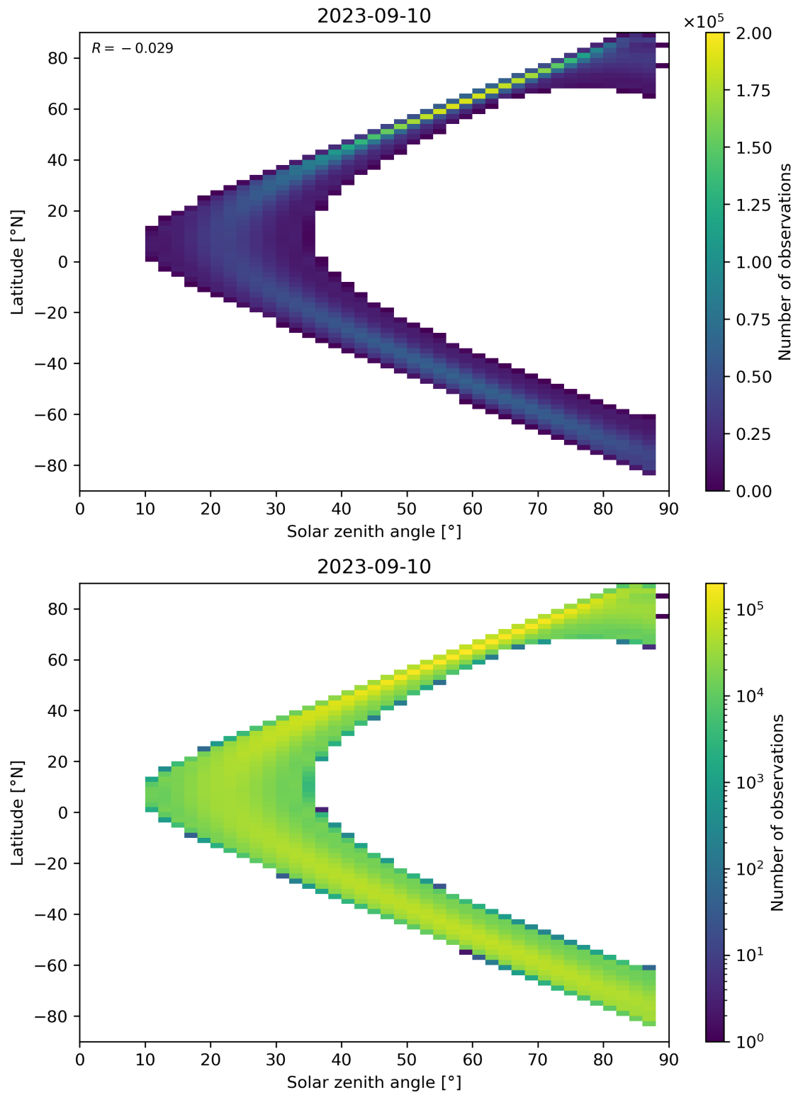
Figure 124: Scatter density plot of “Solar zenith angle” against “Latitude” for 2023-09-10 to 2023-09-11.
