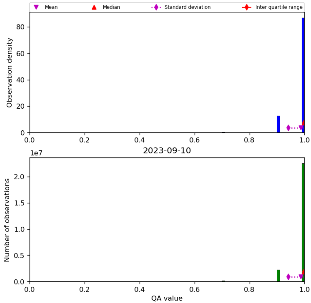
Figure 29: Histogram of “QA value” for 2023-09-10 to 2023-09-11
