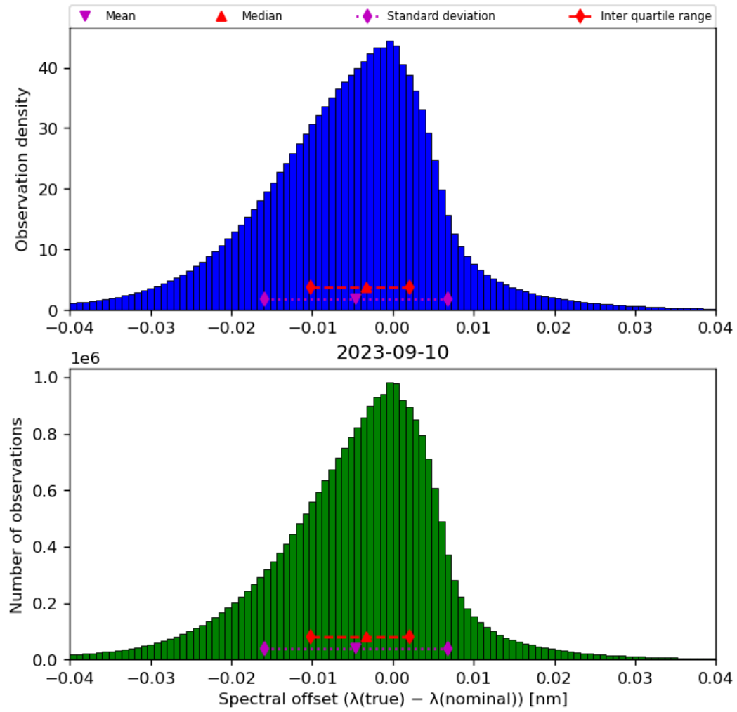
Figure 45: Histogram of “Spectral offset ( \lambda(\text{true}) - \lambda(\text{nominal}) )” for 2023-09-10 to 2023-09-11
