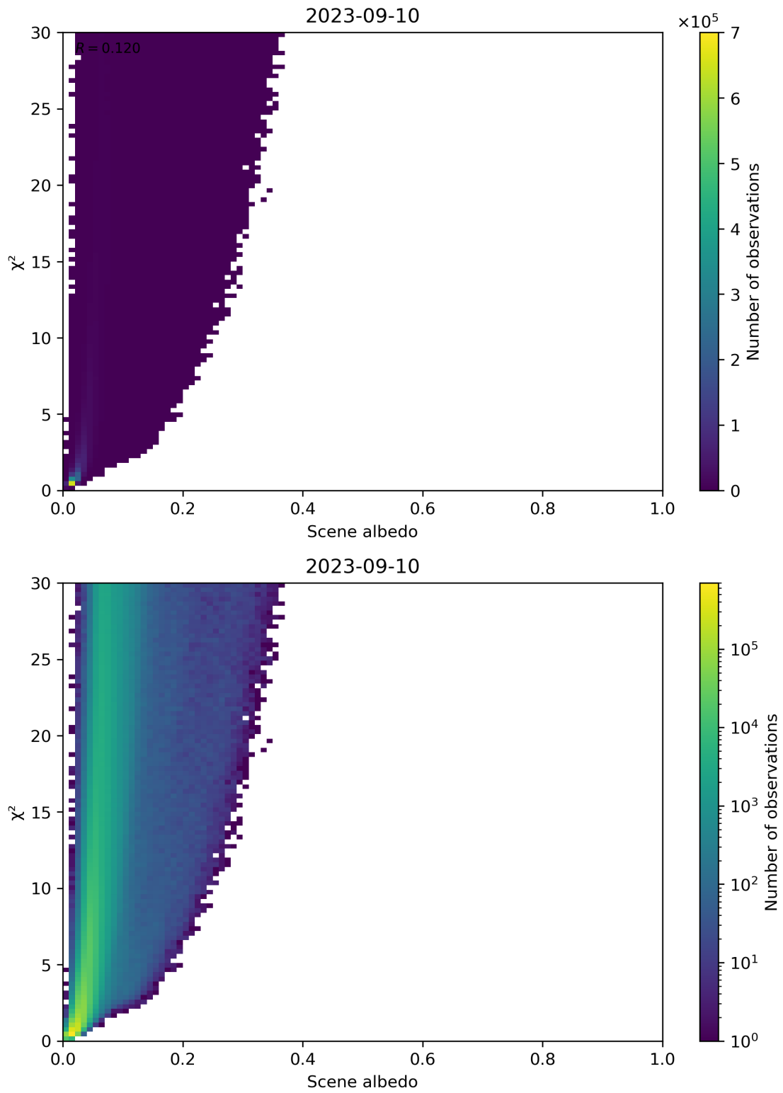
Figure 112: Scatter density plot of “Scene albedo” against “ \chi^2 ” for 2023-09-10 to 2023-09-11.
