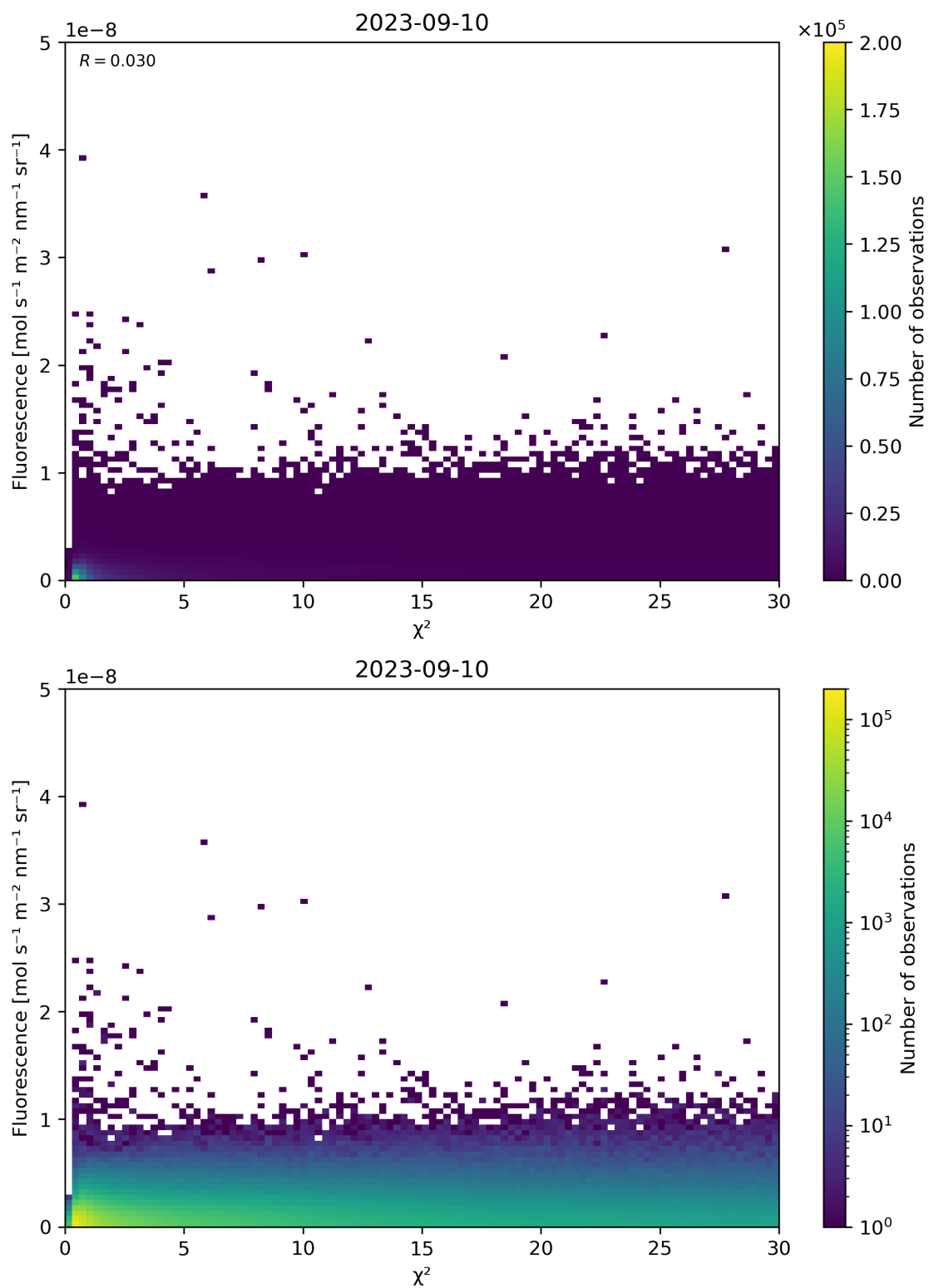
Figure 70: Scatter density plot of “ \chi^2 ” against “Fluorescence” for 2023-09-10 to 2023-09-11.
