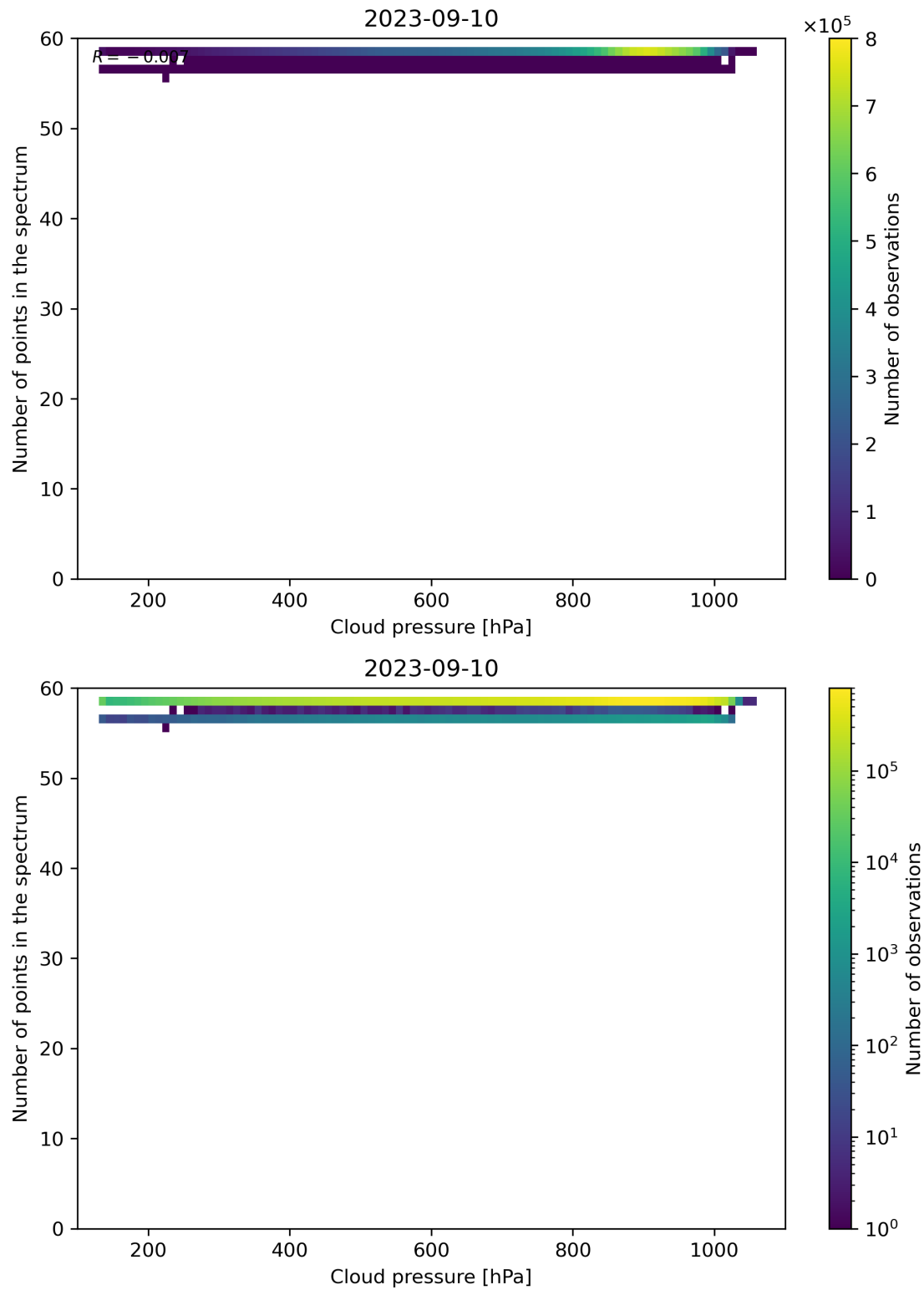
Figure 90: Scatter density plot of “Cloud pressure” against “Number of points in the spectrum” for 2023-09-10 to 2023-09-11.
