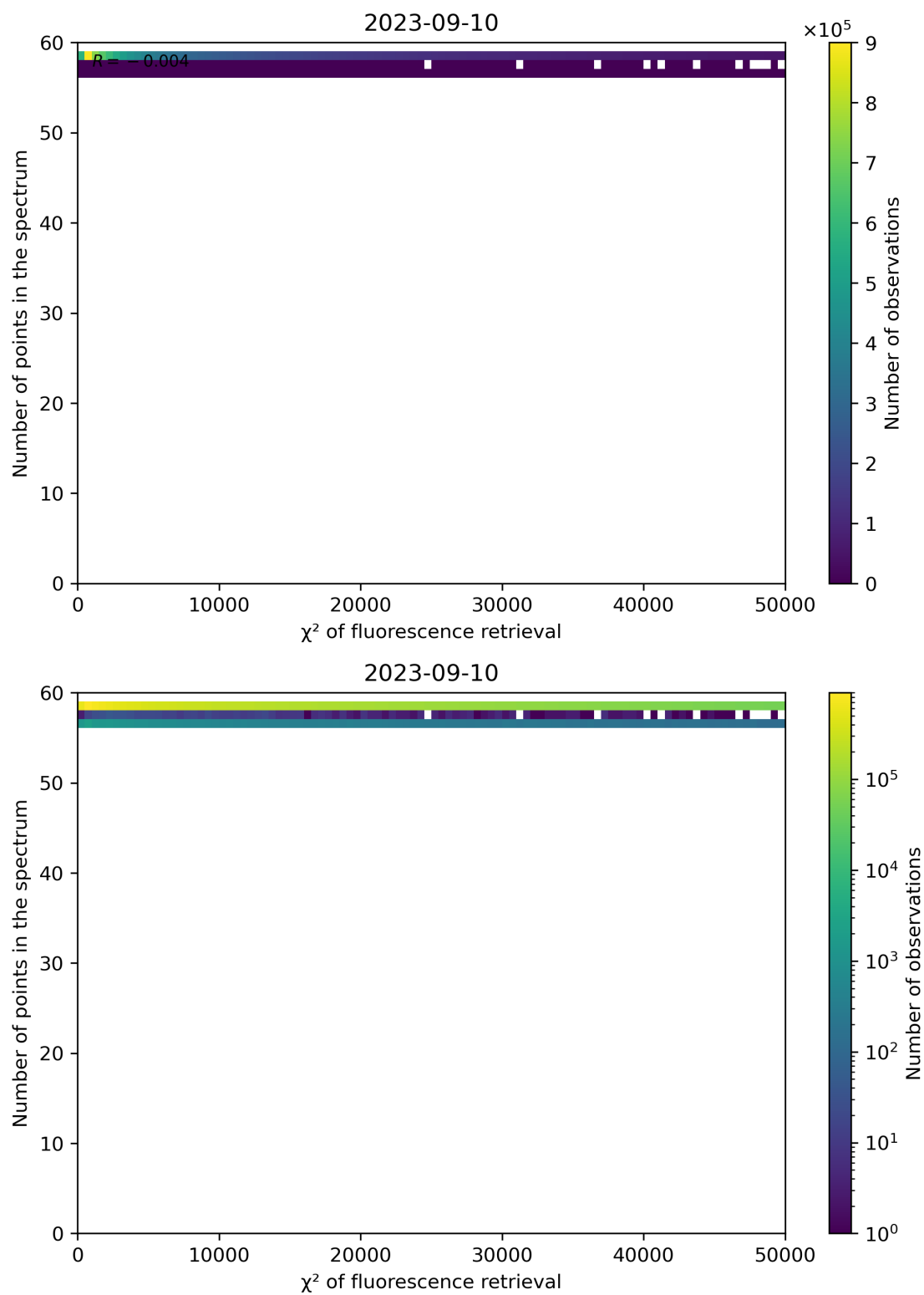
Figure 71: Scatter density plot of " \chi^2 of fluorescence retrieval" against "Number of points in the spectrum" for 2023-09-10 to 2023-09-11.
