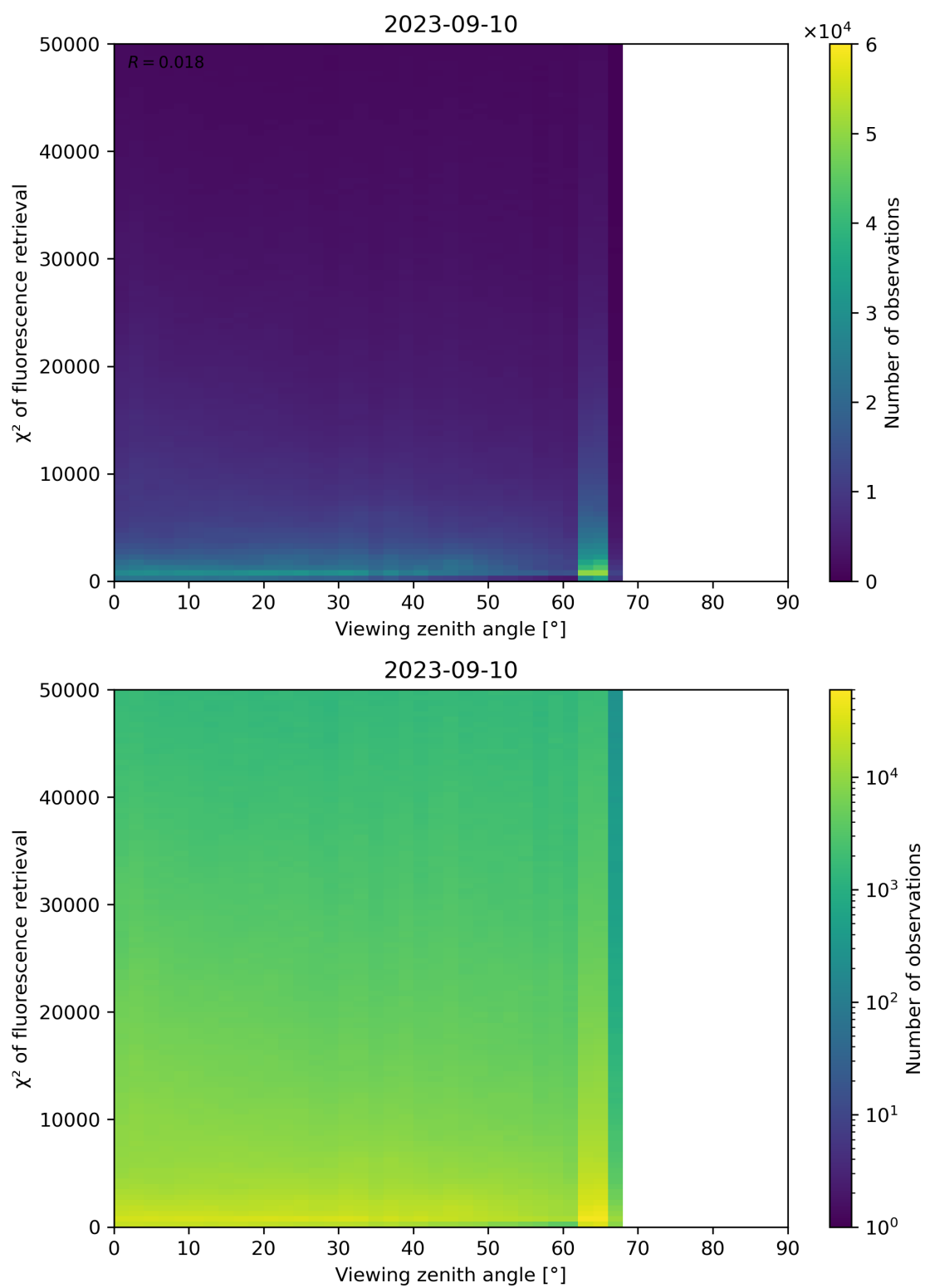
Figure 131: Scatter density plot of “Viewing zenith angle” against “ \chi^2 of fluorescence retrieval” for 2023-09-10 to 2023-09-11.
