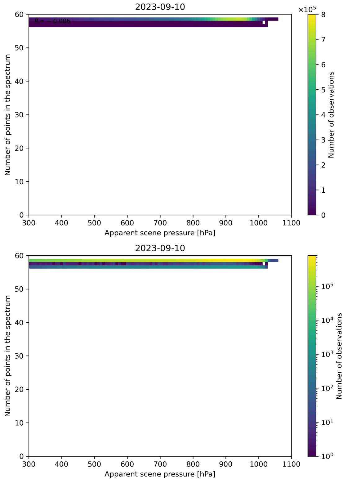
Figure 67: Scatter density plot of “Apparent scene pressure” against “Number of points in the spectrum” for 2023-09-10 to 2023-09-11.
