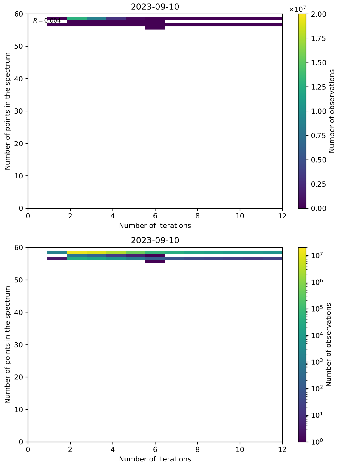
Figure 108: Scatter density plot of “Number of iterations” against “Number of points in the spectrum” for 2023-09-10 to 2023-09-11.
