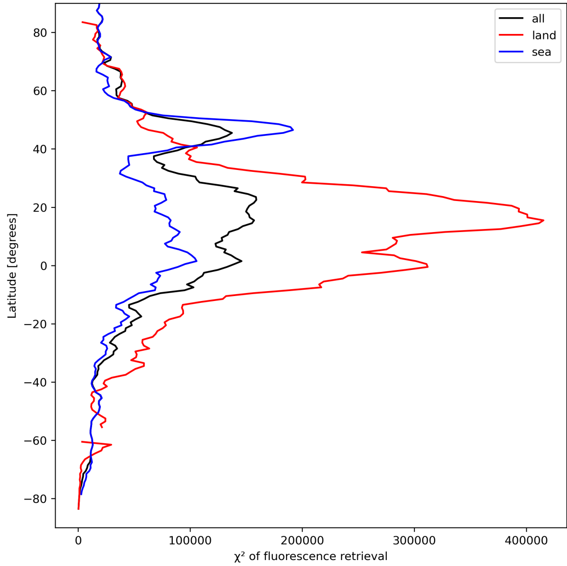
Figure 25: Zonal average of “ \chi^2 of fluorescence retrieval” for 2023-09-10 to 2023-09-11.
