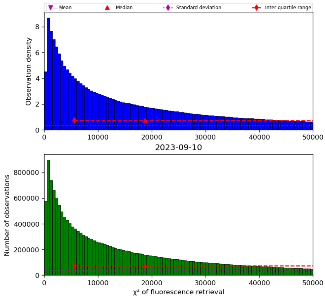
Figure 42: Histogram of “ \chi^2 of fluorescence retrieval” for 2023-09-10 to 2023-09-11
