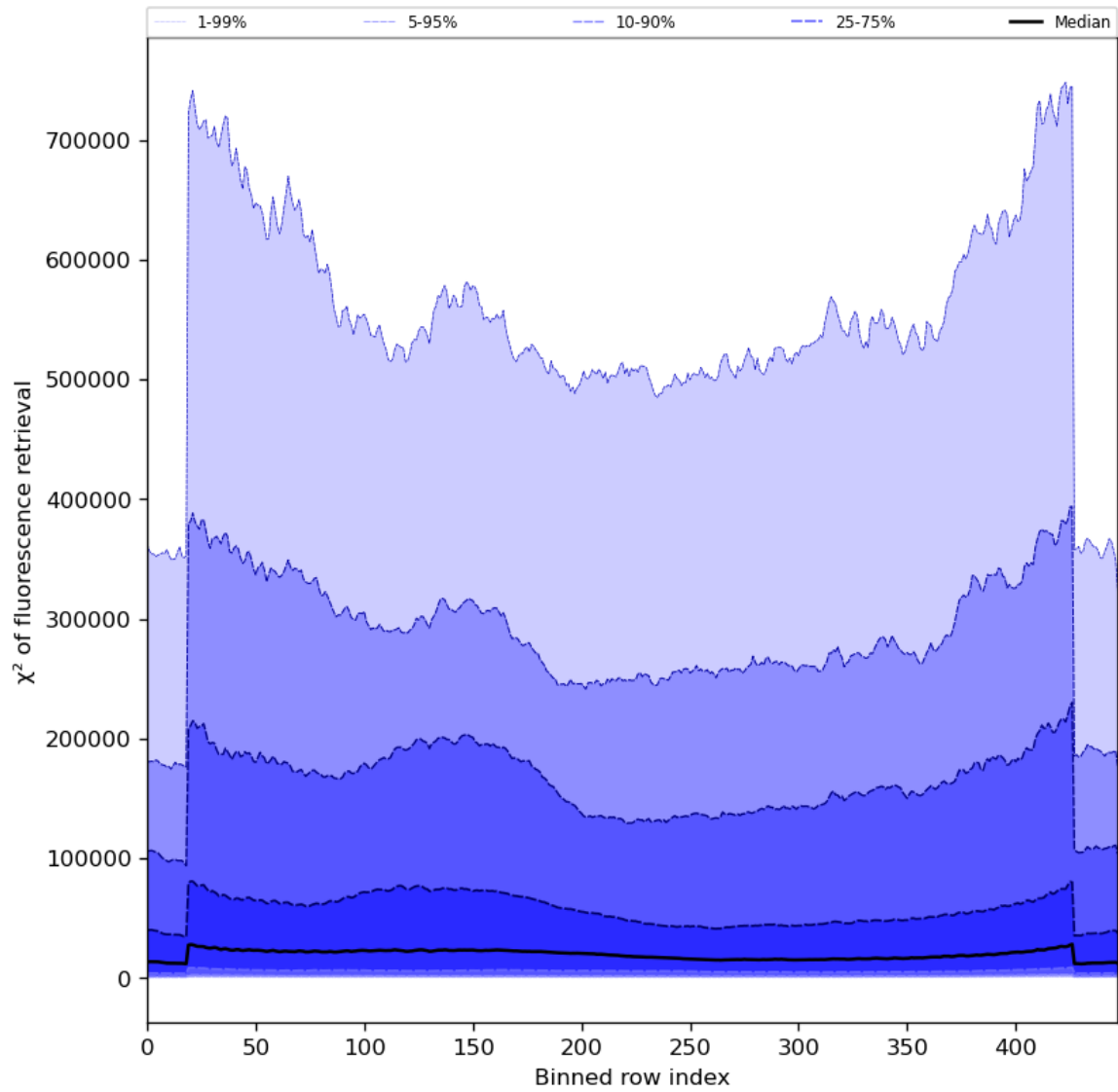
Figure 59: Along track statistics of “ \chi^2 of fluorescence retrieval” for 2023-09-10 to 2023-09-11
