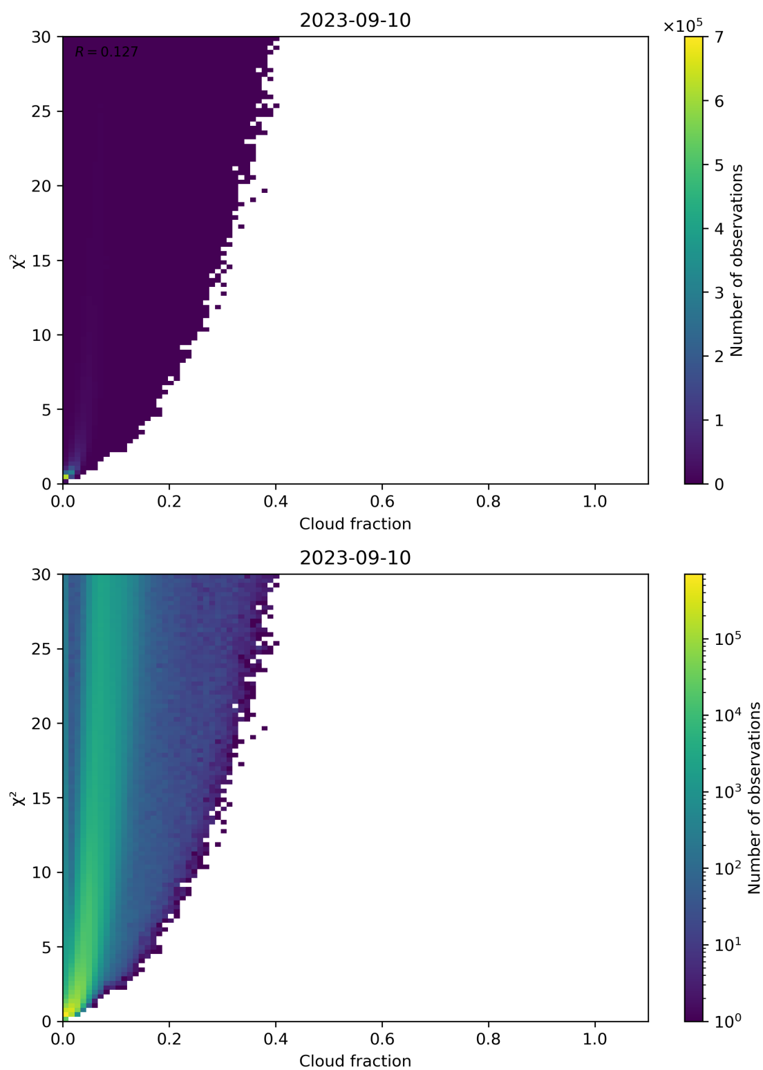
Figure 77: Scatter density plot of “Cloud fraction” against “ \chi^2 ” for 2023-09-10 to 2023-09-11.
