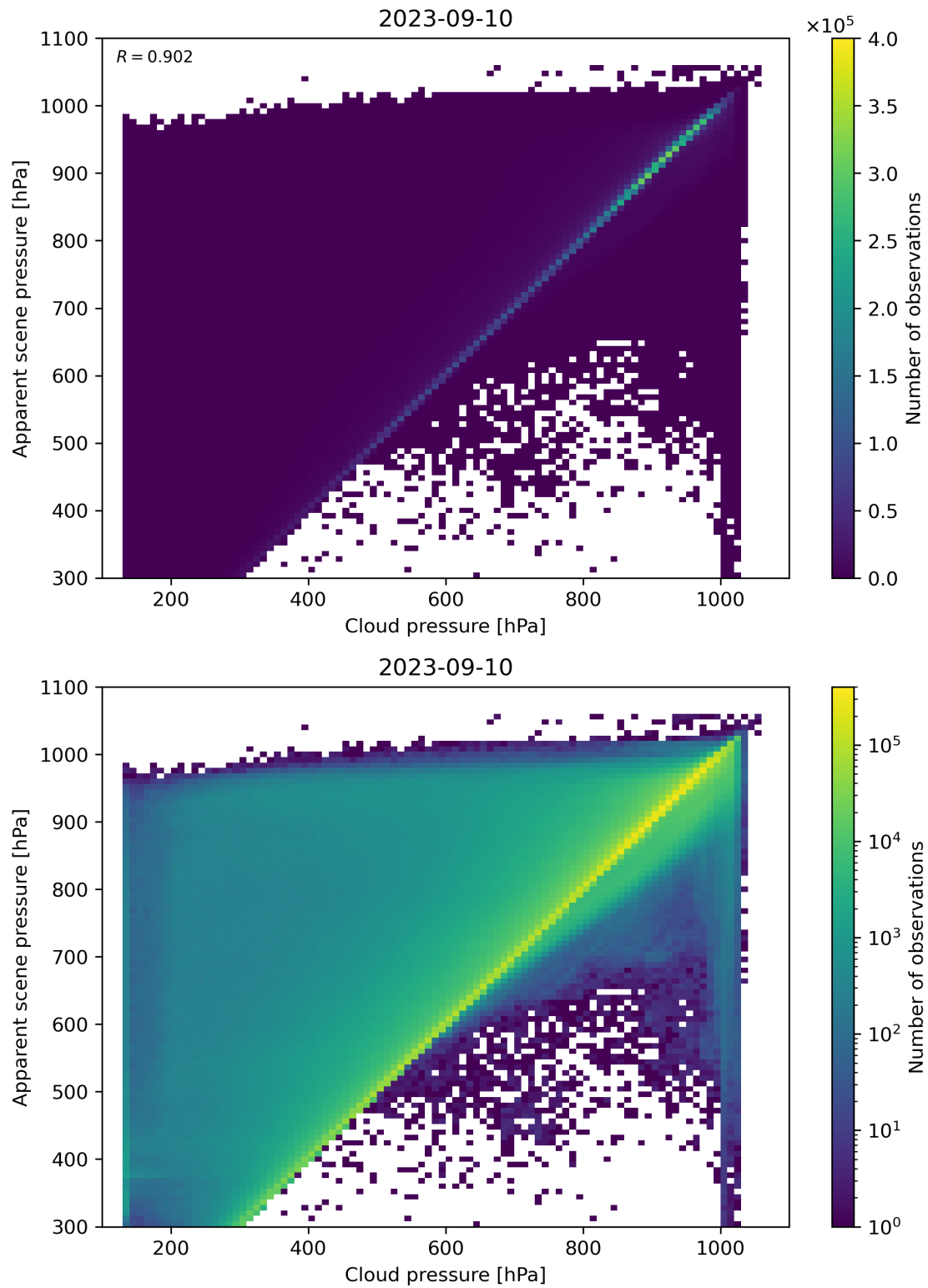
Figure 84: Scatter density plot of “Cloud pressure” against “Apparent scene pressure” for 2023-09-10 to 2023-09-11.
