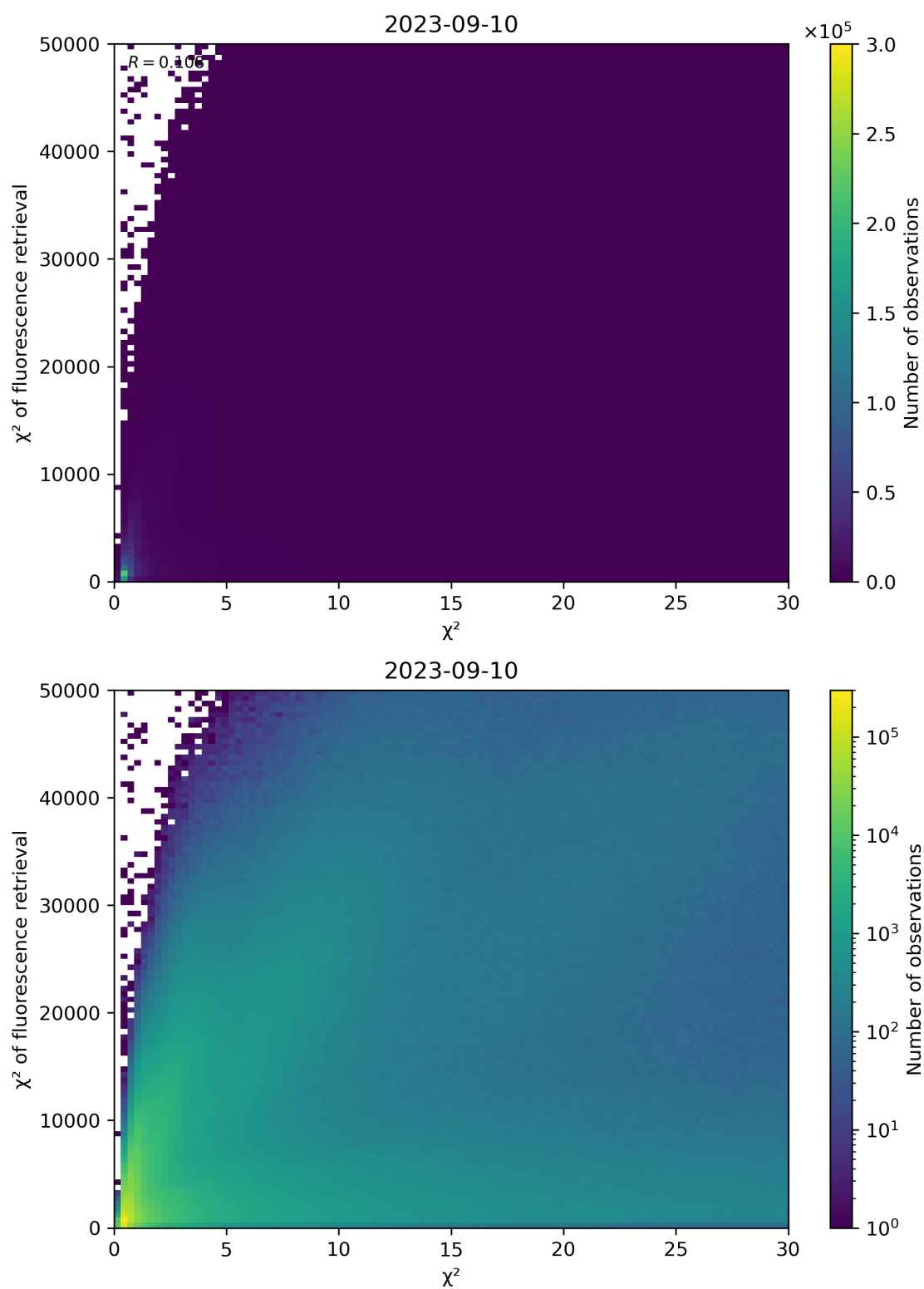
Figure 69: Scatter density plot of “ \chi^2 ” against “ \chi^2 of fluorescence retrieval” for 2023-09-10 to 2023-09-11.
