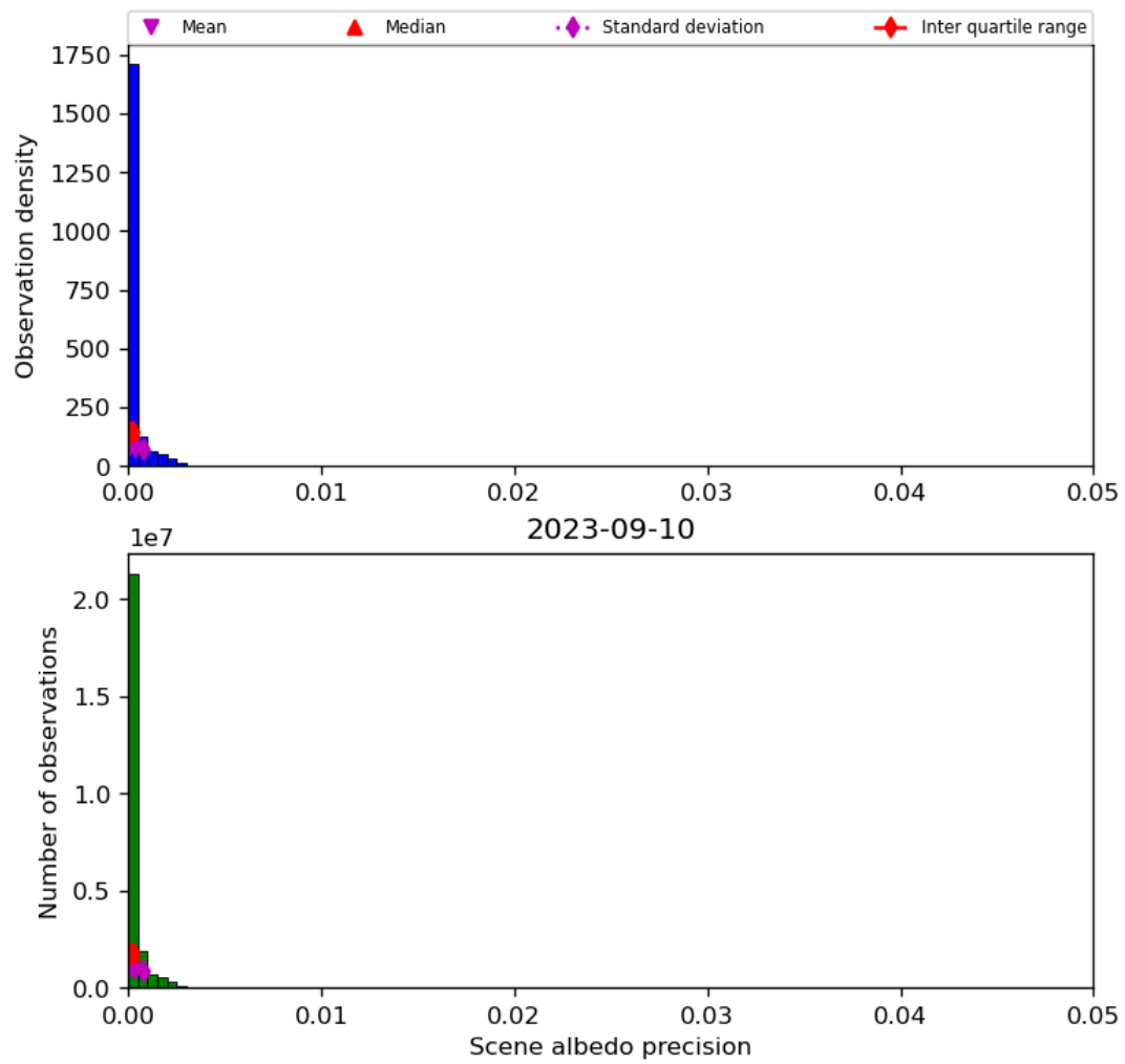
Figure 35: Histogram of “Scene albedo precision” for 2023-09-10 to 2023-09-11
