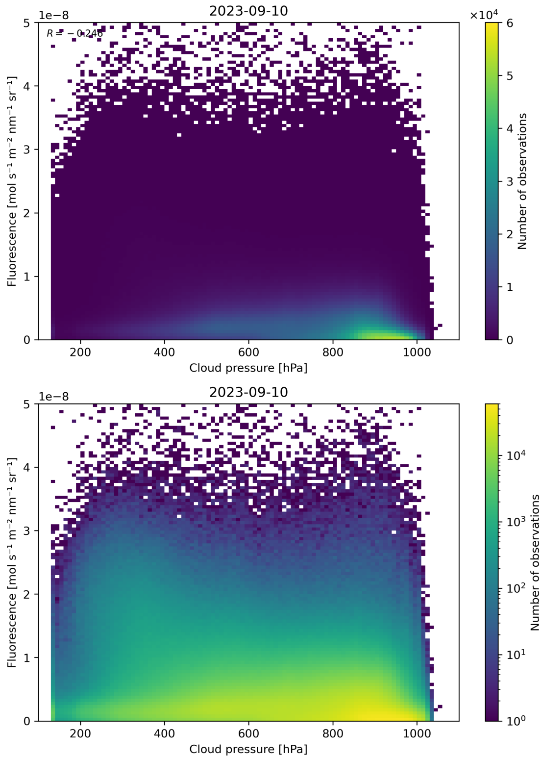
Figure 88: Scatter density plot of “Cloud pressure” against “Fluorescence” for 2023-09-10 to 2023-09-11.
