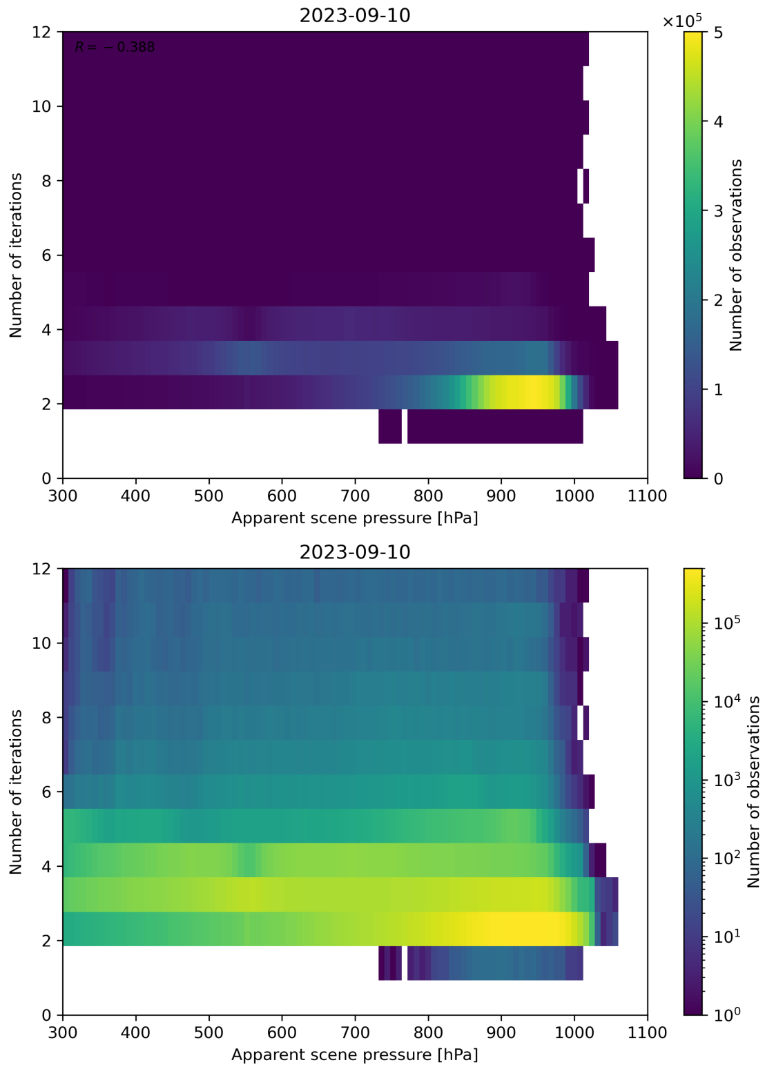
Figure 66: Scatter density plot of “Apparent scene pressure” against “Number of iterations” for 2023-09-10 to 2023-09-11.
