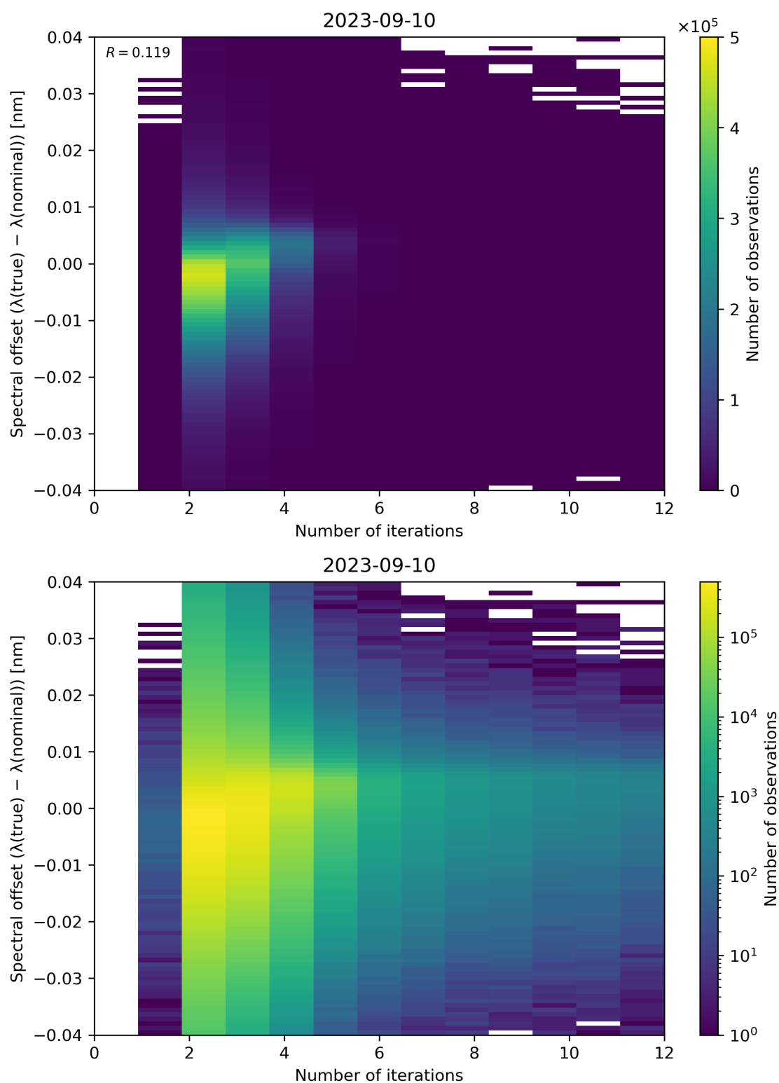
Figure 109: Scatter density plot of “Number of iterations” against “Spectral offset ( \lambda(\text{true}) - \lambda(\text{nominal}) )” for 2023-09-10 to 2023-09-11.
