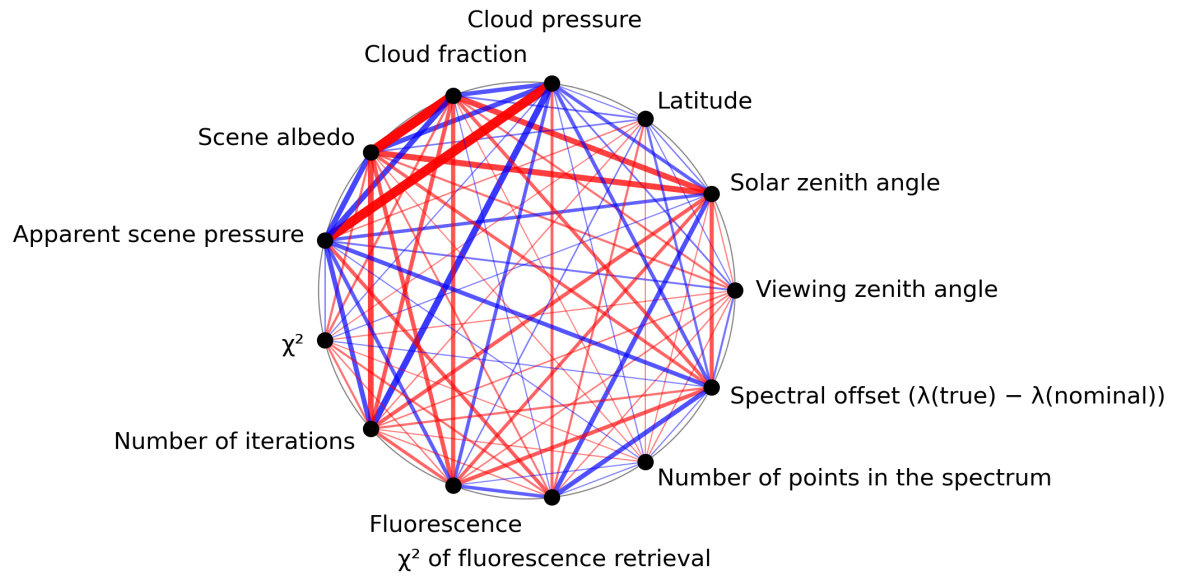
Figure 1: Map of correlation graph for 2023-09-10 to 2023-09-11.
