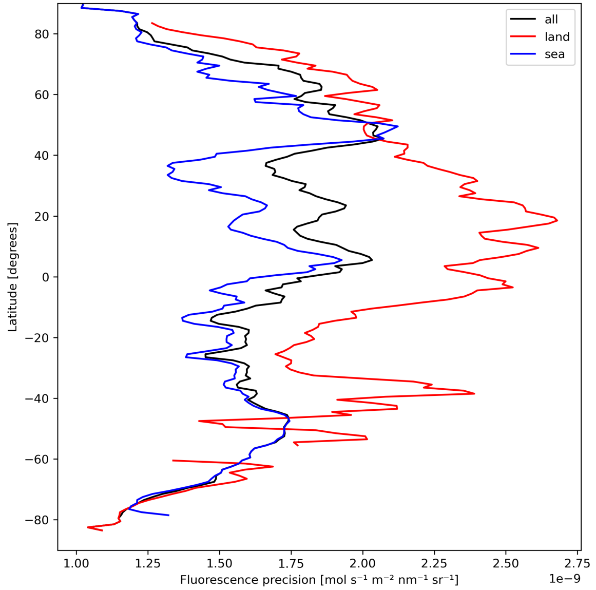
Figure 24: Zonal average of “Fluorescence precision” for 2023-09-10 to 2023-09-11.
