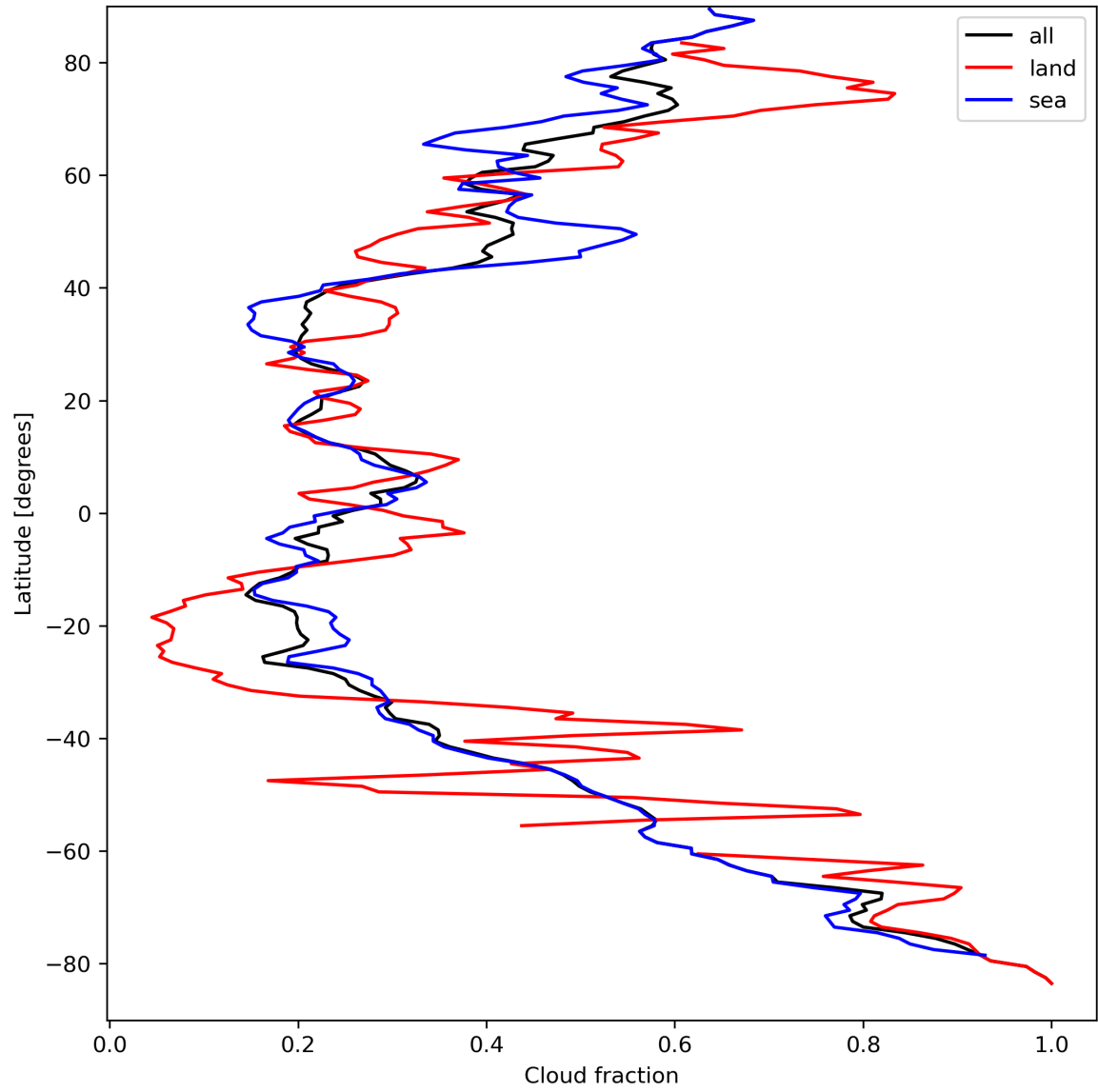
Figure 15: Zonal average of “Cloud fraction” for 2023-09-10 to 2023-09-11.
