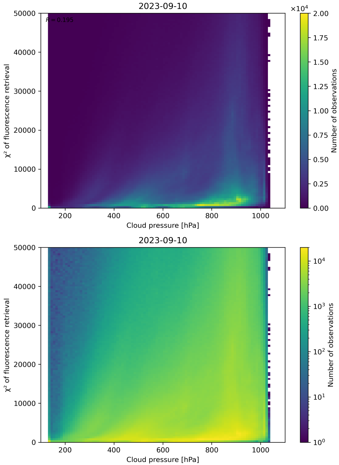
Figure 86: Scatter density plot of “Cloud pressure” against “ \chi^2 of fluorescence retrieval” for 2023-09-10 to 2023-09-11.
