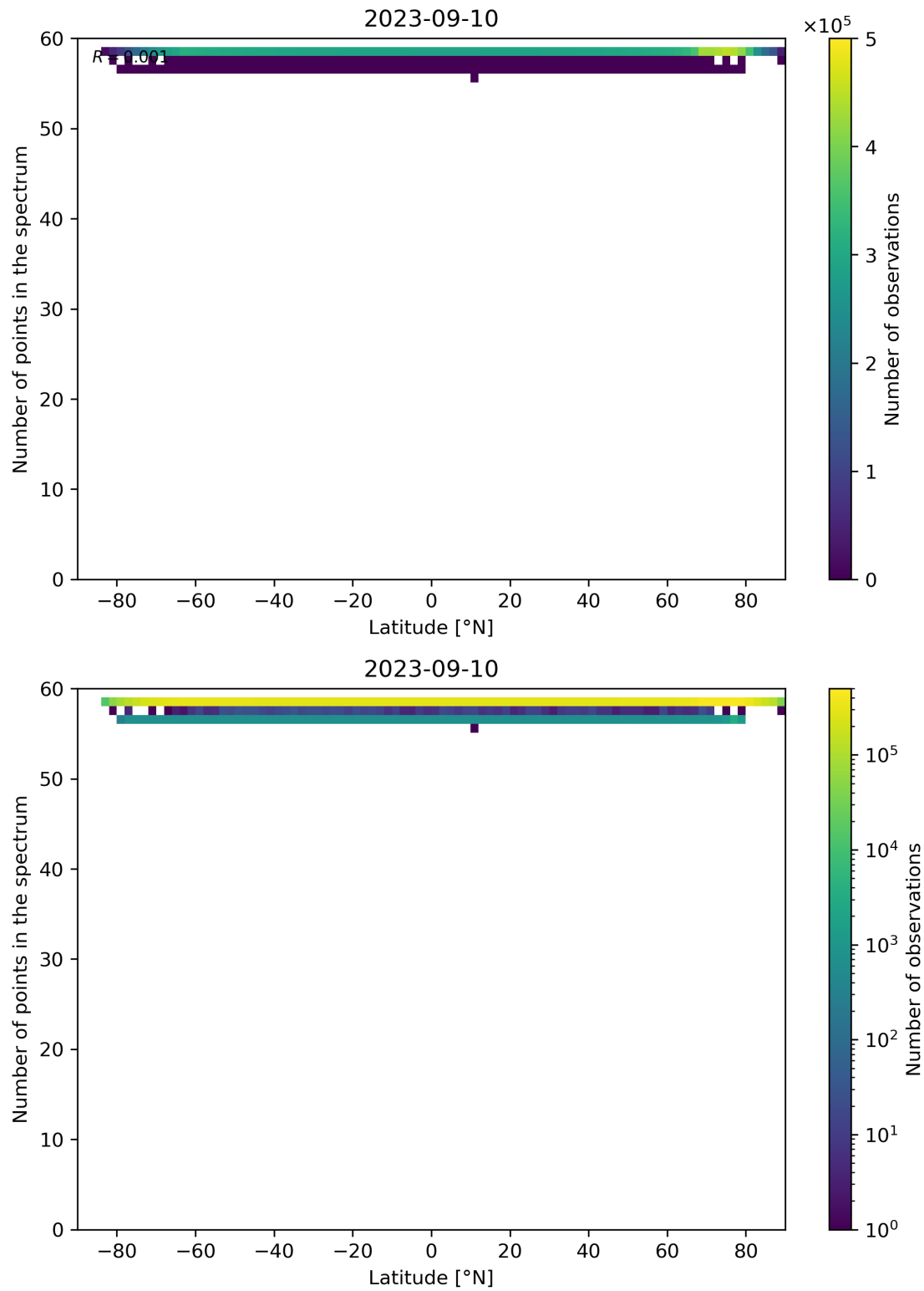
Figure 103: Scatter density plot of “Latitude” against “Number of points in the spectrum” for 2023-09-10 to 2023-09-11.
