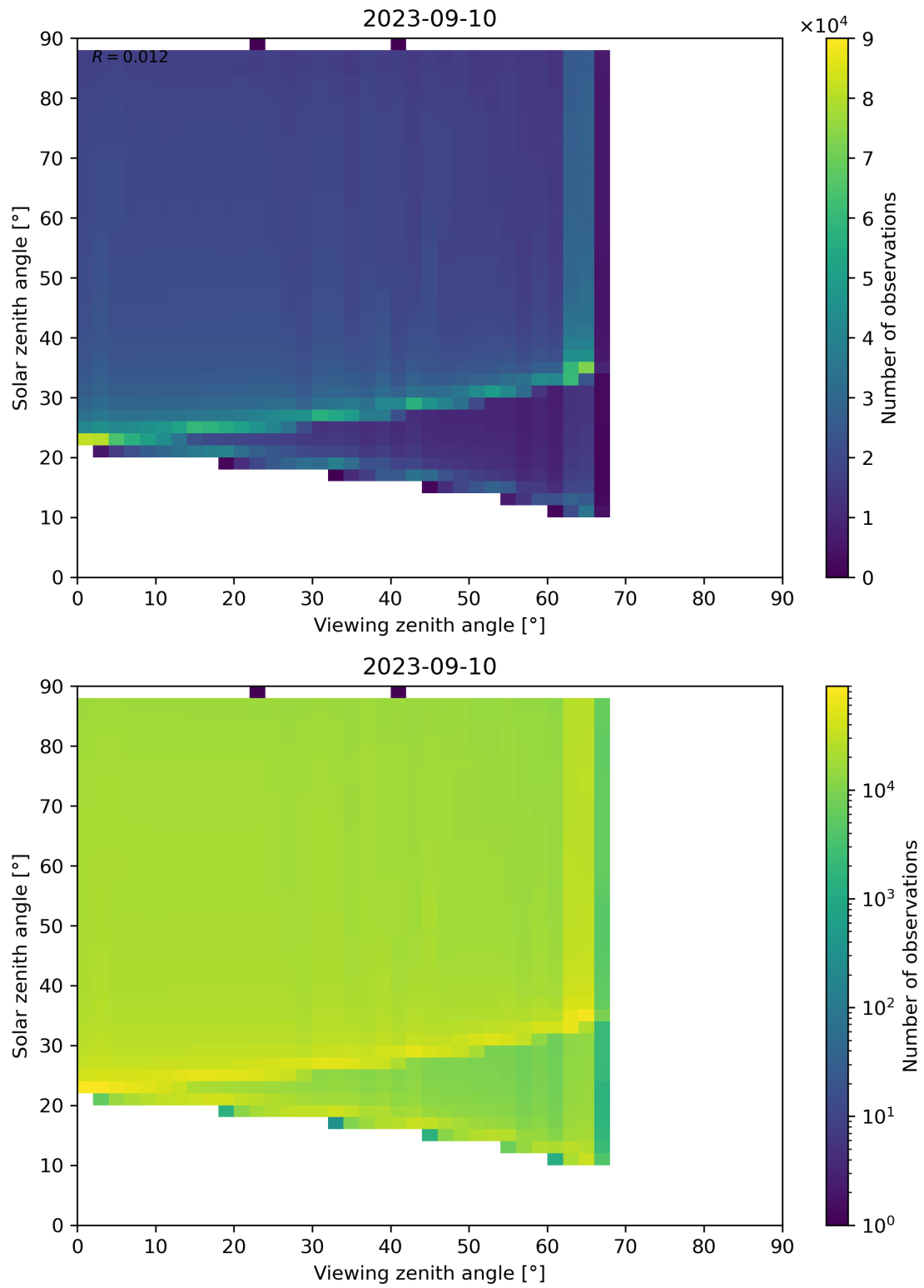
Figure 139: Scatter density plot of “Viewing zenith angle” against “Solar zenith angle” for 2023-09-10 to 2023-09-11.
