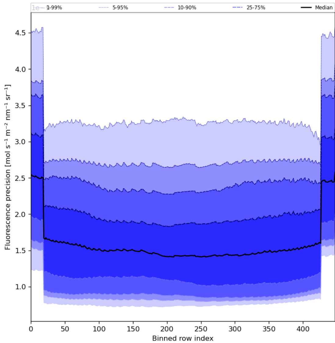
Figure 58: Along track statistics of “Fluorescence precision” for 2023-09-10 to 2023-09-11
