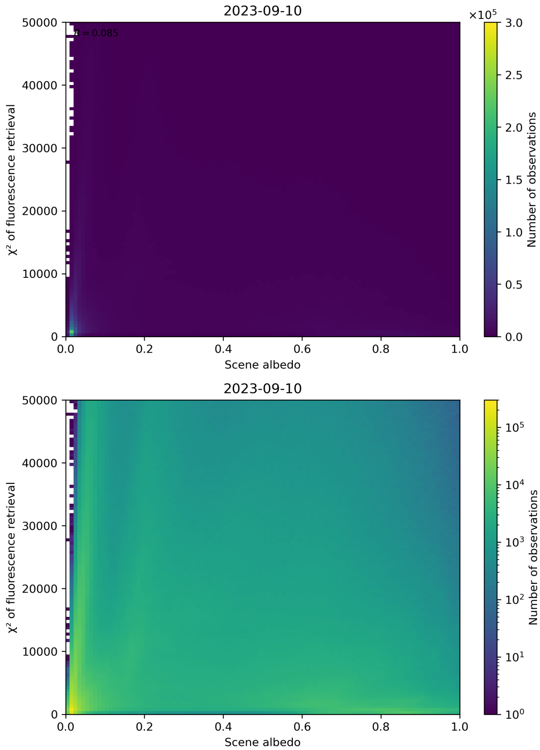
Figure 113: Scatter density plot of “Scene albedo” against “ \chi^2 of fluorescence retrieval” for 2023-09-10 to 2023-09-11.
