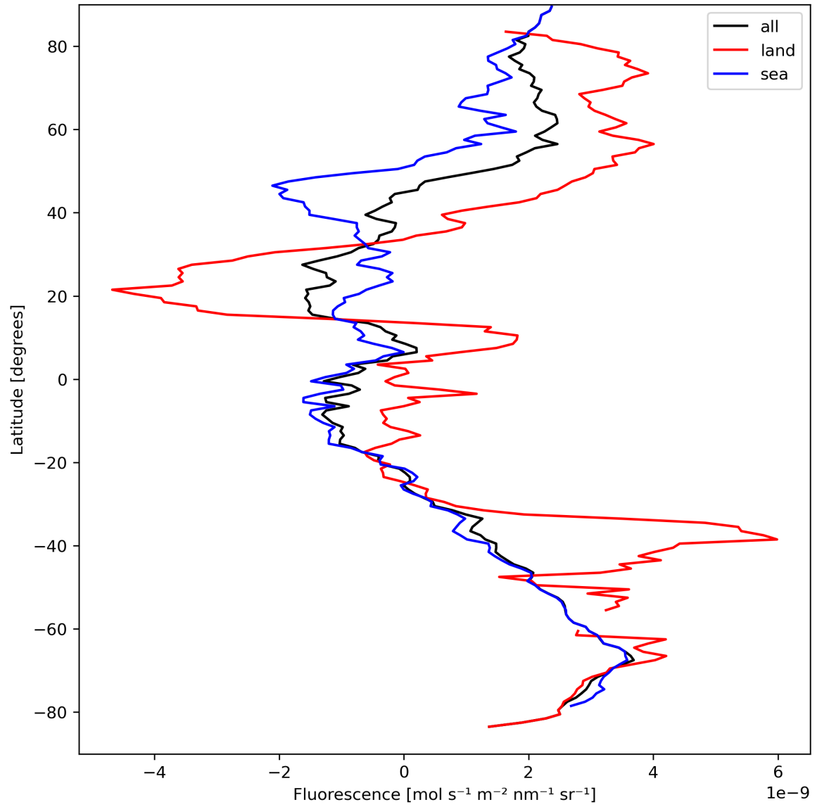
Figure 23: Zonal average of “Fluorescence” for 2023-09-10 to 2023-09-11.
