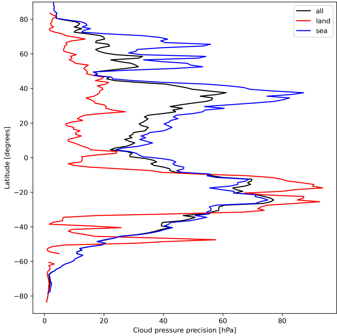
Figure 14: Zonal average of “Cloud pressure precision” for 2023-09-10 to 2023-09-11.
