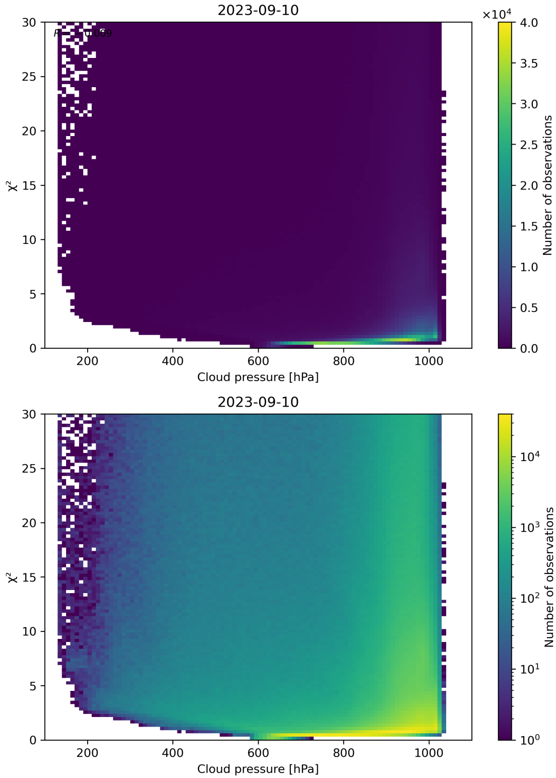
Figure 85: Scatter density plot of “Cloud pressure” against “ \chi^2 ” for 2023-09-10 to 2023-09-11.
