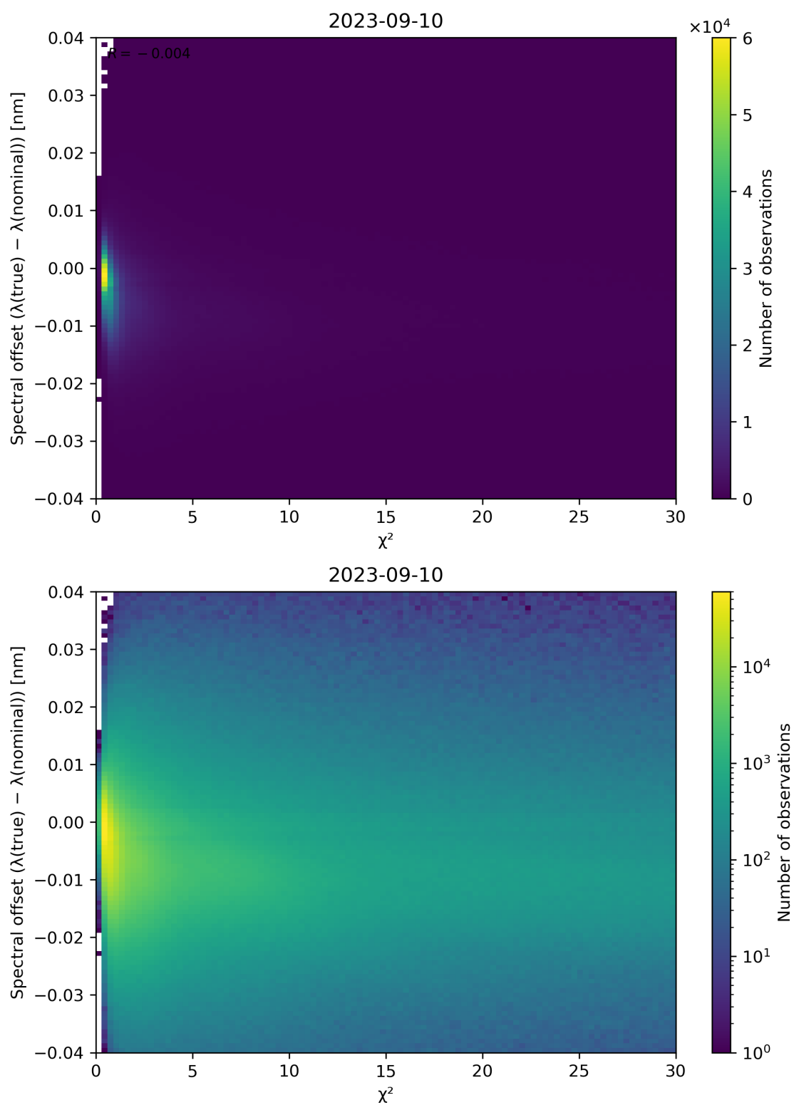
Figure 75: Scatter density plot of “ \chi^2 ” against “Spectral offset ( \lambda(\text{true}) - \lambda(\text{nominal}) )” for 2023-09-10 to 2023-09-11.
