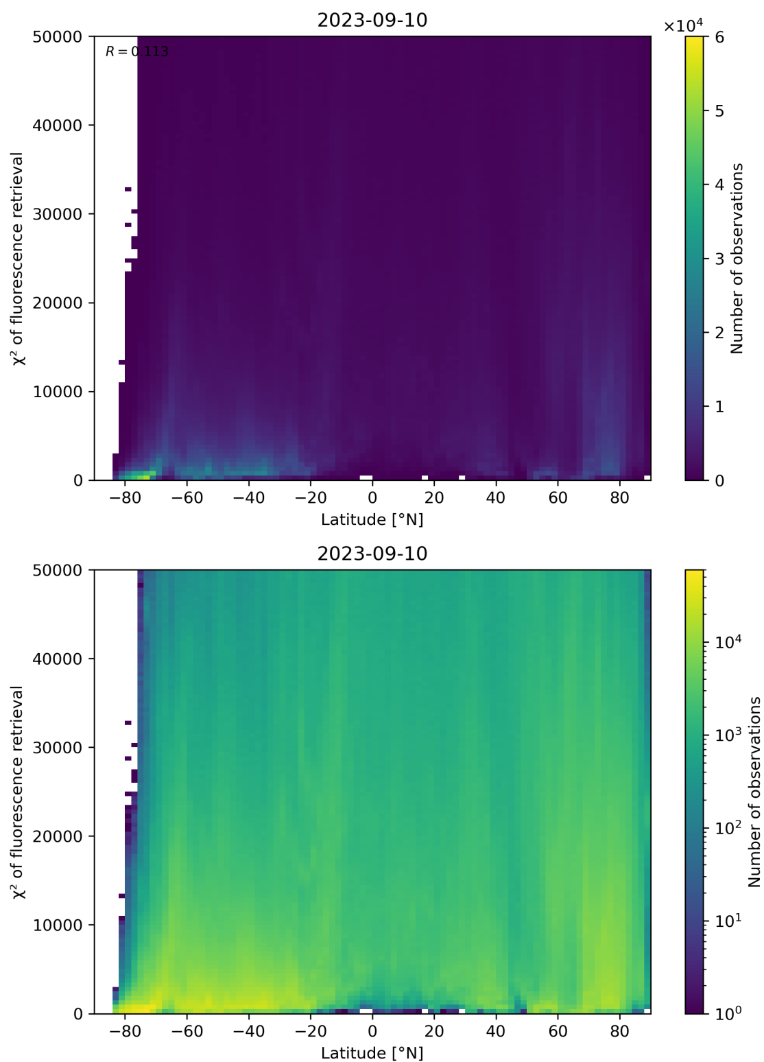
Figure 98: Scatter density plot of “Latitude” against “ \chi^2 of fluorescence retrieval” for 2023-09-10 to 2023-09-11.
