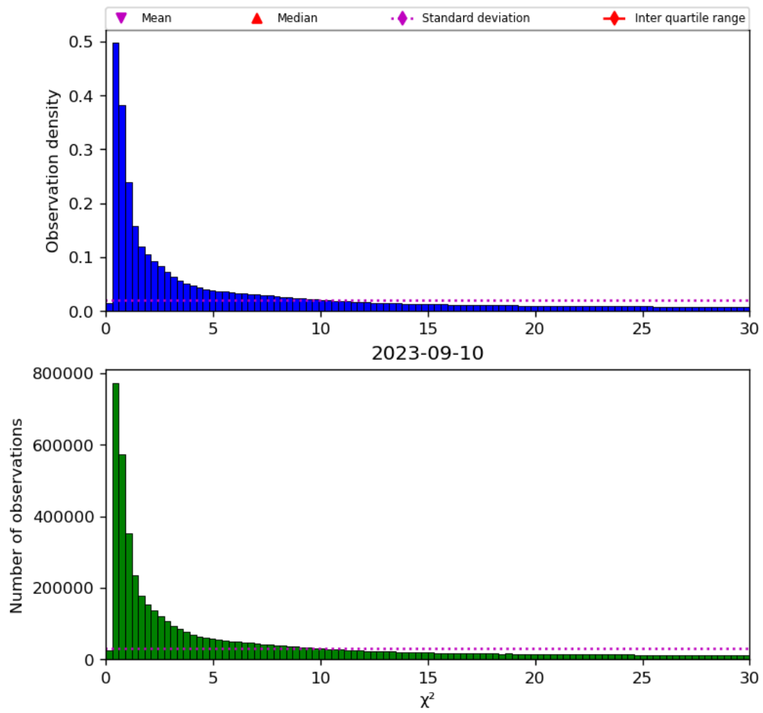
Figure 38: Histogram of “ \chi^2 ” for 2023-09-10 to 2023-09-11
