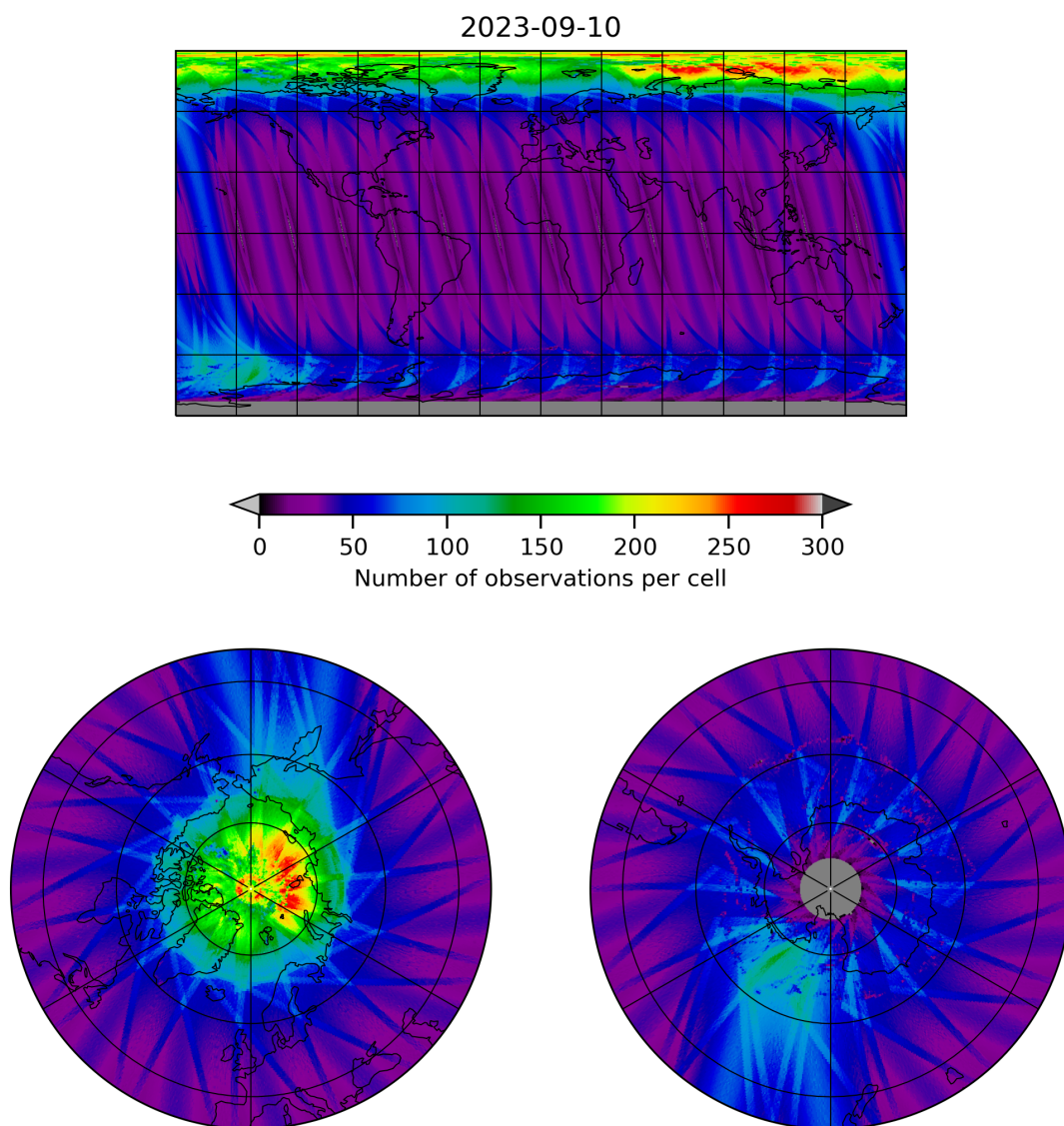
Figure 11: Map of the number of observations for 2023-09-10 to 2023-09-11
