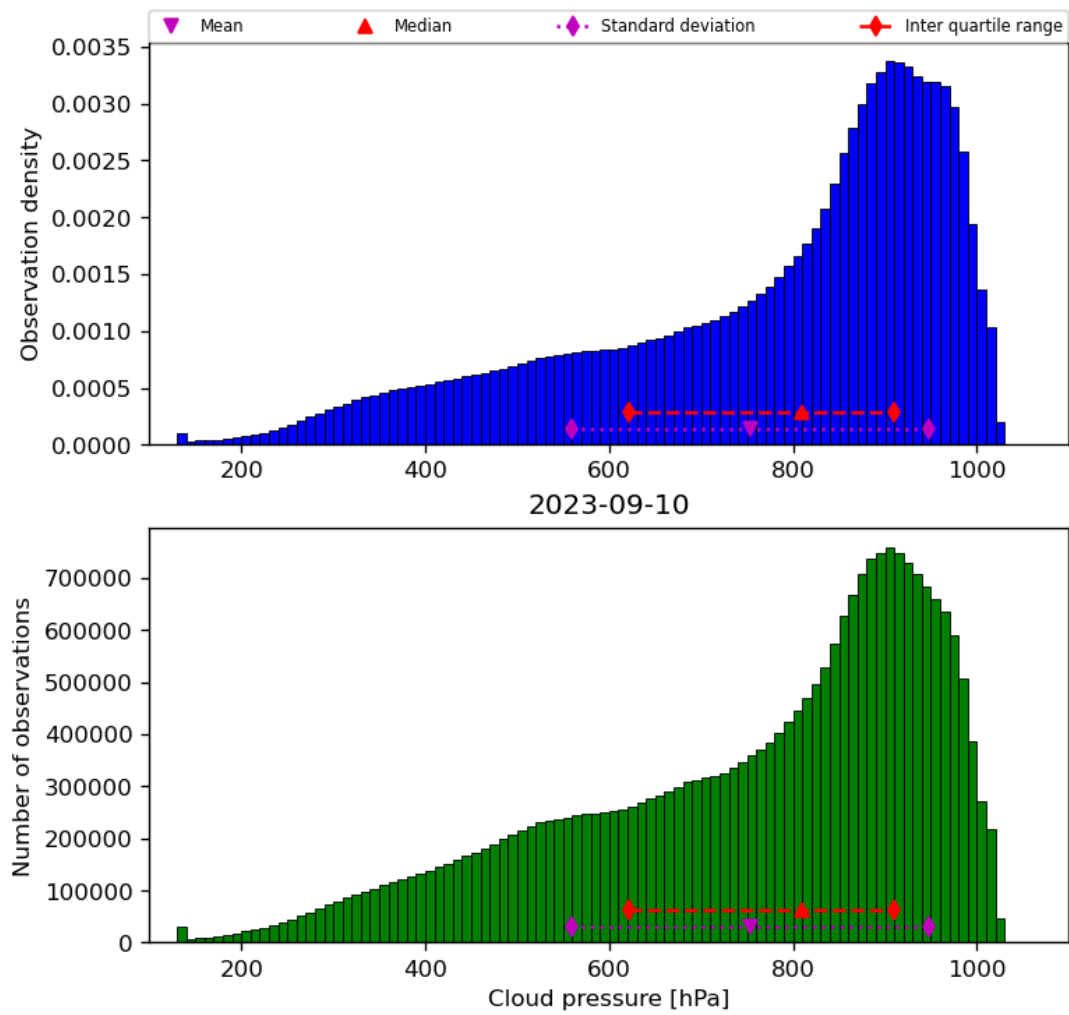
Figure 30: Histogram of “Cloud pressure” for 2023-09-10 to 2023-09-11
