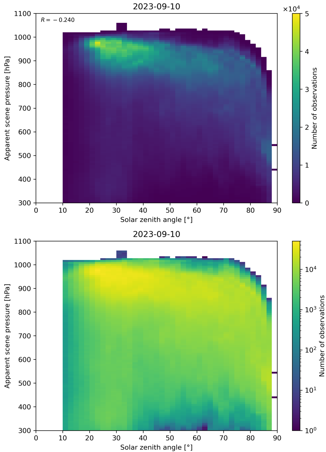
Figure 118: Scatter density plot of “Solar zenith angle” against “Apparent scene pressure” for 2023-09-10 to 2023-09-11.
