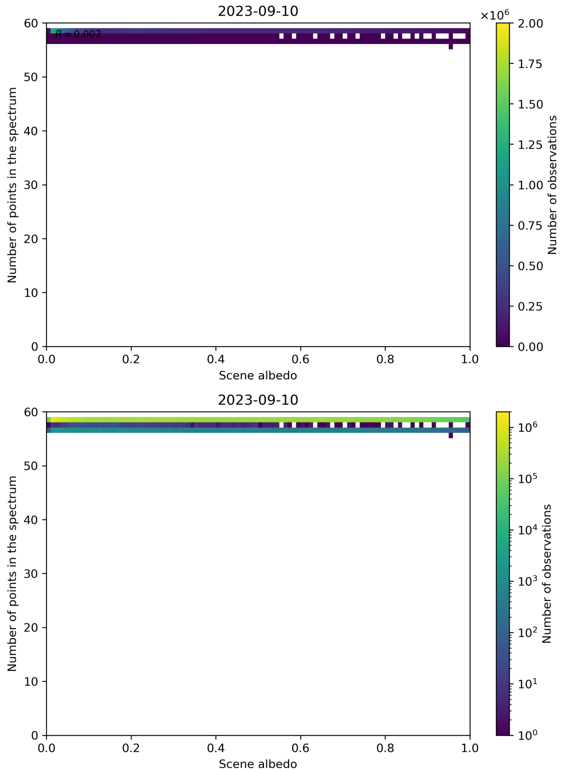
Figure 116: Scatter density plot of “Scene albedo” against “Number of points in the spectrum” for 2023-09-10 to 2023-09-11.
