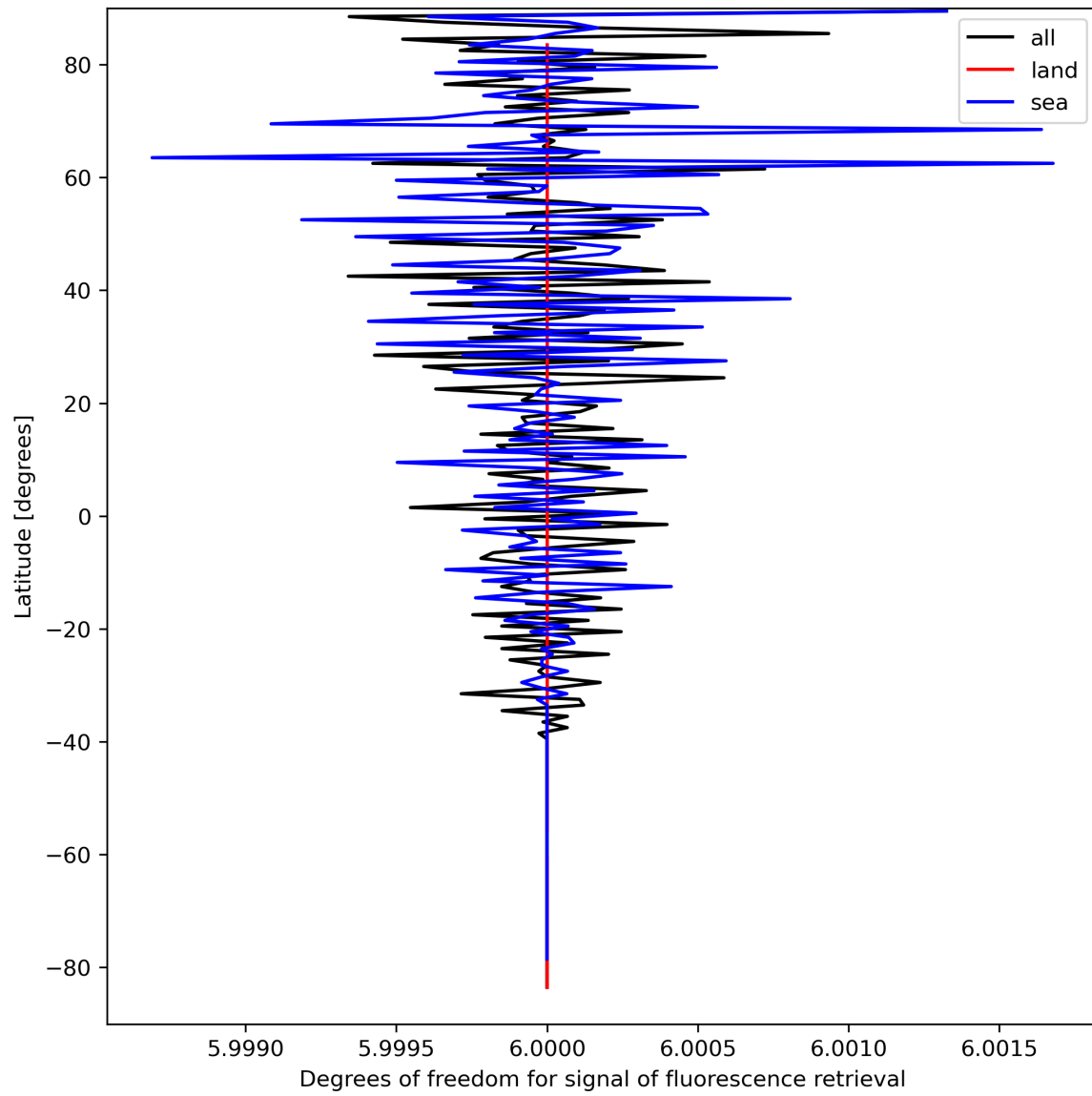
Figure 26: Zonal average of “Degrees of freedom for signal of fluorescence retrieval” for 2023-09-10 to 2023-09-11.
