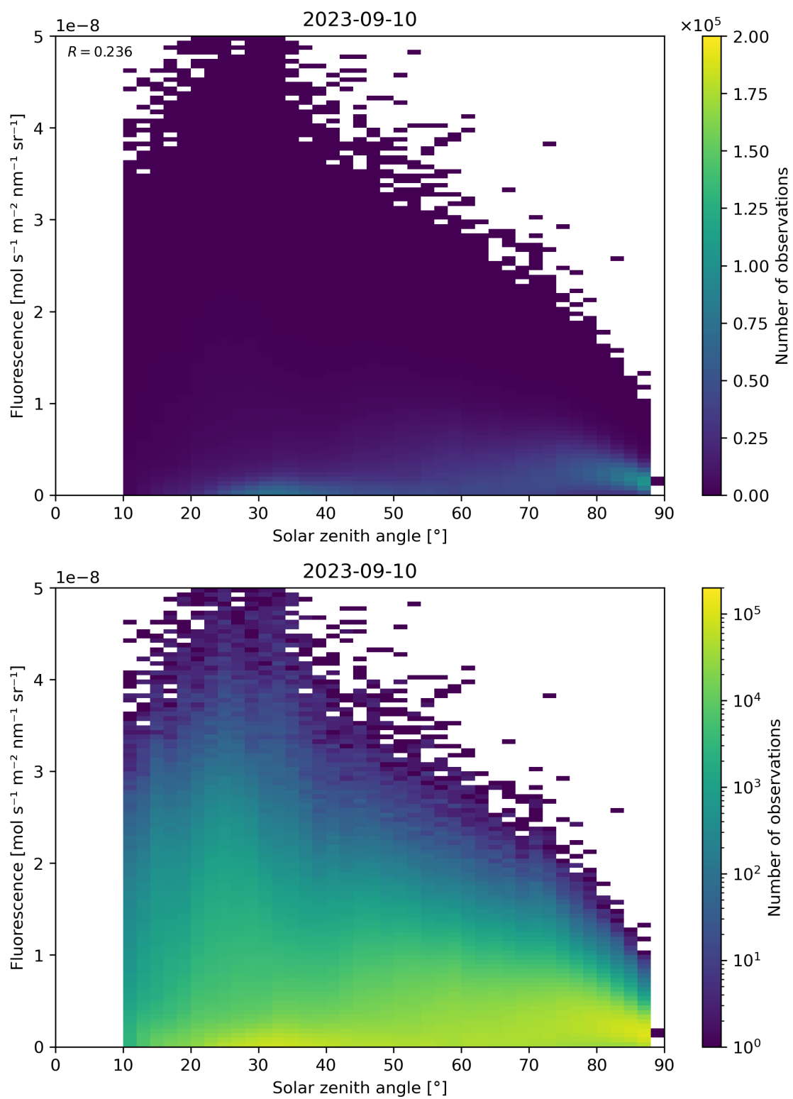
Figure 123: Scatter density plot of “Solar zenith angle” against “Fluorescence” for 2023-09-10 to 2023-09-11.
