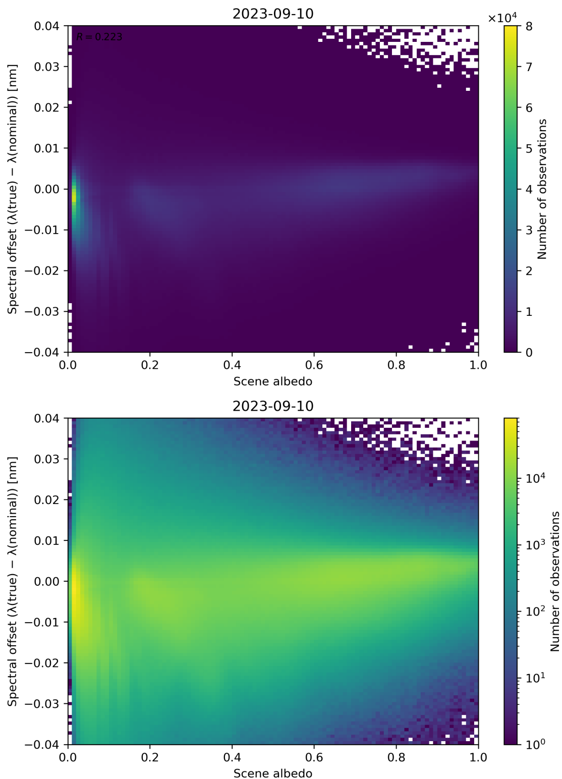
Figure 117: Scatter density plot of “Scene albedo” against “Spectral offset ( \lambda(\text{true}) - \lambda(\text{nominal}) )” for 2023-09-10 to 2023-09-11.
