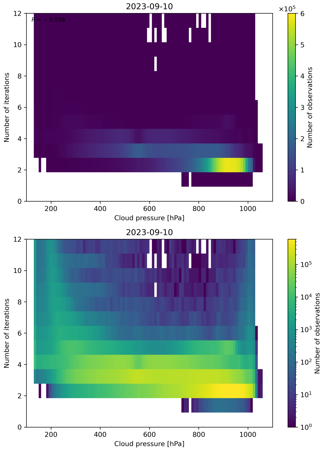
Figure 89: Scatter density plot of “Cloud pressure” against “Number of iterations” for 2023-09-10 to 2023-09-11.
