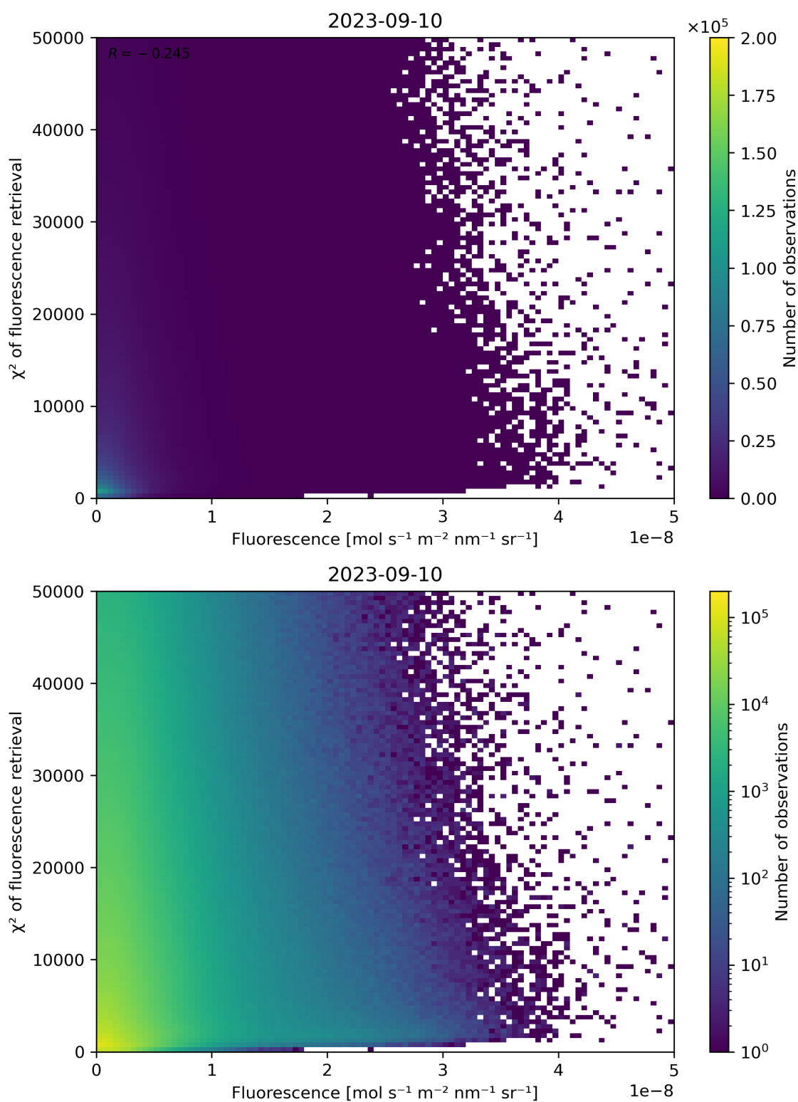
Figure 93: Scatter density plot of “Fluorescence” against “ \chi^2 of fluorescence retrieval” for 2023-09-10 to 2023-09-11.
