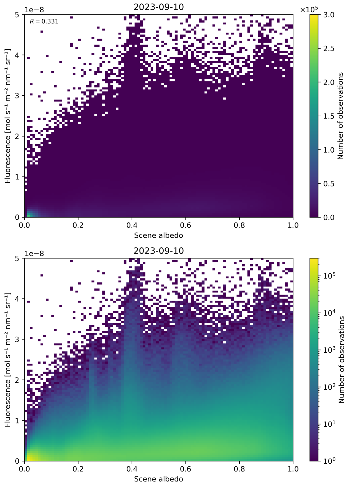
Figure 114: Scatter density plot of “Scene albedo” against “Fluorescence” for 2023-09-10 to 2023-09-11.
