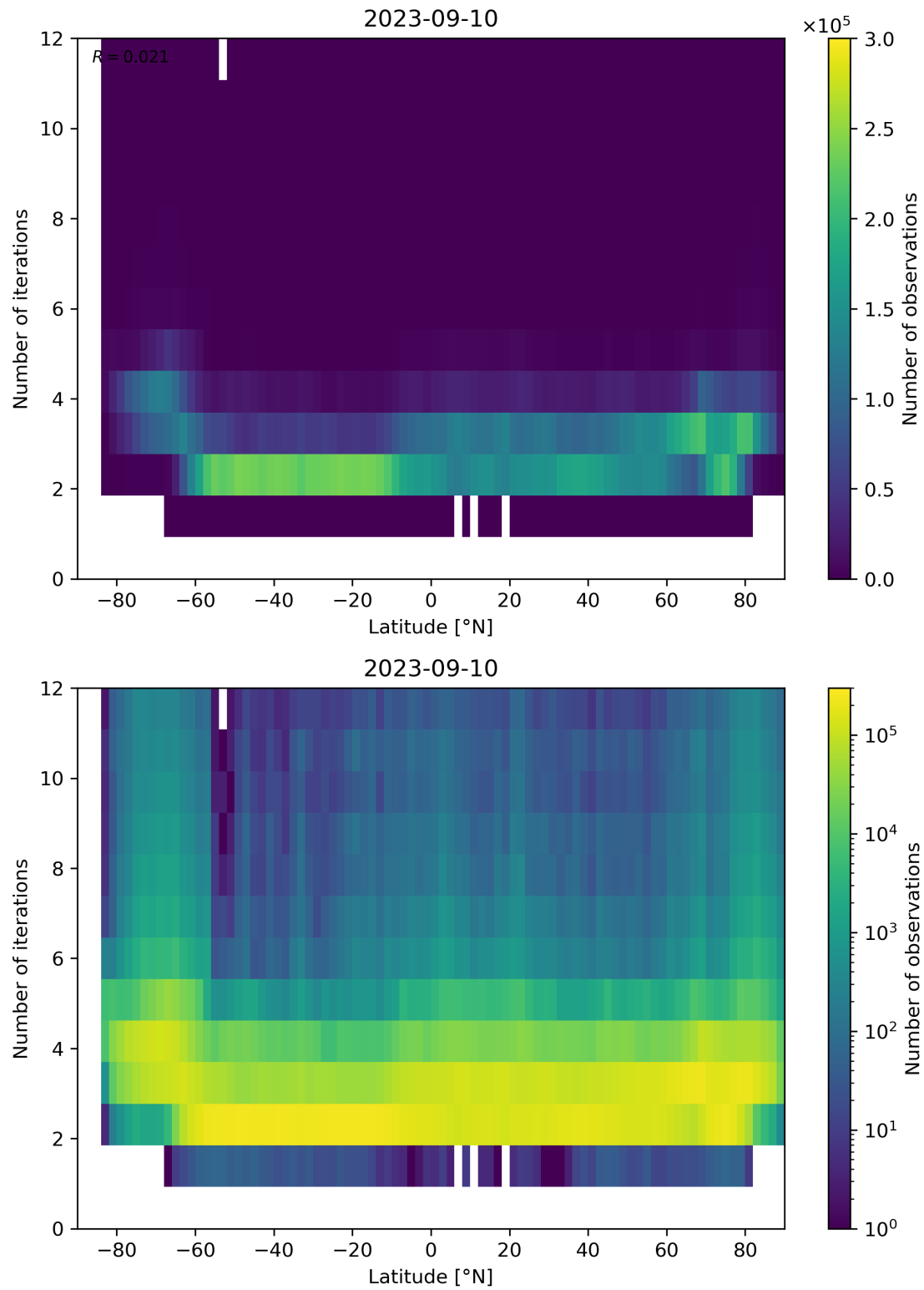
Figure 102: Scatter density plot of “Latitude” against “Number of iterations” for 2023-09-10 to 2023-09-11.
