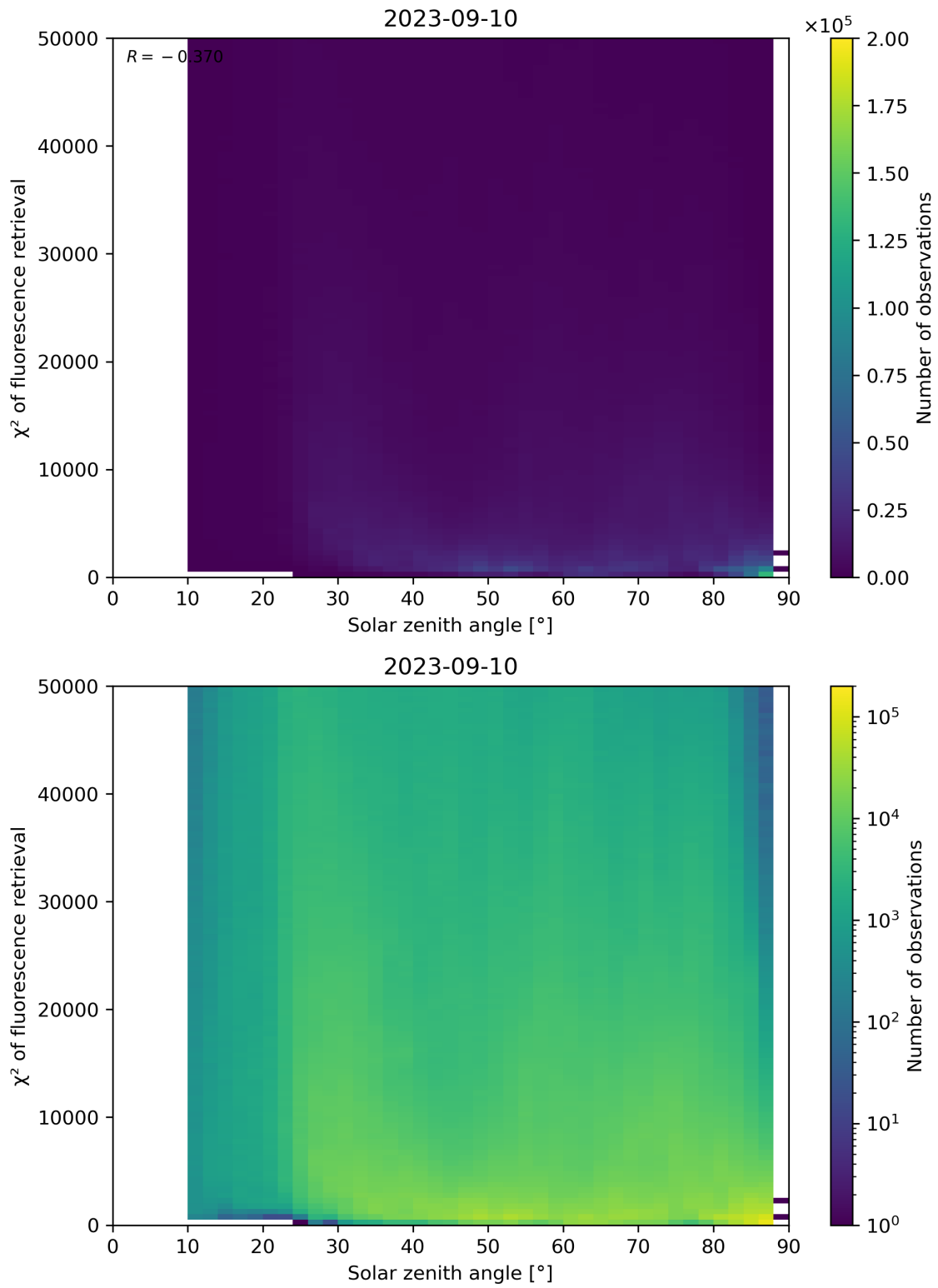
Figure 120: Scatter density plot of “Solar zenith angle” against “ \chi^2 of fluorescence retrieval” for 2023-09-10 to 2023-09-11.
