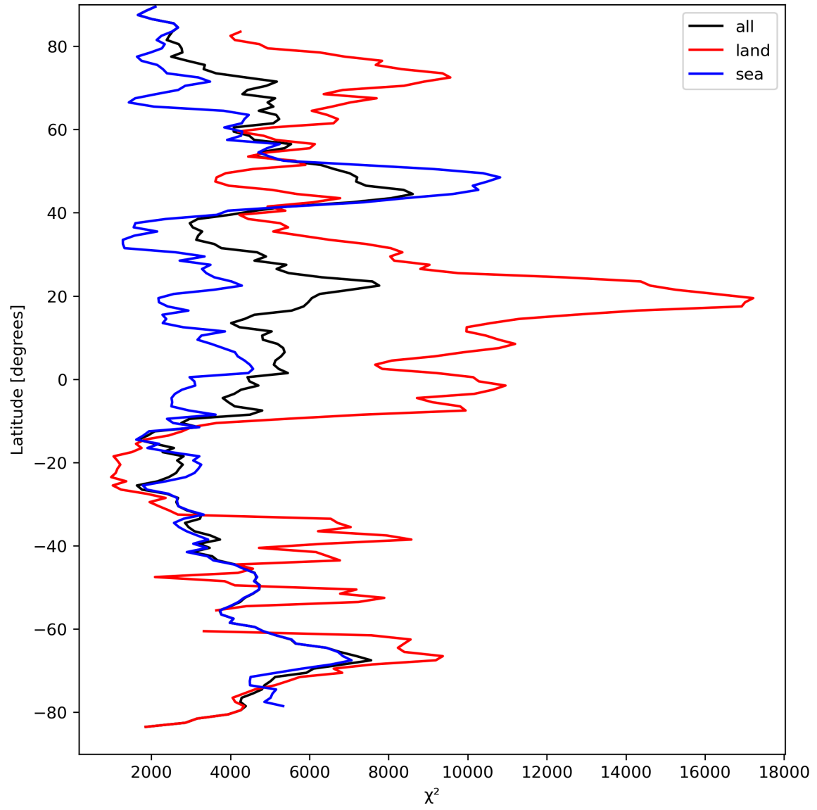
Figure 21: Zonal average of “ \chi^2 ” for 2023-09-10 to 2023-09-11.
