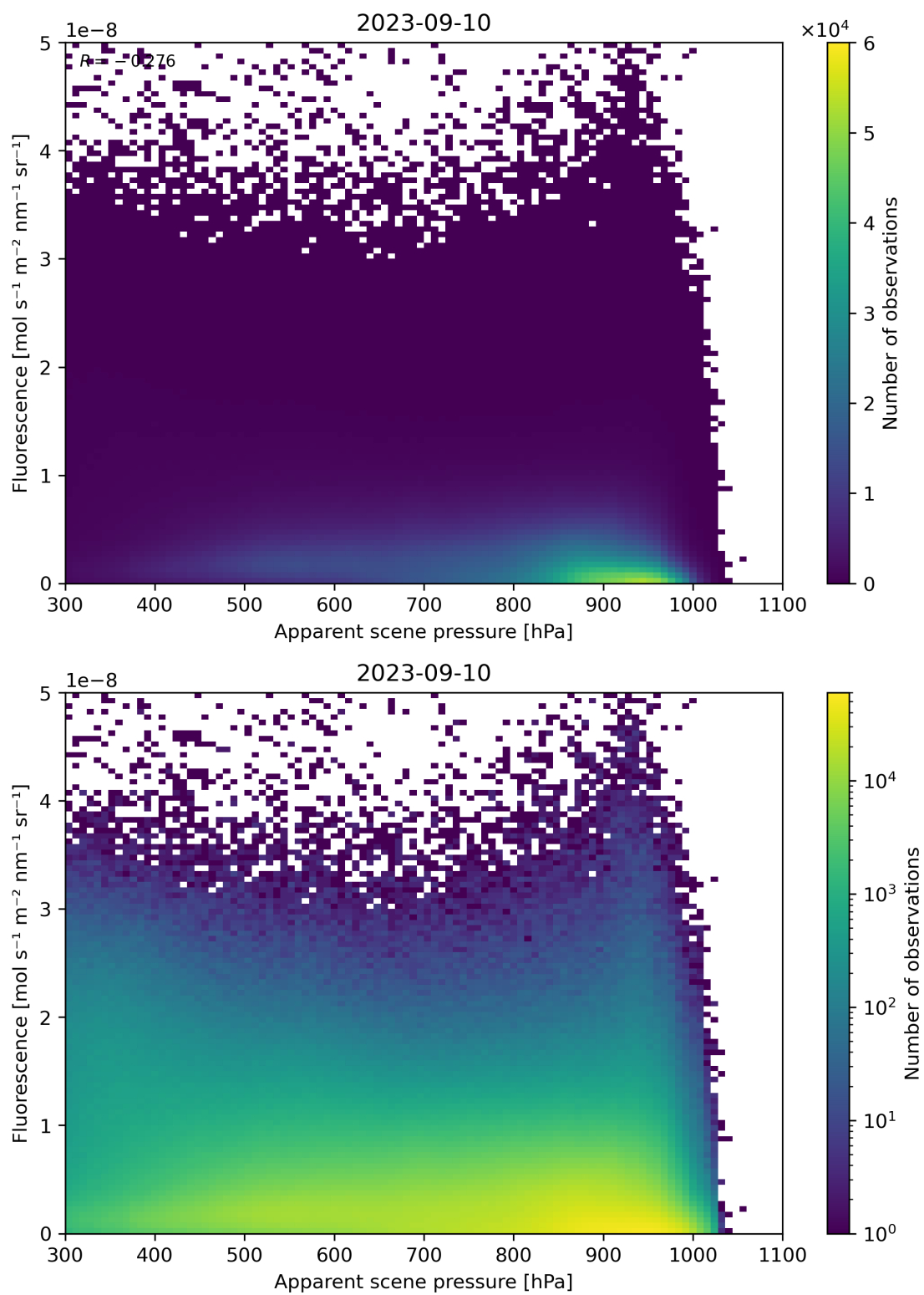
Figure 65: Scatter density plot of “Apparent scene pressure” against “Fluorescence” for 2023-09-10 to 2023-09-11.
