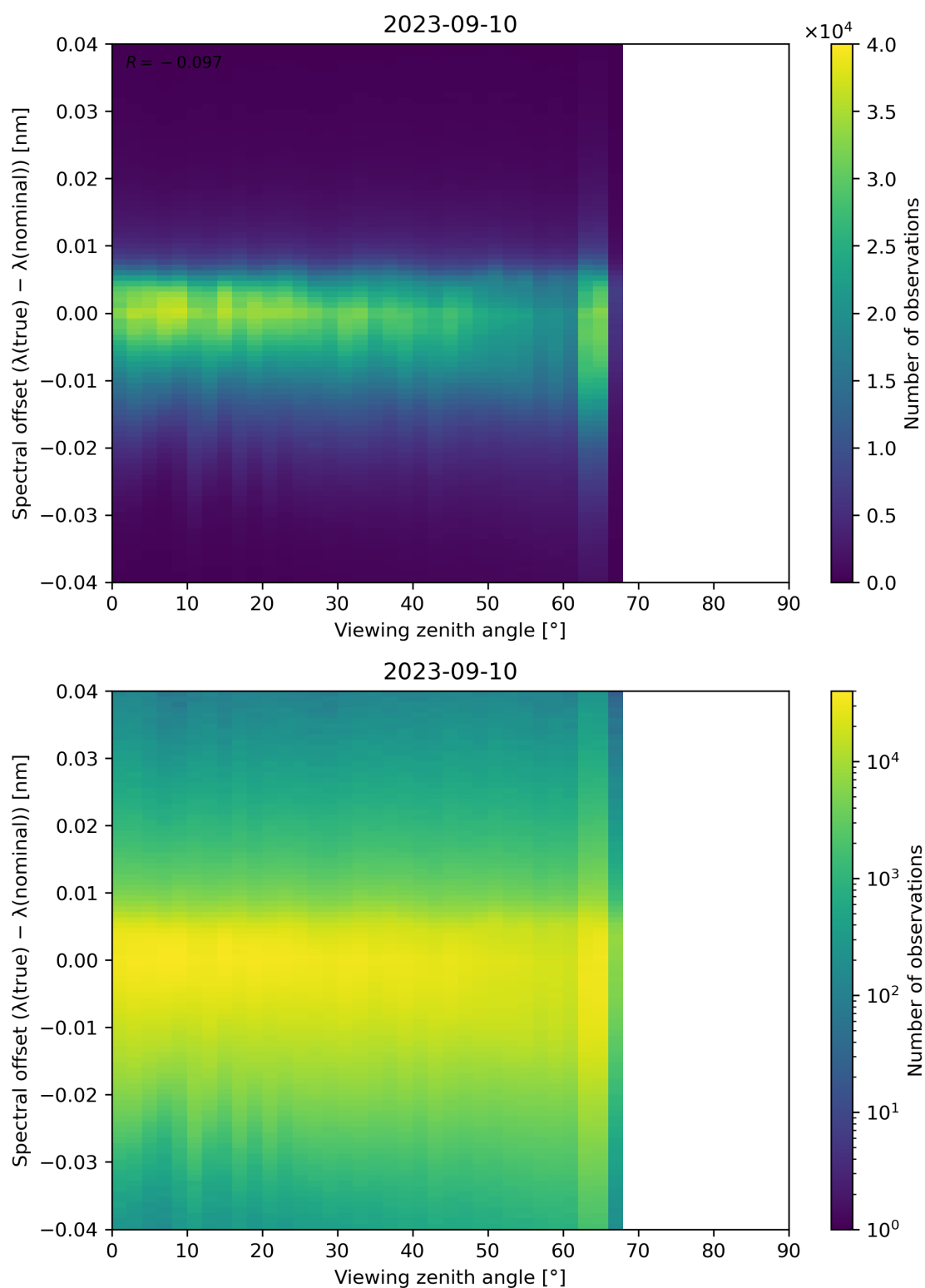
Figure 140: Scatter density plot of “Viewing zenith angle” against “Spectral offset ( \lambda(\text{true}) - \lambda(\text{nominal}) )” for 2023-09-10 to 2023-09-11.
