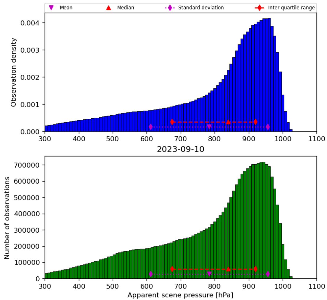
Figure 36: Histogram of “Apparent scene pressure” for 2023-09-10 to 2023-09-11
