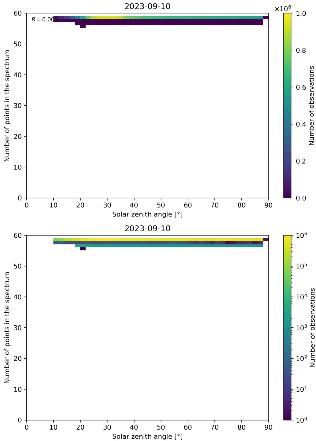
Figure 126: Scatter density plot of “Solar zenith angle” against “Number of points in the spectrum” for 2023-09-10 to 2023-09-11.
