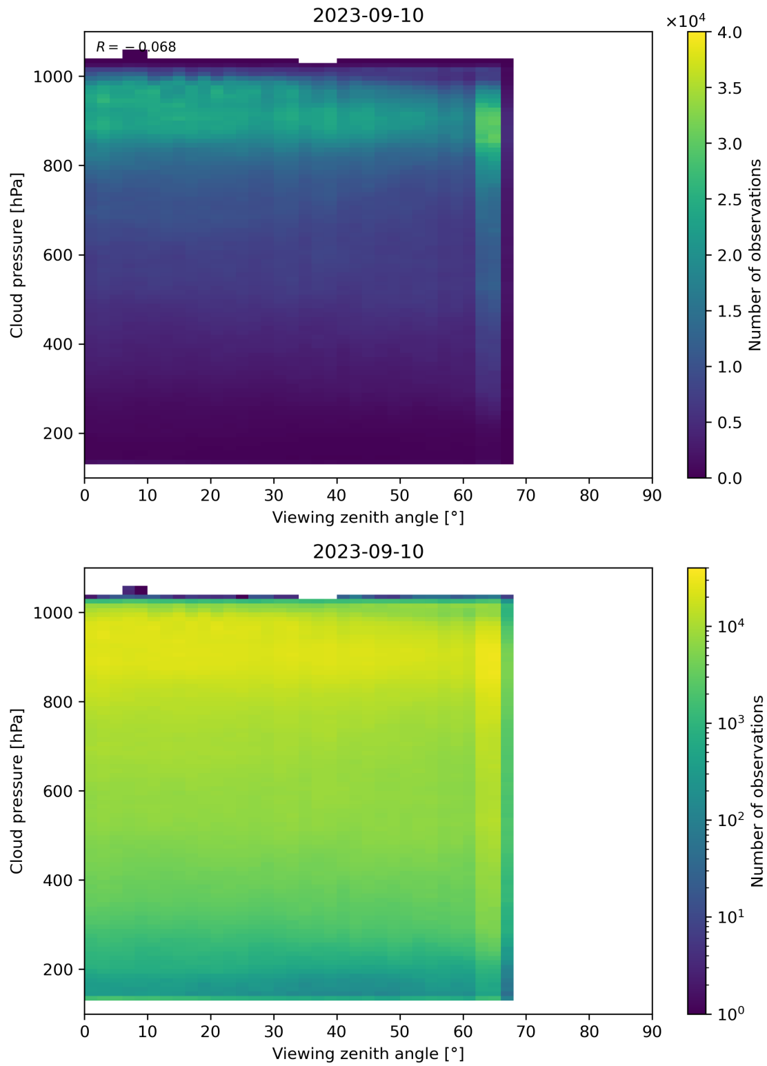
Figure 133: Scatter density plot of “Viewing zenith angle” against “Cloud pressure” for 2023-09-10 to 2023-09-11.
