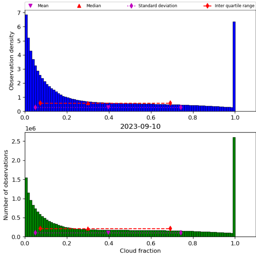
Figure 32: Histogram of “Cloud fraction” for 2023-09-10 to 2023-09-11
