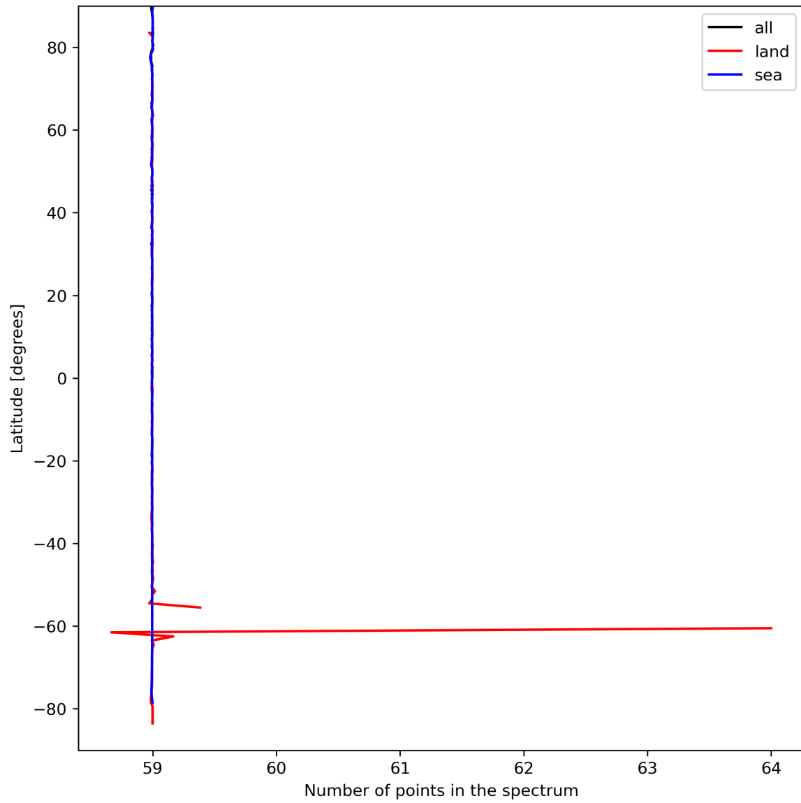
Figure 27: Zonal average of “Number of points in the spectrum” for 2023-09-10 to 2023-09-11.
