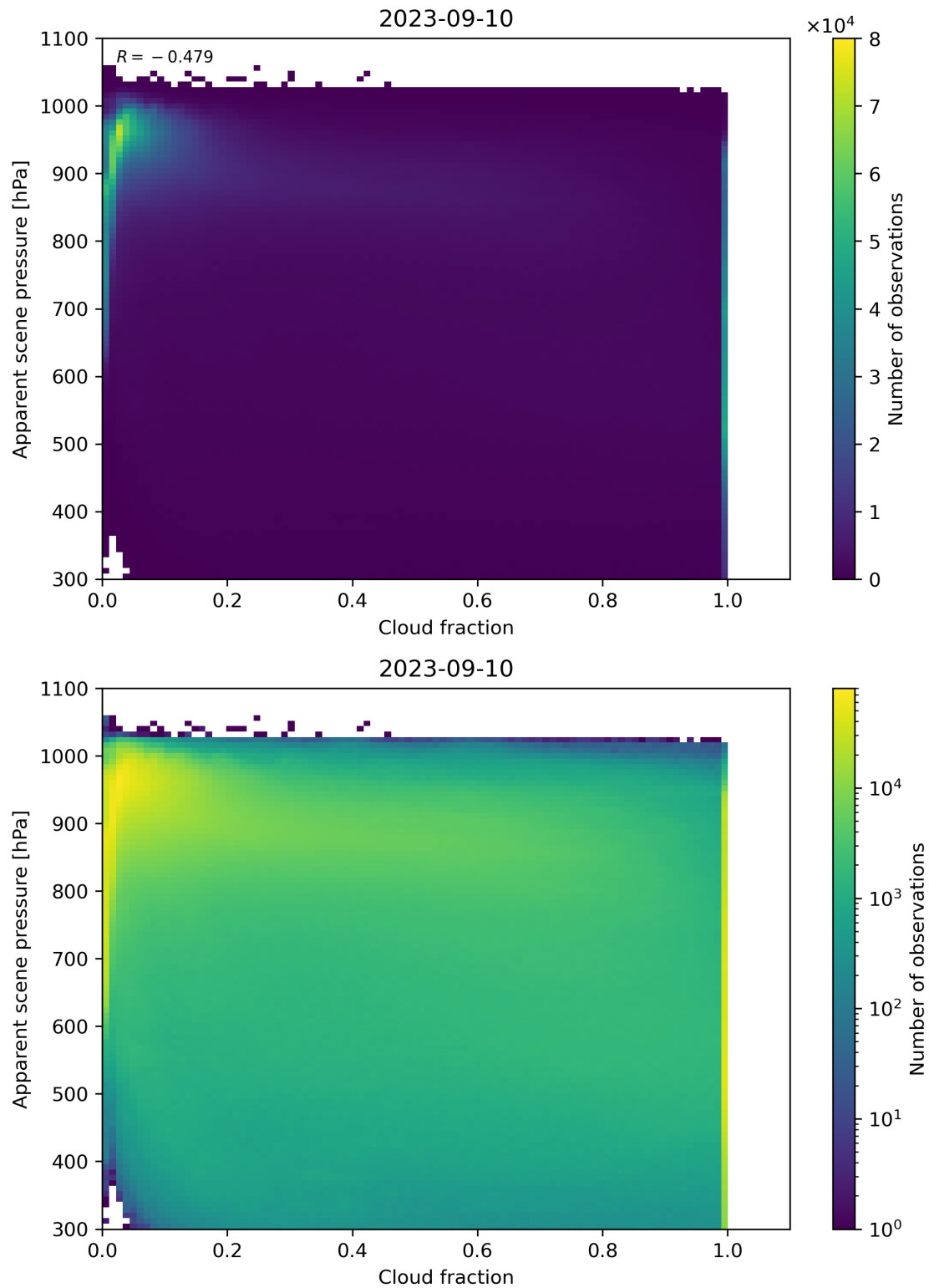
Figure 76: Scatter density plot of “Cloud fraction” against “Apparent scene pressure” for 2023-09-10 to 2023-09-11.
