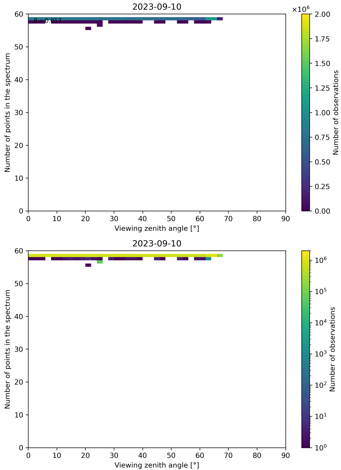
Figure 137: Scatter density plot of “Viewing zenith angle” against “Number of points in the spectrum” for 2023-09-10 to 2023-09-11.
