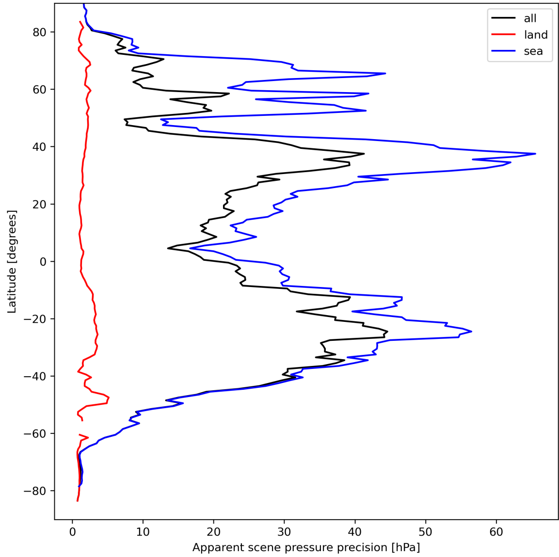
Figure 20: Zonal average of “Apparent scene pressure precision” for 2023-09-10 to 2023-09-11.
