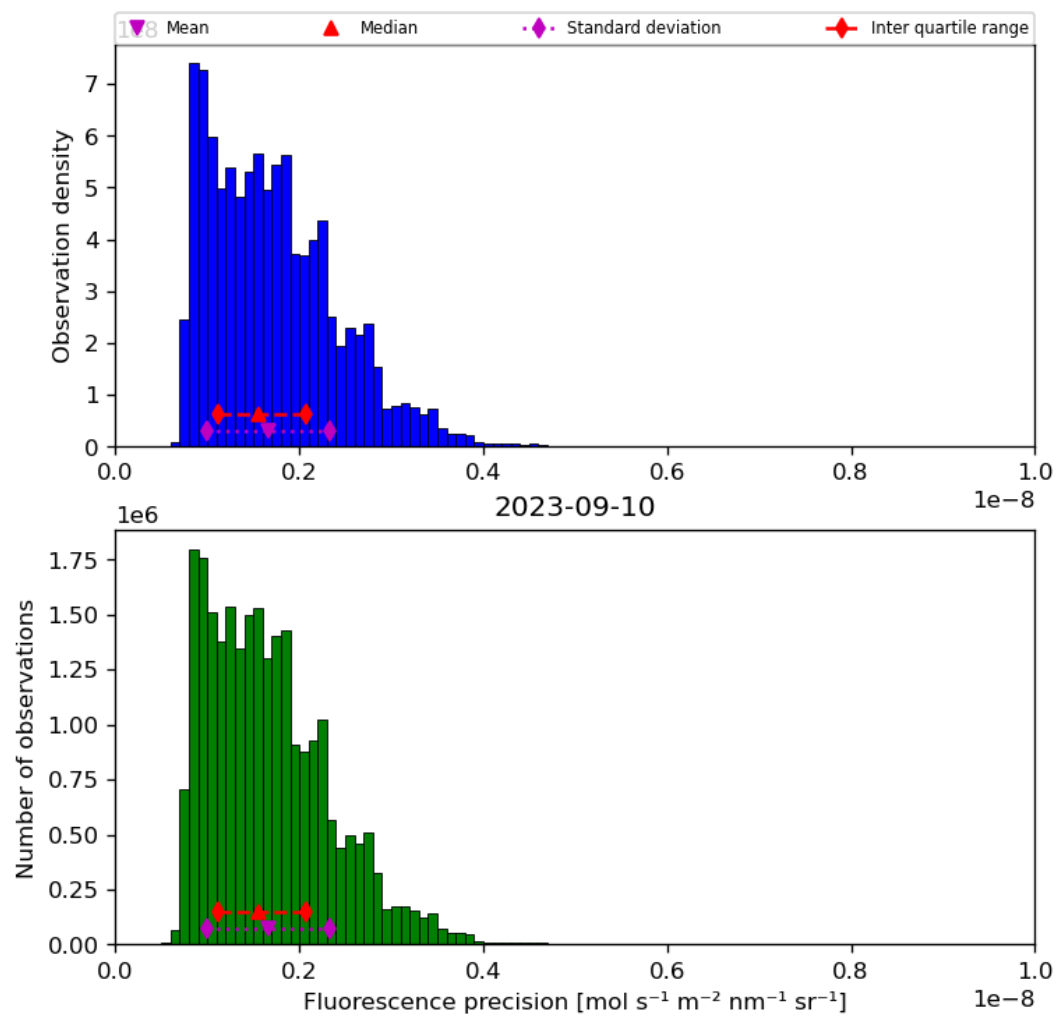
Figure 41: Histogram of “Fluorescence precision” for 2023-09-10 to 2023-09-11
