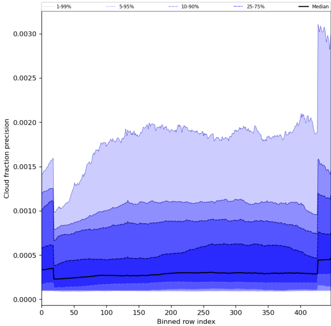
Figure 50: Along track statistics of “Cloud fraction precision” for 2023-09-10 to 2023-09-11
