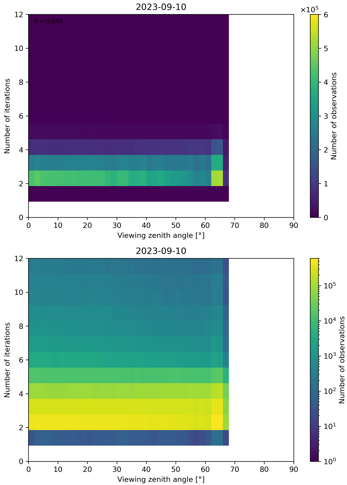
Figure 136: Scatter density plot of “Viewing zenith angle” against “Number of iterations” for 2023-09-10 to 2023-09-11.
