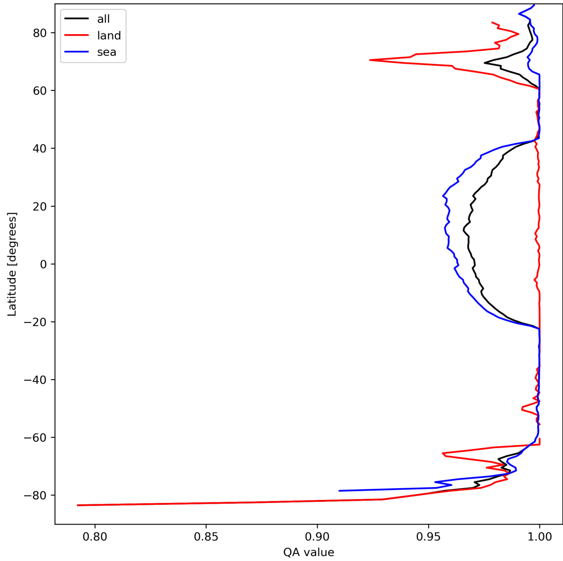
Figure 12: Zonal average of “QA value” for 2023-09-10 to 2023-09-11.
