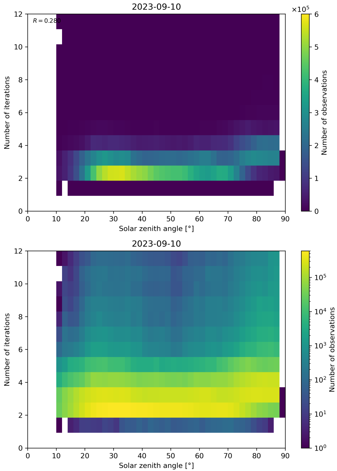
Figure 125: Scatter density plot of “Solar zenith angle” against “Number of iterations” for 2023-09-10 to 2023-09-11.
