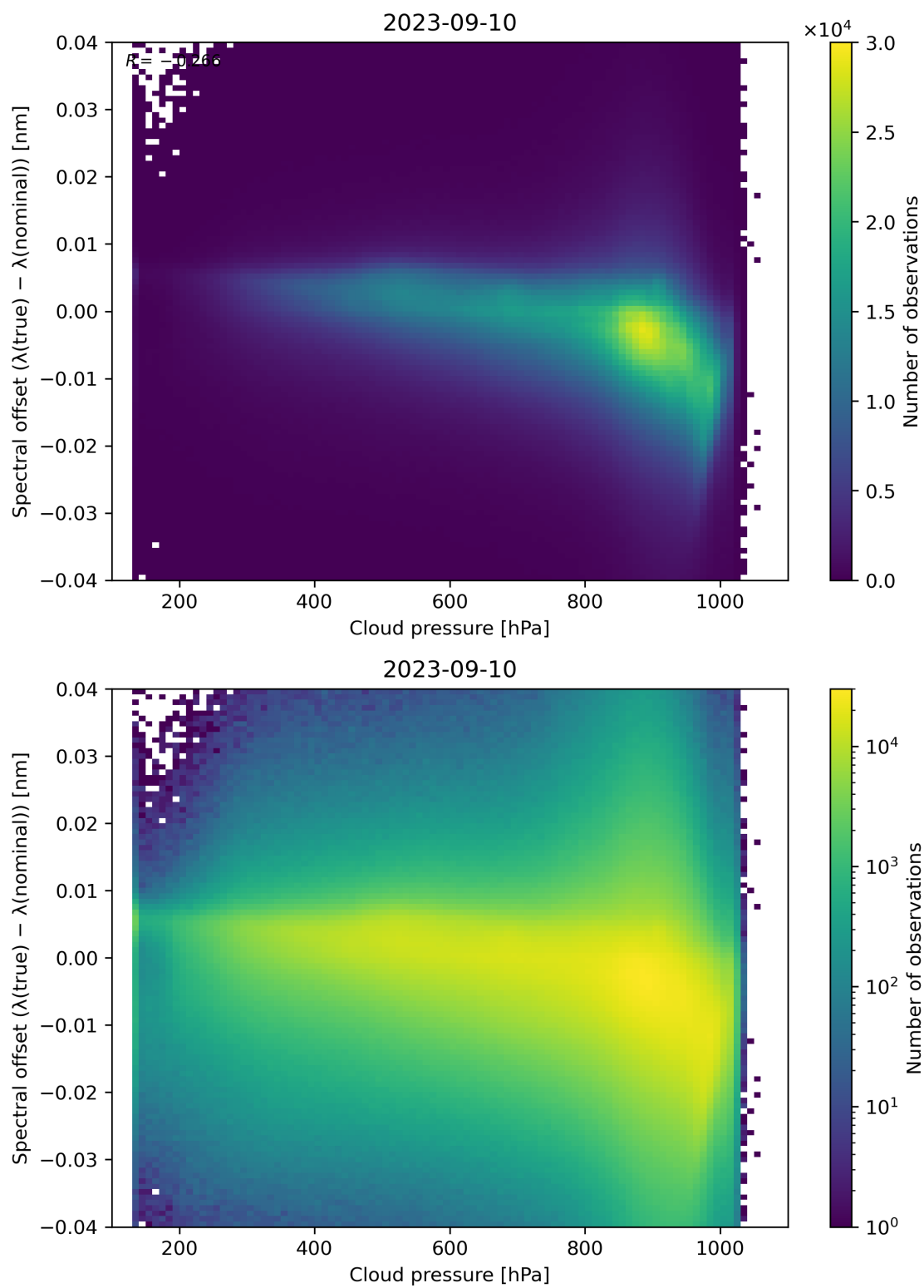
Figure 92: Scatter density plot of “Cloud pressure” against “Spectral offset ( \lambda(\text{true}) - \lambda(\text{nominal}) )” for 2023-09-10 to 2023-09-11.
