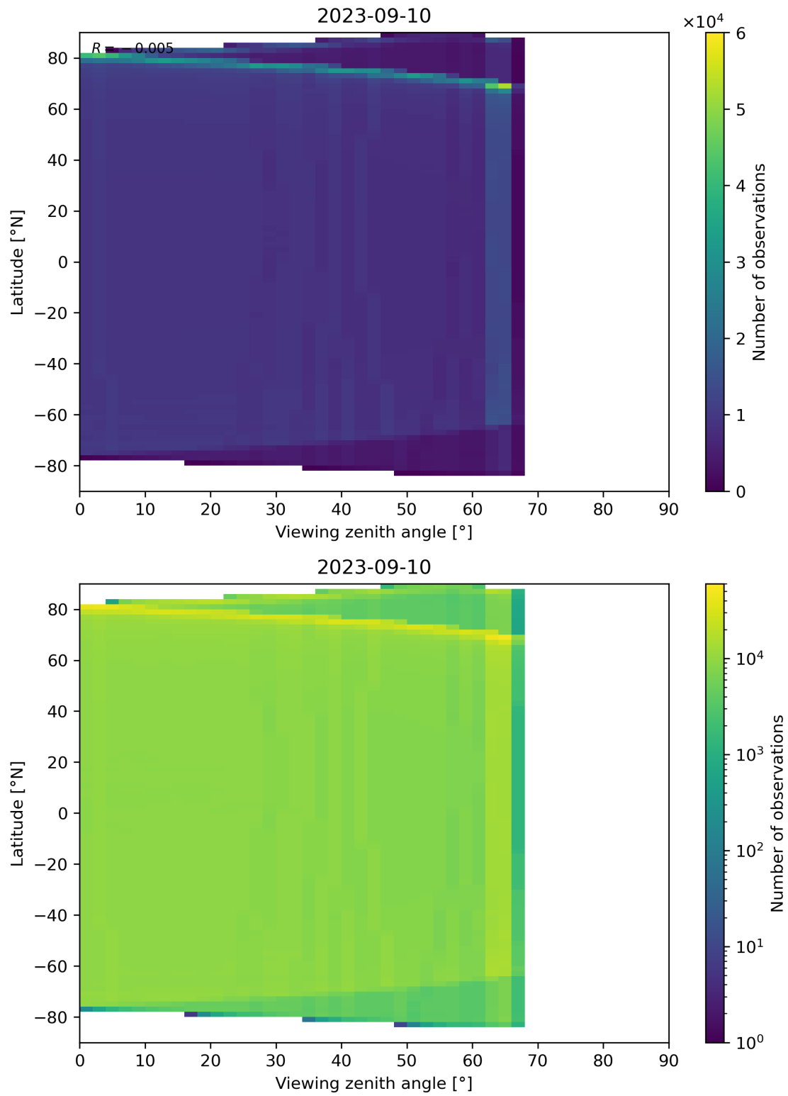
Figure 135: Scatter density plot of “Viewing zenith angle” against “Latitude” for 2023-09-10 to 2023-09-11.
