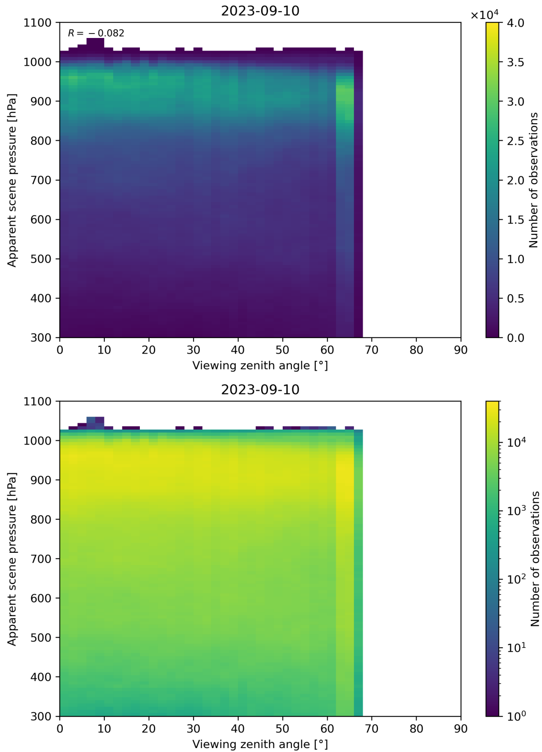
Figure 129: Scatter density plot of “Viewing zenith angle” against “Apparent scene pressure” for 2023-09-10 to 2023-09-11.
