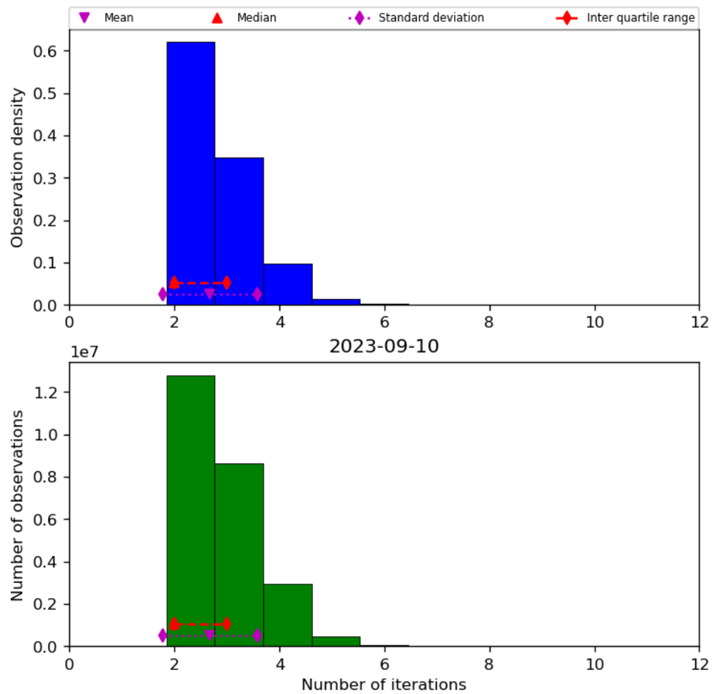
Figure 39: Histogram of “Number of iterations” for 2023-09-10 to 2023-09-11
