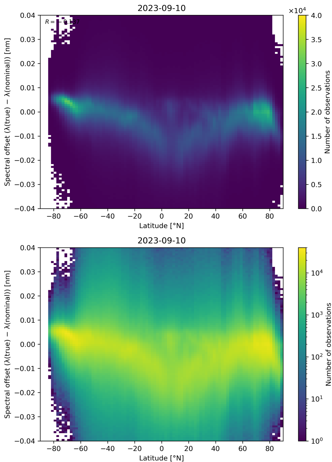
Figure 105: Scatter density plot of “Latitude” against “Spectral offset ( \lambda(\text{true}) - \lambda(\text{nominal}) )” for 2023-09-10 to 2023-09-11.
