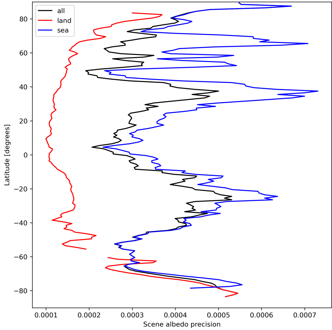
Figure 18: Zonal average of “Scene albedo precision” for 2023-09-10 to 2023-09-11.
