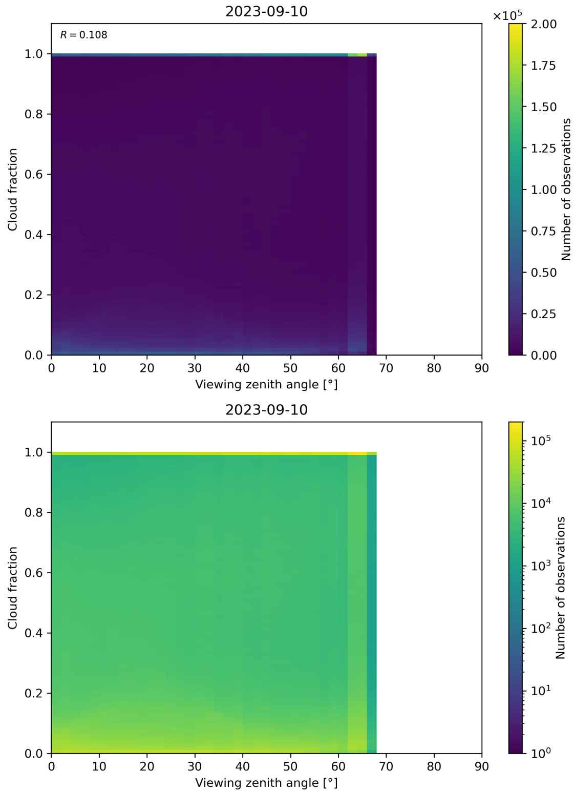
Figure 132: Scatter density plot of “Viewing zenith angle” against “Cloud fraction” for 2023-09-10 to 2023-09-11.
