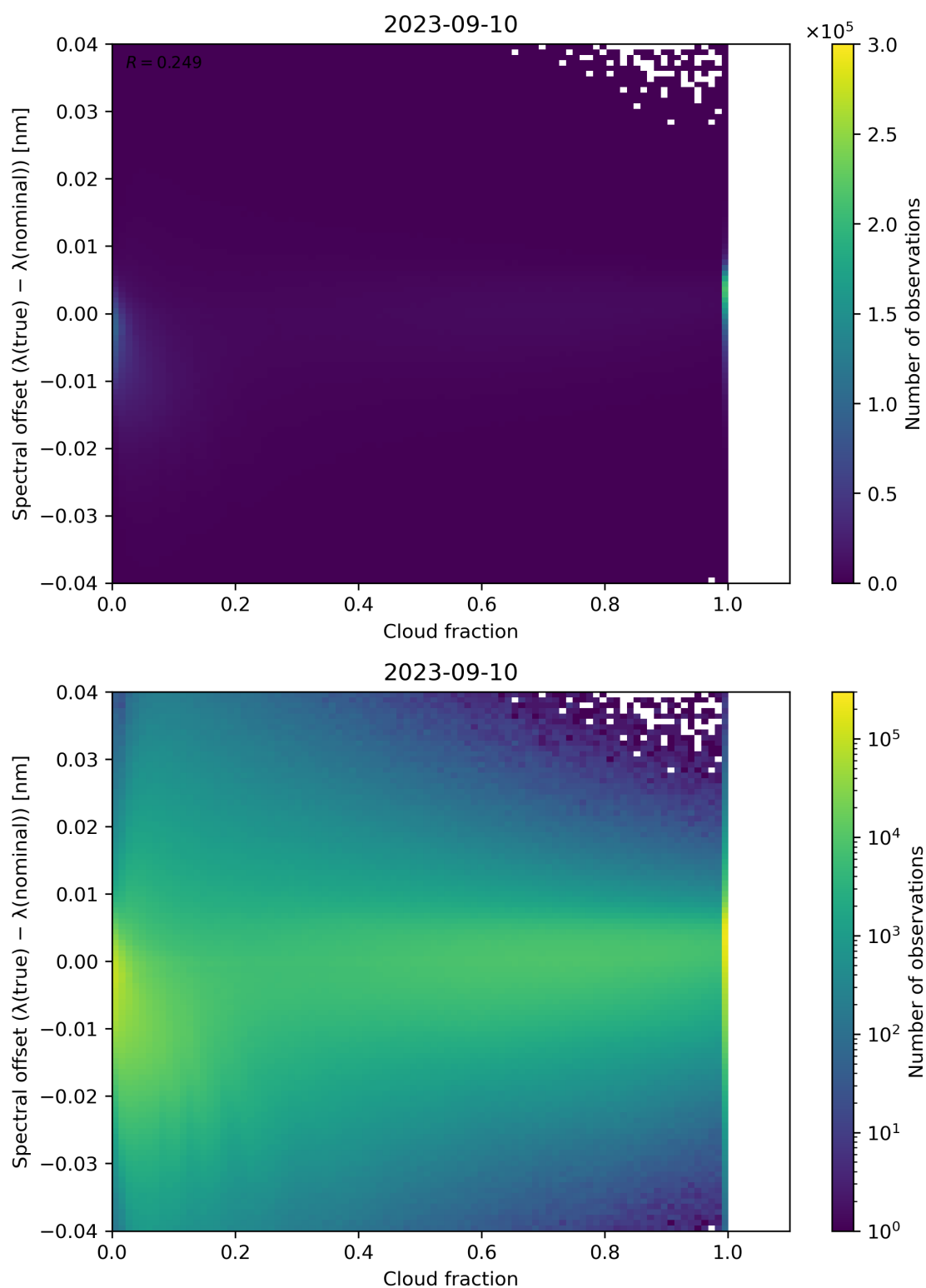
Figure 83: Scatter density plot of “Cloud fraction” against “Spectral offset ( \lambda(\text{true}) - \lambda(\text{nominal}) )” for 2023-09-10 to 2023-09-11.
