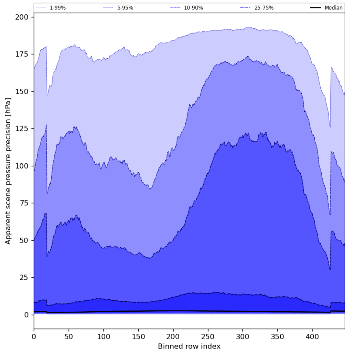
Figure 54: Along track statistics of “Apparent scene pressure precision” for 2023-09-10 to 2023-09-11
