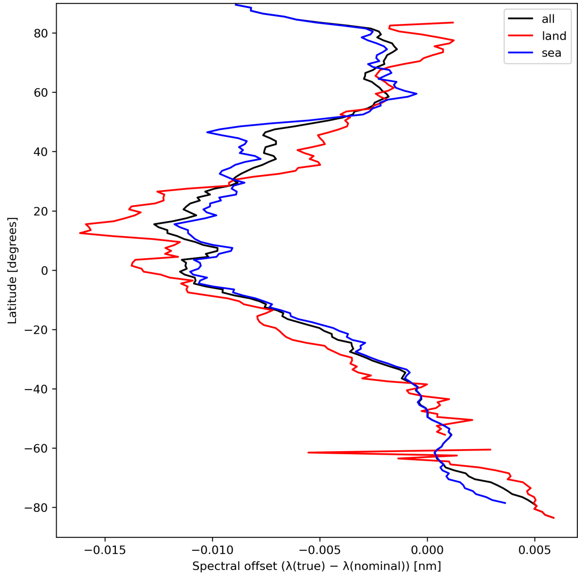
Figure 28: Zonal average of “Spectral offset ( \lambda(\text{true}) - \lambda(\text{nominal}) )” for 2023-09-10 to 2023-09-11.
