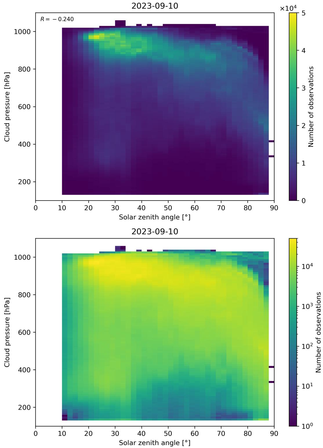
Figure 122: Scatter density plot of “Solar zenith angle” against “Cloud pressure” for 2023-09-10 to 2023-09-11.
