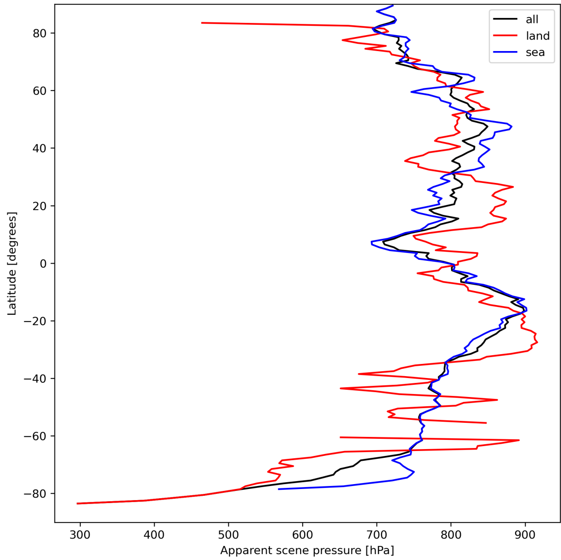
Figure 19: Zonal average of “Apparent scene pressure” for 2023-09-10 to 2023-09-11.
