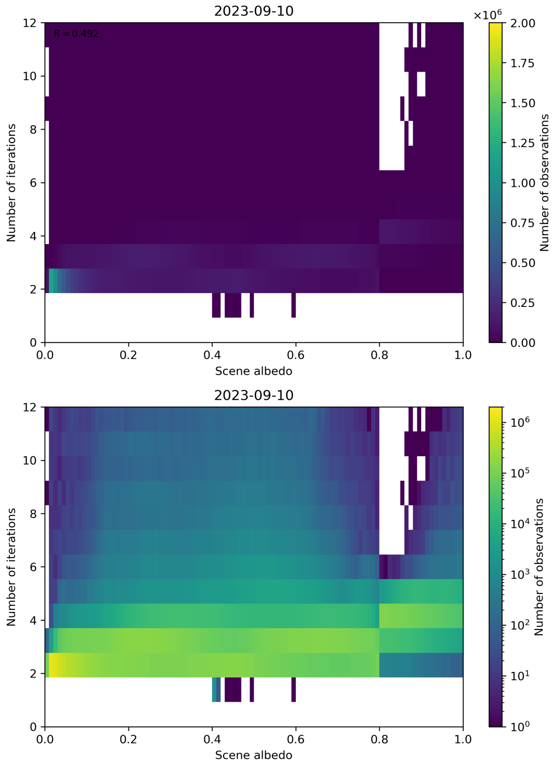
Figure 115: Scatter density plot of “Scene albedo” against “Number of iterations” for 2023-09-10 to 2023-09-11.
