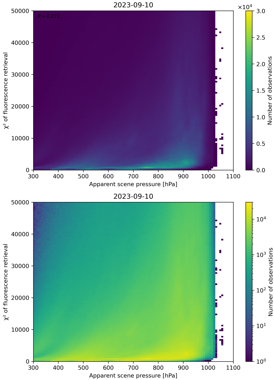
Figure 64: Scatter density plot of “Apparent scene pressure” against “ \chi^2 of fluorescence retrieval” for 2023-09-10 to 2023-09-11.
