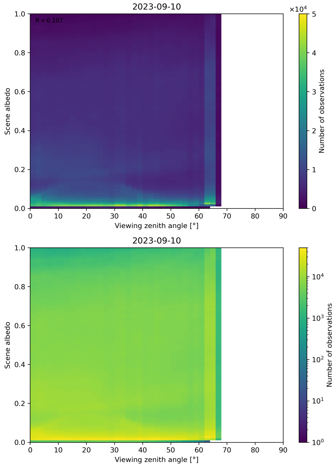
Figure 138: Scatter density plot of “Viewing zenith angle” against “Scene albedo” for 2023-09-10 to 2023-09-11.
