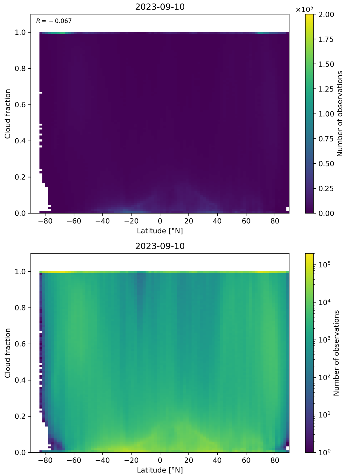
Figure 99: Scatter density plot of “Latitude” against “Cloud fraction” for 2023-09-10 to 2023-09-11.
