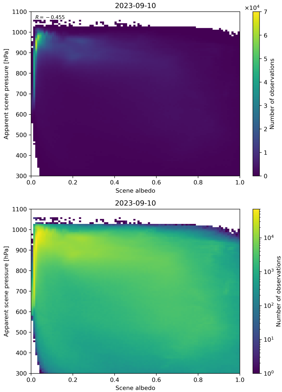
Figure 111: Scatter density plot of “Scene albedo” against “Apparent scene pressure” for 2023-09-10 to 2023-09-11.
