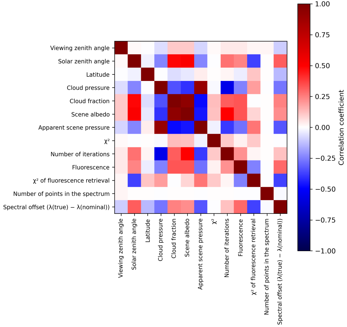
Figure 2: Map of correlation matrix for 2023-09-10 to 2023-09-11.
