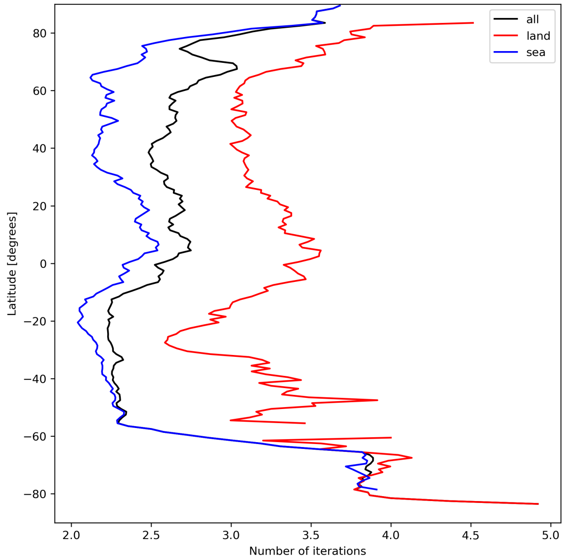
Figure 22: Zonal average of “Number of iterations” for 2023-09-10 to 2023-09-11.
