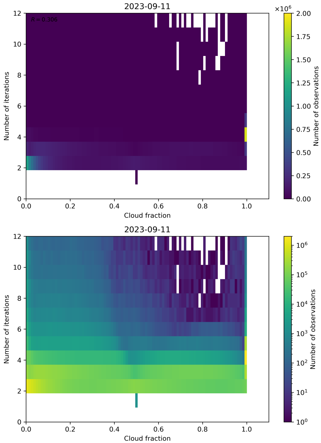
Figure 80: Scatter density plot of “Cloud fraction” against “Number of iterations” for 2023-09-10 to 2023-09-12.
