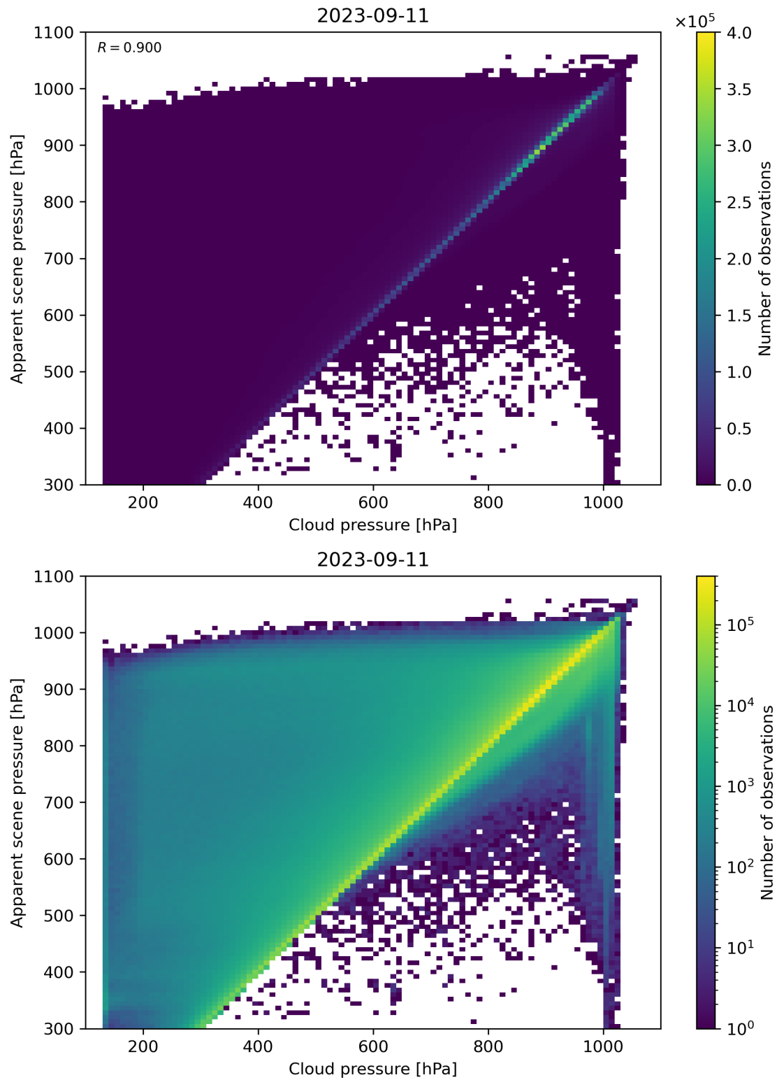
Figure 84: Scatter density plot of “Cloud pressure” against “Apparent scene pressure” for 2023-09-10 to 2023-09-12.
