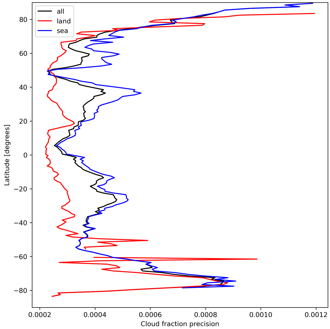
Figure 16: Zonal average of “Cloud fraction precision” for 2023-09-10 to 2023-09-12.
