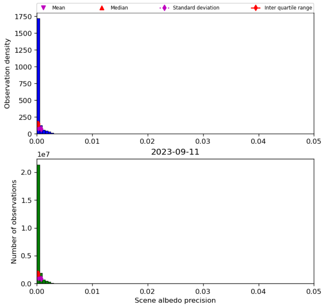
Figure 35: Histogram of “Scene albedo precision” for 2023-09-10 to 2023-09-12
