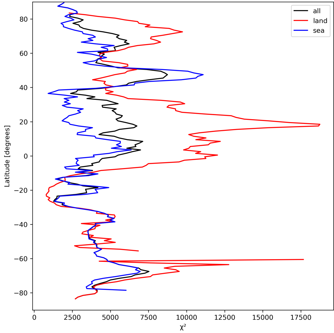
Figure 21: Zonal average of “ \chi^2 ” for 2023-09-10 to 2023-09-12.
