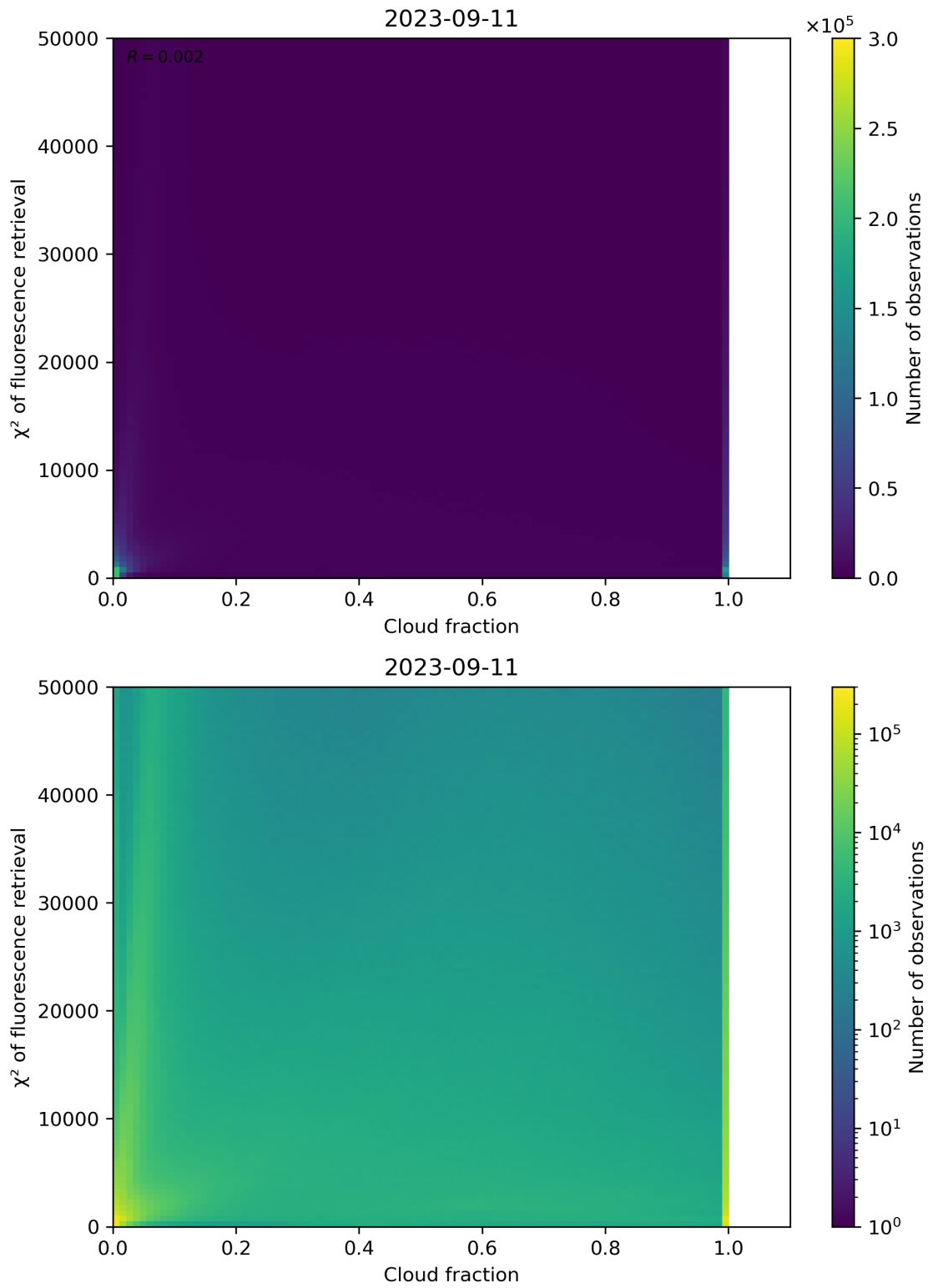
Figure 78: Scatter density plot of “Cloud fraction” against “ \chi^2 of fluorescence retrieval” for 2023-09-10 to 2023-09-12.
