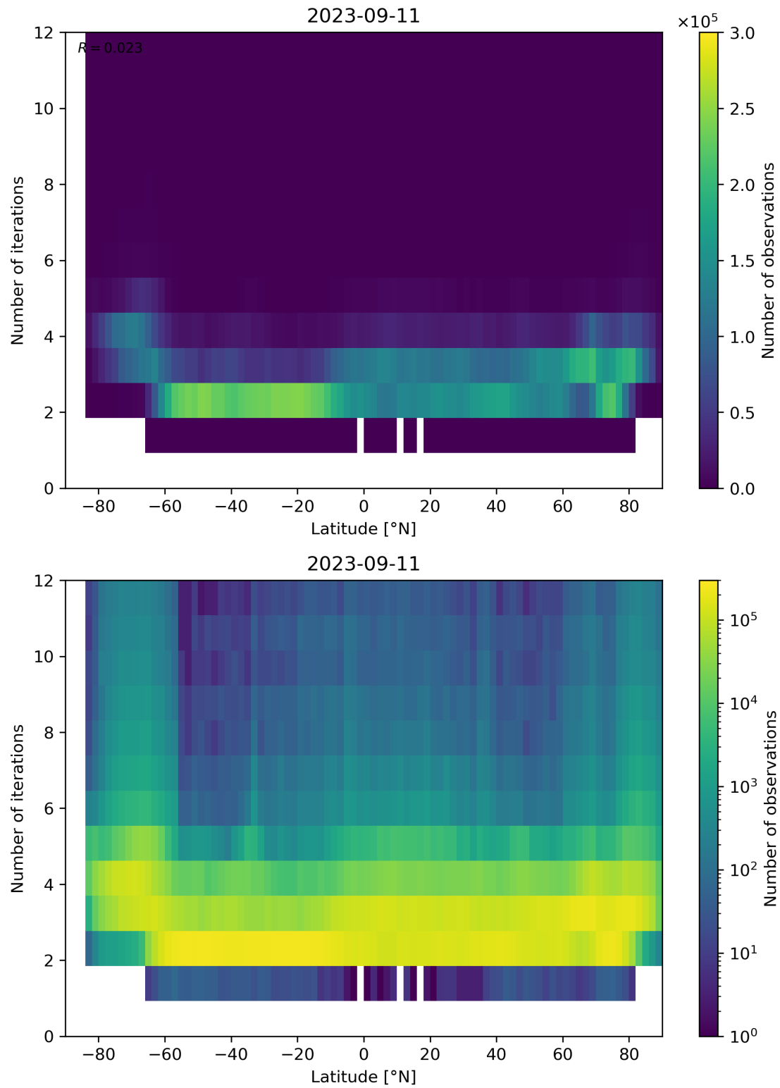
Figure 102: Scatter density plot of “Latitude” against “Number of iterations” for 2023-09-10 to 2023-09-12.
