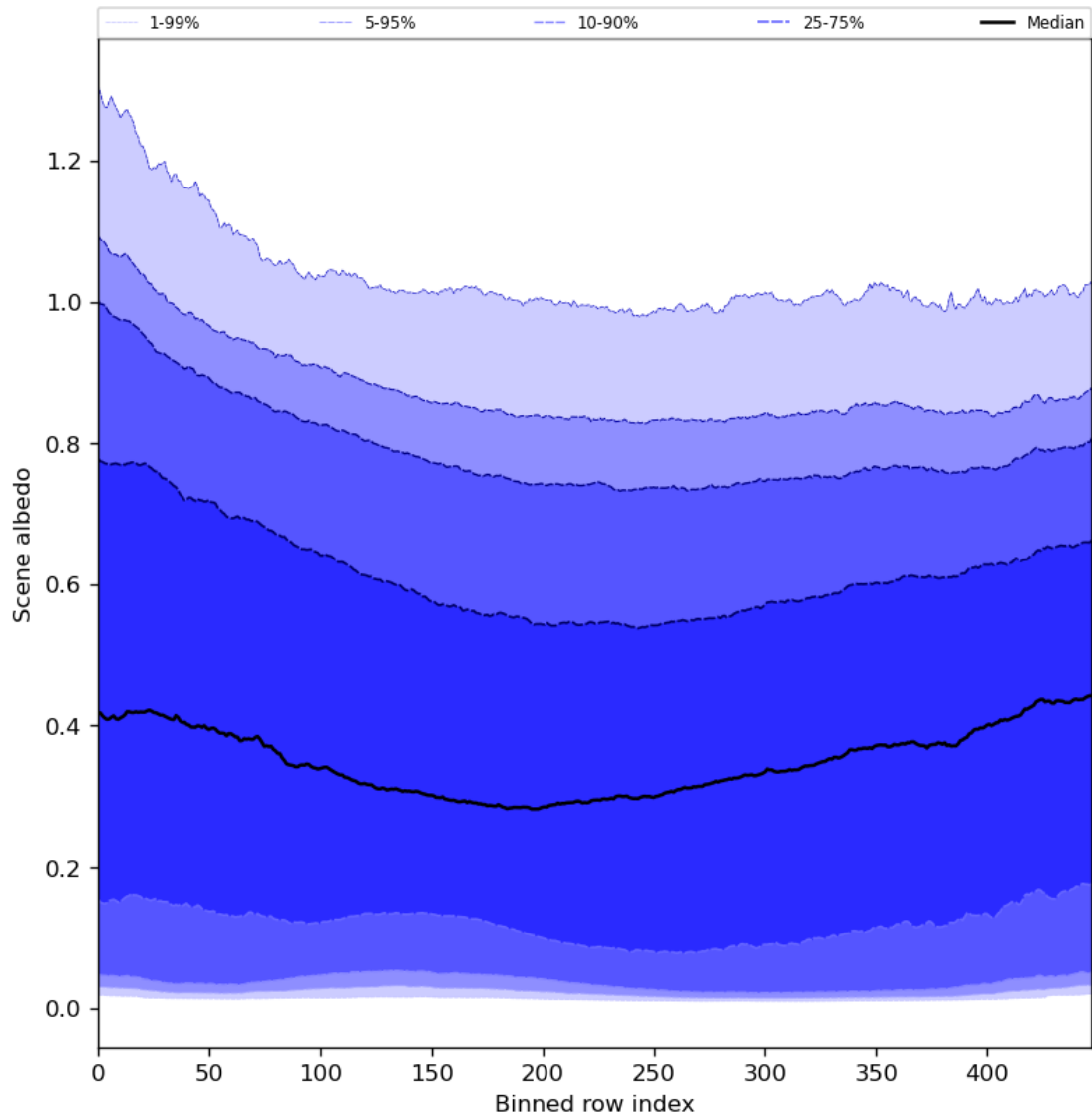
Figure 51: Along track statistics of “Scene albedo” for 2023-09-10 to 2023-09-12
