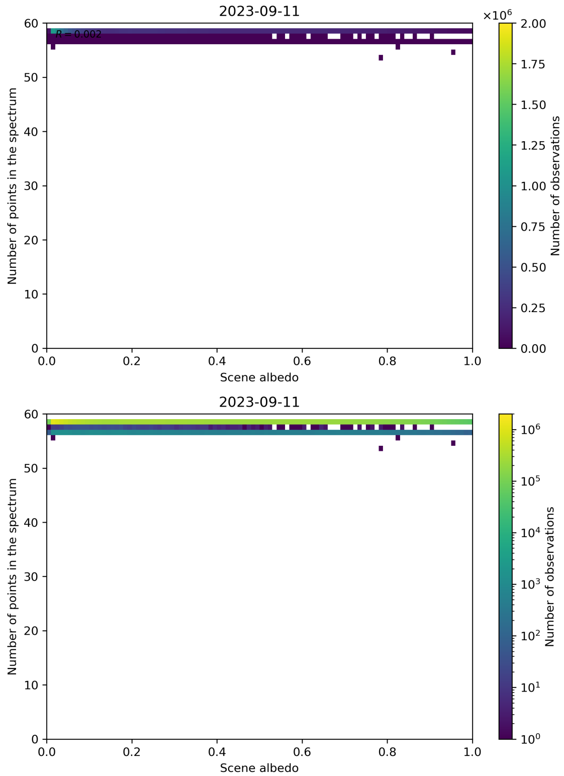
Figure 116: Scatter density plot of “Scene albedo” against “Number of points in the spectrum” for 2023-09-10 to 2023-09-12.
