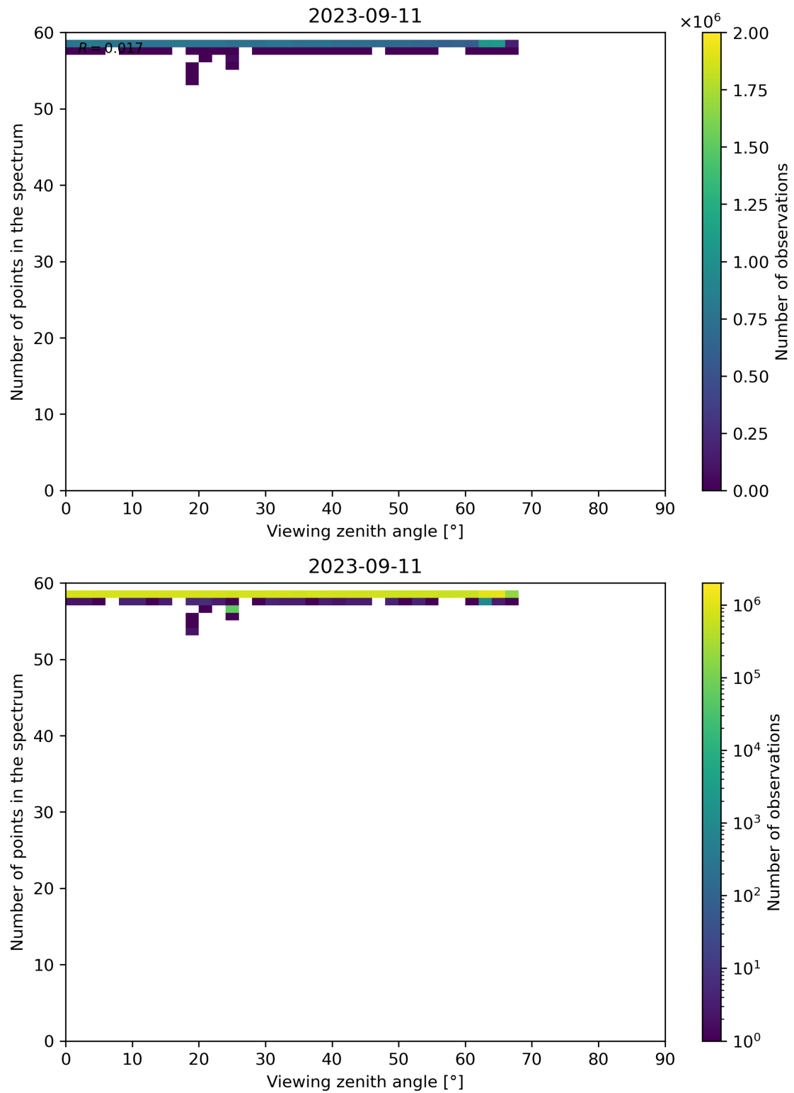
Figure 137: Scatter density plot of “Viewing zenith angle” against “Number of points in the spectrum” for 2023-09-10 to 2023-09-12.
