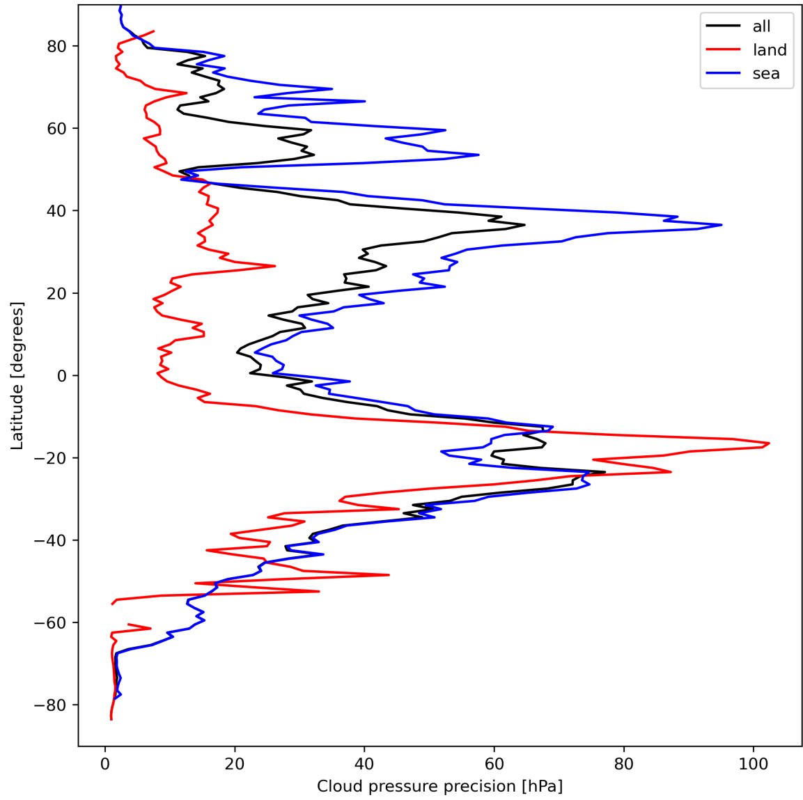
Figure 14: Zonal average of “Cloud pressure precision” for 2023-09-10 to 2023-09-12.
