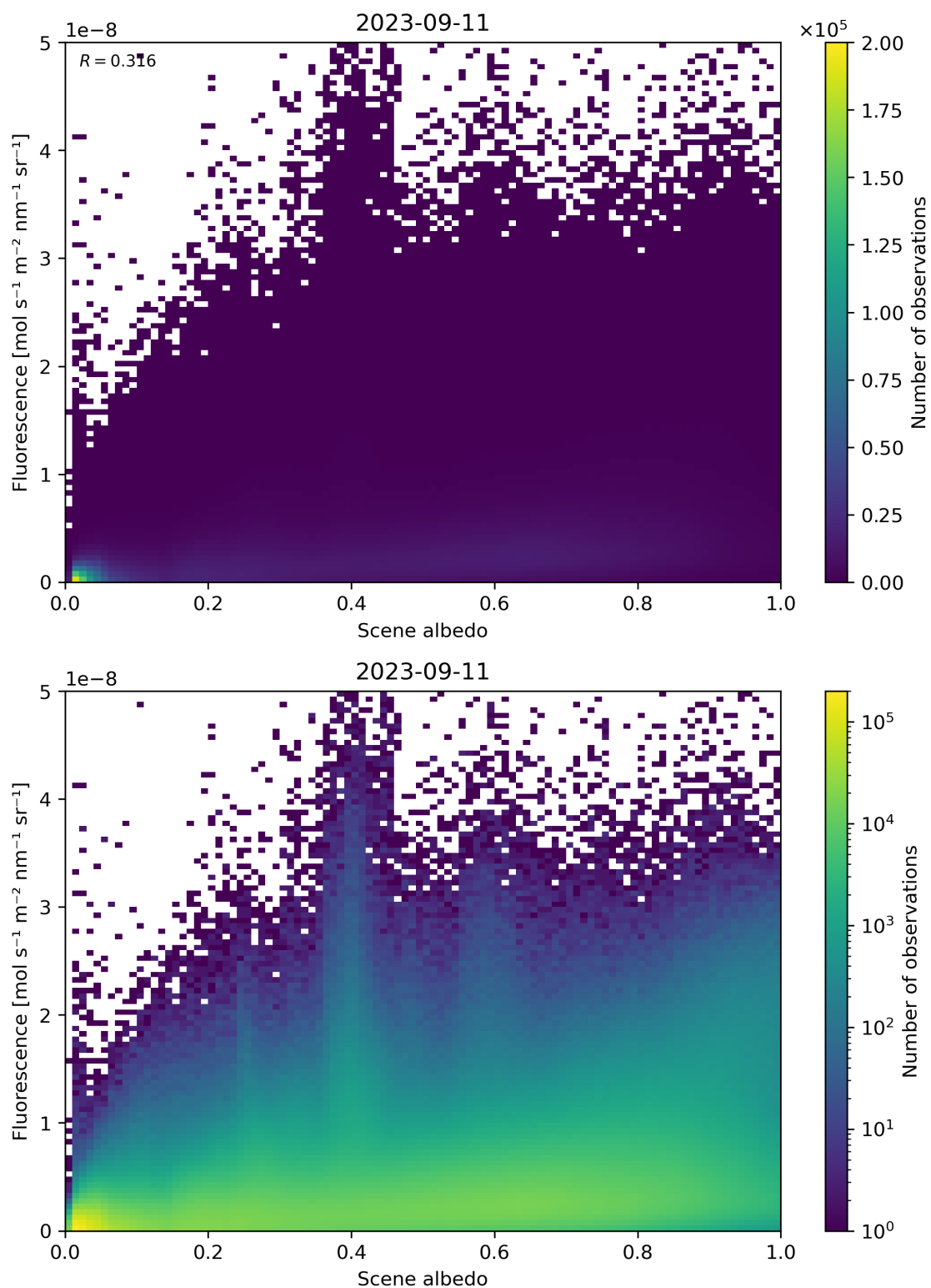
Figure 114: Scatter density plot of “Scene albedo” against “Fluorescence” for 2023-09-10 to 2023-09-12.
