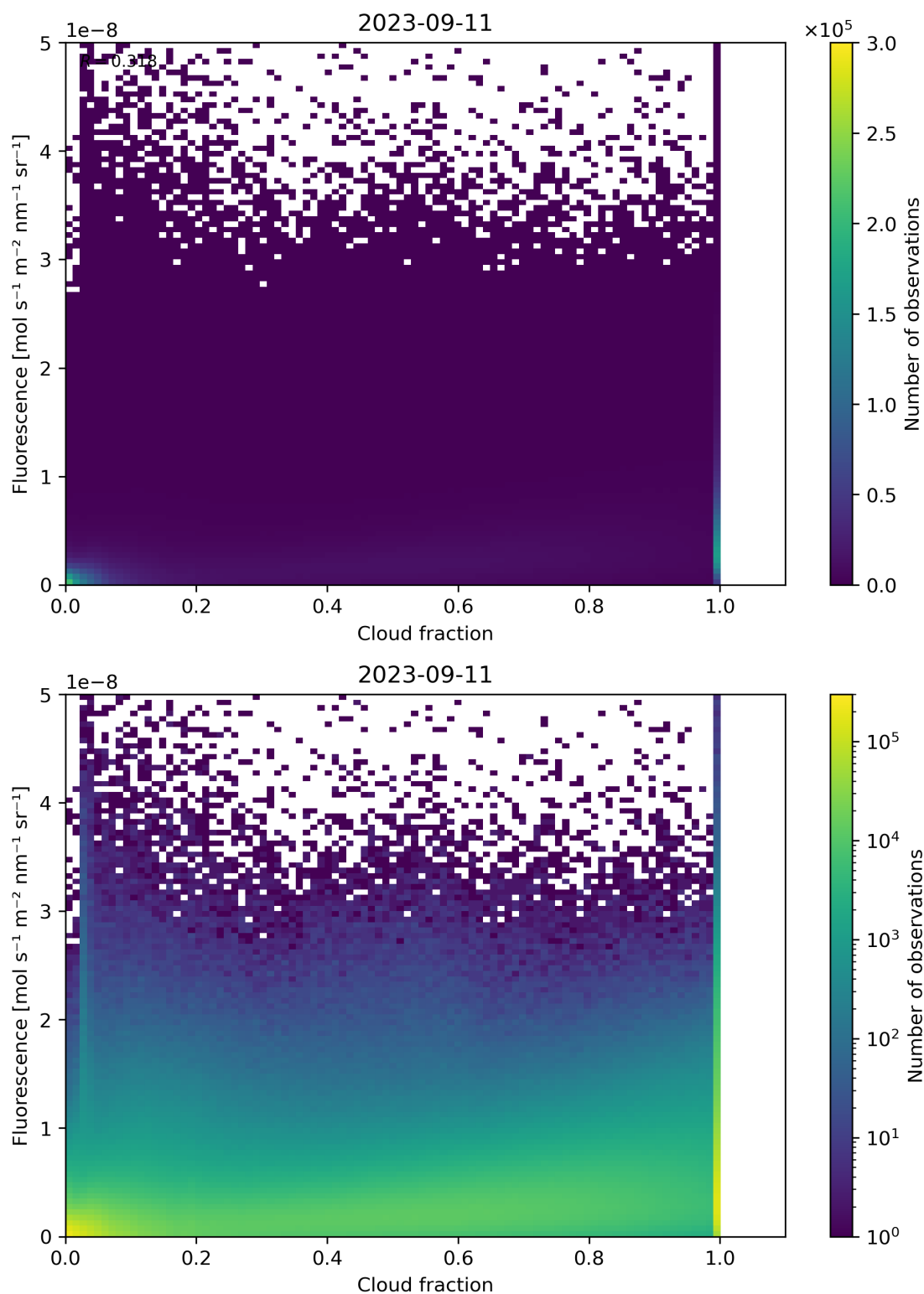
Figure 79: Scatter density plot of “Cloud fraction” against “Fluorescence” for 2023-09-10 to 2023-09-12.
