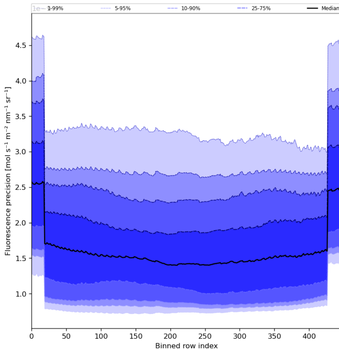
Figure 58: Along track statistics of “Fluorescence precision” for 2023-09-10 to 2023-09-12
