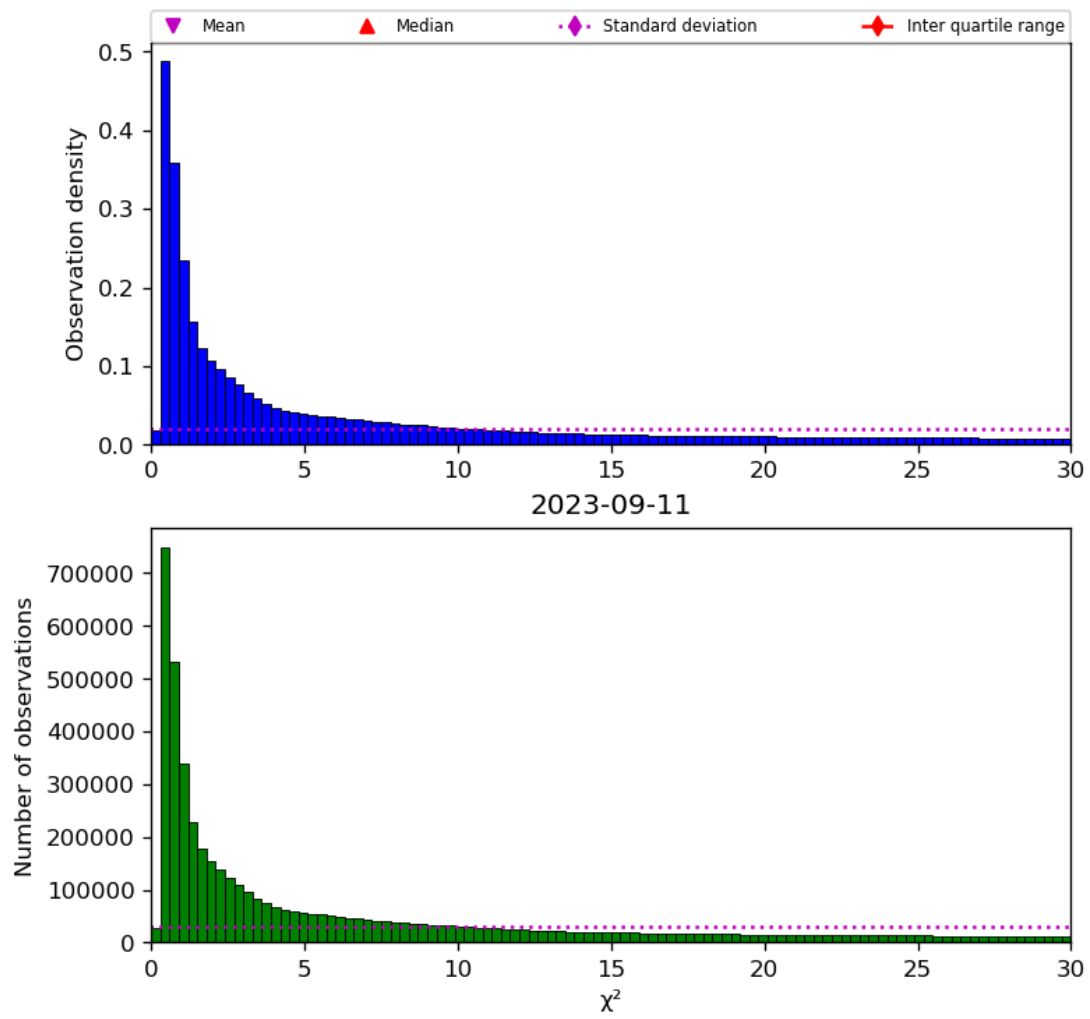
Figure 38: Histogram of “ \chi^2 ” for 2023-09-10 to 2023-09-12
