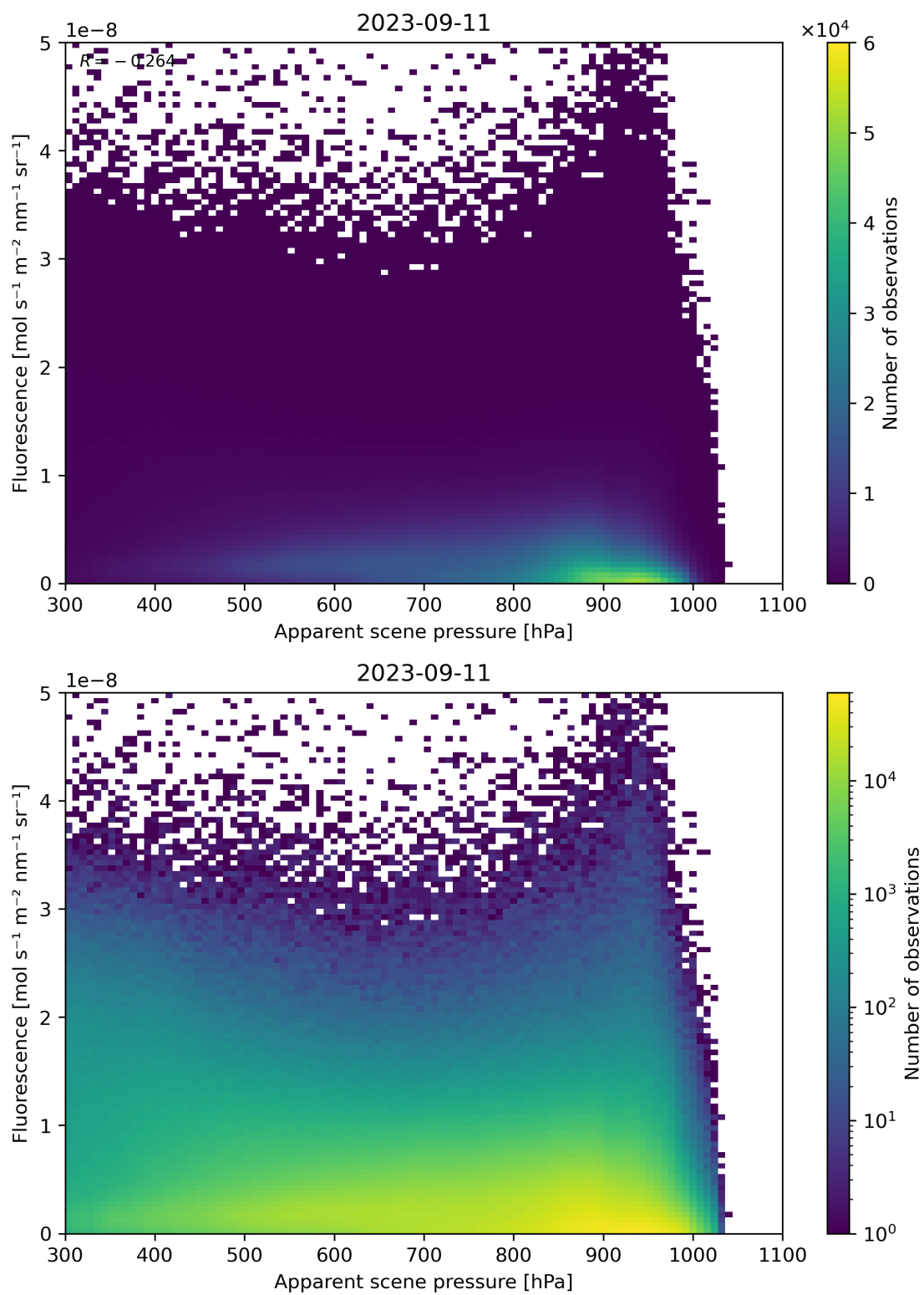
Figure 65: Scatter density plot of “Apparent scene pressure” against “Fluorescence” for 2023-09-10 to 2023-09-12.
