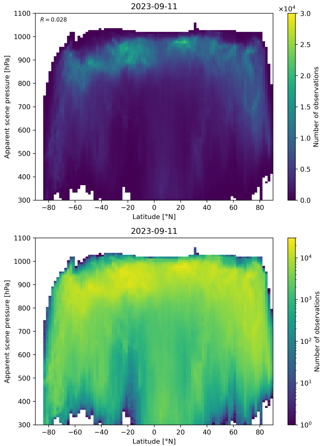
Figure 96: Scatter density plot of “Latitude” against “Apparent scene pressure” for 2023-09-10 to 2023-09-12.
