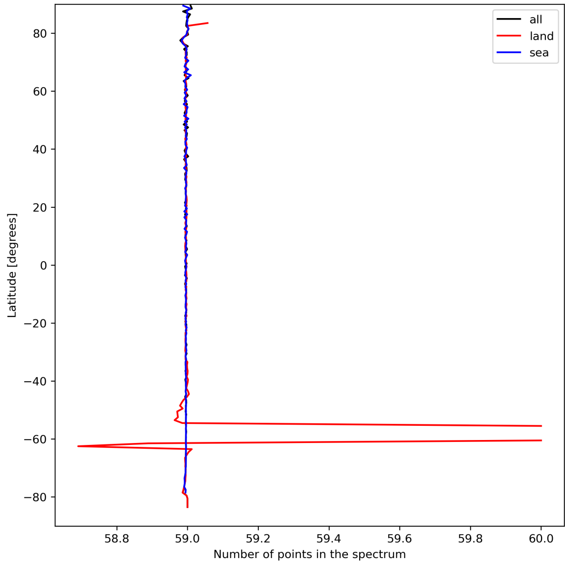
Figure 27: Zonal average of “Number of points in the spectrum” for 2023-09-10 to 2023-09-12.
