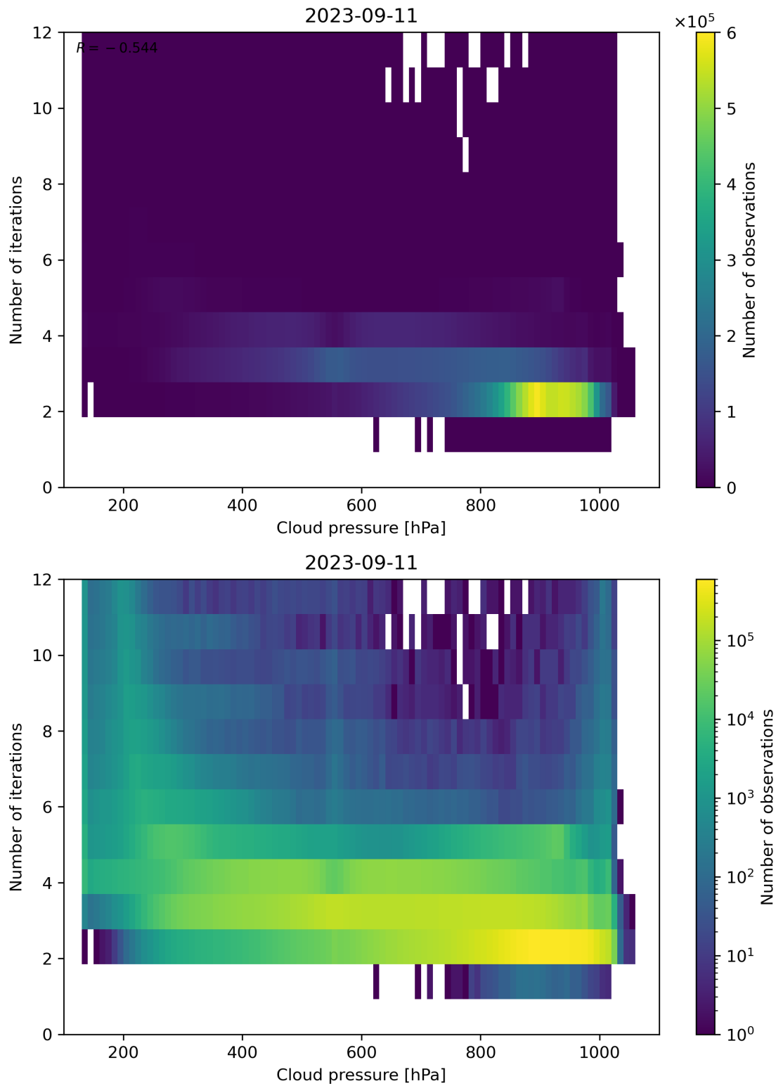
Figure 89: Scatter density plot of “Cloud pressure” against “Number of iterations” for 2023-09-10 to 2023-09-12.
