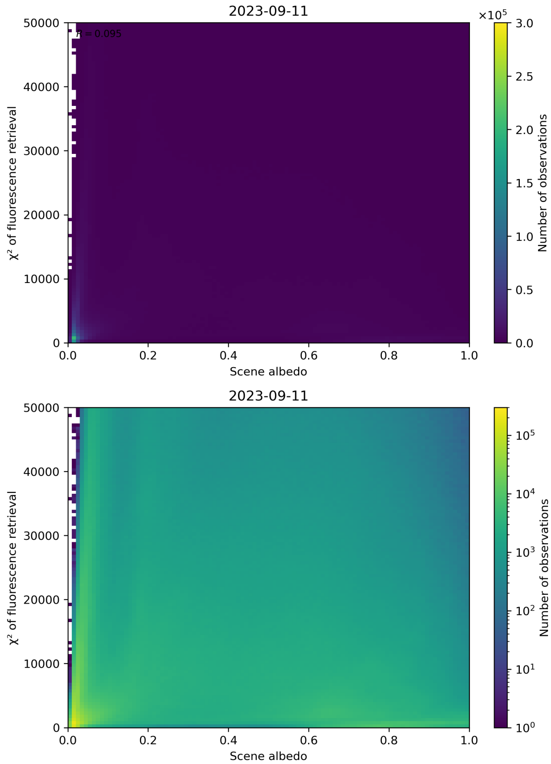
Figure 113: Scatter density plot of “Scene albedo” against “ \chi^2 of fluorescence retrieval” for 2023-09-10 to 2023-09-12.
