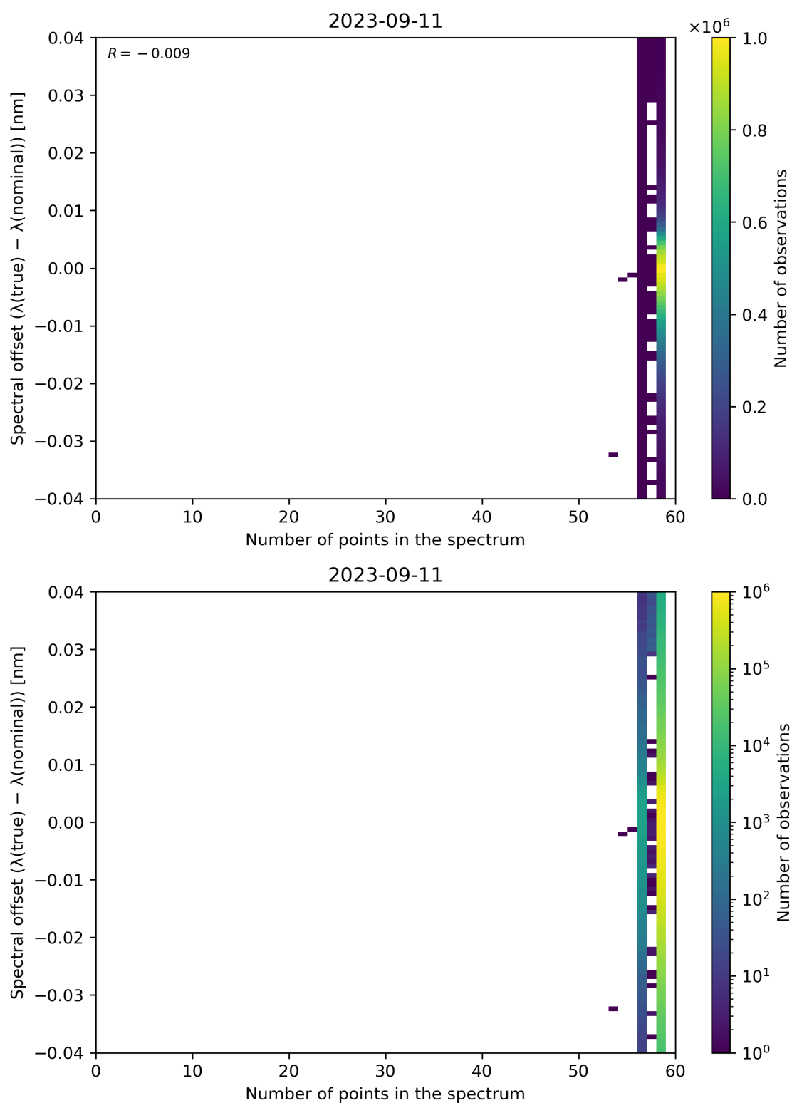
Figure 110: Scatter density plot of “Number of points in the spectrum” against “Spectral offset ( \lambda(\text{true}) - \lambda(\text{nominal}) )” for 2023-09-10 to 2023-09-12.
