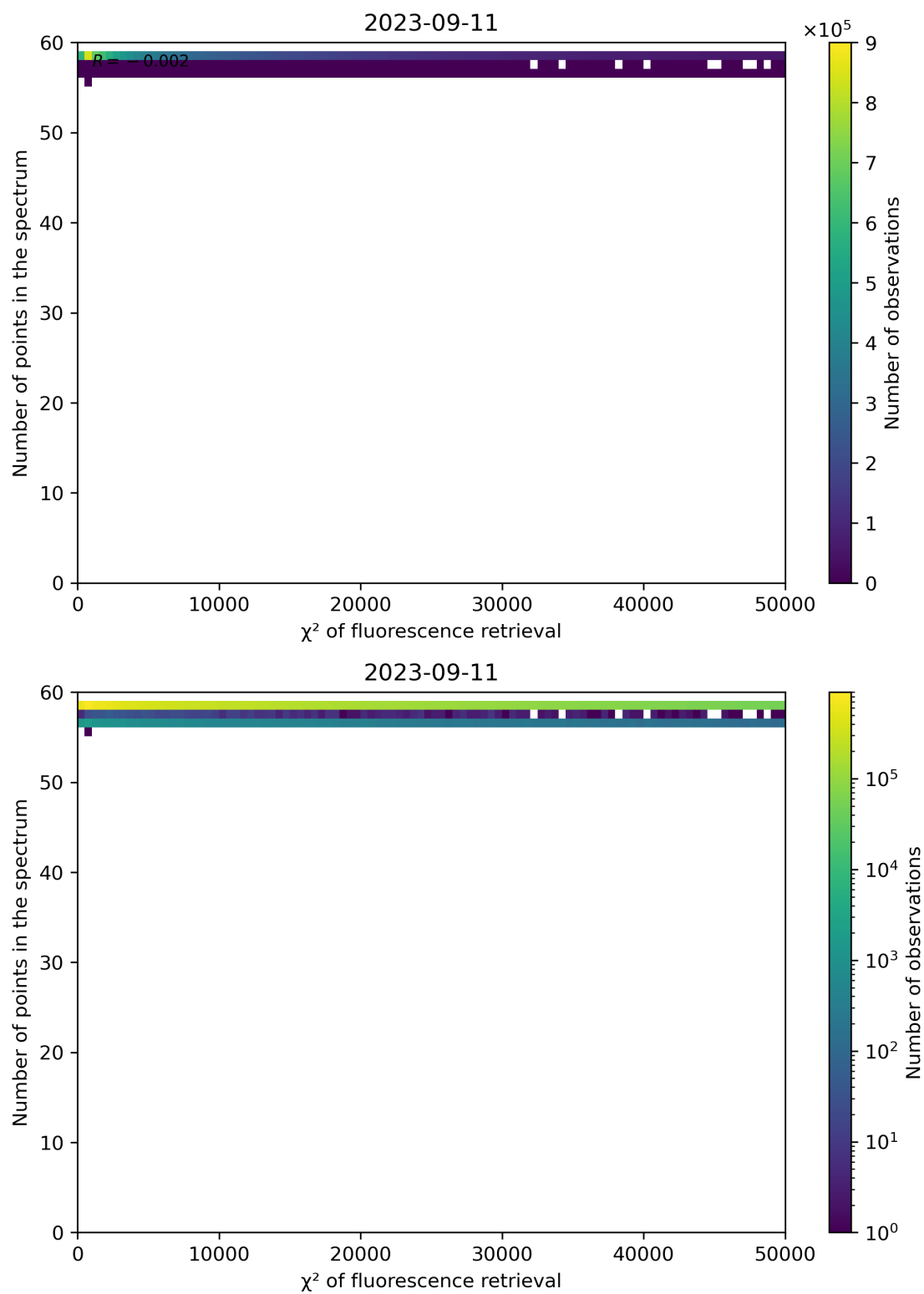
Figure 71: Scatter density plot of " \chi^2 of fluorescence retrieval" against "Number of points in the spectrum" for 2023-09-10 to 2023-09-12.
