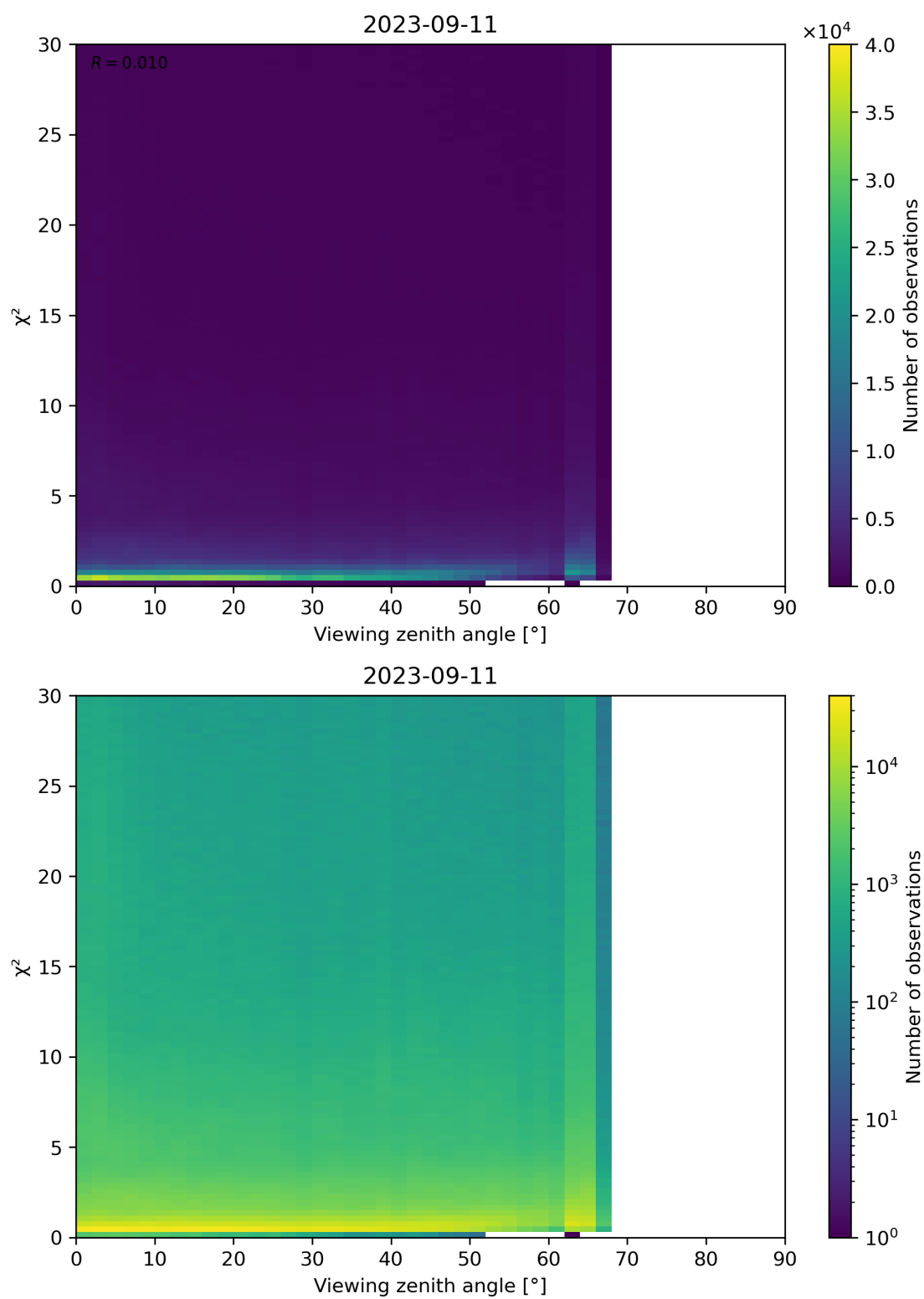
Figure 130: Scatter density plot of “Viewing zenith angle” against “ \chi^2 ” for 2023-09-10 to 2023-09-12.
