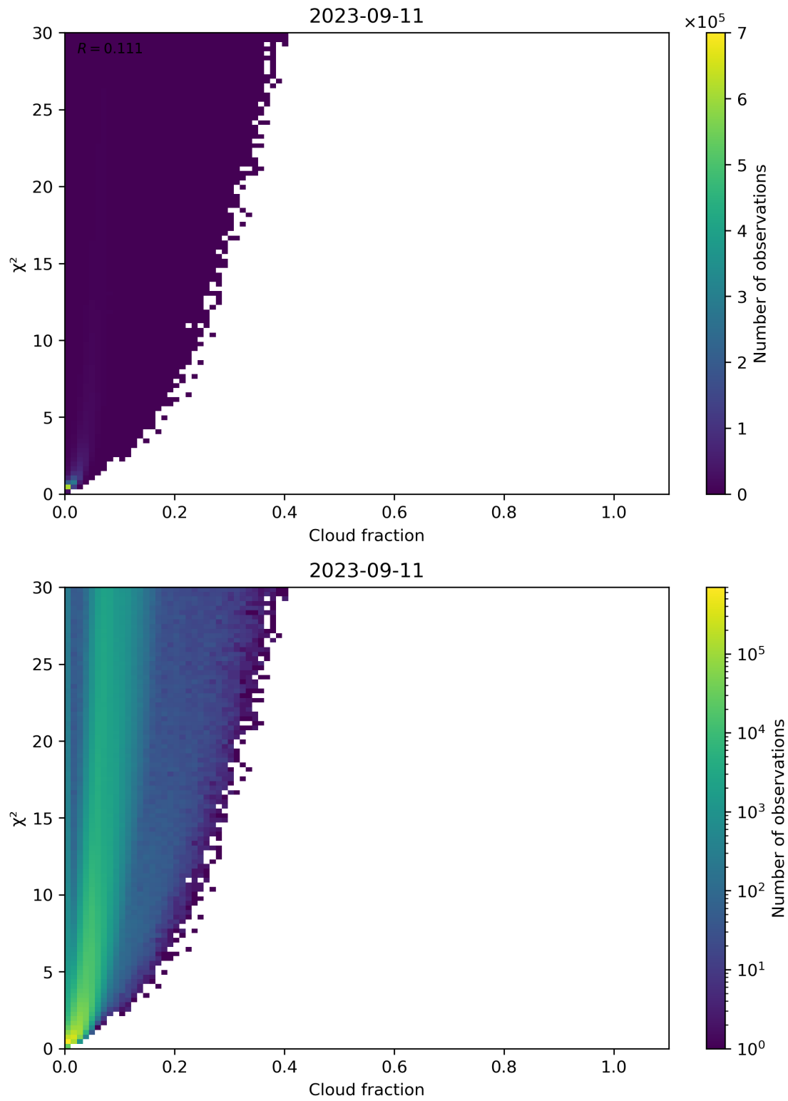
Figure 77: Scatter density plot of “Cloud fraction” against “ \chi^2 ” for 2023-09-10 to 2023-09-12.
