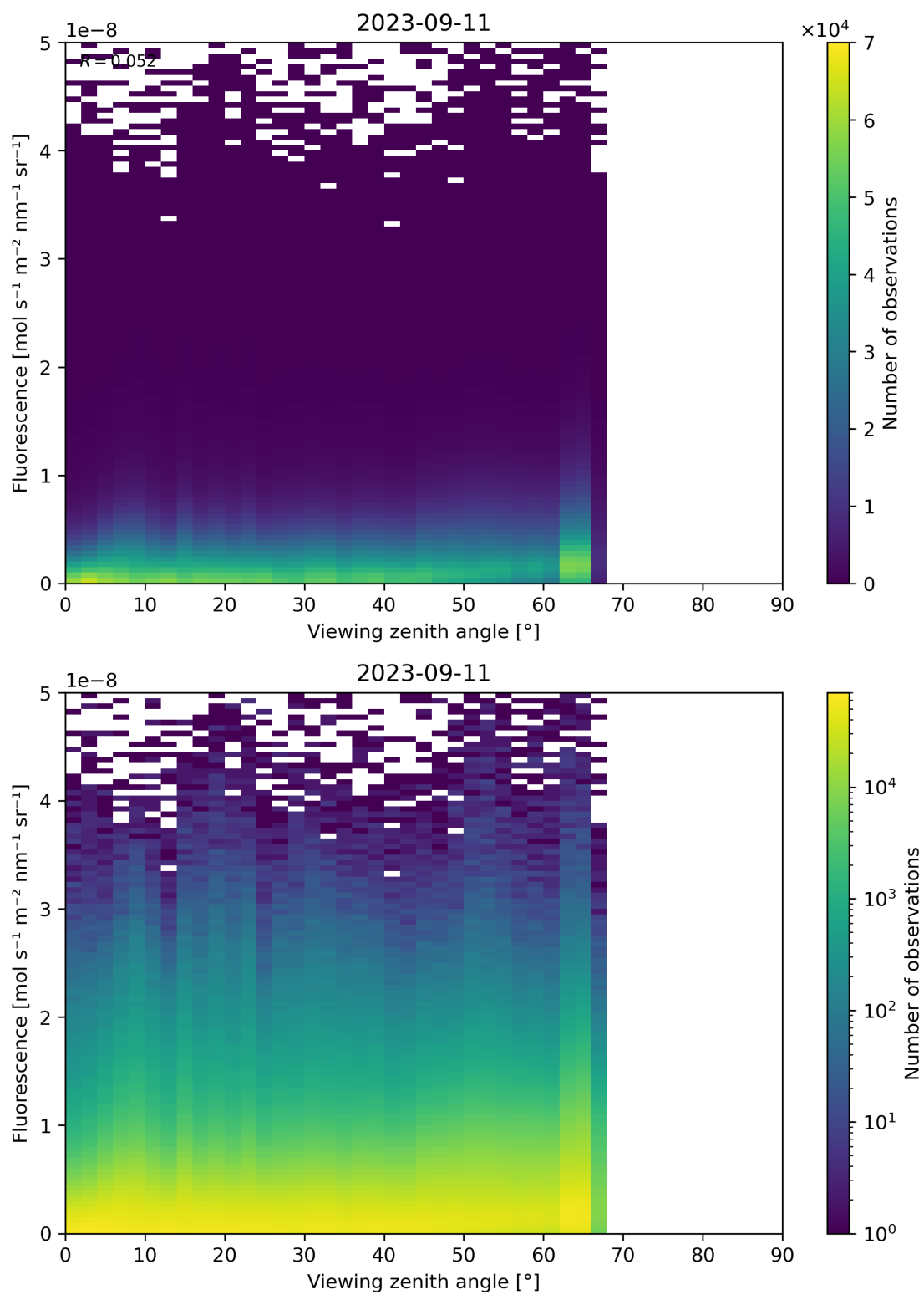
Figure 134: Scatter density plot of “Viewing zenith angle” against “Fluorescence” for 2023-09-10 to 2023-09-12.
