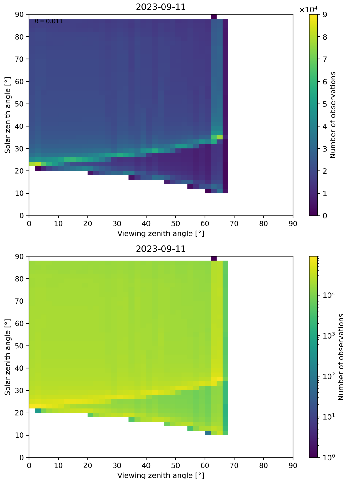
Figure 139: Scatter density plot of “Viewing zenith angle” against “Solar zenith angle” for 2023-09-10 to 2023-09-12.
