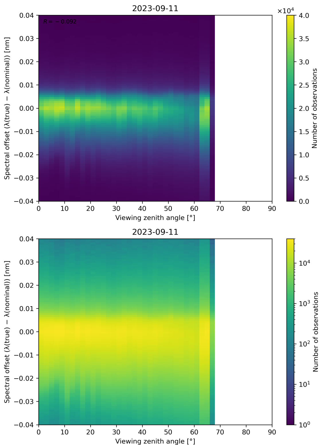
Figure 140: Scatter density plot of “Viewing zenith angle” against “Spectral offset ( \lambda(\text{true}) - \lambda(\text{nominal}) )” for 2023-09-10 to 2023-09-12.
