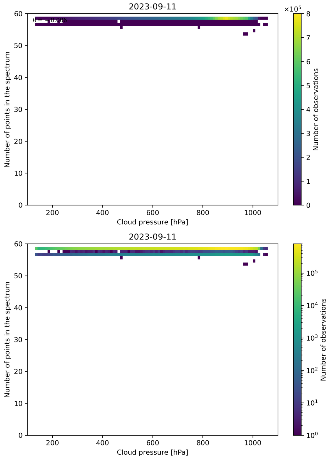
Figure 90: Scatter density plot of “Cloud pressure” against “Number of points in the spectrum” for 2023-09-10 to 2023-09-12.
