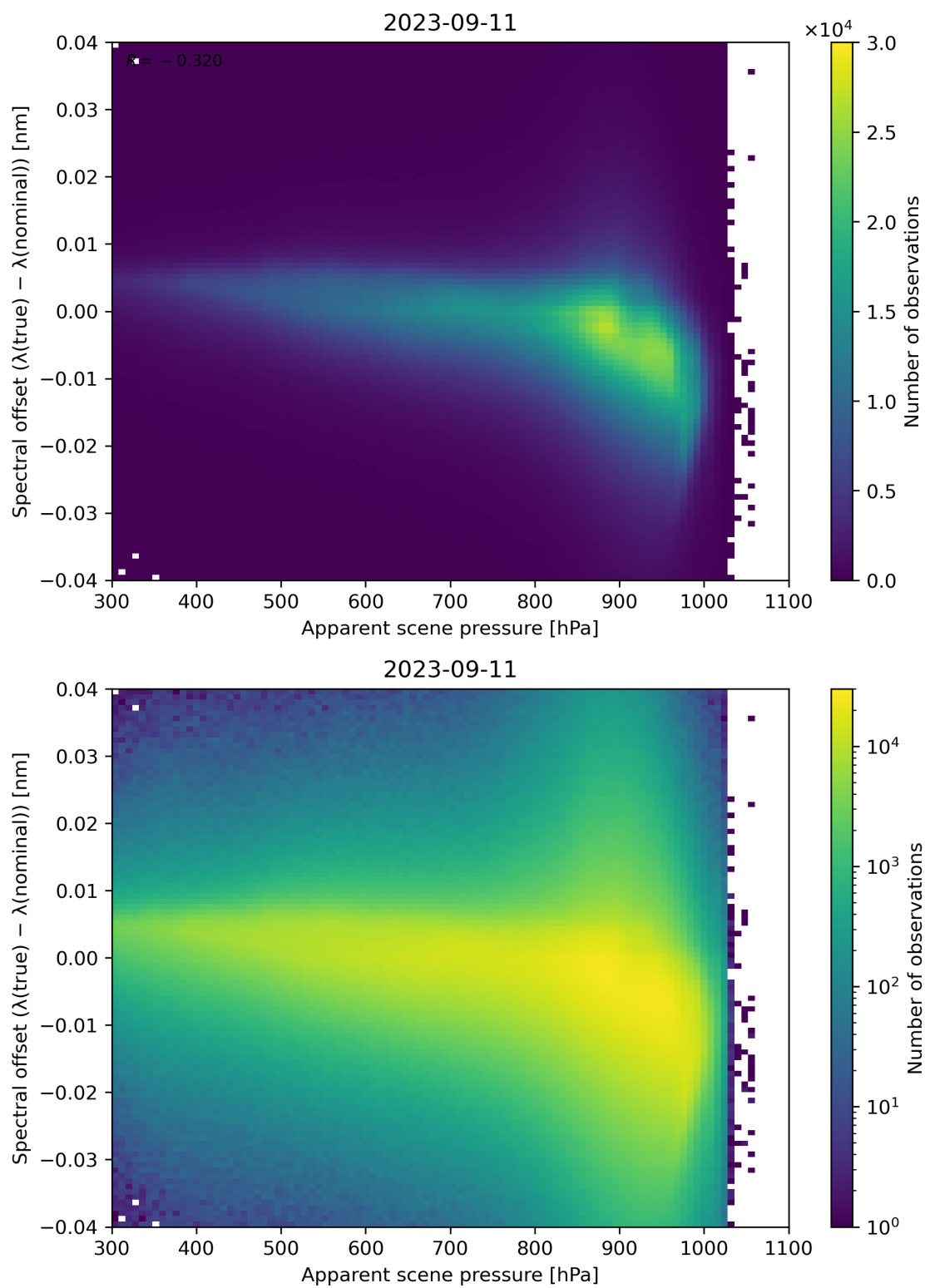
Figure 68: Scatter density plot of “Apparent scene pressure” against “Spectral offset ( \lambda(\text{true}) - \lambda(\text{nominal}) )” for 2023-09-10 to 2023-09-12.
