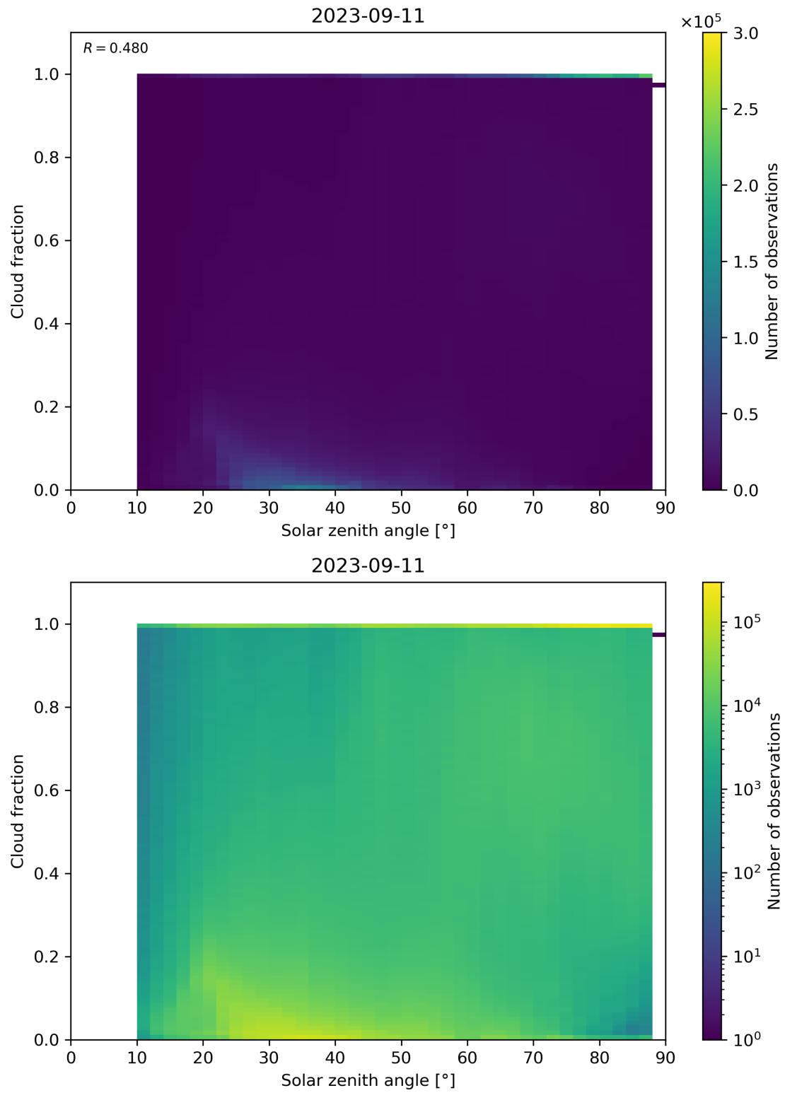
Figure 121: Scatter density plot of “Solar zenith angle” against “Cloud fraction” for 2023-09-10 to 2023-09-12.
