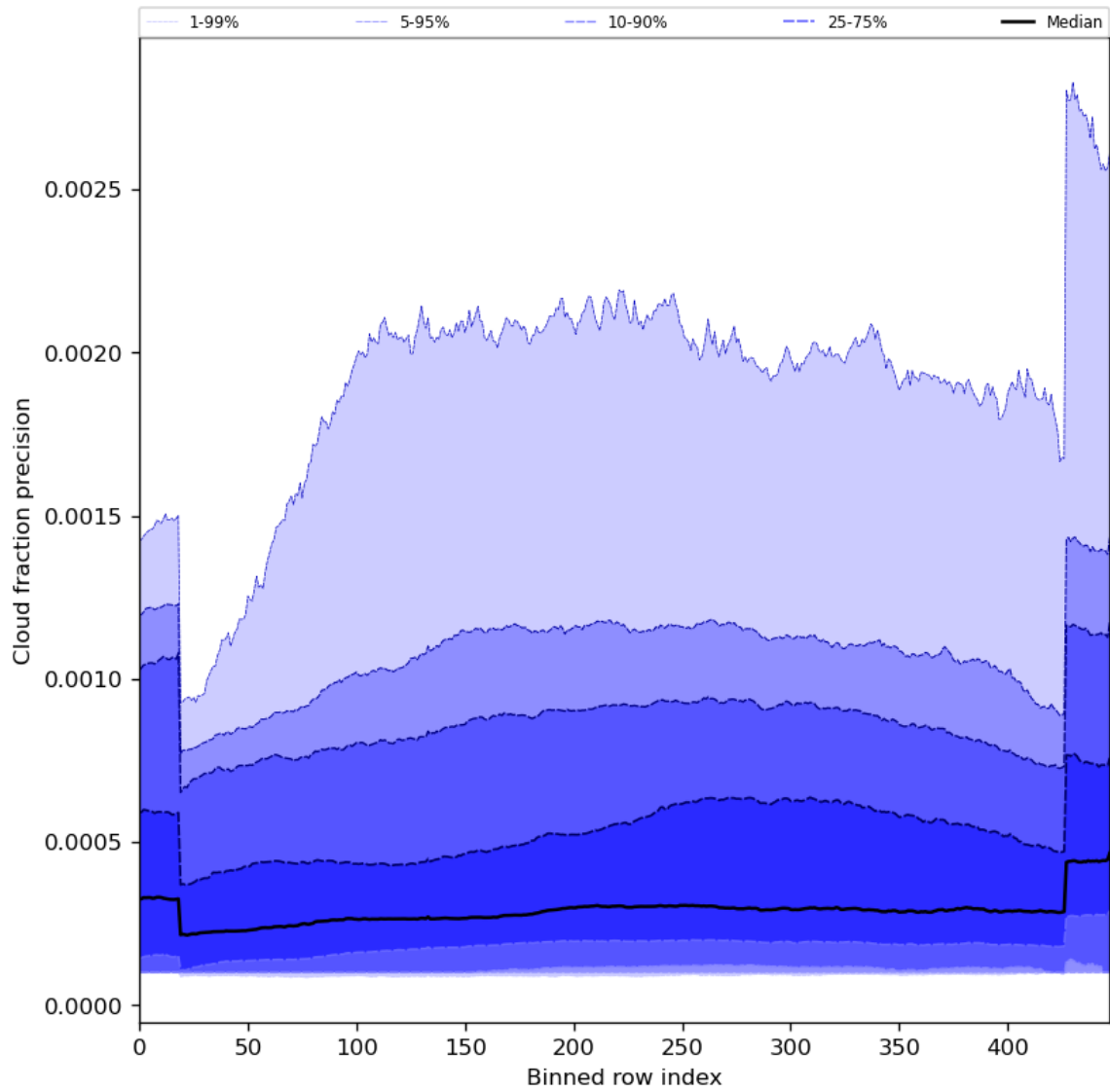
Figure 50: Along track statistics of “Cloud fraction precision” for 2023-09-10 to 2023-09-12
