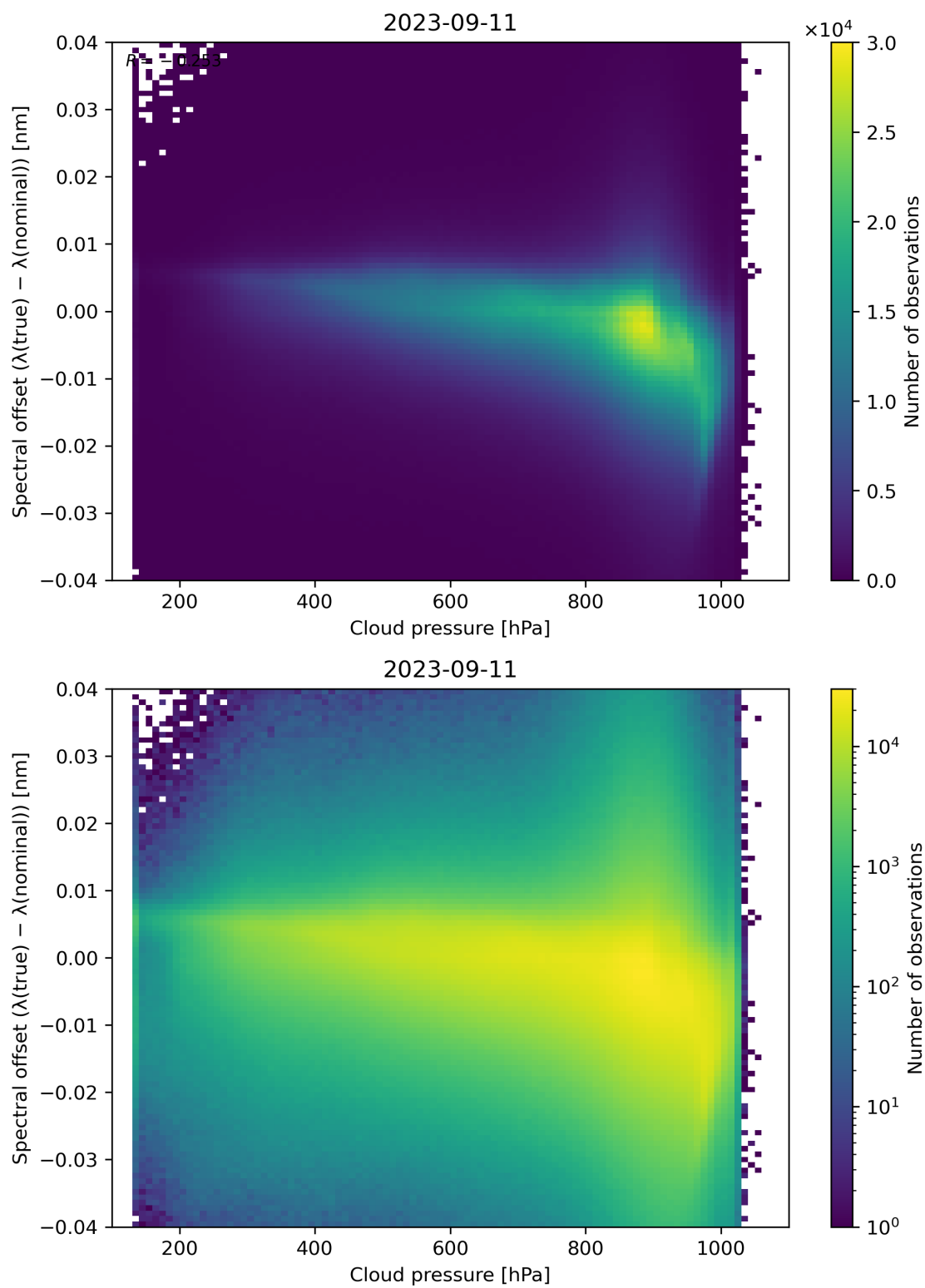
Figure 92: Scatter density plot of “Cloud pressure” against “Spectral offset ( \lambda(\text{true}) - \lambda(\text{nominal}) )” for 2023-09-10 to 2023-09-12.
