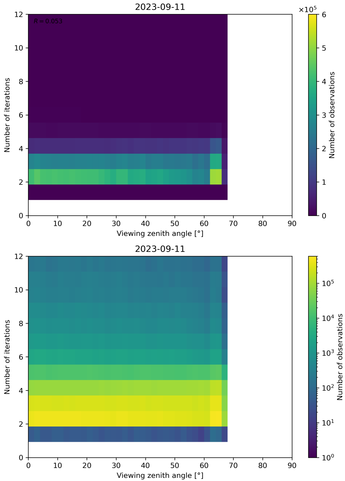
Figure 136: Scatter density plot of “Viewing zenith angle” against “Number of iterations” for 2023-09-10 to 2023-09-12.
