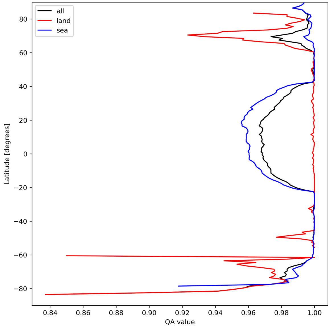
Figure 12: Zonal average of “QA value” for 2023-09-10 to 2023-09-12.
