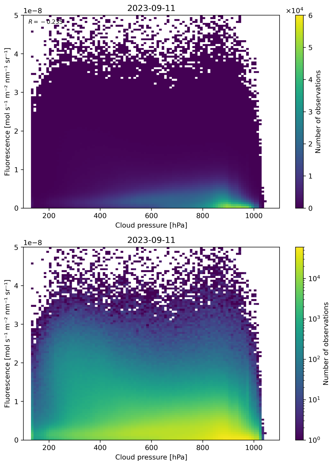
Figure 88: Scatter density plot of “Cloud pressure” against “Fluorescence” for 2023-09-10 to 2023-09-12.
