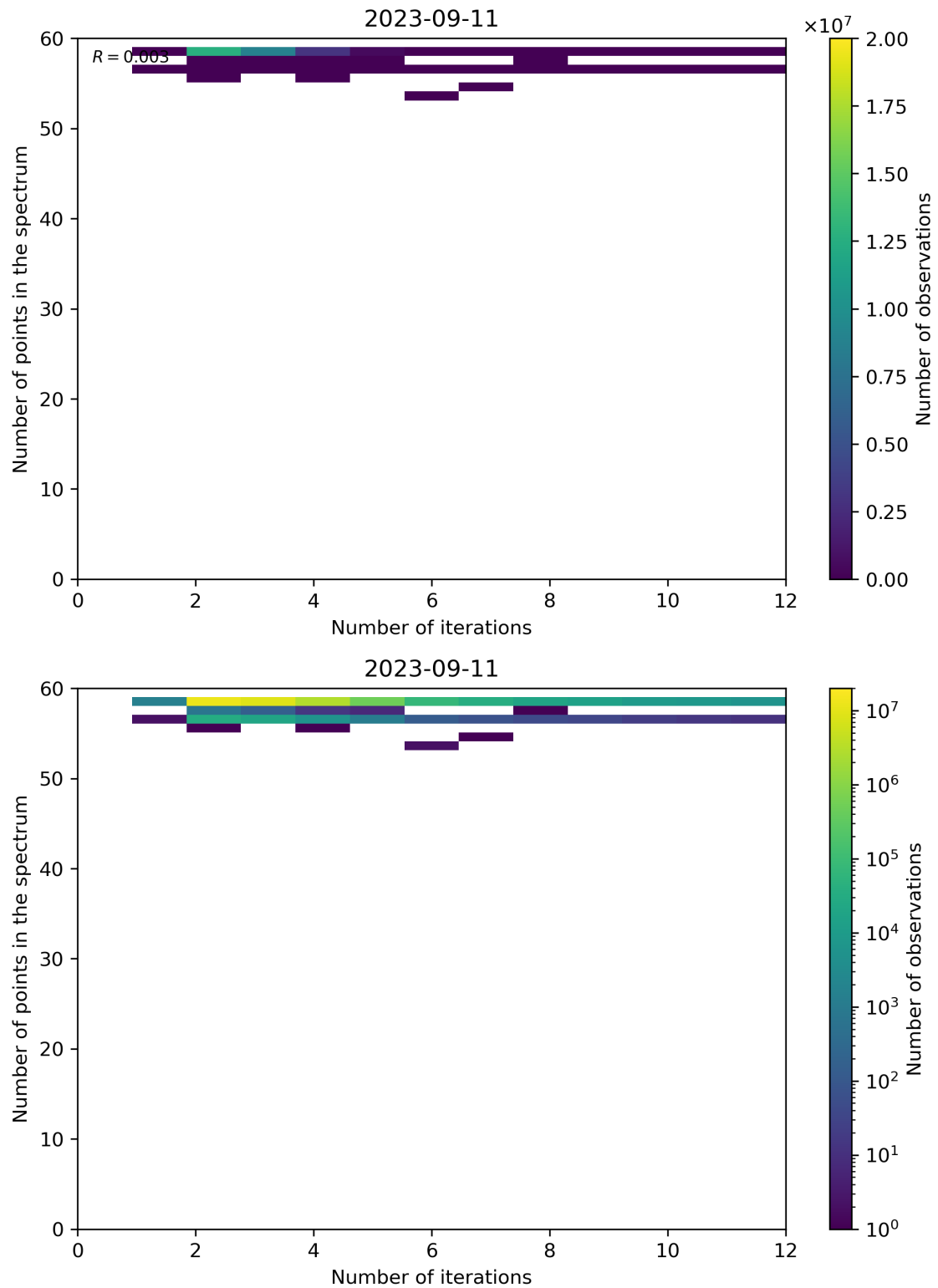
Figure 108: Scatter density plot of “Number of iterations” against “Number of points in the spectrum” for 2023-09-10 to 2023-09-12.
