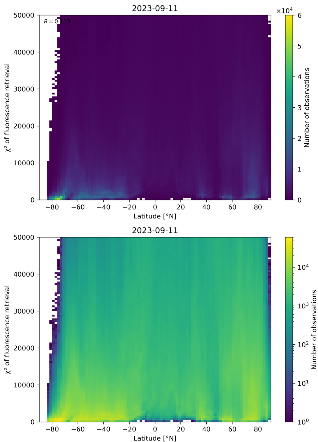
Figure 98: Scatter density plot of “Latitude” against “ \chi^2 of fluorescence retrieval” for 2023-09-10 to 2023-09-12.
