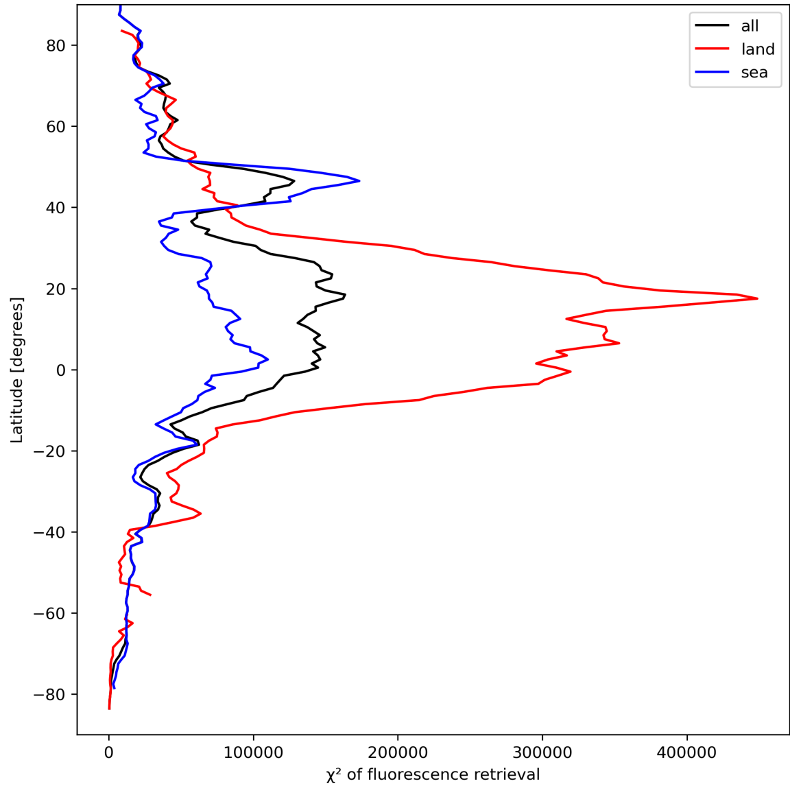
Figure 25: Zonal average of “ \chi^2 of fluorescence retrieval” for 2023-09-10 to 2023-09-12.
