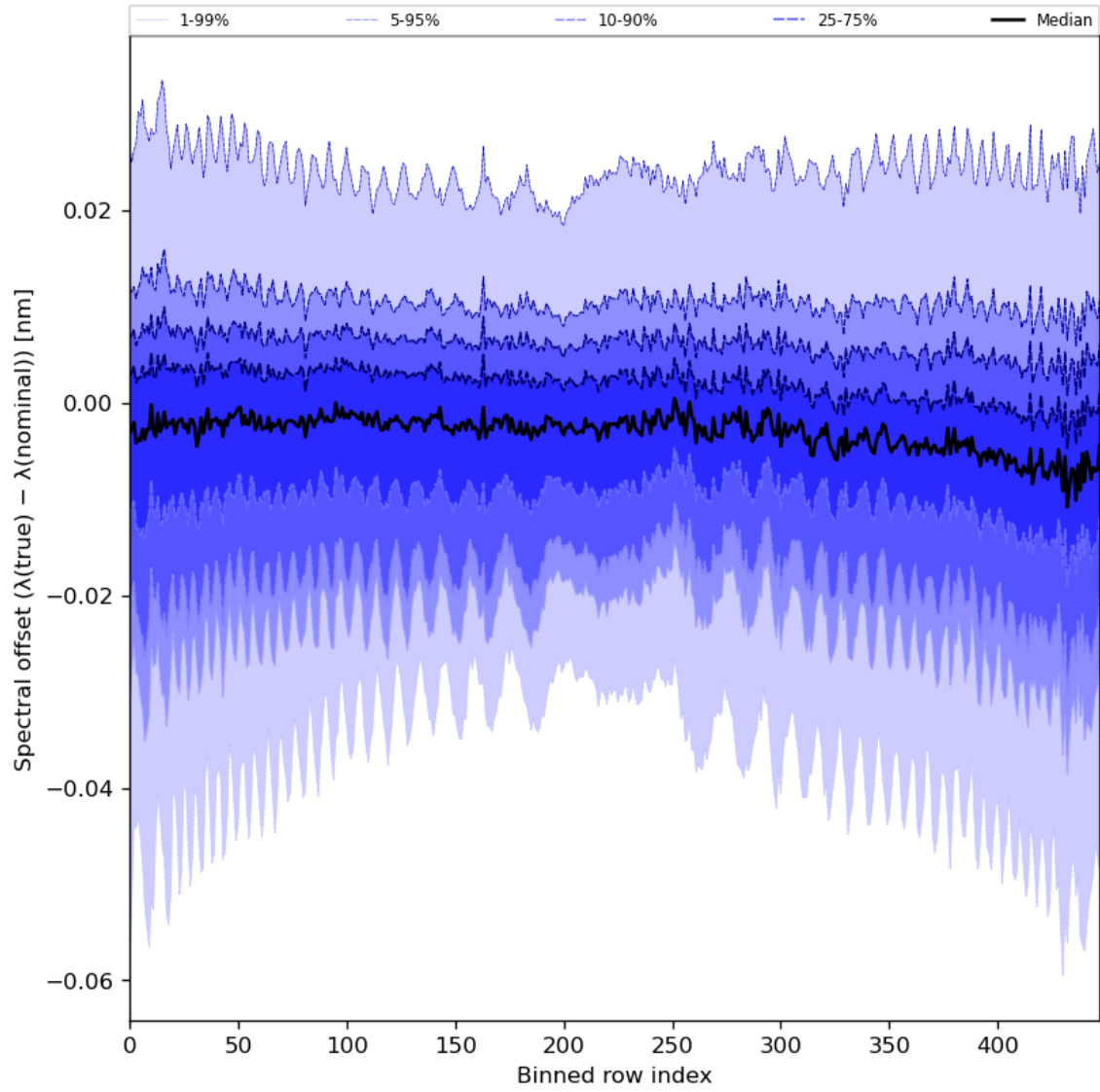
Figure 62: Along track statistics of “Spectral offset ( \lambda(\text{true}) - \lambda(\text{nominal}) )” for 2023-09-10 to 2023-09-12
