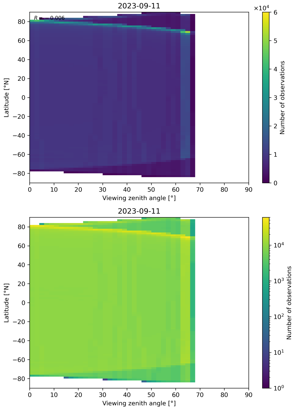
Figure 135: Scatter density plot of “Viewing zenith angle” against “Latitude” for 2023-09-10 to 2023-09-12.
