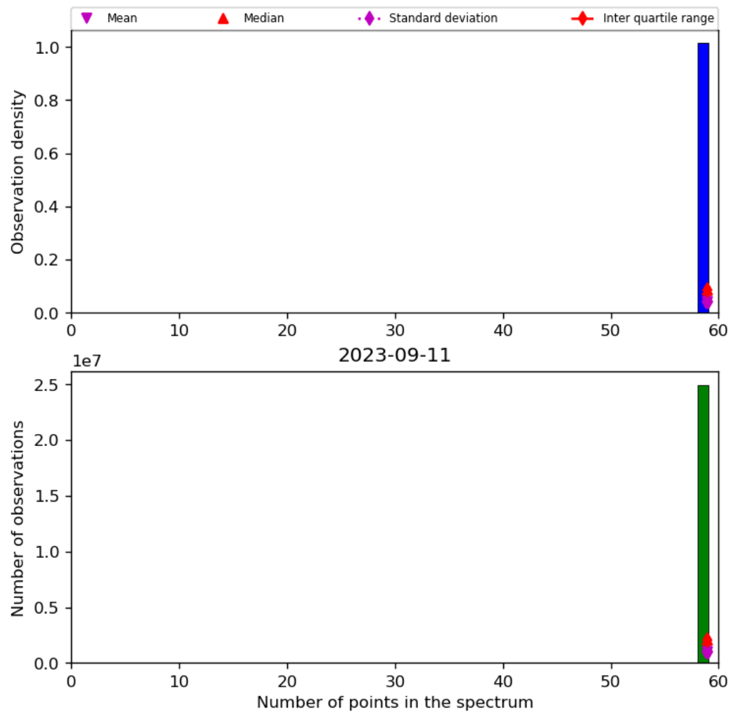
Figure 44: Histogram of “Number of points in the spectrum” for 2023-09-10 to 2023-09-12
