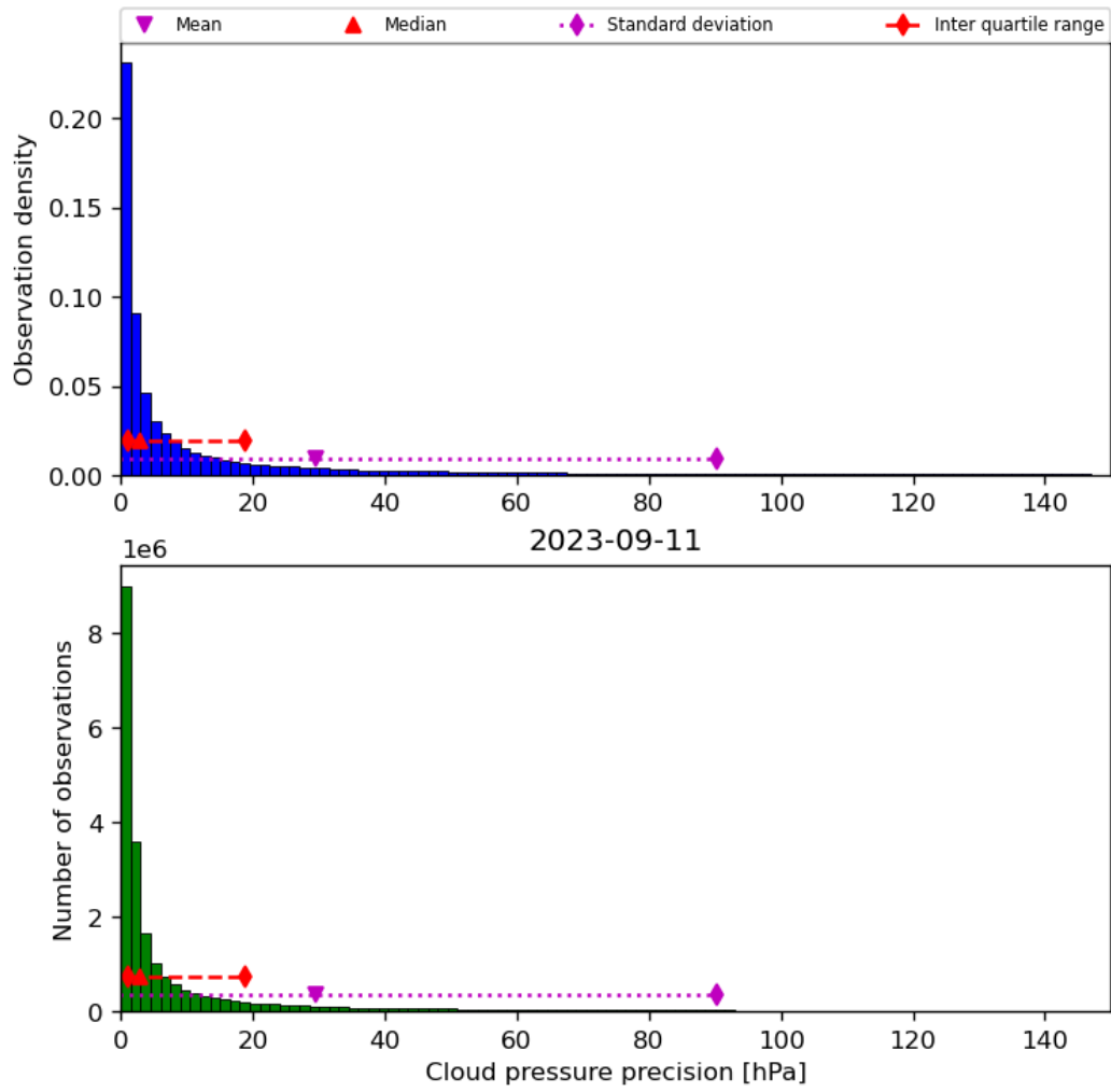
Figure 31: Histogram of “Cloud pressure precision” for 2023-09-10 to 2023-09-12
