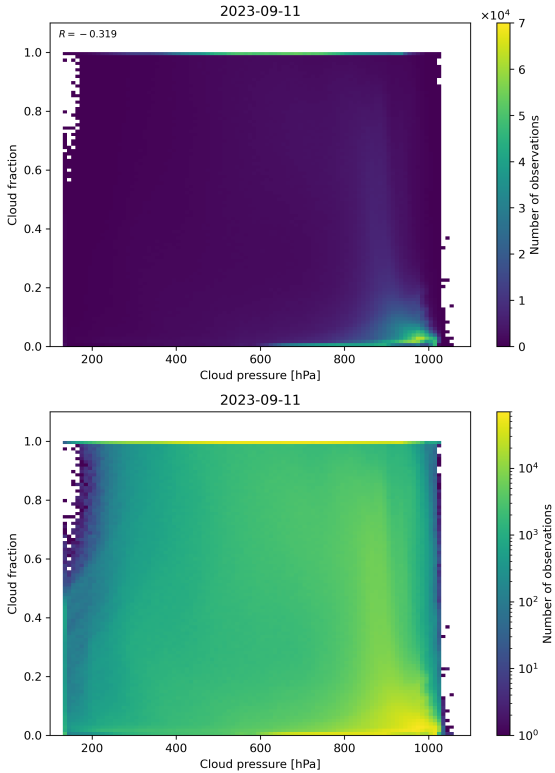
Figure 87: Scatter density plot of “Cloud pressure” against “Cloud fraction” for 2023-09-10 to 2023-09-12.
