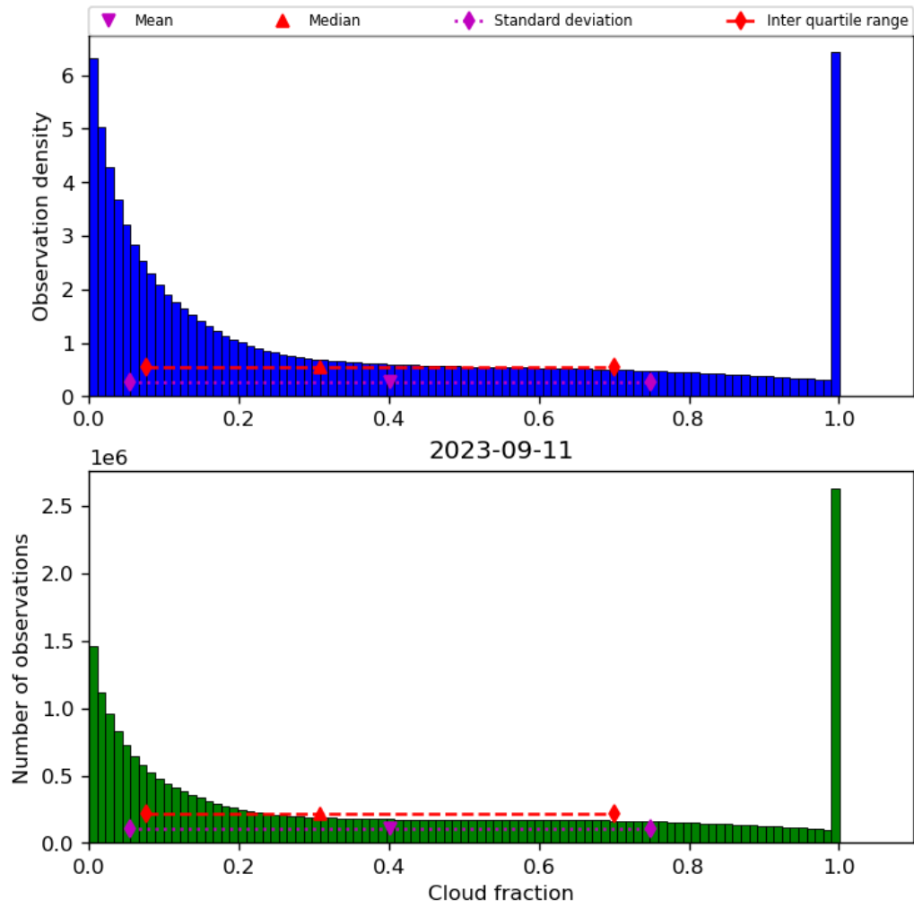
Figure 32: Histogram of “Cloud fraction” for 2023-09-10 to 2023-09-12
