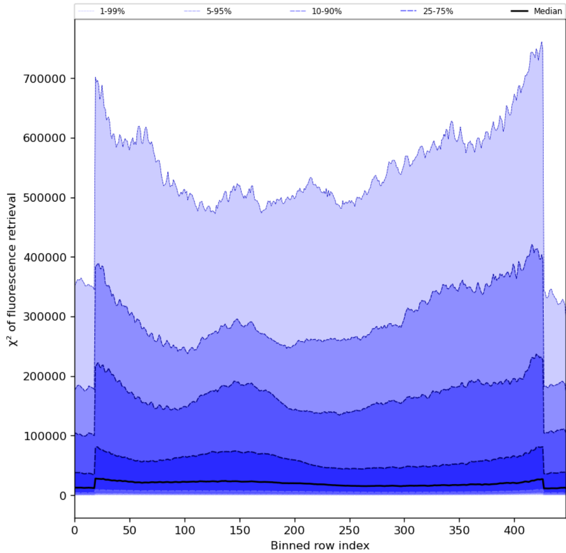
Figure 59: Along track statistics of “ \chi^2 of fluorescence retrieval” for 2023-09-10 to 2023-09-12
