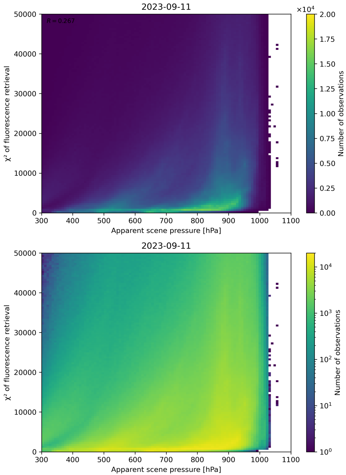
Figure 64: Scatter density plot of “Apparent scene pressure” against “ \chi^2 of fluorescence retrieval” for 2023-09-10 to 2023-09-12.
