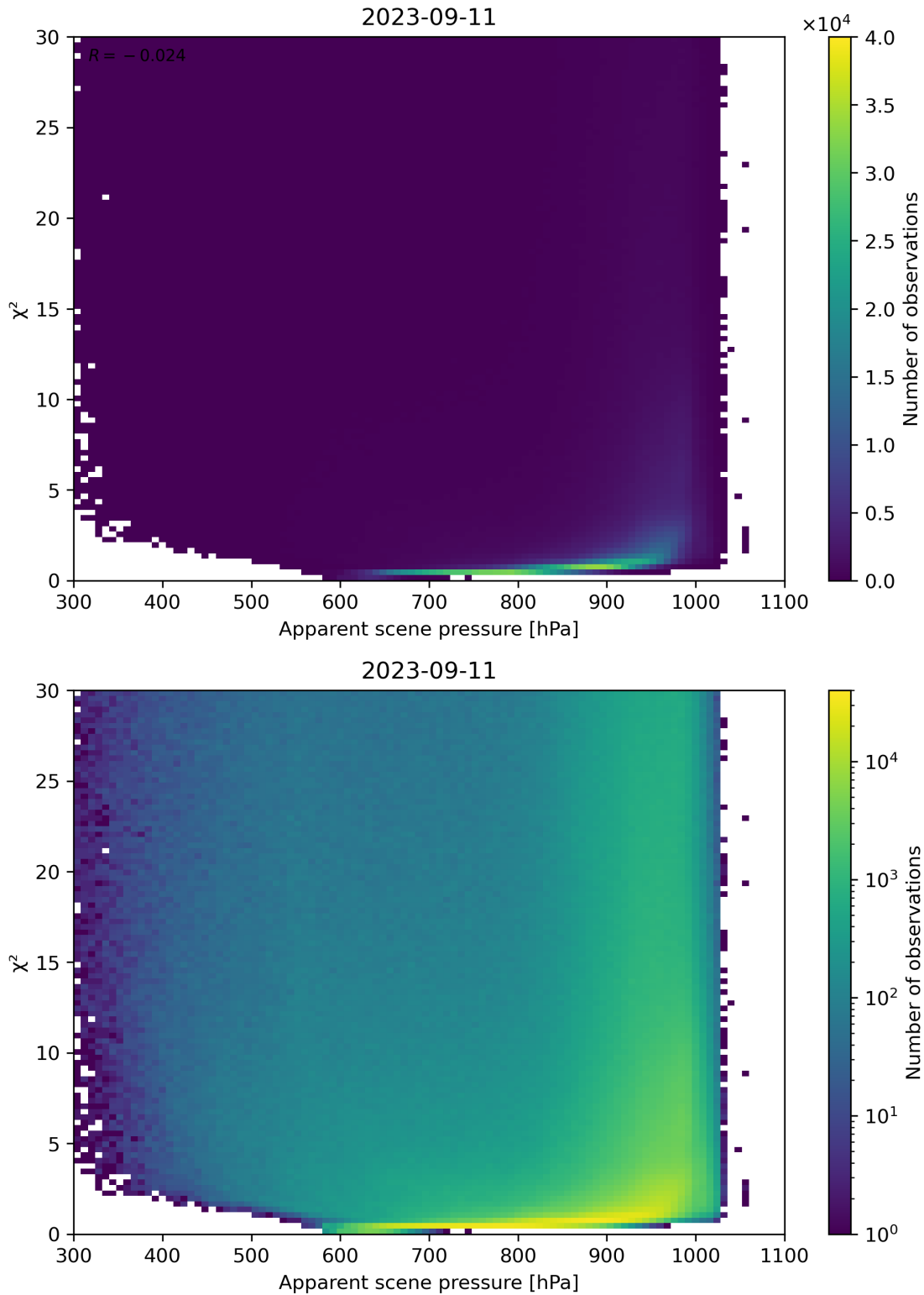
Figure 63: Scatter density plot of “Apparent scene pressure” against “ \chi^2 ” for 2023-09-10 to 2023-09-12.
