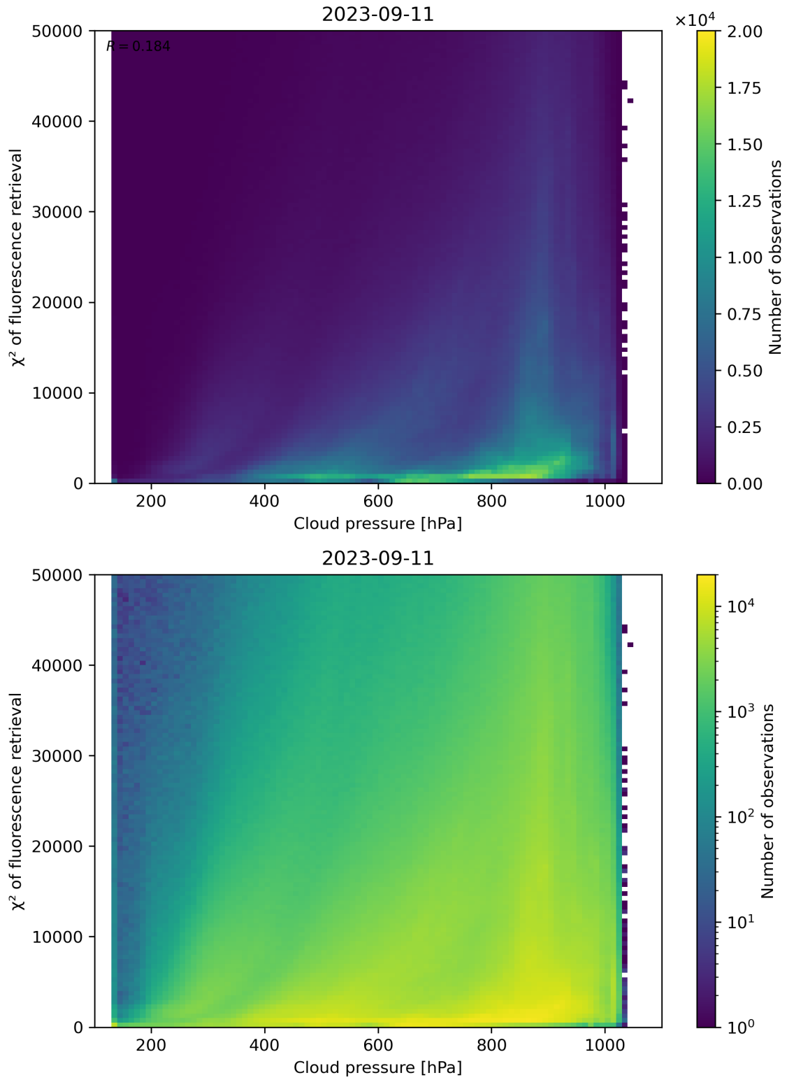
Figure 86: Scatter density plot of “Cloud pressure” against “ \chi^2 of fluorescence retrieval” for 2023-09-10 to 2023-09-12.
