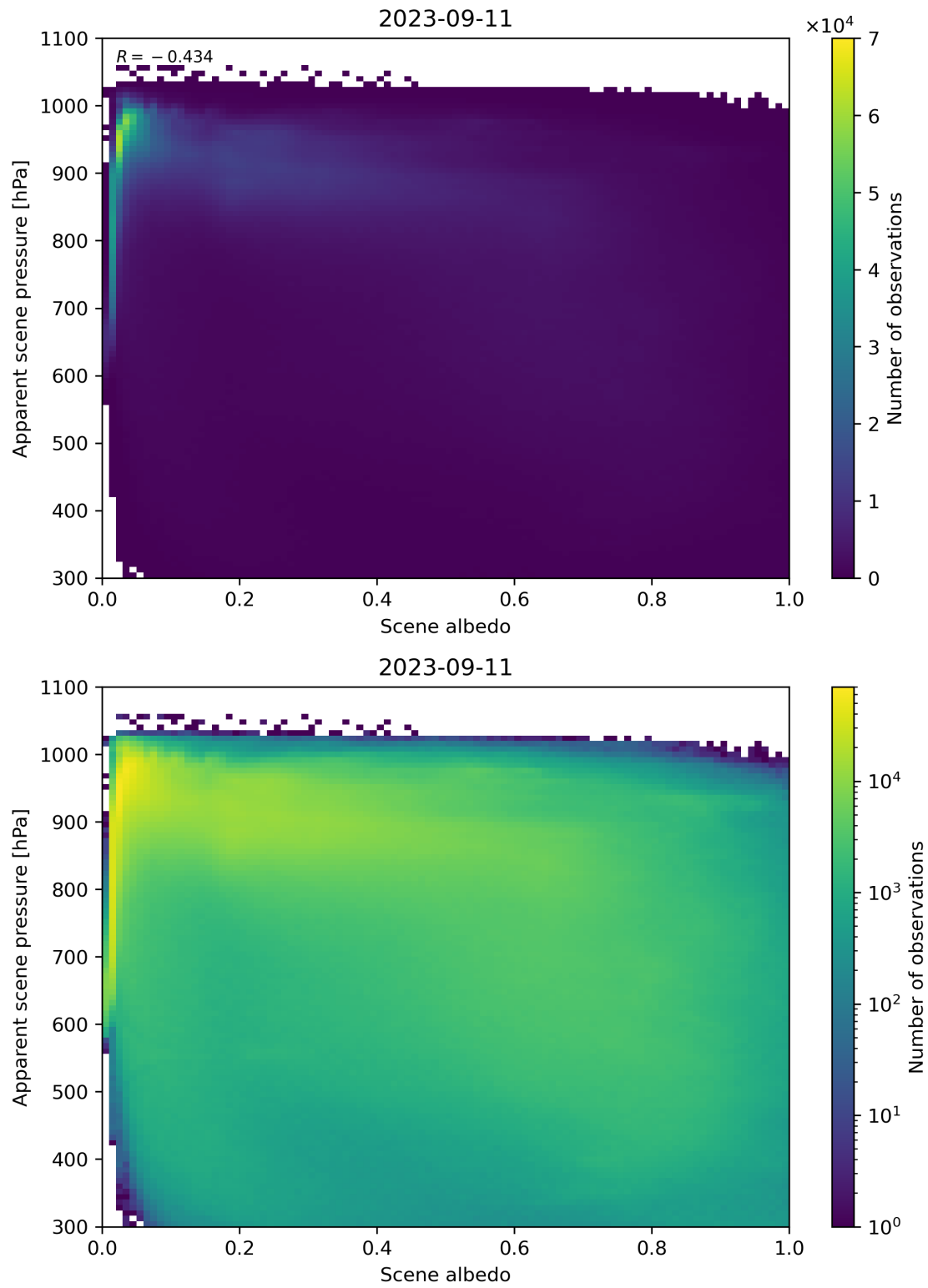
Figure 111: Scatter density plot of “Scene albedo” against “Apparent scene pressure” for 2023-09-10 to 2023-09-12.
