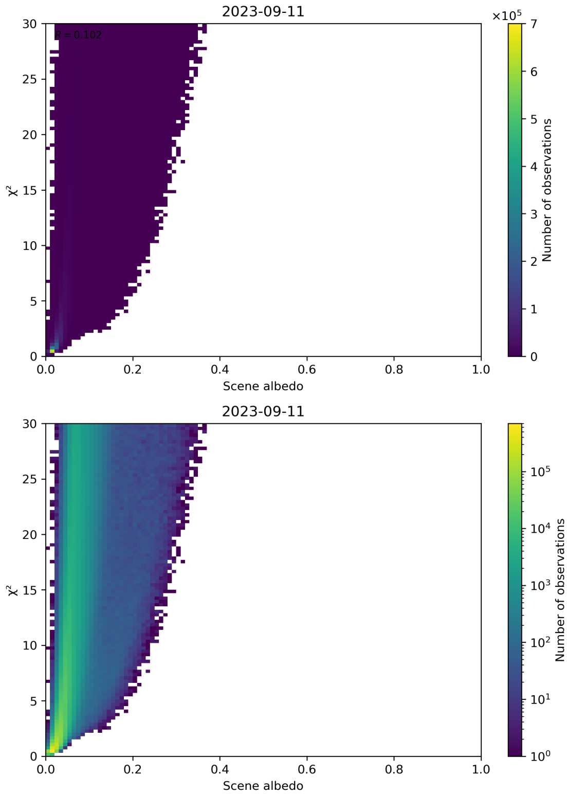
Figure 112: Scatter density plot of “Scene albedo” against “ \chi^2 ” for 2023-09-10 to 2023-09-12.
