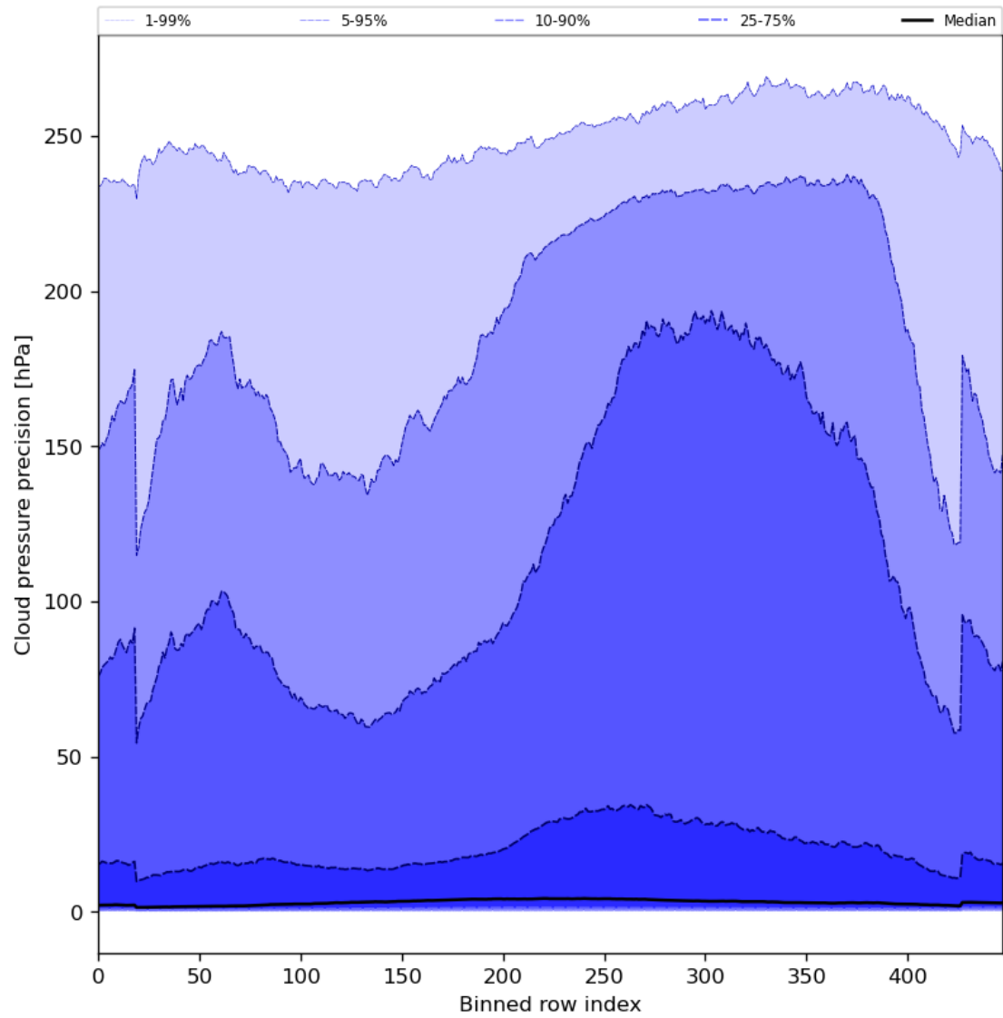
Figure 48: Along track statistics of “Cloud pressure precision” for 2023-09-10 to 2023-09-12
