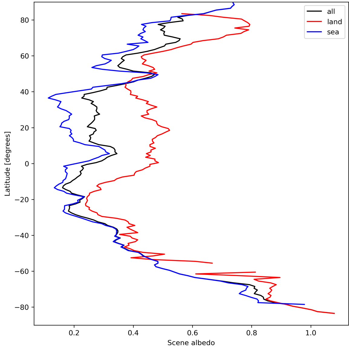
Figure 17: Zonal average of “Scene albedo” for 2023-09-10 to 2023-09-12.
