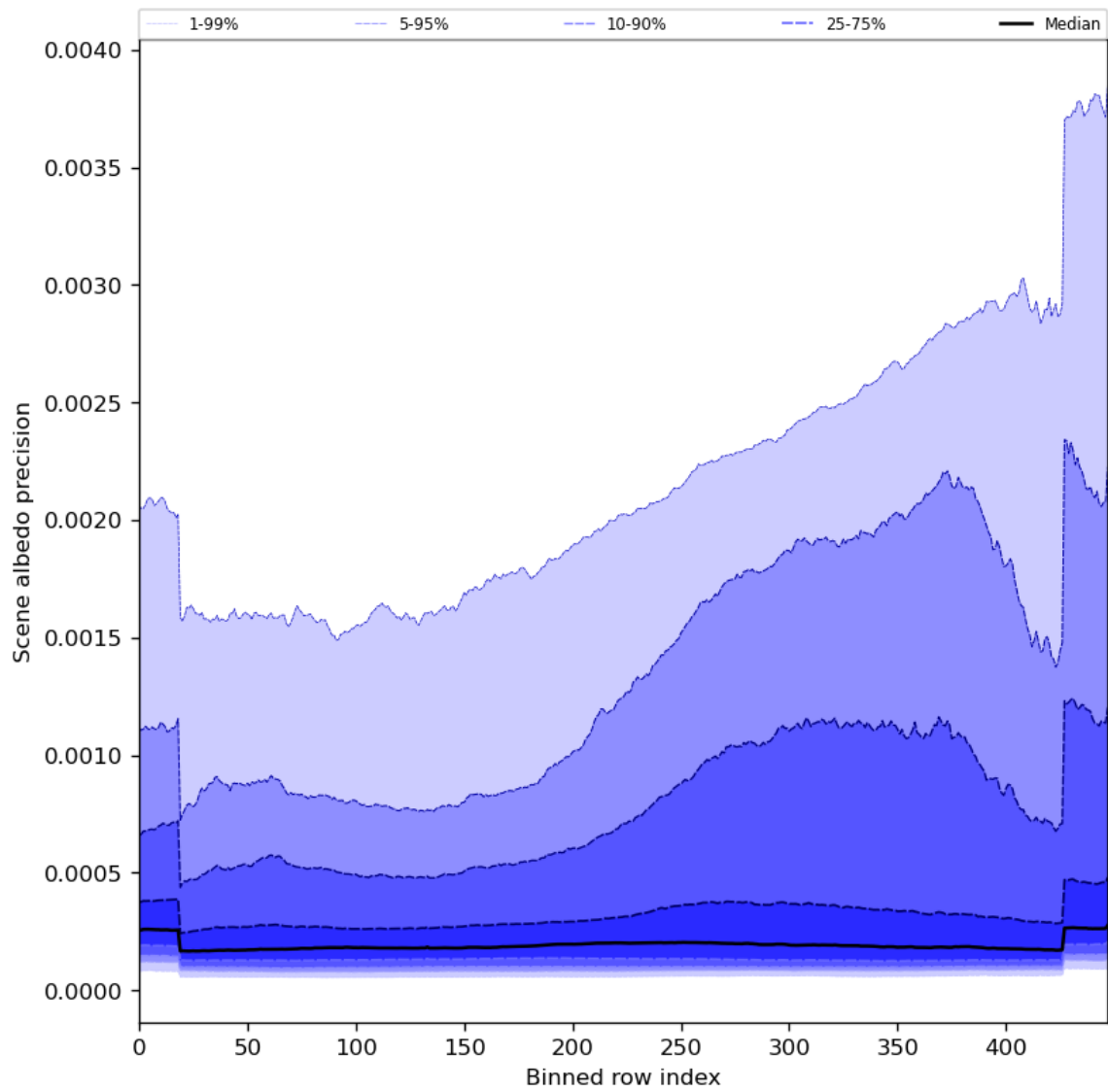
Figure 52: Along track statistics of “Scene albedo precision” for 2023-09-10 to 2023-09-12
