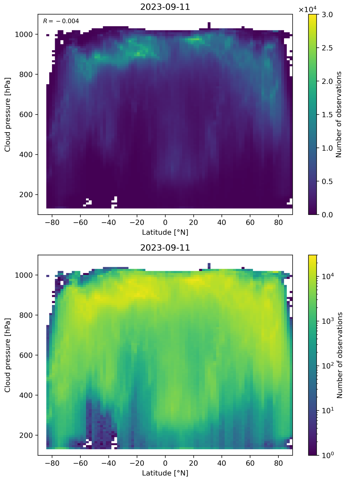
Figure 100: Scatter density plot of “Latitude” against “Cloud pressure” for 2023-09-10 to 2023-09-12.
