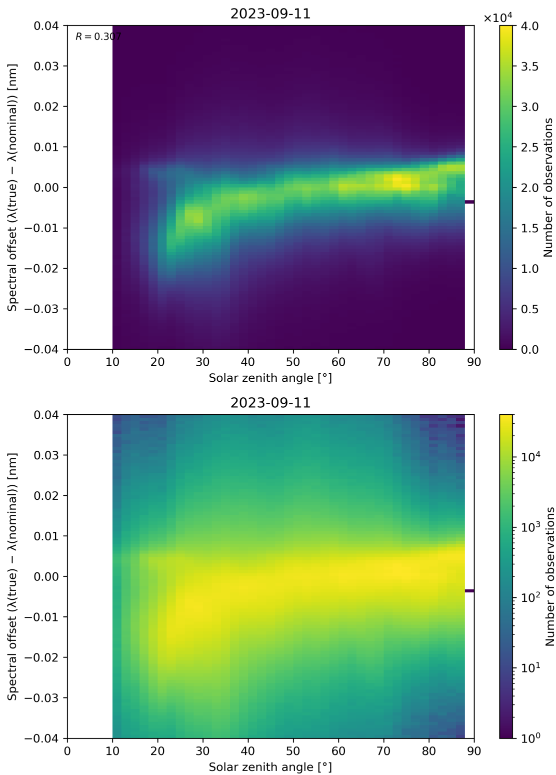
Figure 128: Scatter density plot of “Solar zenith angle” against “Spectral offset ( \lambda(\text{true}) - \lambda(\text{nominal}) )” for 2023-09-10 to 2023-09-12.
