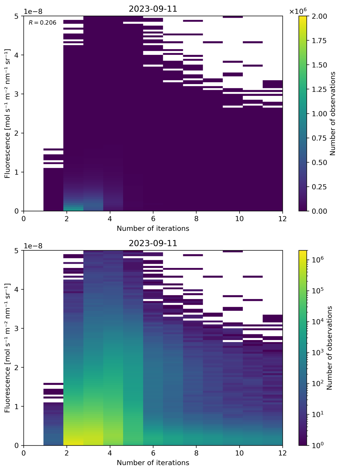
Figure 107: Scatter density plot of “Number of iterations” against “Fluorescence” for 2023-09-10 to 2023-09-12.
