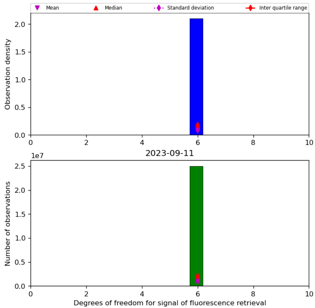
Figure 43: Histogram of “Degrees of freedom for signal of fluorescence retrieval” for 2023-09-10 to 2023-09-12
