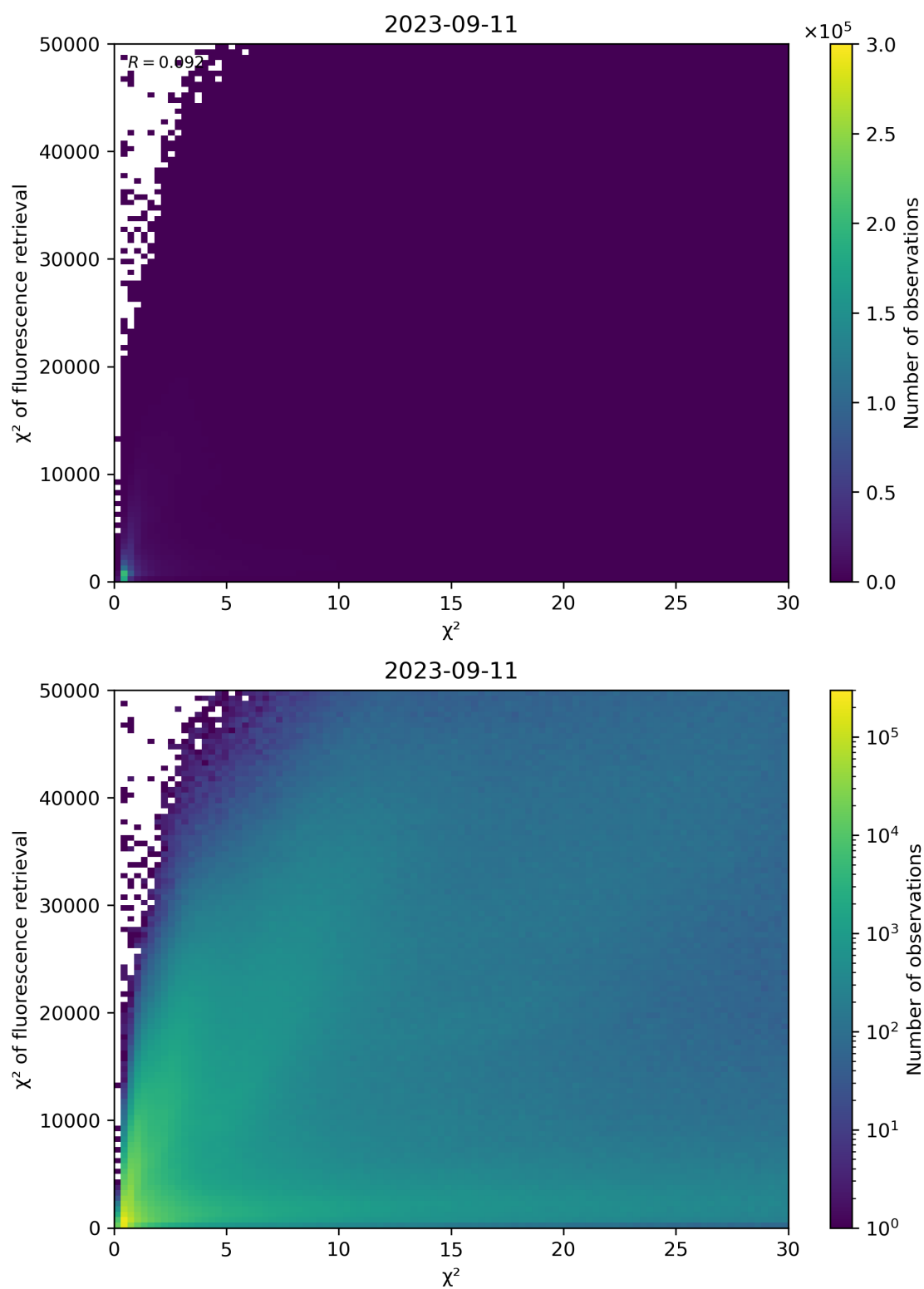
Figure 69: Scatter density plot of “ \chi^2 ” against “ \chi^2 of fluorescence retrieval” for 2023-09-10 to 2023-09-12.
