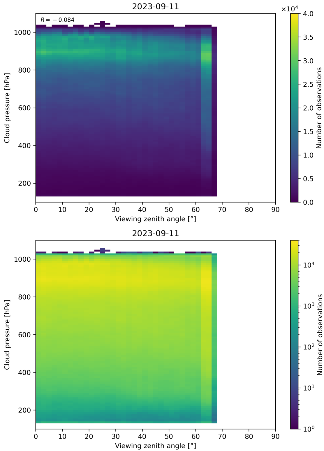
Figure 133: Scatter density plot of “Viewing zenith angle” against “Cloud pressure” for 2023-09-10 to 2023-09-12.
