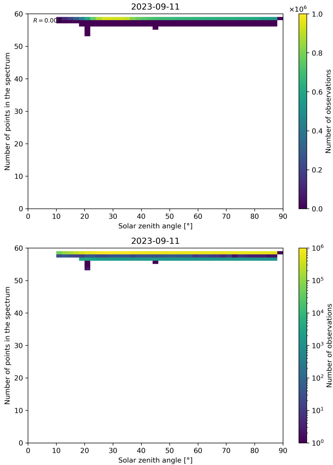
Figure 126: Scatter density plot of “Solar zenith angle” against “Number of points in the spectrum” for 2023-09-10 to 2023-09-12.
