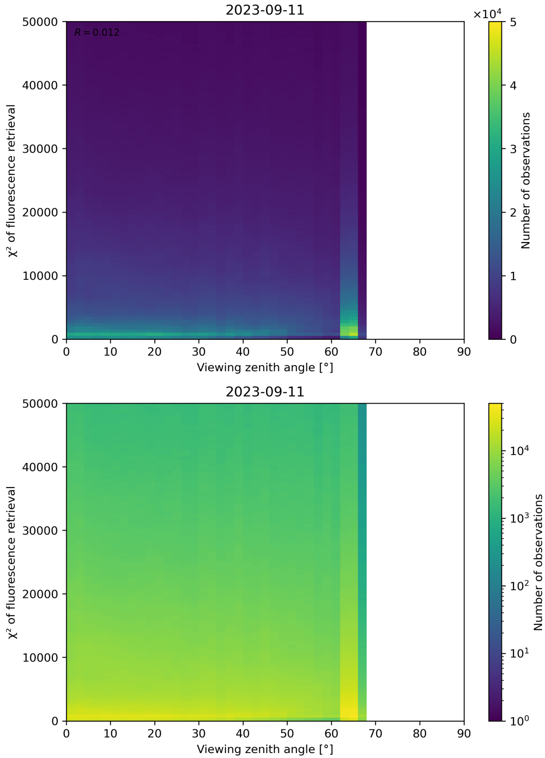
Figure 131: Scatter density plot of “Viewing zenith angle” against “ \chi^2 of fluorescence retrieval” for 2023-09-10 to 2023-09-12.
