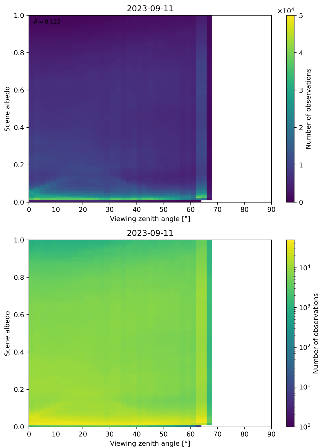
Figure 138: Scatter density plot of “Viewing zenith angle” against “Scene albedo” for 2023-09-10 to 2023-09-12.
