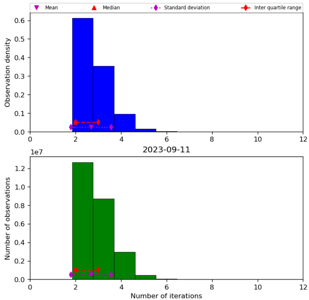
Figure 39: Histogram of “Number of iterations” for 2023-09-10 to 2023-09-12
