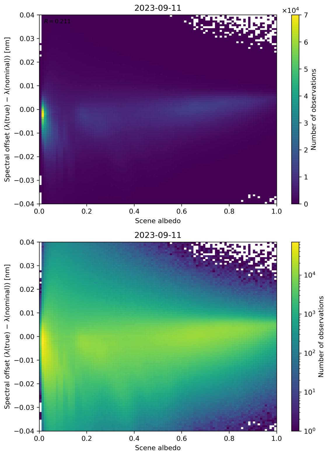
Figure 117: Scatter density plot of “Scene albedo” against “Spectral offset ( \lambda(\text{true}) - \lambda(\text{nominal}) )” for 2023-09-10 to 2023-09-12.
