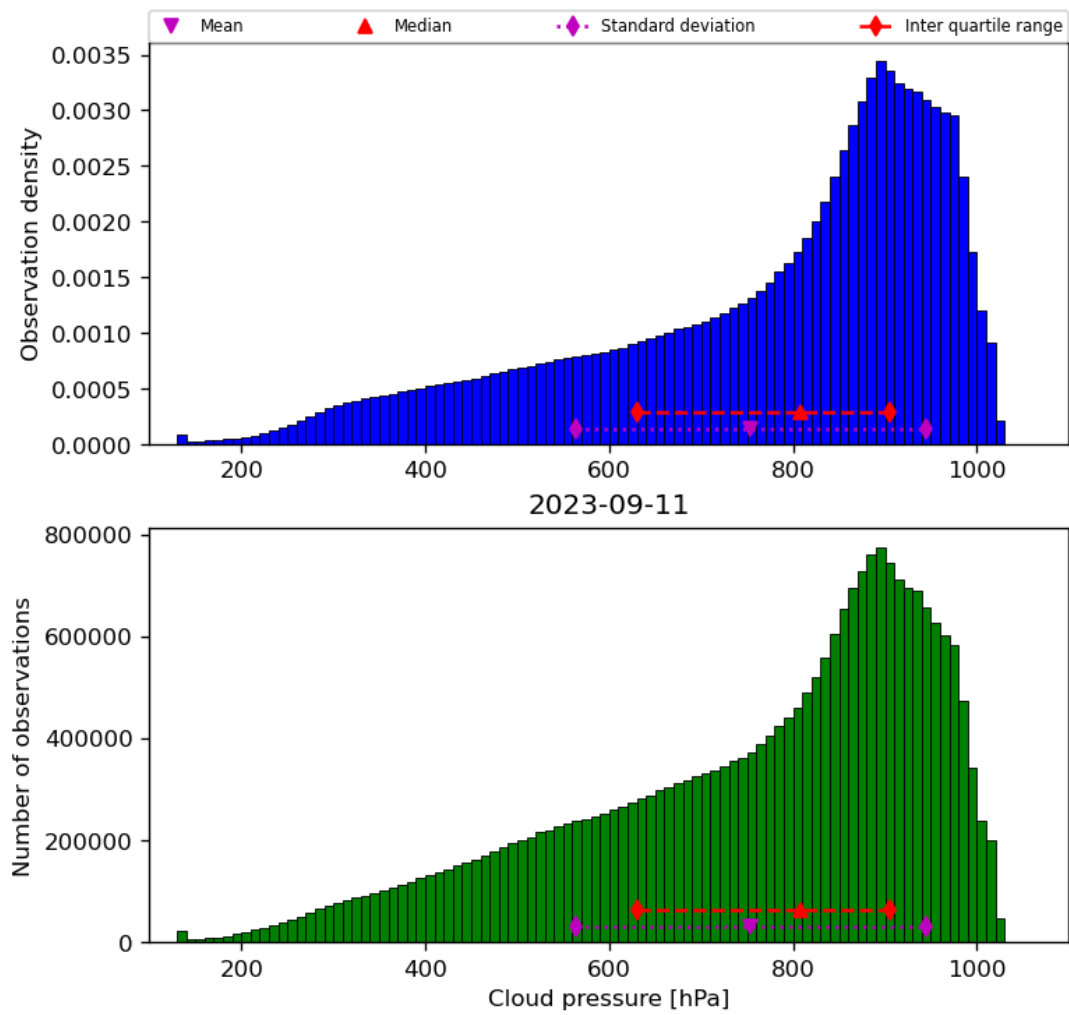
Figure 30: Histogram of “Cloud pressure” for 2023-09-10 to 2023-09-12
