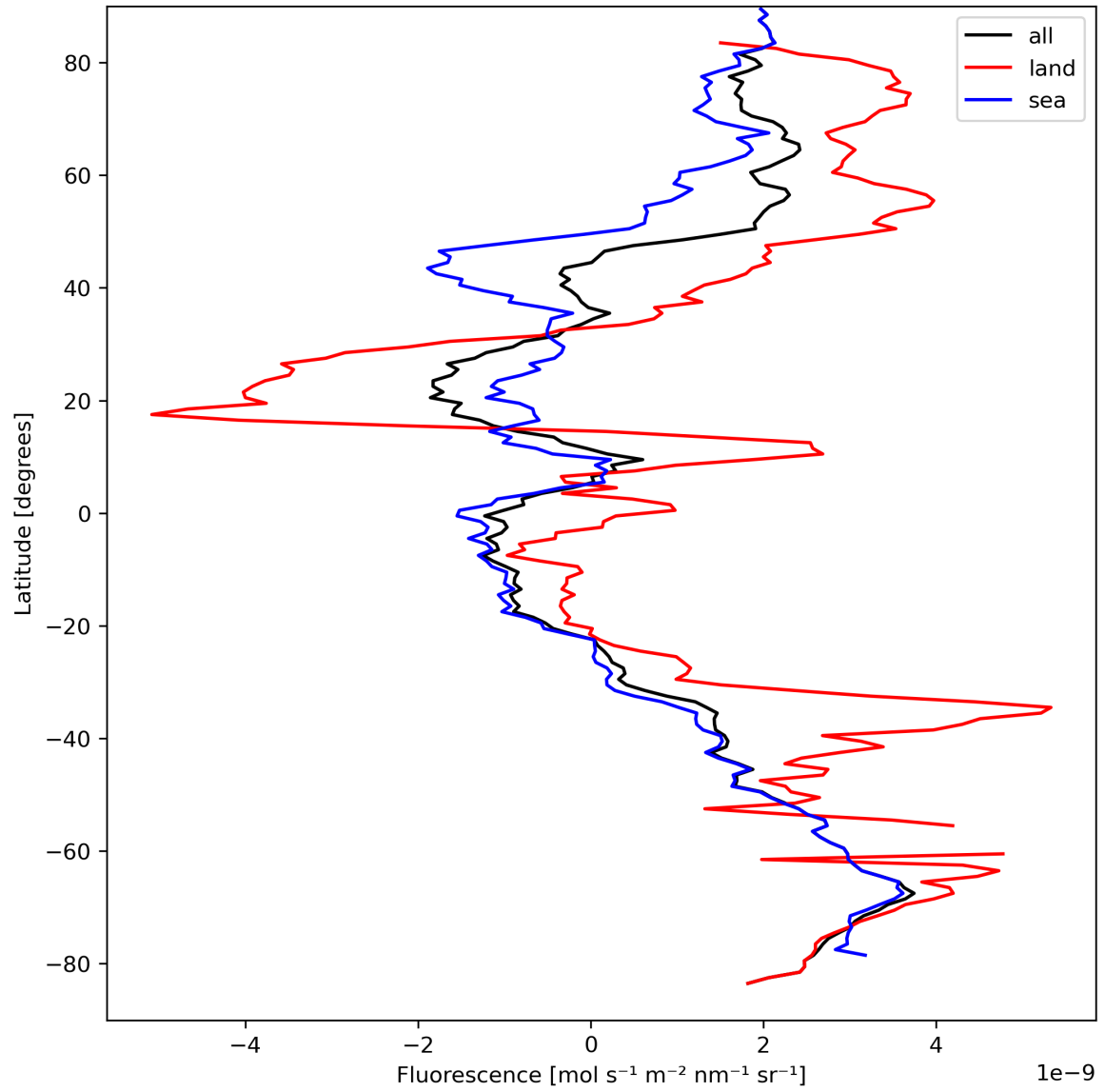
Figure 23: Zonal average of “Fluorescence” for 2023-09-10 to 2023-09-12.
