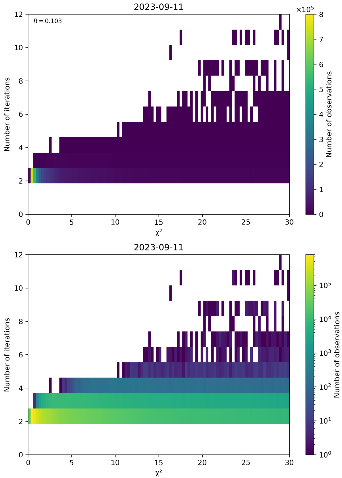
Figure 73: Scatter density plot of “ \chi^2 ” against “Number of iterations” for 2023-09-10 to 2023-09-12.
