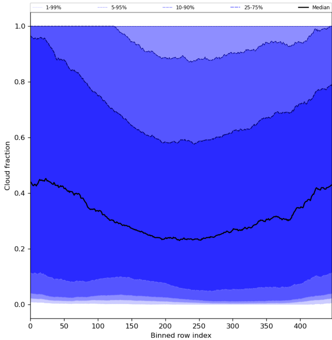
Figure 49: Along track statistics of “Cloud fraction” for 2023-09-10 to 2023-09-12
