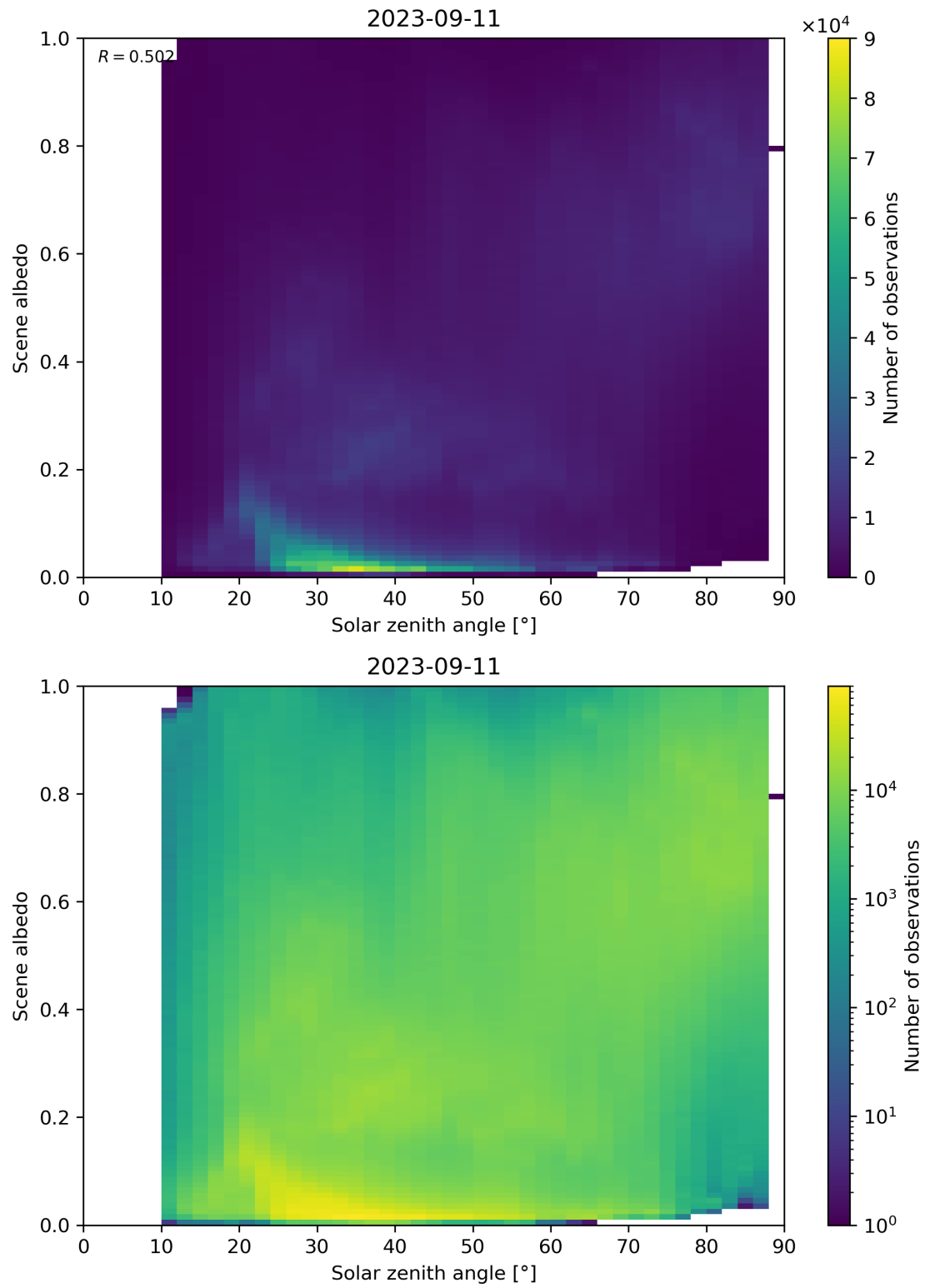
Figure 127: Scatter density plot of “Solar zenith angle” against “Scene albedo” for 2023-09-10 to 2023-09-12.
