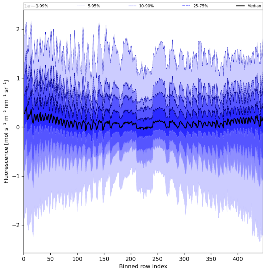
Figure 57: Along track statistics of “Fluorescence” for 2023-09-10 to 2023-09-12
