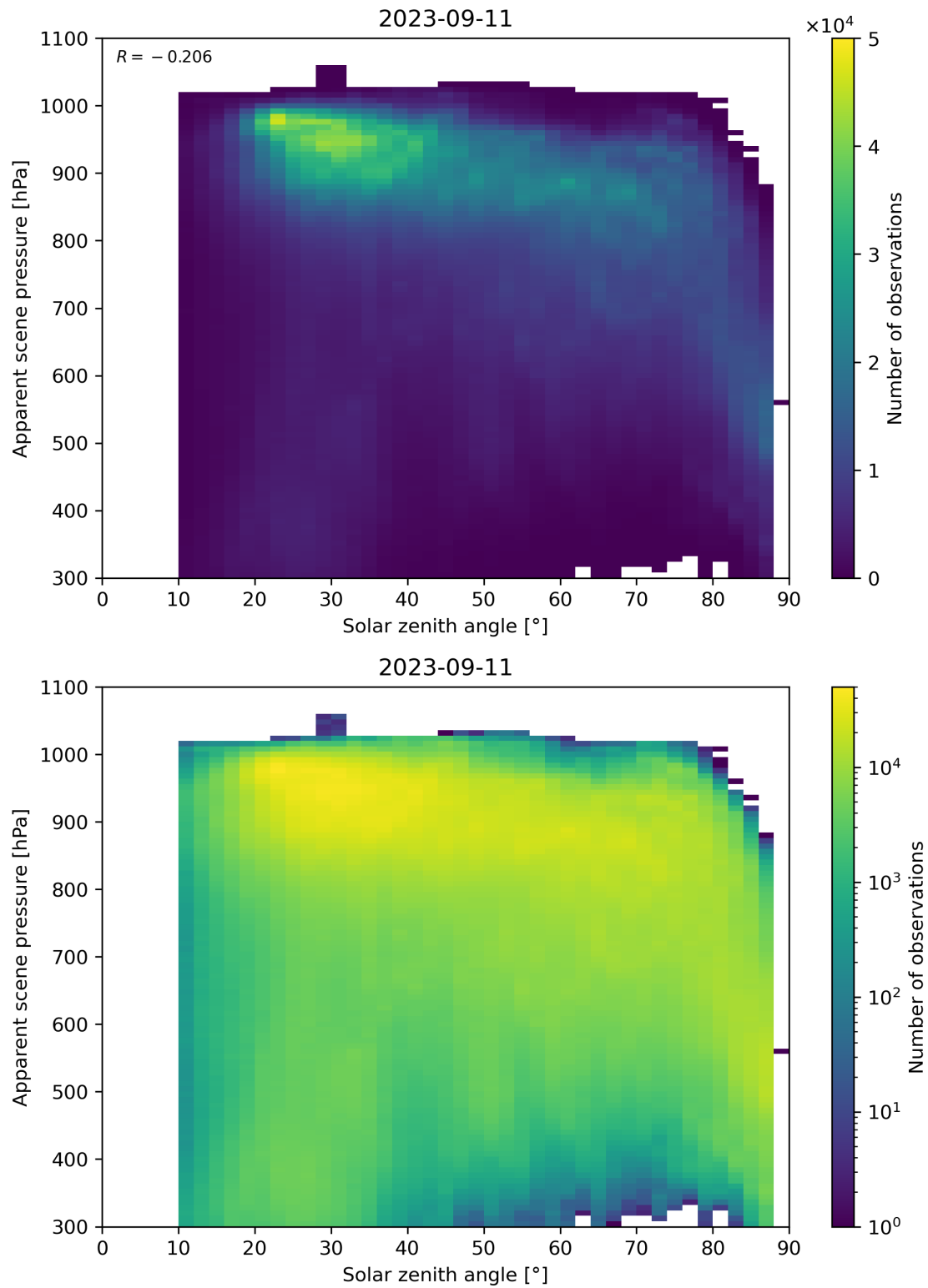
Figure 118: Scatter density plot of “Solar zenith angle” against “Apparent scene pressure” for 2023-09-10 to 2023-09-12.
