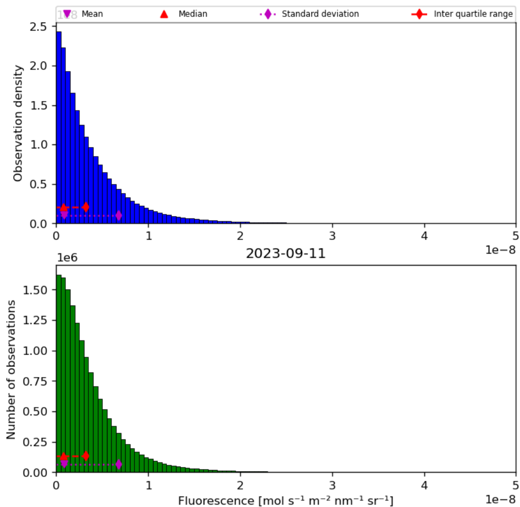
Figure 40: Histogram of “Fluorescence” for 2023-09-10 to 2023-09-12
