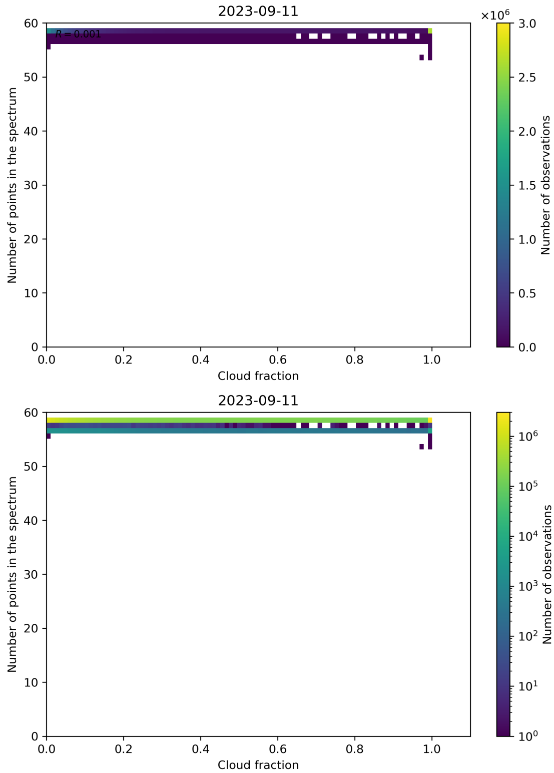
Figure 81: Scatter density plot of “Cloud fraction” against “Number of points in the spectrum” for 2023-09-10 to 2023-09-12.
