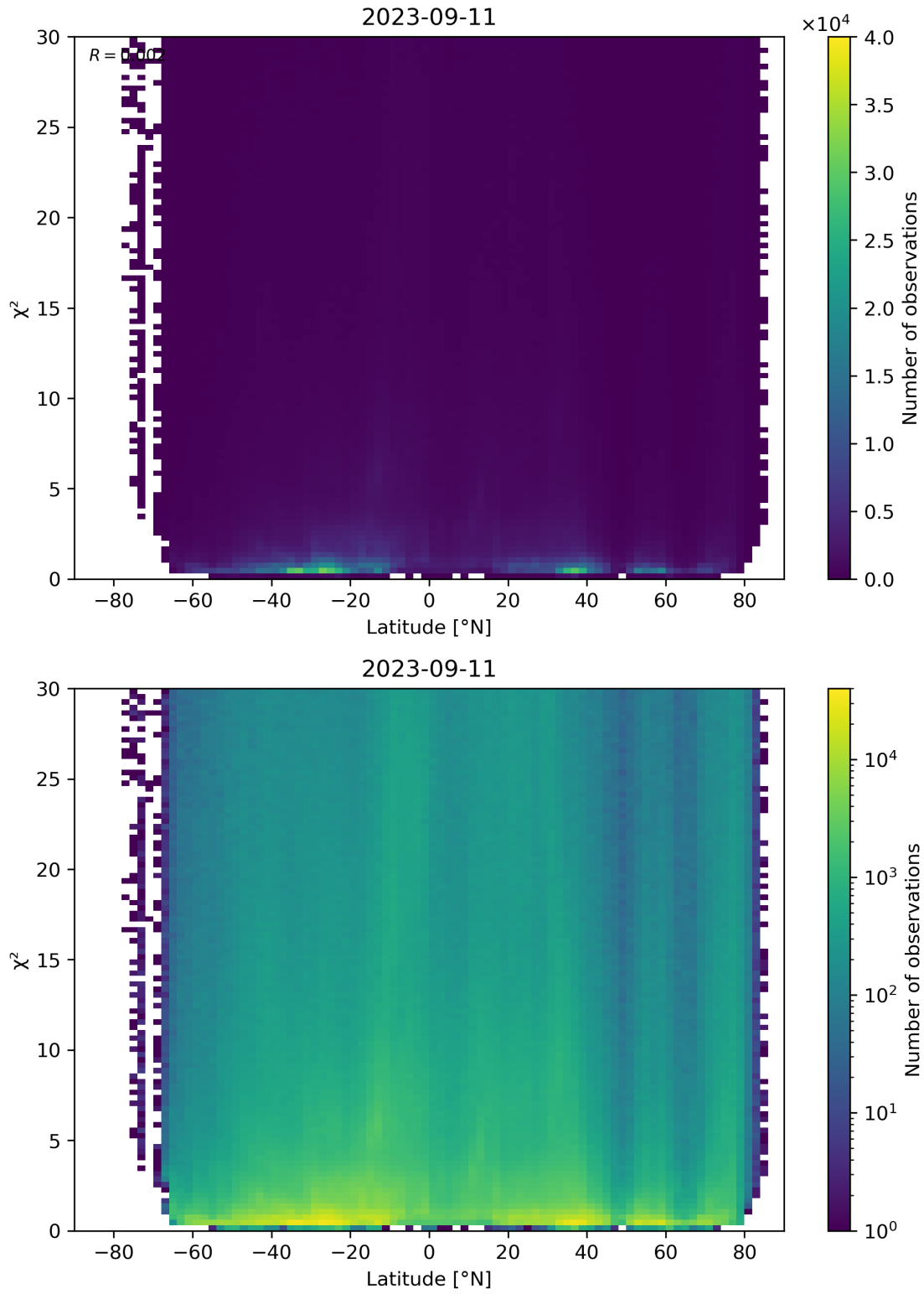
Figure 97: Scatter density plot of “Latitude” against “ \chi^2 ” for 2023-09-10 to 2023-09-12.
