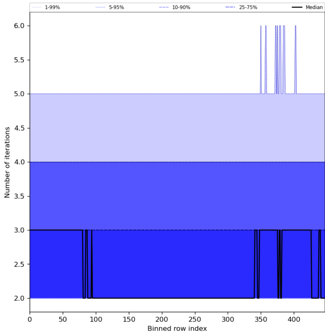
Figure 56: Along track statistics of “Number of iterations” for 2023-09-10 to 2023-09-12
