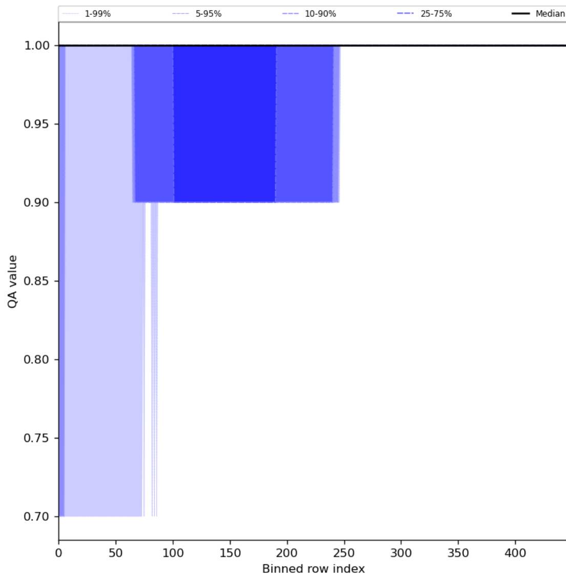
Figure 46: Along track statistics of “QA value” for 2023-09-10 to 2023-09-12
