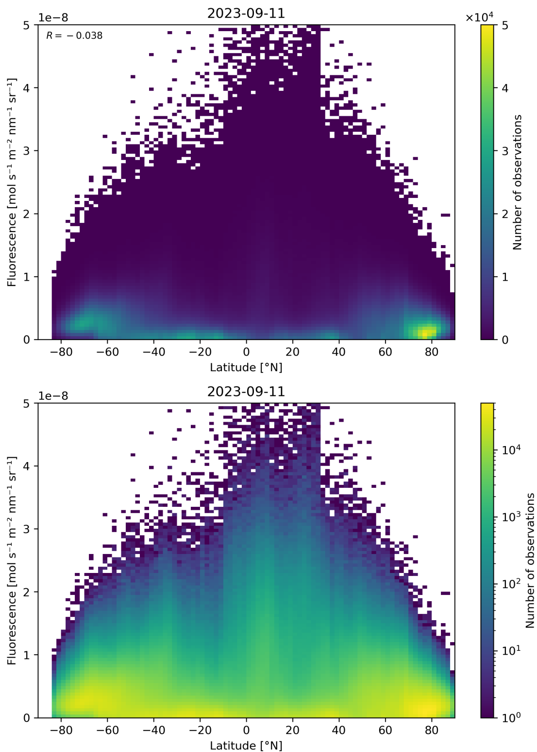
Figure 101: Scatter density plot of “Latitude” against “Fluorescence” for 2023-09-10 to 2023-09-12.
