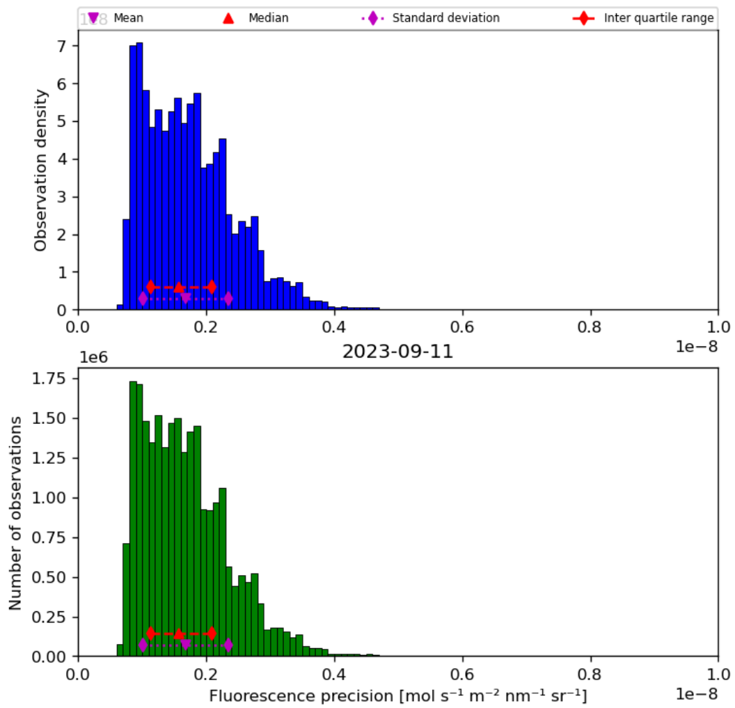
Figure 41: Histogram of “Fluorescence precision” for 2023-09-10 to 2023-09-12
