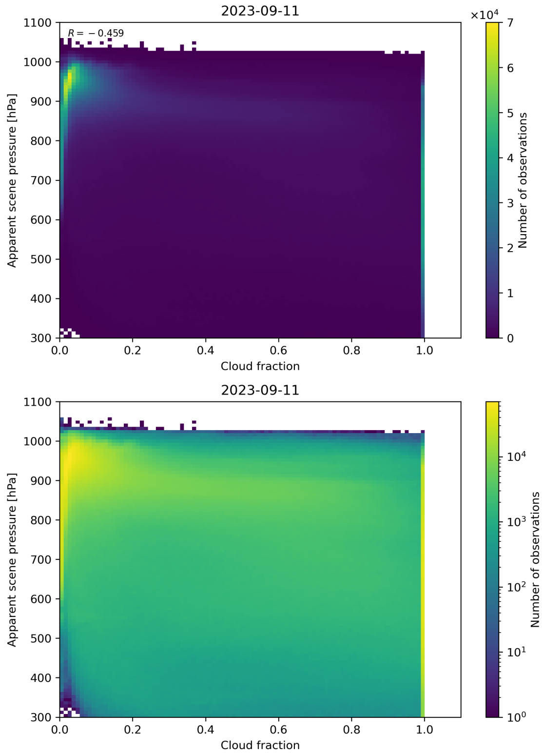
Figure 76: Scatter density plot of “Cloud fraction” against “Apparent scene pressure” for 2023-09-10 to 2023-09-12.
