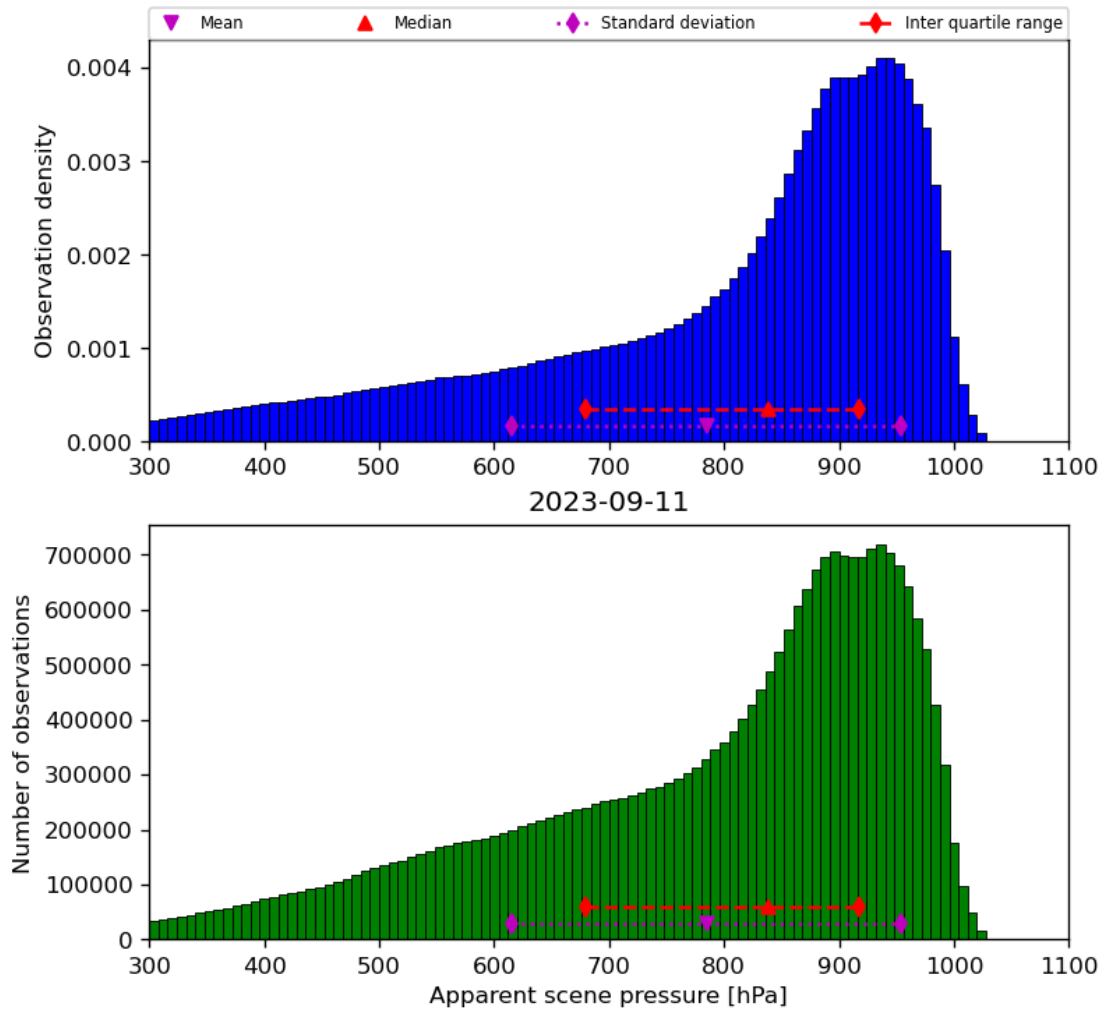
Figure 36: Histogram of “Apparent scene pressure” for 2023-09-10 to 2023-09-12
