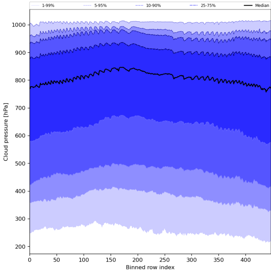
Figure 47: Along track statistics of “Cloud pressure” for 2023-09-10 to 2023-09-12
