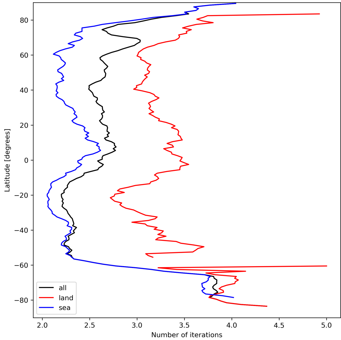
Figure 22: Zonal average of “Number of iterations” for 2023-09-10 to 2023-09-12.
