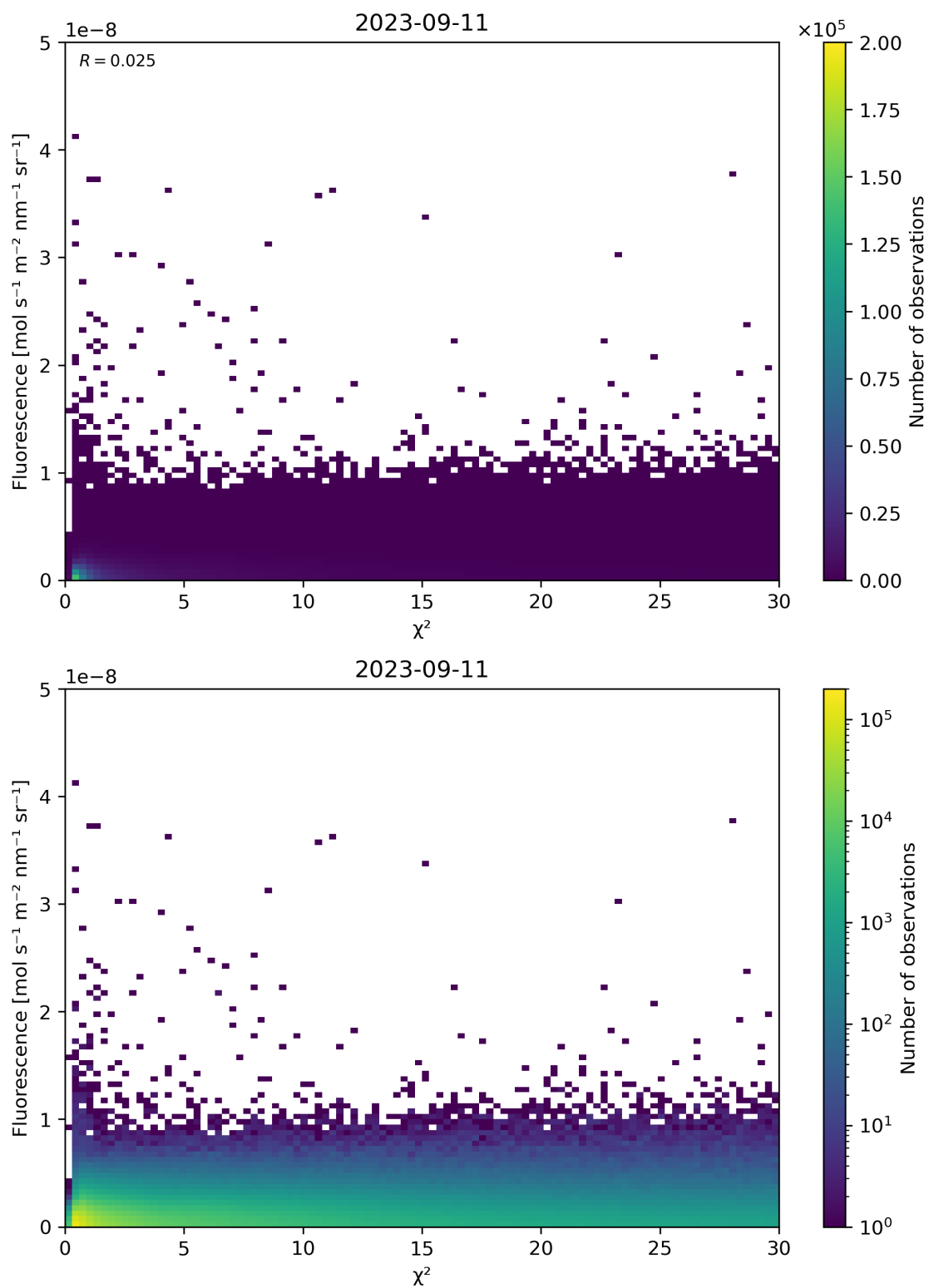
Figure 70: Scatter density plot of “ \chi^2 ” against “Fluorescence” for 2023-09-10 to 2023-09-12.
