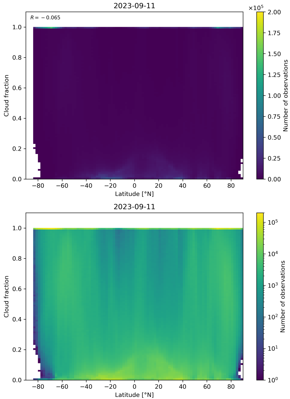
Figure 99: Scatter density plot of “Latitude” against “Cloud fraction” for 2023-09-10 to 2023-09-12.
