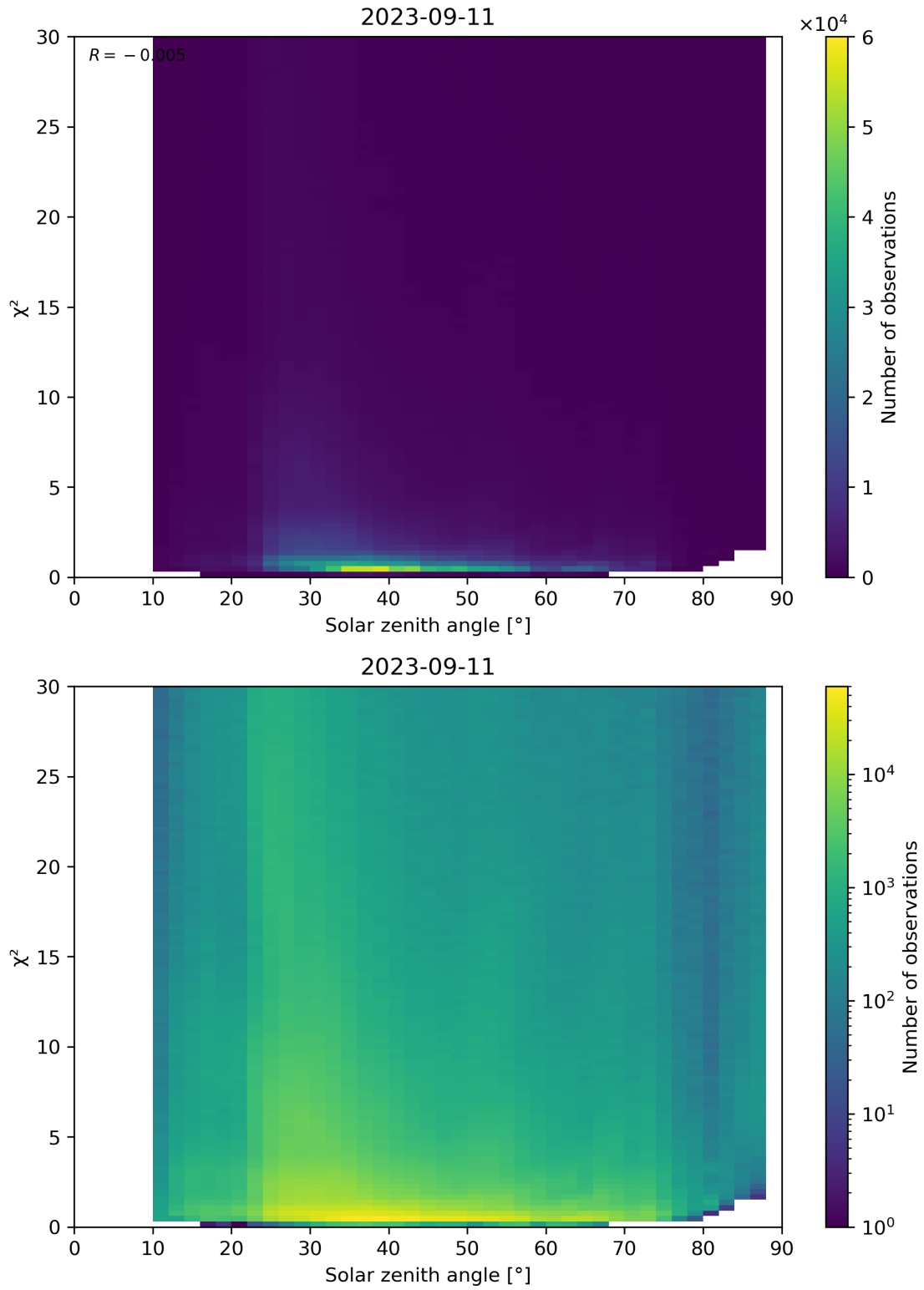
Figure 119: Scatter density plot of “Solar zenith angle” against “ \chi^2 ” for 2023-09-10 to 2023-09-12.
