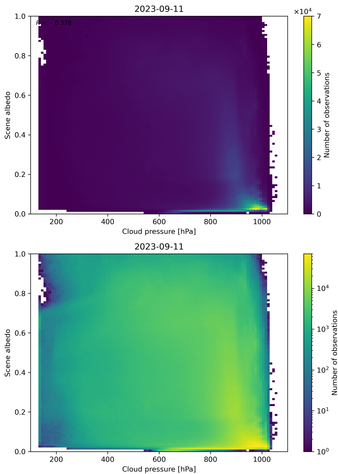
Figure 91: Scatter density plot of “Cloud pressure” against “Scene albedo” for 2023-09-10 to 2023-09-12.
