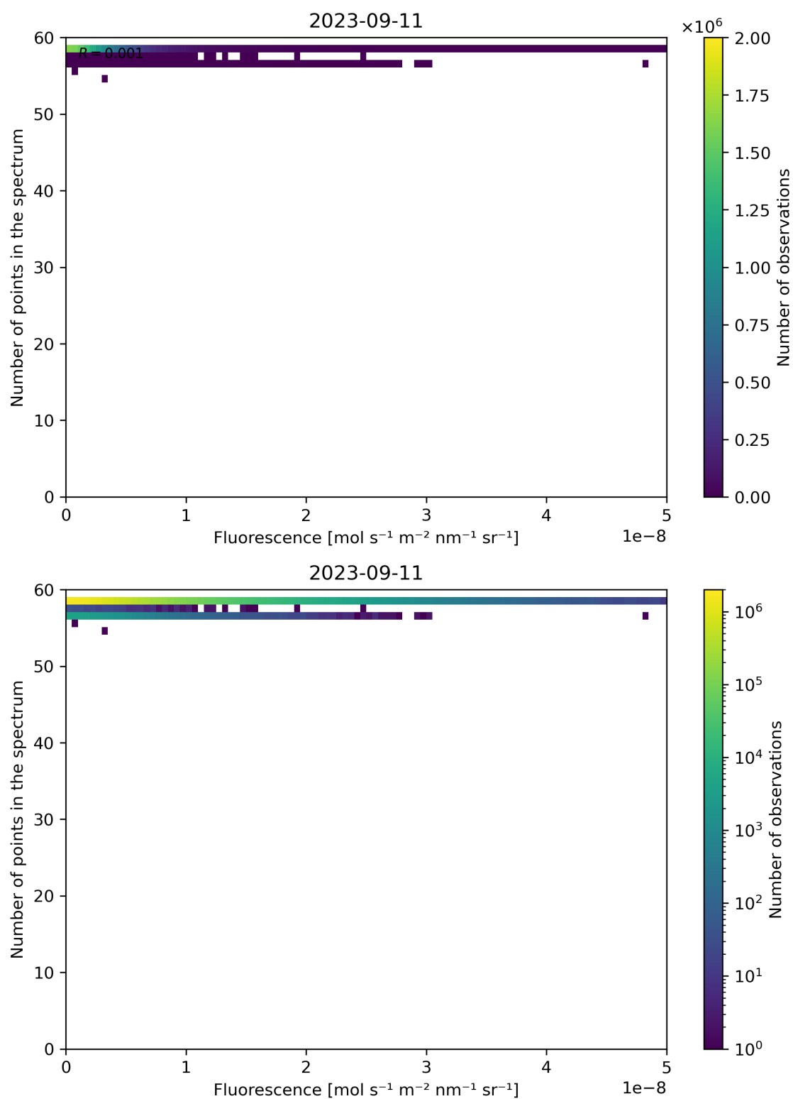
Figure 94: Scatter density plot of “Fluorescence” against “Number of points in the spectrum” for 2023-09-10 to 2023-09-12.
