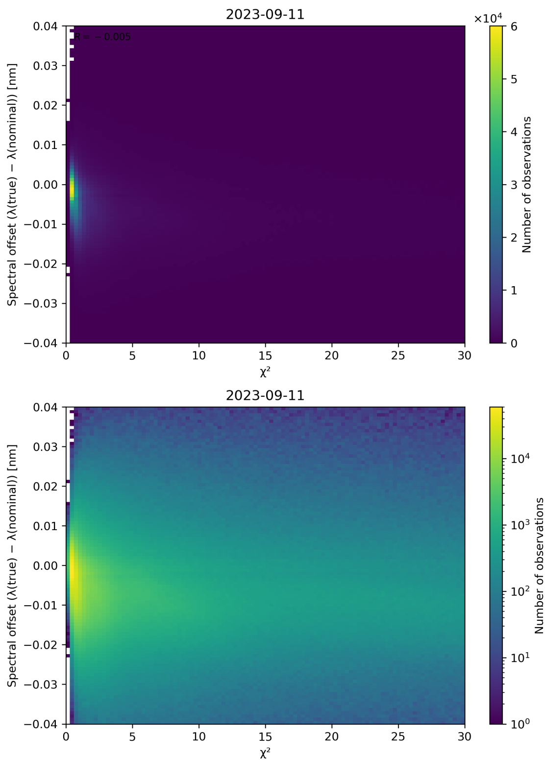
Figure 75: Scatter density plot of “ \chi^2 ” against “Spectral offset ( \lambda(\text{true}) - \lambda(\text{nominal}) )” for 2023-09-10 to 2023-09-12.
