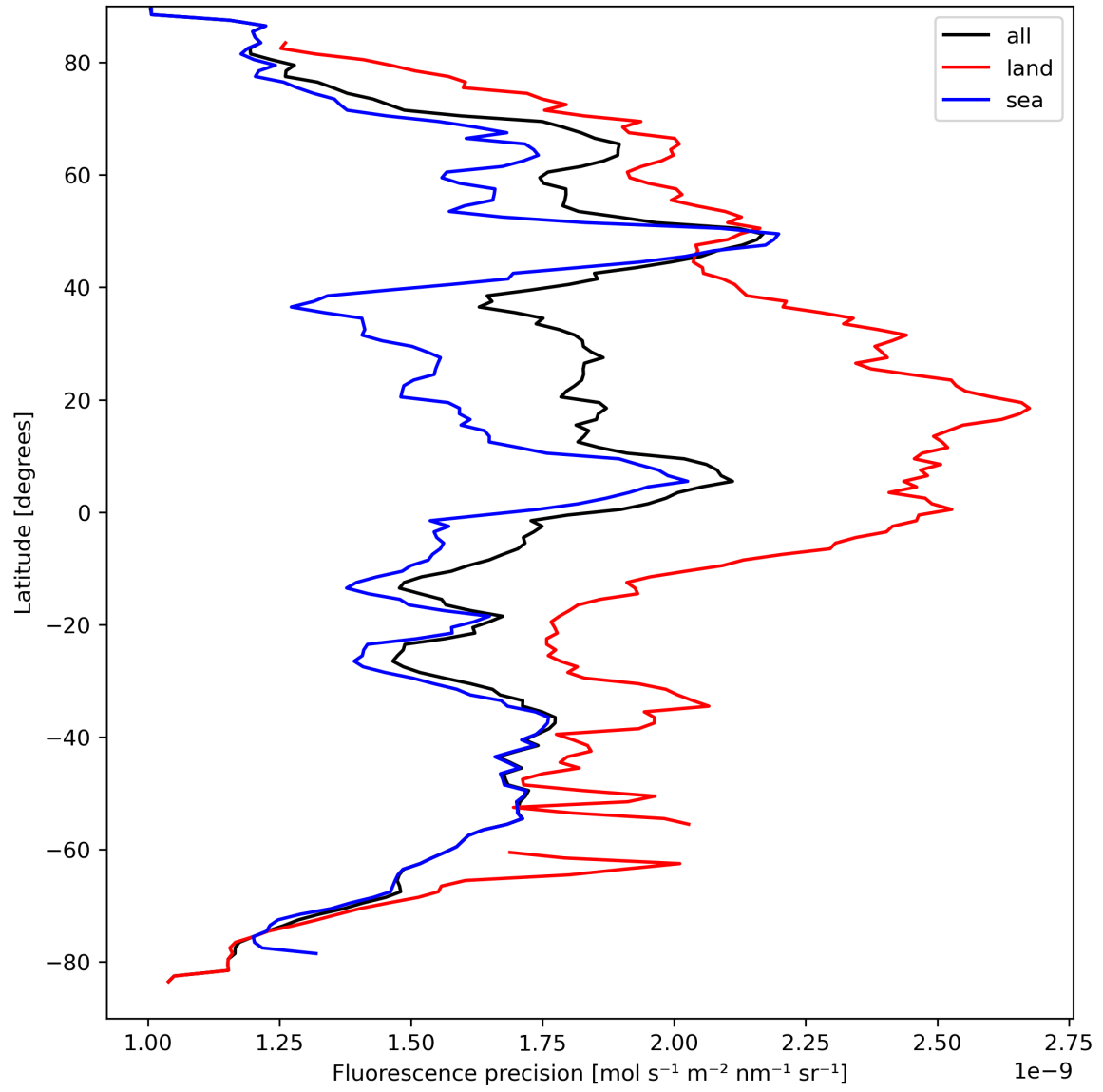
Figure 24: Zonal average of “Fluorescence precision” for 2023-09-10 to 2023-09-12.
