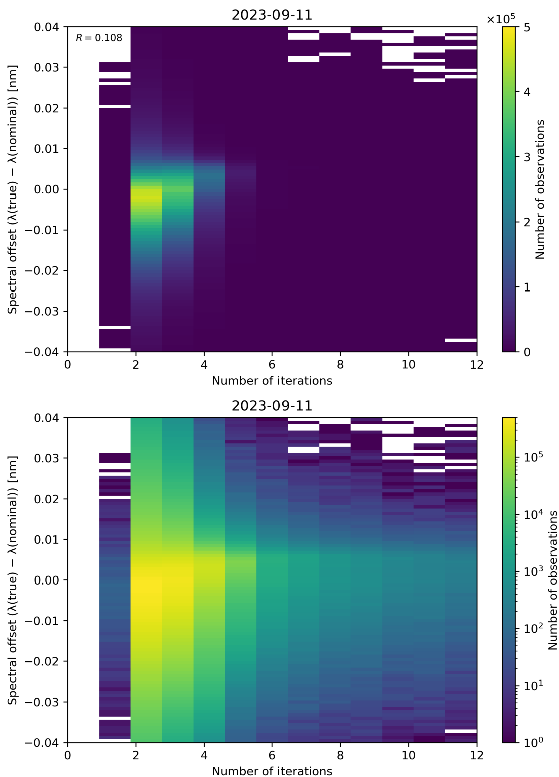
Figure 109: Scatter density plot of “Number of iterations” against “Spectral offset ( \lambda(\text{true}) - \lambda(\text{nominal}) )” for 2023-09-10 to 2023-09-12.
