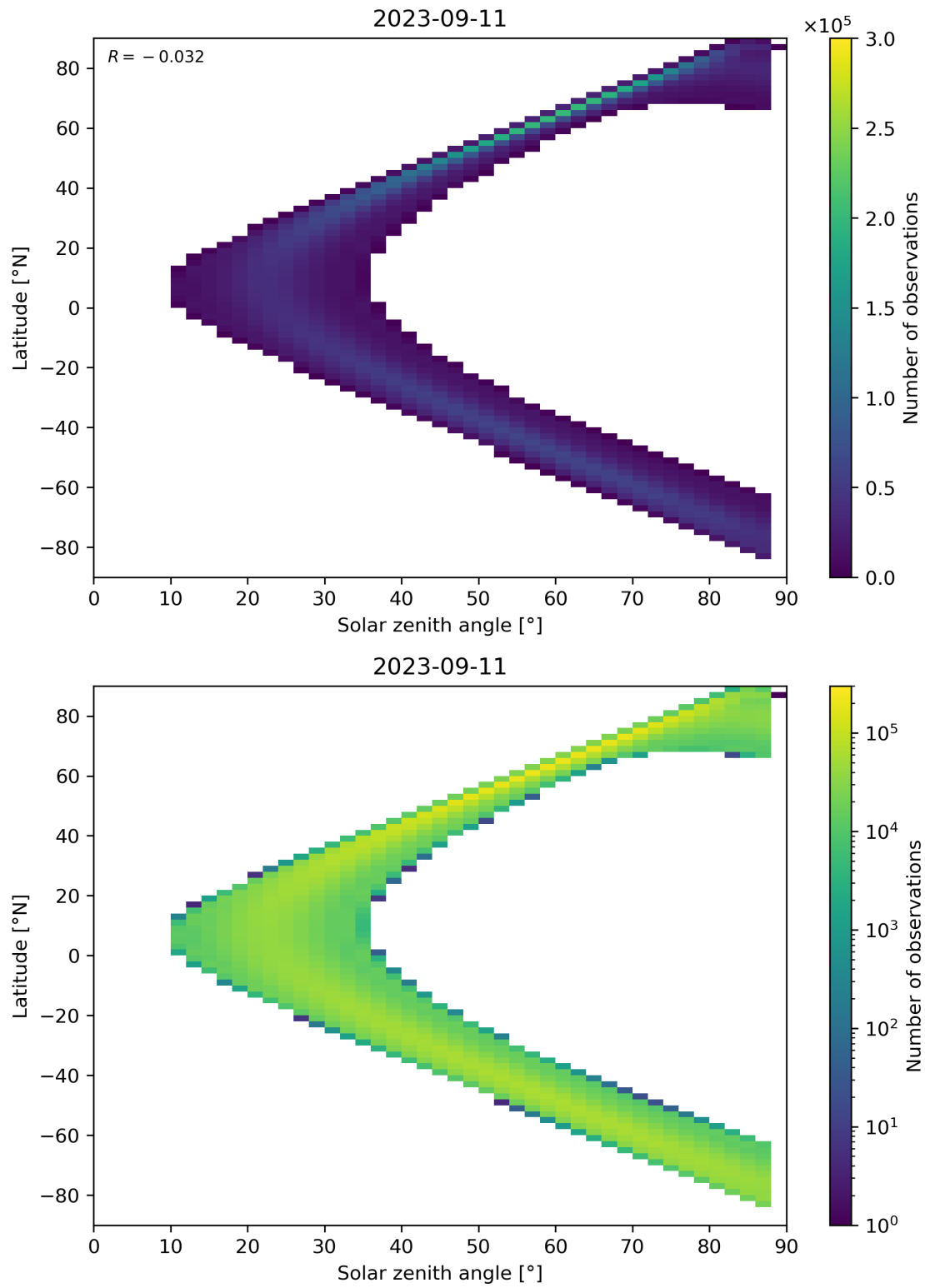
Figure 124: Scatter density plot of “Solar zenith angle” against “Latitude” for 2023-09-10 to 2023-09-12.
