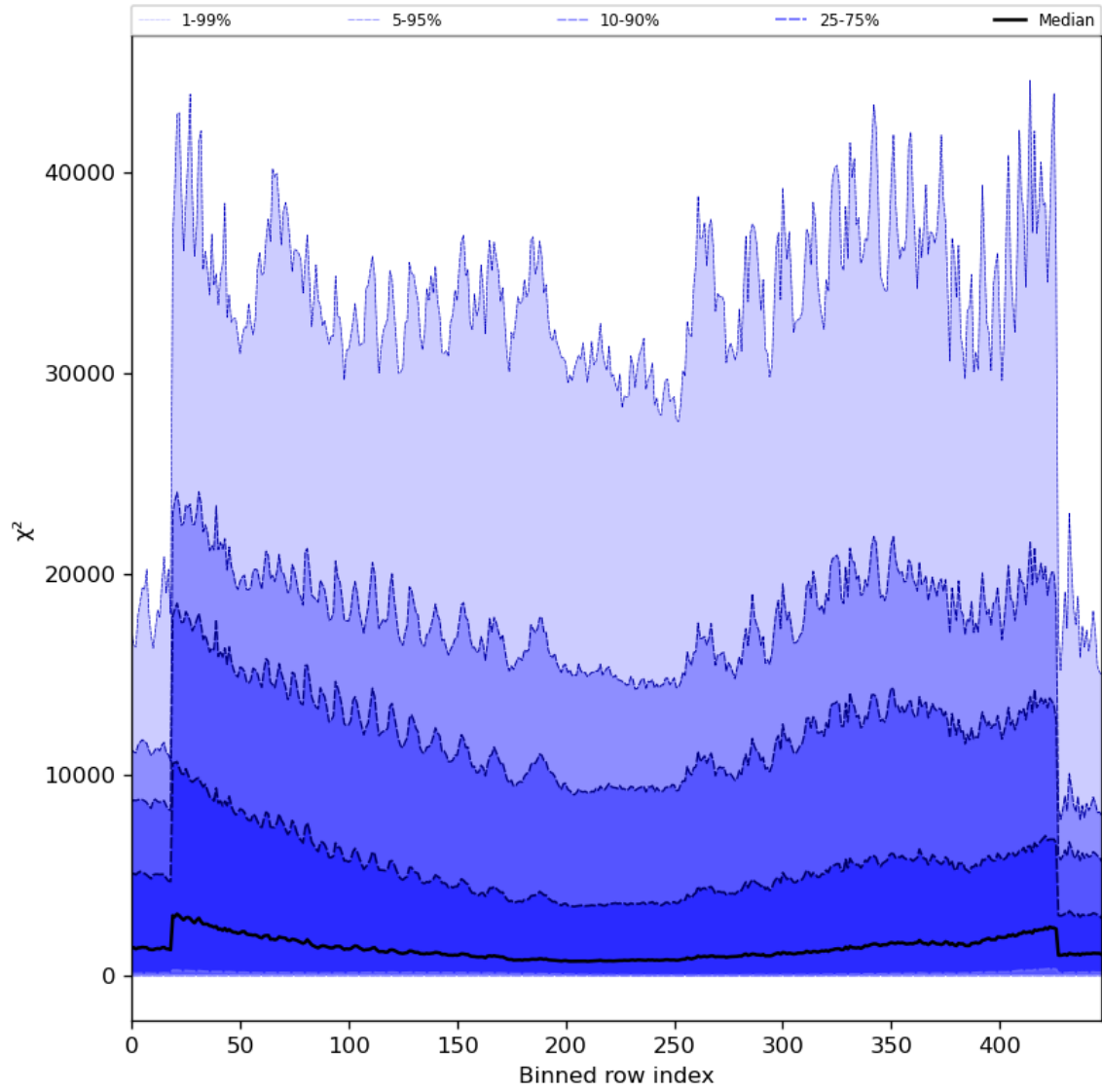
Figure 55: Along track statistics of “ \chi^2 ” for 2023-09-10 to 2023-09-12
