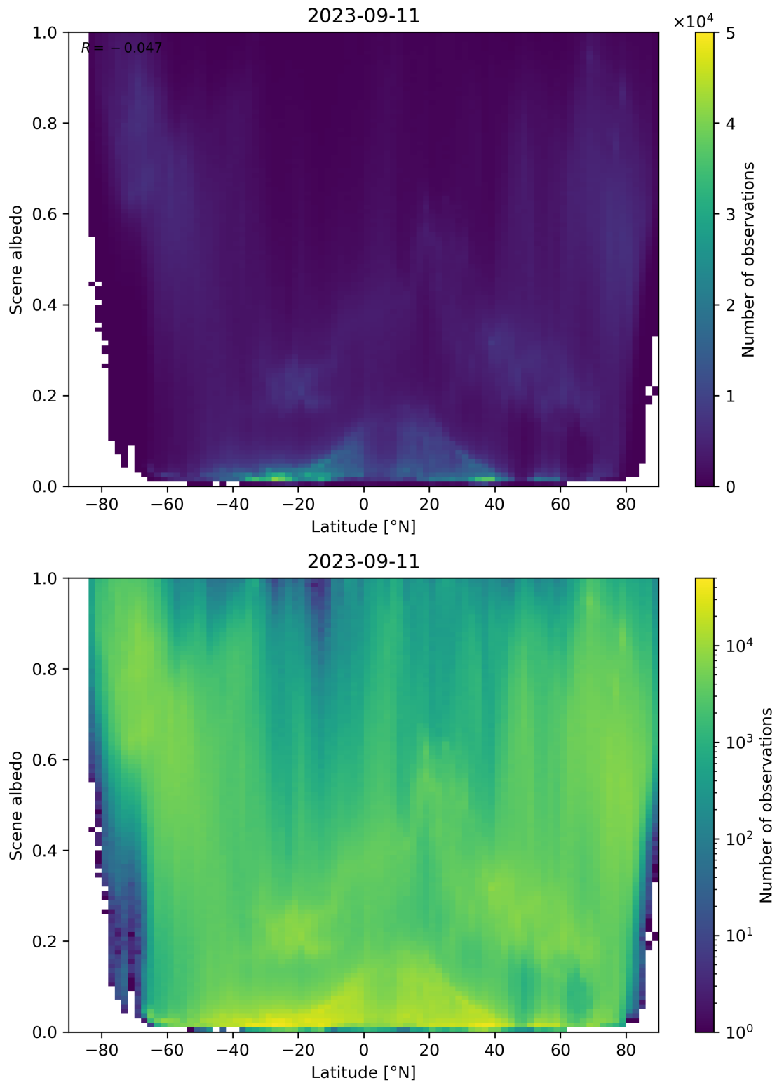
Figure 104: Scatter density plot of “Latitude” against “Scene albedo” for 2023-09-10 to 2023-09-12.
