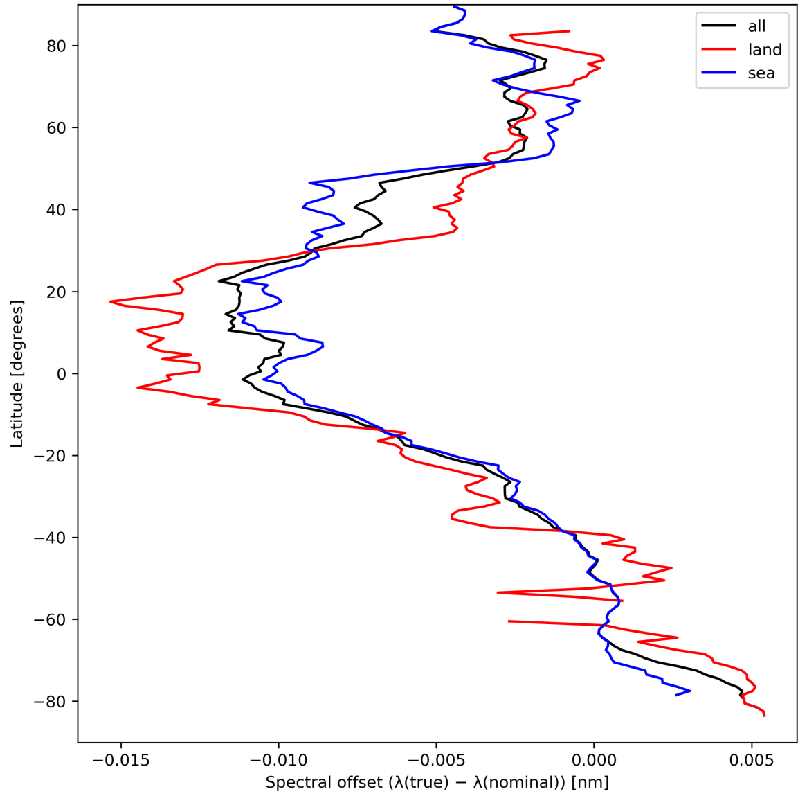
Figure 28: Zonal average of “Spectral offset ( \lambda(\text{true}) - \lambda(\text{nominal}) )” for 2023-09-10 to 2023-09-12.
