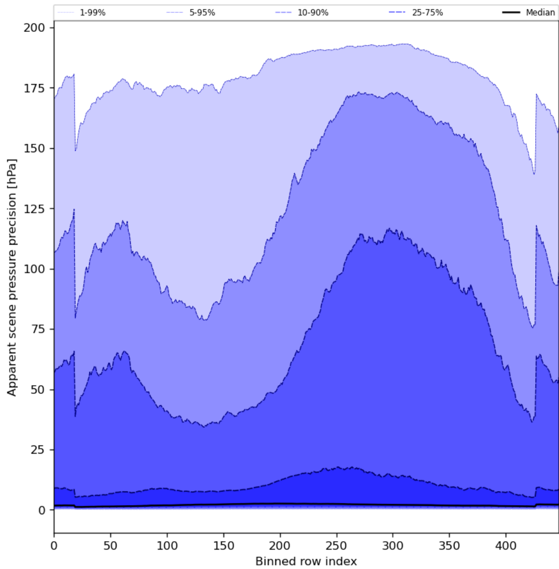
Figure 54: Along track statistics of “Apparent scene pressure precision” for 2023-09-10 to 2023-09-12
