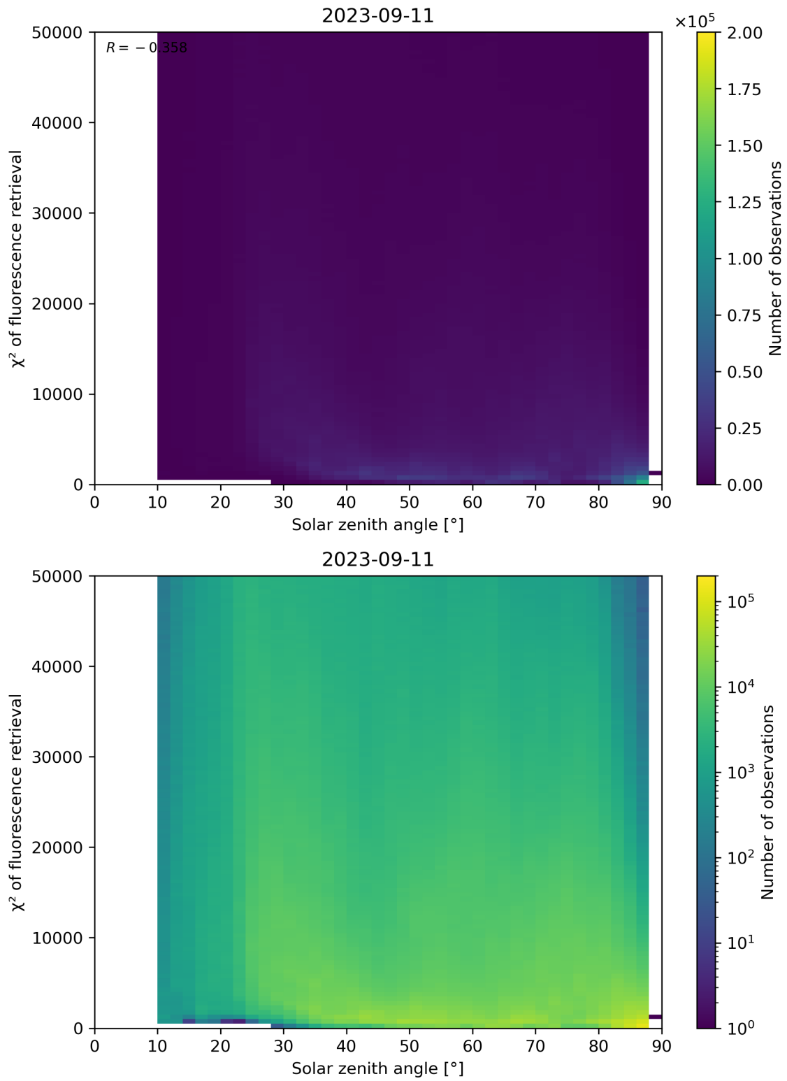
Figure 120: Scatter density plot of “Solar zenith angle” against “ \chi^2 of fluorescence retrieval” for 2023-09-10 to 2023-09-12.
