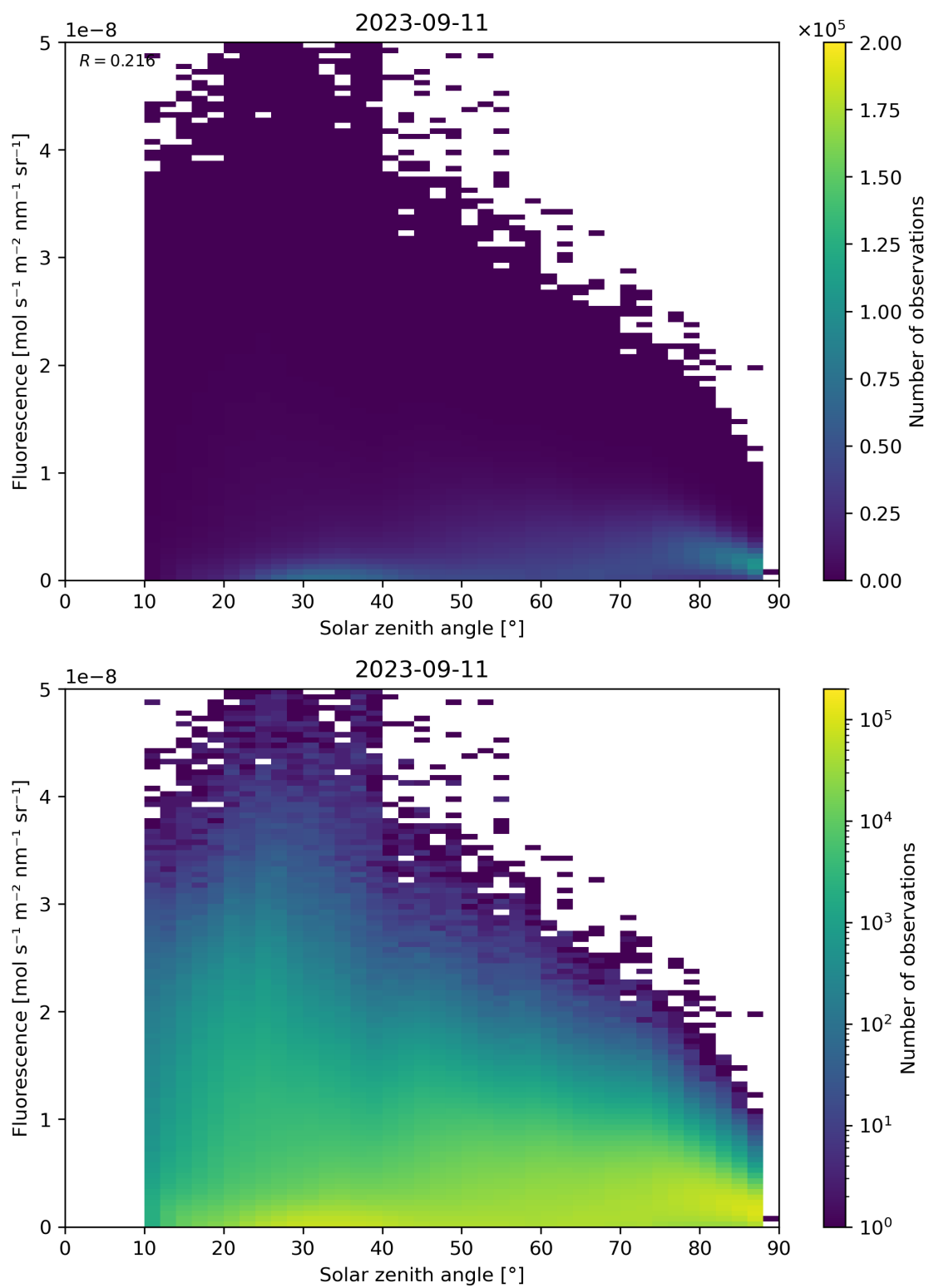
Figure 123: Scatter density plot of “Solar zenith angle” against “Fluorescence” for 2023-09-10 to 2023-09-12.
