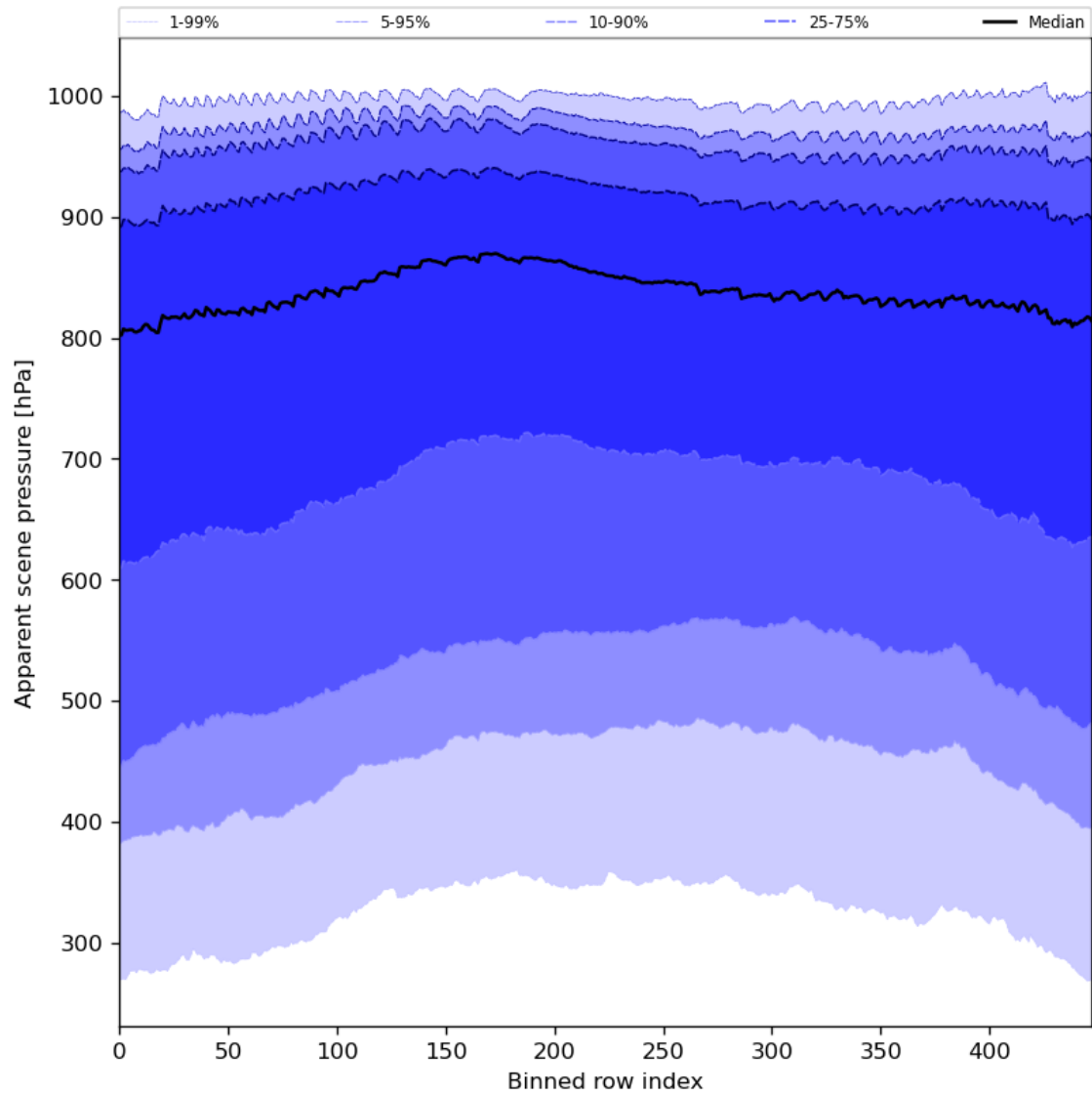
Figure 53: Along track statistics of “Apparent scene pressure” for 2023-09-10 to 2023-09-12
