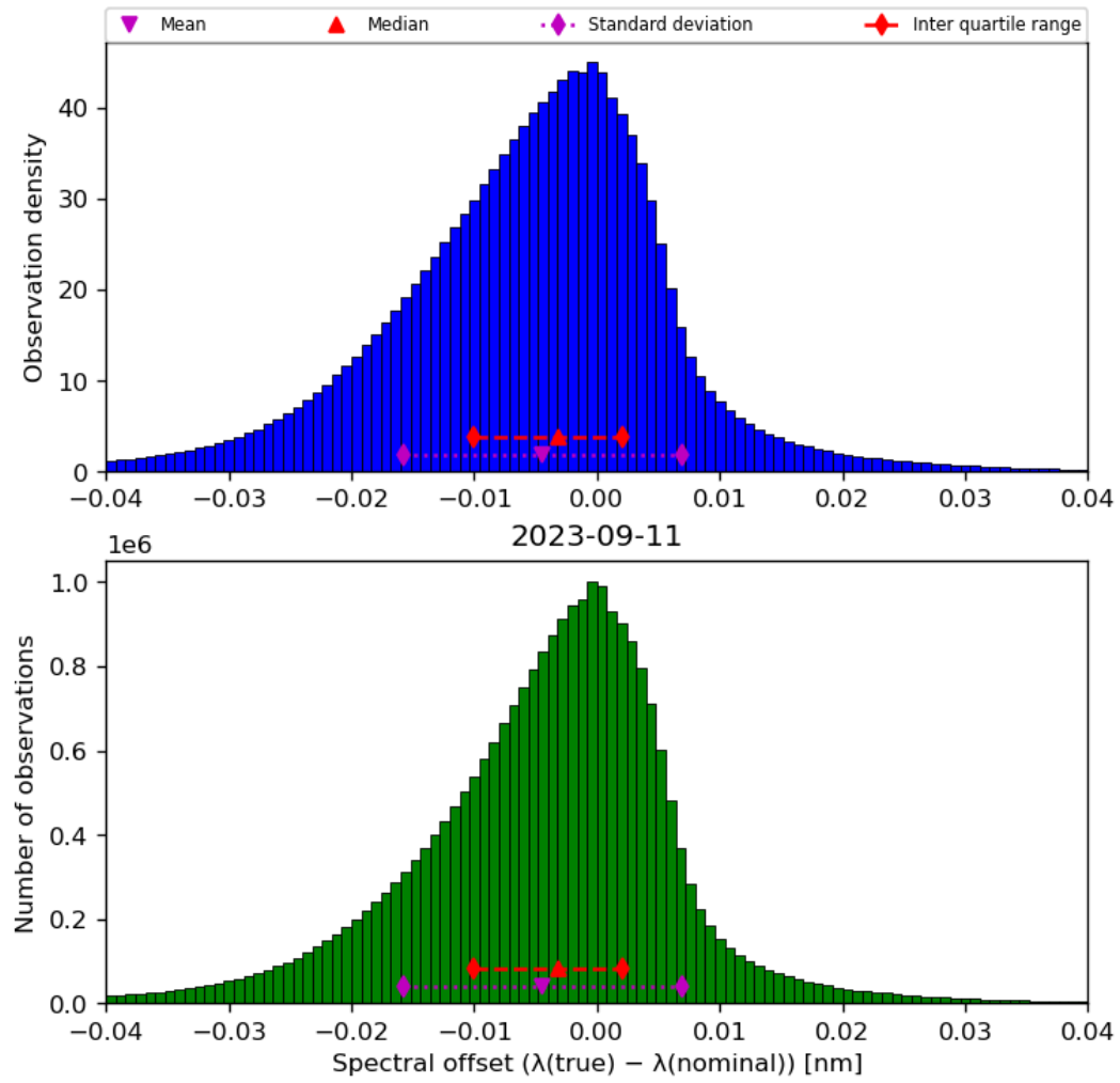
Figure 45: Histogram of “Spectral offset ( \lambda(\text{true}) - \lambda(\text{nominal}) )” for 2023-09-10 to 2023-09-12
