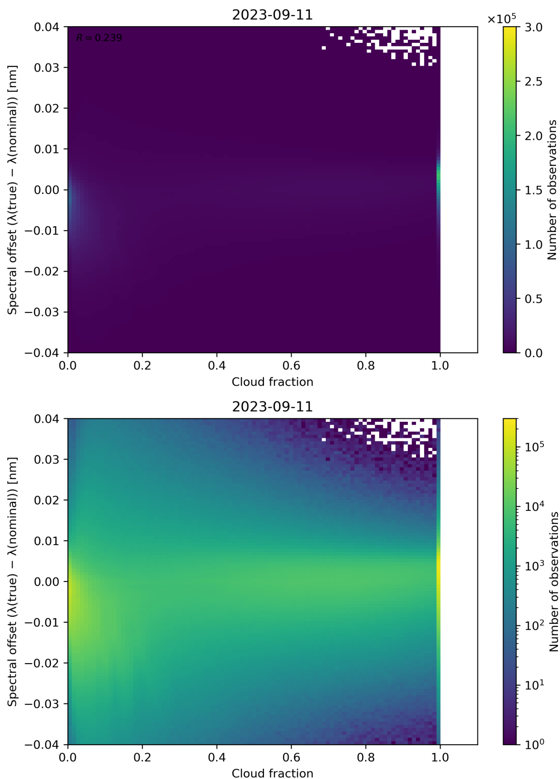
Figure 83: Scatter density plot of “Cloud fraction” against “Spectral offset ( \lambda(\text{true}) - \lambda(\text{nominal}) )” for 2023-09-10 to 2023-09-12.
