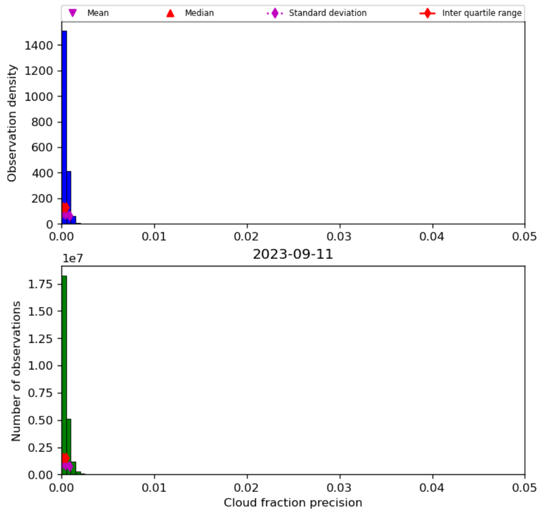
Figure 33: Histogram of “Cloud fraction precision” for 2023-09-10 to 2023-09-12
