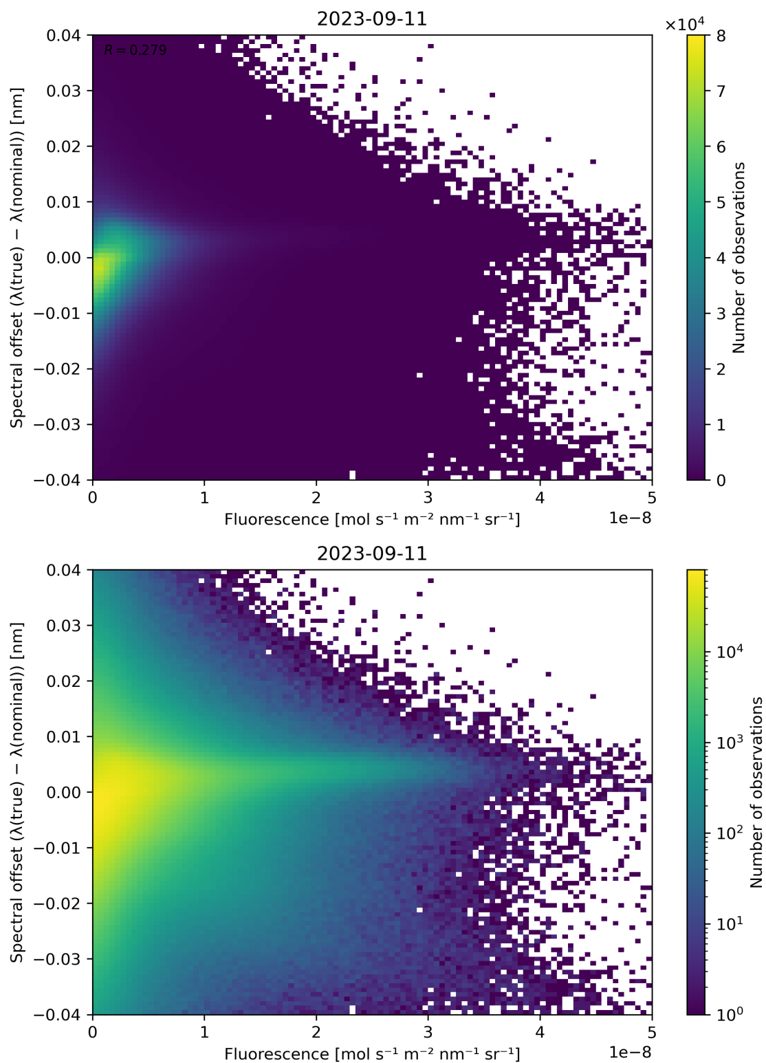
Figure 95: Scatter density plot of “Fluorescence” against “Spectral offset ( \lambda(\text{true}) - \lambda(\text{nominal}) )” for 2023-09-10 to 2023-09-12.
