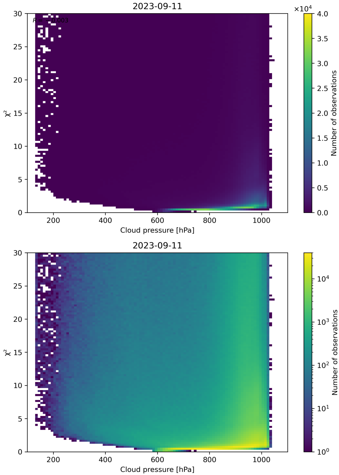
Figure 85: Scatter density plot of “Cloud pressure” against “ \chi^2 ” for 2023-09-10 to 2023-09-12.
