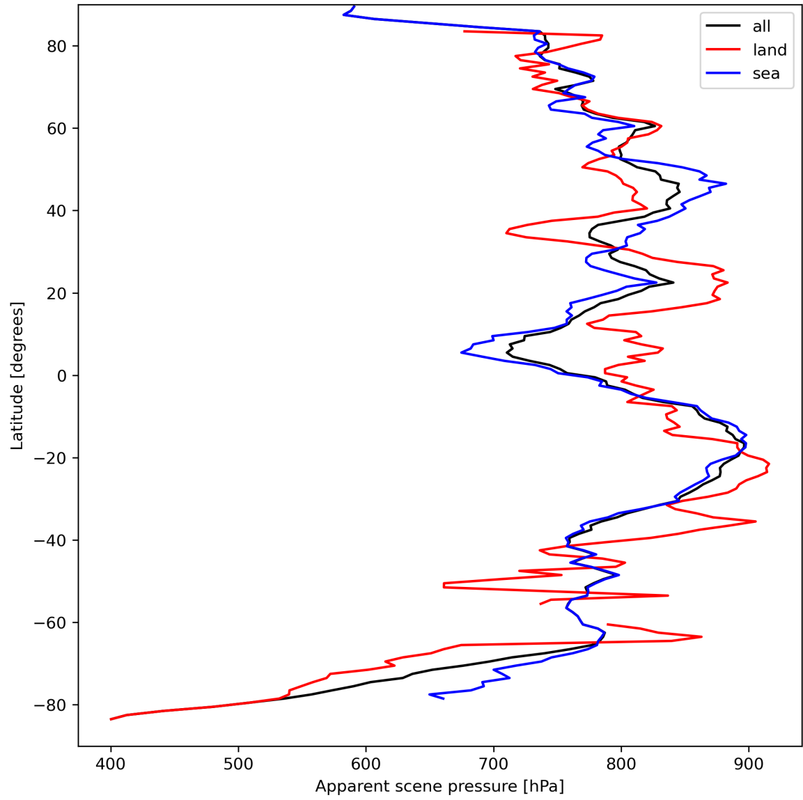
Figure 19: Zonal average of “Apparent scene pressure” for 2023-09-10 to 2023-09-12.
