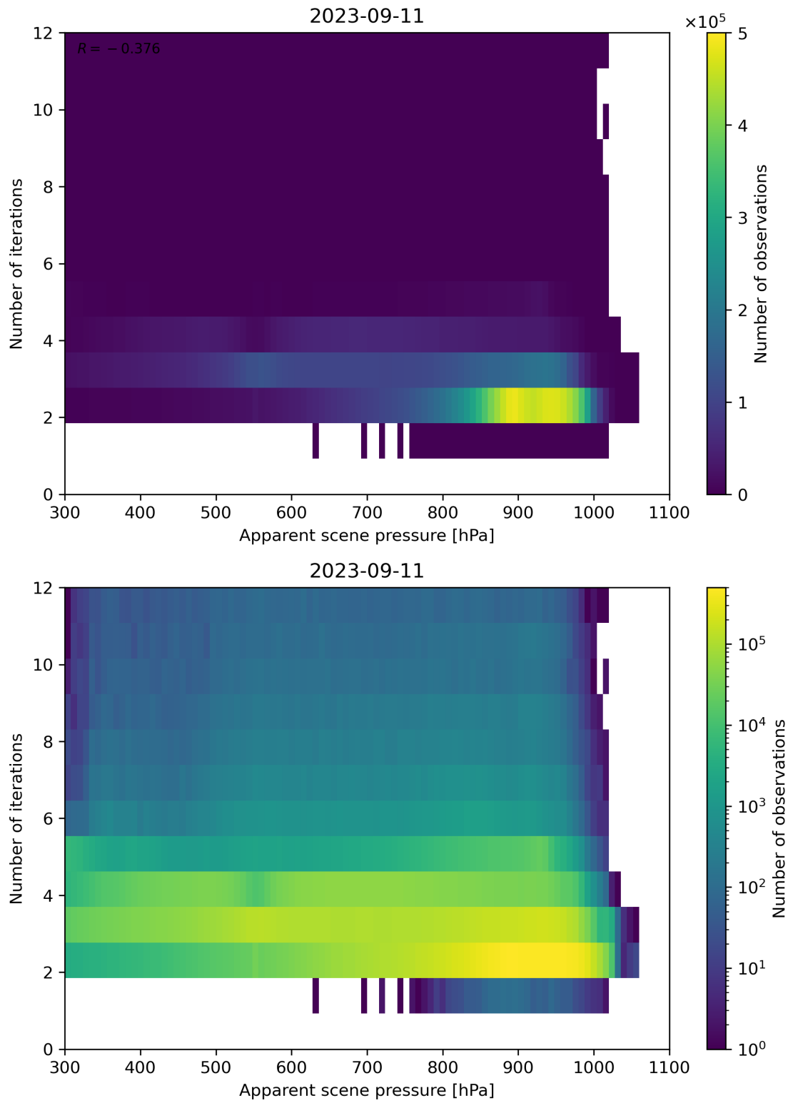
Figure 66: Scatter density plot of “Apparent scene pressure” against “Number of iterations” for 2023-09-10 to 2023-09-12.
