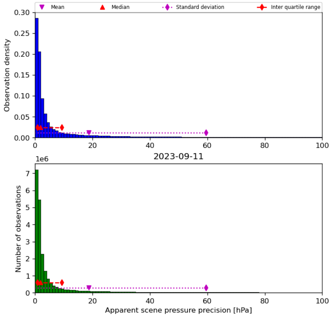
Figure 37: Histogram of “Apparent scene pressure precision” for 2023-09-10 to 2023-09-12
