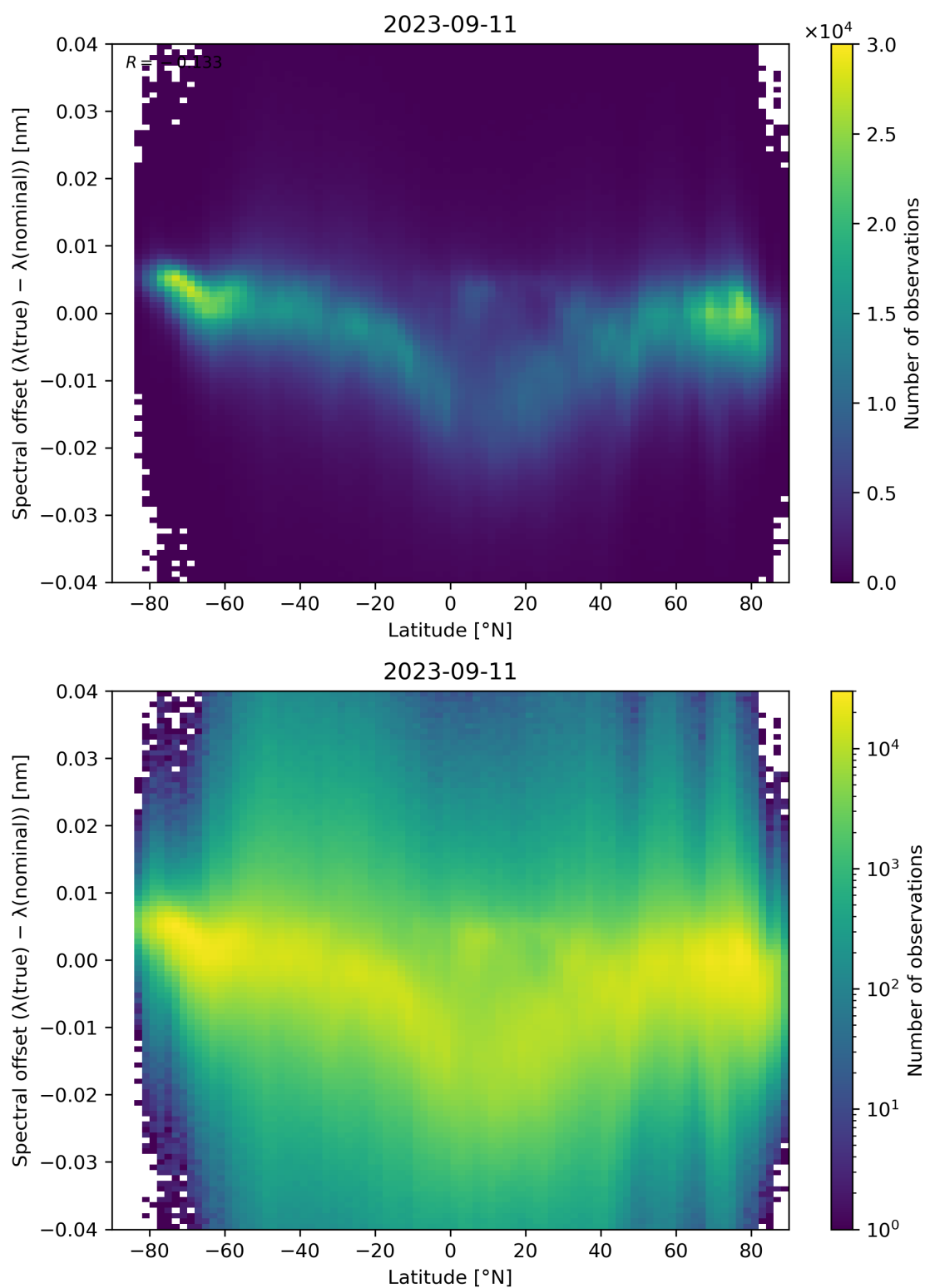
Figure 105: Scatter density plot of “Latitude” against “Spectral offset ( \lambda(\text{true}) - \lambda(\text{nominal}) )” for 2023-09-10 to 2023-09-12.
