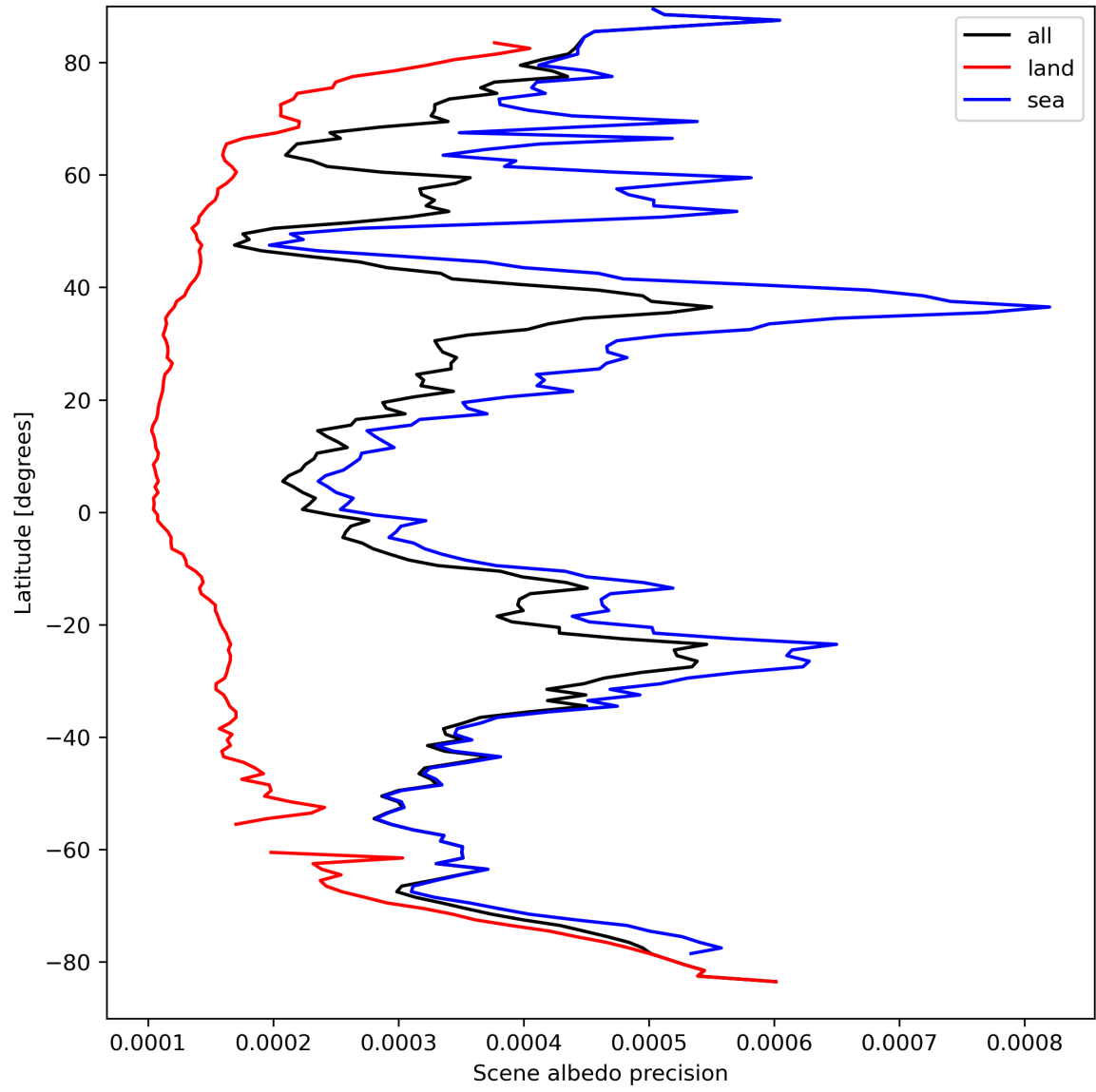
Figure 18: Zonal average of “Scene albedo precision” for 2023-09-10 to 2023-09-12.
