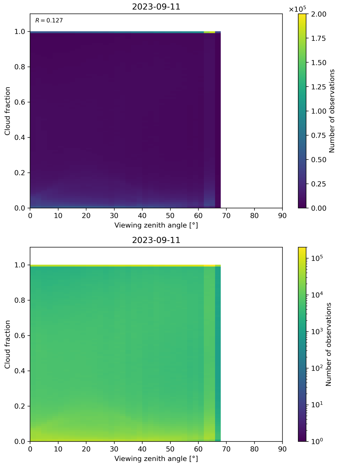
Figure 132: Scatter density plot of “Viewing zenith angle” against “Cloud fraction” for 2023-09-10 to 2023-09-12.
