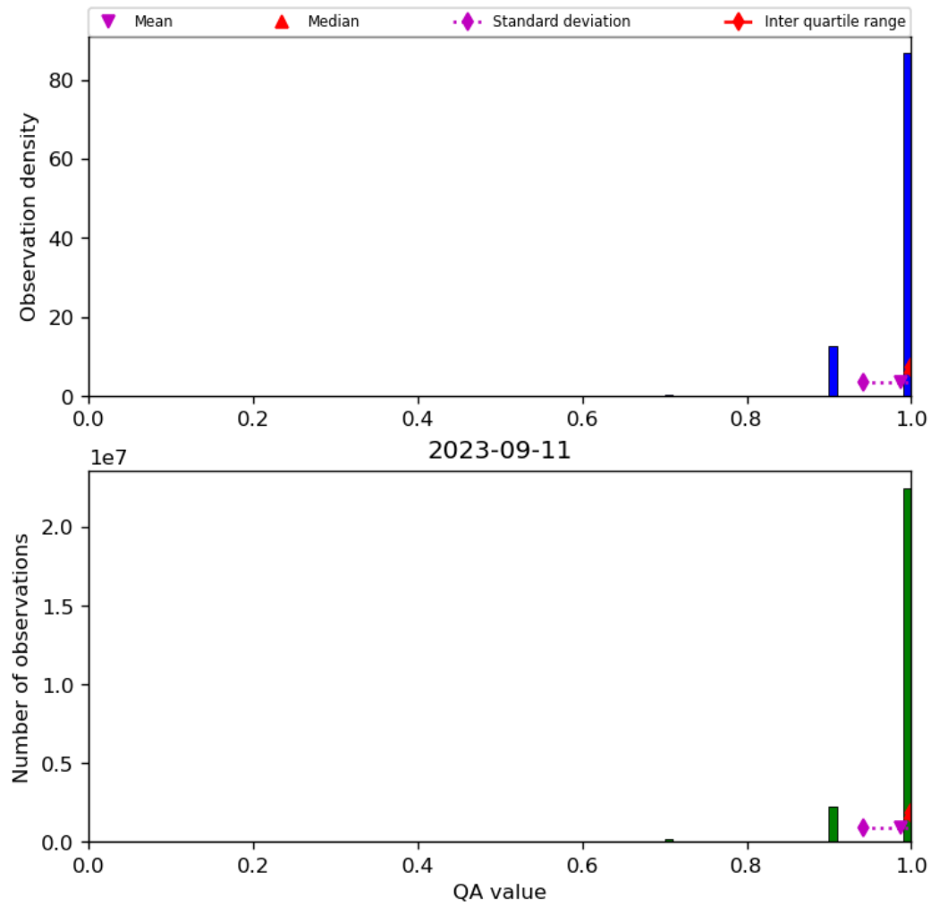
Figure 29: Histogram of “QA value” for 2023-09-10 to 2023-09-12
