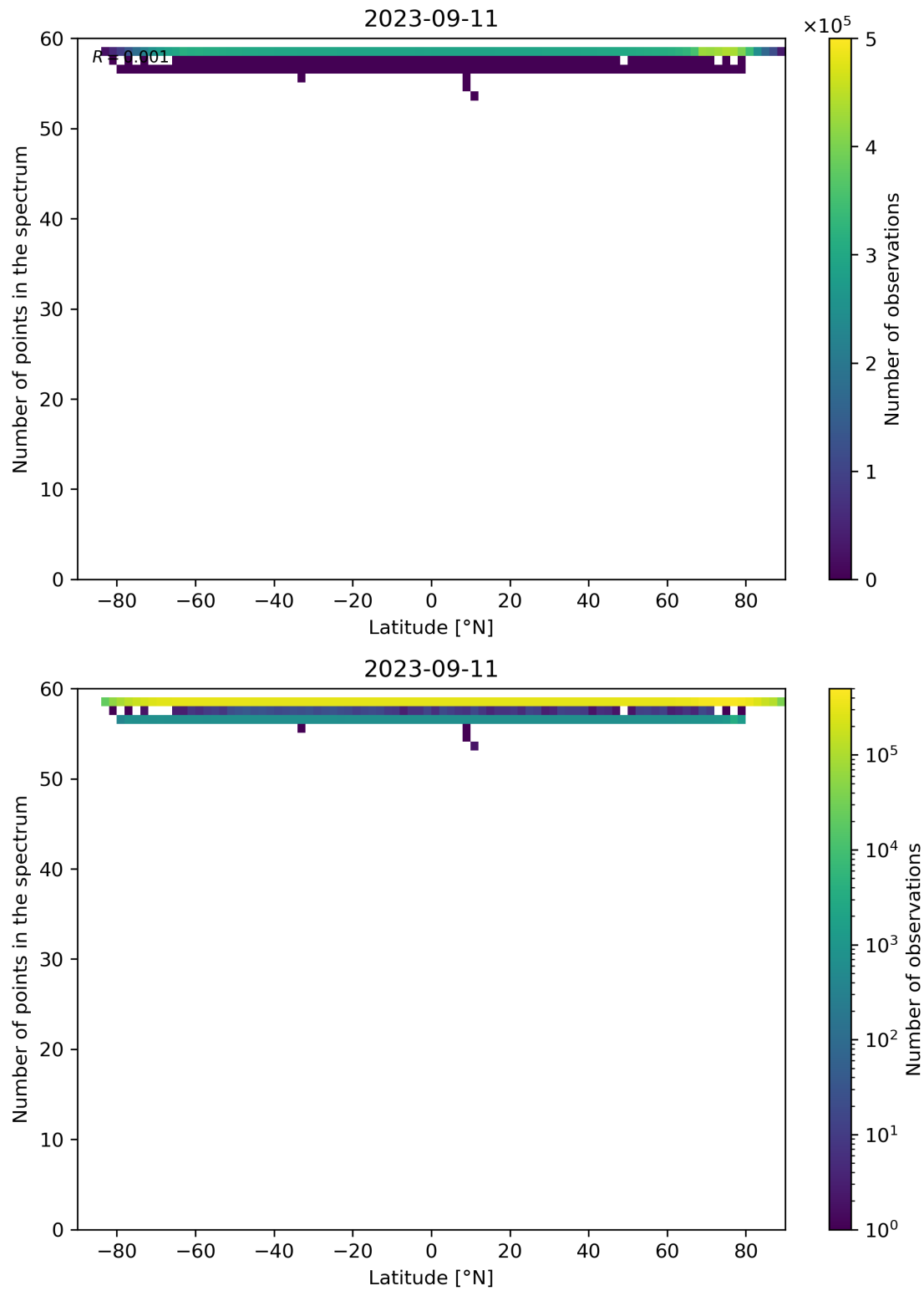
Figure 103: Scatter density plot of “Latitude” against “Number of points in the spectrum” for 2023-09-10 to 2023-09-12.
