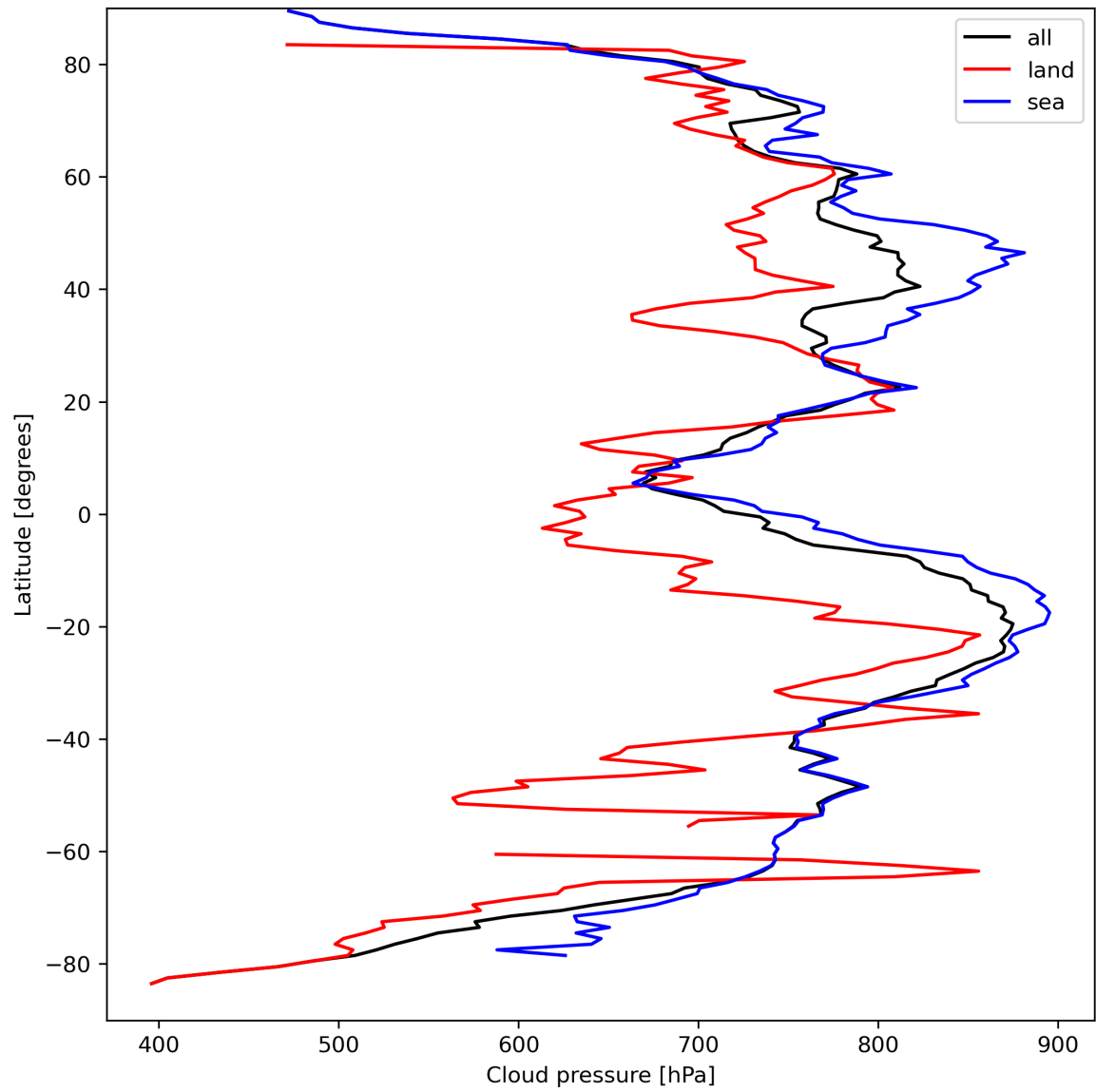
Figure 13: Zonal average of “Cloud pressure” for 2023-09-10 to 2023-09-12.
