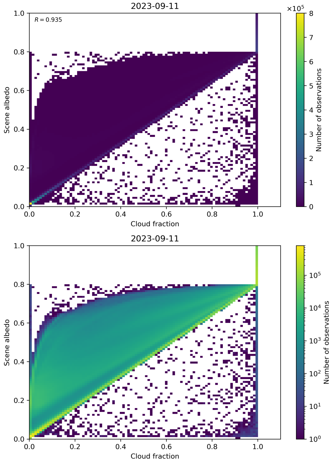
Figure 82: Scatter density plot of “Cloud fraction” against “Scene albedo” for 2023-09-10 to 2023-09-12.
