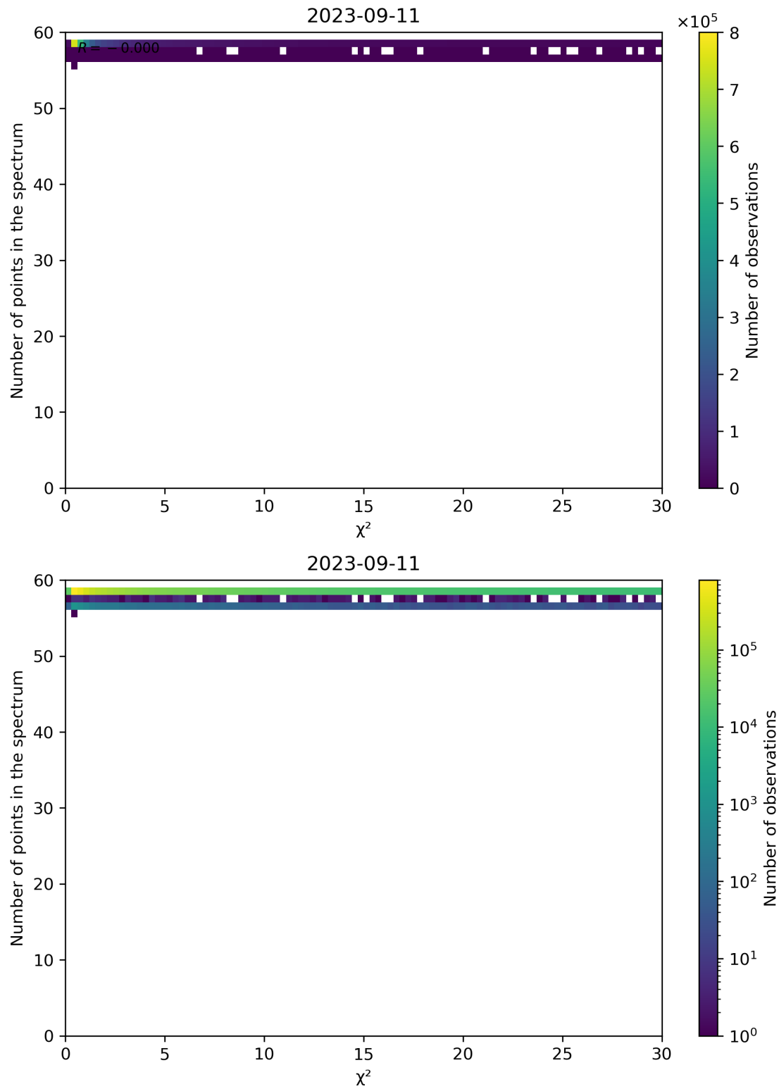
Figure 74: Scatter density plot of " \chi^2 " against "Number of points in the spectrum" for 2023-09-10 to 2023-09-12.
