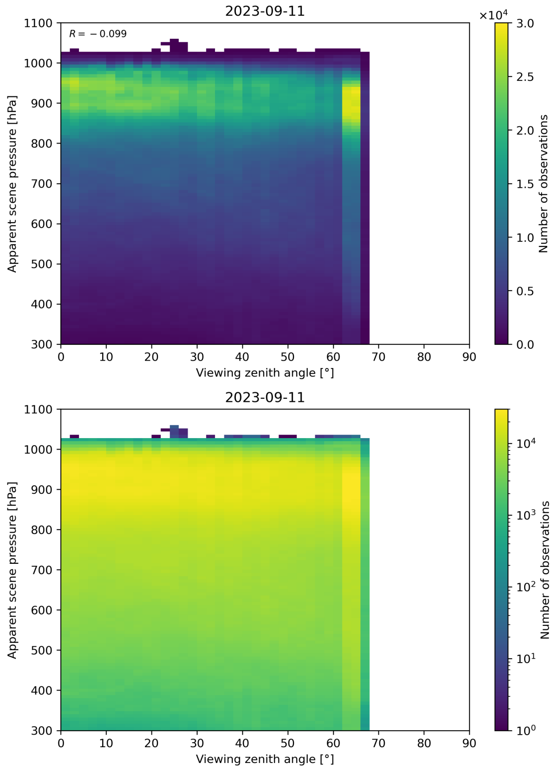
Figure 129: Scatter density plot of “Viewing zenith angle” against “Apparent scene pressure” for 2023-09-10 to 2023-09-12.
