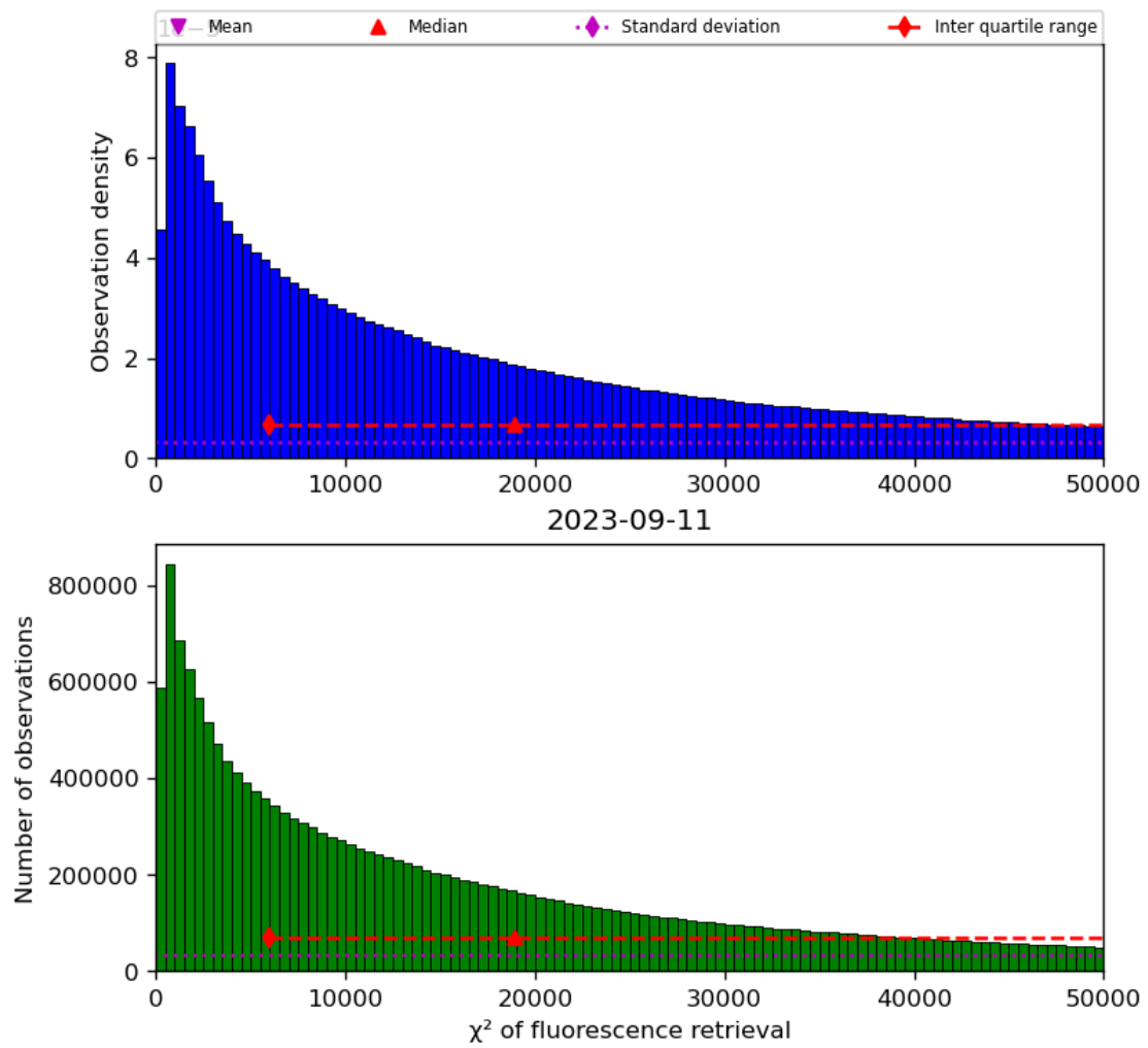
Figure 42: Histogram of “ \chi^2 of fluorescence retrieval” for 2023-09-10 to 2023-09-12
