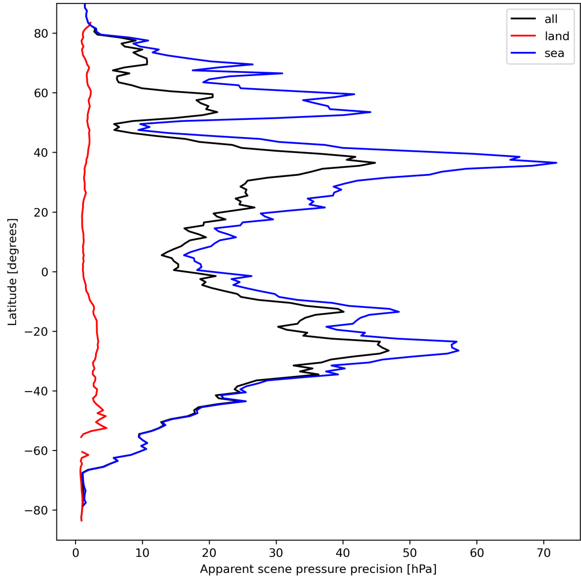
Figure 20: Zonal average of “Apparent scene pressure precision” for 2023-09-10 to 2023-09-12.
