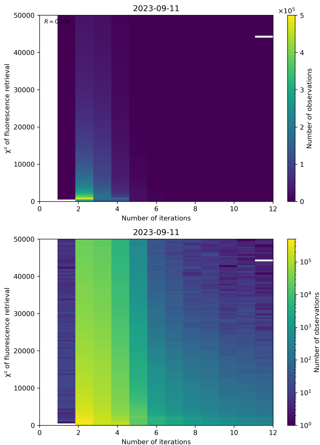
Figure 106: Scatter density plot of “Number of iterations” against “ \chi^2 of fluorescence retrieval” for 2023-09-10 to 2023-09-12.
