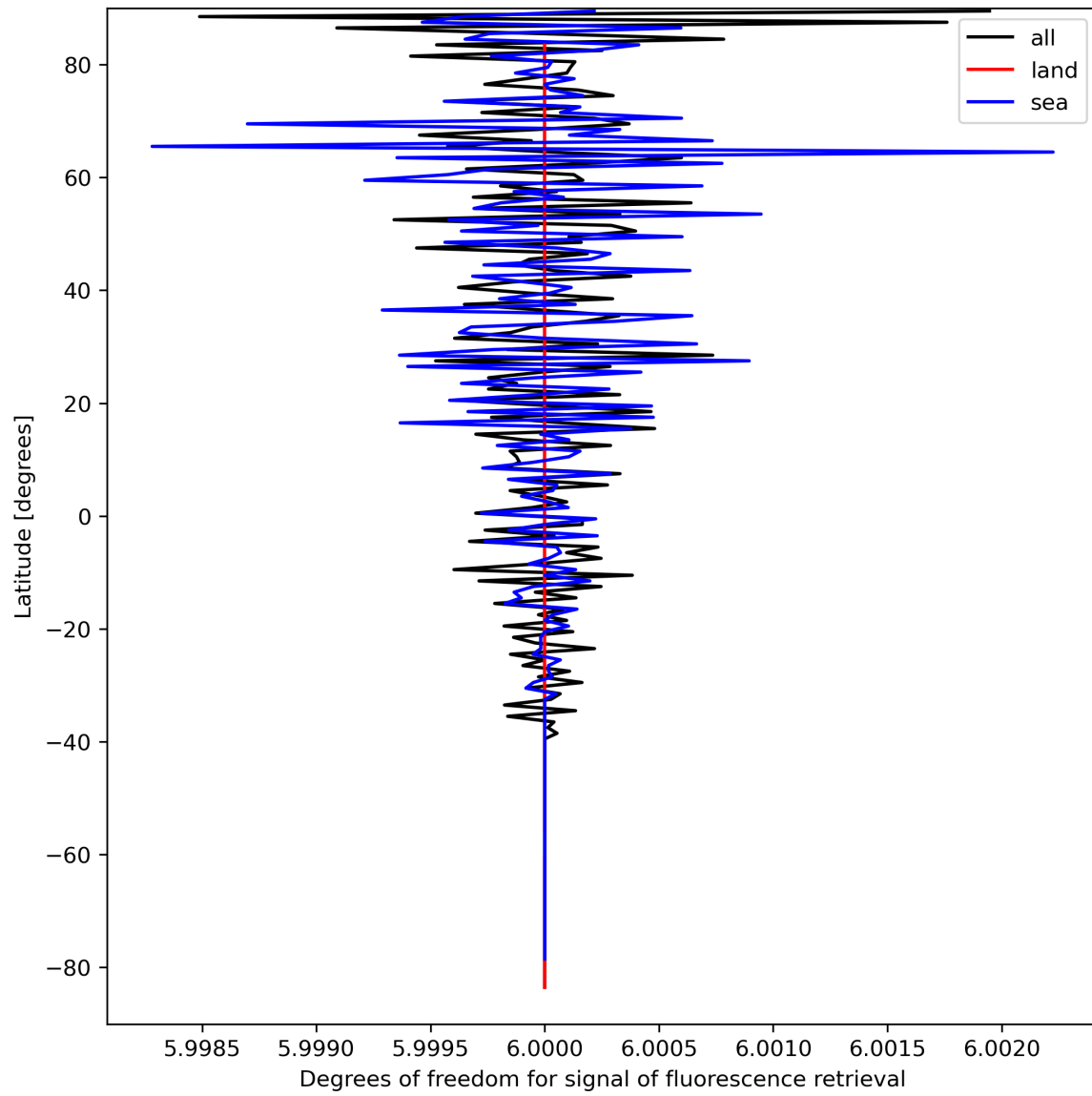
Figure 26: Zonal average of “Degrees of freedom for signal of fluorescence retrieval” for 2023-09-10 to 2023-09-12.
