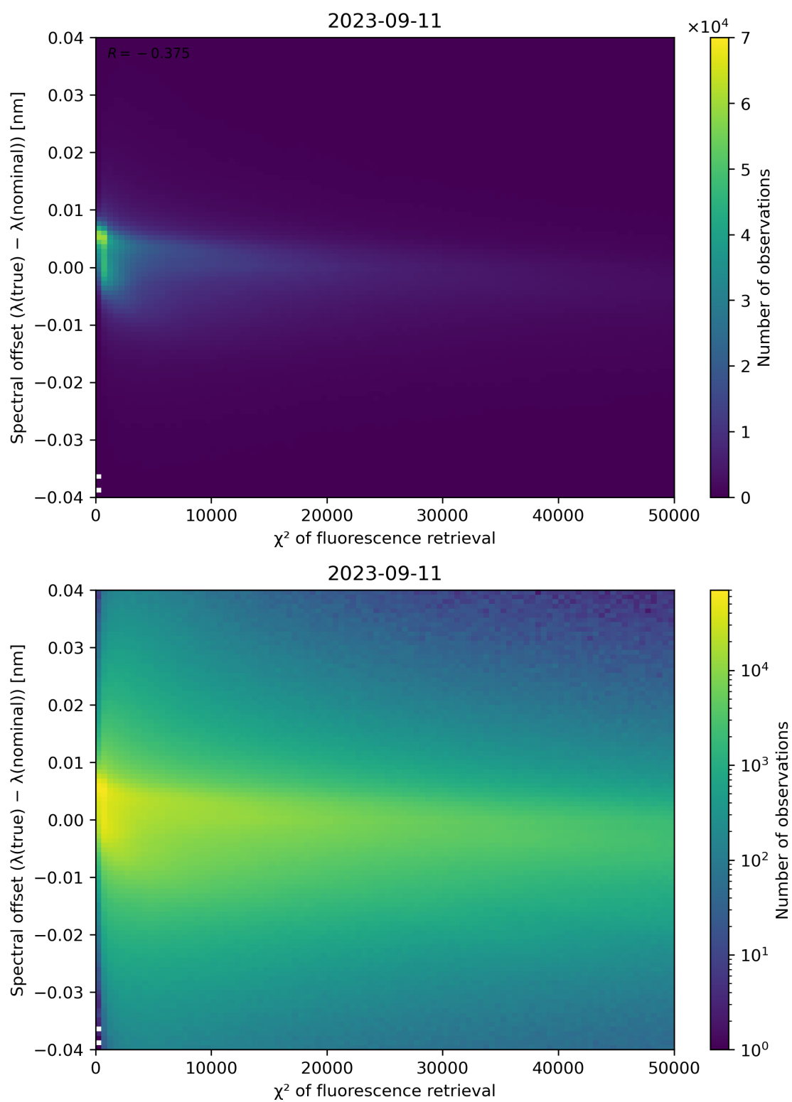
Figure 72: Scatter density plot of " \chi^2 of fluorescence retrieval" against "Spectral offset ( \lambda(\text{true}) - \lambda(\text{nominal}) )" for 2023-09-10 to 2023-09-12.
