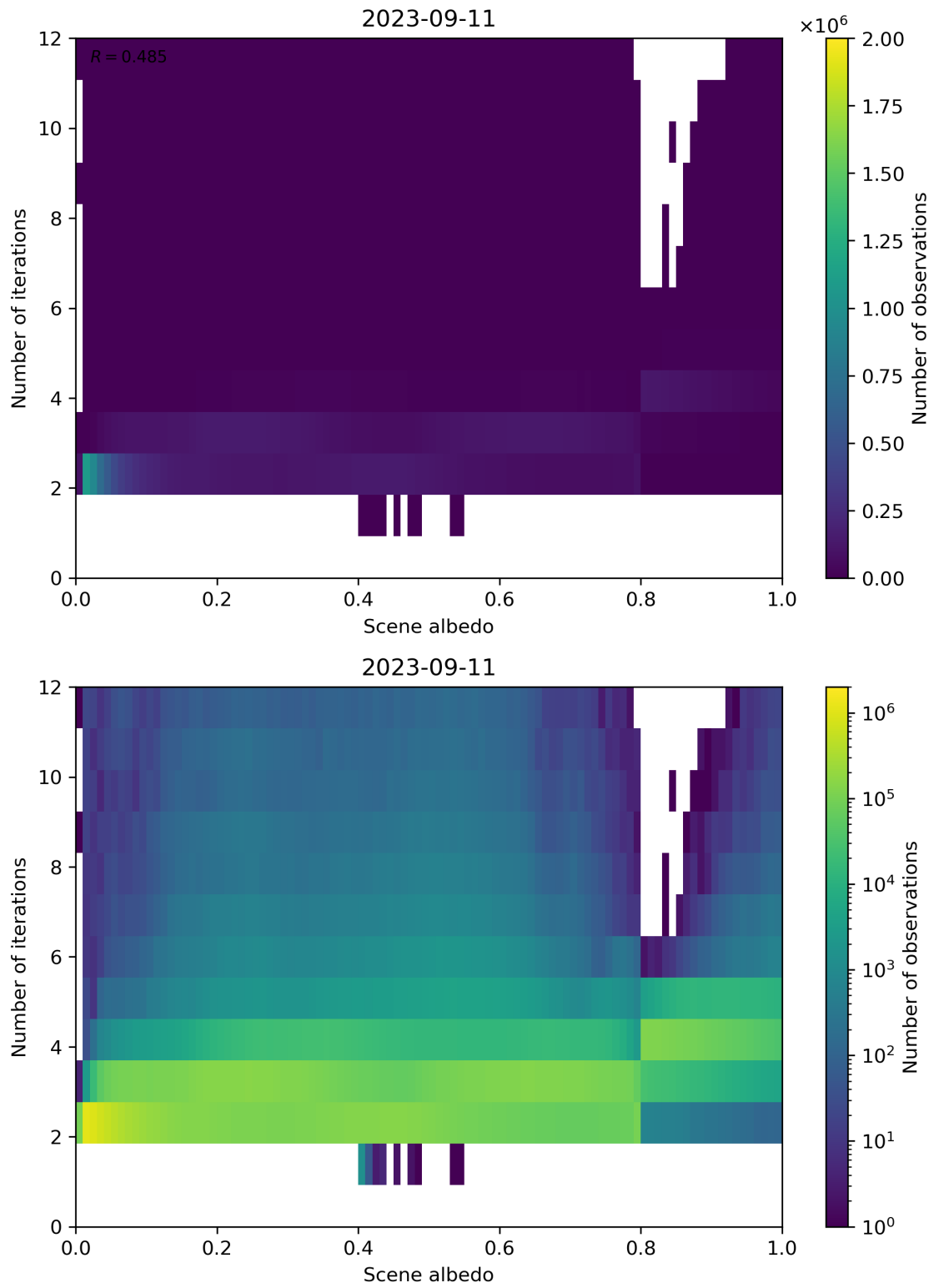
Figure 115: Scatter density plot of “Scene albedo” against “Number of iterations” for 2023-09-10 to 2023-09-12.
