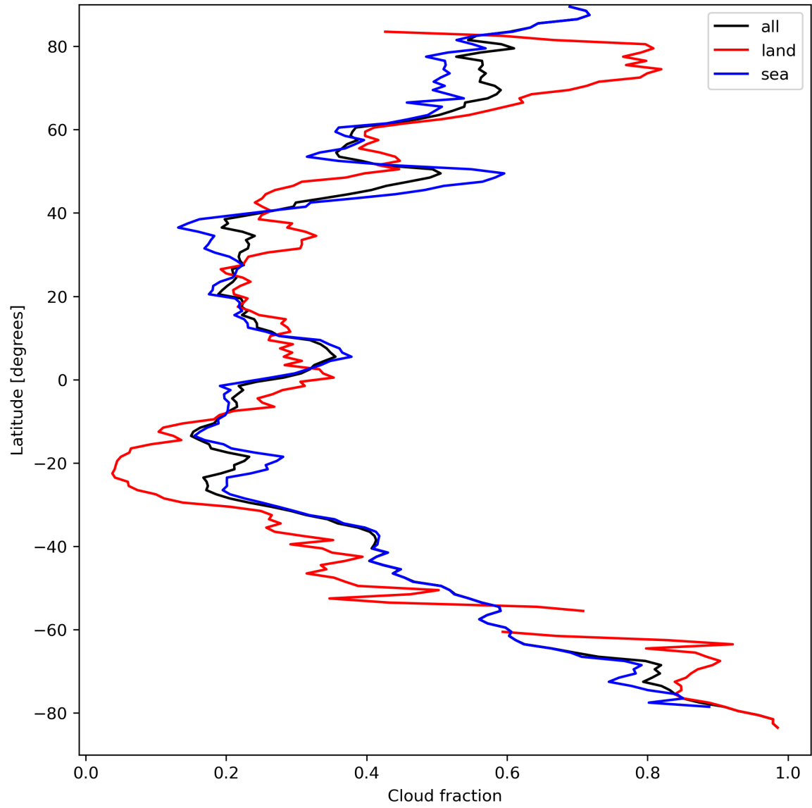
Figure 15: Zonal average of “Cloud fraction” for 2023-09-10 to 2023-09-12.
