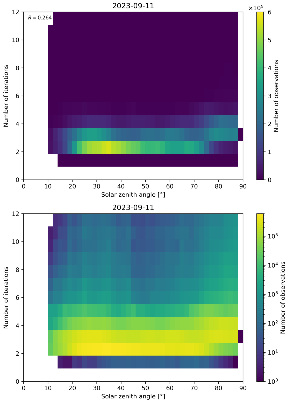
Figure 125: Scatter density plot of “Solar zenith angle” against “Number of iterations” for 2023-09-10 to 2023-09-12.
