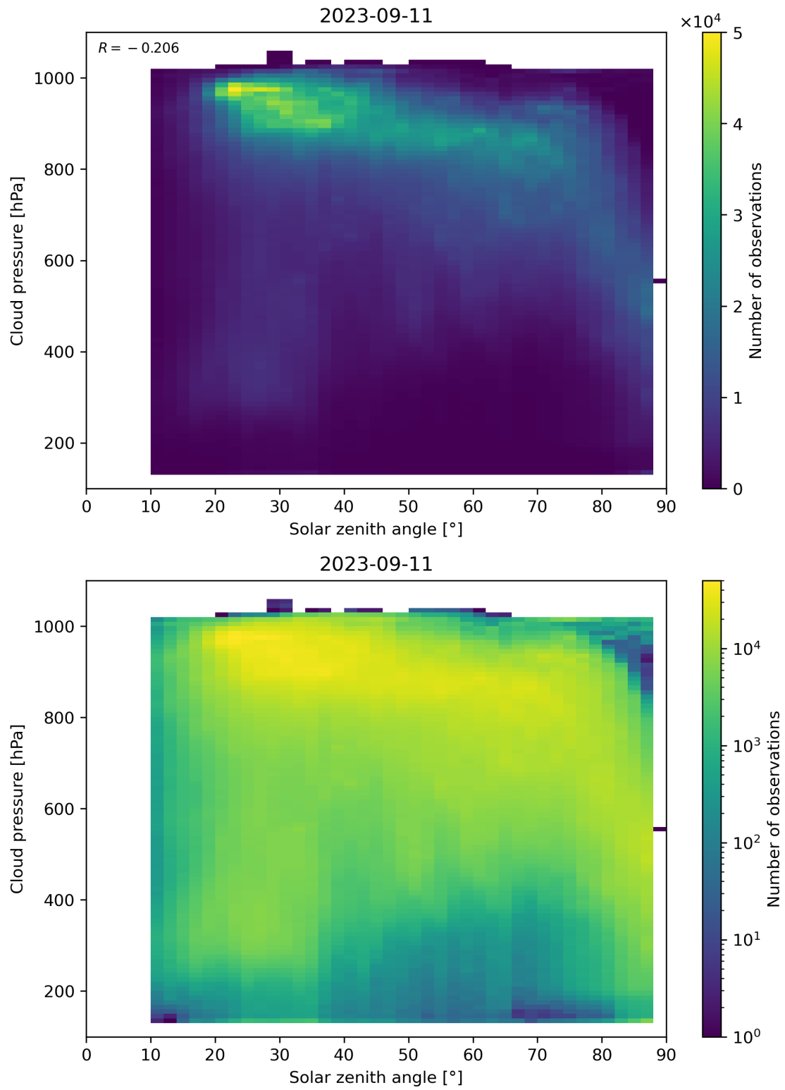
Figure 122: Scatter density plot of “Solar zenith angle” against “Cloud pressure” for 2023-09-10 to 2023-09-12.
