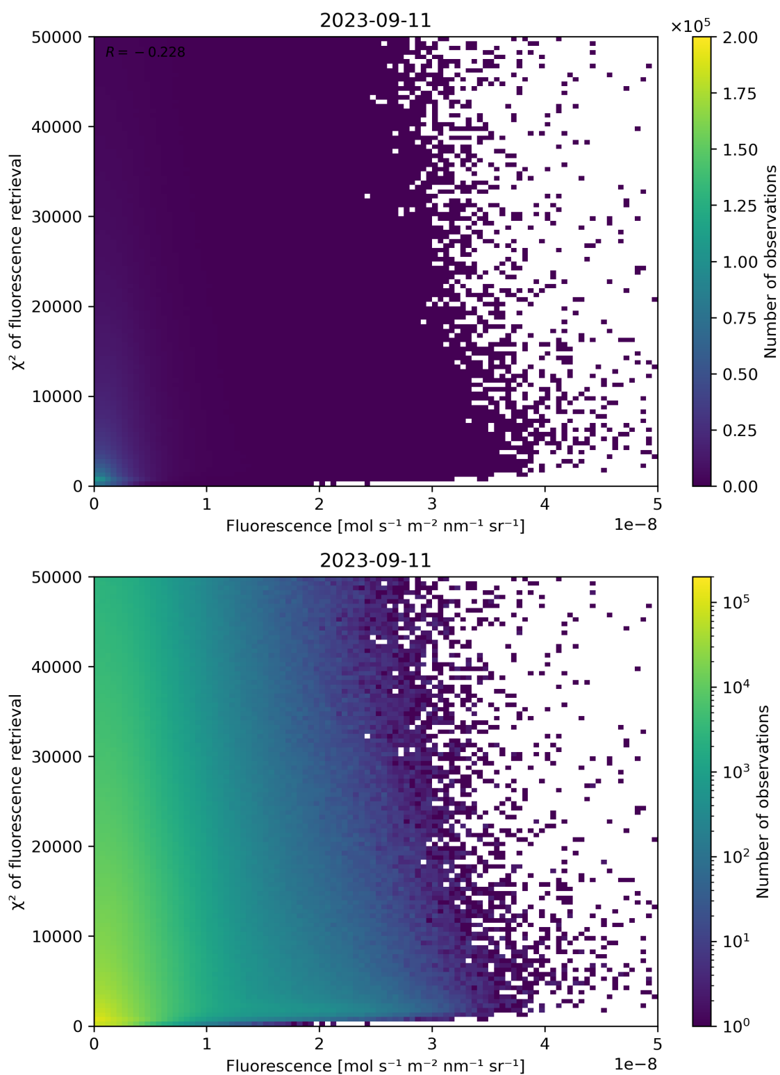
Figure 93: Scatter density plot of “Fluorescence” against “ \chi^2 of fluorescence retrieval” for 2023-09-10 to 2023-09-12.
