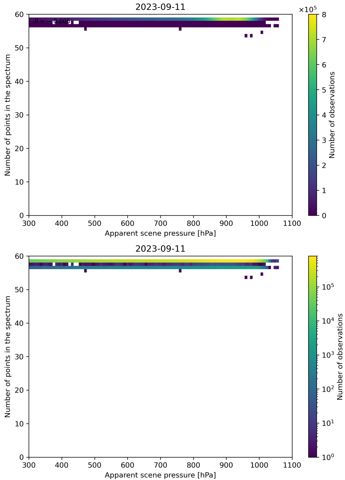
Figure 67: Scatter density plot of “Apparent scene pressure” against “Number of points in the spectrum” for 2023-09-10 to 2023-09-12.
