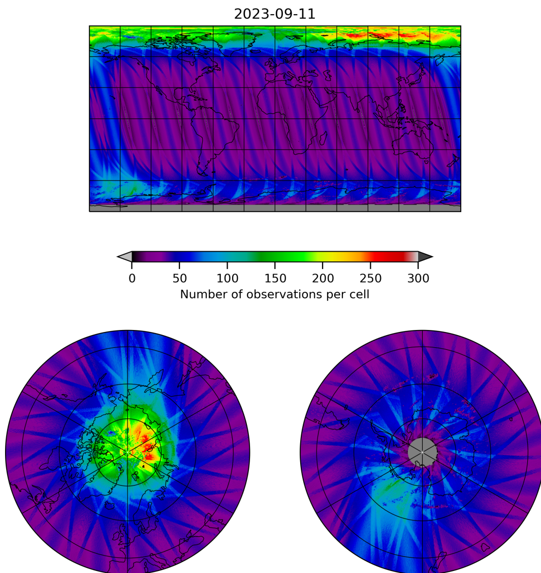
Figure 11: Map of the number of observations for 2023-09-10 to 2023-09-12
