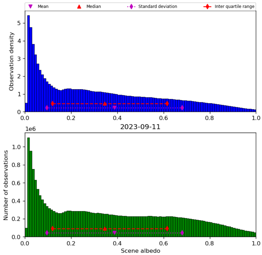
Figure 34: Histogram of “Scene albedo” for 2023-09-10 to 2023-09-12
