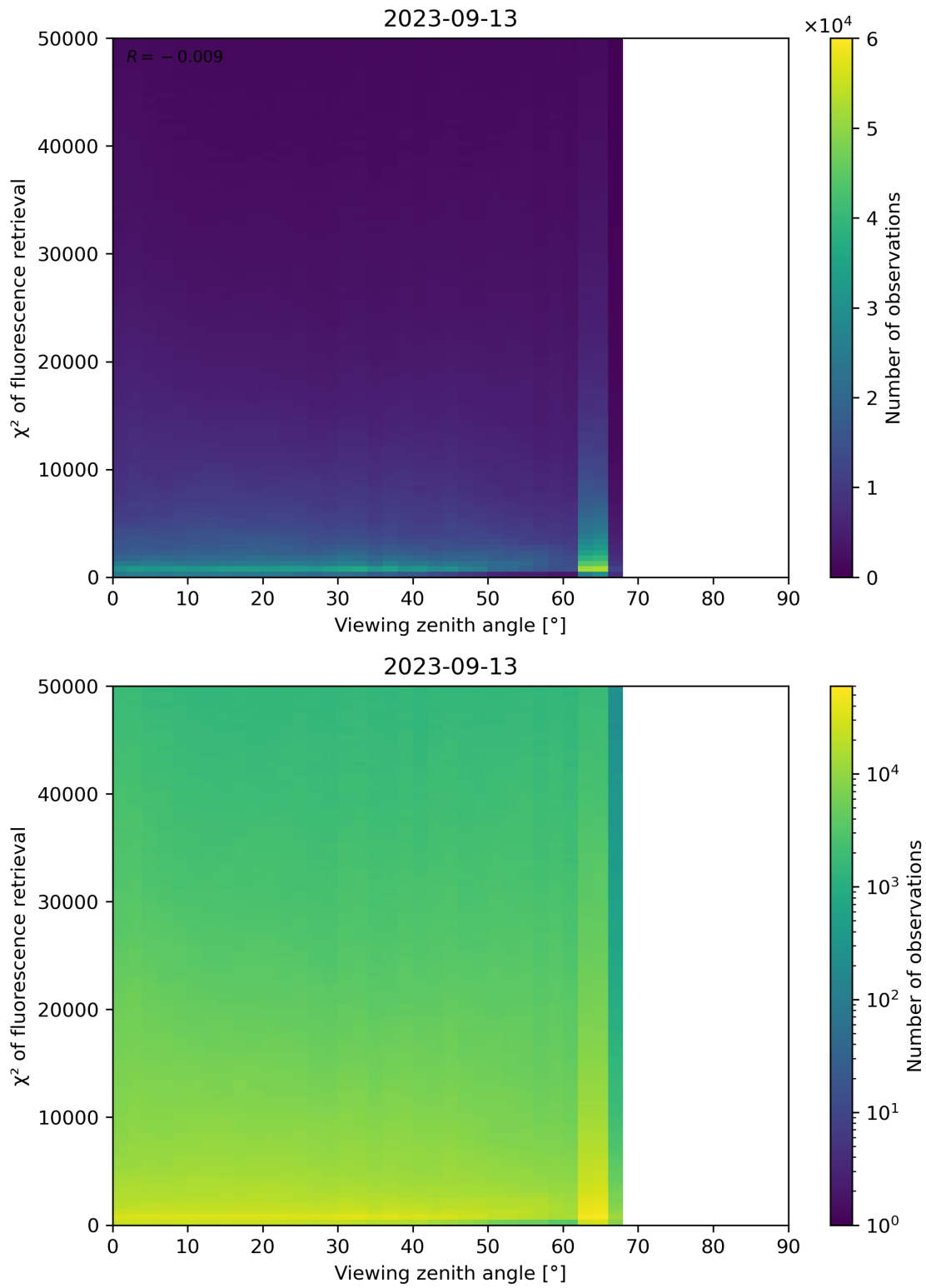
Figure 131: Scatter density plot of “Viewing zenith angle” against “ \chi^2 of fluorescence retrieval” for 2023-09-12 to 2023-09-14.
