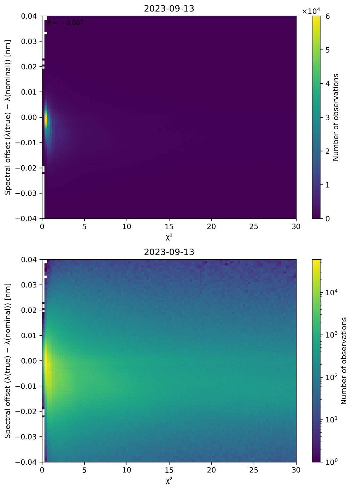
Figure 75: Scatter density plot of " \chi^2 " against "Spectral offset ( \lambda(\text{true}) - \lambda(\text{nominal}) )" for 2023-09-12 to 2023-09-14.
