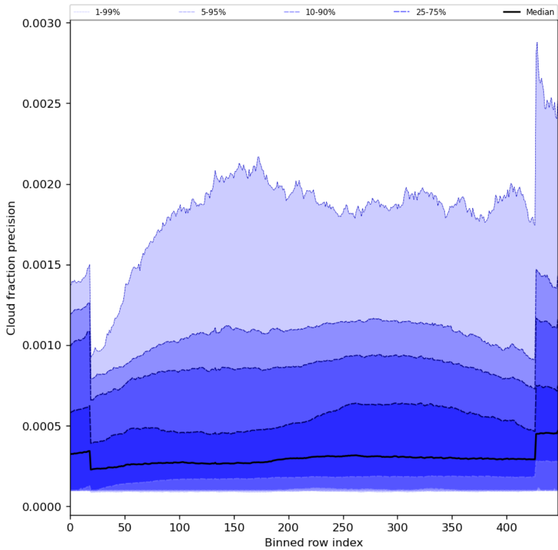
Figure 50: Along track statistics of “Cloud fraction precision” for 2023-09-12 to 2023-09-14
