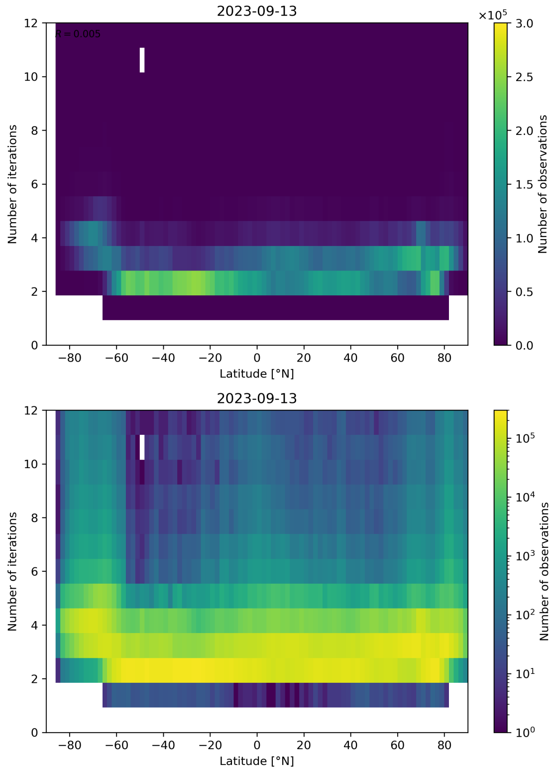
Figure 102: Scatter density plot of “Latitude” against “Number of iterations” for 2023-09-12 to 2023-09-14.
