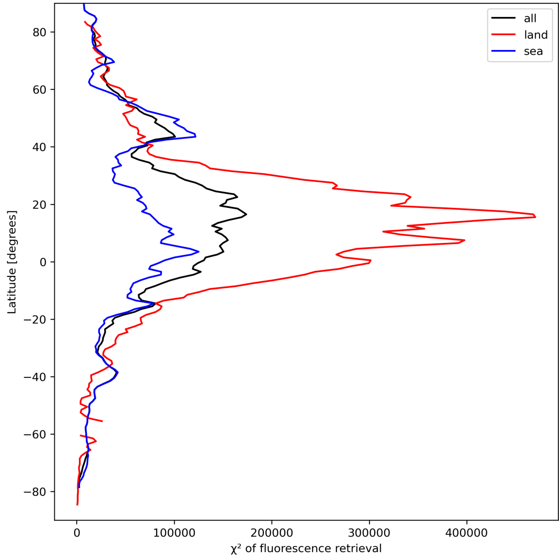
Figure 25: Zonal average of “ \chi^2 of fluorescence retrieval” for 2023-09-12 to 2023-09-14.
