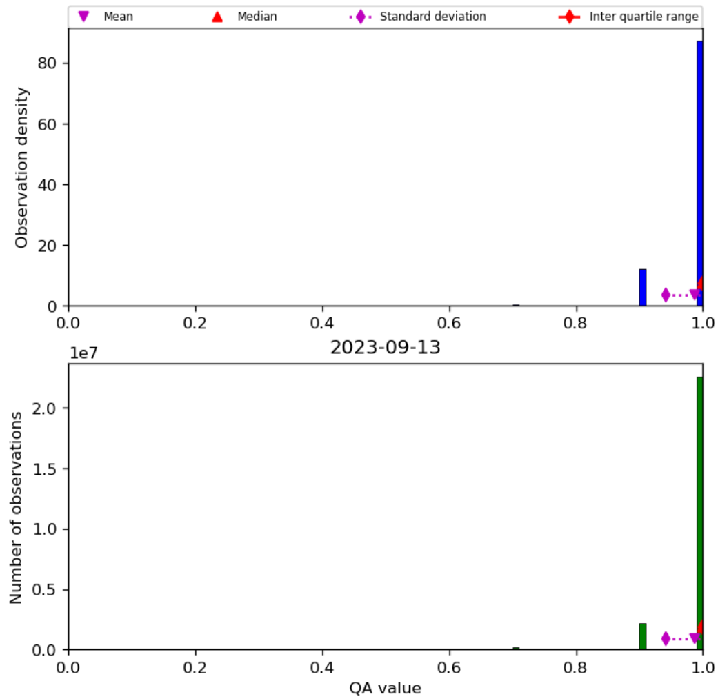
Figure 29: Histogram of “QA value” for 2023-09-12 to 2023-09-14
