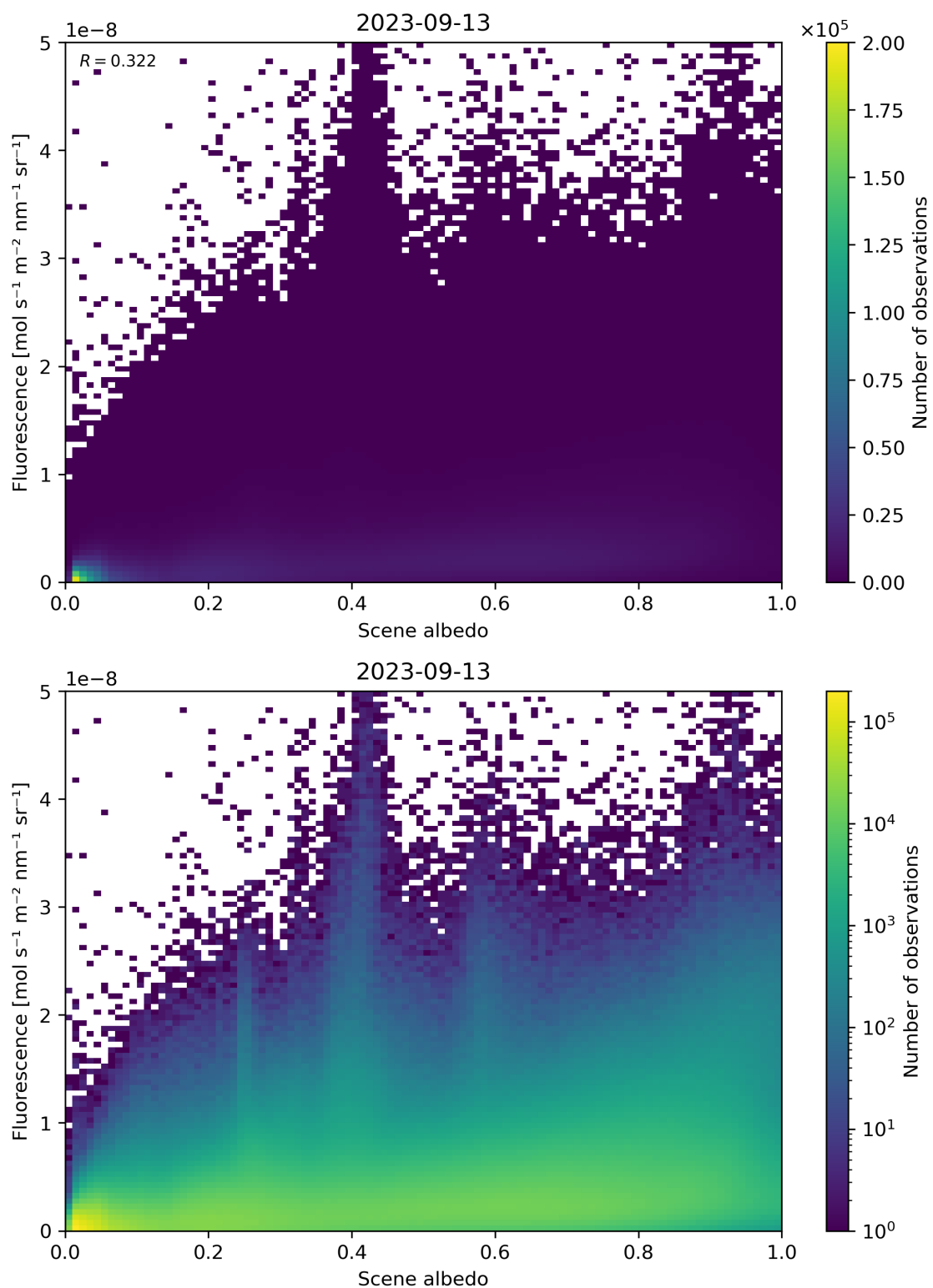
Figure 114: Scatter density plot of “Scene albedo” against “Fluorescence” for 2023-09-12 to 2023-09-14.
