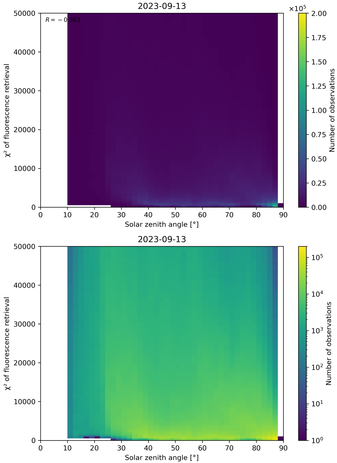
Figure 120: Scatter density plot of “Solar zenith angle” against “ \chi^2 of fluorescence retrieval” for 2023-09-12 to 2023-09-14.
