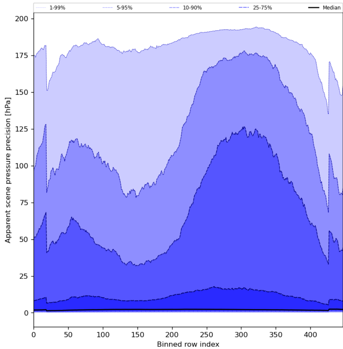
Figure 54: Along track statistics of “Apparent scene pressure precision” for 2023-09-12 to 2023-09-14
