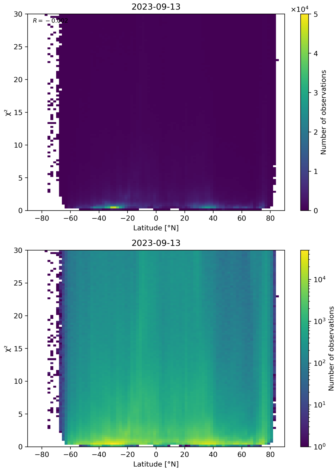
Figure 97: Scatter density plot of “Latitude” against “ \chi^2 ” for 2023-09-12 to 2023-09-14.
