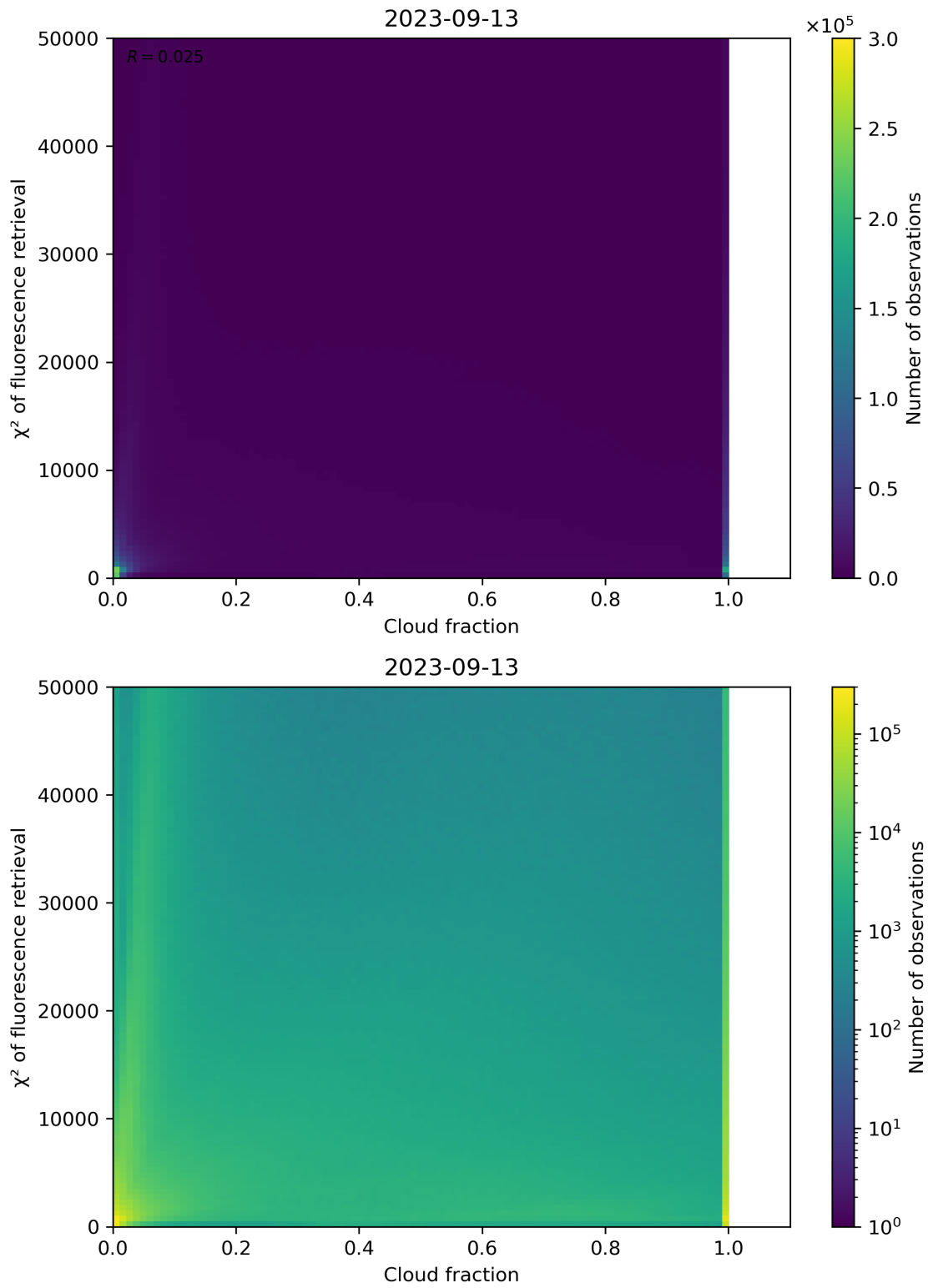
Figure 78: Scatter density plot of “Cloud fraction” against “ \chi^2 of fluorescence retrieval” for 2023-09-12 to 2023-09-14.
