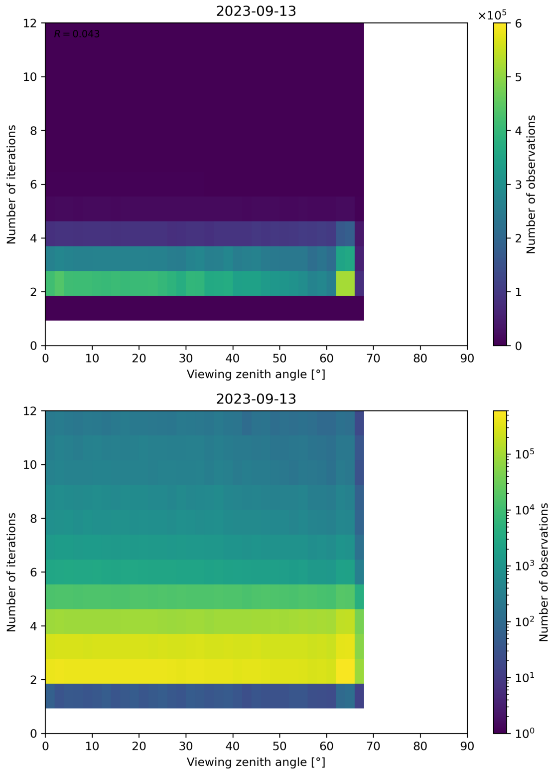
Figure 136: Scatter density plot of “Viewing zenith angle” against “Number of iterations” for 2023-09-12 to 2023-09-14.
