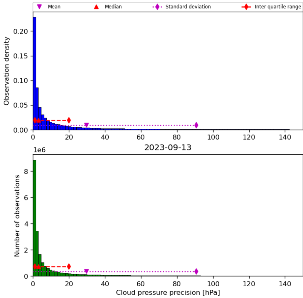
Figure 31: Histogram of “Cloud pressure precision” for 2023-09-12 to 2023-09-14
