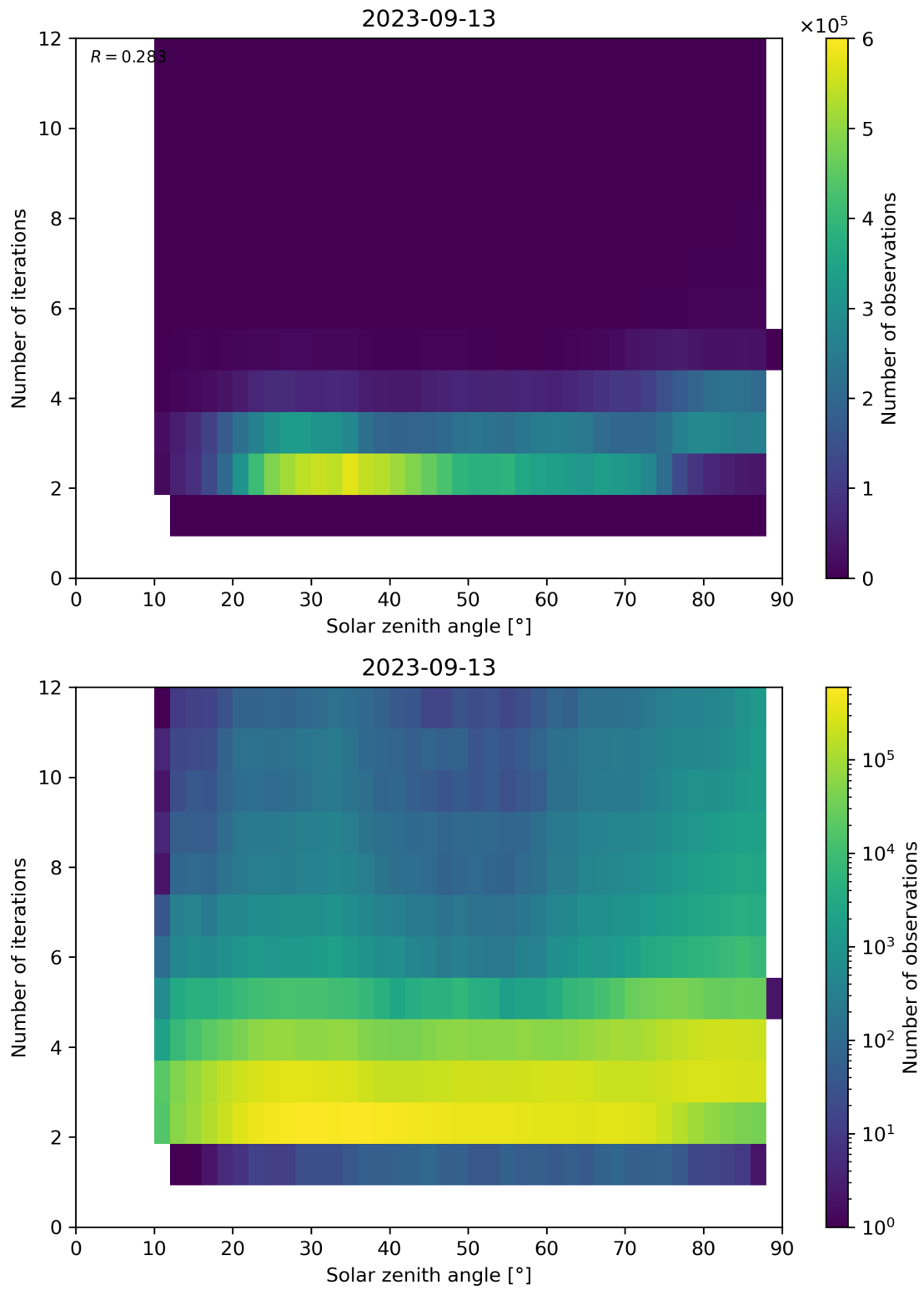
Figure 125: Scatter density plot of “Solar zenith angle” against “Number of iterations” for 2023-09-12 to 2023-09-14.
