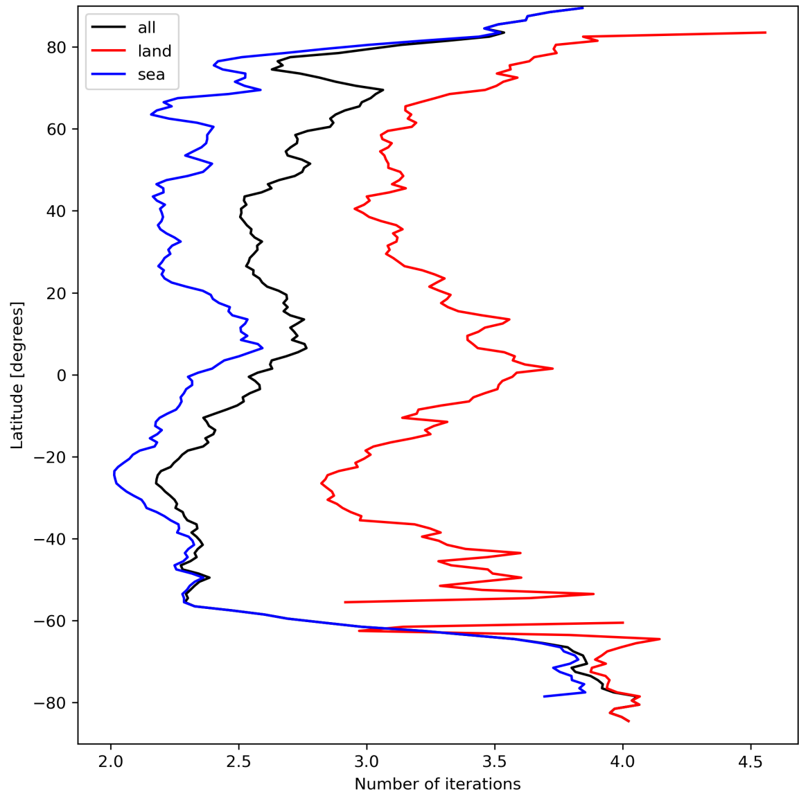
Figure 22: Zonal average of “Number of iterations” for 2023-09-12 to 2023-09-14.
