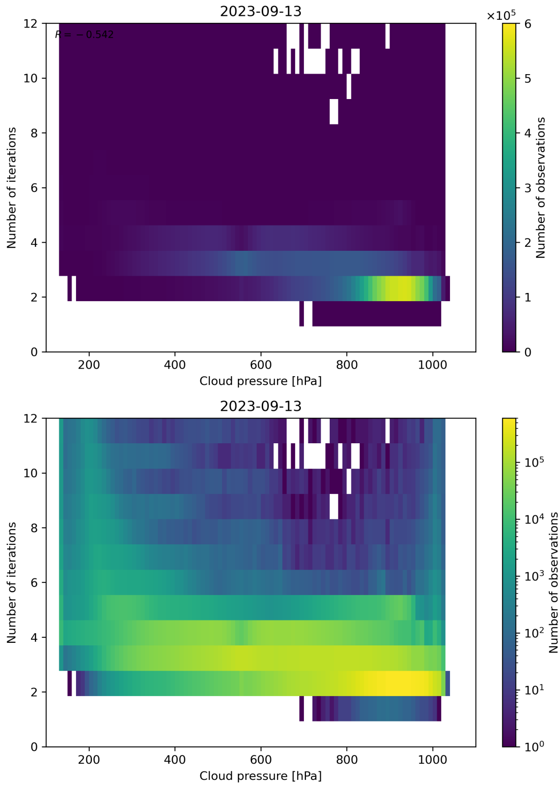
Figure 89: Scatter density plot of “Cloud pressure” against “Number of iterations” for 2023-09-12 to 2023-09-14.
