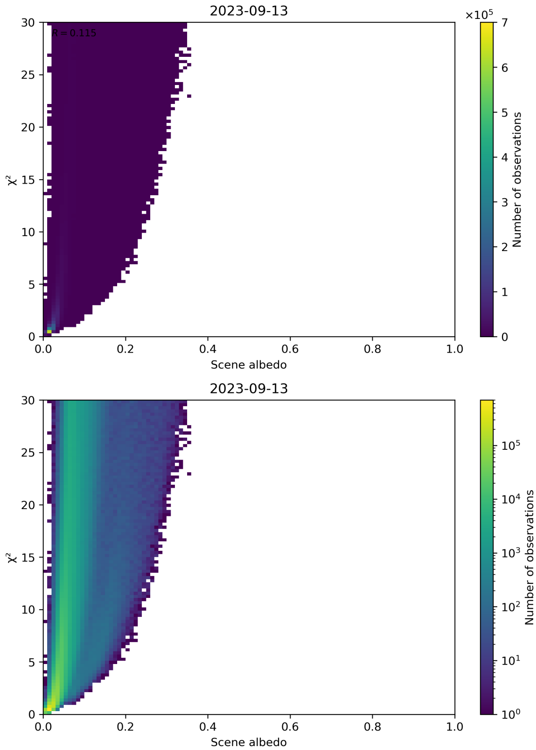
Figure 112: Scatter density plot of “Scene albedo” against “ \chi^2 ” for 2023-09-12 to 2023-09-14.
