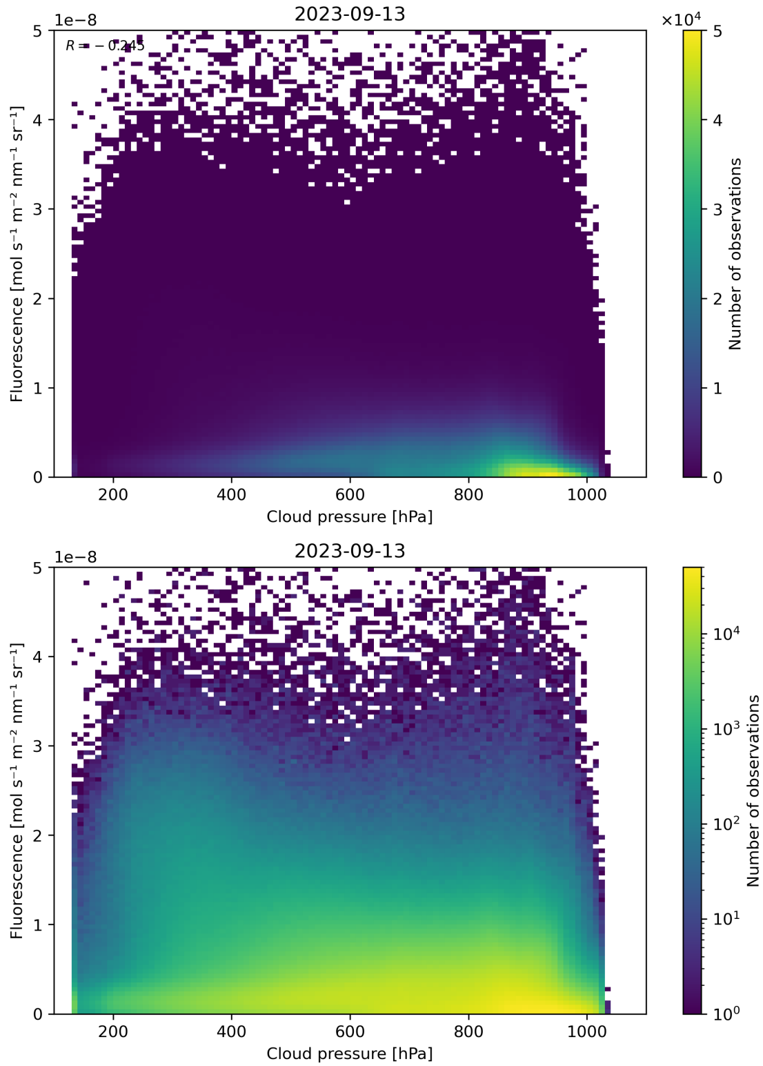
Figure 88: Scatter density plot of “Cloud pressure” against “Fluorescence” for 2023-09-12 to 2023-09-14.
