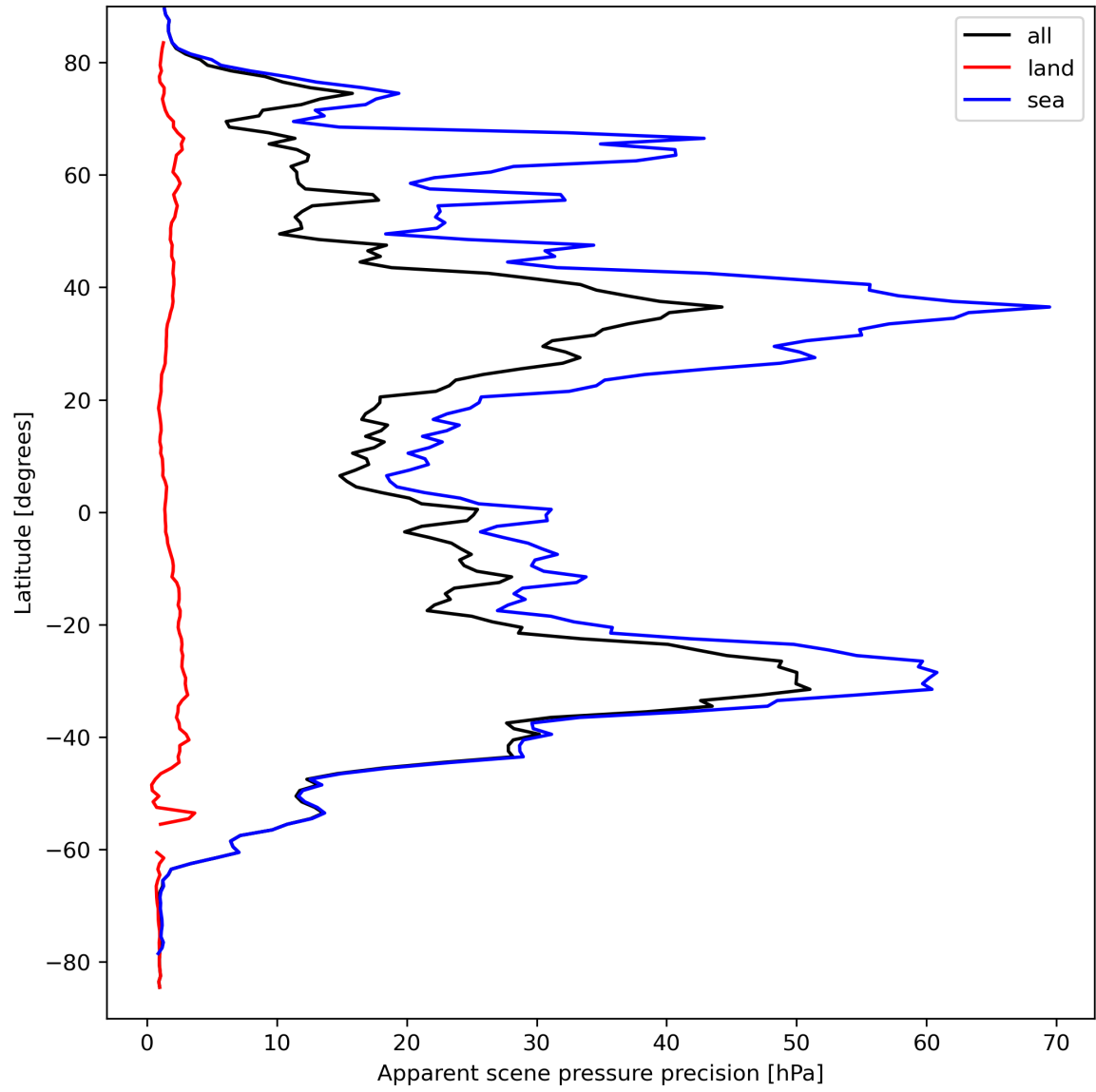
Figure 20: Zonal average of “Apparent scene pressure precision” for 2023-09-12 to 2023-09-14.
