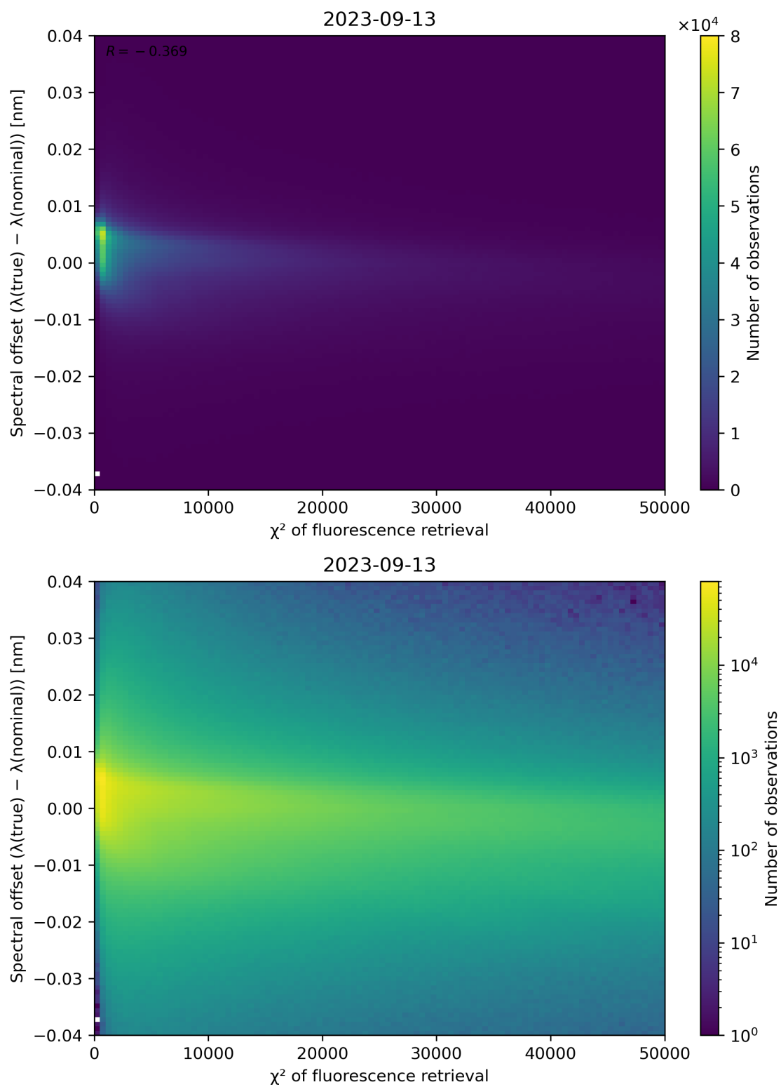
Figure 72: Scatter density plot of “ \chi^2 of fluorescence retrieval” against “Spectral offset ( \lambda(\text{true}) - \lambda(\text{nominal}) )” for 2023-09-12 to 2023-09-14.
