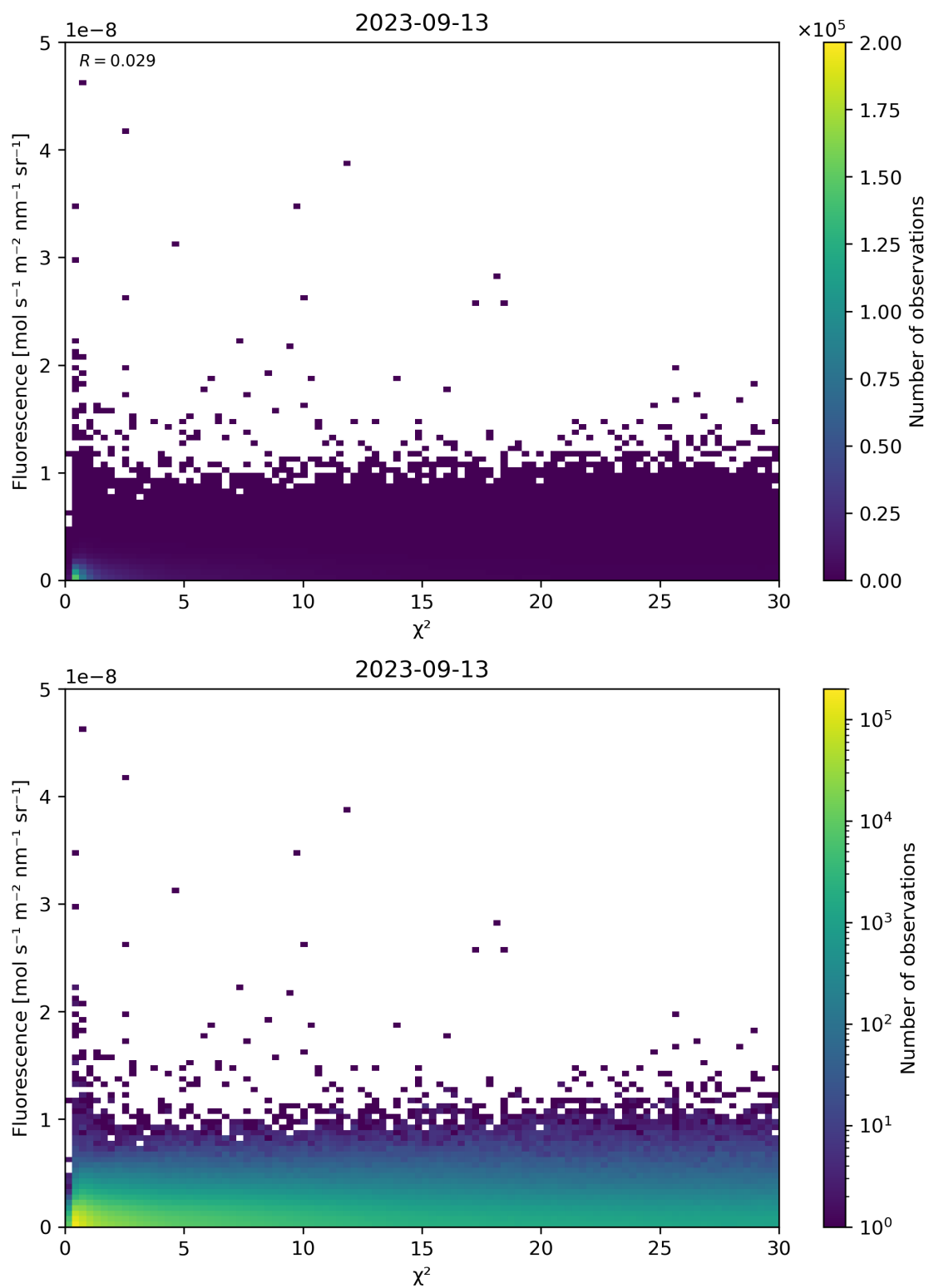
Figure 70: Scatter density plot of “ \chi^2 ” against “Fluorescence” for 2023-09-12 to 2023-09-14.
