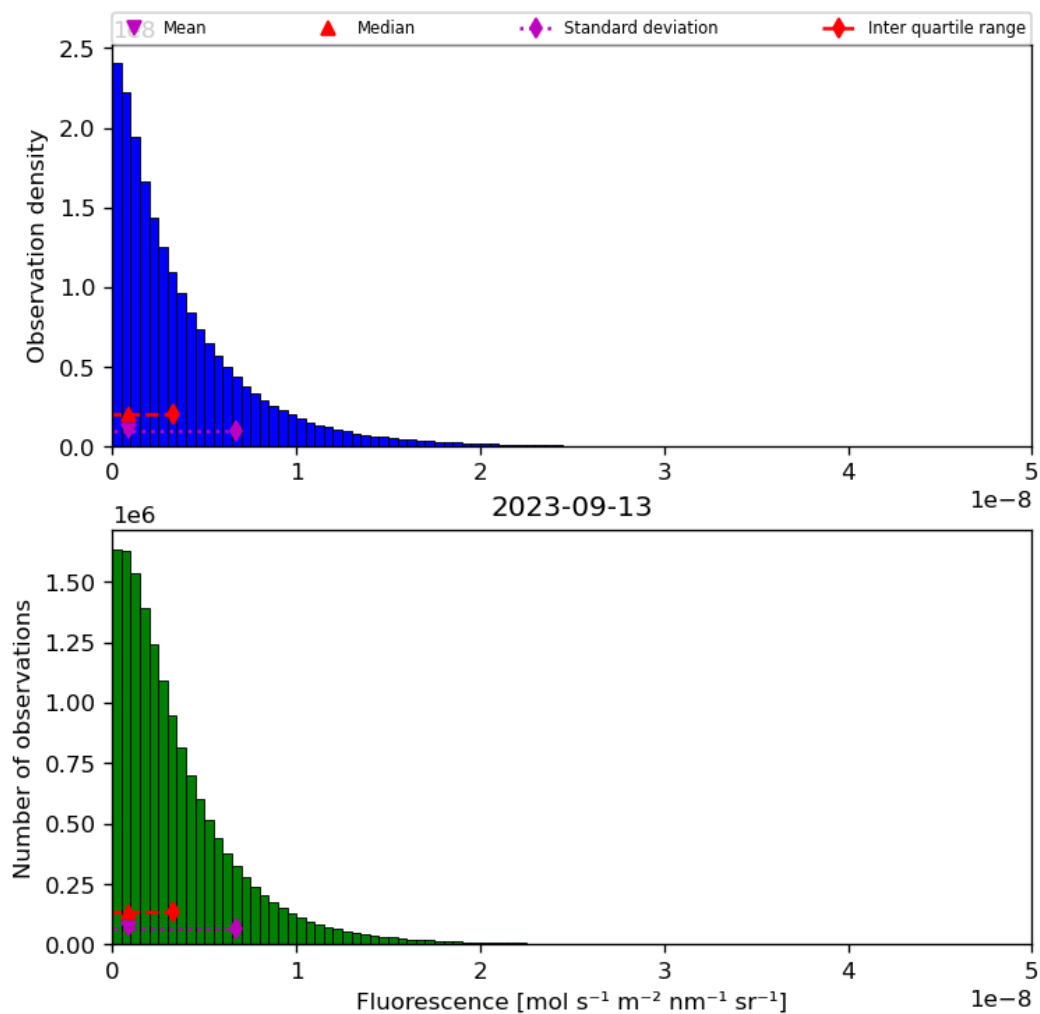
Figure 40: Histogram of “Fluorescence” for 2023-09-12 to 2023-09-14
