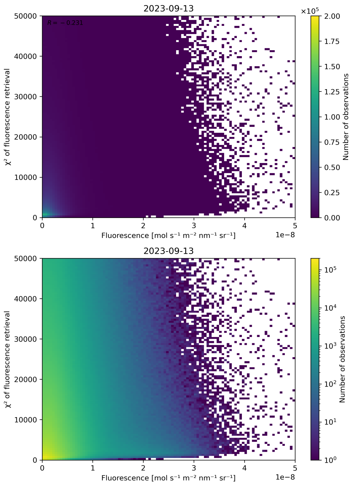
Figure 93: Scatter density plot of “Fluorescence” against “ \chi^2 of fluorescence retrieval” for 2023-09-12 to 2023-09-14.
