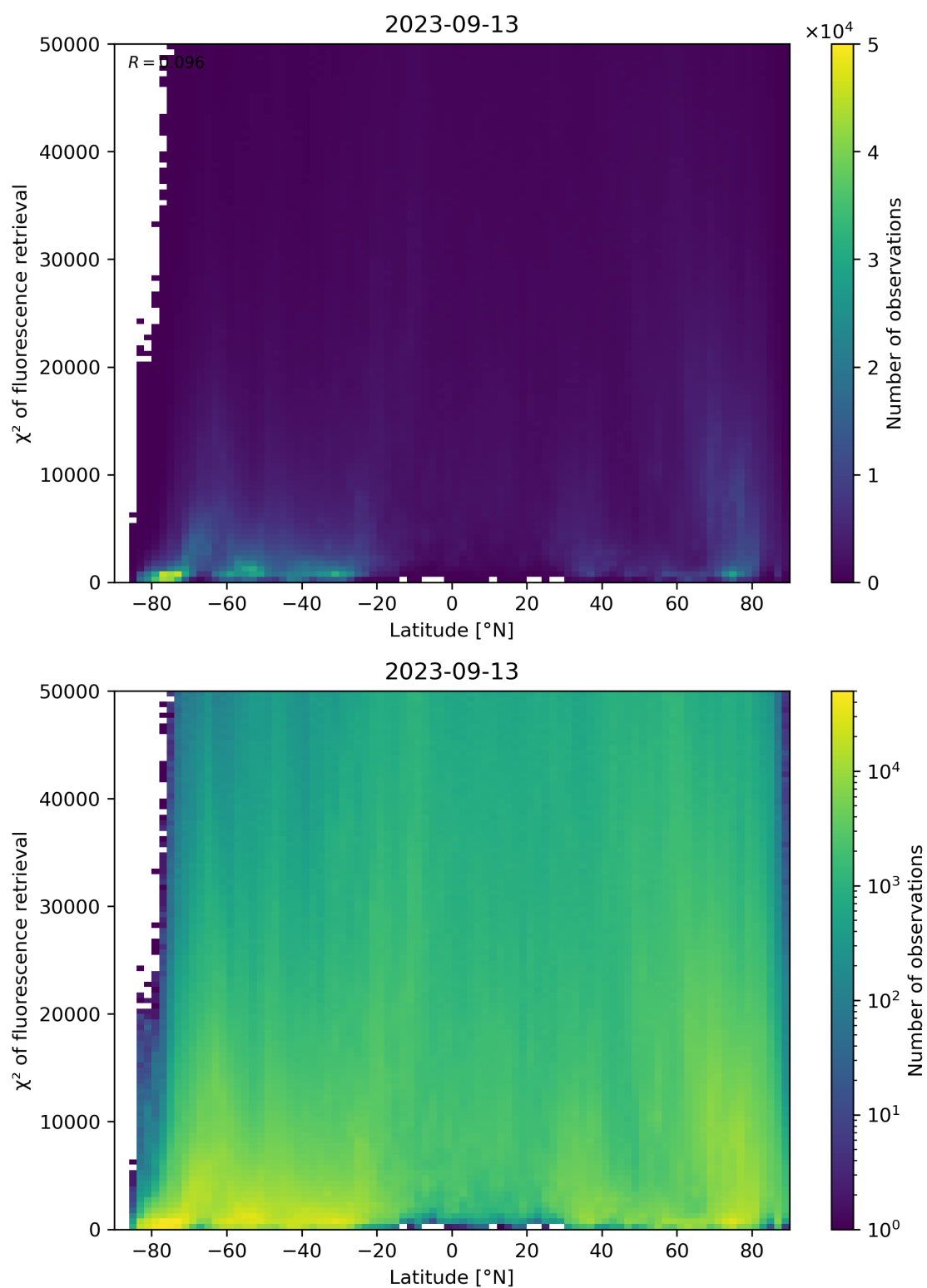
Figure 98: Scatter density plot of “Latitude” against “ \chi^2 of fluorescence retrieval” for 2023-09-12 to 2023-09-14.
