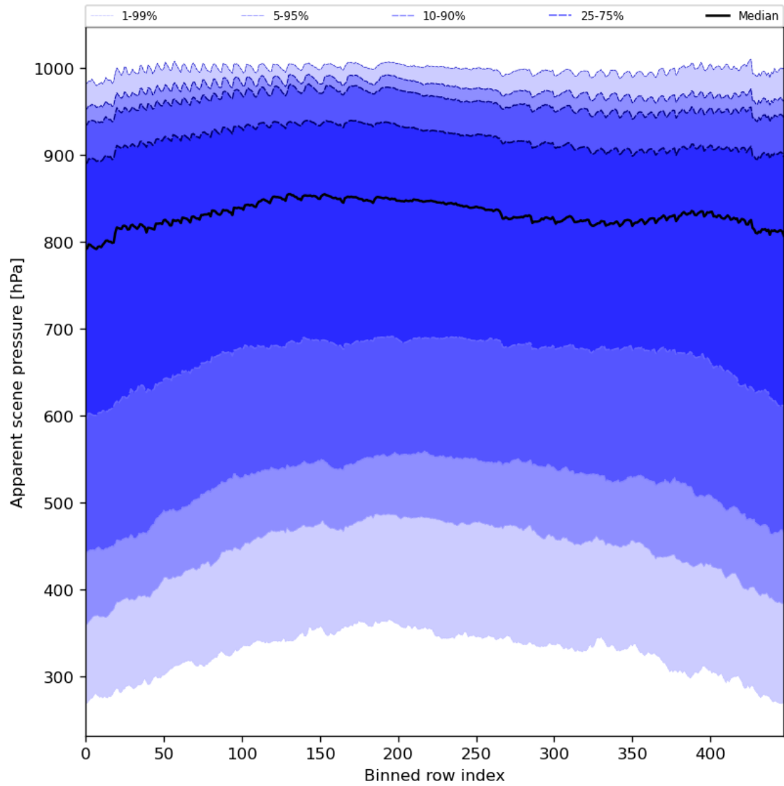
Figure 53: Along track statistics of “Apparent scene pressure” for 2023-09-12 to 2023-09-14
