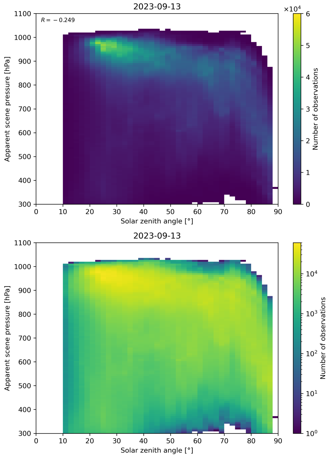
Figure 118: Scatter density plot of “Solar zenith angle” against “Apparent scene pressure” for 2023-09-12 to 2023-09-14.
