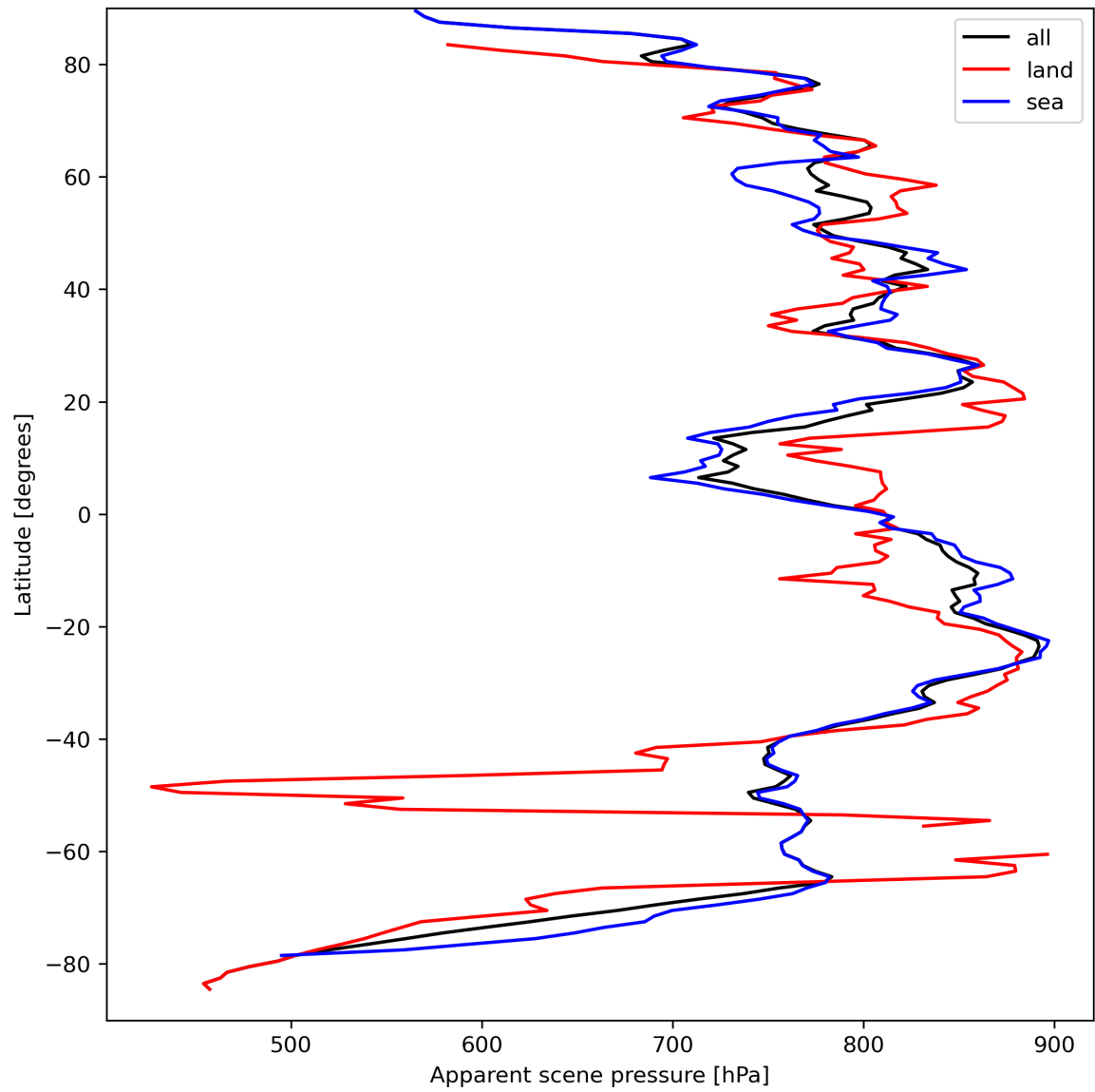
Figure 19: Zonal average of “Apparent scene pressure” for 2023-09-12 to 2023-09-14.
