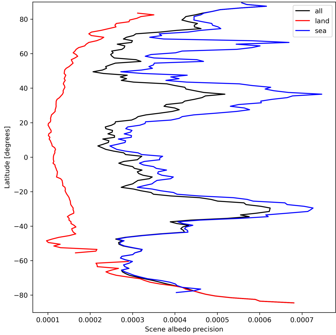
Figure 18: Zonal average of “Scene albedo precision” for 2023-09-12 to 2023-09-14.
