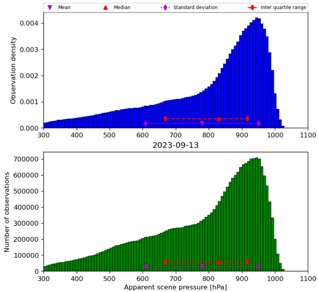
Figure 36: Histogram of “Apparent scene pressure” for 2023-09-12 to 2023-09-14
