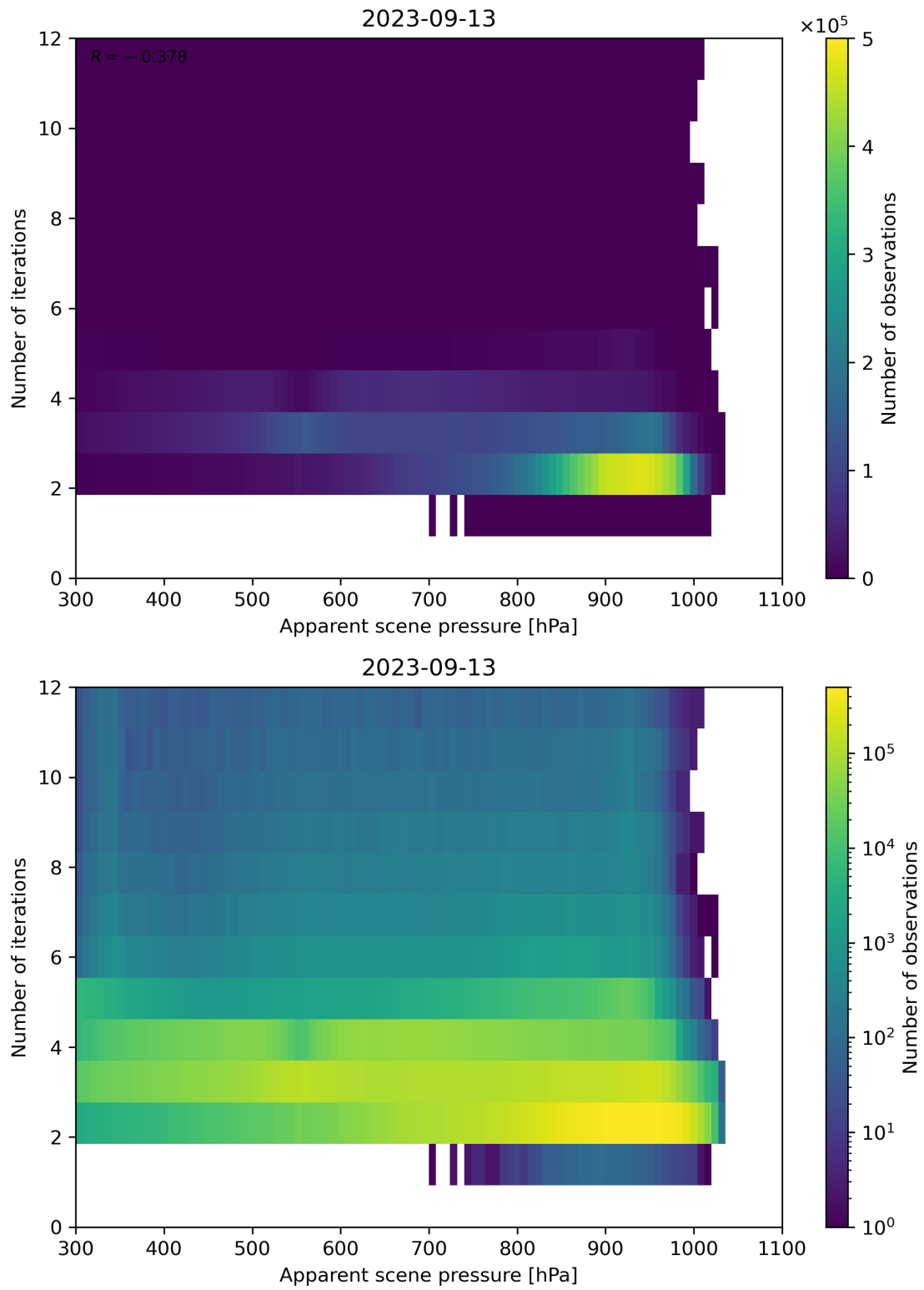
Figure 66: Scatter density plot of “Apparent scene pressure” against “Number of iterations” for 2023-09-12 to 2023-09-14.
