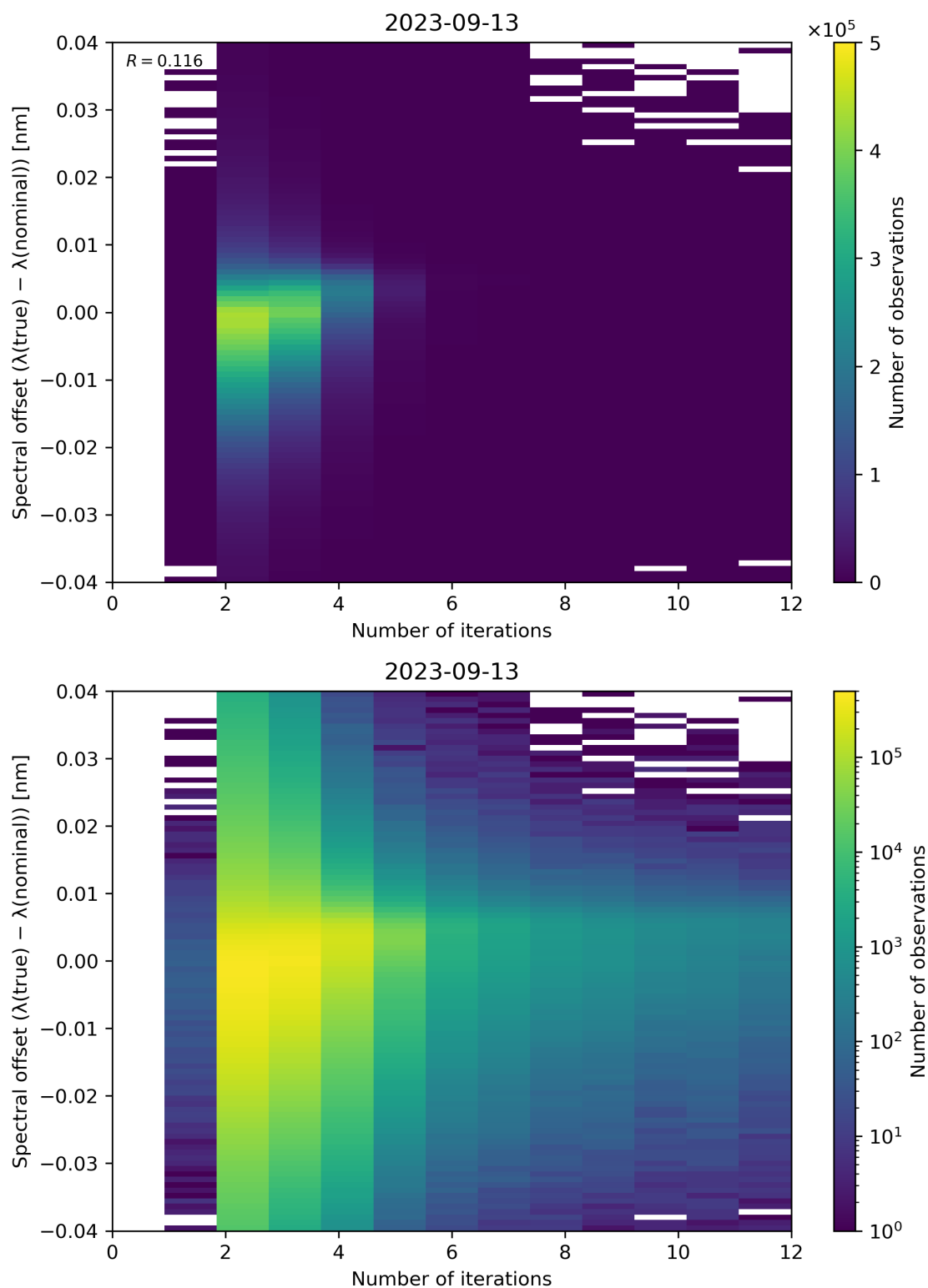
Figure 109: Scatter density plot of “Number of iterations” against “Spectral offset ( \lambda(\text{true}) - \lambda(\text{nominal}) )” for 2023-09-12 to 2023-09-14.
