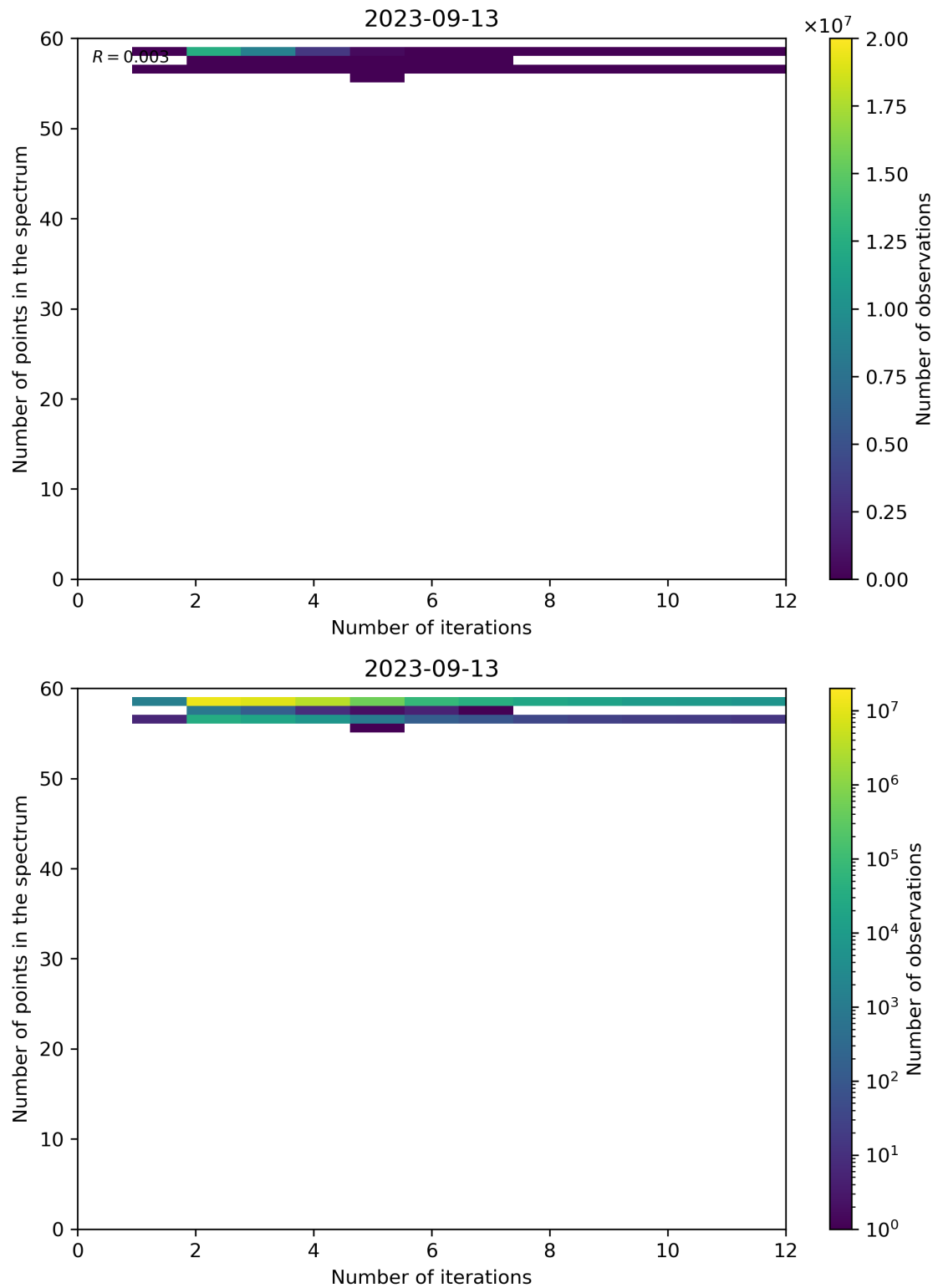
Figure 108: Scatter density plot of “Number of iterations” against “Number of points in the spectrum” for 2023-09-12 to 2023-09-14.
