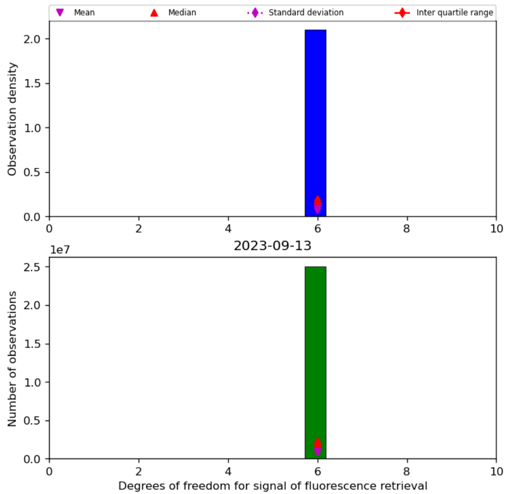
Figure 43: Histogram of “Degrees of freedom for signal of fluorescence retrieval” for 2023-09-12 to 2023-09-14
