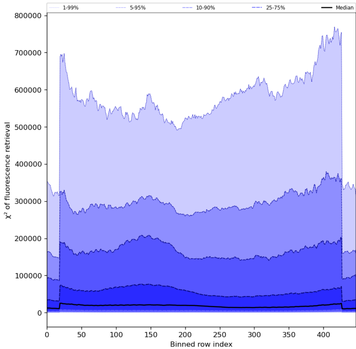
Figure 59: Along track statistics of “ \chi^2 of fluorescence retrieval” for 2023-09-12 to 2023-09-14
