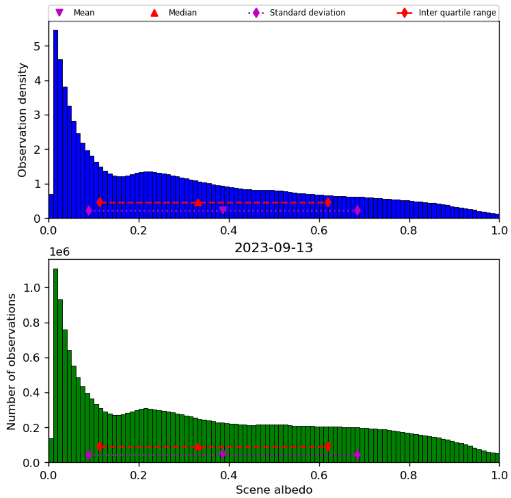
Figure 34: Histogram of “Scene albedo” for 2023-09-12 to 2023-09-14
