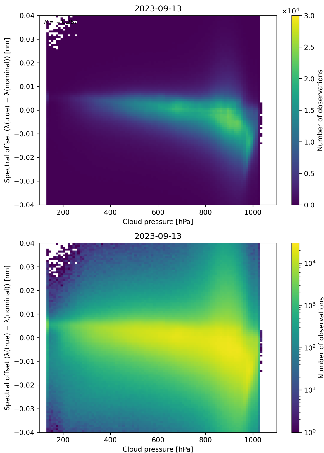
Figure 92: Scatter density plot of “Cloud pressure” against “Spectral offset ( \lambda(\text{true}) - \lambda(\text{nominal}) )” for 2023-09-12 to 2023-09-14.
