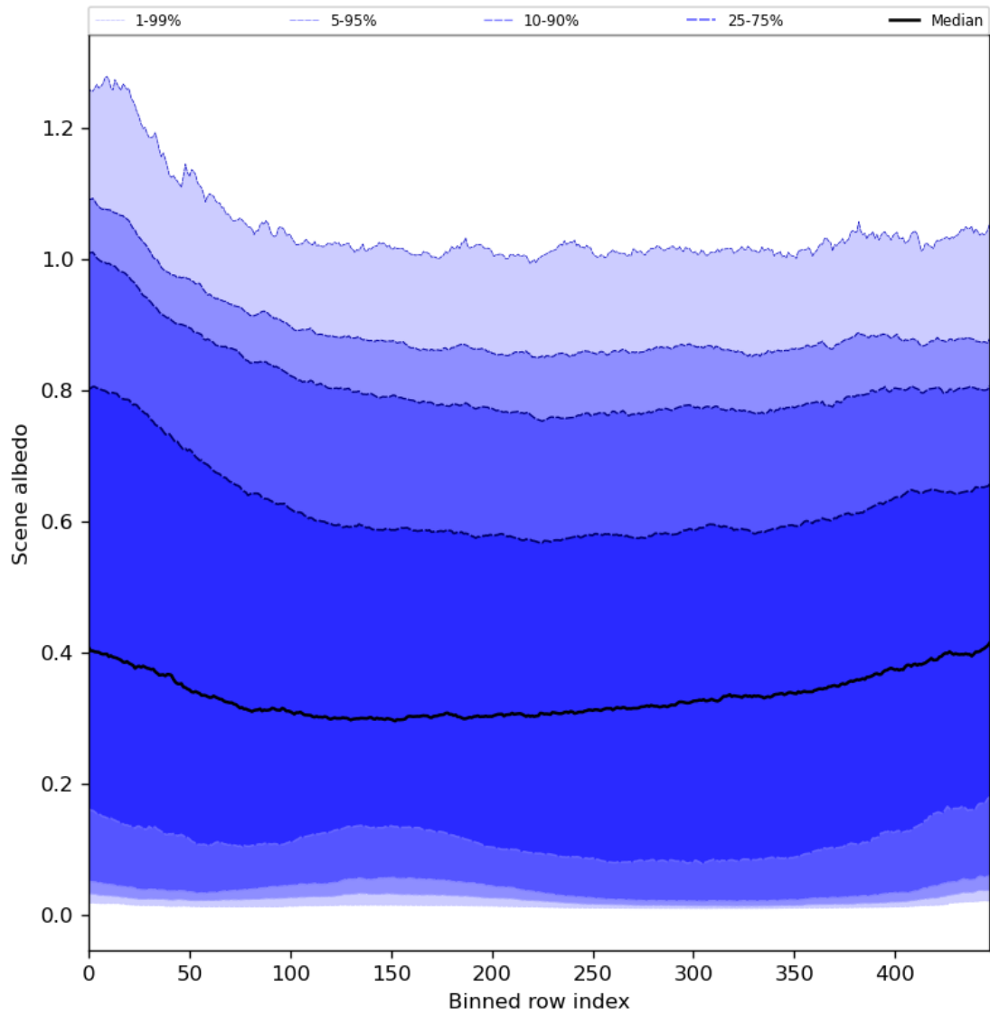
Figure 51: Along track statistics of “Scene albedo” for 2023-09-12 to 2023-09-14
