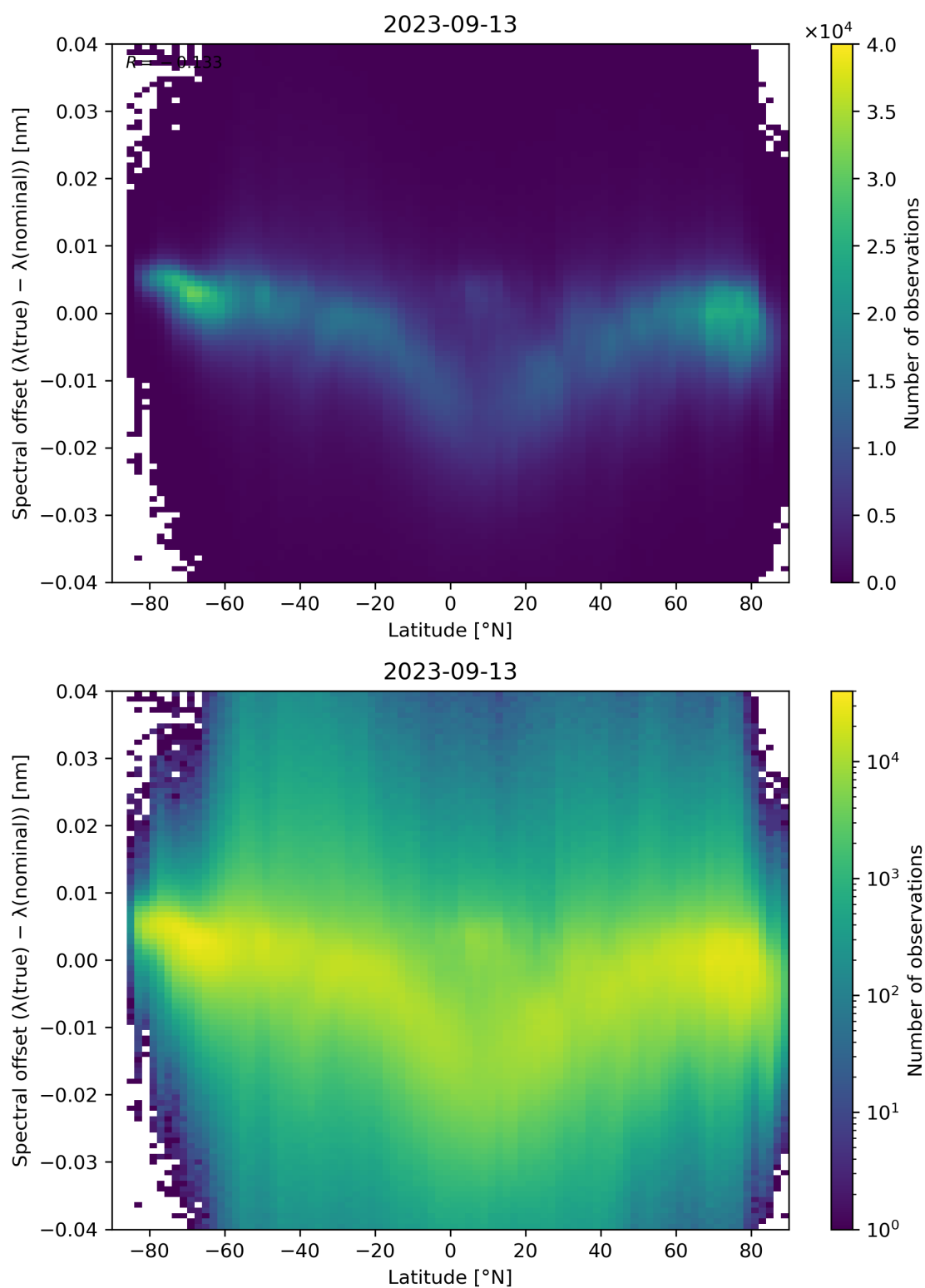
Figure 105: Scatter density plot of “Latitude” against “Spectral offset ( \lambda(\text{true}) - \lambda(\text{nominal}) )” for 2023-09-12 to 2023-09-14.
