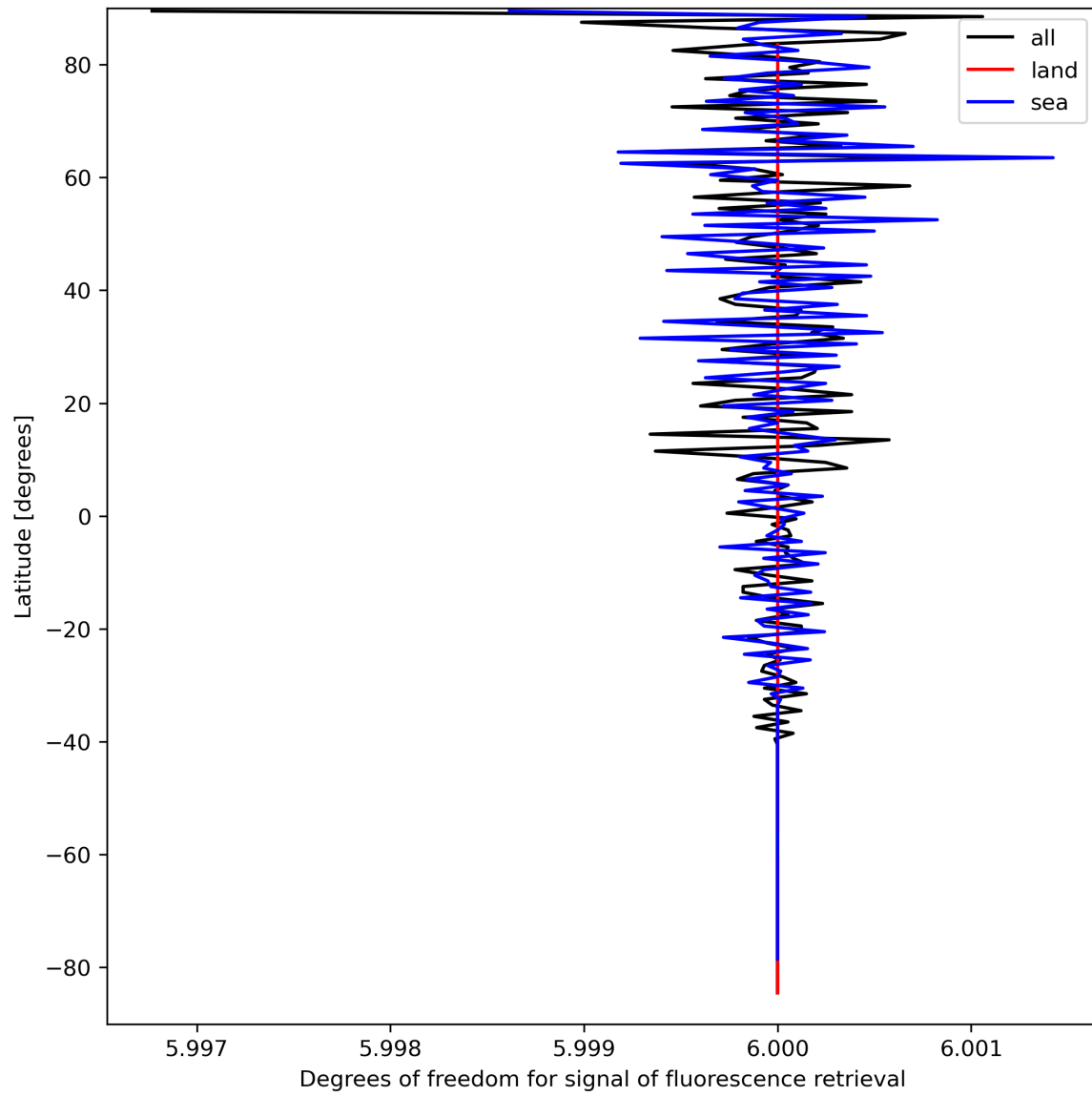
Figure 26: Zonal average of “Degrees of freedom for signal of fluorescence retrieval” for 2023-09-12 to 2023-09-14.
