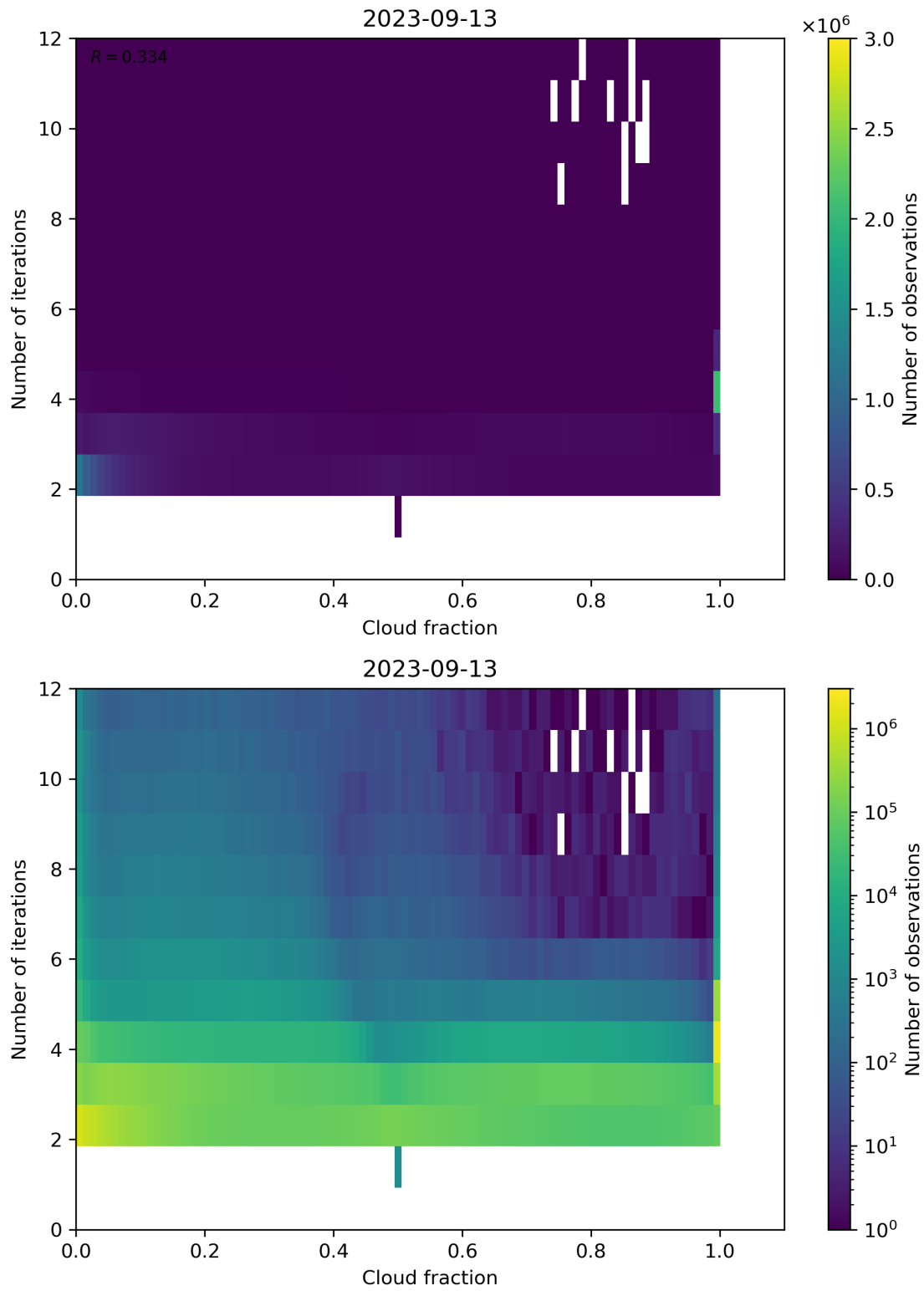
Figure 80: Scatter density plot of “Cloud fraction” against “Number of iterations” for 2023-09-12 to 2023-09-14.
