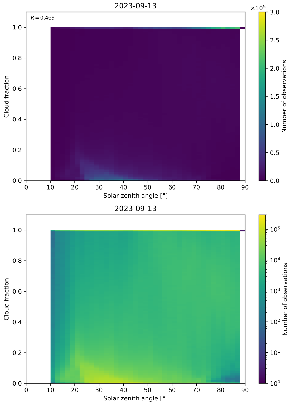
Figure 121: Scatter density plot of “Solar zenith angle” against “Cloud fraction” for 2023-09-12 to 2023-09-14.
