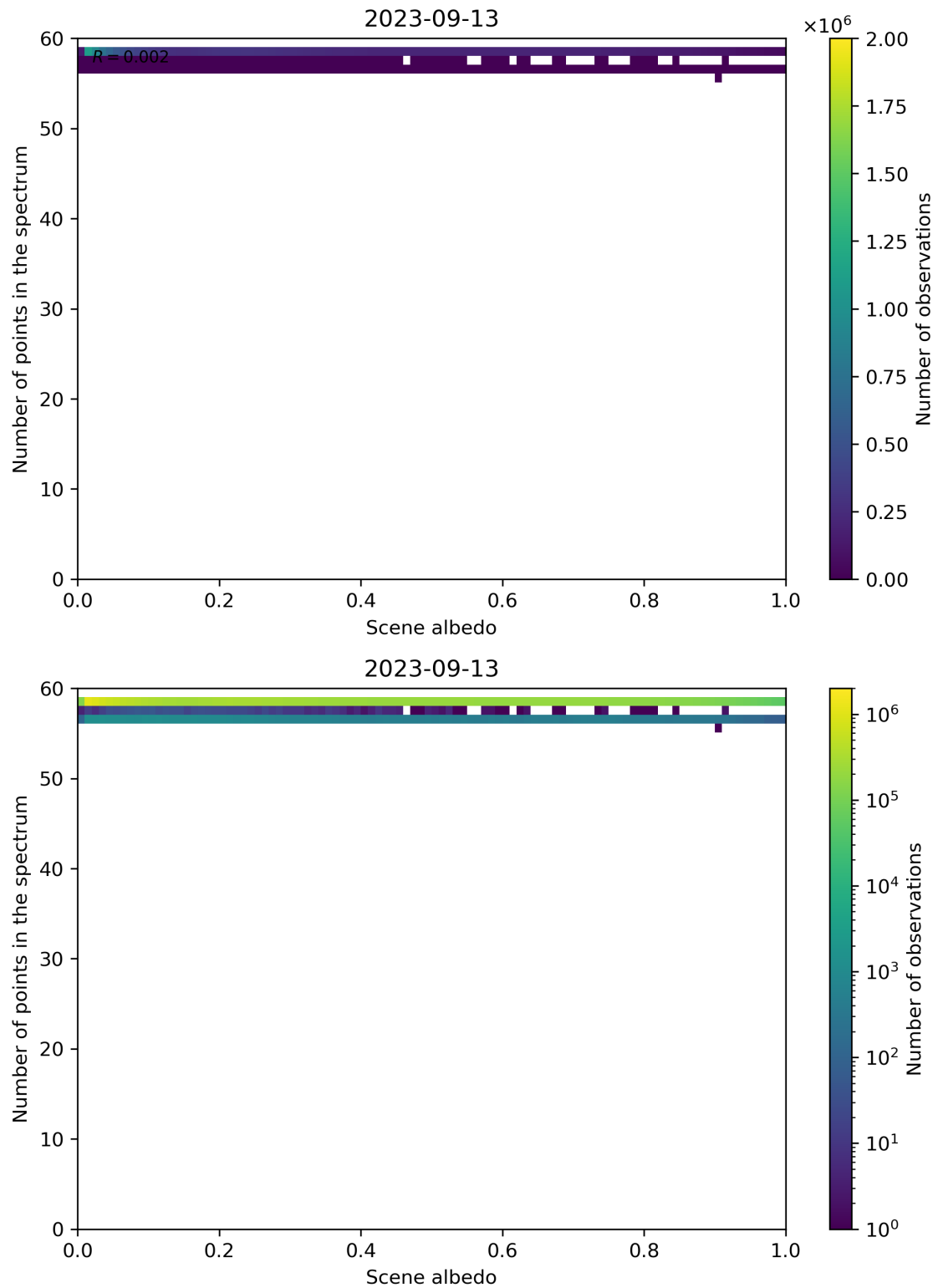
Figure 116: Scatter density plot of “Scene albedo” against “Number of points in the spectrum” for 2023-09-12 to 2023-09-14.
