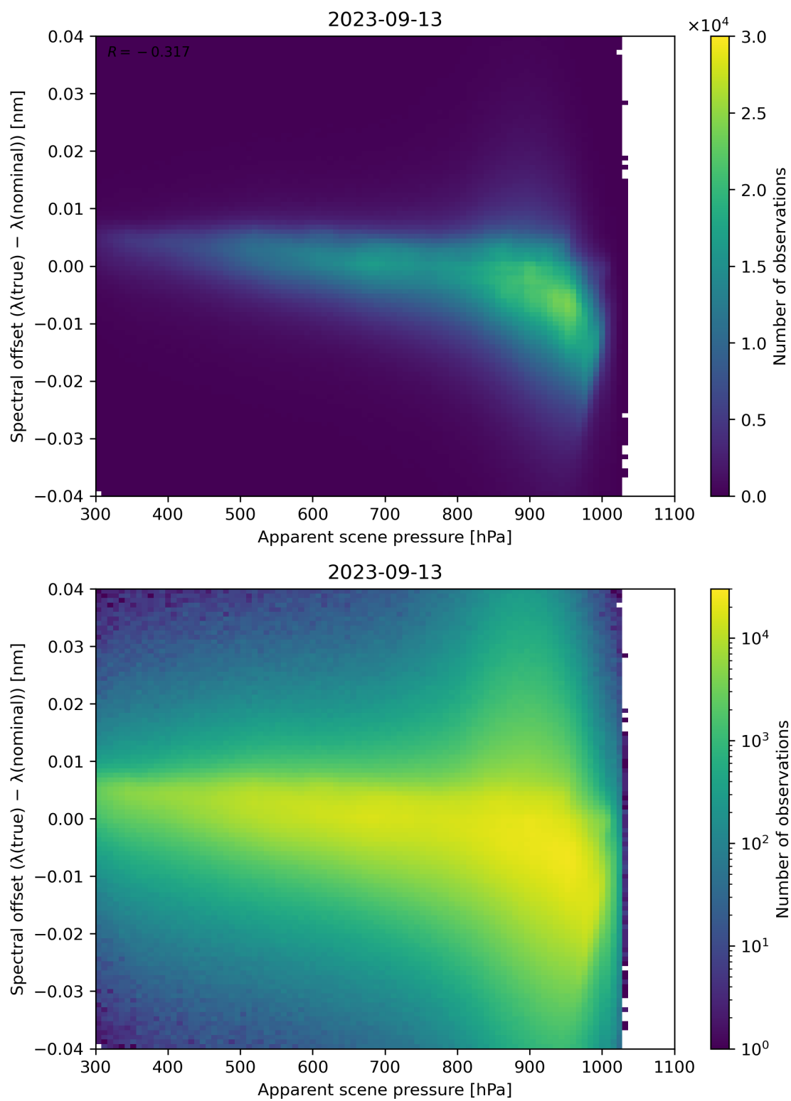
Figure 68: Scatter density plot of “Apparent scene pressure” against “Spectral offset ( \lambda(\text{true}) - \lambda(\text{nominal}) )” for 2023-09-12 to 2023-09-14.
