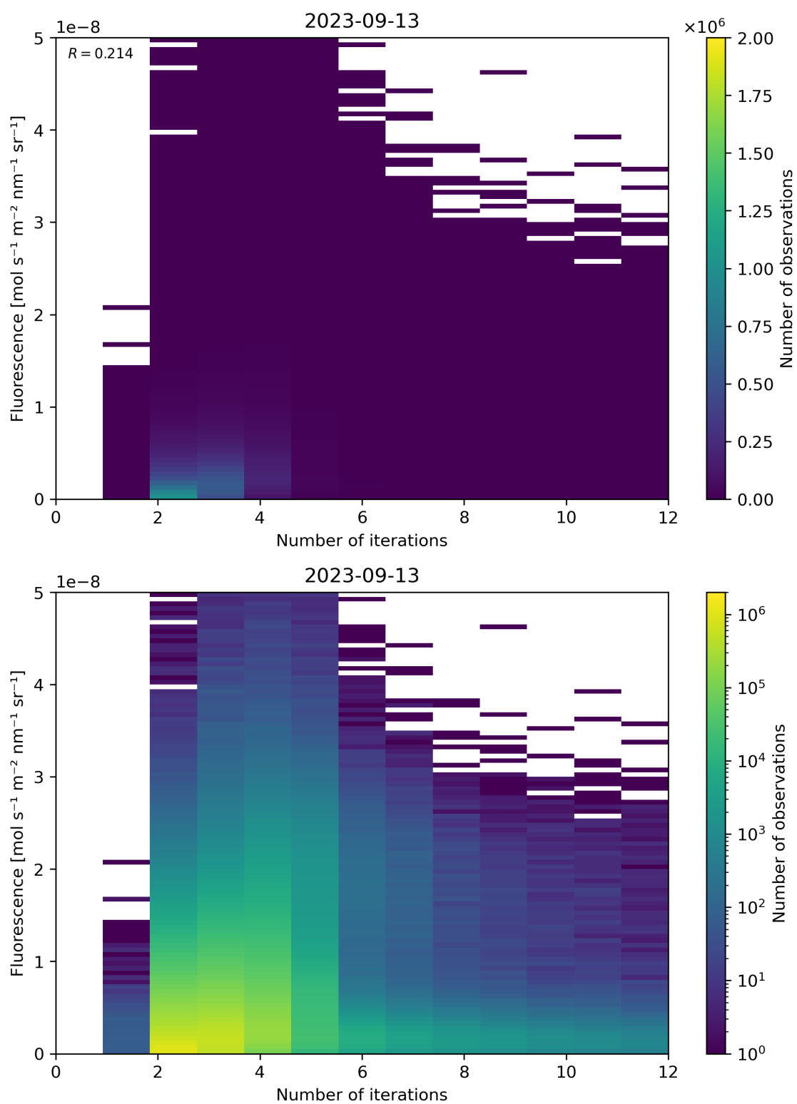
Figure 107: Scatter density plot of “Number of iterations” against “Fluorescence” for 2023-09-12 to 2023-09-14.
