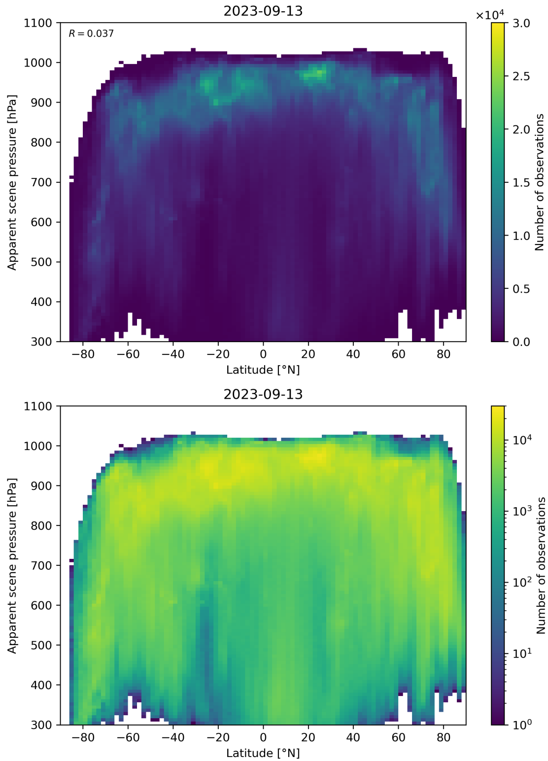
Figure 96: Scatter density plot of “Latitude” against “Apparent scene pressure” for 2023-09-12 to 2023-09-14.
