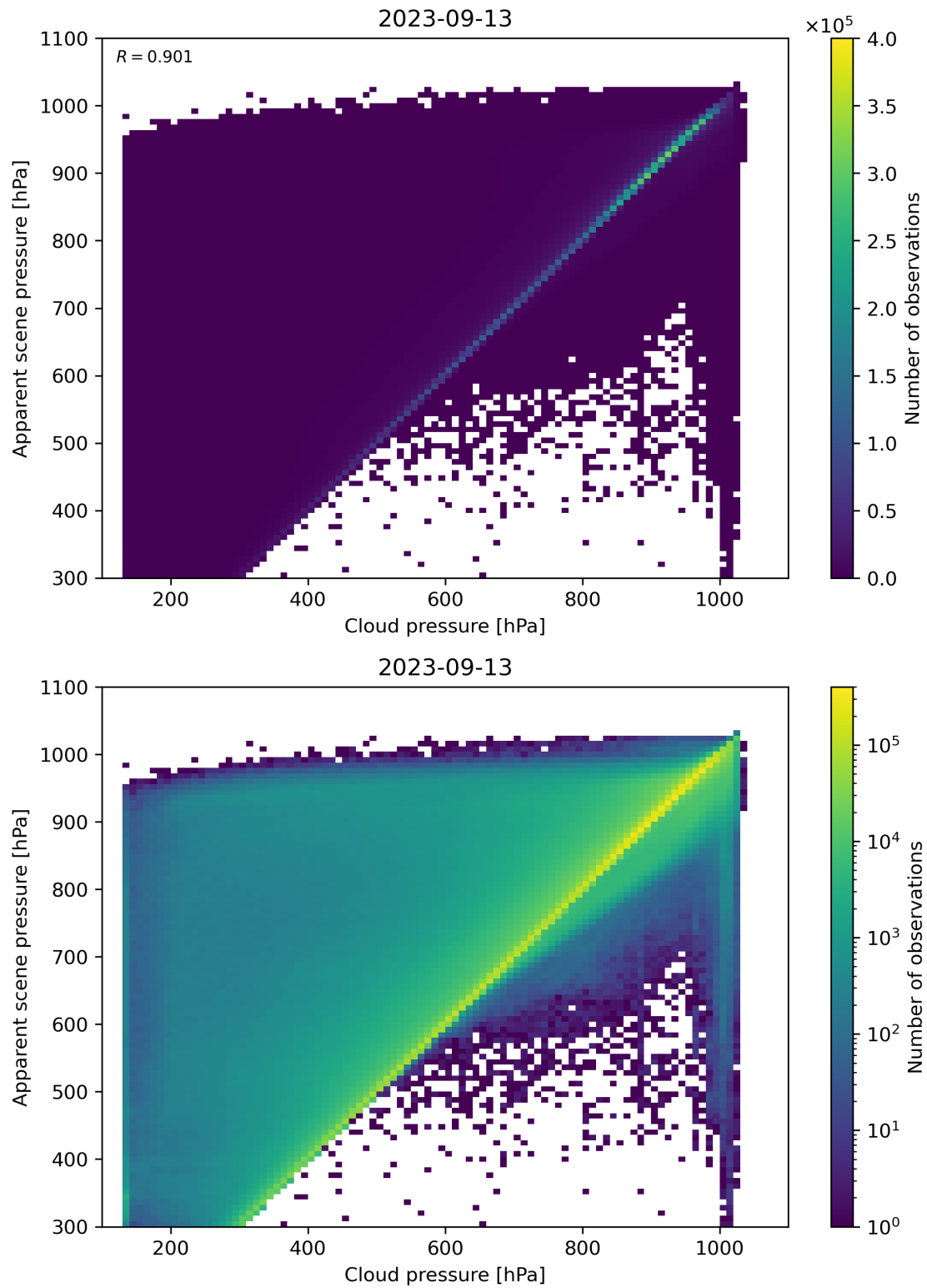
Figure 84: Scatter density plot of “Cloud pressure” against “Apparent scene pressure” for 2023-09-12 to 2023-09-14.
