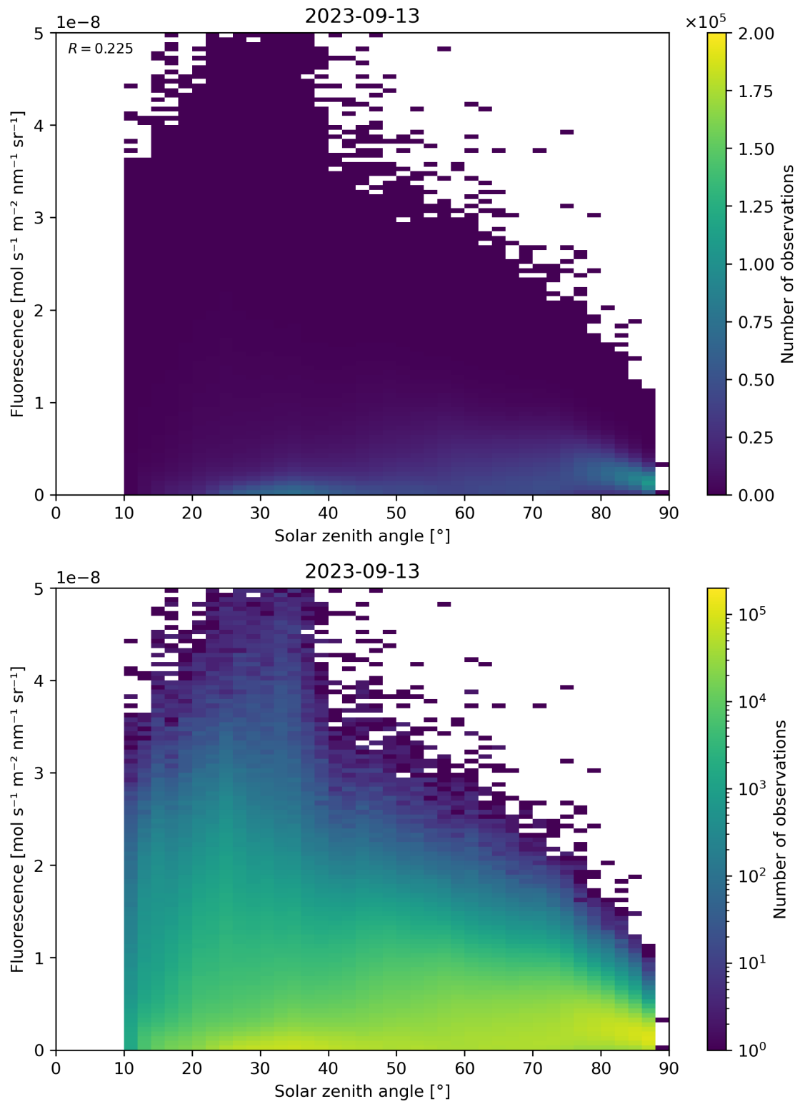
Figure 123: Scatter density plot of “Solar zenith angle” against “Fluorescence” for 2023-09-12 to 2023-09-14.
