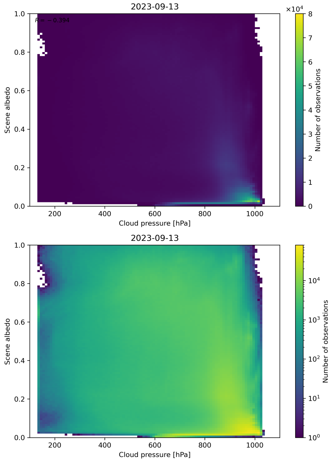
Figure 91: Scatter density plot of “Cloud pressure” against “Scene albedo” for 2023-09-12 to 2023-09-14.
