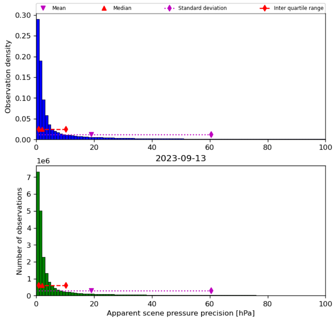
Figure 37: Histogram of “Apparent scene pressure precision” for 2023-09-12 to 2023-09-14
