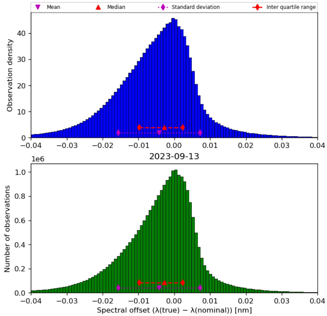
Figure 45: Histogram of “Spectral offset ( \lambda(\text{true}) - \lambda(\text{nominal}) )” for 2023-09-12 to 2023-09-14
