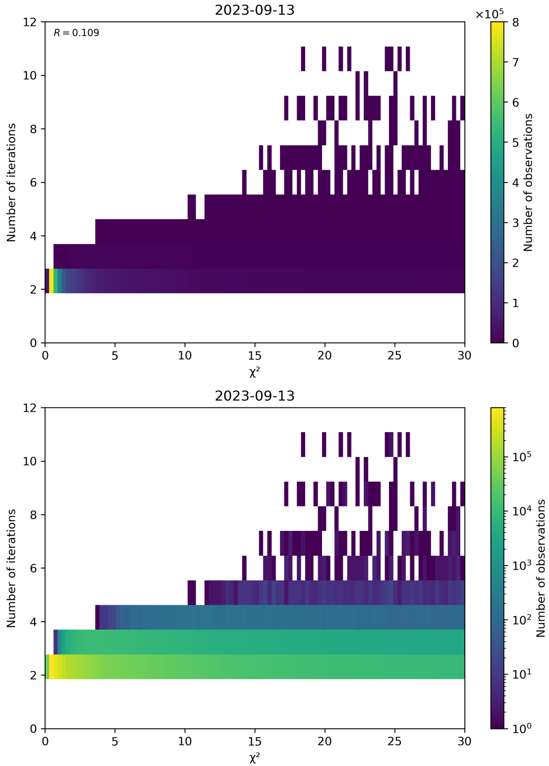
Figure 73: Scatter density plot of “ \chi^2 ” against “Number of iterations” for 2023-09-12 to 2023-09-14.
