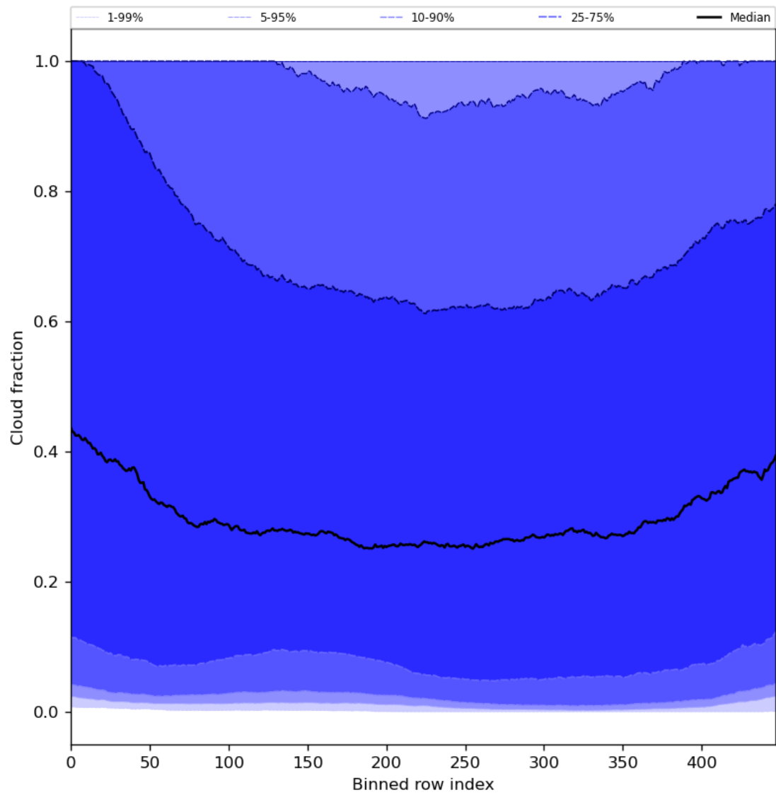
Figure 49: Along track statistics of “Cloud fraction” for 2023-09-12 to 2023-09-14
