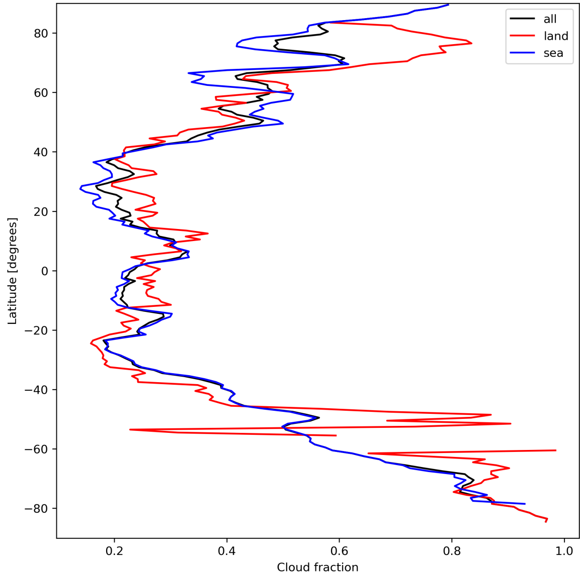
Figure 15: Zonal average of “Cloud fraction” for 2023-09-12 to 2023-09-14.
