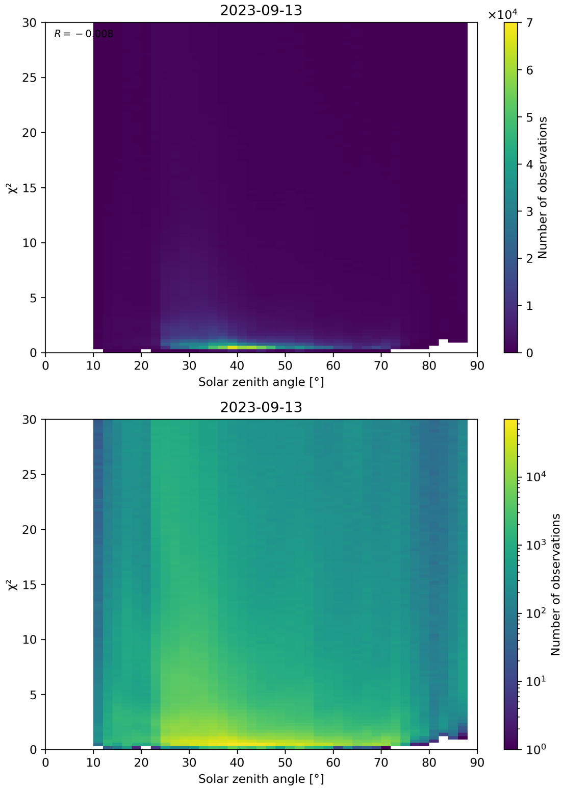
Figure 119: Scatter density plot of “Solar zenith angle” against “ \chi^2 ” for 2023-09-12 to 2023-09-14.
