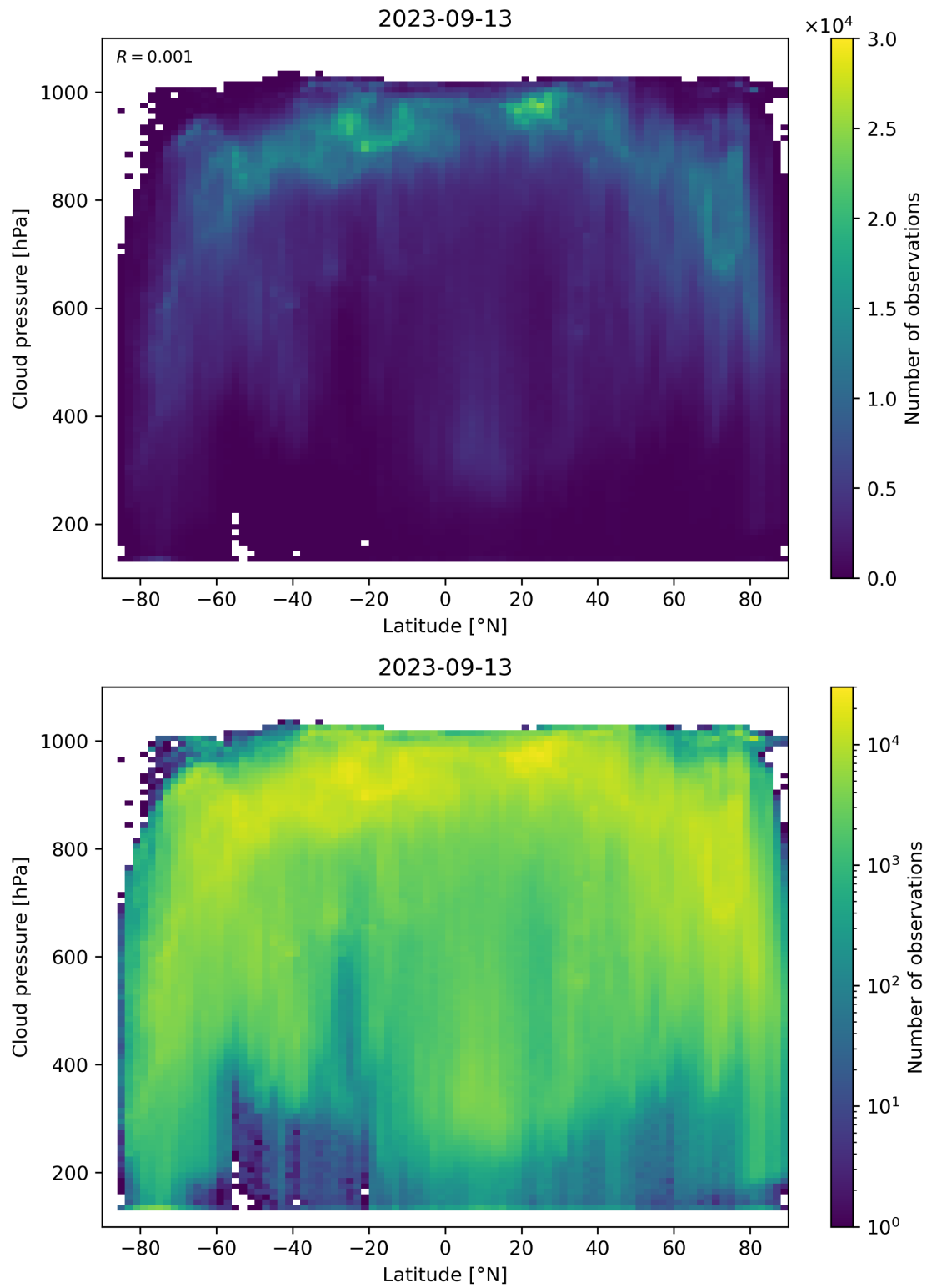
Figure 100: Scatter density plot of “Latitude” against “Cloud pressure” for 2023-09-12 to 2023-09-14.
