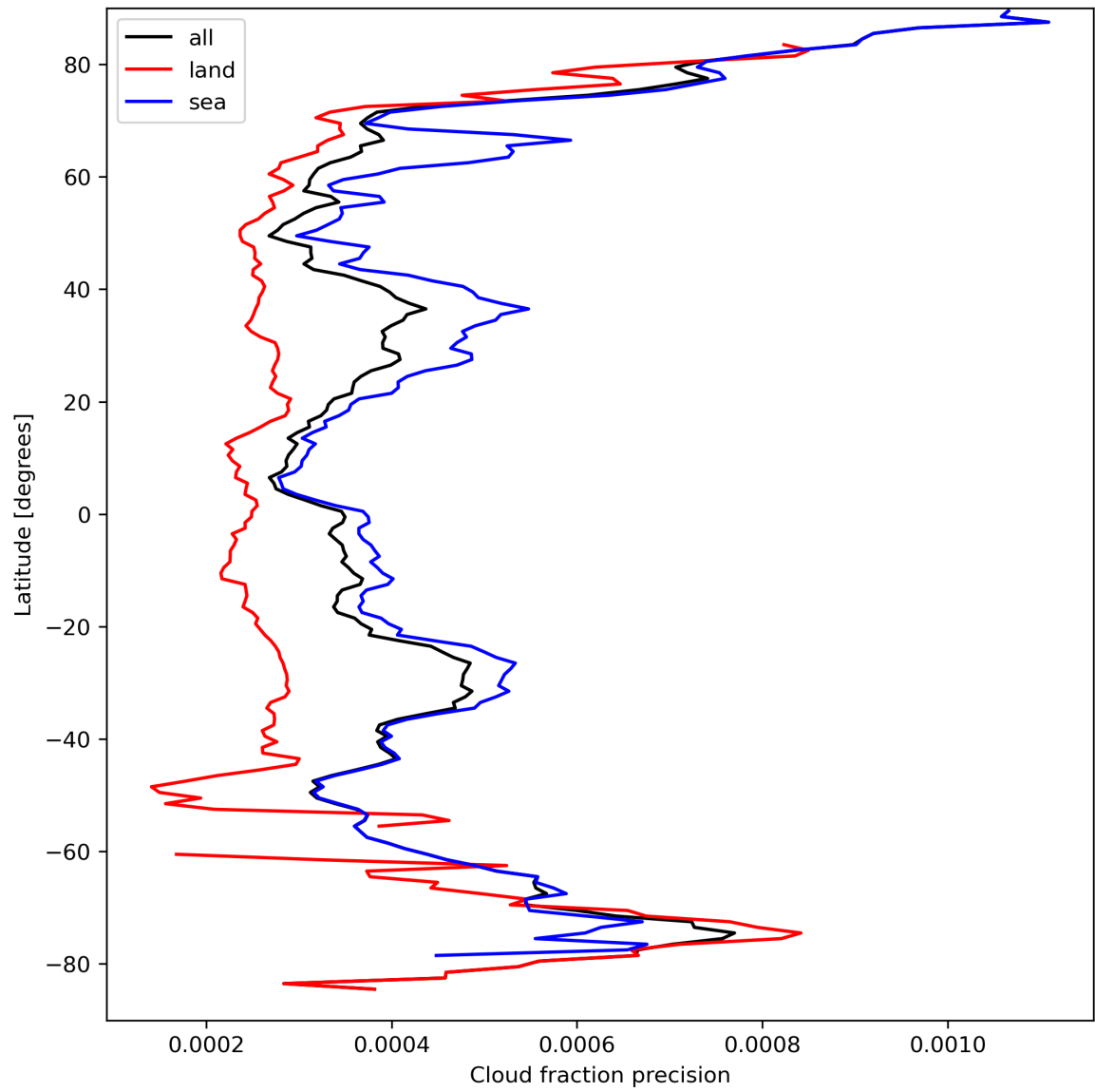
Figure 16: Zonal average of “Cloud fraction precision” for 2023-09-12 to 2023-09-14.
