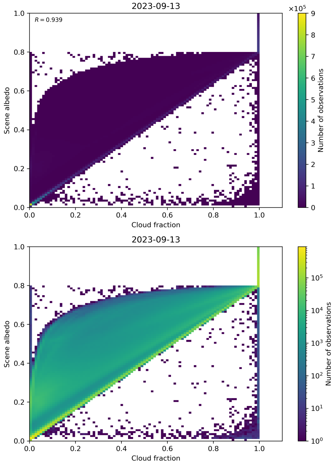
Figure 82: Scatter density plot of “Cloud fraction” against “Scene albedo” for 2023-09-12 to 2023-09-14.
