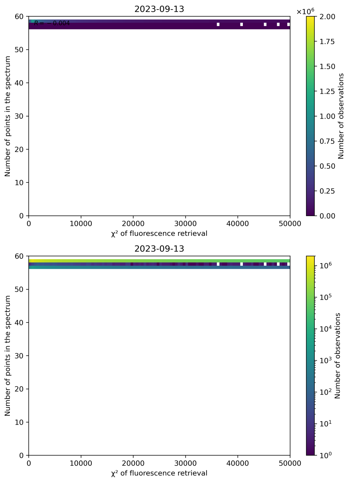
Figure 71: Scatter density plot of " \chi^2 of fluorescence retrieval" against "Number of points in the spectrum" for 2023-09-12 to 2023-09-14.
