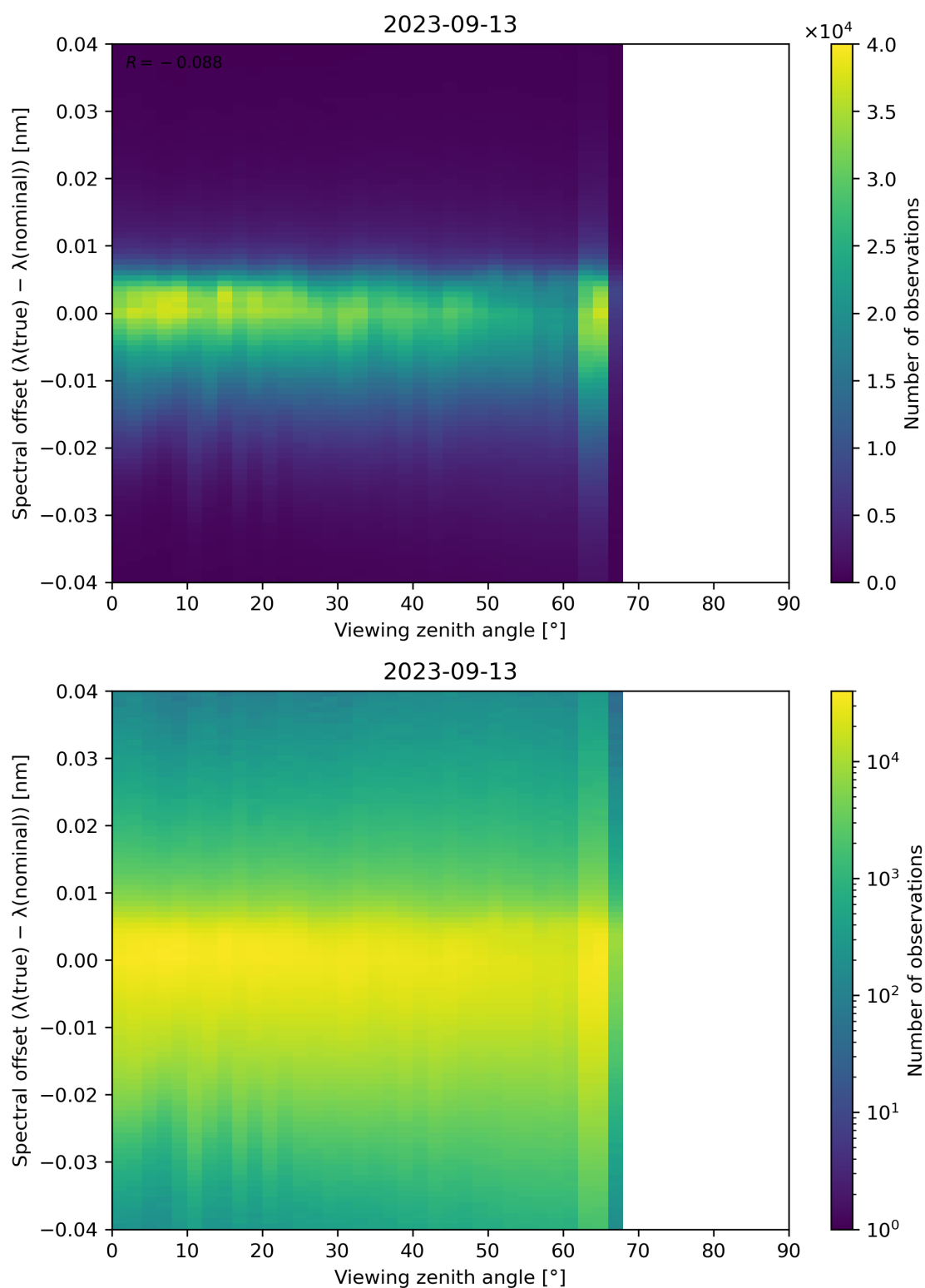
Figure 140: Scatter density plot of “Viewing zenith angle” against “Spectral offset ( \lambda(\text{true}) - \lambda(\text{nominal}) )” for 2023-09-12 to 2023-09-14.
