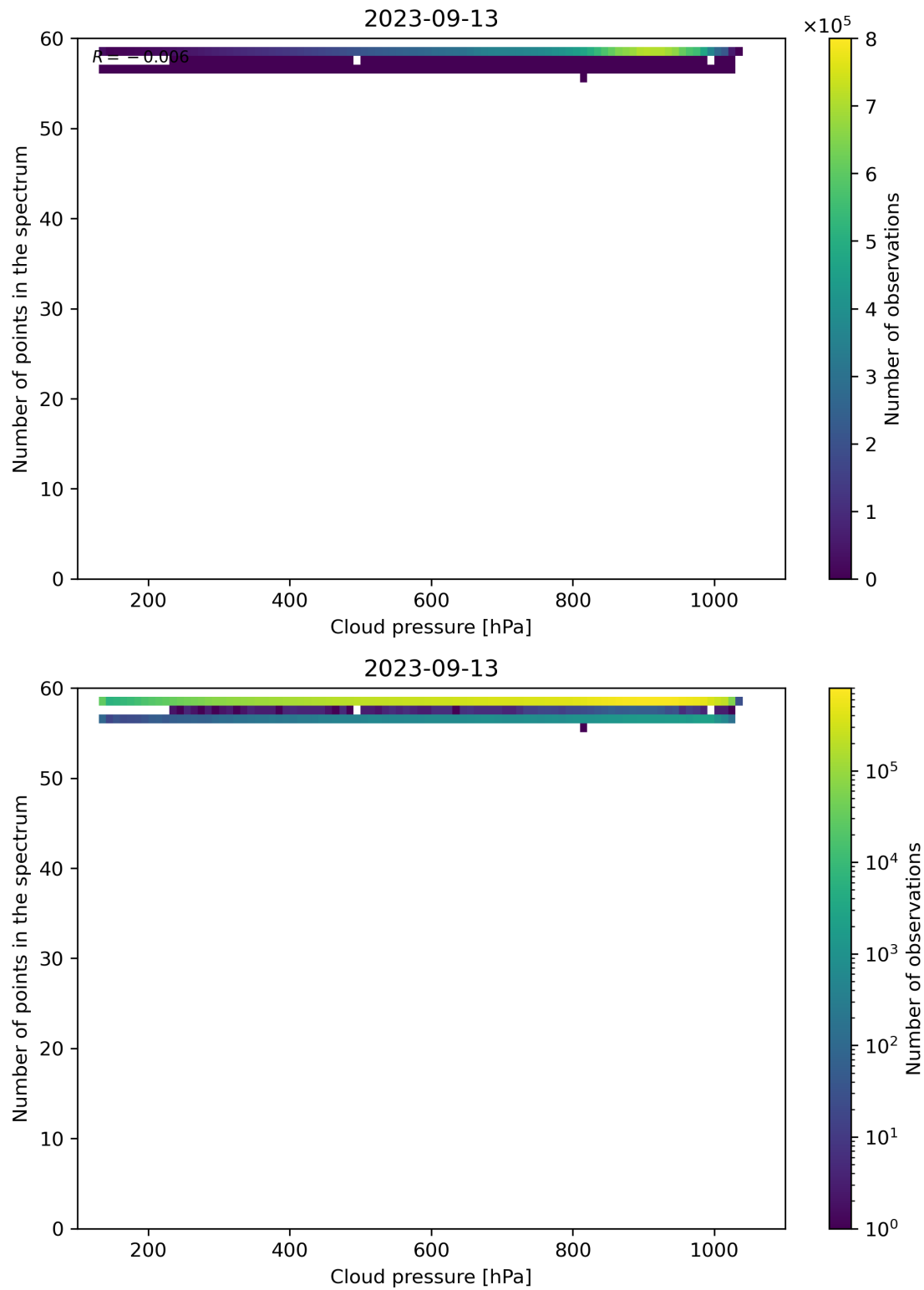
Figure 90: Scatter density plot of “Cloud pressure” against “Number of points in the spectrum” for 2023-09-12 to 2023-09-14.
