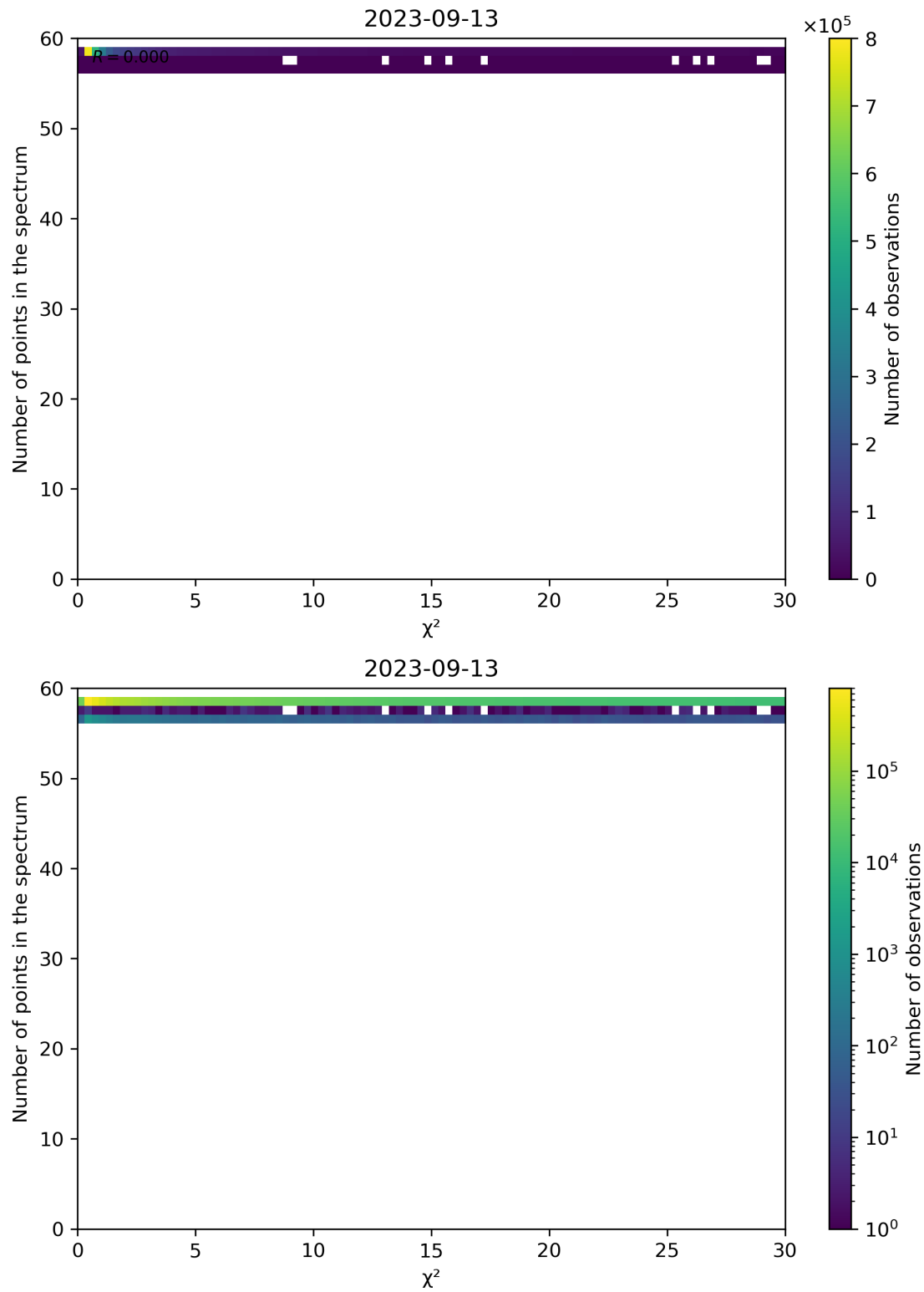
Figure 74: Scatter density plot of “ \chi^2 ” against “Number of points in the spectrum” for 2023-09-12 to 2023-09-14.
