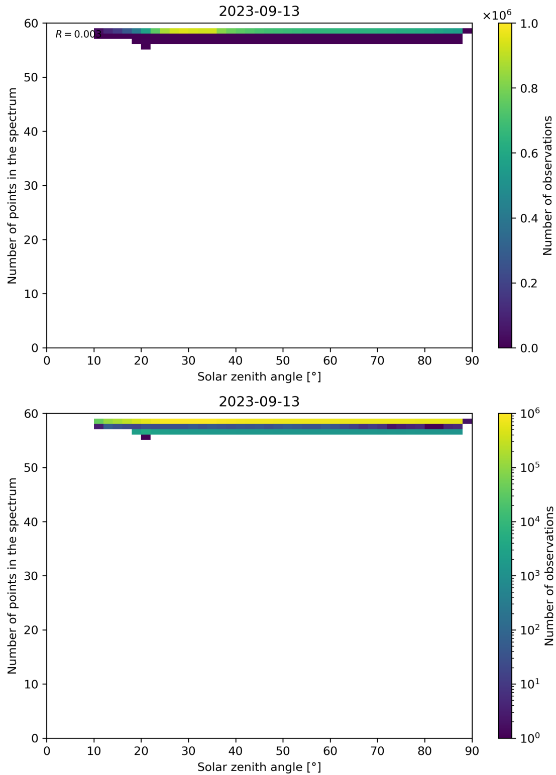
Figure 126: Scatter density plot of “Solar zenith angle” against “Number of points in the spectrum” for 2023-09-12 to 2023-09-14.
