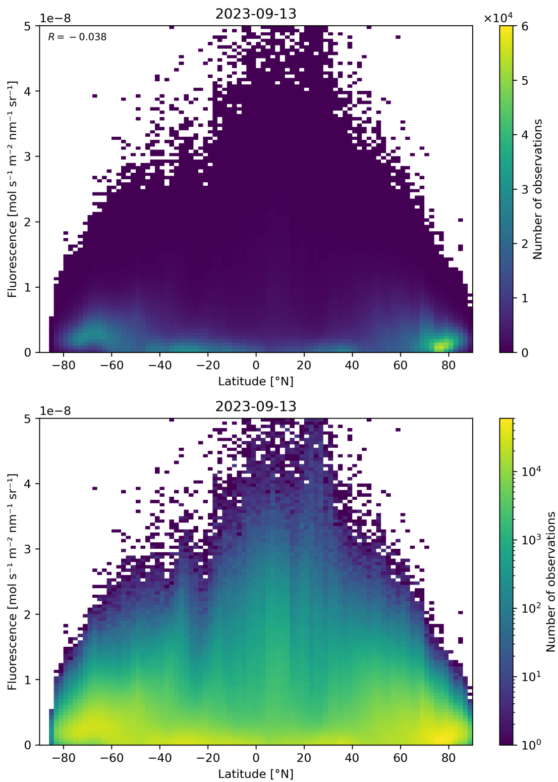
Figure 101: Scatter density plot of “Latitude” against “Fluorescence” for 2023-09-12 to 2023-09-14.
