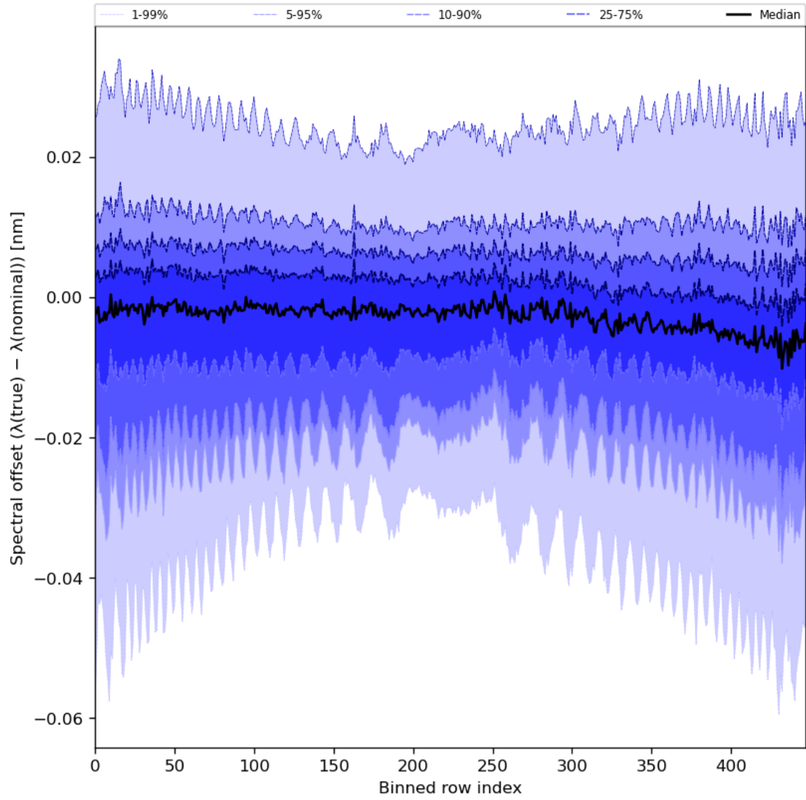
Figure 62: Along track statistics of “Spectral offset ( \lambda(\text{true}) - \lambda(\text{nominal}) )” for 2023-09-12 to 2023-09-14
