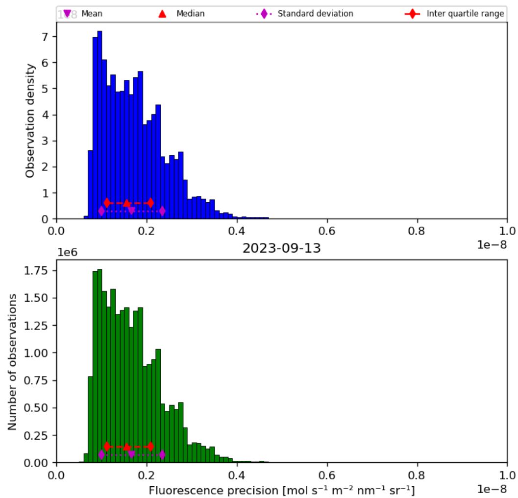
Figure 41: Histogram of “Fluorescence precision” for 2023-09-12 to 2023-09-14
