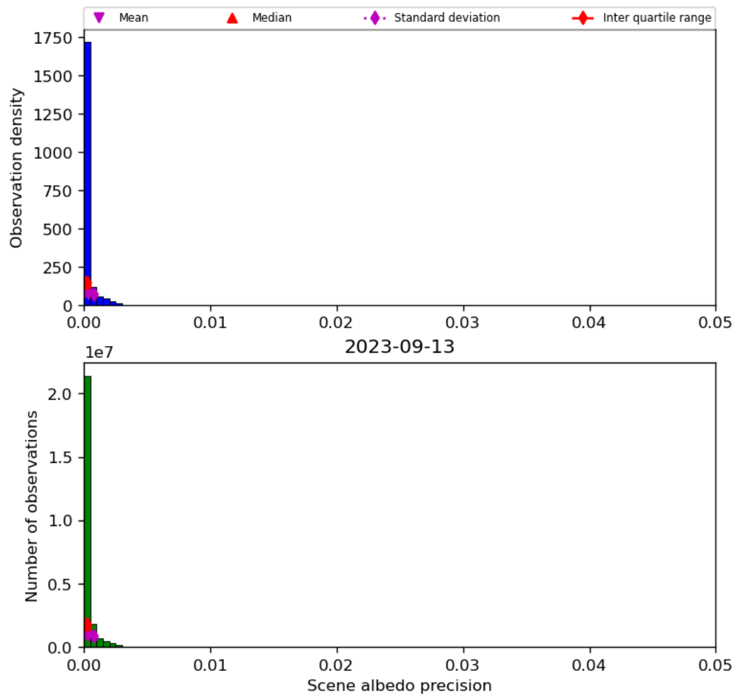
Figure 35: Histogram of “Scene albedo precision” for 2023-09-12 to 2023-09-14
