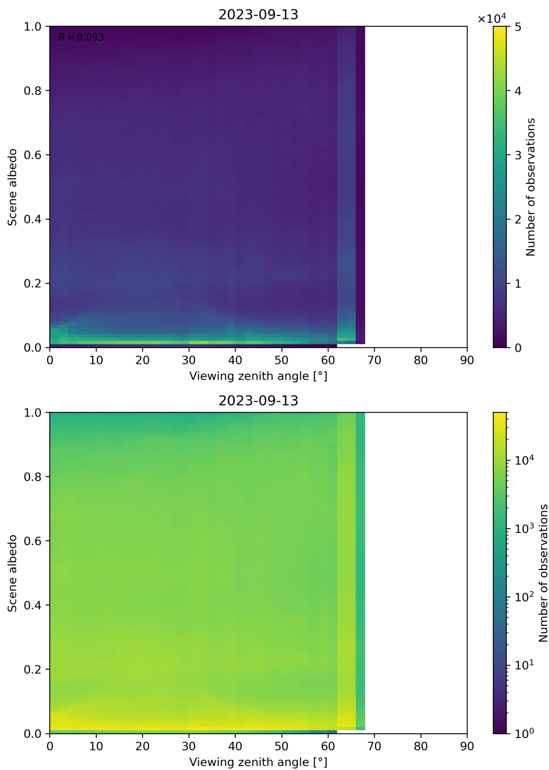
Figure 138: Scatter density plot of “Viewing zenith angle” against “Scene albedo” for 2023-09-12 to 2023-09-14.
