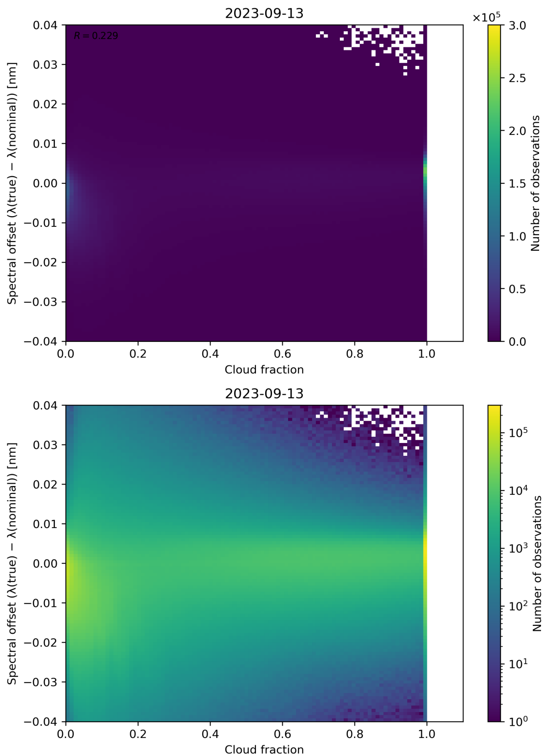
Figure 83: Scatter density plot of “Cloud fraction” against “Spectral offset ( \lambda(\text{true}) - \lambda(\text{nominal}) )” for 2023-09-12 to 2023-09-14.
