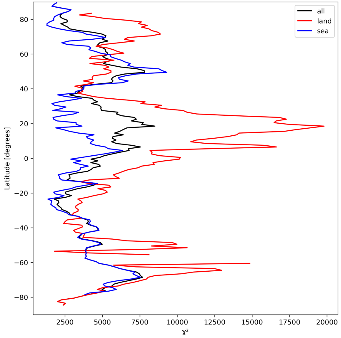
Figure 21: Zonal average of “ \chi^2 ” for 2023-09-12 to 2023-09-14.
