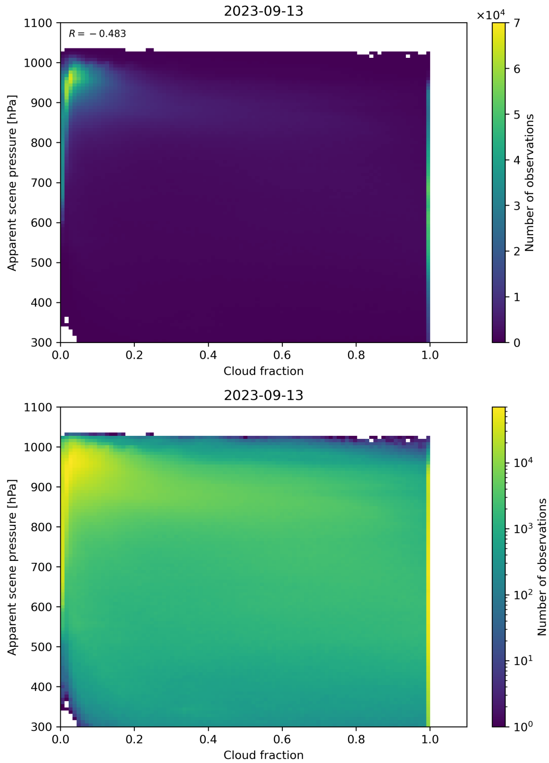
Figure 76: Scatter density plot of “Cloud fraction” against “Apparent scene pressure” for 2023-09-12 to 2023-09-14.
