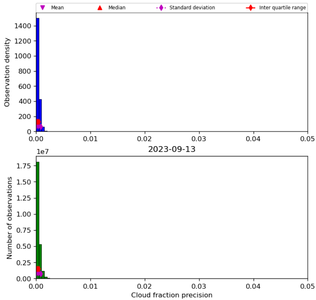
Figure 33: Histogram of “Cloud fraction precision” for 2023-09-12 to 2023-09-14
