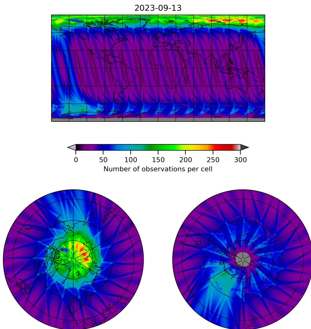
Figure 11: Map of the number of observations for 2023-09-12 to 2023-09-14
