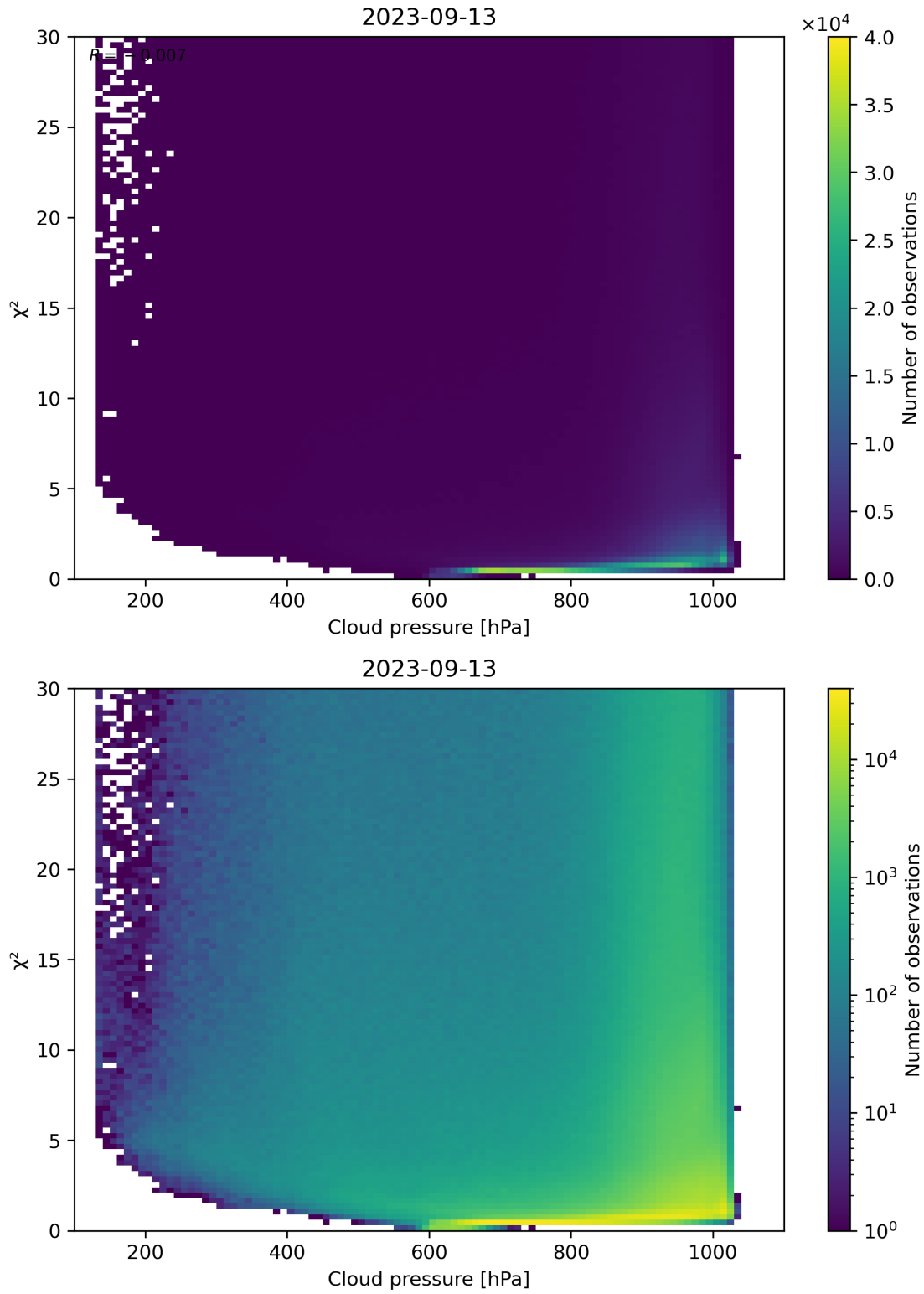
Figure 85: Scatter density plot of “Cloud pressure” against “ \chi^2 ” for 2023-09-12 to 2023-09-14.
