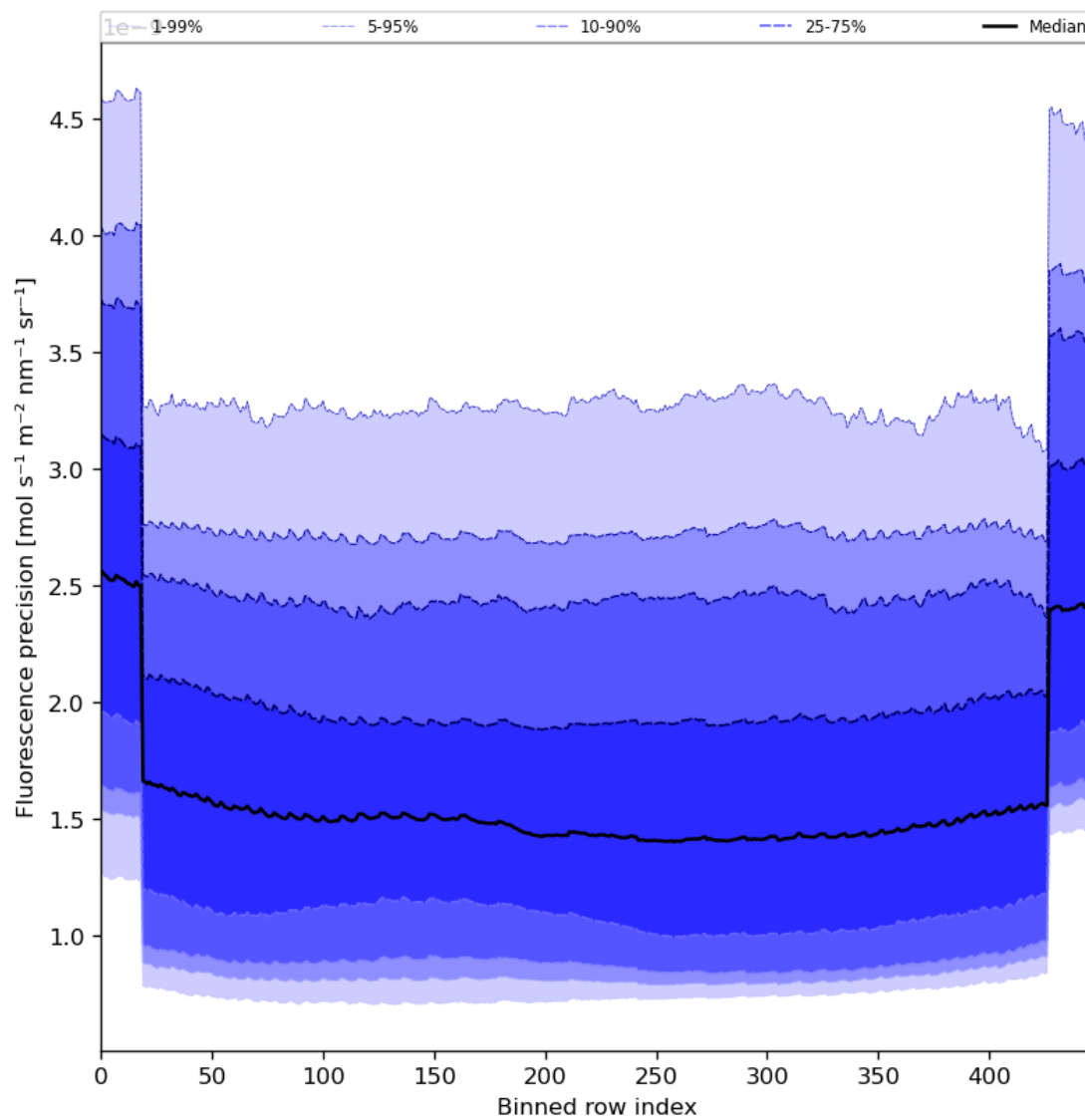
Figure 58: Along track statistics of “Fluorescence precision” for 2023-09-12 to 2023-09-14
