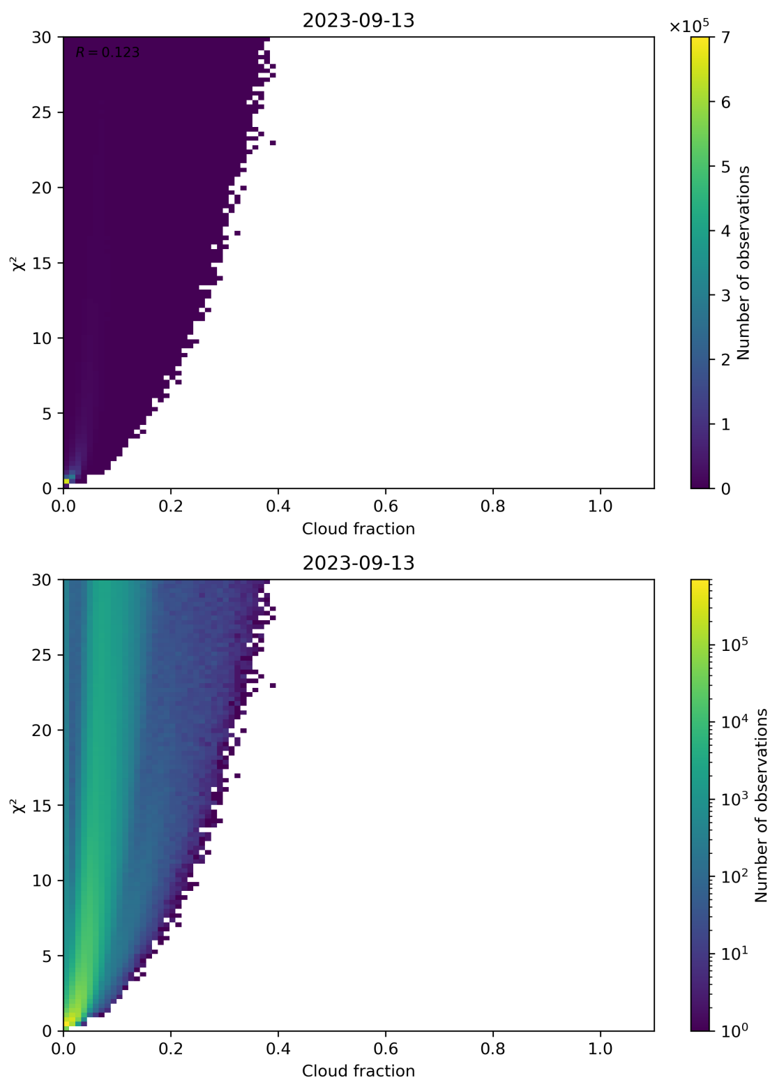
Figure 77: Scatter density plot of “Cloud fraction” against “ \chi^2 ” for 2023-09-12 to 2023-09-14.
