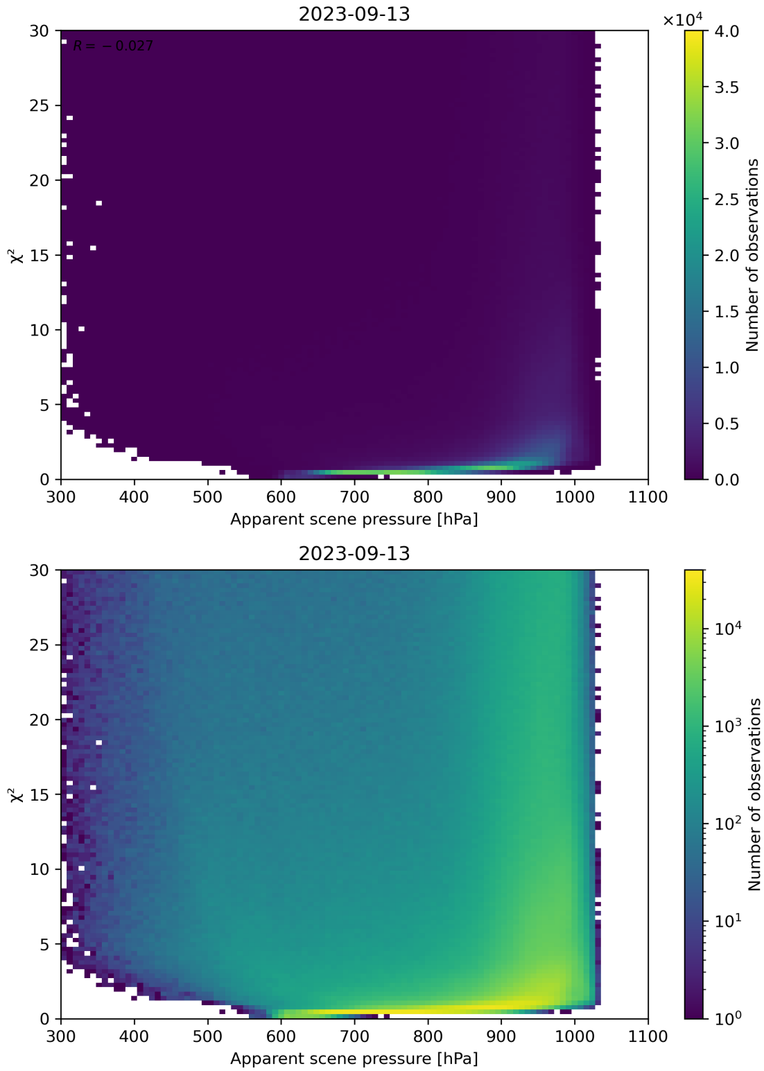
Figure 63: Scatter density plot of “Apparent scene pressure” against “ \chi^2 ” for 2023-09-12 to 2023-09-14.
