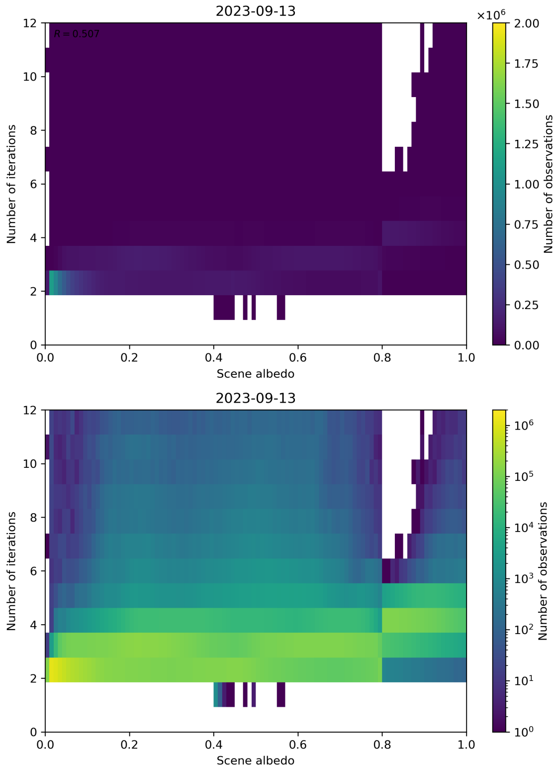
Figure 115: Scatter density plot of “Scene albedo” against “Number of iterations” for 2023-09-12 to 2023-09-14.
