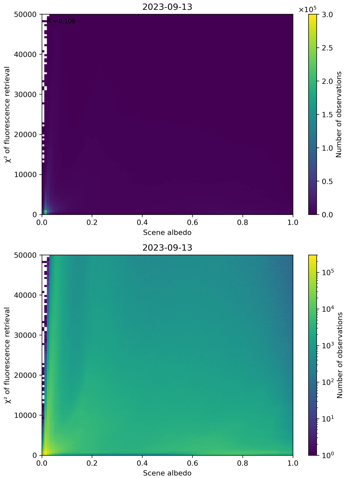
Figure 113: Scatter density plot of “Scene albedo” against “ \chi^2 of fluorescence retrieval” for 2023-09-12 to 2023-09-14.
