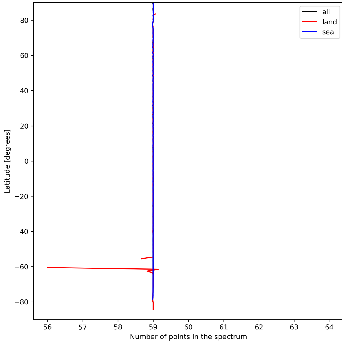
Figure 27: Zonal average of “Number of points in the spectrum” for 2023-09-12 to 2023-09-14.
