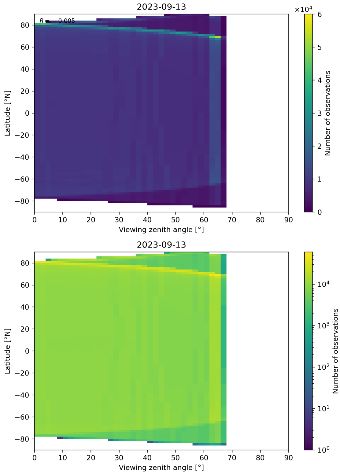
Figure 135: Scatter density plot of “Viewing zenith angle” against “Latitude” for 2023-09-12 to 2023-09-14.
