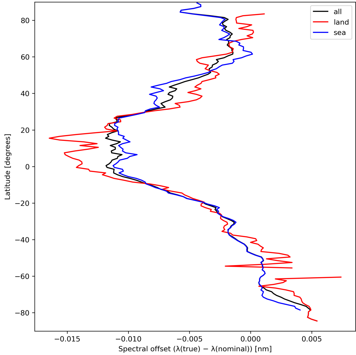
Figure 28: Zonal average of “Spectral offset ( \lambda(\text{true}) - \lambda(\text{nominal}) )” for 2023-09-12 to 2023-09-14.
