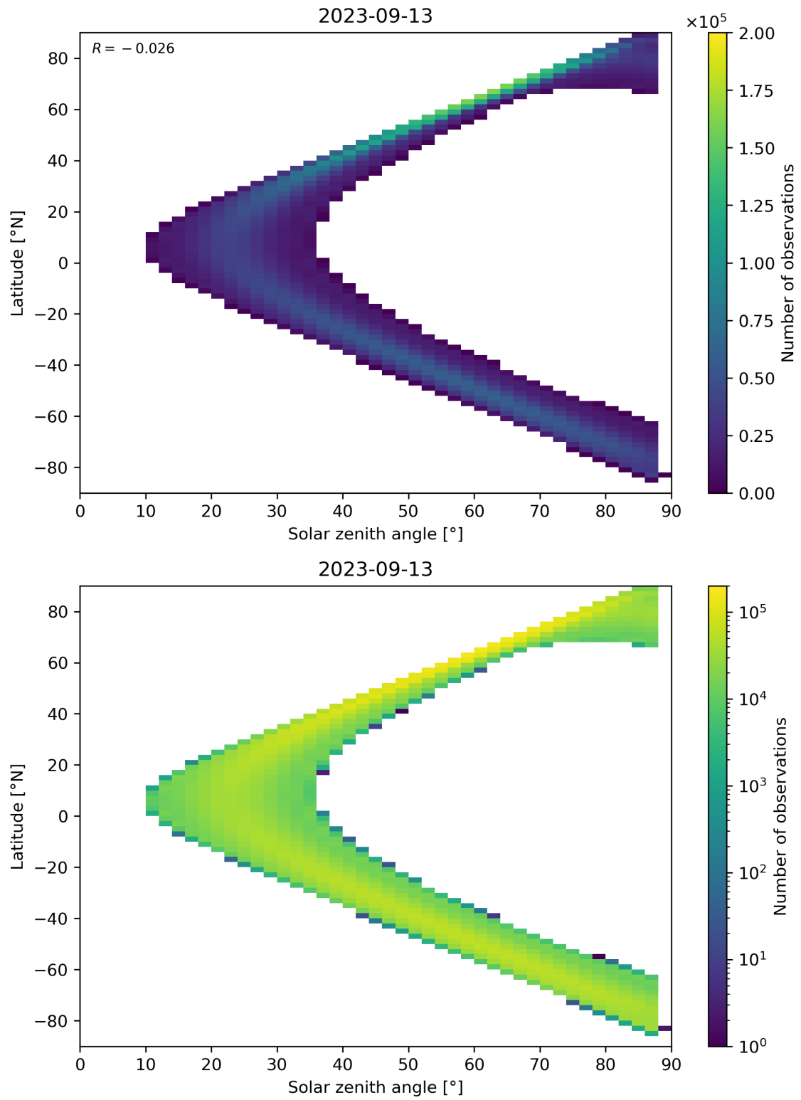
Figure 124: Scatter density plot of “Solar zenith angle” against “Latitude” for 2023-09-12 to 2023-09-14.
