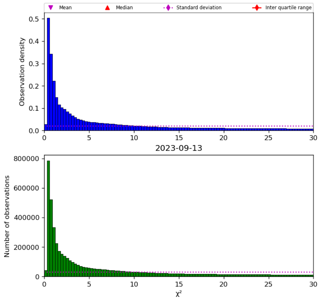
Figure 38: Histogram of “ \chi^2 ” for 2023-09-12 to 2023-09-14
