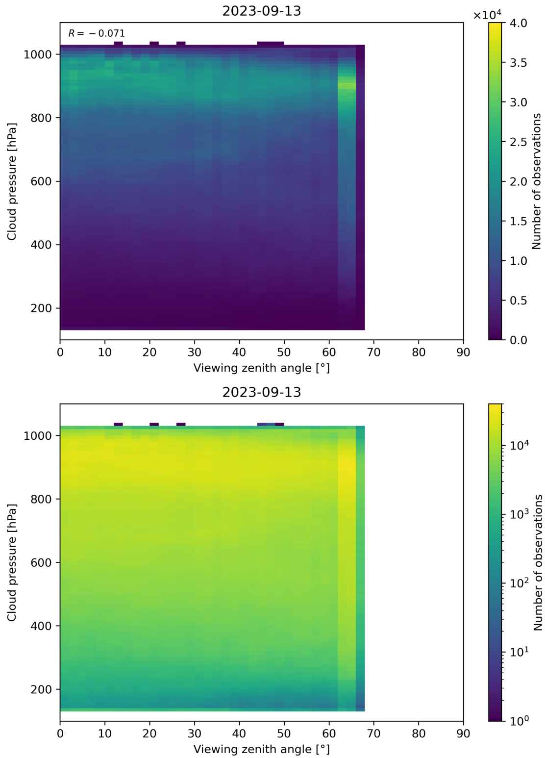
Figure 133: Scatter density plot of “Viewing zenith angle” against “Cloud pressure” for 2023-09-12 to 2023-09-14.
