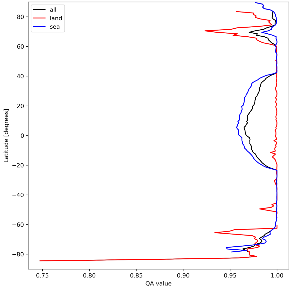
Figure 12: Zonal average of “QA value” for 2023-09-12 to 2023-09-14.
