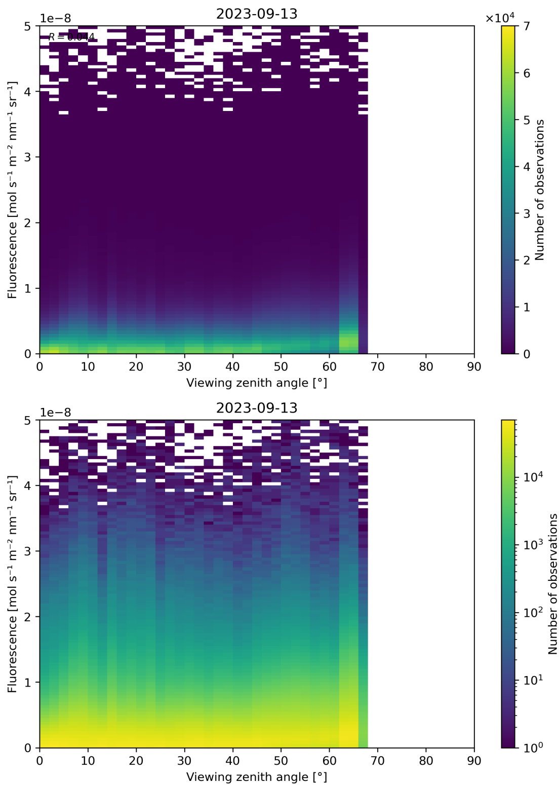
Figure 134: Scatter density plot of “Viewing zenith angle” against “Fluorescence” for 2023-09-12 to 2023-09-14.
