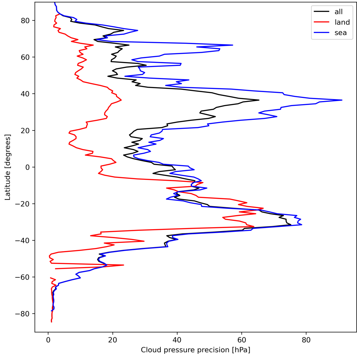
Figure 14: Zonal average of “Cloud pressure precision” for 2023-09-12 to 2023-09-14.
