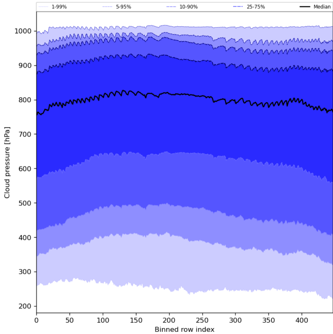
Figure 47: Along track statistics of “Cloud pressure” for 2023-09-12 to 2023-09-14
