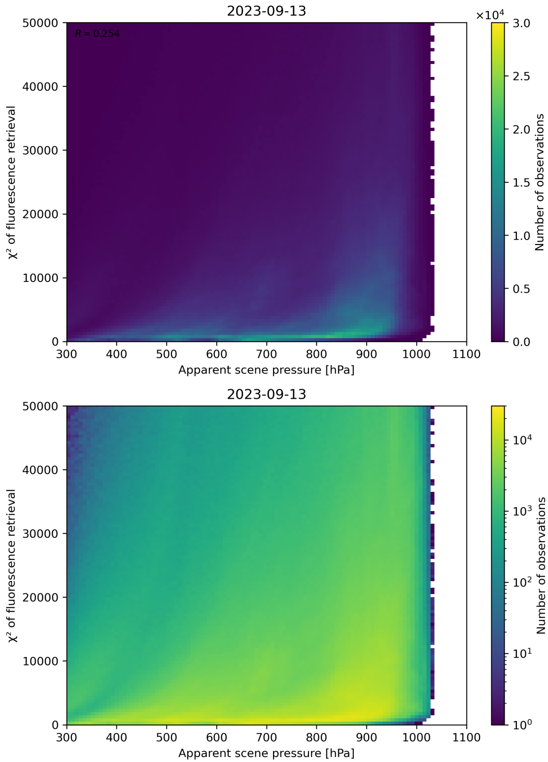
Figure 64: Scatter density plot of “Apparent scene pressure” against “ \chi^2 of fluorescence retrieval” for 2023-09-12 to 2023-09-14.
