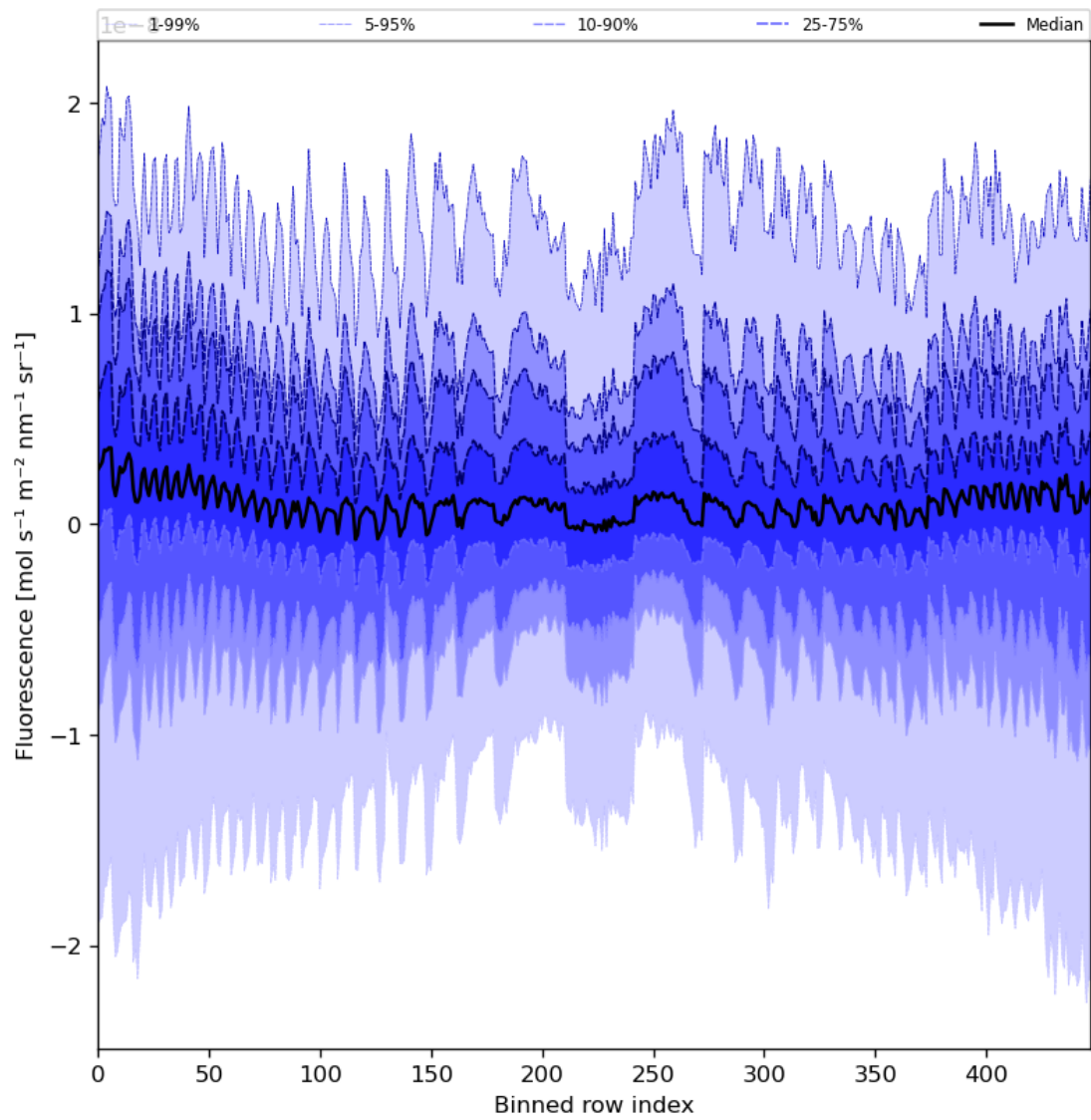
Figure 57: Along track statistics of “Fluorescence” for 2023-09-12 to 2023-09-14
