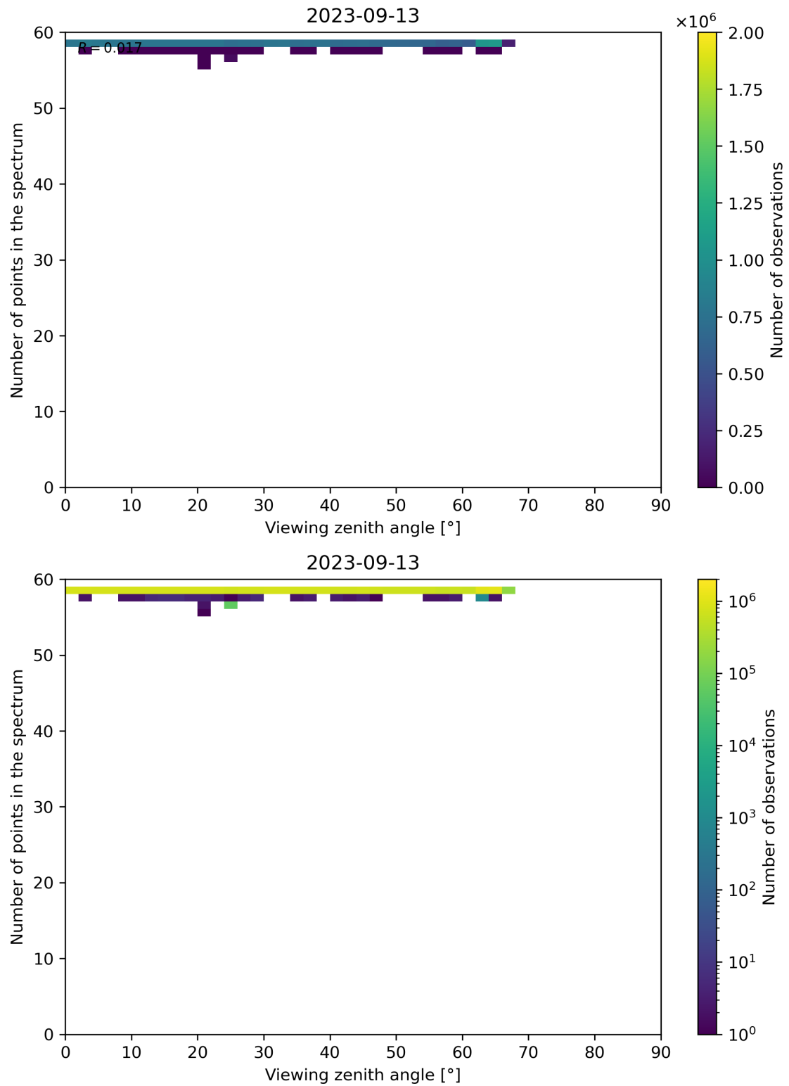
Figure 137: Scatter density plot of “Viewing zenith angle” against “Number of points in the spectrum” for 2023-09-12 to 2023-09-14.
