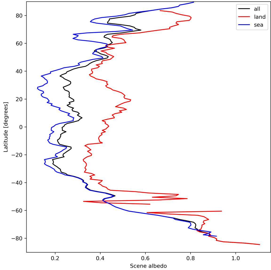
Figure 17: Zonal average of “Scene albedo” for 2023-09-12 to 2023-09-14.
