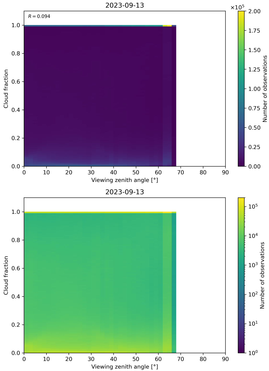
Figure 132: Scatter density plot of “Viewing zenith angle” against “Cloud fraction” for 2023-09-12 to 2023-09-14.
