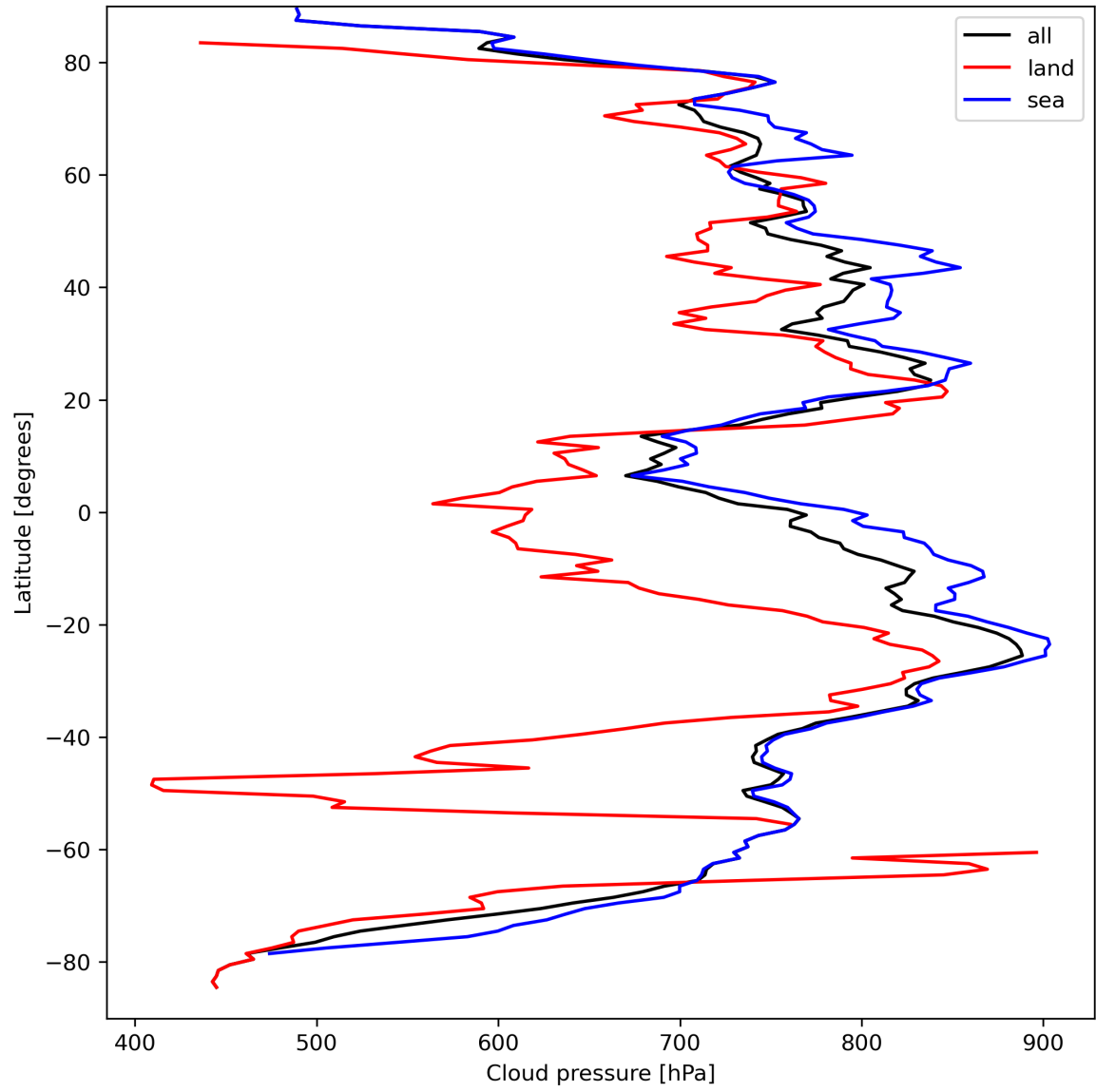
Figure 13: Zonal average of “Cloud pressure” for 2023-09-12 to 2023-09-14.
