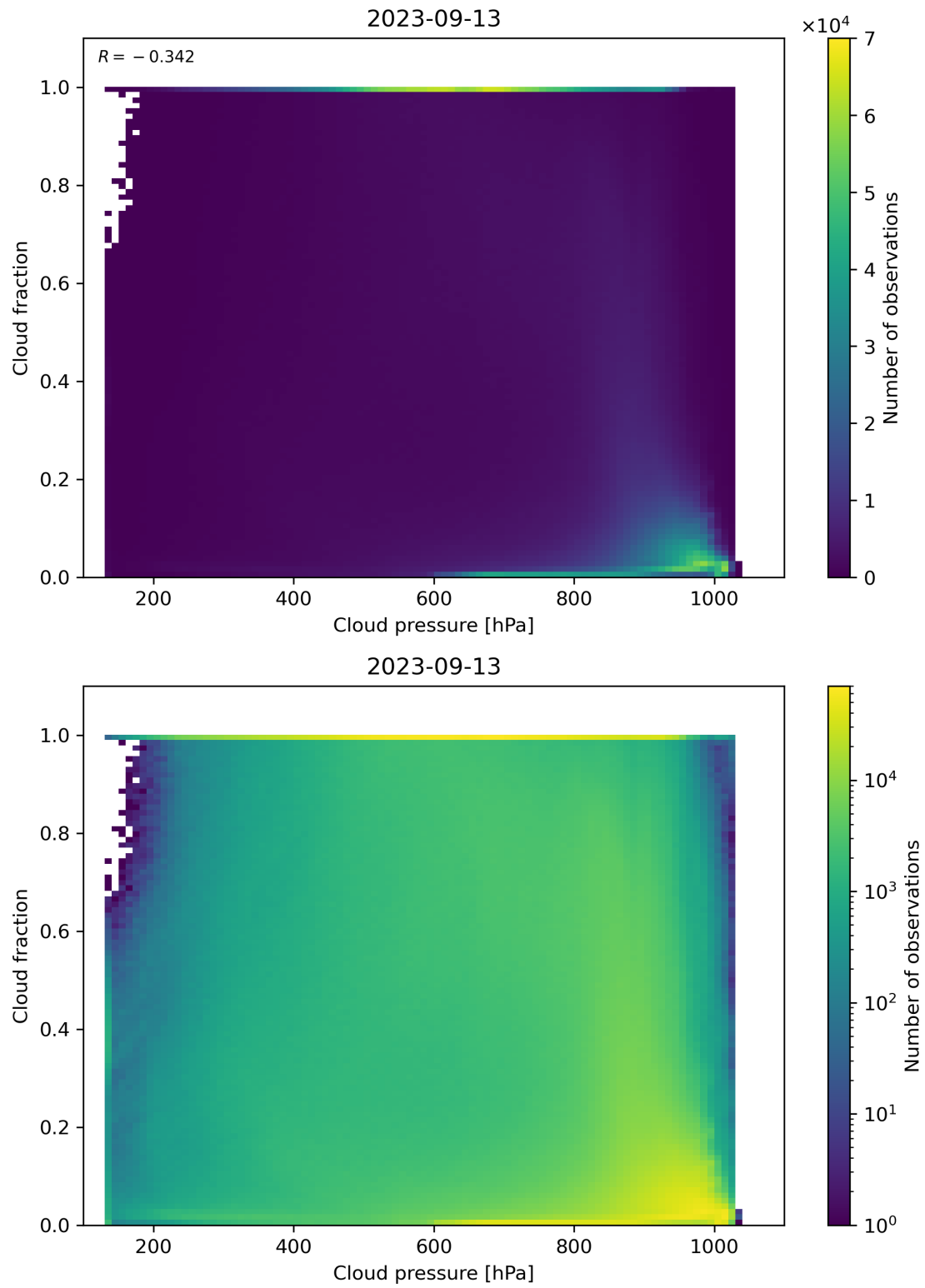
Figure 87: Scatter density plot of “Cloud pressure” against “Cloud fraction” for 2023-09-12 to 2023-09-14.
