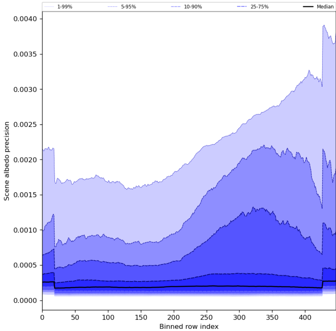
Figure 52: Along track statistics of “Scene albedo precision” for 2023-09-12 to 2023-09-14
