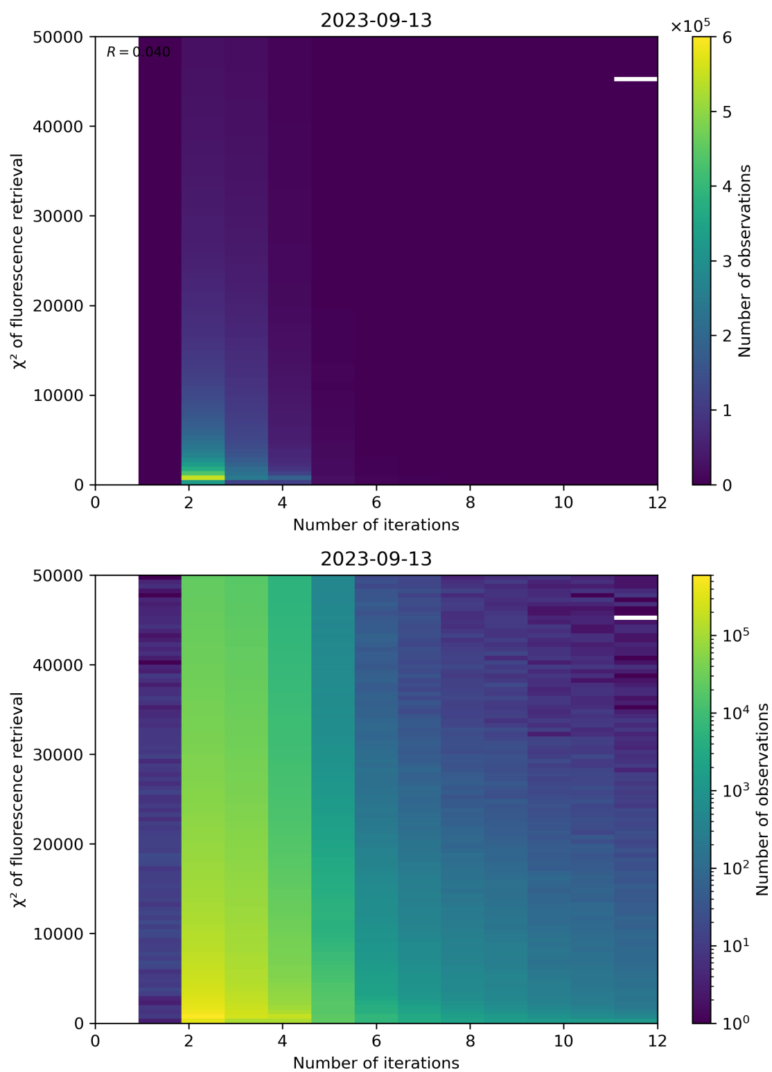
Figure 106: Scatter density plot of “Number of iterations” against “ \chi^2 of fluorescence retrieval” for 2023-09-12 to 2023-09-14.
