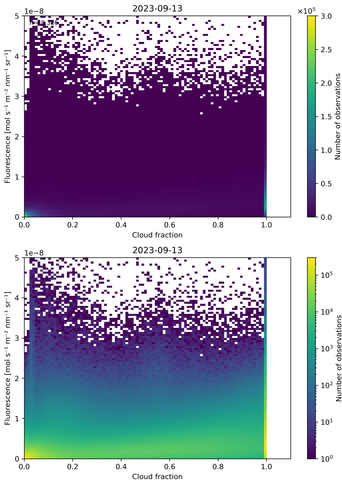
Figure 79: Scatter density plot of “Cloud fraction” against “Fluorescence” for 2023-09-12 to 2023-09-14.
