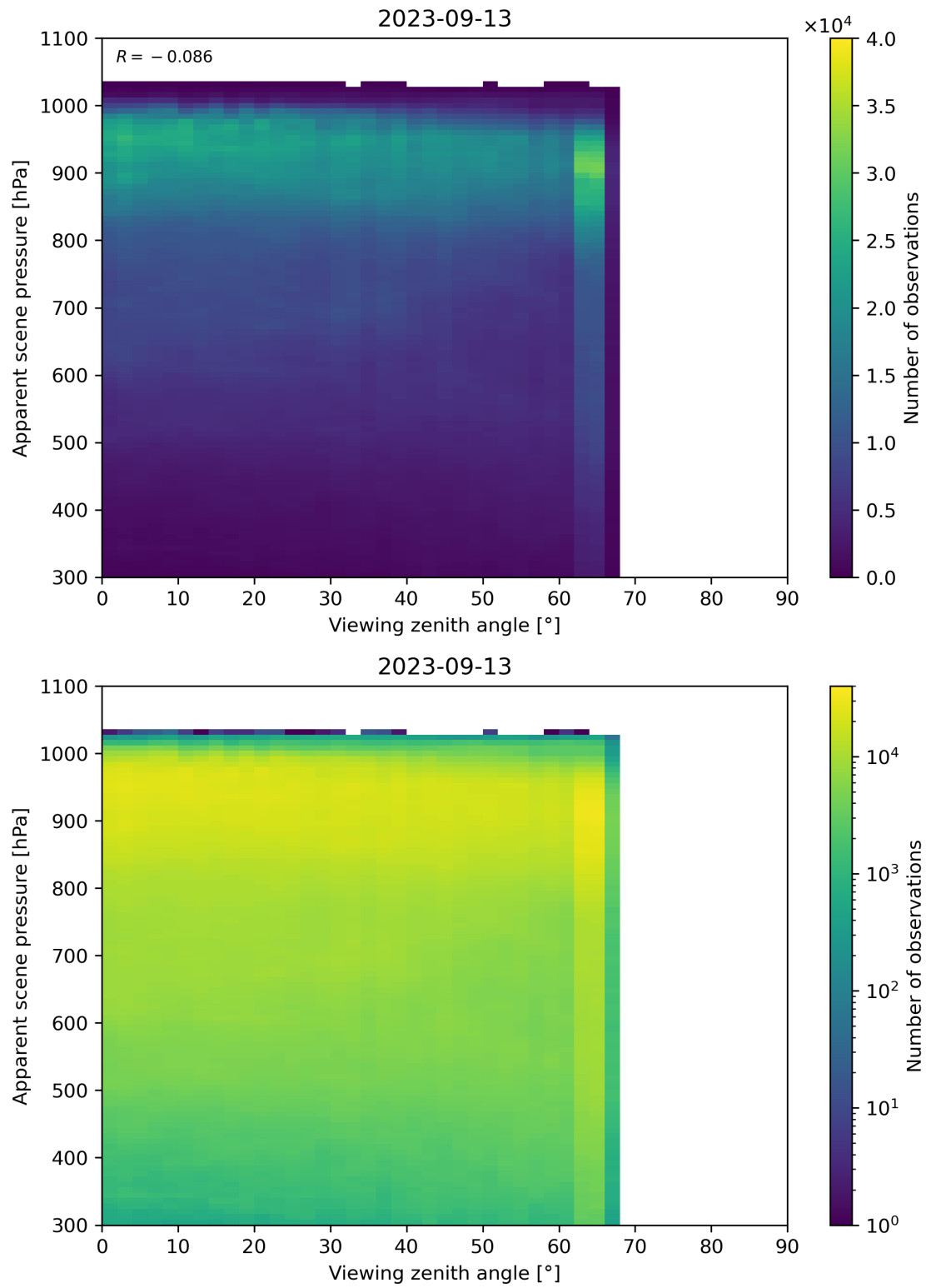
Figure 129: Scatter density plot of “Viewing zenith angle” against “Apparent scene pressure” for 2023-09-12 to 2023-09-14.
