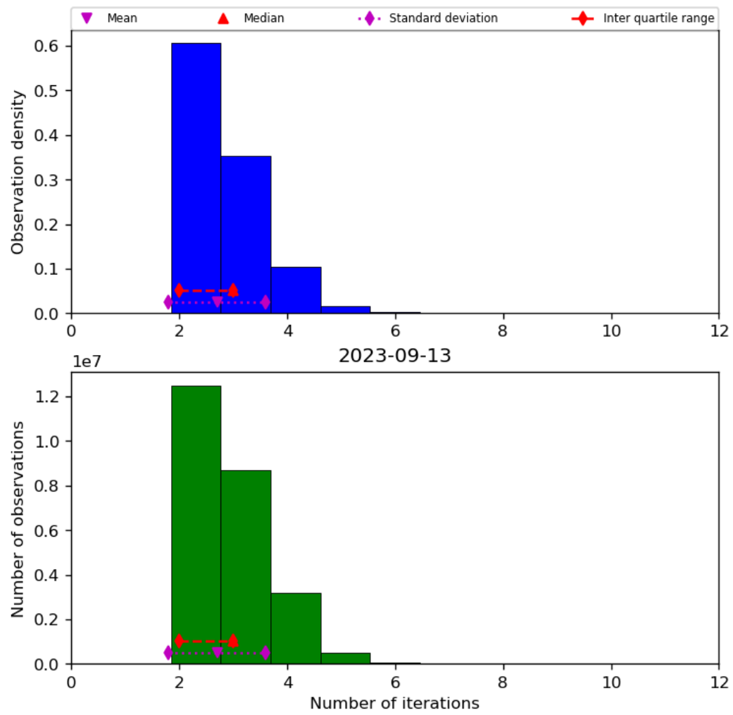
Figure 39: Histogram of “Number of iterations” for 2023-09-12 to 2023-09-14
