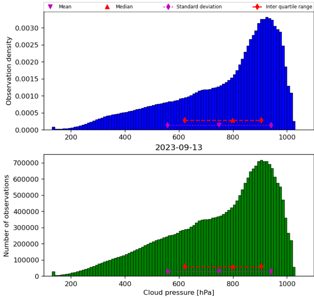
Figure 30: Histogram of “Cloud pressure” for 2023-09-12 to 2023-09-14
