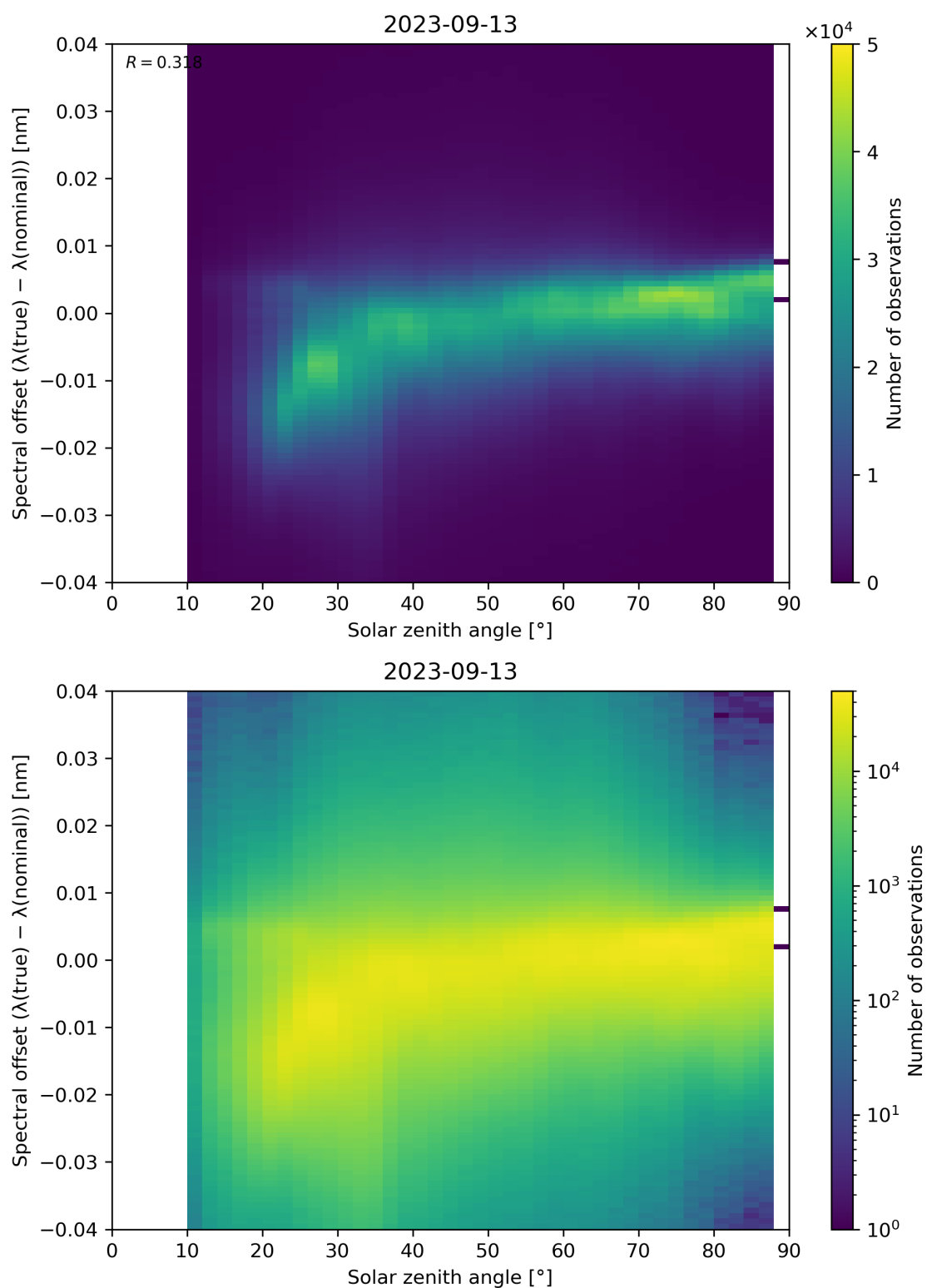
Figure 128: Scatter density plot of “Solar zenith angle” against “Spectral offset ( \lambda(\text{true}) - \lambda(\text{nominal}) )” for 2023-09-12 to 2023-09-14.
