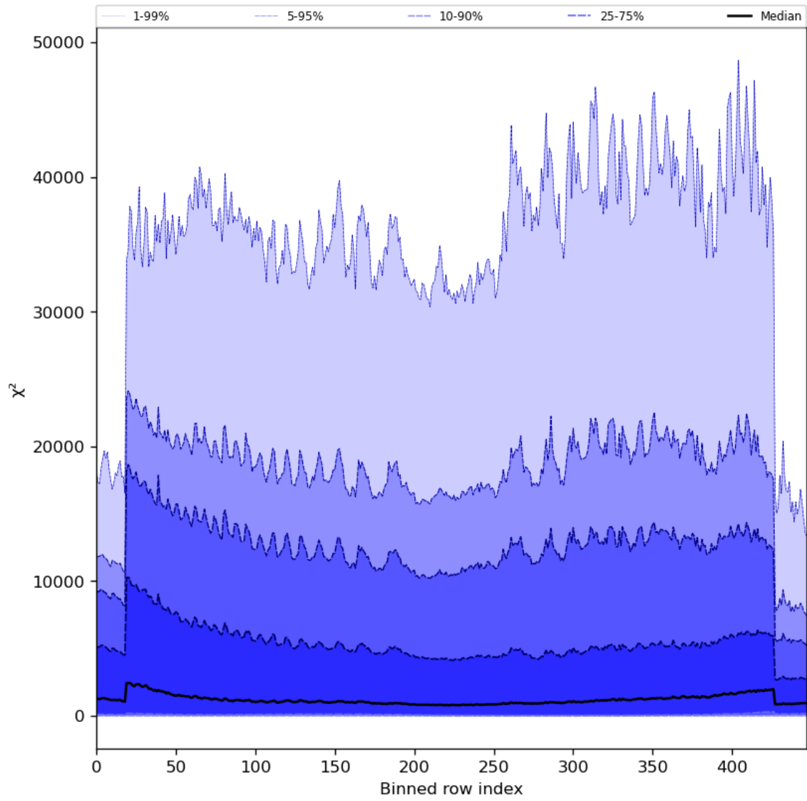
Figure 55: Along track statistics of “ \chi^2 ” for 2023-09-12 to 2023-09-14
