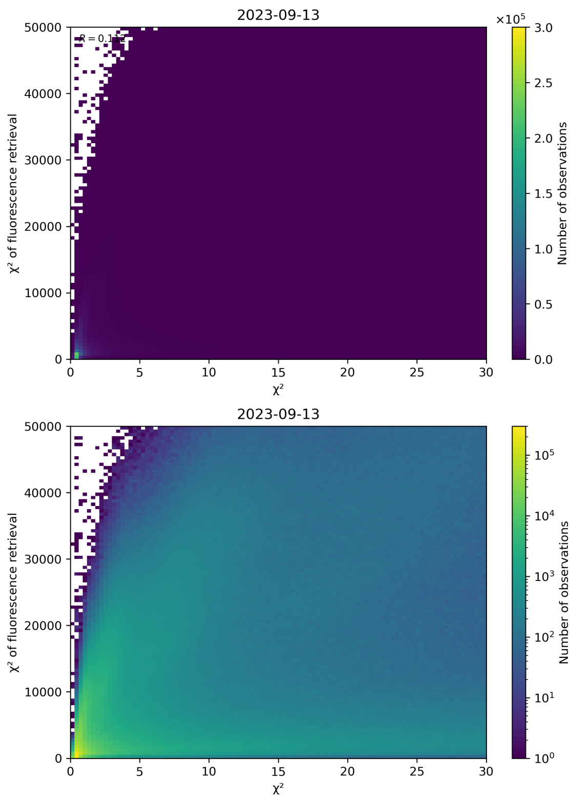
Figure 69: Scatter density plot of “ \chi^2 ” against “ \chi^2 of fluorescence retrieval” for 2023-09-12 to 2023-09-14.
