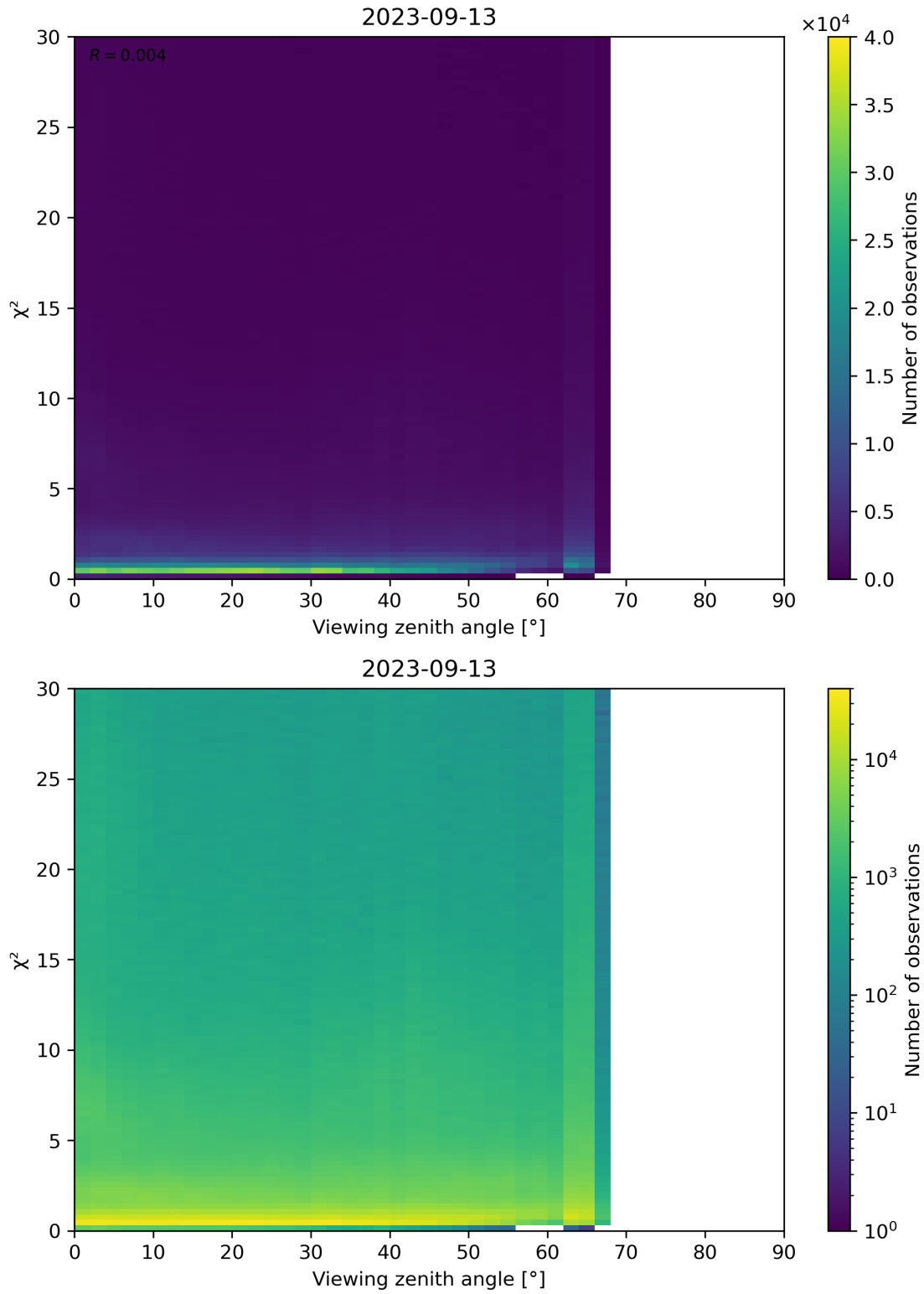
Figure 130: Scatter density plot of “Viewing zenith angle” against “ \chi^2 ” for 2023-09-12 to 2023-09-14.
