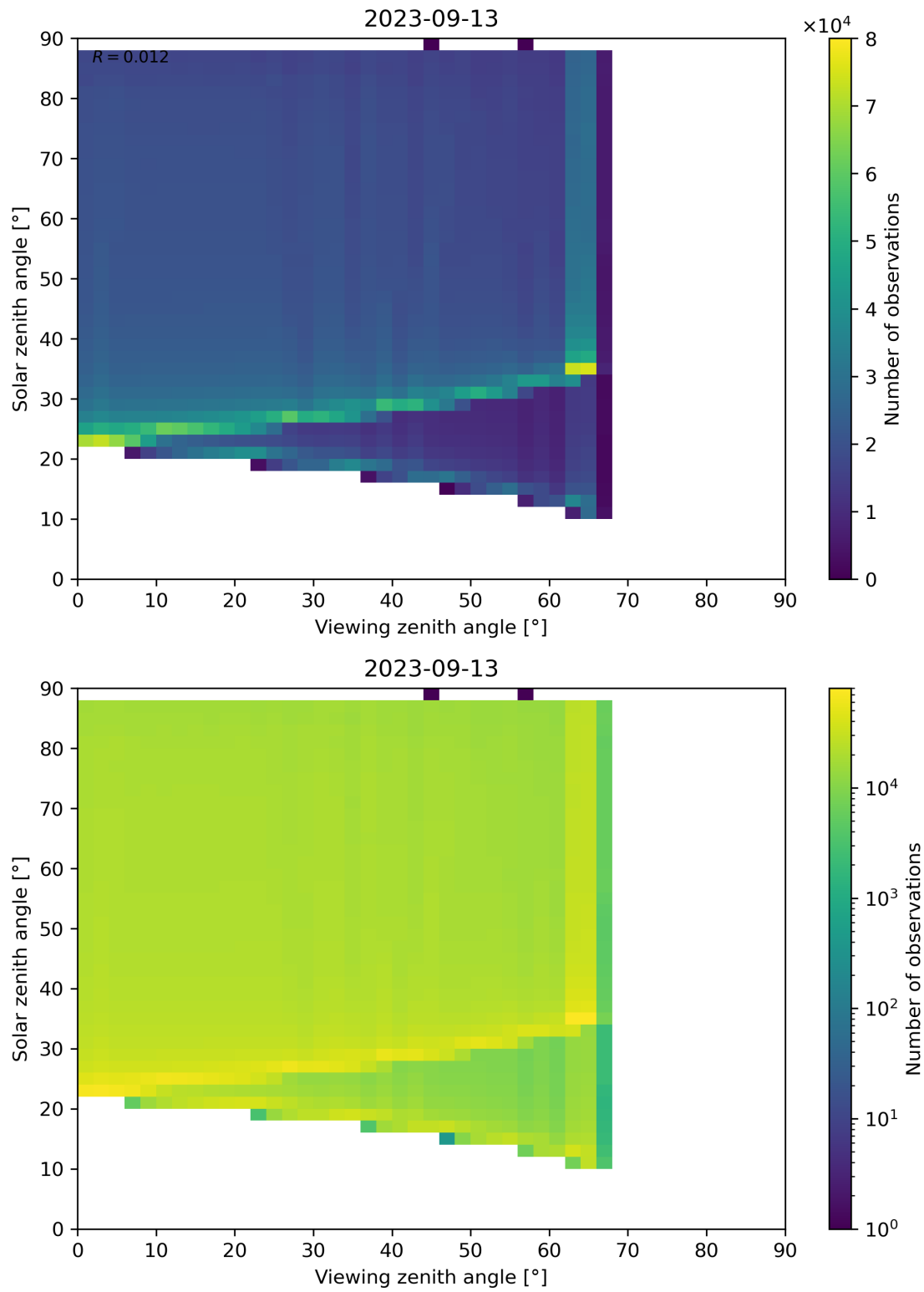
Figure 139: Scatter density plot of “Viewing zenith angle” against “Solar zenith angle” for 2023-09-12 to 2023-09-14.
