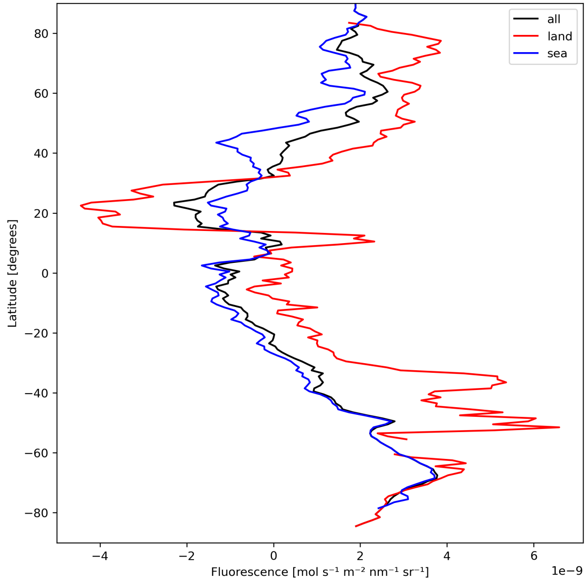
Figure 23: Zonal average of “Fluorescence” for 2023-09-12 to 2023-09-14.
