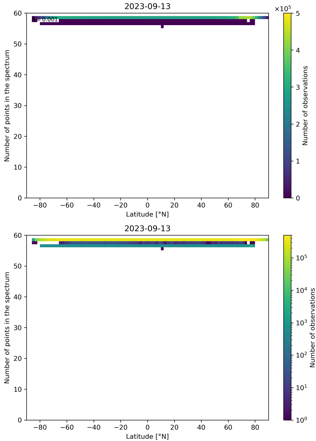
Figure 103: Scatter density plot of “Latitude” against “Number of points in the spectrum” for 2023-09-12 to 2023-09-14.
