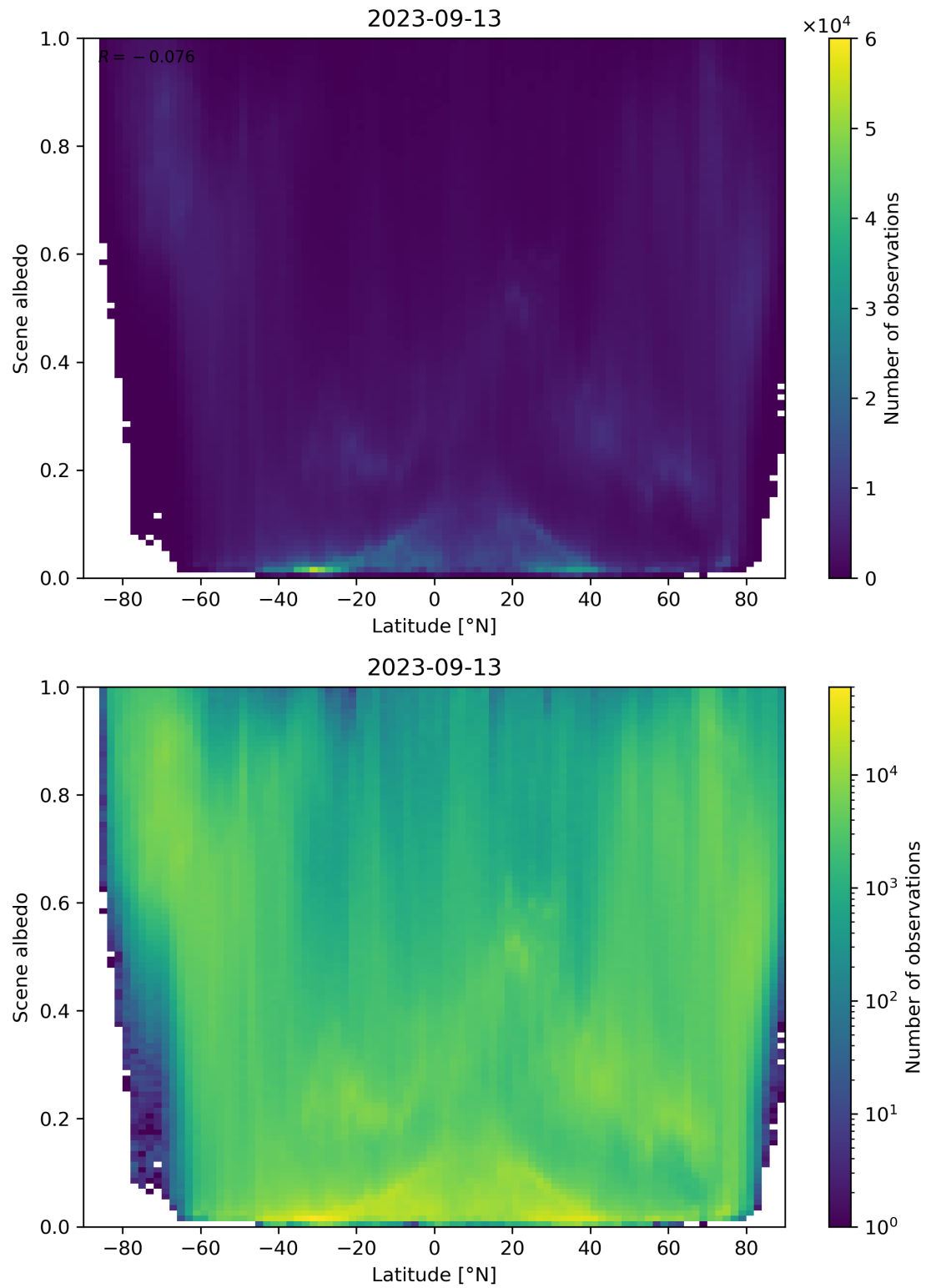
Figure 104: Scatter density plot of “Latitude” against “Scene albedo” for 2023-09-12 to 2023-09-14.
