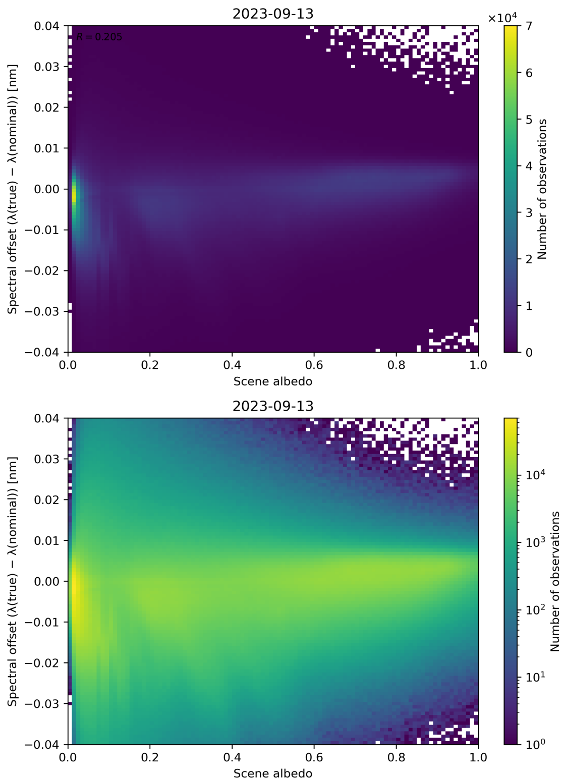
Figure 117: Scatter density plot of “Scene albedo” against “Spectral offset ( \lambda(\text{true}) - \lambda(\text{nominal}) )” for 2023-09-12 to 2023-09-14.
