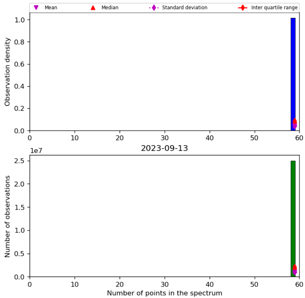
Figure 44: Histogram of “Number of points in the spectrum” for 2023-09-12 to 2023-09-14
