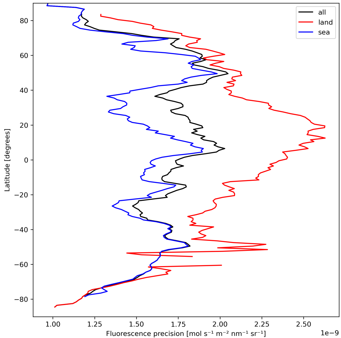
Figure 24: Zonal average of “Fluorescence precision” for 2023-09-12 to 2023-09-14.
