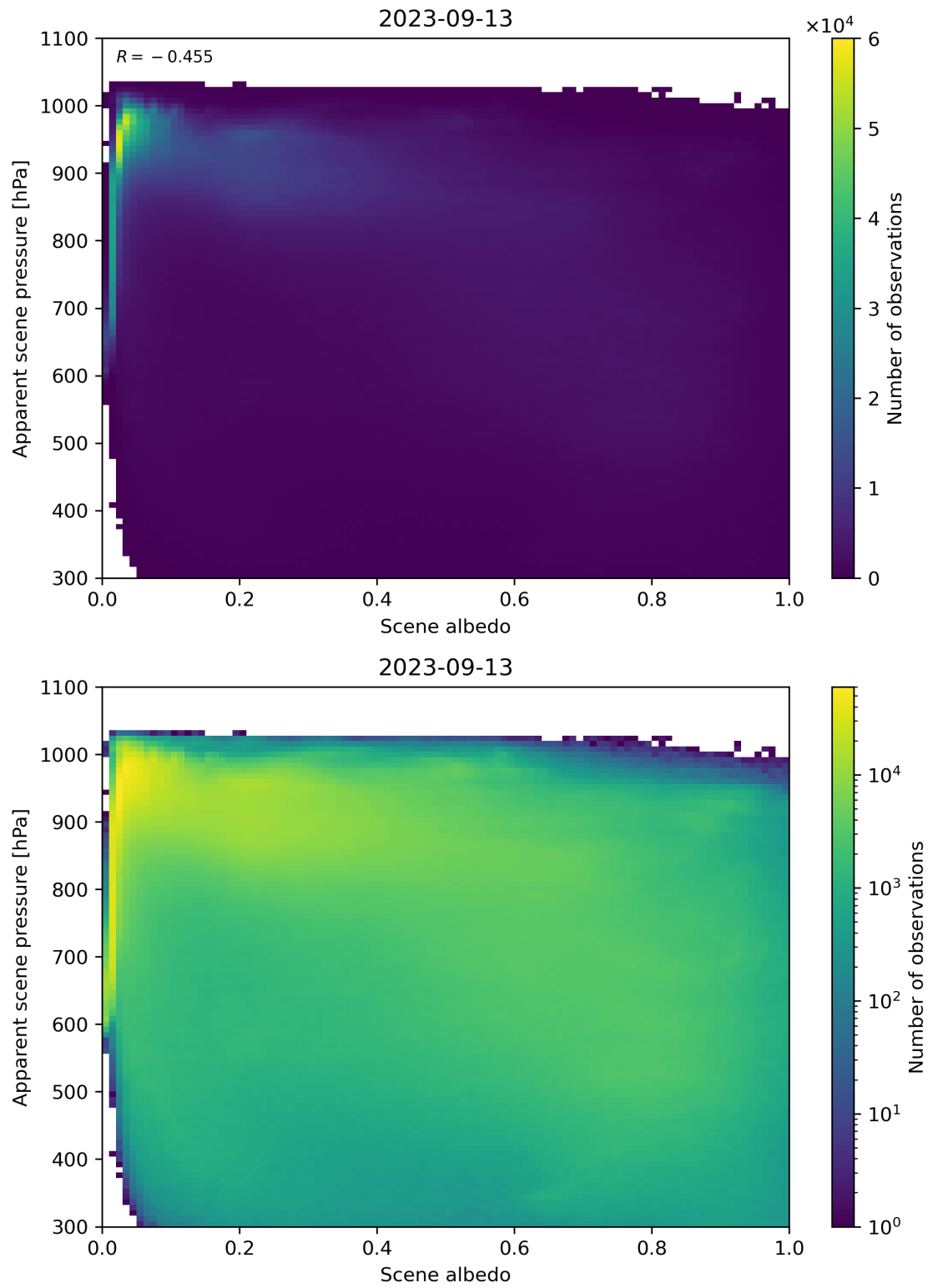
Figure 111: Scatter density plot of “Scene albedo” against “Apparent scene pressure” for 2023-09-12 to 2023-09-14.
