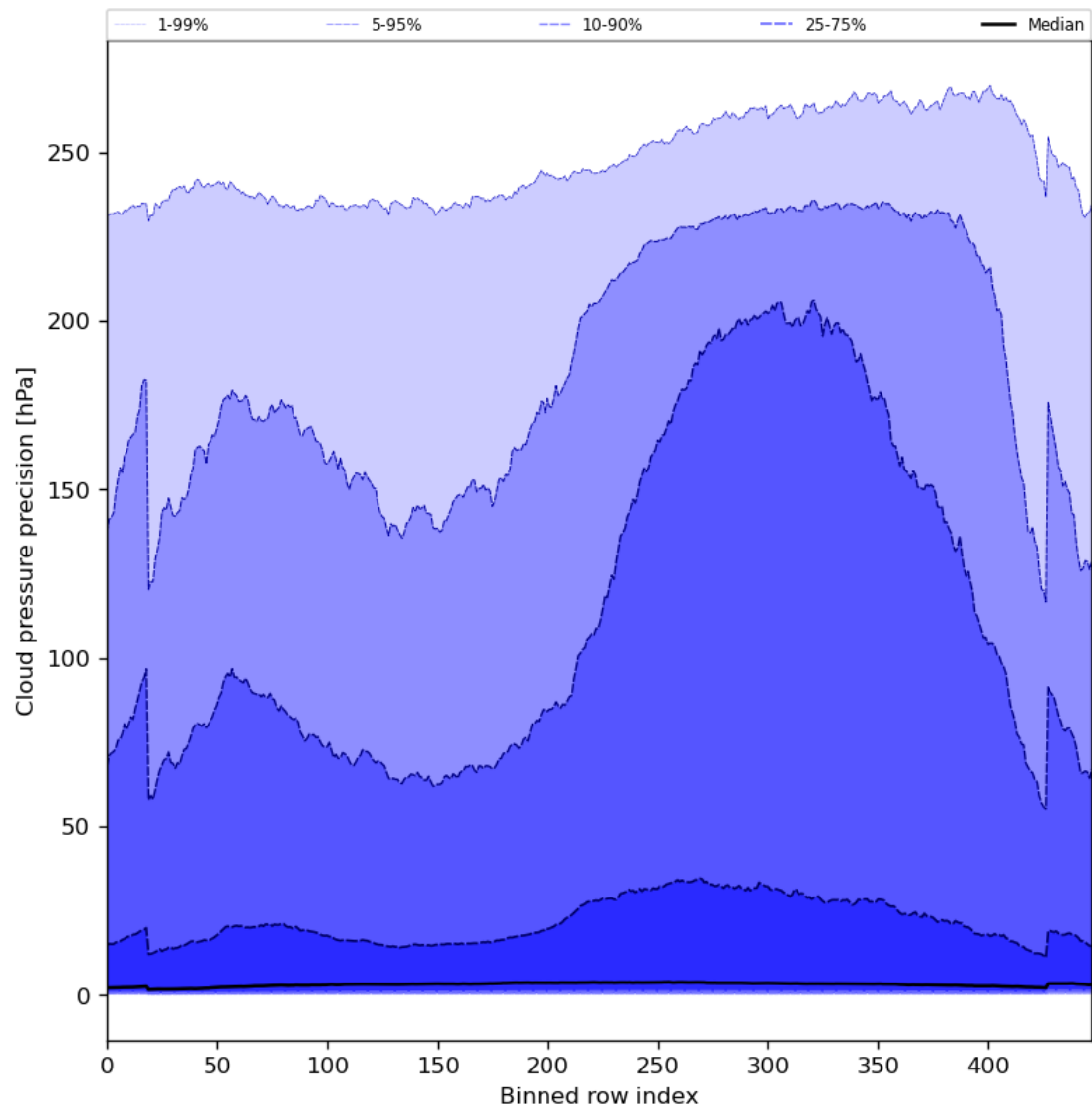
Figure 48: Along track statistics of “Cloud pressure precision” for 2023-09-12 to 2023-09-14
