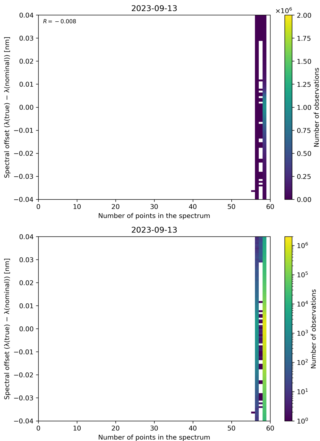
Figure 110: Scatter density plot of “Number of points in the spectrum” against “Spectral offset ( \lambda(\text{true}) - \lambda(\text{nominal}) )” for 2023-09-12 to 2023-09-14.
