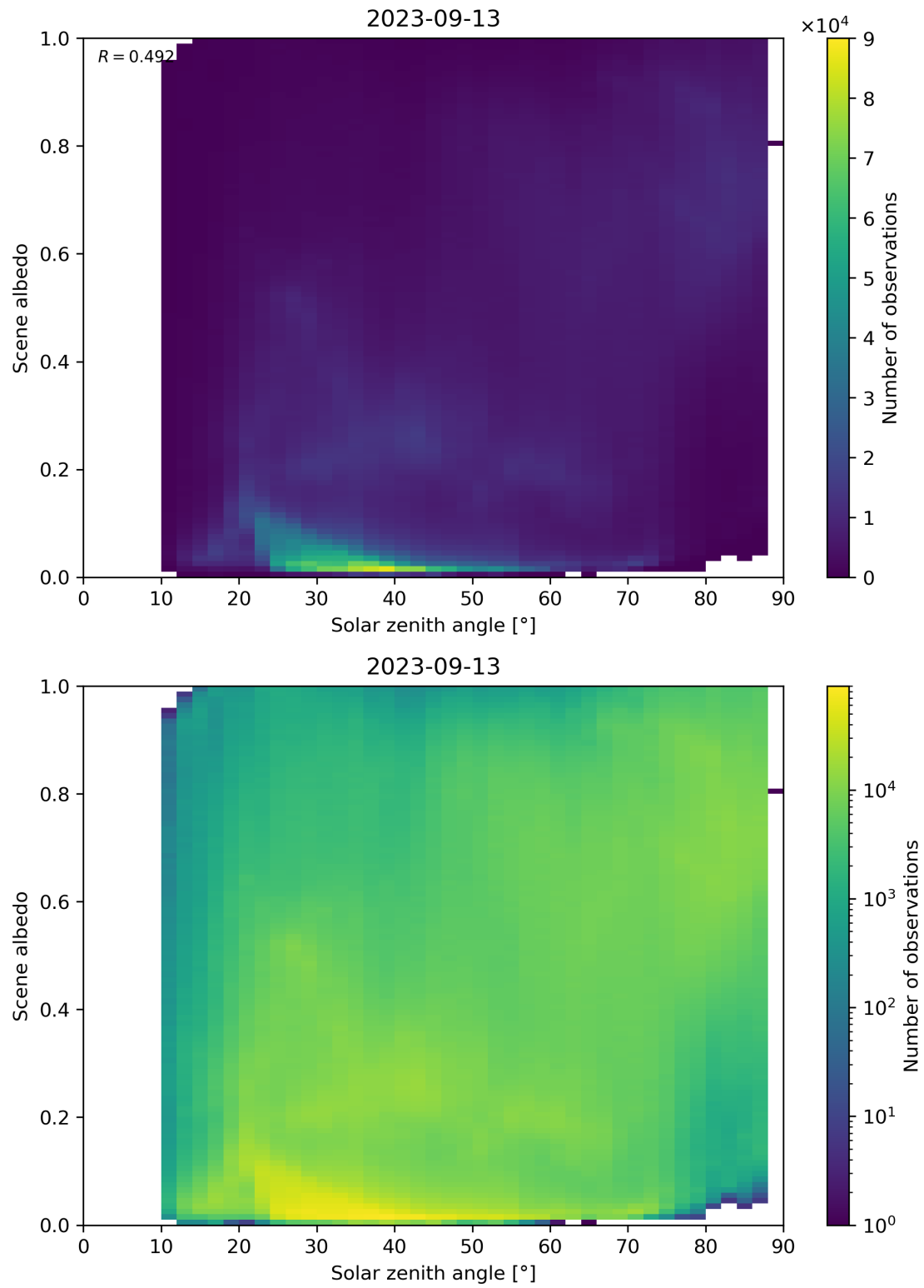
Figure 127: Scatter density plot of “Solar zenith angle” against “Scene albedo” for 2023-09-12 to 2023-09-14.
