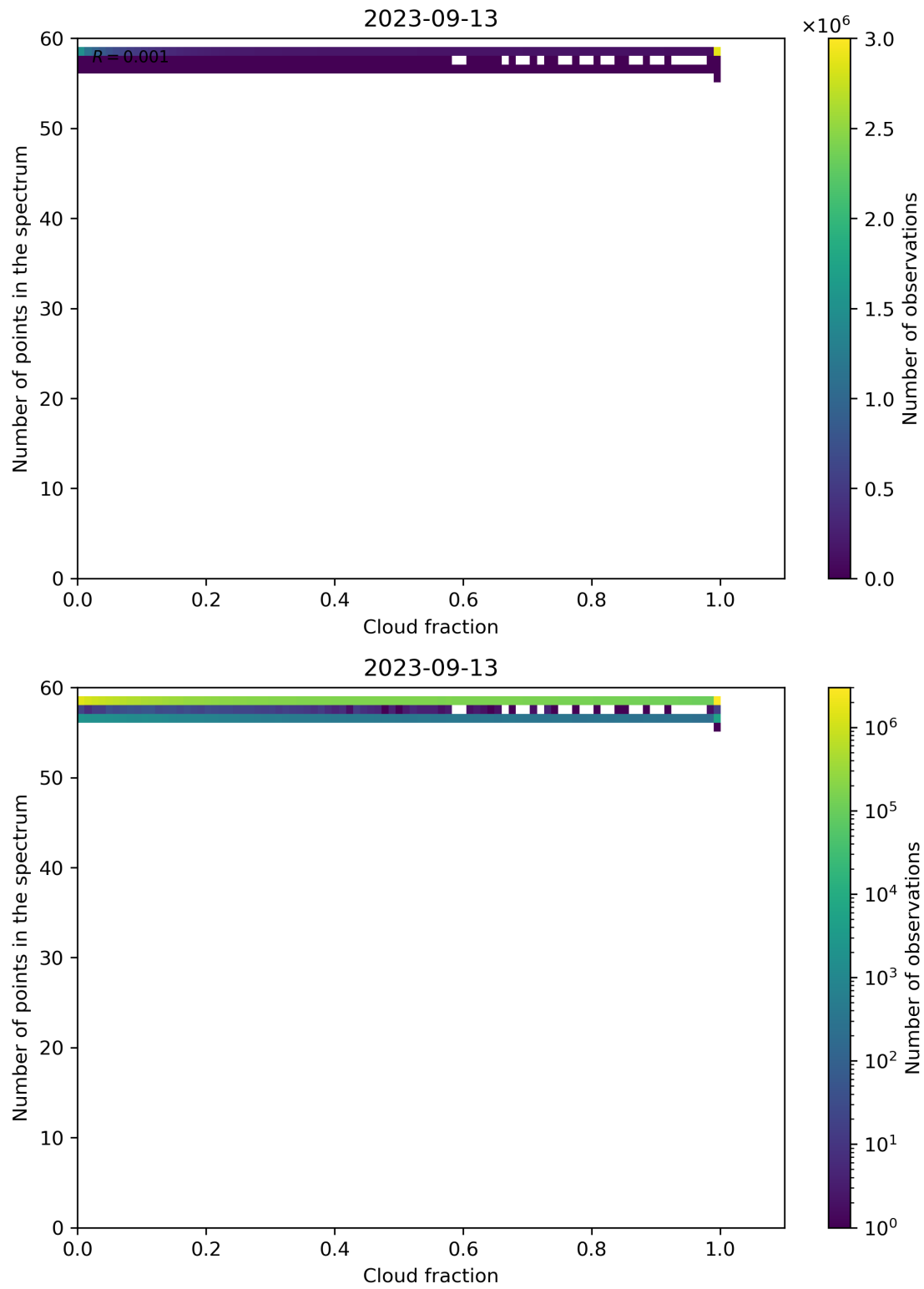
Figure 81: Scatter density plot of “Cloud fraction” against “Number of points in the spectrum” for 2023-09-12 to 2023-09-14.
