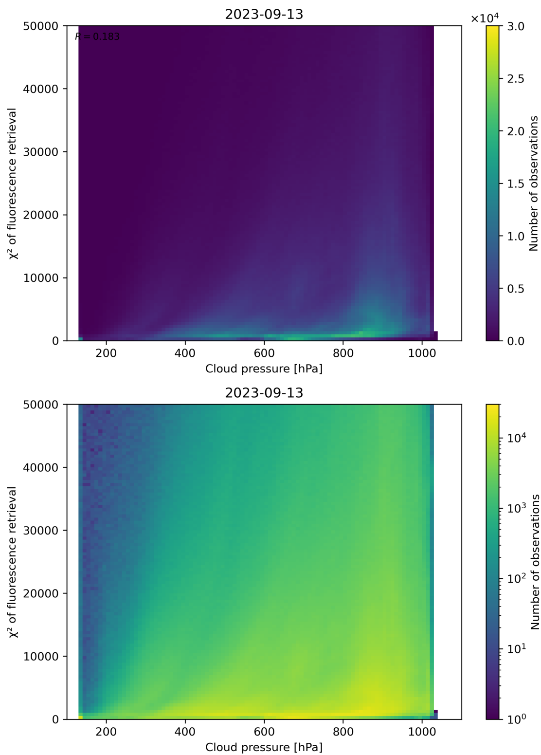
Figure 86: Scatter density plot of “Cloud pressure” against “ \chi^2 of fluorescence retrieval” for 2023-09-12 to 2023-09-14.
