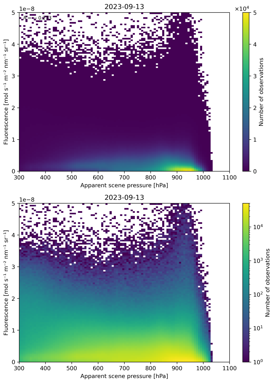
Figure 65: Scatter density plot of “Apparent scene pressure” against “Fluorescence” for 2023-09-12 to 2023-09-14.
