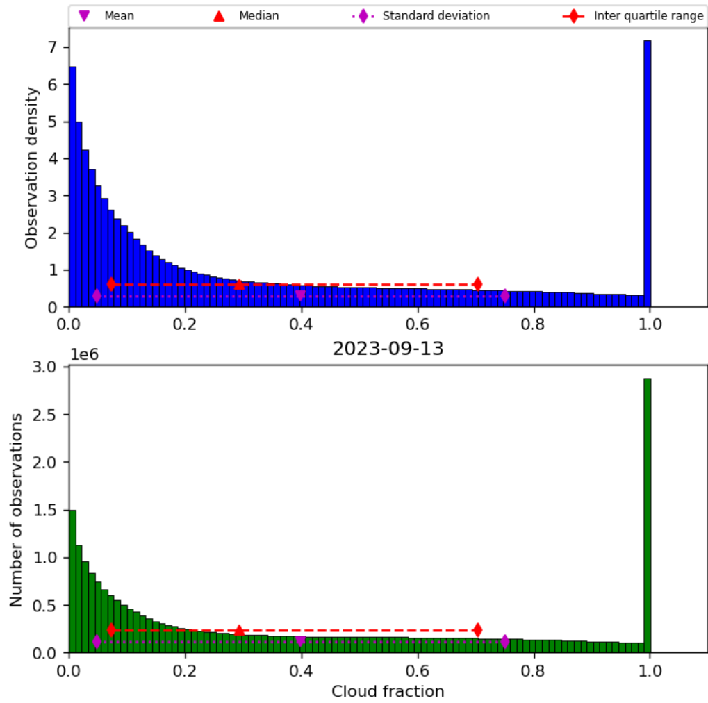
Figure 32: Histogram of “Cloud fraction” for 2023-09-12 to 2023-09-14
