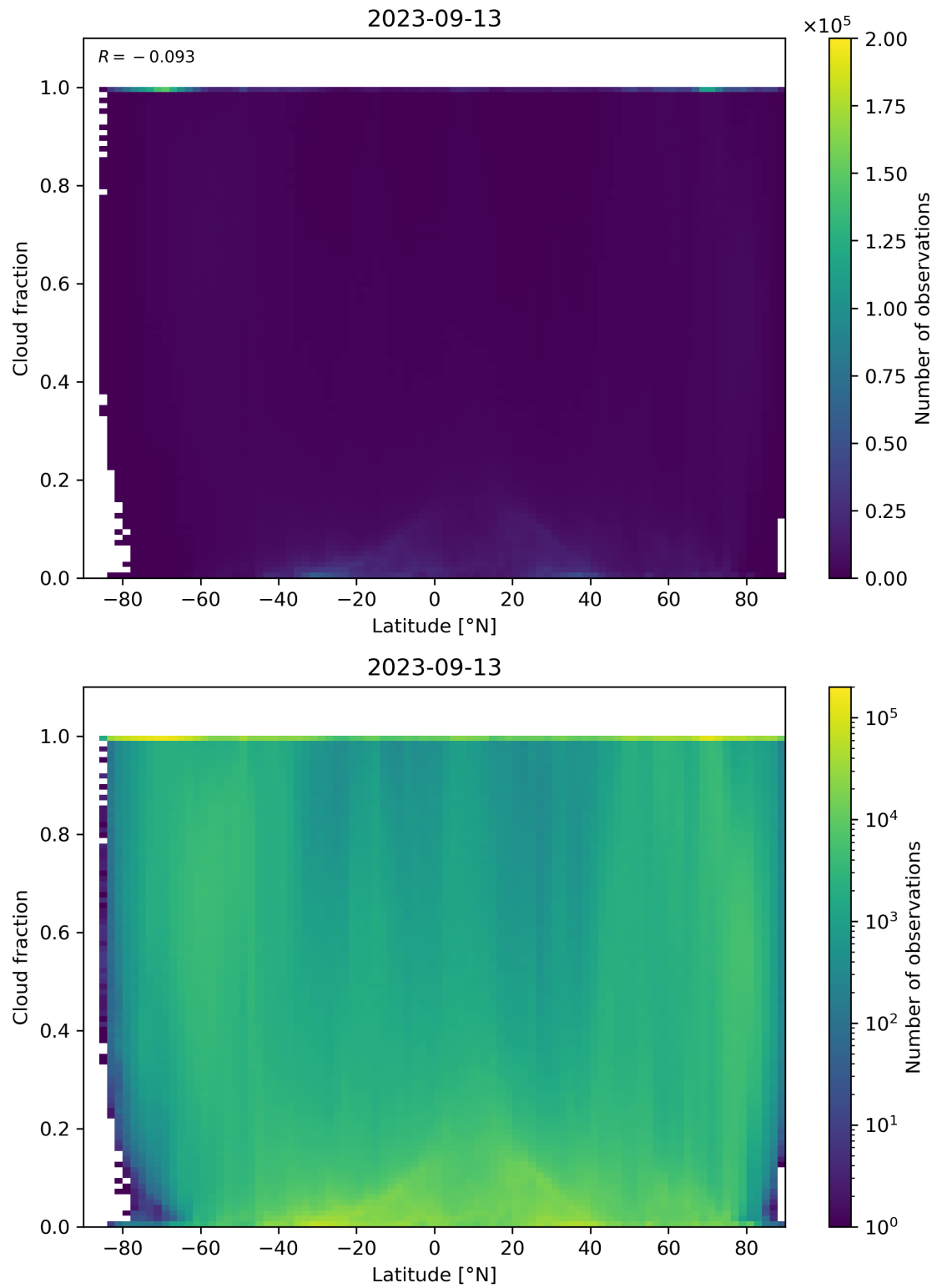
Figure 99: Scatter density plot of “Latitude” against “Cloud fraction” for 2023-09-12 to 2023-09-14.
