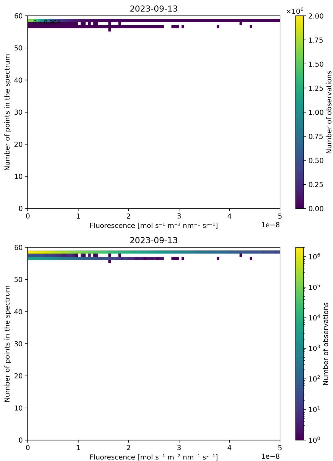
Figure 94: Scatter density plot of “Fluorescence” against “Number of points in the spectrum” for 2023-09-12 to 2023-09-14.
