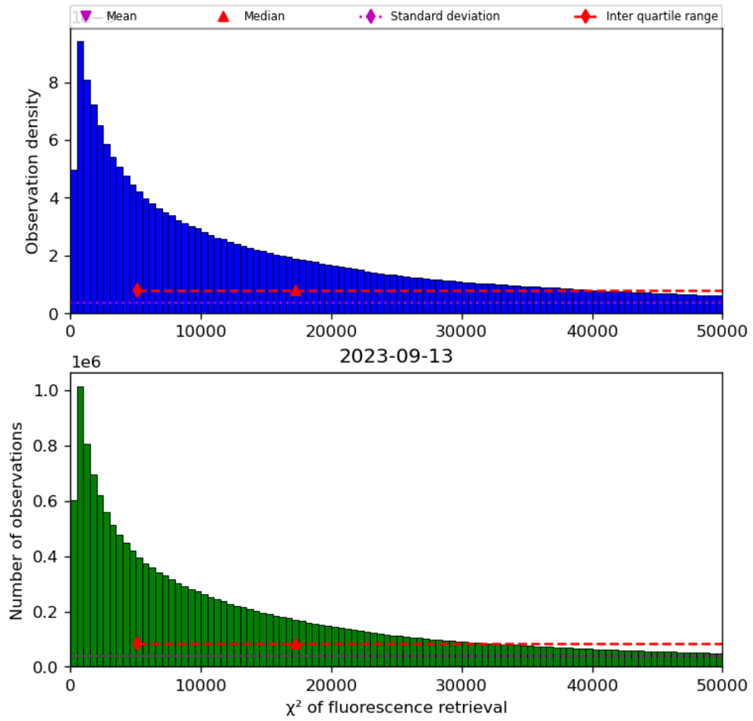
Figure 42: Histogram of “ \chi^2 of fluorescence retrieval” for 2023-09-12 to 2023-09-14
