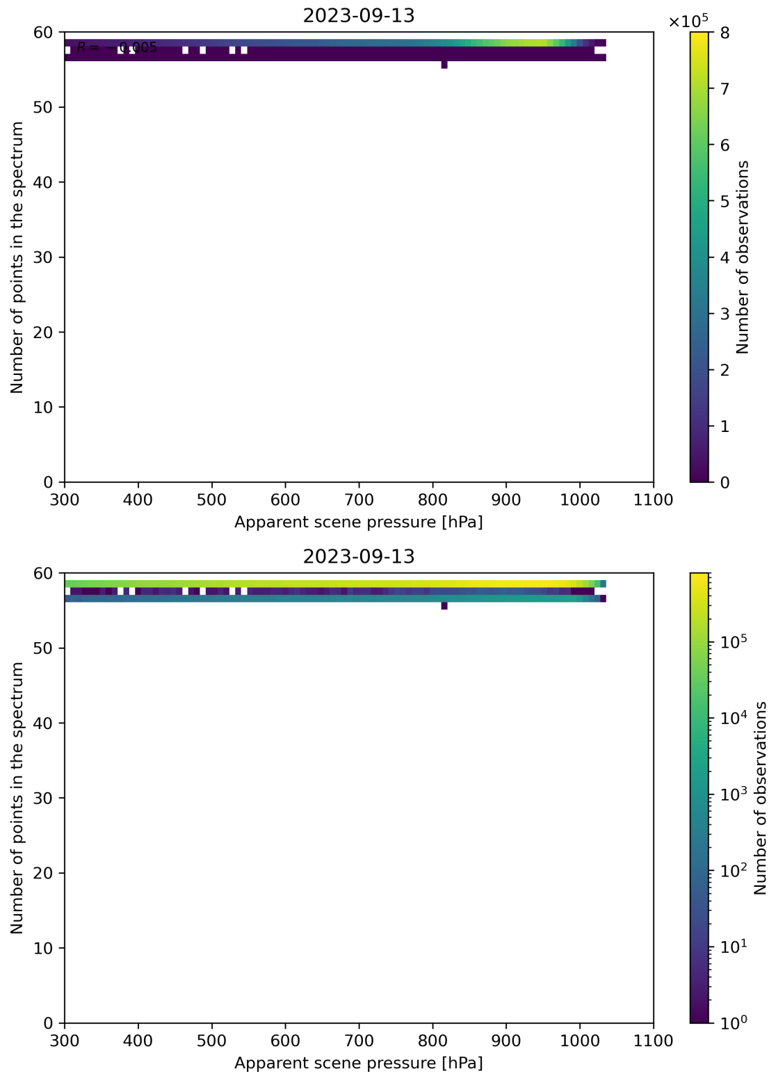
Figure 67: Scatter density plot of “Apparent scene pressure” against “Number of points in the spectrum” for 2023-09-12 to 2023-09-14.
