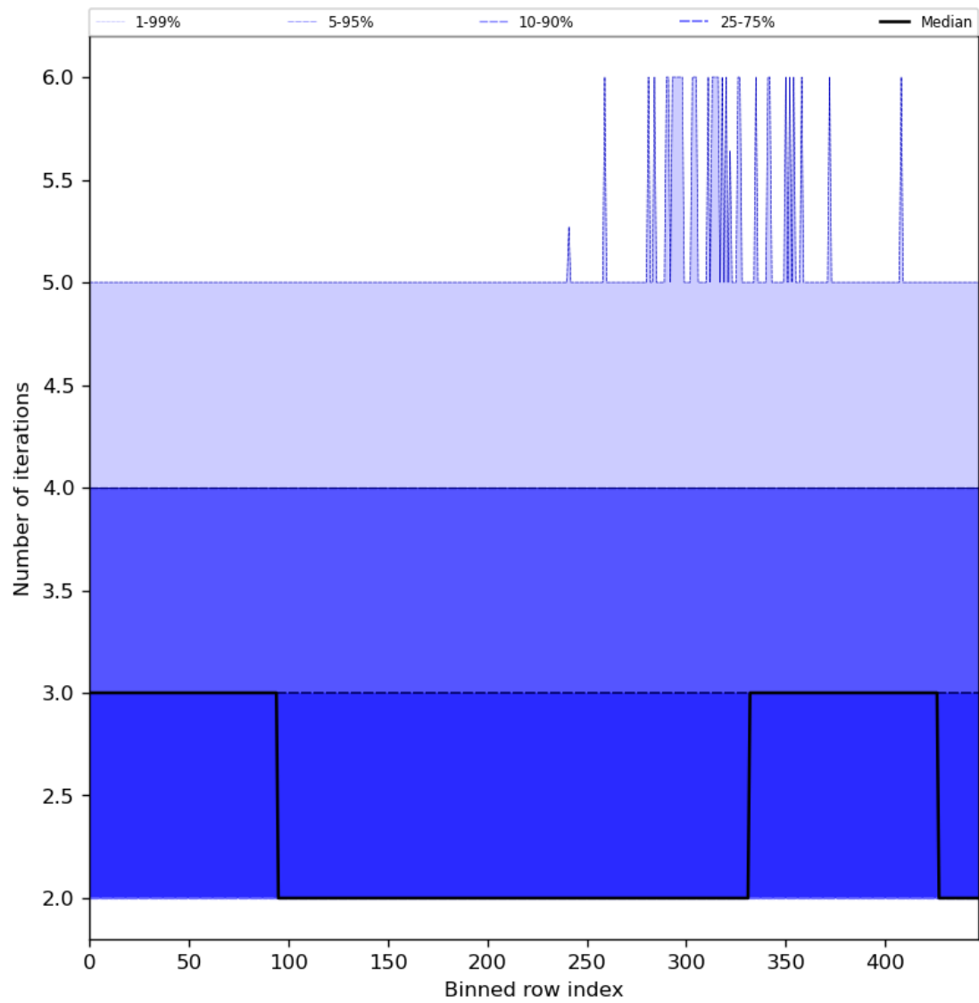
Figure 56: Along track statistics of “Number of iterations” for 2023-09-12 to 2023-09-14
