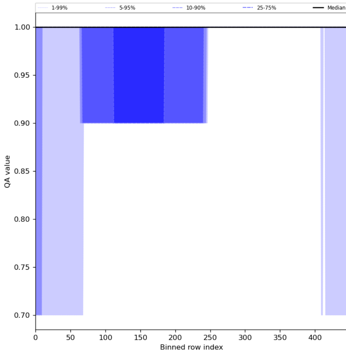
Figure 46: Along track statistics of “QA value” for 2023-09-12 to 2023-09-14
