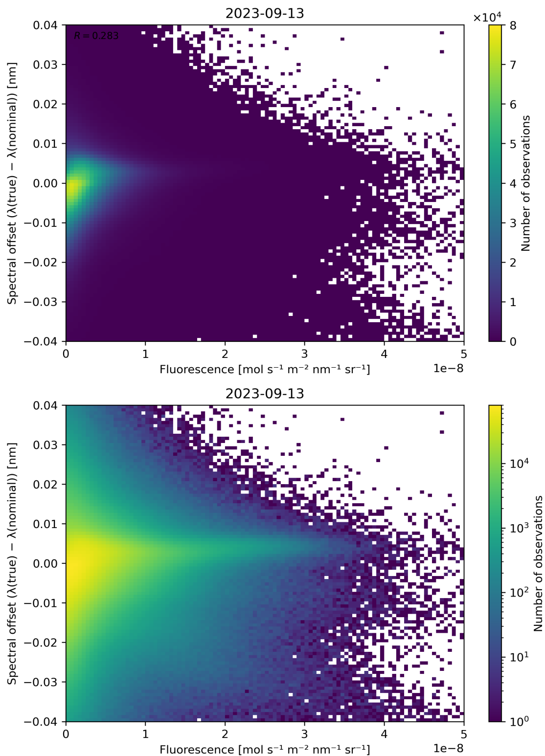
Figure 95: Scatter density plot of “Fluorescence” against “Spectral offset ( \lambda(\text{true}) - \lambda(\text{nominal}) )” for 2023-09-12 to 2023-09-14.
