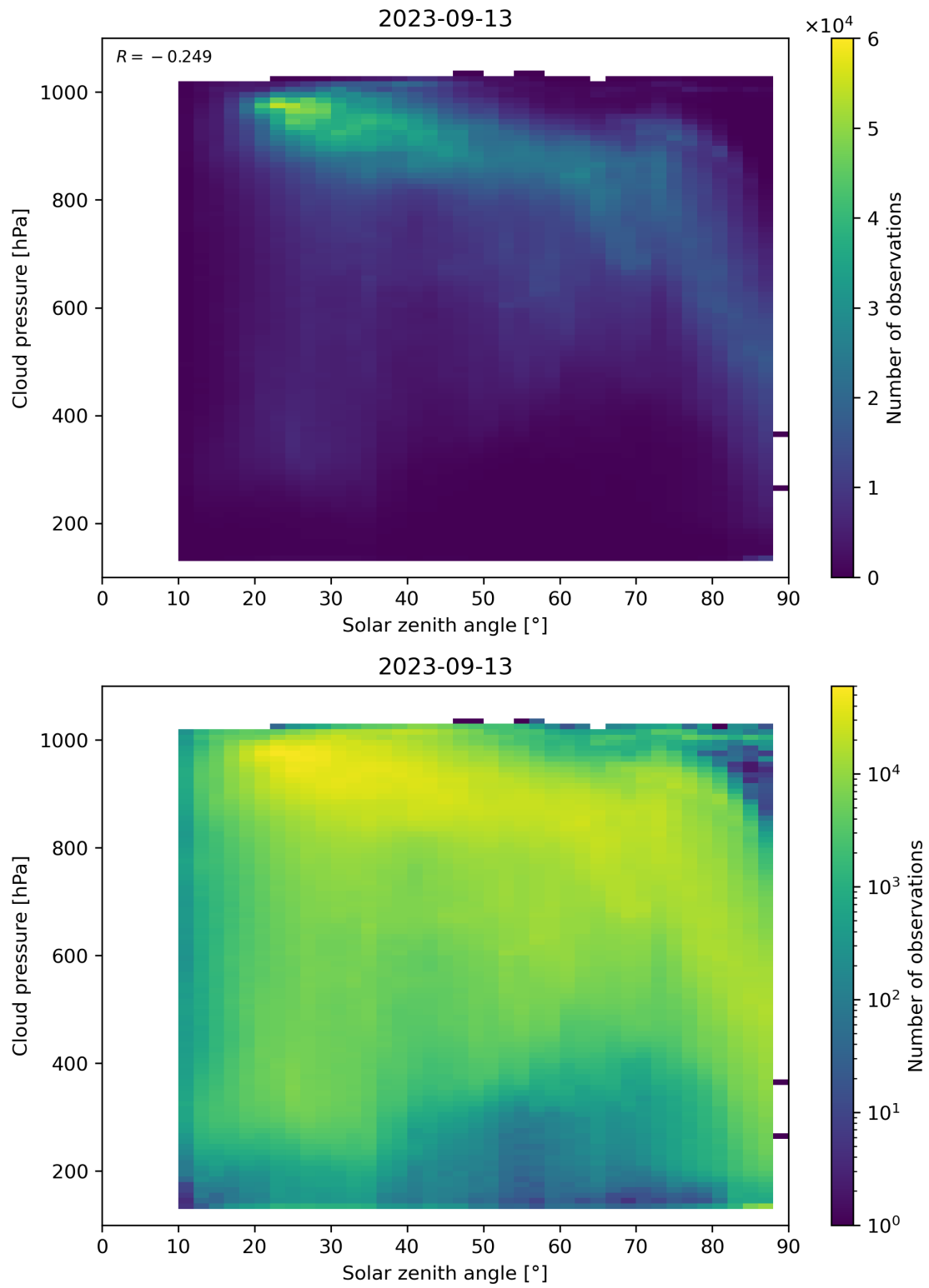
Figure 122: Scatter density plot of “Solar zenith angle” against “Cloud pressure” for 2023-09-12 to 2023-09-14.
