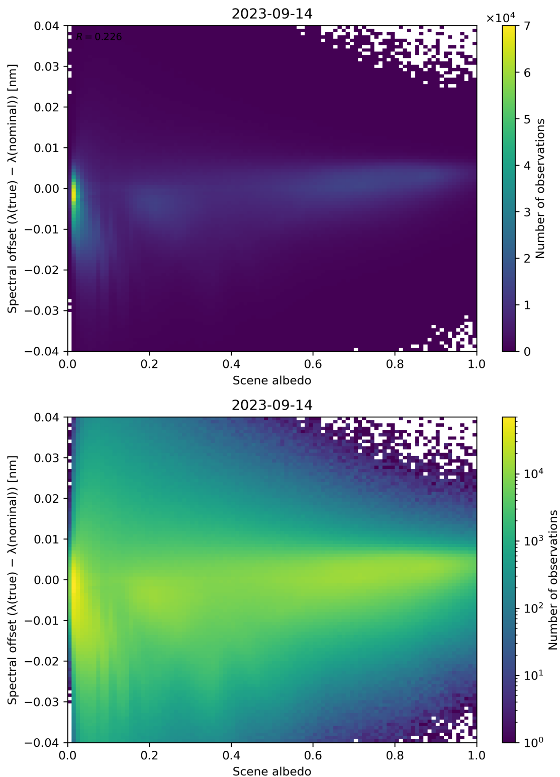
Figure 117: Scatter density plot of “Scene albedo” against “Spectral offset ( \lambda(\text{true}) - \lambda(\text{nominal}) )” for 2023-09-13 to 2023-09-15.
