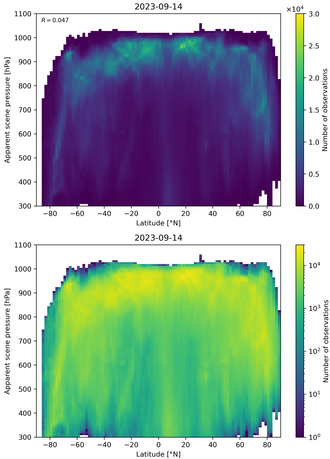
Figure 96: Scatter density plot of “Latitude” against “Apparent scene pressure” for 2023-09-13 to 2023-09-15.
