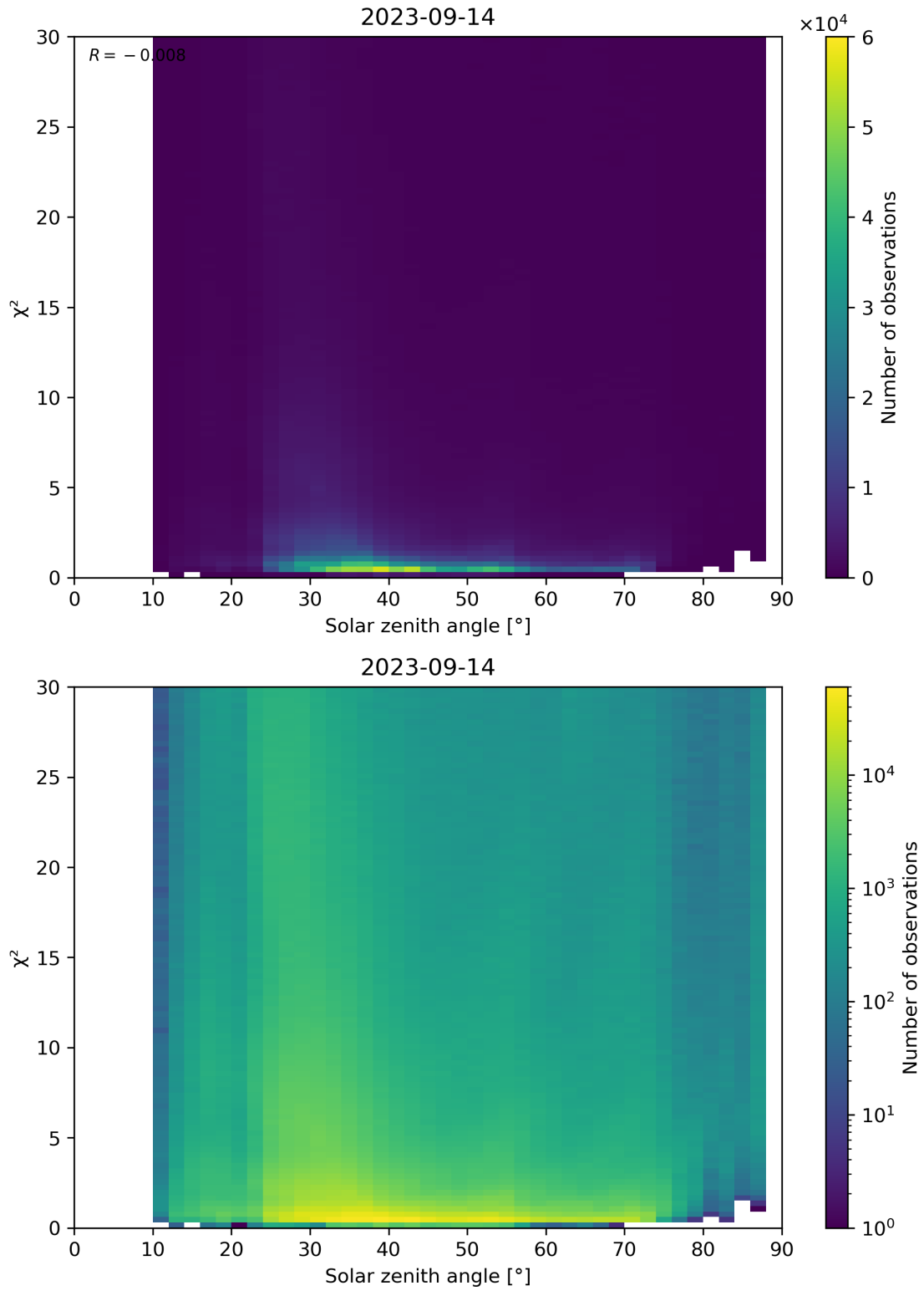
Figure 119: Scatter density plot of “Solar zenith angle” against “ \chi^2 ” for 2023-09-13 to 2023-09-15.
