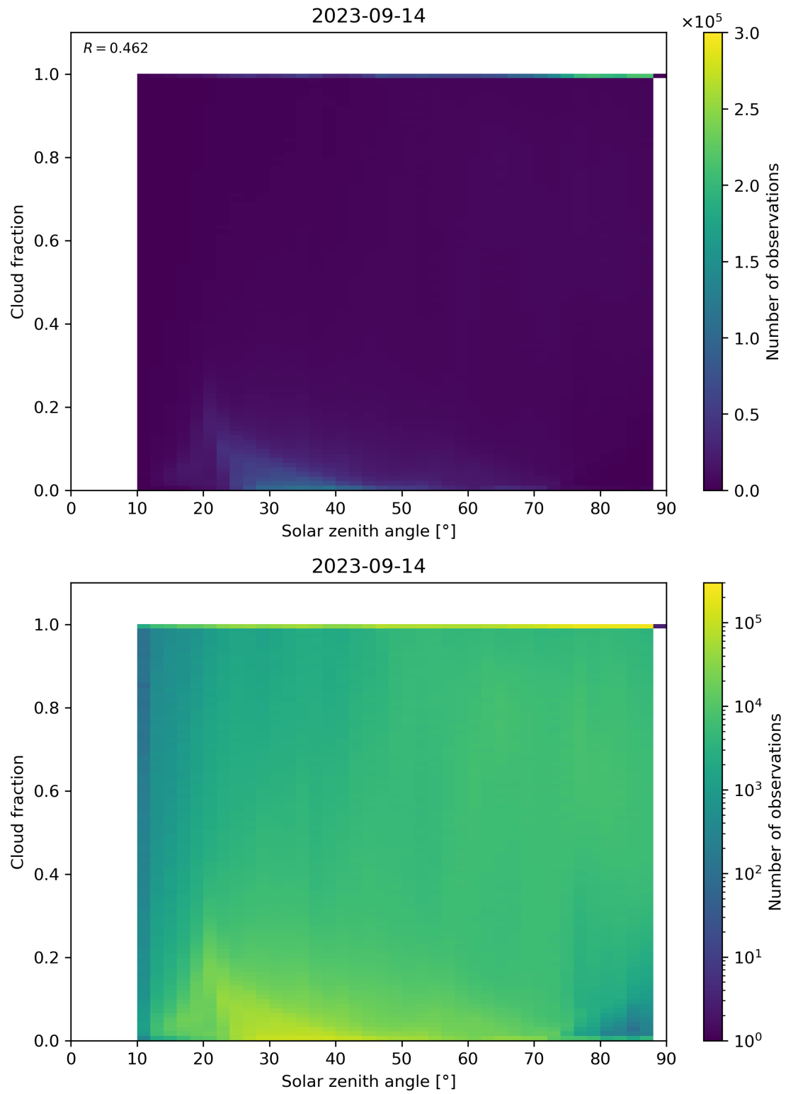
Figure 121: Scatter density plot of “Solar zenith angle” against “Cloud fraction” for 2023-09-13 to 2023-09-15.
