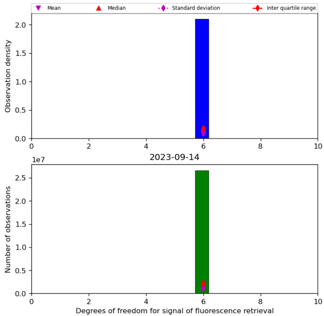
Figure 43: Histogram of “Degrees of freedom for signal of fluorescence retrieval” for 2023-09-13 to 2023-09-15
