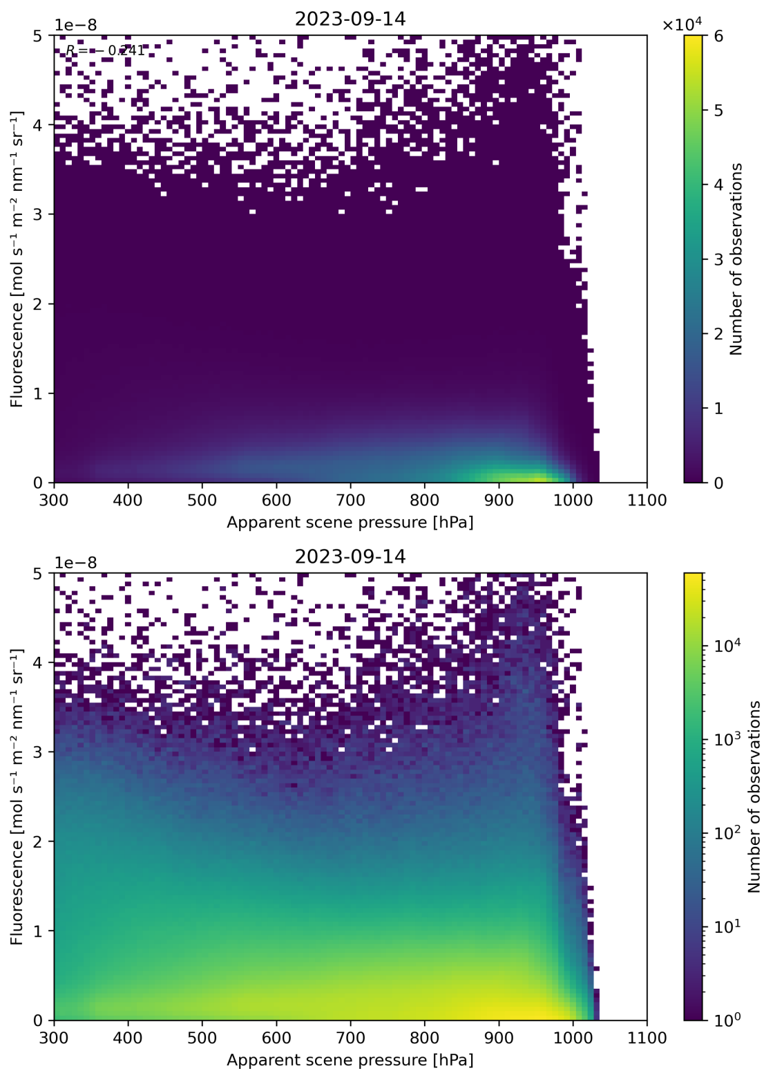
Figure 65: Scatter density plot of “Apparent scene pressure” against “Fluorescence” for 2023-09-13 to 2023-09-15.
