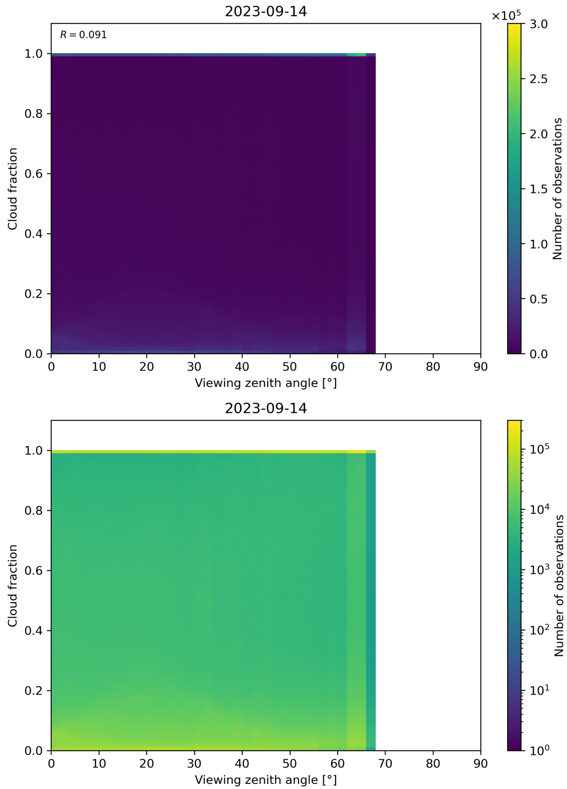
Figure 132: Scatter density plot of “Viewing zenith angle” against “Cloud fraction” for 2023-09-13 to 2023-09-15.
