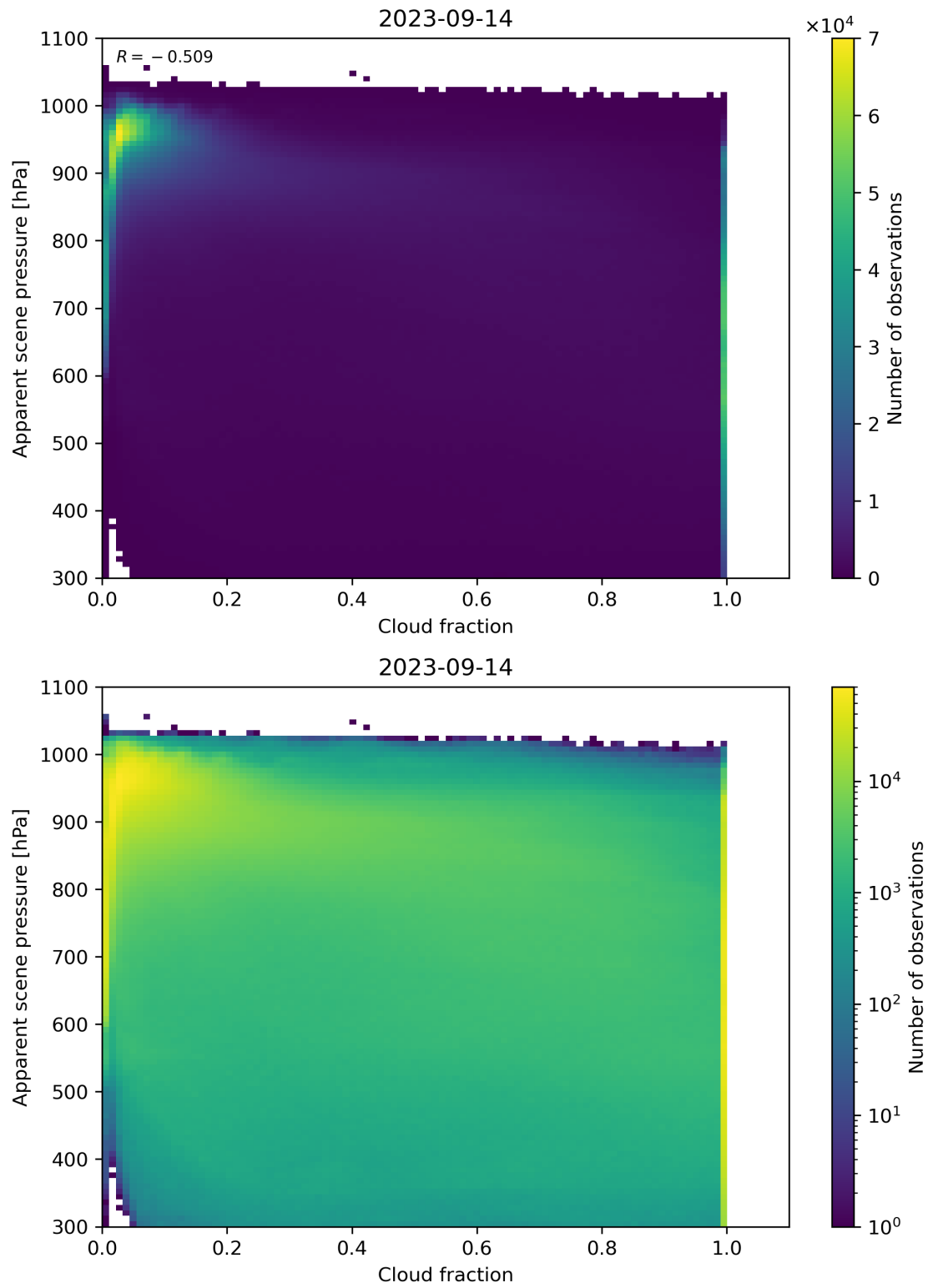
Figure 76: Scatter density plot of “Cloud fraction” against “Apparent scene pressure” for 2023-09-13 to 2023-09-15.
