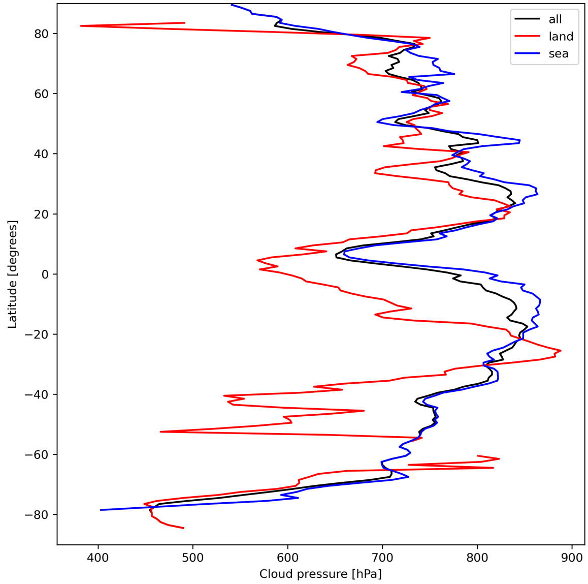
Figure 13: Zonal average of “Cloud pressure” for 2023-09-13 to 2023-09-15.
