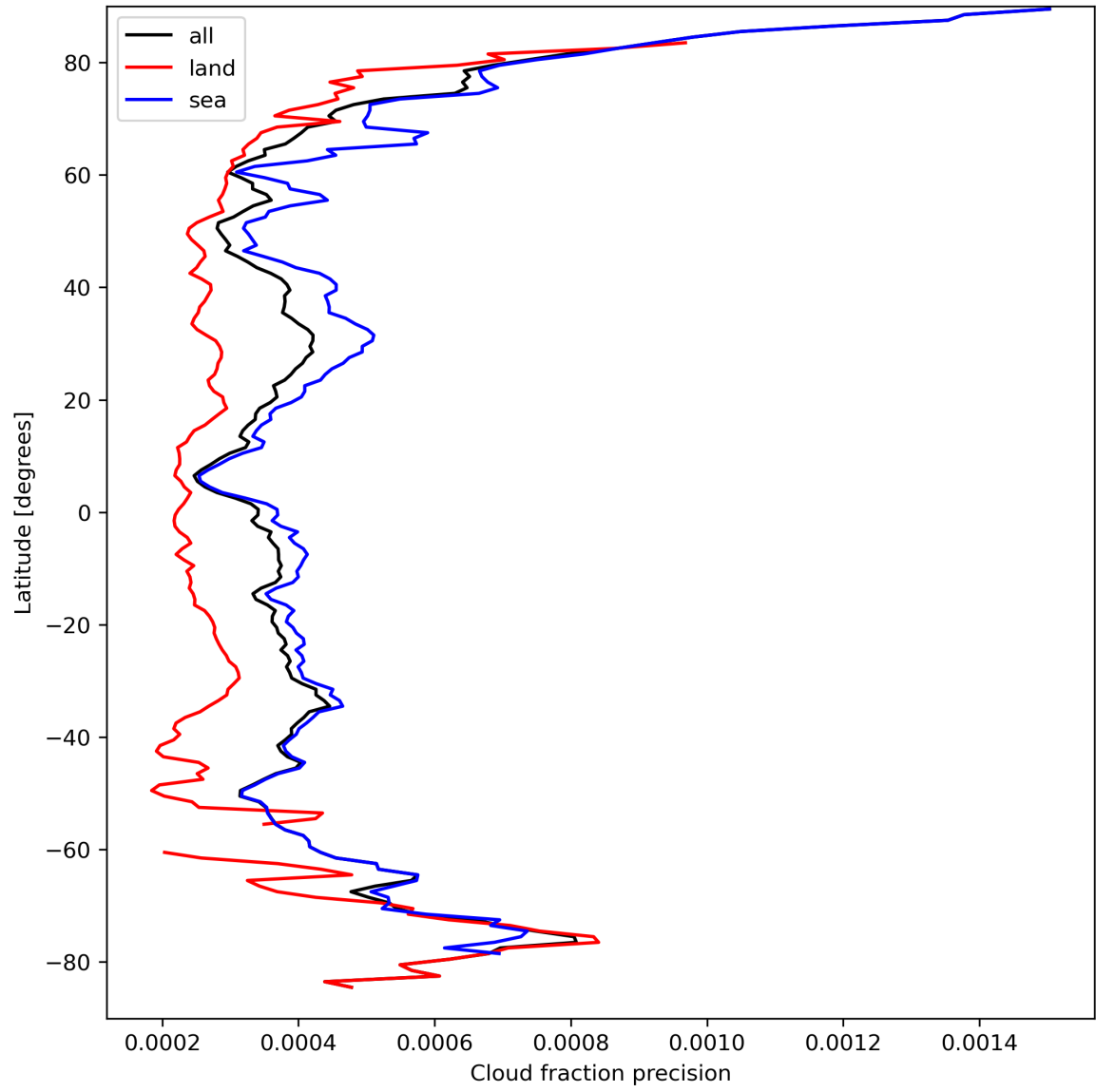
Figure 16: Zonal average of “Cloud fraction precision” for 2023-09-13 to 2023-09-15.
