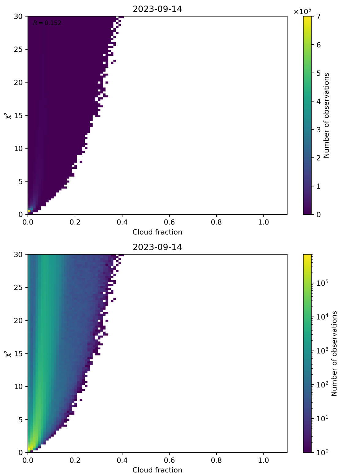
Figure 77: Scatter density plot of “Cloud fraction” against “ \chi^2 ” for 2023-09-13 to 2023-09-15.
