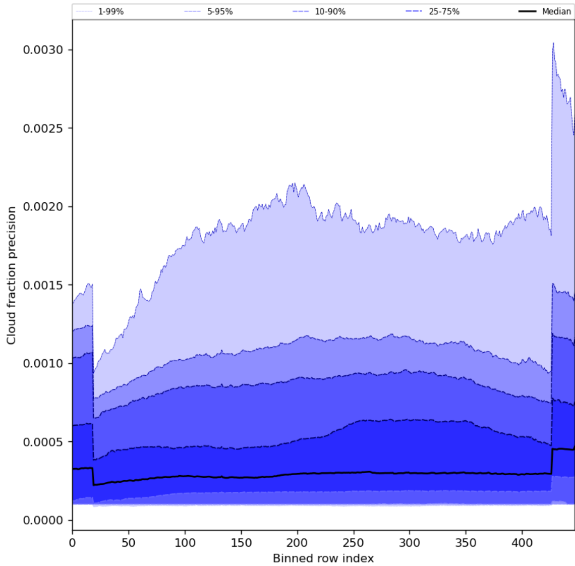
Figure 50: Along track statistics of “Cloud fraction precision” for 2023-09-13 to 2023-09-15
