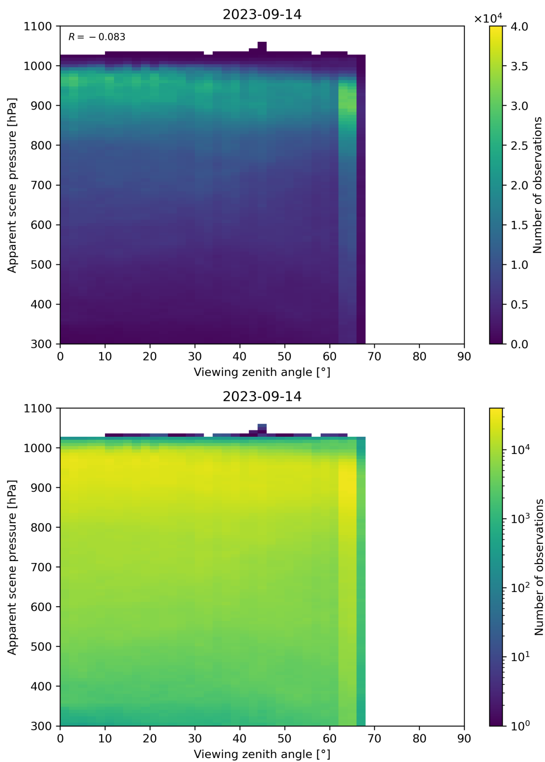
Figure 129: Scatter density plot of “Viewing zenith angle” against “Apparent scene pressure” for 2023-09-13 to 2023-09-15.
