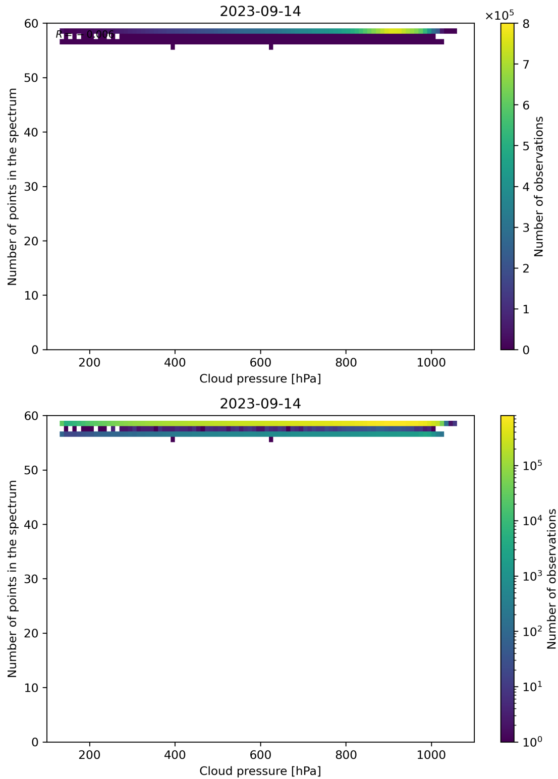
Figure 90: Scatter density plot of “Cloud pressure” against “Number of points in the spectrum” for 2023-09-13 to 2023-09-15.
