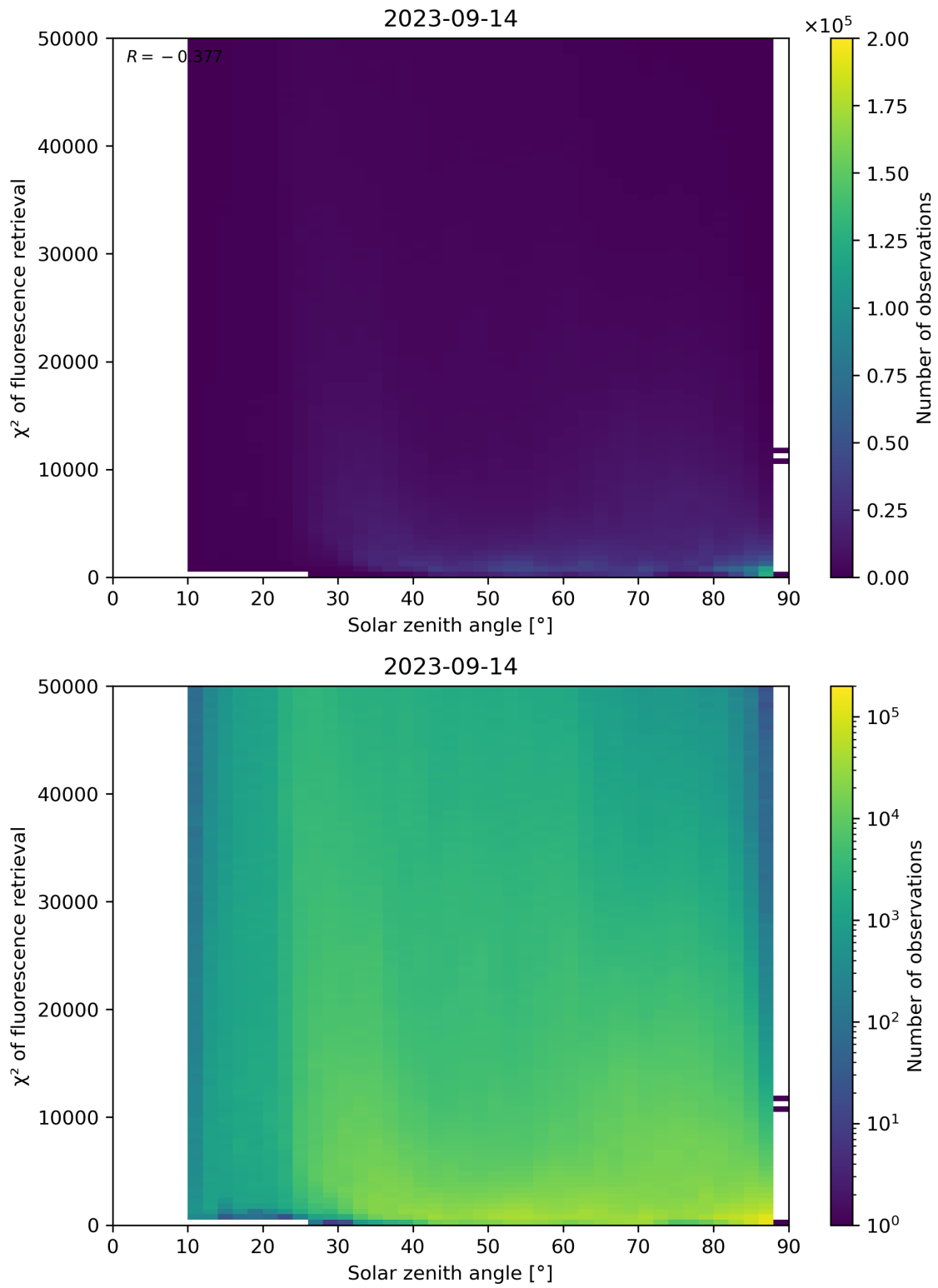
Figure 120: Scatter density plot of “Solar zenith angle” against “ \chi^2 of fluorescence retrieval” for 2023-09-13 to 2023-09-15.
