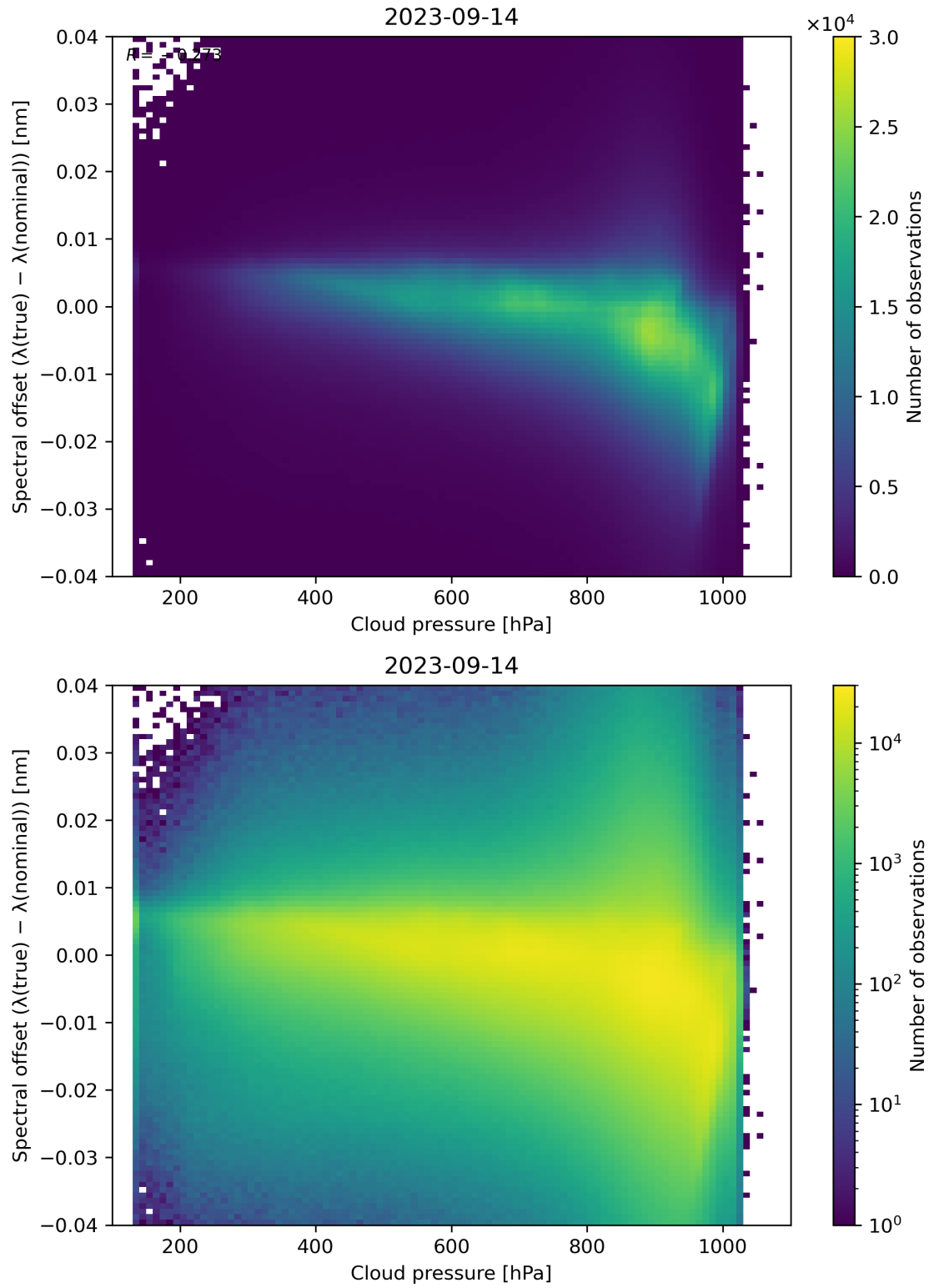
Figure 92: Scatter density plot of “Cloud pressure” against “Spectral offset ( \lambda(\text{true}) - \lambda(\text{nominal}) )” for 2023-09-13 to 2023-09-15.
