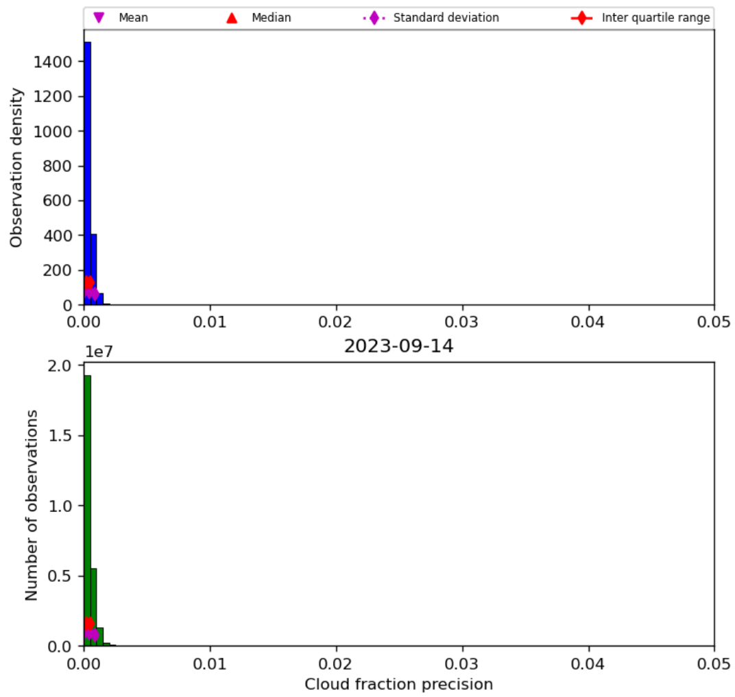
Figure 33: Histogram of “Cloud fraction precision” for 2023-09-13 to 2023-09-15
