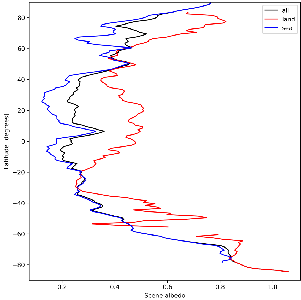
Figure 17: Zonal average of “Scene albedo” for 2023-09-13 to 2023-09-15.
