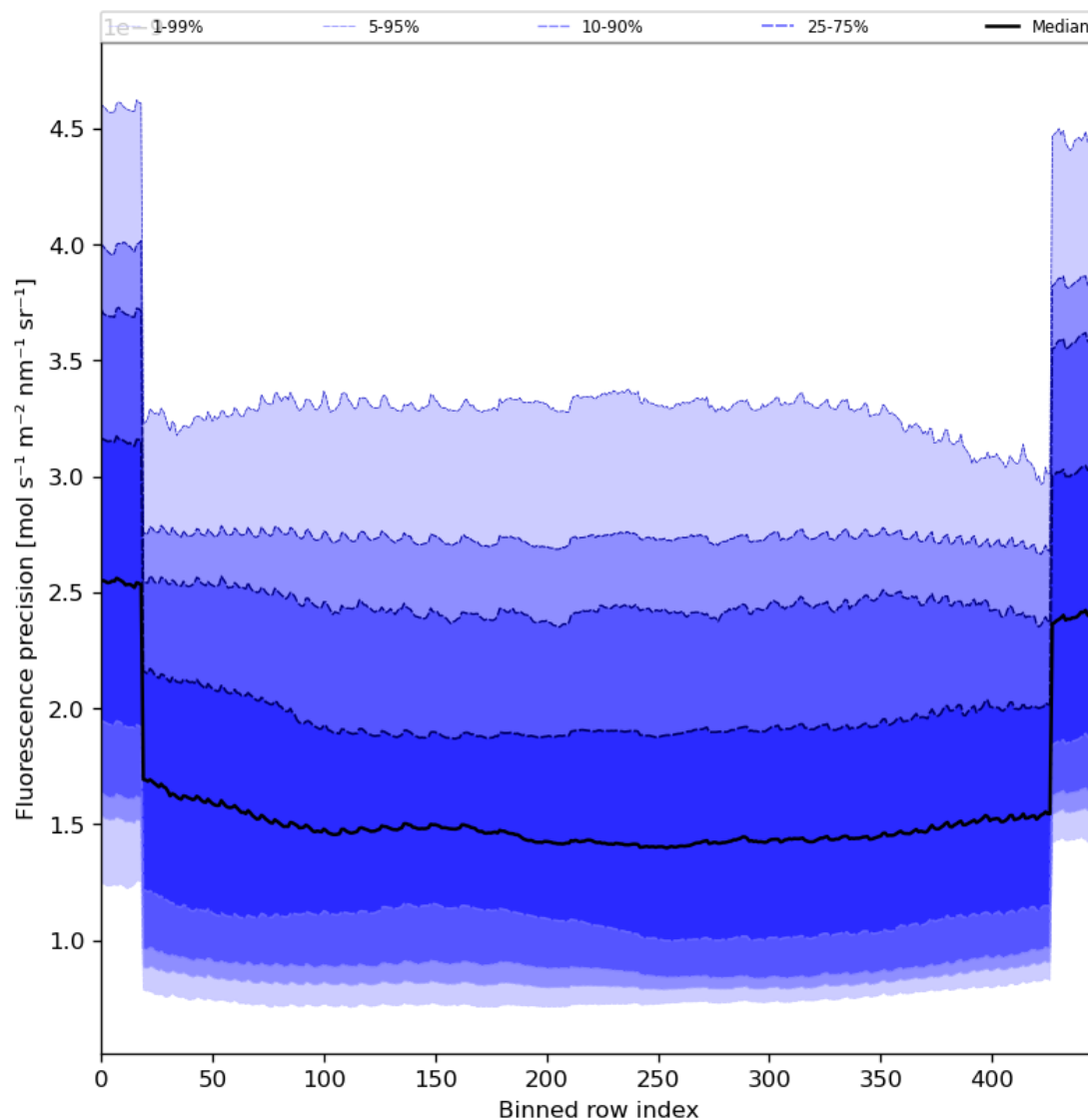
Figure 58: Along track statistics of “Fluorescence precision” for 2023-09-13 to 2023-09-15
