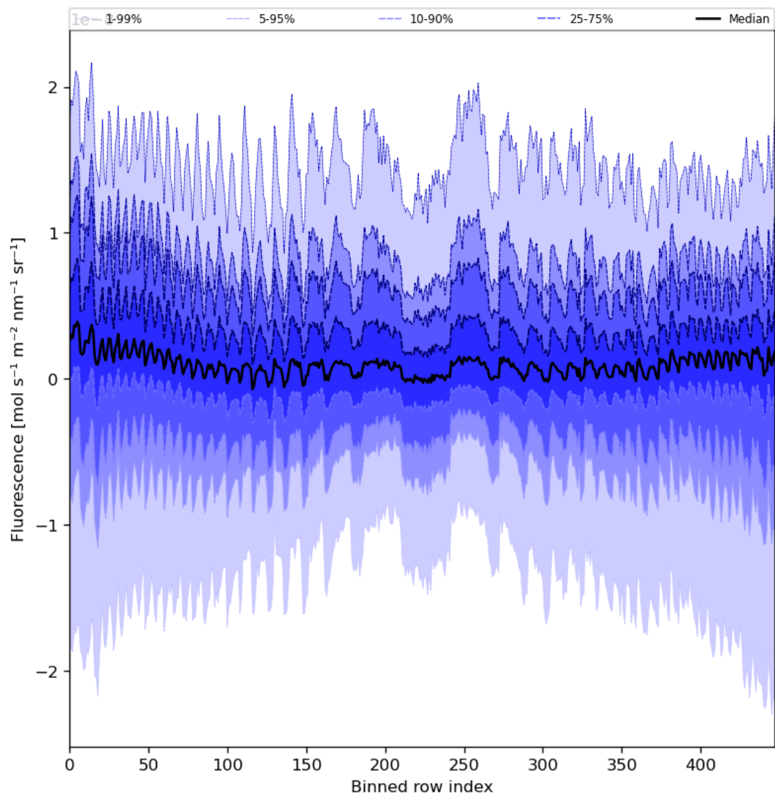
Figure 57: Along track statistics of “Fluorescence” for 2023-09-13 to 2023-09-15
