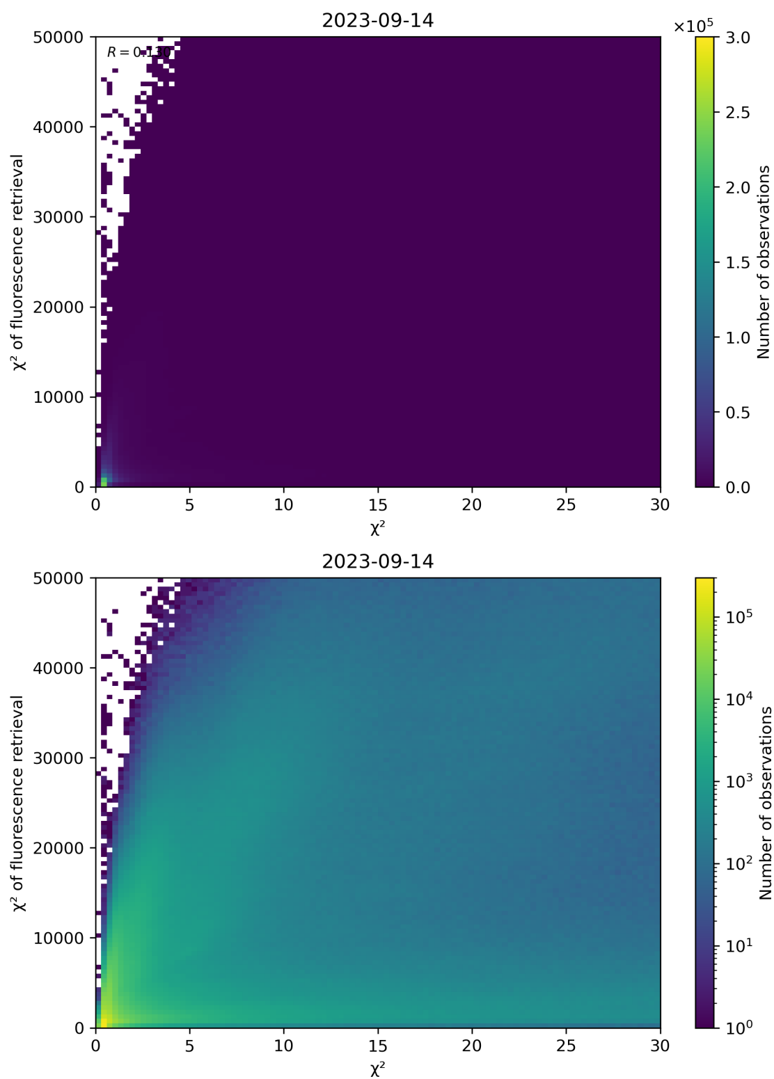
Figure 69: Scatter density plot of “ \chi^2 ” against “ \chi^2 of fluorescence retrieval” for 2023-09-13 to 2023-09-15.
