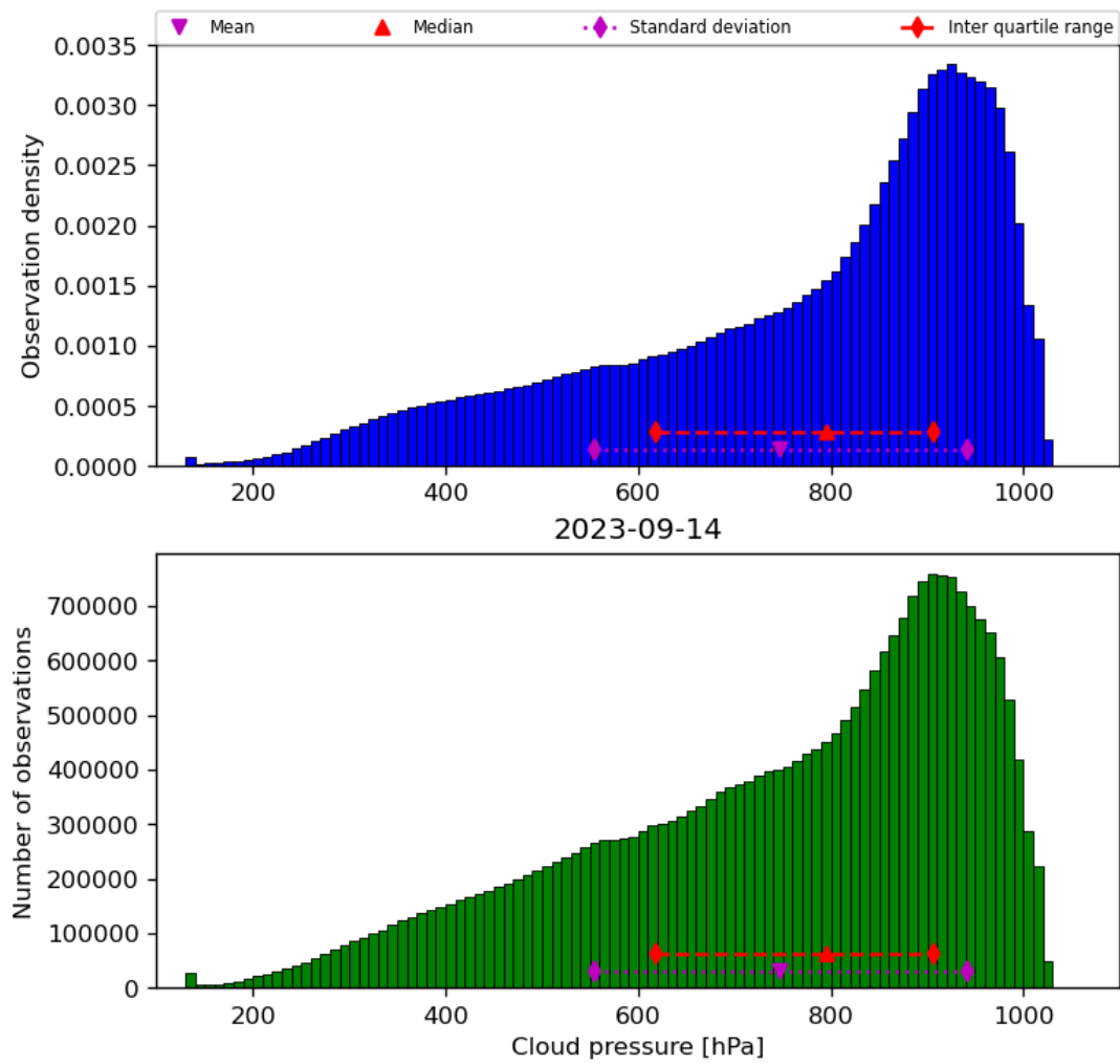
Figure 30: Histogram of “Cloud pressure” for 2023-09-13 to 2023-09-15
