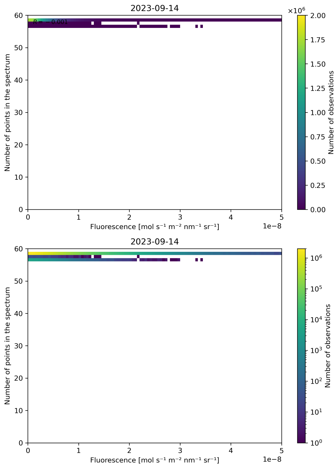
Figure 94: Scatter density plot of “Fluorescence” against “Number of points in the spectrum” for 2023-09-13 to 2023-09-15.
