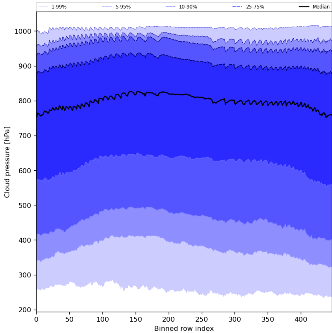
Figure 47: Along track statistics of “Cloud pressure” for 2023-09-13 to 2023-09-15
