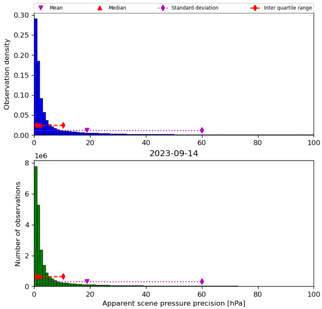
Figure 37: Histogram of “Apparent scene pressure precision” for 2023-09-13 to 2023-09-15
