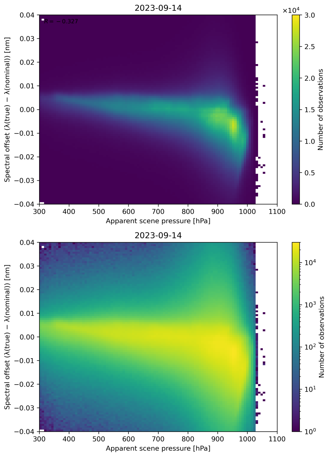
Figure 68: Scatter density plot of “Apparent scene pressure” against “Spectral offset ( \lambda(\text{true}) - \lambda(\text{nominal}) )” for 2023-09-13 to 2023-09-15.
