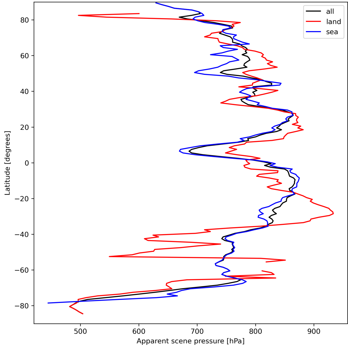
Figure 19: Zonal average of “Apparent scene pressure” for 2023-09-13 to 2023-09-15.
