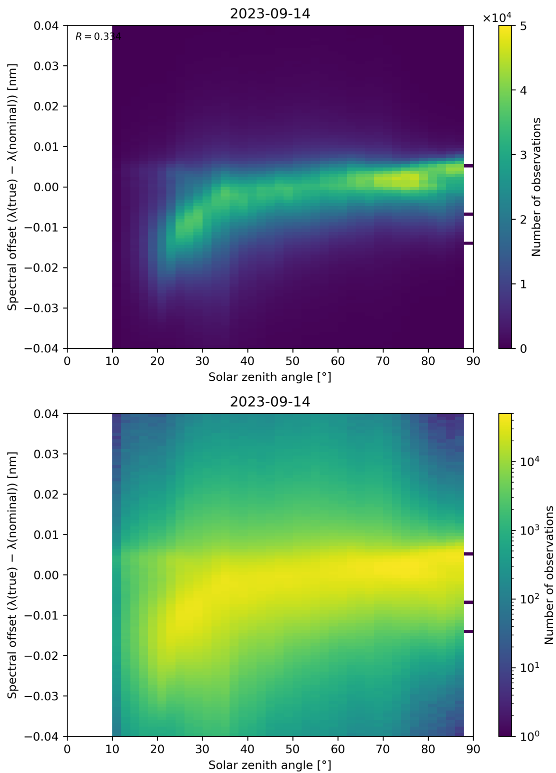
Figure 128: Scatter density plot of “Solar zenith angle” against “Spectral offset ( \lambda(\text{true}) - \lambda(\text{nominal}) )” for 2023-09-13 to 2023-09-15.
