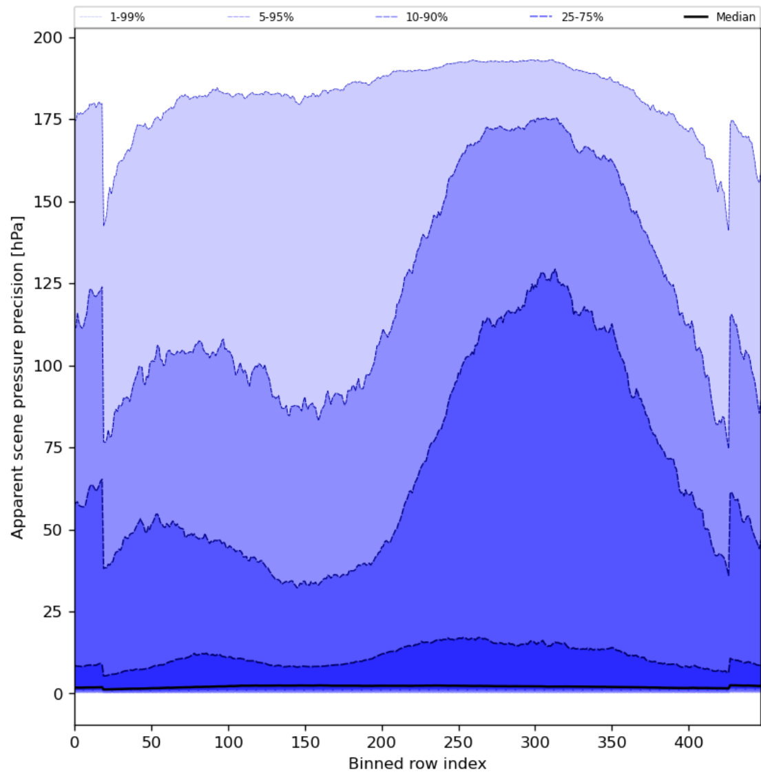
Figure 54: Along track statistics of “Apparent scene pressure precision” for 2023-09-13 to 2023-09-15
