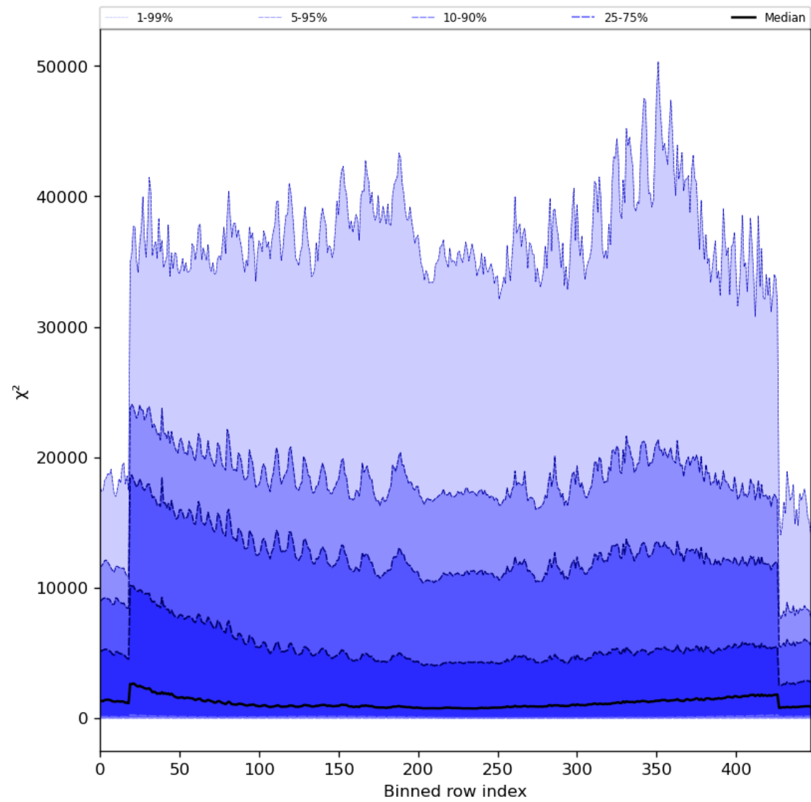
Figure 55: Along track statistics of “ \chi^2 ” for 2023-09-13 to 2023-09-15
