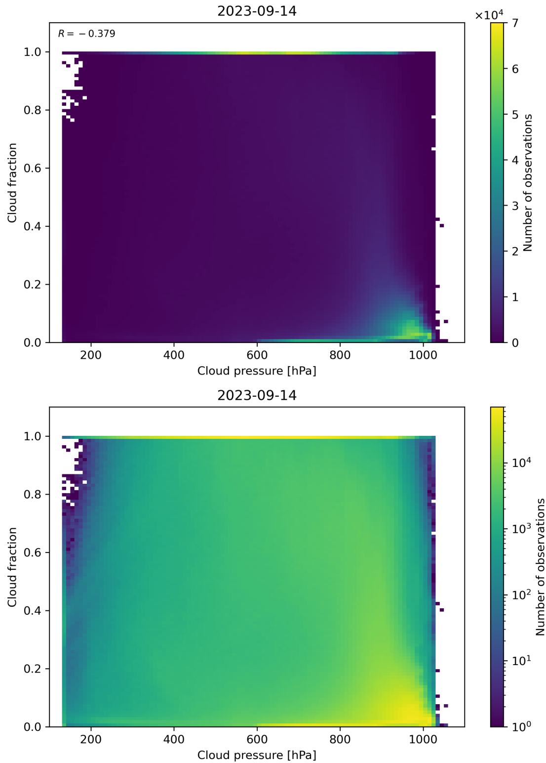
Figure 87: Scatter density plot of “Cloud pressure” against “Cloud fraction” for 2023-09-13 to 2023-09-15.
