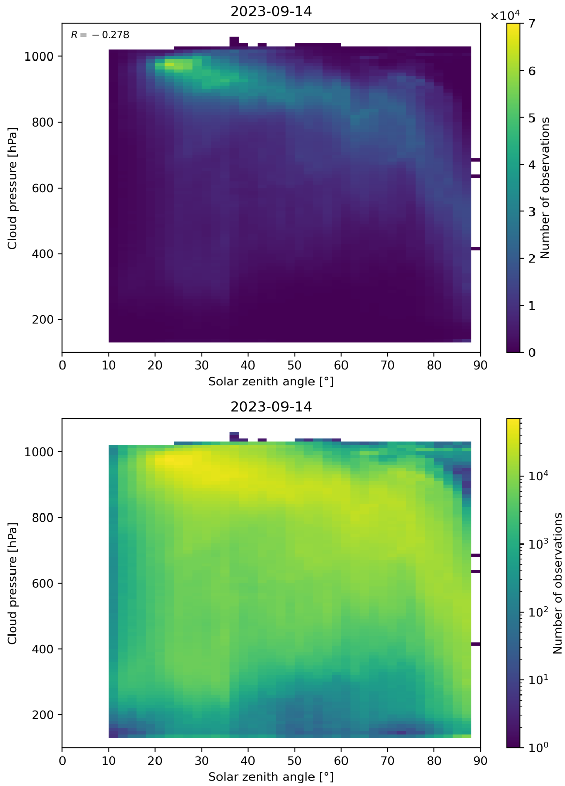
Figure 122: Scatter density plot of “Solar zenith angle” against “Cloud pressure” for 2023-09-13 to 2023-09-15.
