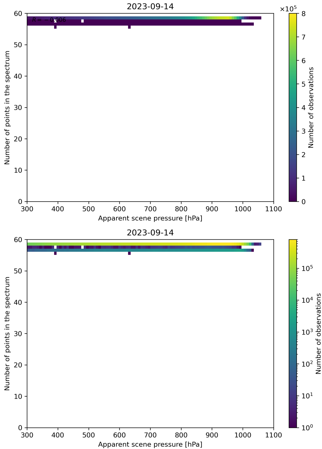
Figure 67: Scatter density plot of “Apparent scene pressure” against “Number of points in the spectrum” for 2023-09-13 to 2023-09-15.
