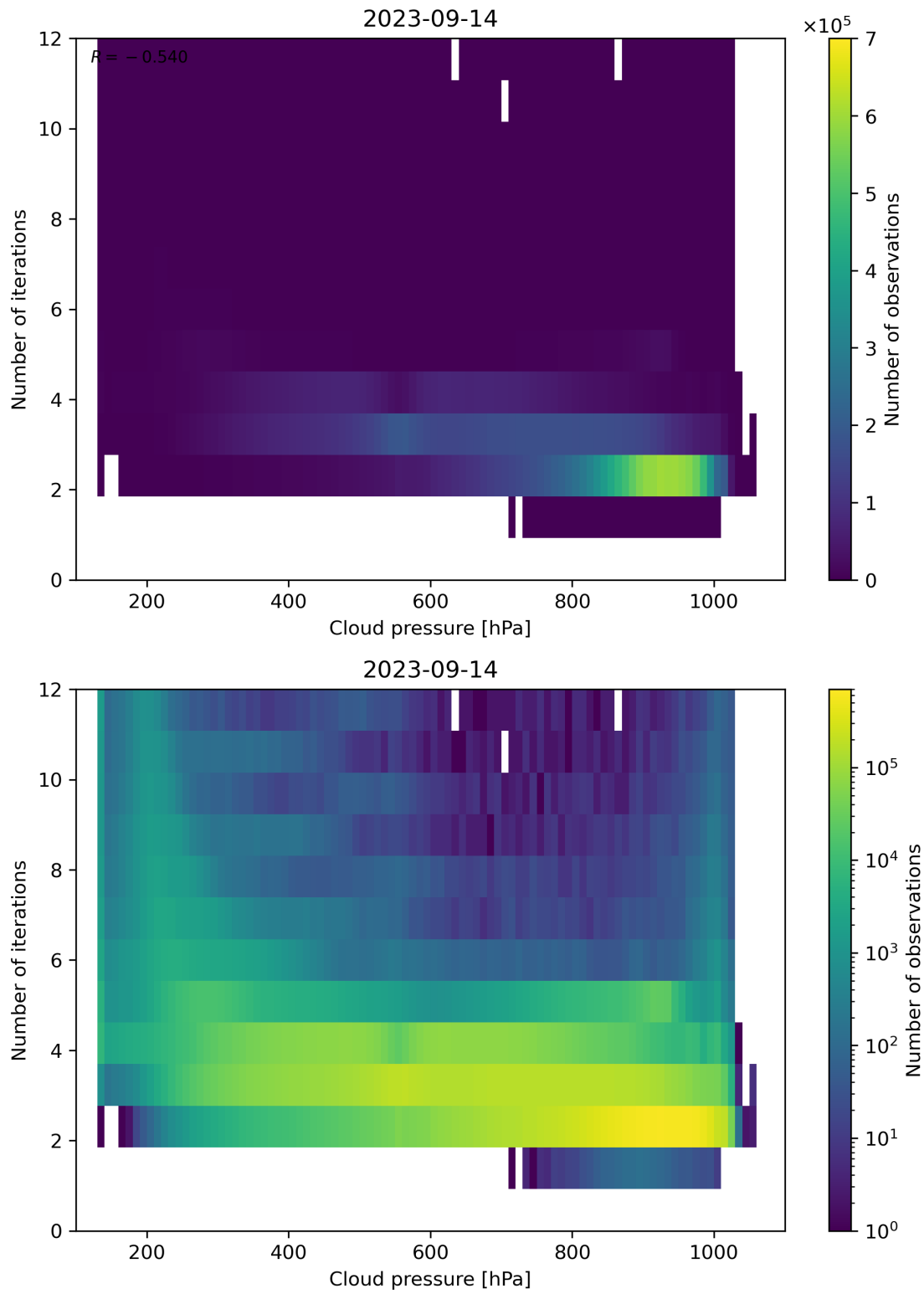
Figure 89: Scatter density plot of “Cloud pressure” against “Number of iterations” for 2023-09-13 to 2023-09-15.
