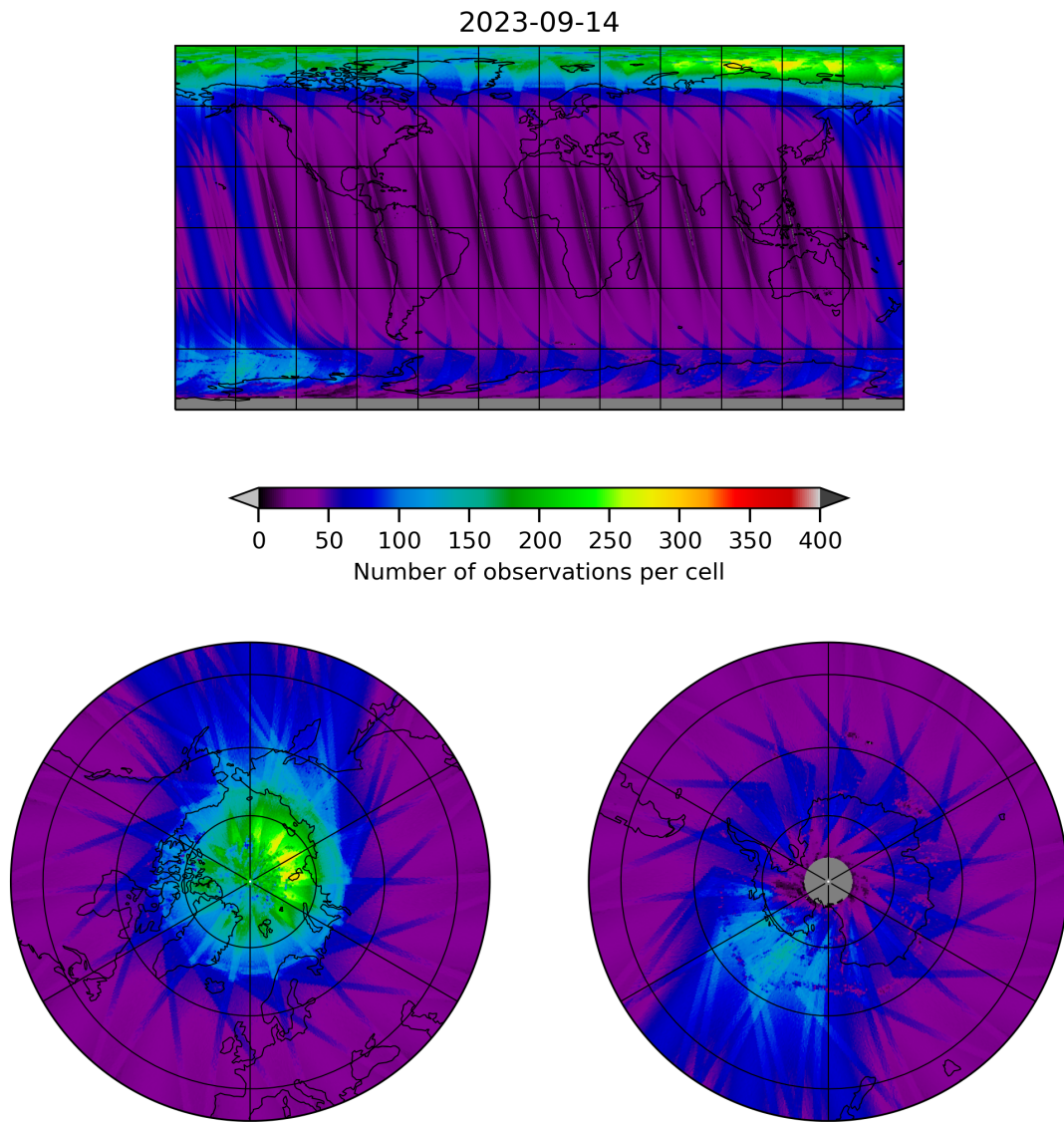
Figure 11: Map of the number of observations for 2023-09-13 to 2023-09-15
