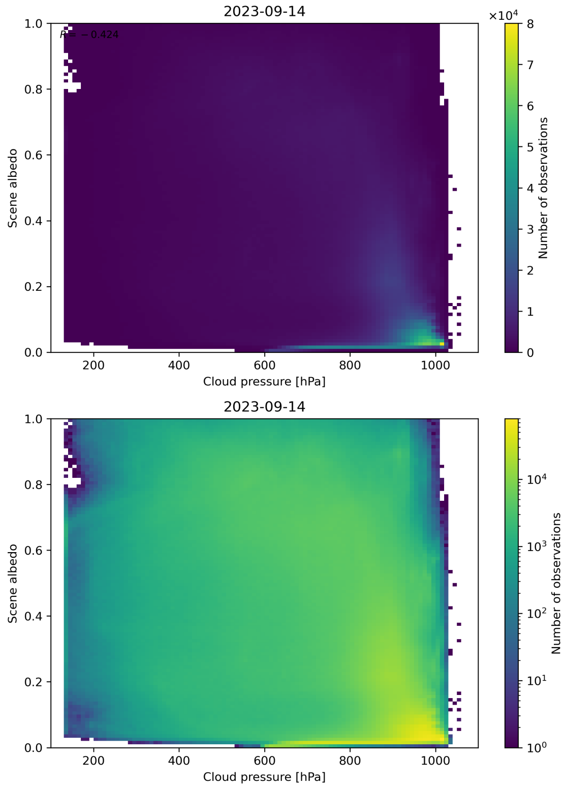
Figure 91: Scatter density plot of “Cloud pressure” against “Scene albedo” for 2023-09-13 to 2023-09-15.
