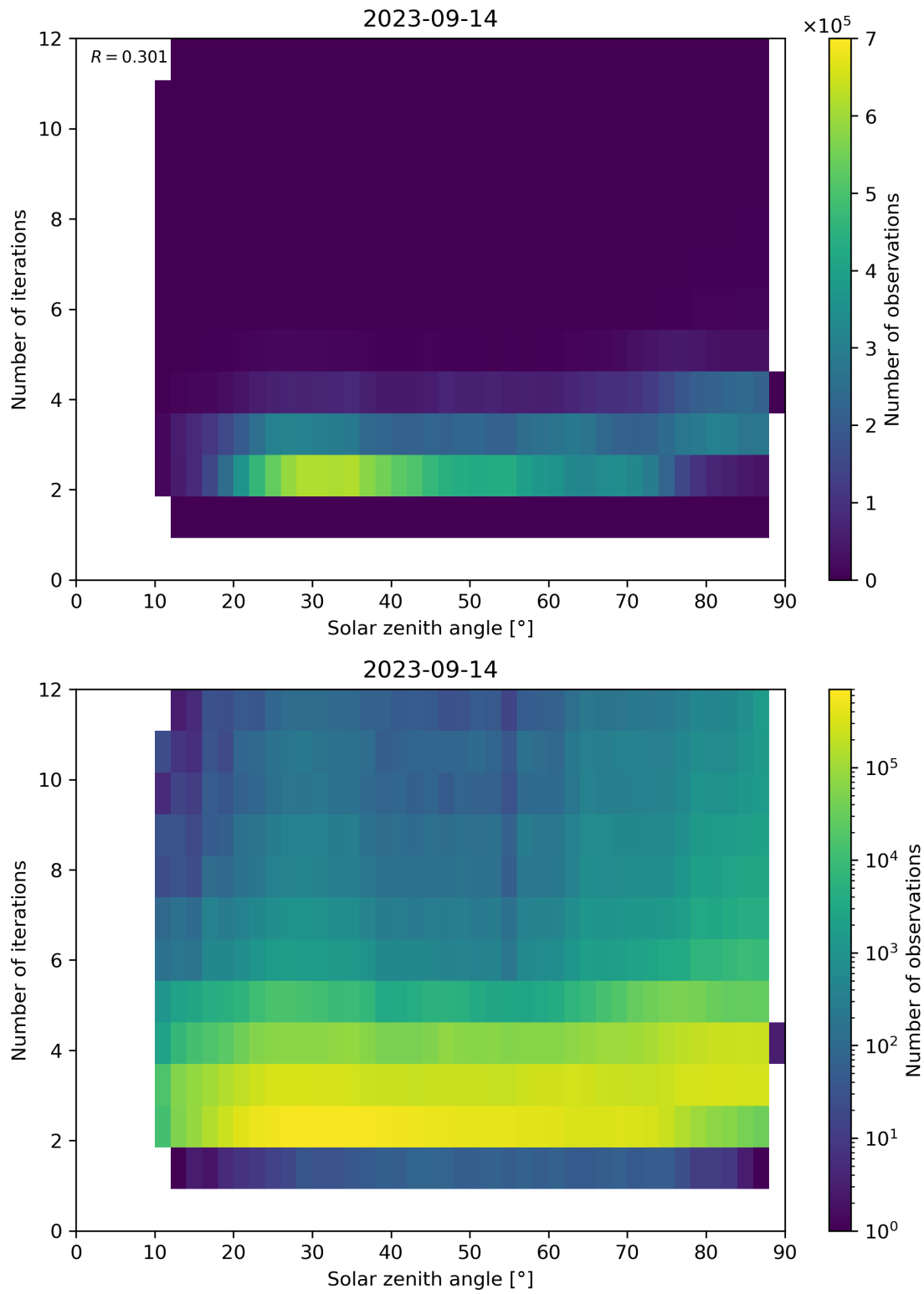
Figure 125: Scatter density plot of “Solar zenith angle” against “Number of iterations” for 2023-09-13 to 2023-09-15.
