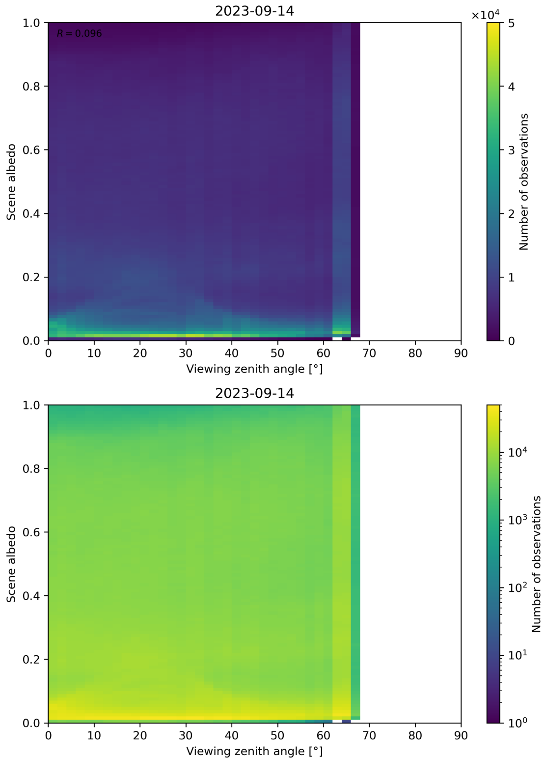
Figure 138: Scatter density plot of “Viewing zenith angle” against “Scene albedo” for 2023-09-13 to 2023-09-15.
