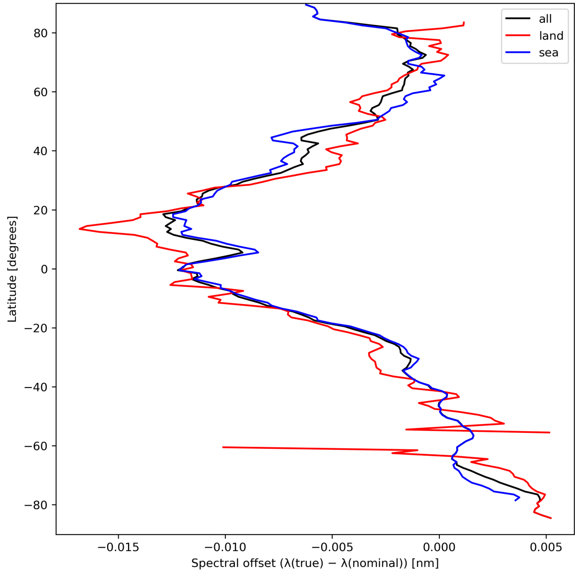
Figure 28: Zonal average of “Spectral offset ( \lambda(\text{true}) - \lambda(\text{nominal}) )” for 2023-09-13 to 2023-09-15.
