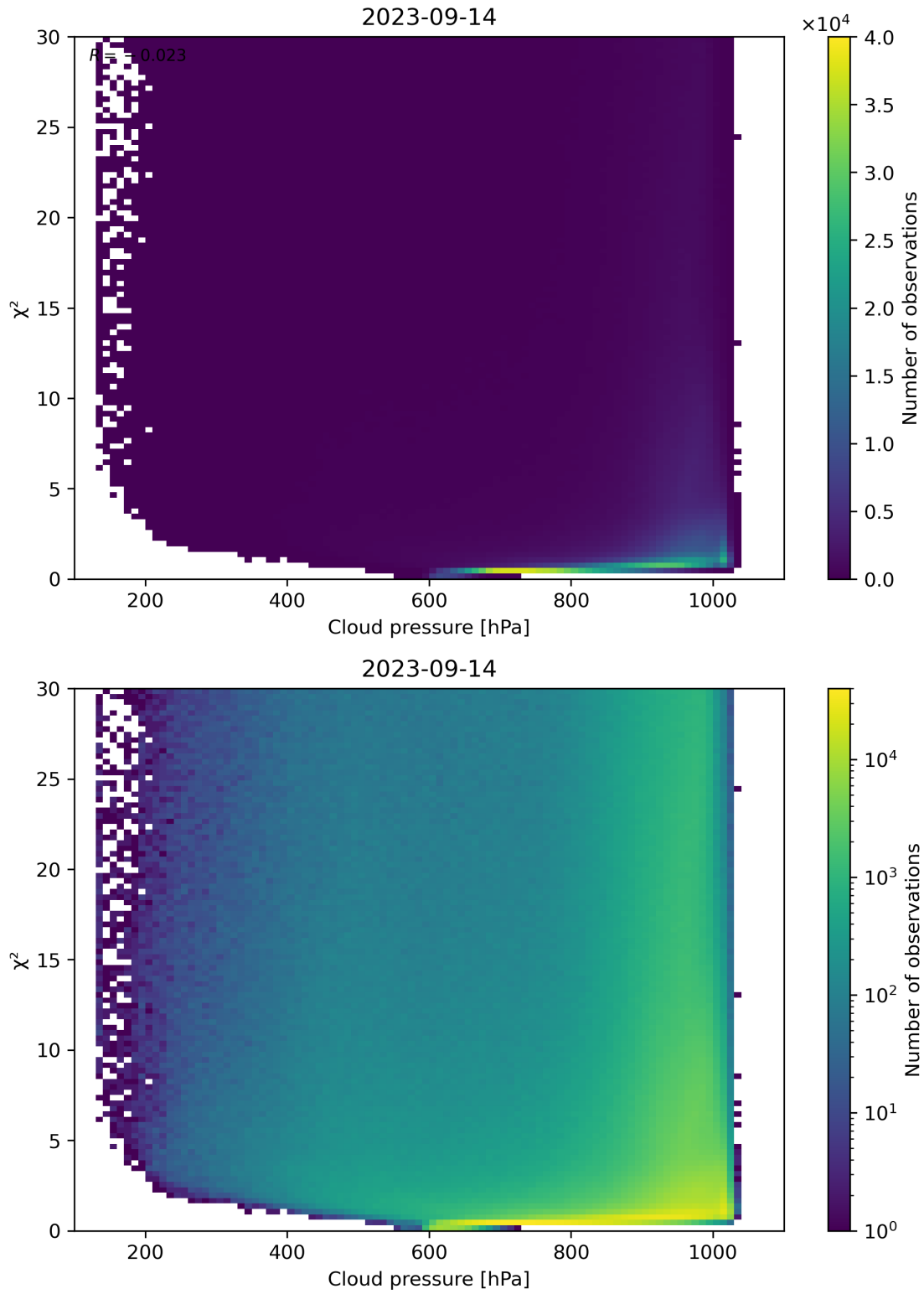
Figure 85: Scatter density plot of “Cloud pressure” against “ \chi^2 ” for 2023-09-13 to 2023-09-15.
