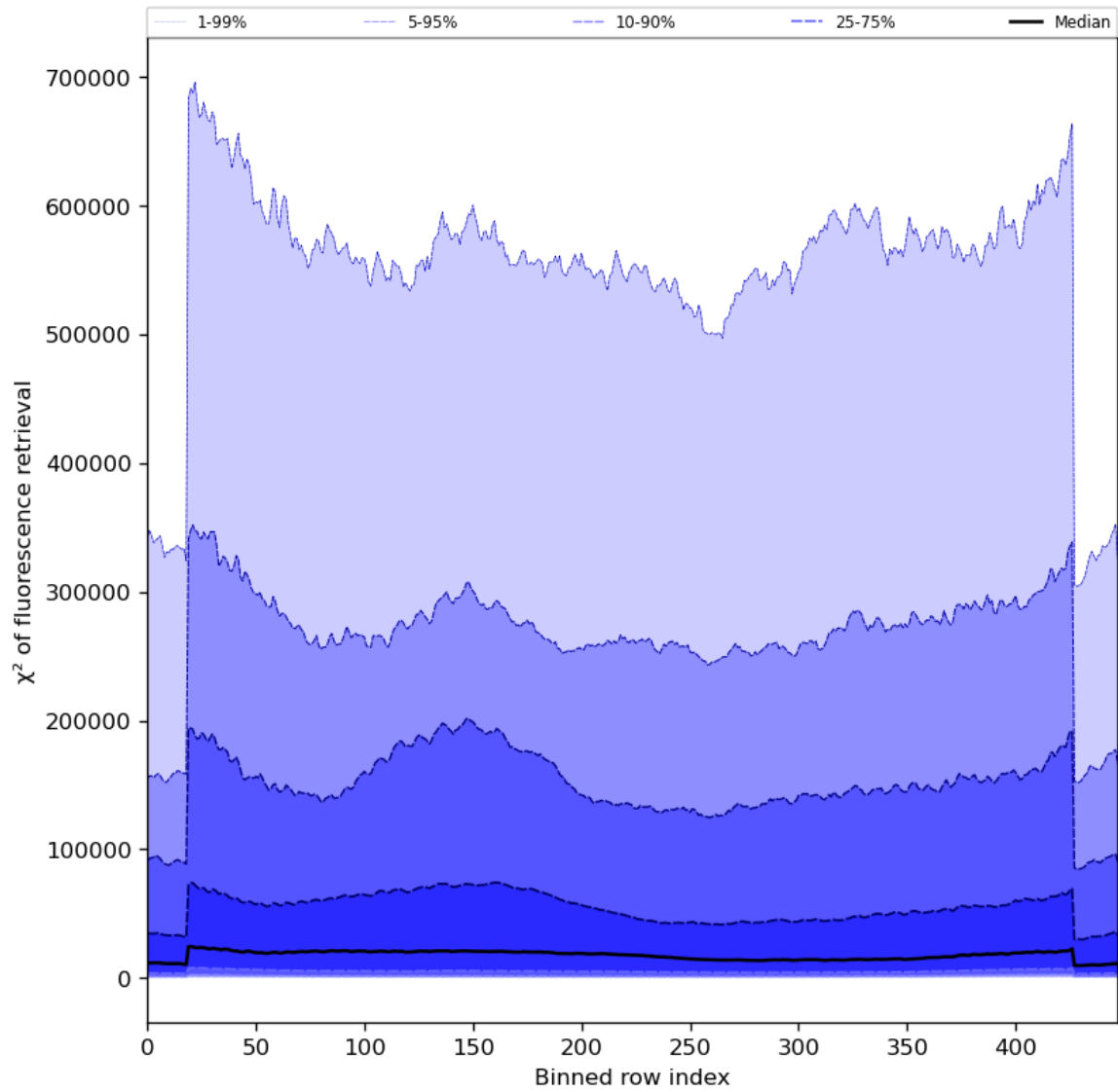
Figure 59: Along track statistics of “ \chi^2 of fluorescence retrieval” for 2023-09-13 to 2023-09-15
