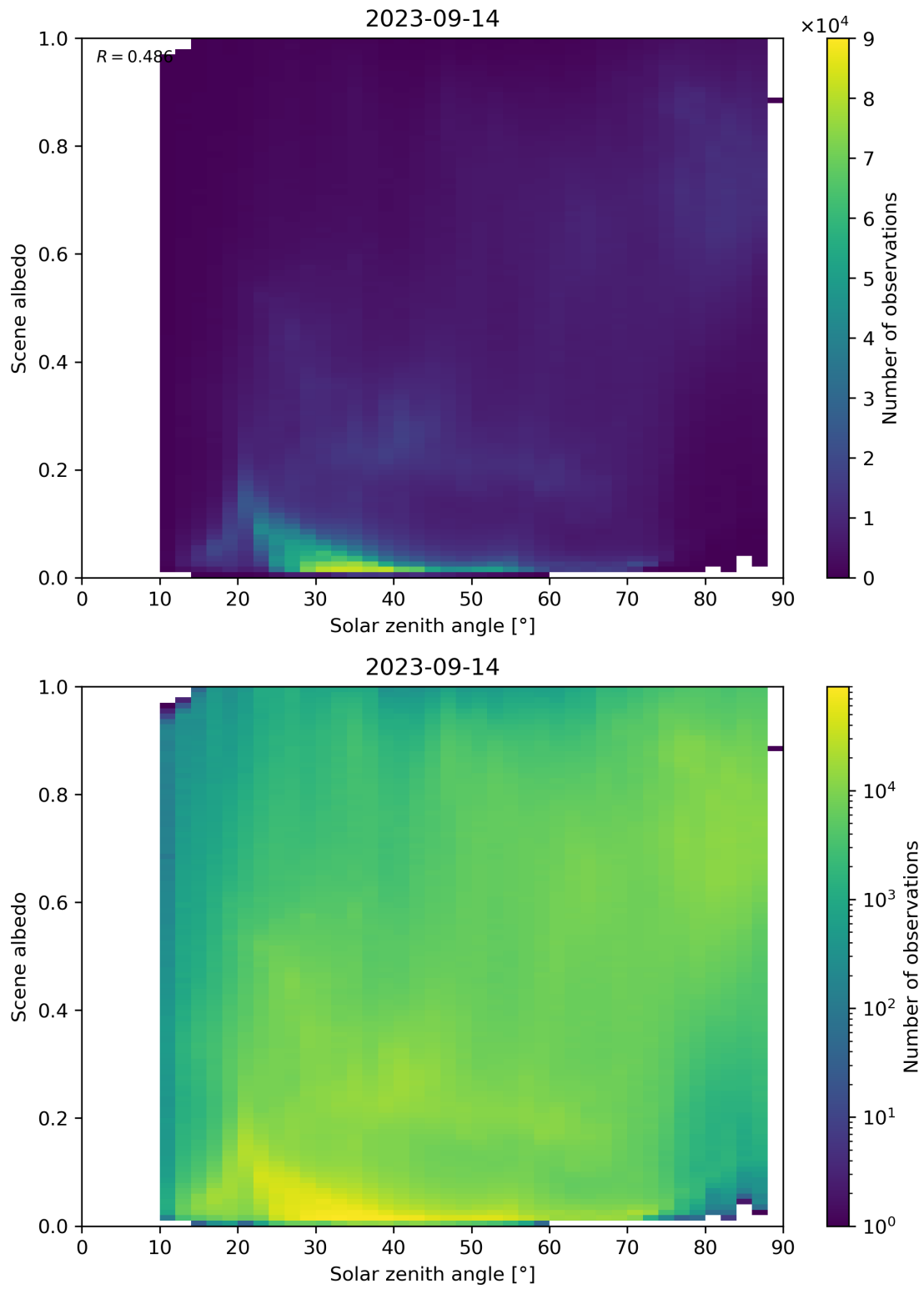
Figure 127: Scatter density plot of “Solar zenith angle” against “Scene albedo” for 2023-09-13 to 2023-09-15.
