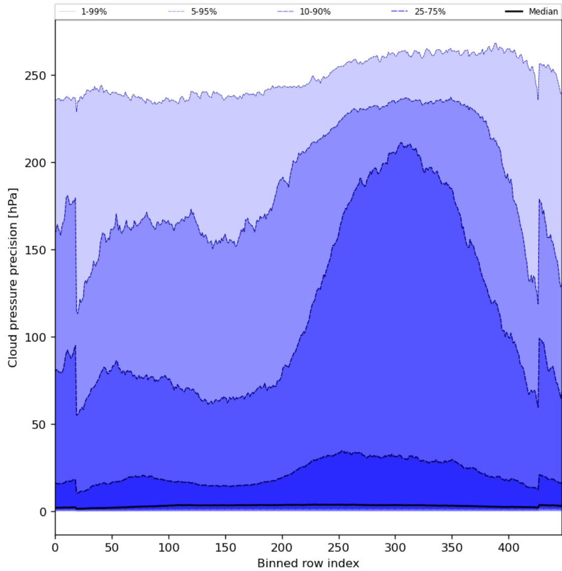
Figure 48: Along track statistics of “Cloud pressure precision” for 2023-09-13 to 2023-09-15
