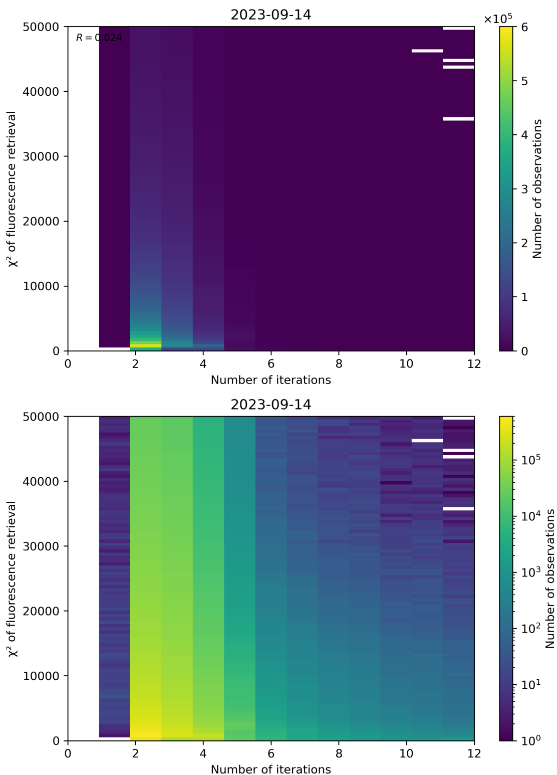
Figure 106: Scatter density plot of “Number of iterations” against “ \chi^2 of fluorescence retrieval” for 2023-09-13 to 2023-09-15.
