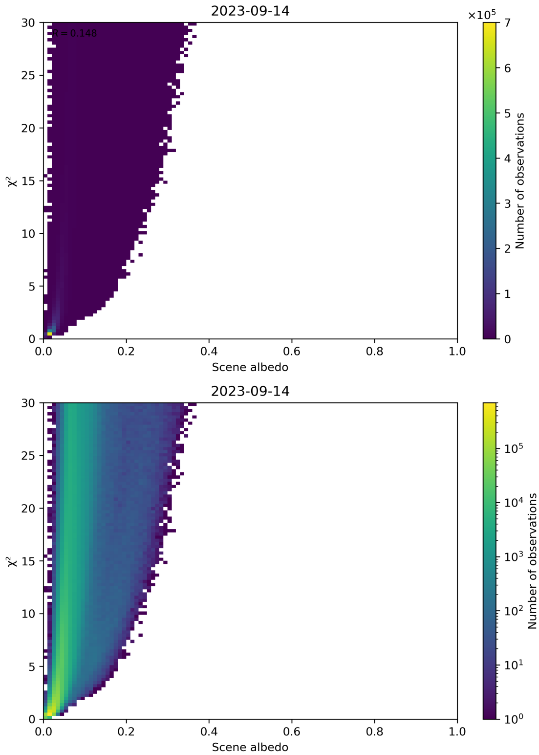
Figure 112: Scatter density plot of “Scene albedo” against “ \chi^2 ” for 2023-09-13 to 2023-09-15.
