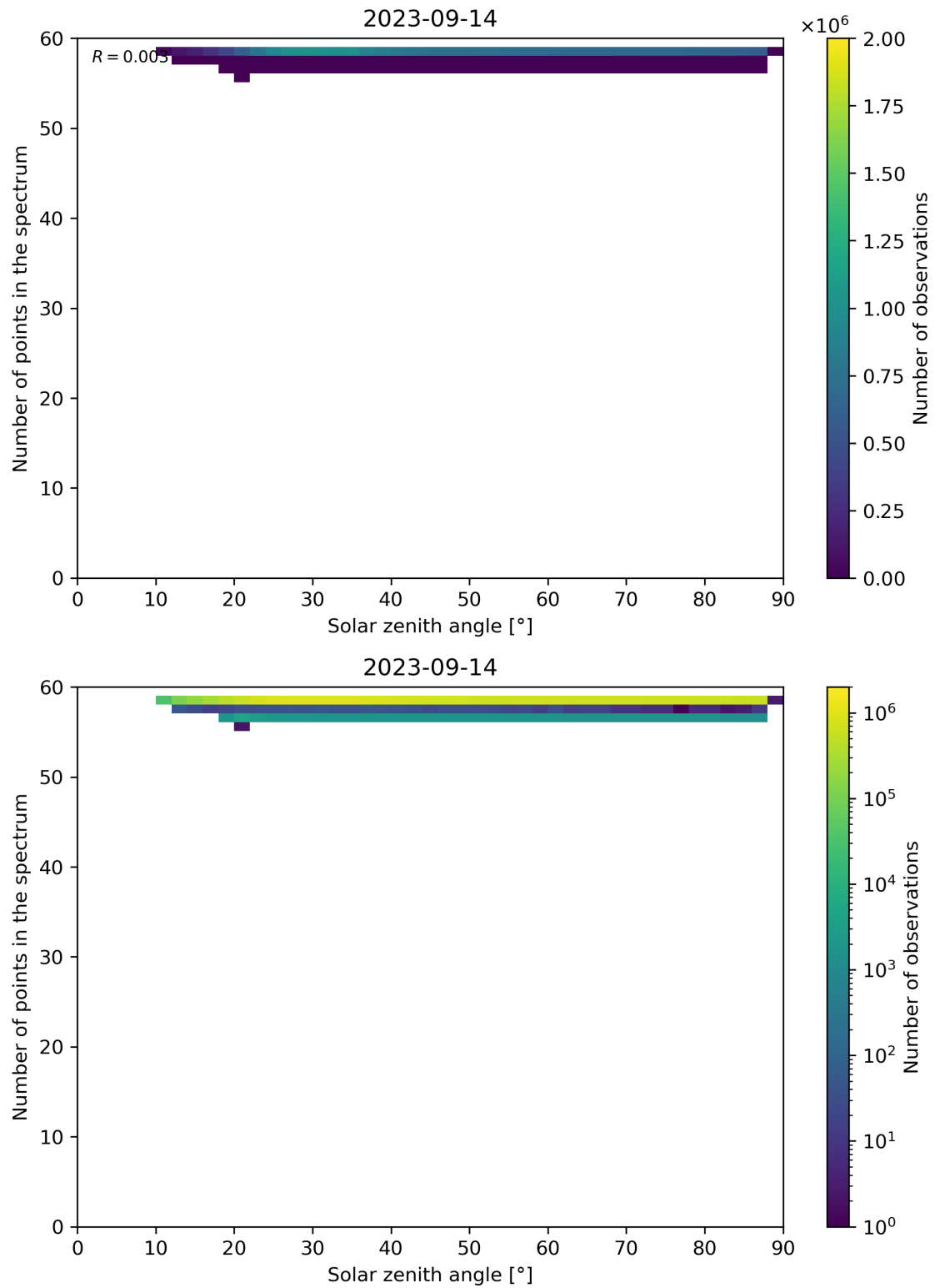
Figure 126: Scatter density plot of “Solar zenith angle” against “Number of points in the spectrum” for 2023-09-13 to 2023-09-15.
