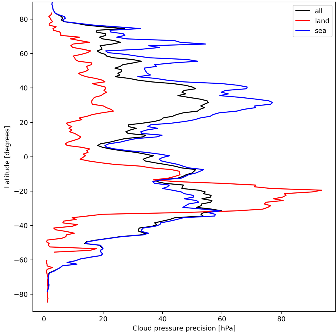
Figure 14: Zonal average of “Cloud pressure precision” for 2023-09-13 to 2023-09-15.
