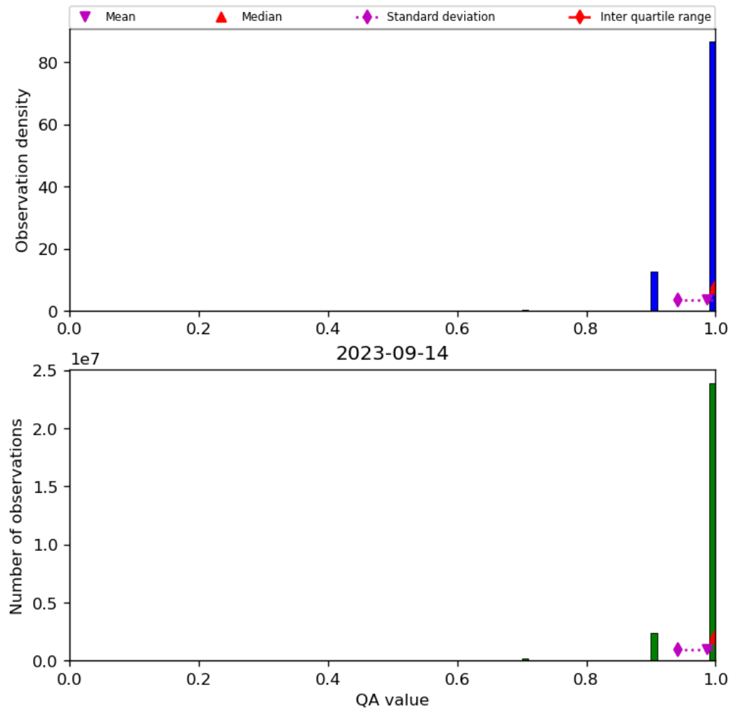
Figure 29: Histogram of “QA value” for 2023-09-13 to 2023-09-15
