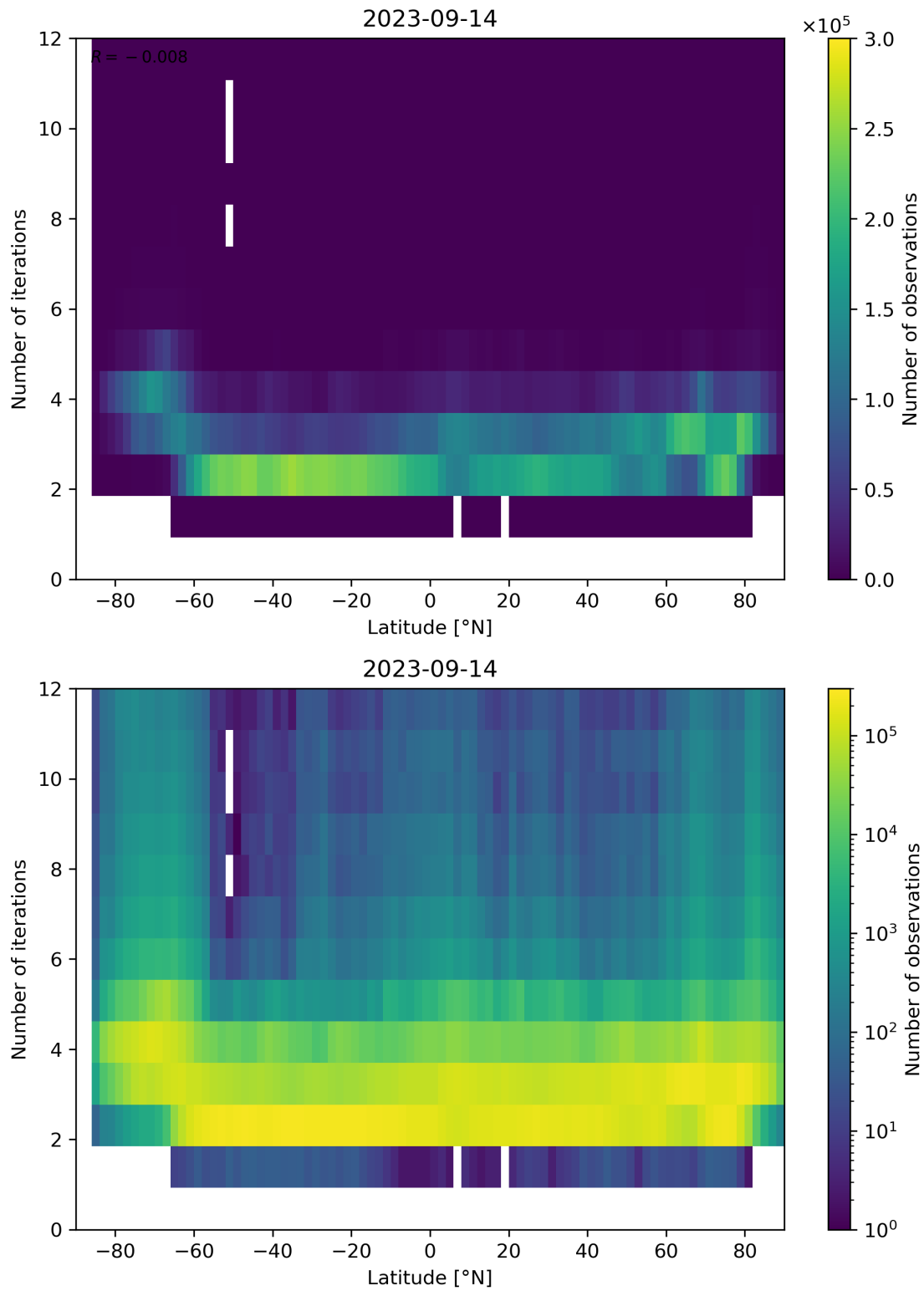
Figure 102: Scatter density plot of “Latitude” against “Number of iterations” for 2023-09-13 to 2023-09-15.
