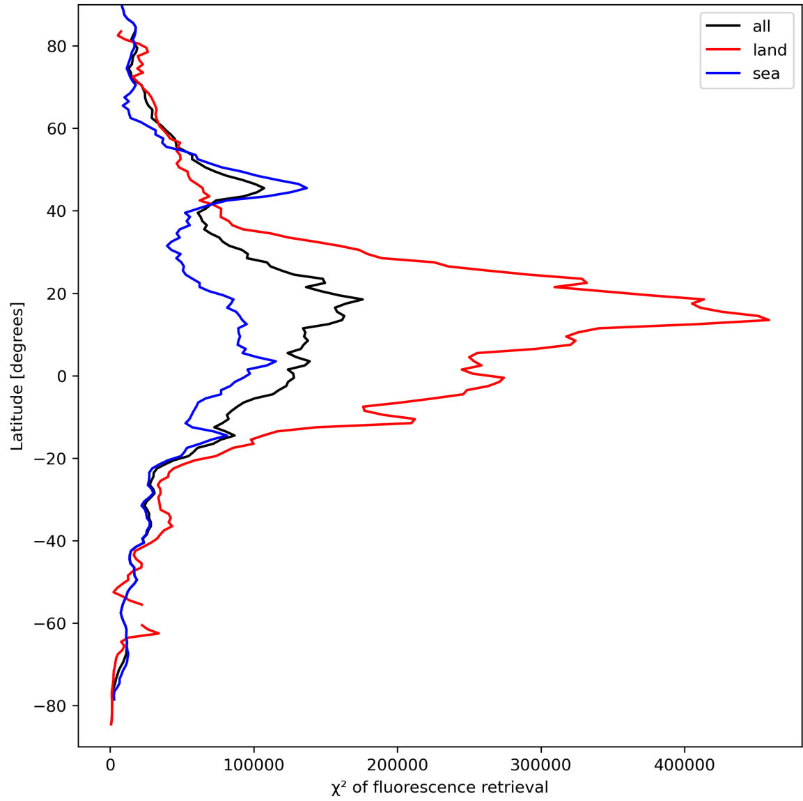
Figure 25: Zonal average of “ \chi^2 of fluorescence retrieval” for 2023-09-13 to 2023-09-15.
