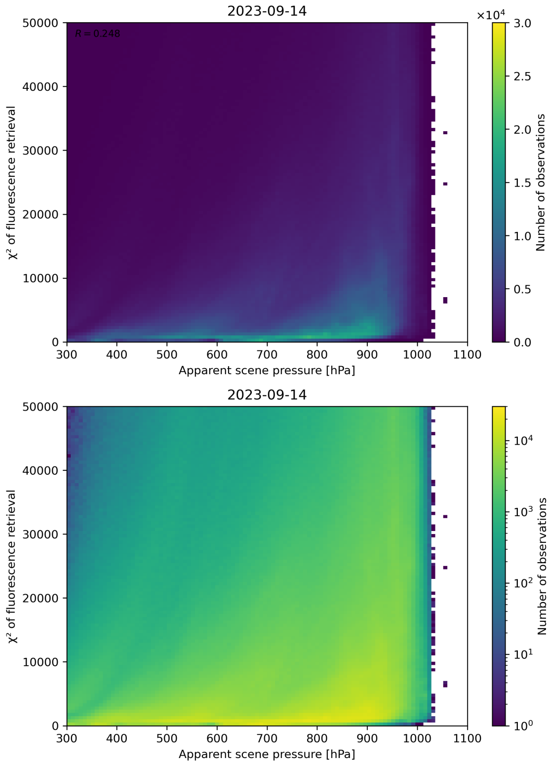
Figure 64: Scatter density plot of “Apparent scene pressure” against “ \chi^2 of fluorescence retrieval” for 2023-09-13 to 2023-09-15.
