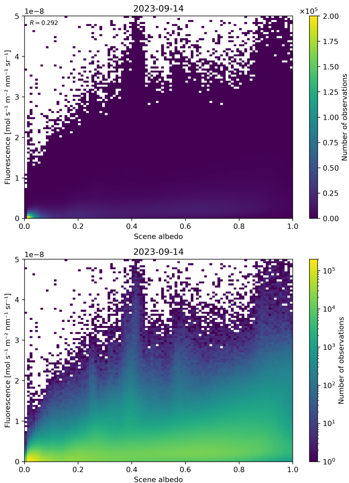
Figure 114: Scatter density plot of “Scene albedo” against “Fluorescence” for 2023-09-13 to 2023-09-15.
