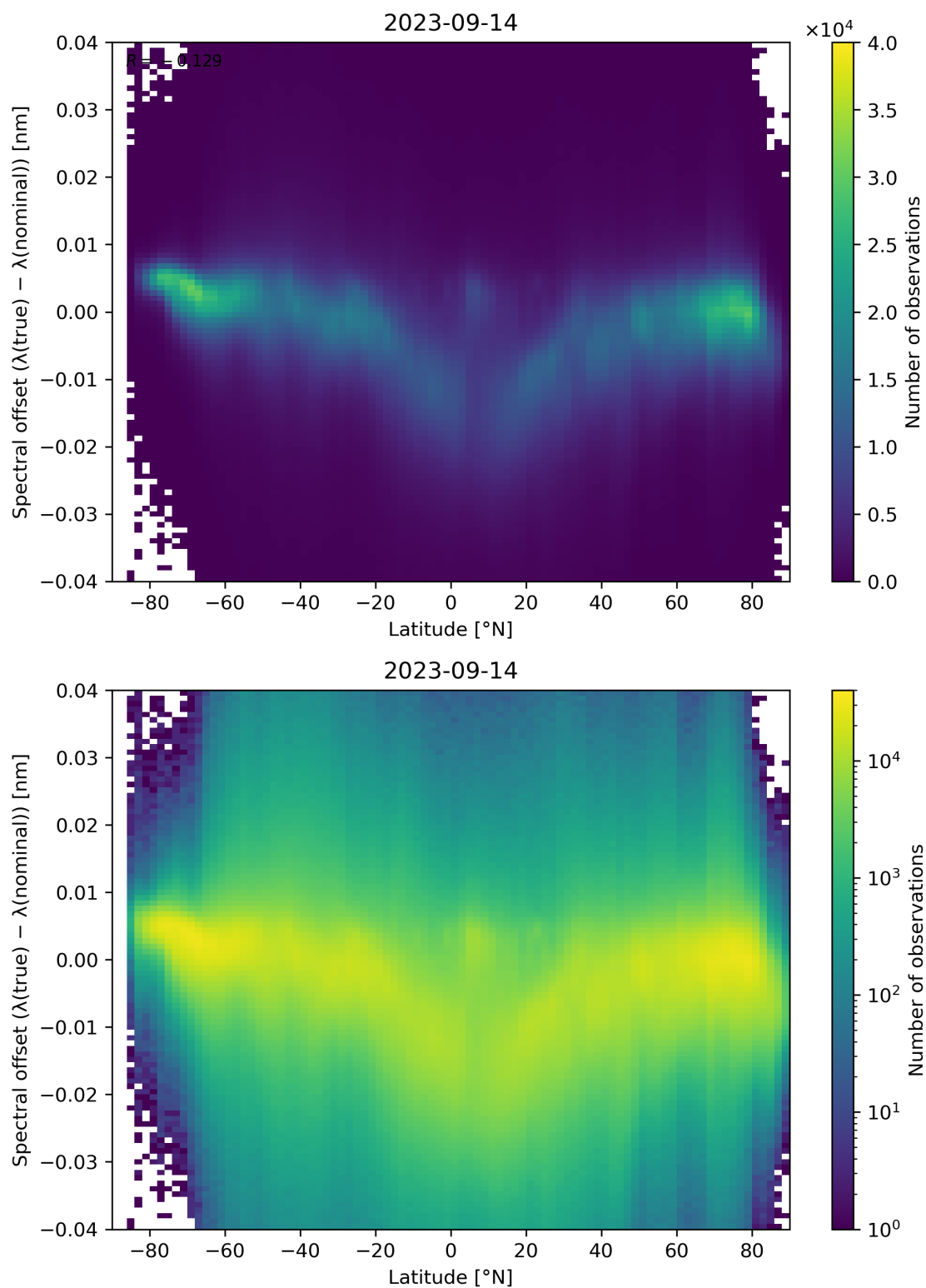
Figure 105: Scatter density plot of “Latitude” against “Spectral offset ( \lambda(\text{true}) - \lambda(\text{nominal}) )” for 2023-09-13 to 2023-09-15.
