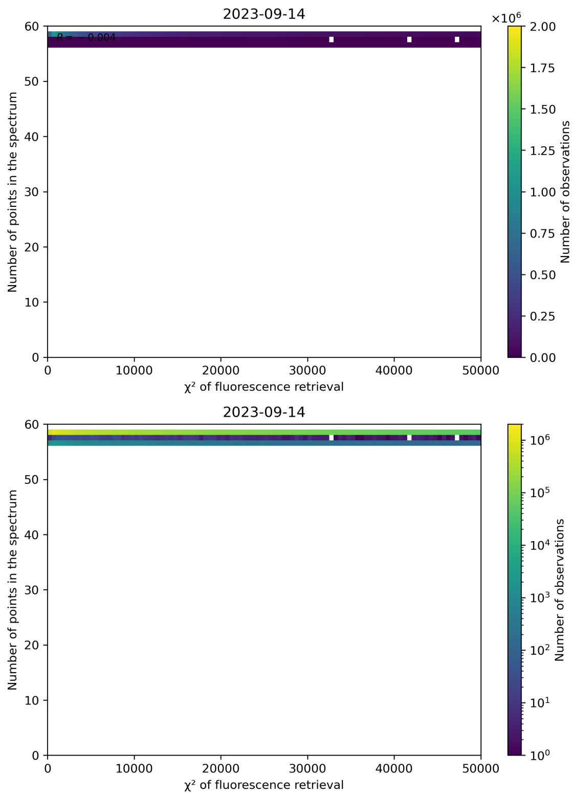
Figure 71: Scatter density plot of “ \chi^2 of fluorescence retrieval” against “Number of points in the spectrum” for 2023-09-13 to 2023-09-15.
