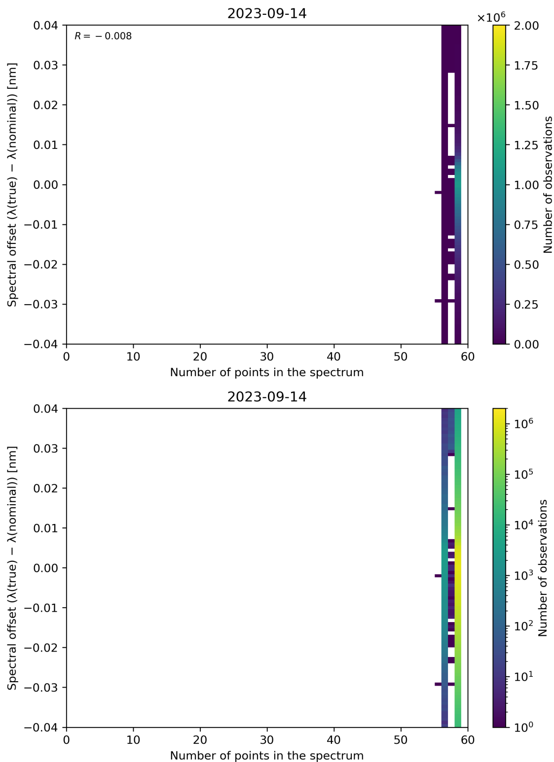
Figure 110: Scatter density plot of “Number of points in the spectrum” against “Spectral offset ( \lambda(\text{true}) - \lambda(\text{nominal}) )” for 2023-09-13 to 2023-09-15.
