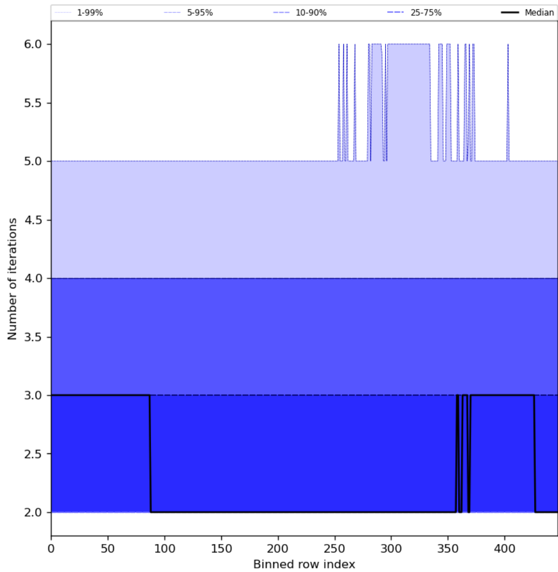
Figure 56: Along track statistics of “Number of iterations” for 2023-09-13 to 2023-09-15
