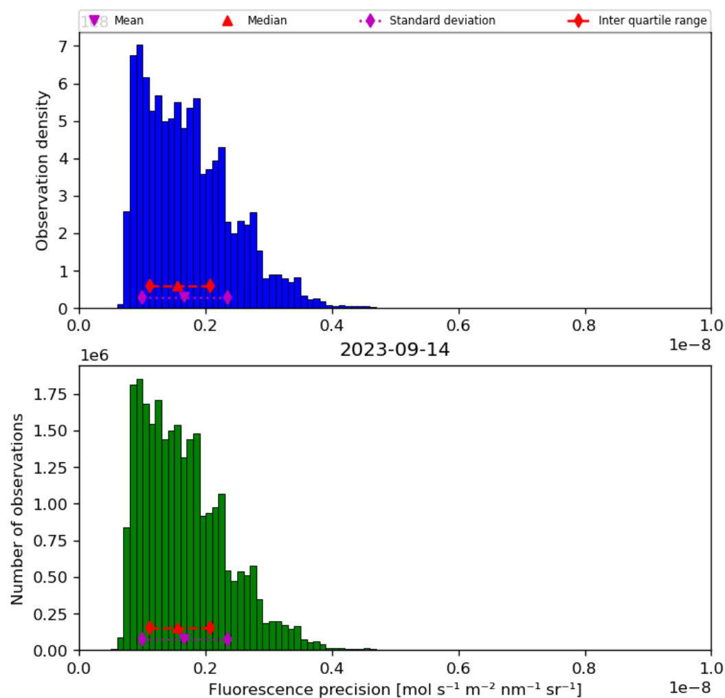
Figure 41: Histogram of “Fluorescence precision” for 2023-09-13 to 2023-09-15
