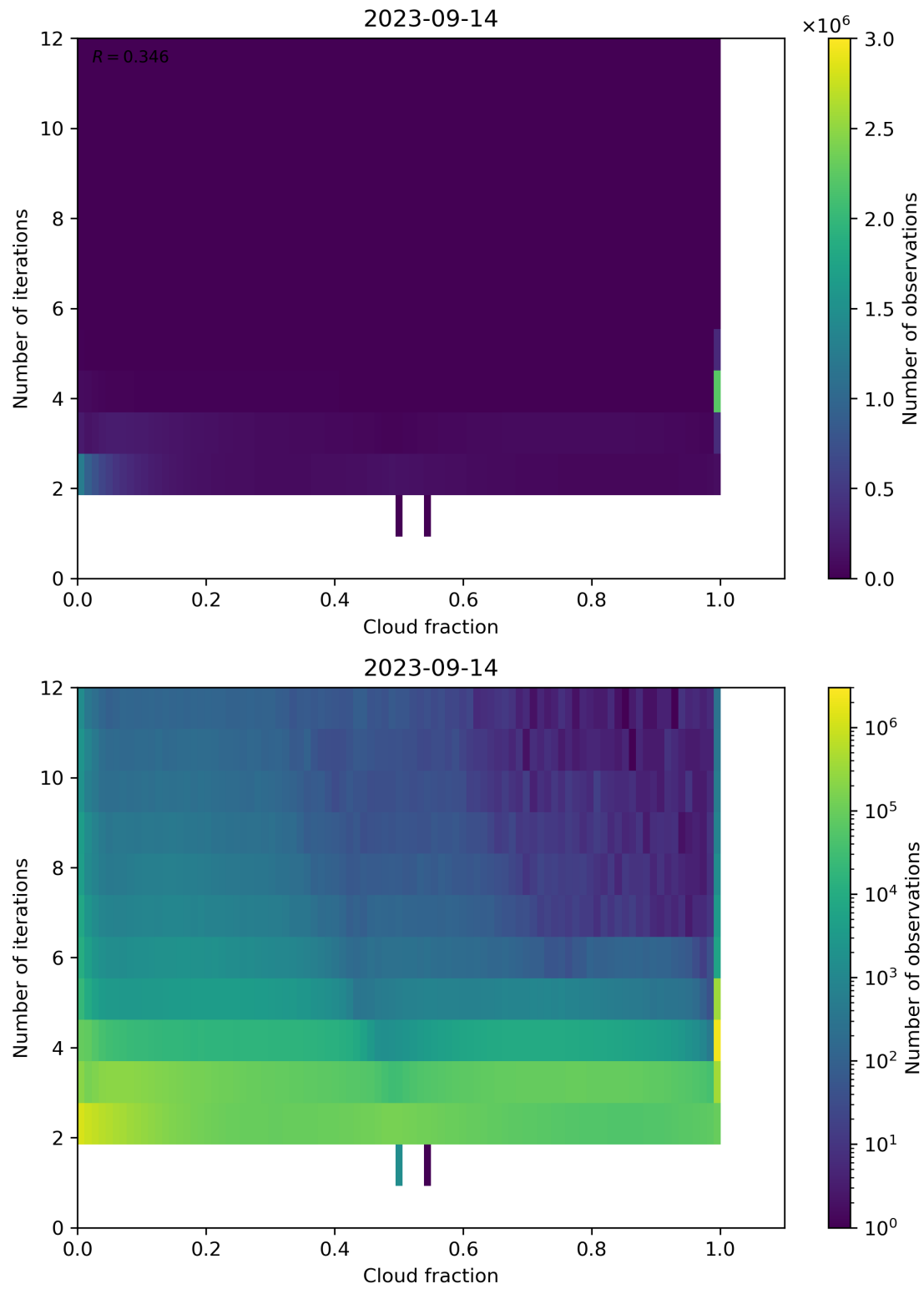
Figure 80: Scatter density plot of “Cloud fraction” against “Number of iterations” for 2023-09-13 to 2023-09-15.
