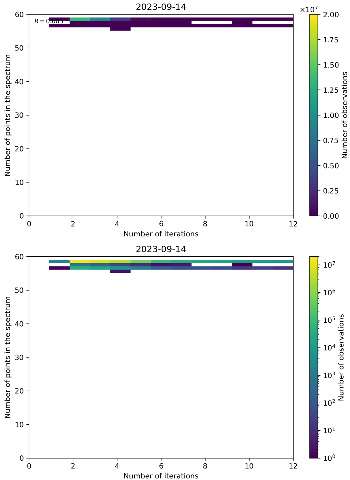
Figure 108: Scatter density plot of “Number of iterations” against “Number of points in the spectrum” for 2023-09-13 to 2023-09-15.
