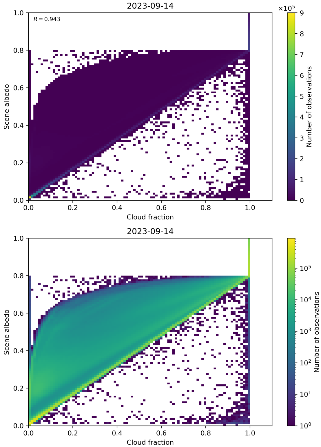
Figure 82: Scatter density plot of “Cloud fraction” against “Scene albedo” for 2023-09-13 to 2023-09-15.
