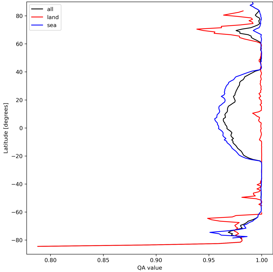
Figure 12: Zonal average of “QA value” for 2023-09-13 to 2023-09-15.
