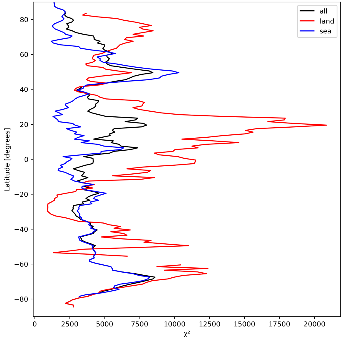
Figure 21: Zonal average of “ \chi^2 ” for 2023-09-13 to 2023-09-15.
