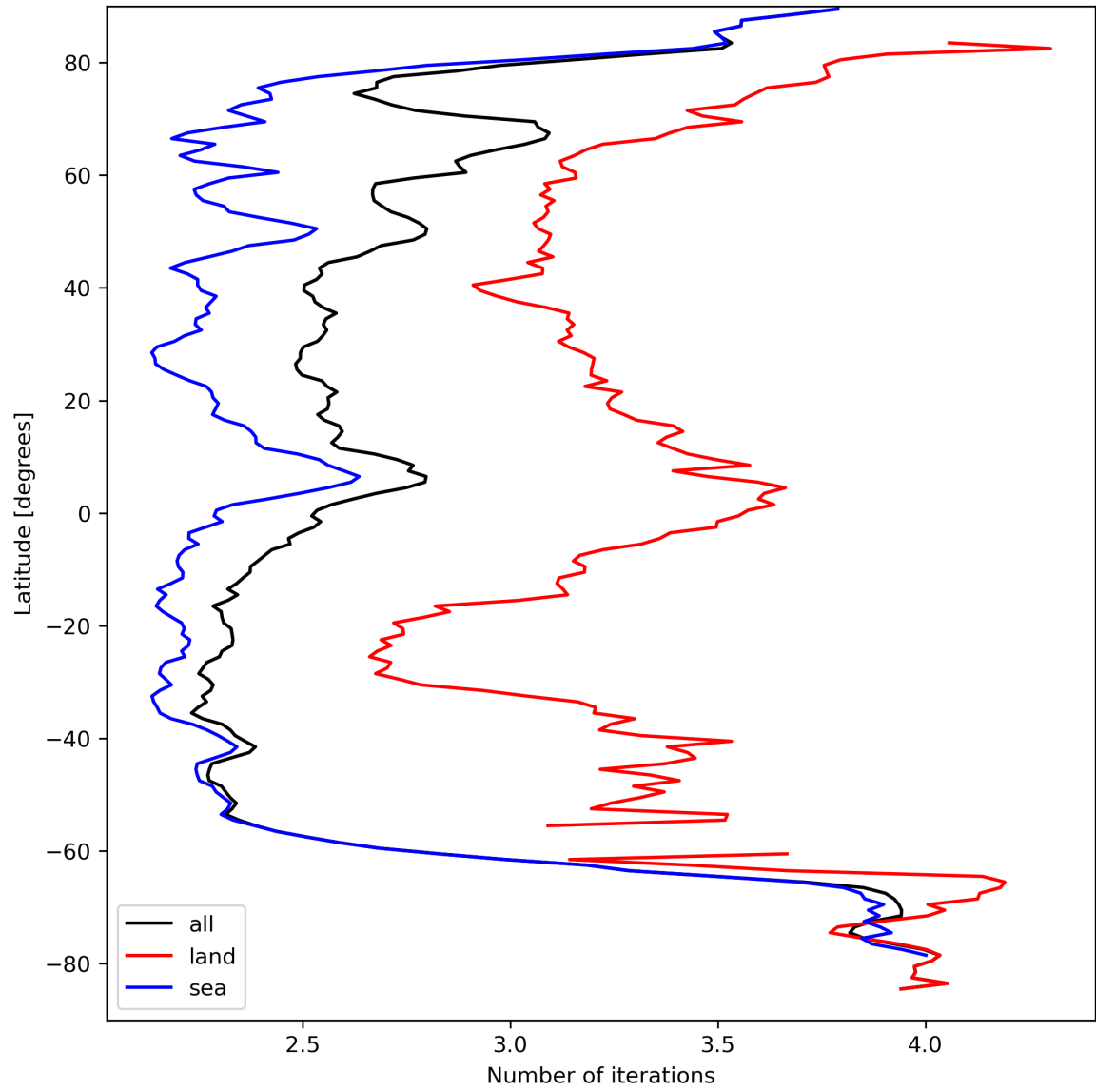
Figure 22: Zonal average of “Number of iterations” for 2023-09-13 to 2023-09-15.
