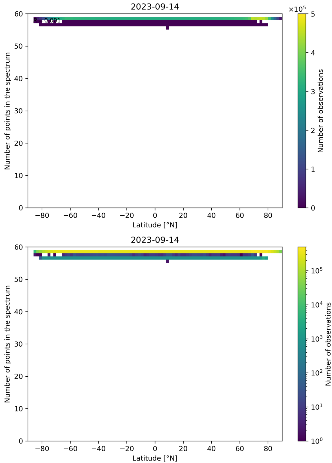
Figure 103: Scatter density plot of “Latitude” against “Number of points in the spectrum” for 2023-09-13 to 2023-09-15.
