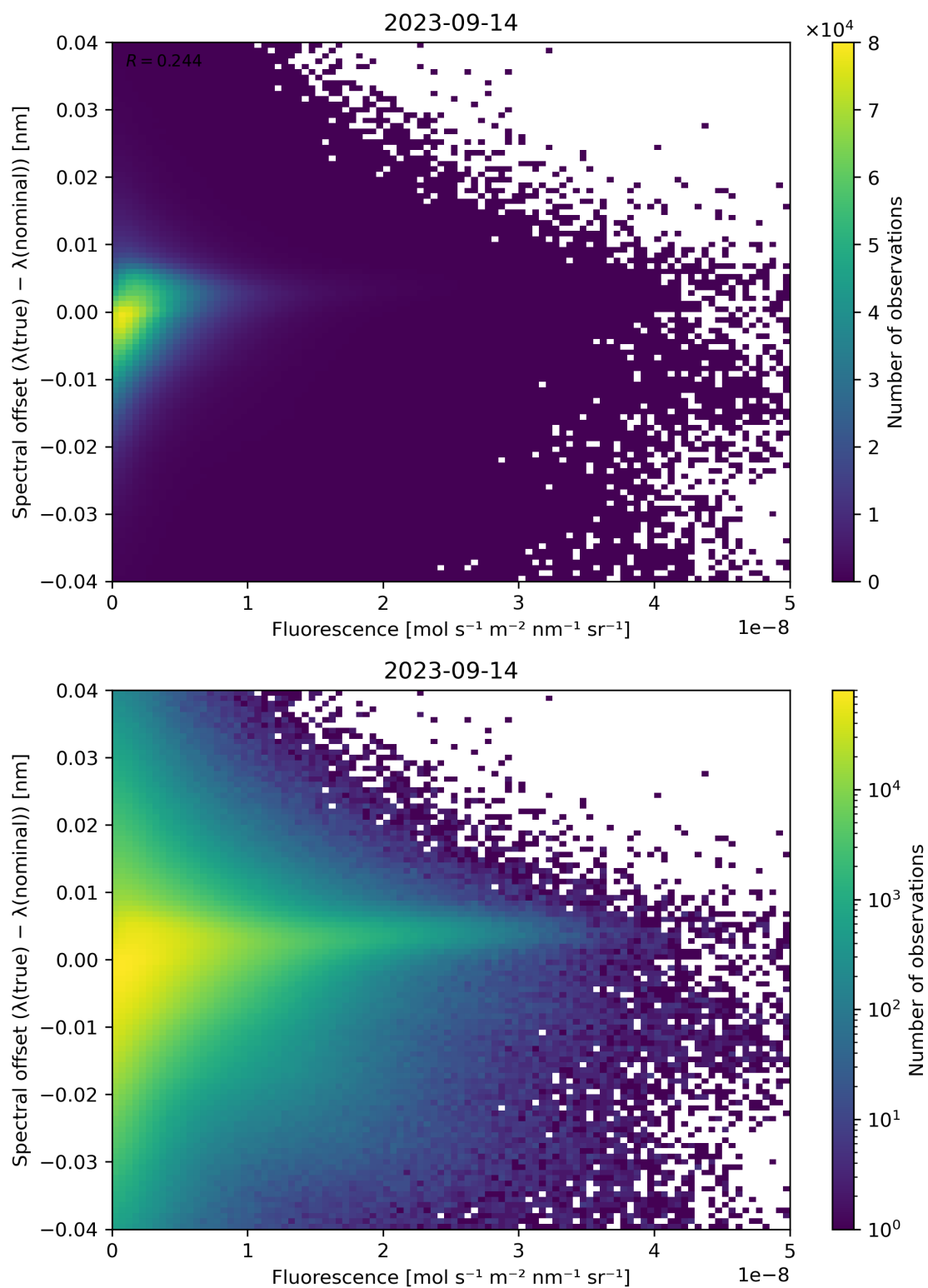
Figure 95: Scatter density plot of “Fluorescence” against “Spectral offset ( \lambda(\text{true}) - \lambda(\text{nominal}) )” for 2023-09-13 to 2023-09-15.
