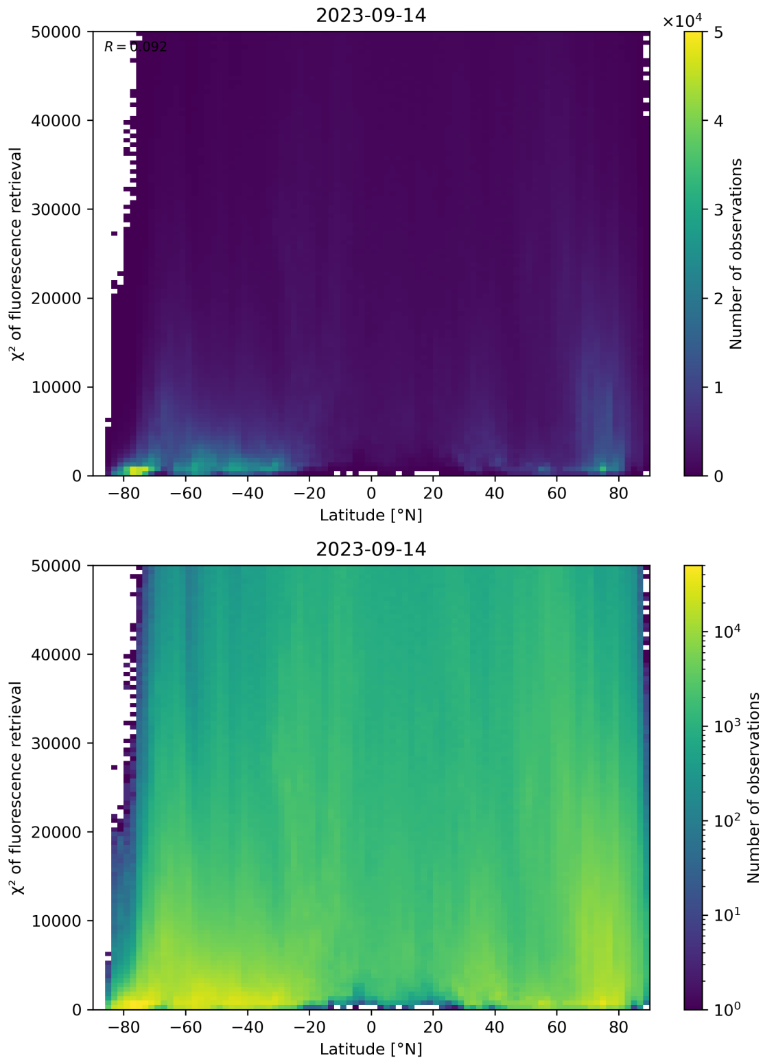
Figure 98: Scatter density plot of “Latitude” against “ \chi^2 of fluorescence retrieval” for 2023-09-13 to 2023-09-15.
