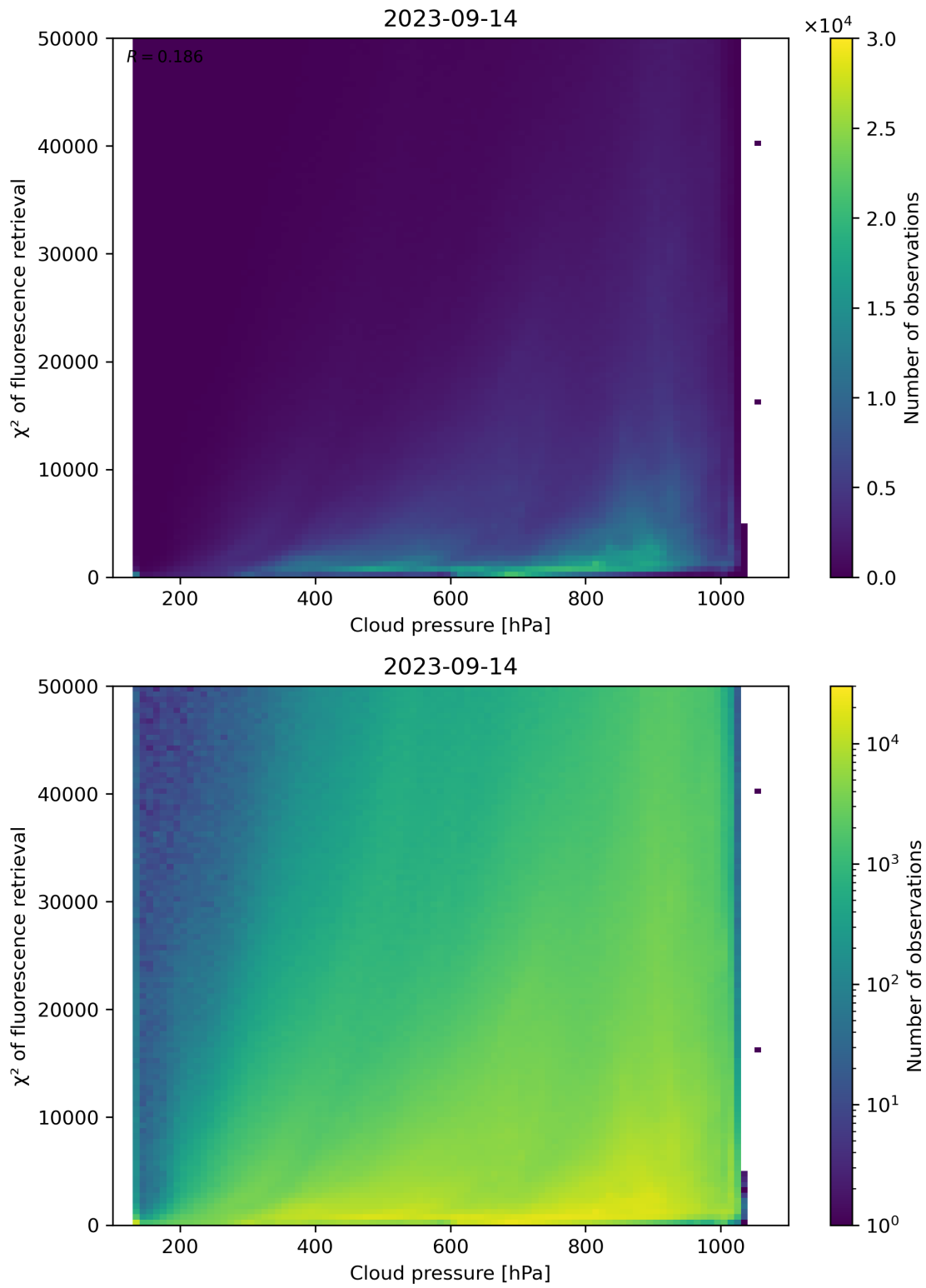
Figure 86: Scatter density plot of “Cloud pressure” against “ \chi^2 of fluorescence retrieval” for 2023-09-13 to 2023-09-15.
