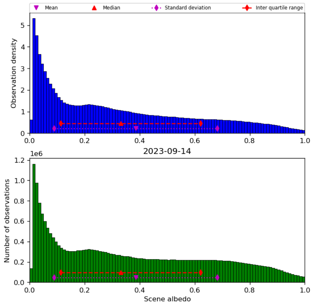
Figure 34: Histogram of “Scene albedo” for 2023-09-13 to 2023-09-15
