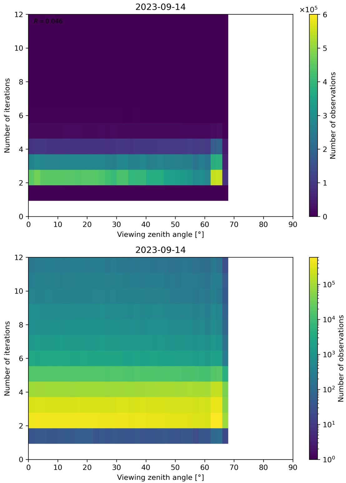
Figure 136: Scatter density plot of “Viewing zenith angle” against “Number of iterations” for 2023-09-13 to 2023-09-15.
