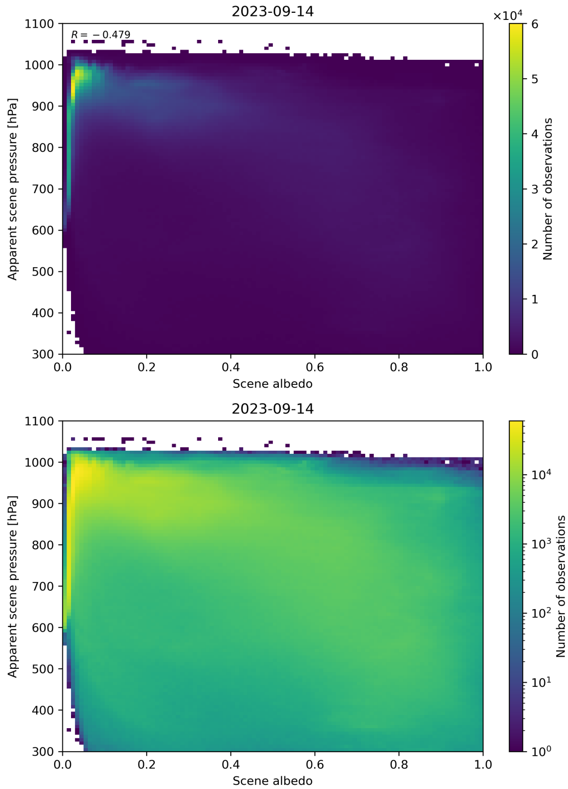
Figure 111: Scatter density plot of “Scene albedo” against “Apparent scene pressure” for 2023-09-13 to 2023-09-15.
