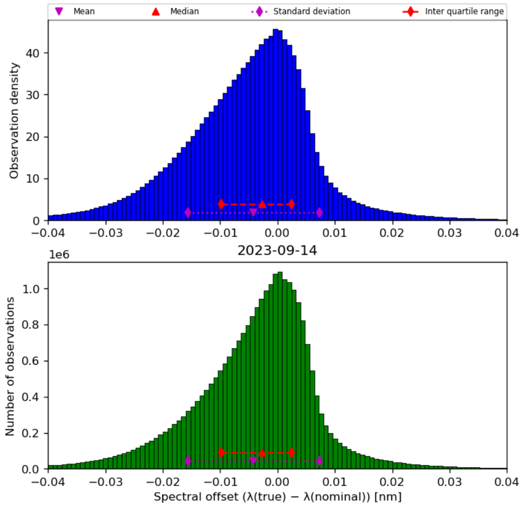
Figure 45: Histogram of “Spectral offset ( \lambda(\text{true}) - \lambda(\text{nominal}) )” for 2023-09-13 to 2023-09-15
