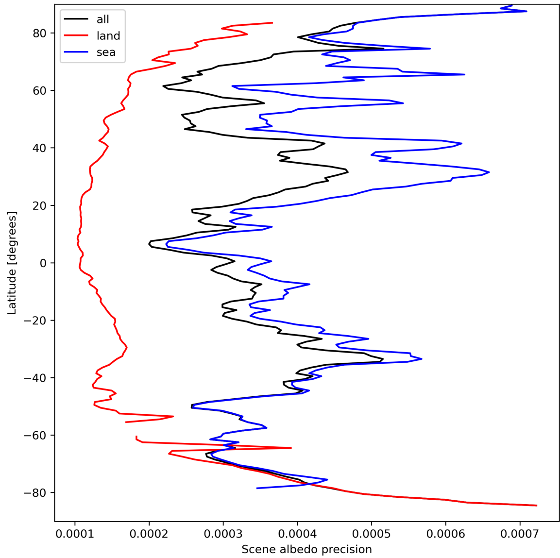
Figure 18: Zonal average of “Scene albedo precision” for 2023-09-13 to 2023-09-15.
