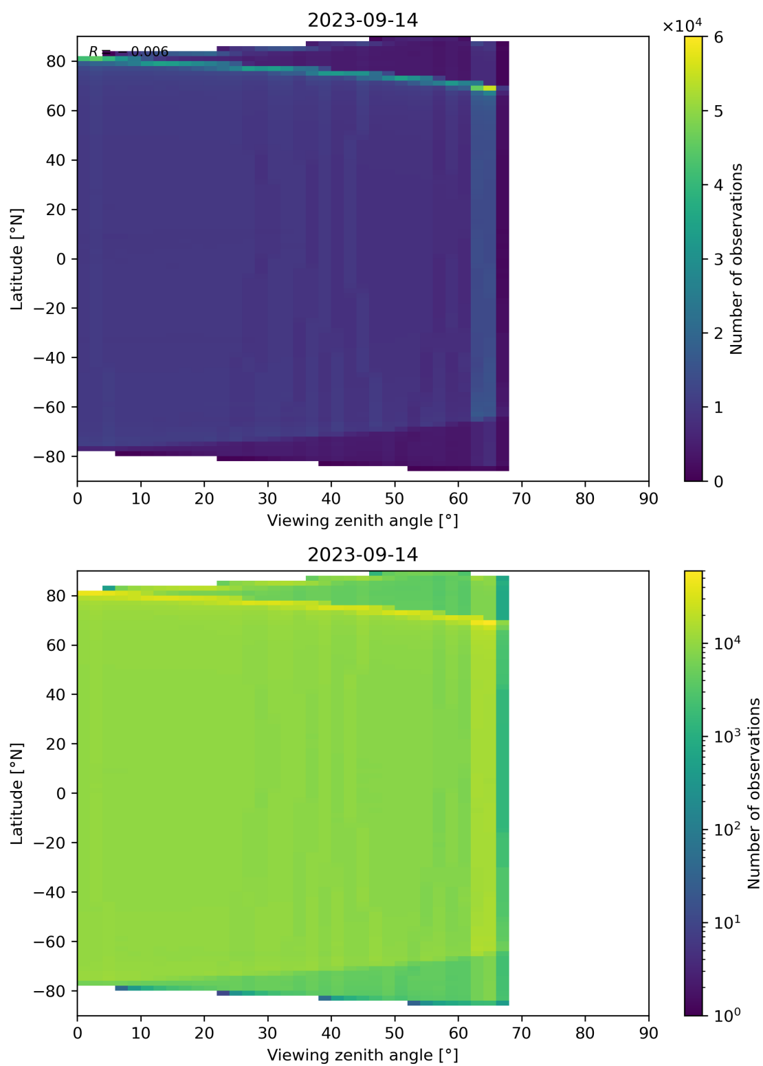
Figure 135: Scatter density plot of “Viewing zenith angle” against “Latitude” for 2023-09-13 to 2023-09-15.
