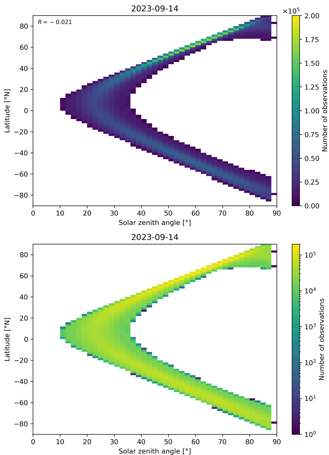
Figure 124: Scatter density plot of “Solar zenith angle” against “Latitude” for 2023-09-13 to 2023-09-15.
