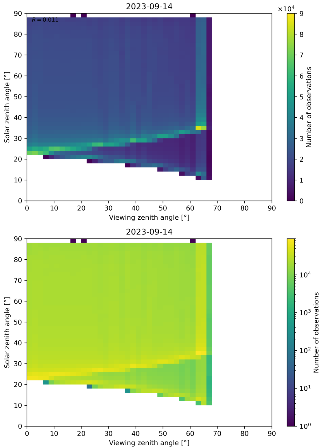
Figure 139: Scatter density plot of “Viewing zenith angle” against “Solar zenith angle” for 2023-09-13 to 2023-09-15.
