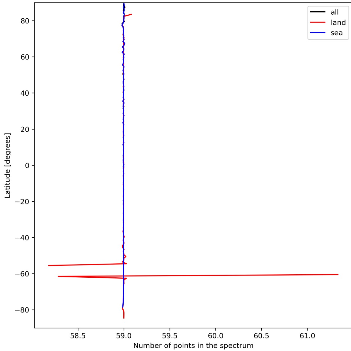
Figure 27: Zonal average of “Number of points in the spectrum” for 2023-09-13 to 2023-09-15.
