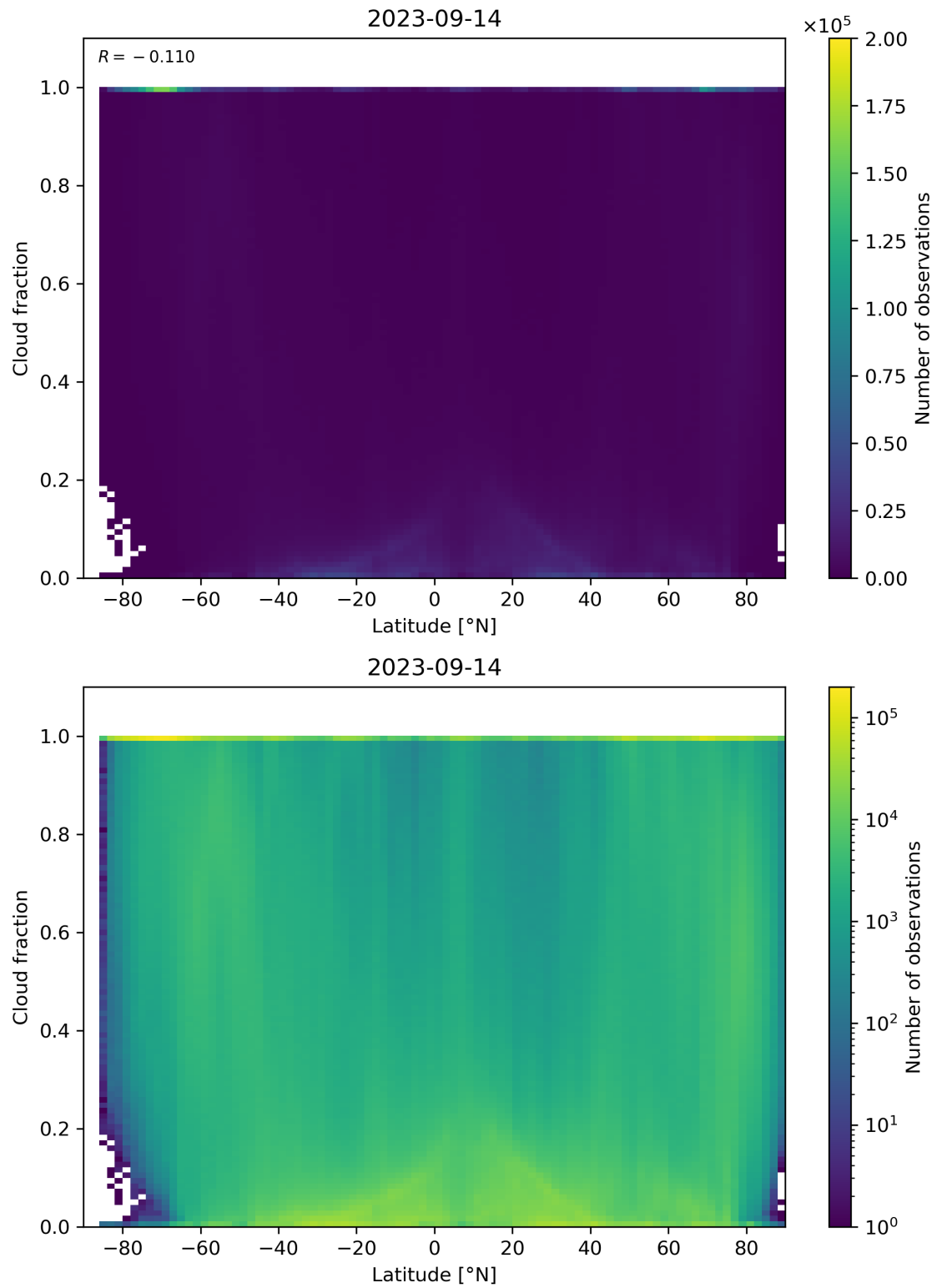
Figure 99: Scatter density plot of “Latitude” against “Cloud fraction” for 2023-09-13 to 2023-09-15.
