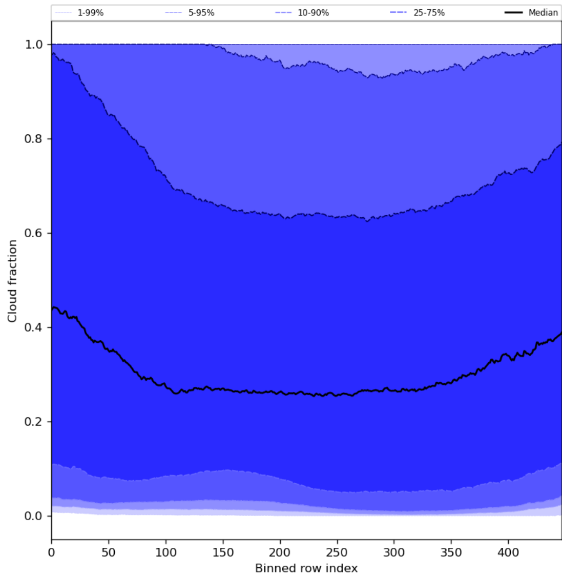
Figure 49: Along track statistics of “Cloud fraction” for 2023-09-13 to 2023-09-15
