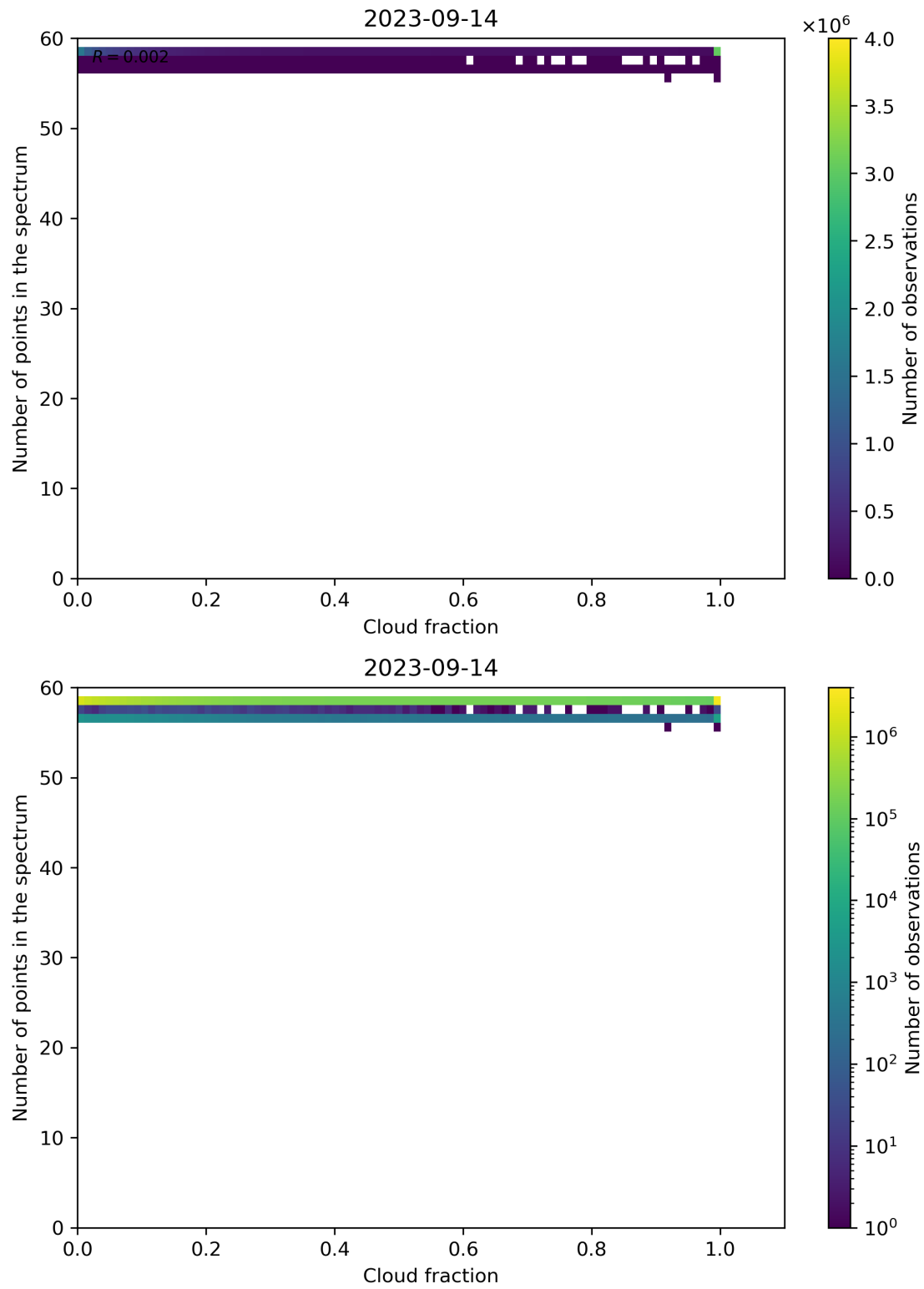
Figure 81: Scatter density plot of “Cloud fraction” against “Number of points in the spectrum” for 2023-09-13 to 2023-09-15.
