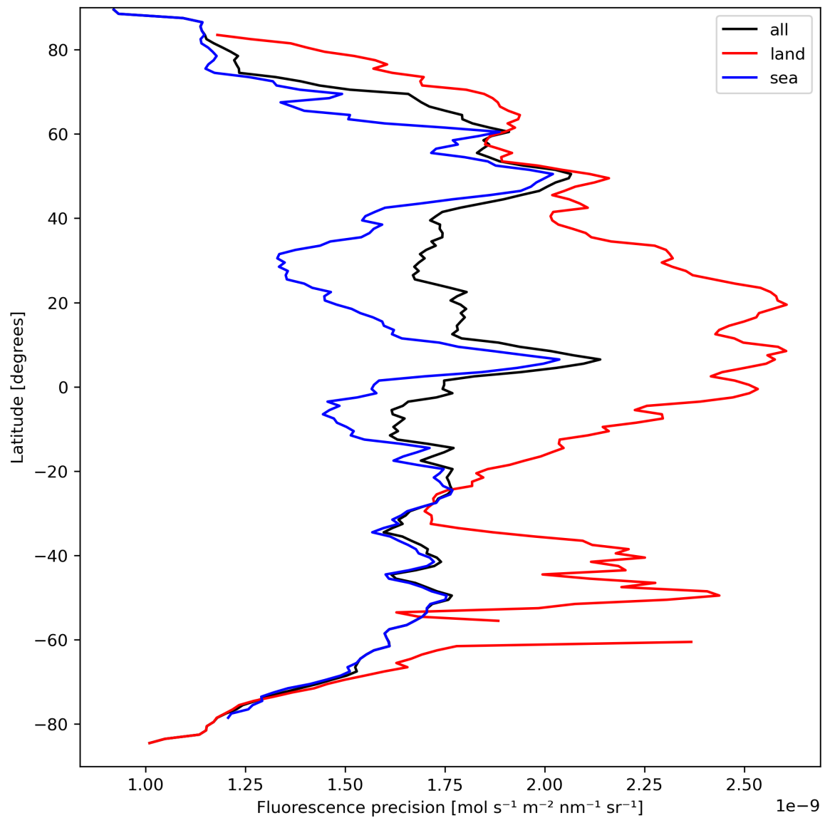
Figure 24: Zonal average of “Fluorescence precision” for 2023-09-13 to 2023-09-15.
