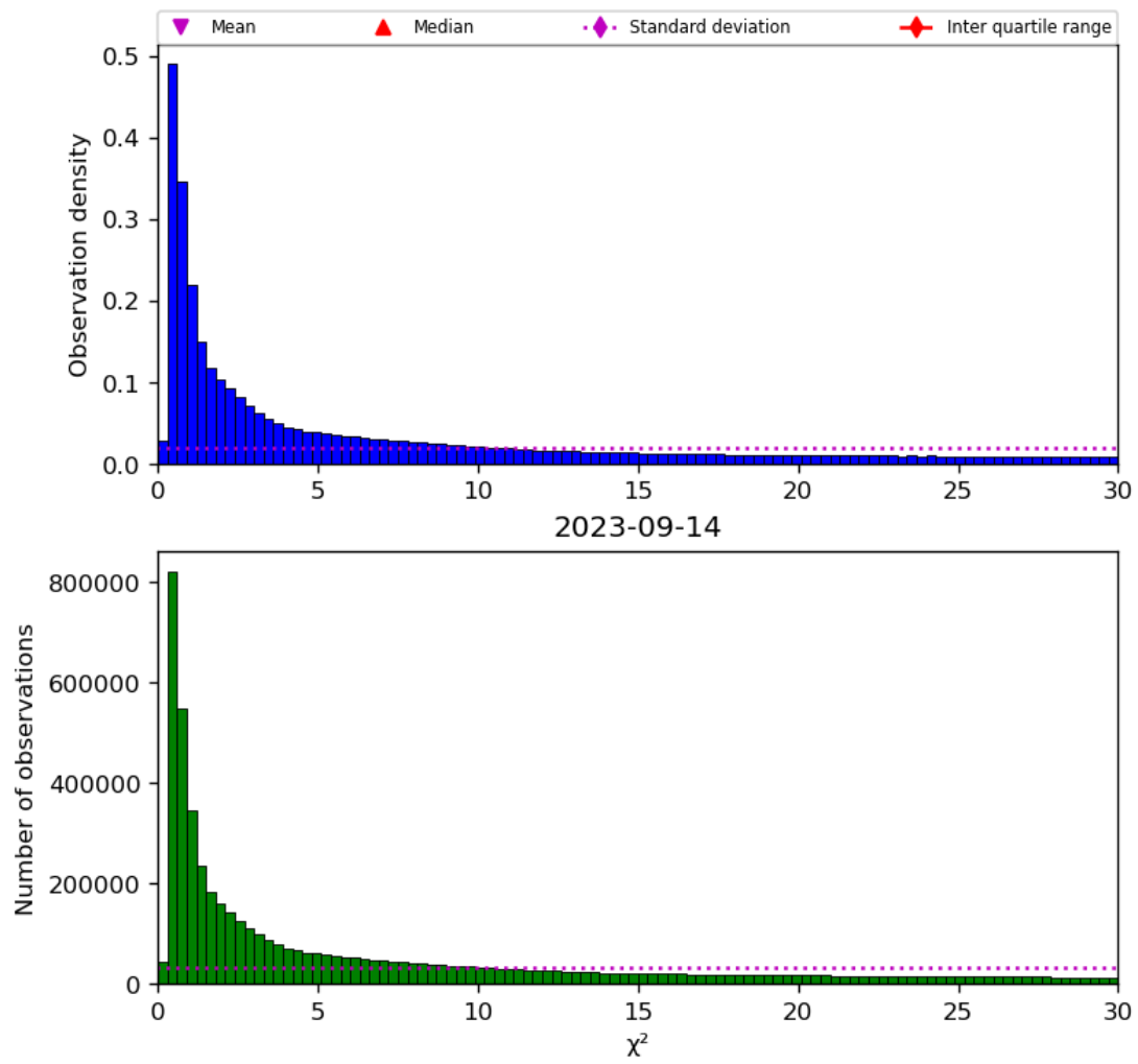
Figure 38: Histogram of “ \chi^2 ” for 2023-09-13 to 2023-09-15
