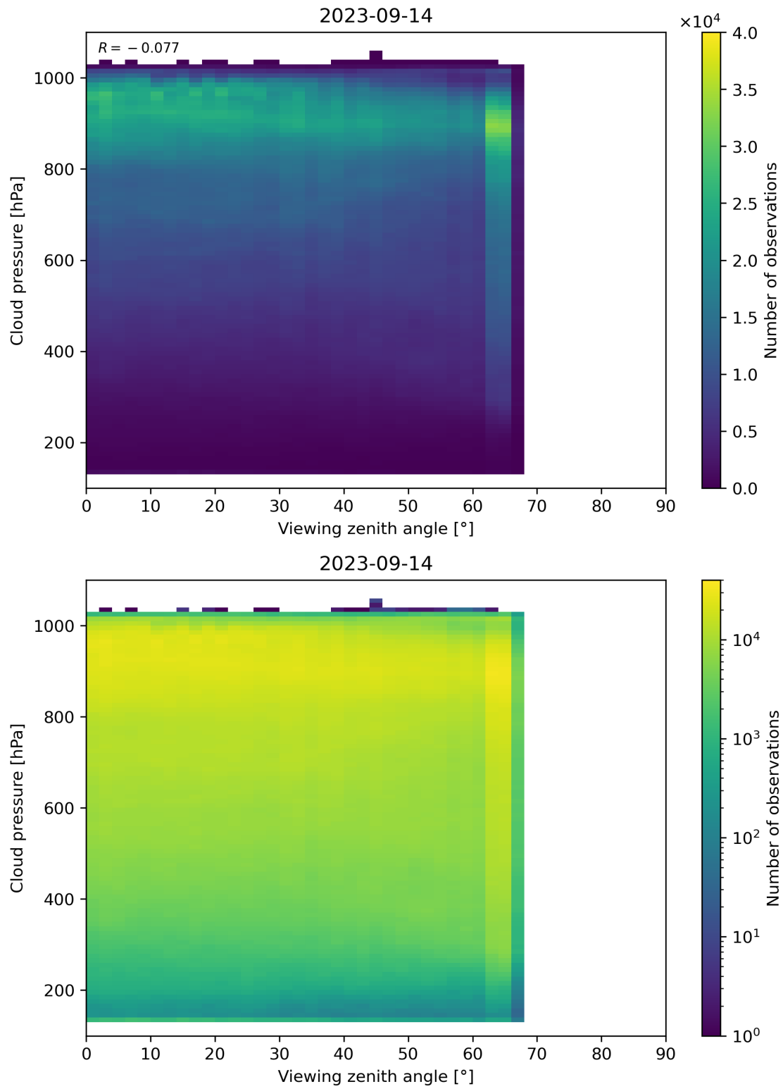
Figure 133: Scatter density plot of “Viewing zenith angle” against “Cloud pressure” for 2023-09-13 to 2023-09-15.
