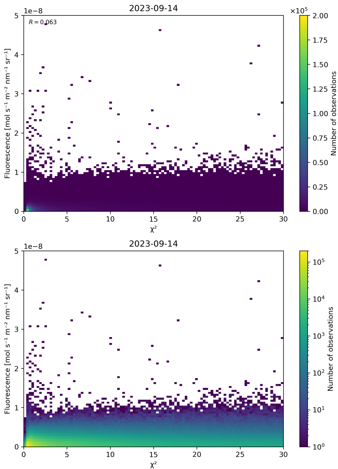
Figure 70: Scatter density plot of “ \chi^2 ” against “Fluorescence” for 2023-09-13 to 2023-09-15.
