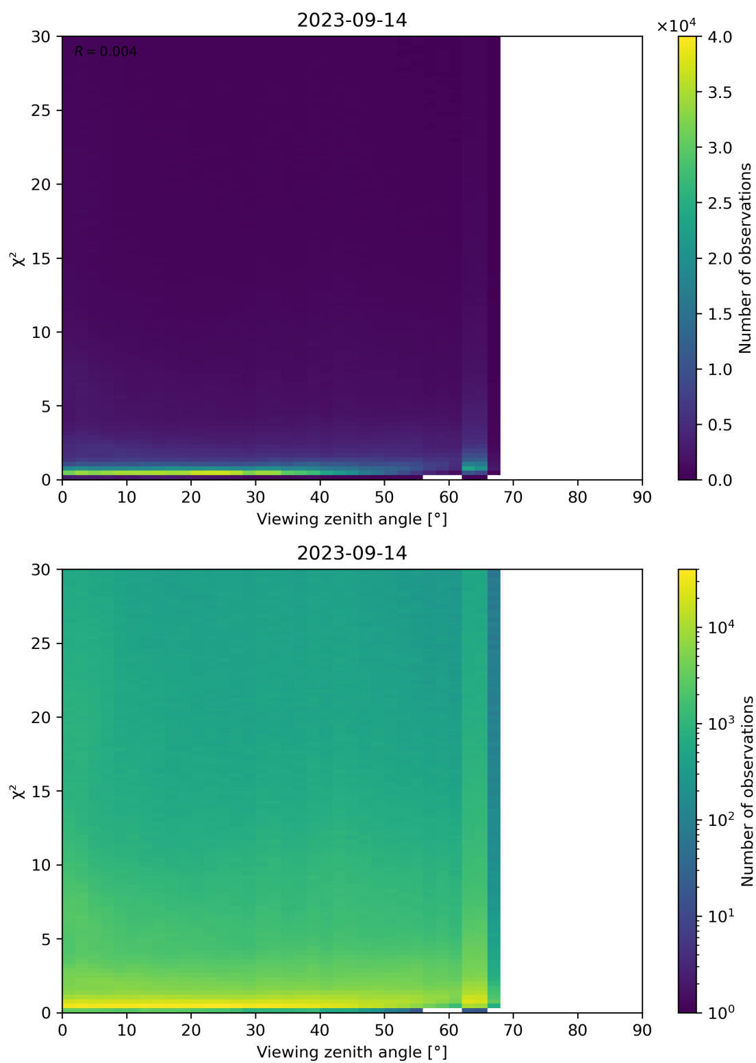
Figure 130: Scatter density plot of “Viewing zenith angle” against “ \chi^2 ” for 2023-09-13 to 2023-09-15.
