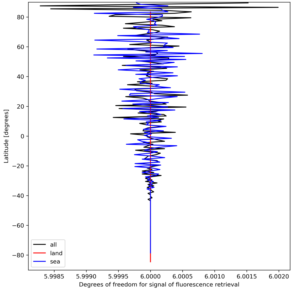
Figure 26: Zonal average of “Degrees of freedom for signal of fluorescence retrieval” for 2023-09-13 to 2023-09-15.
