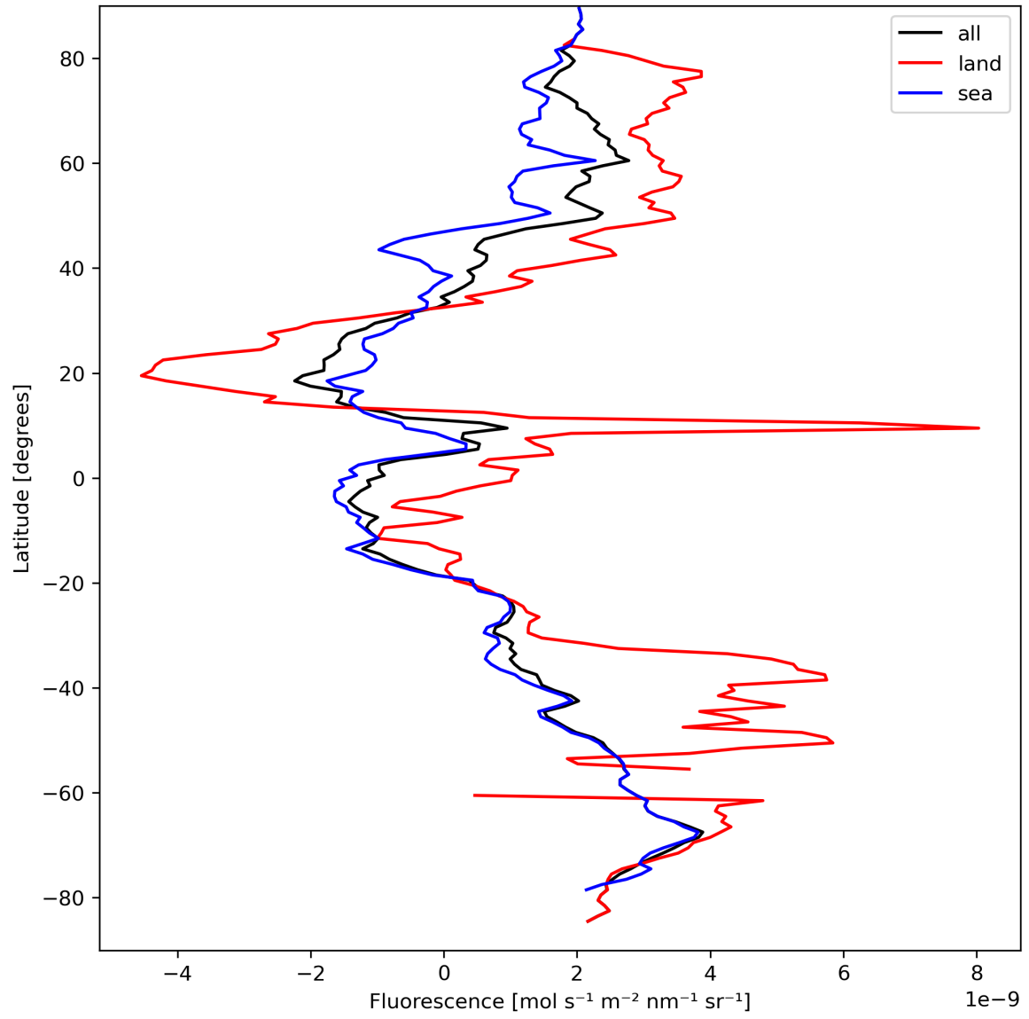
Figure 23: Zonal average of “Fluorescence” for 2023-09-13 to 2023-09-15.
