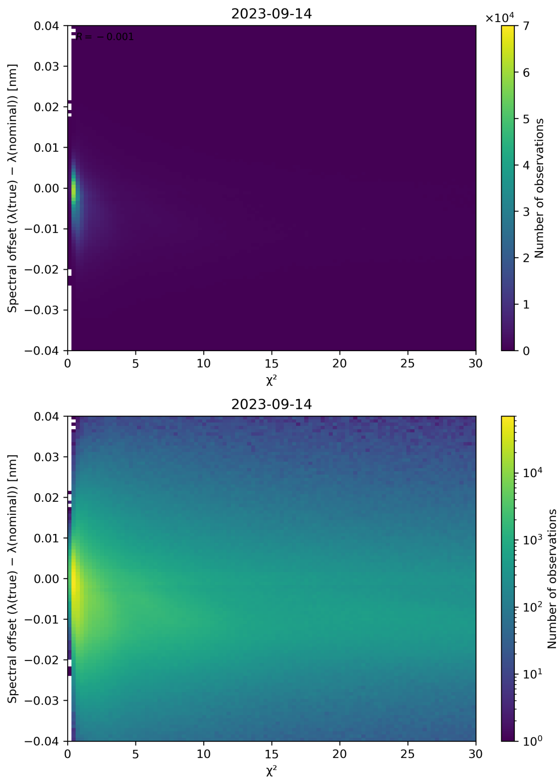
Figure 75: Scatter density plot of " \chi^2 " against "Spectral offset ( \lambda(\text{true}) - \lambda(\text{nominal}) )" for 2023-09-13 to 2023-09-15.
