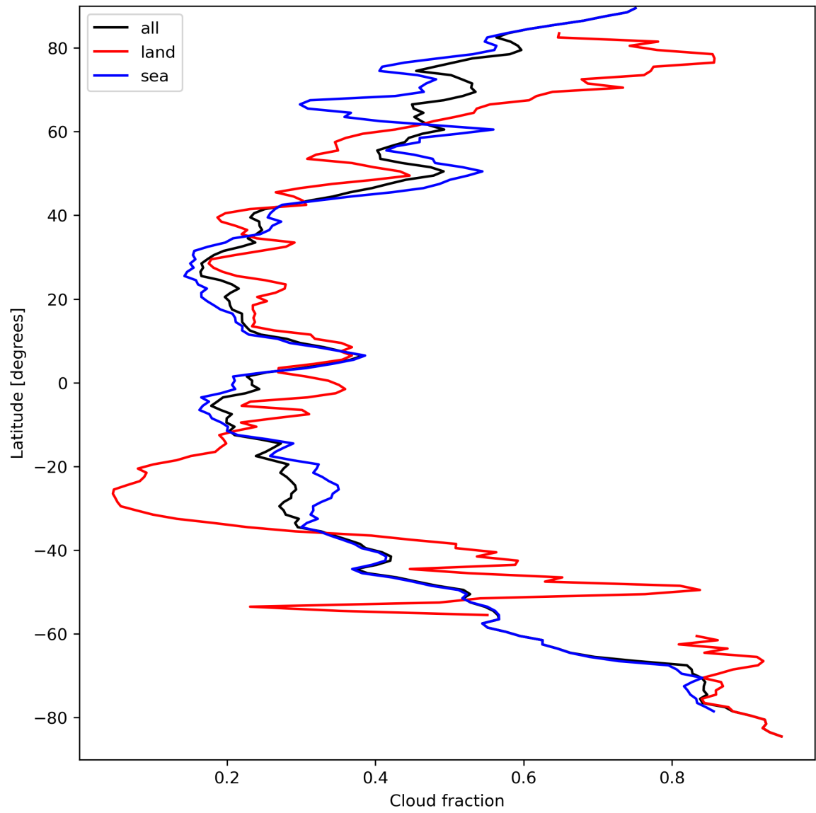
Figure 15: Zonal average of “Cloud fraction” for 2023-09-13 to 2023-09-15.
