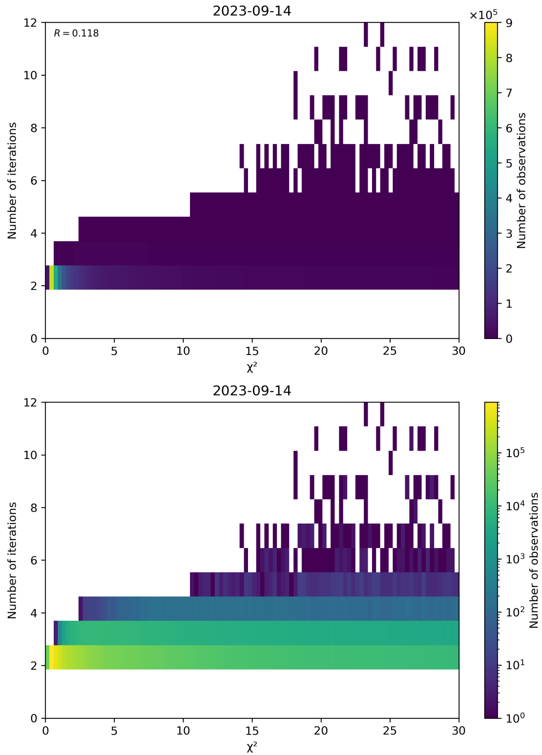
Figure 73: Scatter density plot of “ \chi^2 ” against “Number of iterations” for 2023-09-13 to 2023-09-15.
