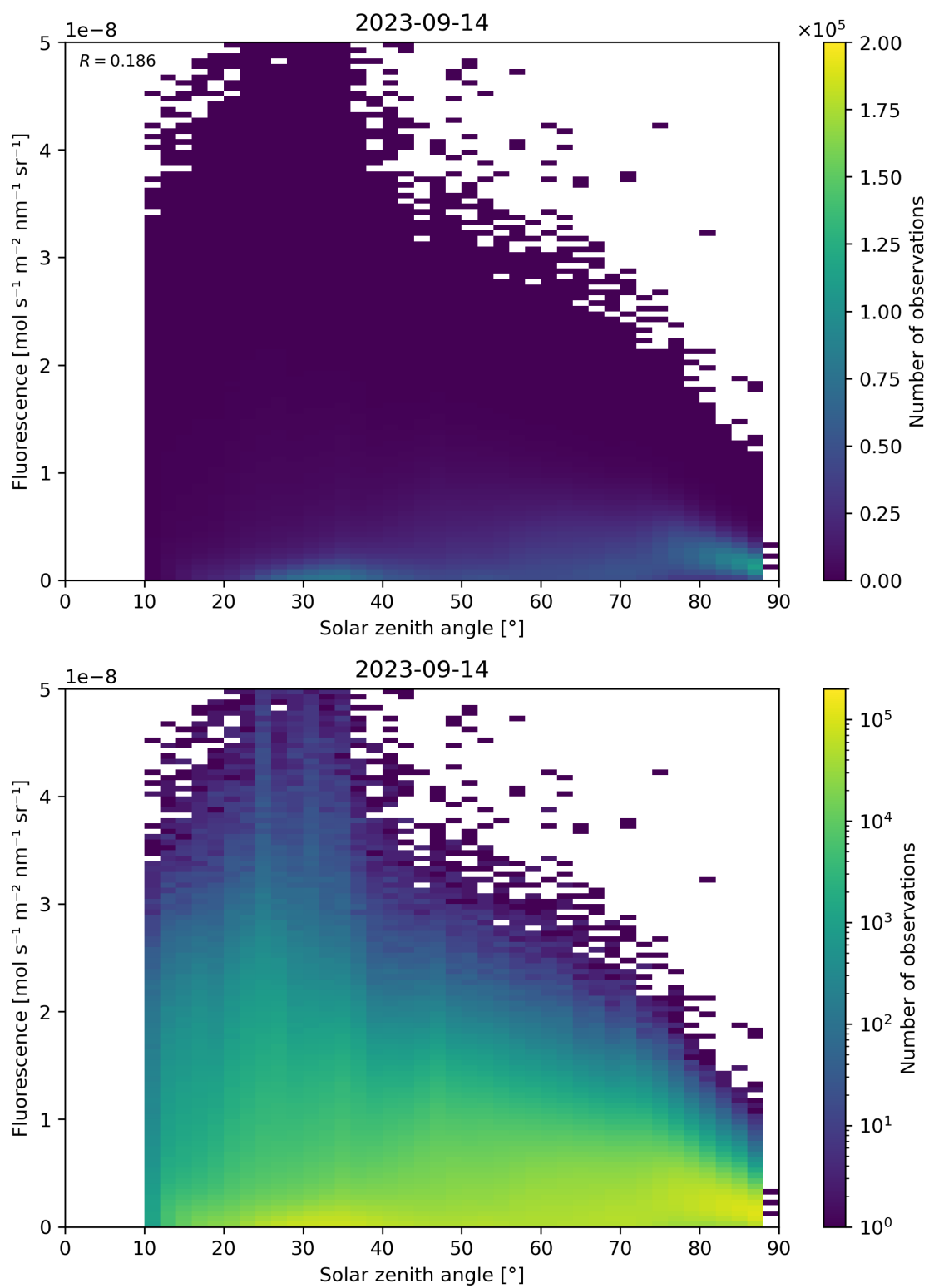
Figure 123: Scatter density plot of “Solar zenith angle” against “Fluorescence” for 2023-09-13 to 2023-09-15.
