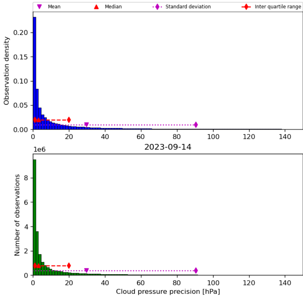
Figure 31: Histogram of “Cloud pressure precision” for 2023-09-13 to 2023-09-15
