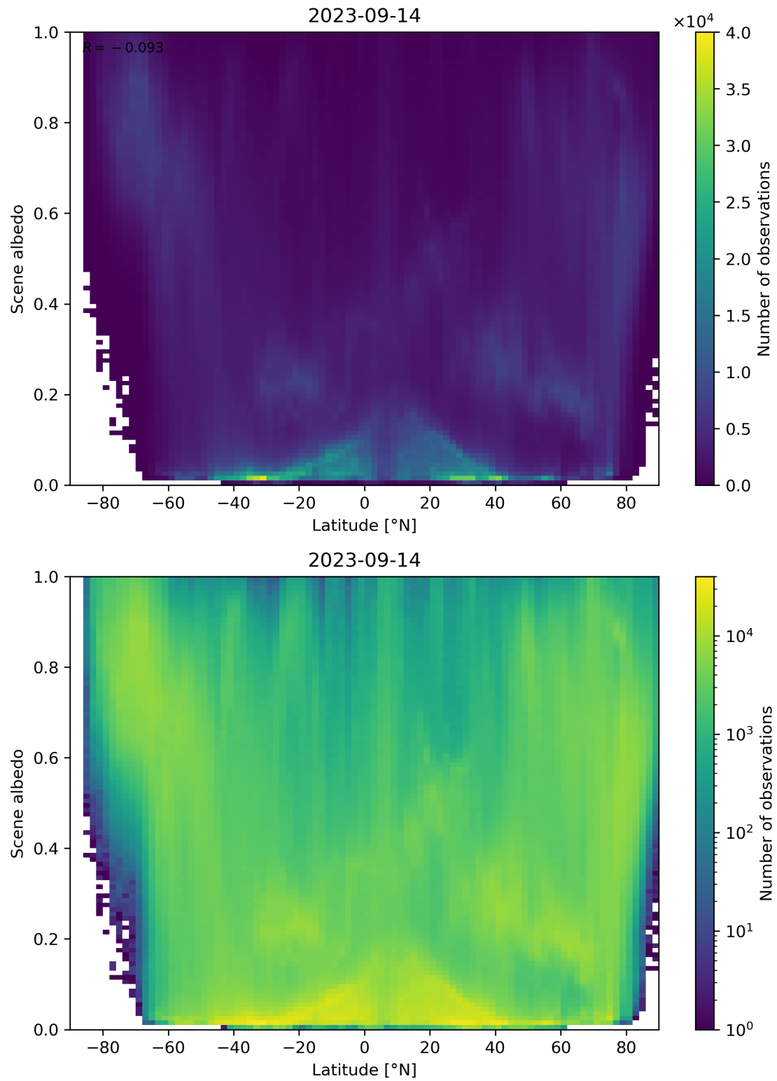
Figure 104: Scatter density plot of “Latitude” against “Scene albedo” for 2023-09-13 to 2023-09-15.
