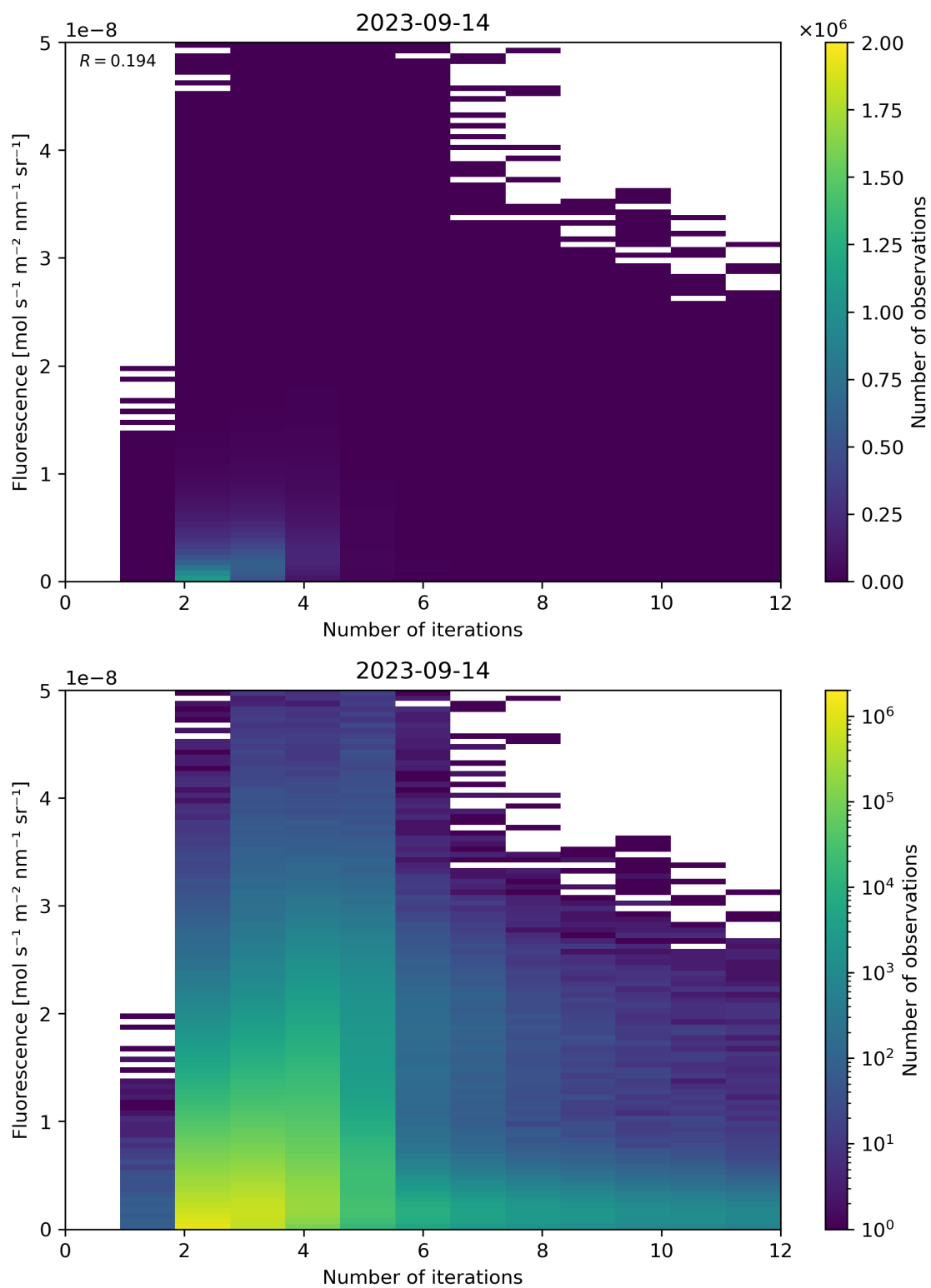
Figure 107: Scatter density plot of “Number of iterations” against “Fluorescence” for 2023-09-13 to 2023-09-15.
