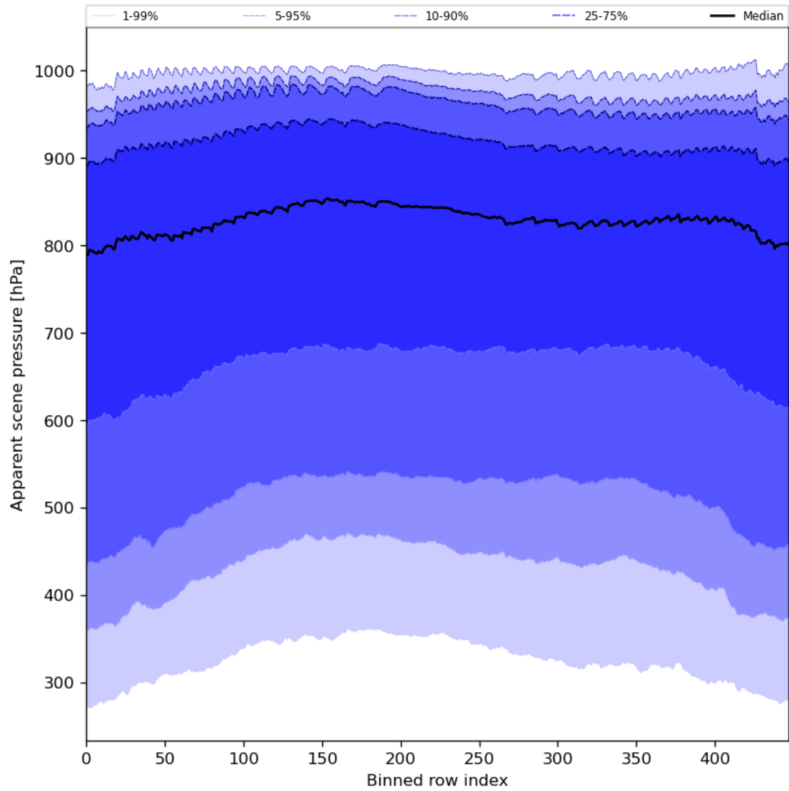
Figure 53: Along track statistics of “Apparent scene pressure” for 2023-09-13 to 2023-09-15
