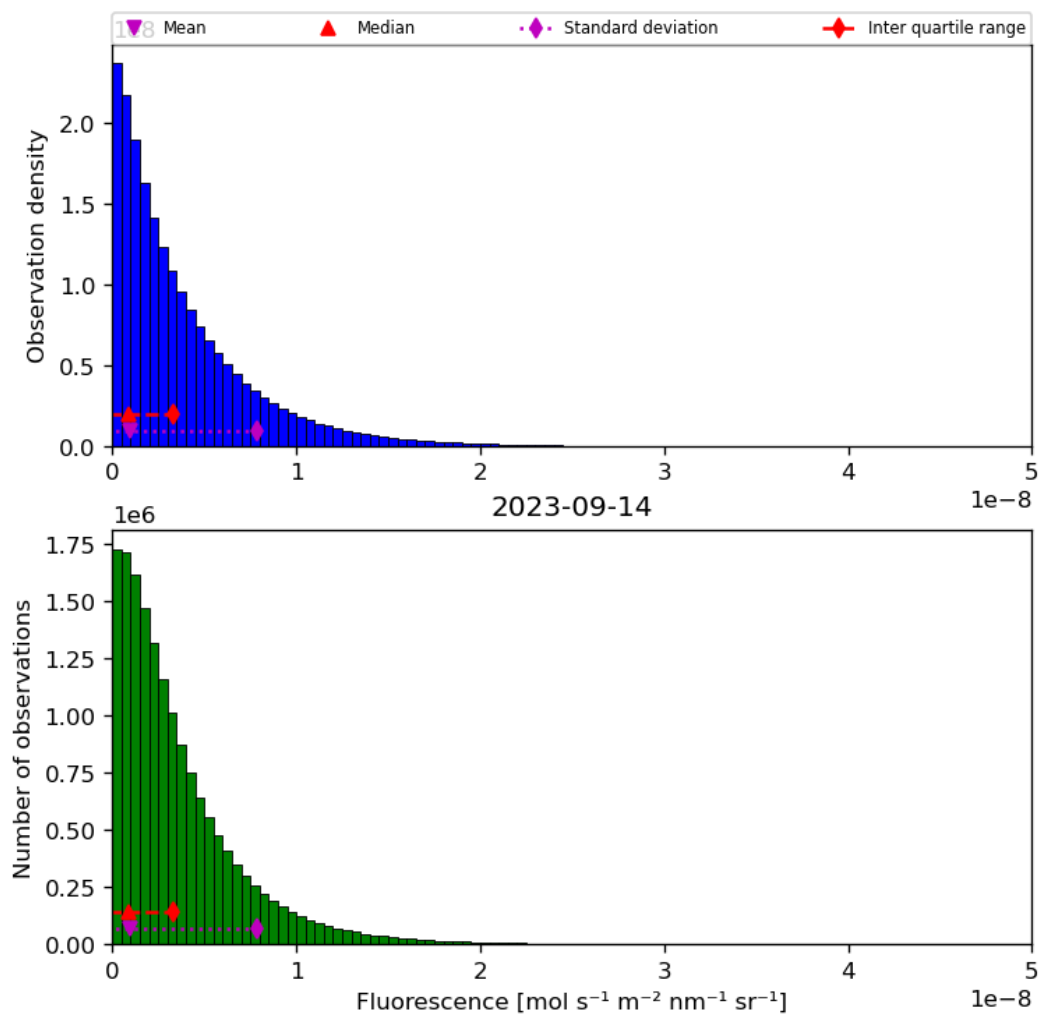
Figure 40: Histogram of “Fluorescence” for 2023-09-13 to 2023-09-15
