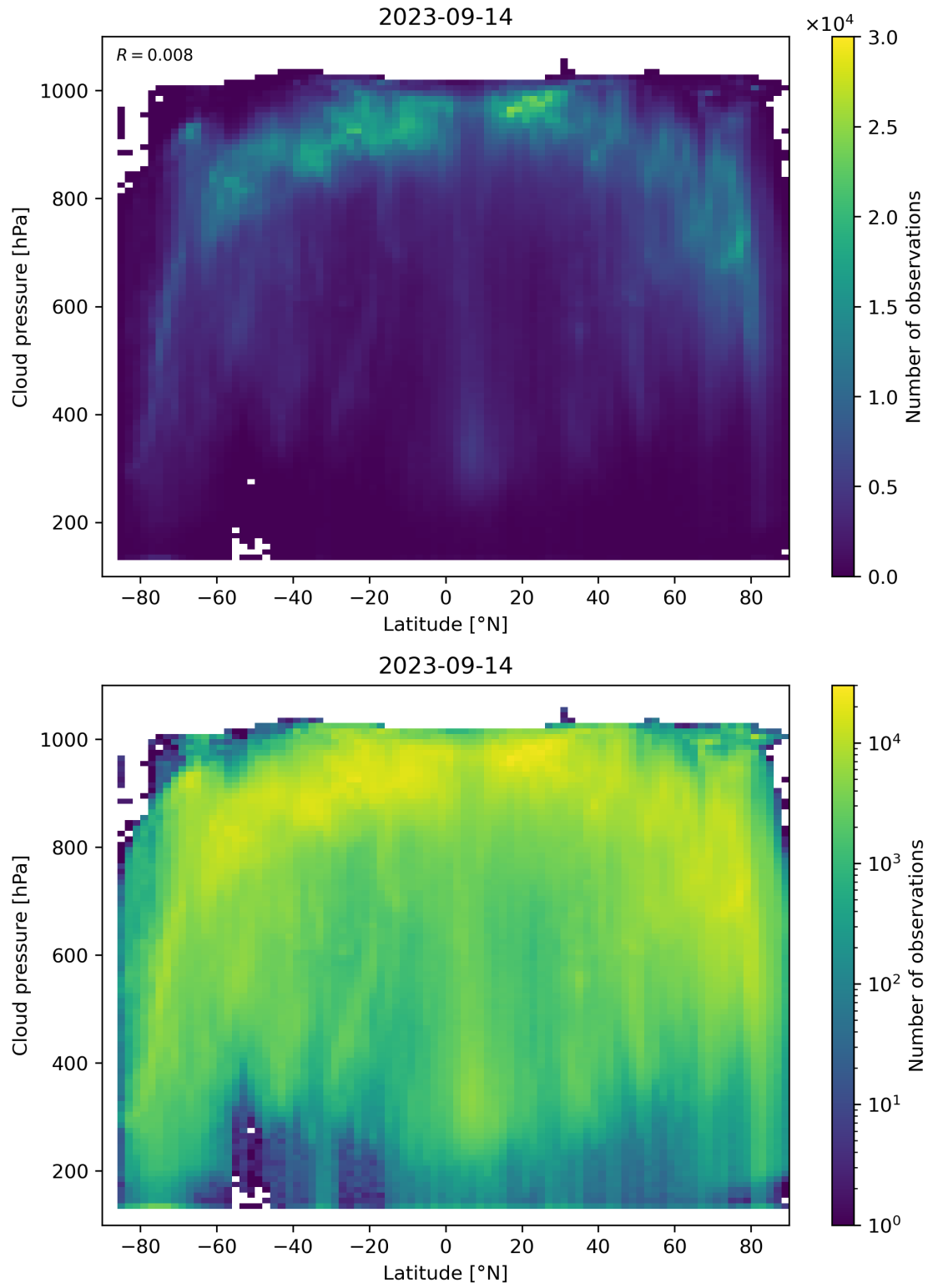
Figure 100: Scatter density plot of “Latitude” against “Cloud pressure” for 2023-09-13 to 2023-09-15.
