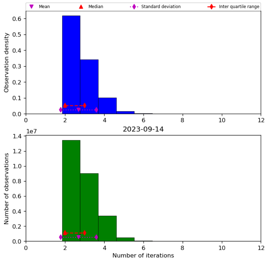
Figure 39: Histogram of “Number of iterations” for 2023-09-13 to 2023-09-15
