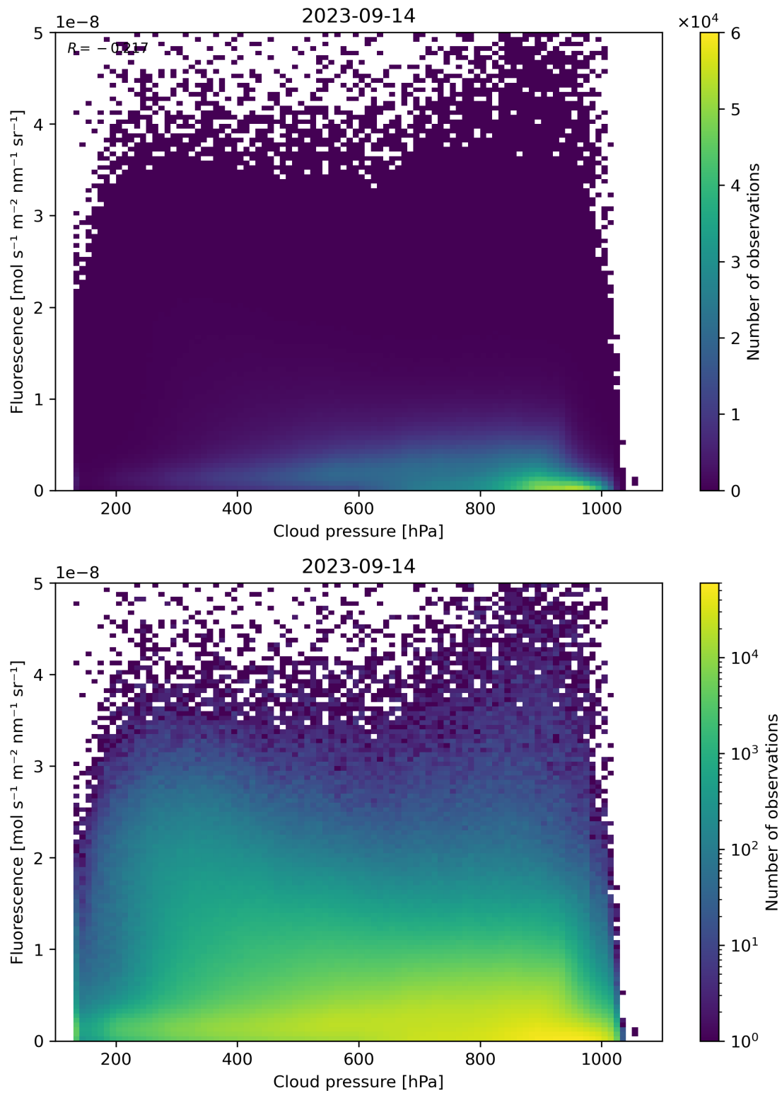
Figure 88: Scatter density plot of “Cloud pressure” against “Fluorescence” for 2023-09-13 to 2023-09-15.
