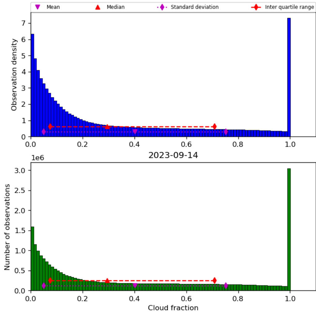
Figure 32: Histogram of “Cloud fraction” for 2023-09-13 to 2023-09-15
