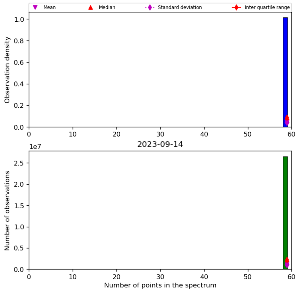
Figure 44: Histogram of “Number of points in the spectrum” for 2023-09-13 to 2023-09-15
