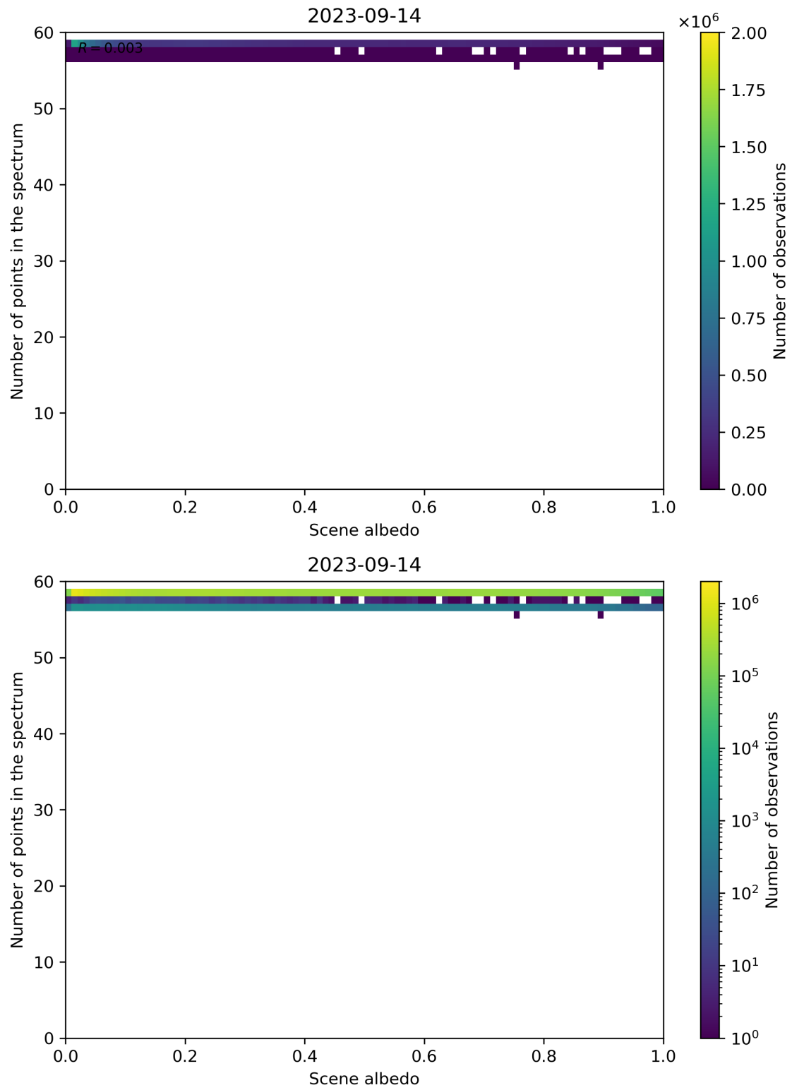
Figure 116: Scatter density plot of “Scene albedo” against “Number of points in the spectrum” for 2023-09-13 to 2023-09-15.
