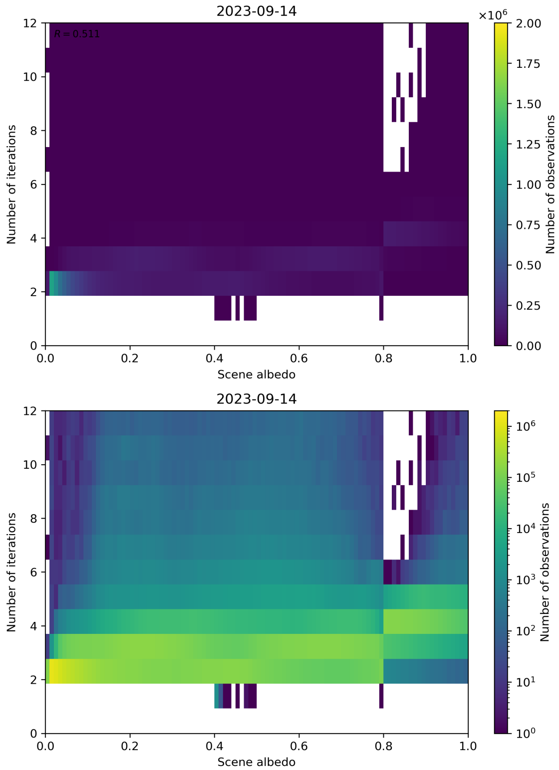
Figure 115: Scatter density plot of “Scene albedo” against “Number of iterations” for 2023-09-13 to 2023-09-15.
