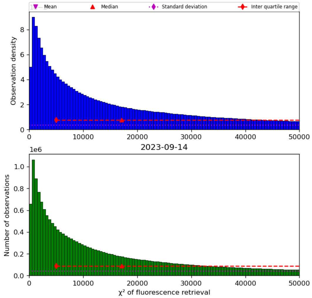
Figure 42: Histogram of “ \chi^2 of fluorescence retrieval” for 2023-09-13 to 2023-09-15
