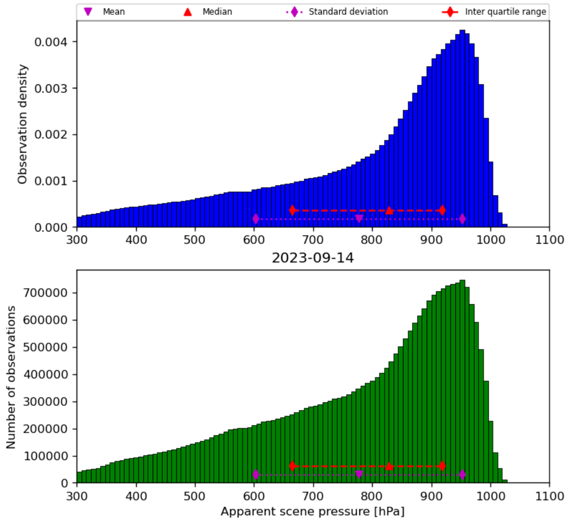
Figure 36: Histogram of “Apparent scene pressure” for 2023-09-13 to 2023-09-15
