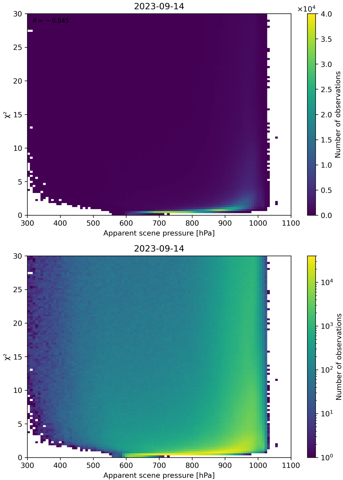
Figure 63: Scatter density plot of “Apparent scene pressure” against “ \chi^2 ” for 2023-09-13 to 2023-09-15.
