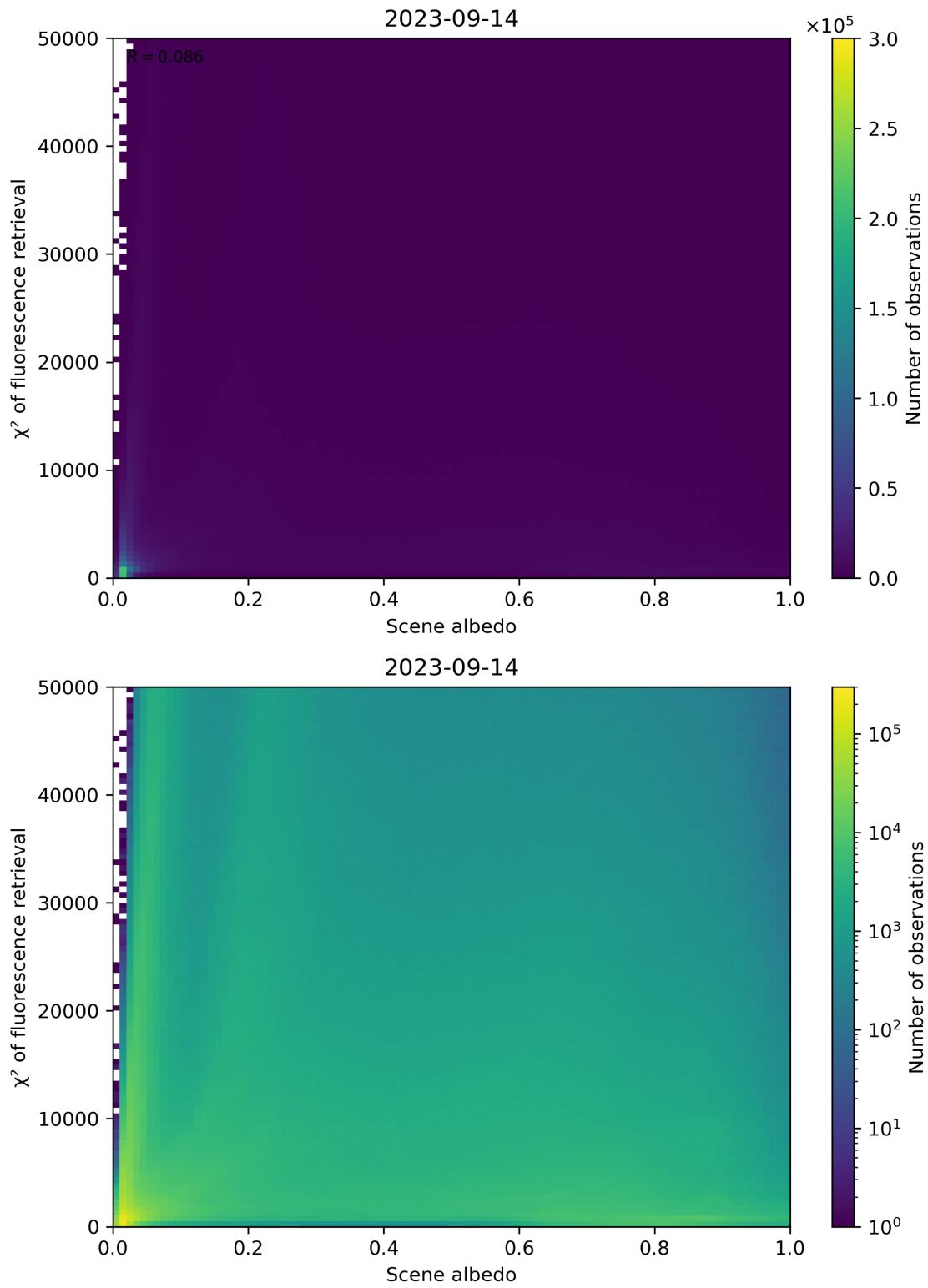
Figure 113: Scatter density plot of “Scene albedo” against “ \chi^2 of fluorescence retrieval” for 2023-09-13 to 2023-09-15.
