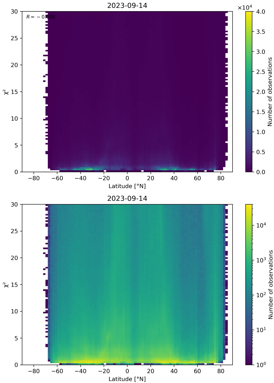
Figure 97: Scatter density plot of “Latitude” against “ \chi^2 ” for 2023-09-13 to 2023-09-15.
