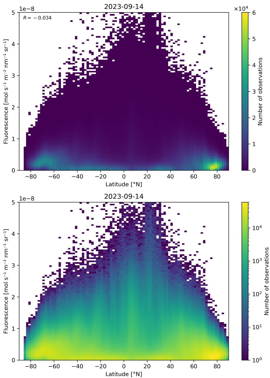
Figure 101: Scatter density plot of “Latitude” against “Fluorescence” for 2023-09-13 to 2023-09-15.
