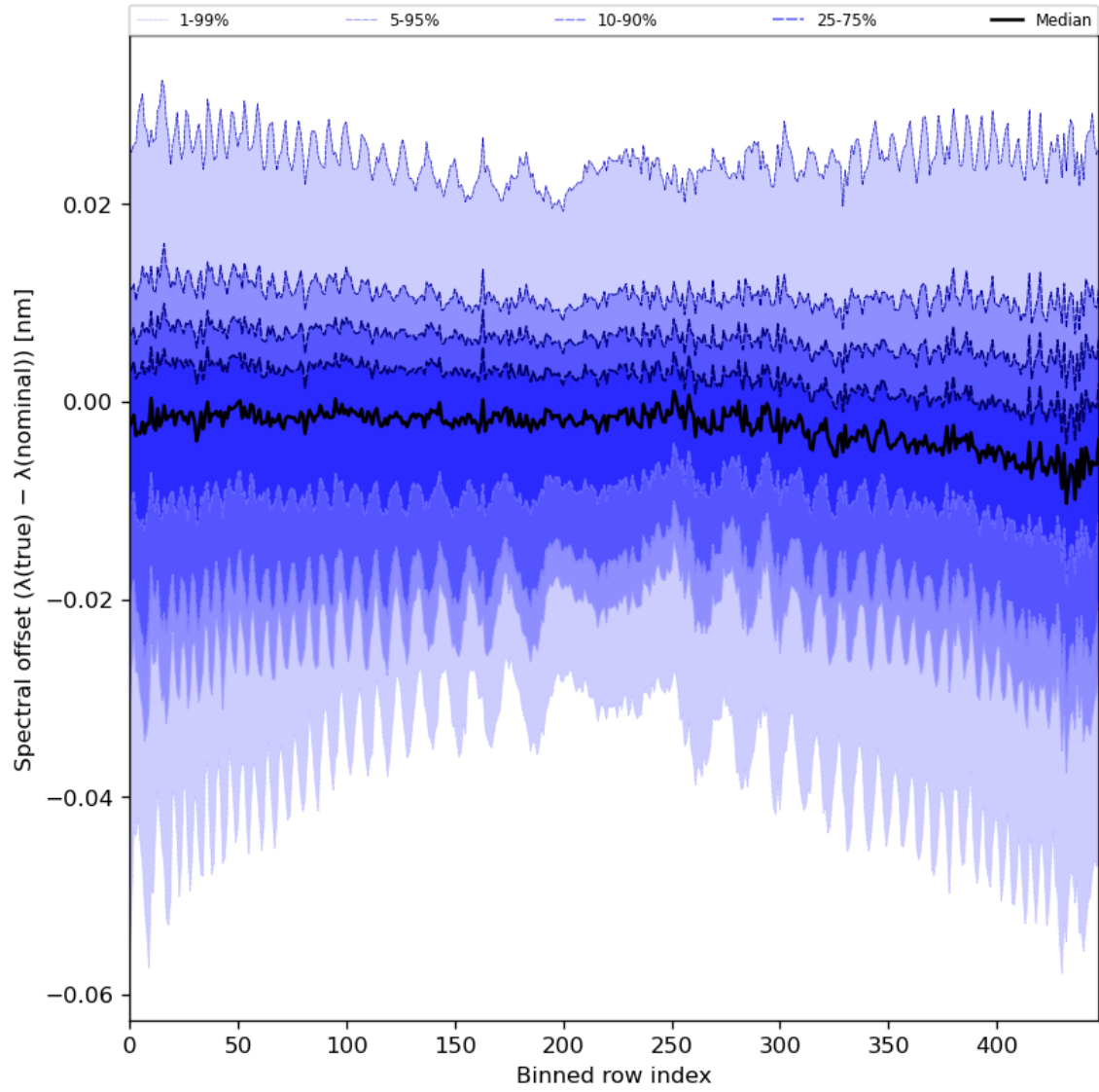
Figure 62: Along track statistics of “Spectral offset ( \lambda(\text{true}) - \lambda(\text{nominal}) )” for 2023-09-13 to 2023-09-15
