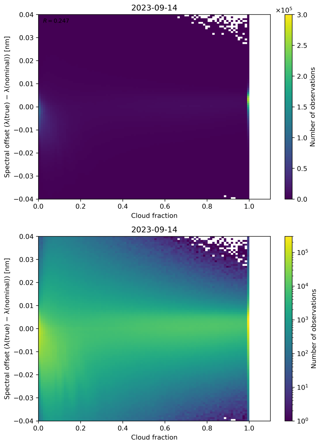
Figure 83: Scatter density plot of “Cloud fraction” against “Spectral offset ( \lambda(\text{true}) - \lambda(\text{nominal}) )” for 2023-09-13 to 2023-09-15.
