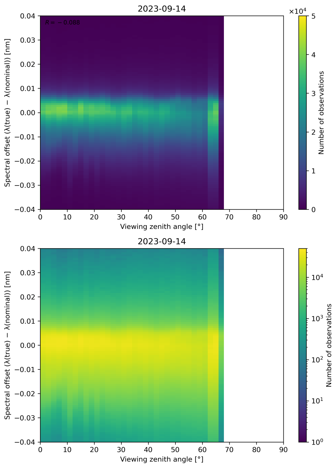
Figure 140: Scatter density plot of “Viewing zenith angle” against “Spectral offset ( \lambda(\text{true}) - \lambda(\text{nominal}) )” for 2023-09-13 to 2023-09-15.
