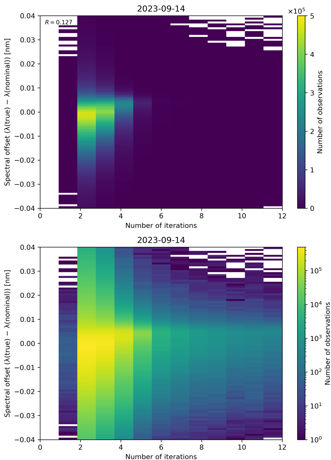
Figure 109: Scatter density plot of “Number of iterations” against “Spectral offset ( \lambda(\text{true}) - \lambda(\text{nominal}) )” for 2023-09-13 to 2023-09-15.
