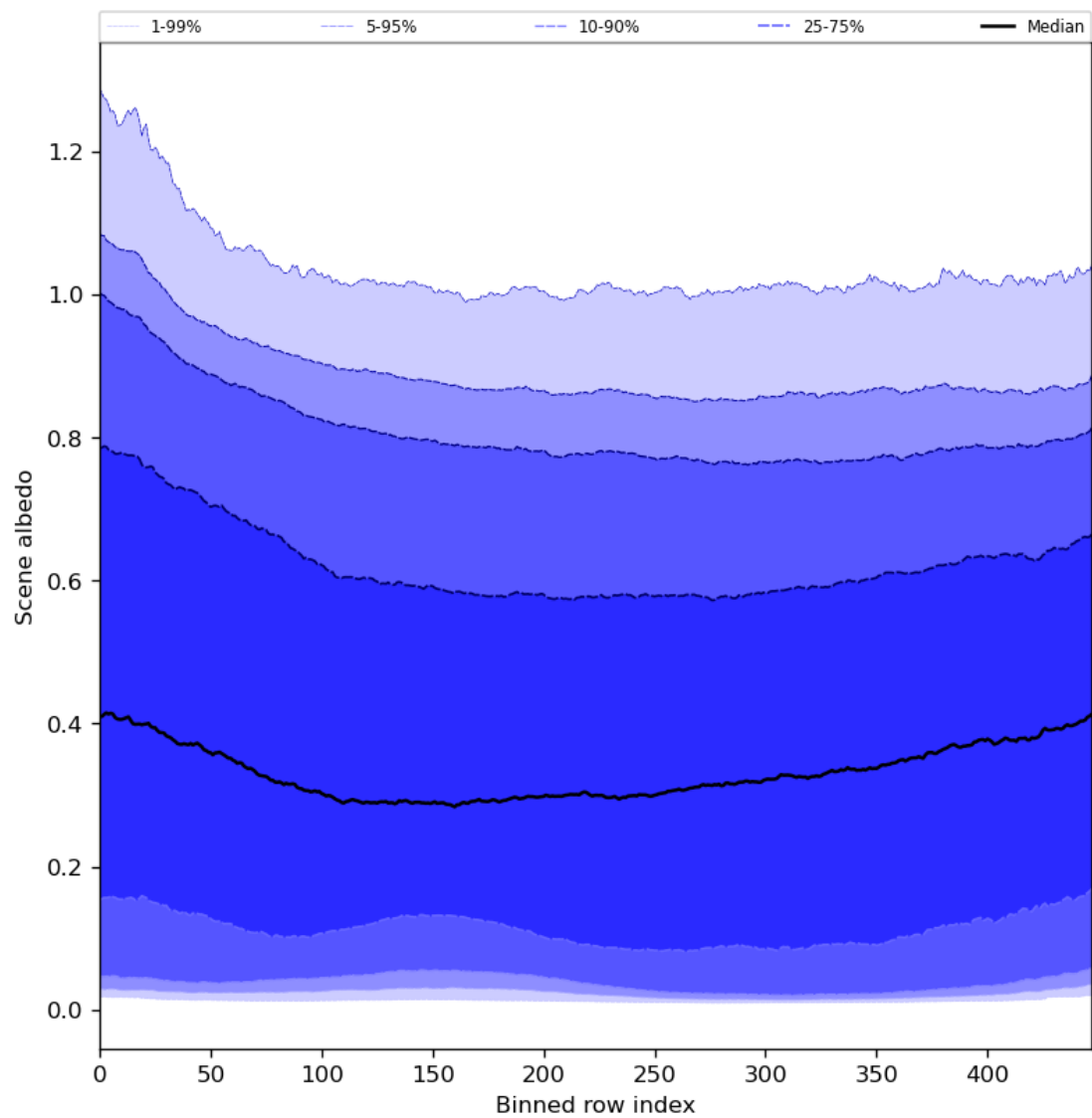
Figure 51: Along track statistics of “Scene albedo” for 2023-09-13 to 2023-09-15
