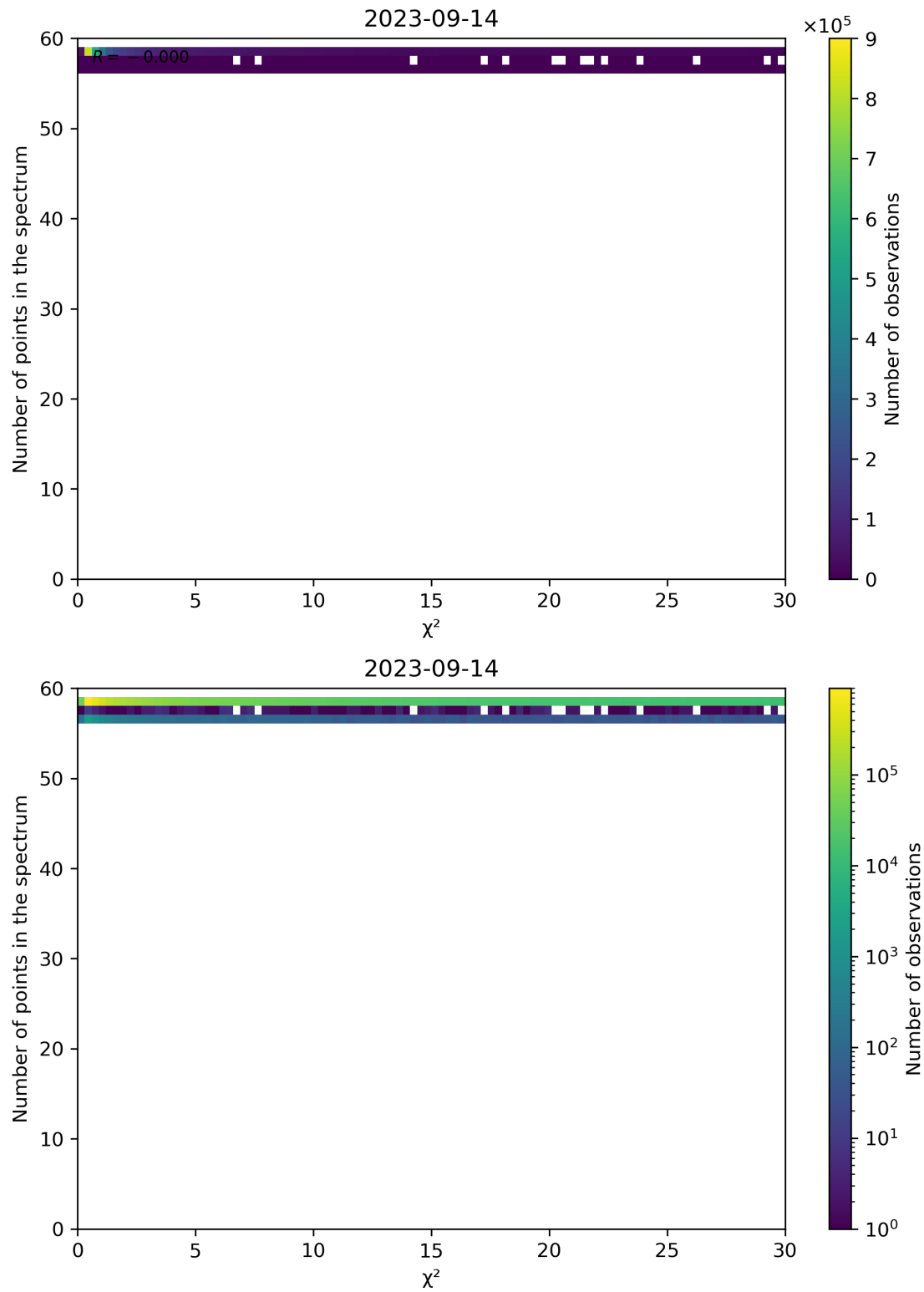
Figure 74: Scatter density plot of “ \chi^2 ” against “Number of points in the spectrum” for 2023-09-13 to 2023-09-15.
