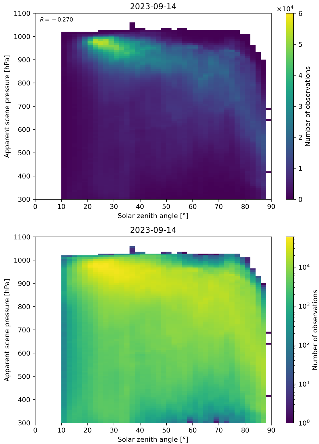
Figure 118: Scatter density plot of “Solar zenith angle” against “Apparent scene pressure” for 2023-09-13 to 2023-09-15.
