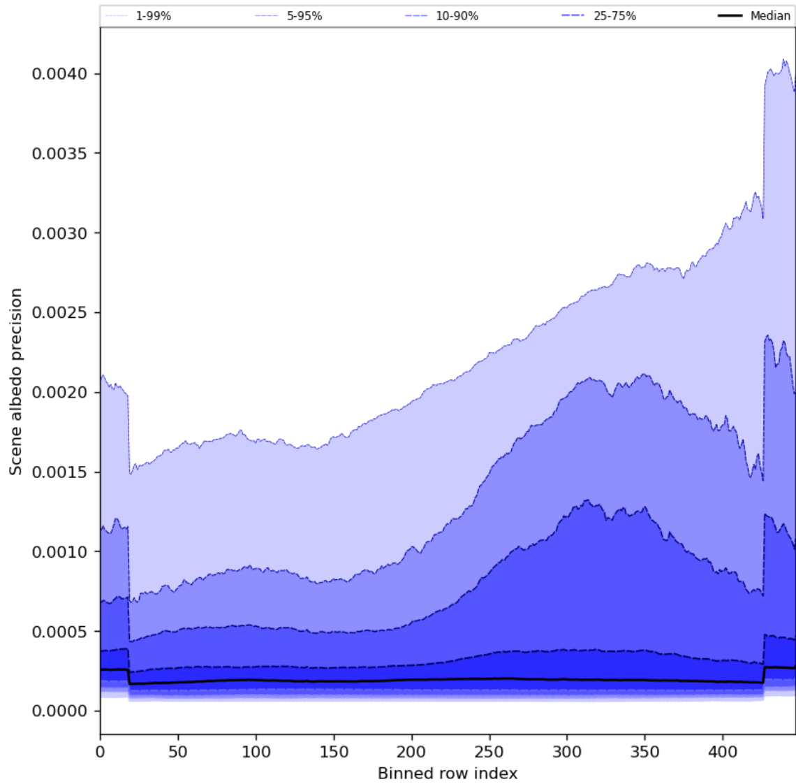
Figure 52: Along track statistics of “Scene albedo precision” for 2023-09-13 to 2023-09-15
