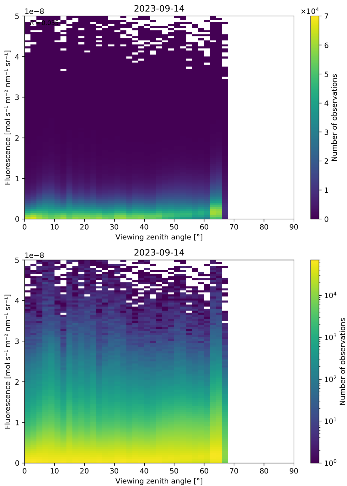
Figure 134: Scatter density plot of “Viewing zenith angle” against “Fluorescence” for 2023-09-13 to 2023-09-15.
