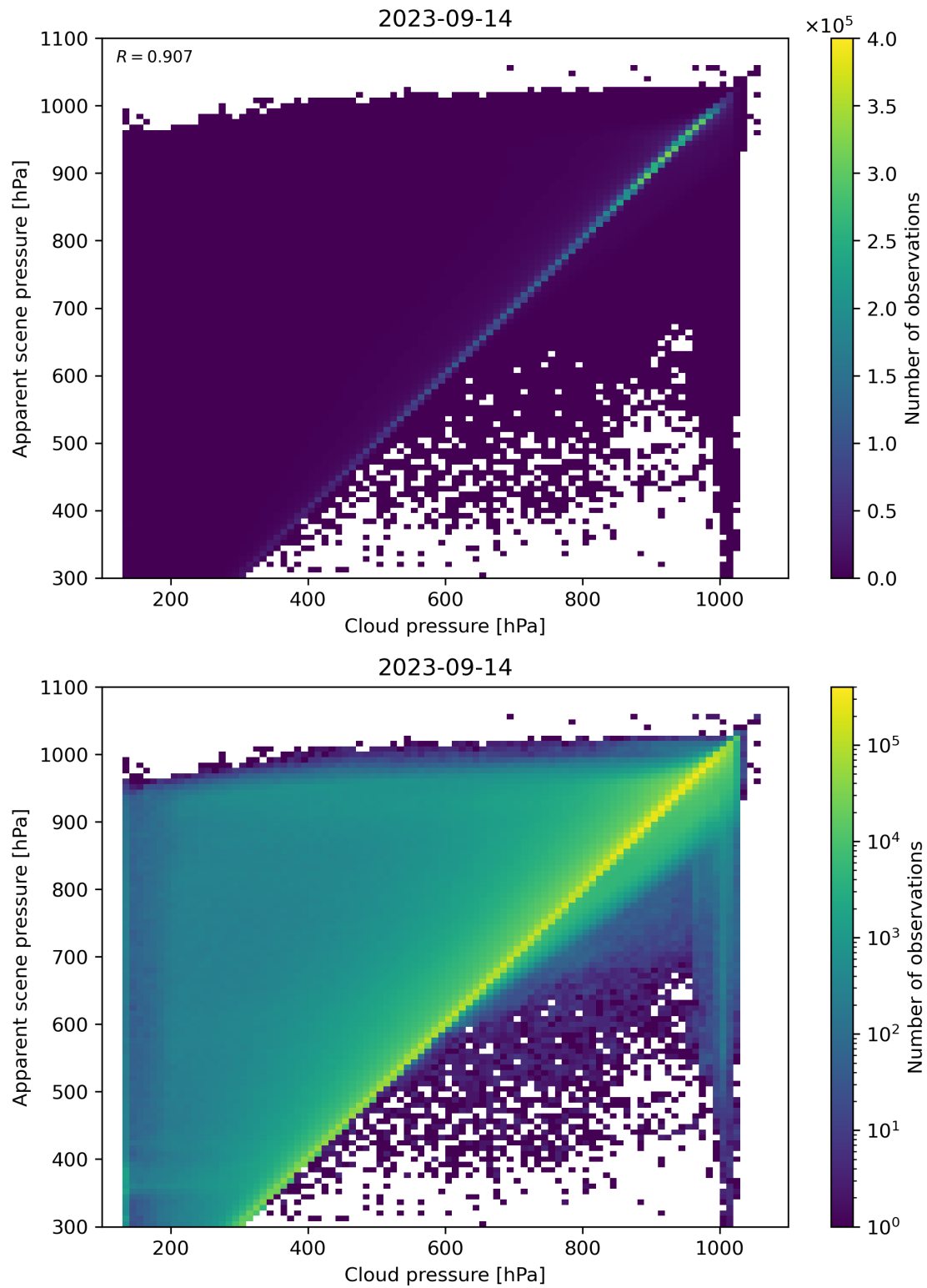
Figure 84: Scatter density plot of “Cloud pressure” against “Apparent scene pressure” for 2023-09-13 to 2023-09-15.
