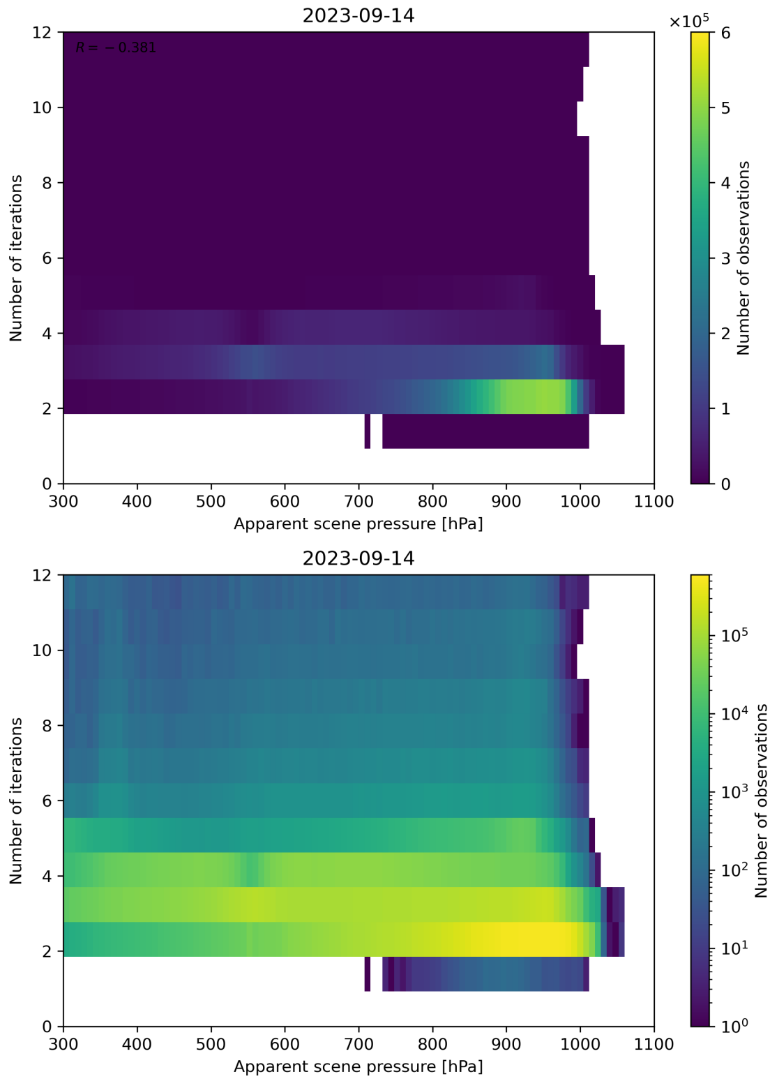
Figure 66: Scatter density plot of “Apparent scene pressure” against “Number of iterations” for 2023-09-13 to 2023-09-15.
