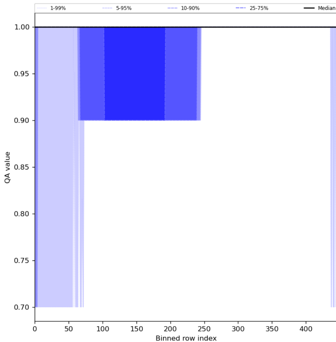
Figure 46: Along track statistics of “QA value” for 2023-09-13 to 2023-09-15
