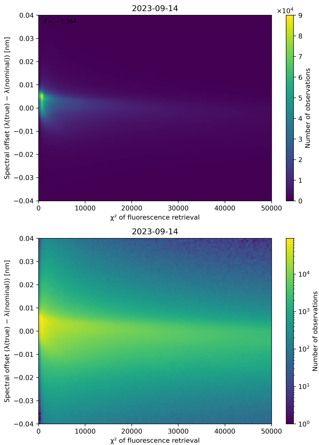
Figure 72: Scatter density plot of “ \chi^2 of fluorescence retrieval” against “Spectral offset ( \lambda(\text{true}) - \lambda(\text{nominal}) )” for 2023-09-13 to 2023-09-15.
