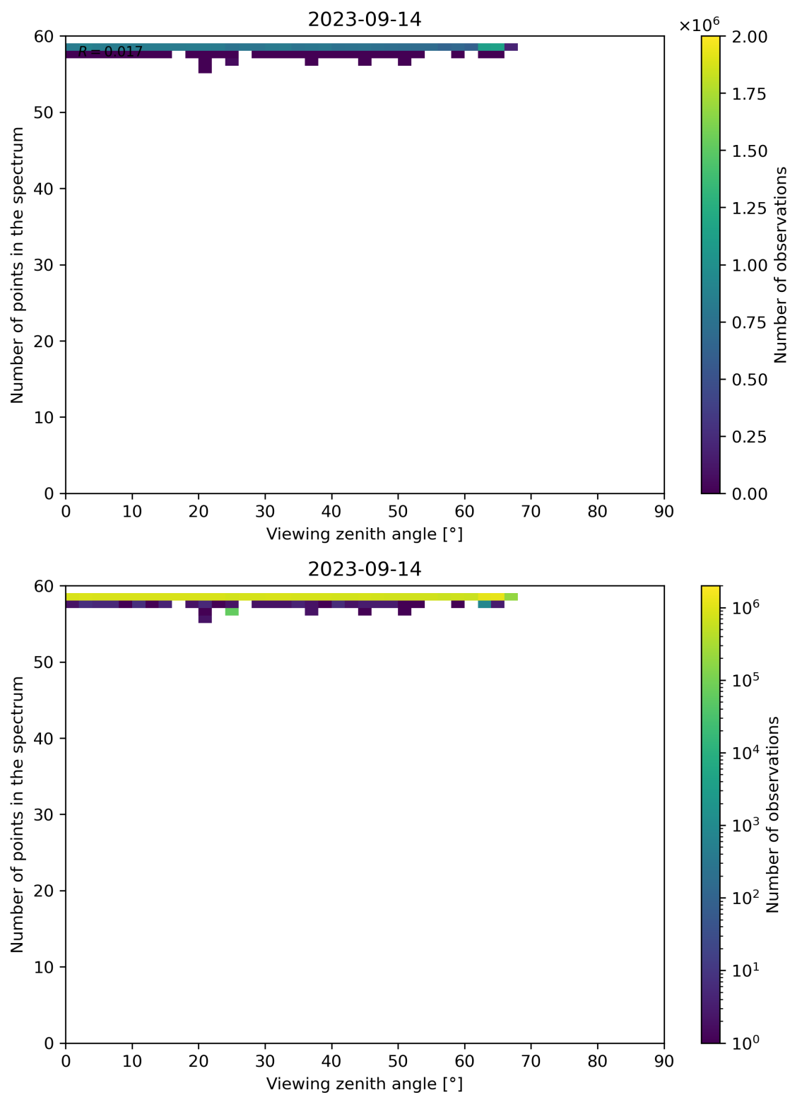
Figure 137: Scatter density plot of “Viewing zenith angle” against “Number of points in the spectrum” for 2023-09-13 to 2023-09-15.
