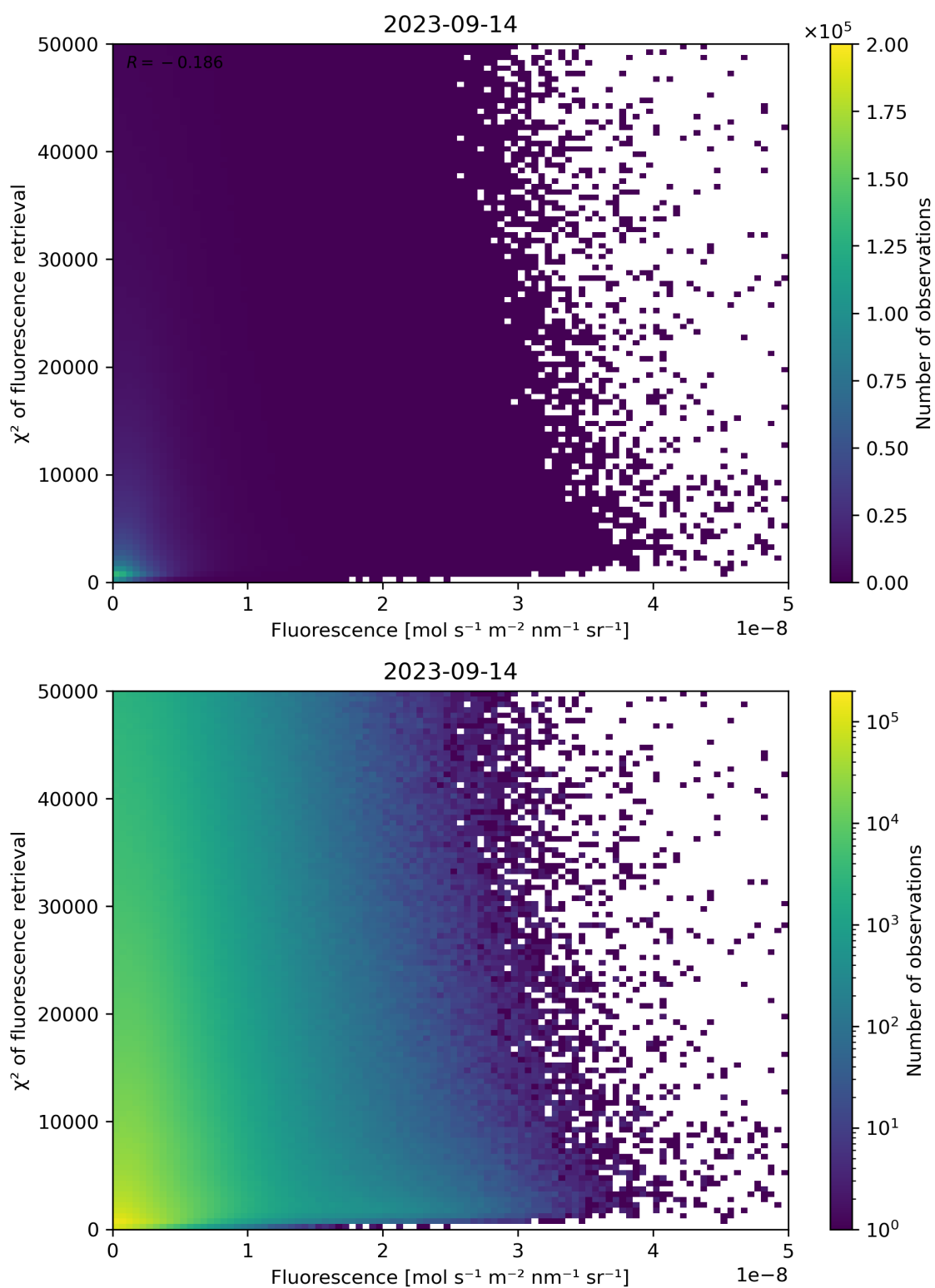
Figure 93: Scatter density plot of “Fluorescence” against “ \chi^2 of fluorescence retrieval” for 2023-09-13 to 2023-09-15.
