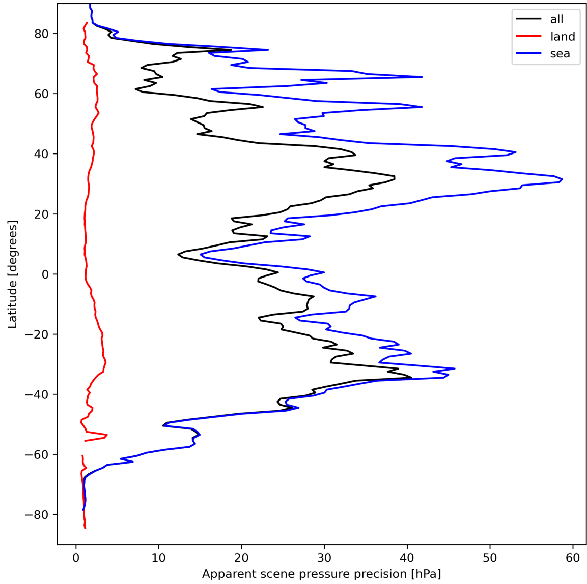
Figure 20: Zonal average of “Apparent scene pressure precision” for 2023-09-13 to 2023-09-15.
