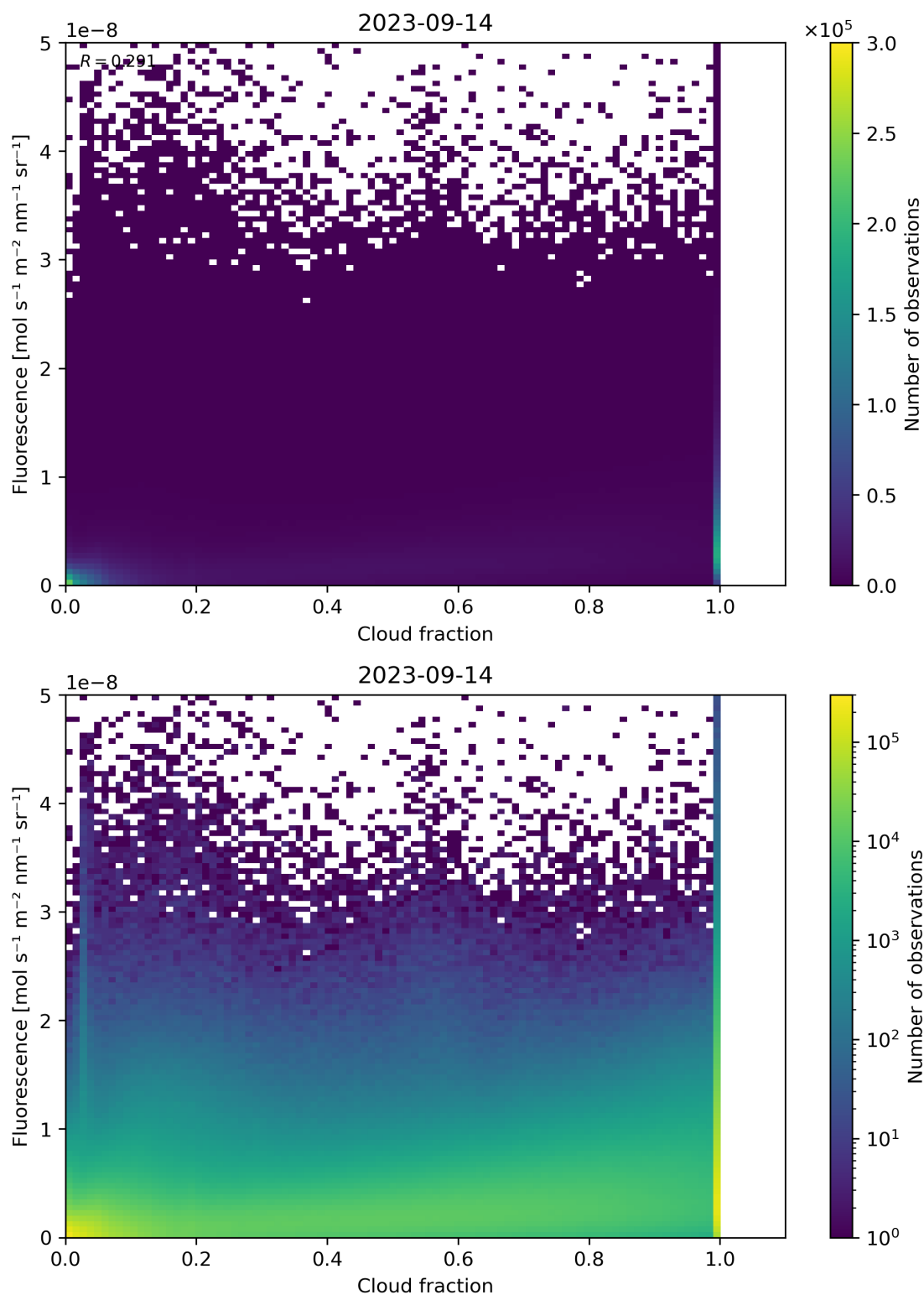
Figure 79: Scatter density plot of “Cloud fraction” against “Fluorescence” for 2023-09-13 to 2023-09-15.
