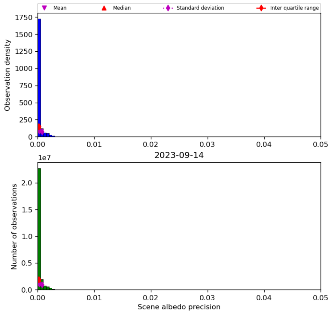
Figure 35: Histogram of “Scene albedo precision” for 2023-09-13 to 2023-09-15
