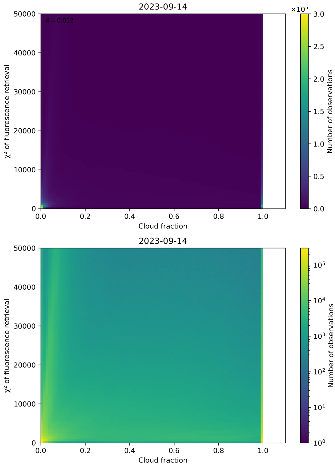
Figure 78: Scatter density plot of “Cloud fraction” against “ \chi^2 of fluorescence retrieval” for 2023-09-13 to 2023-09-15.
