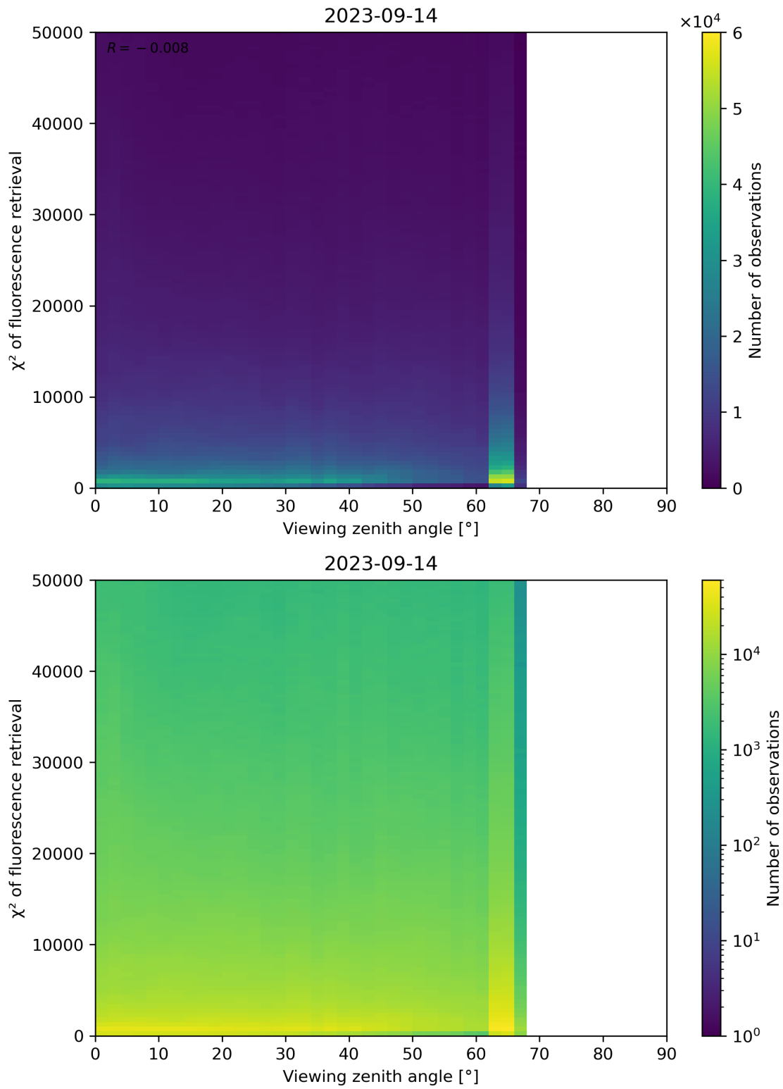
Figure 131: Scatter density plot of “Viewing zenith angle” against “ \chi^2 of fluorescence retrieval” for 2023-09-13 to 2023-09-15.
