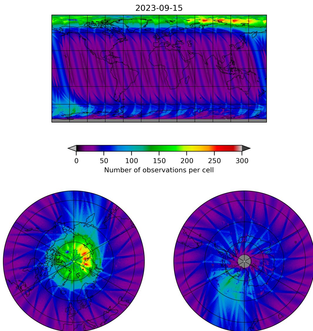
Figure 11: Map of the number of observations for 2023-09-15 to 2023-09-16
