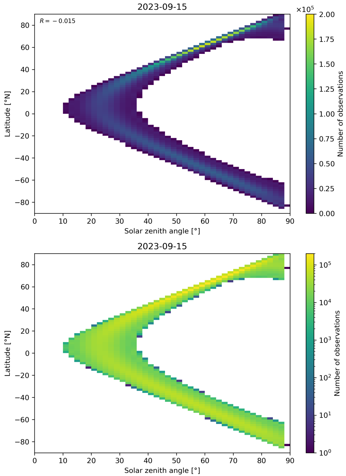
Figure 124: Scatter density plot of “Solar zenith angle” against “Latitude” for 2023-09-15 to 2023-09-16.
