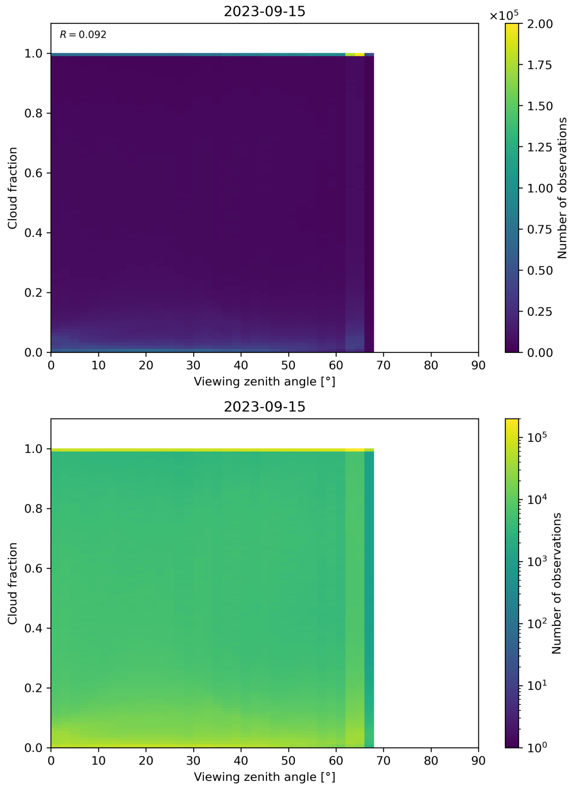
Figure 132: Scatter density plot of “Viewing zenith angle” against “Cloud fraction” for 2023-09-15 to 2023-09-16.
