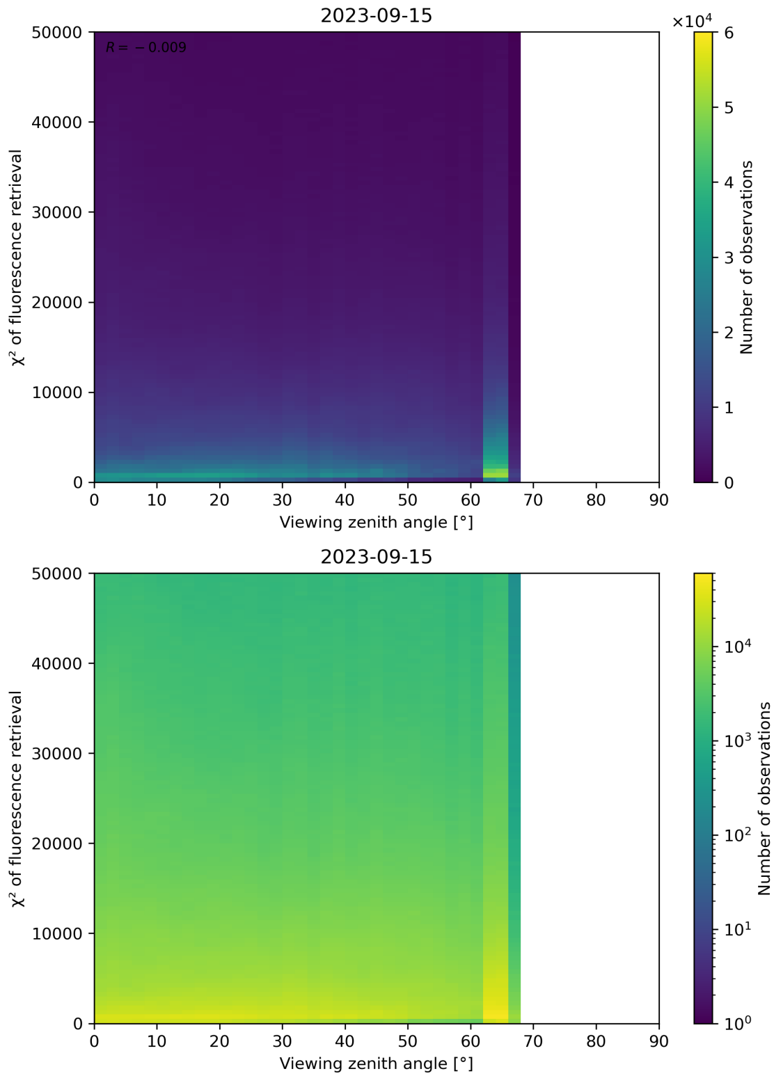
Figure 131: Scatter density plot of “Viewing zenith angle” against “ \chi^2 of fluorescence retrieval” for 2023-09-15 to 2023-09-16.
