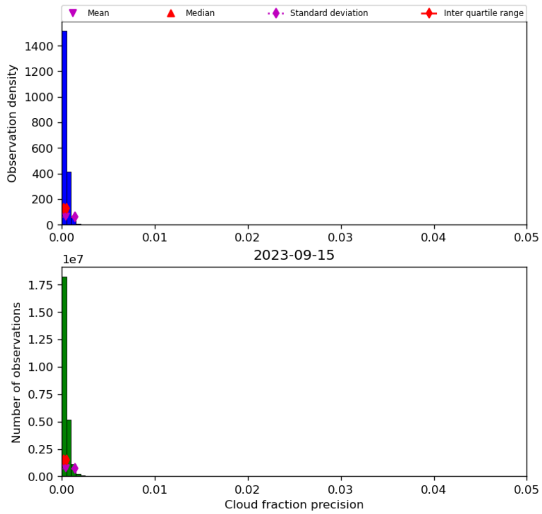
Figure 33: Histogram of “Cloud fraction precision” for 2023-09-15 to 2023-09-16
