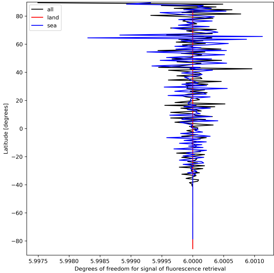
Figure 26: Zonal average of “Degrees of freedom for signal of fluorescence retrieval” for 2023-09-15 to 2023-09-16.
