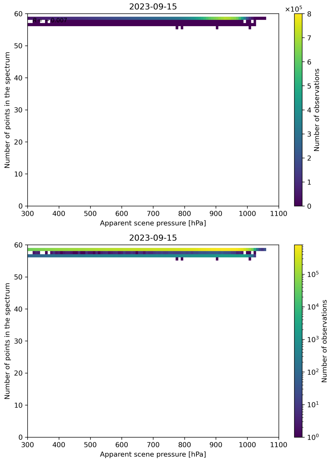
Figure 67: Scatter density plot of “Apparent scene pressure” against “Number of points in the spectrum” for 2023-09-15 to 2023-09-16.
