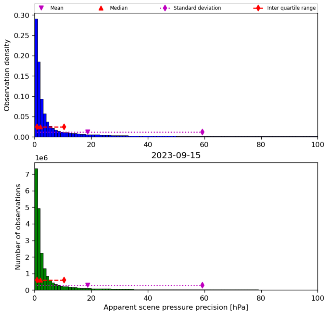
Figure 37: Histogram of “Apparent scene pressure precision” for 2023-09-15 to 2023-09-16
