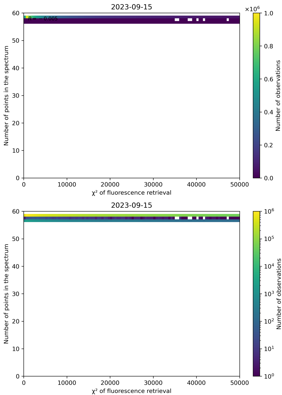
Figure 71: Scatter density plot of “ \chi^2 of fluorescence retrieval” against “Number of points in the spectrum” for 2023-09-15 to 2023-09-16.
