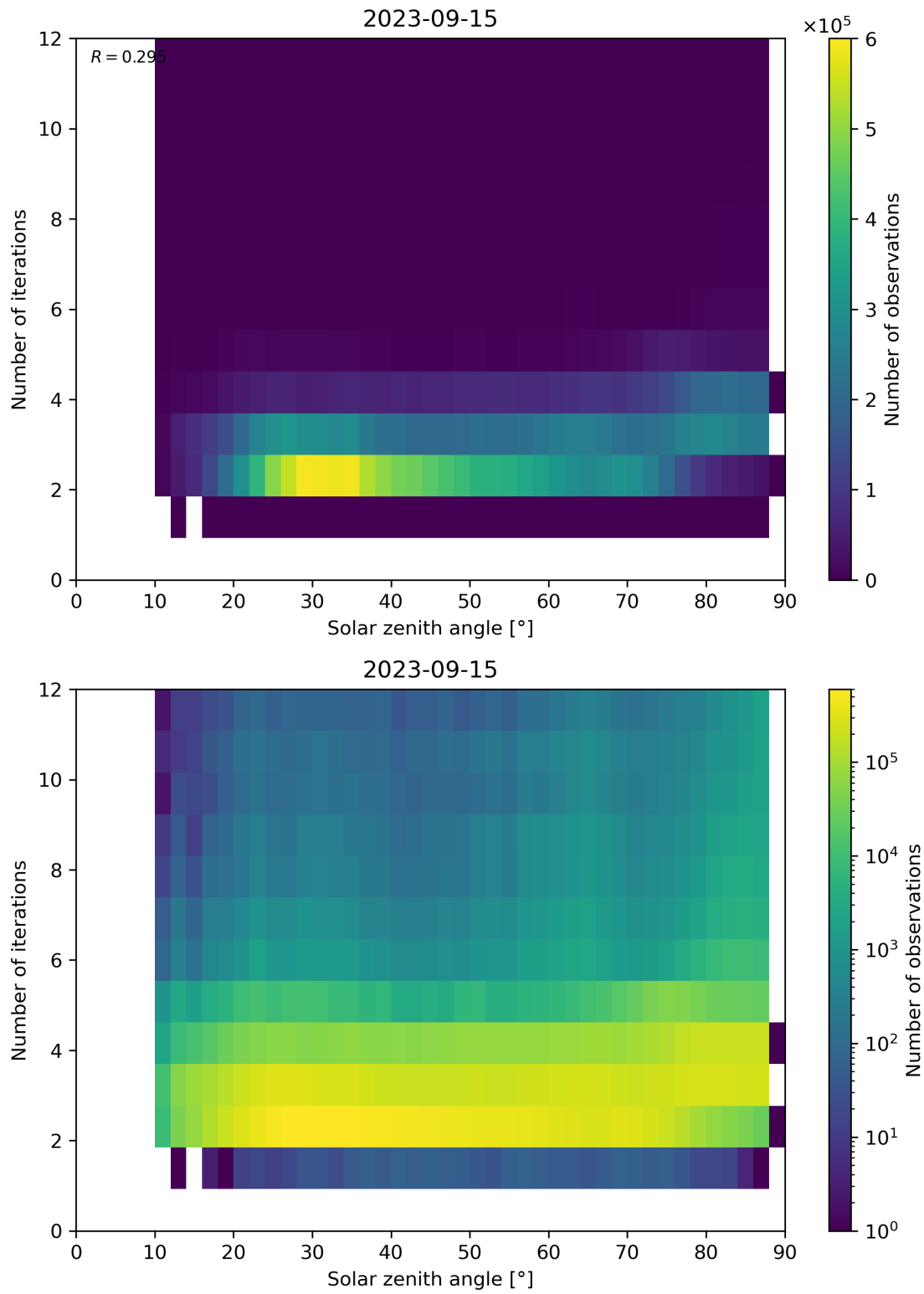
Figure 125: Scatter density plot of “Solar zenith angle” against “Number of iterations” for 2023-09-15 to 2023-09-16.
