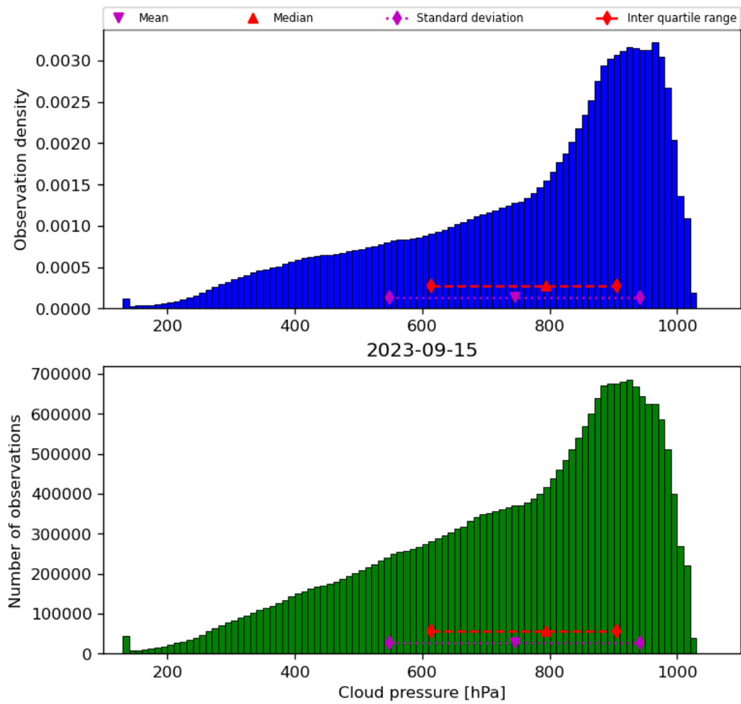
Figure 30: Histogram of “Cloud pressure” for 2023-09-15 to 2023-09-16
