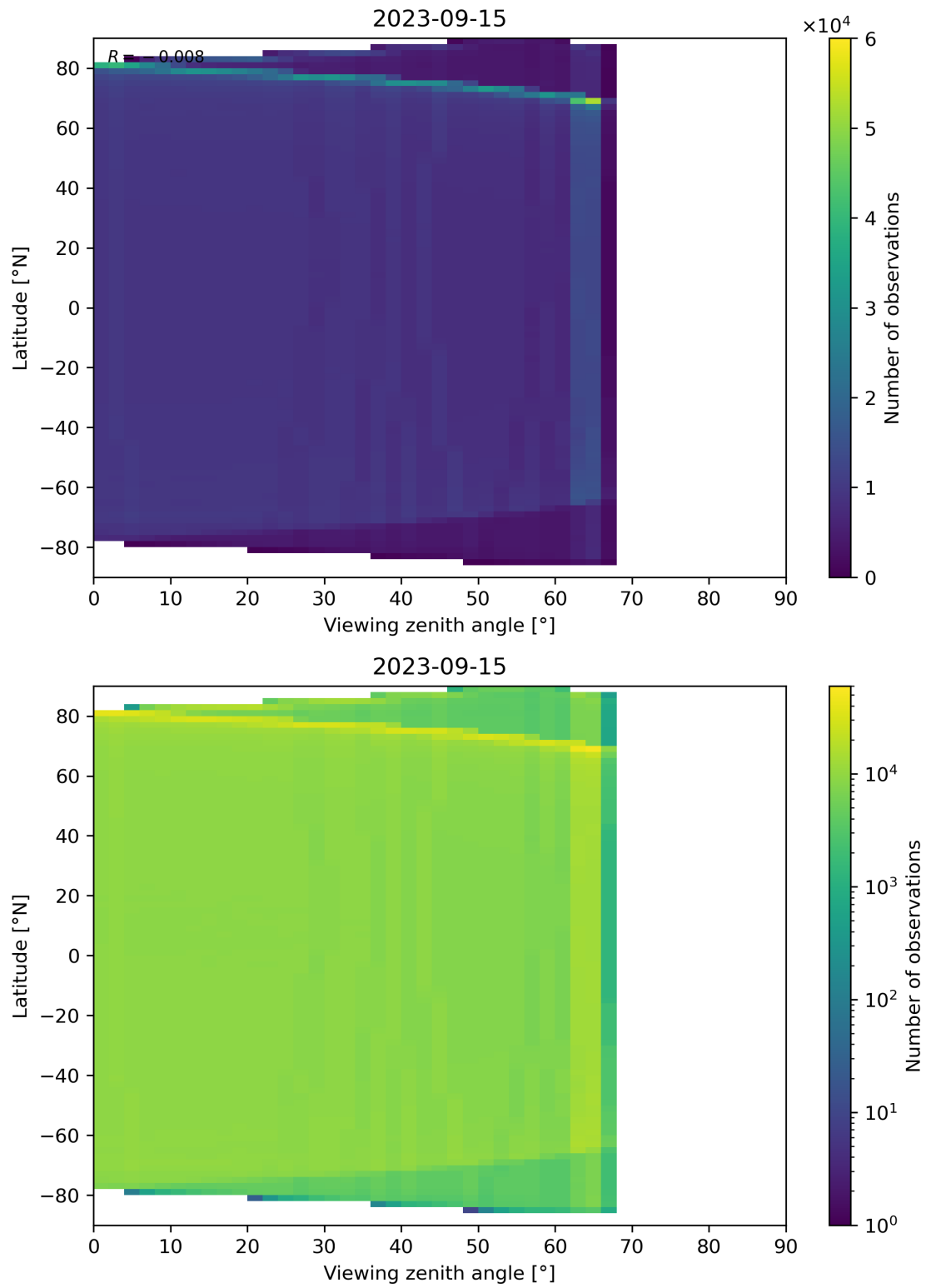
Figure 135: Scatter density plot of “Viewing zenith angle” against “Latitude” for 2023-09-15 to 2023-09-16.
