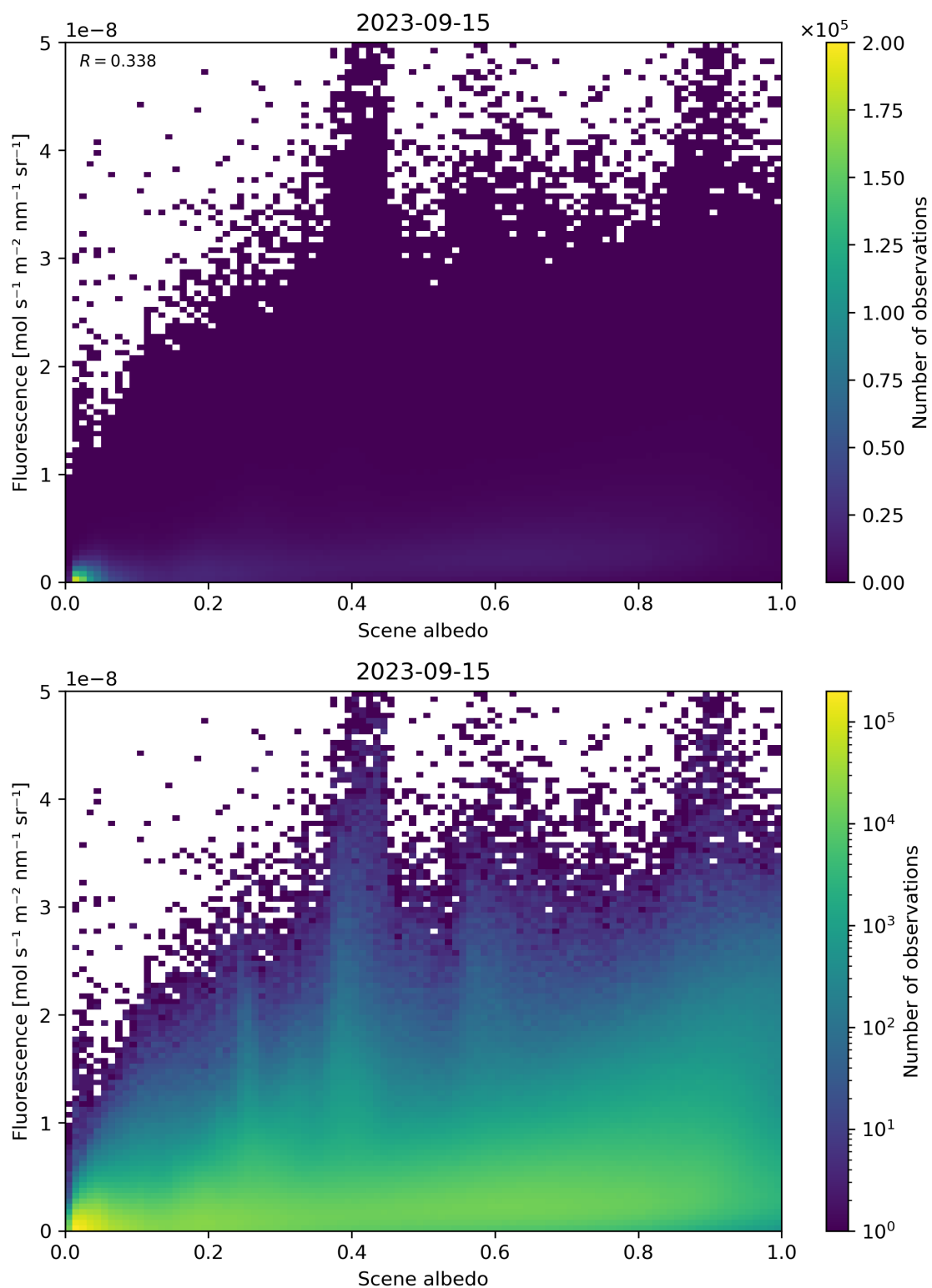
Figure 114: Scatter density plot of “Scene albedo” against “Fluorescence” for 2023-09-15 to 2023-09-16.
