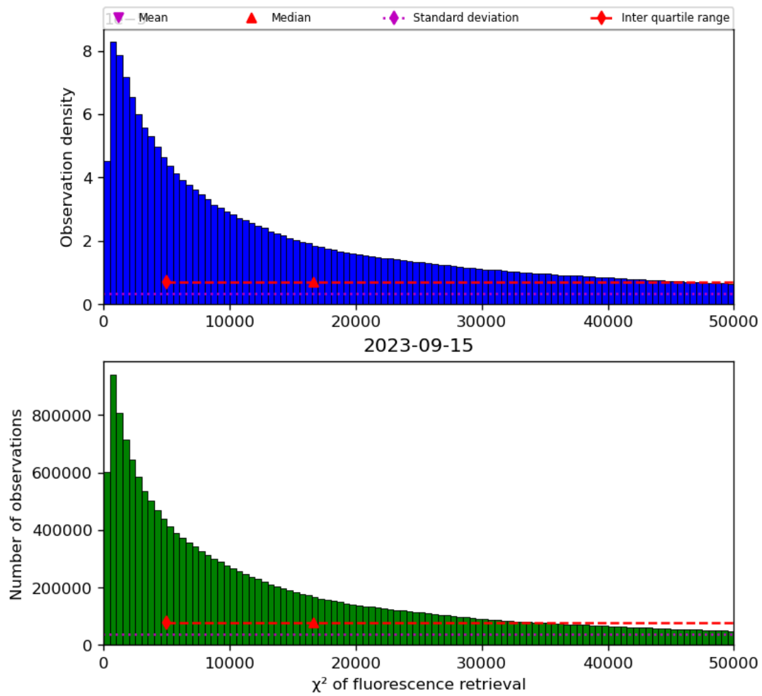
Figure 42: Histogram of “ \chi^2 of fluorescence retrieval” for 2023-09-15 to 2023-09-16
