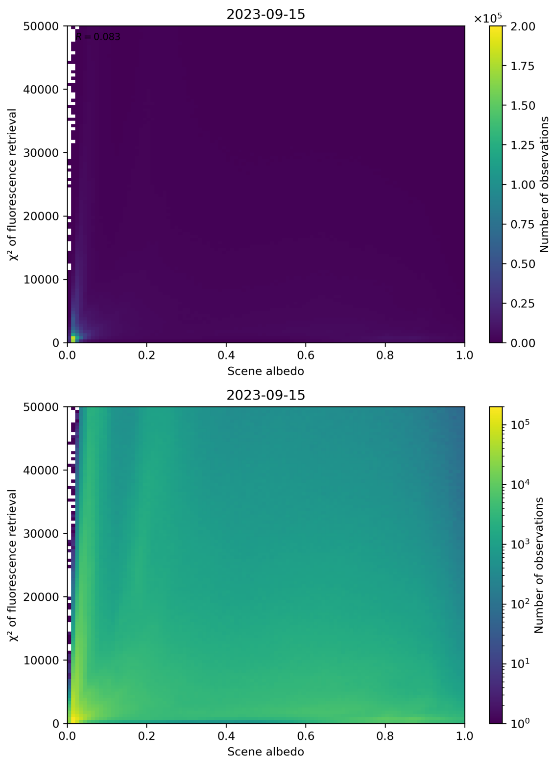
Figure 113: Scatter density plot of “Scene albedo” against “ \chi^2 of fluorescence retrieval” for 2023-09-15 to 2023-09-16.
