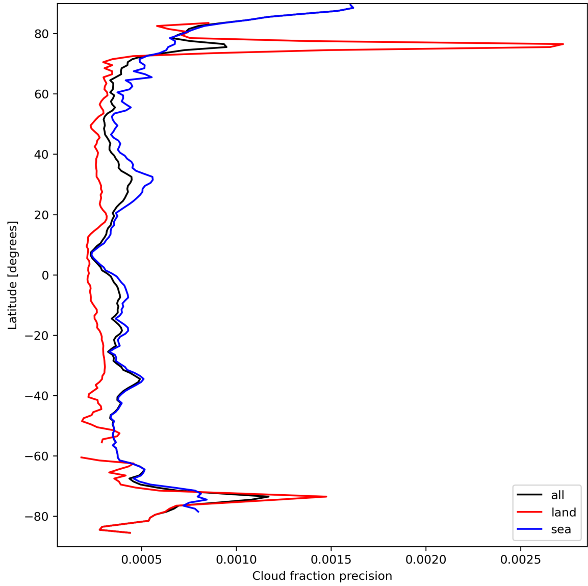
Figure 16: Zonal average of “Cloud fraction precision” for 2023-09-15 to 2023-09-16.
