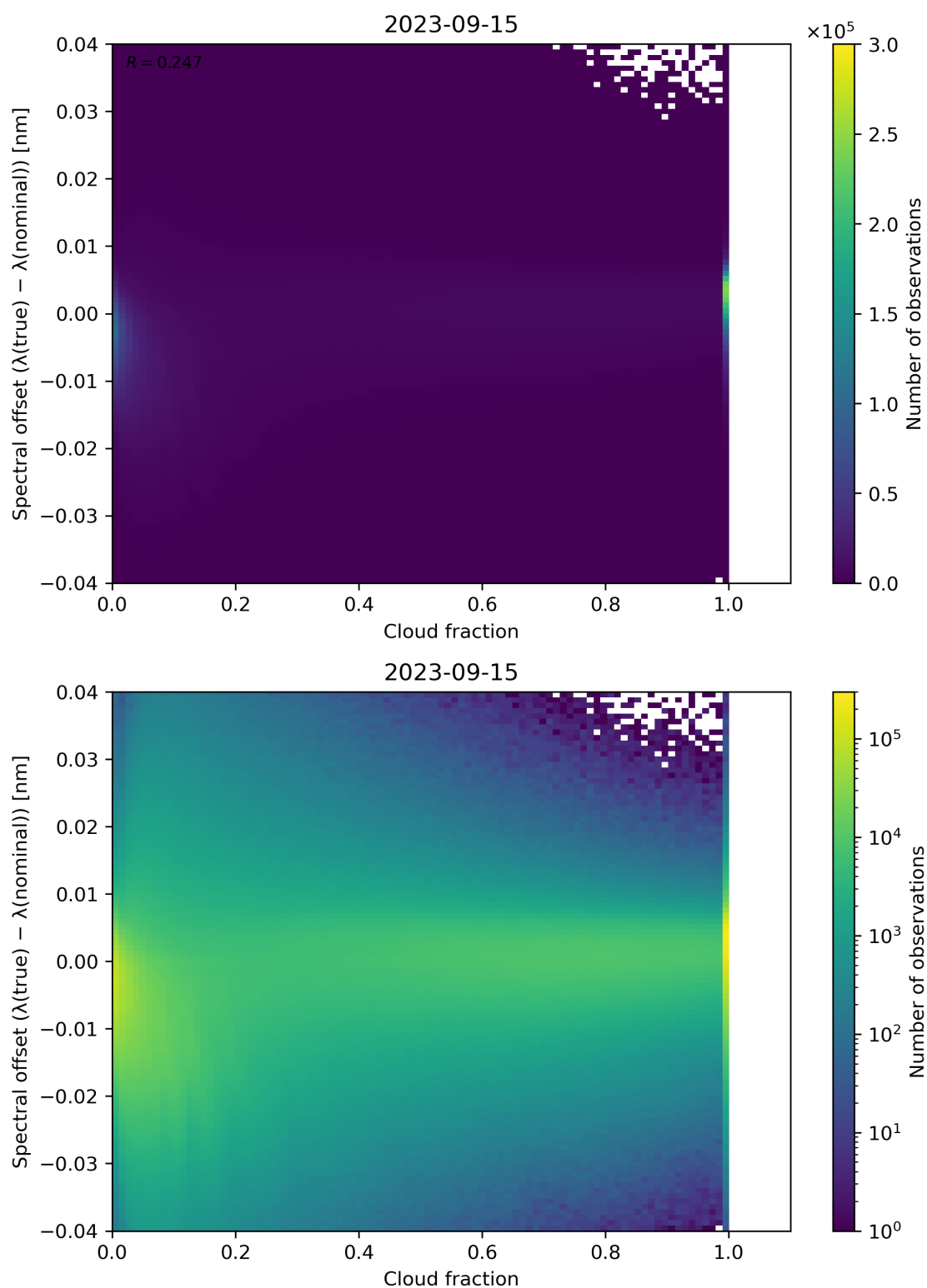
Figure 83: Scatter density plot of “Cloud fraction” against “Spectral offset ( \lambda(\text{true}) - \lambda(\text{nominal}) )” for 2023-09-15 to 2023-09-16.
