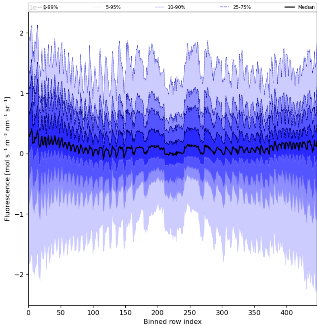
Figure 57: Along track statistics of “Fluorescence” for 2023-09-15 to 2023-09-16
