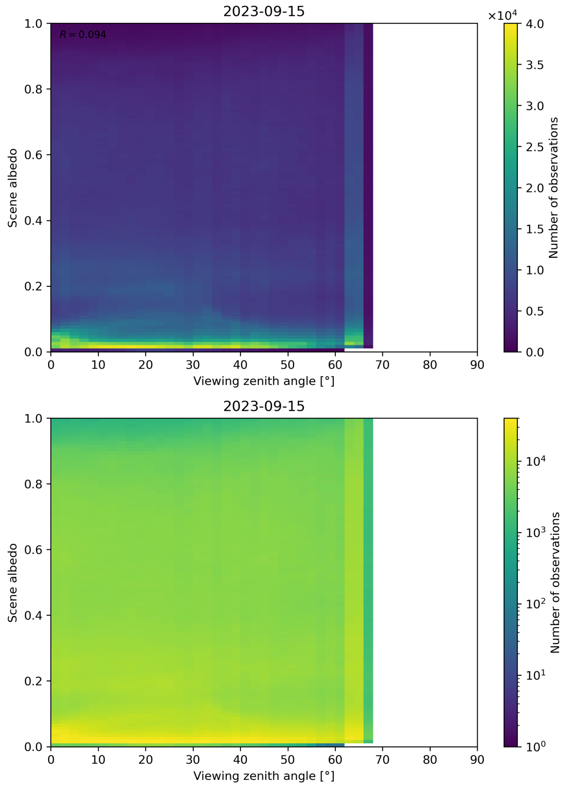
Figure 138: Scatter density plot of “Viewing zenith angle” against “Scene albedo” for 2023-09-15 to 2023-09-16.
