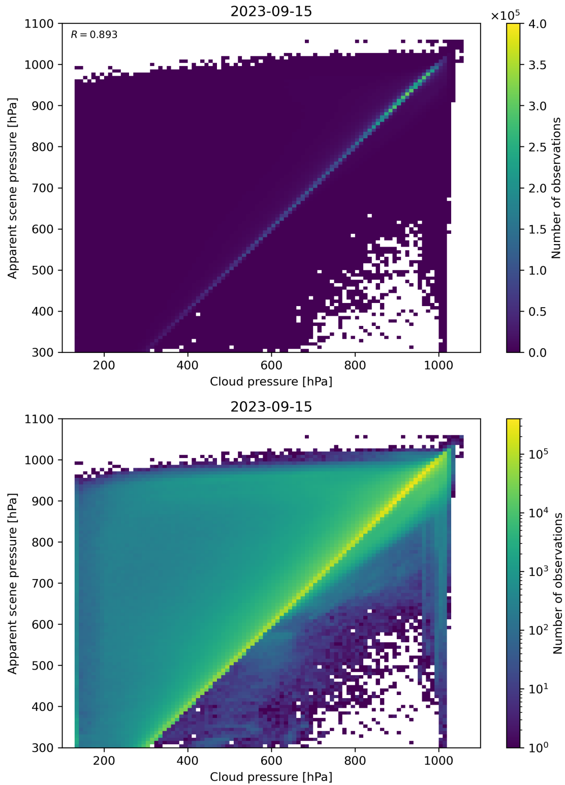
Figure 84: Scatter density plot of “Cloud pressure” against “Apparent scene pressure” for 2023-09-15 to 2023-09-16.
