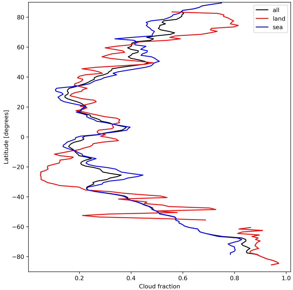
Figure 15: Zonal average of “Cloud fraction” for 2023-09-15 to 2023-09-16.
