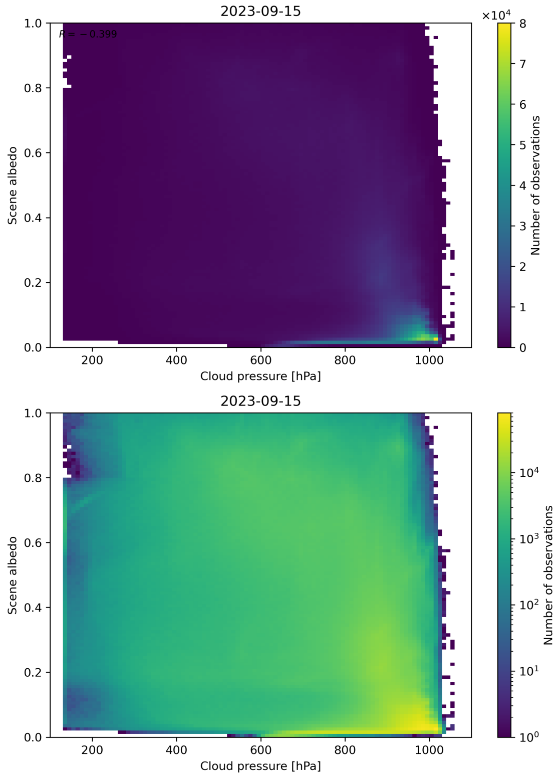
Figure 91: Scatter density plot of “Cloud pressure” against “Scene albedo” for 2023-09-15 to 2023-09-16.
