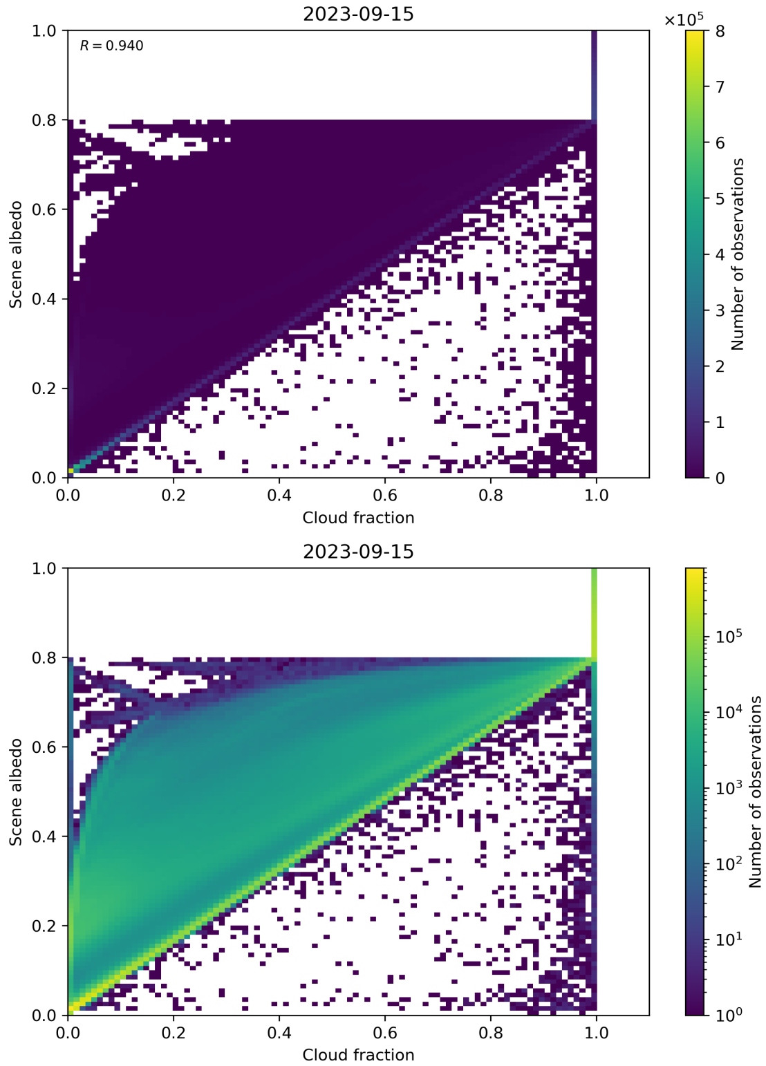
Figure 82: Scatter density plot of “Cloud fraction” against “Scene albedo” for 2023-09-15 to 2023-09-16.
