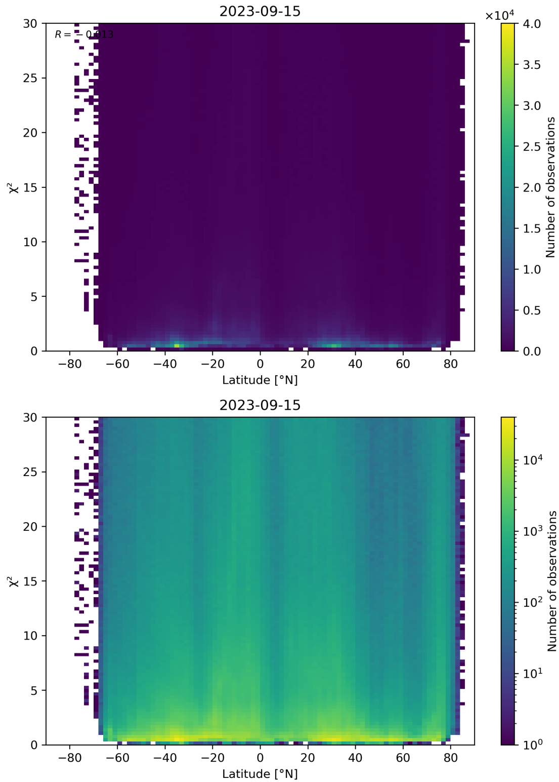
Figure 97: Scatter density plot of “Latitude” against “ \chi^2 ” for 2023-09-15 to 2023-09-16.
