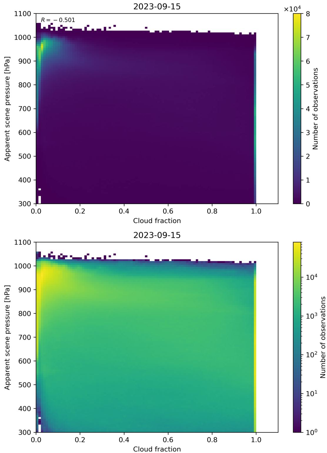
Figure 76: Scatter density plot of “Cloud fraction” against “Apparent scene pressure” for 2023-09-15 to 2023-09-16.
