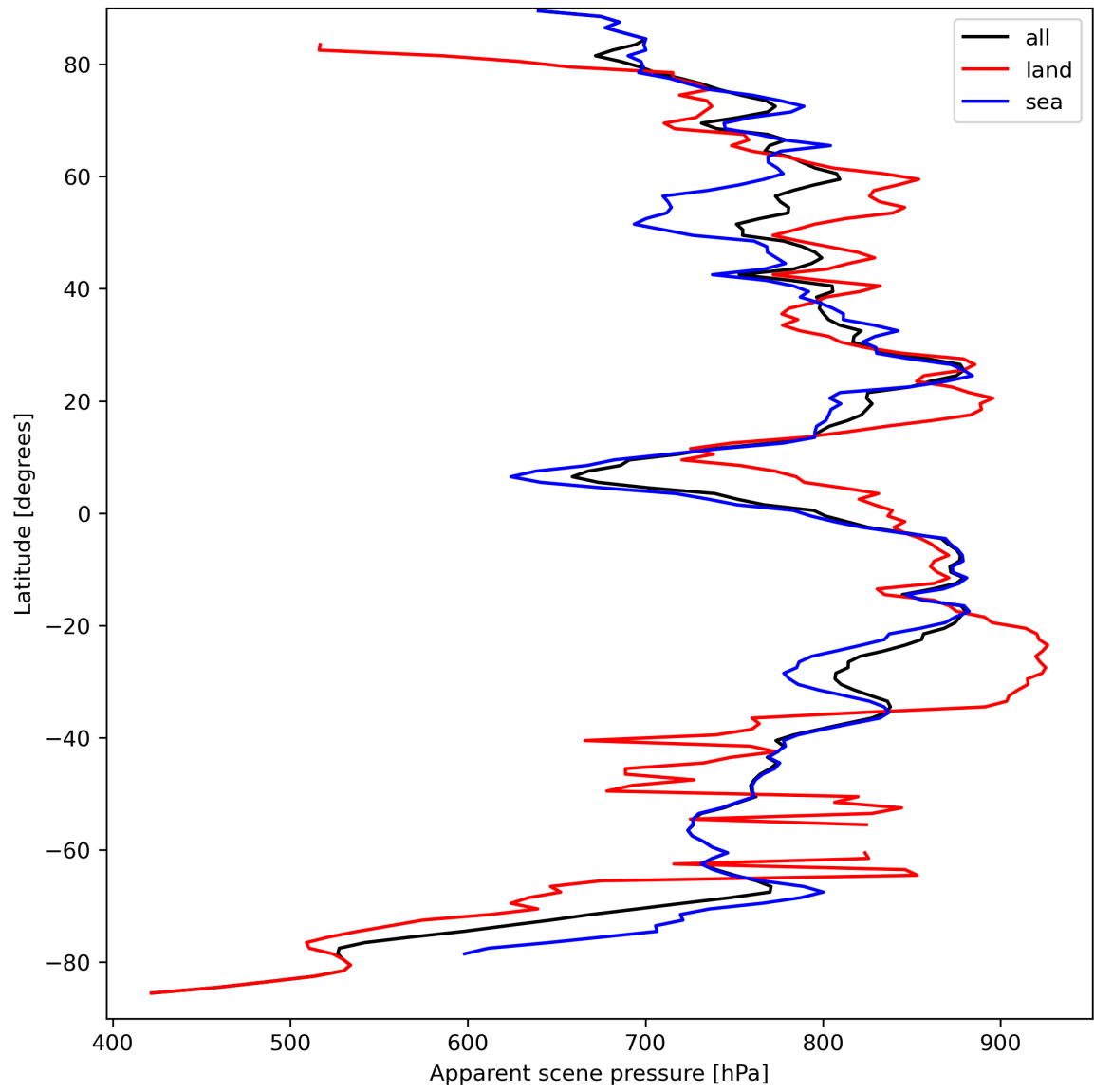
Figure 19: Zonal average of “Apparent scene pressure” for 2023-09-15 to 2023-09-16.
