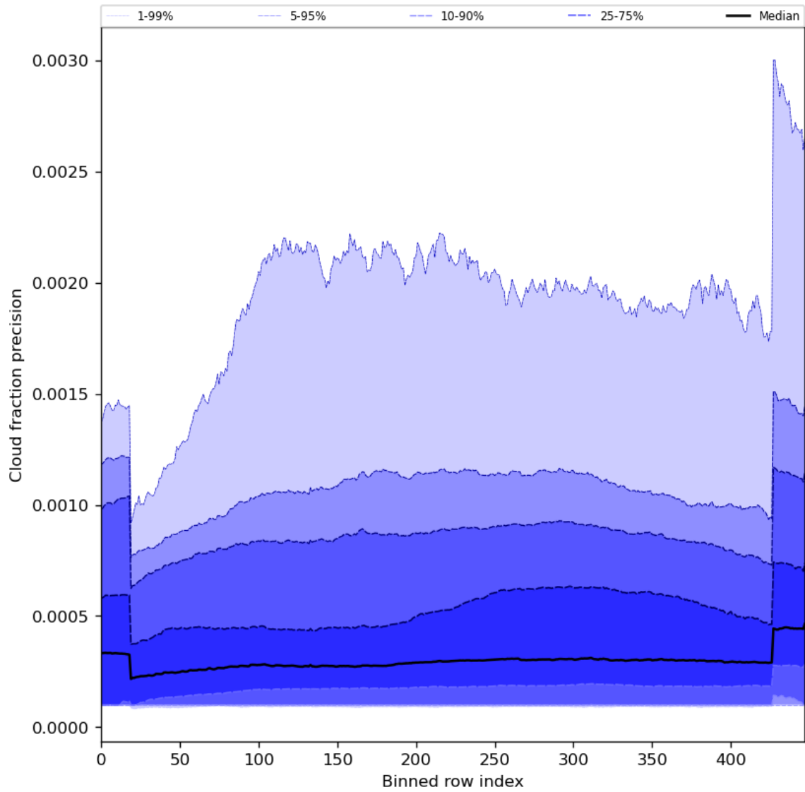
Figure 50: Along track statistics of “Cloud fraction precision” for 2023-09-15 to 2023-09-16
