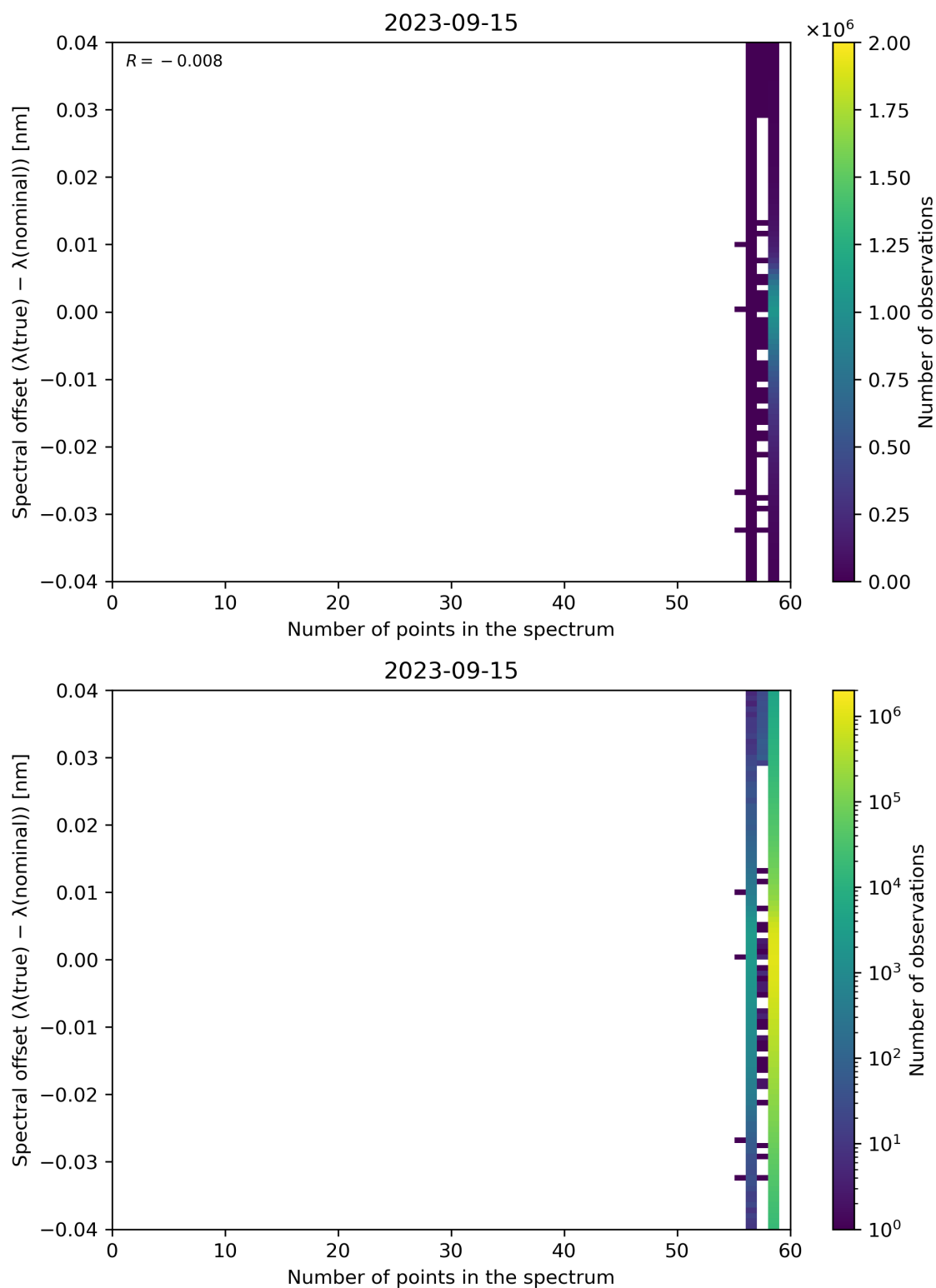
Figure 110: Scatter density plot of “Number of points in the spectrum” against “Spectral offset ( \lambda(\text{true}) - \lambda(\text{nominal})) ” for 2023-09-15 to 2023-09-16.
