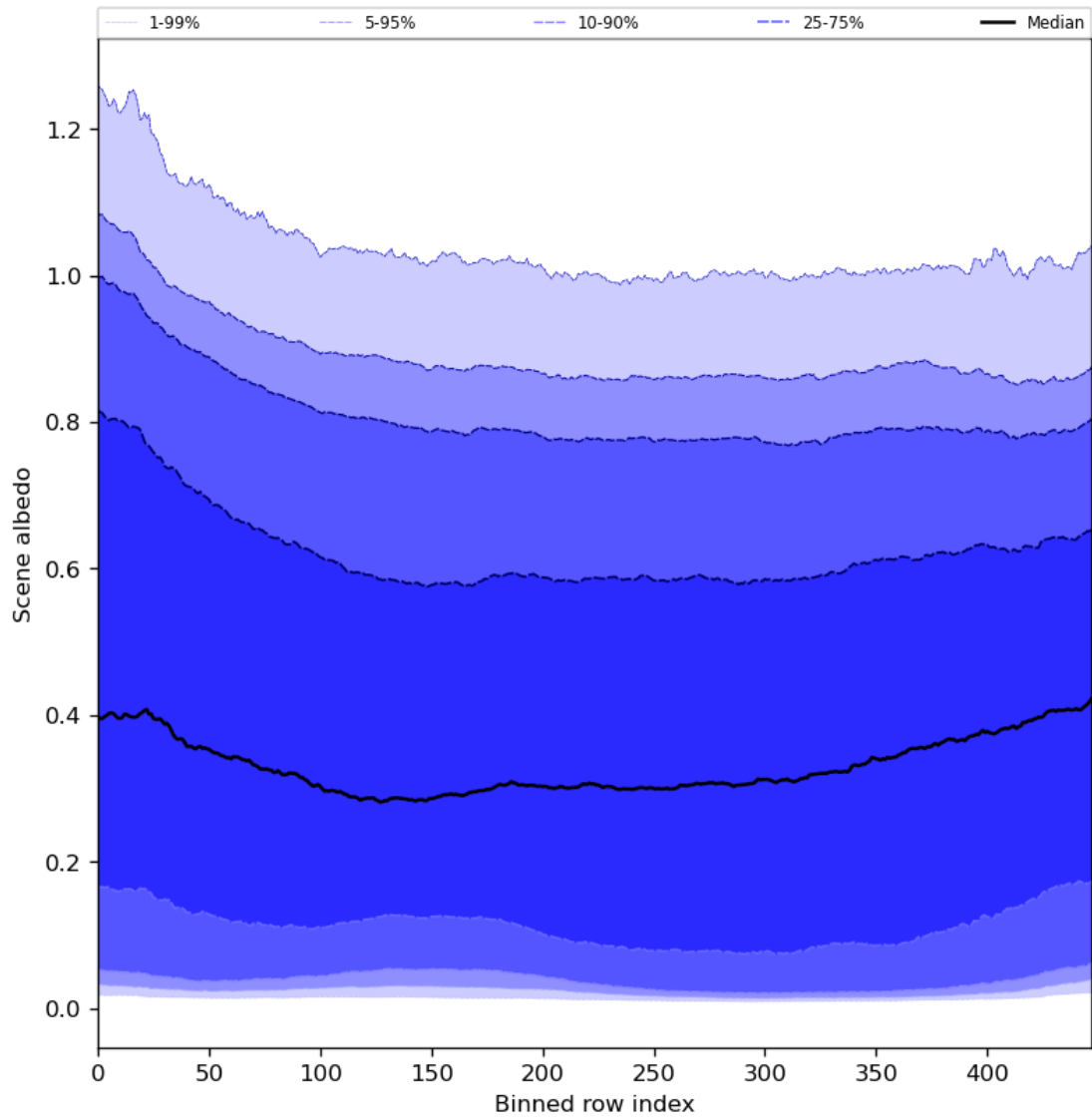
Figure 51: Along track statistics of “Scene albedo” for 2023-09-15 to 2023-09-16
