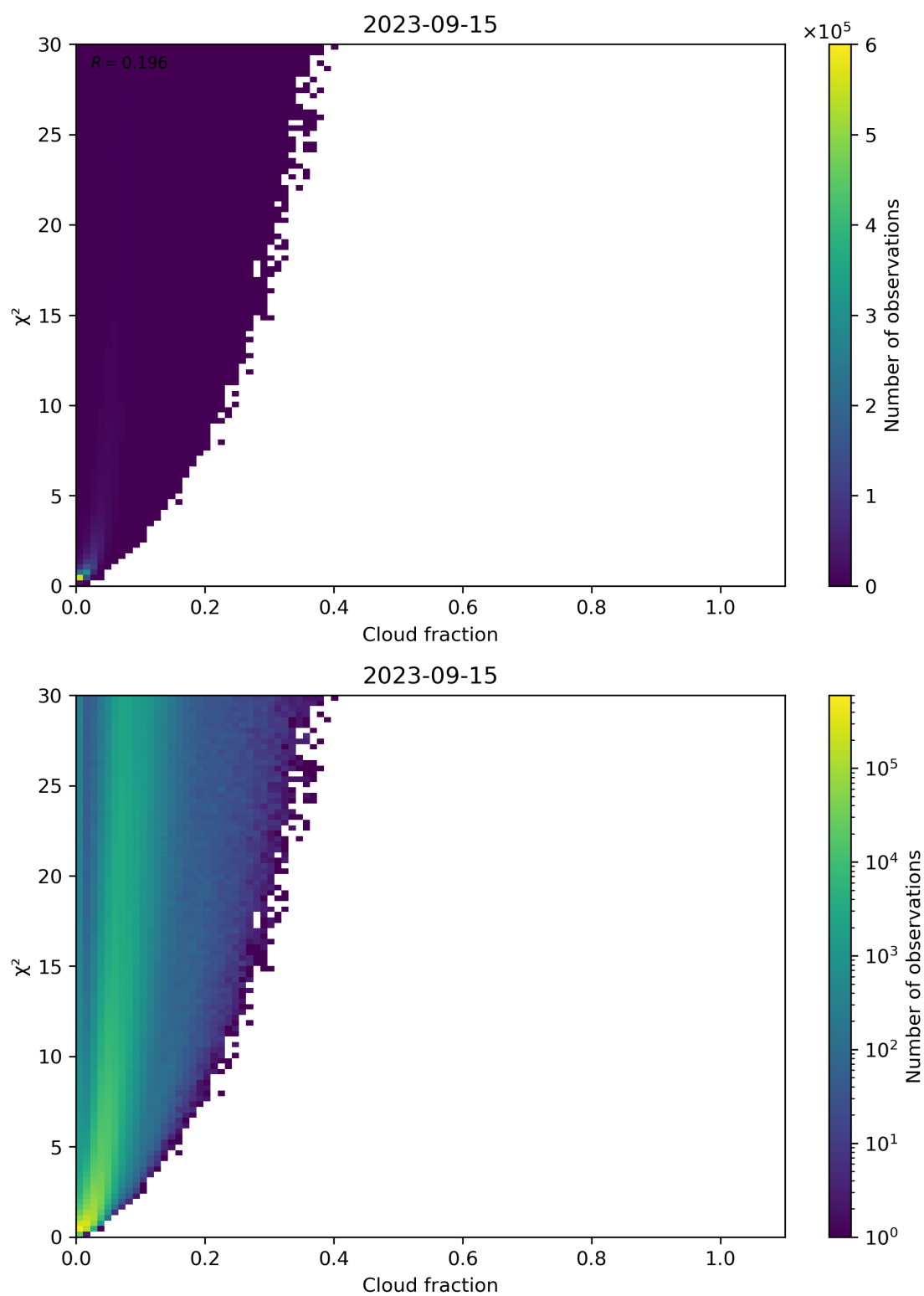
Figure 77: Scatter density plot of “Cloud fraction” against “ \chi^2 ” for 2023-09-15 to 2023-09-16.
