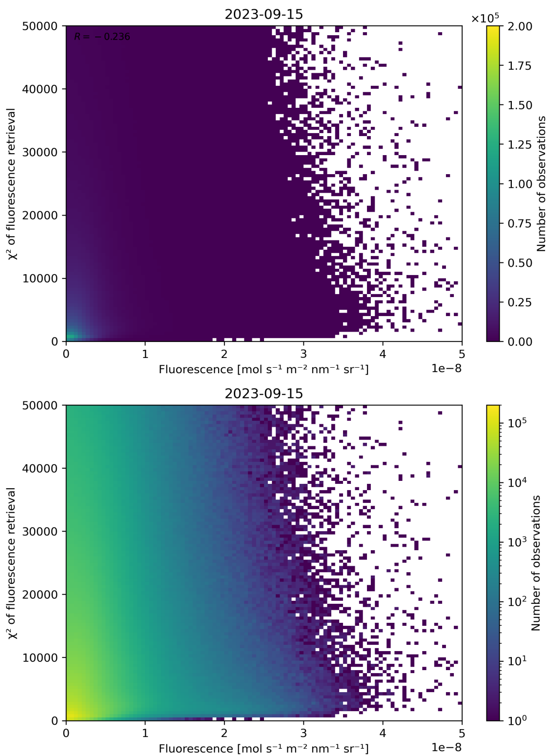
Figure 93: Scatter density plot of “Fluorescence” against “ \chi^2 of fluorescence retrieval” for 2023-09-15 to 2023-09-16.
