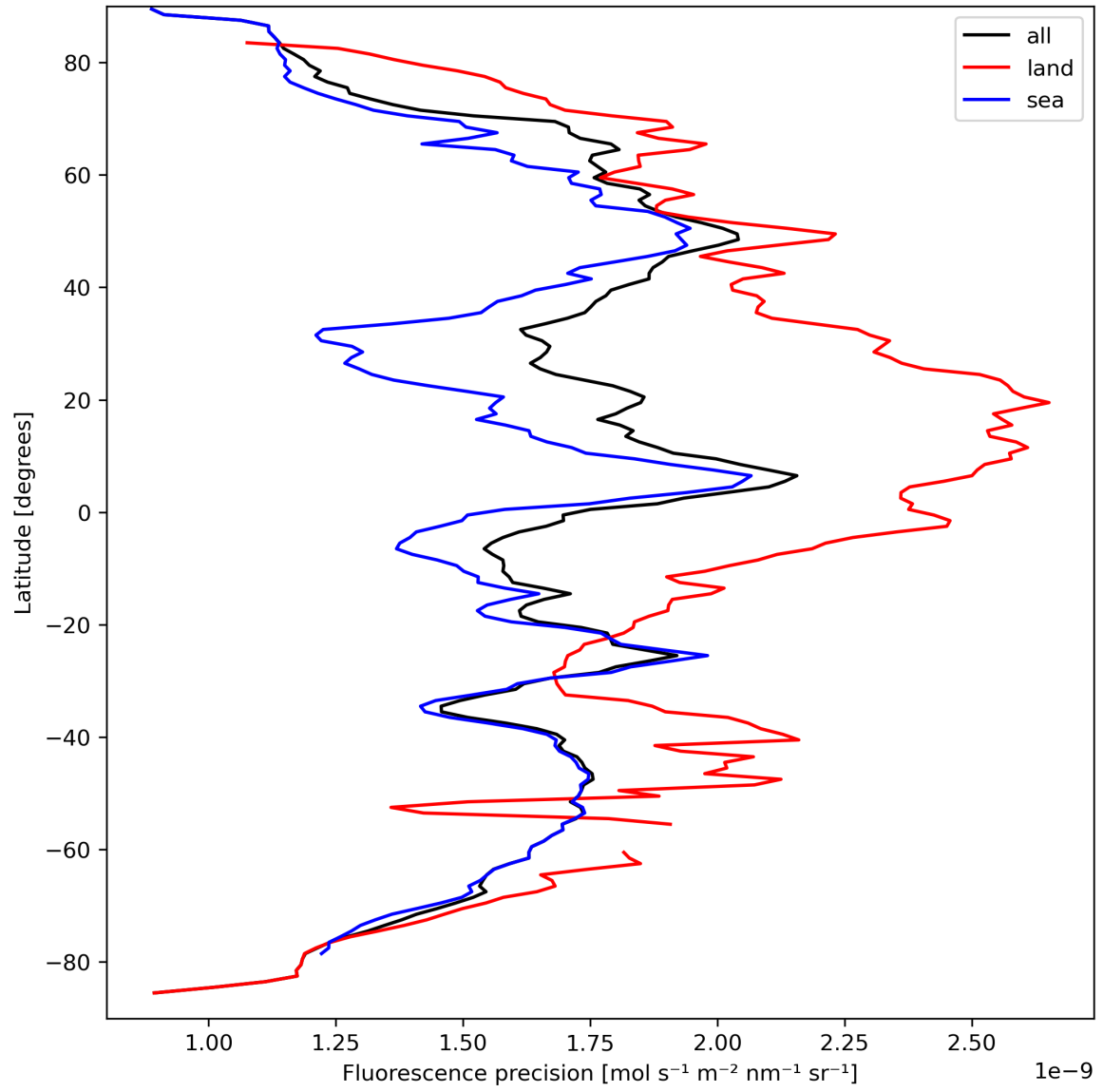
Figure 24: Zonal average of “Fluorescence precision” for 2023-09-15 to 2023-09-16.
