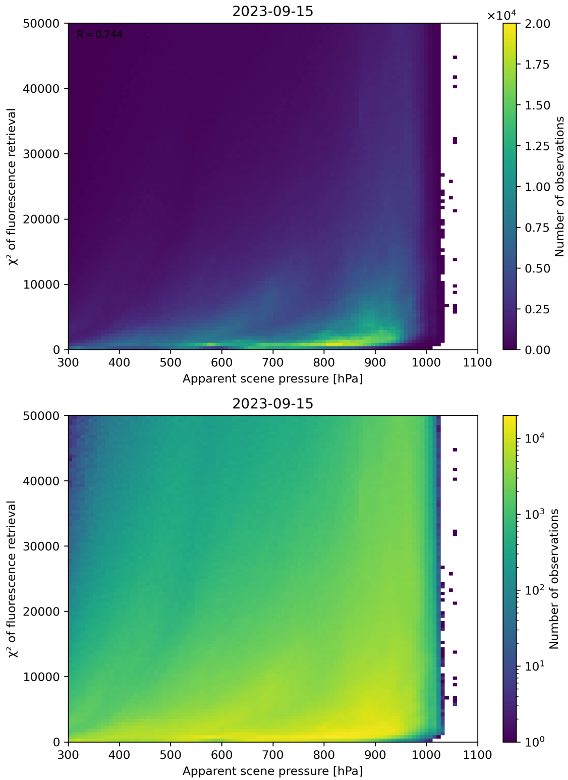
Figure 64: Scatter density plot of “Apparent scene pressure” against “ \chi^2 of fluorescence retrieval” for 2023-09-15 to 2023-09-16.
