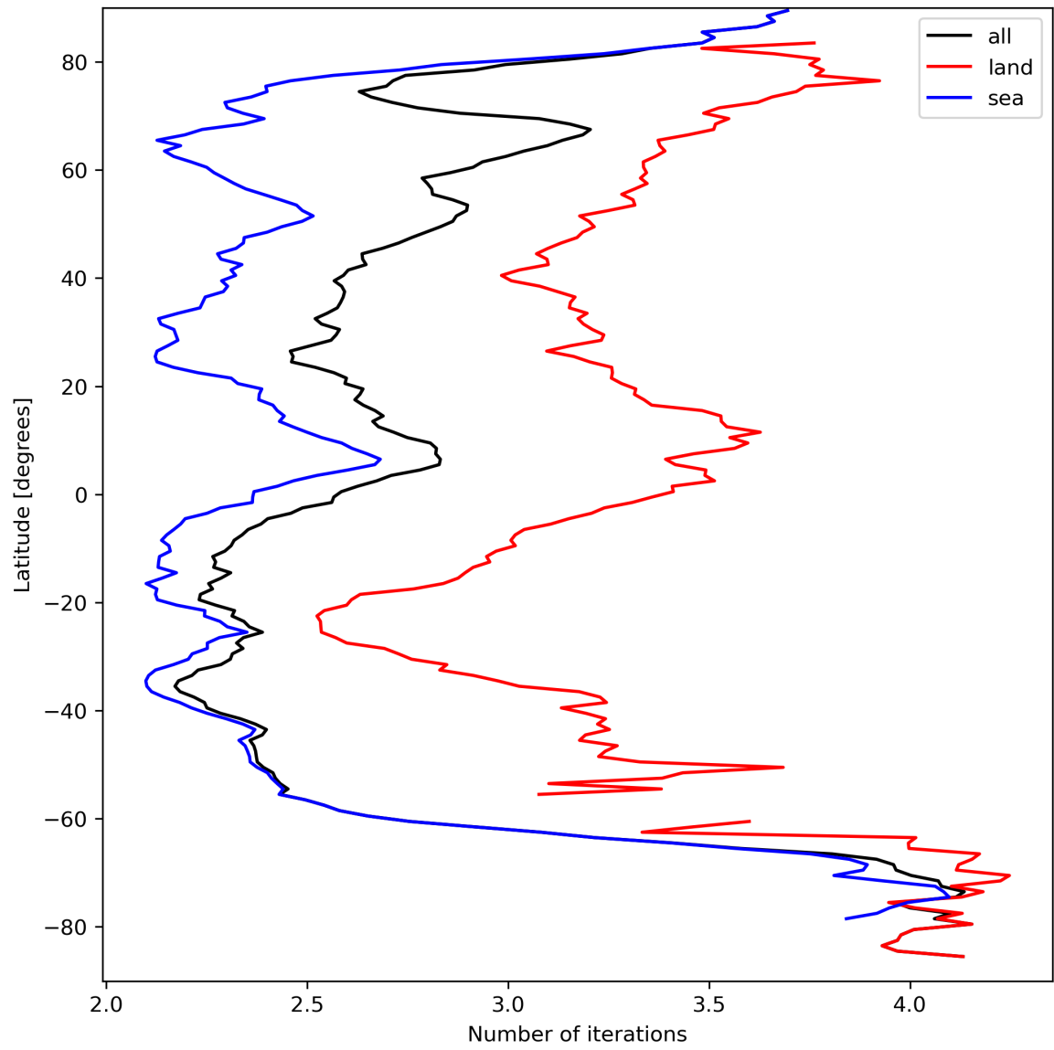
Figure 22: Zonal average of “Number of iterations” for 2023-09-15 to 2023-09-16.
