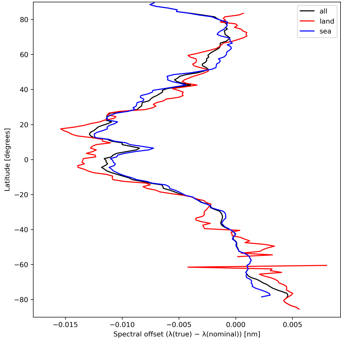
Figure 28: Zonal average of “Spectral offset ( \lambda(\text{true}) - \lambda(\text{nominal}) )” for 2023-09-15 to 2023-09-16.
