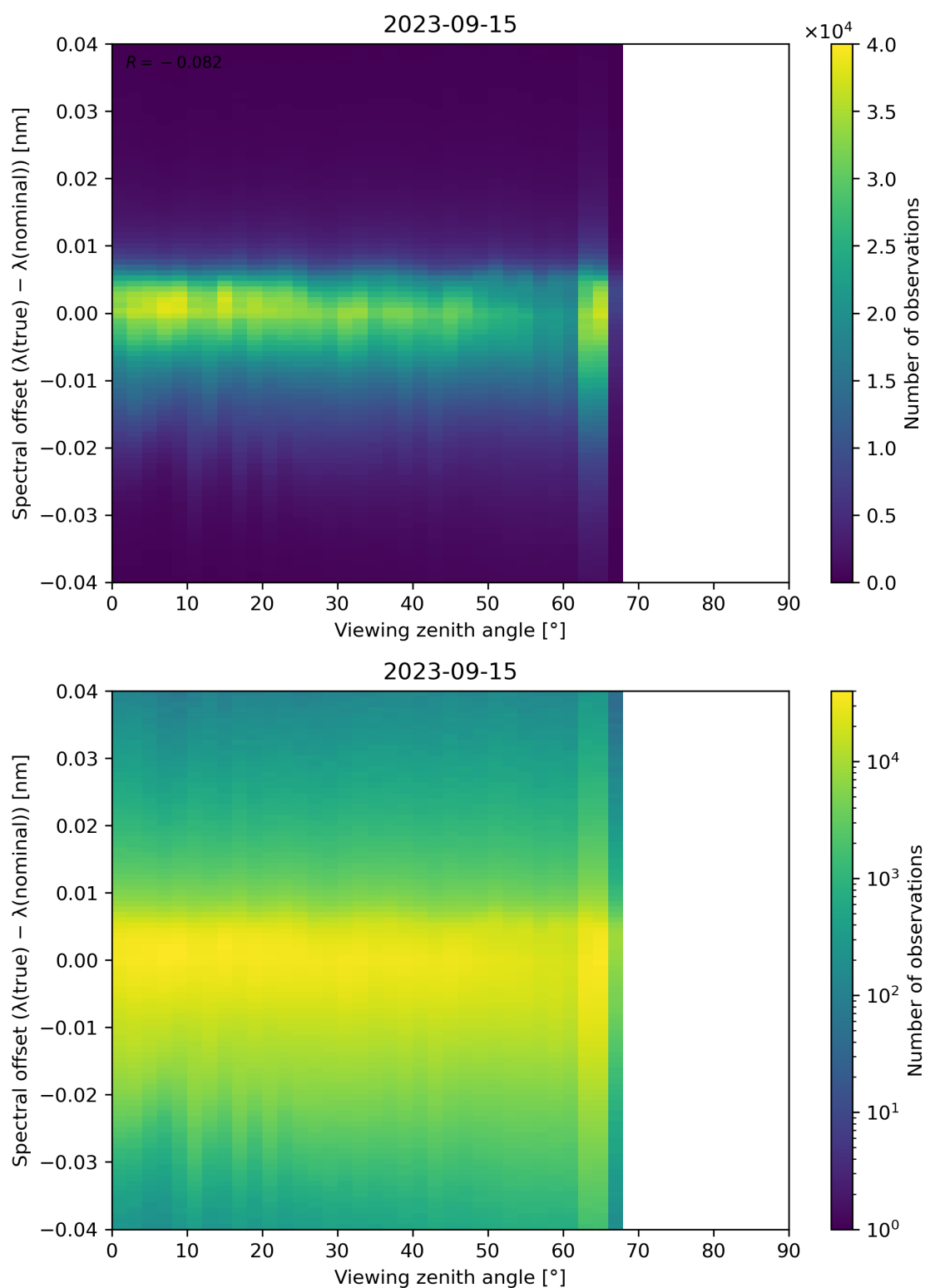
Figure 140: Scatter density plot of “Viewing zenith angle” against “Spectral offset ( \lambda(\text{true}) - \lambda(\text{nominal}) )” for 2023-09-15 to 2023-09-16.
