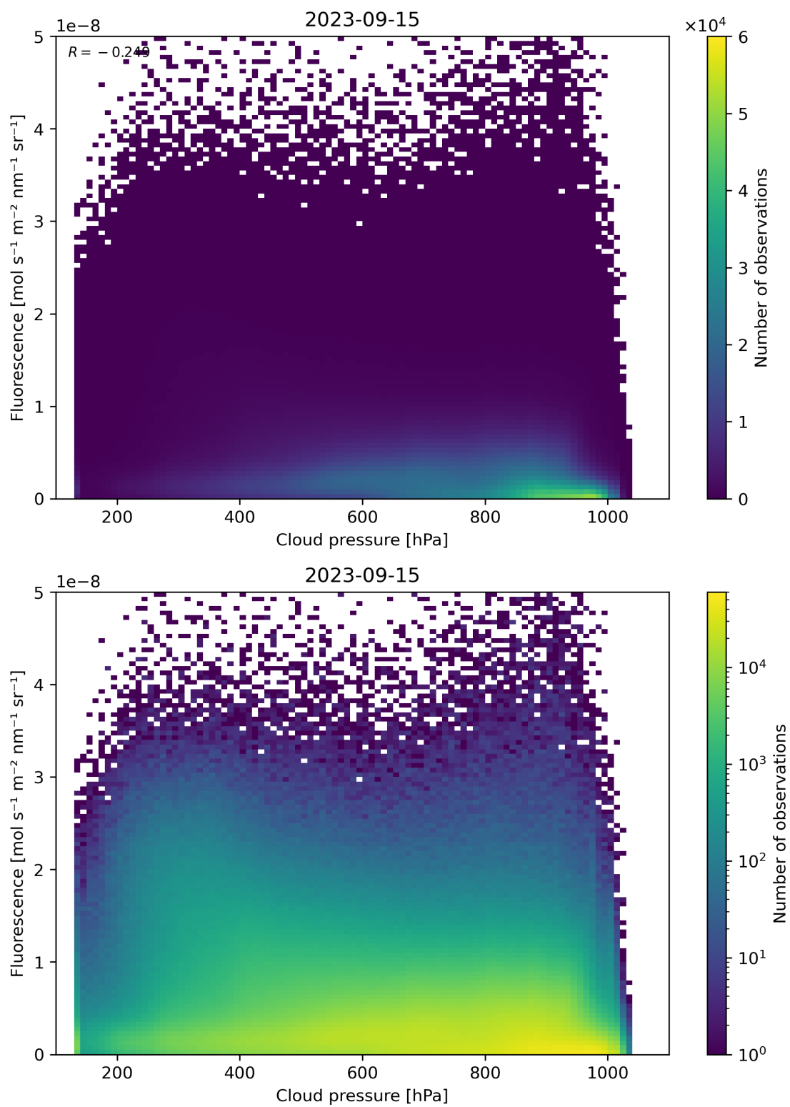
Figure 88: Scatter density plot of “Cloud pressure” against “Fluorescence” for 2023-09-15 to 2023-09-16.
