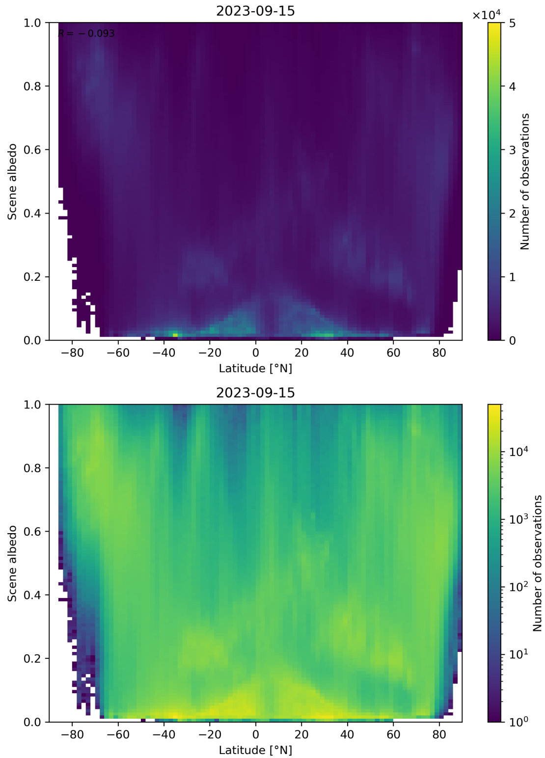
Figure 104: Scatter density plot of “Latitude” against “Scene albedo” for 2023-09-15 to 2023-09-16.
