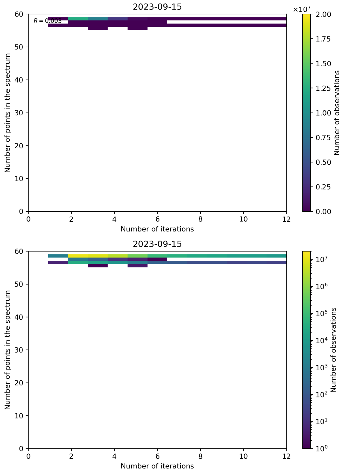
Figure 108: Scatter density plot of “Number of iterations” against “Number of points in the spectrum” for 2023-09-15 to 2023-09-16.
