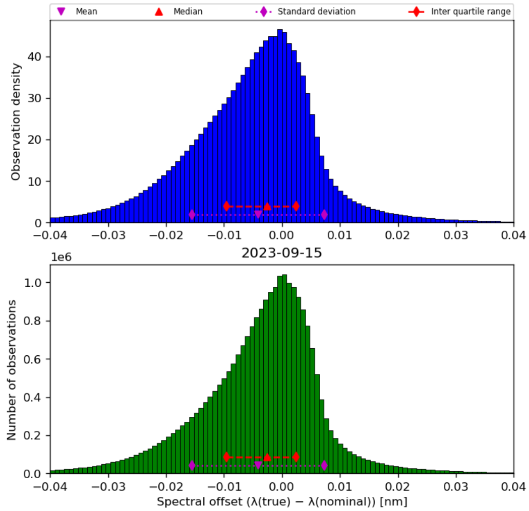
Figure 45: Histogram of “Spectral offset ( \lambda(\text{true}) - \lambda(\text{nominal}) )” for 2023-09-15 to 2023-09-16
