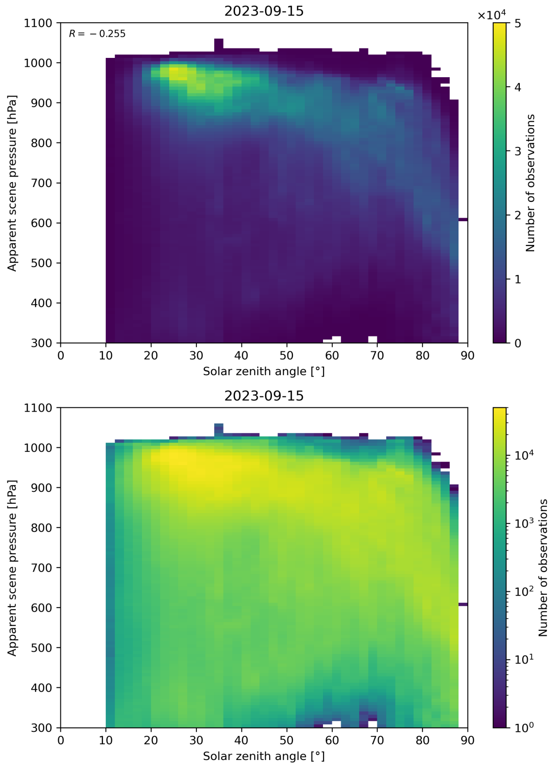
Figure 118: Scatter density plot of “Solar zenith angle” against “Apparent scene pressure” for 2023-09-15 to 2023-09-16.
