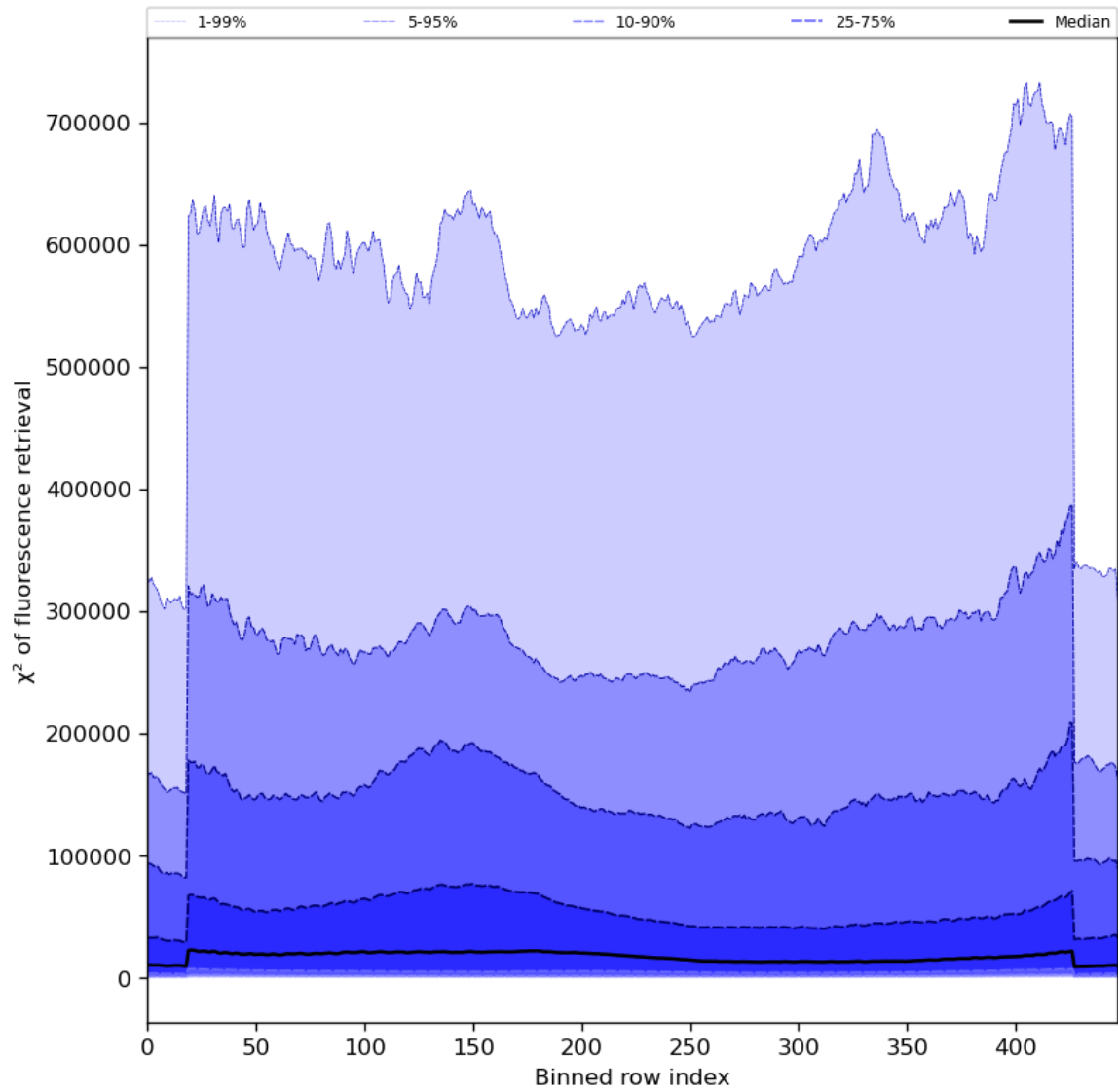
Figure 59: Along track statistics of “ \chi^2 of fluorescence retrieval” for 2023-09-15 to 2023-09-16
