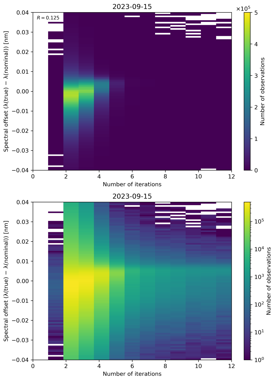
Figure 109: Scatter density plot of “Number of iterations” against “Spectral offset ( \lambda(\text{true}) - \lambda(\text{nominal}) )” for 2023-09-15 to 2023-09-16.
