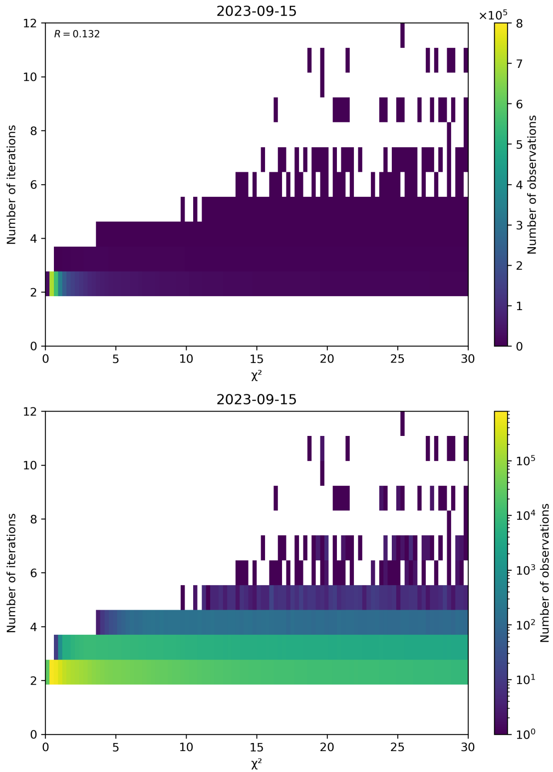
Figure 73: Scatter density plot of “ \chi^2 ” against “Number of iterations” for 2023-09-15 to 2023-09-16.
