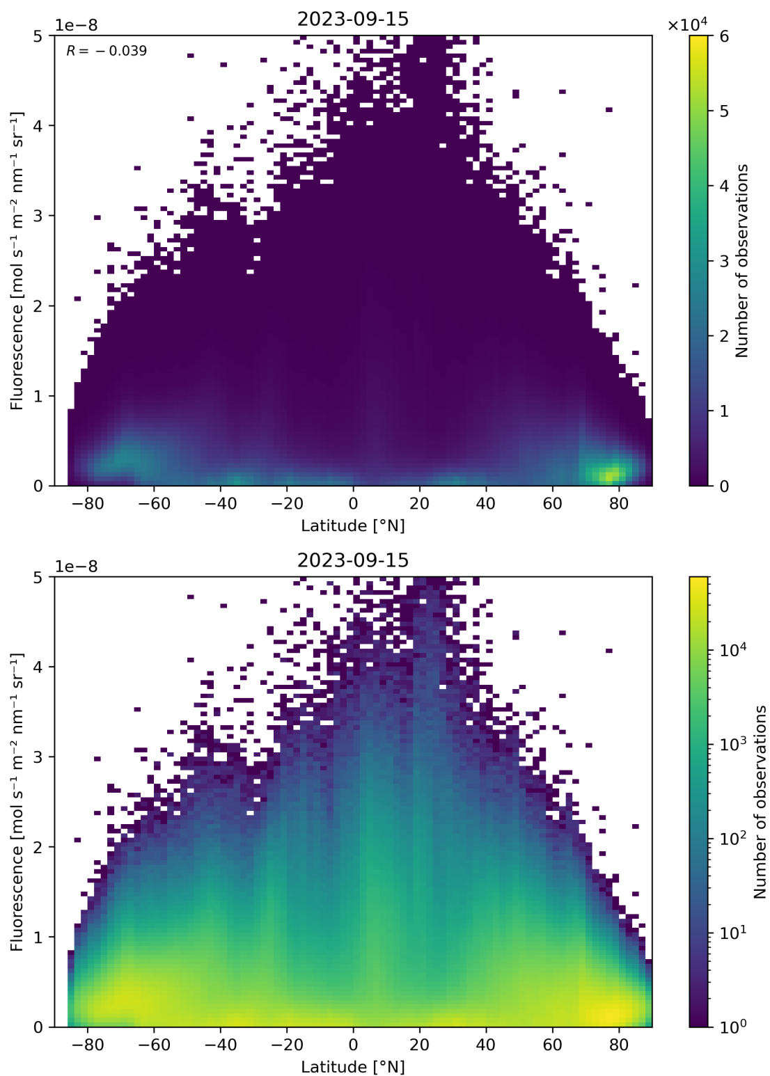
Figure 101: Scatter density plot of “Latitude” against “Fluorescence” for 2023-09-15 to 2023-09-16.
