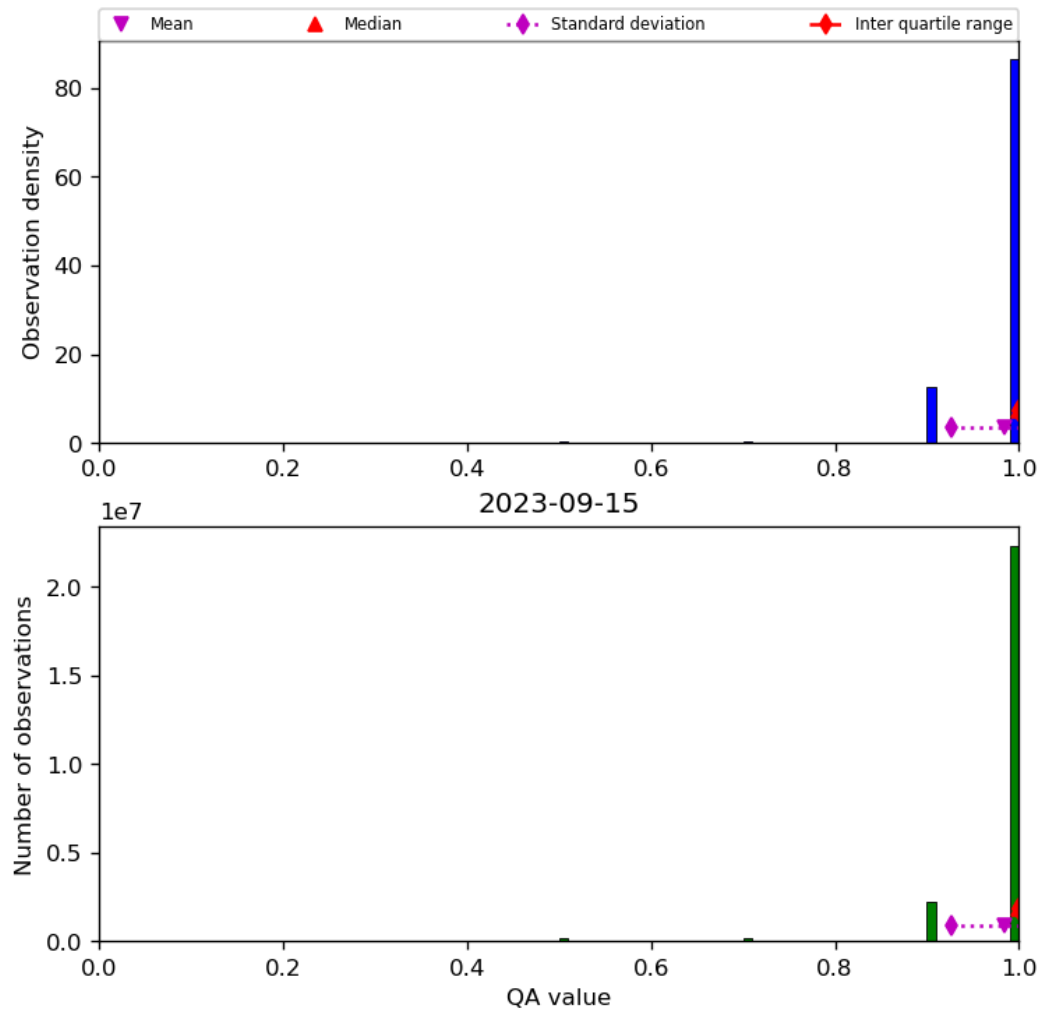
Figure 29: Histogram of “QA value” for 2023-09-15 to 2023-09-16
