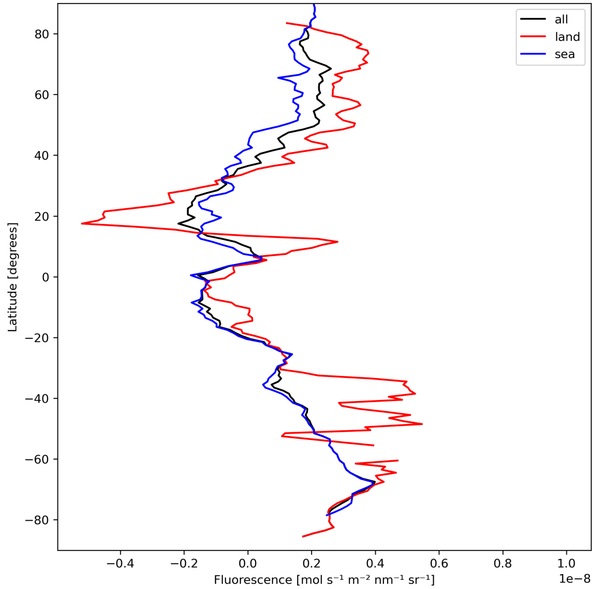
Figure 23: Zonal average of “Fluorescence” for 2023-09-15 to 2023-09-16.
