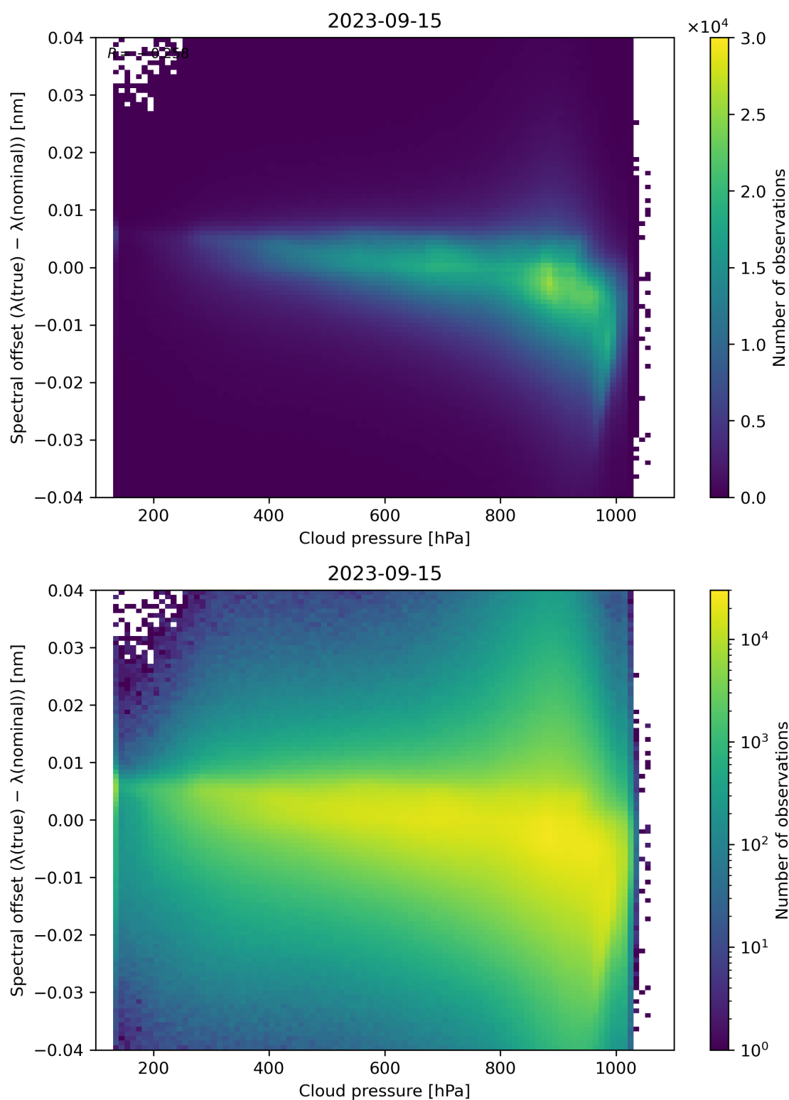
Figure 92: Scatter density plot of “Cloud pressure” against “Spectral offset ( \lambda(\text{true}) - \lambda(\text{nominal}) )” for 2023-09-15 to 2023-09-16.
