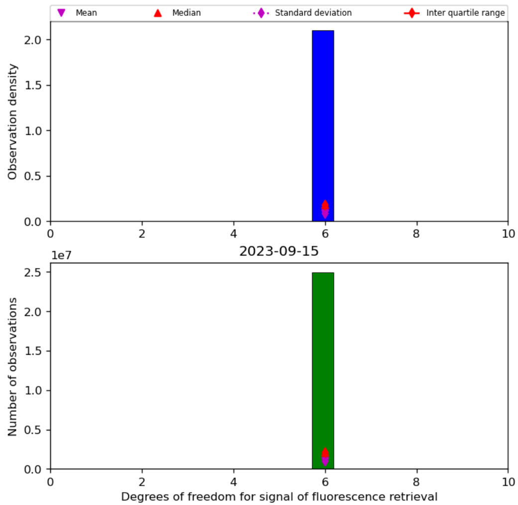
Figure 43: Histogram of “Degrees of freedom for signal of fluorescence retrieval” for 2023-09-15 to 2023-09-16
