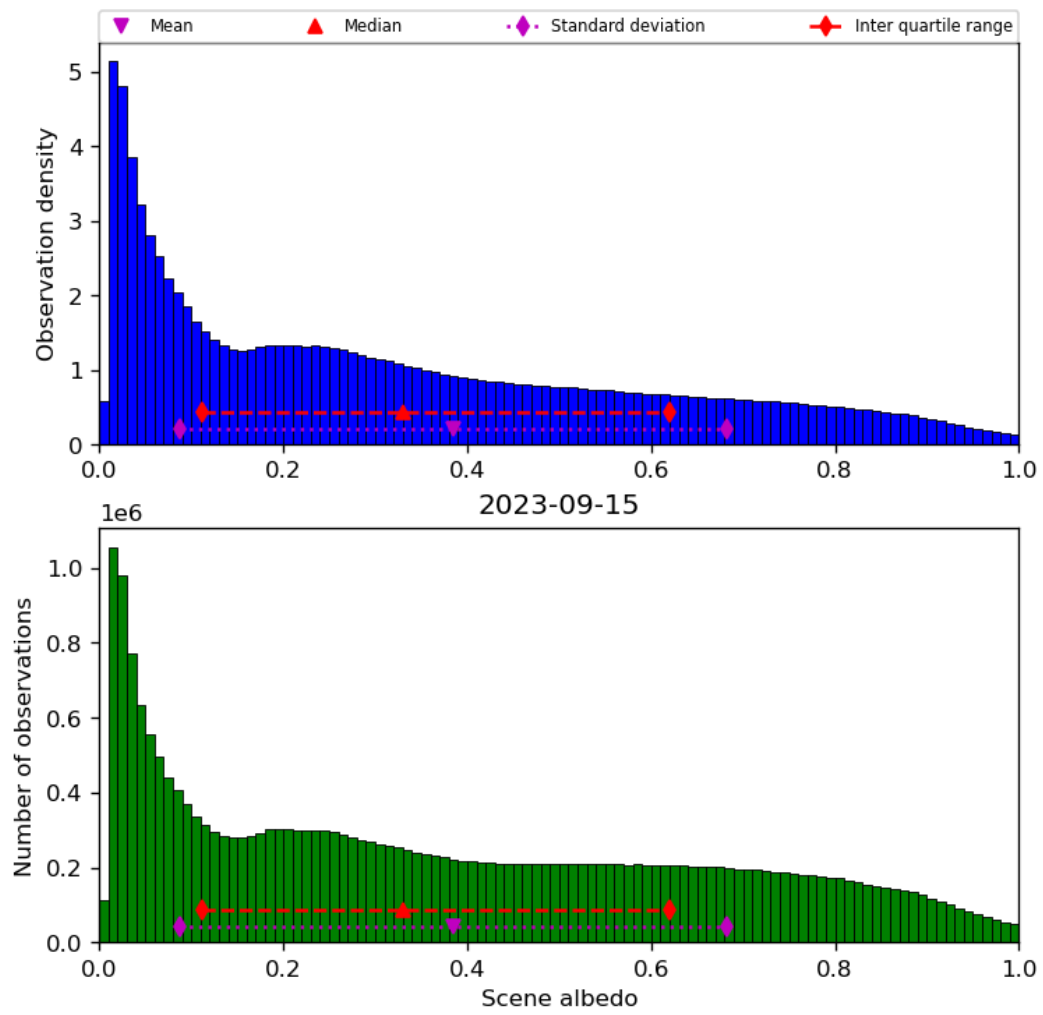
Figure 34: Histogram of “Scene albedo” for 2023-09-15 to 2023-09-16
