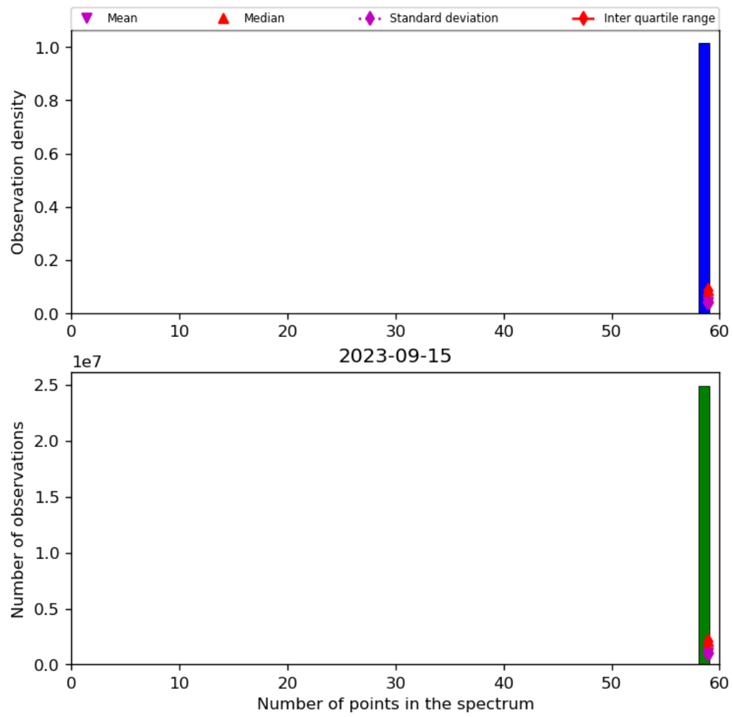
Figure 44: Histogram of “Number of points in the spectrum” for 2023-09-15 to 2023-09-16
