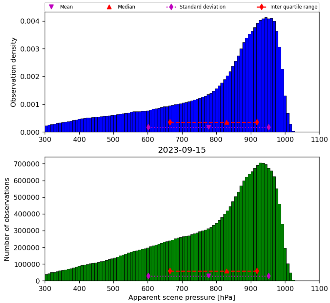
Figure 36: Histogram of “Apparent scene pressure” for 2023-09-15 to 2023-09-16
