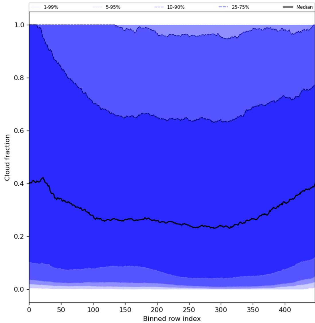
Figure 49: Along track statistics of “Cloud fraction” for 2023-09-15 to 2023-09-16
