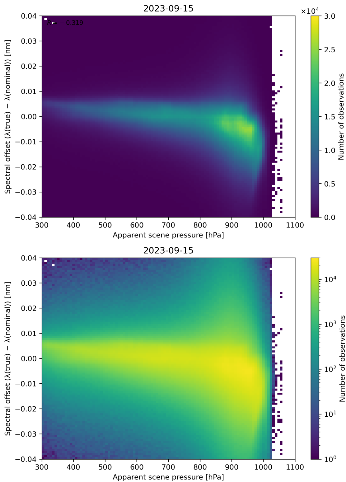
Figure 68: Scatter density plot of “Apparent scene pressure” against “Spectral offset ( \lambda(\text{true}) - \lambda(\text{nominal}) )” for 2023-09-15 to 2023-09-16.
