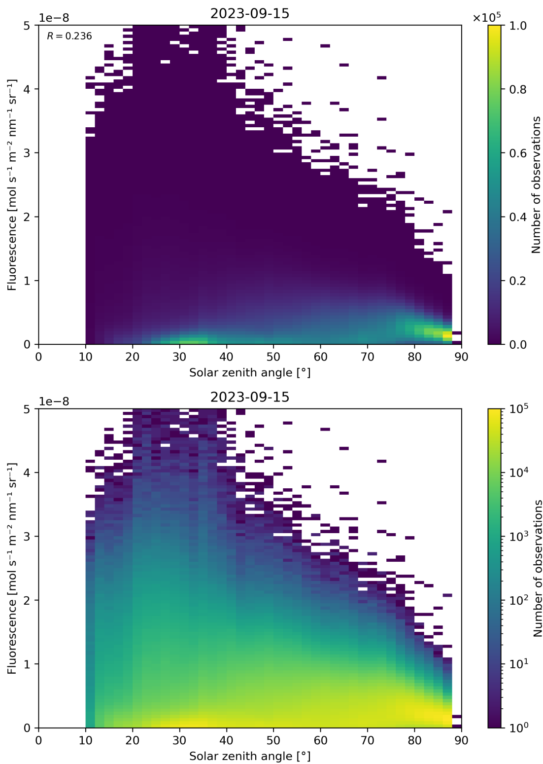
Figure 123: Scatter density plot of “Solar zenith angle” against “Fluorescence” for 2023-09-15 to 2023-09-16.
