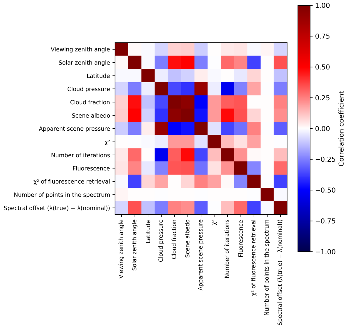
Figure 2: Map of correlation matrix for 2023-09-15 to 2023-09-16.
