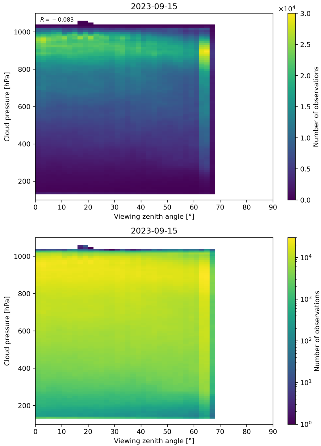
Figure 133: Scatter density plot of “Viewing zenith angle” against “Cloud pressure” for 2023-09-15 to 2023-09-16.
