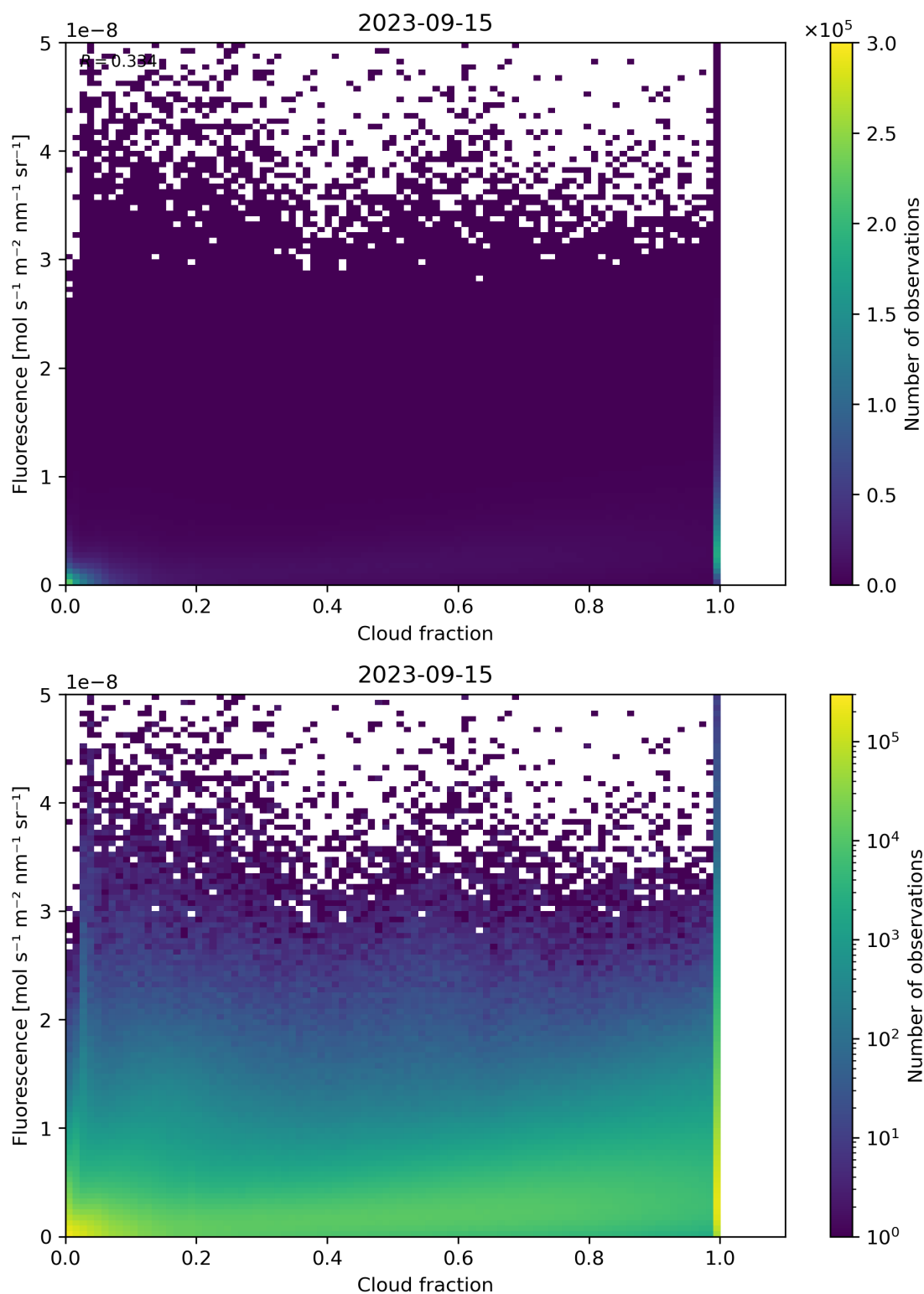
Figure 79: Scatter density plot of “Cloud fraction” against “Fluorescence” for 2023-09-15 to 2023-09-16.
