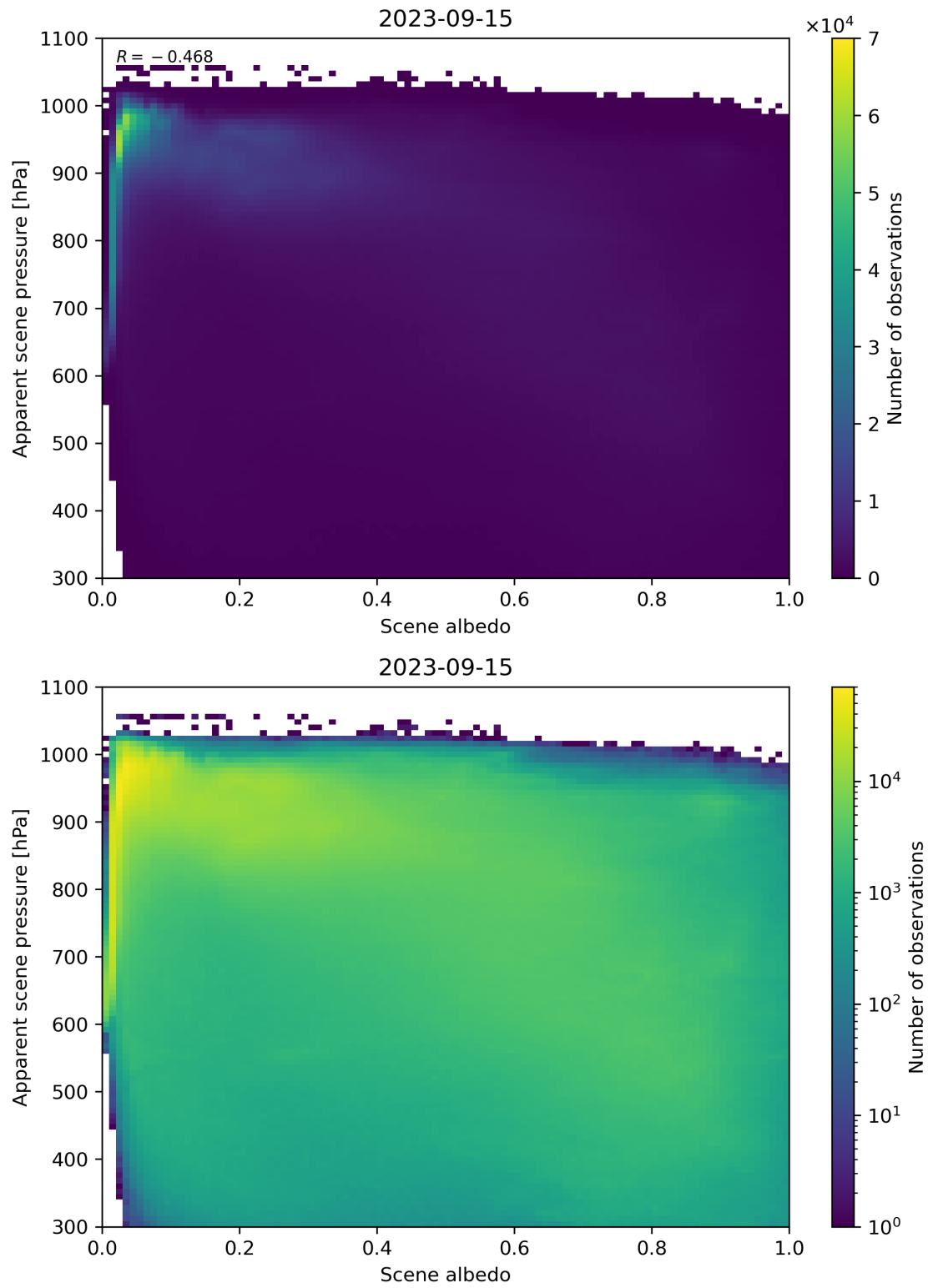
Figure 111: Scatter density plot of “Scene albedo” against “Apparent scene pressure” for 2023-09-15 to 2023-09-16.
