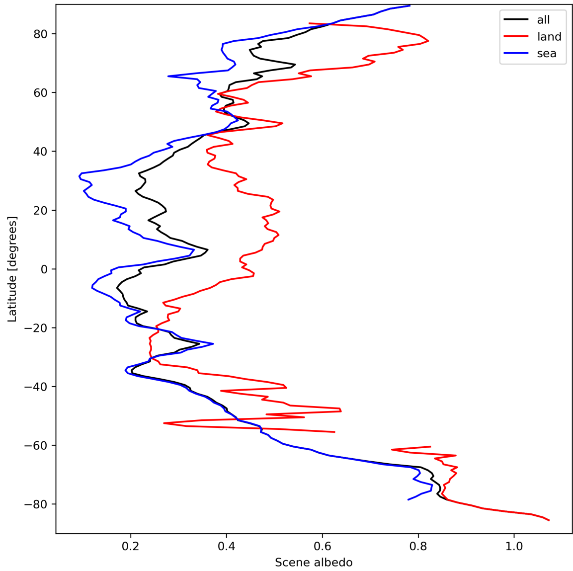
Figure 17: Zonal average of “Scene albedo” for 2023-09-15 to 2023-09-16.
