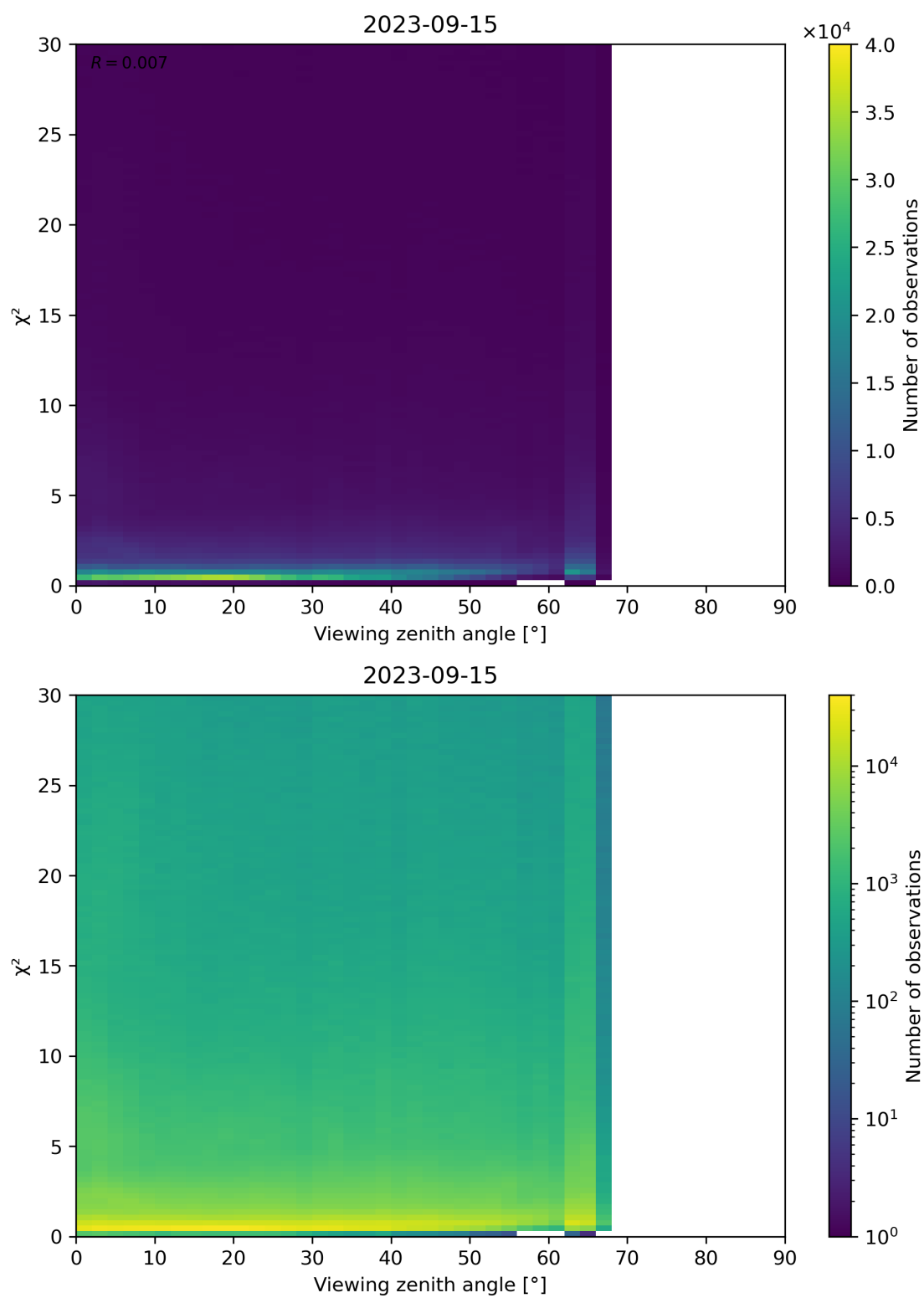
Figure 130: Scatter density plot of “Viewing zenith angle” against “ \chi^2 ” for 2023-09-15 to 2023-09-16.
