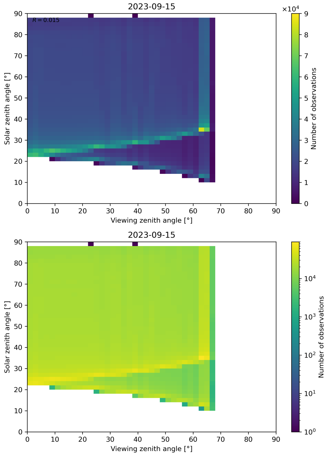
Figure 139: Scatter density plot of “Viewing zenith angle” against “Solar zenith angle” for 2023-09-15 to 2023-09-16.
