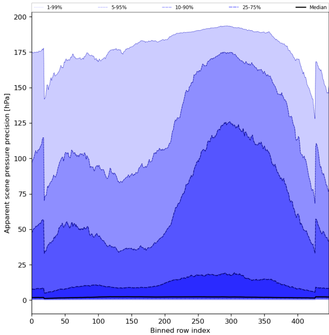
Figure 54: Along track statistics of “Apparent scene pressure precision” for 2023-09-15 to 2023-09-16
