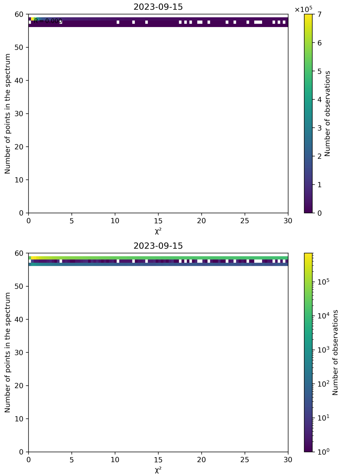
Figure 74: Scatter density plot of " \chi^2 " against "Number of points in the spectrum" for 2023-09-15 to 2023-09-16.
