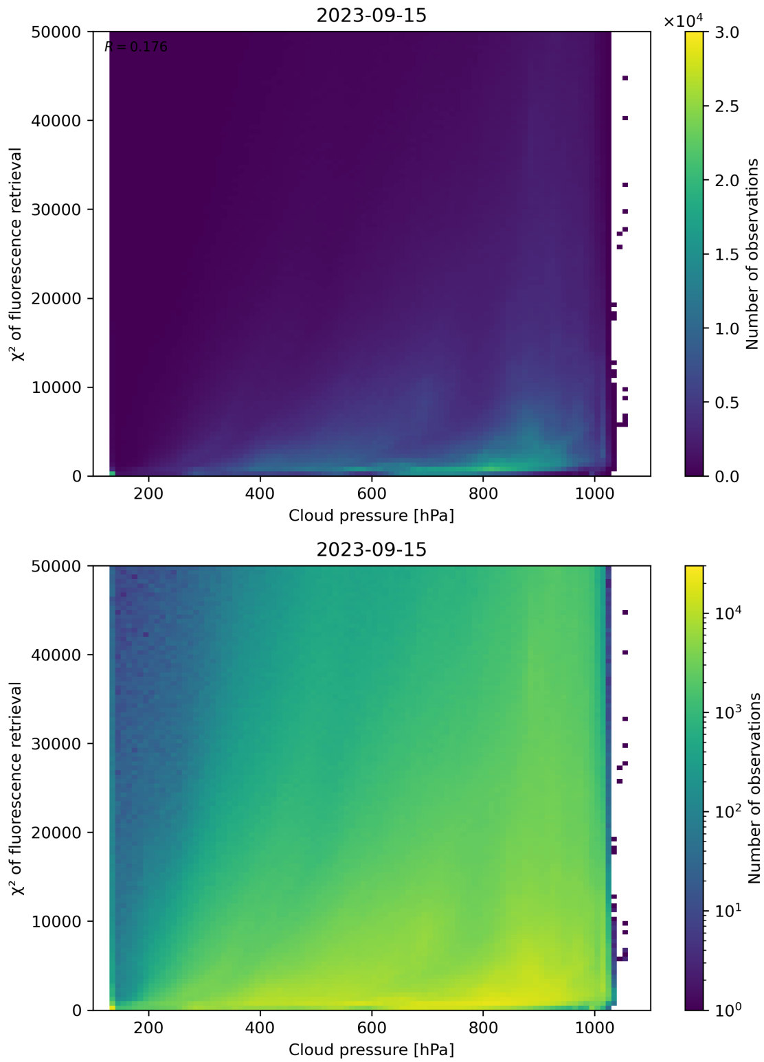
Figure 86: Scatter density plot of “Cloud pressure” against “ \chi^2 of fluorescence retrieval” for 2023-09-15 to 2023-09-16.
