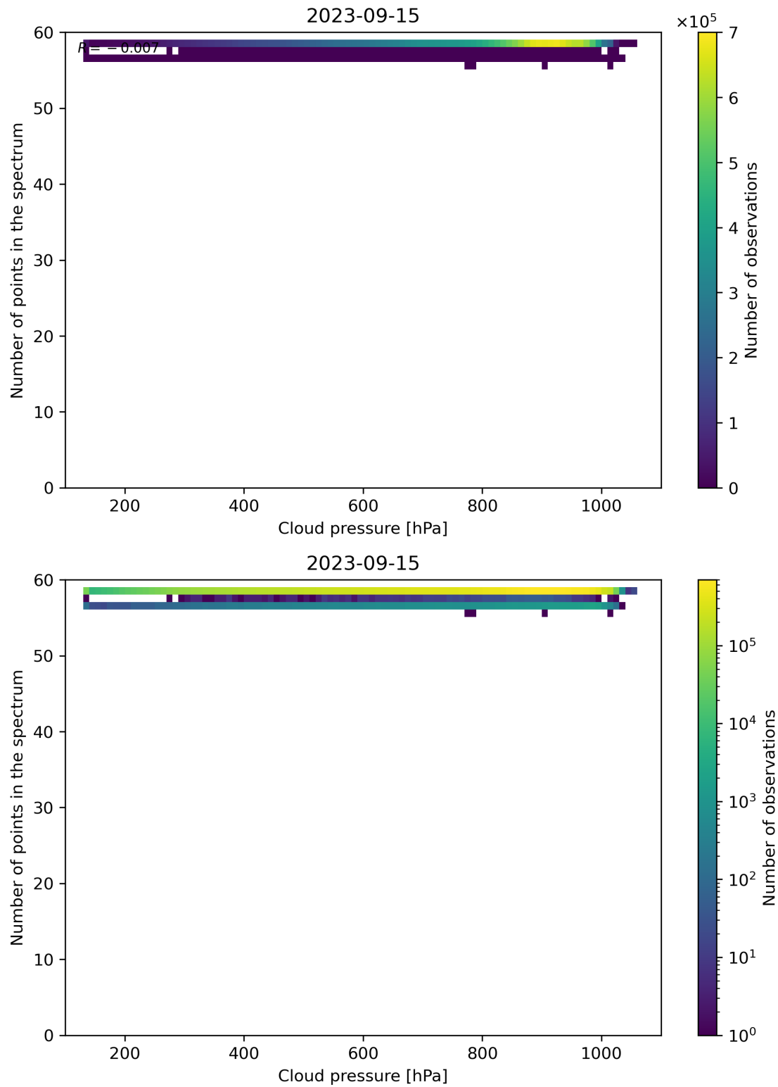
Figure 90: Scatter density plot of “Cloud pressure” against “Number of points in the spectrum” for 2023-09-15 to 2023-09-16.
