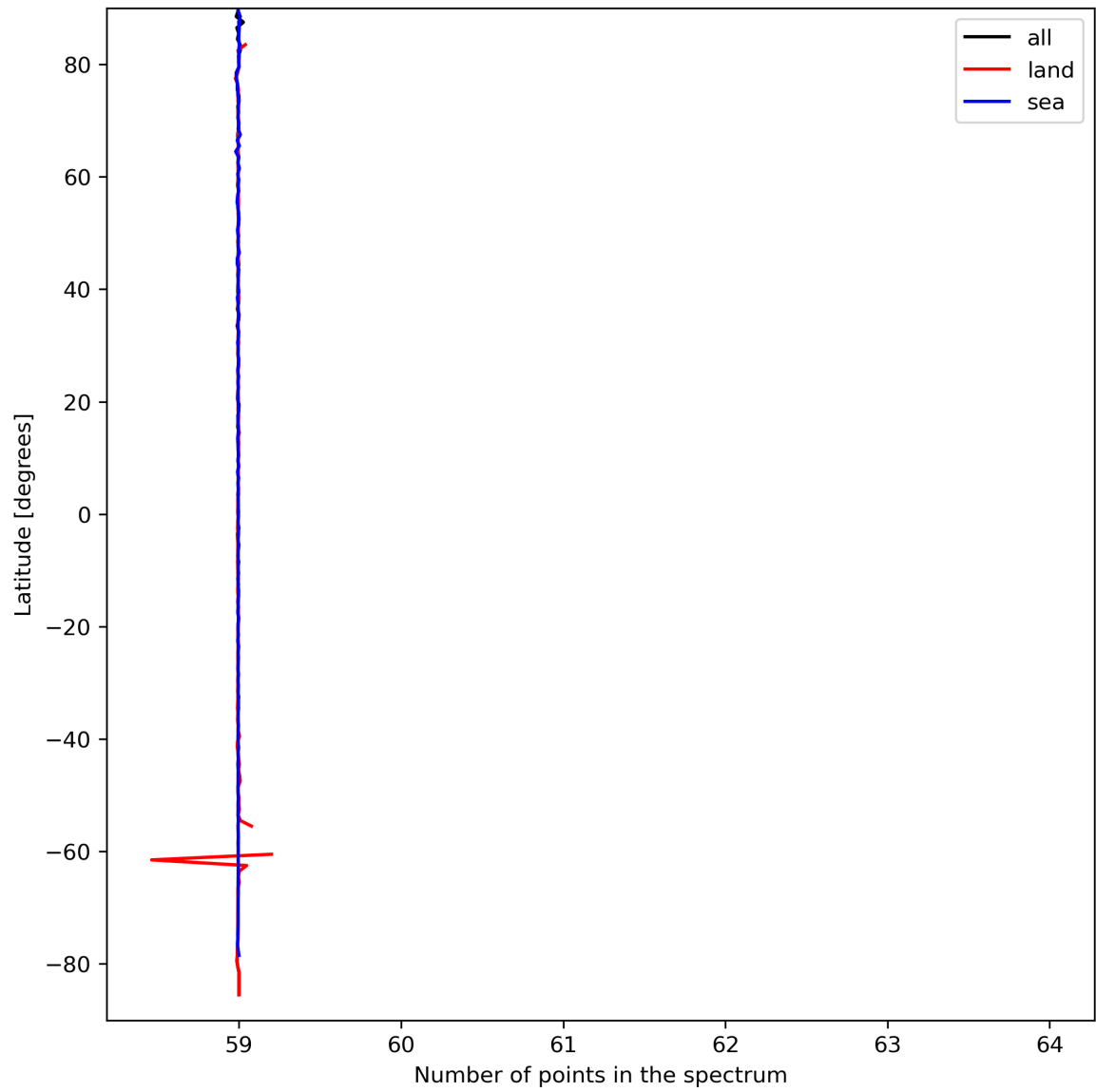
Figure 27: Zonal average of “Number of points in the spectrum” for 2023-09-15 to 2023-09-16.
