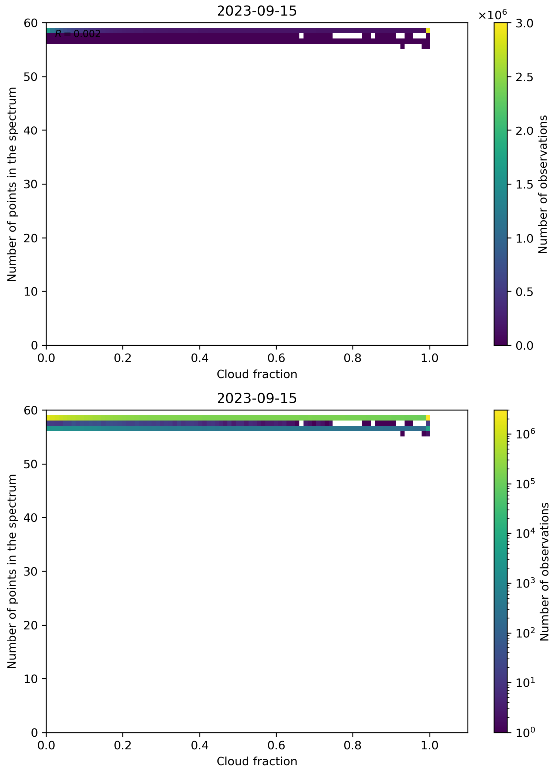
Figure 81: Scatter density plot of “Cloud fraction” against “Number of points in the spectrum” for 2023-09-15 to 2023-09-16.
