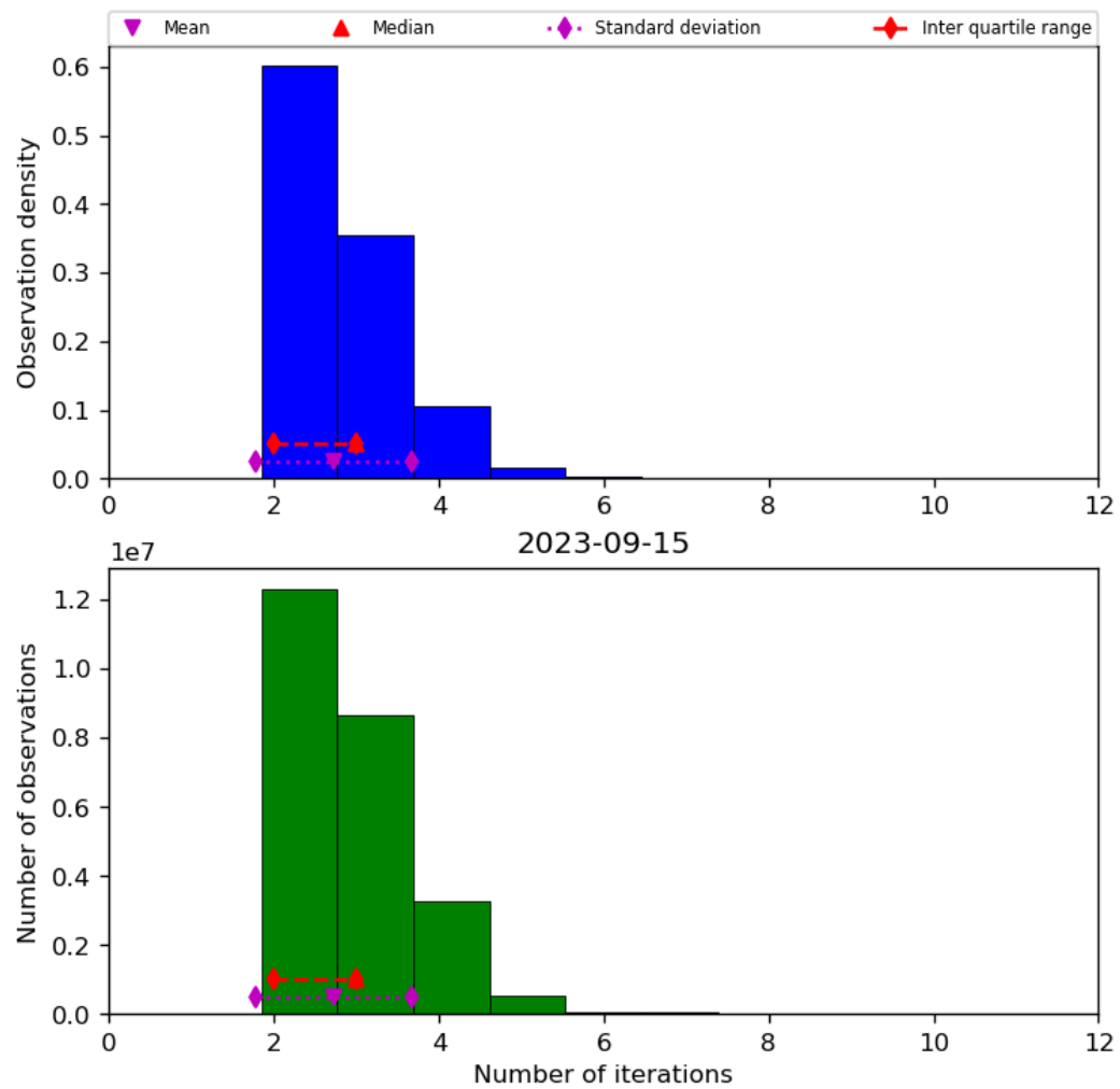
Figure 39: Histogram of “Number of iterations” for 2023-09-15 to 2023-09-16
