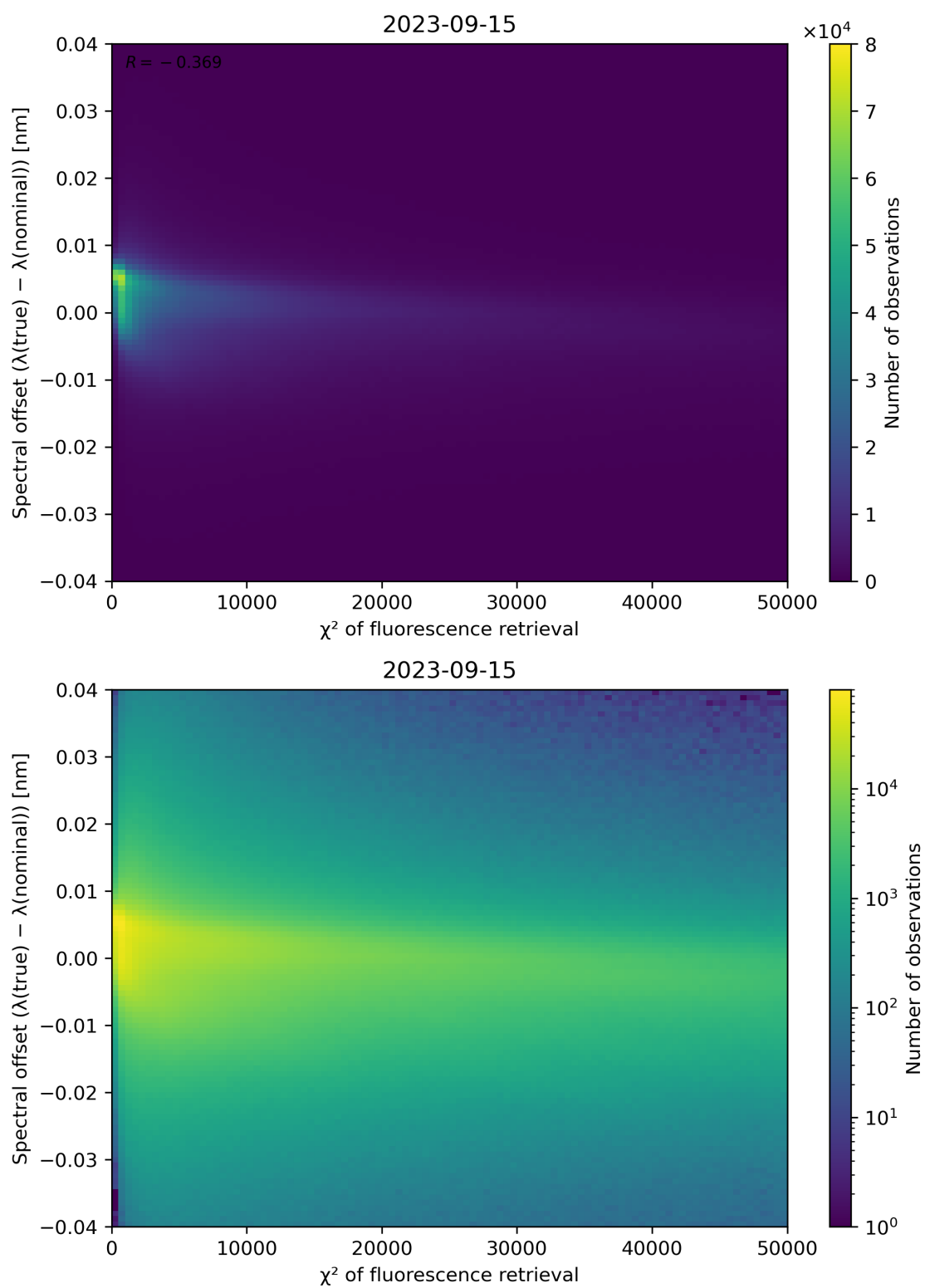
Figure 72: Scatter density plot of " \chi^2 of fluorescence retrieval" against "Spectral offset ( \lambda(\text{true}) - \lambda(\text{nominal}) )" for 2023-09-15 to 2023-09-16.
