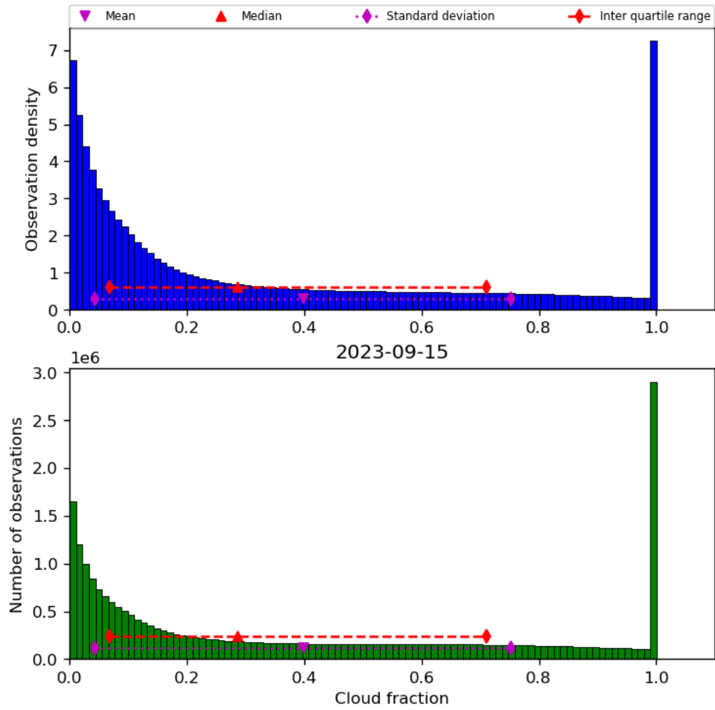
Figure 32: Histogram of “Cloud fraction” for 2023-09-15 to 2023-09-16
