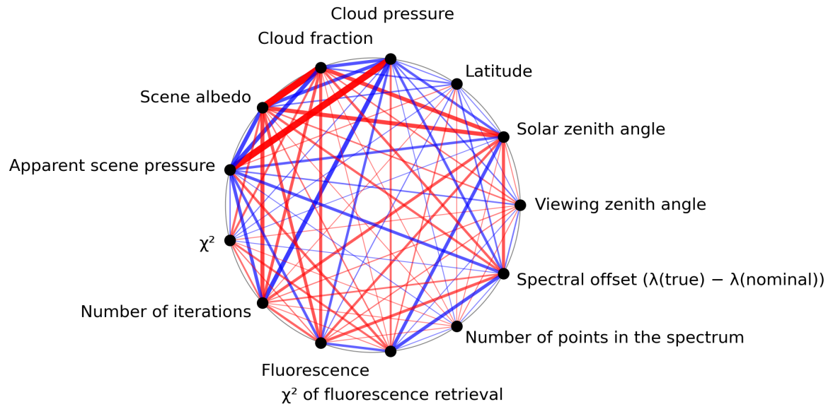
Figure 1: Map of correlation graph for 2023-09-15 to 2023-09-16.
