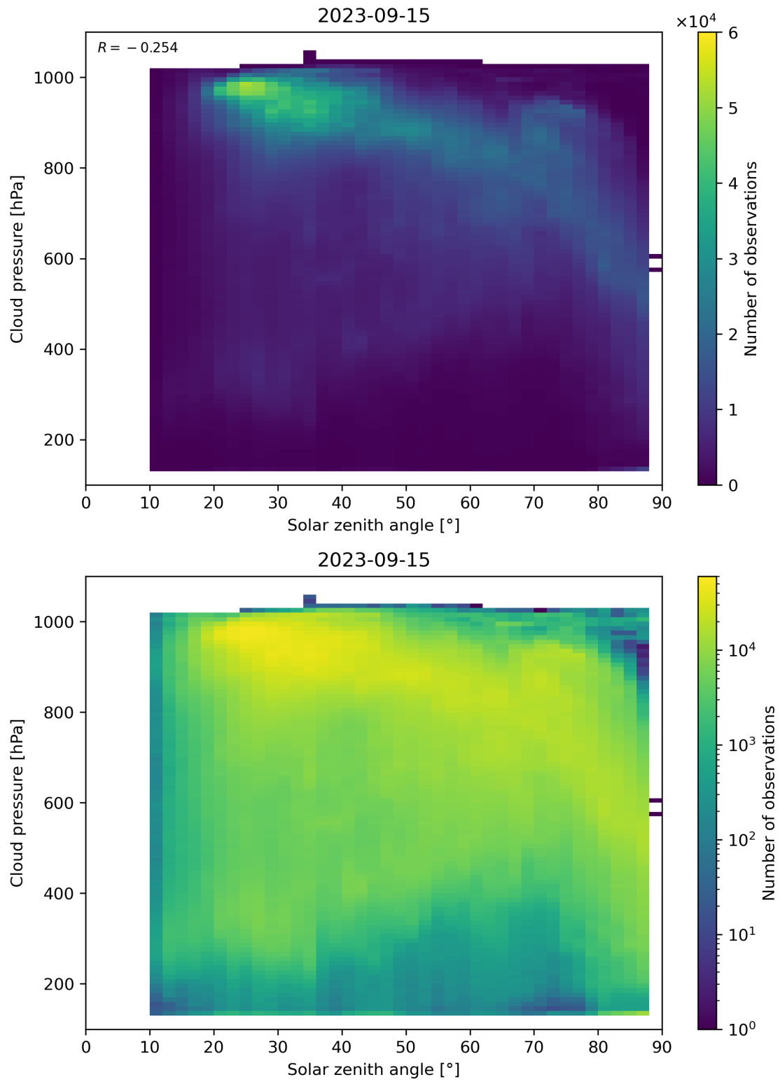
Figure 122: Scatter density plot of “Solar zenith angle” against “Cloud pressure” for 2023-09-15 to 2023-09-16.
