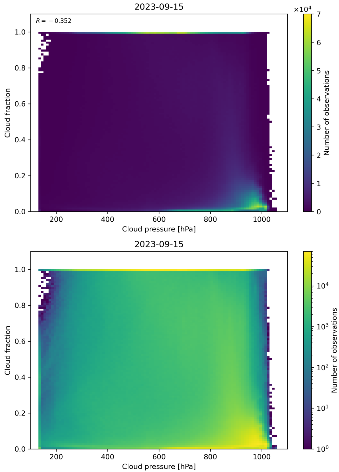
Figure 87: Scatter density plot of “Cloud pressure” against “Cloud fraction” for 2023-09-15 to 2023-09-16.
