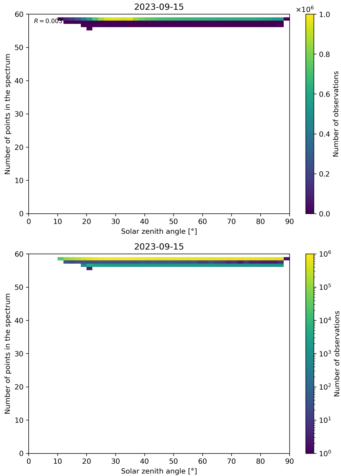
Figure 126: Scatter density plot of “Solar zenith angle” against “Number of points in the spectrum” for 2023-09-15 to 2023-09-16.
