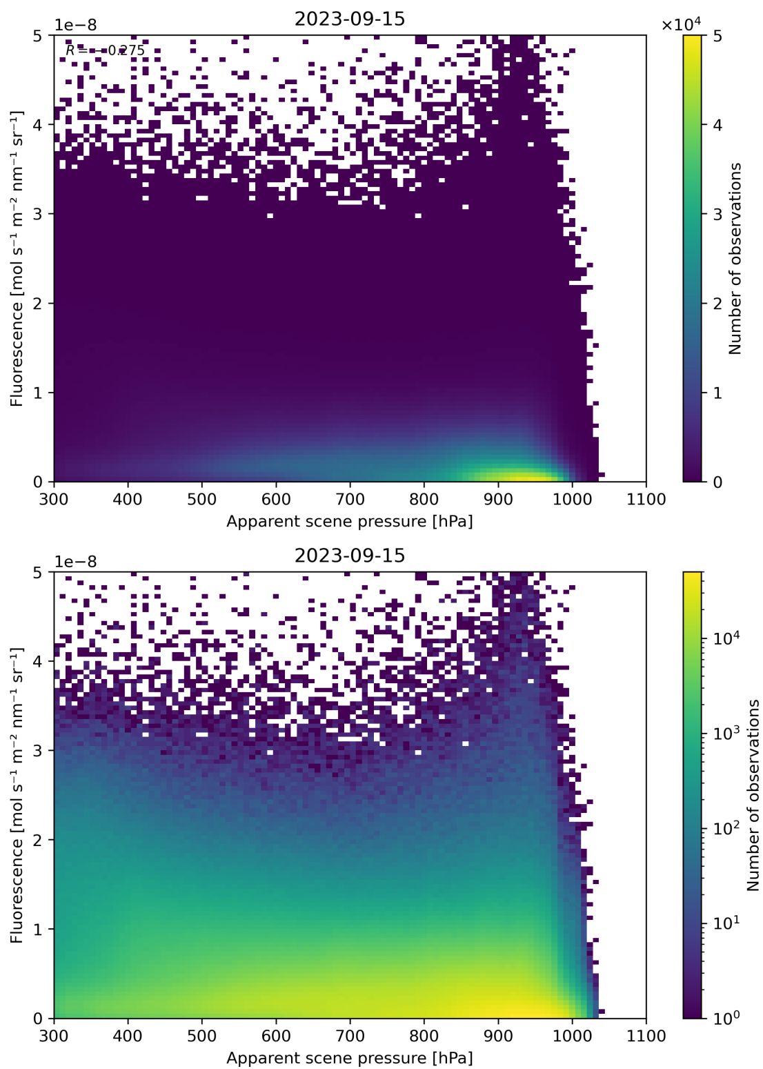
Figure 65: Scatter density plot of “Apparent scene pressure” against “Fluorescence” for 2023-09-15 to 2023-09-16.
