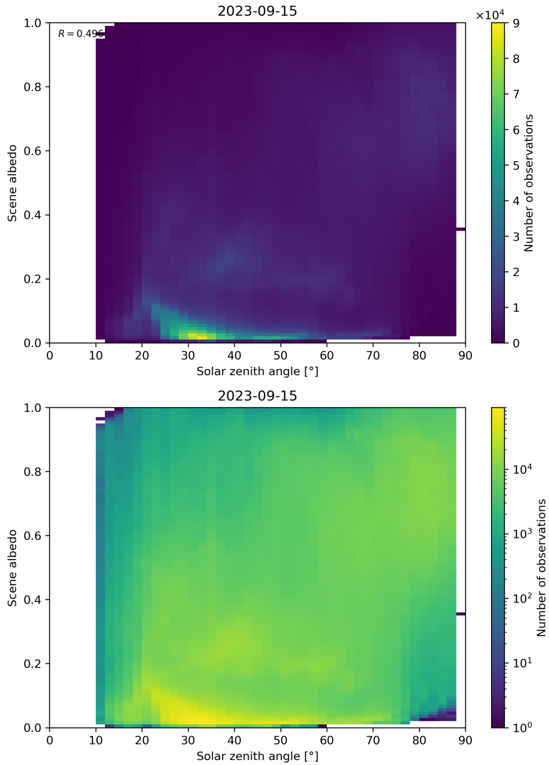
Figure 127: Scatter density plot of “Solar zenith angle” against “Scene albedo” for 2023-09-15 to 2023-09-16.
