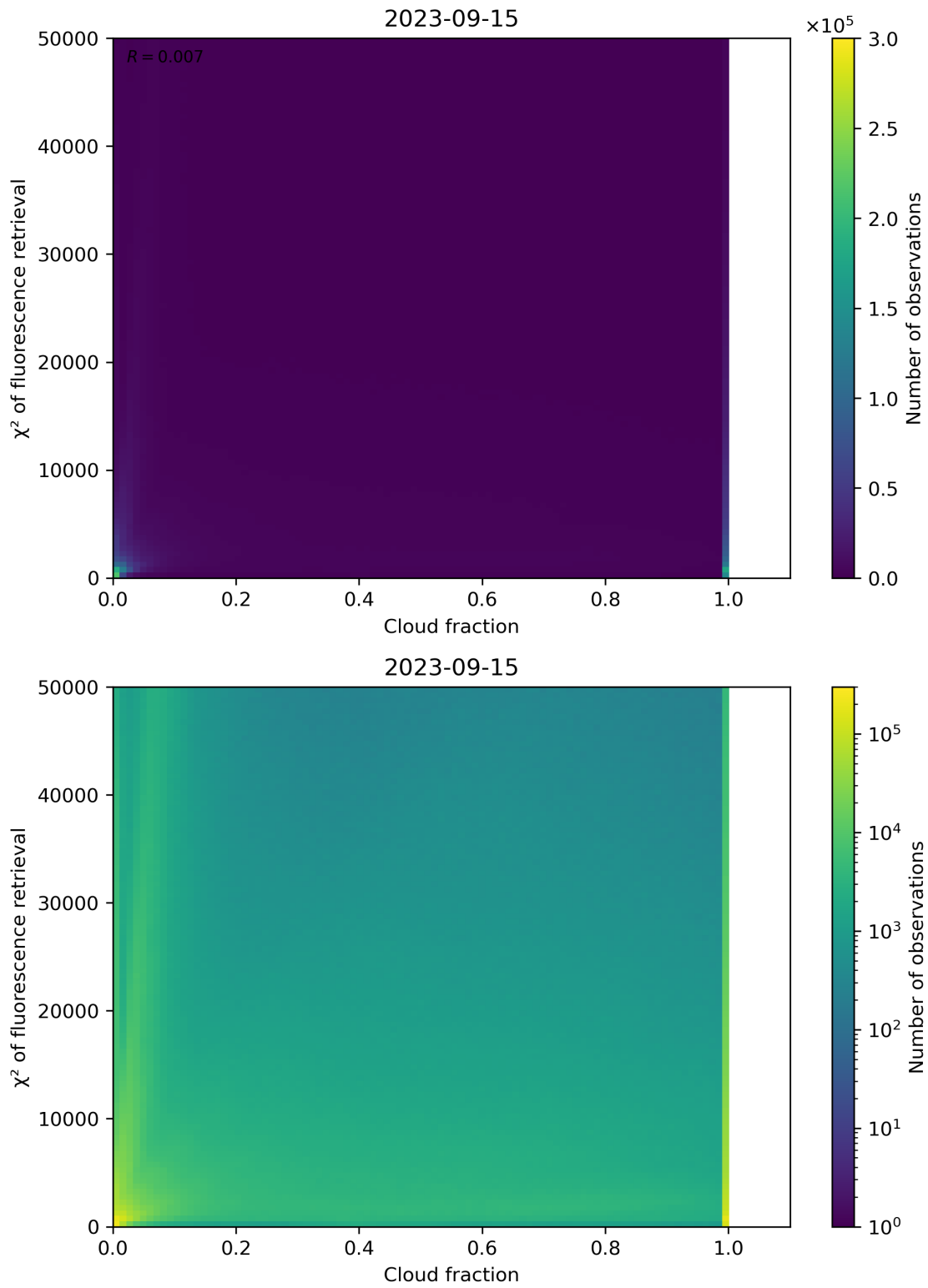
Figure 78: Scatter density plot of “Cloud fraction” against “ \chi^2 of fluorescence retrieval” for 2023-09-15 to 2023-09-16.
