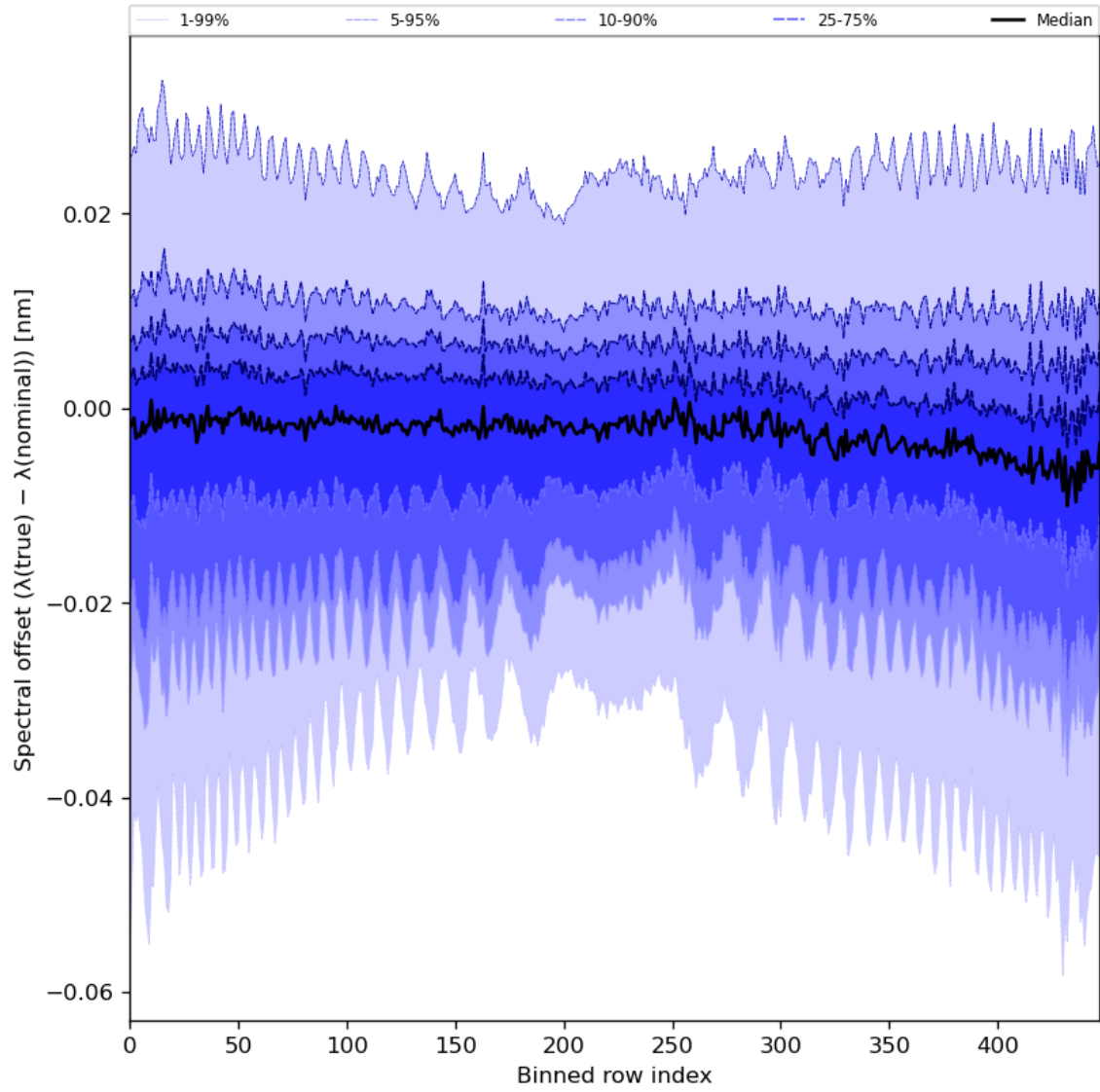
Figure 62: Along track statistics of “Spectral offset ( \lambda(\text{true}) - \lambda(\text{nominal}) )” for 2023-09-15 to 2023-09-16
