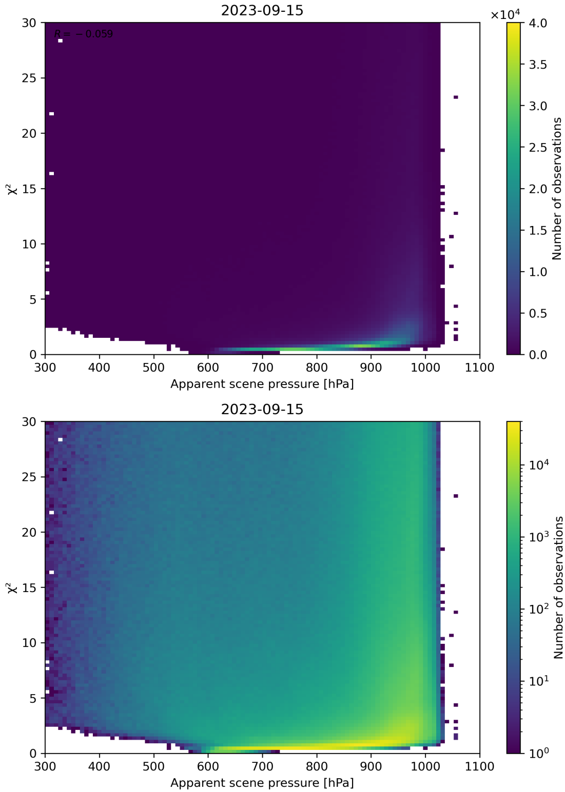
Figure 63: Scatter density plot of “Apparent scene pressure” against “ \chi^2 ” for 2023-09-15 to 2023-09-16.
