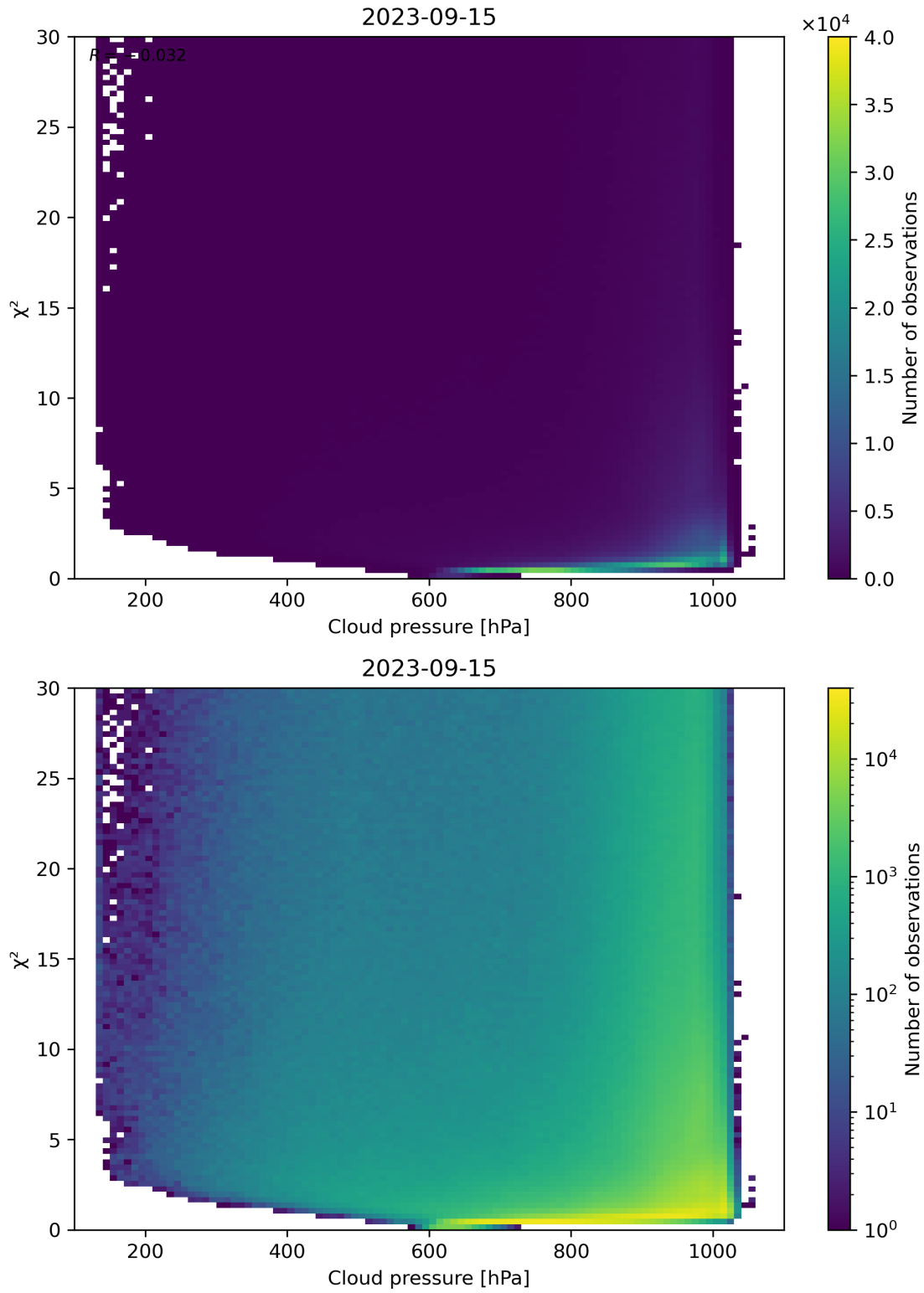
Figure 85: Scatter density plot of “Cloud pressure” against “ \chi^2 ” for 2023-09-15 to 2023-09-16.
