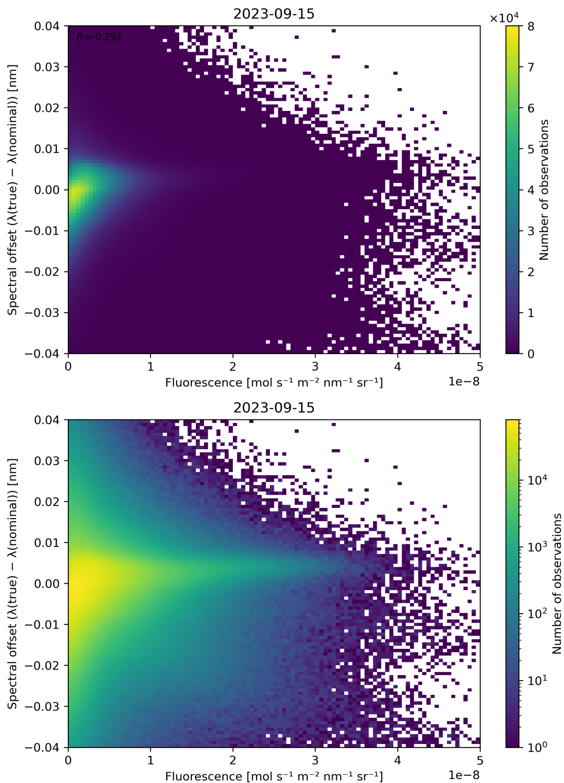
Figure 95: Scatter density plot of “Fluorescence” against “Spectral offset ( \lambda(\text{true}) - \lambda(\text{nominal}) )” for 2023-09-15 to 2023-09-16.
