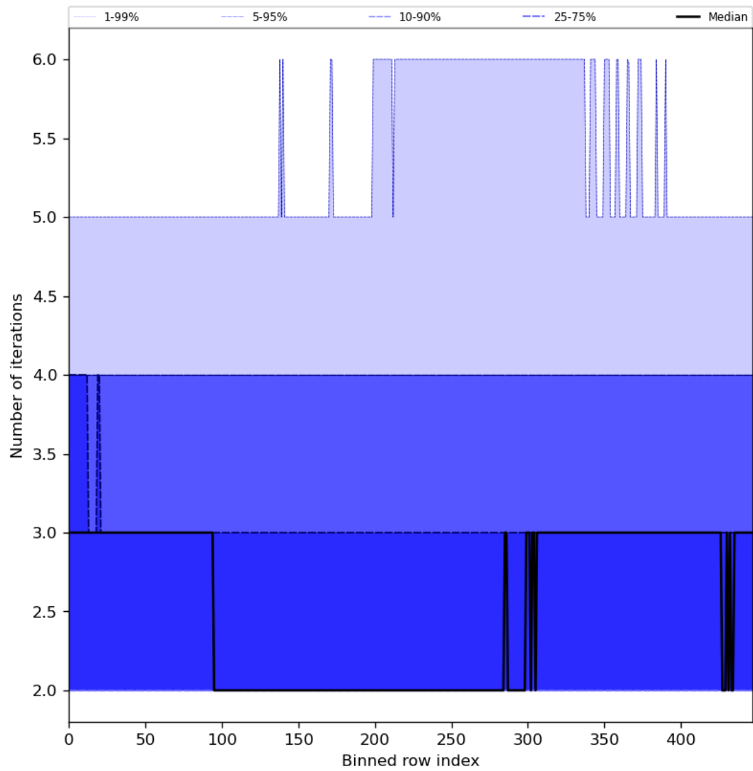
Figure 56: Along track statistics of “Number of iterations” for 2023-09-15 to 2023-09-16
