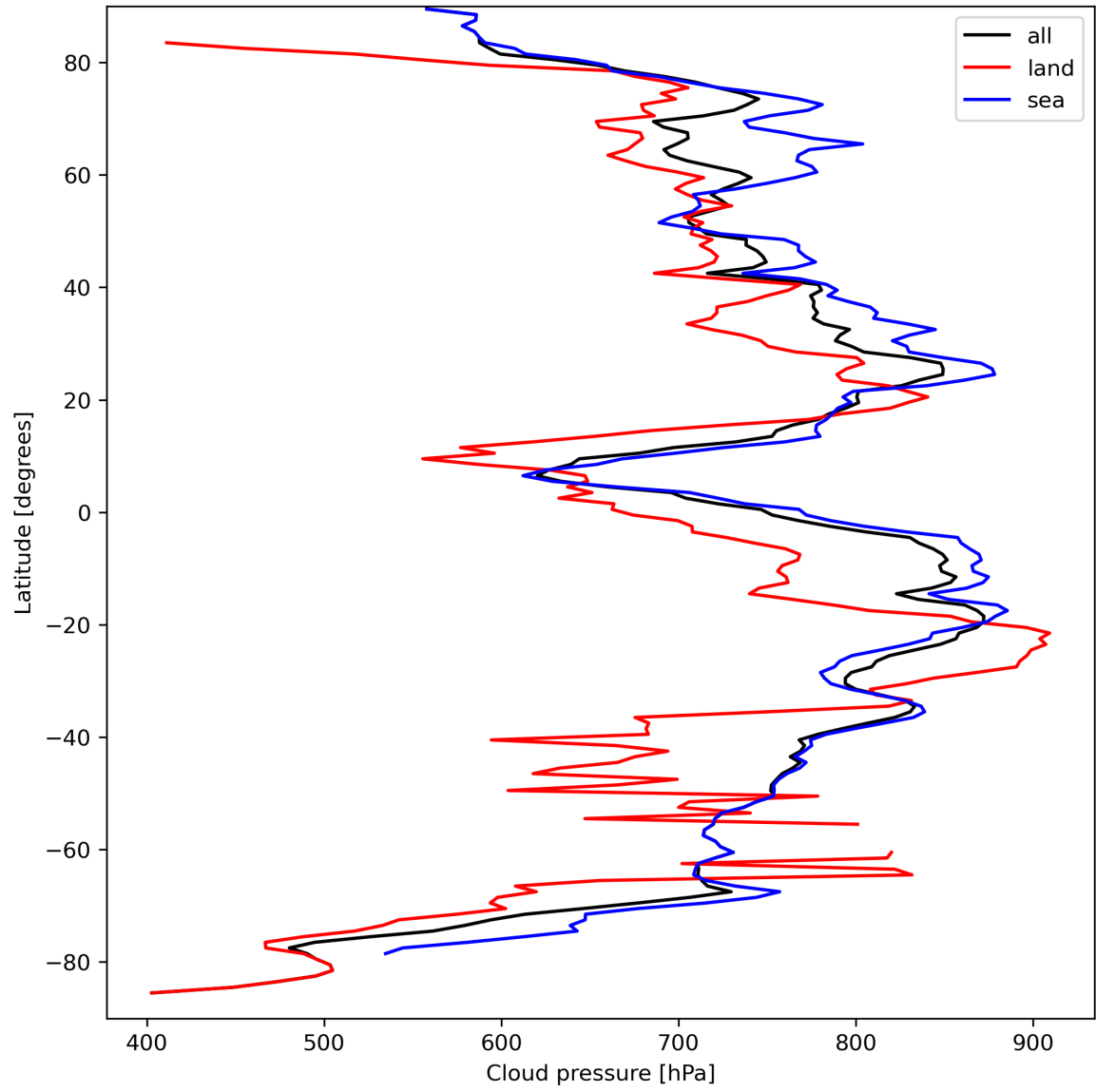
Figure 13: Zonal average of “Cloud pressure” for 2023-09-15 to 2023-09-16.
