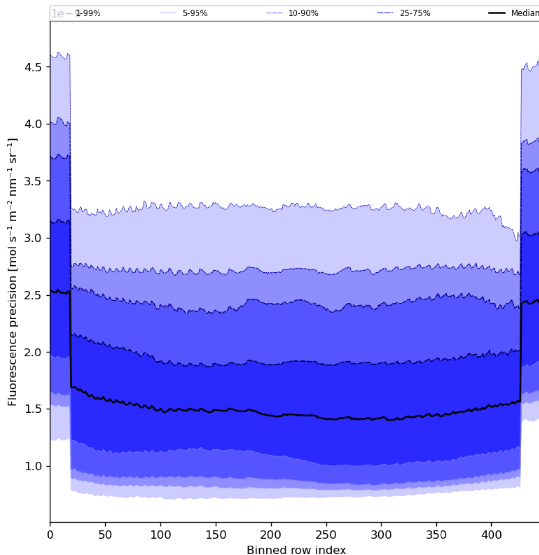
Figure 58: Along track statistics of “Fluorescence precision” for 2023-09-15 to 2023-09-16
