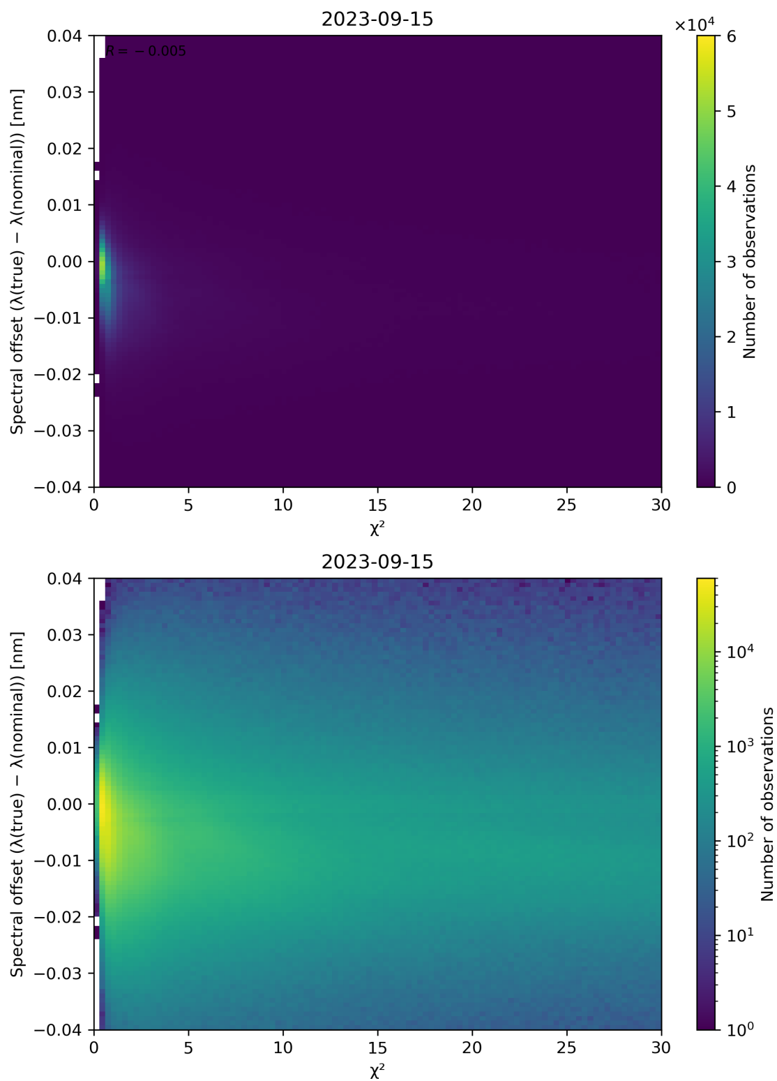
Figure 75: Scatter density plot of “ \chi^2 ” against “Spectral offset ( \lambda(\text{true}) - \lambda(\text{nominal}) )” for 2023-09-15 to 2023-09-16.
