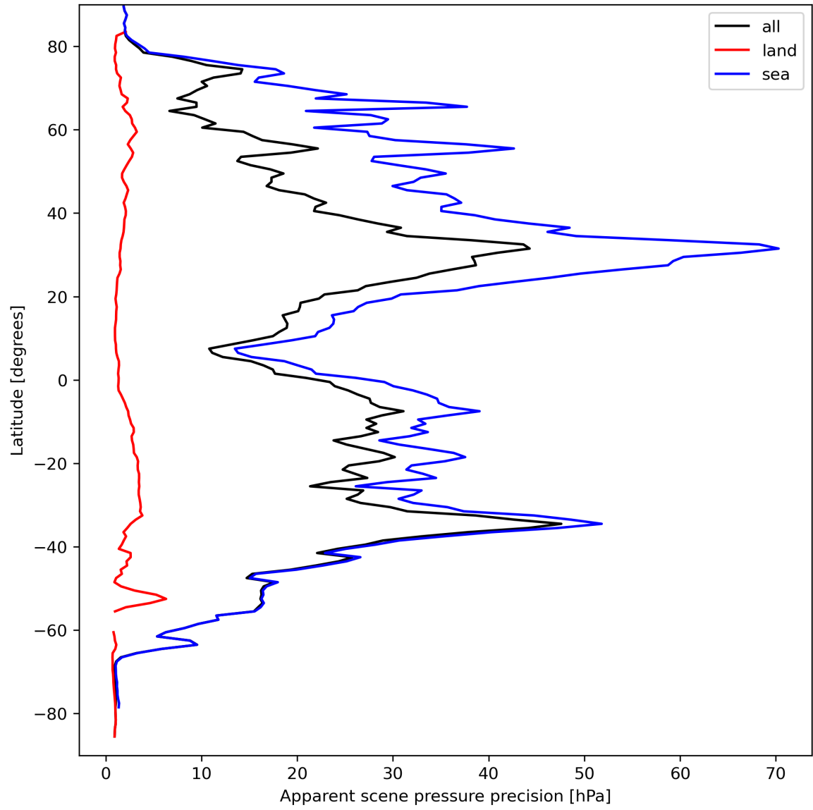
Figure 20: Zonal average of “Apparent scene pressure precision” for 2023-09-15 to 2023-09-16.
