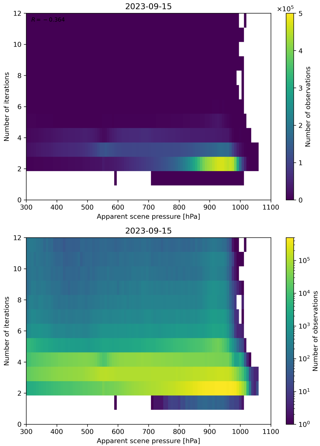
Figure 66: Scatter density plot of “Apparent scene pressure” against “Number of iterations” for 2023-09-15 to 2023-09-16.
