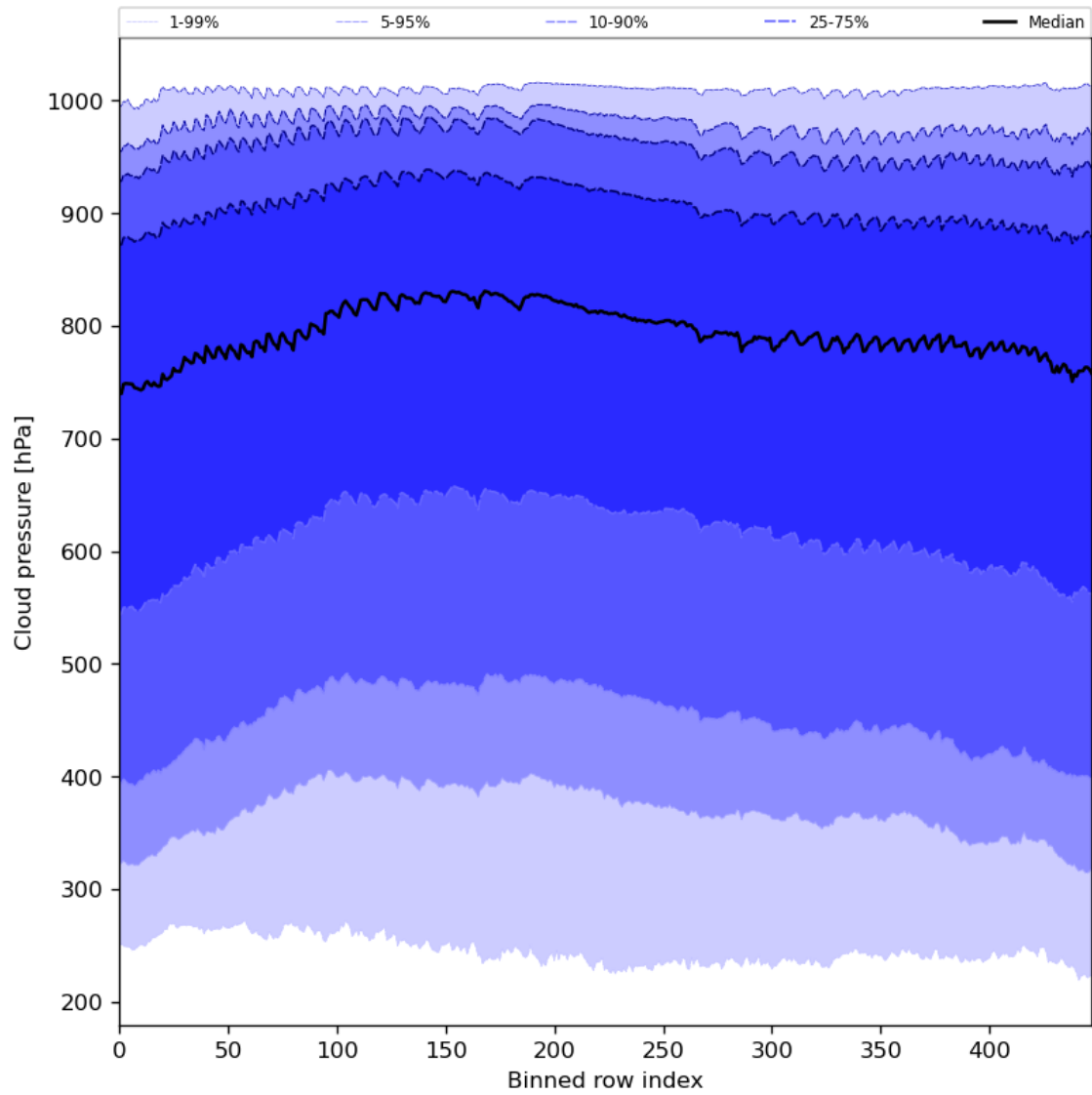
Figure 47: Along track statistics of “Cloud pressure” for 2023-09-15 to 2023-09-16
