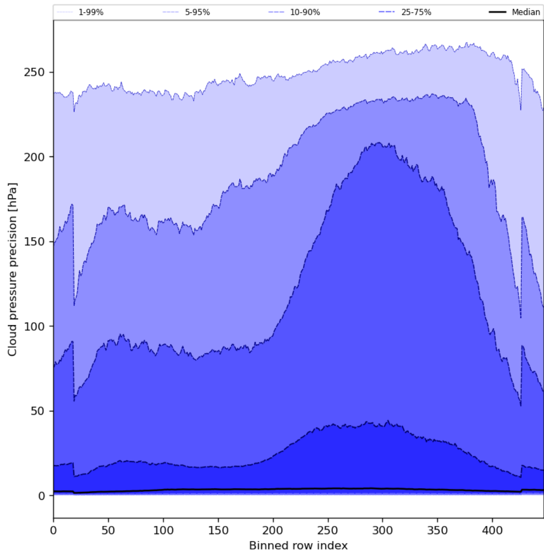
Figure 48: Along track statistics of “Cloud pressure precision” for 2023-09-15 to 2023-09-16
