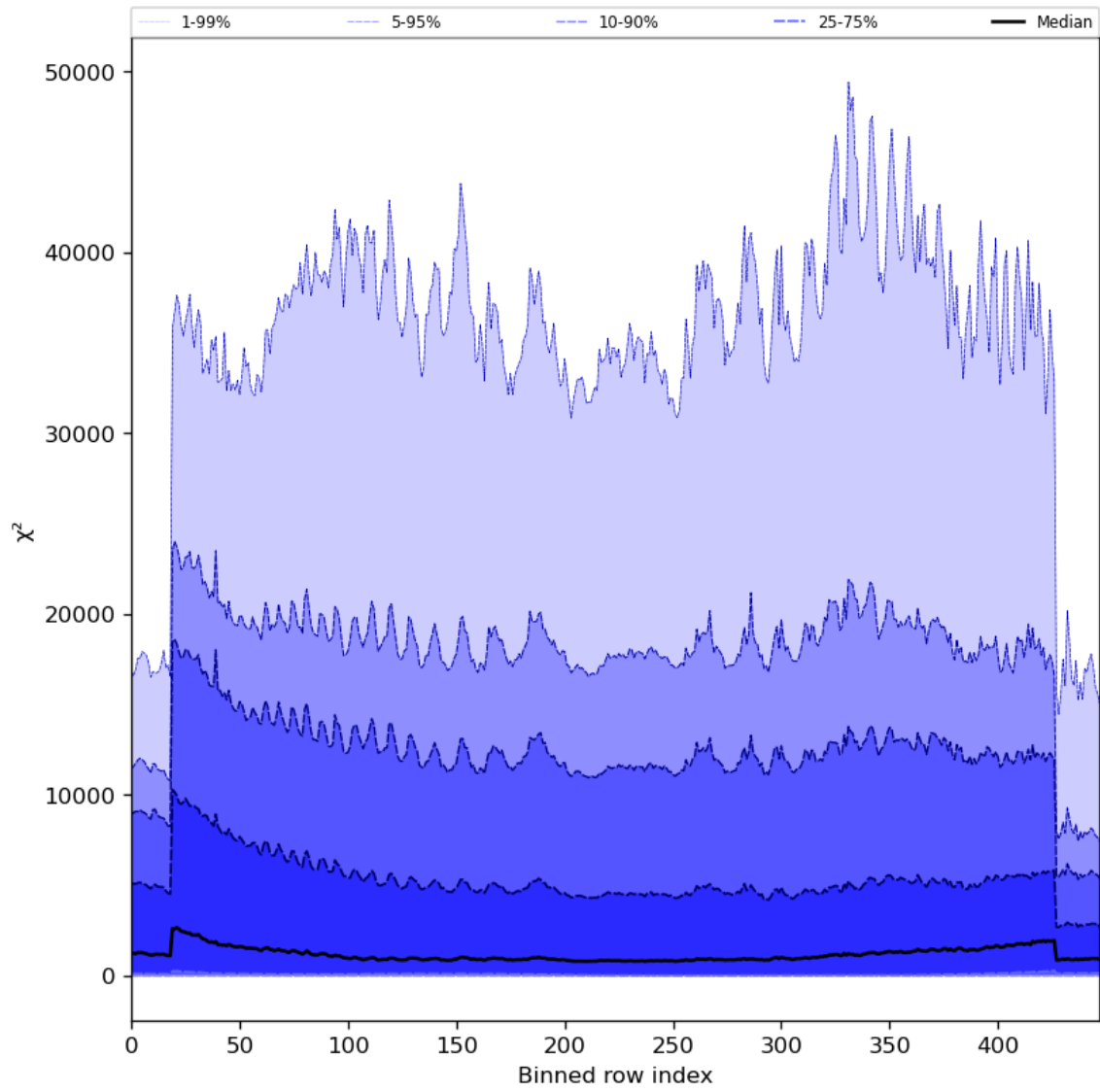
Figure 55: Along track statistics of “ \chi^2 ” for 2023-09-15 to 2023-09-16
