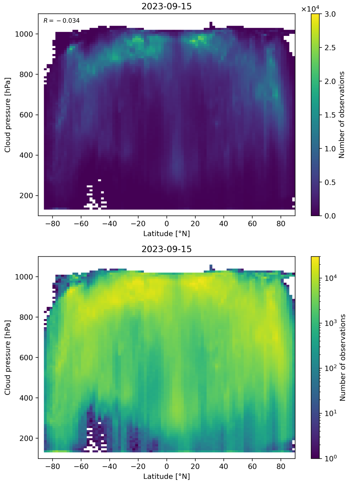
Figure 100: Scatter density plot of “Latitude” against “Cloud pressure” for 2023-09-15 to 2023-09-16.
