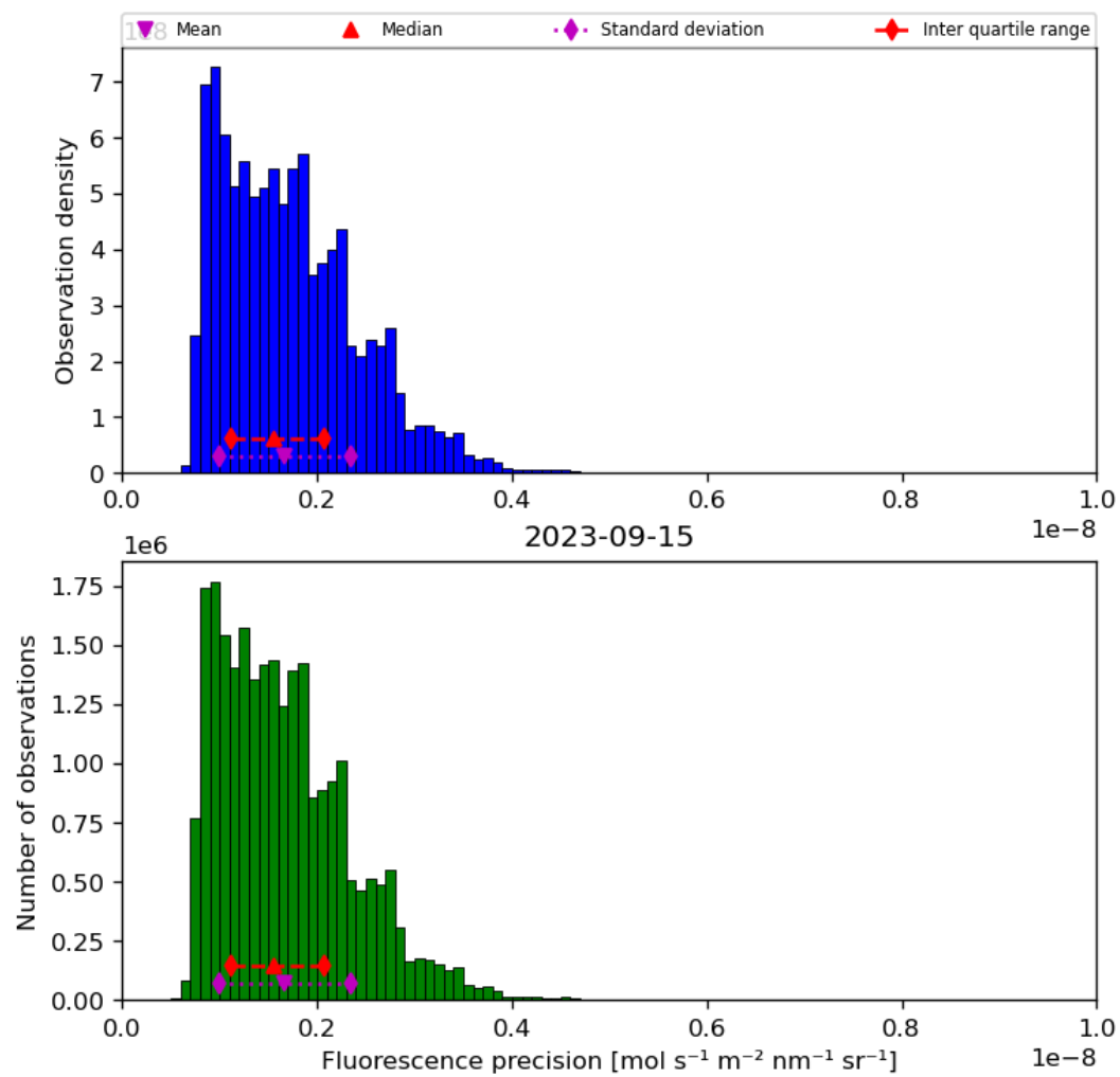
Figure 41: Histogram of “Fluorescence precision” for 2023-09-15 to 2023-09-16
