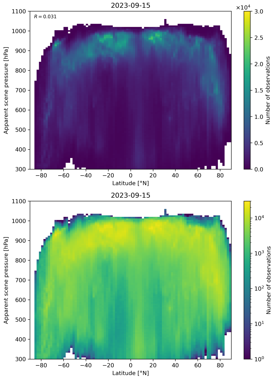
Figure 96: Scatter density plot of “Latitude” against “Apparent scene pressure” for 2023-09-15 to 2023-09-16.
