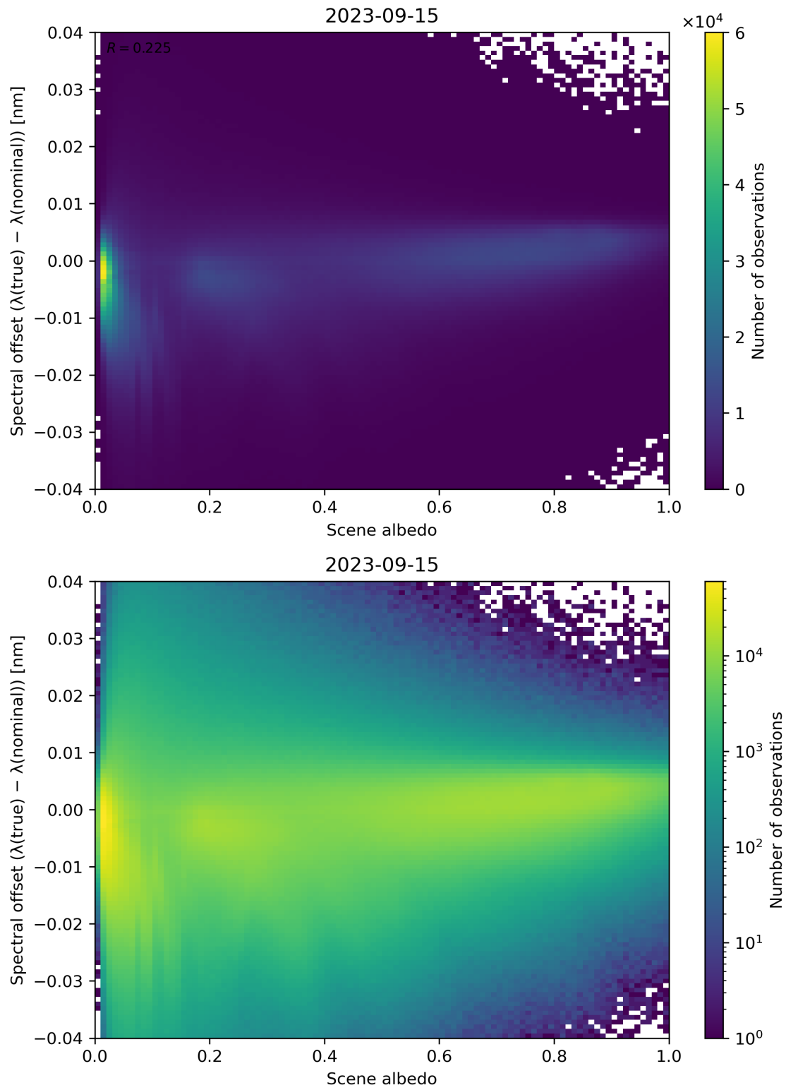
Figure 117: Scatter density plot of “Scene albedo” against “Spectral offset ( \lambda(\text{true}) - \lambda(\text{nominal}) )” for 2023-09-15 to 2023-09-16.
