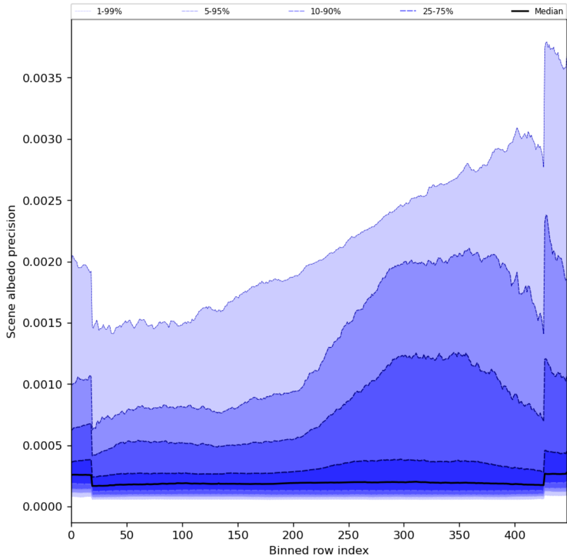
Figure 52: Along track statistics of “Scene albedo precision” for 2023-09-15 to 2023-09-16
