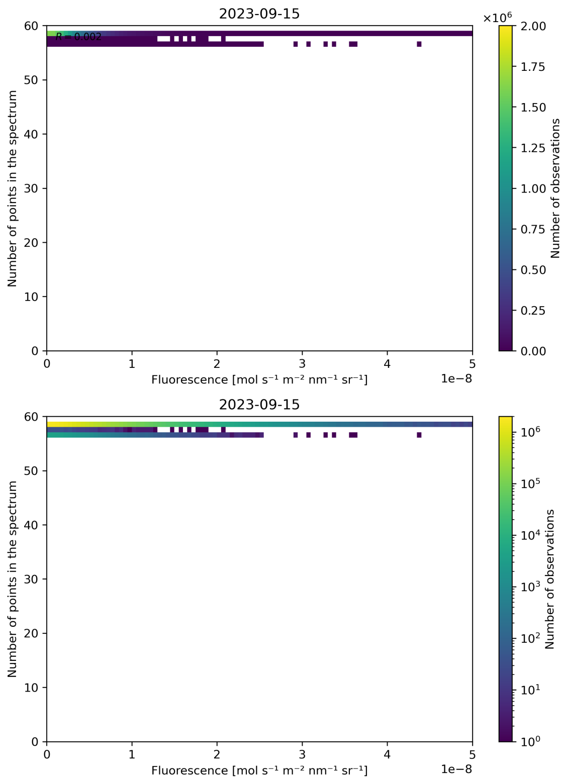
Figure 94: Scatter density plot of “Fluorescence” against “Number of points in the spectrum” for 2023-09-15 to 2023-09-16.
