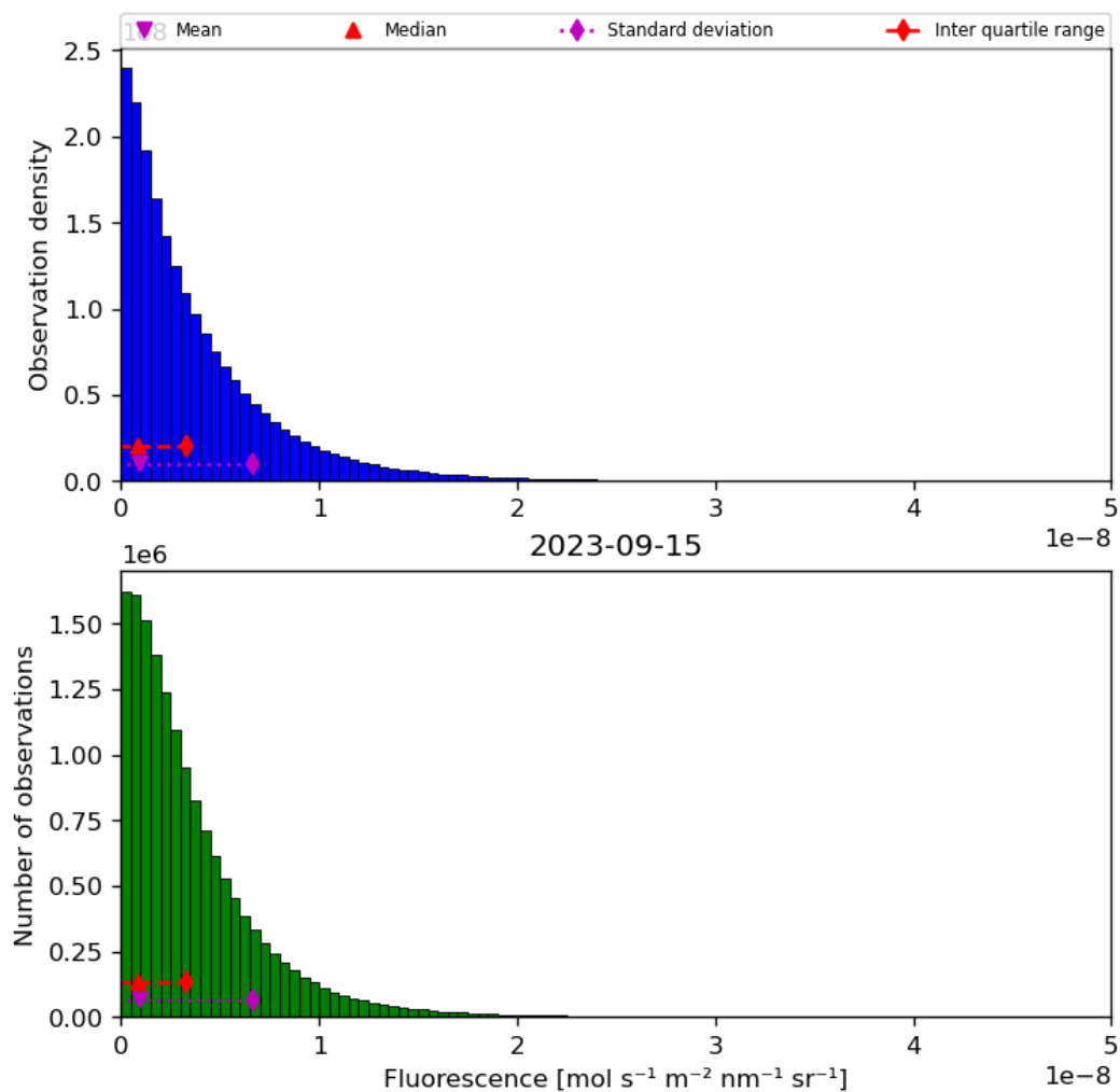
Figure 40: Histogram of “Fluorescence” for 2023-09-15 to 2023-09-16
