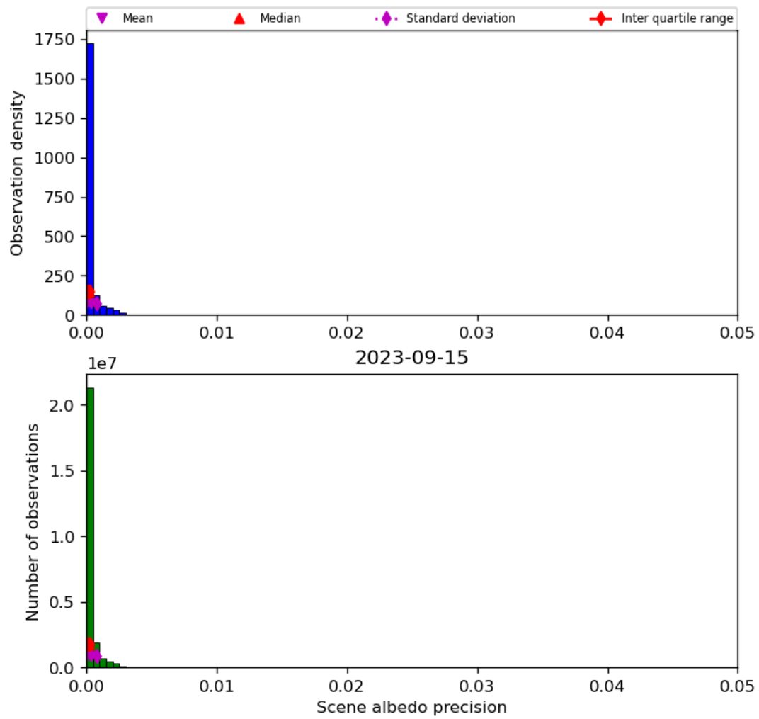
Figure 35: Histogram of “Scene albedo precision” for 2023-09-15 to 2023-09-16
