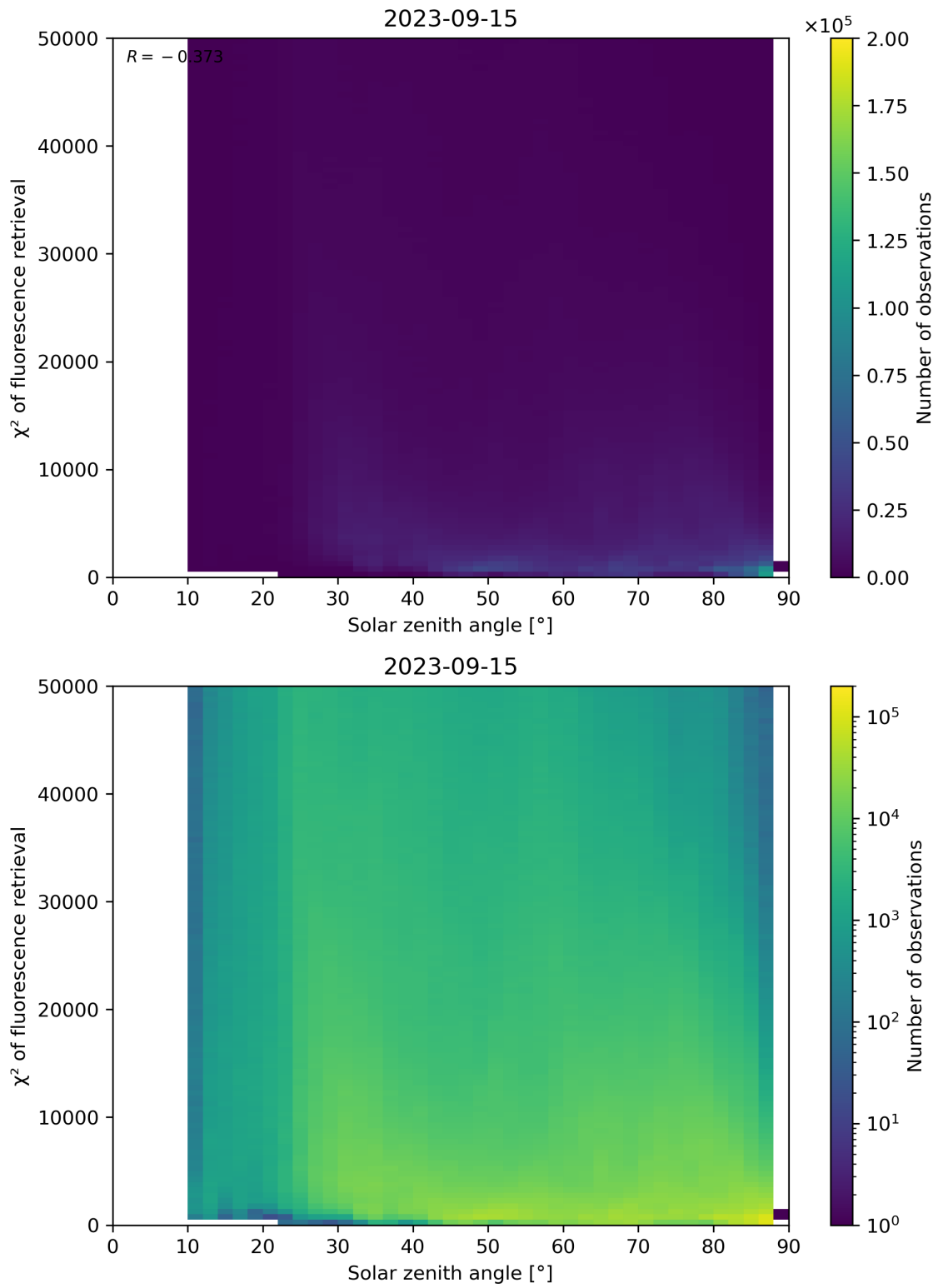
Figure 120: Scatter density plot of “Solar zenith angle” against “ \chi^2 of fluorescence retrieval” for 2023-09-15 to 2023-09-16.
