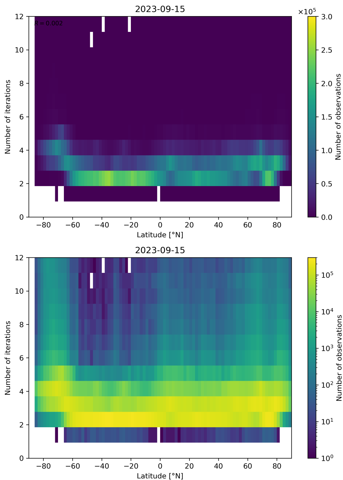
Figure 102: Scatter density plot of “Latitude” against “Number of iterations” for 2023-09-15 to 2023-09-16.
