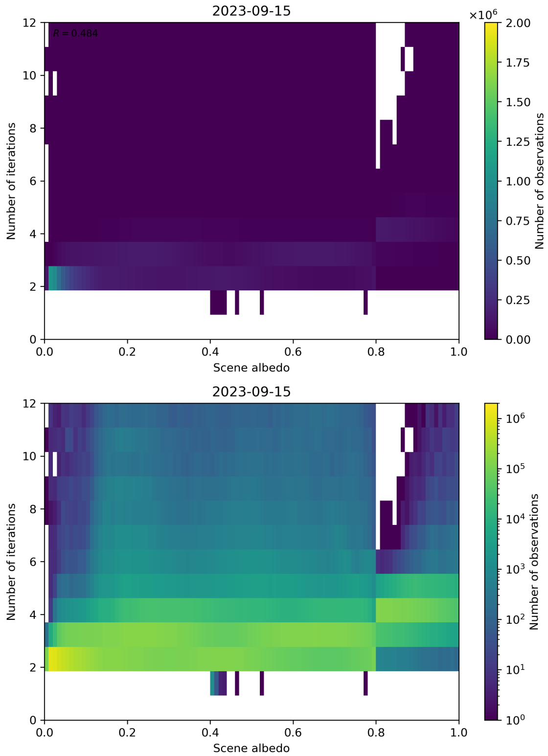
Figure 115: Scatter density plot of “Scene albedo” against “Number of iterations” for 2023-09-15 to 2023-09-16.
