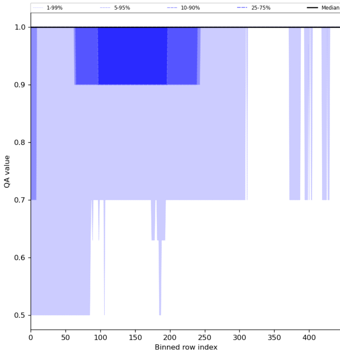
Figure 46: Along track statistics of “QA value” for 2023-09-15 to 2023-09-16
