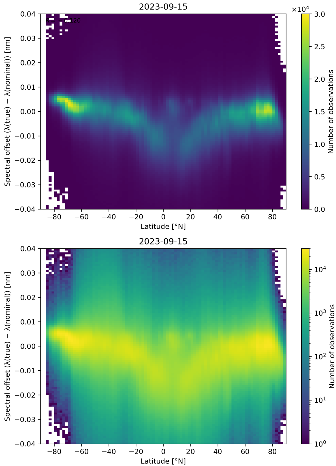
Figure 105: Scatter density plot of “Latitude” against “Spectral offset ( \lambda(\text{true}) - \lambda(\text{nominal}) )” for 2023-09-15 to 2023-09-16.
