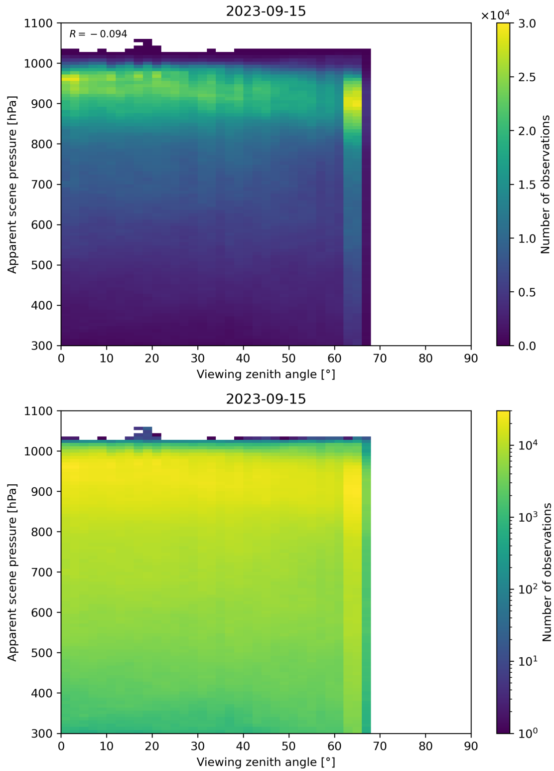
Figure 129: Scatter density plot of “Viewing zenith angle” against “Apparent scene pressure” for 2023-09-15 to 2023-09-16.
