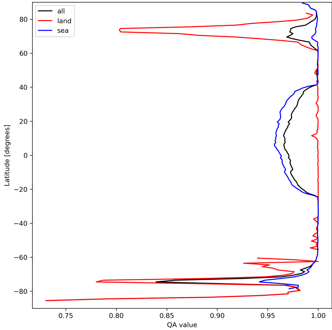
Figure 12: Zonal average of “QA value” for 2023-09-15 to 2023-09-16.
