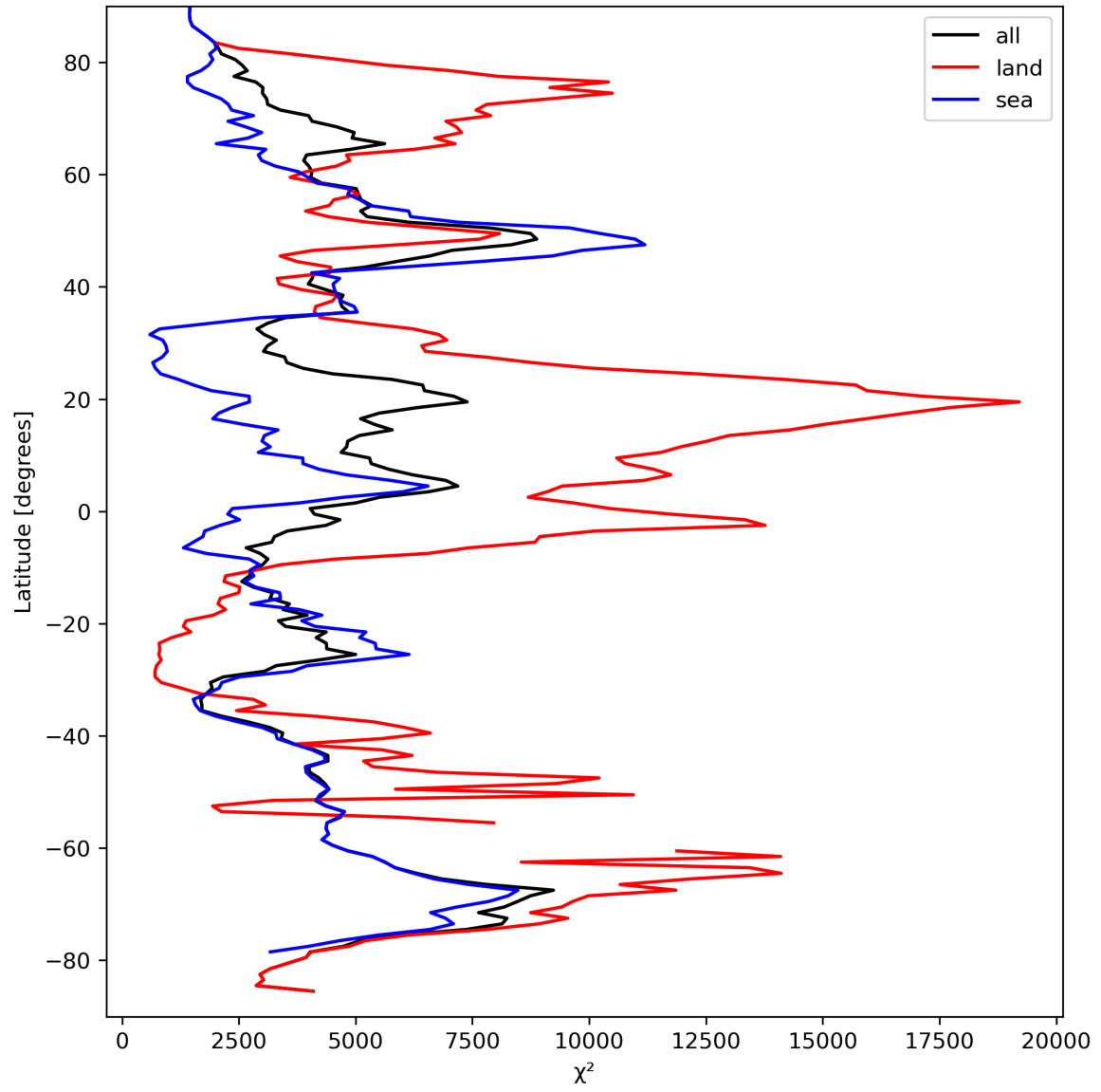
Figure 21: Zonal average of “ \chi^2 ” for 2023-09-15 to 2023-09-16.
