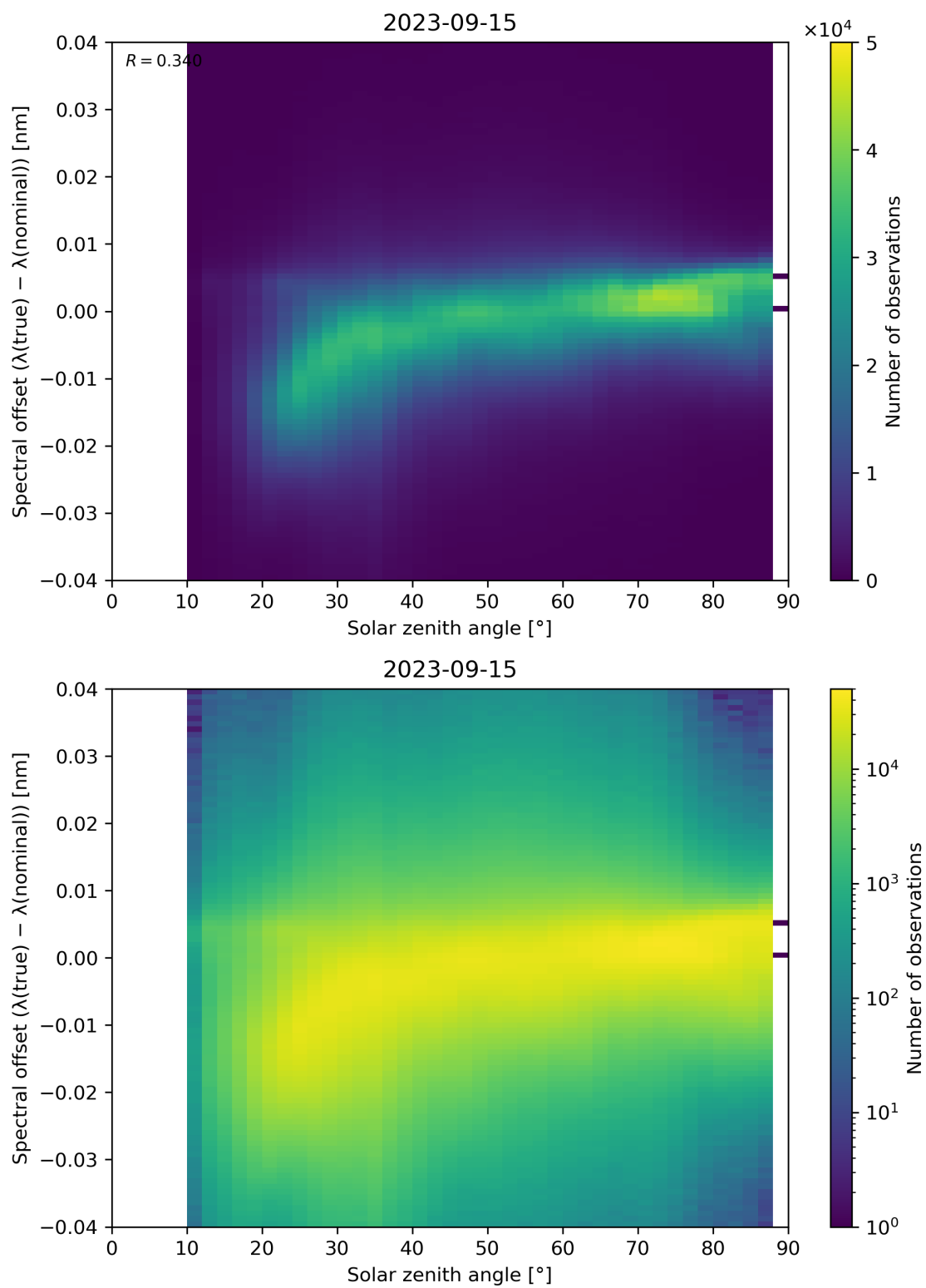
Figure 128: Scatter density plot of “Solar zenith angle” against “Spectral offset ( \lambda(\text{true}) - \lambda(\text{nominal}) )” for 2023-09-15 to 2023-09-16.
