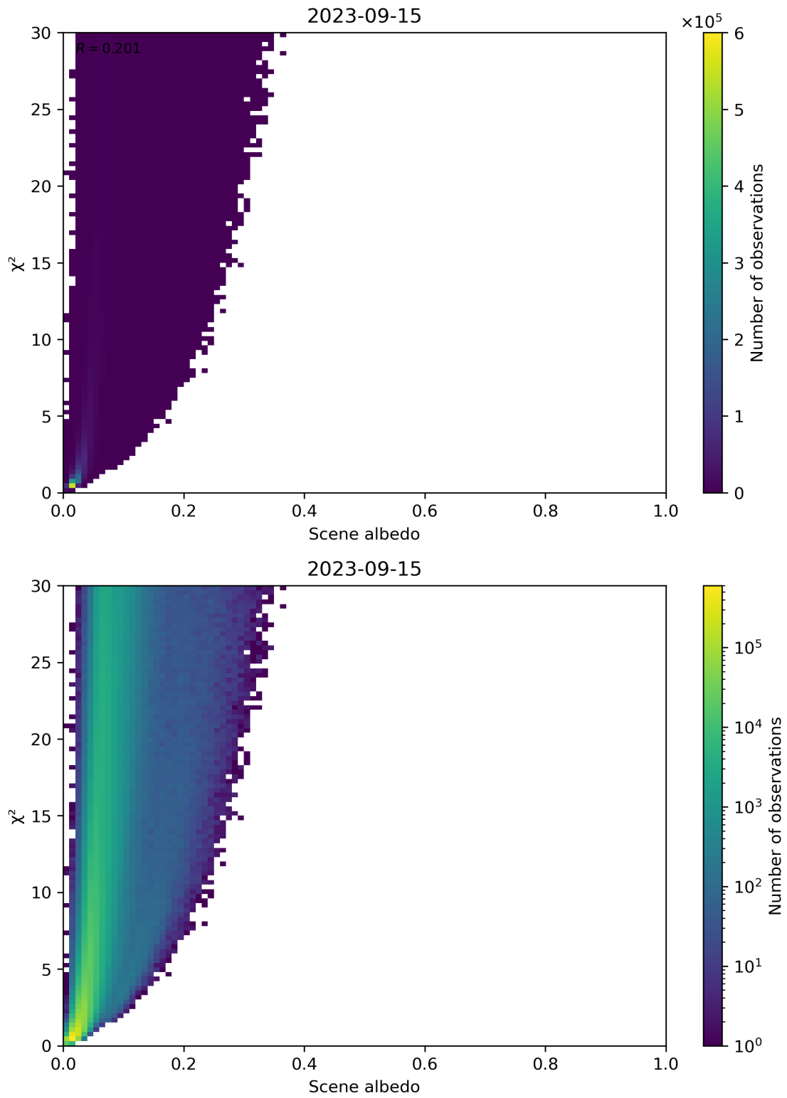
Figure 112: Scatter density plot of “Scene albedo” against “ \chi^2 ” for 2023-09-15 to 2023-09-16.
