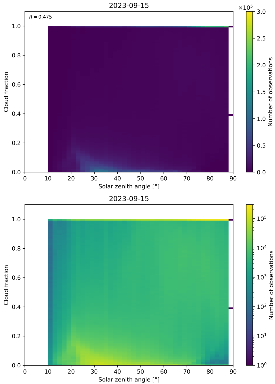
Figure 121: Scatter density plot of “Solar zenith angle” against “Cloud fraction” for 2023-09-15 to 2023-09-16.
