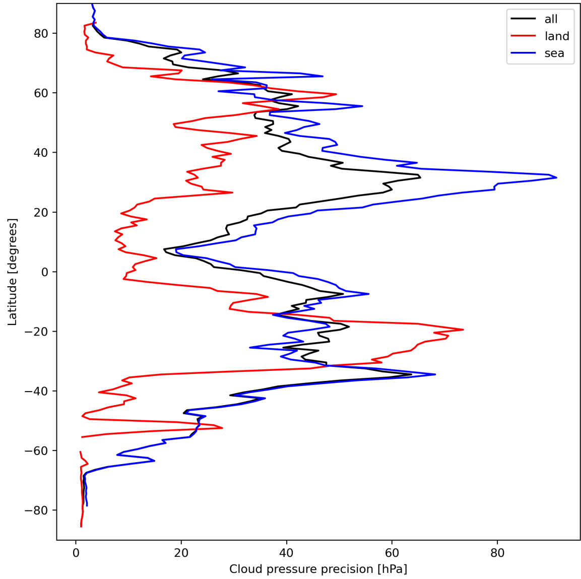
Figure 14: Zonal average of “Cloud pressure precision” for 2023-09-15 to 2023-09-16.
