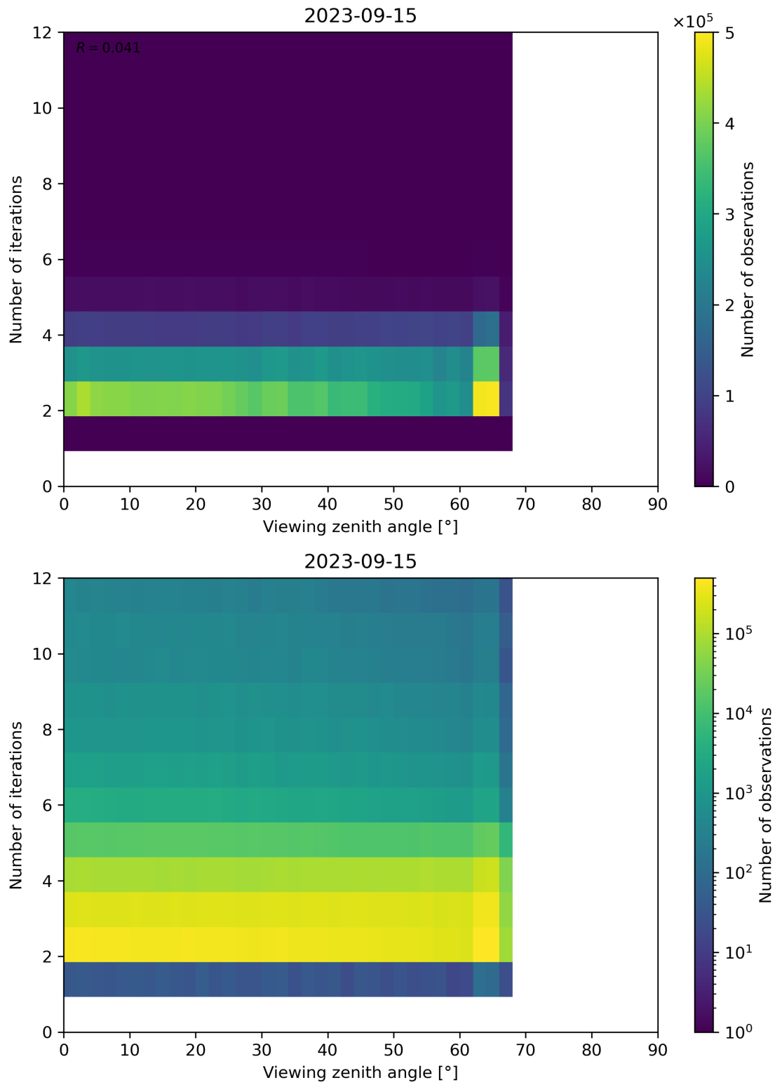
Figure 136: Scatter density plot of “Viewing zenith angle” against “Number of iterations” for 2023-09-15 to 2023-09-16.
