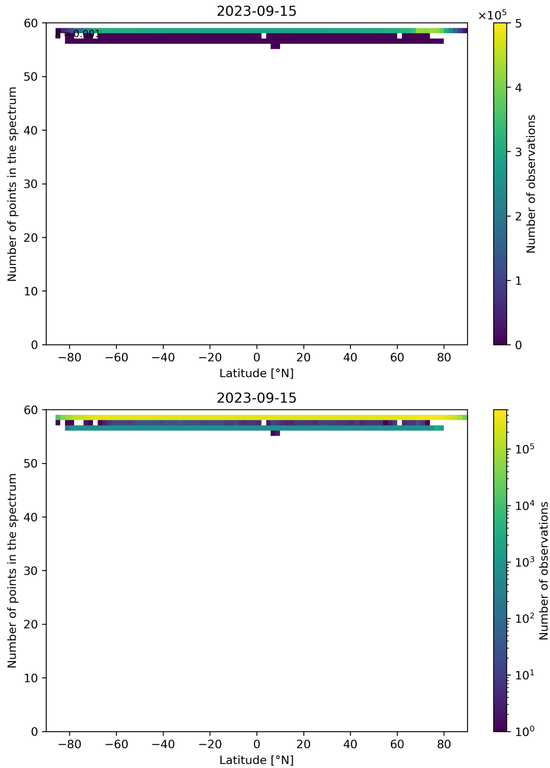
Figure 103: Scatter density plot of “Latitude” against “Number of points in the spectrum” for 2023-09-15 to 2023-09-16.
