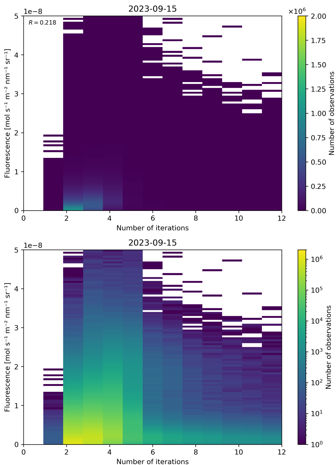
Figure 107: Scatter density plot of "Number of iterations" against "Fluorescence" for 2023-09-15 to 2023-09-16.
