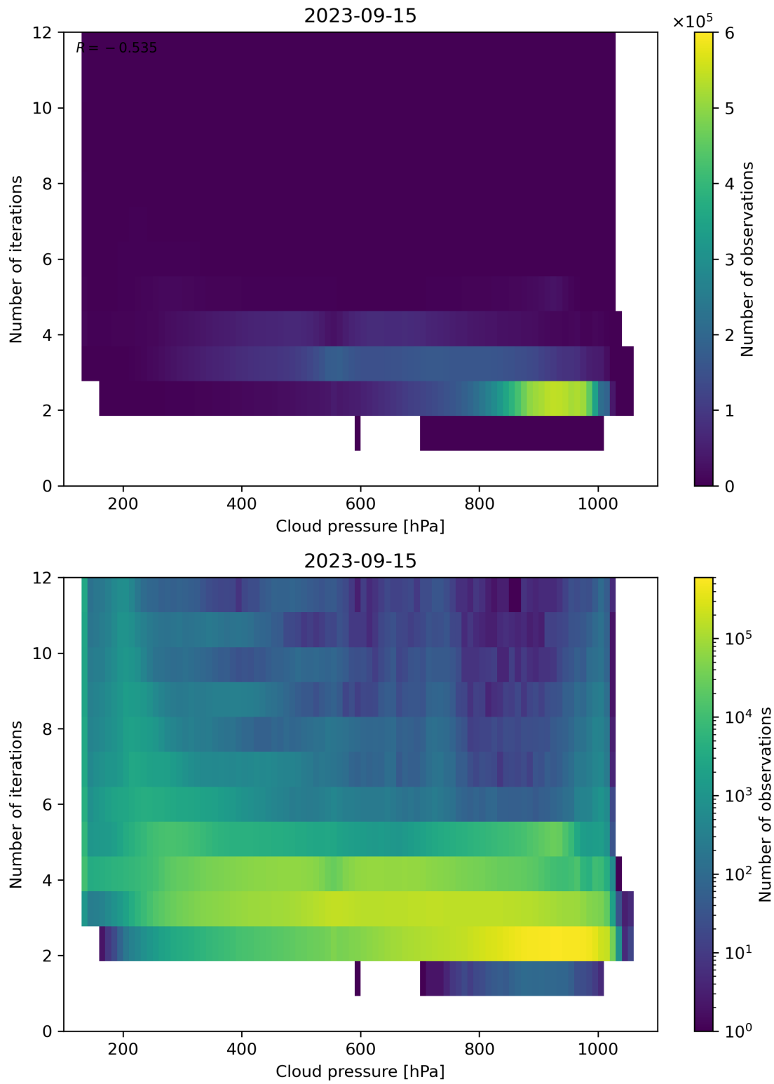
Figure 89: Scatter density plot of “Cloud pressure” against “Number of iterations” for 2023-09-15 to 2023-09-16.
