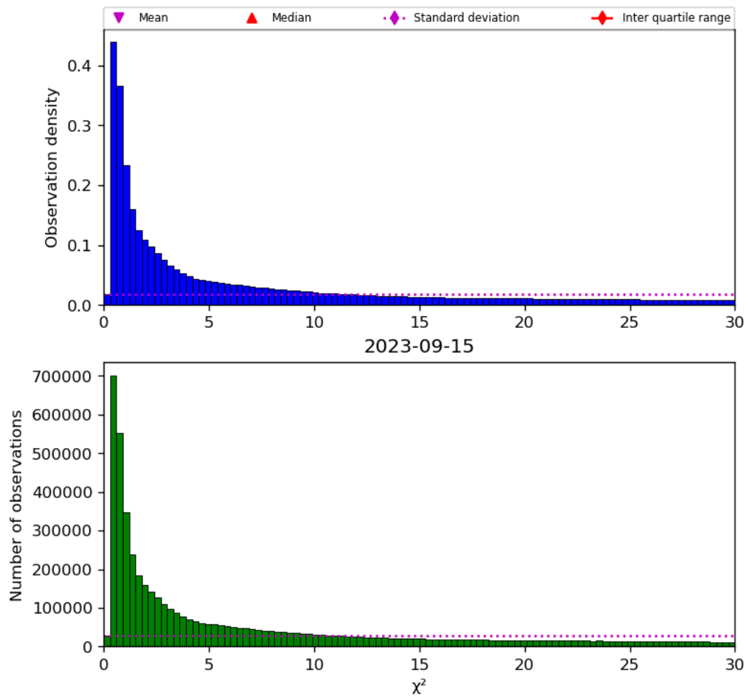
Figure 38: Histogram of “ \chi^2 ” for 2023-09-15 to 2023-09-16
