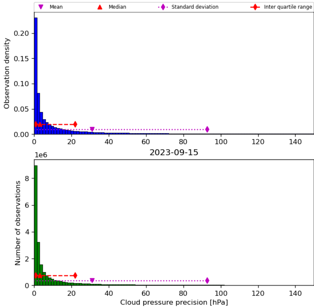
Figure 31: Histogram of “Cloud pressure precision” for 2023-09-15 to 2023-09-16
