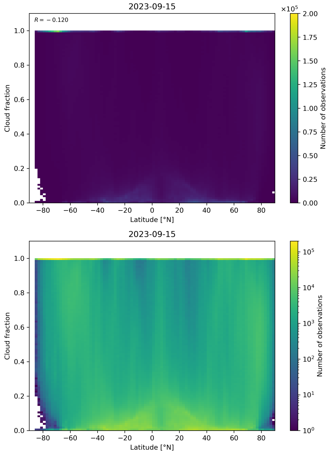
Figure 99: Scatter density plot of “Latitude” against “Cloud fraction” for 2023-09-15 to 2023-09-16.
