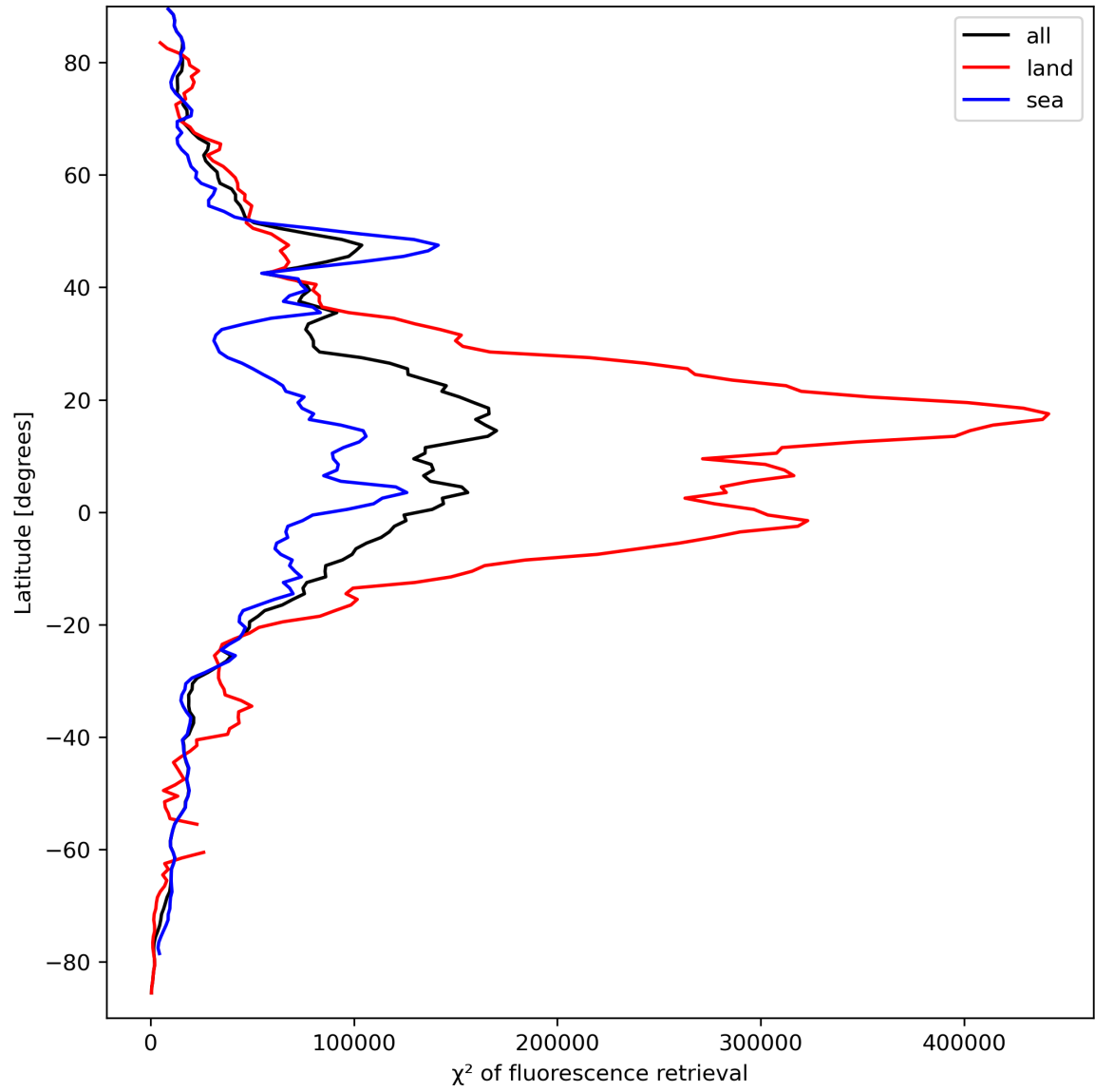
Figure 25: Zonal average of “ \chi^2 of fluorescence retrieval” for 2023-09-15 to 2023-09-16.
