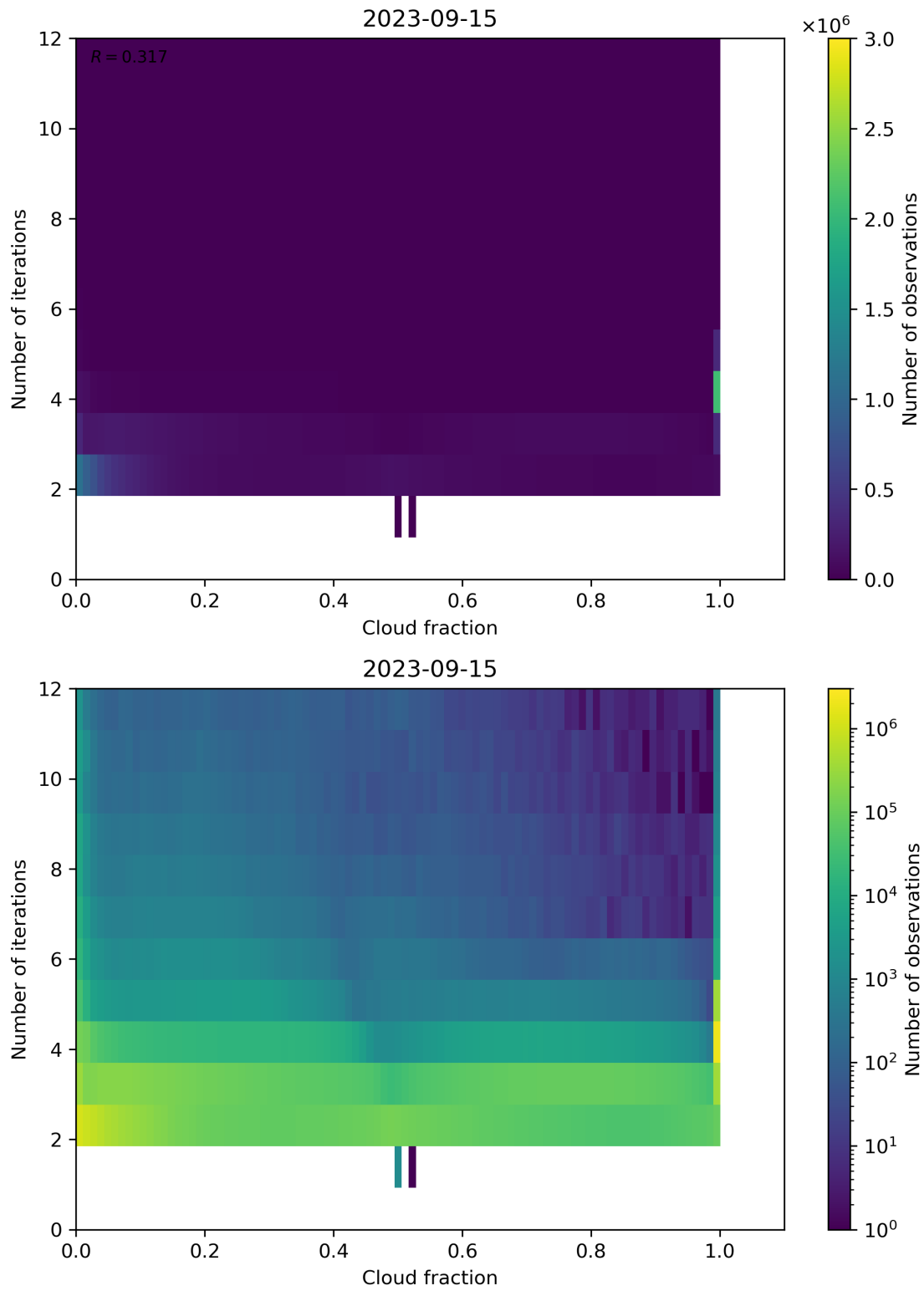
Figure 80: Scatter density plot of “Cloud fraction” against “Number of iterations” for 2023-09-15 to 2023-09-16.
