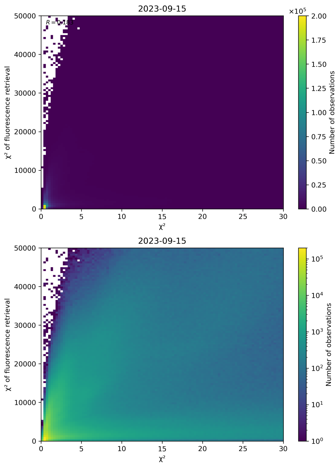
Figure 69: Scatter density plot of “ \chi^2 ” against “ \chi^2 of fluorescence retrieval” for 2023-09-15 to 2023-09-16.
