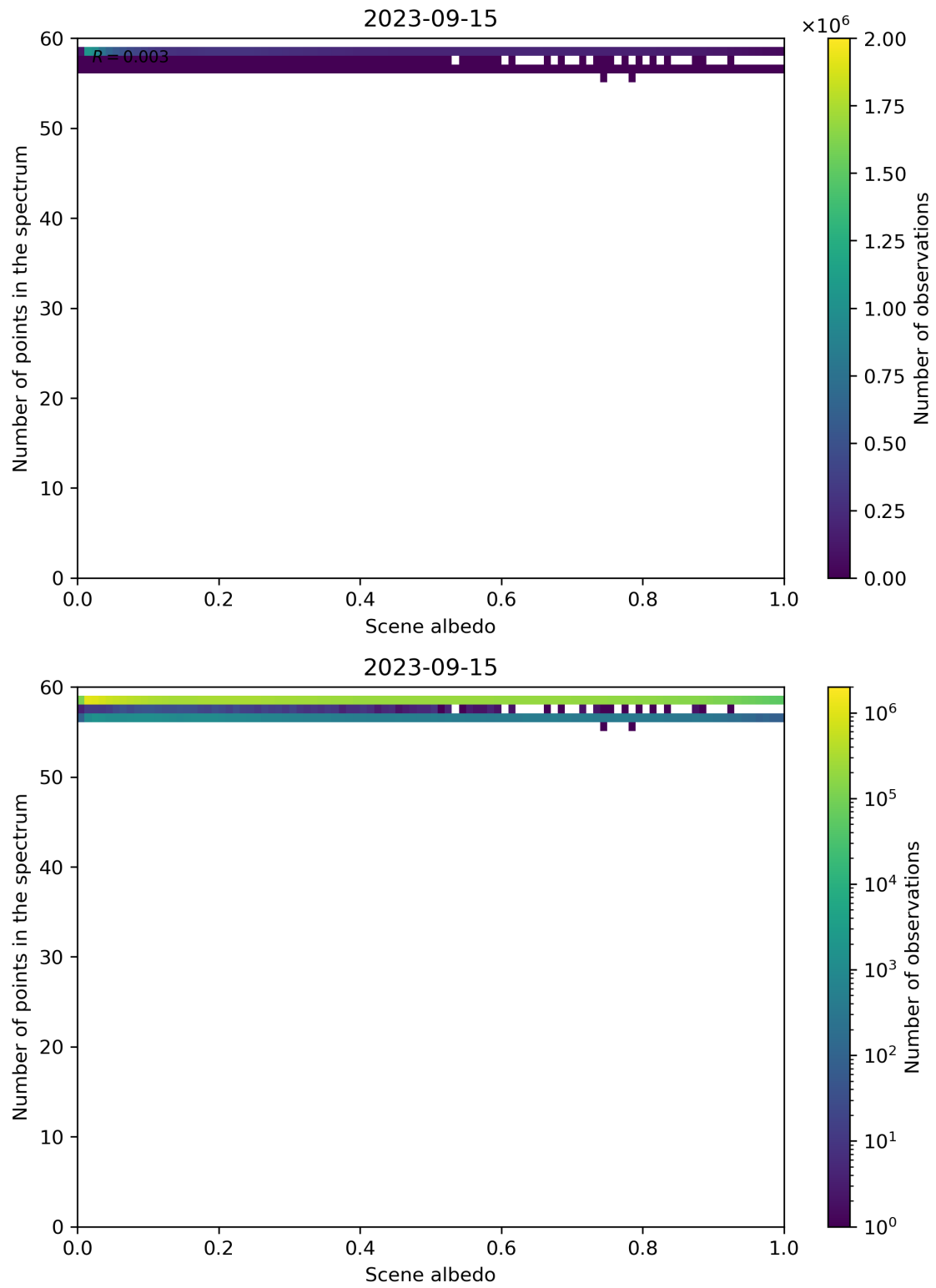
Figure 116: Scatter density plot of “Scene albedo” against “Number of points in the spectrum” for 2023-09-15 to 2023-09-16.
