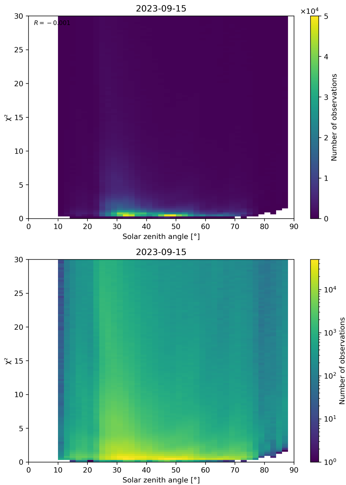
Figure 119: Scatter density plot of “Solar zenith angle” against “ \chi^2 ” for 2023-09-15 to 2023-09-16.
