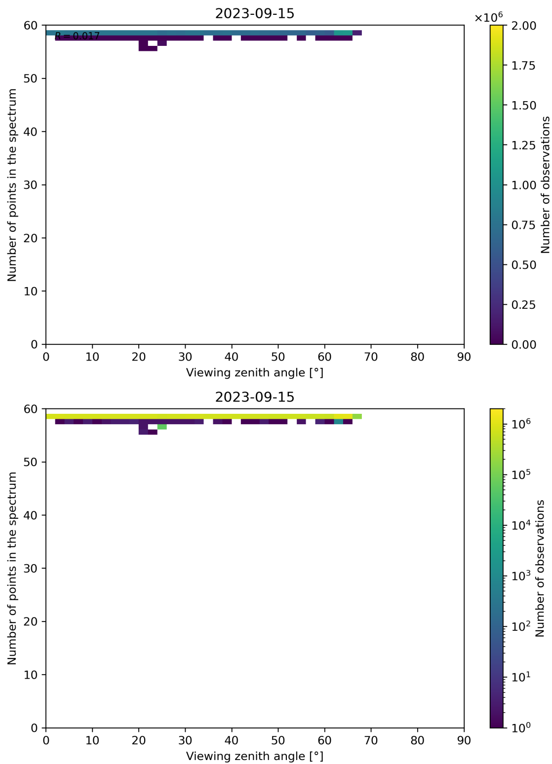
Figure 137: Scatter density plot of “Viewing zenith angle” against “Number of points in the spectrum” for 2023-09-15 to 2023-09-16.
