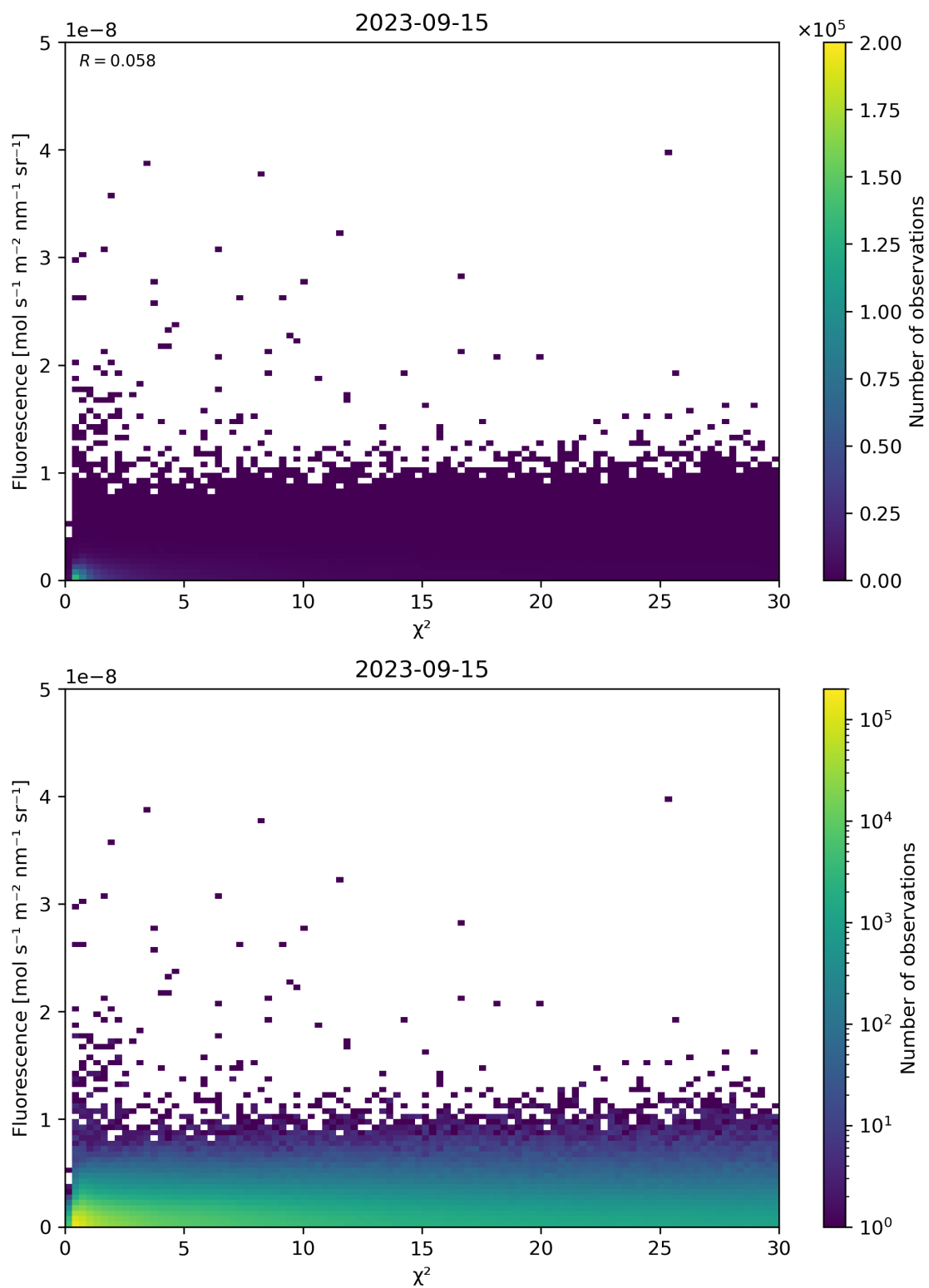
Figure 70: Scatter density plot of “ \chi^2 ” against “Fluorescence” for 2023-09-15 to 2023-09-16.
