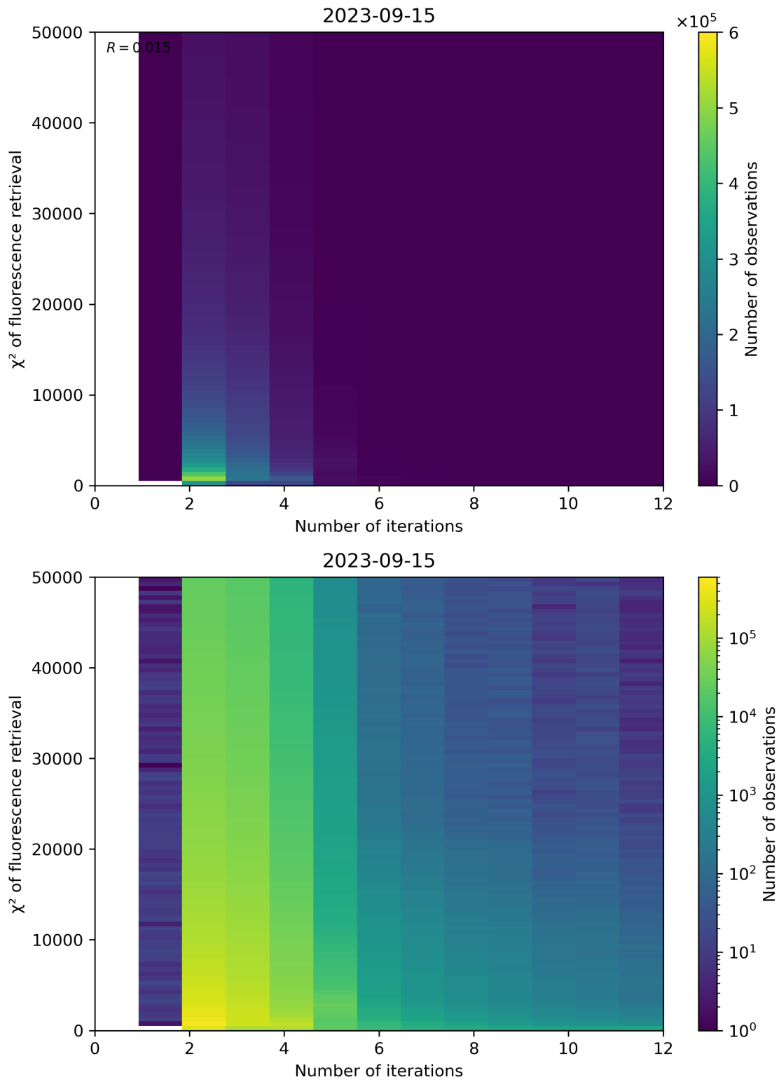
Figure 106: Scatter density plot of “Number of iterations” against “ \chi^2 of fluorescence retrieval” for 2023-09-15 to 2023-09-16.
