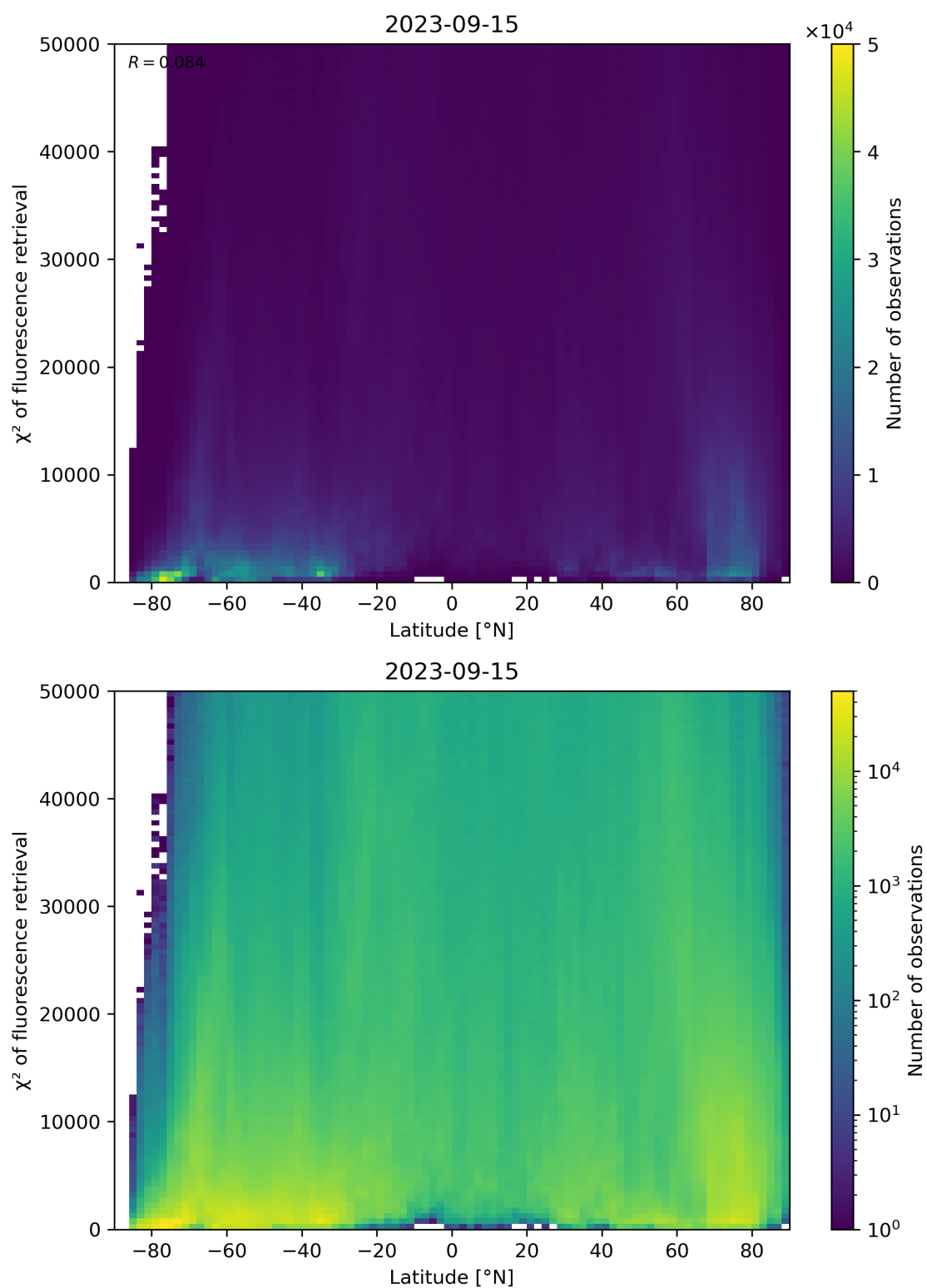
Figure 98: Scatter density plot of “Latitude” against “ \chi^2 of fluorescence retrieval” for 2023-09-15 to 2023-09-16.
