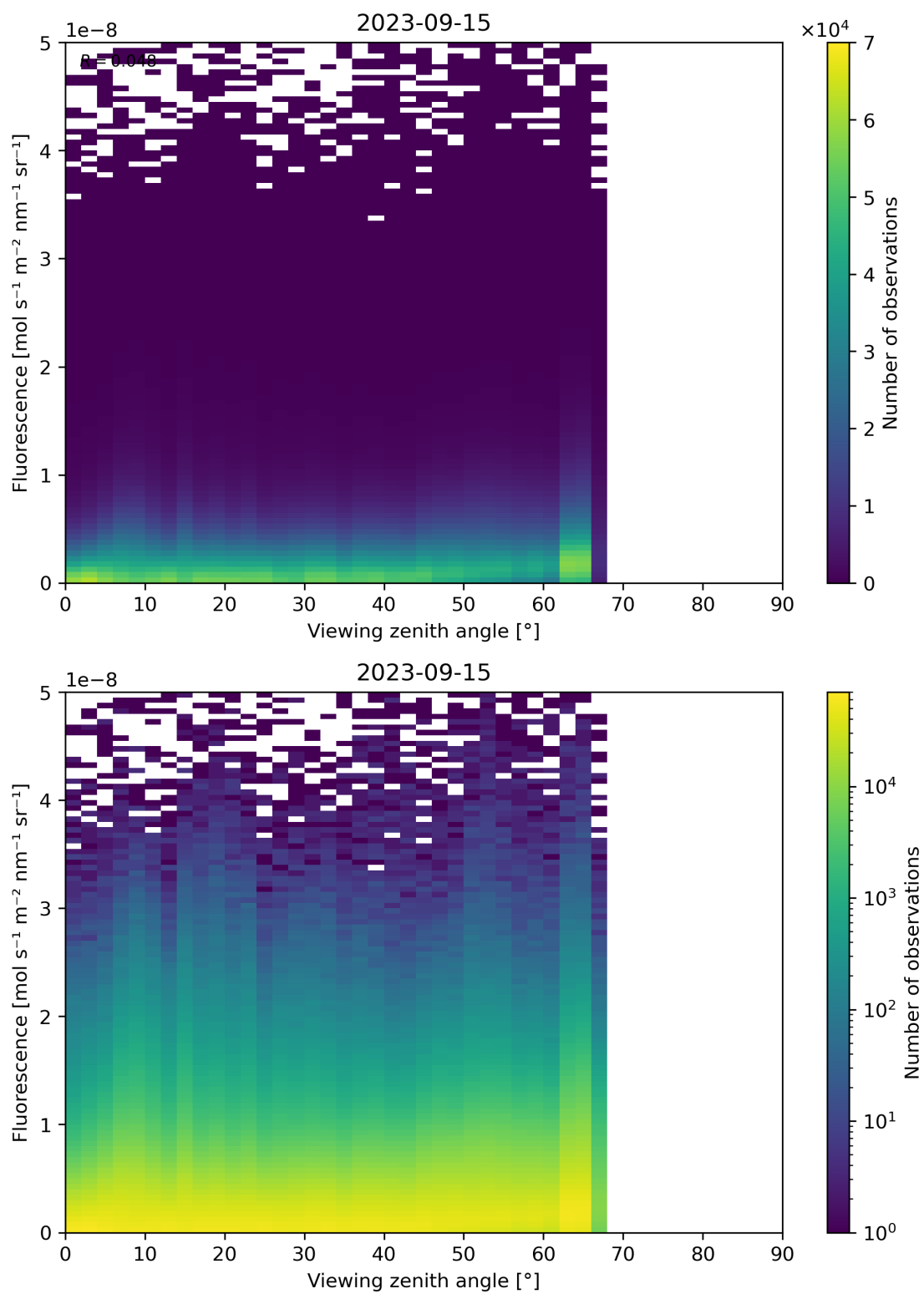
Figure 134: Scatter density plot of “Viewing zenith angle” against “Fluorescence” for 2023-09-15 to 2023-09-16.
