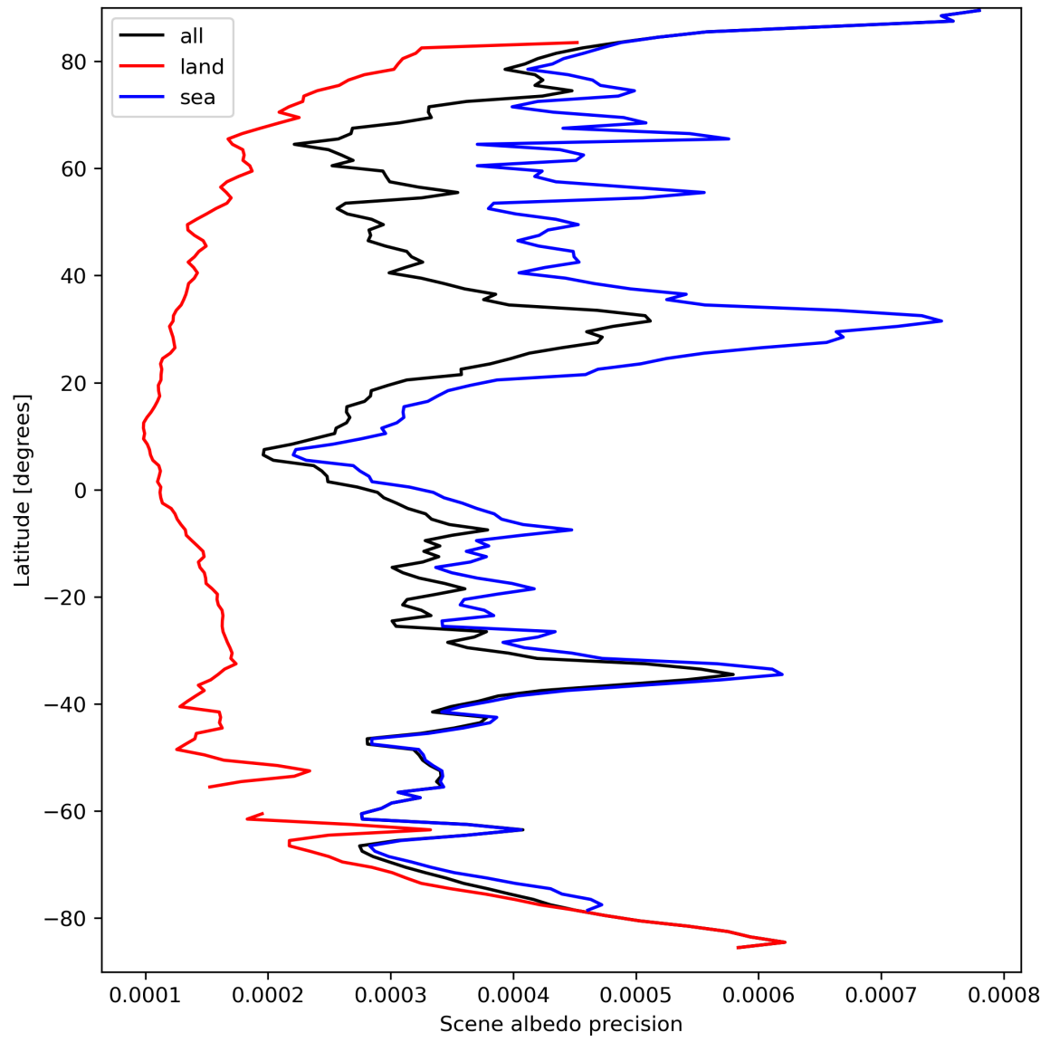
Figure 18: Zonal average of “Scene albedo precision” for 2023-09-15 to 2023-09-16.
