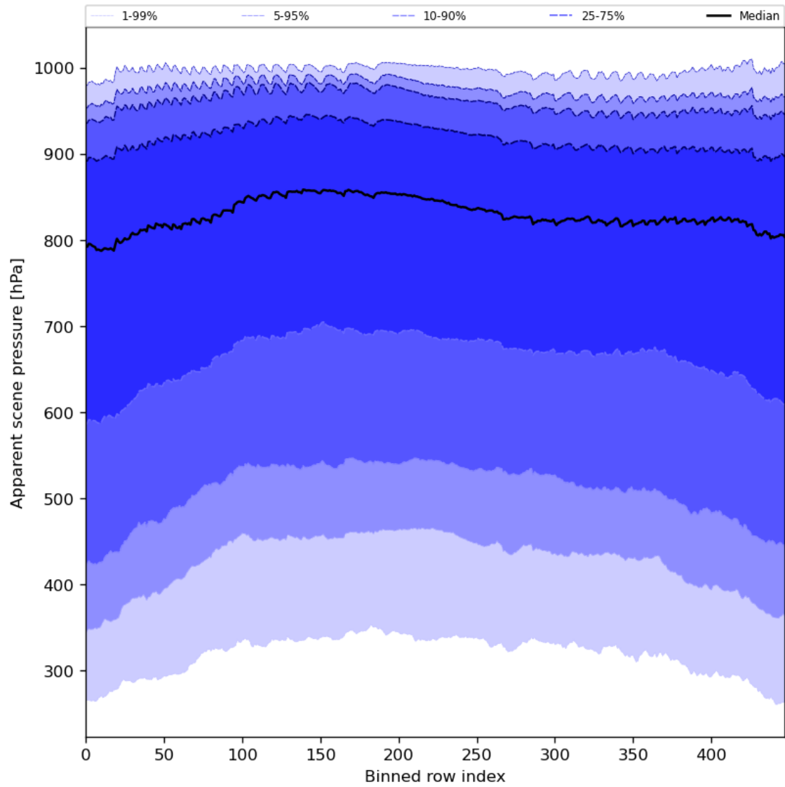
Figure 53: Along track statistics of “Apparent scene pressure” for 2023-09-15 to 2023-09-16
