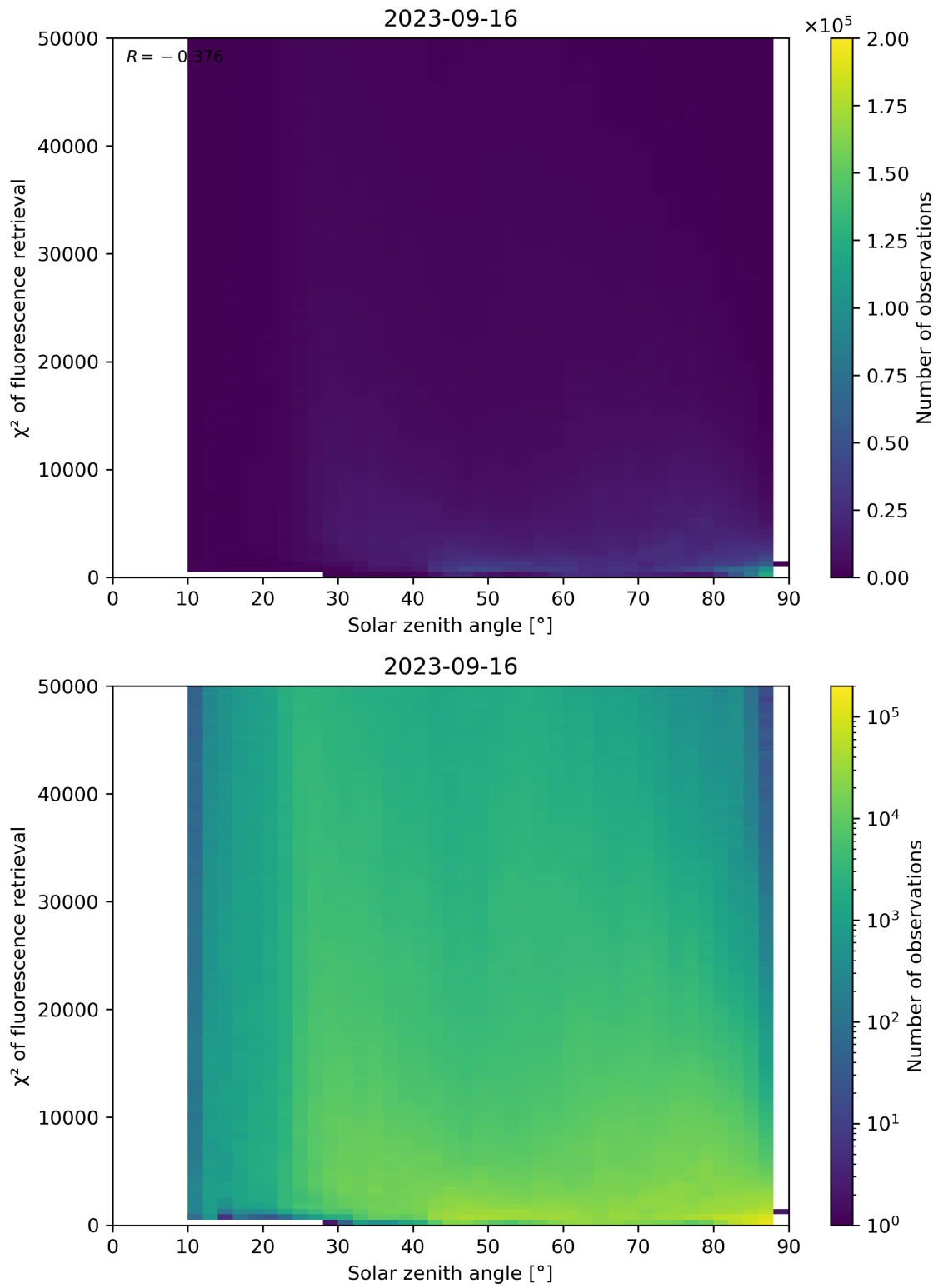
Figure 120: Scatter density plot of “Solar zenith angle” against “ \chi^2 of fluorescence retrieval” for 2023-09-15 to 2023-09-17.
