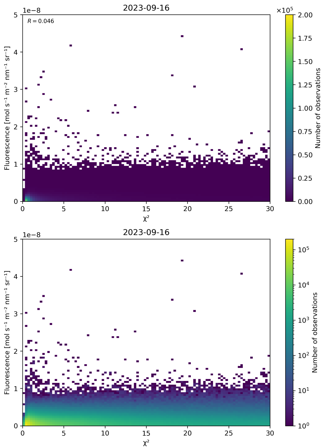
Figure 70: Scatter density plot of “ \chi^2 ” against “Fluorescence” for 2023-09-15 to 2023-09-17.
