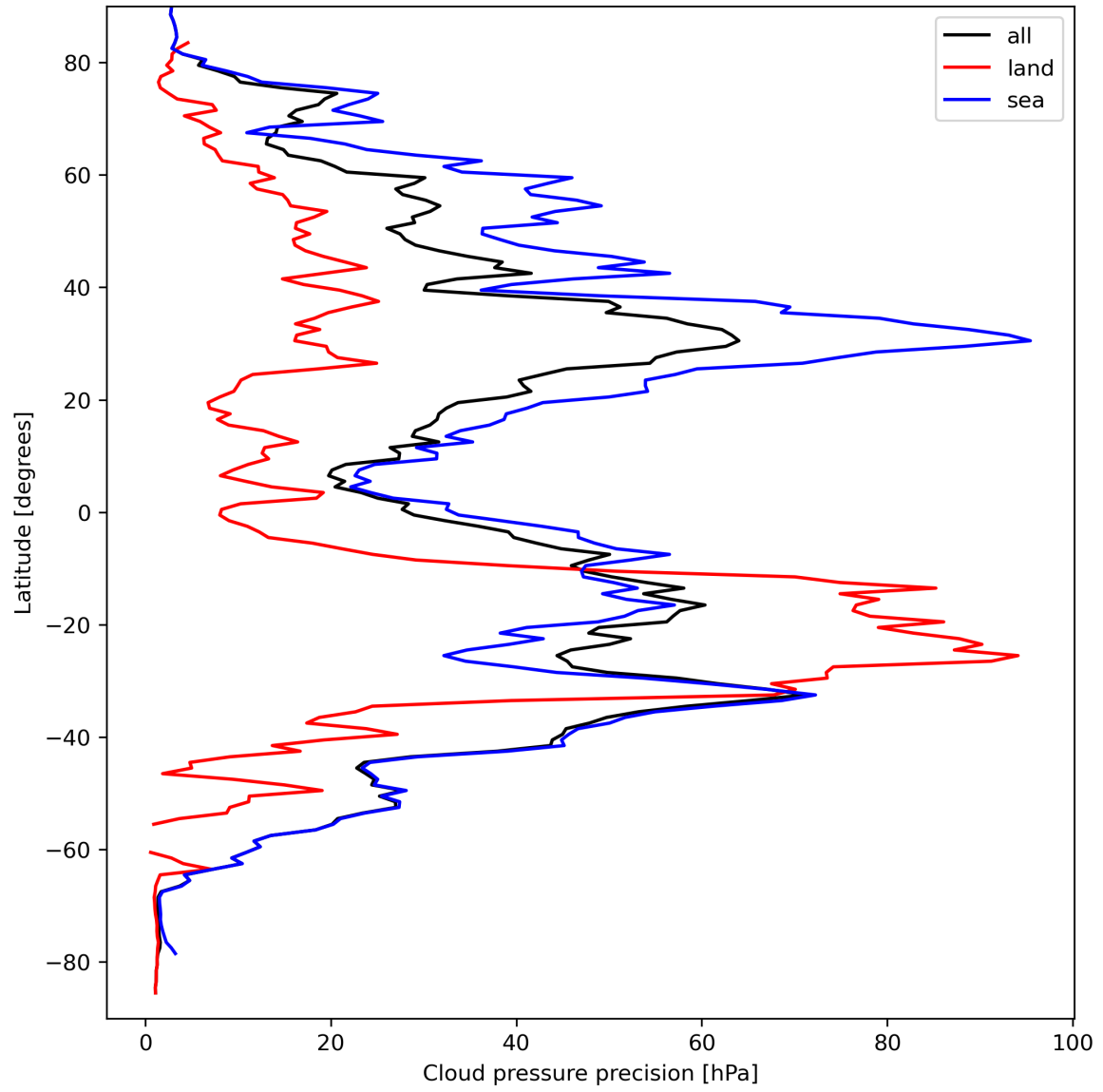
Figure 14: Zonal average of “Cloud pressure precision” for 2023-09-15 to 2023-09-17.
