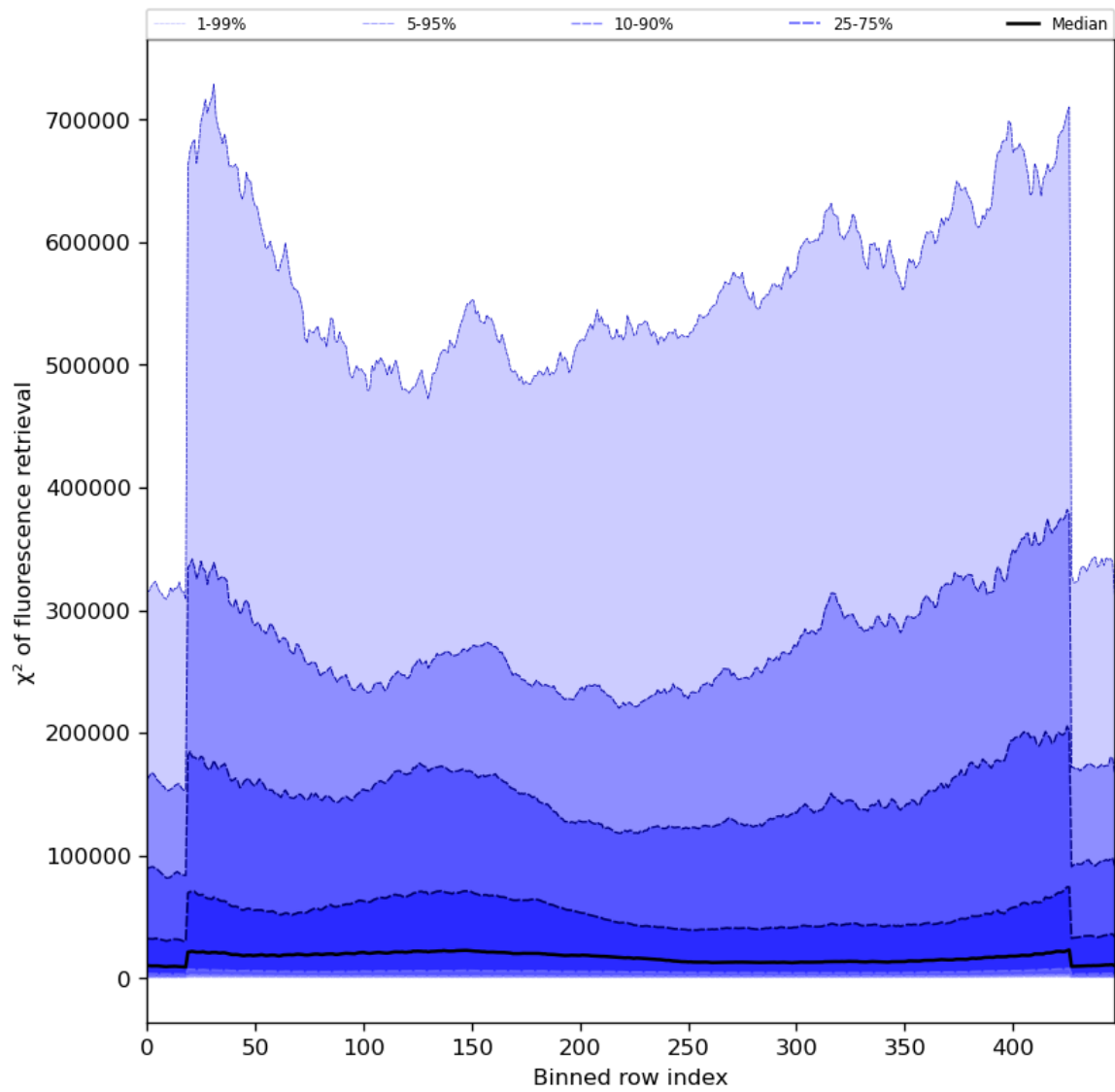
Figure 59: Along track statistics of “ \chi^2 of fluorescence retrieval” for 2023-09-15 to 2023-09-17
