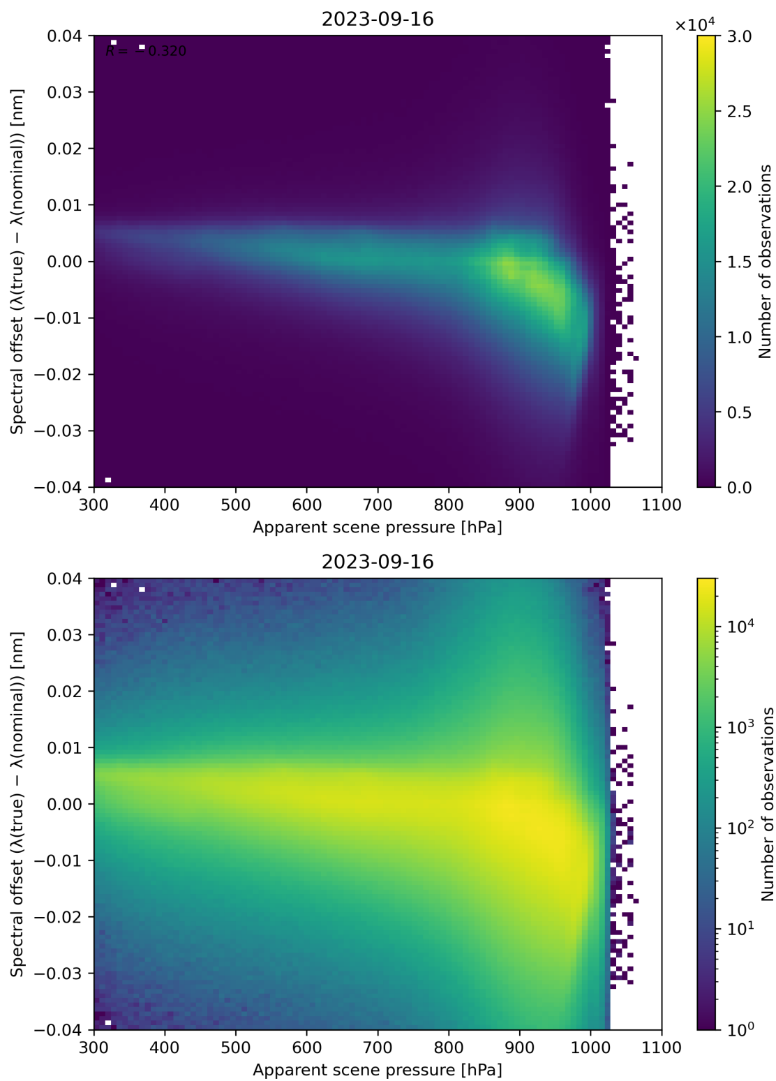
Figure 68: Scatter density plot of “Apparent scene pressure” against “Spectral offset ( \lambda(\text{true}) - \lambda(\text{nominal}) )” for 2023-09-15 to 2023-09-17.
