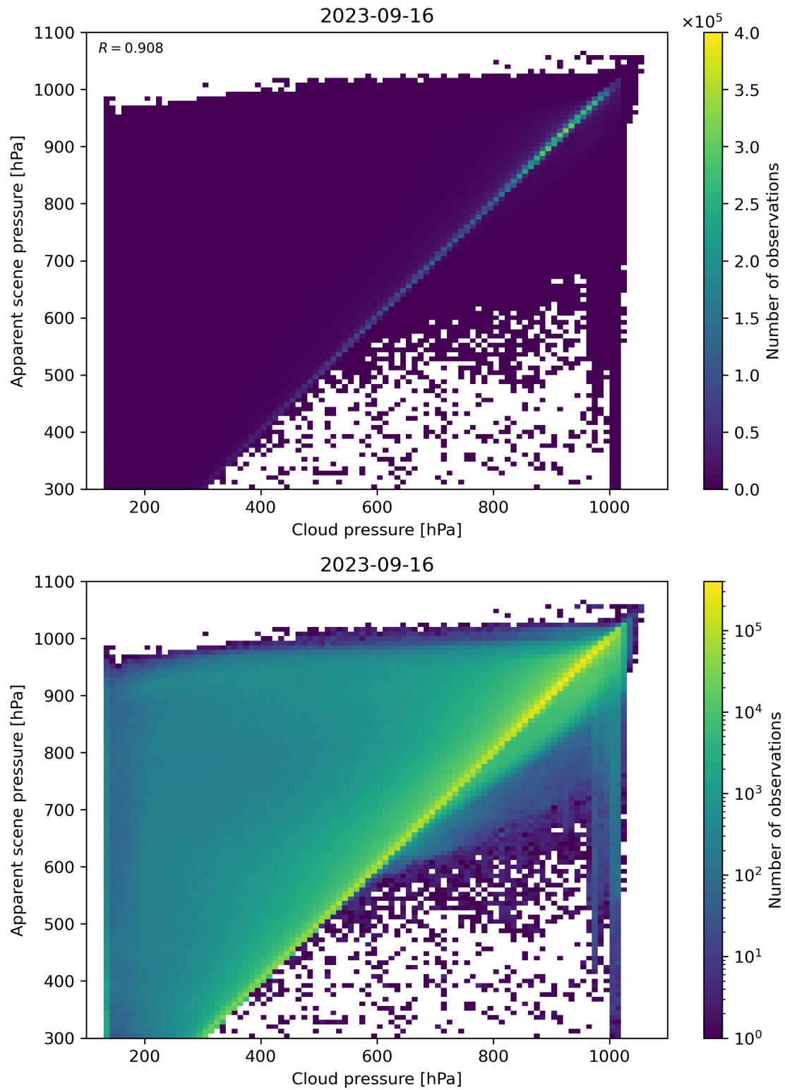
Figure 84: Scatter density plot of “Cloud pressure” against “Apparent scene pressure” for 2023-09-15 to 2023-09-17.
