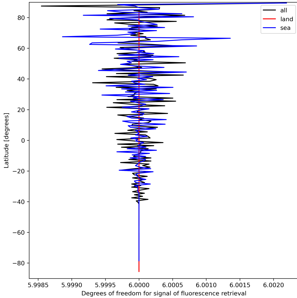
Figure 26: Zonal average of “Degrees of freedom for signal of fluorescence retrieval” for 2023-09-15 to 2023-09-17.
