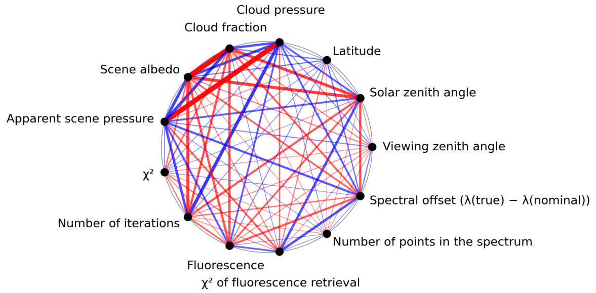
Figure 1: Map of correlation graph for 2023-09-15 to 2023-09-17.
