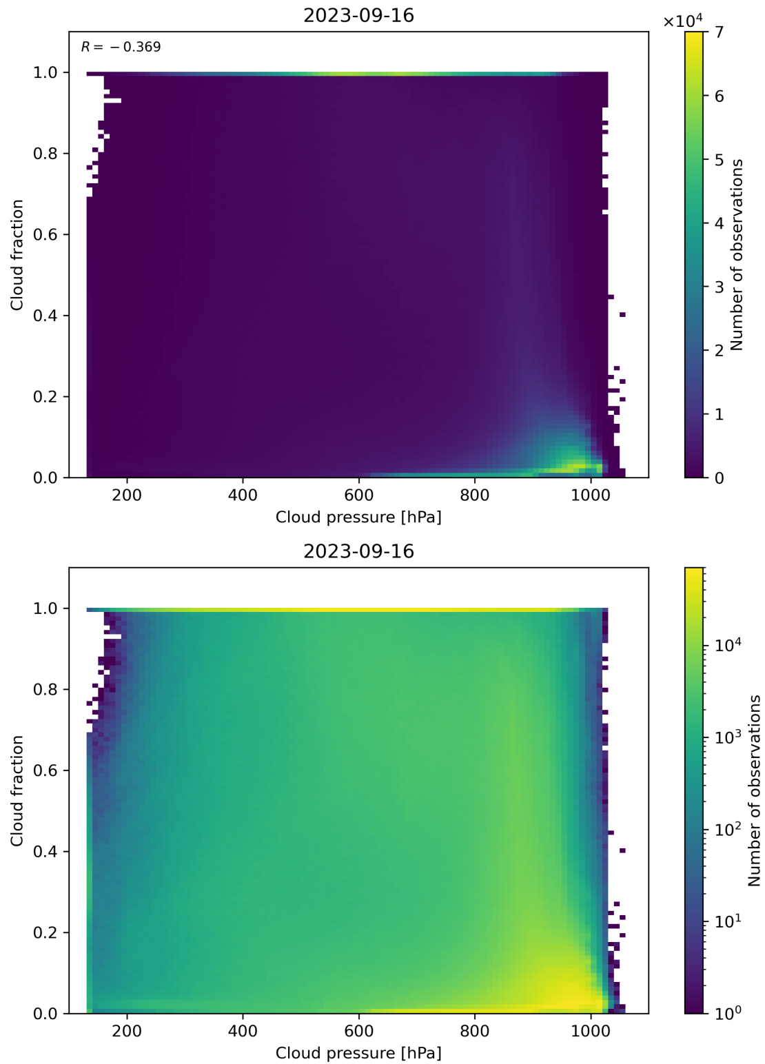
Figure 87: Scatter density plot of “Cloud pressure” against “Cloud fraction” for 2023-09-15 to 2023-09-17.
