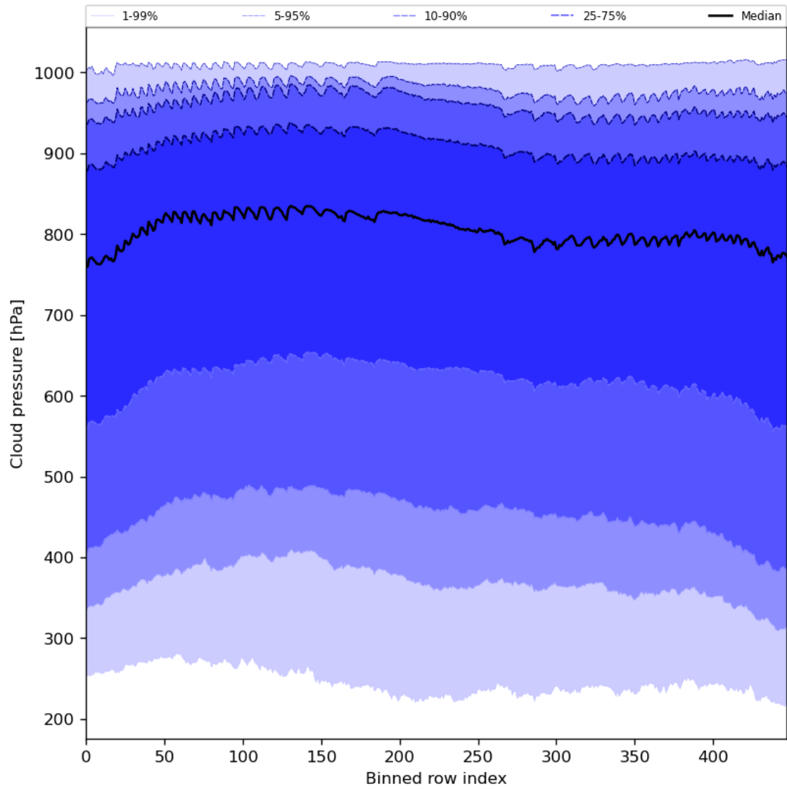
Figure 47: Along track statistics of “Cloud pressure” for 2023-09-15 to 2023-09-17
