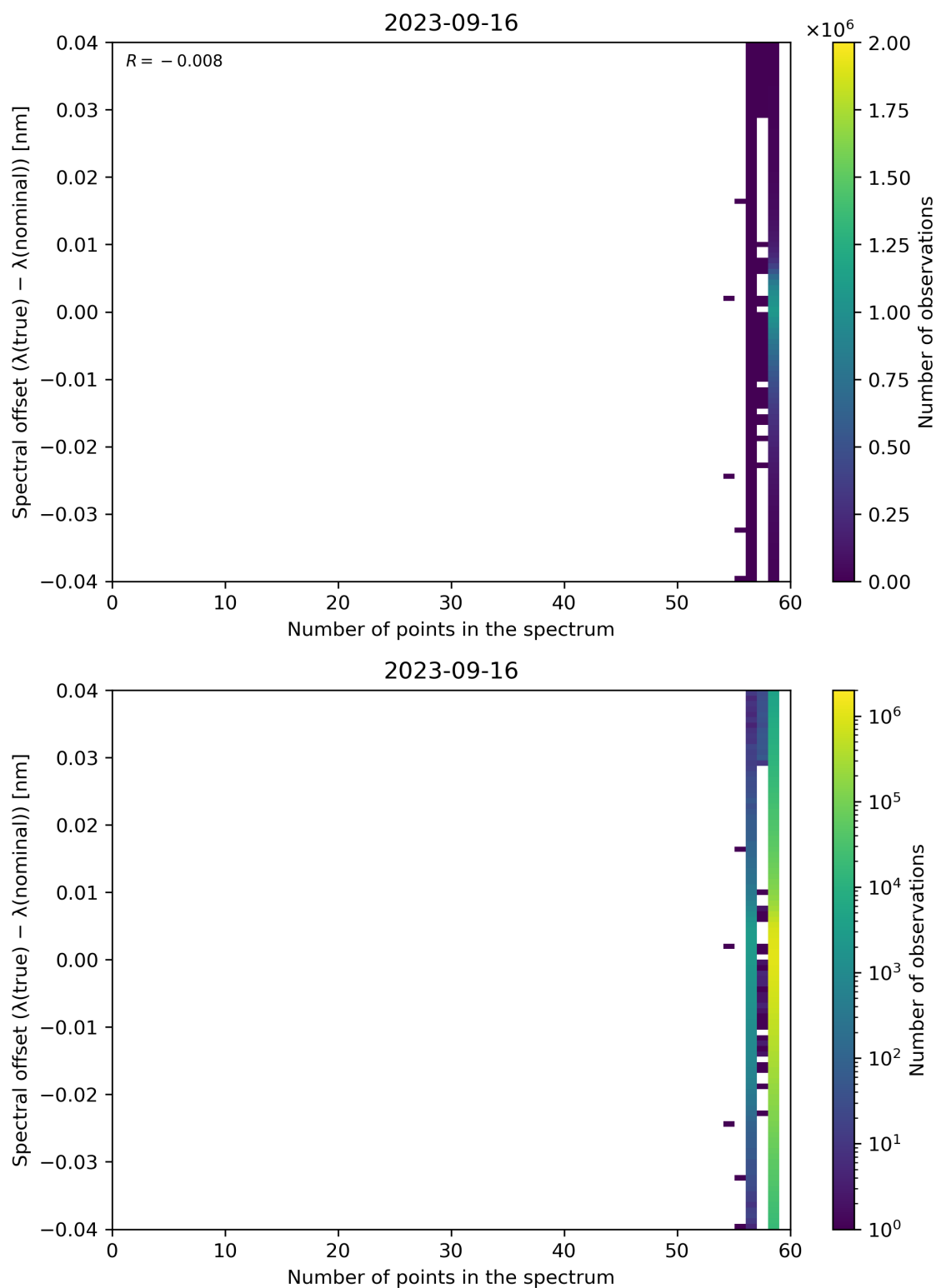
Figure 110: Scatter density plot of “Number of points in the spectrum” against “Spectral offset ( \lambda(\text{true}) - \lambda(\text{nominal}) )” for 2023-09-15 to 2023-09-17.
