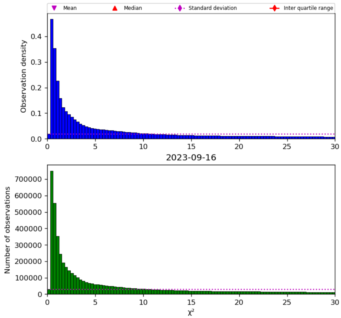
Figure 38: Histogram of " \chi^2 " for 2023-09-15 to 2023-09-17
