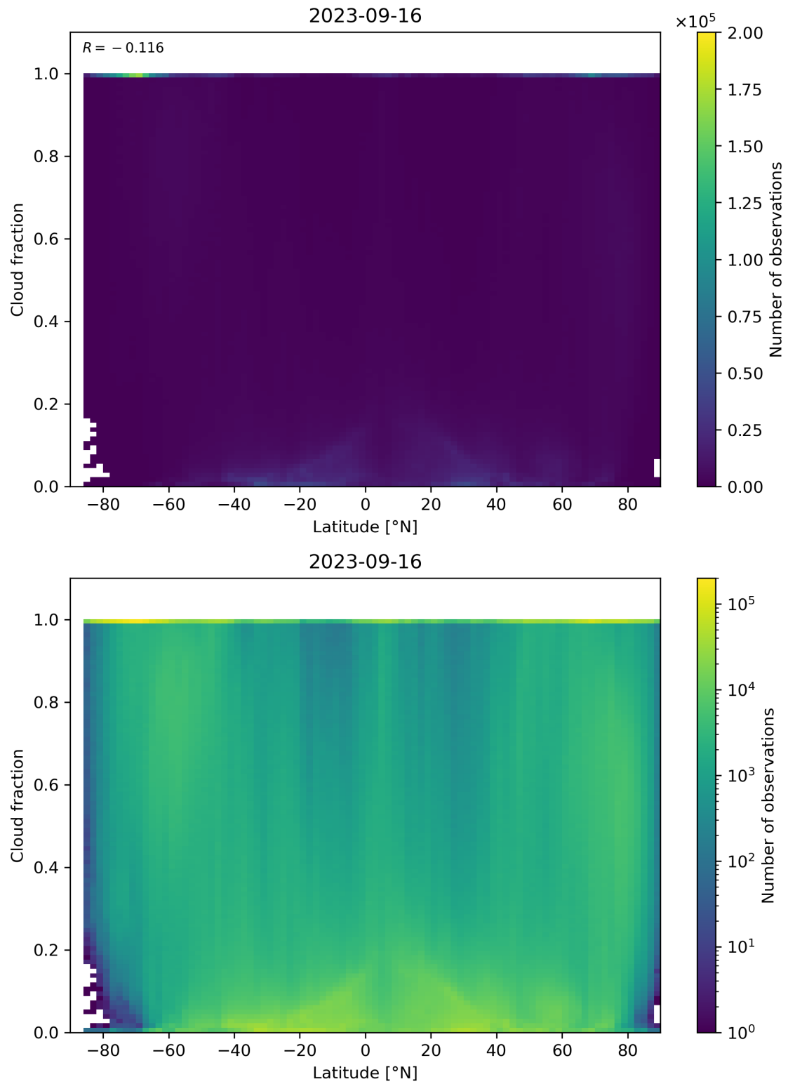
Figure 99: Scatter density plot of “Latitude” against “Cloud fraction” for 2023-09-15 to 2023-09-17.
