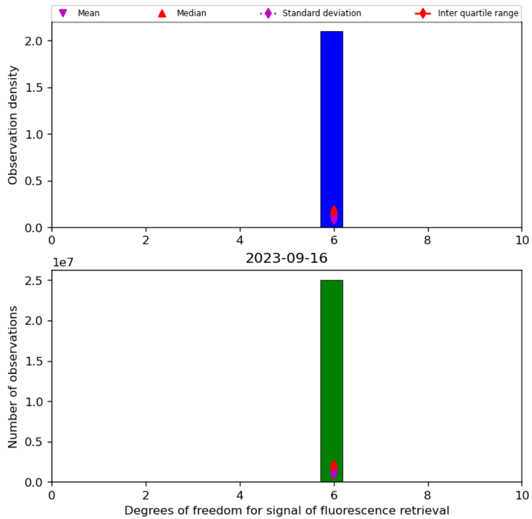
Figure 43: Histogram of “Degrees of freedom for signal of fluorescence retrieval” for 2023-09-15 to 2023-09-17
