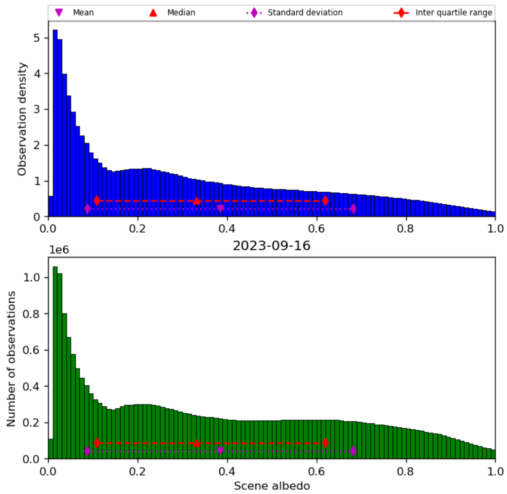
Figure 34: Histogram of “Scene albedo” for 2023-09-15 to 2023-09-17
