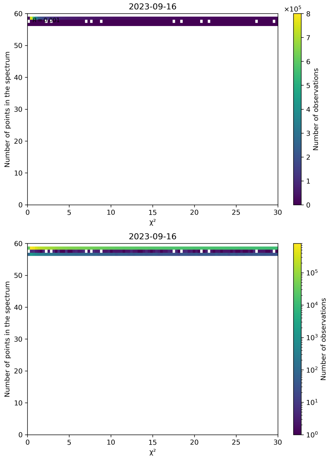
Figure 74: Scatter density plot of “ \chi^2 ” against “Number of points in the spectrum” for 2023-09-15 to 2023-09-17.
