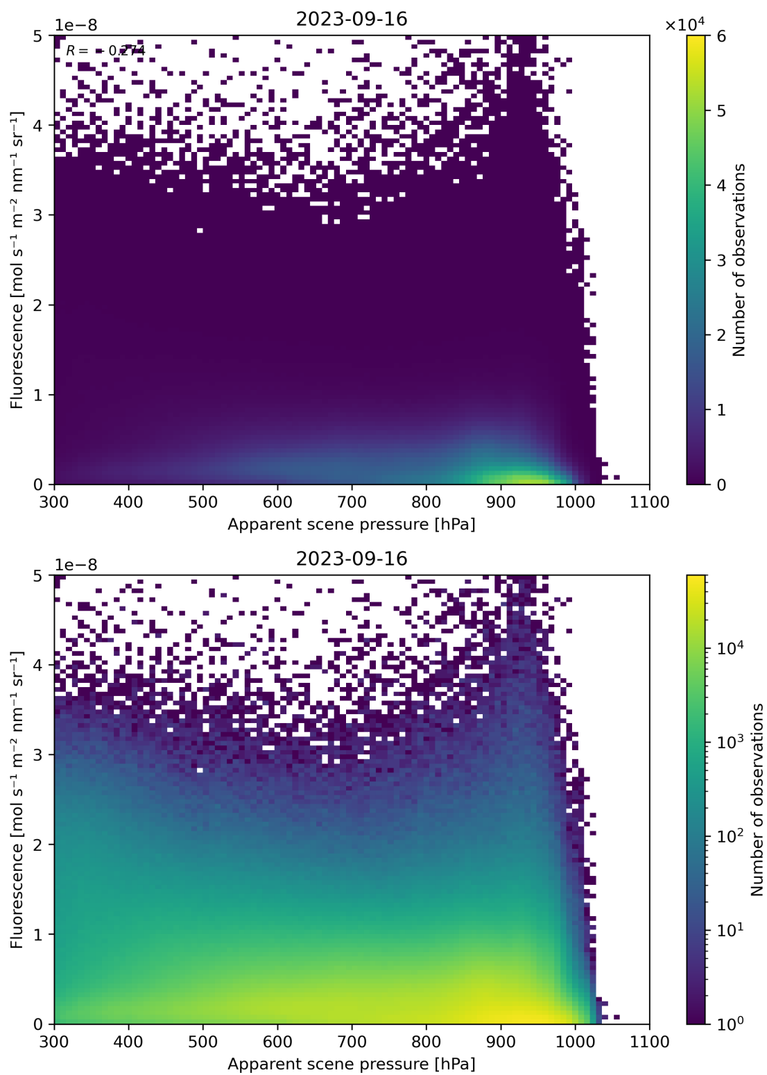
Figure 65: Scatter density plot of “Apparent scene pressure” against “Fluorescence” for 2023-09-15 to 2023-09-17.
