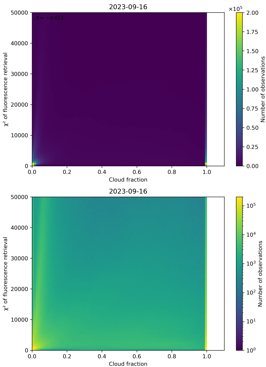
Figure 78: Scatter density plot of “Cloud fraction” against “ \chi^2 of fluorescence retrieval” for 2023-09-15 to 2023-09-17.
