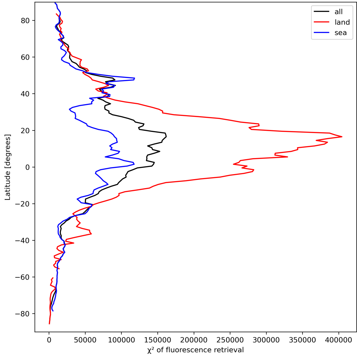
Figure 25: Zonal average of “ \chi^2 of fluorescence retrieval” for 2023-09-15 to 2023-09-17.
