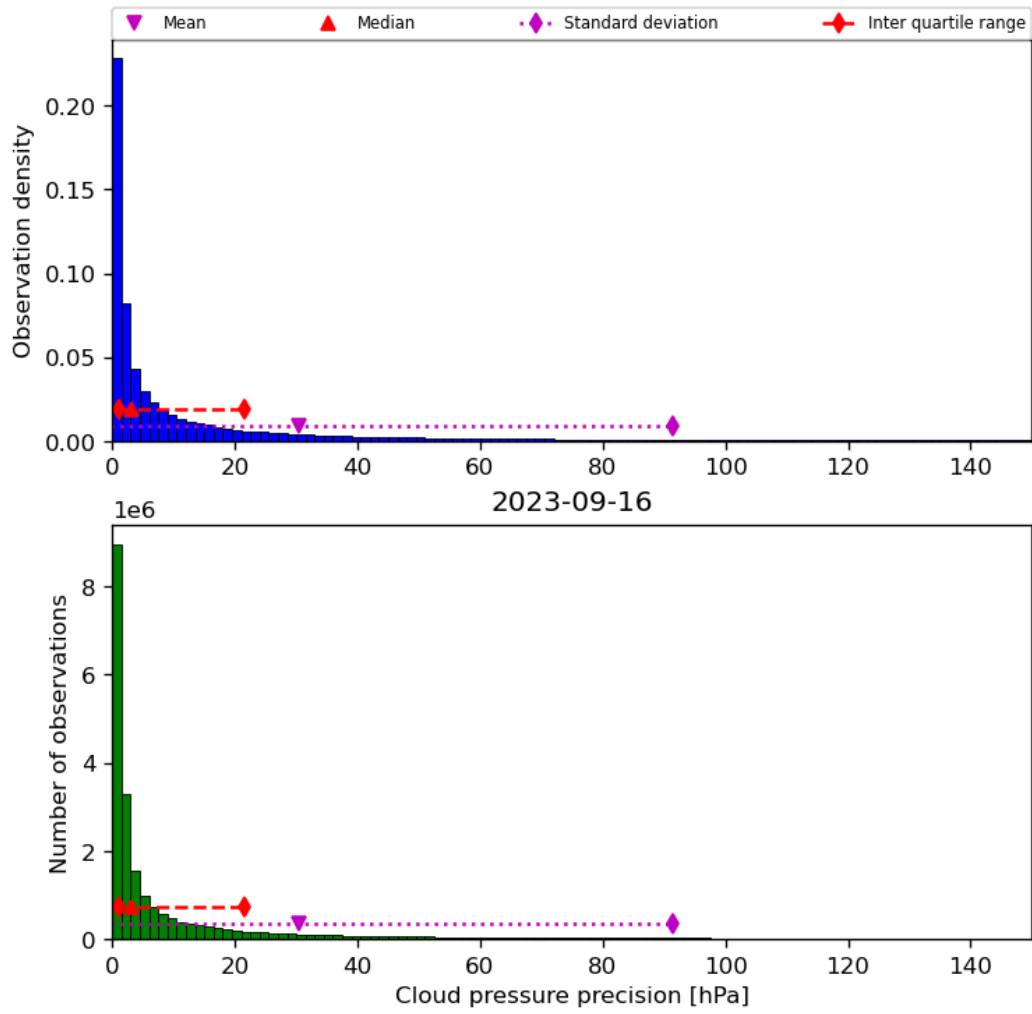
Figure 31: Histogram of “Cloud pressure precision” for 2023-09-15 to 2023-09-17
