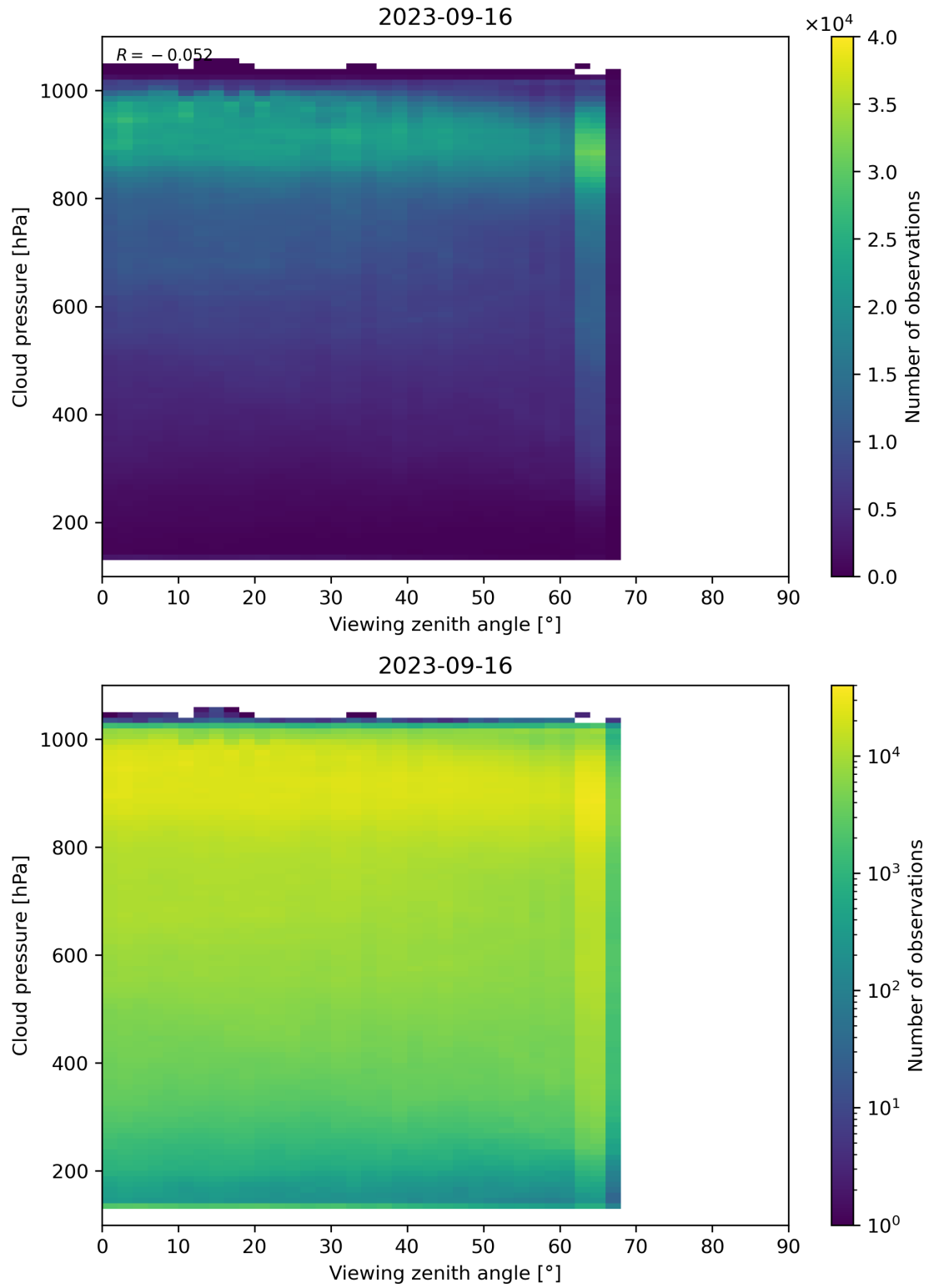
Figure 133: Scatter density plot of “Viewing zenith angle” against “Cloud pressure” for 2023-09-15 to 2023-09-17.
