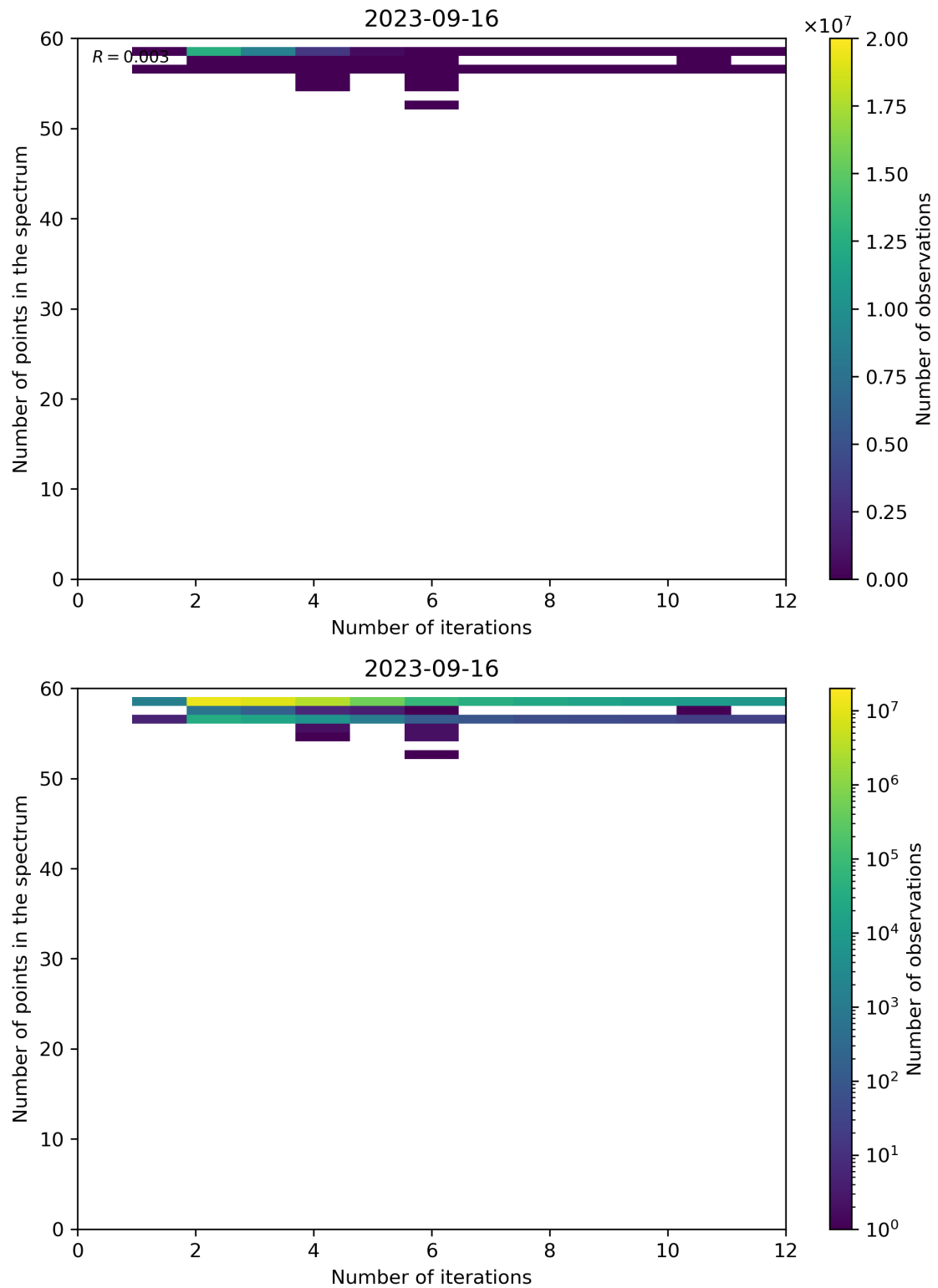
Figure 108: Scatter density plot of “Number of iterations” against “Number of points in the spectrum” for 2023-09-15 to 2023-09-17.
