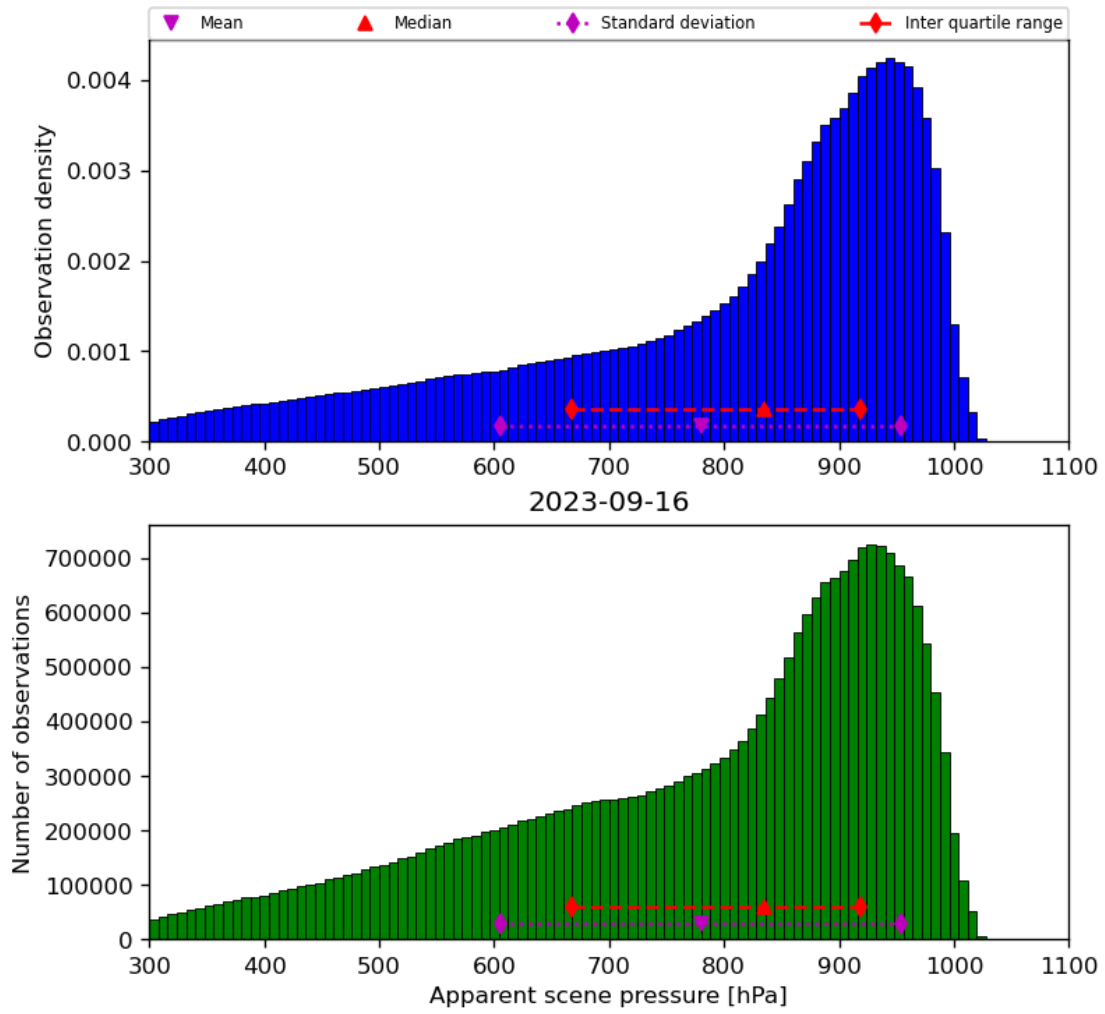
Figure 36: Histogram of “Apparent scene pressure” for 2023-09-15 to 2023-09-17
