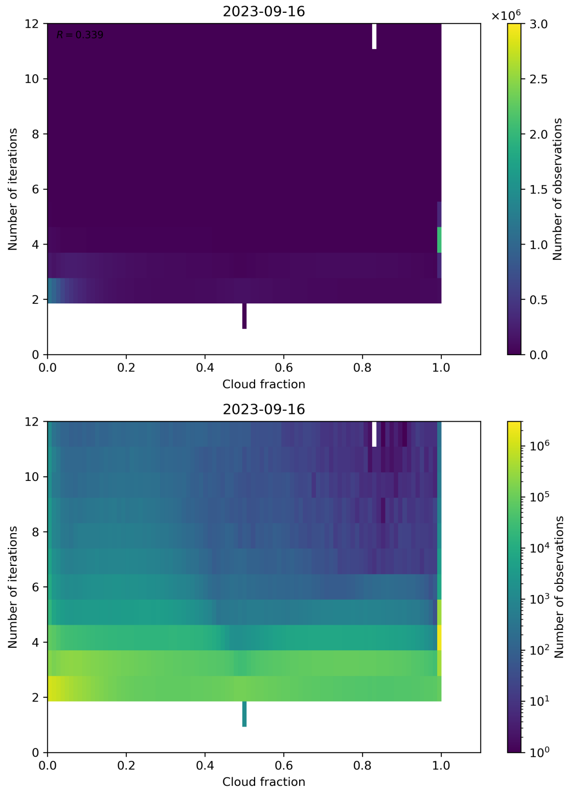
Figure 80: Scatter density plot of “Cloud fraction” against “Number of iterations” for 2023-09-15 to 2023-09-17.
