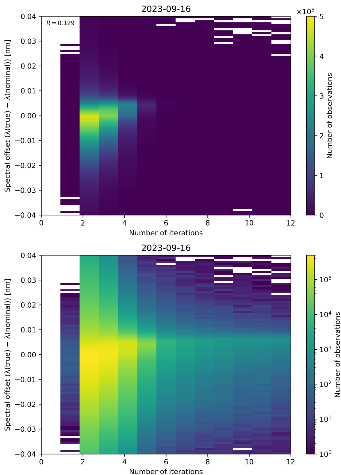
Figure 109: Scatter density plot of “Number of iterations” against “Spectral offset ( \lambda(\text{true}) - \lambda(\text{nominal}) )” for 2023-09-15 to 2023-09-17.
