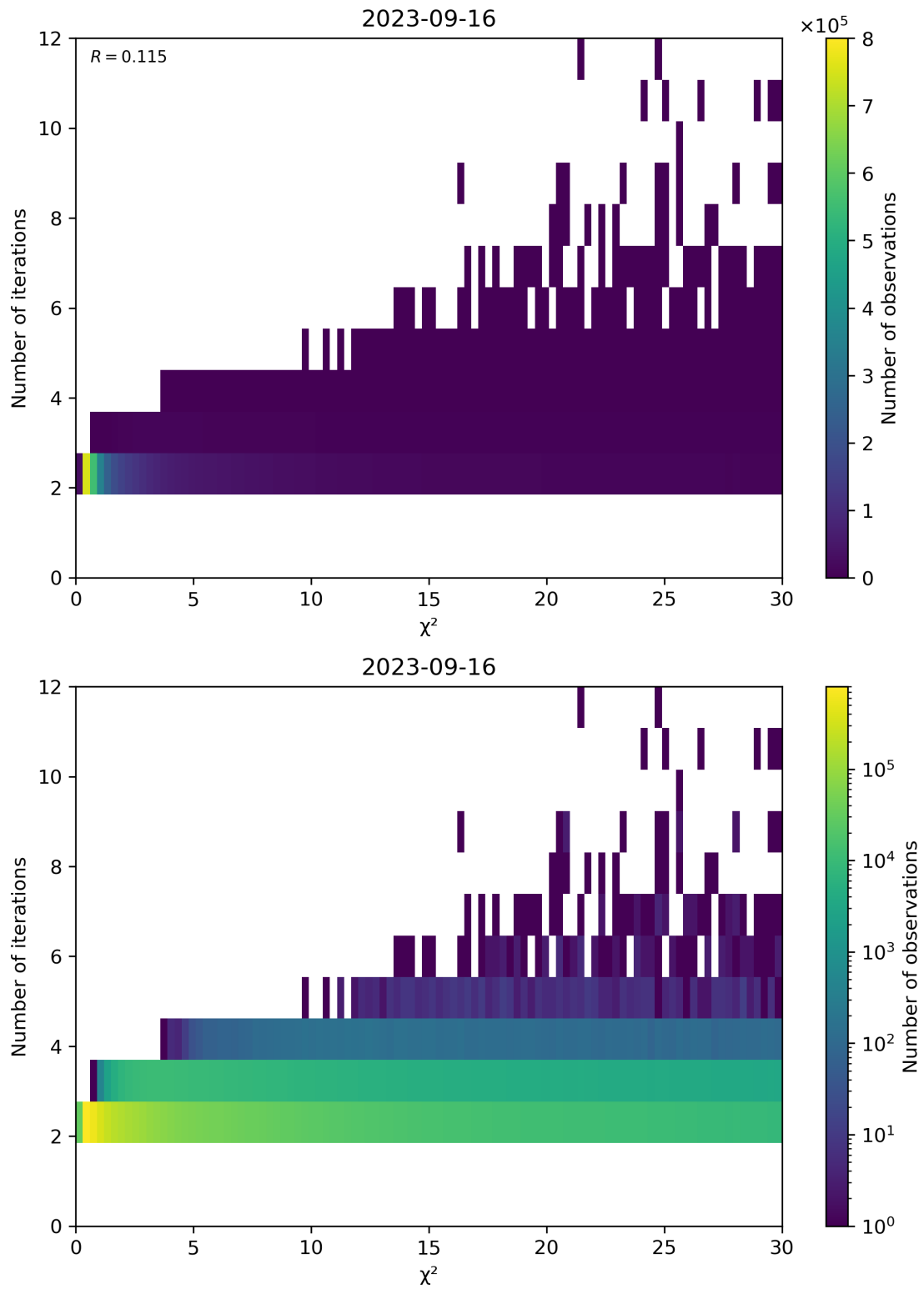
Figure 73: Scatter density plot of “ \chi^2 ” against “Number of iterations” for 2023-09-15 to 2023-09-17.
