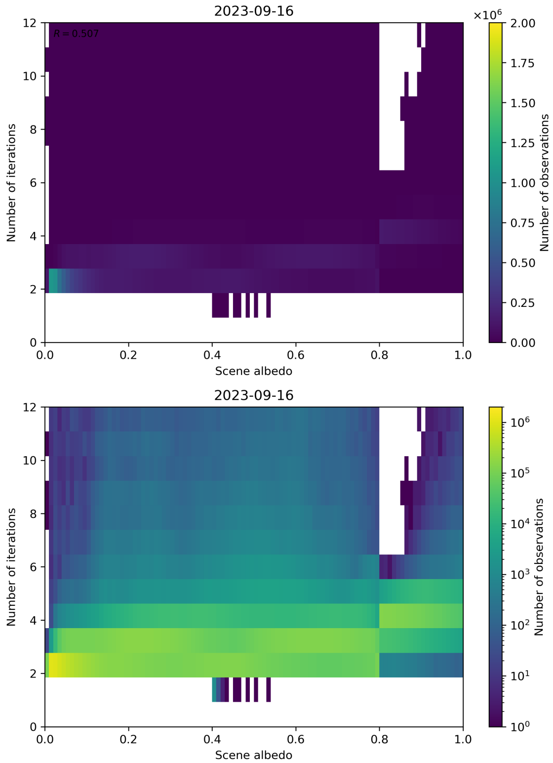
Figure 115: Scatter density plot of “Scene albedo” against “Number of iterations” for 2023-09-15 to 2023-09-17.
