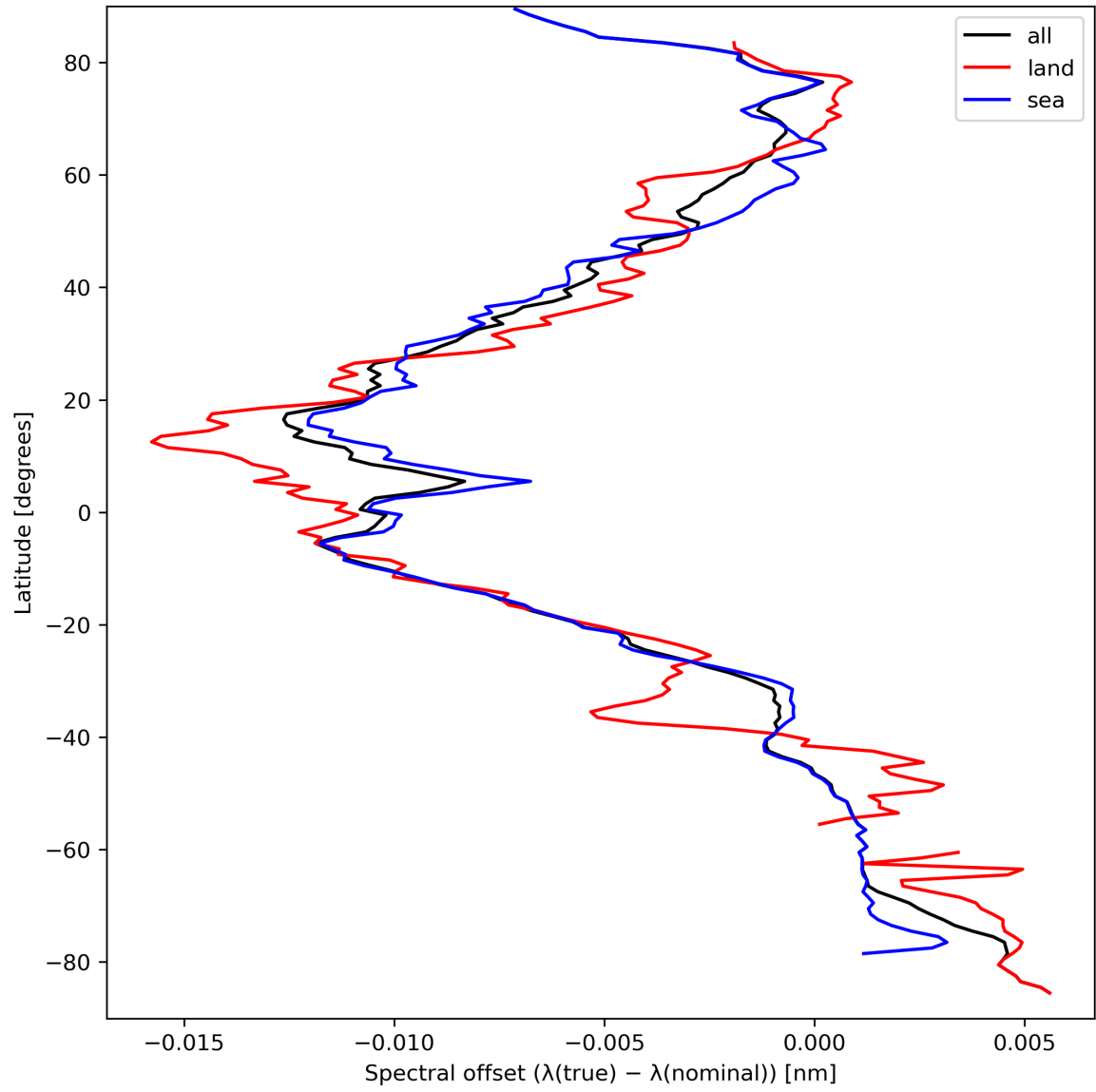
Figure 28: Zonal average of “Spectral offset ( \lambda(\text{true}) - \lambda(\text{nominal}) )” for 2023-09-15 to 2023-09-17.
