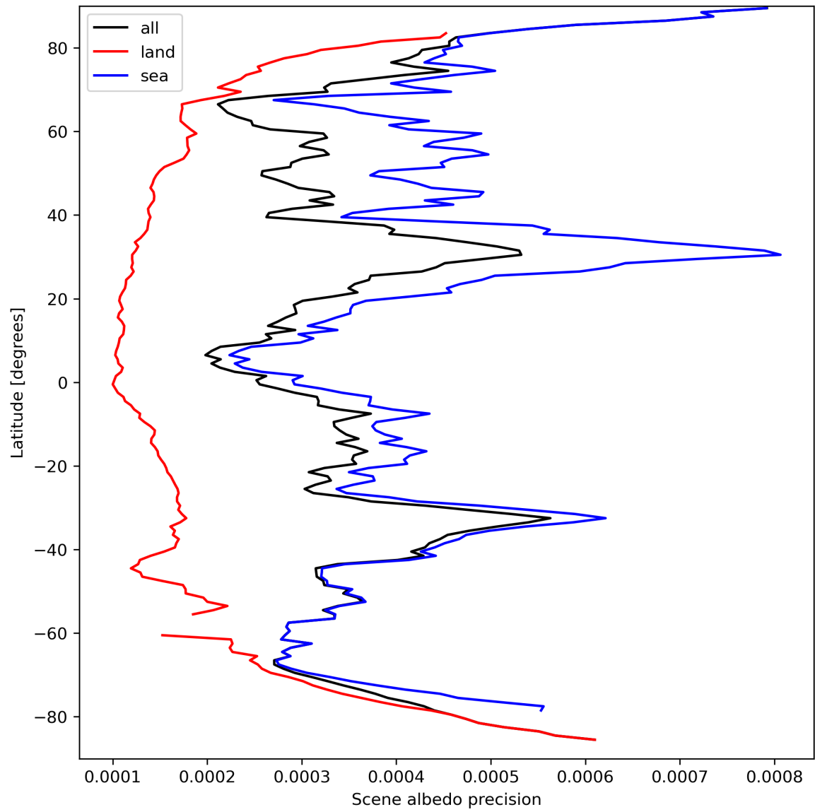
Figure 18: Zonal average of “Scene albedo precision” for 2023-09-15 to 2023-09-17.
