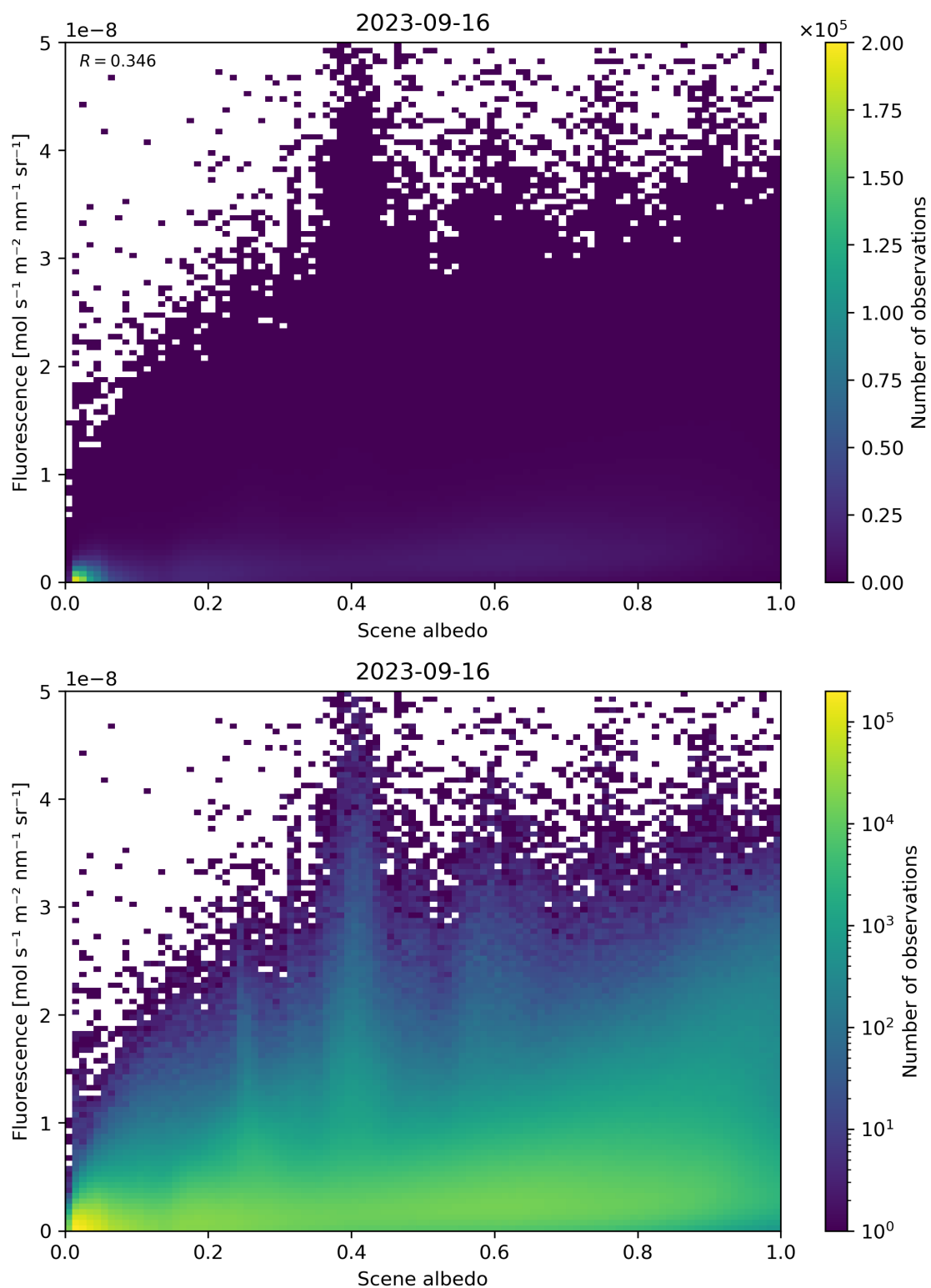
Figure 114: Scatter density plot of “Scene albedo” against “Fluorescence” for 2023-09-15 to 2023-09-17.
