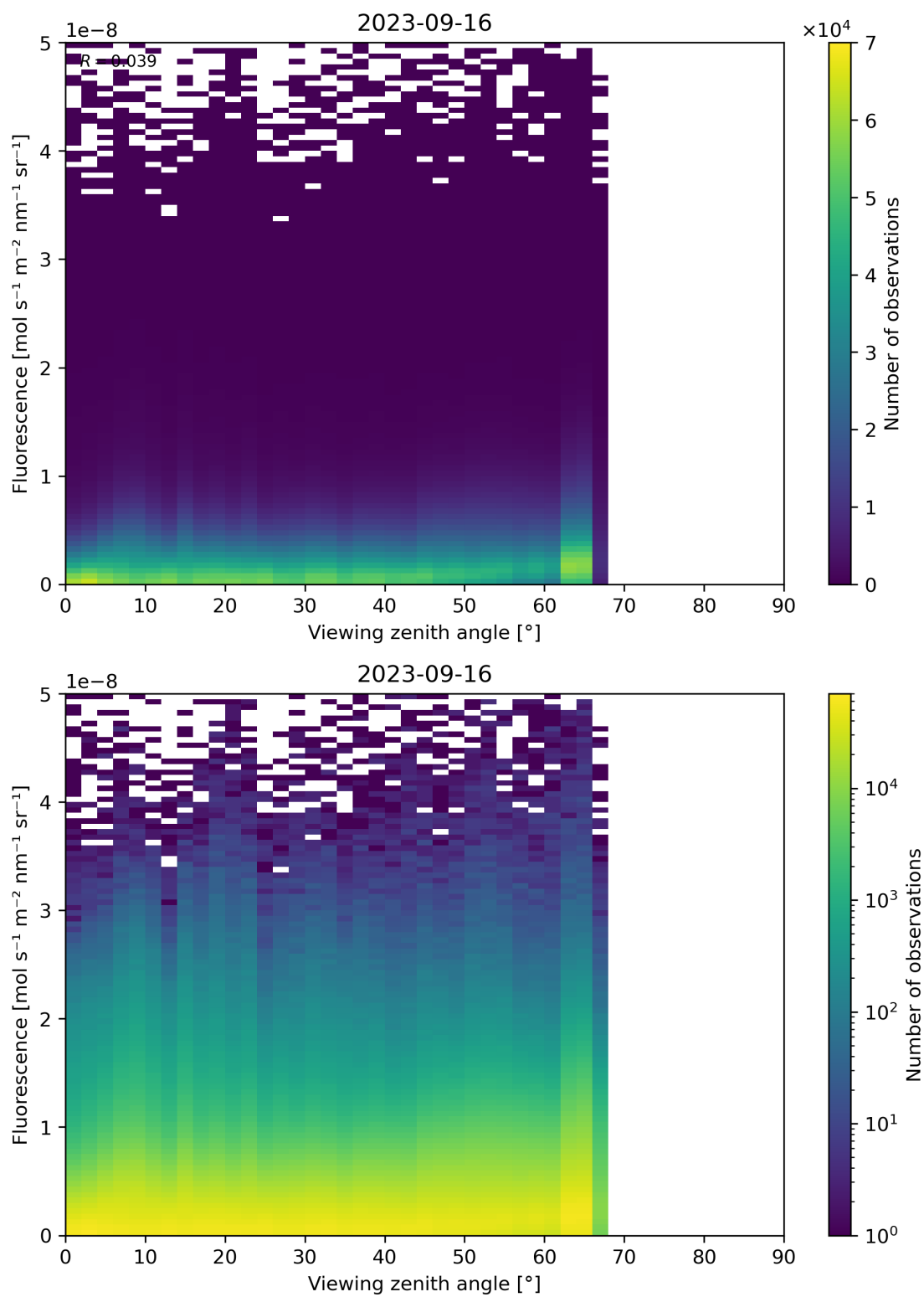
Figure 134: Scatter density plot of “Viewing zenith angle” against “Fluorescence” for 2023-09-15 to 2023-09-17.
