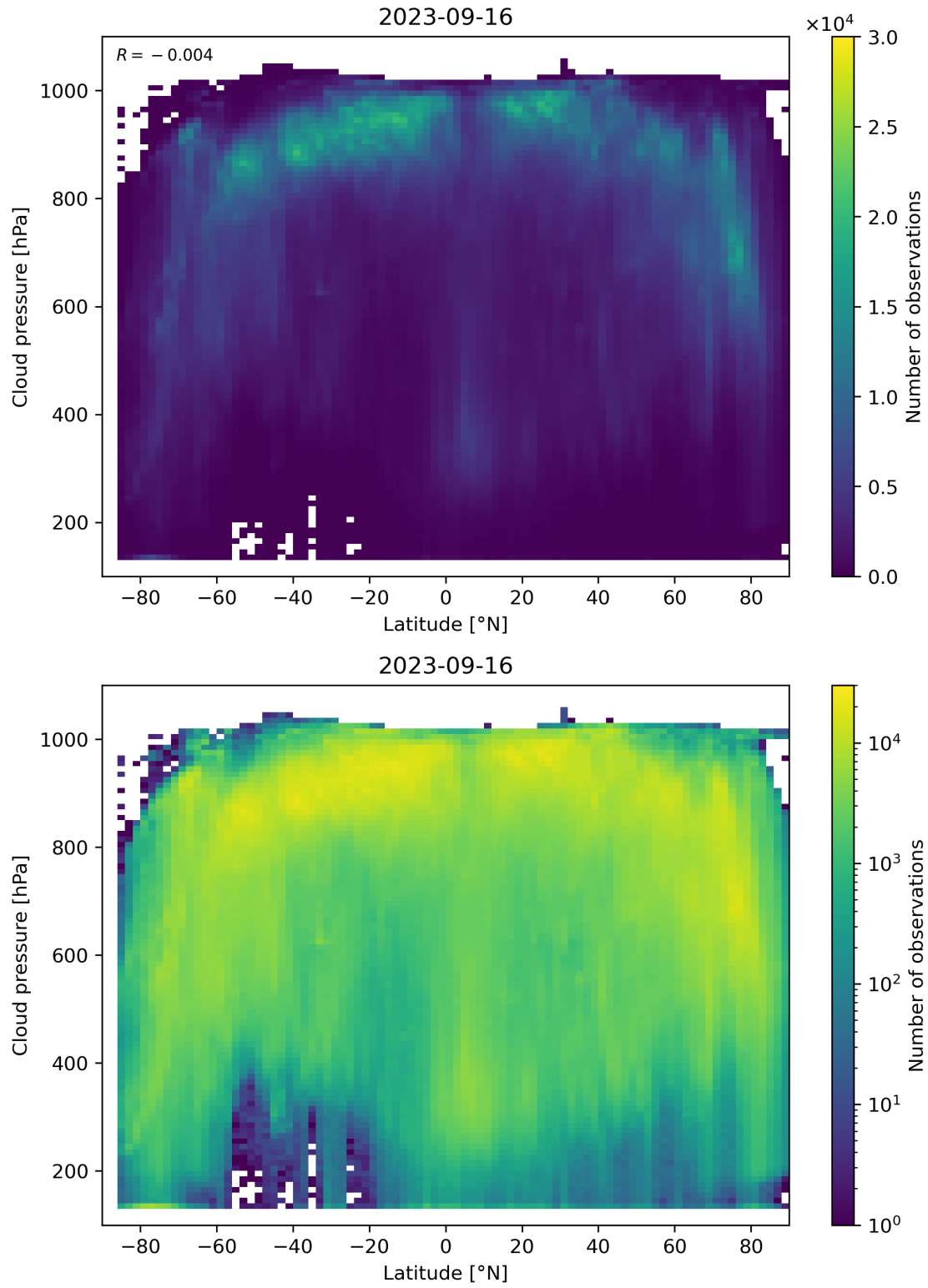
Figure 100: Scatter density plot of “Latitude” against “Cloud pressure” for 2023-09-15 to 2023-09-17.
