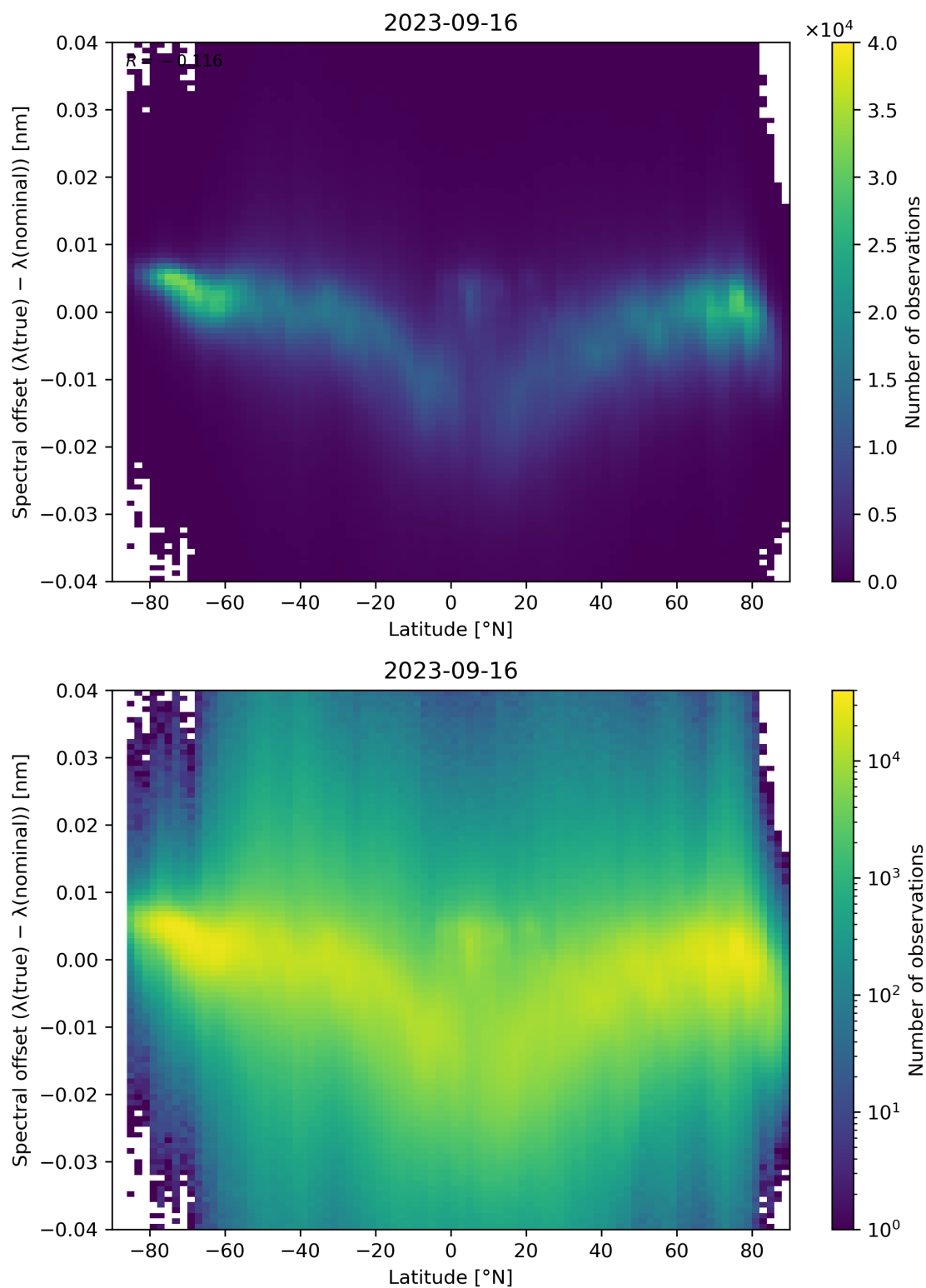
Figure 105: Scatter density plot of “Latitude” against “Spectral offset ( \lambda(\text{true}) - \lambda(\text{nominal}) )” for 2023-09-15 to 2023-09-17.
