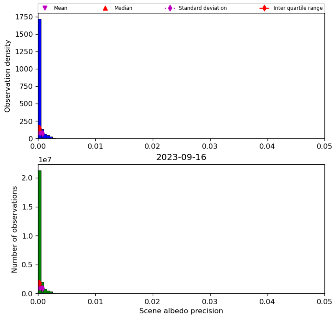
Figure 35: Histogram of “Scene albedo precision” for 2023-09-15 to 2023-09-17
