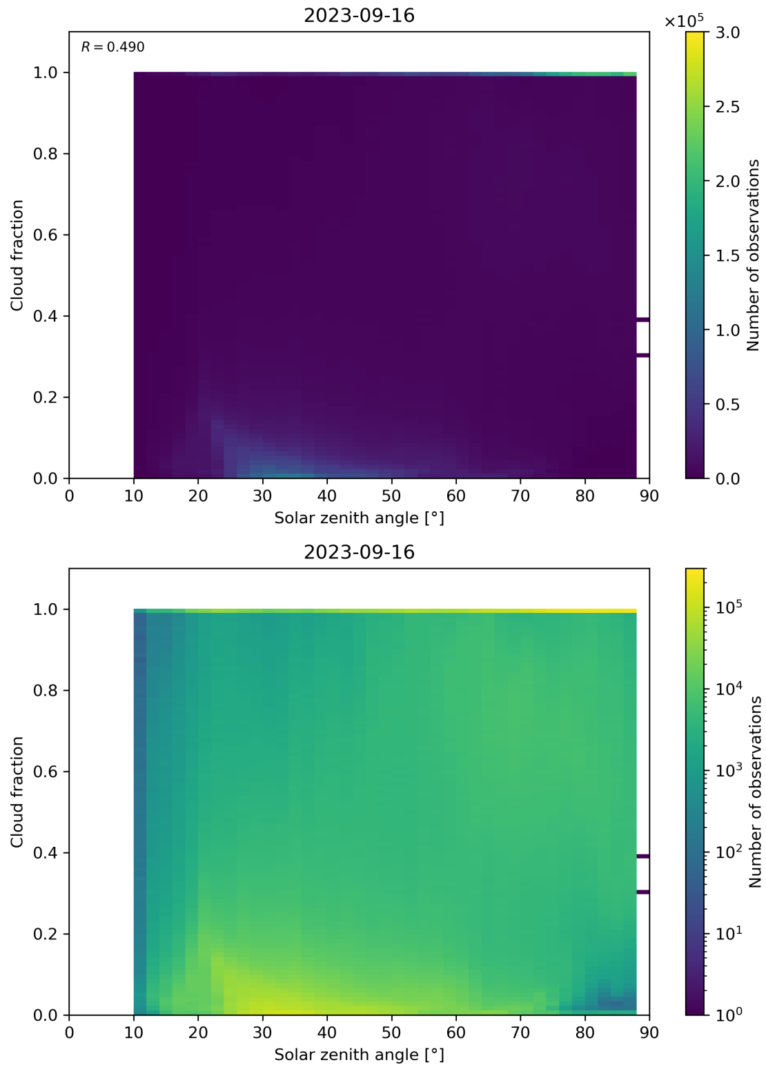
Figure 121: Scatter density plot of “Solar zenith angle” against “Cloud fraction” for 2023-09-15 to 2023-09-17.
