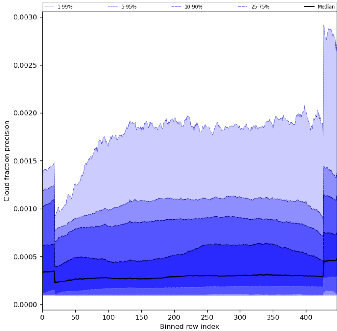
Figure 50: Along track statistics of “Cloud fraction precision” for 2023-09-15 to 2023-09-17
