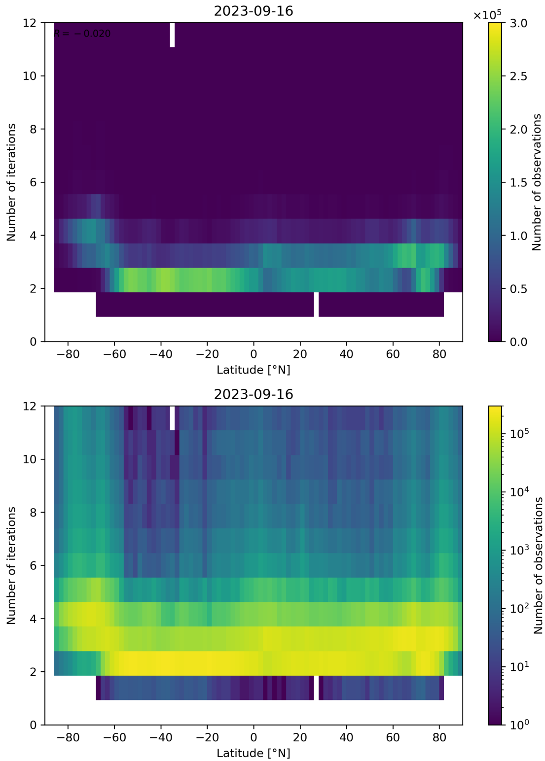
Figure 102: Scatter density plot of “Latitude” against “Number of iterations” for 2023-09-15 to 2023-09-17.
