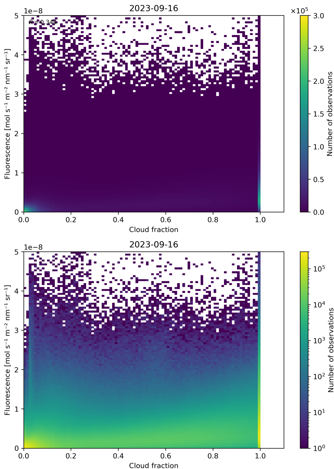
Figure 79: Scatter density plot of “Cloud fraction” against “Fluorescence” for 2023-09-15 to 2023-09-17.
