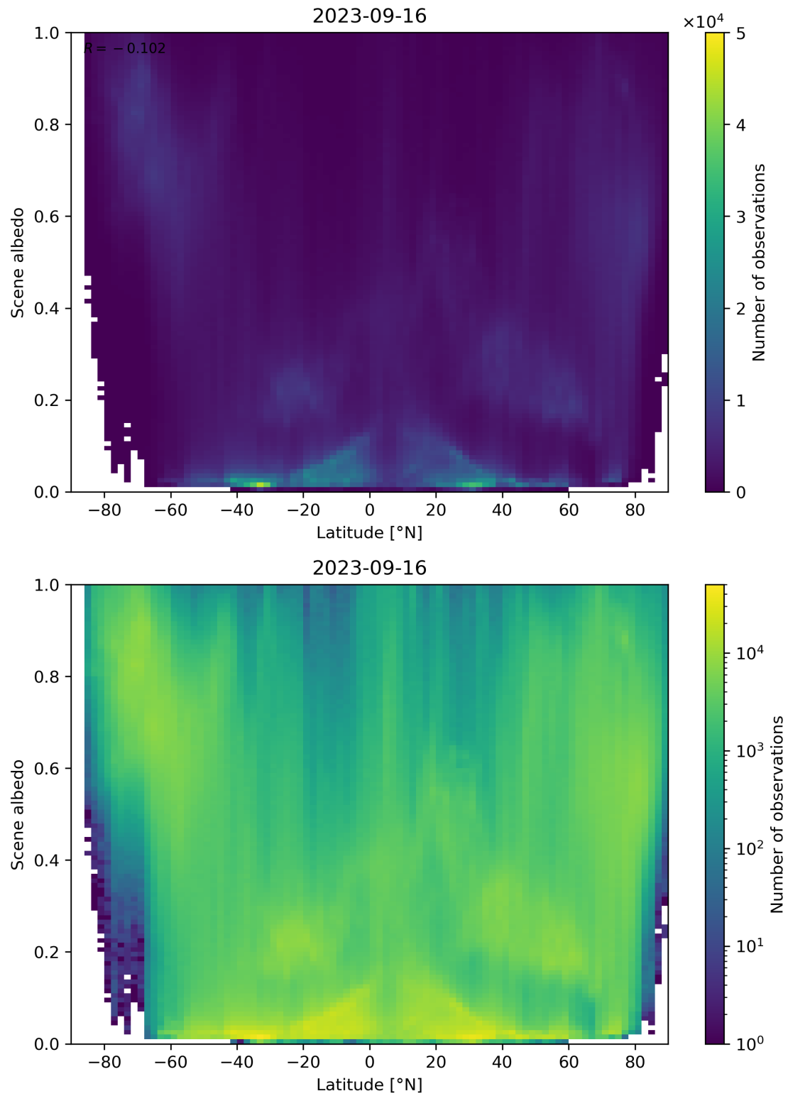
Figure 104: Scatter density plot of “Latitude” against “Scene albedo” for 2023-09-15 to 2023-09-17.
