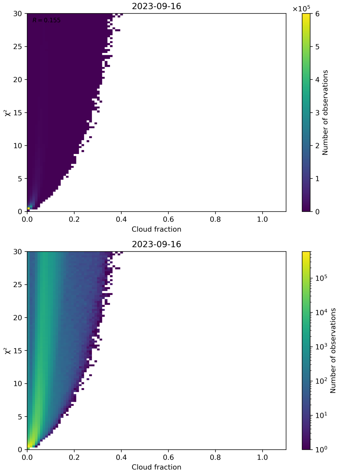
Figure 77: Scatter density plot of “Cloud fraction” against “ \chi^2 ” for 2023-09-15 to 2023-09-17.
