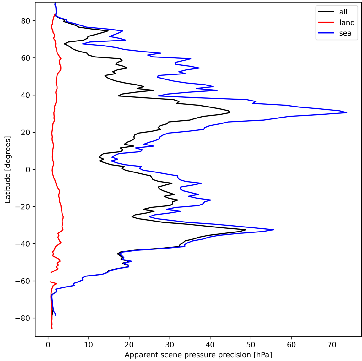
Figure 20: Zonal average of “Apparent scene pressure precision” for 2023-09-15 to 2023-09-17.
