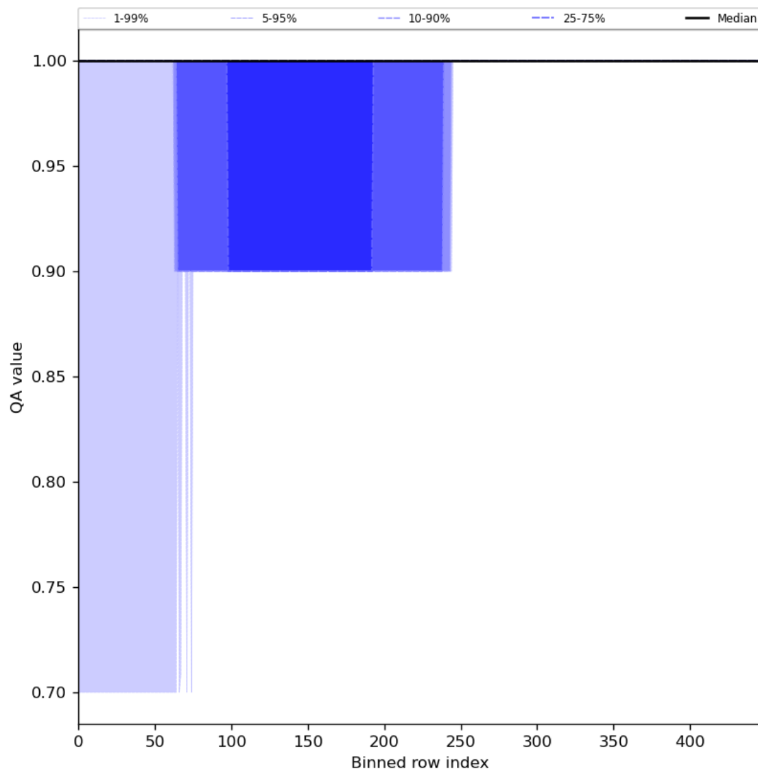
Figure 46: Along track statistics of “QA value” for 2023-09-15 to 2023-09-17
