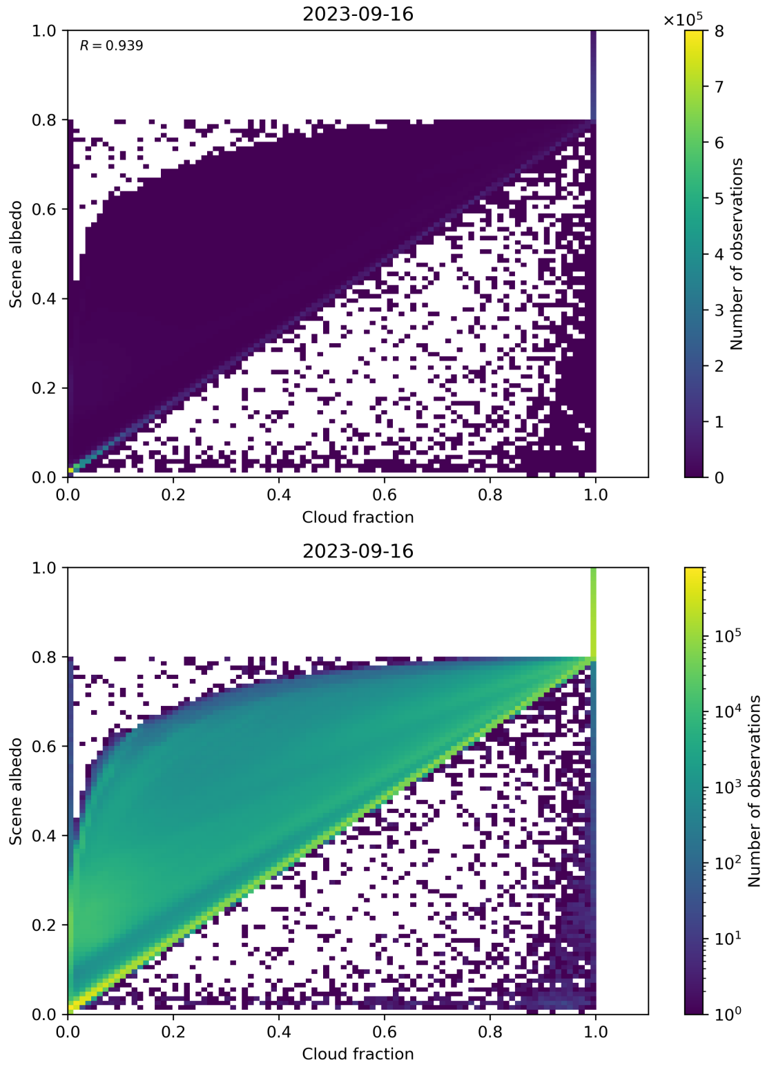
Figure 82: Scatter density plot of “Cloud fraction” against “Scene albedo” for 2023-09-15 to 2023-09-17.
