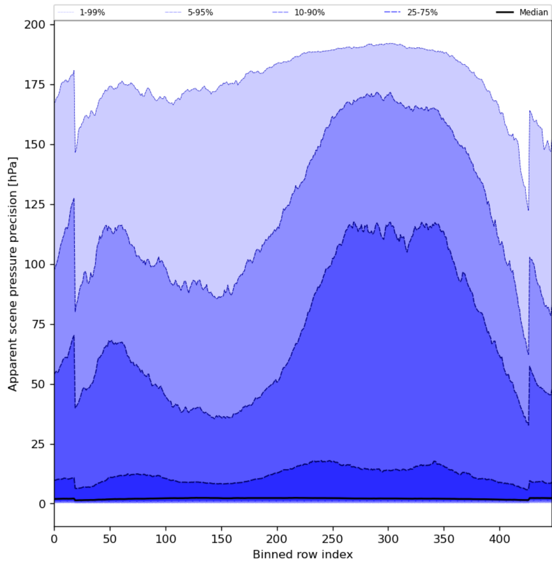
Figure 54: Along track statistics of “Apparent scene pressure precision” for 2023-09-15 to 2023-09-17
