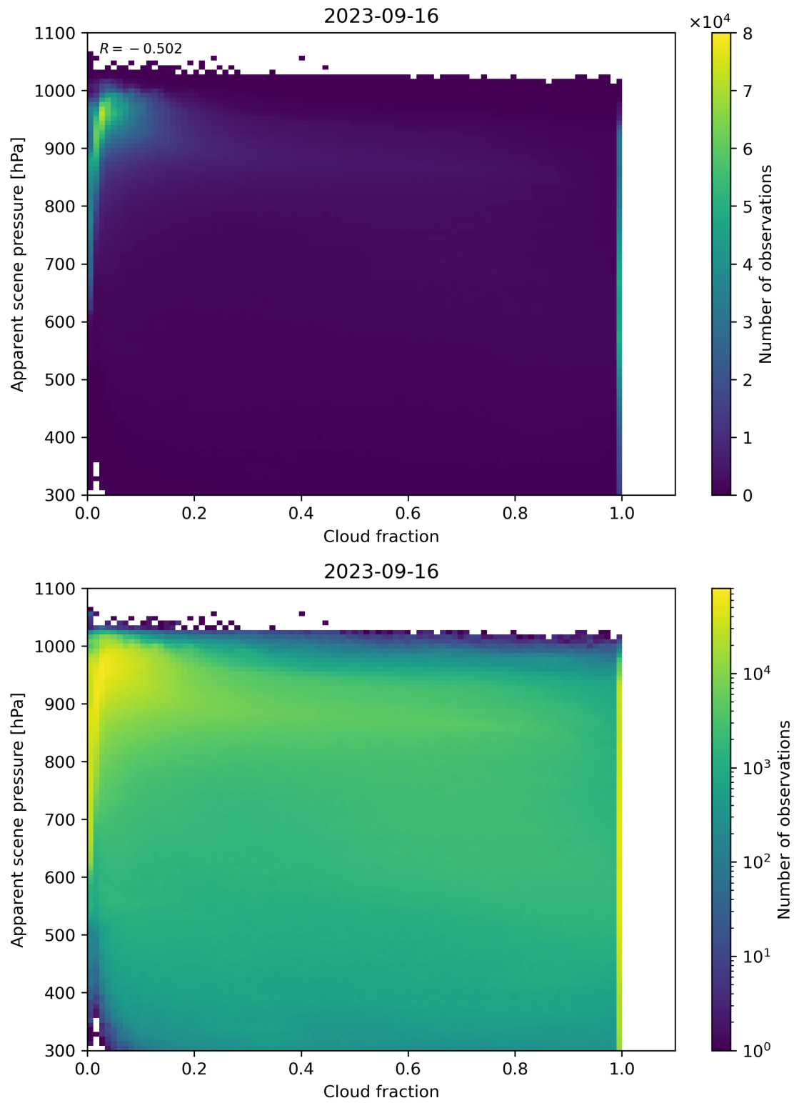
Figure 76: Scatter density plot of “Cloud fraction” against “Apparent scene pressure” for 2023-09-15 to 2023-09-17.
