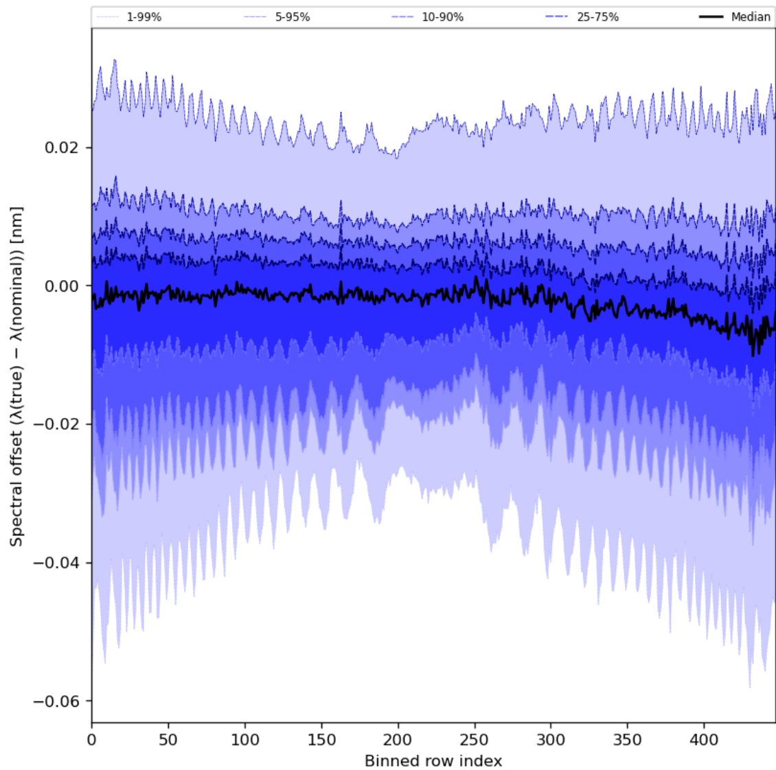
Figure 62: Along track statistics of “Spectral offset ( \lambda(\text{true}) - \lambda(\text{nominal}) )” for 2023-09-15 to 2023-09-17
