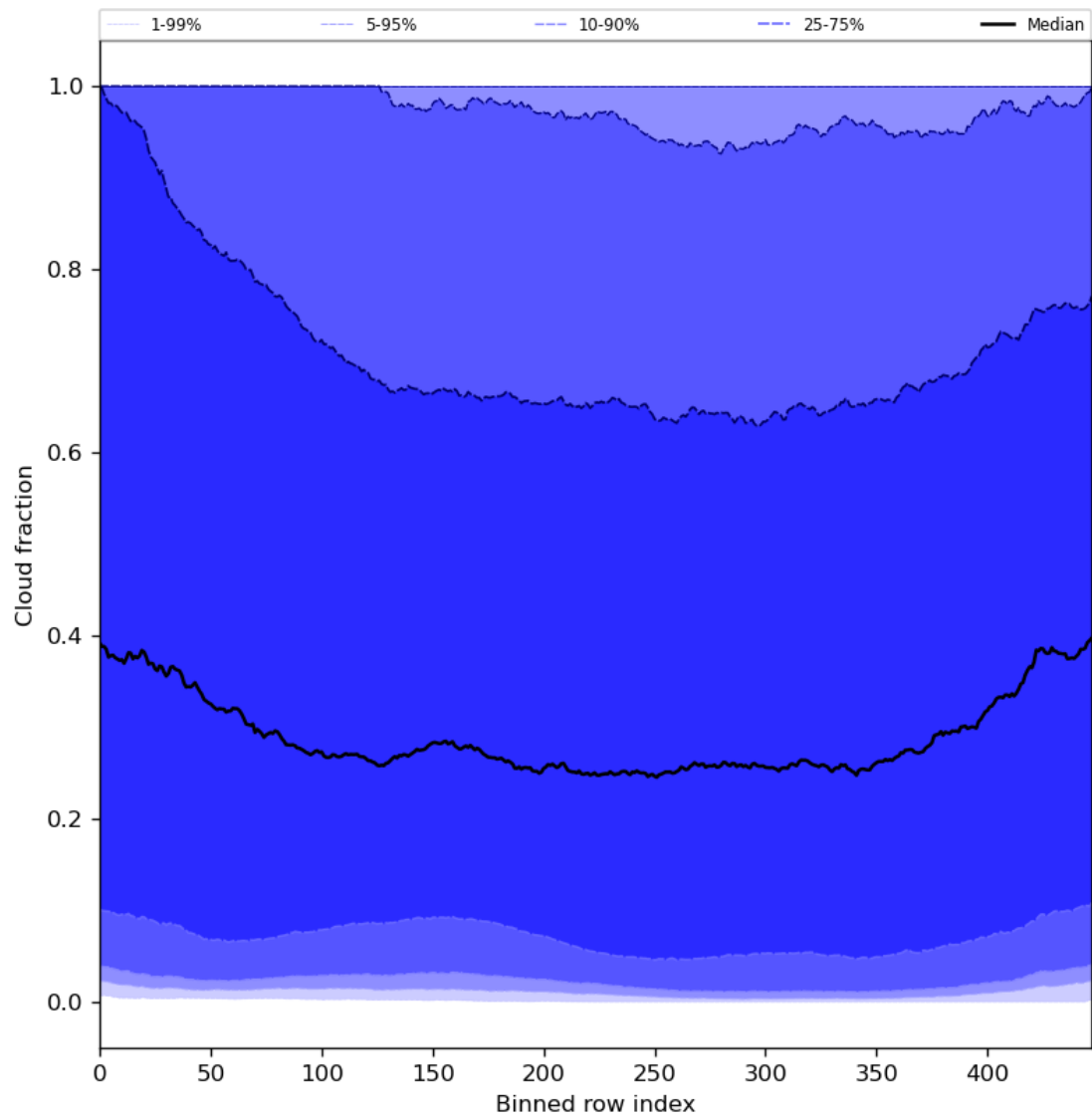
Figure 49: Along track statistics of “Cloud fraction” for 2023-09-15 to 2023-09-17
