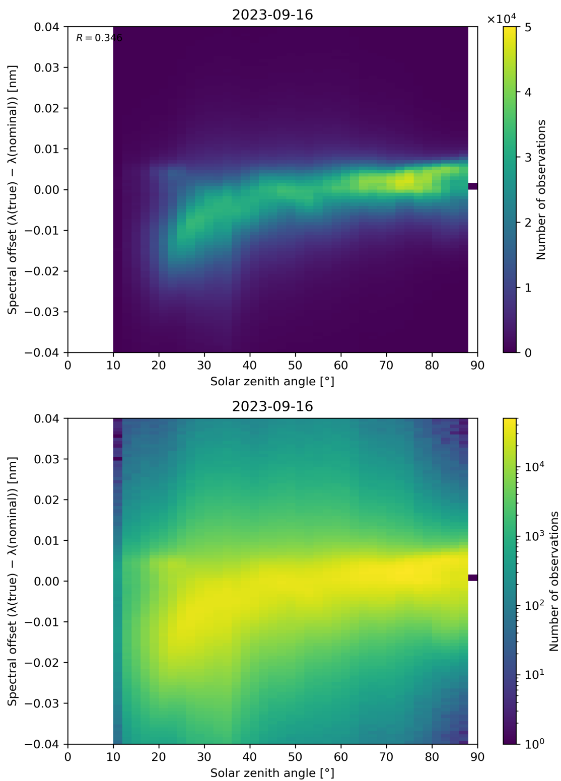
Figure 128: Scatter density plot of “Solar zenith angle” against “Spectral offset ( \lambda(\text{true}) - \lambda(\text{nominal}) )” for 2023-09-15 to 2023-09-17.
