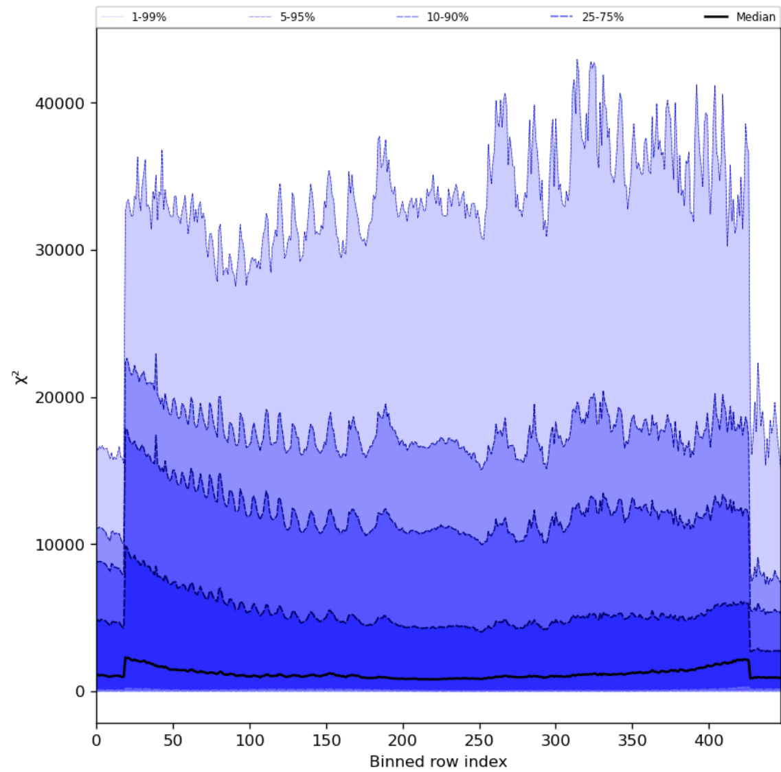
Figure 55: Along track statistics of “ \chi^2 ” for 2023-09-15 to 2023-09-17
