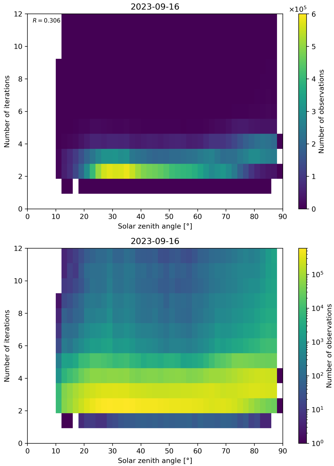
Figure 125: Scatter density plot of “Solar zenith angle” against “Number of iterations” for 2023-09-15 to 2023-09-17.
