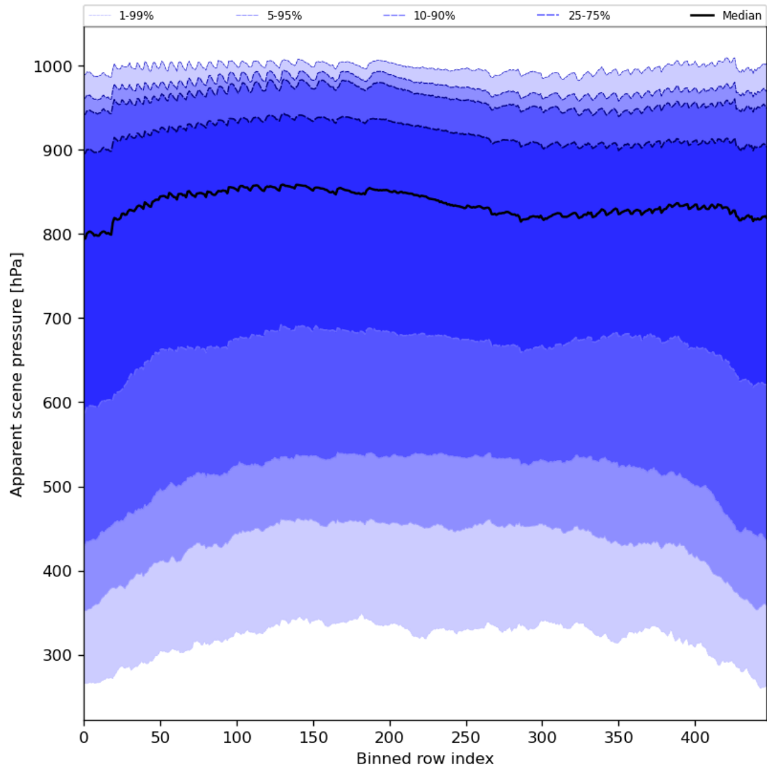
Figure 53: Along track statistics of “Apparent scene pressure” for 2023-09-15 to 2023-09-17
