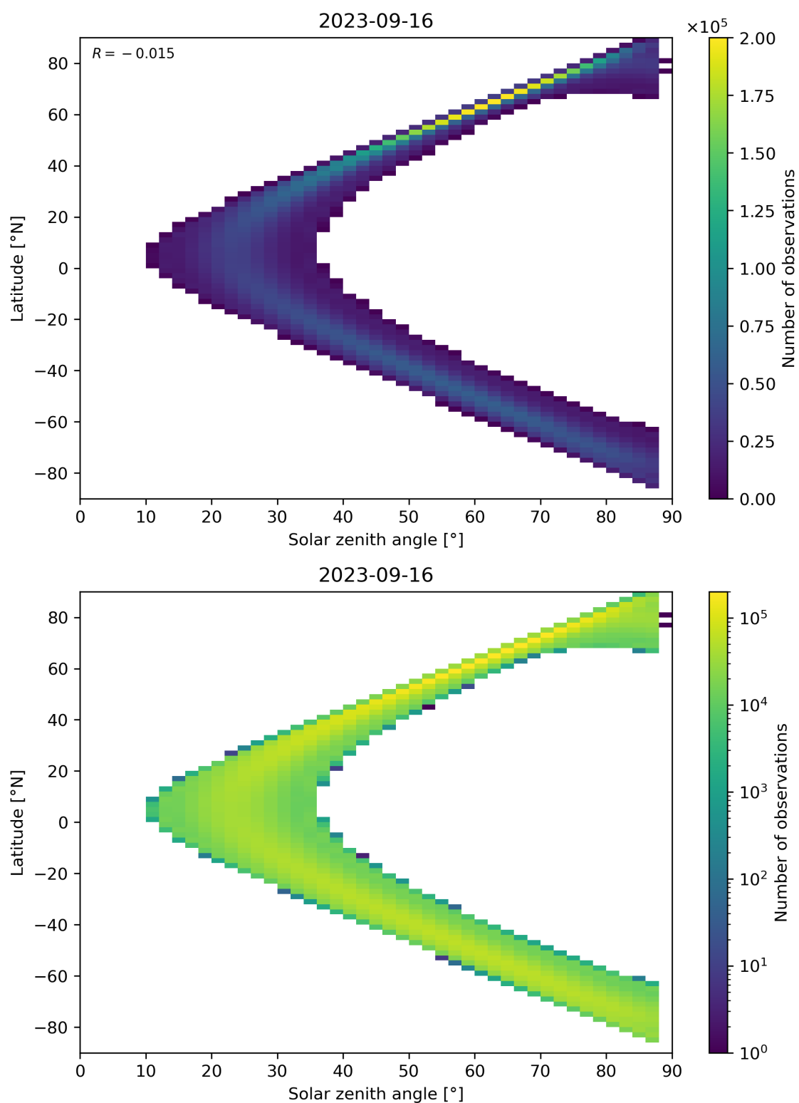
Figure 124: Scatter density plot of “Solar zenith angle” against “Latitude” for 2023-09-15 to 2023-09-17.
