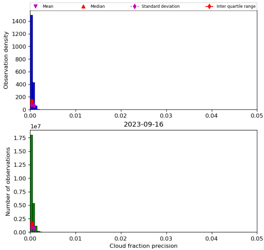
Figure 33: Histogram of “Cloud fraction precision” for 2023-09-15 to 2023-09-17
