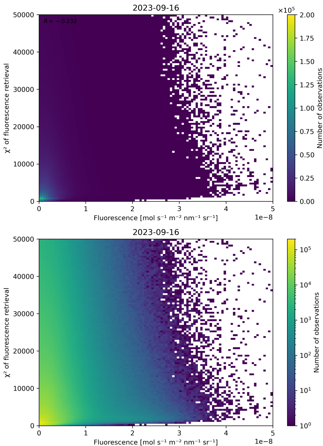
Figure 93: Scatter density plot of “Fluorescence” against “ \chi^2 of fluorescence retrieval” for 2023-09-15 to 2023-09-17.
