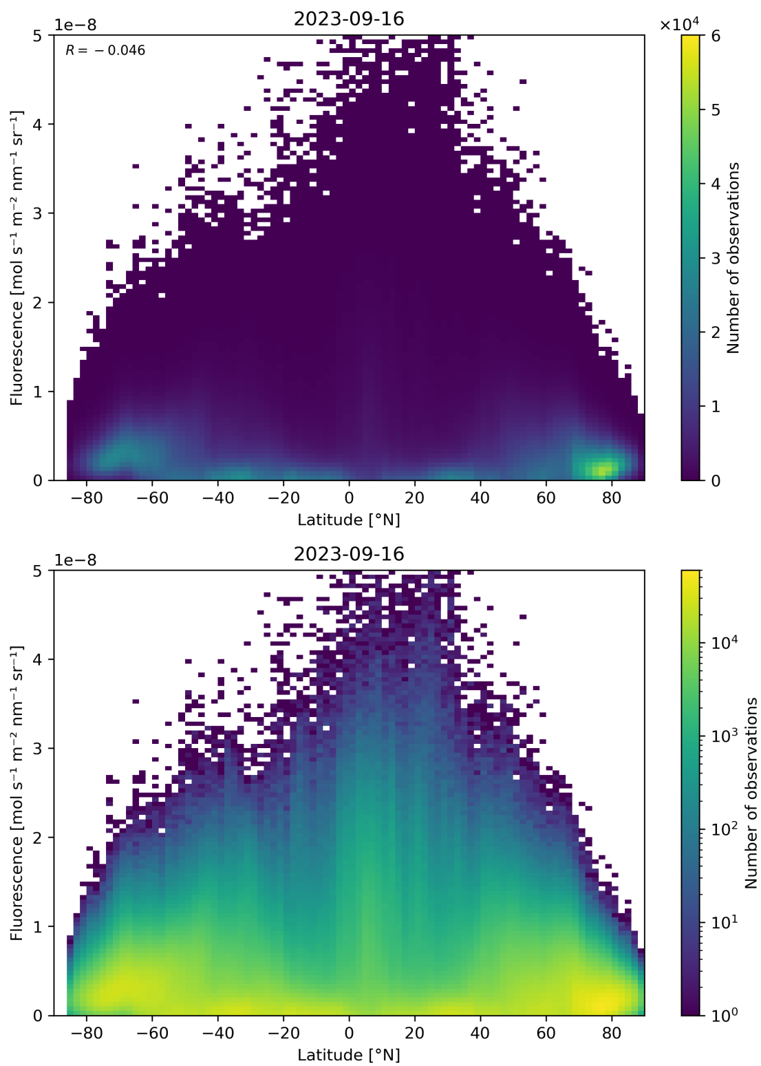
Figure 101: Scatter density plot of “Latitude” against “Fluorescence” for 2023-09-15 to 2023-09-17.
