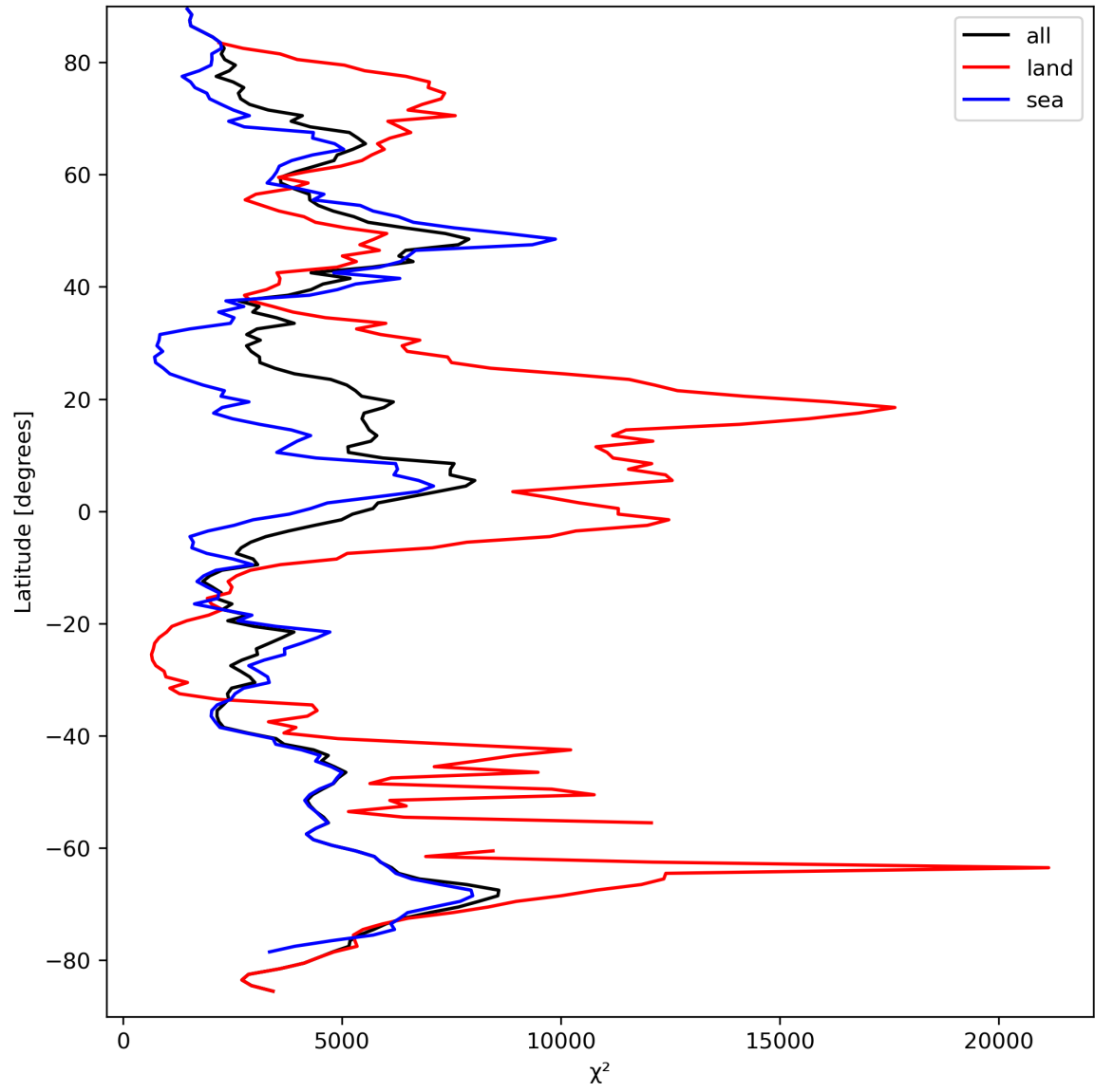
Figure 21: Zonal average of “ \chi^2 ” for 2023-09-15 to 2023-09-17.
