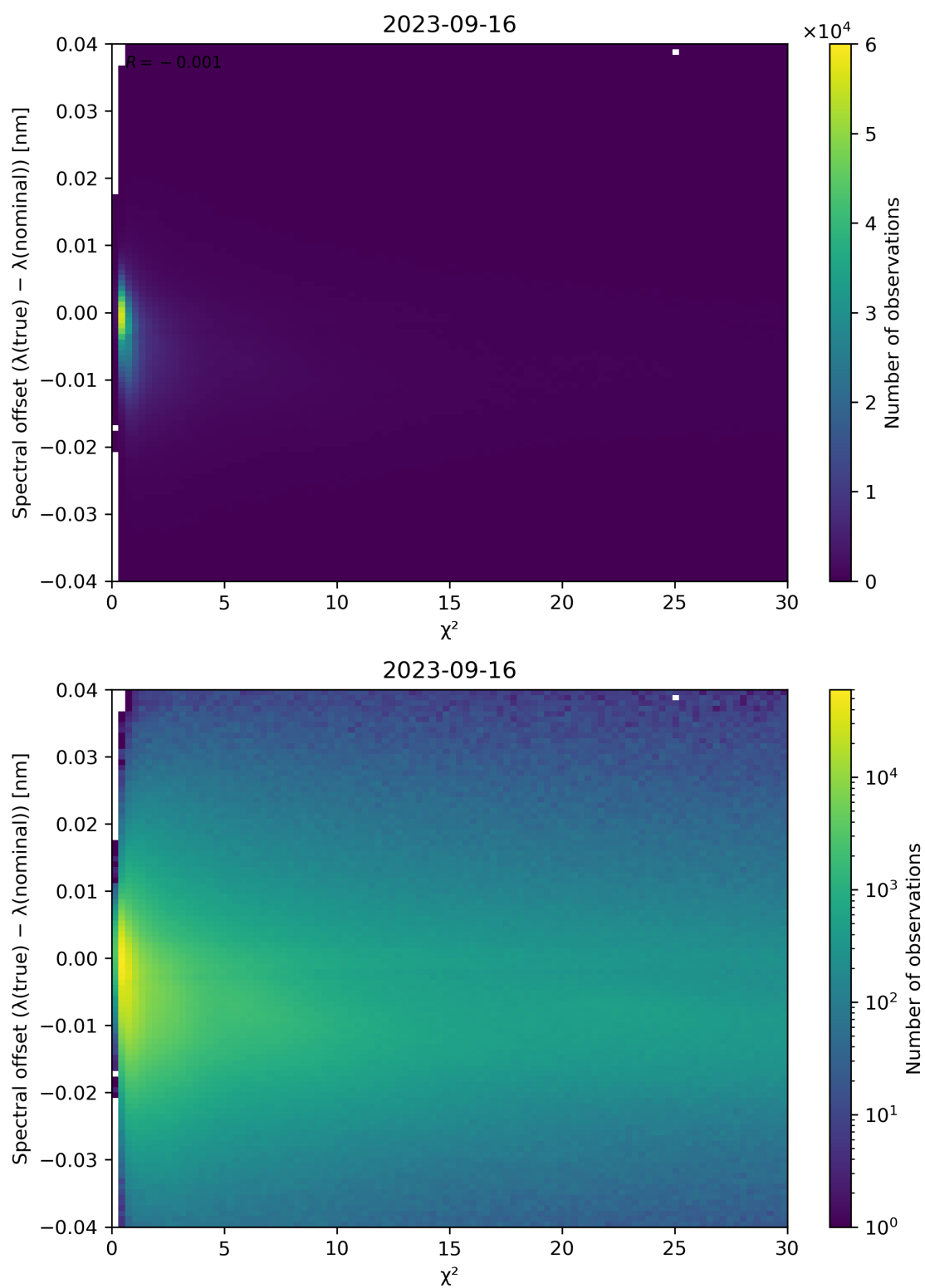
Figure 75: Scatter density plot of “ \chi^2 ” against “Spectral offset ( \lambda(\text{true}) - \lambda(\text{nominal}) )” for 2023-09-15 to 2023-09-17.
