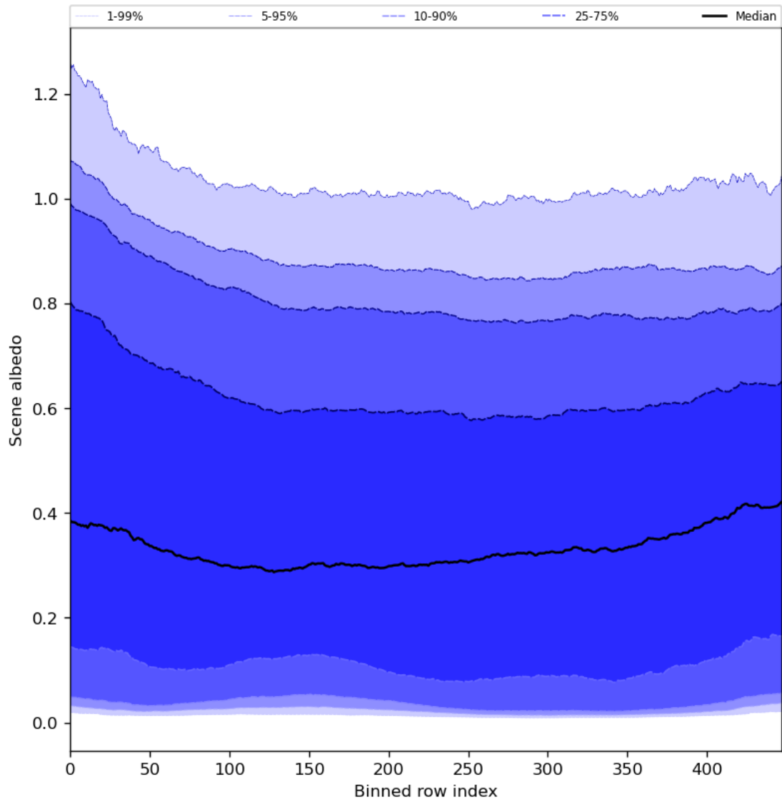
Figure 51: Along track statistics of “Scene albedo” for 2023-09-15 to 2023-09-17
