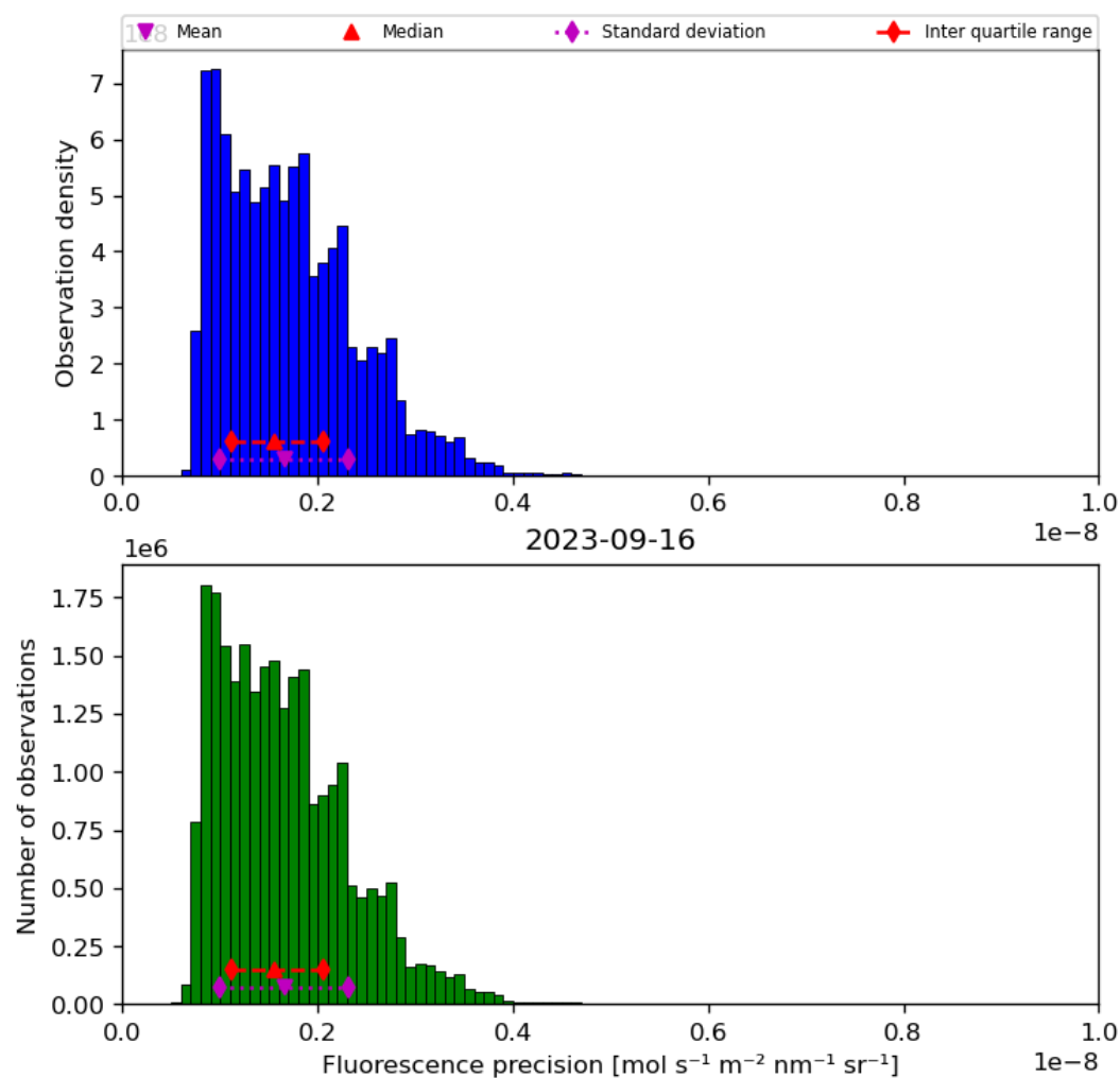
Figure 41: Histogram of “Fluorescence precision” for 2023-09-15 to 2023-09-17
