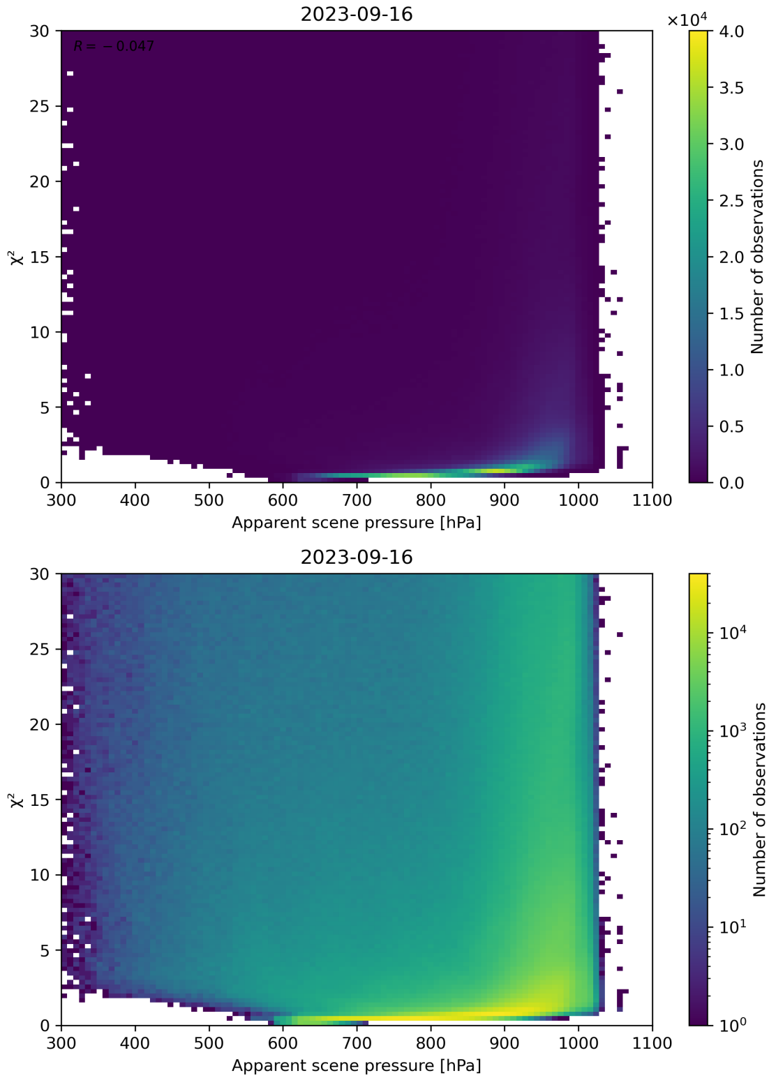
Figure 63: Scatter density plot of “Apparent scene pressure” against “ \chi^2 ” for 2023-09-15 to 2023-09-17.
