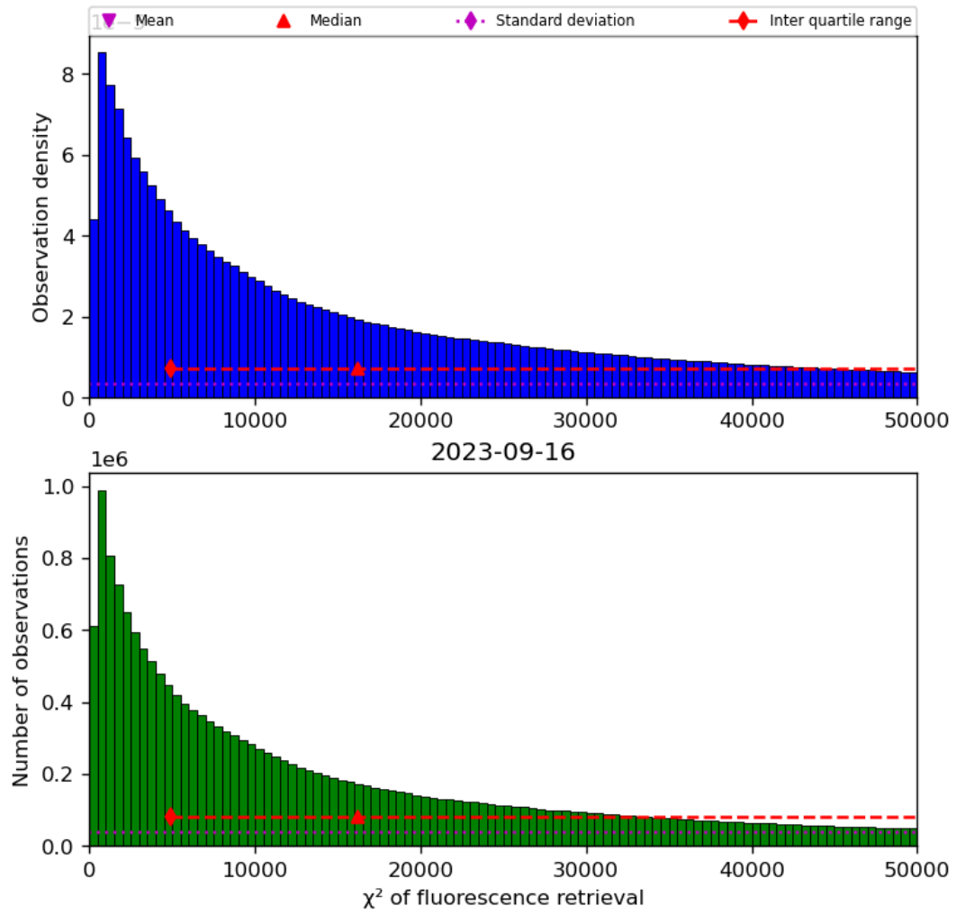
Figure 42: Histogram of “ \chi^2 of fluorescence retrieval” for 2023-09-15 to 2023-09-17
