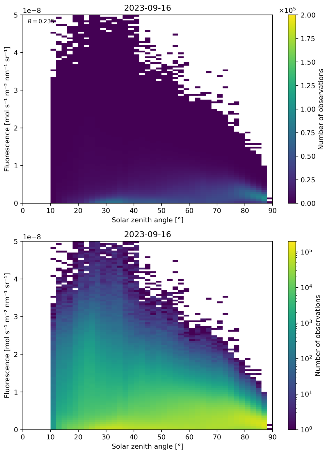
Figure 123: Scatter density plot of “Solar zenith angle” against “Fluorescence” for 2023-09-15 to 2023-09-17.
