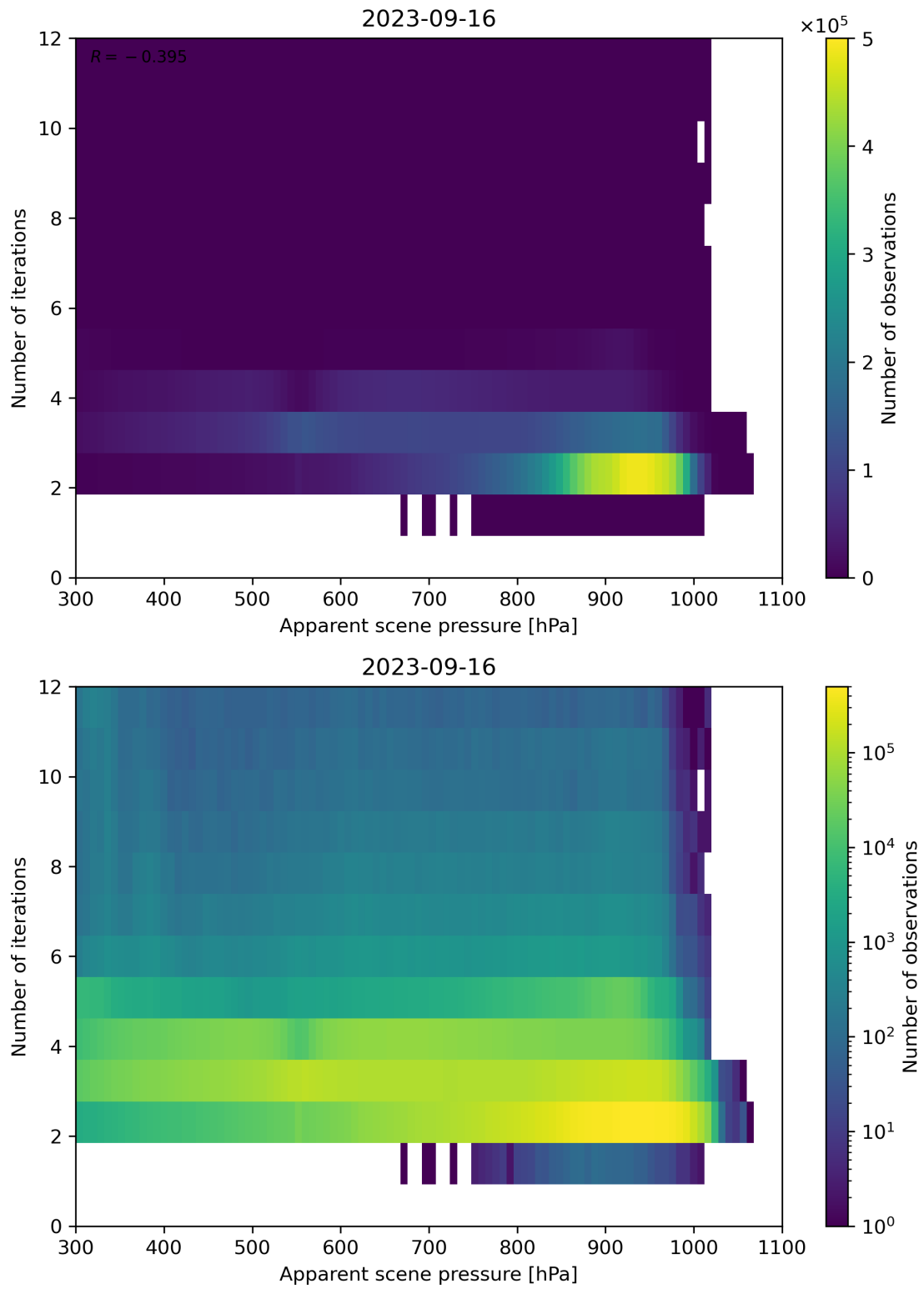
Figure 66: Scatter density plot of “Apparent scene pressure” against “Number of iterations” for 2023-09-15 to 2023-09-17.
