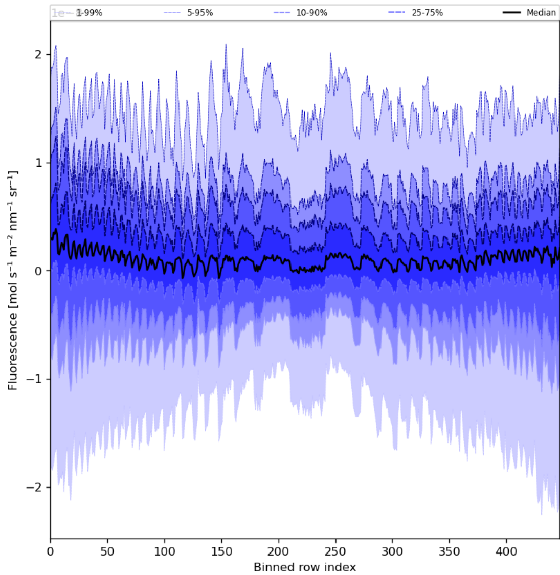
Figure 57: Along track statistics of “Fluorescence” for 2023-09-15 to 2023-09-17
