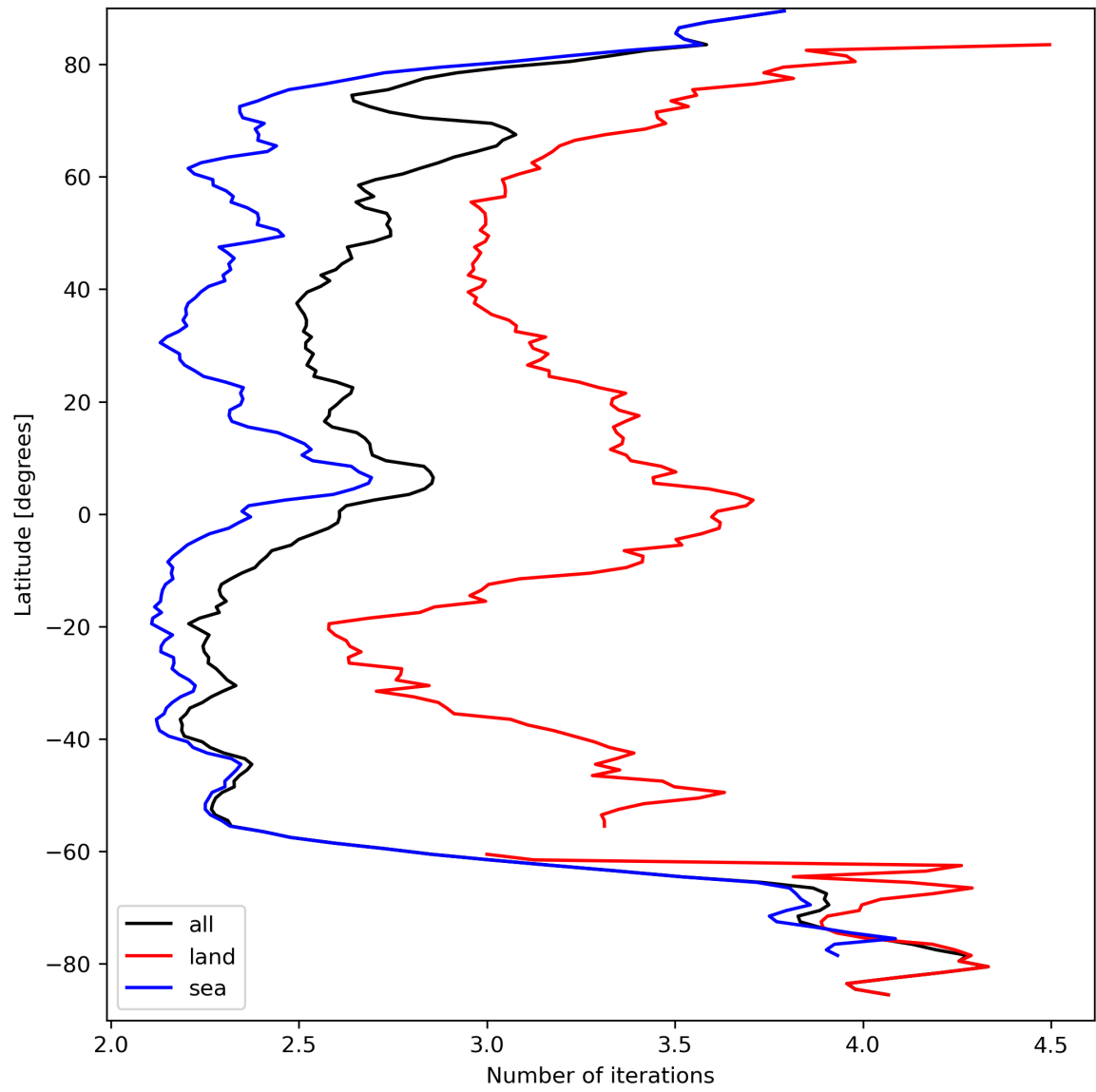
Figure 22: Zonal average of “Number of iterations” for 2023-09-15 to 2023-09-17.
