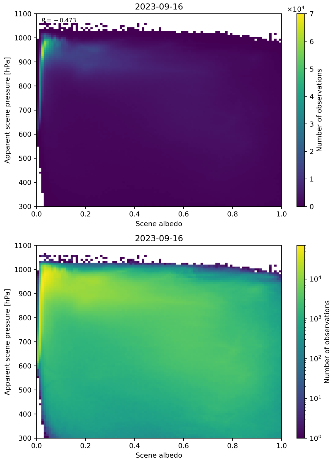
Figure 111: Scatter density plot of “Scene albedo” against “Apparent scene pressure” for 2023-09-15 to 2023-09-17.
