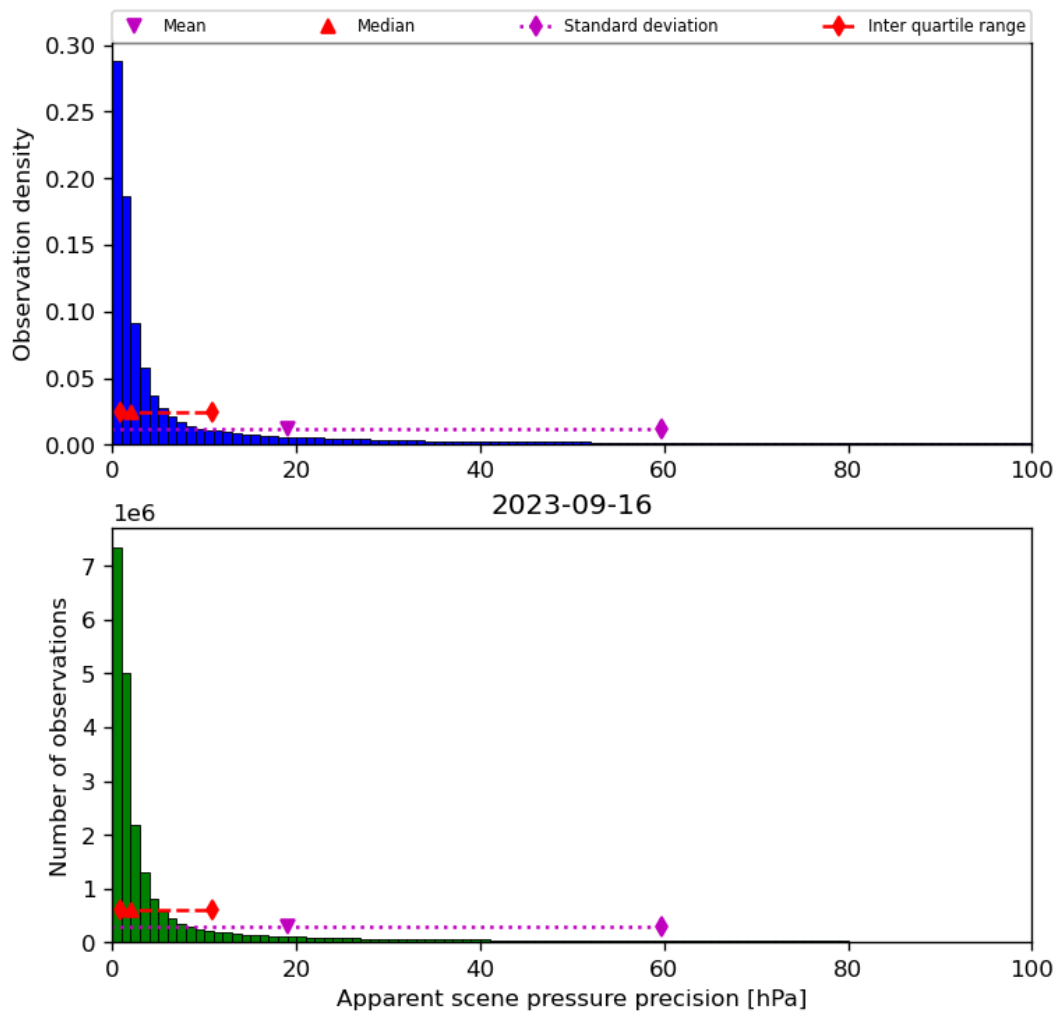
Figure 37: Histogram of “Apparent scene pressure precision” for 2023-09-15 to 2023-09-17
