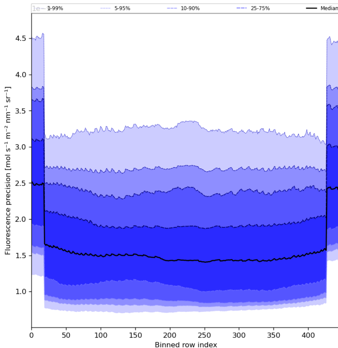
Figure 58: Along track statistics of “Fluorescence precision” for 2023-09-15 to 2023-09-17
