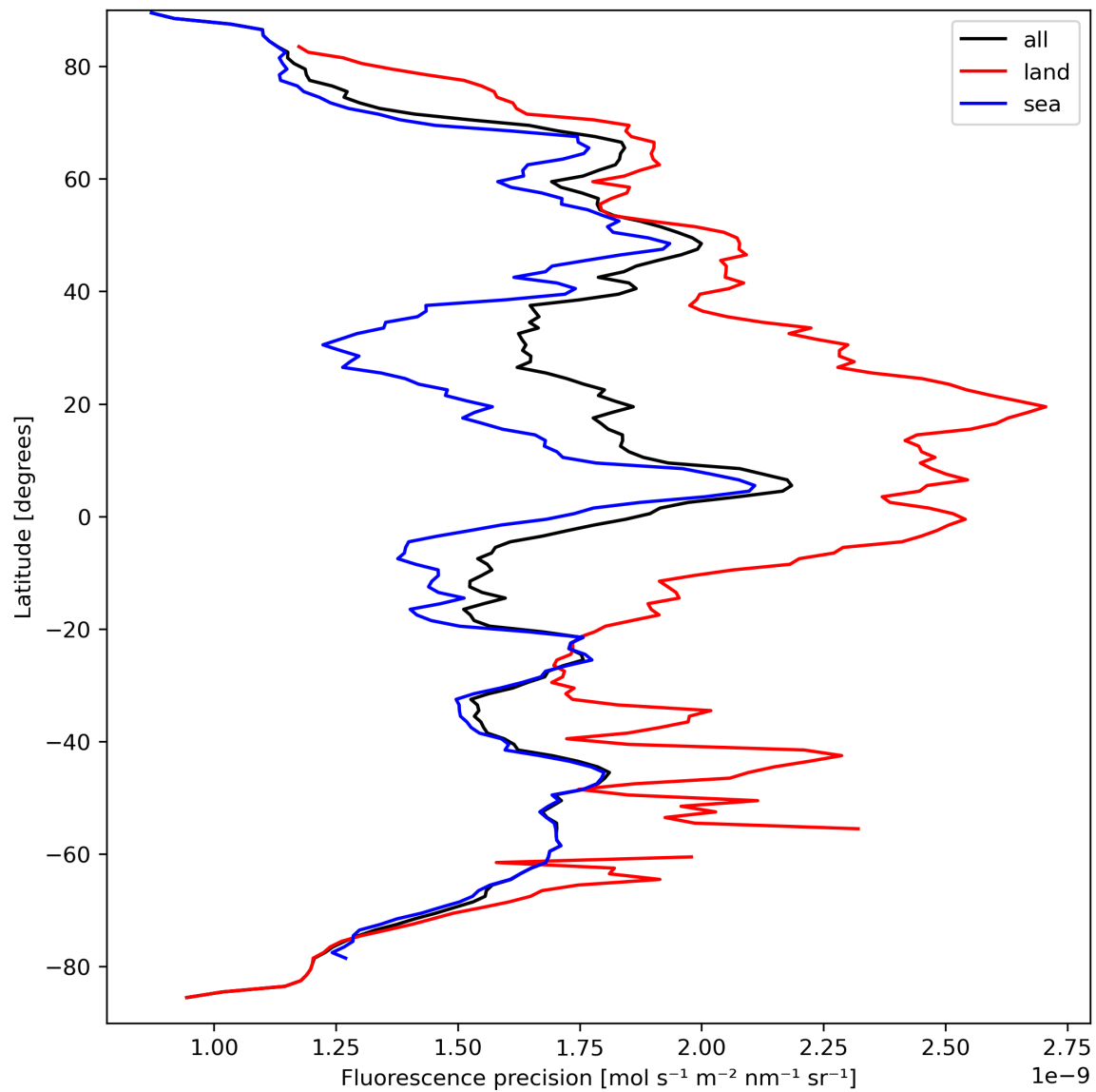
Figure 24: Zonal average of “Fluorescence precision” for 2023-09-15 to 2023-09-17.
