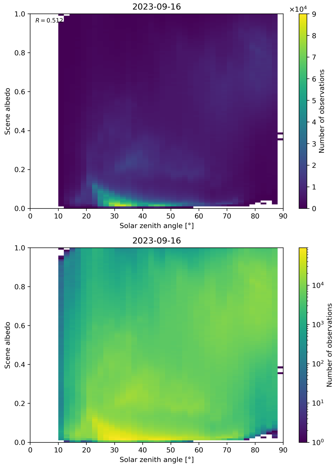
Figure 127: Scatter density plot of “Solar zenith angle” against “Scene albedo” for 2023-09-15 to 2023-09-17.
