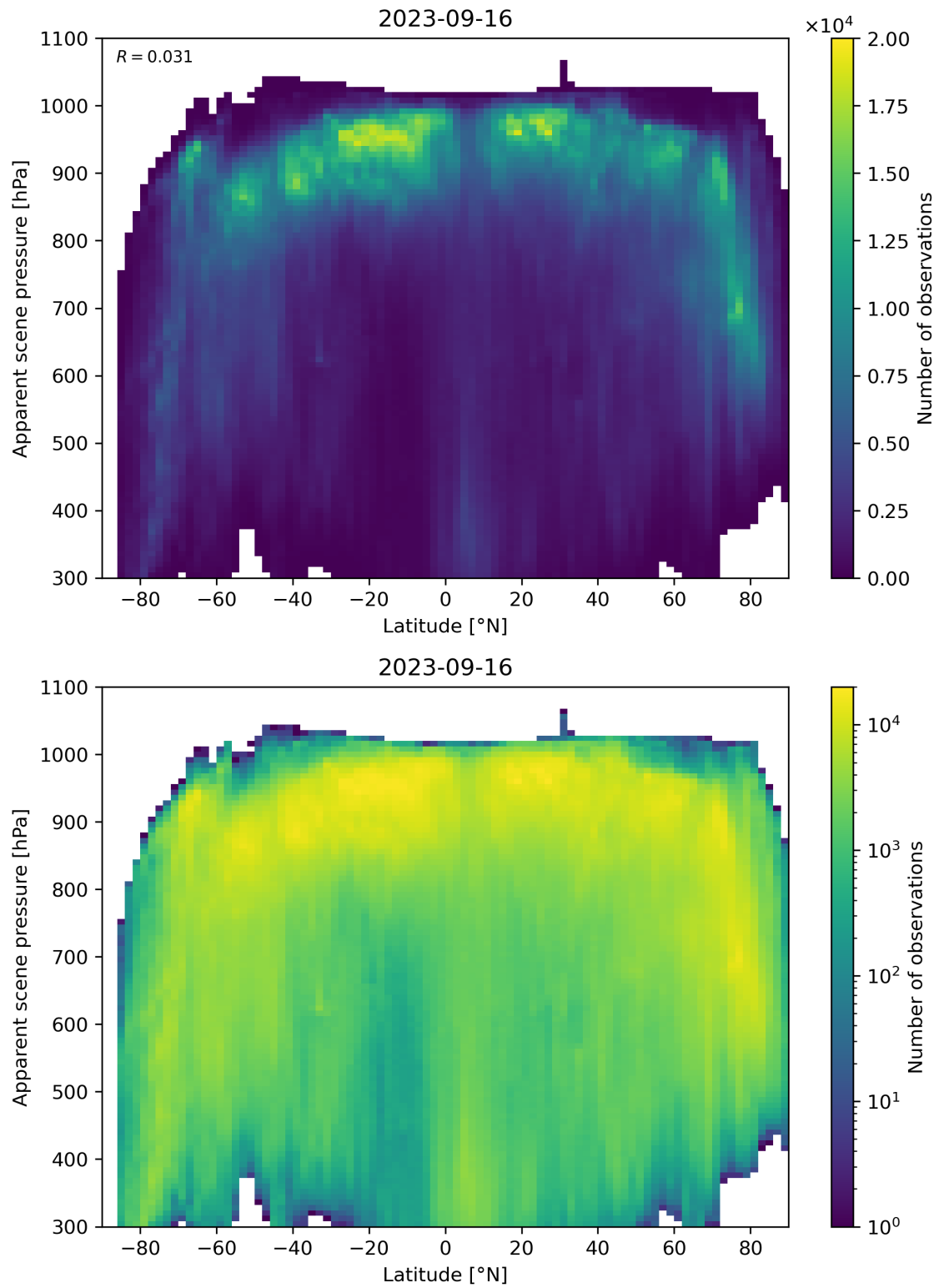
Figure 96: Scatter density plot of “Latitude” against “Apparent scene pressure” for 2023-09-15 to 2023-09-17.
