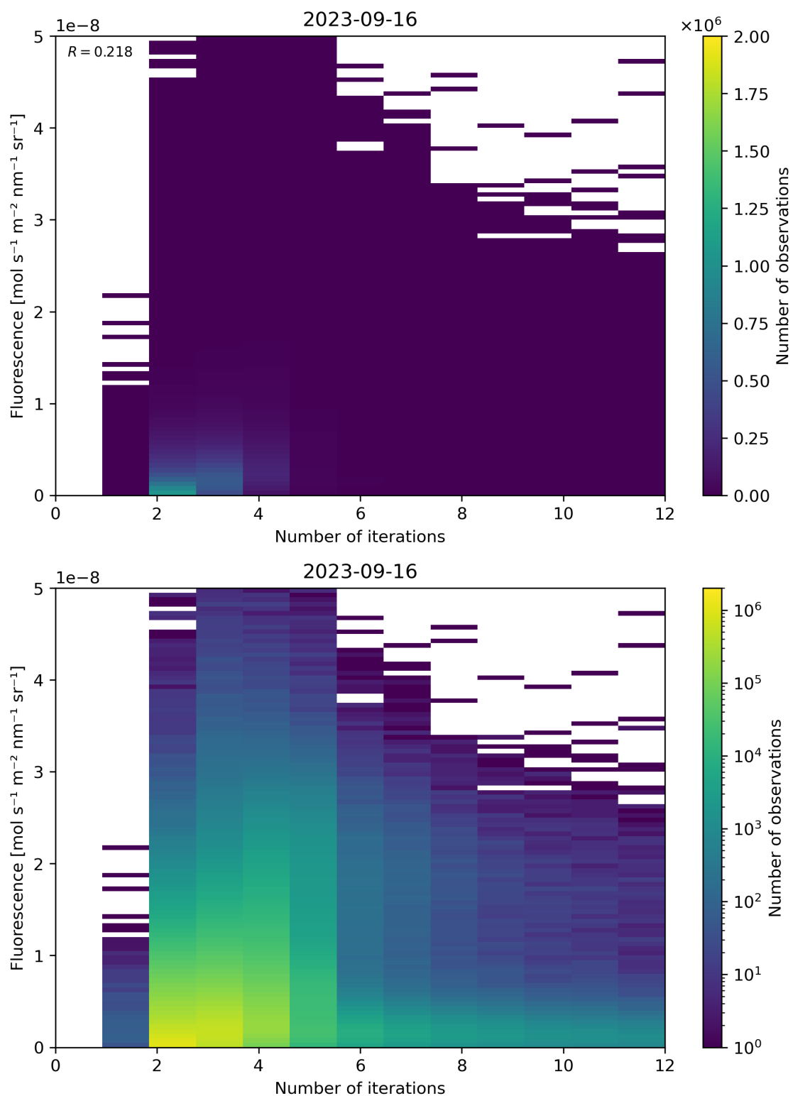
Figure 107: Scatter density plot of “Number of iterations” against “Fluorescence” for 2023-09-15 to 2023-09-17.
