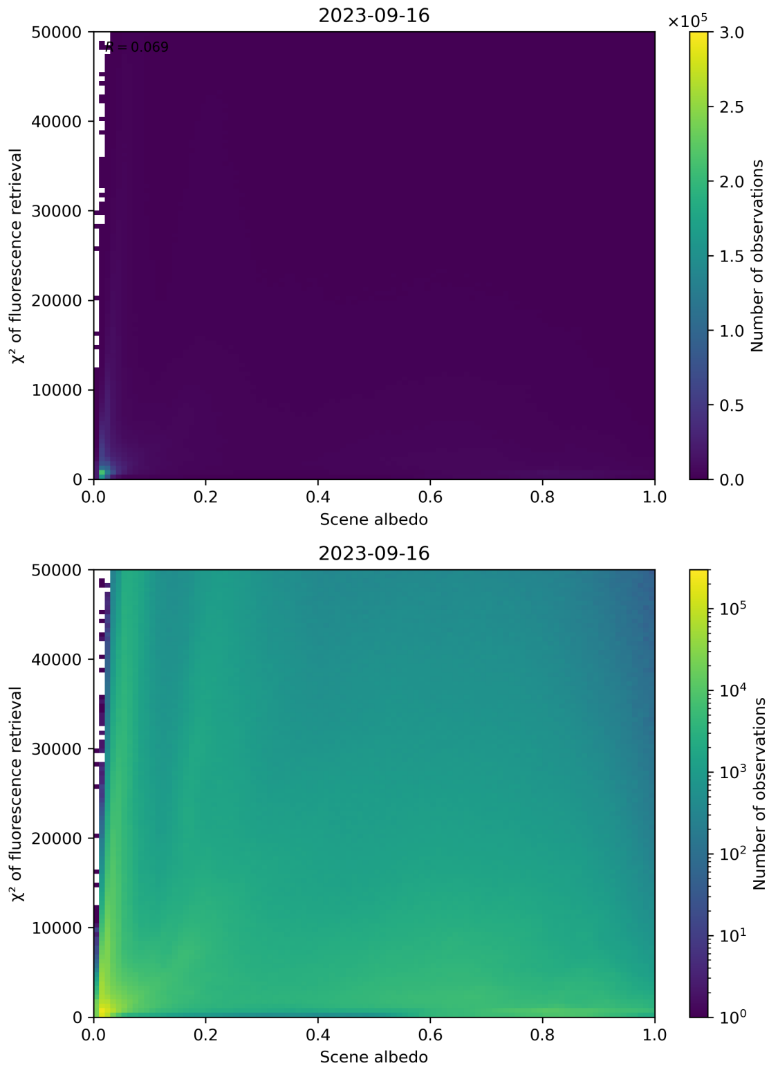
Figure 113: Scatter density plot of “Scene albedo” against “ \chi^2 of fluorescence retrieval” for 2023-09-15 to 2023-09-17.
