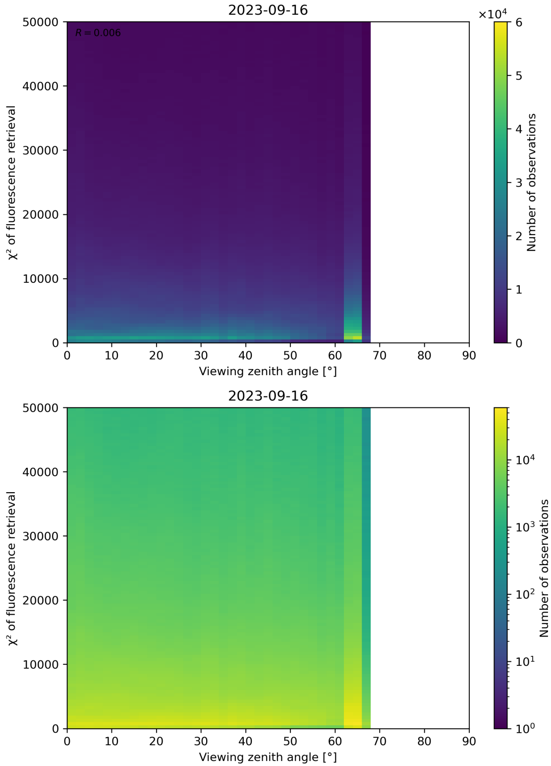
Figure 131: Scatter density plot of “Viewing zenith angle” against “ \chi^2 of fluorescence retrieval” for 2023-09-15 to 2023-09-17.
