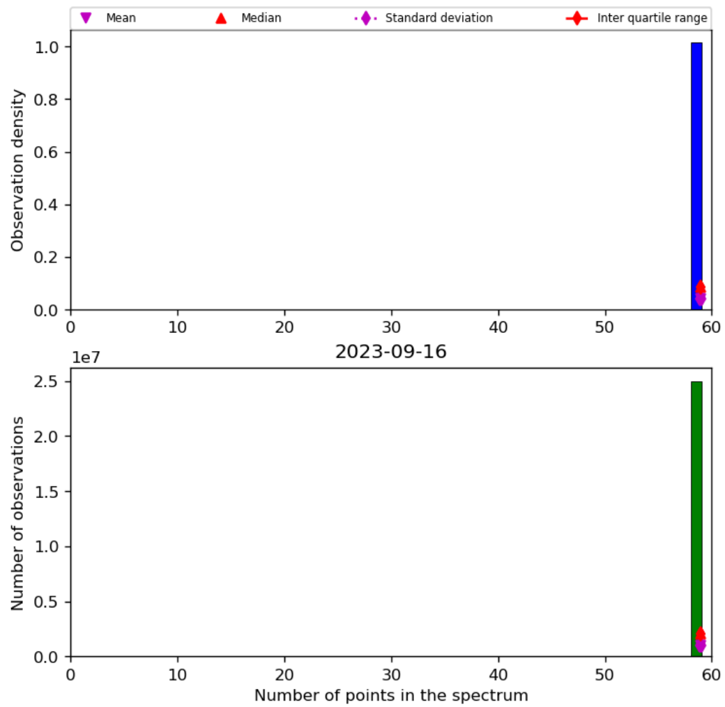
Figure 44: Histogram of "Number of points in the spectrum" for 2023-09-15 to 2023-09-17
