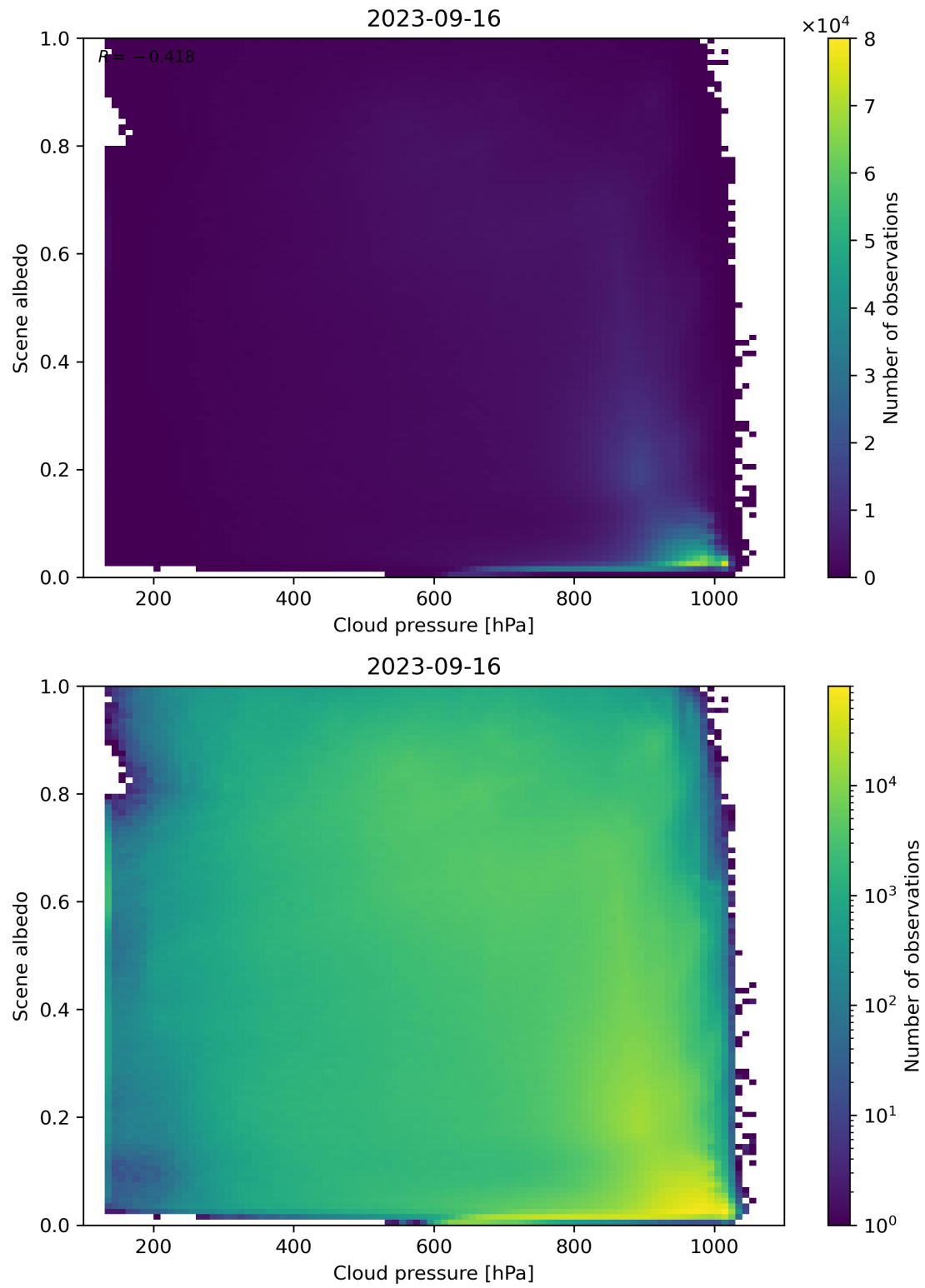
Figure 91: Scatter density plot of “Cloud pressure” against “Scene albedo” for 2023-09-15 to 2023-09-17.
