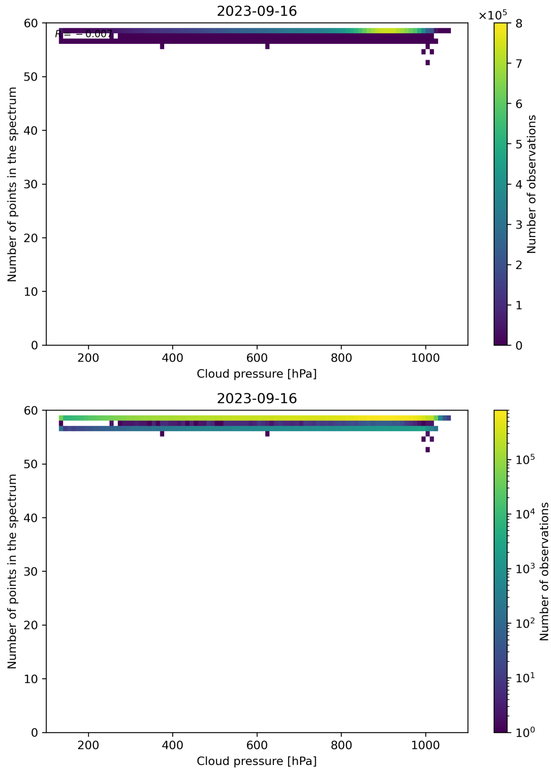
Figure 90: Scatter density plot of “Cloud pressure” against “Number of points in the spectrum” for 2023-09-15 to 2023-09-17.
