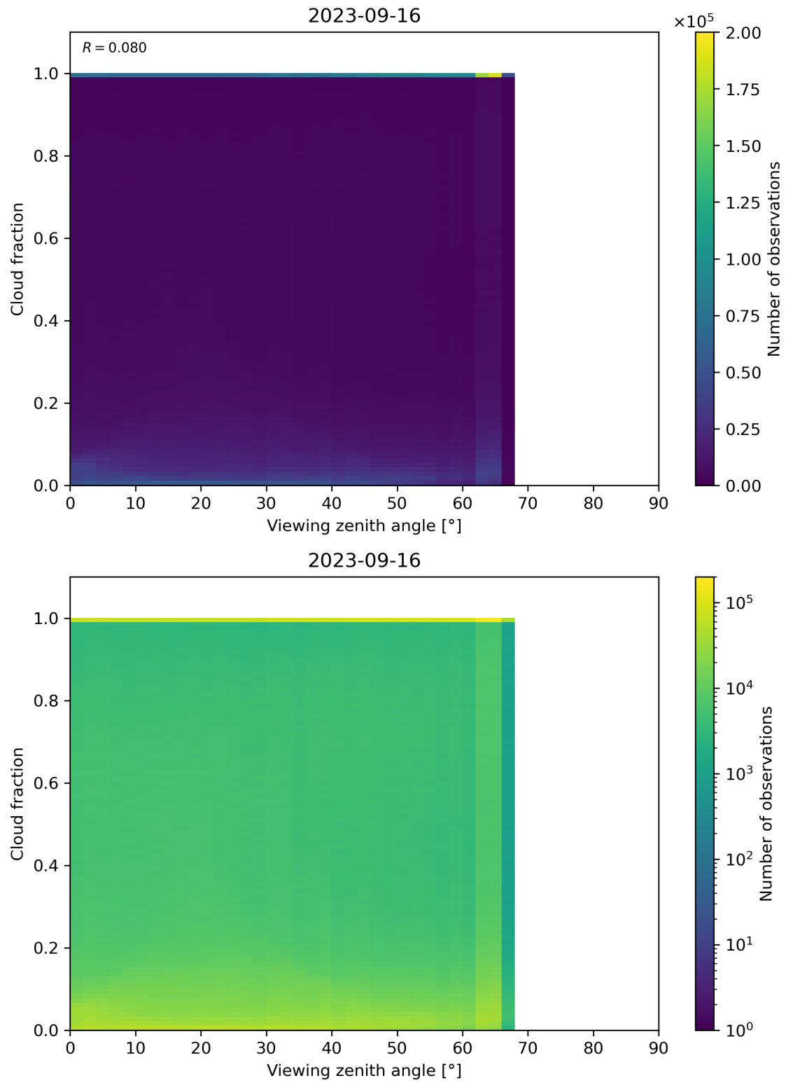
Figure 132: Scatter density plot of “Viewing zenith angle” against “Cloud fraction” for 2023-09-15 to 2023-09-17.
