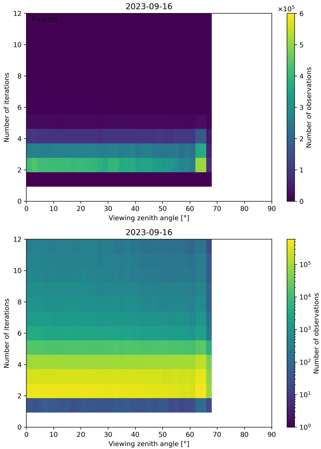
Figure 136: Scatter density plot of “Viewing zenith angle” against “Number of iterations” for 2023-09-15 to 2023-09-17.
