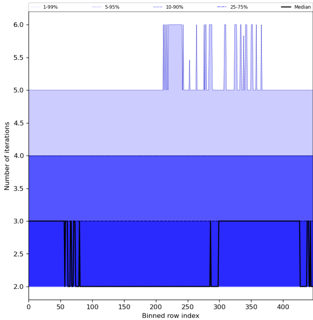
Figure 56: Along track statistics of “Number of iterations” for 2023-09-15 to 2023-09-17
