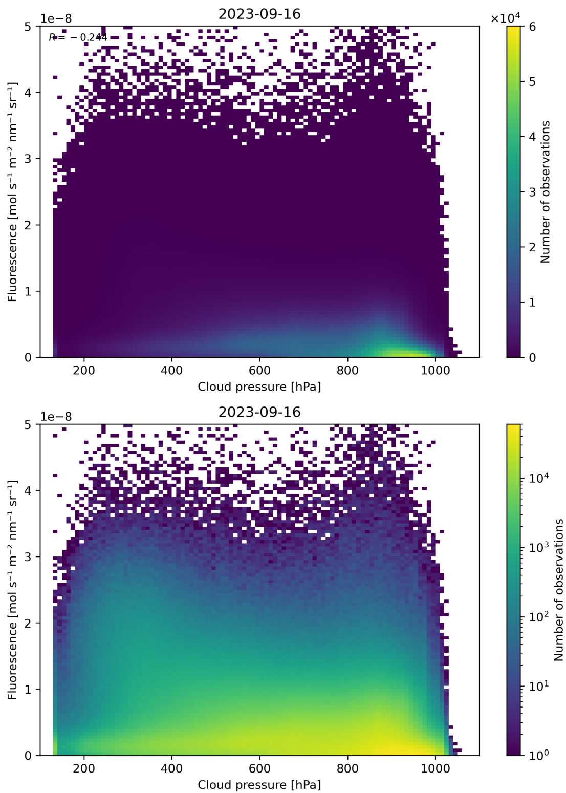
Figure 88: Scatter density plot of “Cloud pressure” against “Fluorescence” for 2023-09-15 to 2023-09-17.
