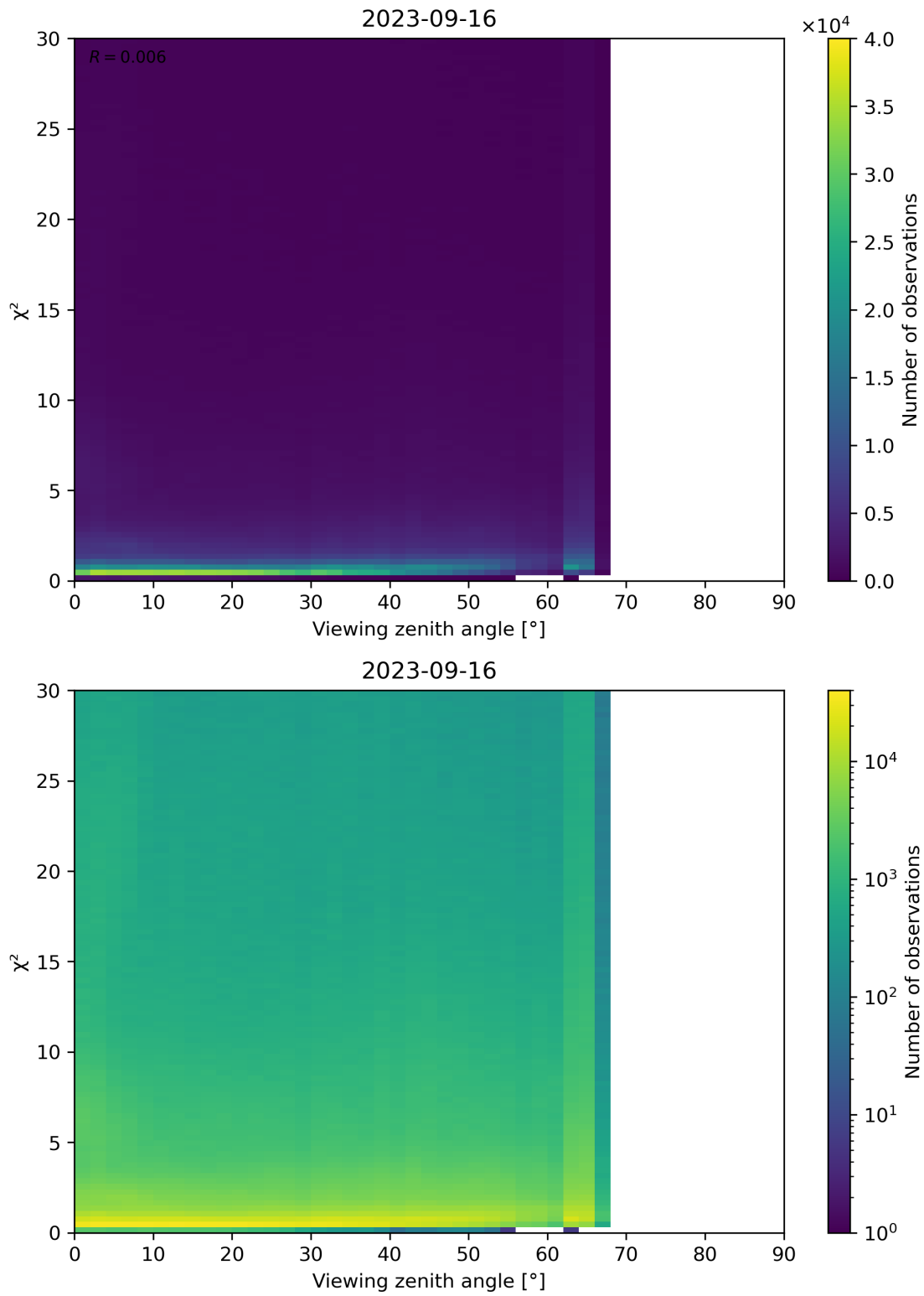
Figure 130: Scatter density plot of “Viewing zenith angle” against “ \chi^2 ” for 2023-09-15 to 2023-09-17.
