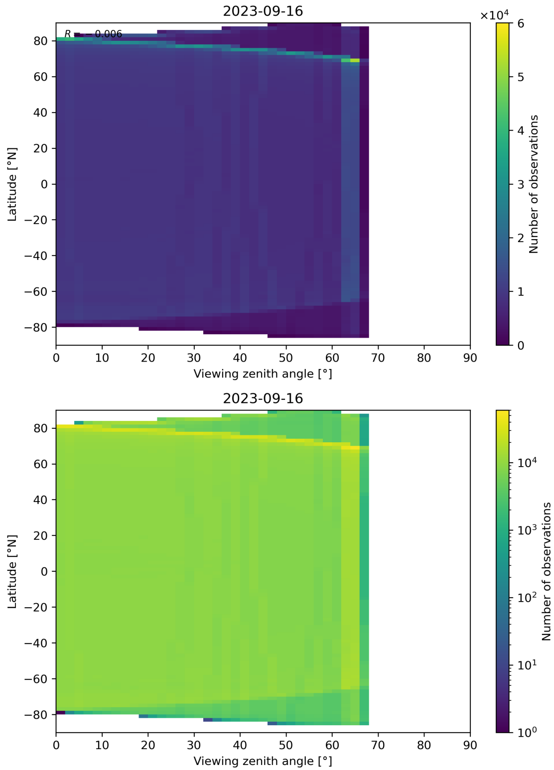
Figure 135: Scatter density plot of “Viewing zenith angle” against “Latitude” for 2023-09-15 to 2023-09-17.
