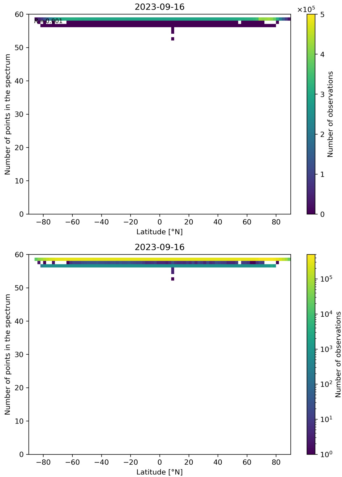
Figure 103: Scatter density plot of “Latitude” against “Number of points in the spectrum” for 2023-09-15 to 2023-09-17.
