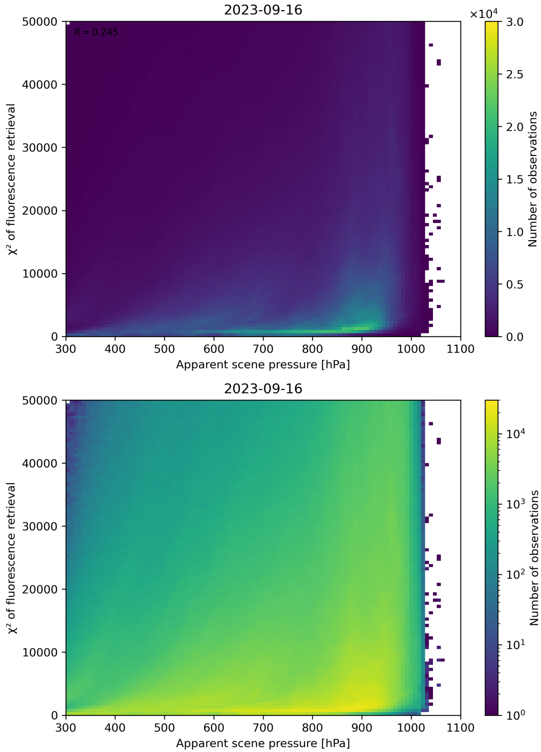
Figure 64: Scatter density plot of “Apparent scene pressure” against “ \chi^2 of fluorescence retrieval” for 2023-09-15 to 2023-09-17.
