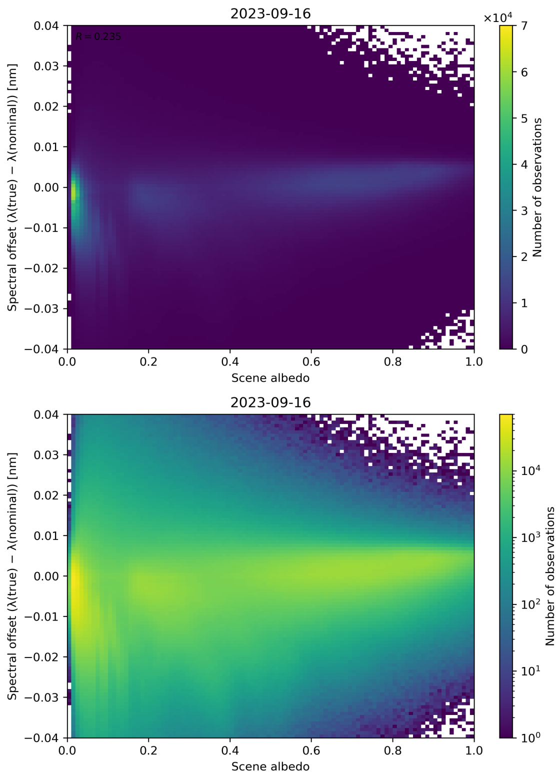
Figure 117: Scatter density plot of “Scene albedo” against “Spectral offset ( \lambda(\text{true}) - \lambda(\text{nominal}) )” for 2023-09-15 to 2023-09-17.
