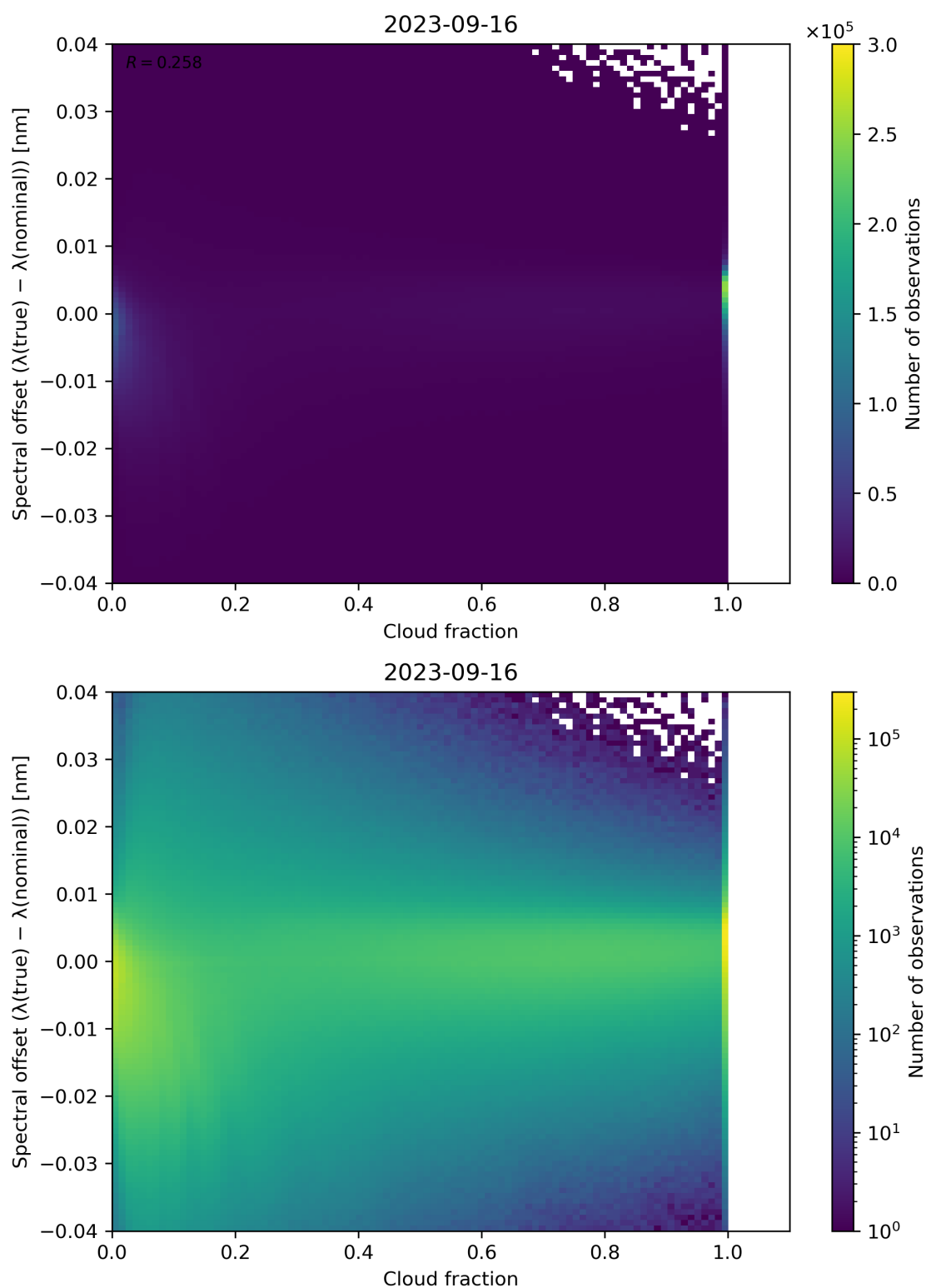
Figure 83: Scatter density plot of “Cloud fraction” against “Spectral offset ( \lambda(\text{true}) - \lambda(\text{nominal}) )” for 2023-09-15 to 2023-09-17.
