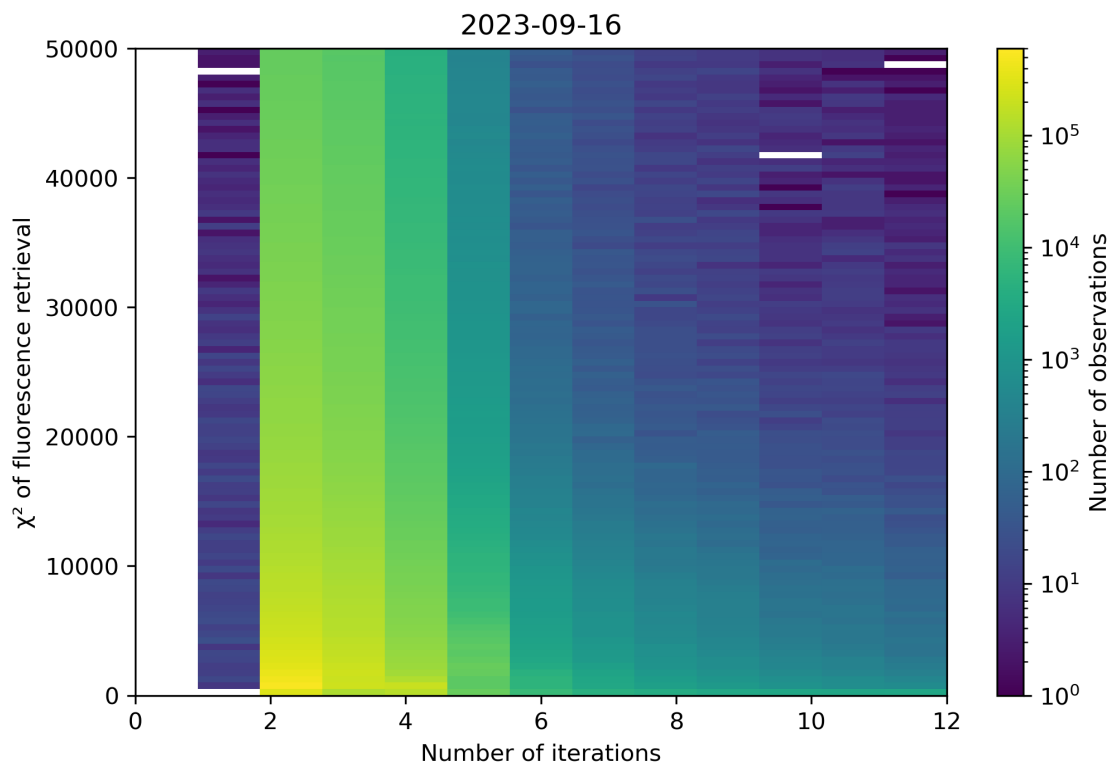
Figure 106: Scatter density plot of “Number of iterations” against “ \chi^2 of fluorescence retrieval” for 2023-09-15 to 2023-09-17.
