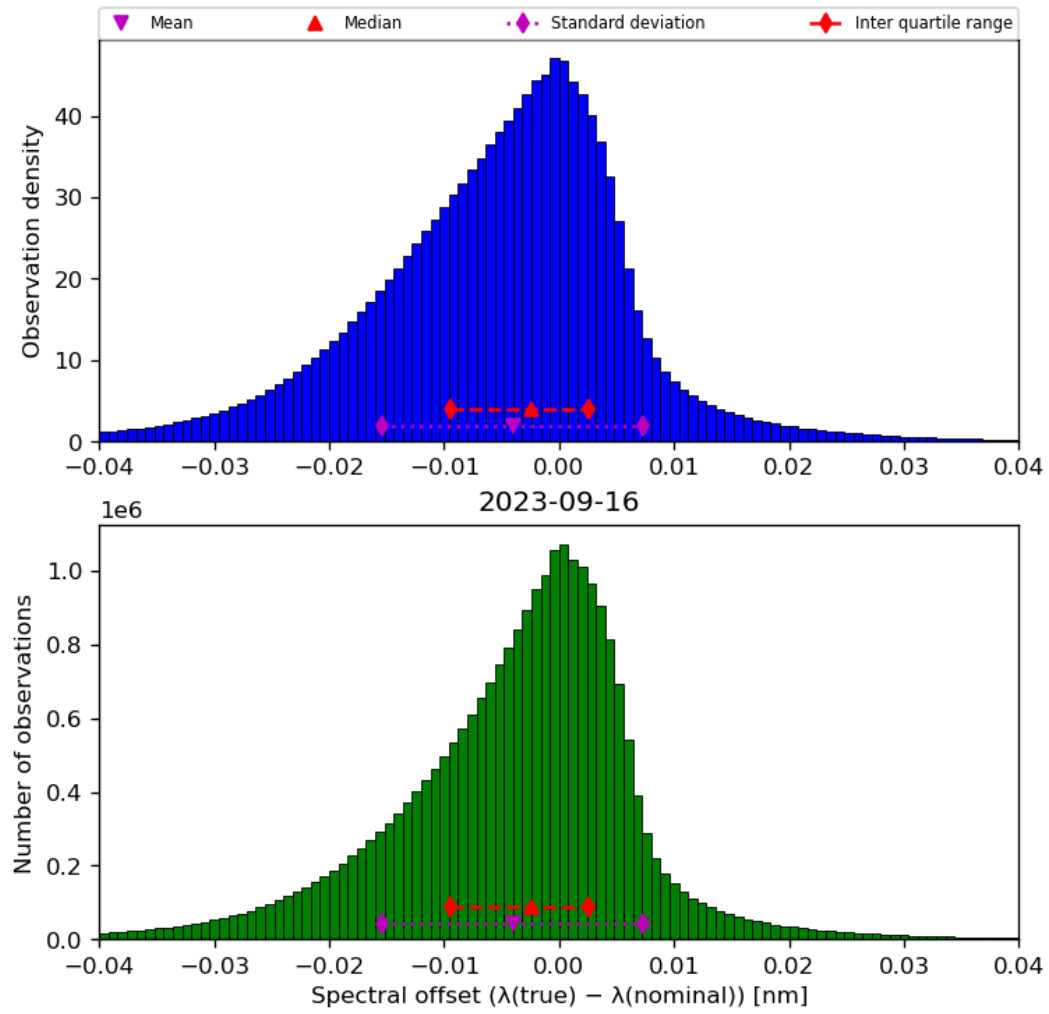
Figure 45: Histogram of “Spectral offset ( \lambda(\text{true}) - \lambda(\text{nominal}) )” for 2023-09-15 to 2023-09-17
