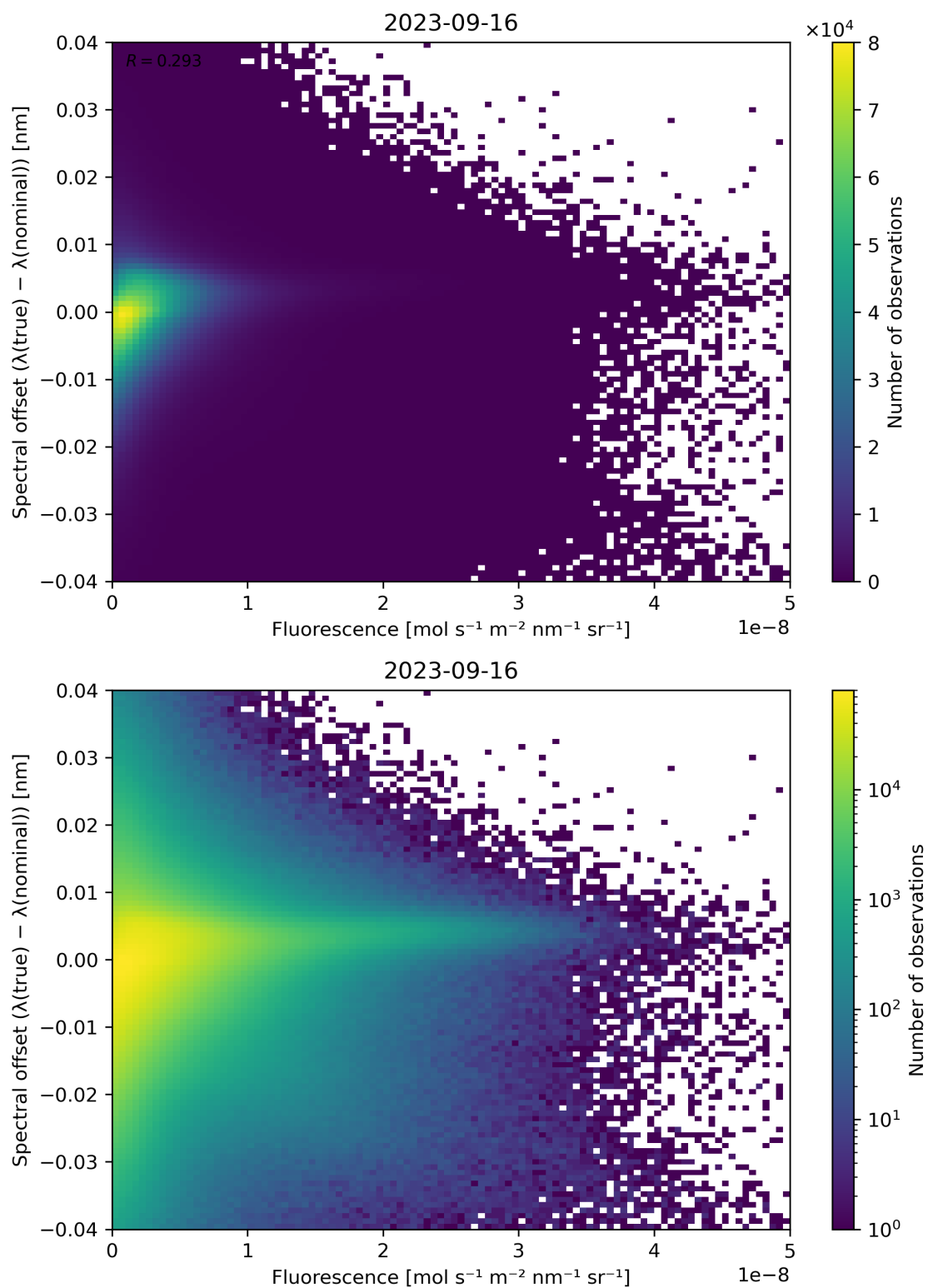
Figure 95: Scatter density plot of “Fluorescence” against “Spectral offset ( \lambda(\text{true}) - \lambda(\text{nominal}) )” for 2023-09-15 to 2023-09-17.
