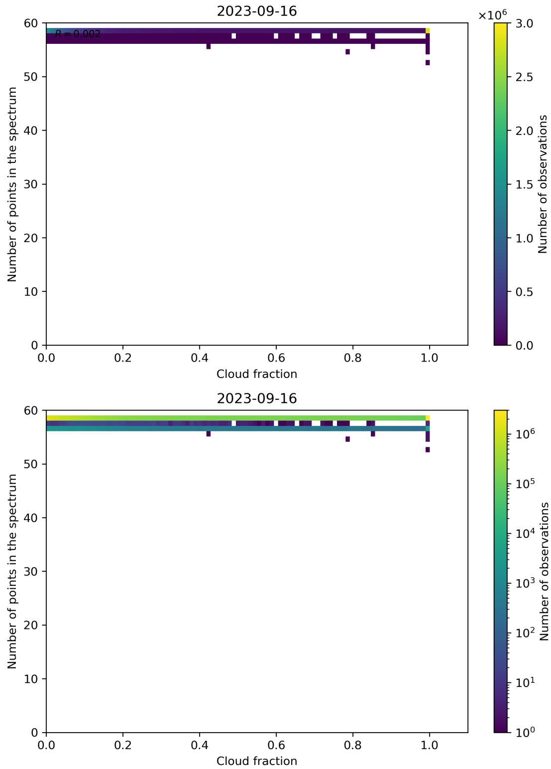
Figure 81: Scatter density plot of “Cloud fraction” against “Number of points in the spectrum” for 2023-09-15 to 2023-09-17.
