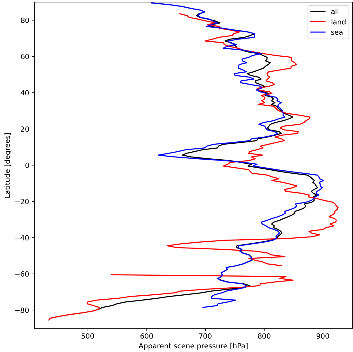
Figure 19: Zonal average of “Apparent scene pressure” for 2023-09-15 to 2023-09-17.
