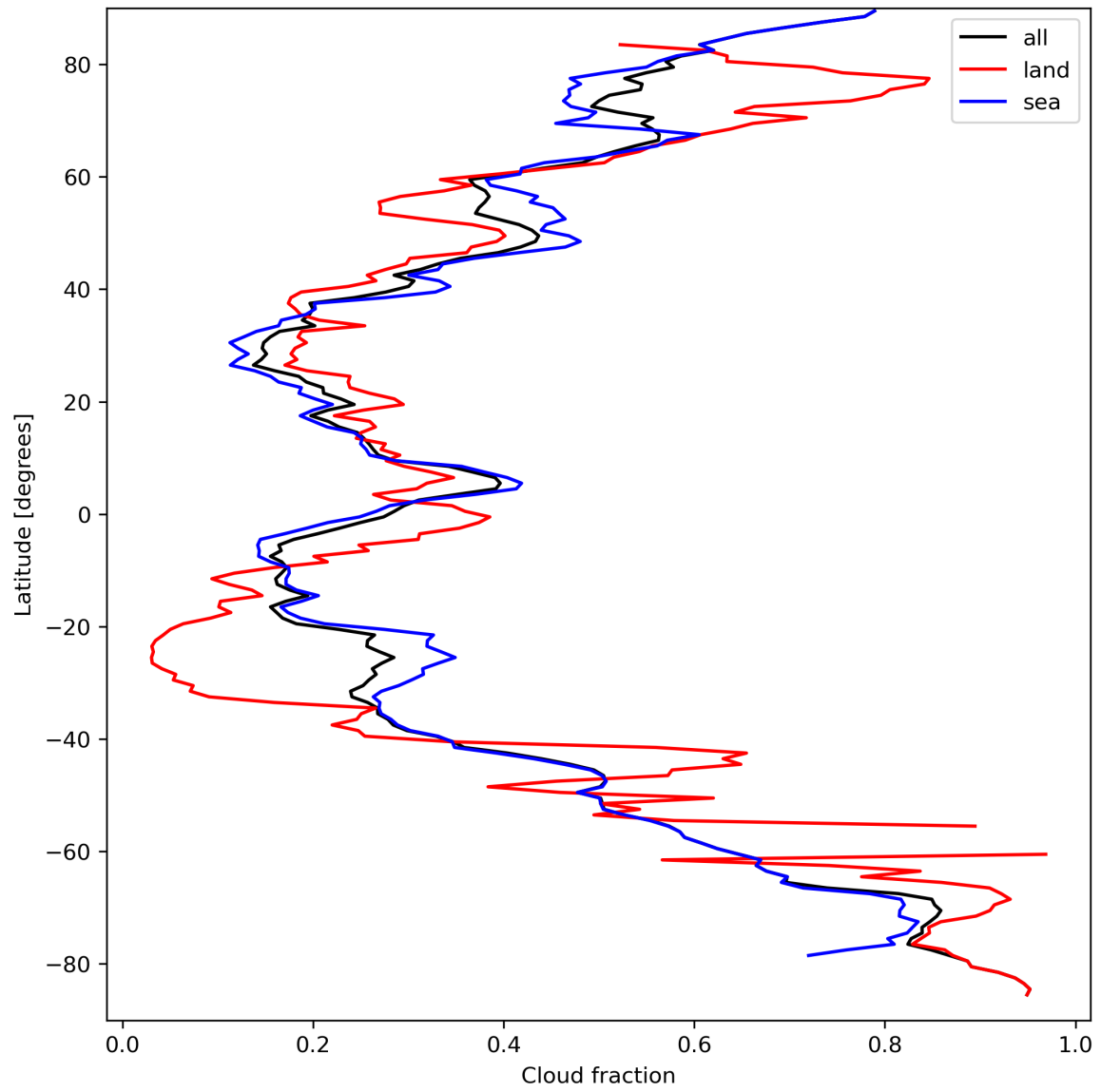
Figure 15: Zonal average of “Cloud fraction” for 2023-09-15 to 2023-09-17.
