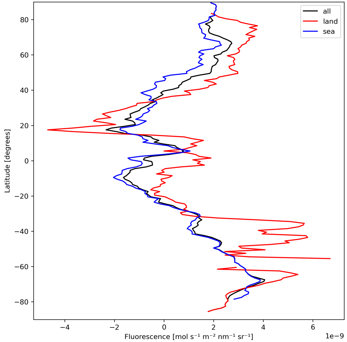
Figure 23: Zonal average of “Fluorescence” for 2023-09-15 to 2023-09-17.
