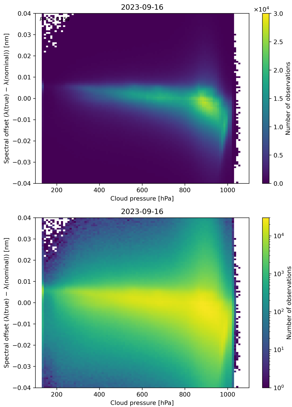
Figure 92: Scatter density plot of “Cloud pressure” against “Spectral offset ( \lambda(\text{true}) - \lambda(\text{nominal}) )” for 2023-09-15 to 2023-09-17.
