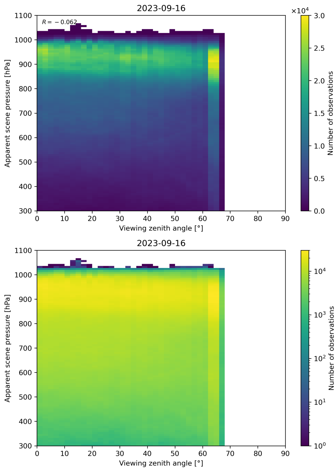
Figure 129: Scatter density plot of “Viewing zenith angle” against “Apparent scene pressure” for 2023-09-15 to 2023-09-17.
