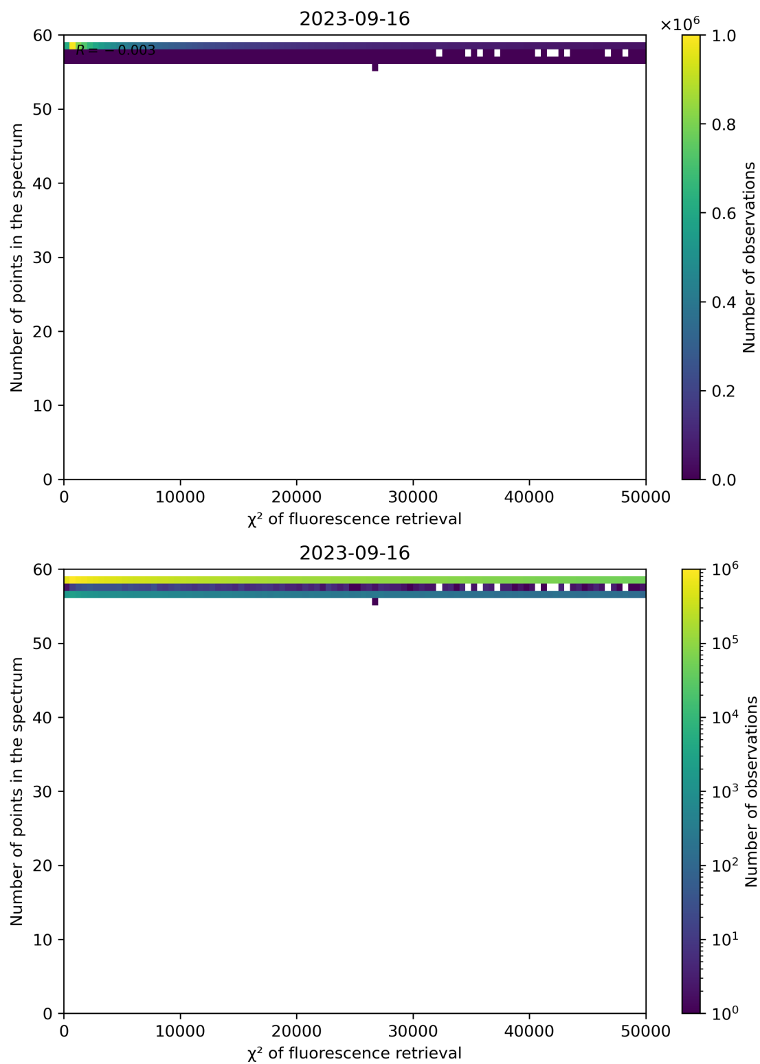
Figure 71: Scatter density plot of “ \chi^2 of fluorescence retrieval” against “Number of points in the spectrum” for 2023-09-15 to 2023-09-17.
