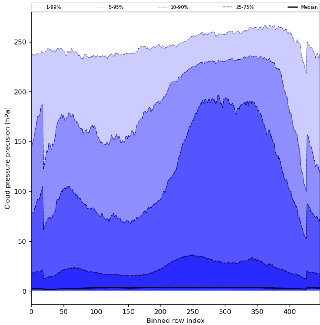
Figure 48: Along track statistics of “Cloud pressure precision” for 2023-09-15 to 2023-09-17
