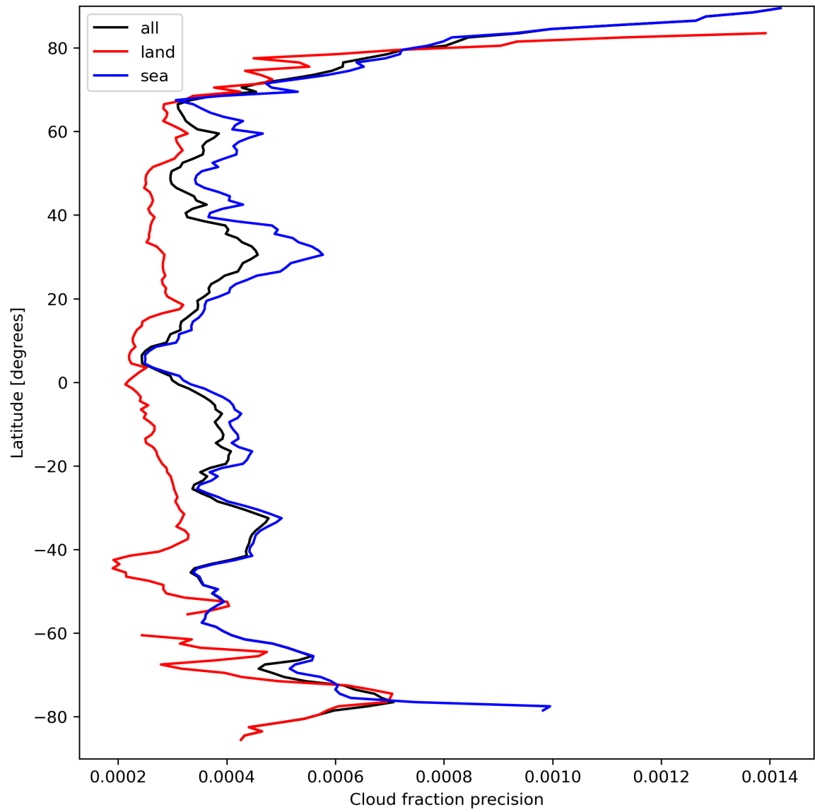
Figure 16: Zonal average of “Cloud fraction precision” for 2023-09-15 to 2023-09-17.
