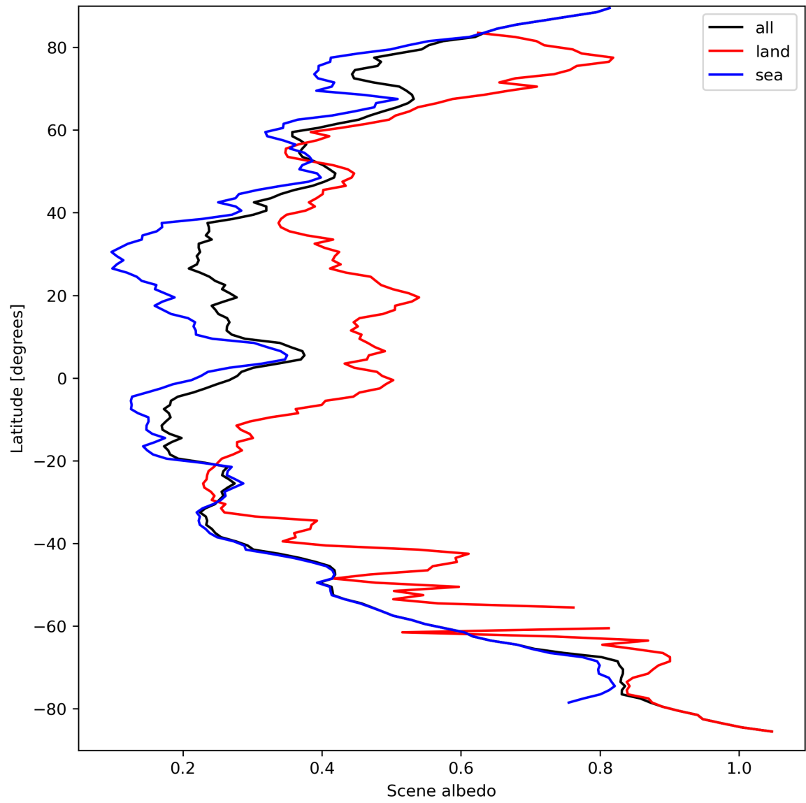
Figure 17: Zonal average of “Scene albedo” for 2023-09-15 to 2023-09-17.
