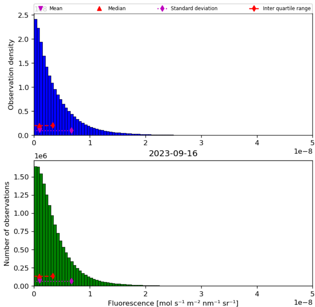
Figure 40: Histogram of “Fluorescence” for 2023-09-15 to 2023-09-17
