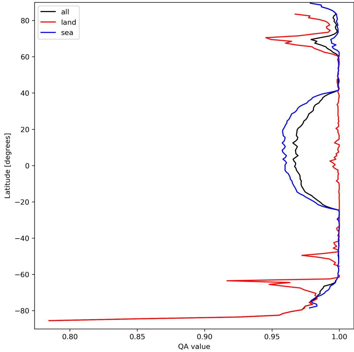
Figure 12: Zonal average of “QA value” for 2023-09-15 to 2023-09-17.
