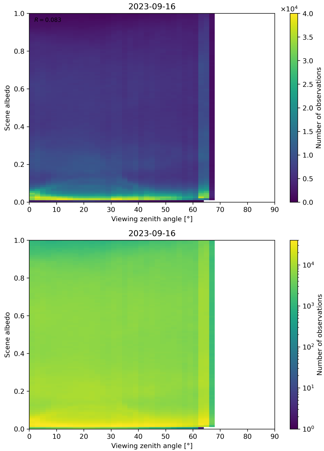
Figure 138: Scatter density plot of “Viewing zenith angle” against “Scene albedo” for 2023-09-15 to 2023-09-17.
