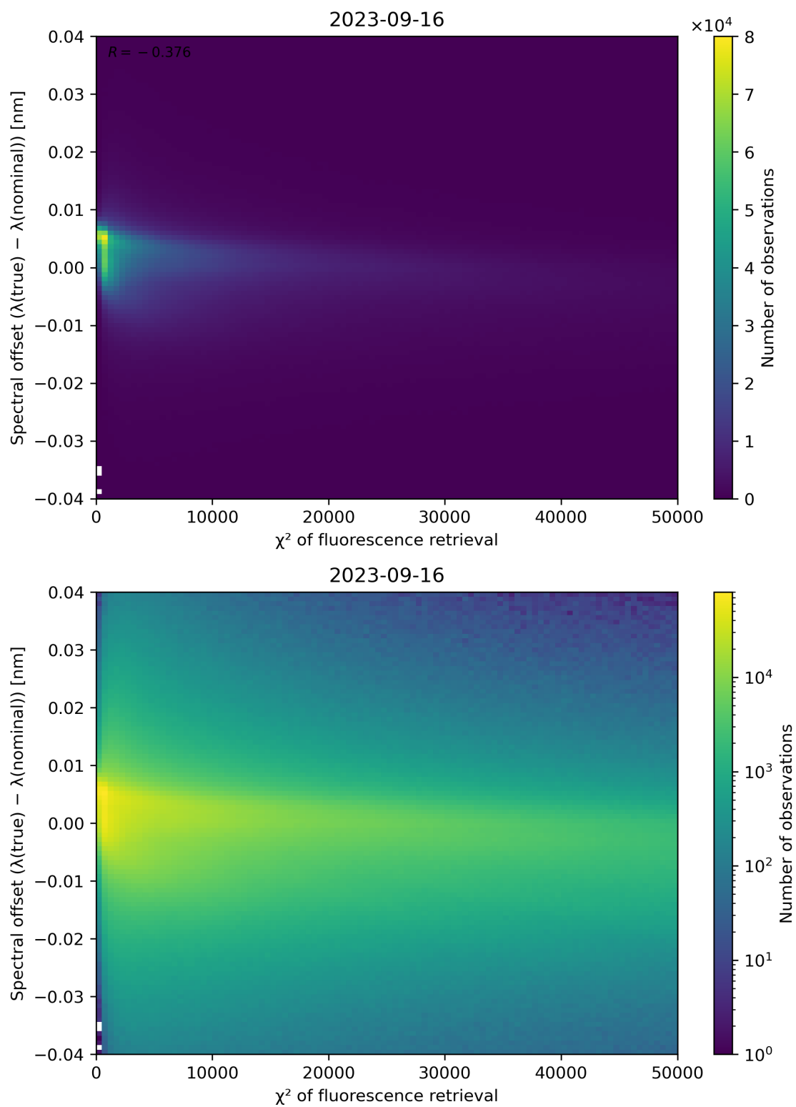
Figure 72: Scatter density plot of “ \chi^2 of fluorescence retrieval” against “Spectral offset ( \lambda(\text{true}) - \lambda(\text{nominal}) )” for 2023-09-15 to 2023-09-17.
