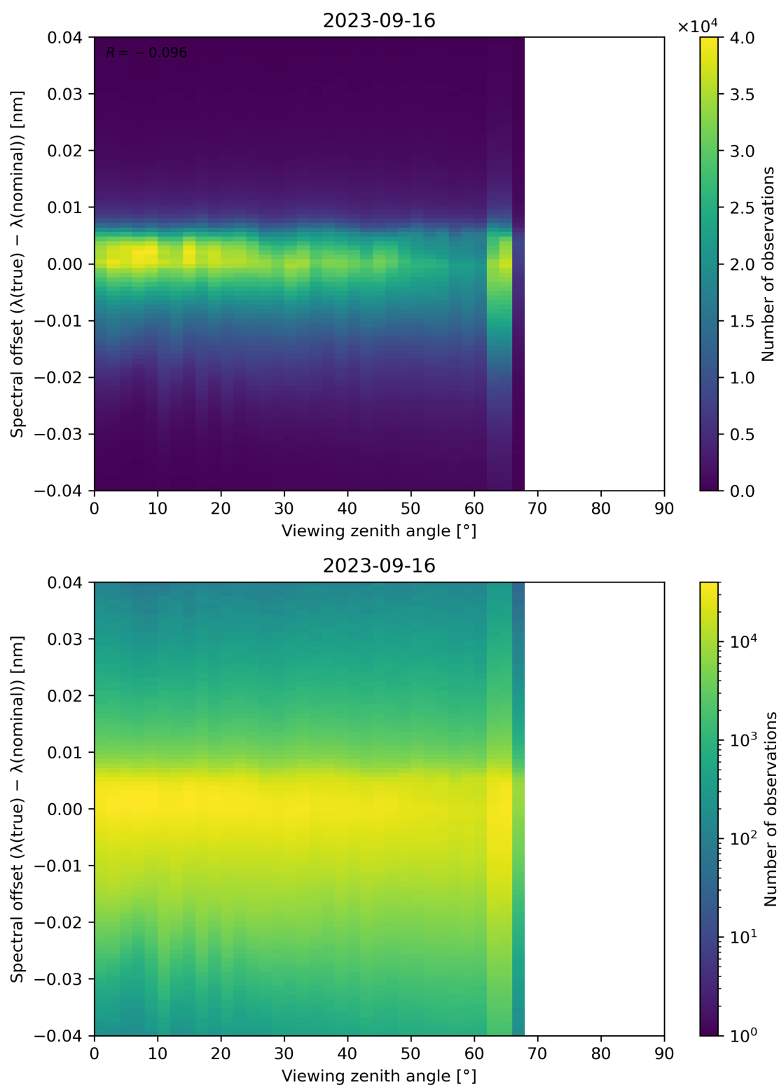
Figure 140: Scatter density plot of “Viewing zenith angle” against “Spectral offset ( \lambda(\text{true}) - \lambda(\text{nominal}) )” for 2023-09-15 to 2023-09-17.
