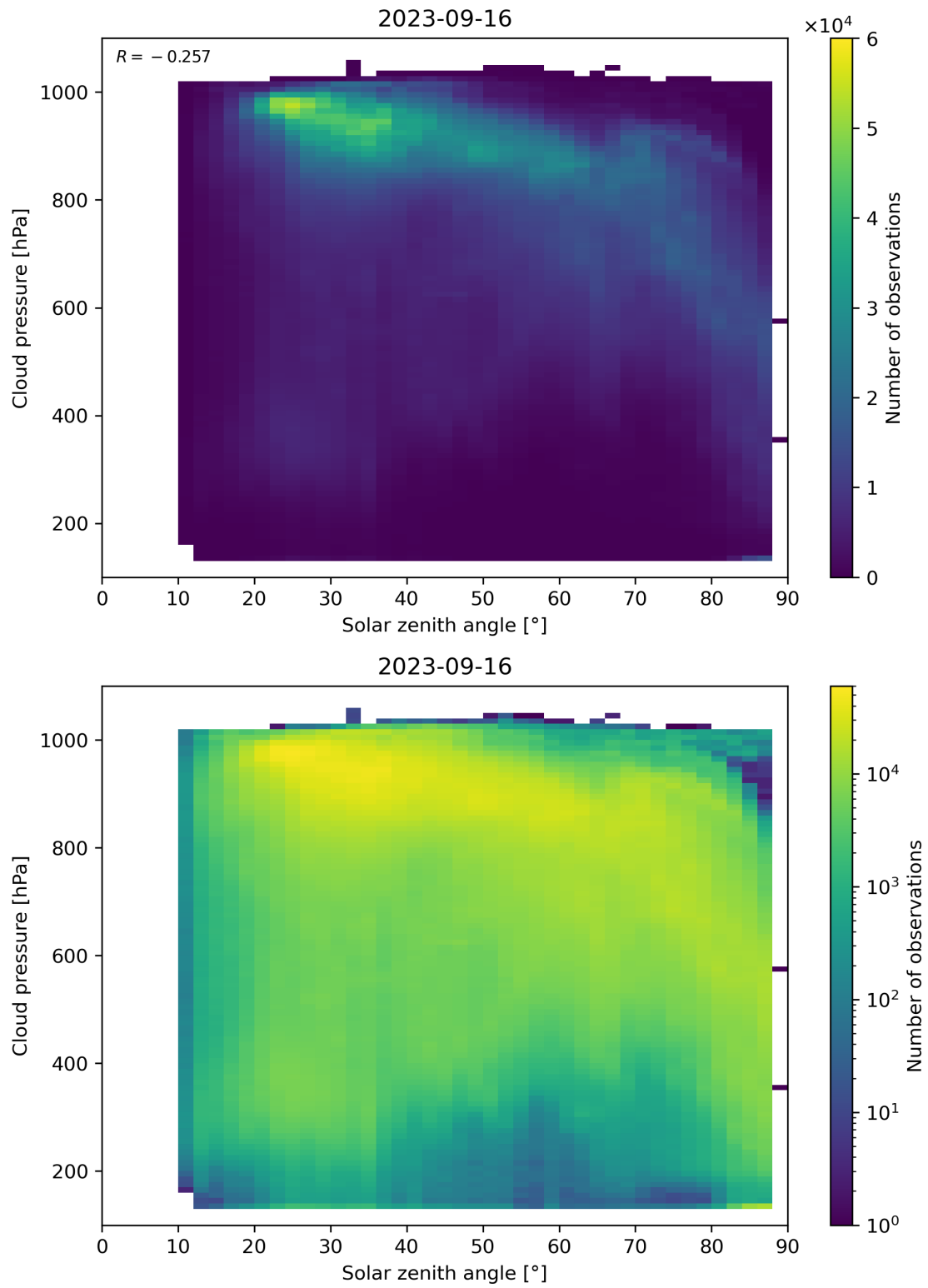
Figure 122: Scatter density plot of “Solar zenith angle” against “Cloud pressure” for 2023-09-15 to 2023-09-17.
