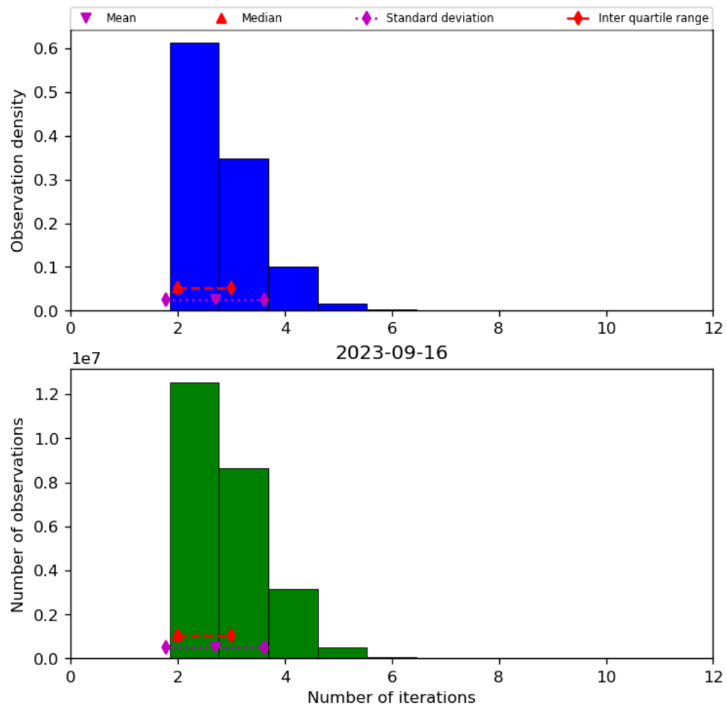
Figure 39: Histogram of “Number of iterations” for 2023-09-15 to 2023-09-17
