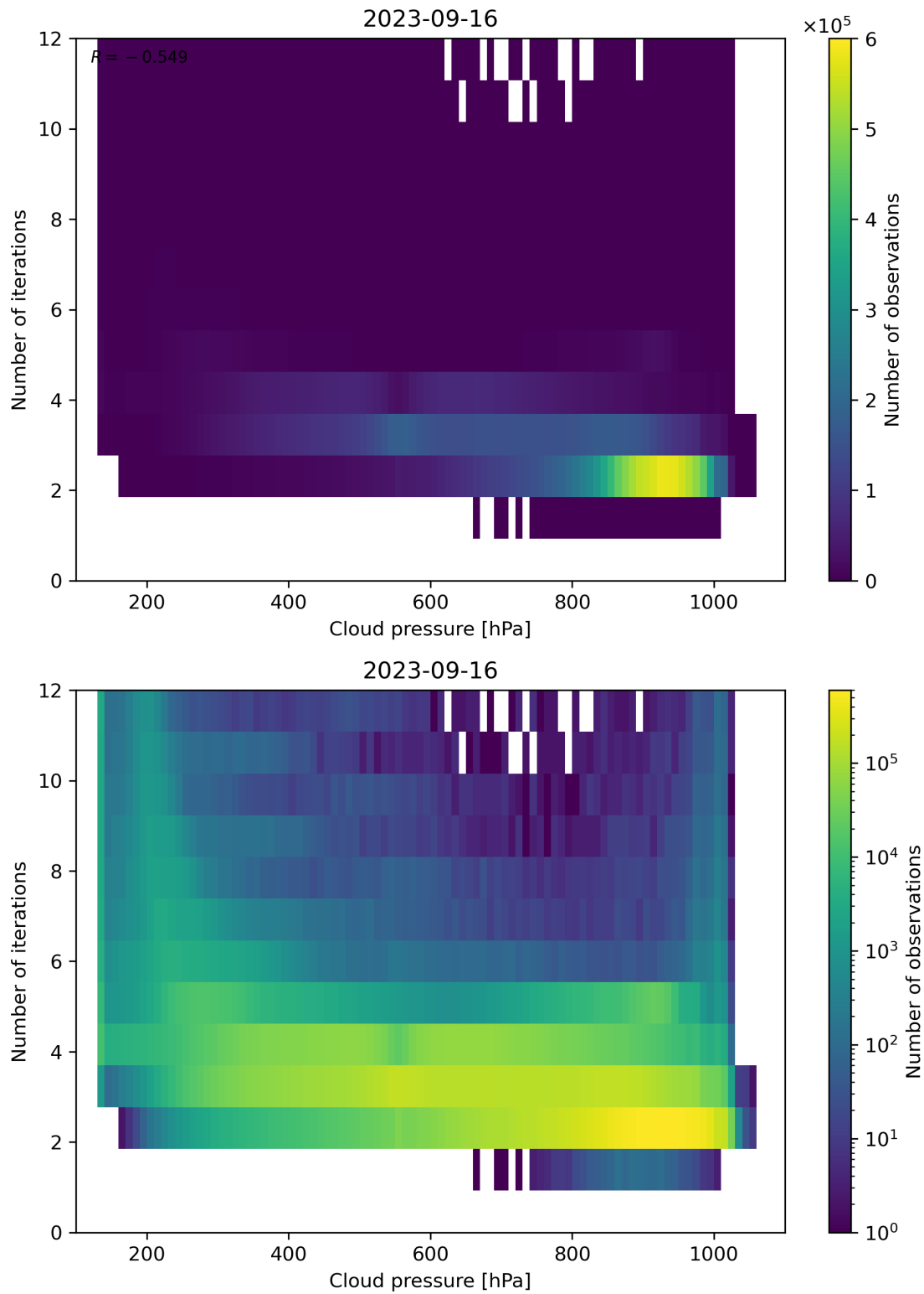
Figure 89: Scatter density plot of “Cloud pressure” against “Number of iterations” for 2023-09-15 to 2023-09-17.
