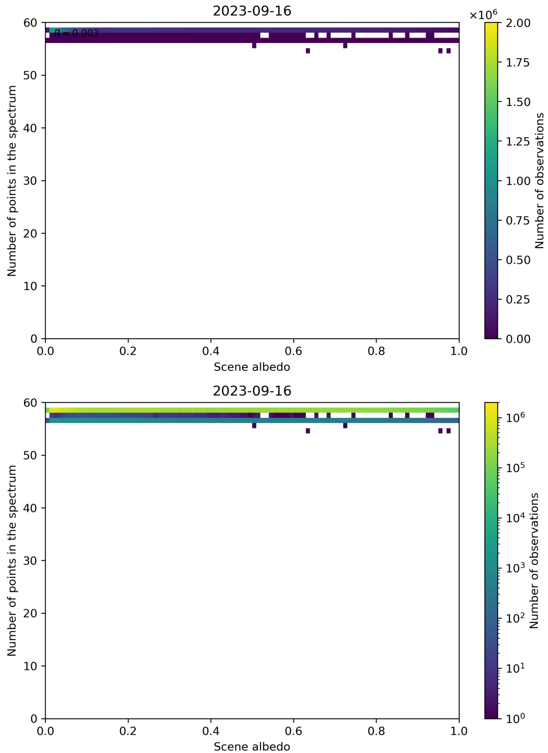
Figure 116: Scatter density plot of “Scene albedo” against “Number of points in the spectrum” for 2023-09-15 to 2023-09-17.
