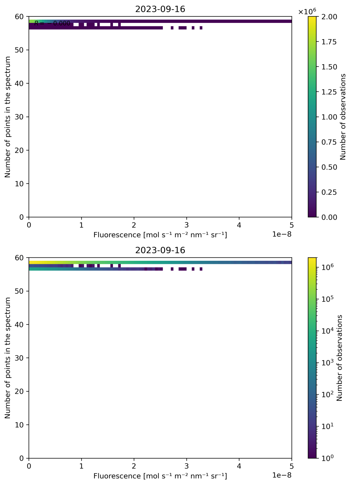
Figure 94: Scatter density plot of “Fluorescence” against “Number of points in the spectrum” for 2023-09-15 to 2023-09-17.
