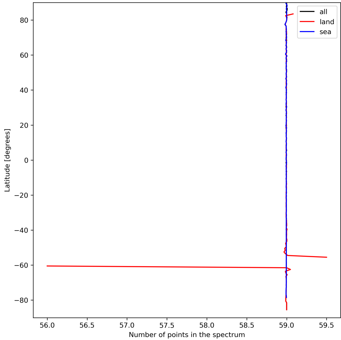
Figure 27: Zonal average of “Number of points in the spectrum” for 2023-09-15 to 2023-09-17.
