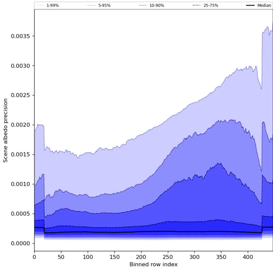
Figure 52: Along track statistics of “Scene albedo precision” for 2023-09-15 to 2023-09-17
