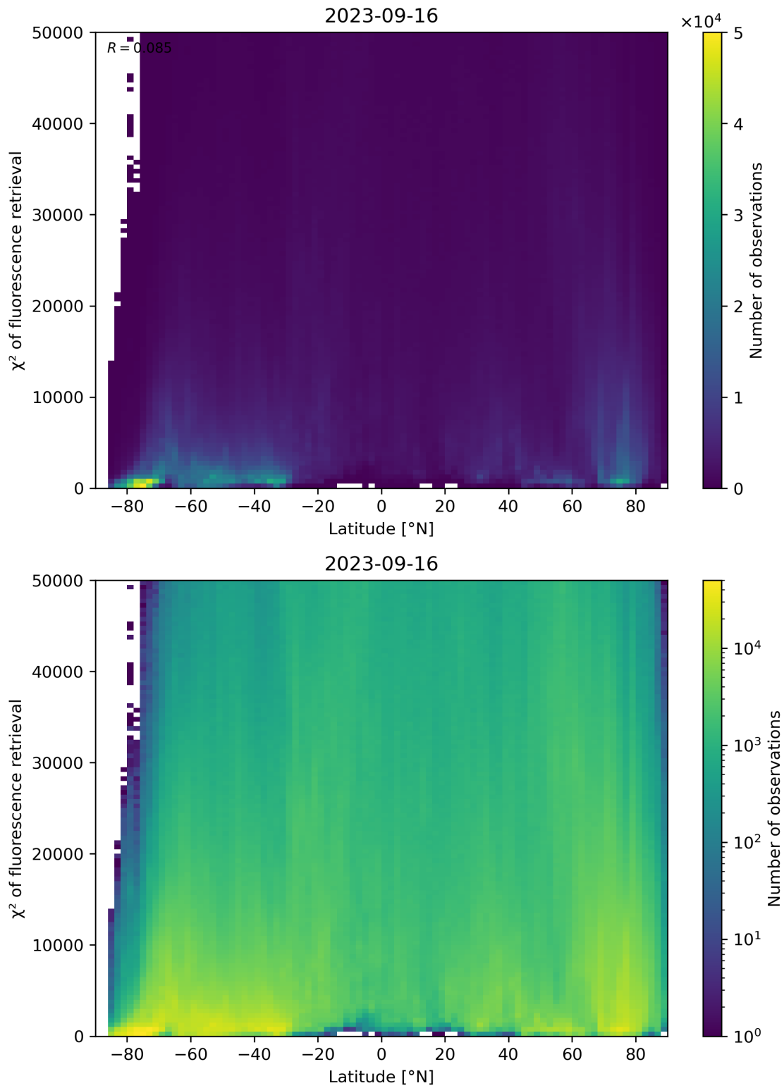
Figure 98: Scatter density plot of “Latitude” against “ \chi^2 of fluorescence retrieval” for 2023-09-15 to 2023-09-17.
