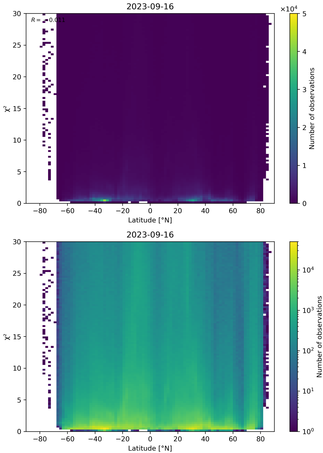
Figure 97: Scatter density plot of “Latitude” against “ \chi^2 ” for 2023-09-15 to 2023-09-17.
