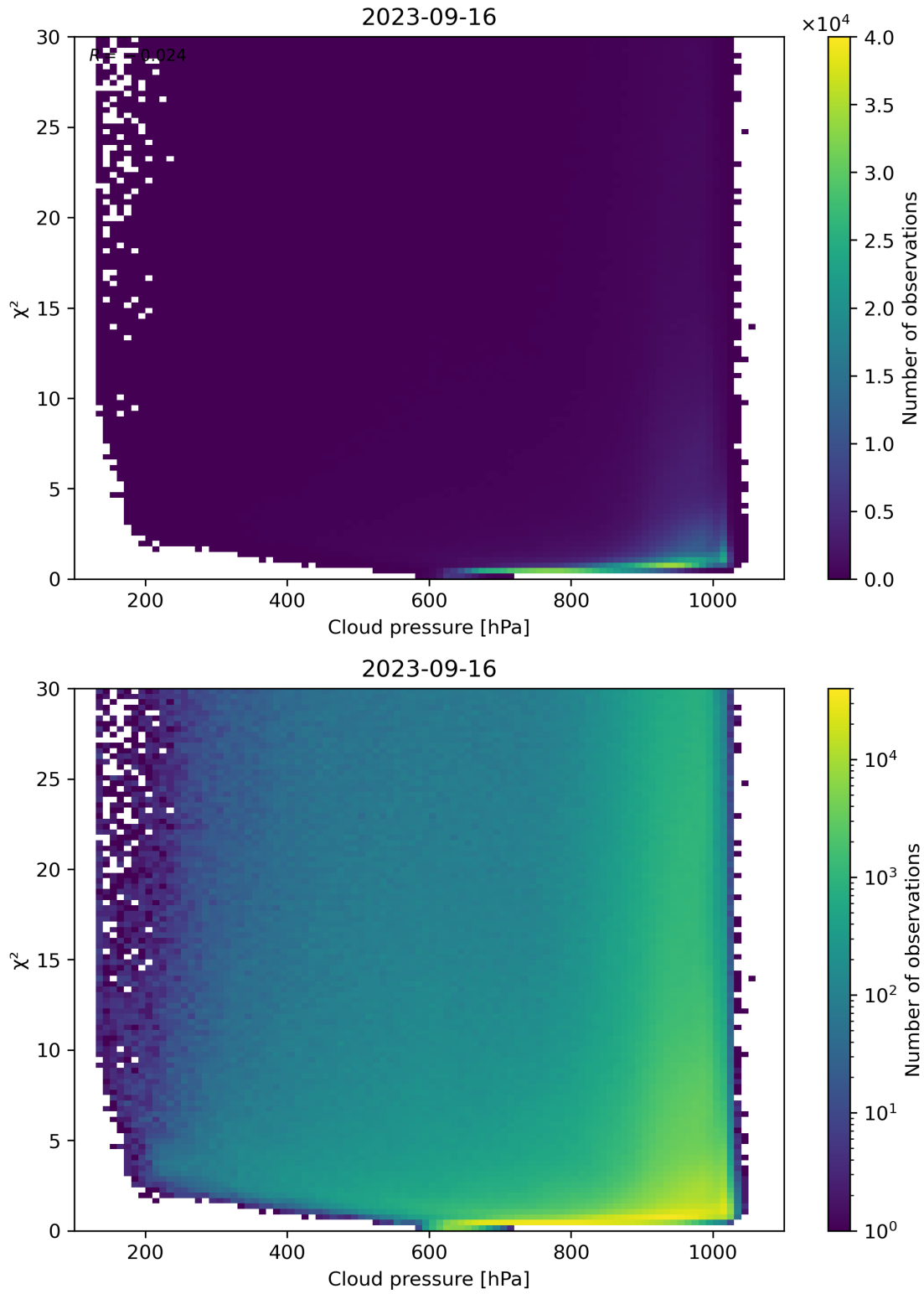
Figure 85: Scatter density plot of “Cloud pressure” against “ \chi^2 ” for 2023-09-15 to 2023-09-17.
