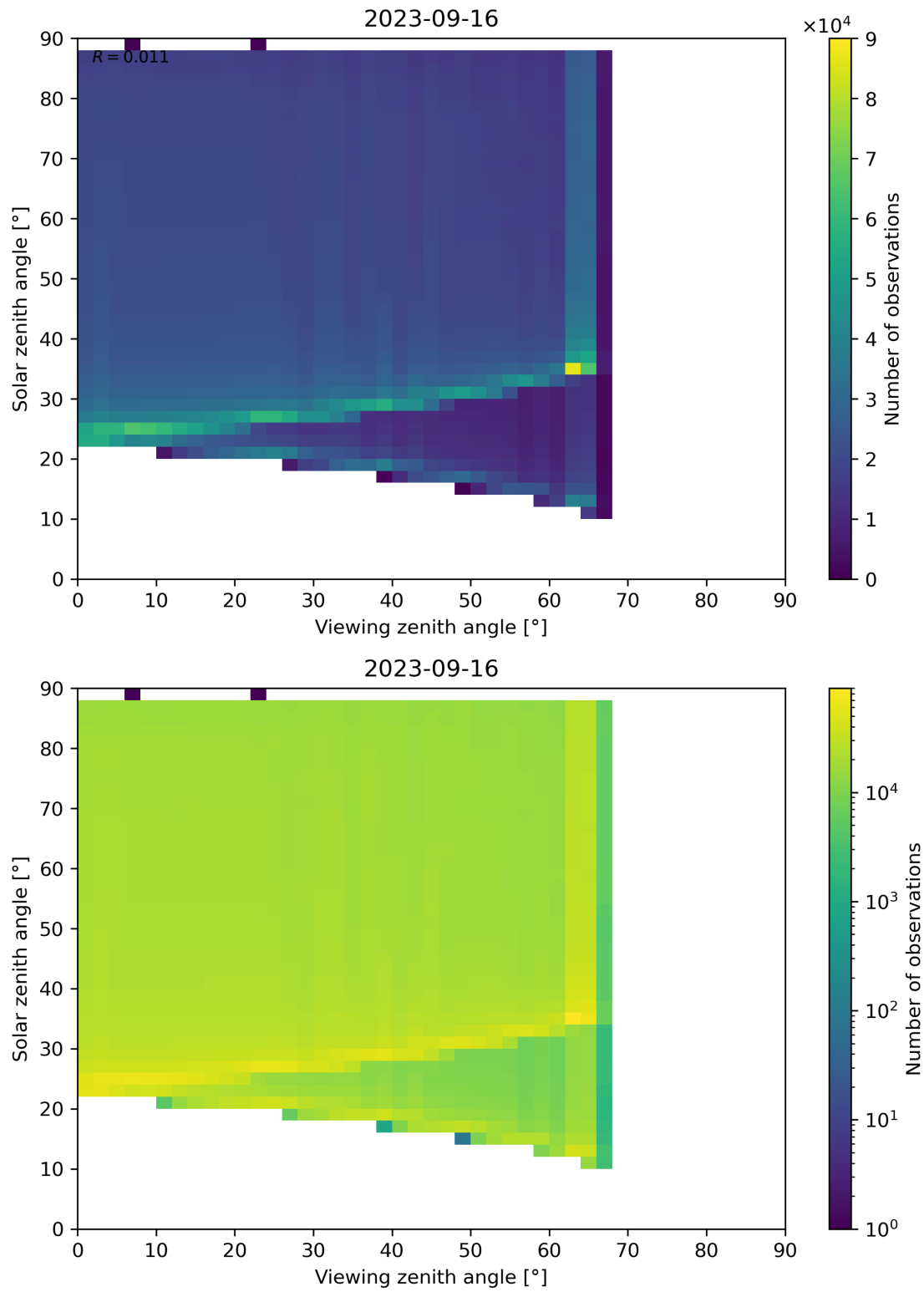
Figure 139: Scatter density plot of “Viewing zenith angle” against “Solar zenith angle” for 2023-09-15 to 2023-09-17.
