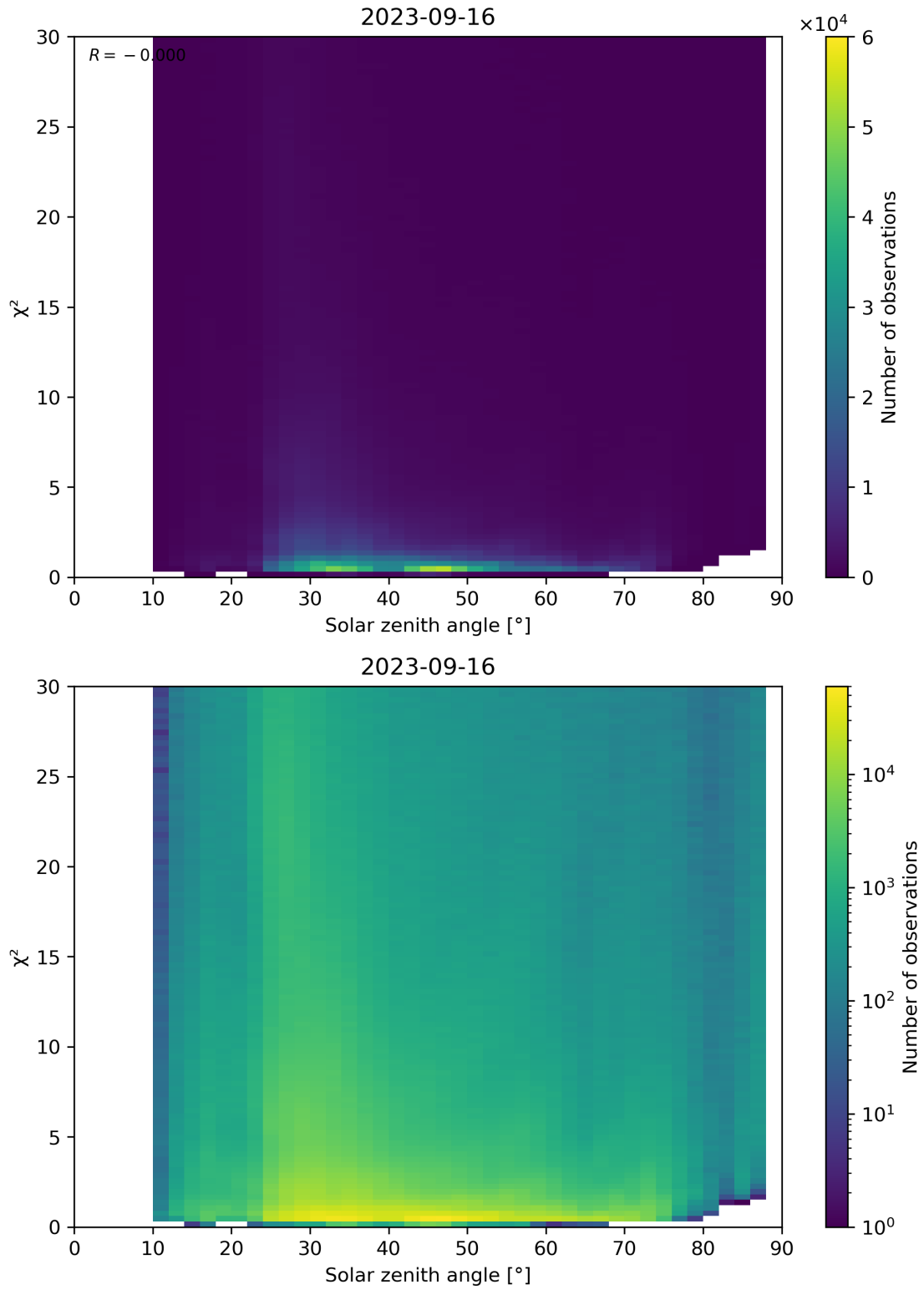
Figure 119: Scatter density plot of “Solar zenith angle” against “ \chi^2 ” for 2023-09-15 to 2023-09-17.
