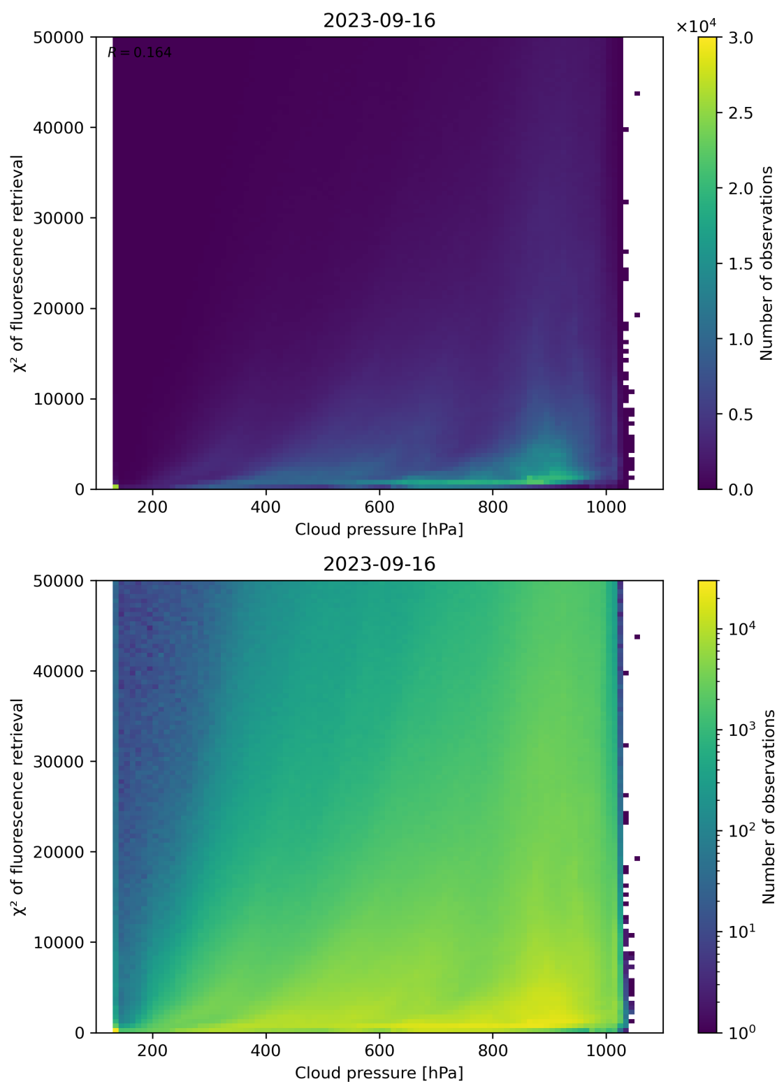
Figure 86: Scatter density plot of “Cloud pressure” against “ \chi^2 of fluorescence retrieval” for 2023-09-15 to 2023-09-17.
