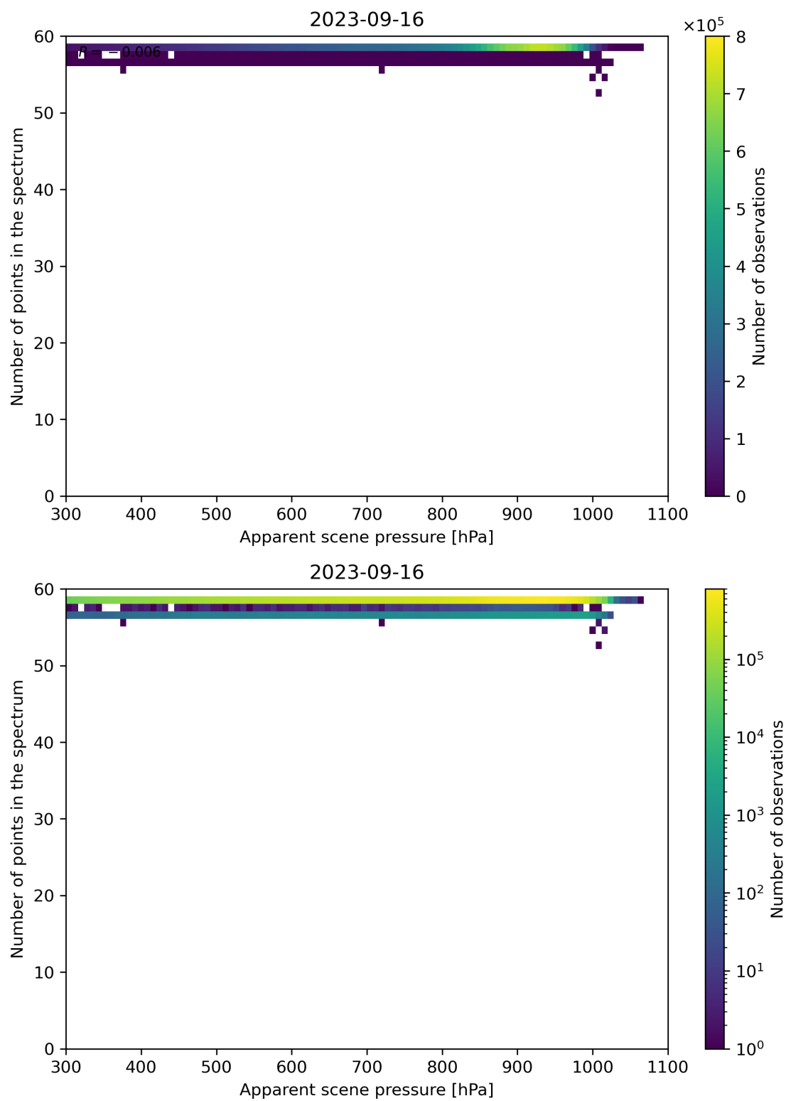
Figure 67: Scatter density plot of “Apparent scene pressure” against “Number of points in the spectrum” for 2023-09-15 to 2023-09-17.
