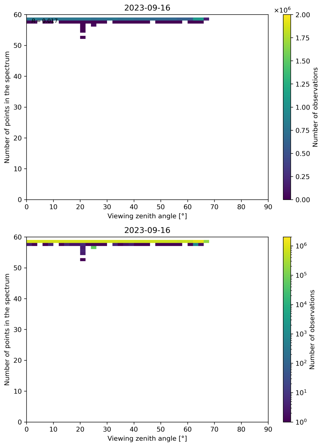
Figure 137: Scatter density plot of “Viewing zenith angle” against “Number of points in the spectrum” for 2023-09-15 to 2023-09-17.
