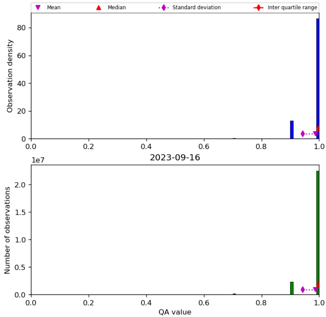
Figure 29: Histogram of “QA value” for 2023-09-15 to 2023-09-17
