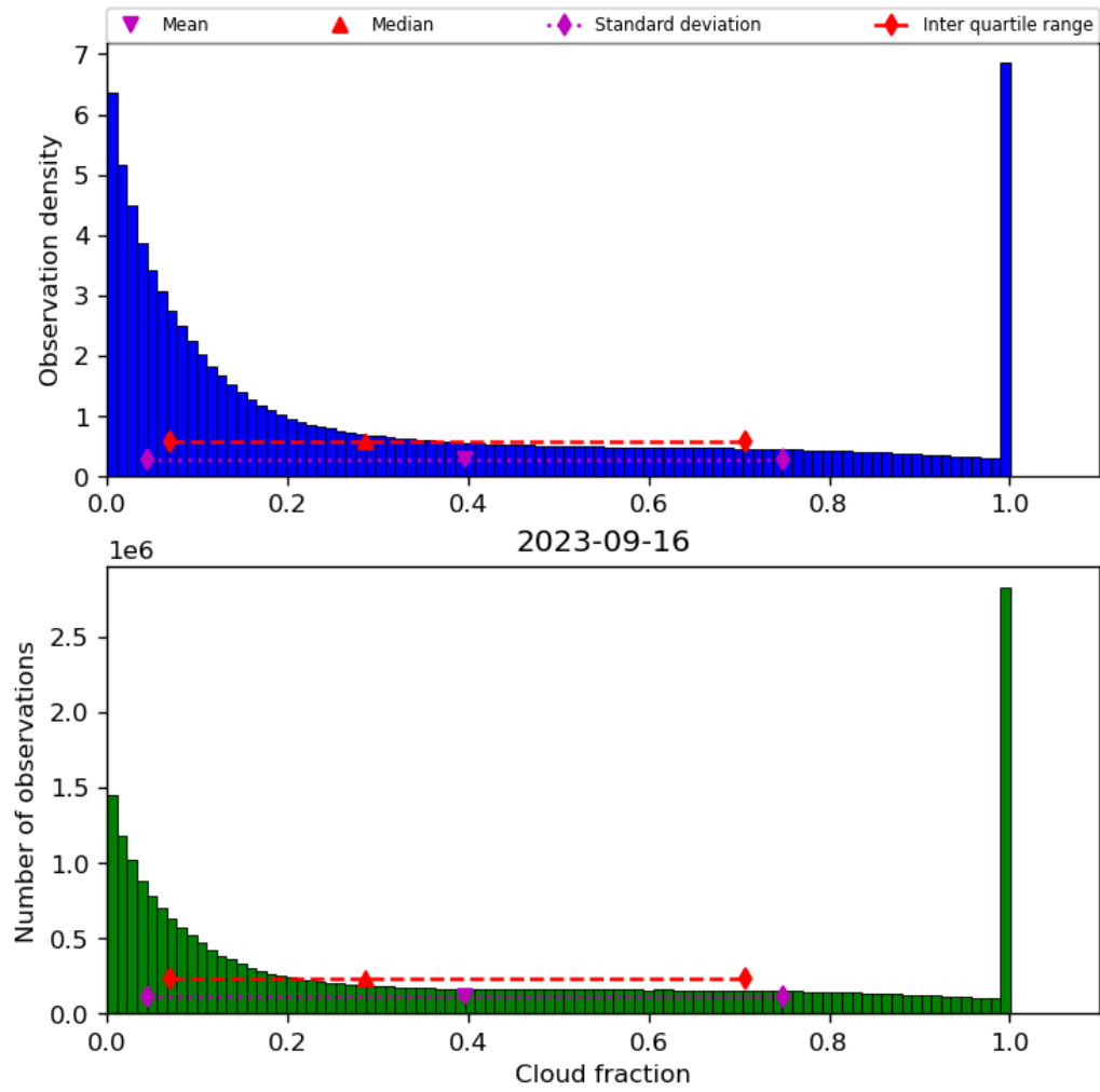
Figure 32: Histogram of “Cloud fraction” for 2023-09-15 to 2023-09-17
