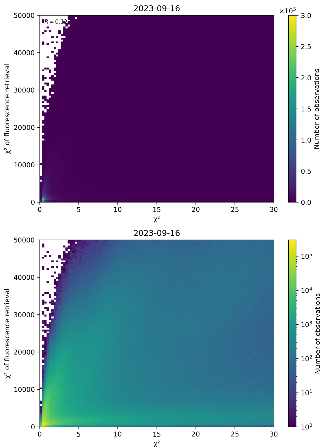
Figure 69: Scatter density plot of “ \chi^2 ” against “ \chi^2 of fluorescence retrieval” for 2023-09-15 to 2023-09-17.
