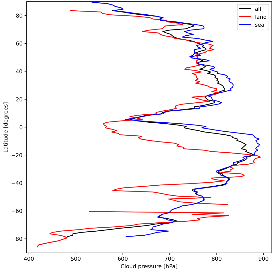
Figure 13: Zonal average of “Cloud pressure” for 2023-09-15 to 2023-09-17.
