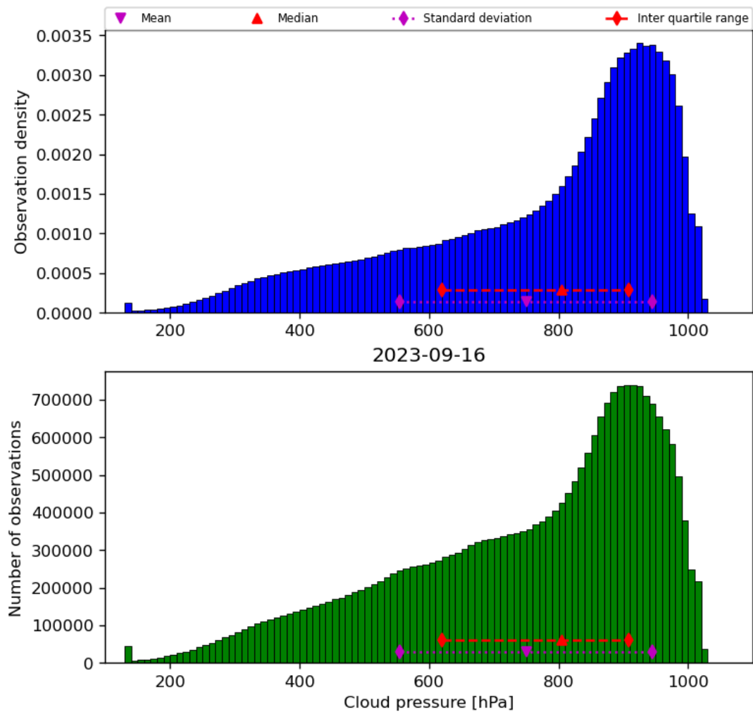
Figure 30: Histogram of “Cloud pressure” for 2023-09-15 to 2023-09-17
