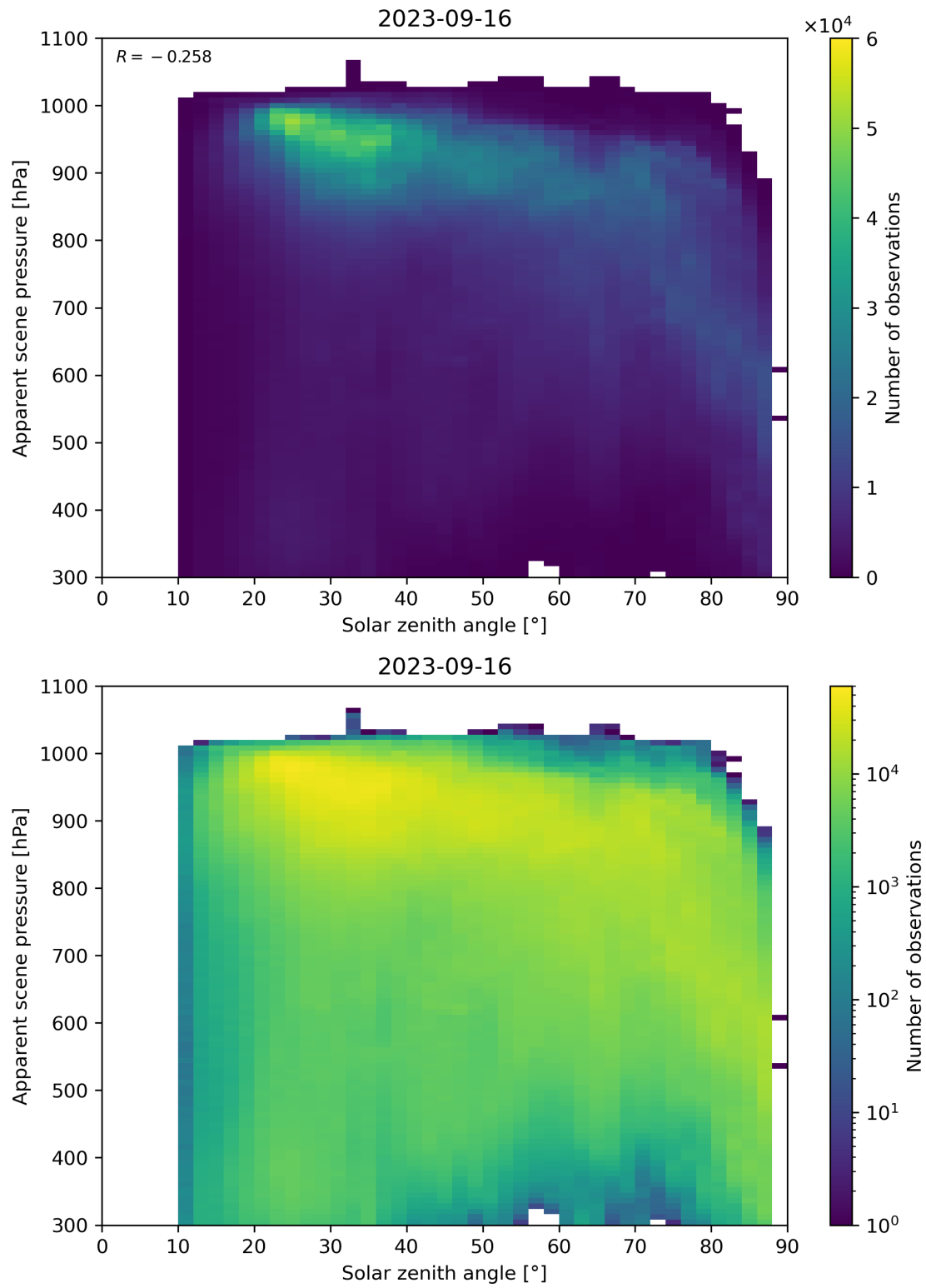
Figure 118: Scatter density plot of “Solar zenith angle” against “Apparent scene pressure” for 2023-09-15 to 2023-09-17.
