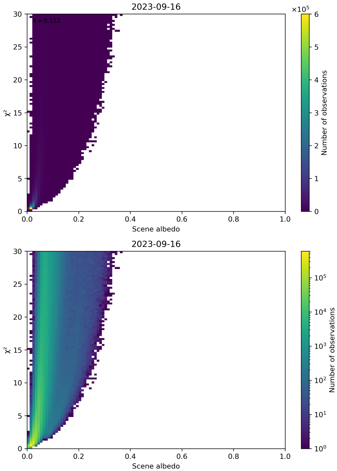
Figure 112: Scatter density plot of “Scene albedo” against “ \chi^2 ” for 2023-09-15 to 2023-09-17.
