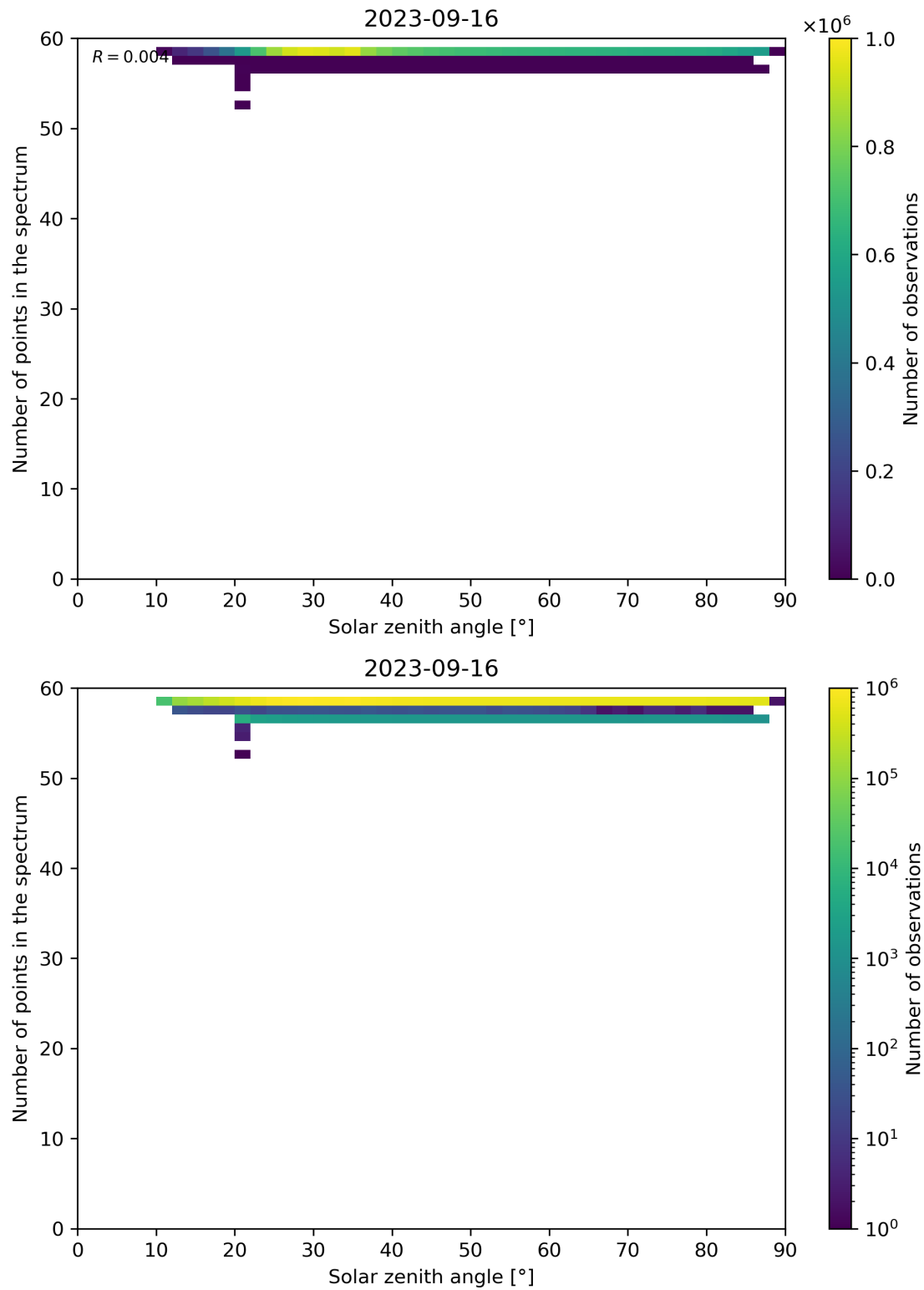
Figure 126: Scatter density plot of “Solar zenith angle” against “Number of points in the spectrum” for 2023-09-15 to 2023-09-17.
