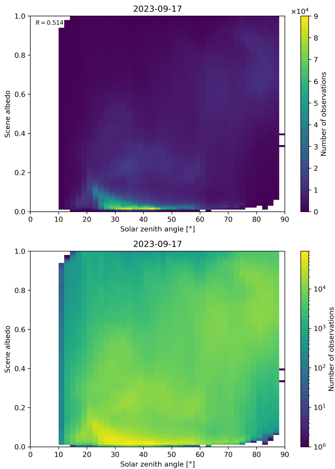
Figure 127: Scatter density plot of “Solar zenith angle” against “Scene albedo” for 2023-09-16 to 2023-09-18.
