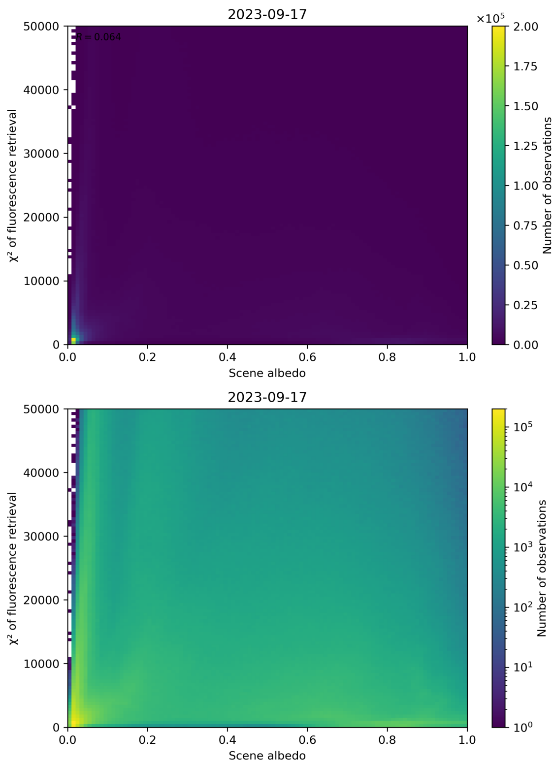
Figure 113: Scatter density plot of “Scene albedo” against “ \chi^2 of fluorescence retrieval” for 2023-09-16 to 2023-09-18.
