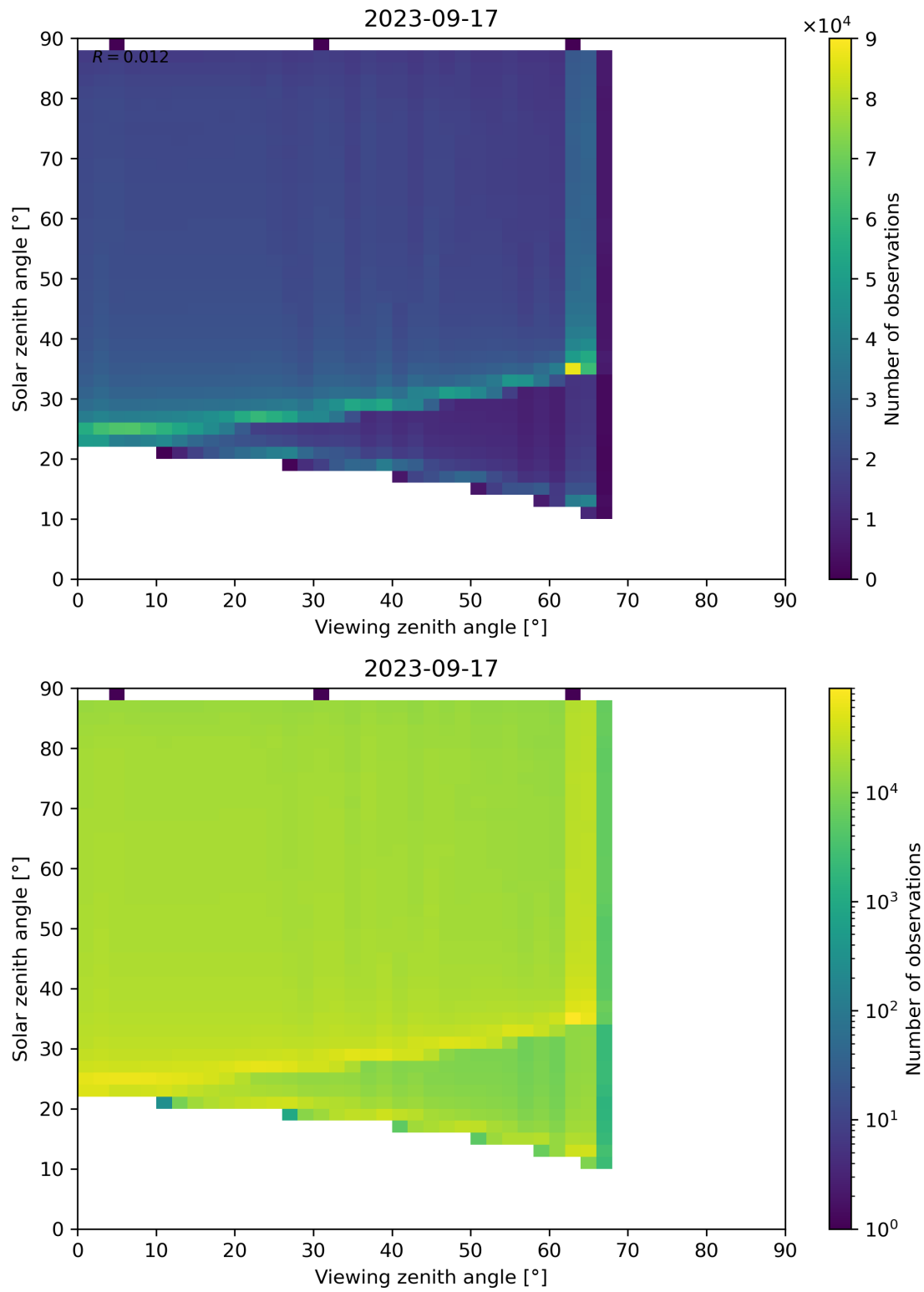
Figure 139: Scatter density plot of “Viewing zenith angle” against “Solar zenith angle” for 2023-09-16 to 2023-09-18.
