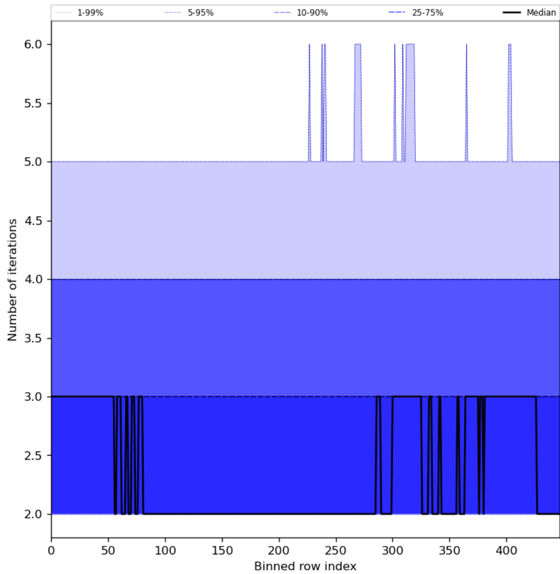
Figure 56: Along track statistics of "Number of iterations" for 2023-09-16 to 2023-09-18
