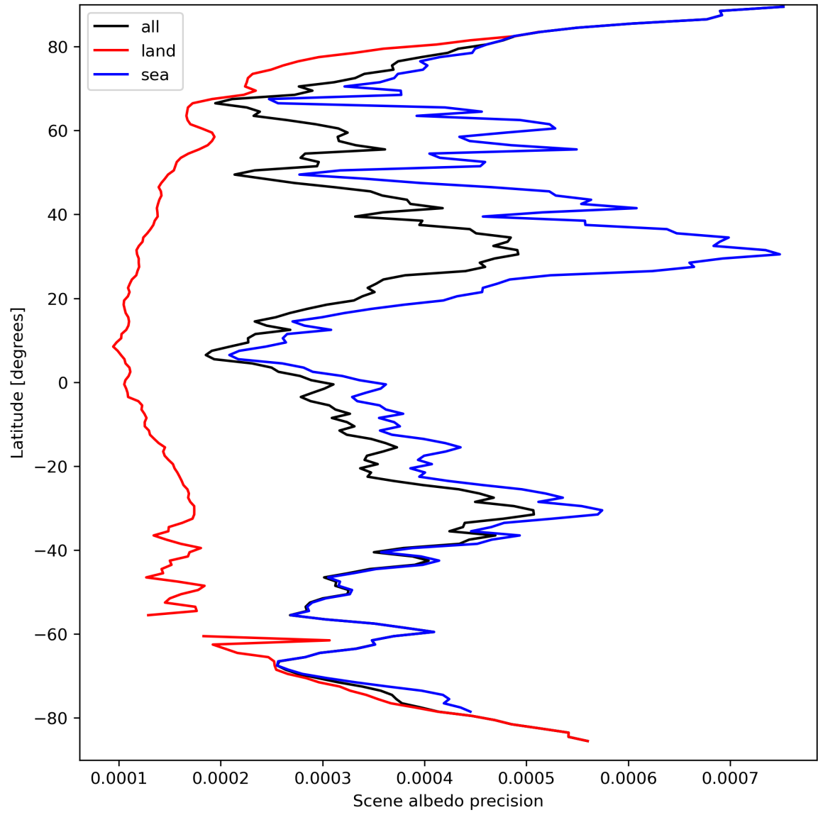
Figure 18: Zonal average of “Scene albedo precision” for 2023-09-16 to 2023-09-18.
