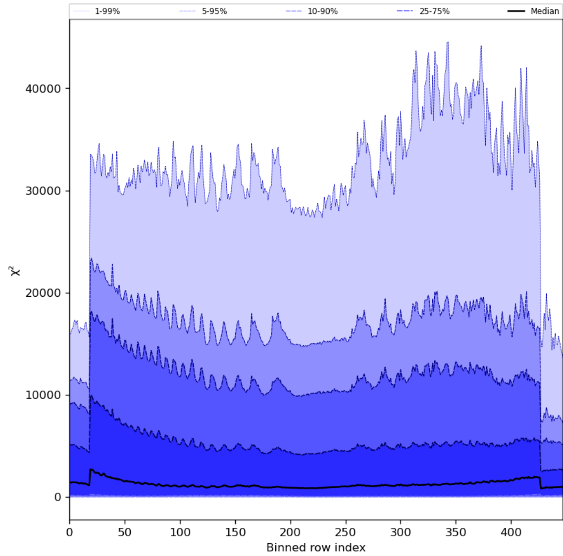
Figure 55: Along track statistics of “ \chi^2 ” for 2023-09-16 to 2023-09-18
