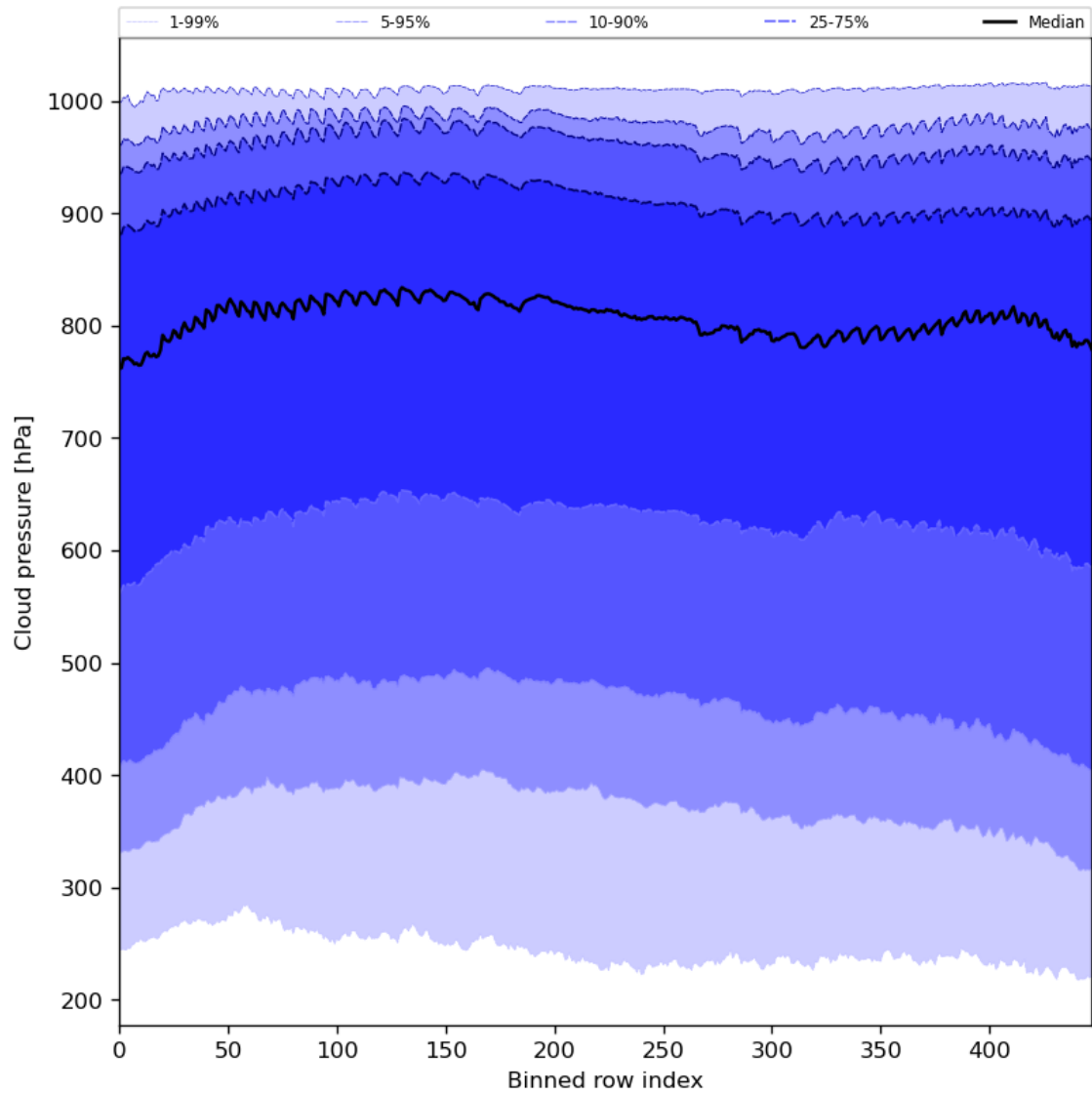
Figure 47: Along track statistics of “Cloud pressure” for 2023-09-16 to 2023-09-18
