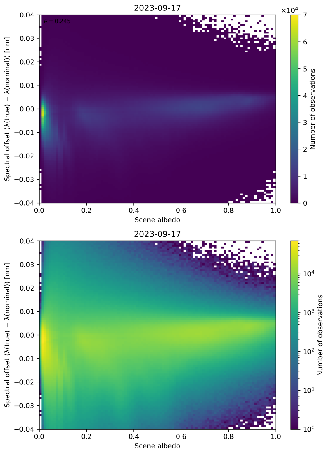
Figure 117: Scatter density plot of “Scene albedo” against “Spectral offset ( \lambda(\text{true}) - \lambda(\text{nominal}) )” for 2023-09-16 to 2023-09-18.
