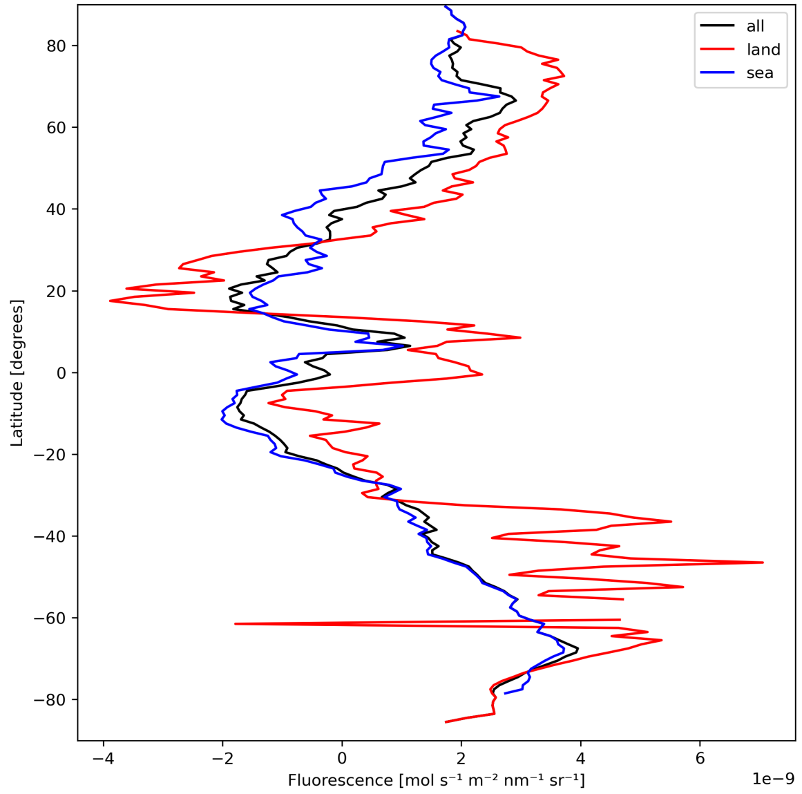
Figure 23: Zonal average of “Fluorescence” for 2023-09-16 to 2023-09-18.
