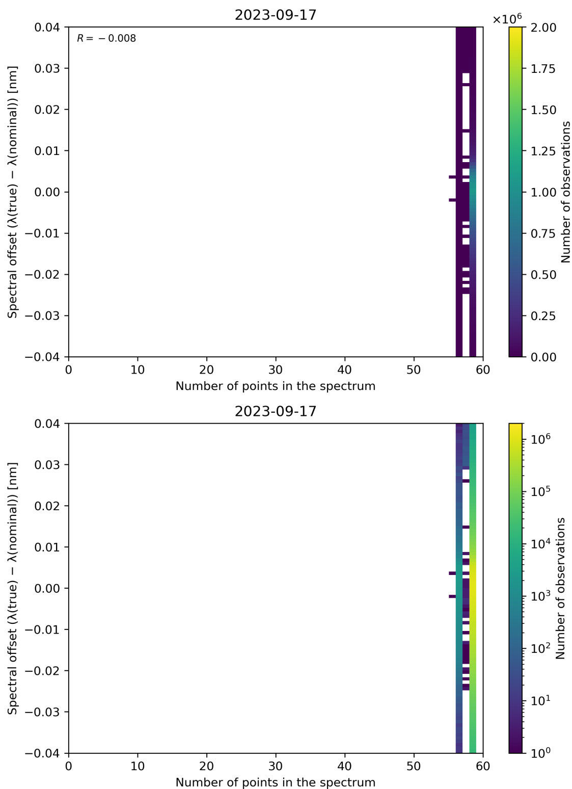
Figure 110: Scatter density plot of “Number of points in the spectrum” against “Spectral offset ( \lambda(\text{true}) - \lambda(\text{nominal}) )” for 2023-09-16 to 2023-09-18.
