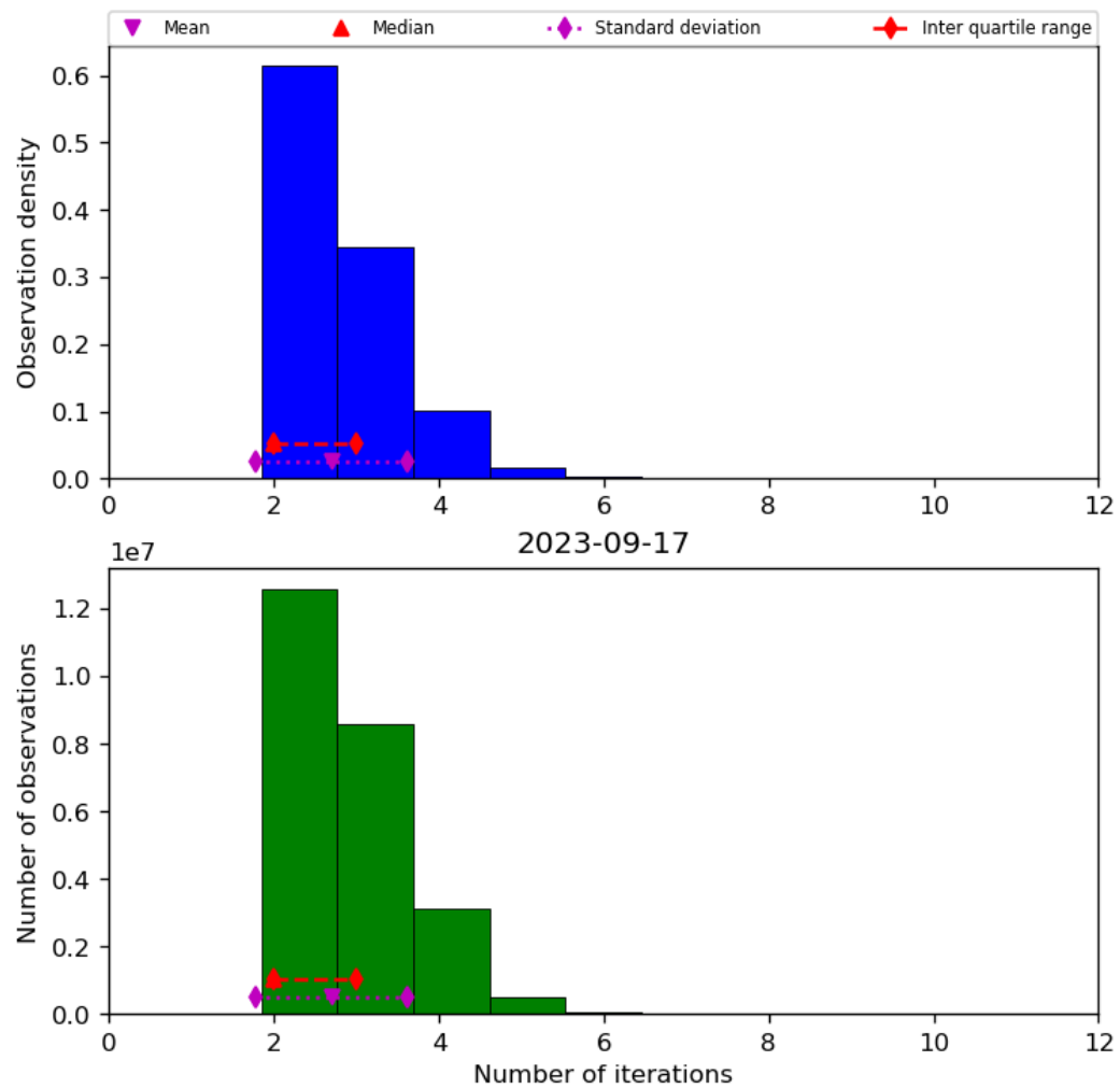
Figure 39: Histogram of “Number of iterations” for 2023-09-16 to 2023-09-18
