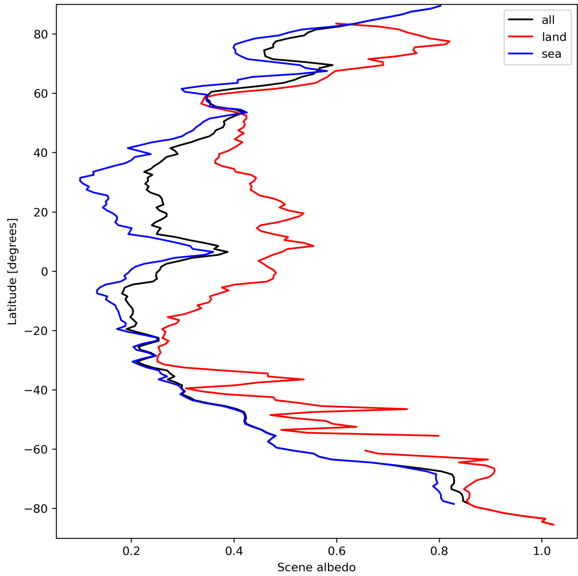
Figure 17: Zonal average of “Scene albedo” for 2023-09-16 to 2023-09-18.
