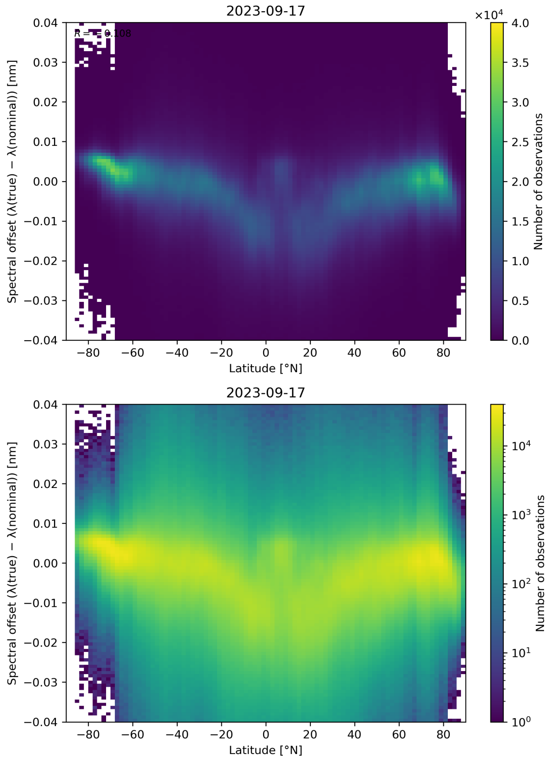
Figure 105: Scatter density plot of “Latitude” against “Spectral offset ( \lambda(\text{true}) - \lambda(\text{nominal}) )” for 2023-09-16 to 2023-09-18.
