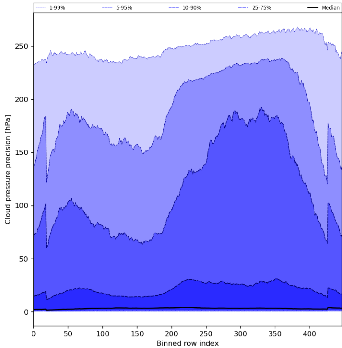
Figure 48: Along track statistics of “Cloud pressure precision” for 2023-09-16 to 2023-09-18
