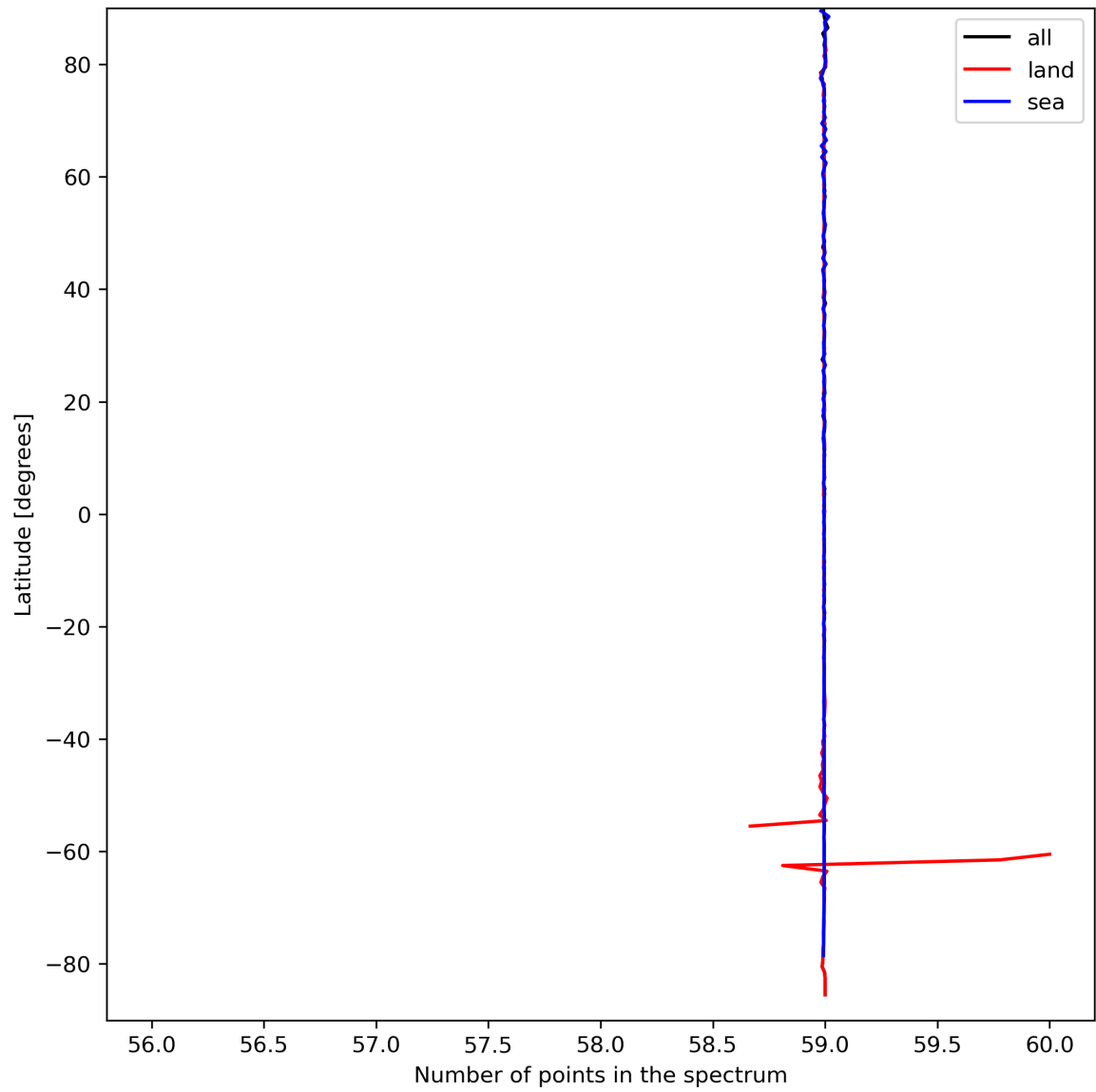
Figure 27: Zonal average of “Number of points in the spectrum” for 2023-09-16 to 2023-09-18.
