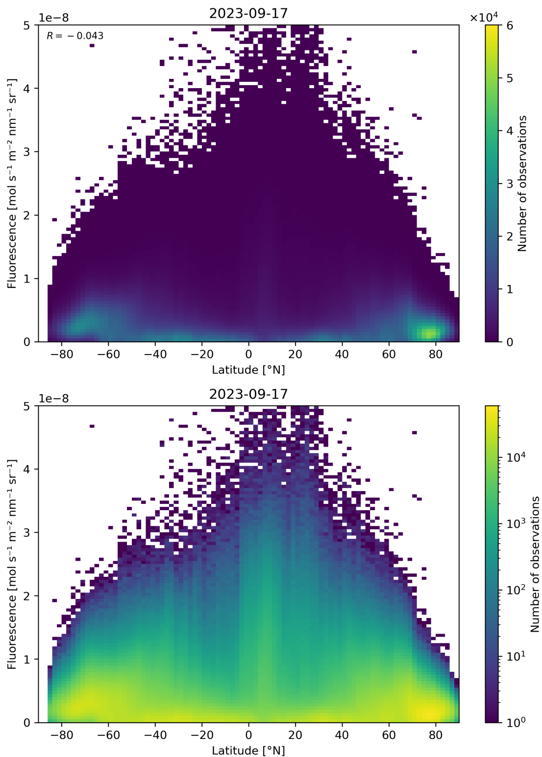
Figure 101: Scatter density plot of “Latitude” against “Fluorescence” for 2023-09-16 to 2023-09-18.
