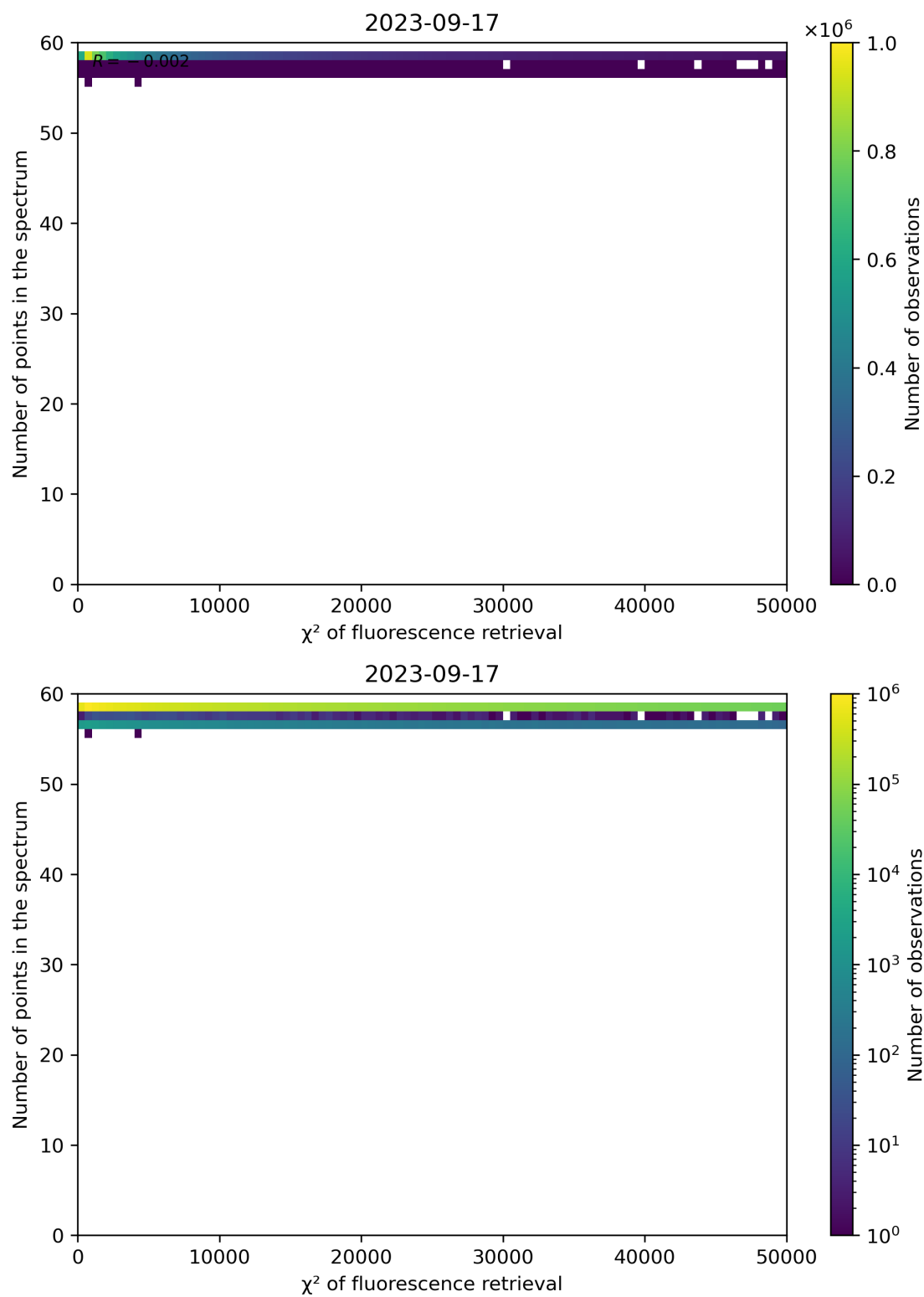
Figure 71: Scatter density plot of “ \chi^2 of fluorescence retrieval” against “Number of points in the spectrum” for 2023-09-16 to 2023-09-18.
