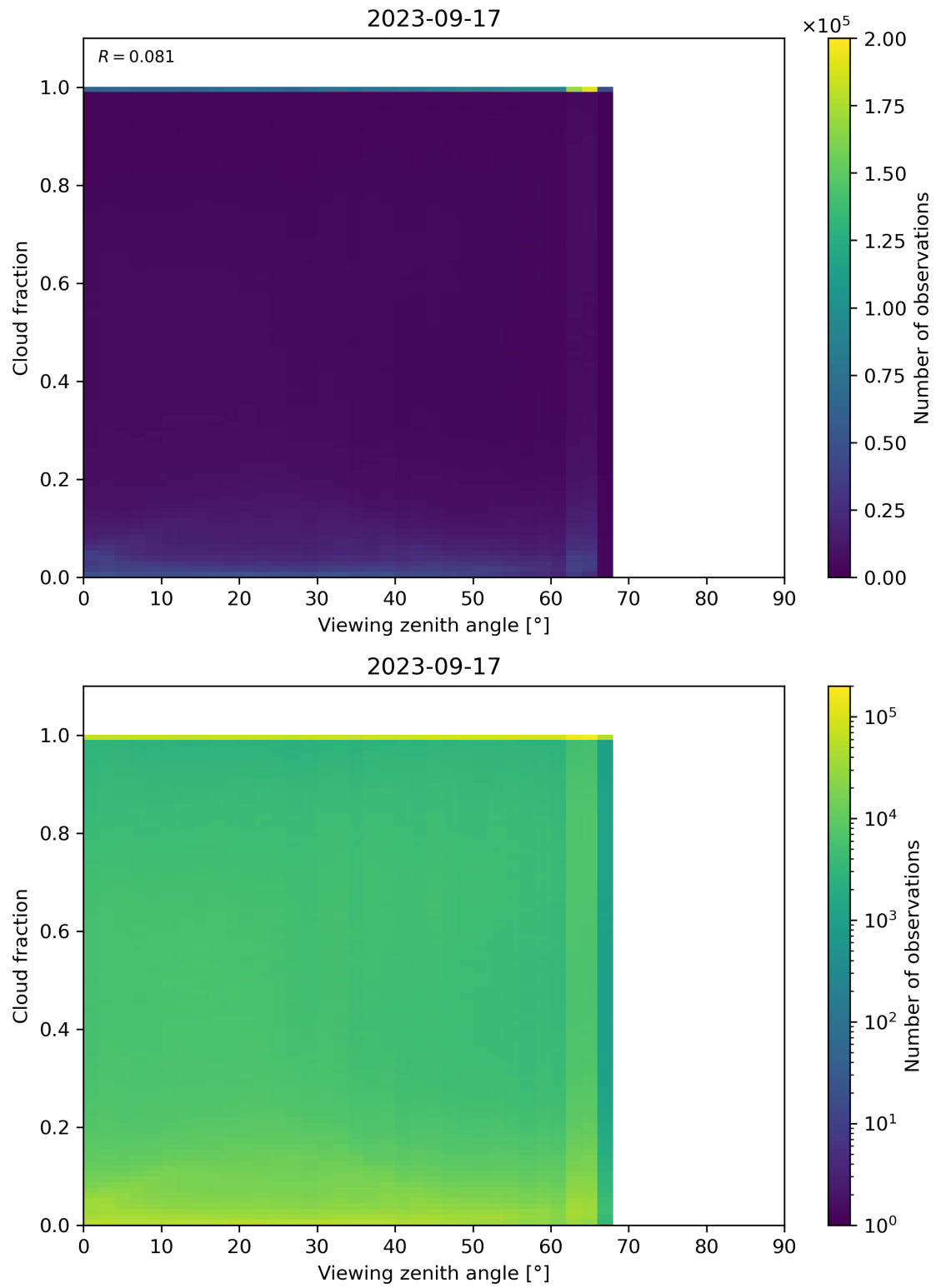
Figure 132: Scatter density plot of “Viewing zenith angle” against “Cloud fraction” for 2023-09-16 to 2023-09-18.
