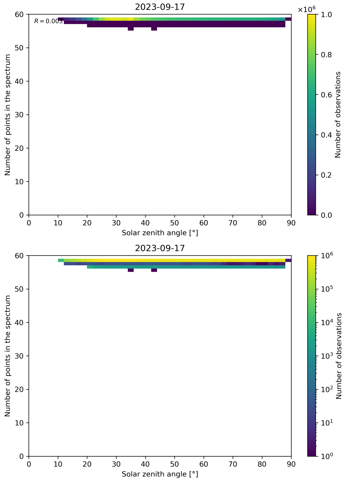
Figure 126: Scatter density plot of “Solar zenith angle” against “Number of points in the spectrum” for 2023-09-16 to 2023-09-18.
