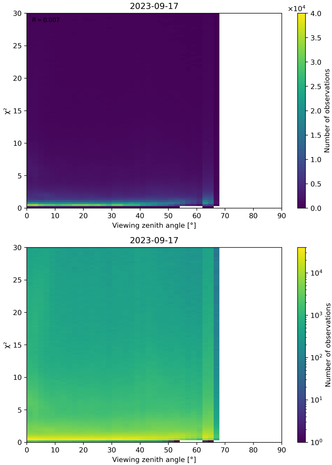
Figure 130: Scatter density plot of “Viewing zenith angle” against “ \chi^2 ” for 2023-09-16 to 2023-09-18.
