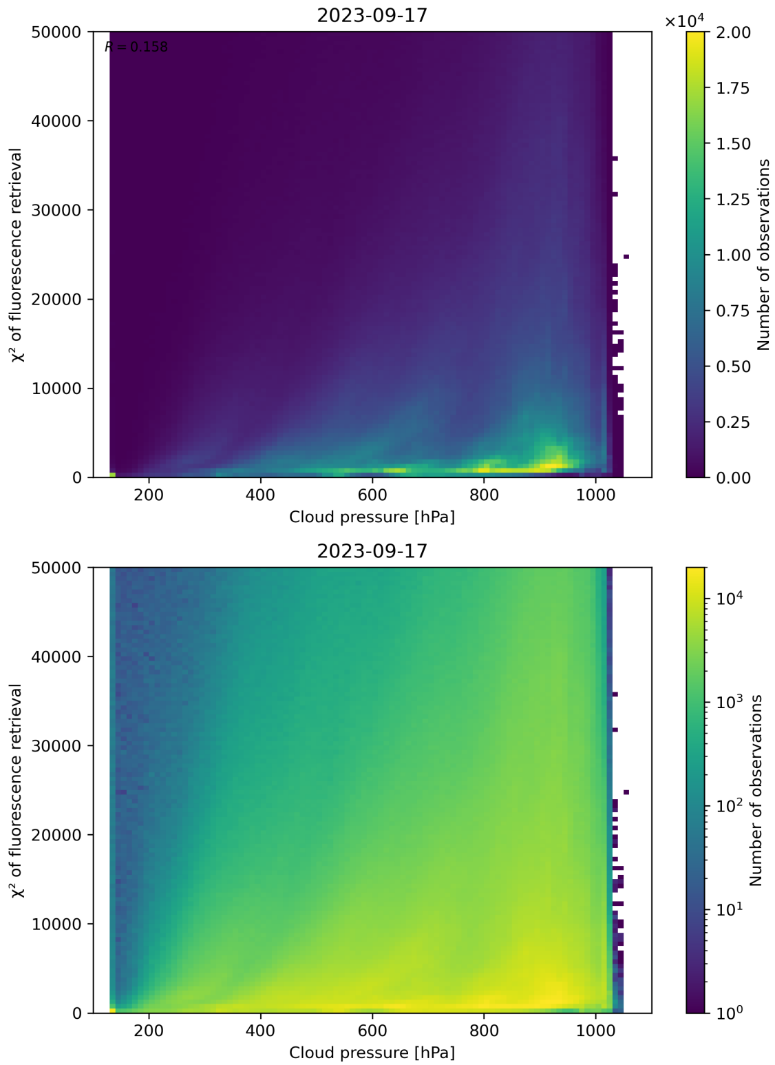
Figure 86: Scatter density plot of “Cloud pressure” against “ \chi^2 of fluorescence retrieval” for 2023-09-16 to 2023-09-18.
