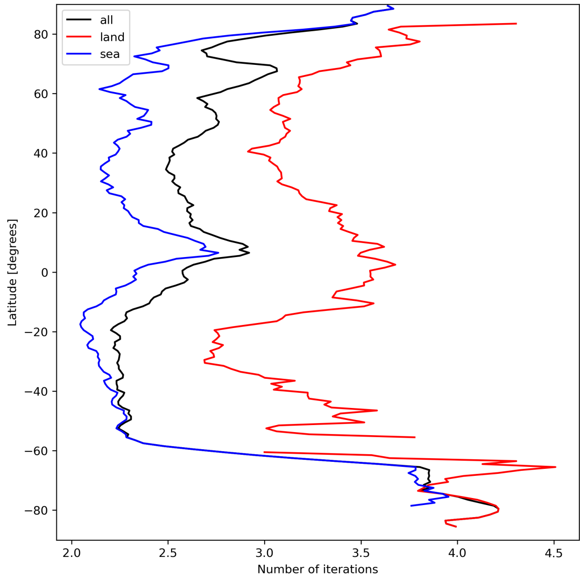
Figure 22: Zonal average of “Number of iterations” for 2023-09-16 to 2023-09-18.
