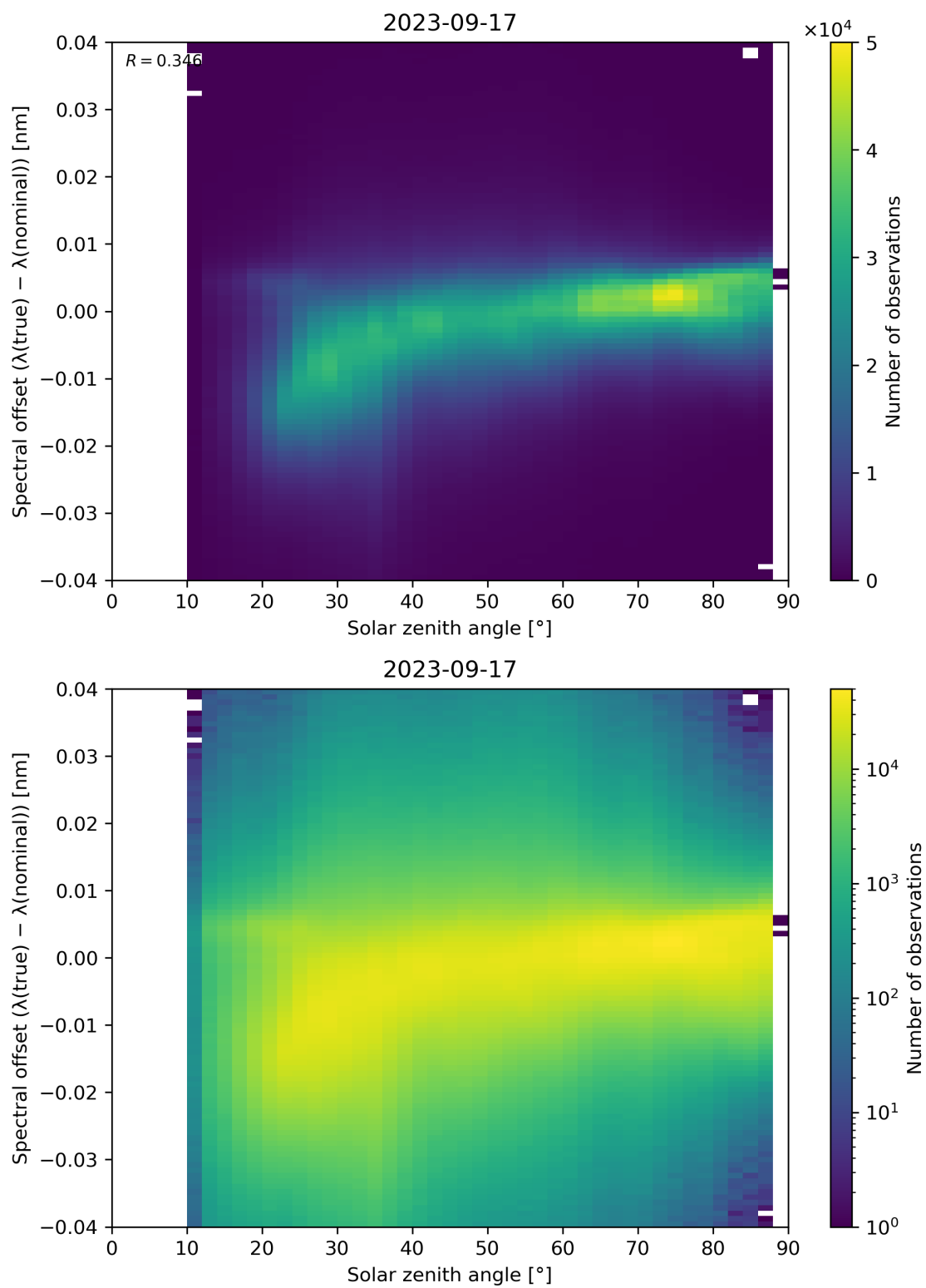
Figure 128: Scatter density plot of “Solar zenith angle” against “Spectral offset ( \lambda(\text{true}) - \lambda(\text{nominal}) )” for 2023-09-16 to 2023-09-18.
