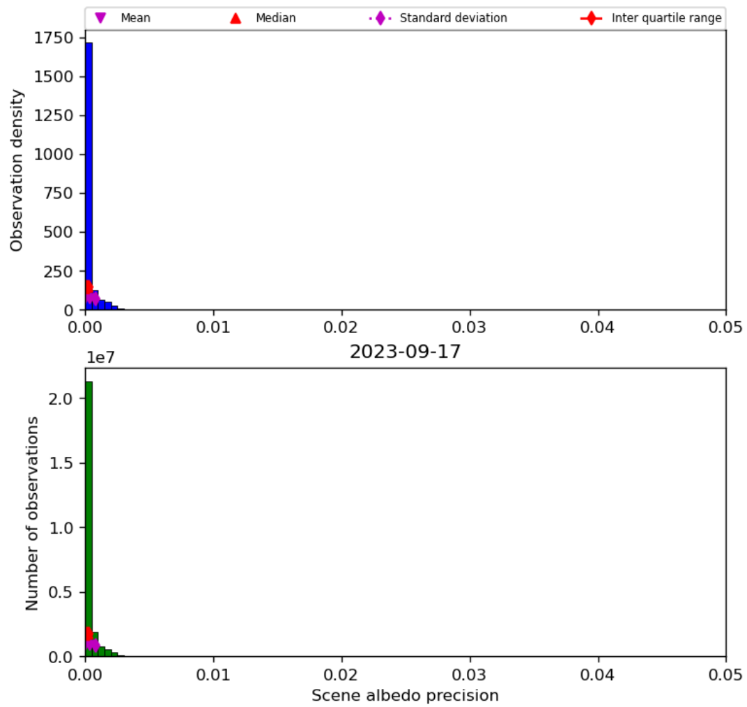
Figure 35: Histogram of “Scene albedo precision” for 2023-09-16 to 2023-09-18
