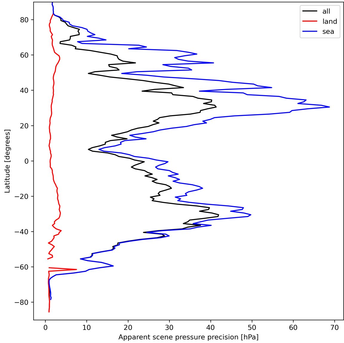
Figure 20: Zonal average of “Apparent scene pressure precision” for 2023-09-16 to 2023-09-18.
