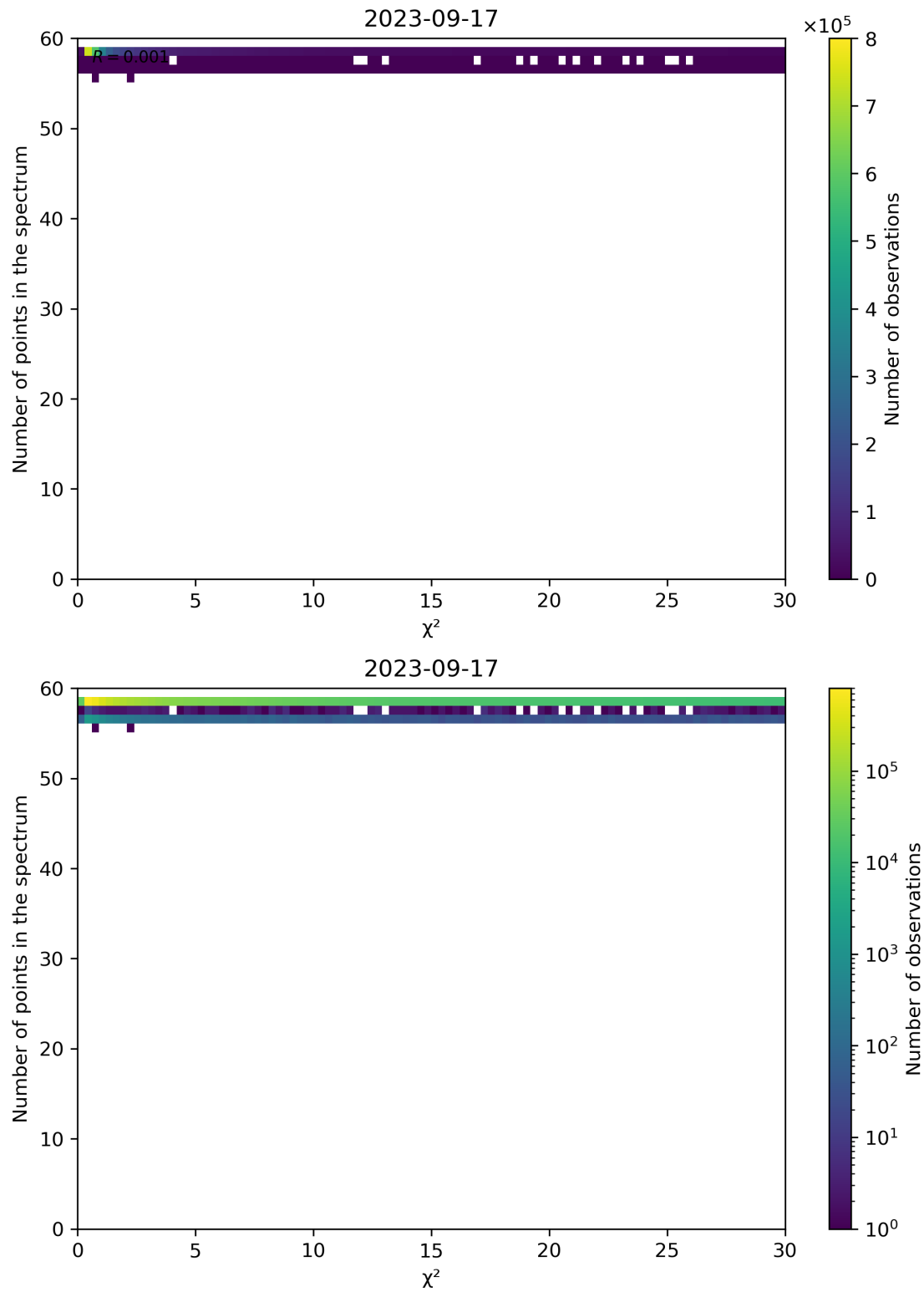
Figure 74: Scatter density plot of “ \chi^2 ” against “Number of points in the spectrum” for 2023-09-16 to 2023-09-18.
