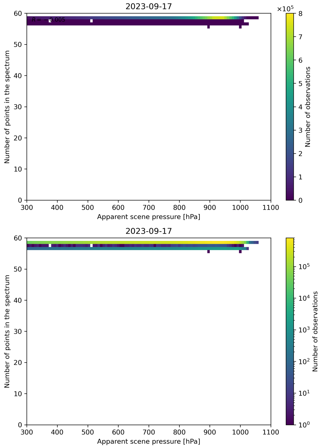
Figure 67: Scatter density plot of “Apparent scene pressure” against “Number of points in the spectrum” for 2023-09-16 to 2023-09-18.
