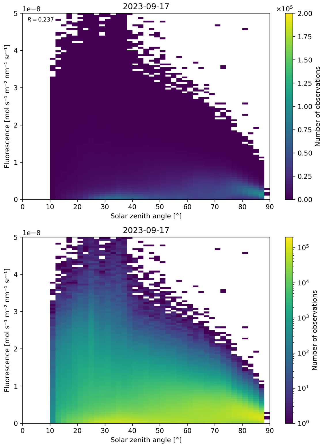
Figure 123: Scatter density plot of “Solar zenith angle” against “Fluorescence” for 2023-09-16 to 2023-09-18.
