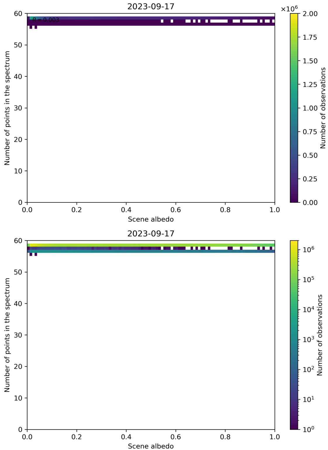
Figure 116: Scatter density plot of “Scene albedo” against “Number of points in the spectrum” for 2023-09-16 to 2023-09-18.
