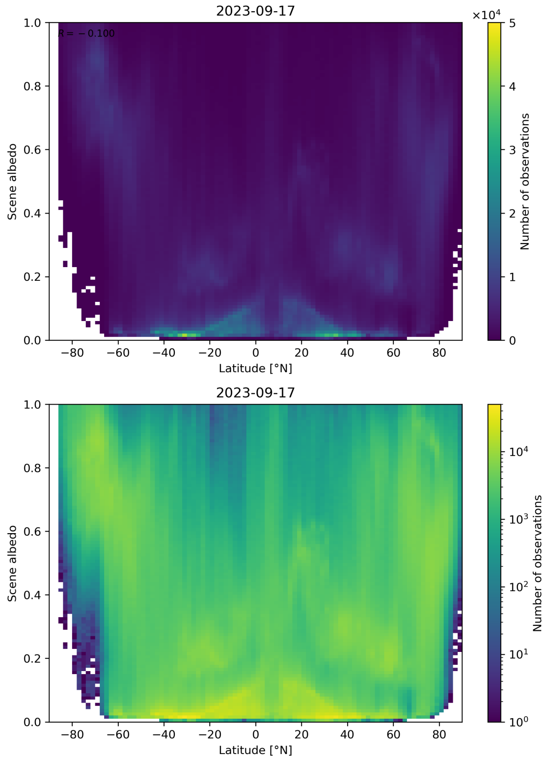
Figure 104: Scatter density plot of “Latitude” against “Scene albedo” for 2023-09-16 to 2023-09-18.
