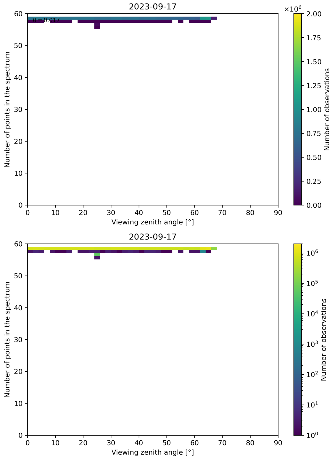
Figure 137: Scatter density plot of “Viewing zenith angle” against “Number of points in the spectrum” for 2023-09-16 to 2023-09-18.
