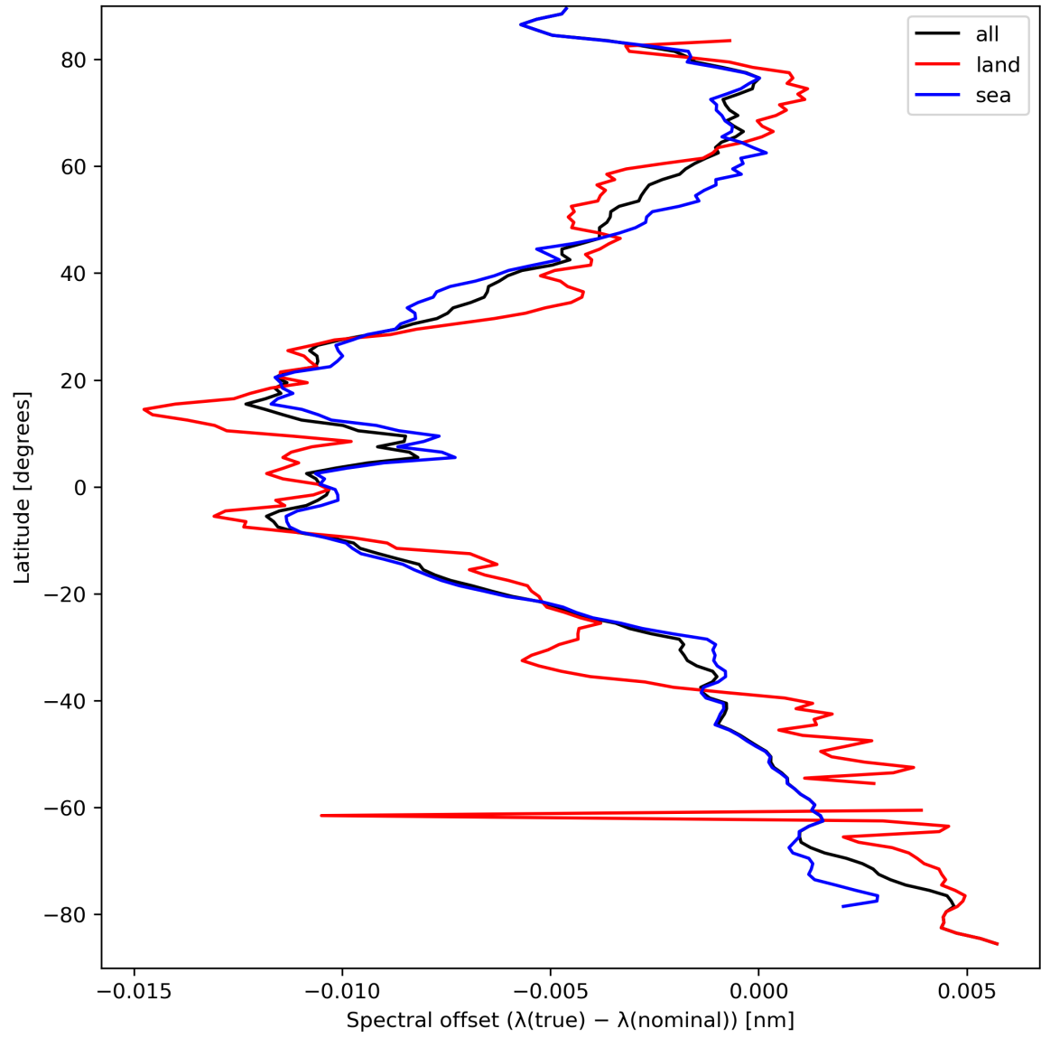
Figure 28: Zonal average of “Spectral offset ( \lambda(\text{true}) - \lambda(\text{nominal}) )” for 2023-09-16 to 2023-09-18.
