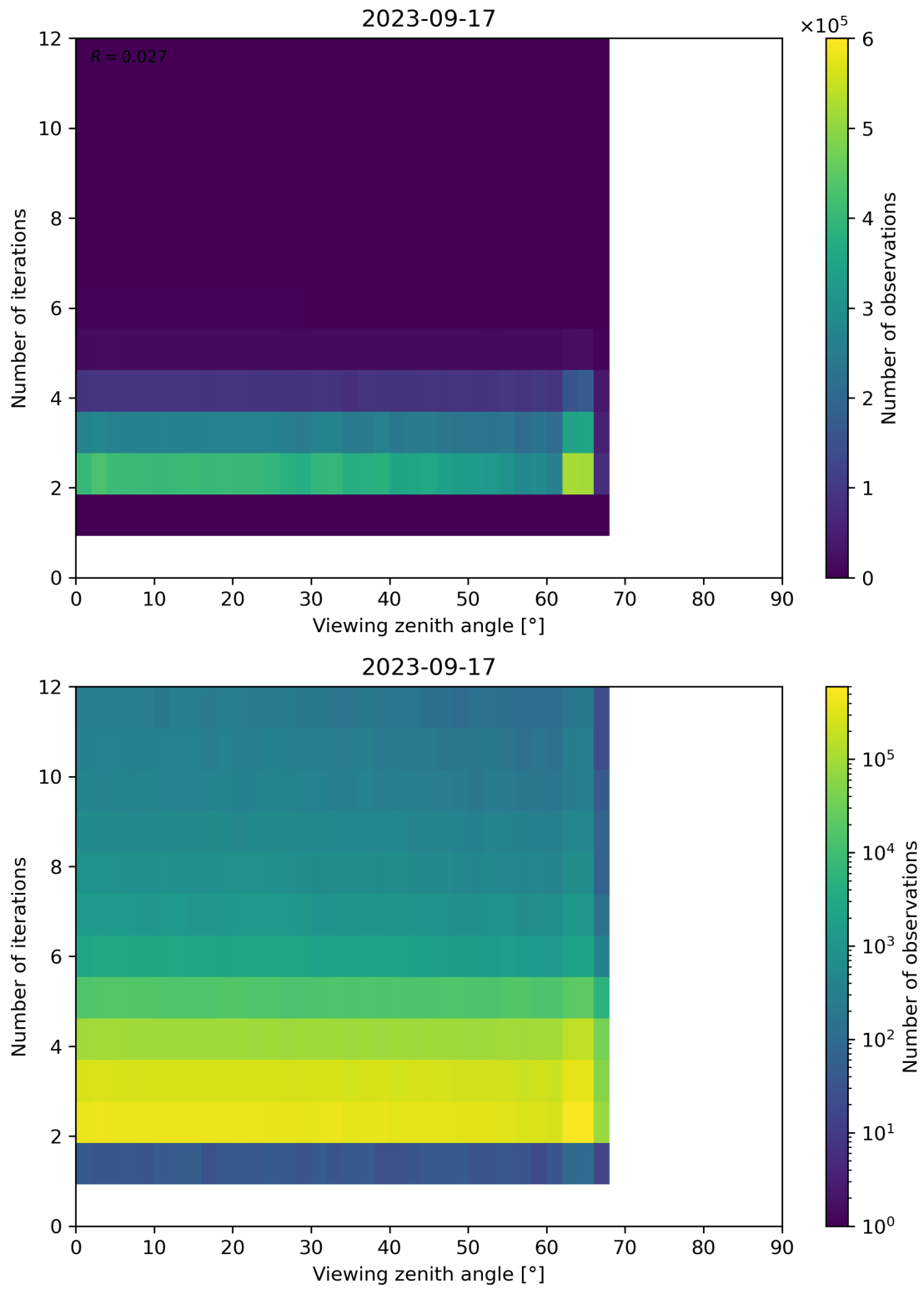
Figure 136: Scatter density plot of “Viewing zenith angle” against “Number of iterations” for 2023-09-16 to 2023-09-18.
