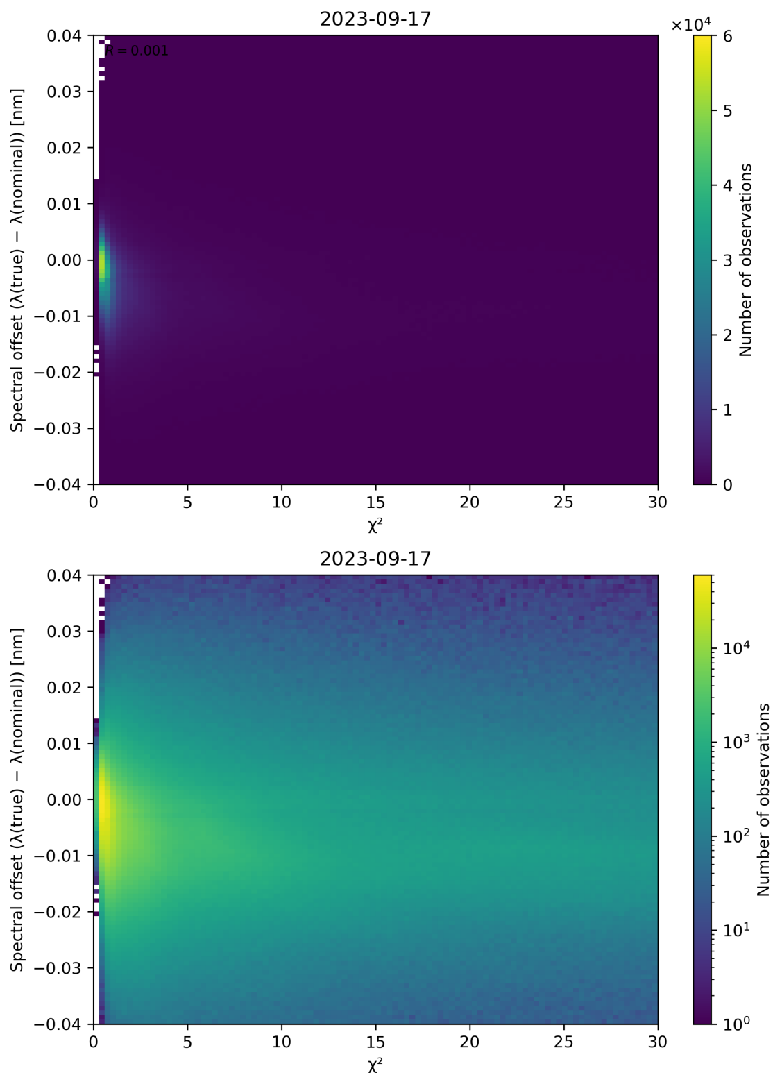
Figure 75: Scatter density plot of “ \chi^2 ” against “Spectral offset ( \lambda(\text{true}) - \lambda(\text{nominal}) )” for 2023-09-16 to 2023-09-18.
