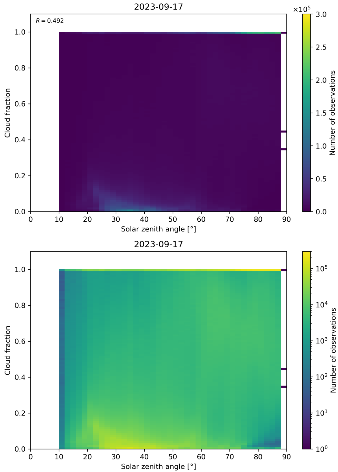
Figure 121: Scatter density plot of “Solar zenith angle” against “Cloud fraction” for 2023-09-16 to 2023-09-18.
