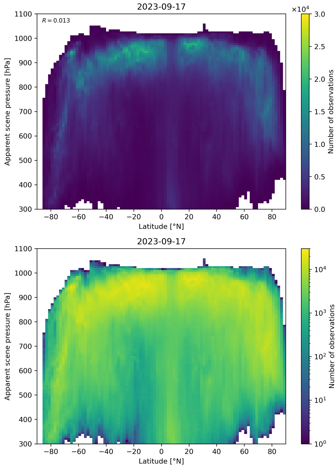
Figure 96: Scatter density plot of “Latitude” against “Apparent scene pressure” for 2023-09-16 to 2023-09-18.
