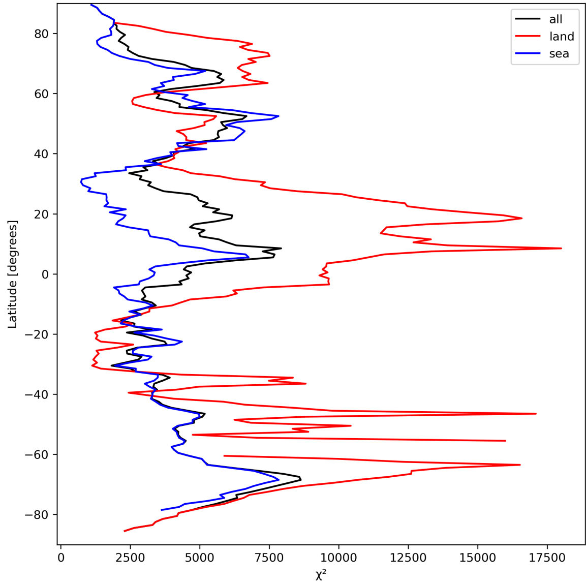
Figure 21: Zonal average of “ \chi^2 ” for 2023-09-16 to 2023-09-18.
