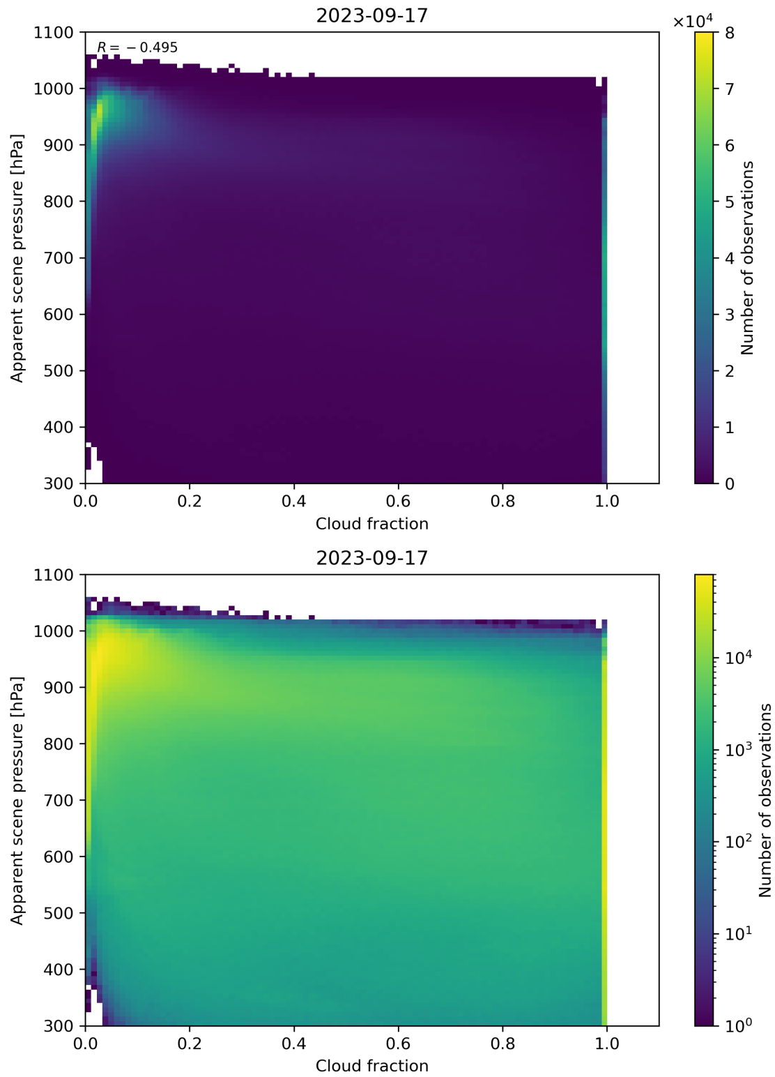
Figure 76: Scatter density plot of “Cloud fraction” against “Apparent scene pressure” for 2023-09-16 to 2023-09-18.
