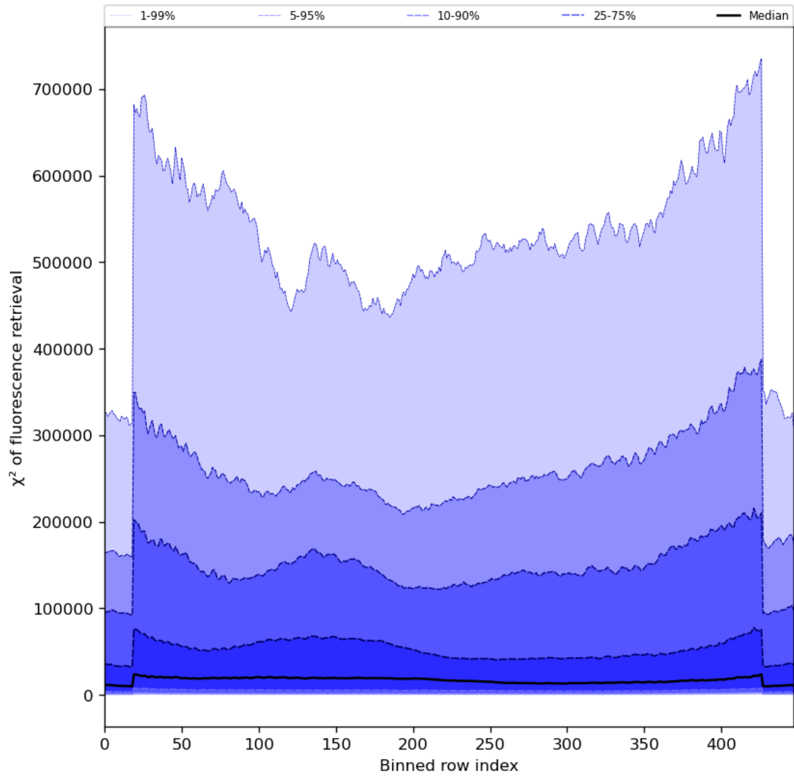
Figure 59: Along track statistics of “ \chi^2 of fluorescence retrieval” for 2023-09-16 to 2023-09-18
