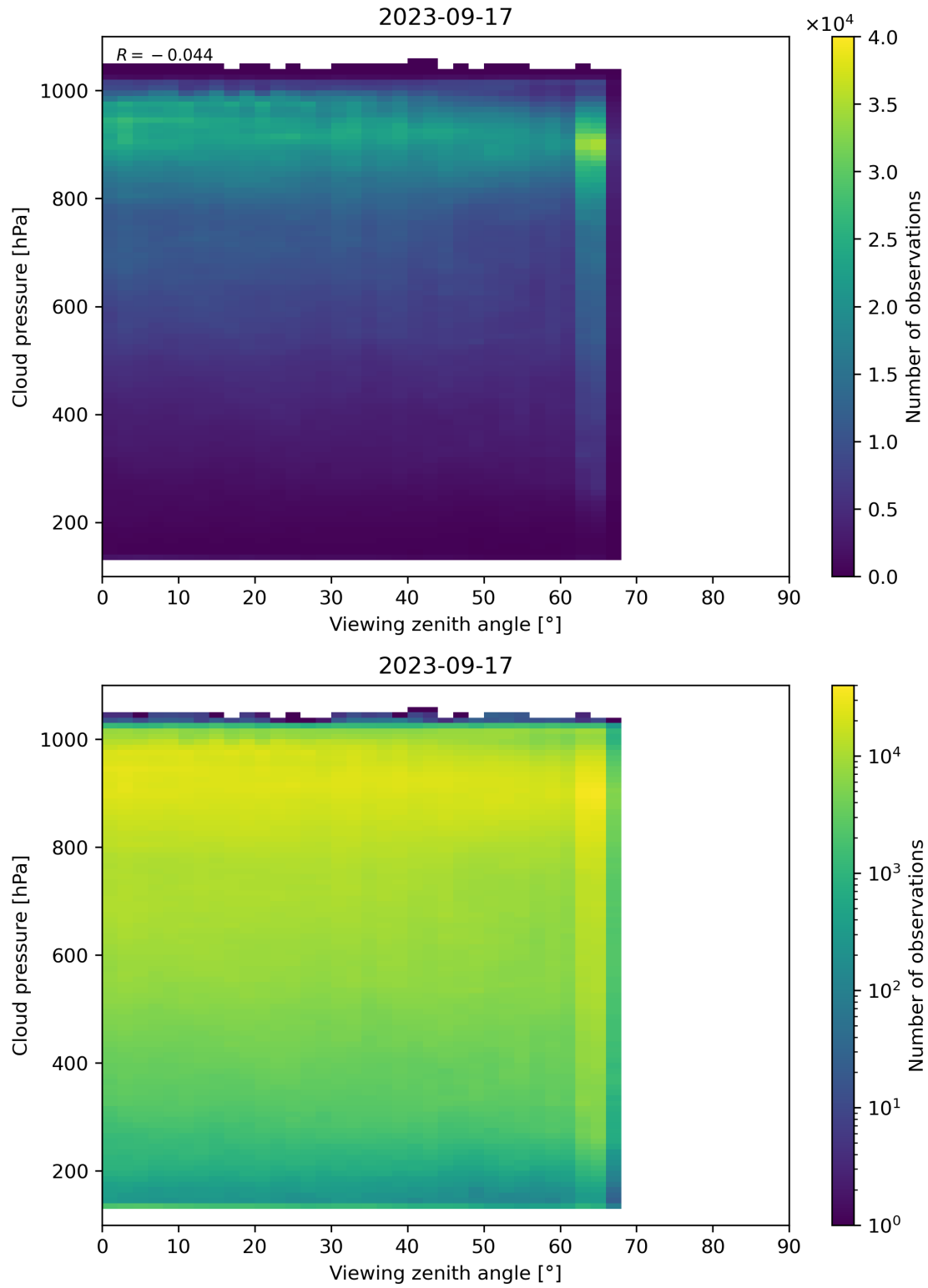
Figure 133: Scatter density plot of “Viewing zenith angle” against “Cloud pressure” for 2023-09-16 to 2023-09-18.
