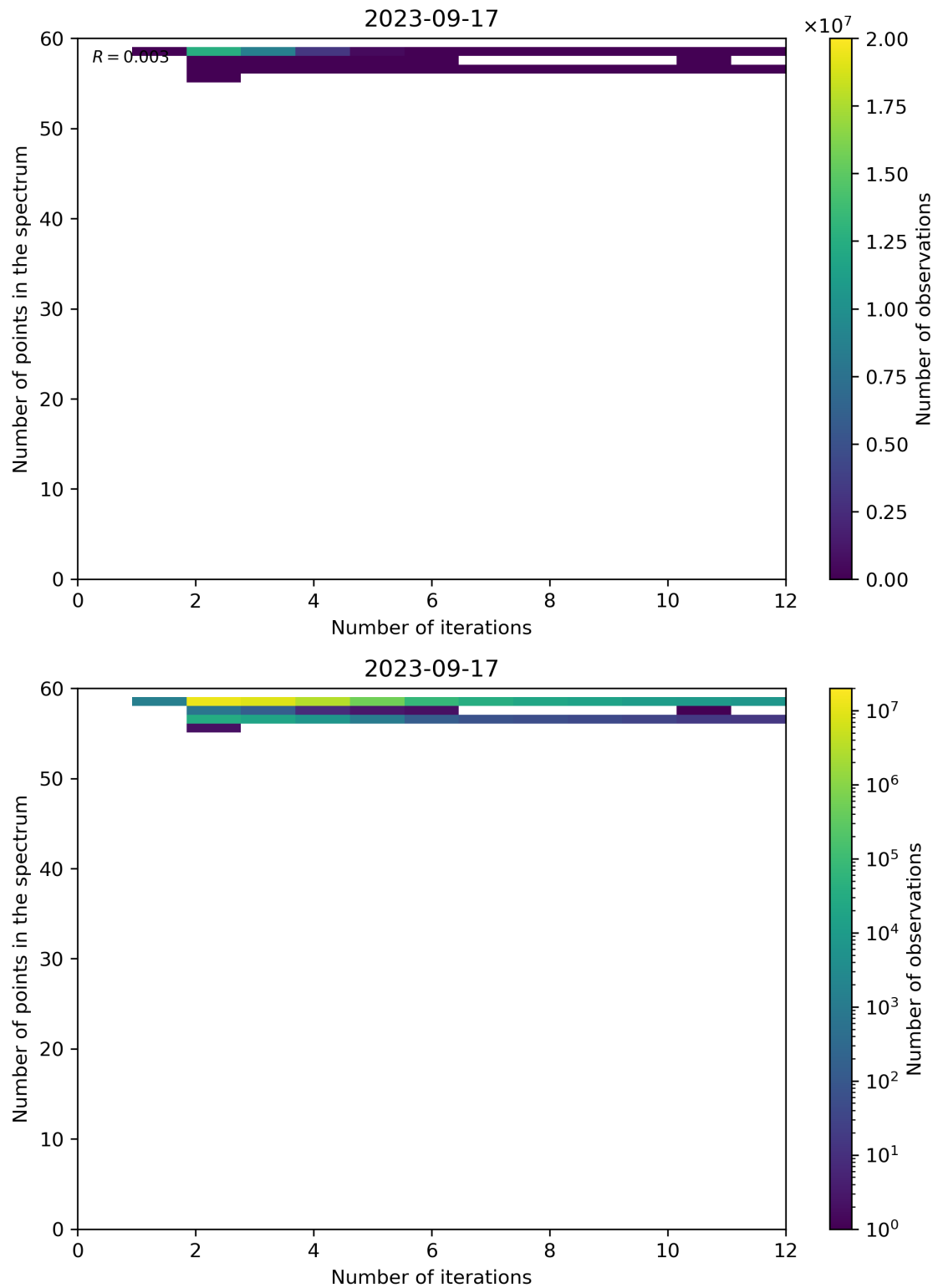
Figure 108: Scatter density plot of “Number of iterations” against “Number of points in the spectrum” for 2023-09-16 to 2023-09-18.
