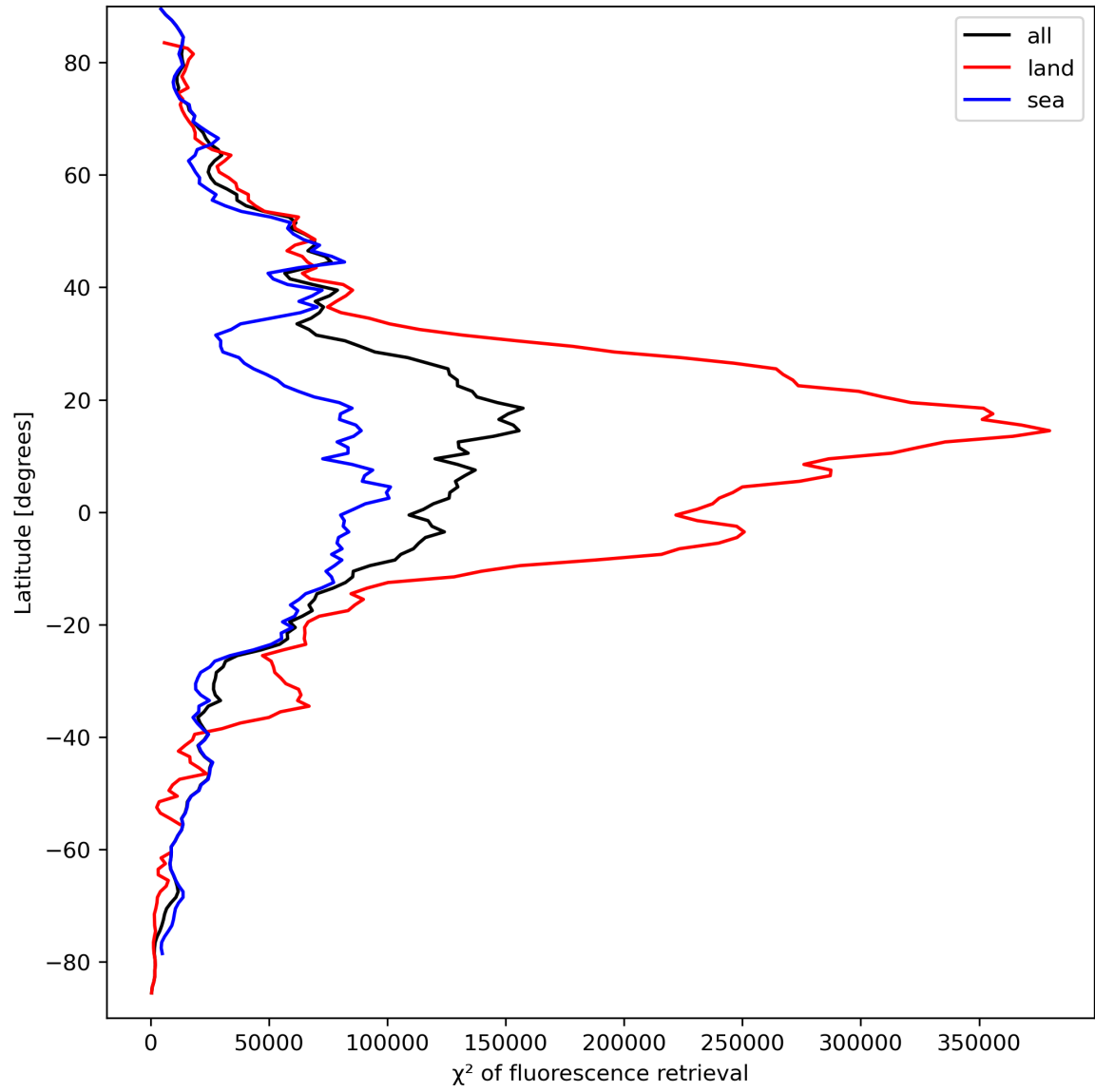
Figure 25: Zonal average of “ \chi^2 of fluorescence retrieval” for 2023-09-16 to 2023-09-18.
