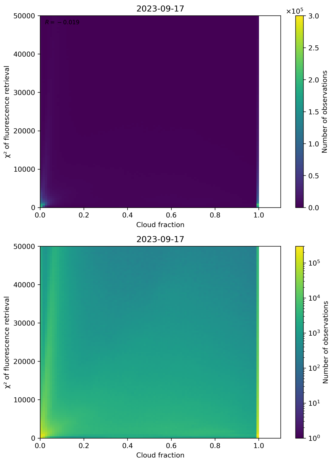
Figure 78: Scatter density plot of “Cloud fraction” against “ \chi^2 of fluorescence retrieval” for 2023-09-16 to 2023-09-18.
