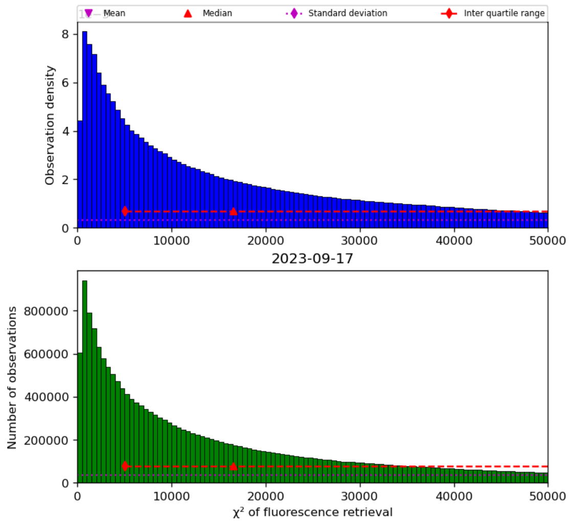
Figure 42: Histogram of “ \chi^2 of fluorescence retrieval” for 2023-09-16 to 2023-09-18
