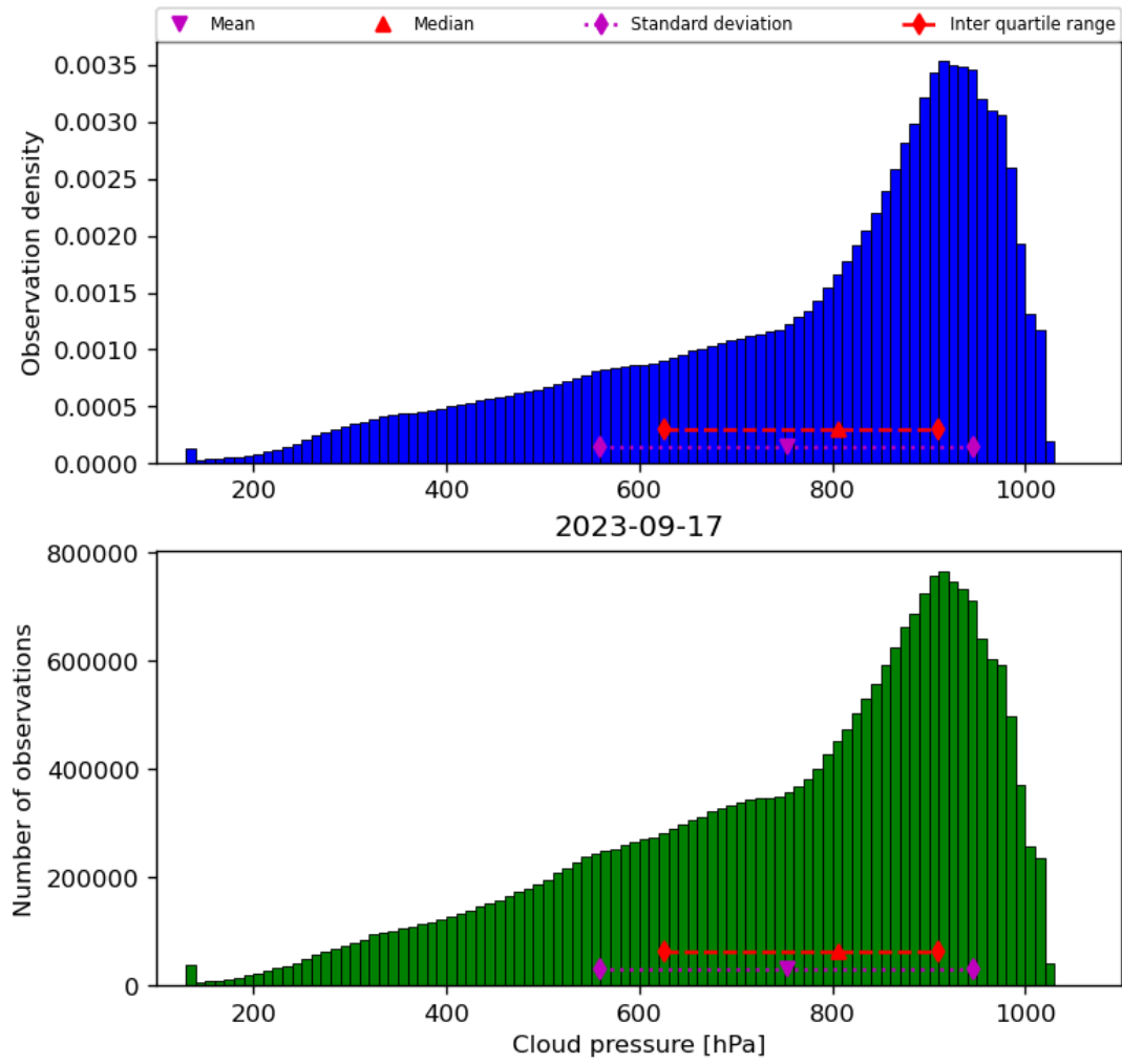
Figure 30: Histogram of “Cloud pressure” for 2023-09-16 to 2023-09-18
