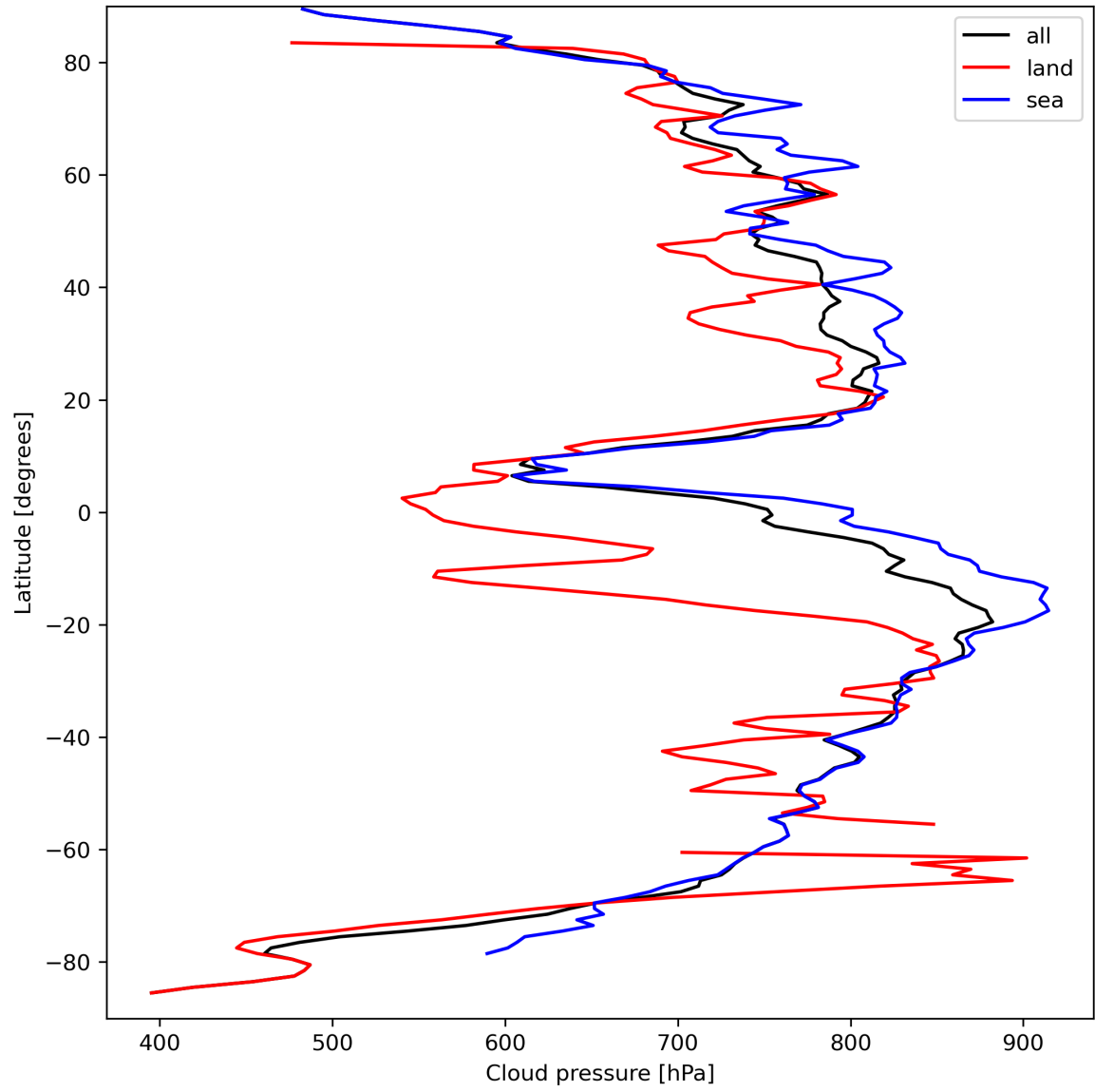
Figure 13: Zonal average of “Cloud pressure” for 2023-09-16 to 2023-09-18.
