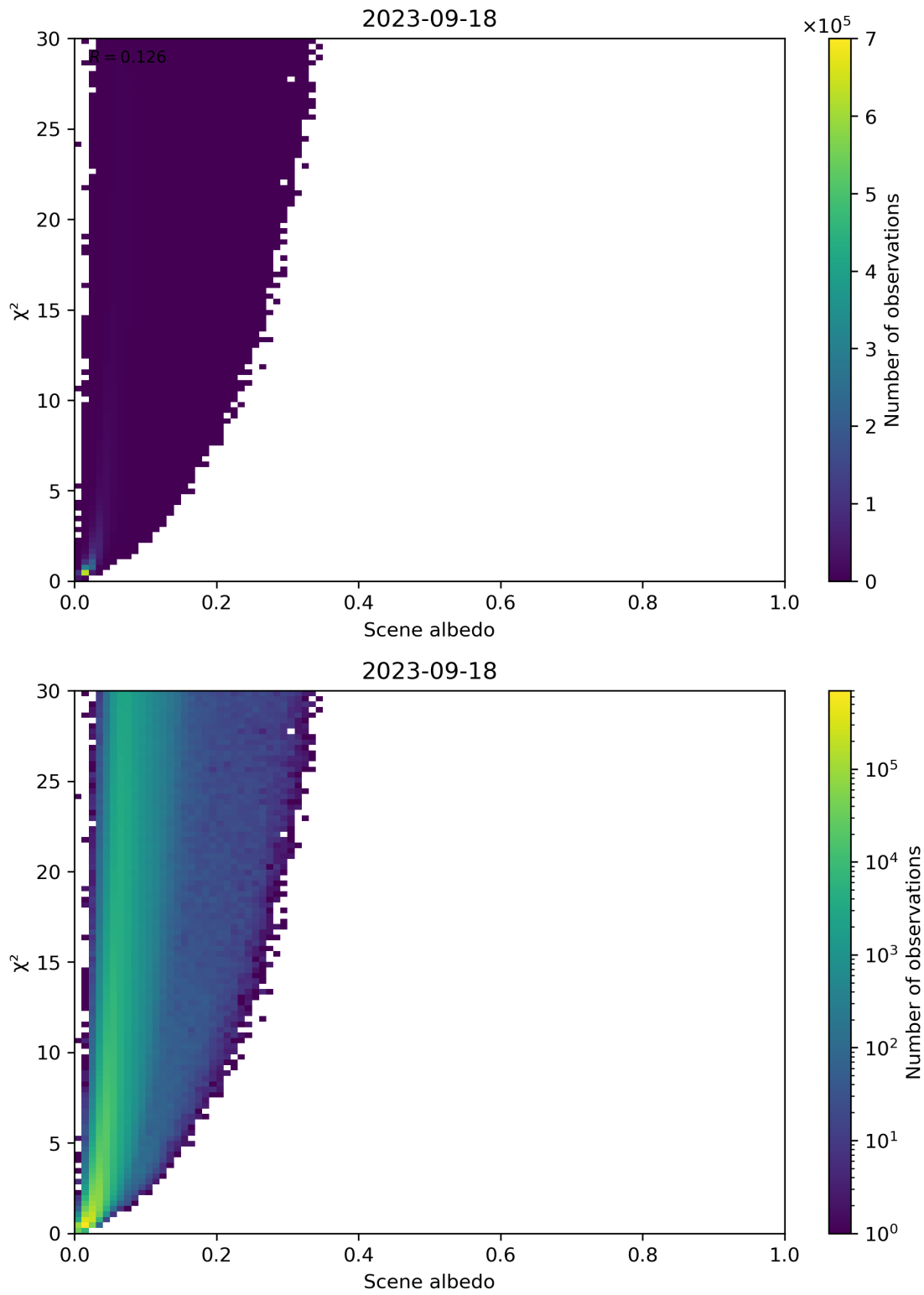
Figure 112: Scatter density plot of “Scene albedo” against “ \chi^2 ” for 2023-09-17 to 2023-09-19.
