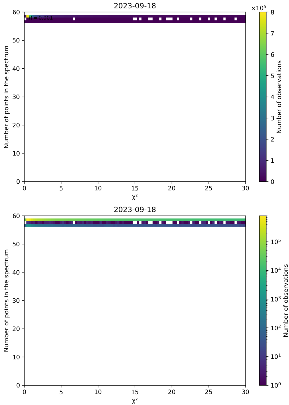
Figure 74: Scatter density plot of " \chi^2 " against "Number of points in the spectrum" for 2023-09-17 to 2023-09-19.
