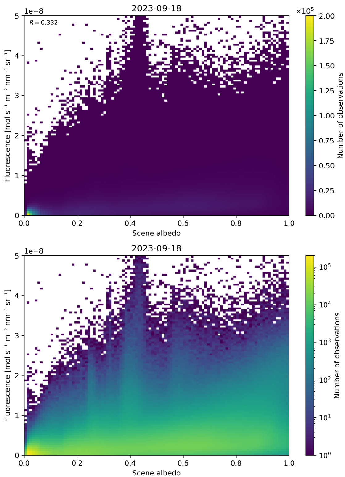
Figure 114: Scatter density plot of “Scene albedo” against “Fluorescence” for 2023-09-17 to 2023-09-19.
