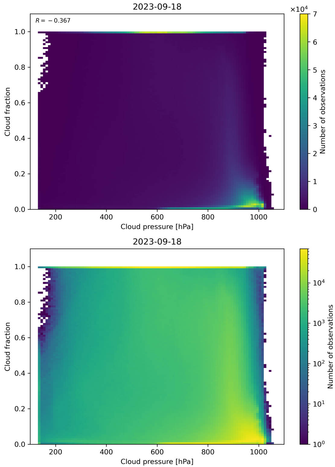
Figure 87: Scatter density plot of “Cloud pressure” against “Cloud fraction” for 2023-09-17 to 2023-09-19.
