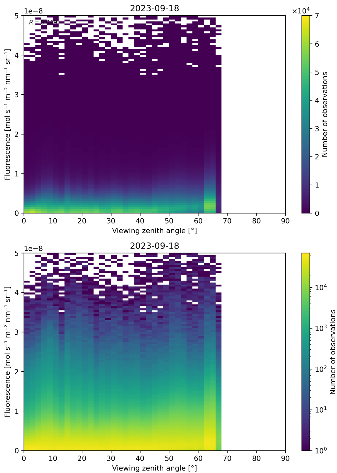
Figure 134: Scatter density plot of “Viewing zenith angle” against “Fluorescence” for 2023-09-17 to 2023-09-19.
