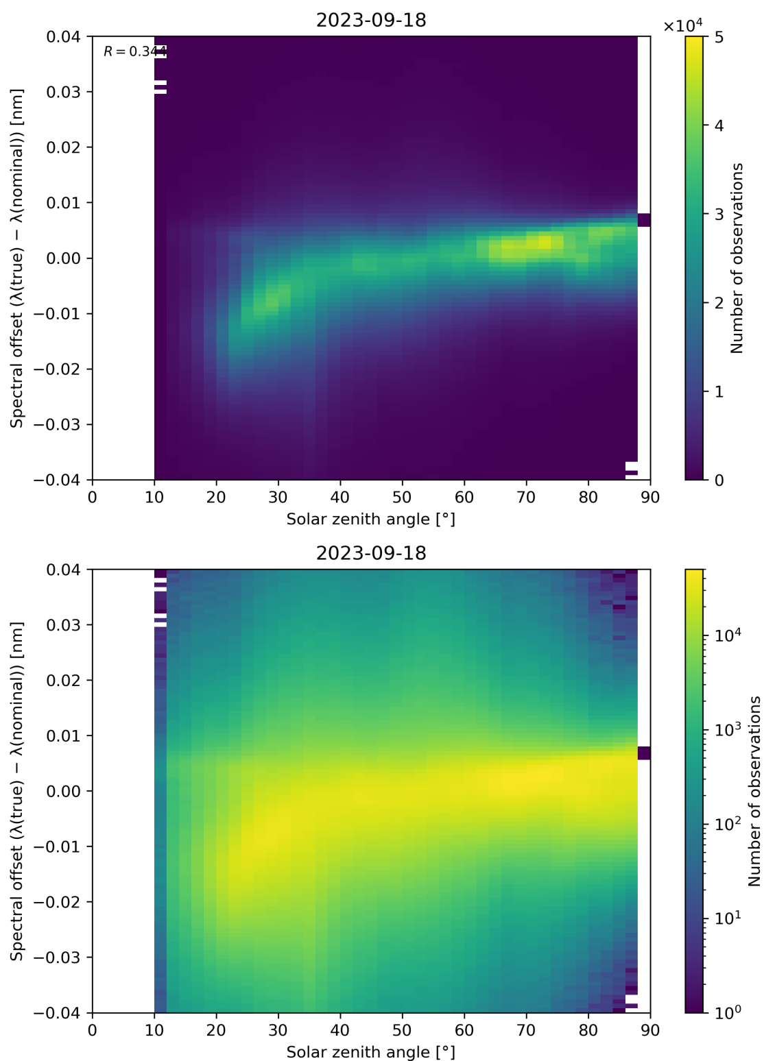
Figure 128: Scatter density plot of “Solar zenith angle” against “Spectral offset ( \lambda(\text{true}) - \lambda(\text{nominal}) )” for 2023-09-17 to 2023-09-19.
