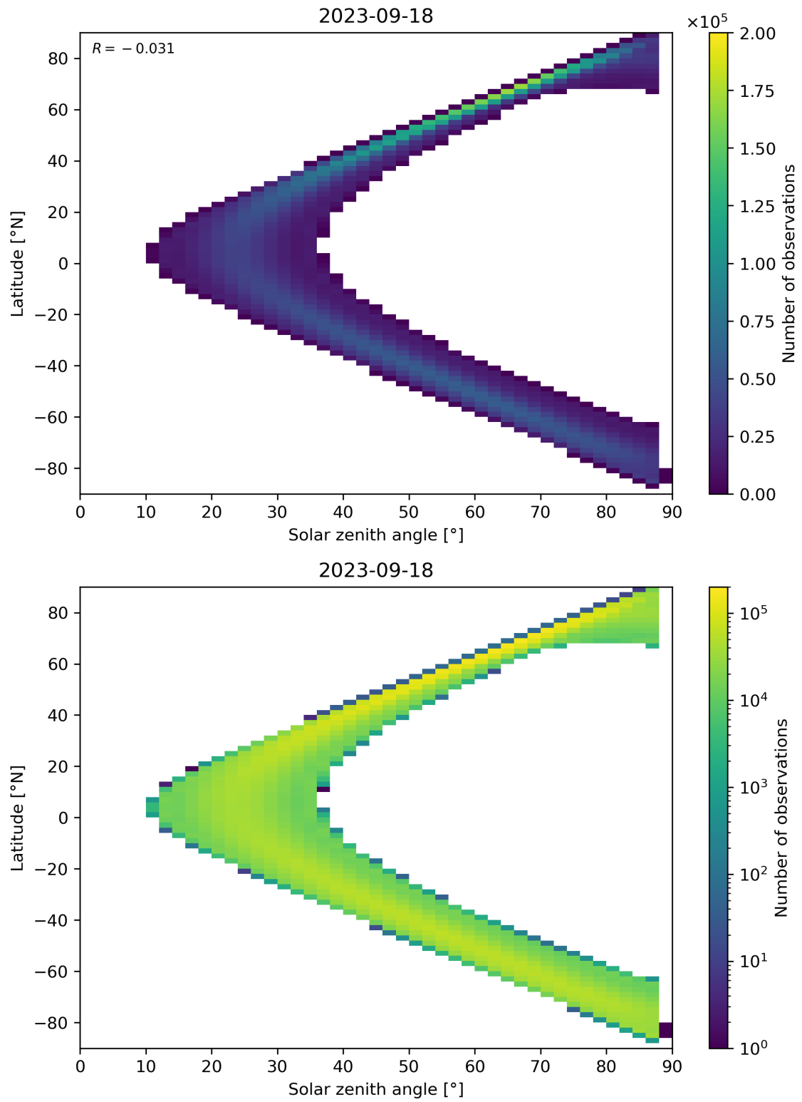
Figure 124: Scatter density plot of “Solar zenith angle” against “Latitude” for 2023-09-17 to 2023-09-19.
