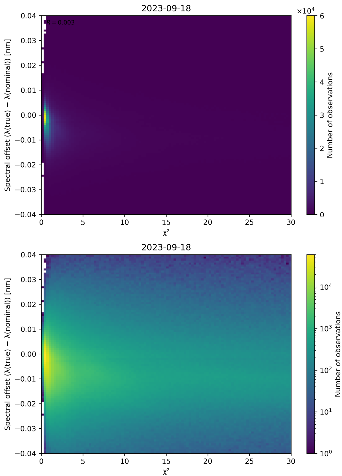
Figure 75: Scatter density plot of “ \chi^2 ” against “Spectral offset ( \lambda(\text{true}) - \lambda(\text{nominal}) )” for 2023-09-17 to 2023-09-19.
