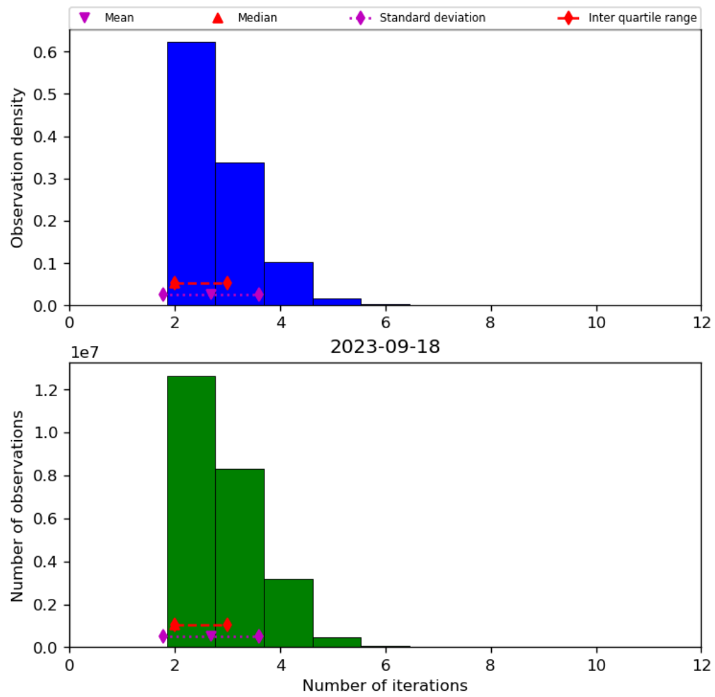
Figure 39: Histogram of “Number of iterations” for 2023-09-17 to 2023-09-19
