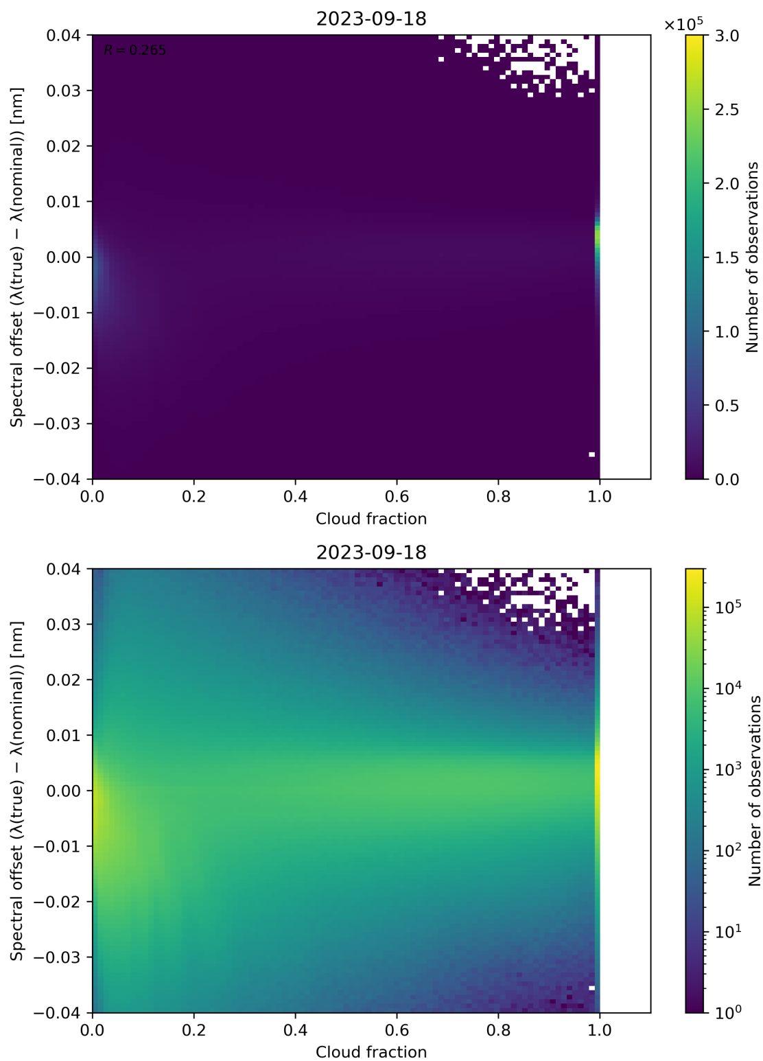
Figure 83: Scatter density plot of “Cloud fraction” against “Spectral offset ( \lambda(\text{true}) - \lambda(\text{nominal}) )” for 2023-09-17 to 2023-09-19.
