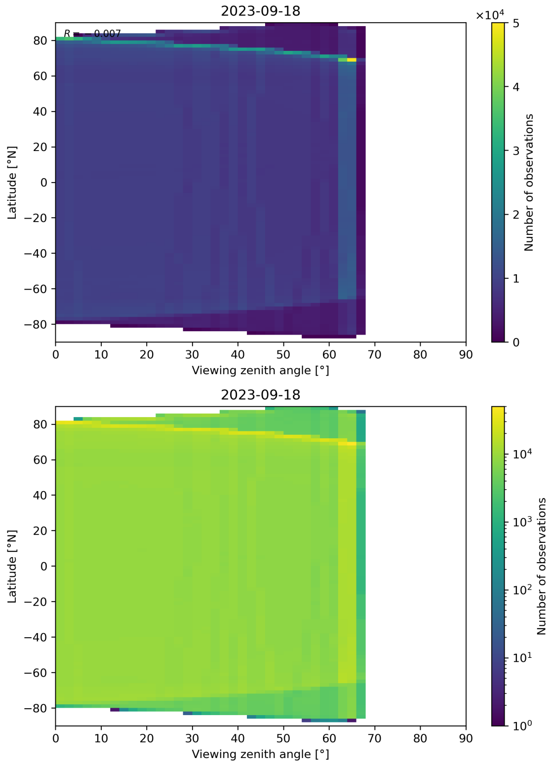
Figure 135: Scatter density plot of “Viewing zenith angle” against “Latitude” for 2023-09-17 to 2023-09-19.
