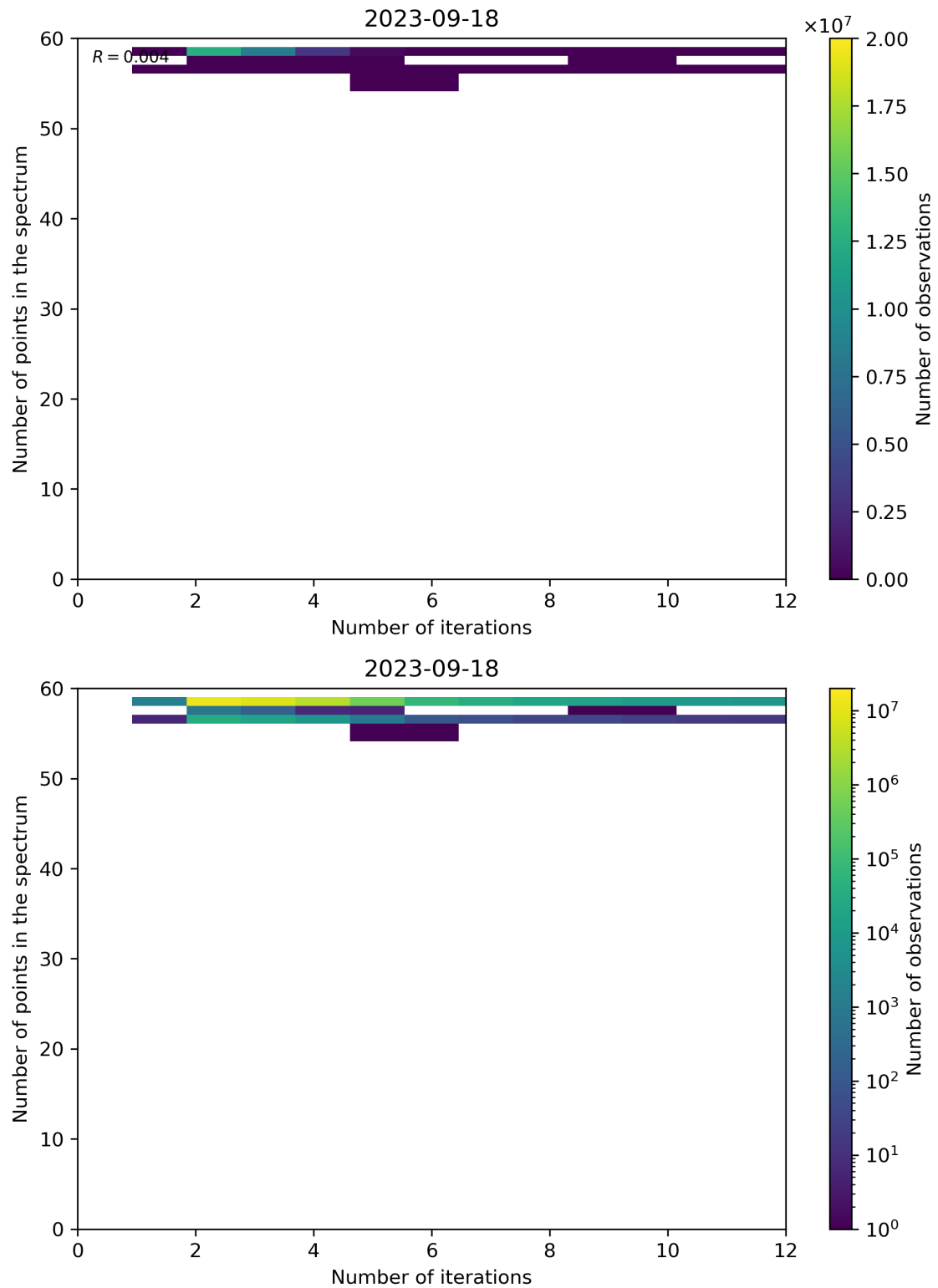
Figure 108: Scatter density plot of “Number of iterations” against “Number of points in the spectrum” for 2023-09-17 to 2023-09-19.
