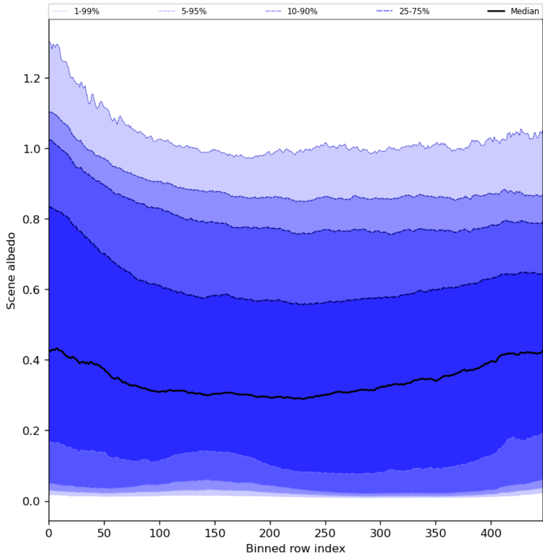
Figure 51: Along track statistics of “Scene albedo” for 2023-09-17 to 2023-09-19
