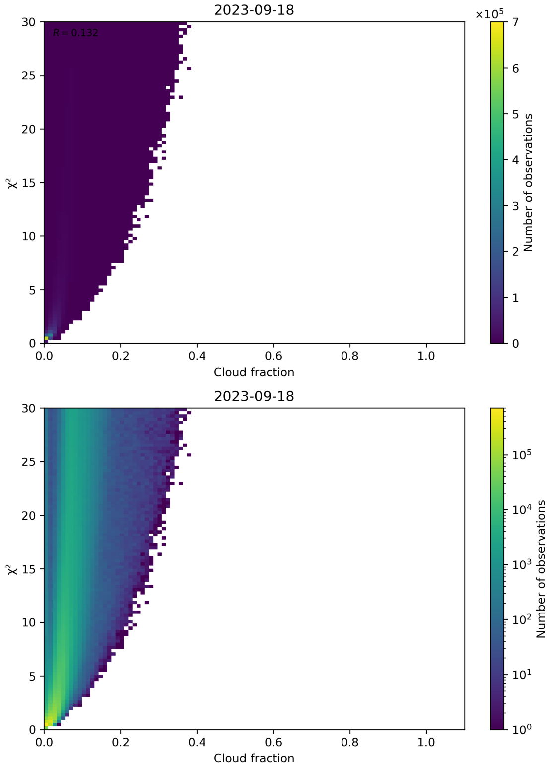
Figure 77: Scatter density plot of “Cloud fraction” against “ \chi^2 ” for 2023-09-17 to 2023-09-19.
