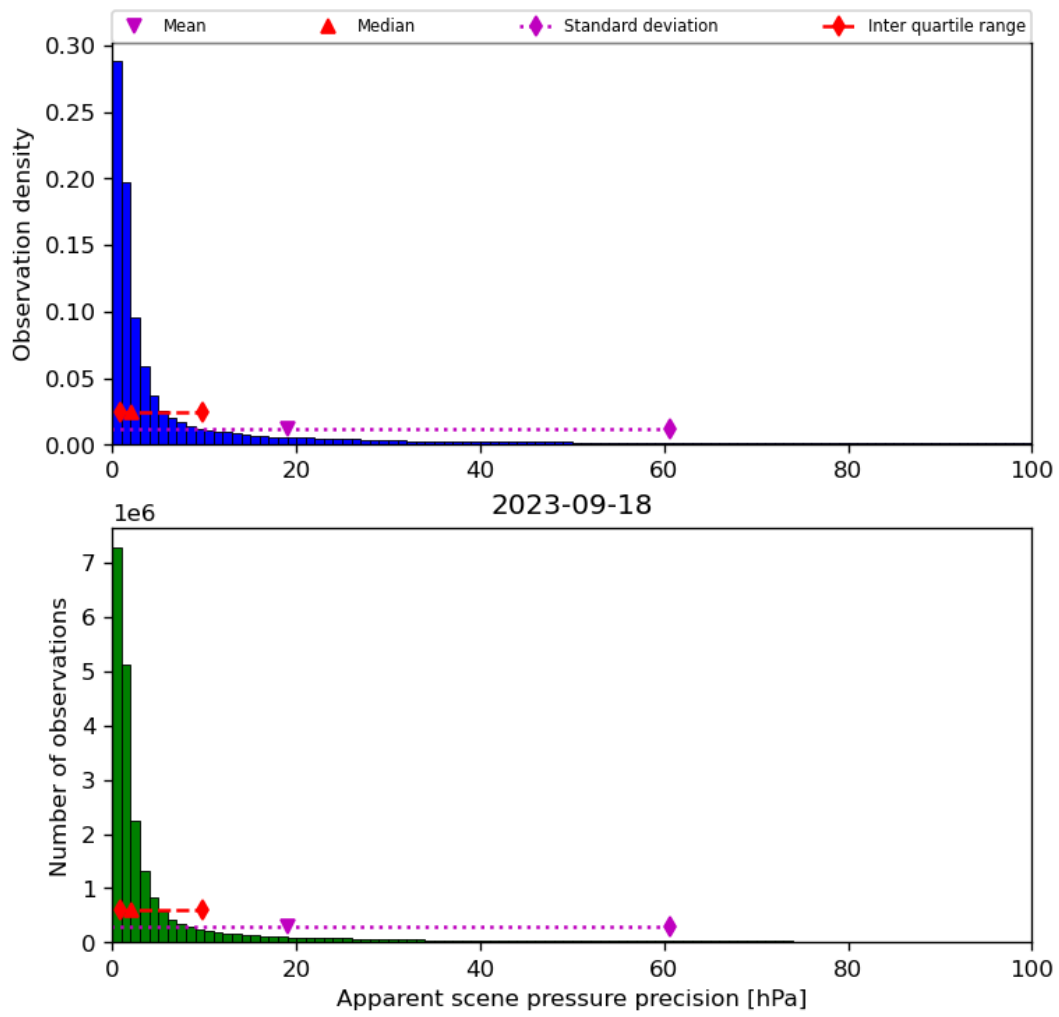
Figure 37: Histogram of “Apparent scene pressure precision” for 2023-09-17 to 2023-09-19
