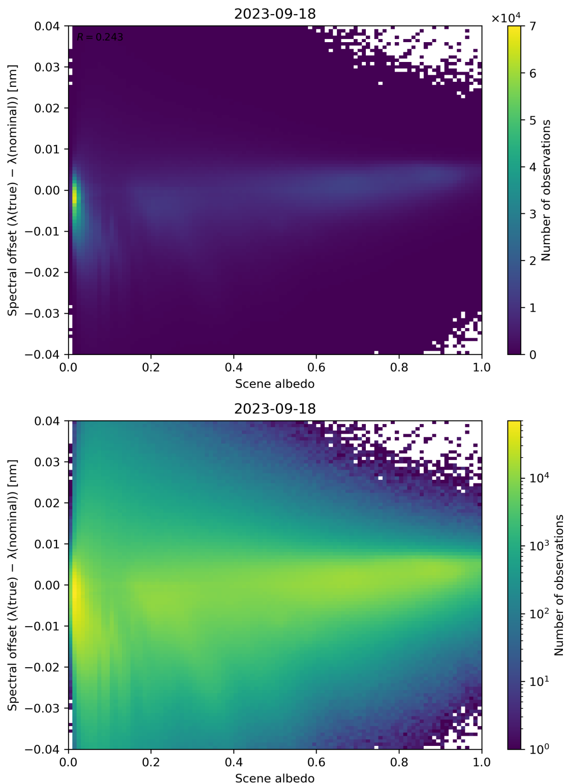
Figure 117: Scatter density plot of “Scene albedo” against “Spectral offset ( \lambda(\text{true}) - \lambda(\text{nominal}) )” for 2023-09-17 to 2023-09-19.
