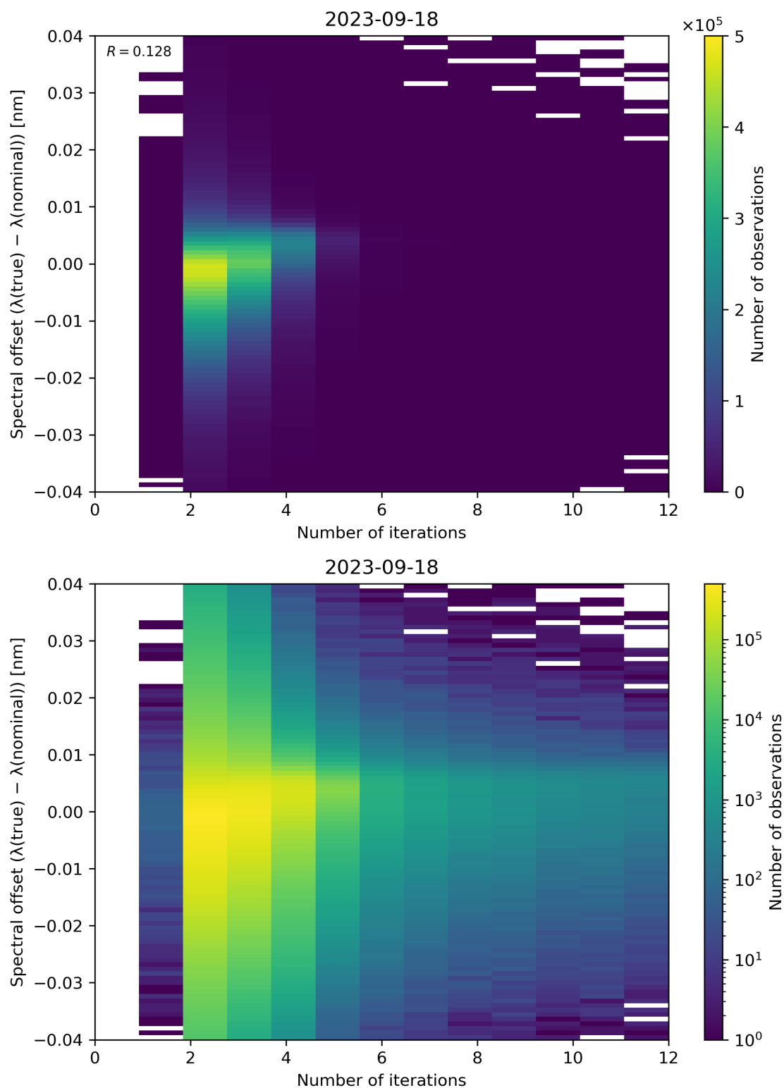
Figure 109: Scatter density plot of “Number of iterations” against “Spectral offset ( \lambda(\text{true}) - \lambda(\text{nominal}) )” for 2023-09-17 to 2023-09-19.
