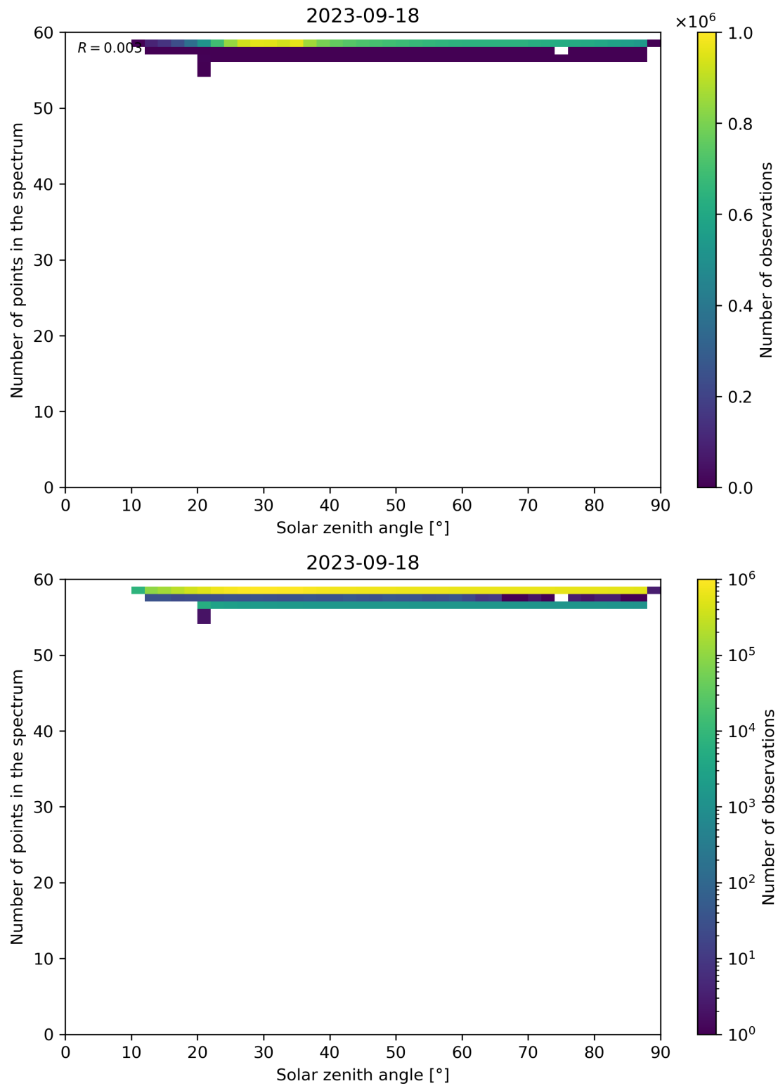
Figure 126: Scatter density plot of “Solar zenith angle” against “Number of points in the spectrum” for 2023-09-17 to 2023-09-19.
