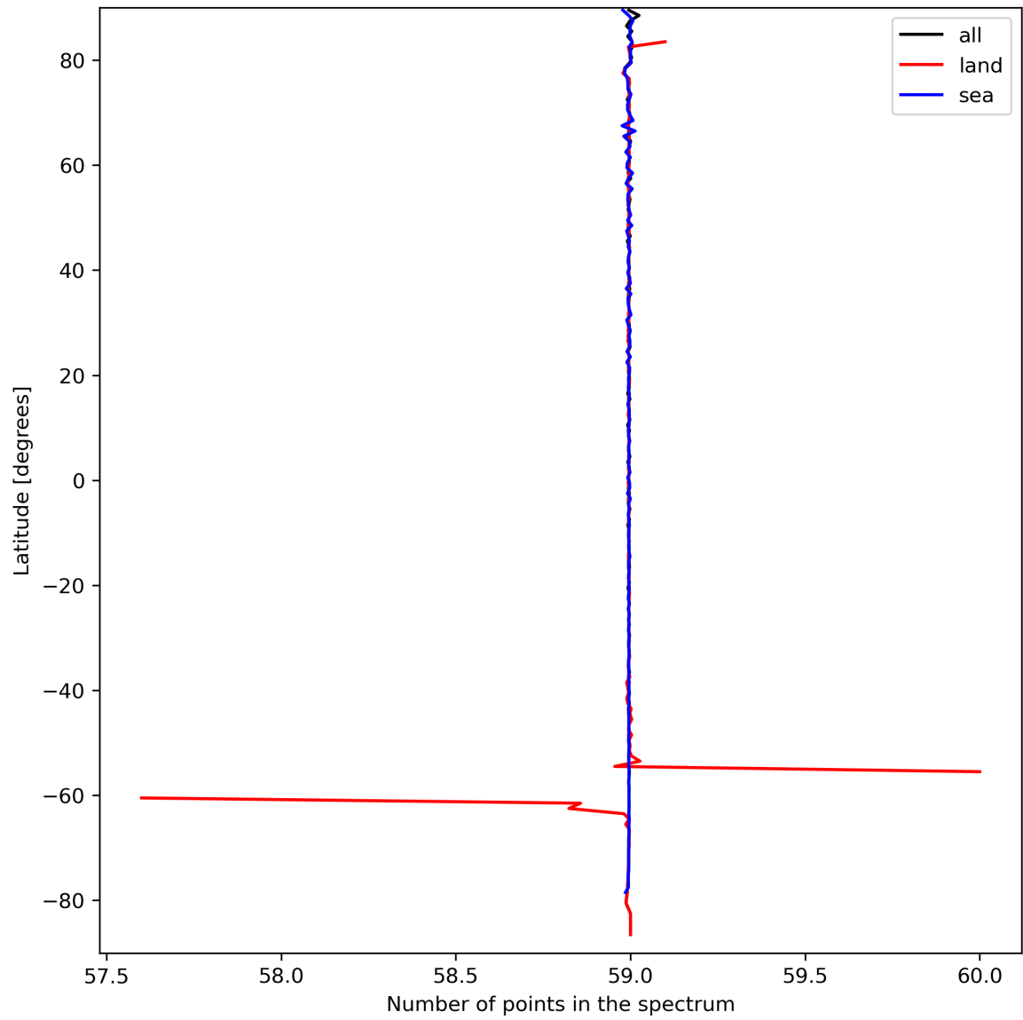
Figure 27: Zonal average of “Number of points in the spectrum” for 2023-09-17 to 2023-09-19.
