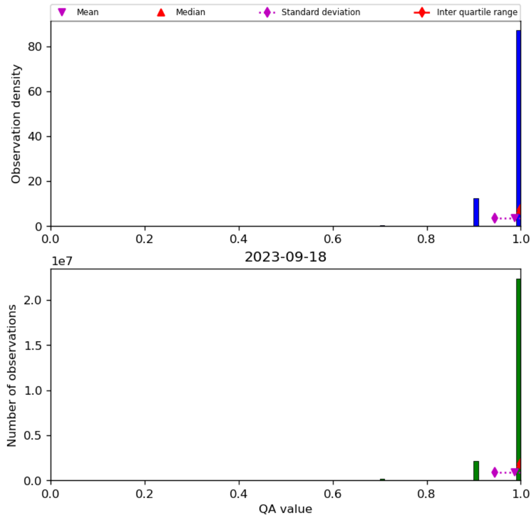
Figure 29: Histogram of “QA value” for 2023-09-17 to 2023-09-19
