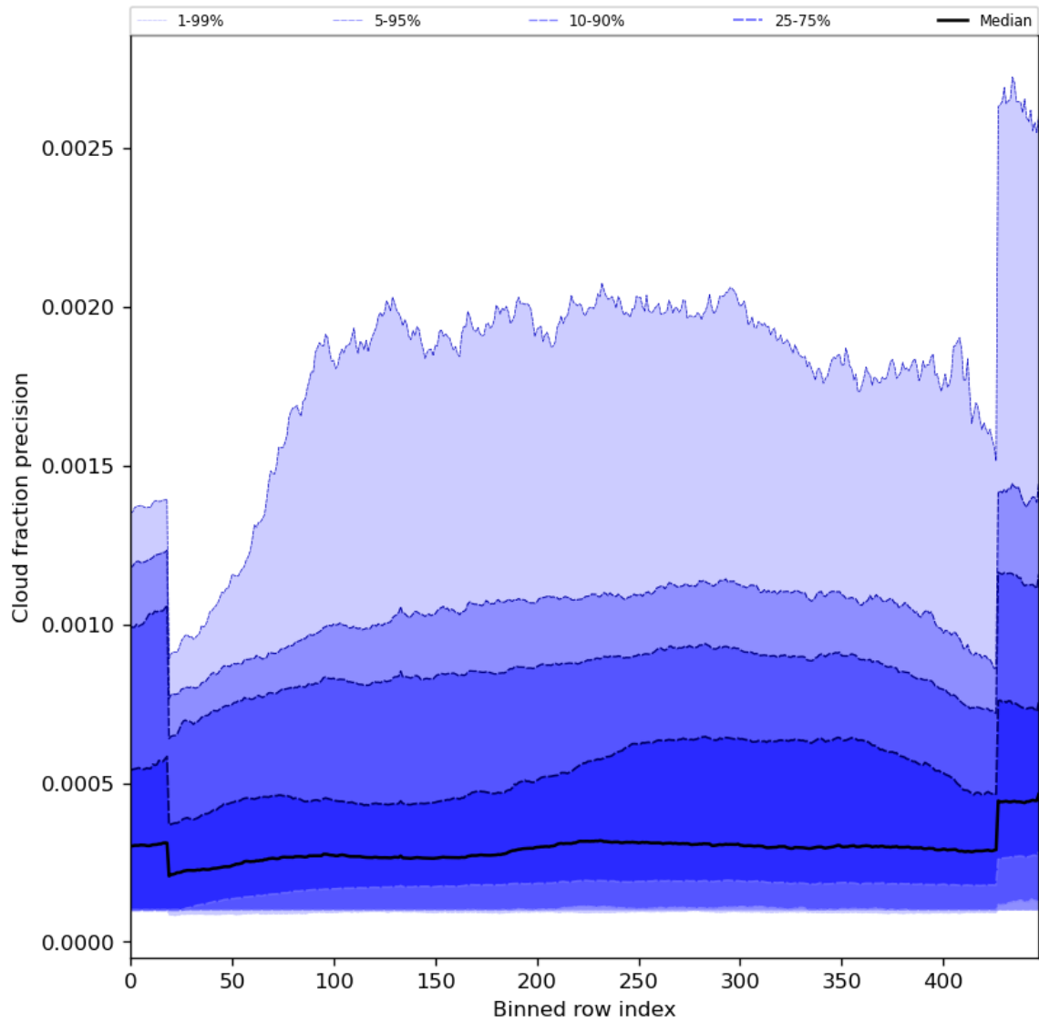
Figure 50: Along track statistics of “Cloud fraction precision” for 2023-09-17 to 2023-09-19
