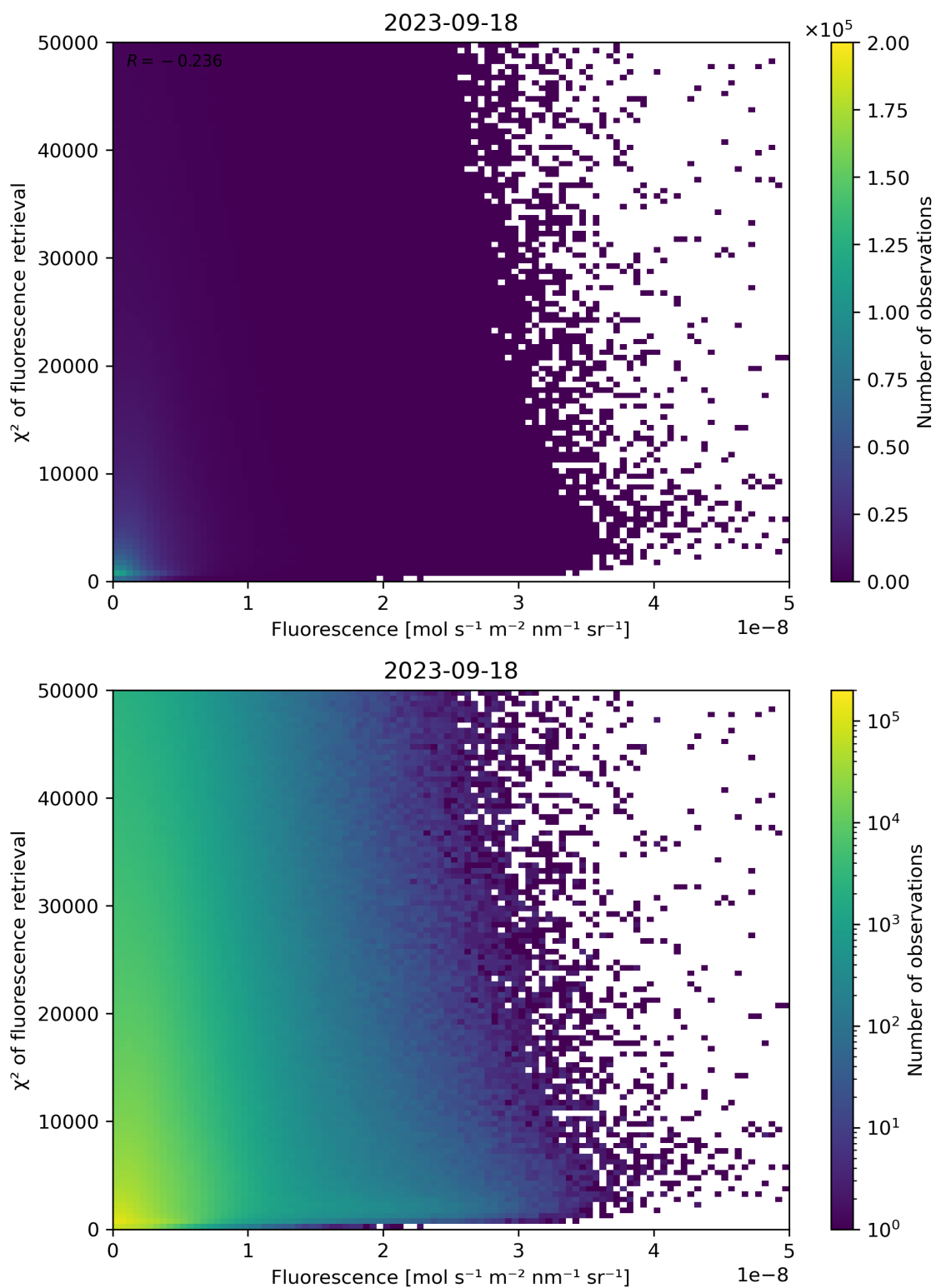
Figure 93: Scatter density plot of “Fluorescence” against “ \chi^2 of fluorescence retrieval” for 2023-09-17 to 2023-09-19.
