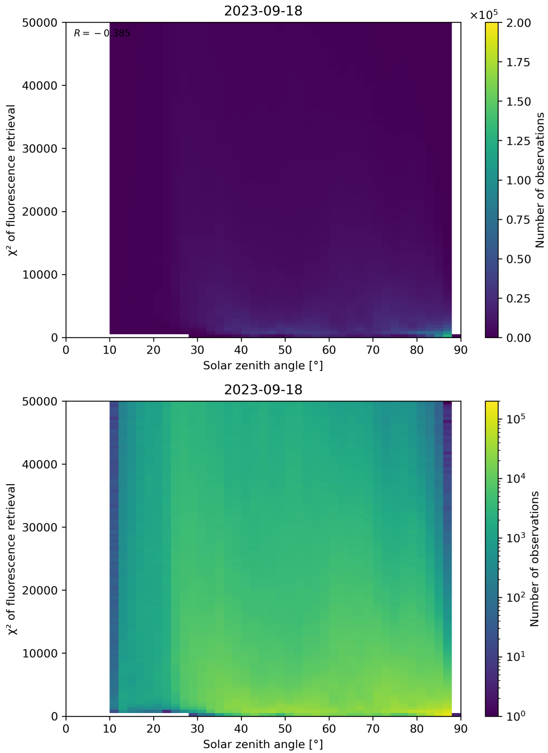
Figure 120: Scatter density plot of “Solar zenith angle” against “ \chi^2 of fluorescence retrieval” for 2023-09-17 to 2023-09-19.
