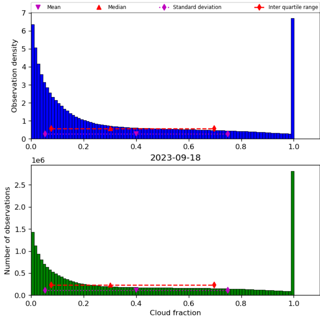
Figure 32: Histogram of “Cloud fraction” for 2023-09-17 to 2023-09-19
