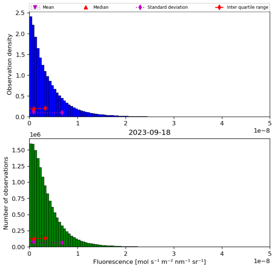
Figure 40: Histogram of “Fluorescence” for 2023-09-17 to 2023-09-19
