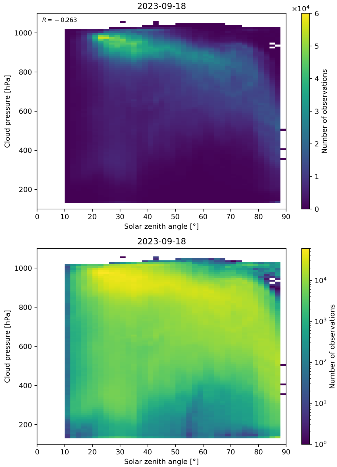
Figure 122: Scatter density plot of “Solar zenith angle” against “Cloud pressure” for 2023-09-17 to 2023-09-19.
