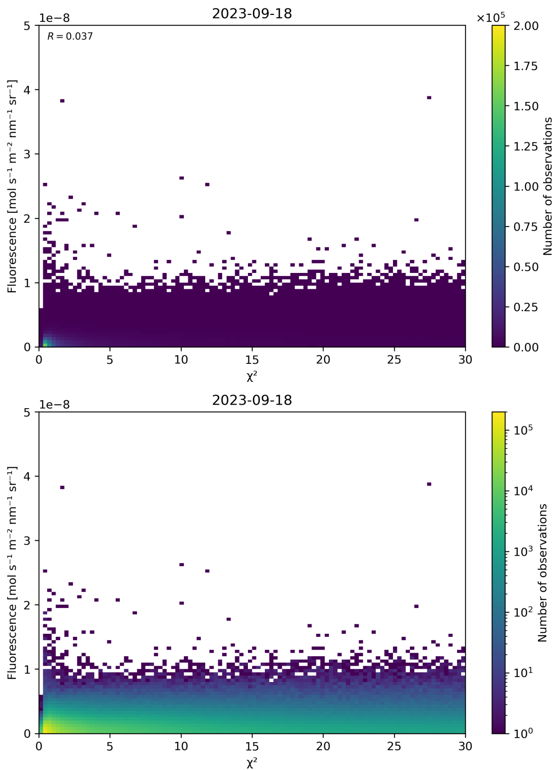
Figure 70: Scatter density plot of “ \chi^2 ” against “Fluorescence” for 2023-09-17 to 2023-09-19.
