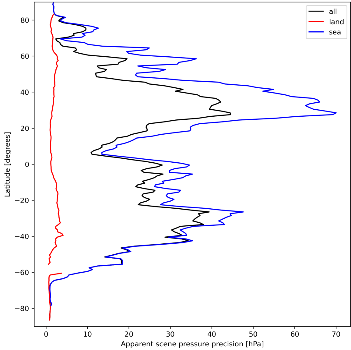
Figure 20: Zonal average of “Apparent scene pressure precision” for 2023-09-17 to 2023-09-19.
