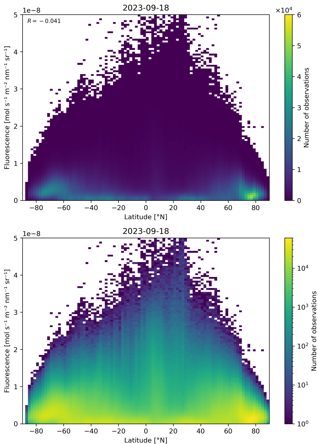
Figure 101: Scatter density plot of “Latitude” against “Fluorescence” for 2023-09-17 to 2023-09-19.
