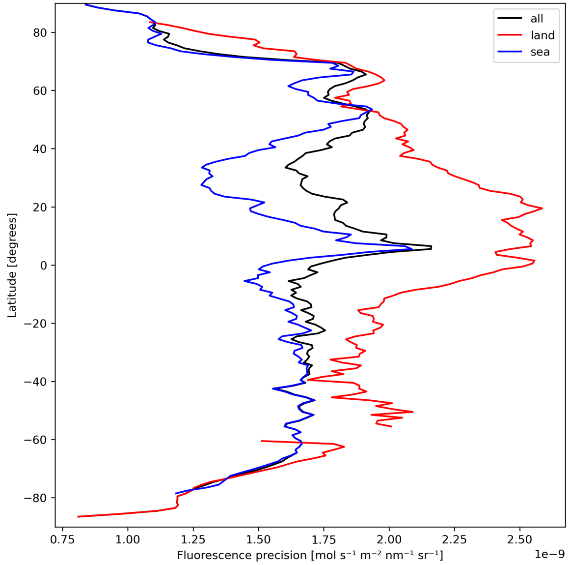
Figure 24: Zonal average of “Fluorescence precision” for 2023-09-17 to 2023-09-19.
