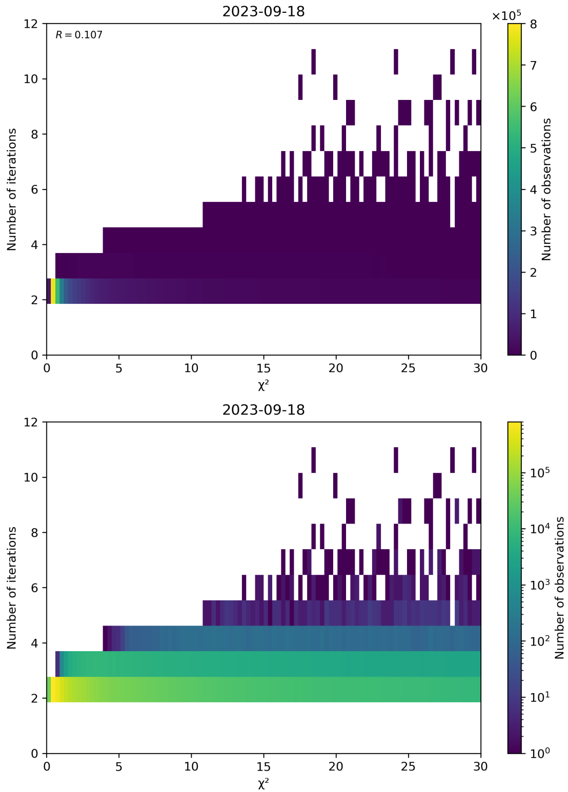
Figure 73: Scatter density plot of “ \chi^2 ” against “Number of iterations” for 2023-09-17 to 2023-09-19.
