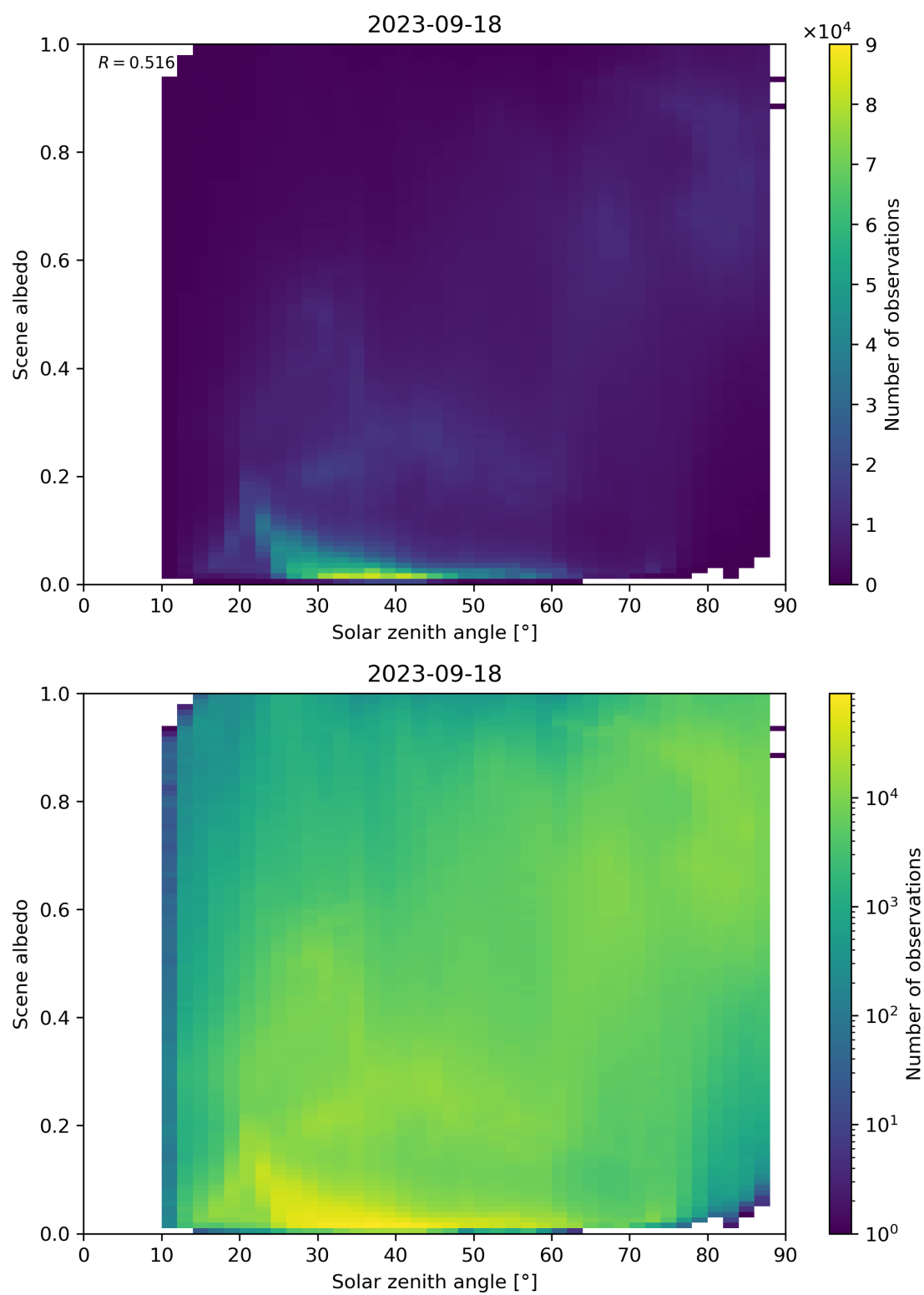
Figure 127: Scatter density plot of “Solar zenith angle” against “Scene albedo” for 2023-09-17 to 2023-09-19.
