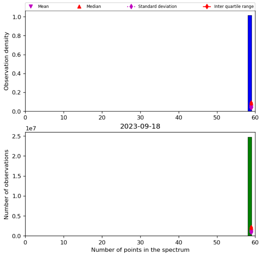
Figure 44: Histogram of “Number of points in the spectrum” for 2023-09-17 to 2023-09-19
