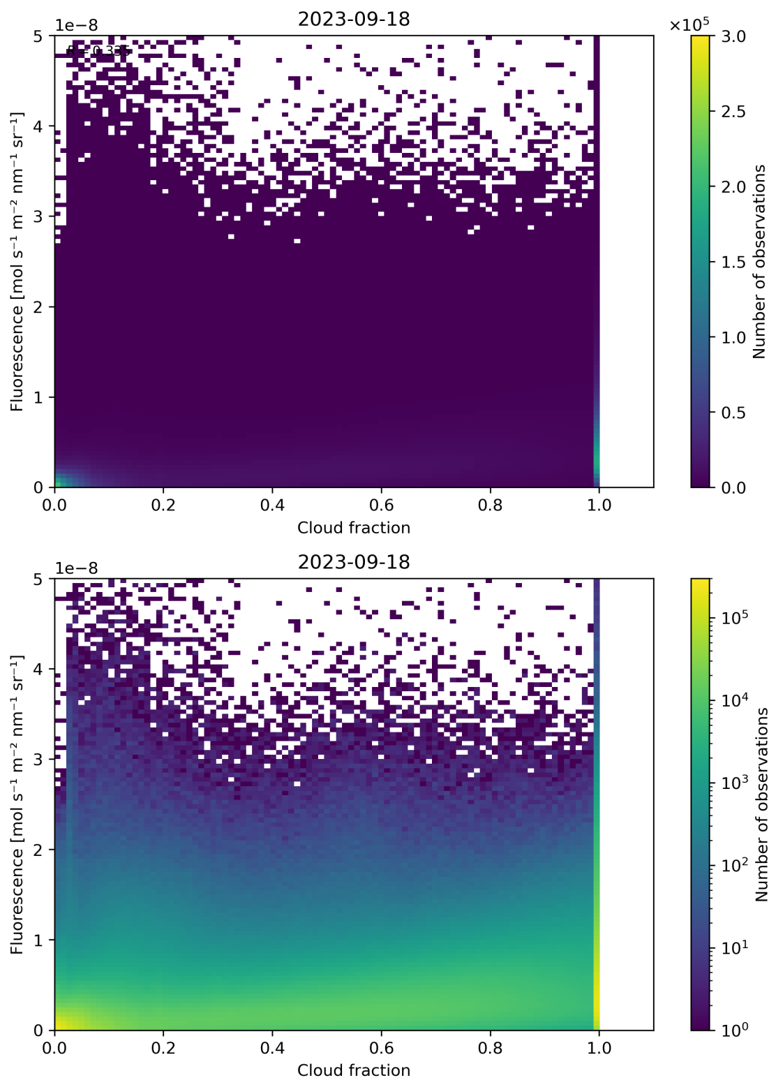
Figure 79: Scatter density plot of “Cloud fraction” against “Fluorescence” for 2023-09-17 to 2023-09-19.
