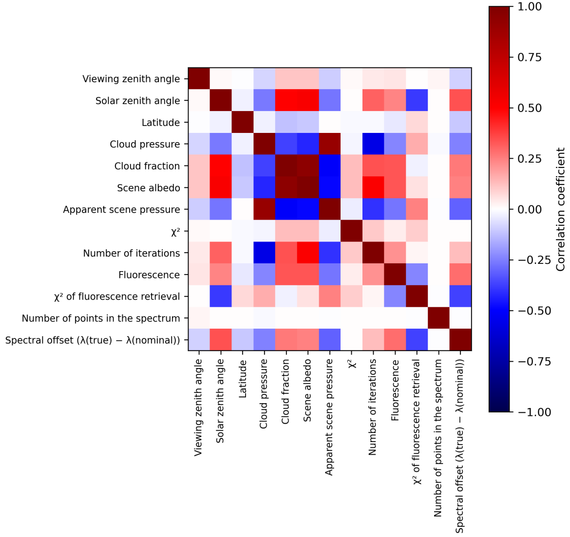
Figure 2: Map of correlation matrix for 2023-09-17 to 2023-09-19.
