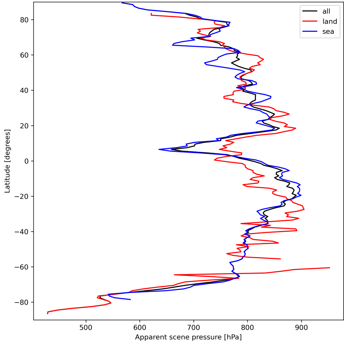
Figure 19: Zonal average of “Apparent scene pressure” for 2023-09-17 to 2023-09-19.
