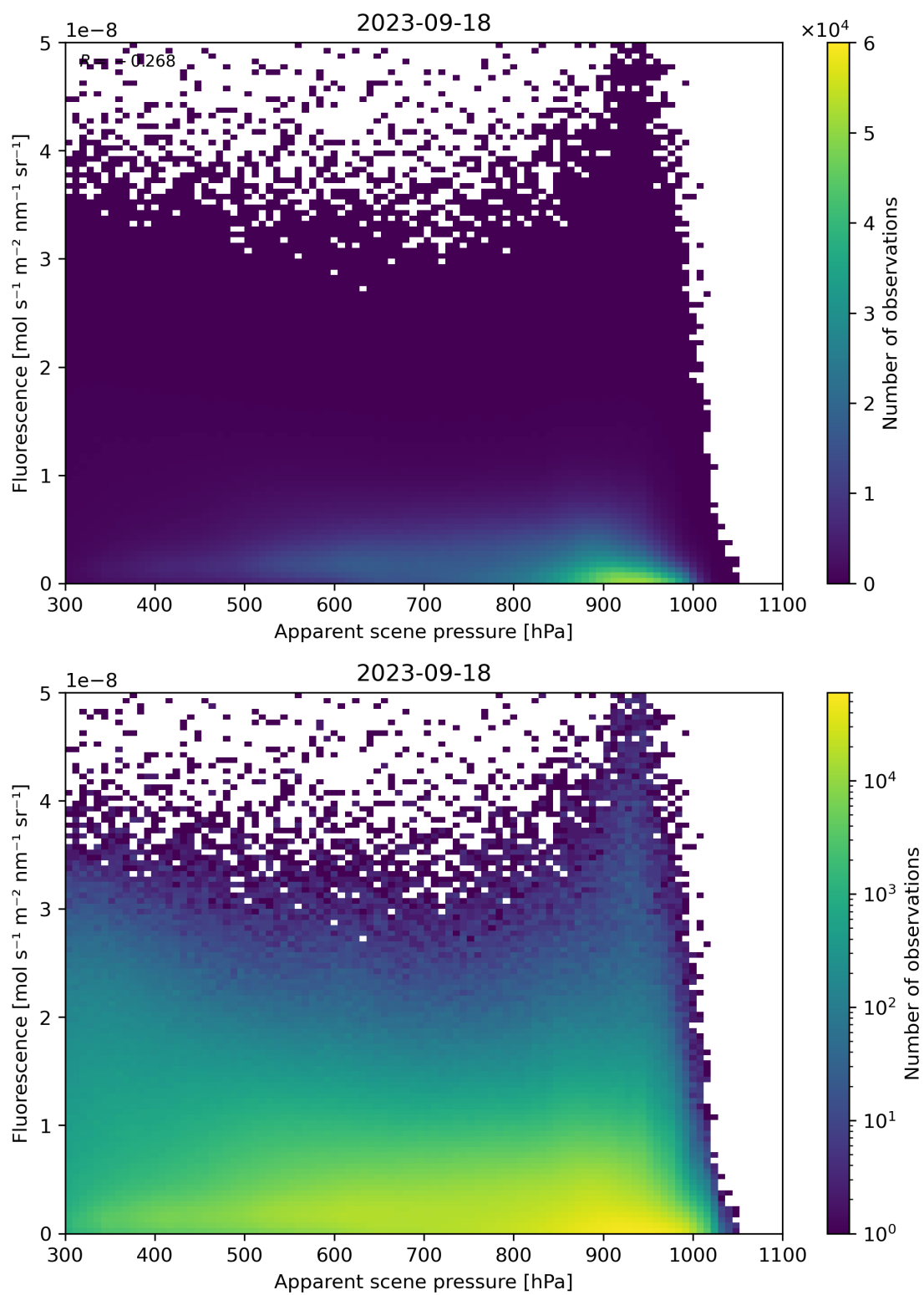
Figure 65: Scatter density plot of “Apparent scene pressure” against “Fluorescence” for 2023-09-17 to 2023-09-19.
