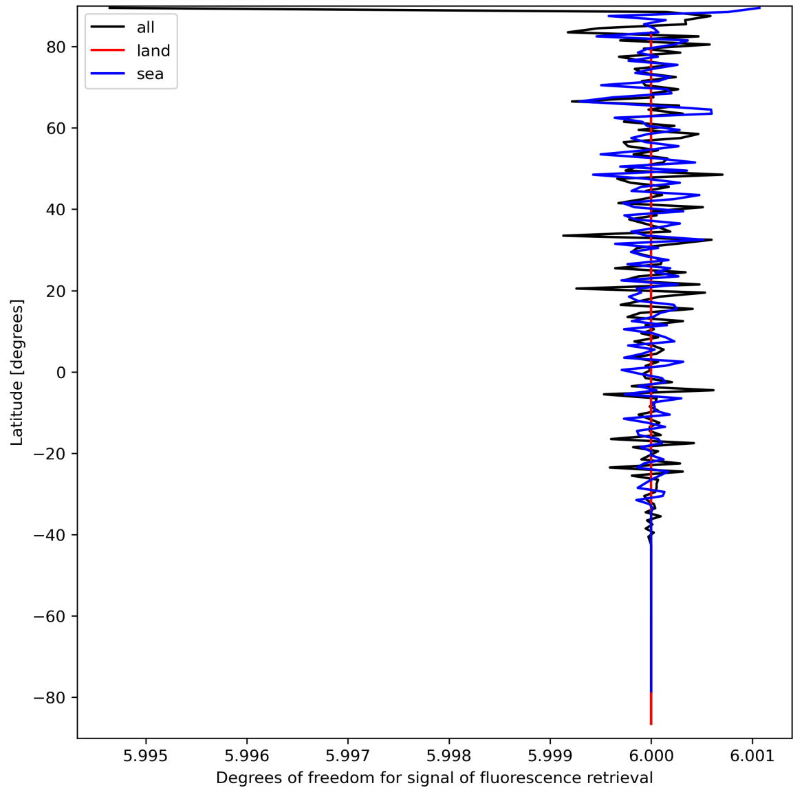
Figure 26: Zonal average of “Degrees of freedom for signal of fluorescence retrieval” for 2023-09-17 to 2023-09-19.
