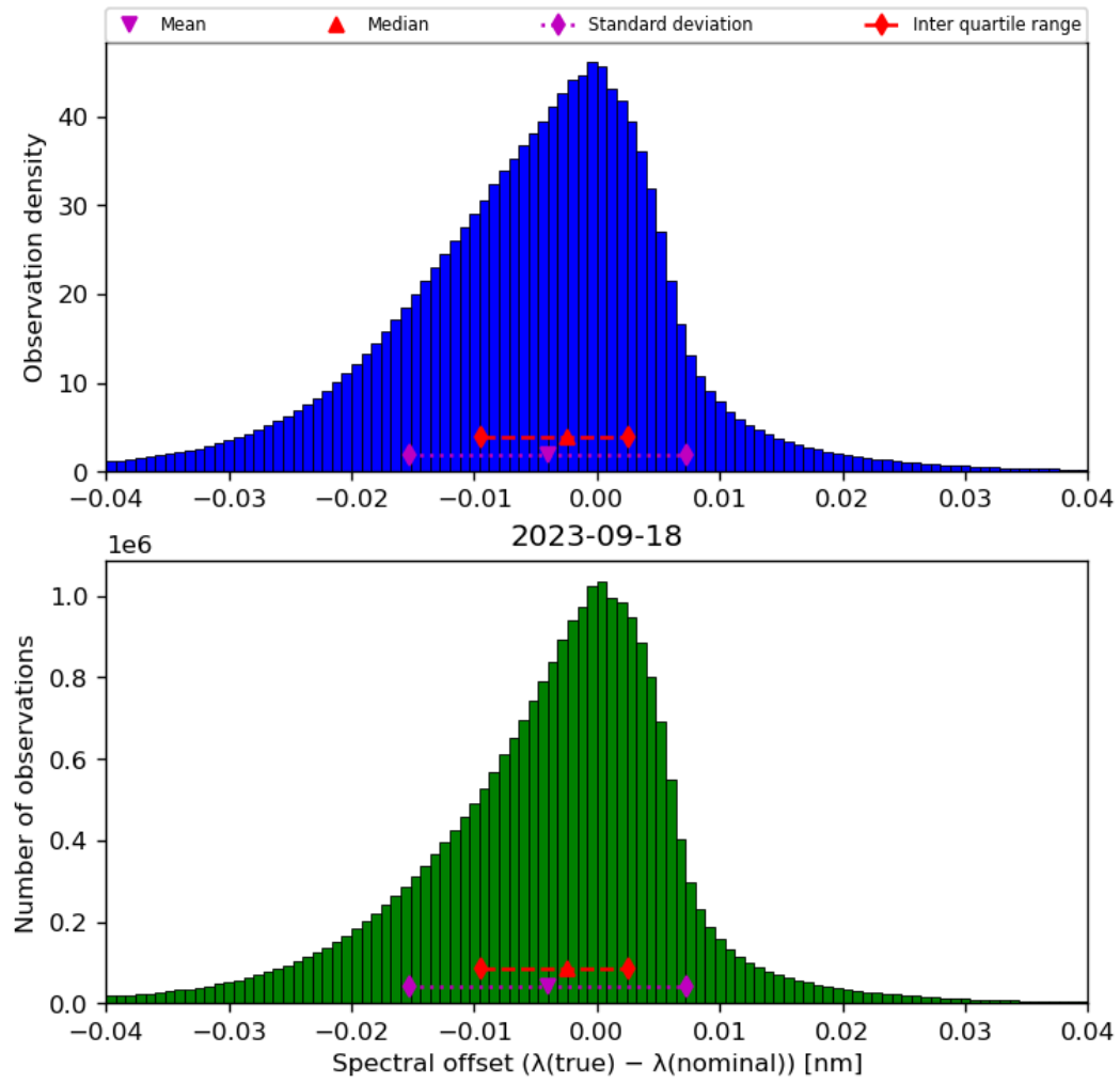
Figure 45: Histogram of “Spectral offset ( \lambda(\text{true}) - \lambda(\text{nominal}) )” for 2023-09-17 to 2023-09-19
