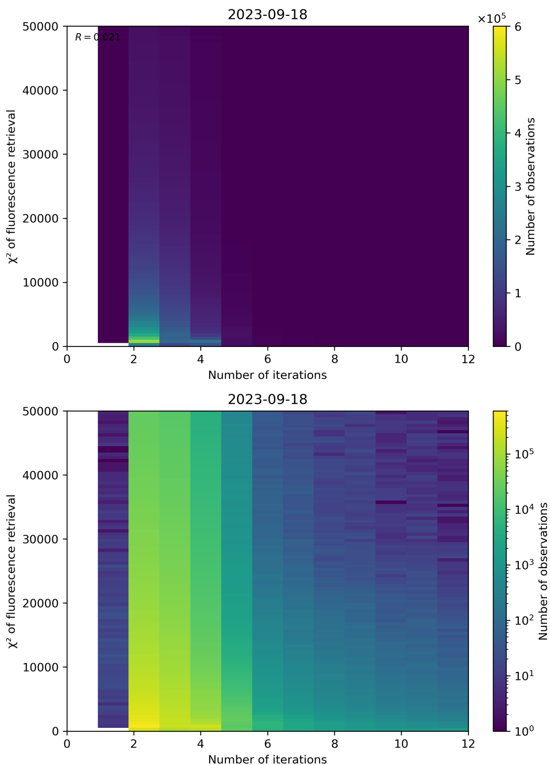
Figure 106: Scatter density plot of “Number of iterations” against “ \chi^2 of fluorescence retrieval” for 2023-09-17 to 2023-09-19.
