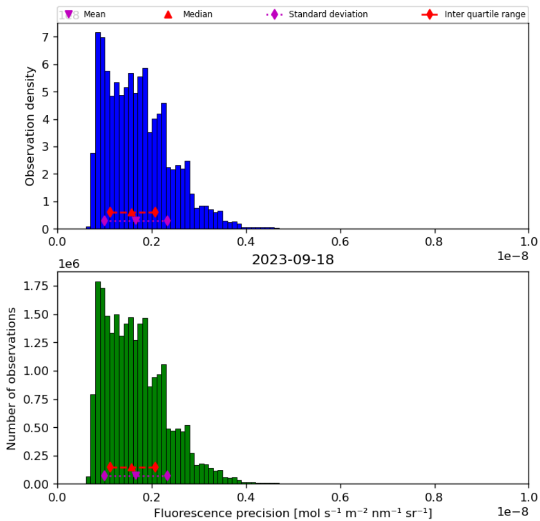
Figure 41: Histogram of “Fluorescence precision” for 2023-09-17 to 2023-09-19
