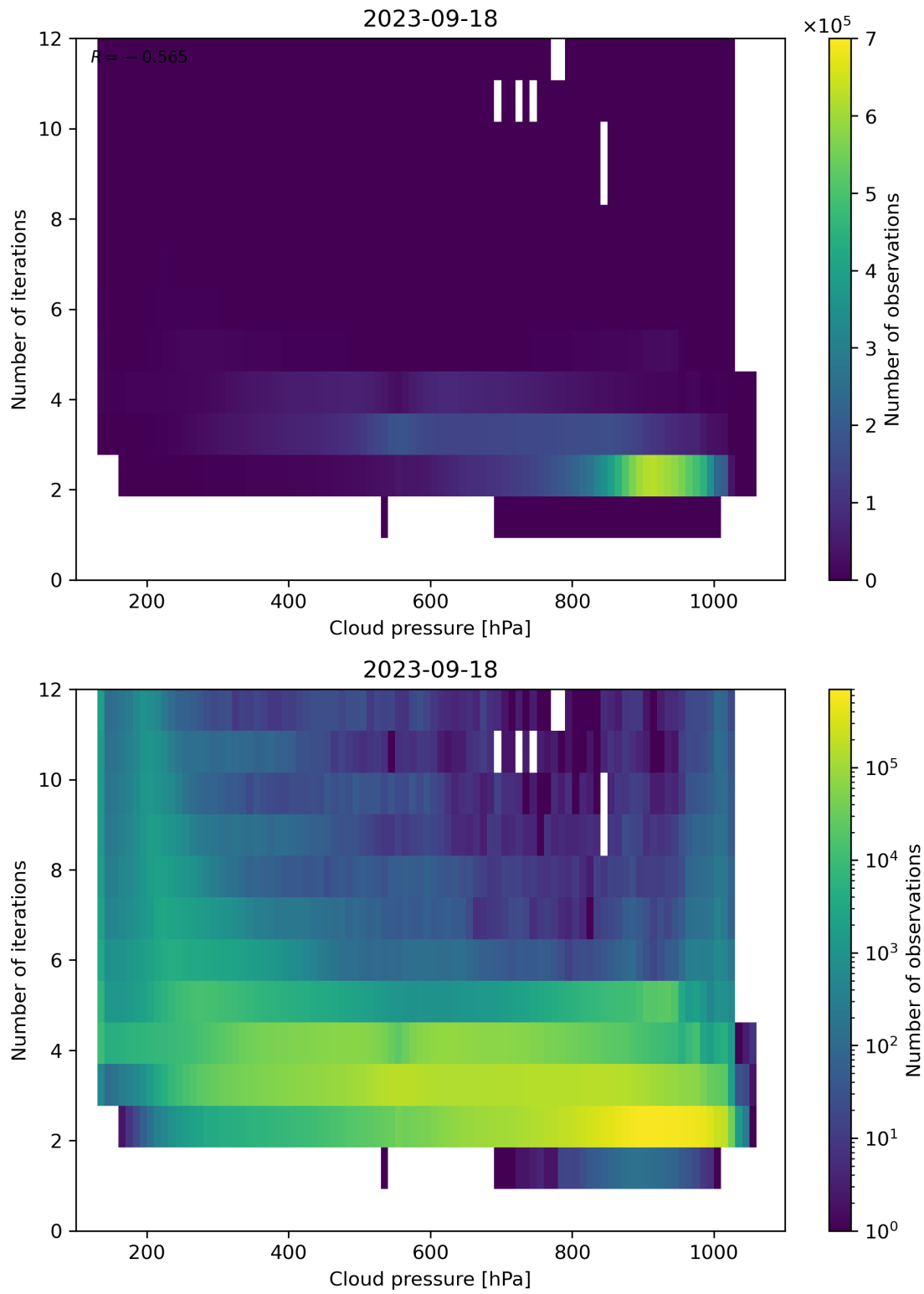
Figure 89: Scatter density plot of “Cloud pressure” against “Number of iterations” for 2023-09-17 to 2023-09-19.
