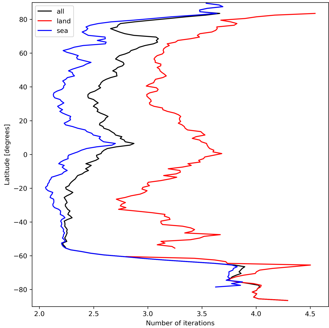
Figure 22: Zonal average of “Number of iterations” for 2023-09-17 to 2023-09-19.
