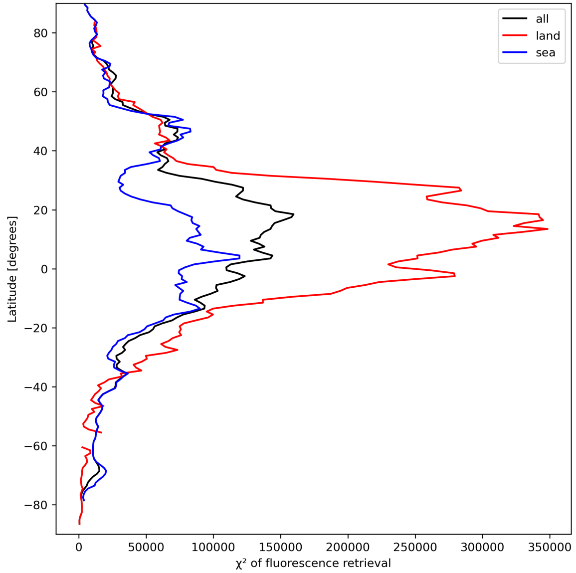
Figure 25: Zonal average of “ \chi^2 of fluorescence retrieval” for 2023-09-17 to 2023-09-19.
