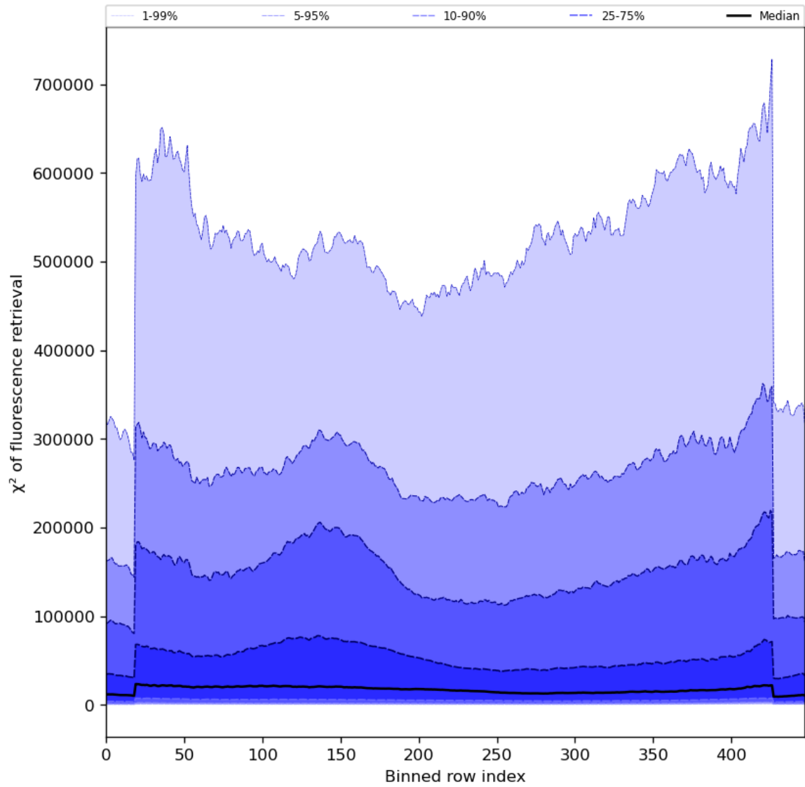
Figure 59: Along track statistics of “ \chi^2 of fluorescence retrieval” for 2023-09-17 to 2023-09-19
