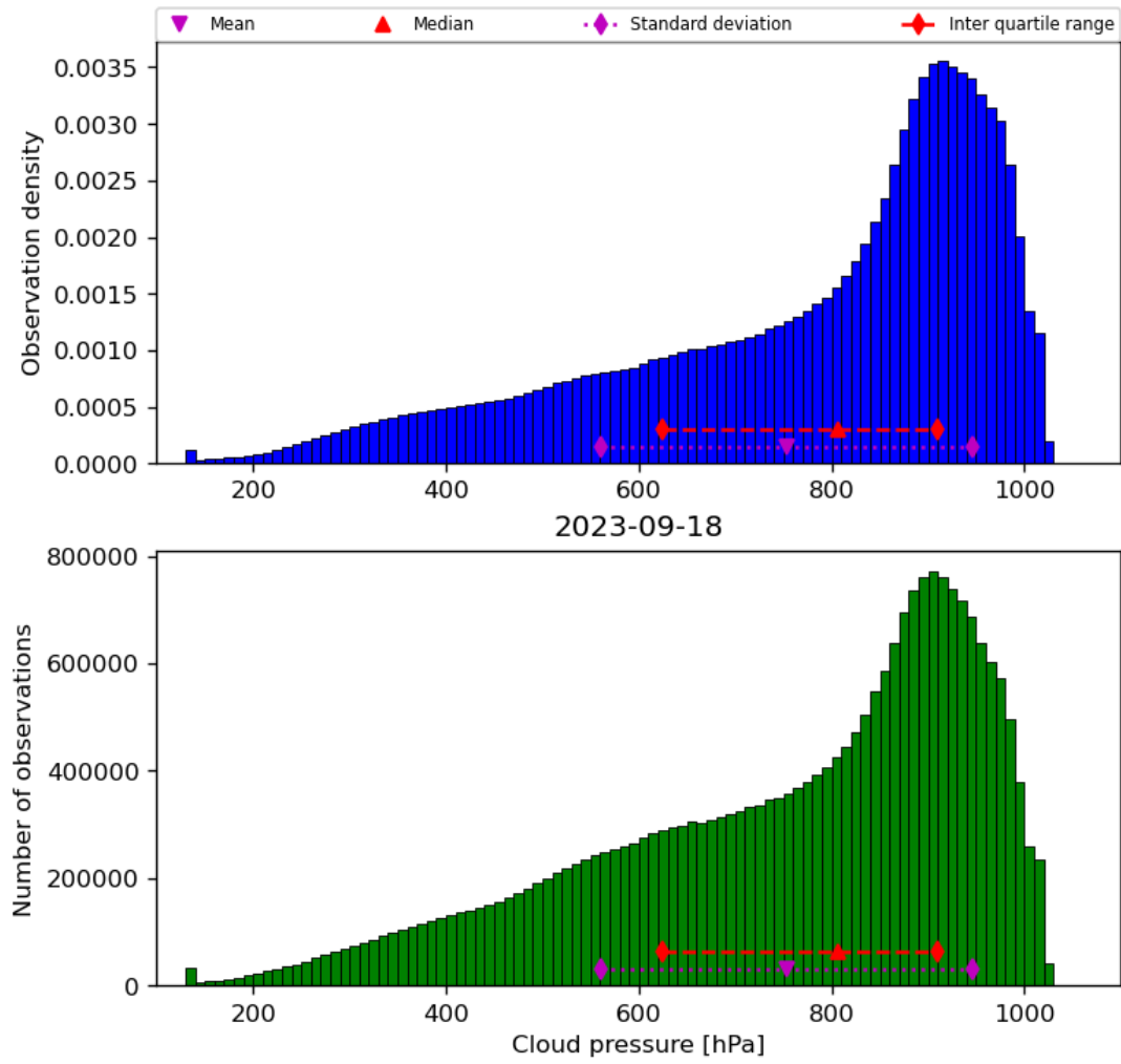
Figure 30: Histogram of “Cloud pressure” for 2023-09-17 to 2023-09-19
