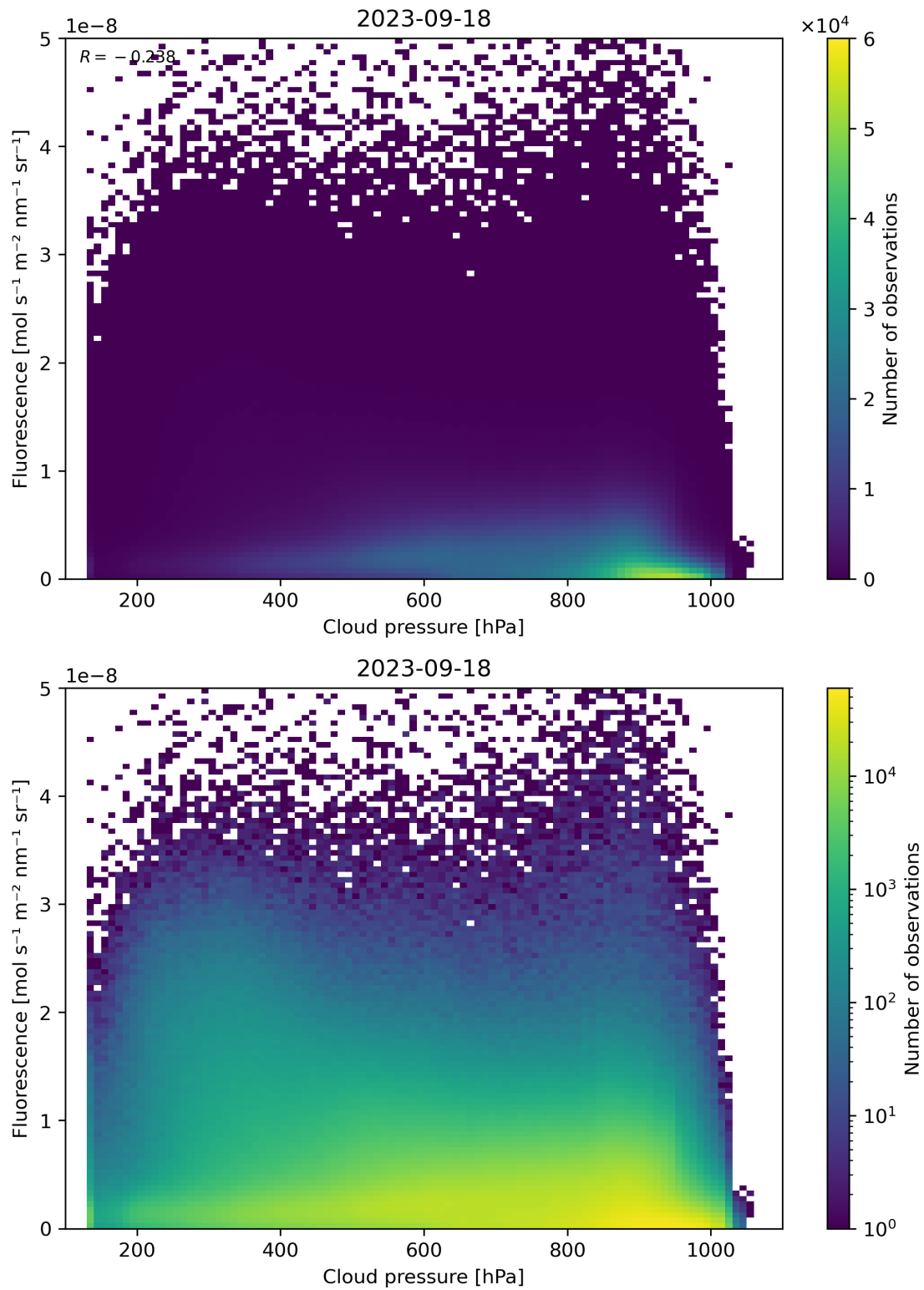
Figure 88: Scatter density plot of “Cloud pressure” against “Fluorescence” for 2023-09-17 to 2023-09-19.
