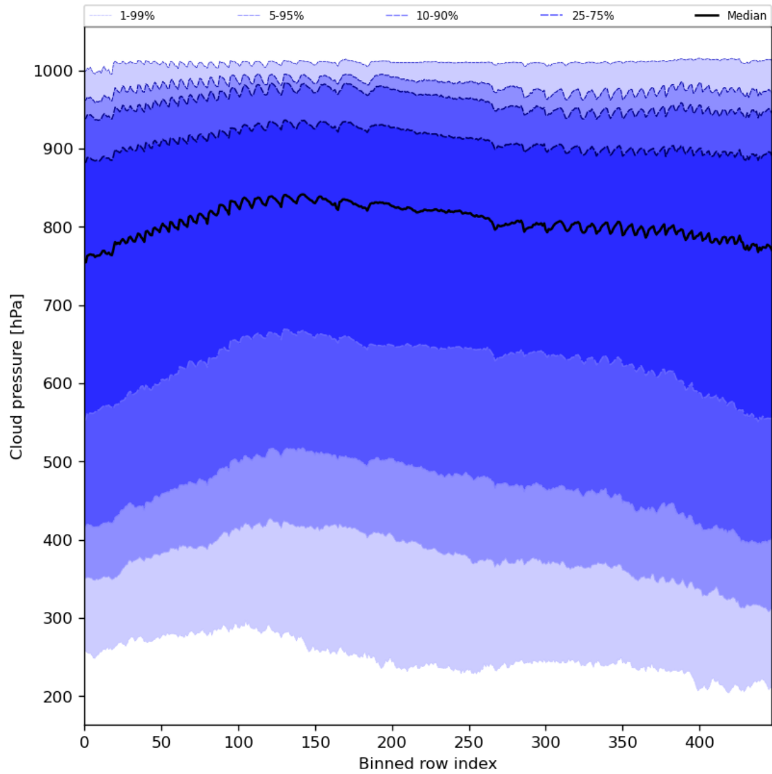
Figure 47: Along track statistics of “Cloud pressure” for 2023-09-17 to 2023-09-19
