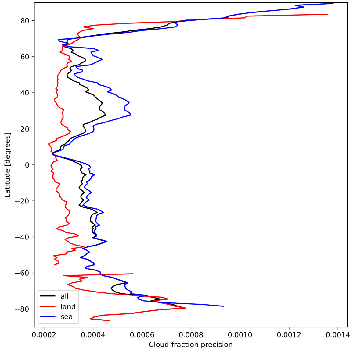
Figure 16: Zonal average of “Cloud fraction precision” for 2023-09-17 to 2023-09-19.
