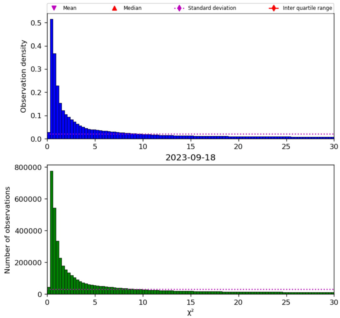
Figure 38: Histogram of “ \chi^2 ” for 2023-09-17 to 2023-09-19
