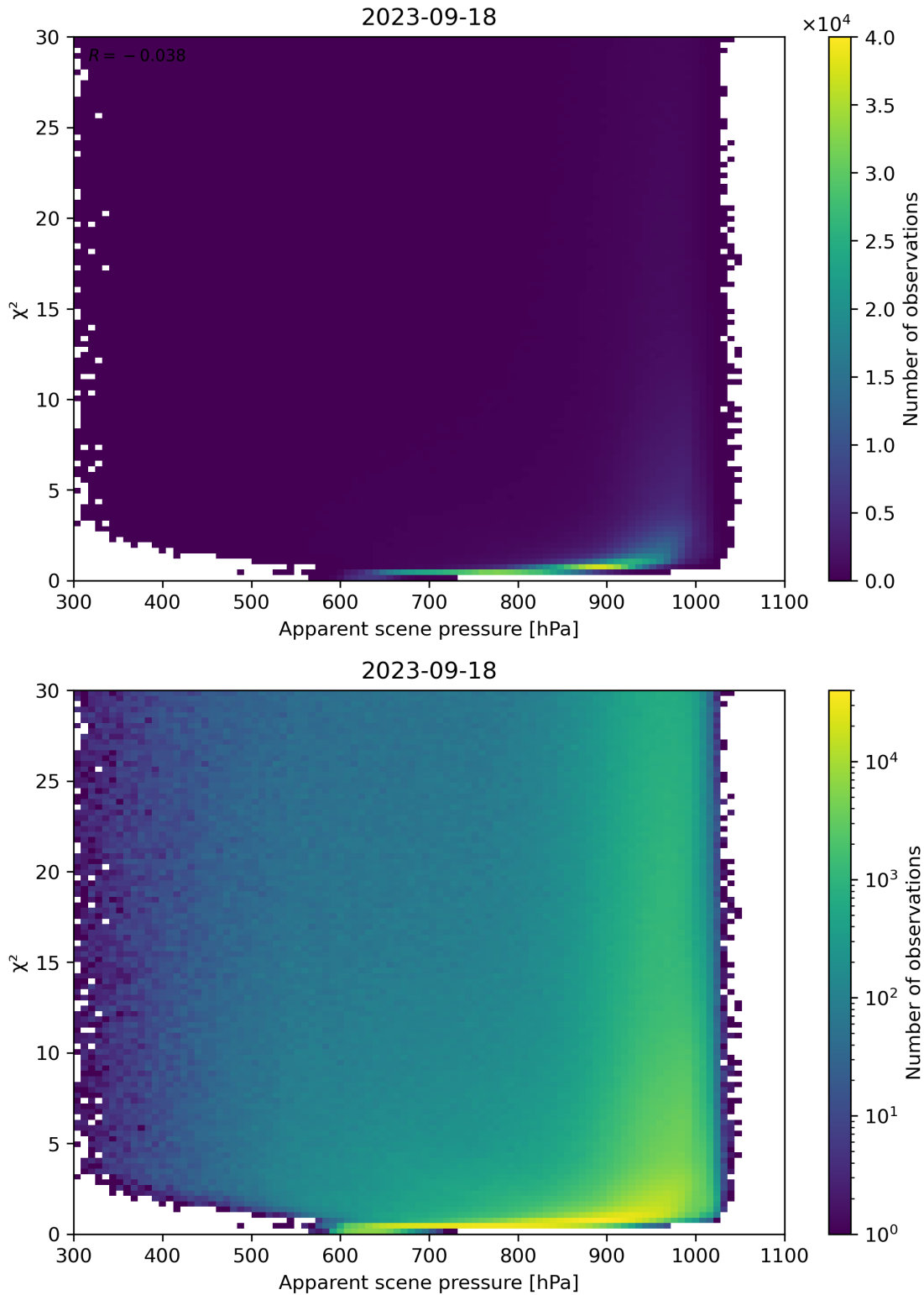
Figure 63: Scatter density plot of “Apparent scene pressure” against “ \chi^2 ” for 2023-09-17 to 2023-09-19.
