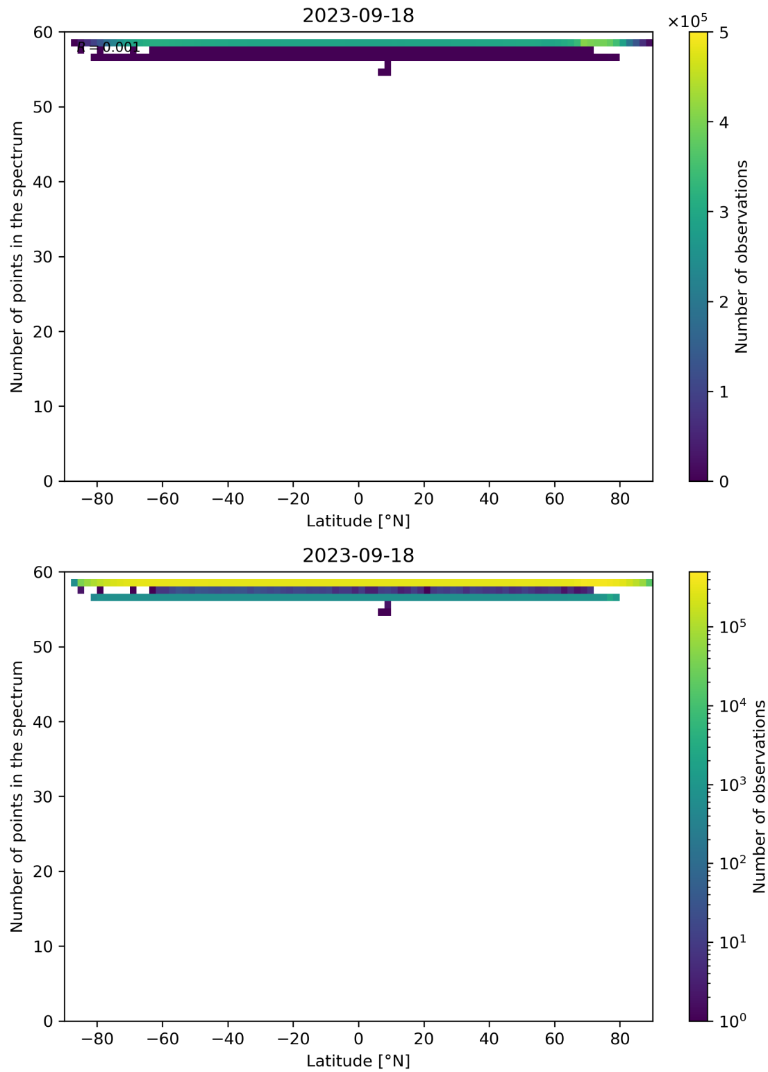
Figure 103: Scatter density plot of “Latitude” against “Number of points in the spectrum” for 2023-09-17 to 2023-09-19.
