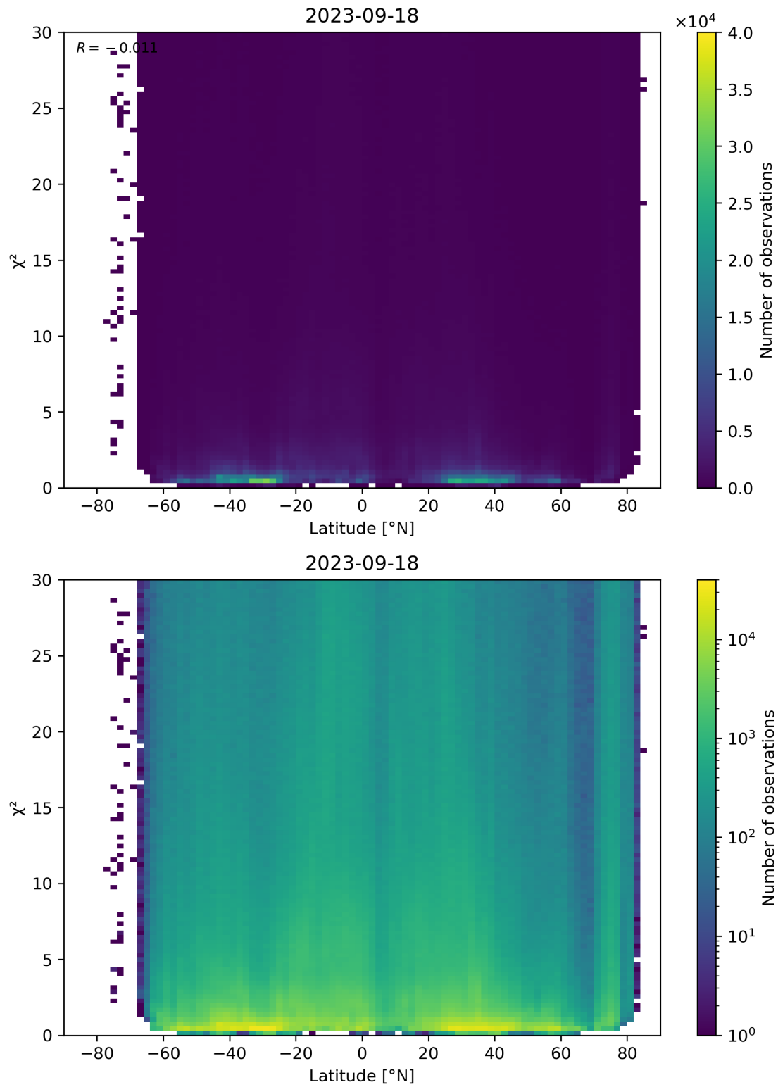
Figure 97: Scatter density plot of “Latitude” against “ \chi^2 ” for 2023-09-17 to 2023-09-19.
