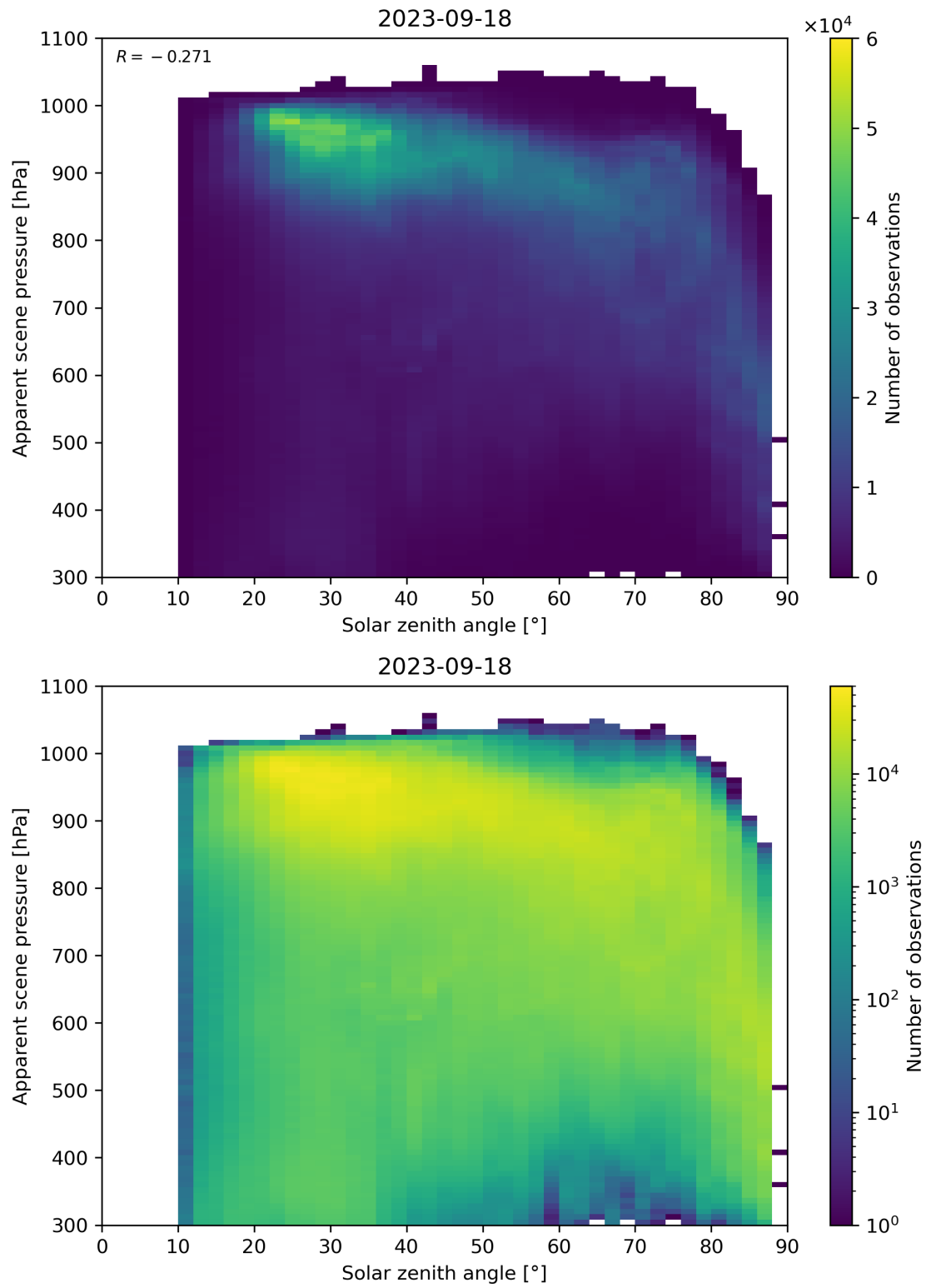
Figure 118: Scatter density plot of “Solar zenith angle” against “Apparent scene pressure” for 2023-09-17 to 2023-09-19.
