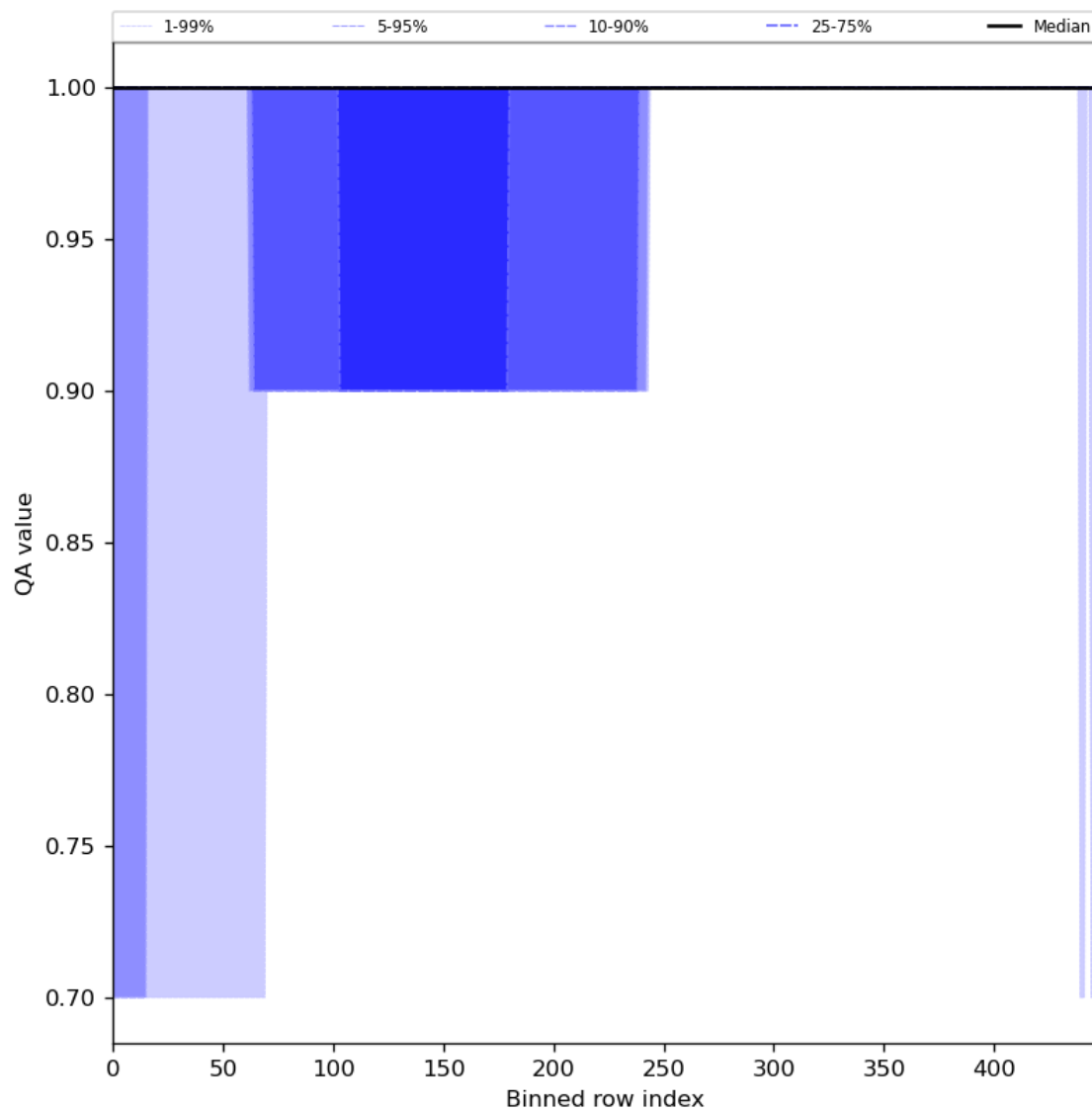
Figure 46: Along track statistics of “QA value” for 2023-09-17 to 2023-09-19
