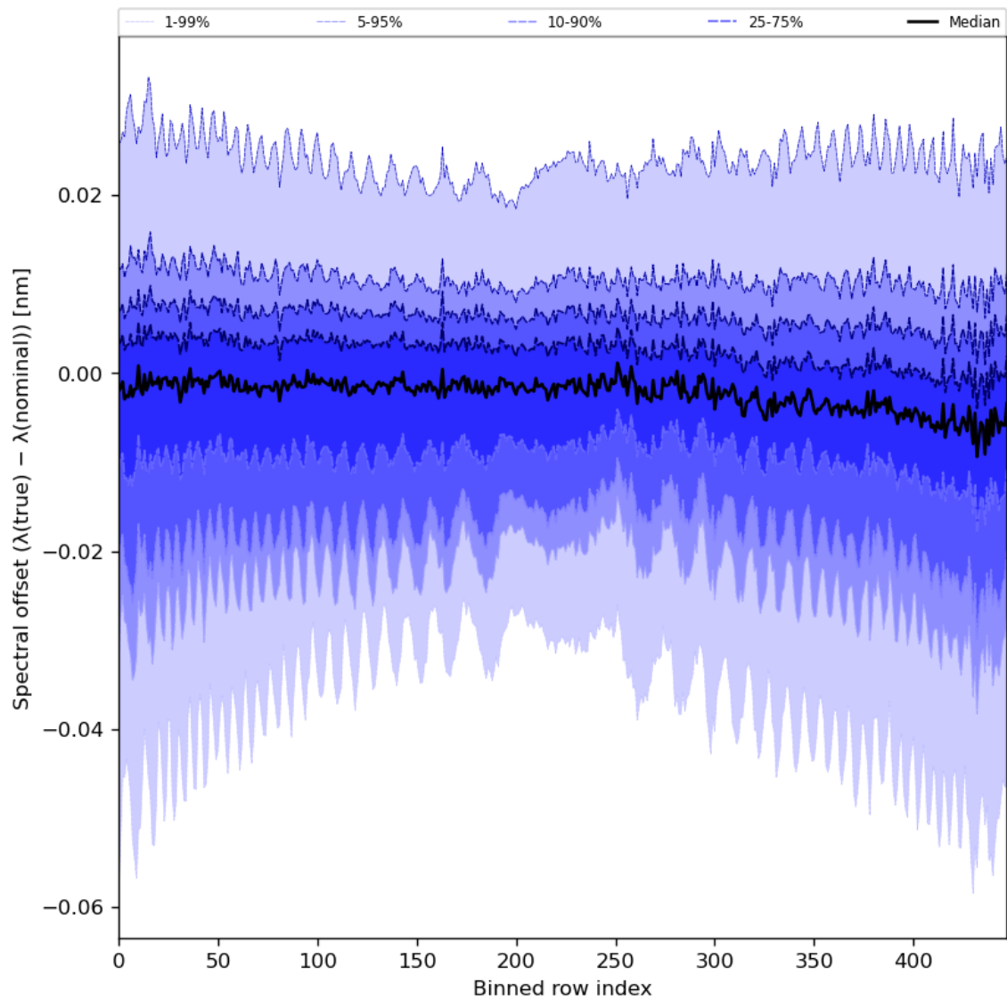
Figure 62: Along track statistics of “Spectral offset ( \lambda(\text{true}) - \lambda(\text{nominal}) )” for 2023-09-17 to 2023-09-19
