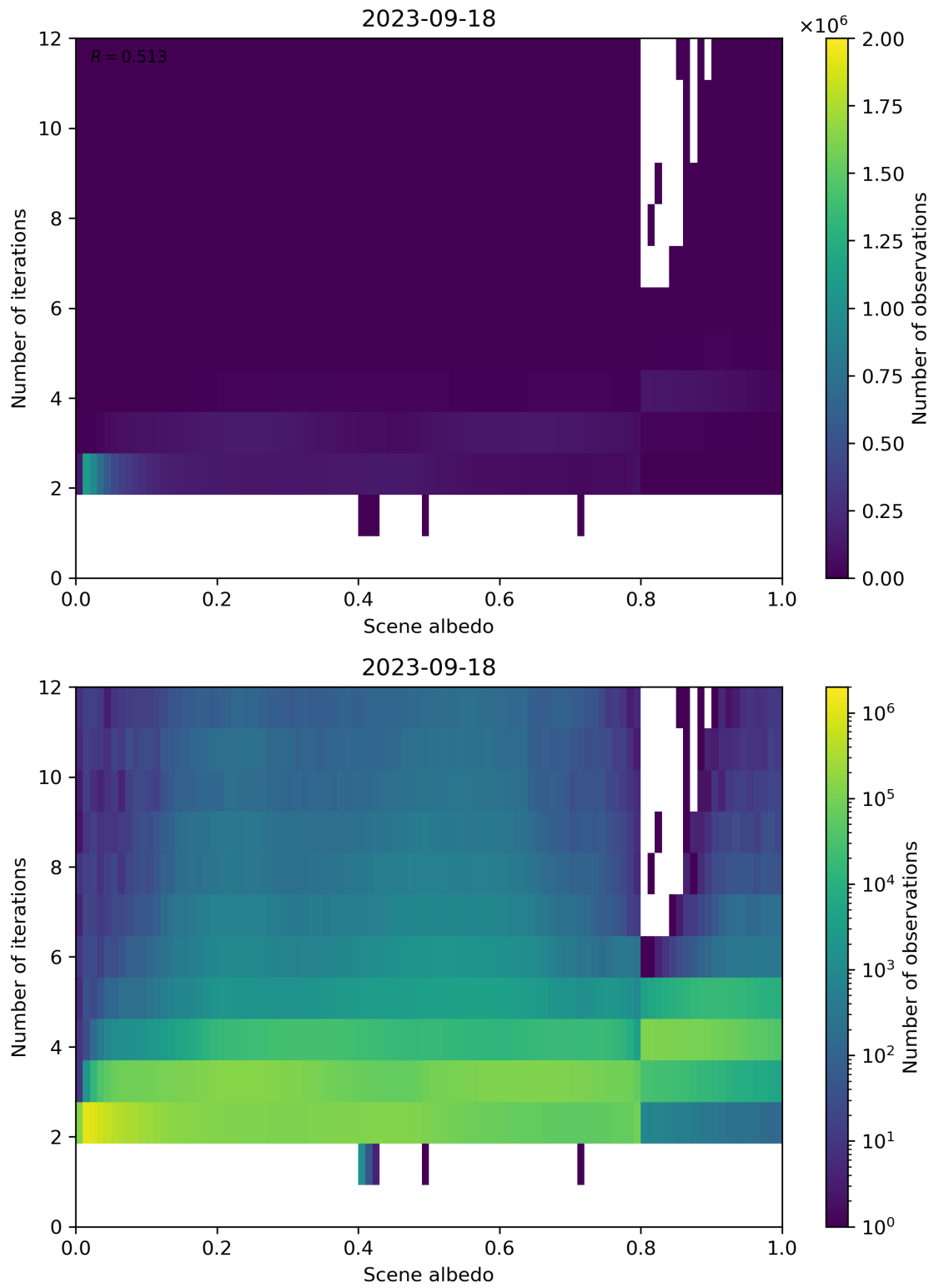
Figure 115: Scatter density plot of “Scene albedo” against “Number of iterations” for 2023-09-17 to 2023-09-19.
