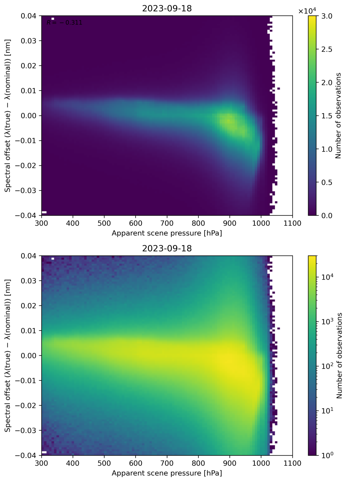
Figure 68: Scatter density plot of “Apparent scene pressure” against “Spectral offset ( \lambda(\text{true}) - \lambda(\text{nominal}) )” for 2023-09-17 to 2023-09-19.
