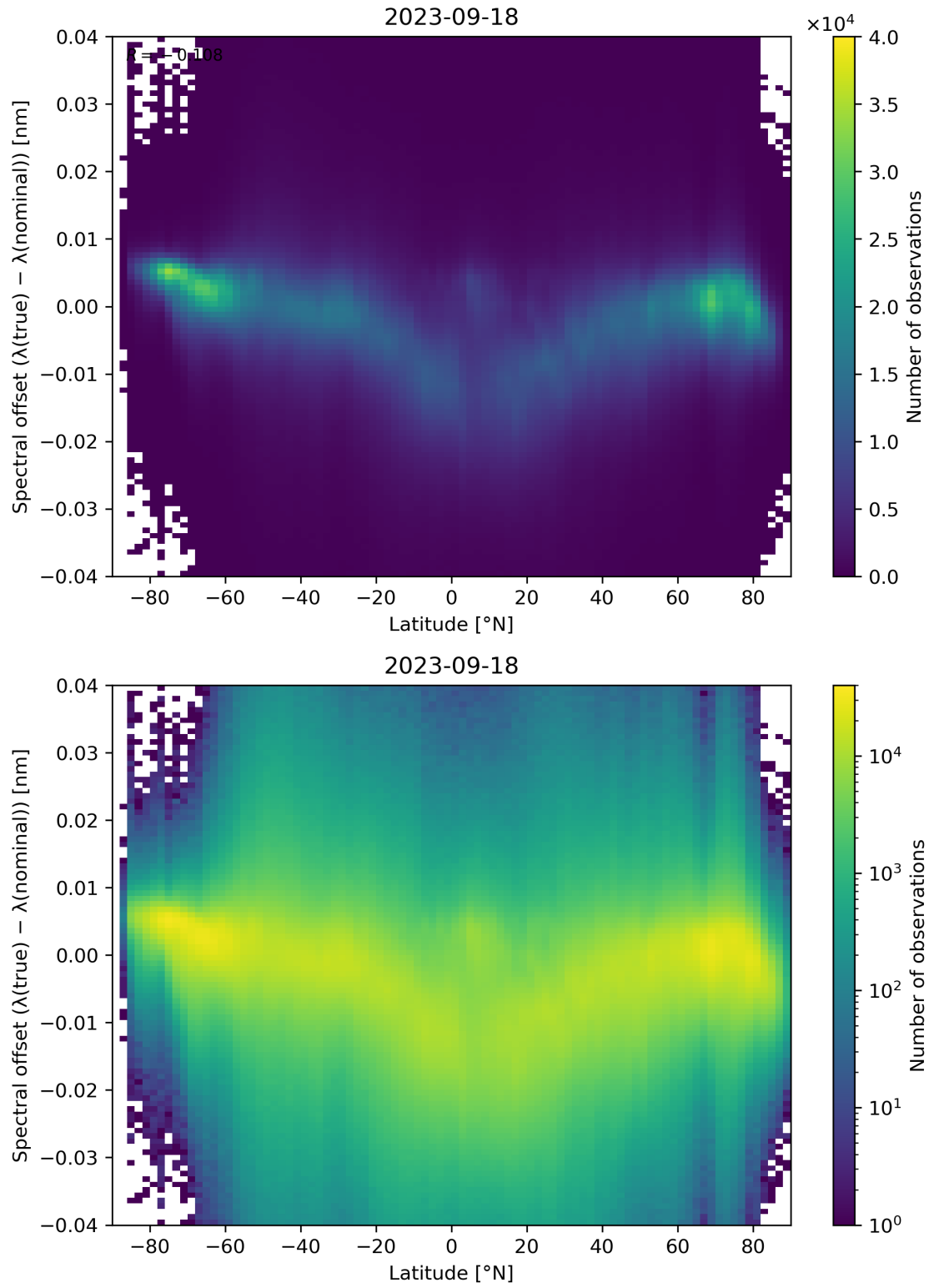
Figure 105: Scatter density plot of “Latitude” against “Spectral offset ( \lambda(\text{true}) - \lambda(\text{nominal}) )” for 2023-09-17 to 2023-09-19.
