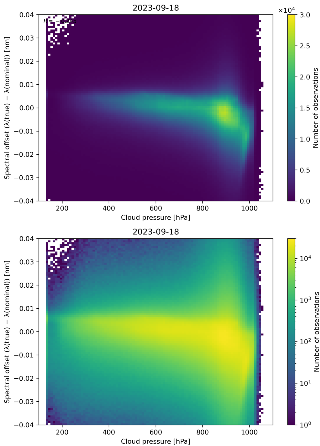
Figure 92: Scatter density plot of “Cloud pressure” against “Spectral offset ( \lambda(\text{true}) - \lambda(\text{nominal}) )” for 2023-09-17 to 2023-09-19.
