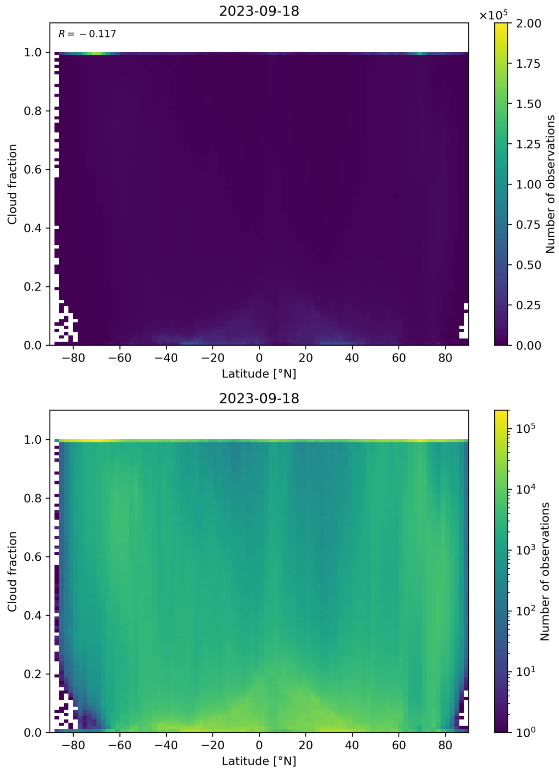
Figure 99: Scatter density plot of “Latitude” against “Cloud fraction” for 2023-09-17 to 2023-09-19.
