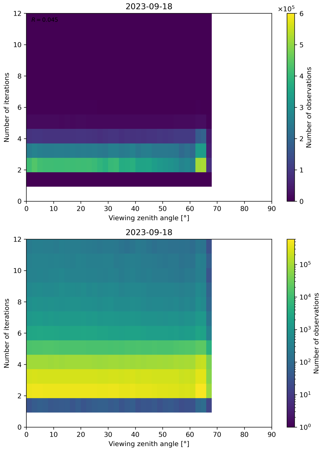
Figure 136: Scatter density plot of “Viewing zenith angle” against “Number of iterations” for 2023-09-17 to 2023-09-19.
