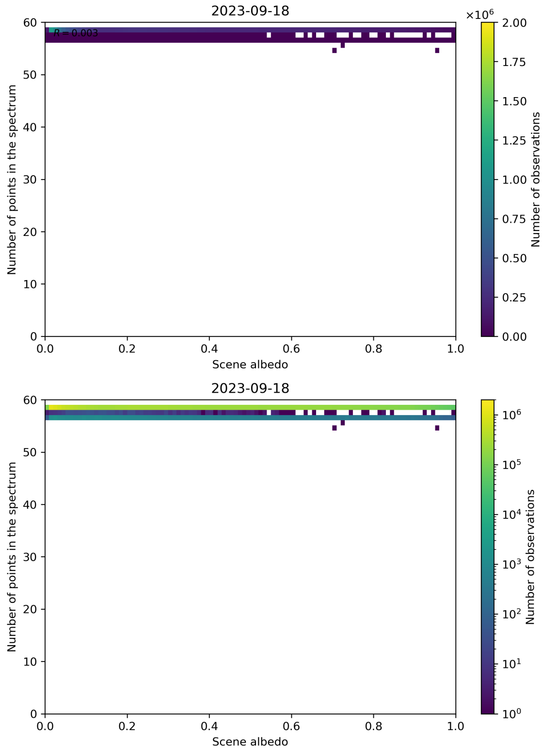
Figure 116: Scatter density plot of “Scene albedo” against “Number of points in the spectrum” for 2023-09-17 to 2023-09-19.
