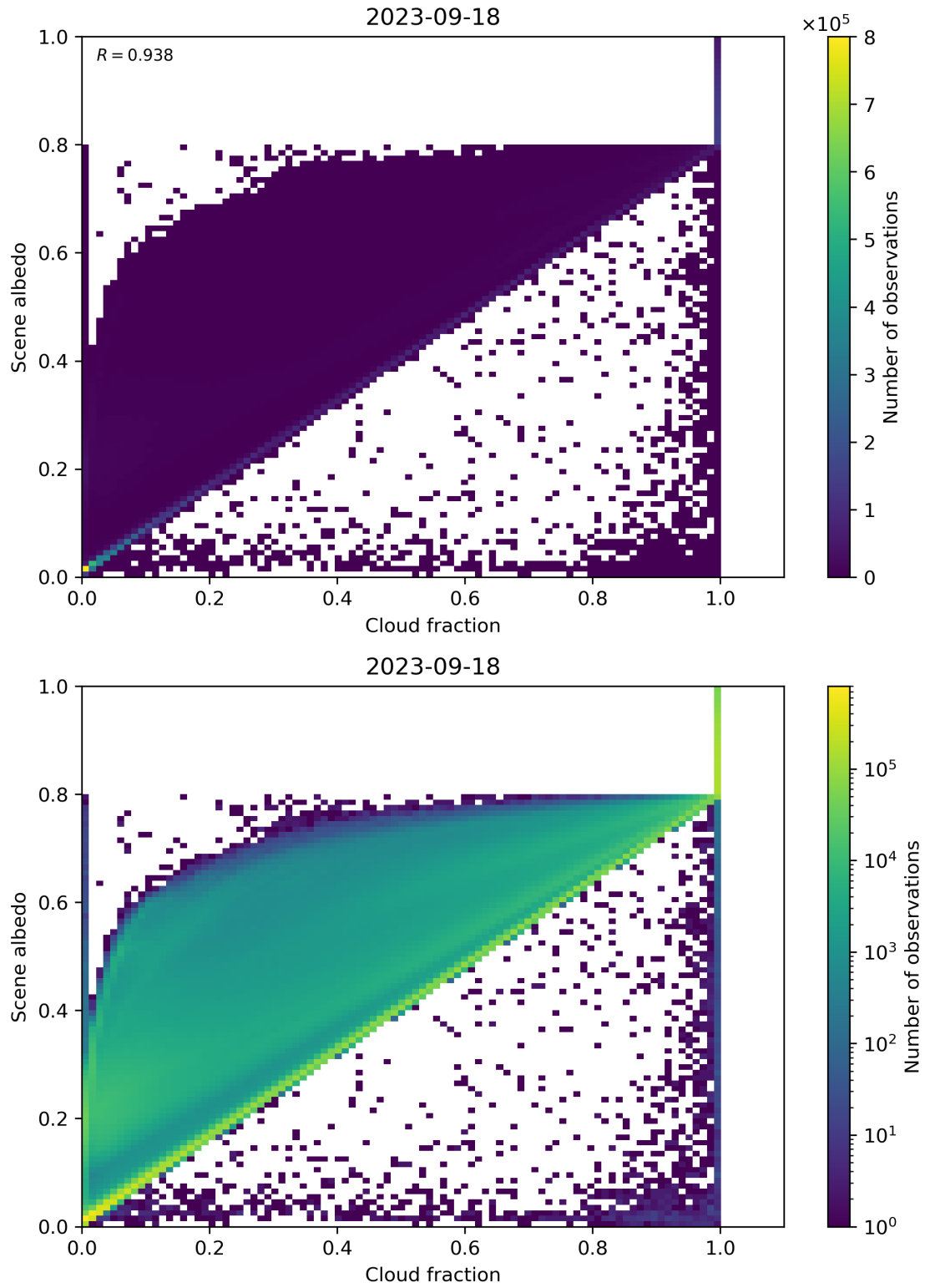
Figure 82: Scatter density plot of “Cloud fraction” against “Scene albedo” for 2023-09-17 to 2023-09-19.
