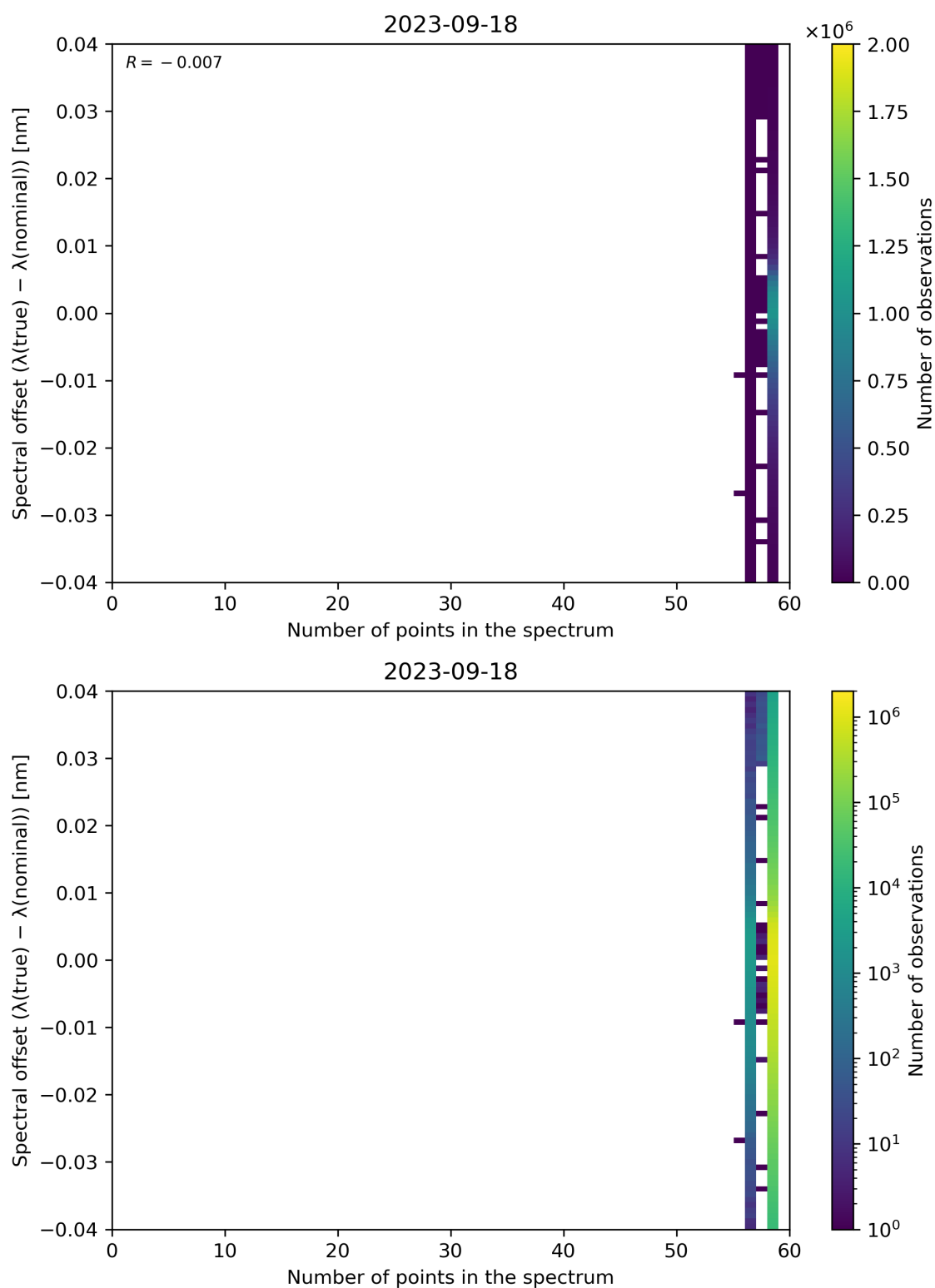
Figure 110: Scatter density plot of “Number of points in the spectrum” against “Spectral offset ( \lambda(\text{true}) - \lambda(\text{nominal}) )” for 2023-09-17 to 2023-09-19.
