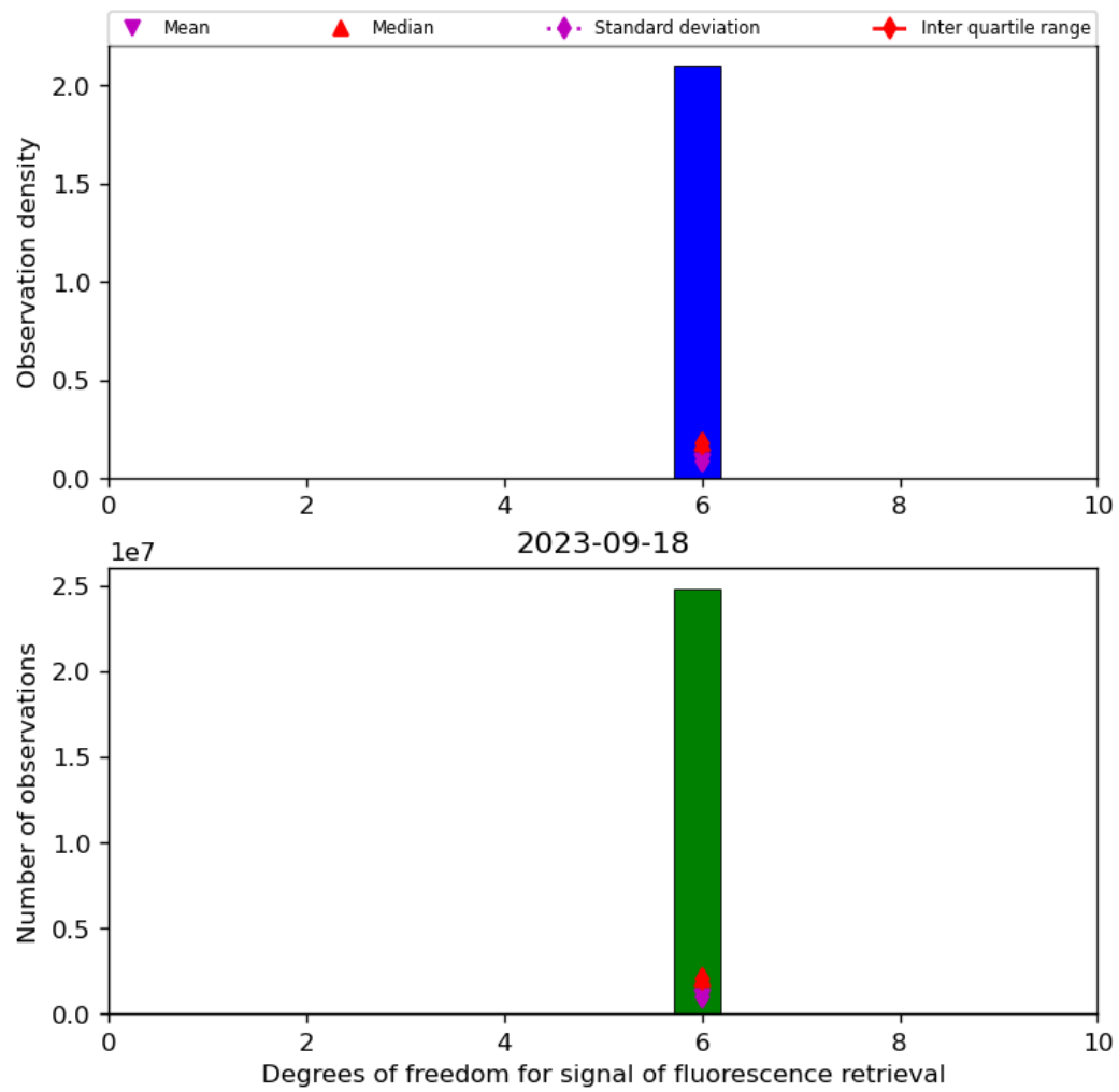
Figure 43: Histogram of “Degrees of freedom for signal of fluorescence retrieval” for 2023-09-17 to 2023-09-19
