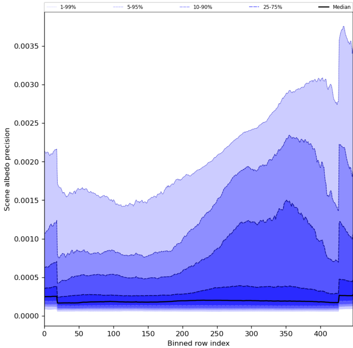
Figure 52: Along track statistics of “Scene albedo precision” for 2023-09-17 to 2023-09-19
