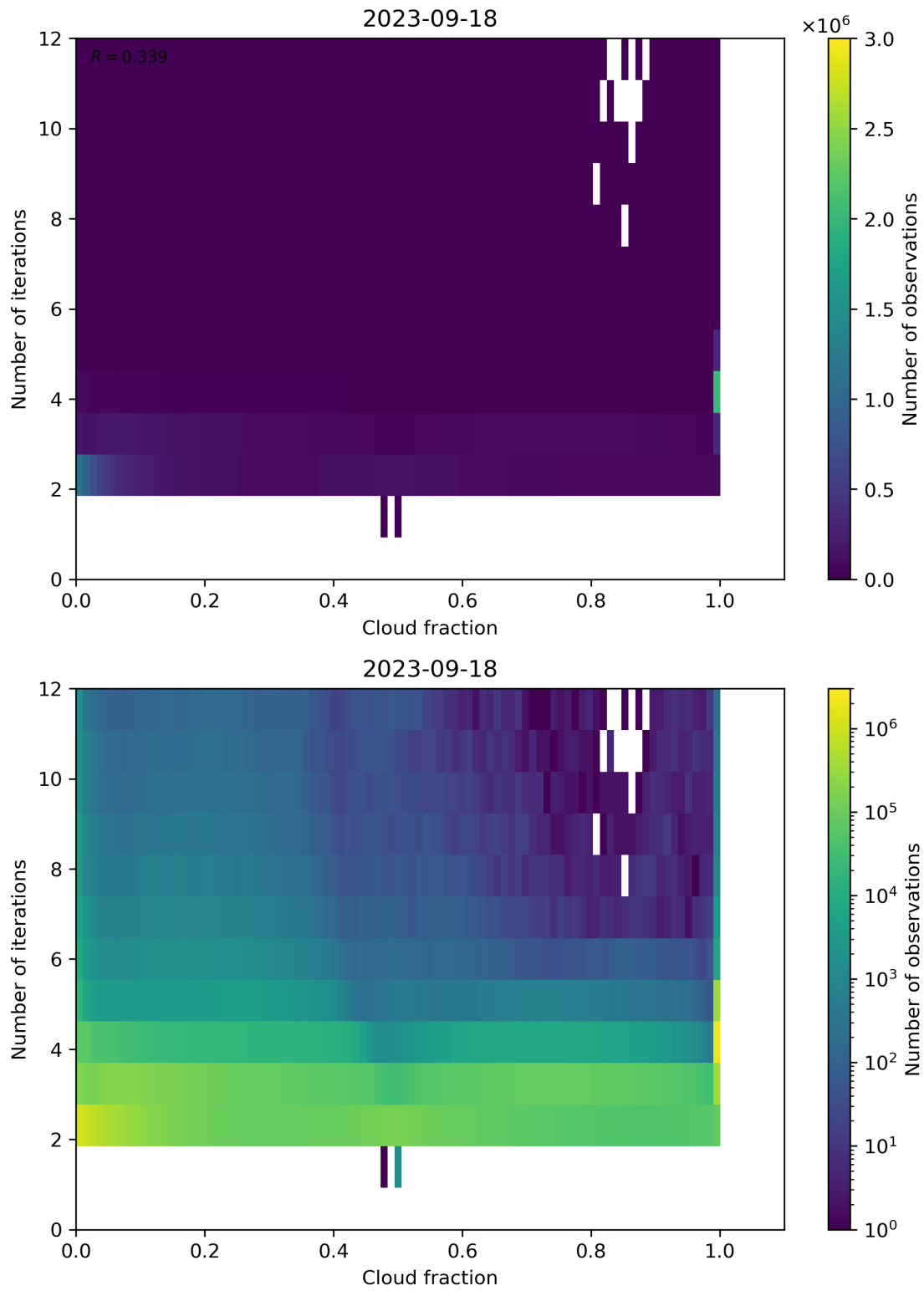
Figure 80: Scatter density plot of “Cloud fraction” against “Number of iterations” for 2023-09-17 to 2023-09-19.
