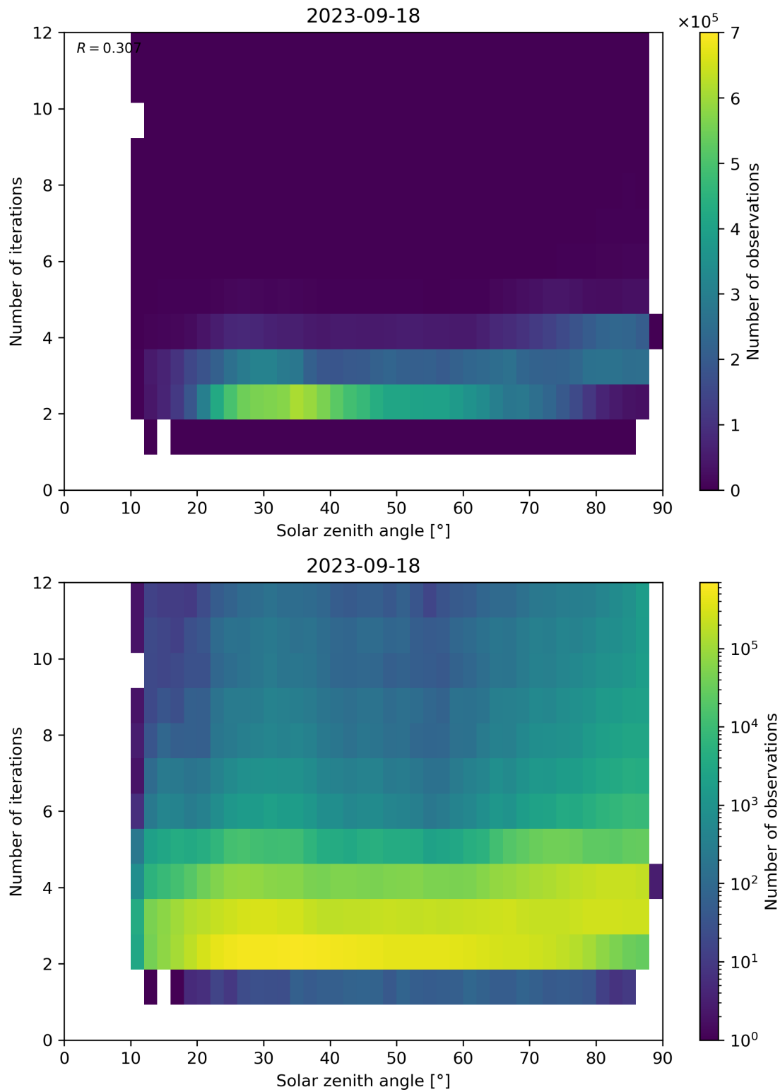
Figure 125: Scatter density plot of “Solar zenith angle” against “Number of iterations” for 2023-09-17 to 2023-09-19.
