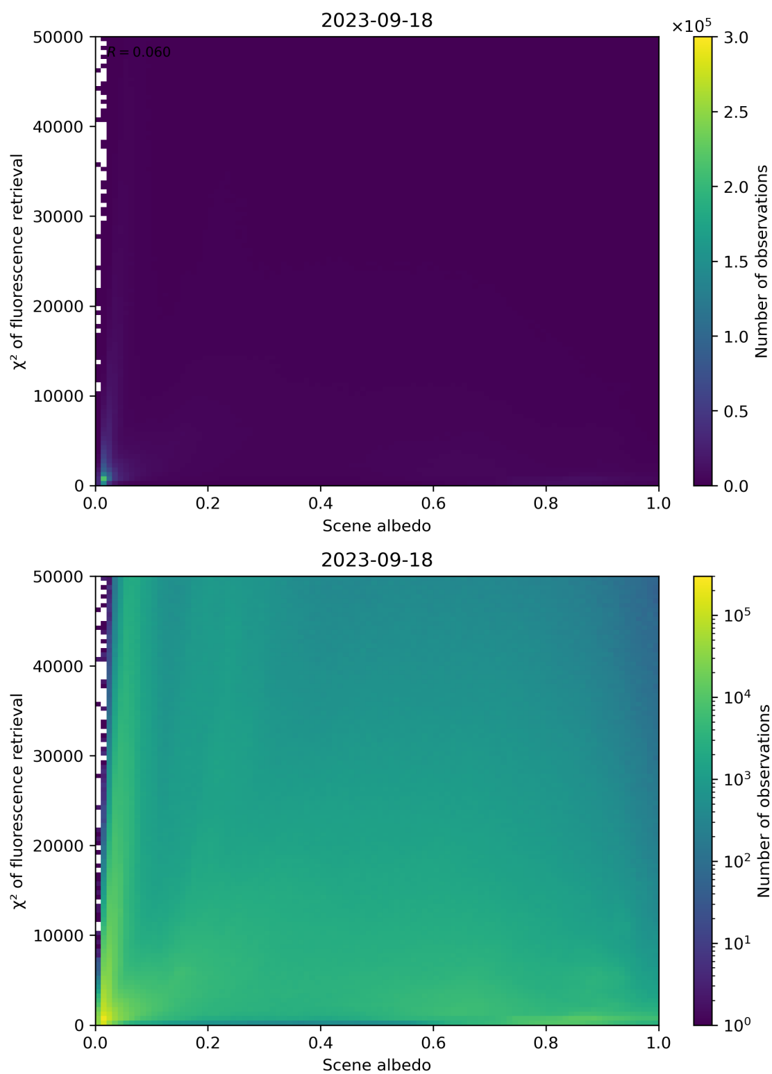
Figure 113: Scatter density plot of “Scene albedo” against “ \chi^2 of fluorescence retrieval” for 2023-09-17 to 2023-09-19.
