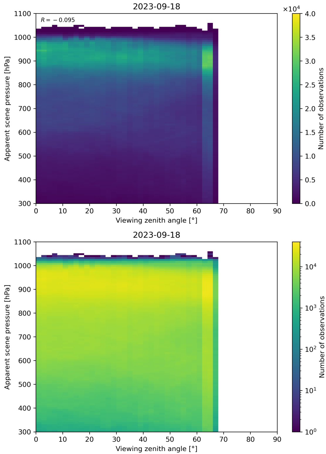
Figure 129: Scatter density plot of “Viewing zenith angle” against “Apparent scene pressure” for 2023-09-17 to 2023-09-19.
