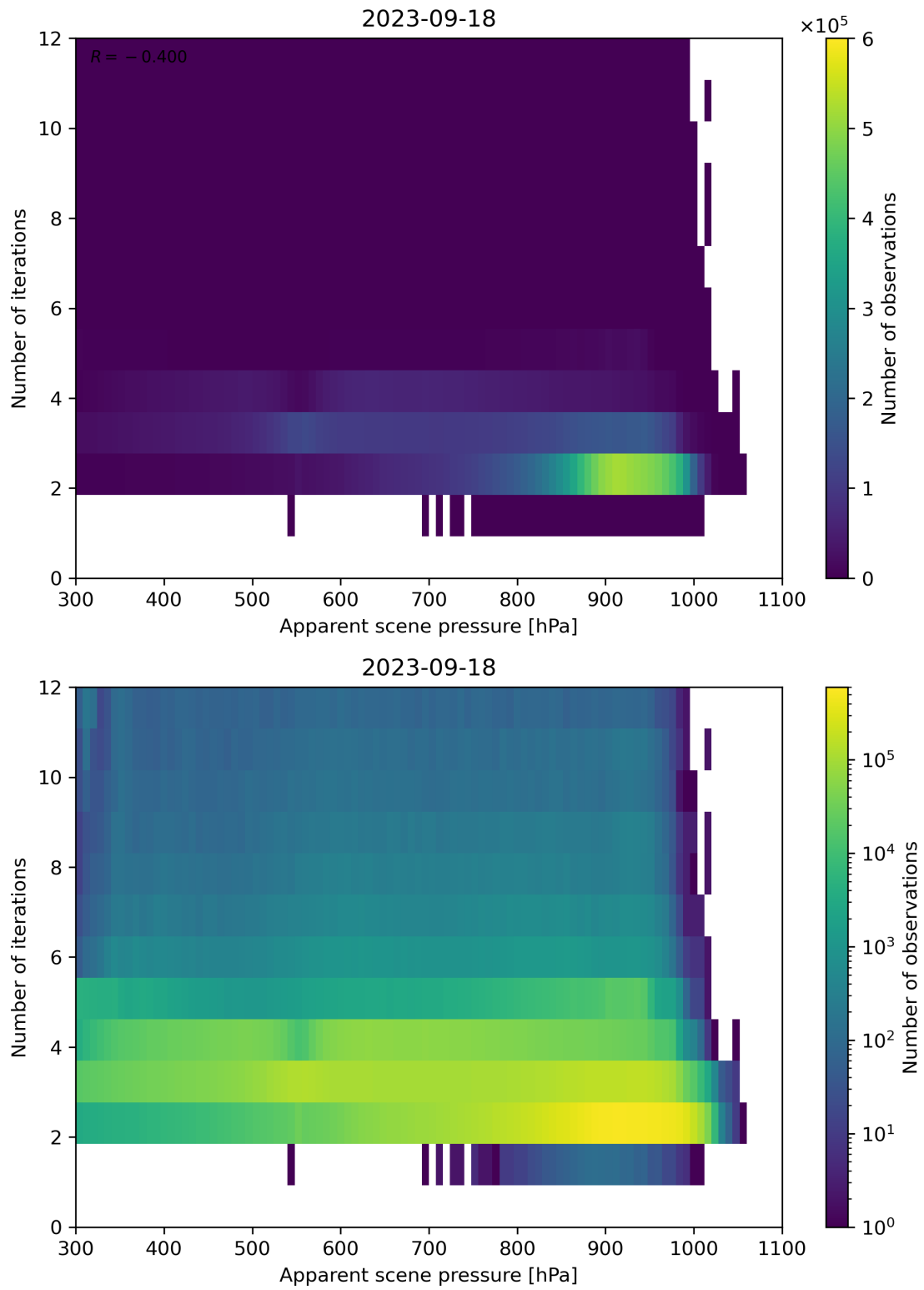
Figure 66: Scatter density plot of “Apparent scene pressure” against “Number of iterations” for 2023-09-17 to 2023-09-19.
