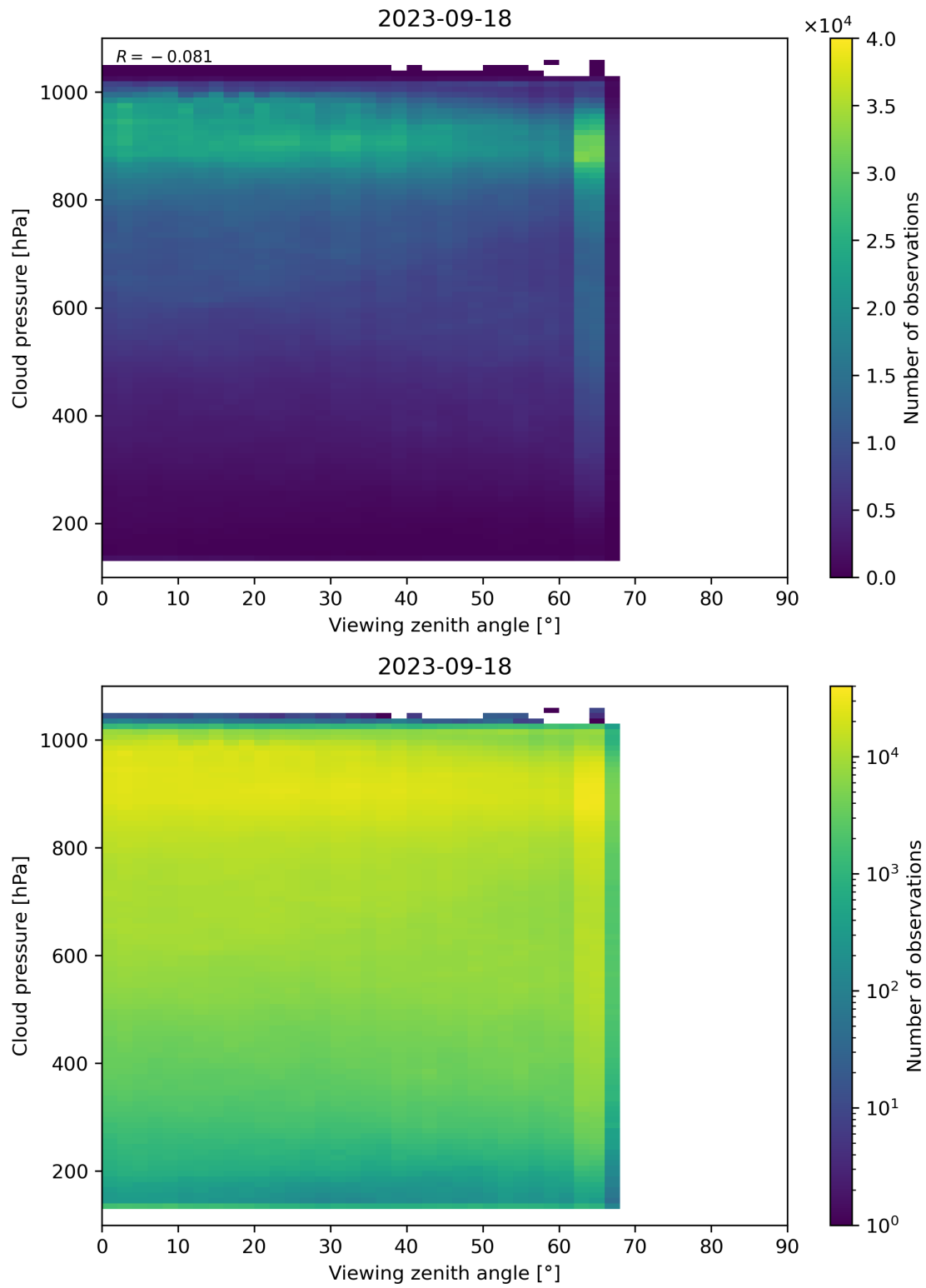
Figure 133: Scatter density plot of “Viewing zenith angle” against “Cloud pressure” for 2023-09-17 to 2023-09-19.
