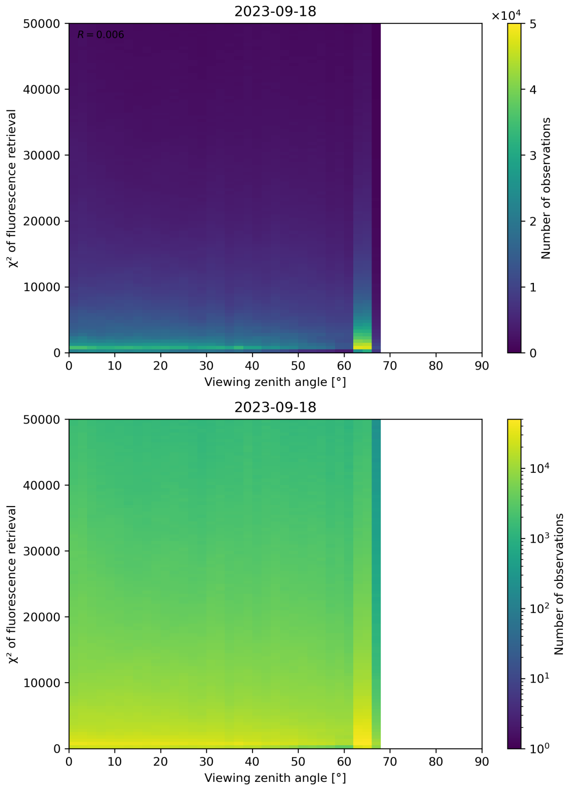
Figure 131: Scatter density plot of “Viewing zenith angle” against “ \chi^2 of fluorescence retrieval” for 2023-09-17 to 2023-09-19.
