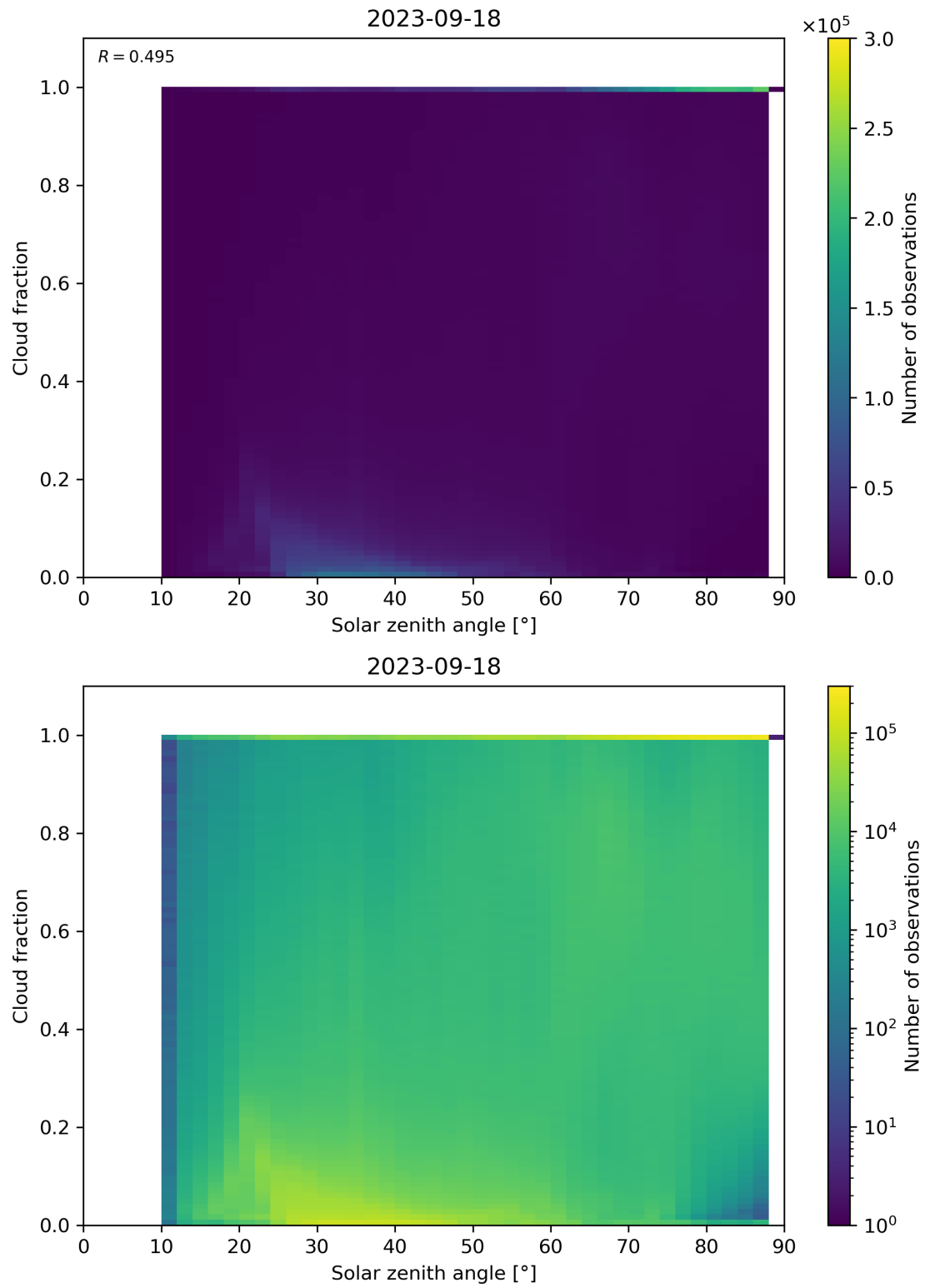
Figure 121: Scatter density plot of “Solar zenith angle” against “Cloud fraction” for 2023-09-17 to 2023-09-19.
