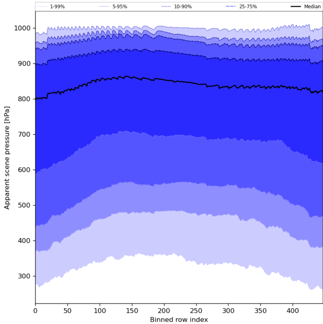
Figure 53: Along track statistics of “Apparent scene pressure” for 2023-09-17 to 2023-09-19
