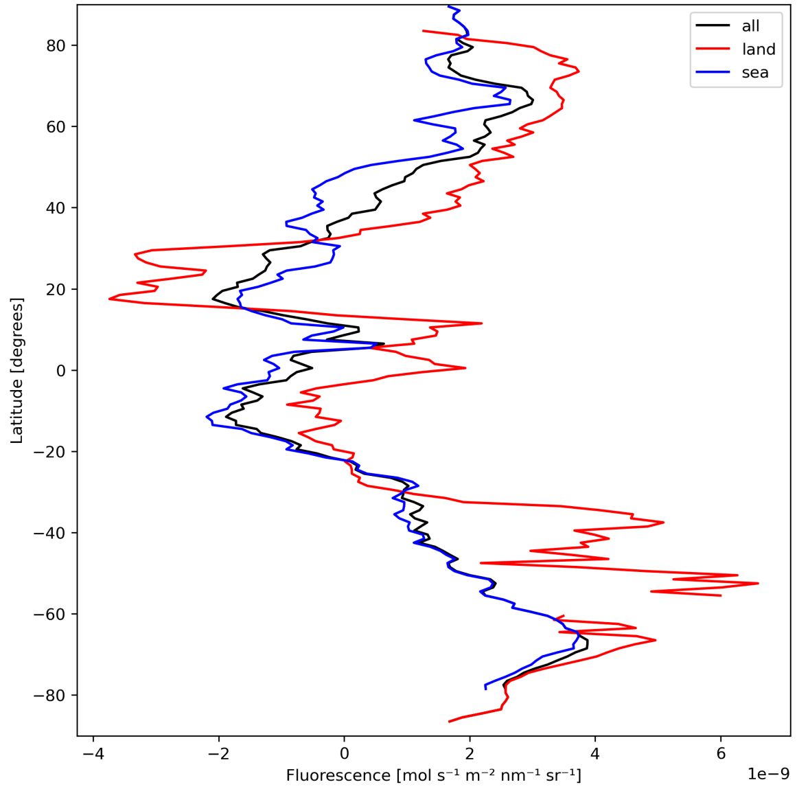
Figure 23: Zonal average of “Fluorescence” for 2023-09-17 to 2023-09-19.
