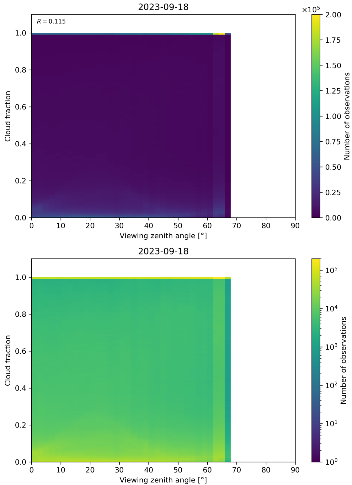
Figure 132: Scatter density plot of “Viewing zenith angle” against “Cloud fraction” for 2023-09-17 to 2023-09-19.
