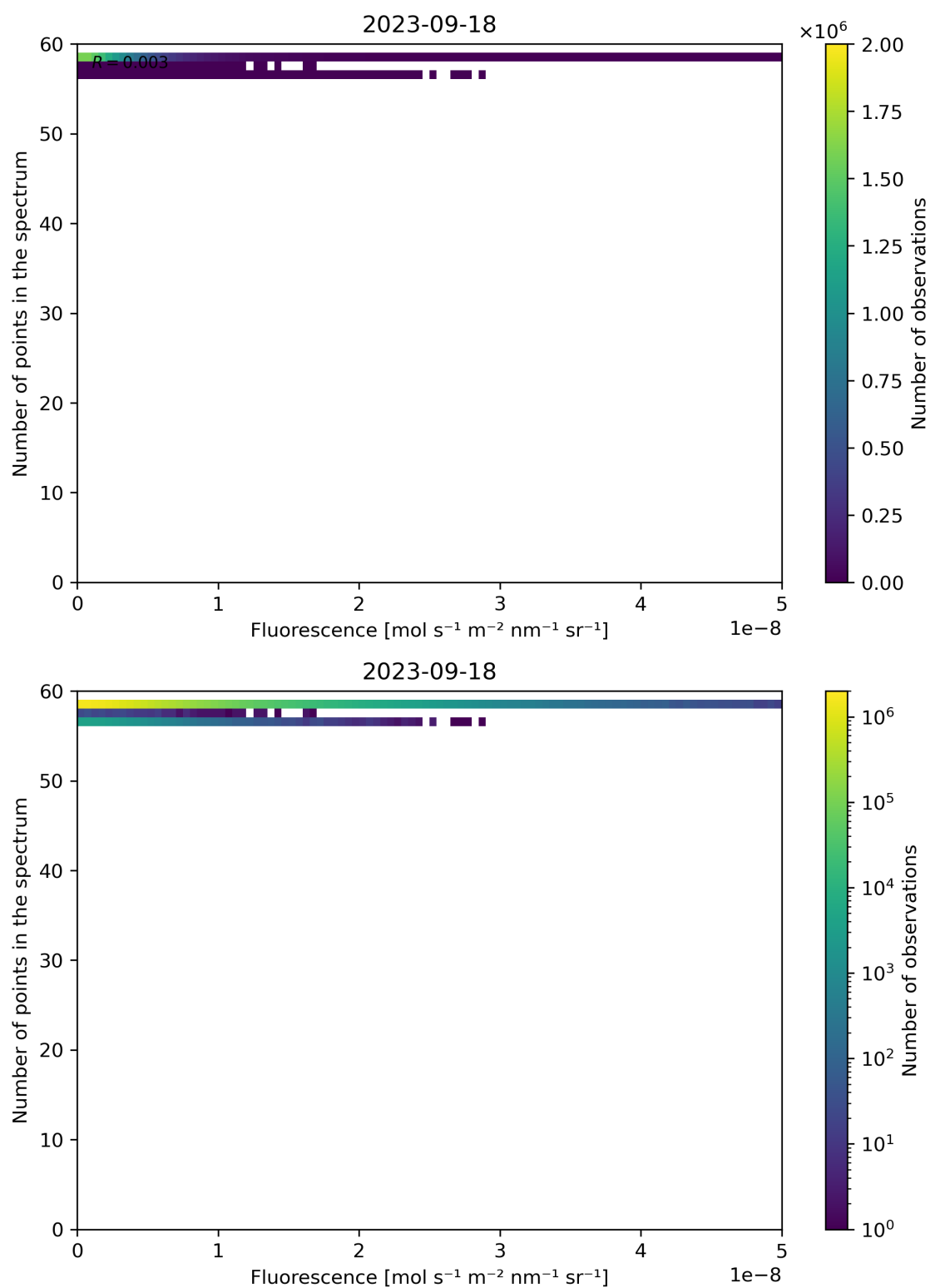
Figure 94: Scatter density plot of “Fluorescence” against “Number of points in the spectrum” for 2023-09-17 to 2023-09-19.
