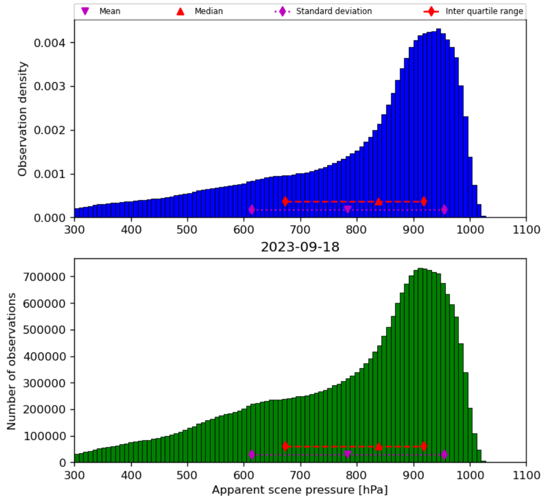
Figure 36: Histogram of “Apparent scene pressure” for 2023-09-17 to 2023-09-19
