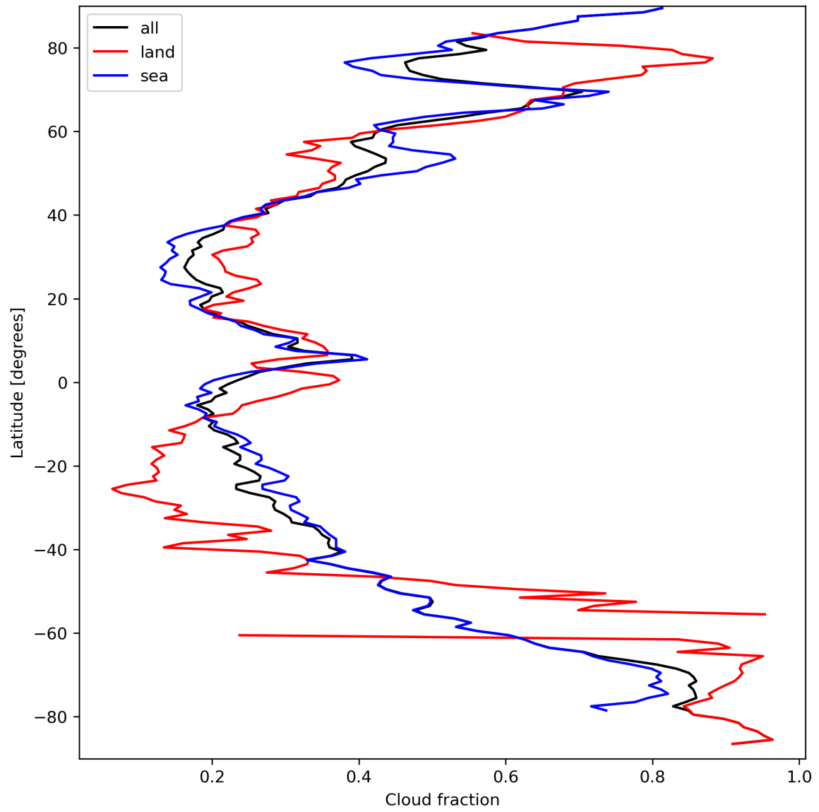
Figure 15: Zonal average of “Cloud fraction” for 2023-09-17 to 2023-09-19.
