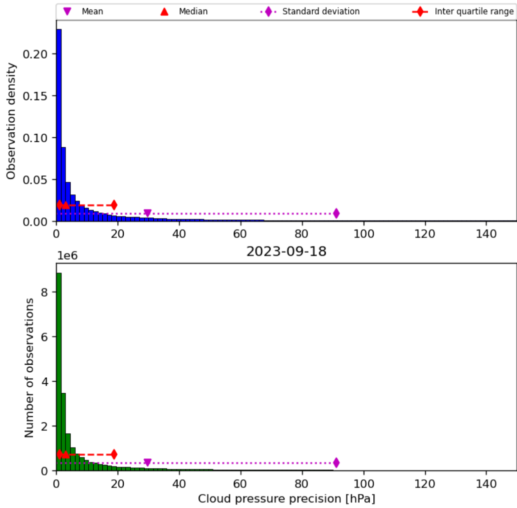
Figure 31: Histogram of “Cloud pressure precision” for 2023-09-17 to 2023-09-19
