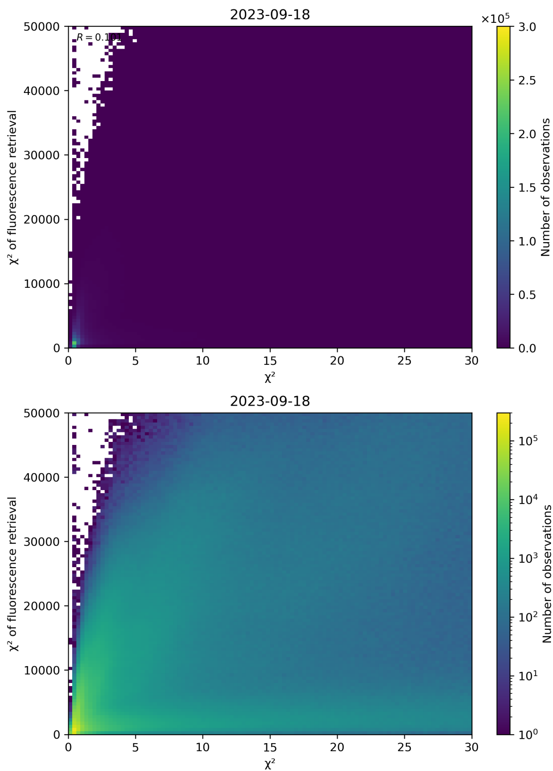
Figure 69: Scatter density plot of “ \chi^2 ” against “ \chi^2 of fluorescence retrieval” for 2023-09-17 to 2023-09-19.
