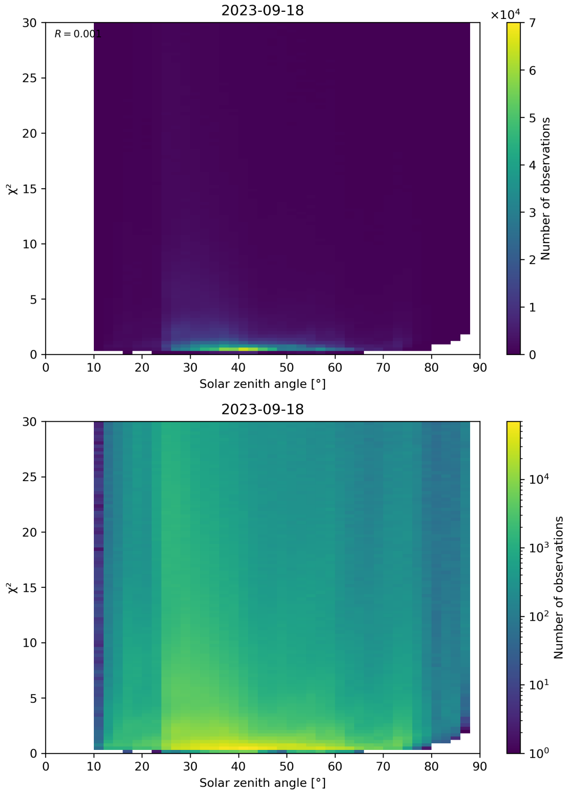
Figure 119: Scatter density plot of “Solar zenith angle” against “ \chi^2 ” for 2023-09-17 to 2023-09-19.
