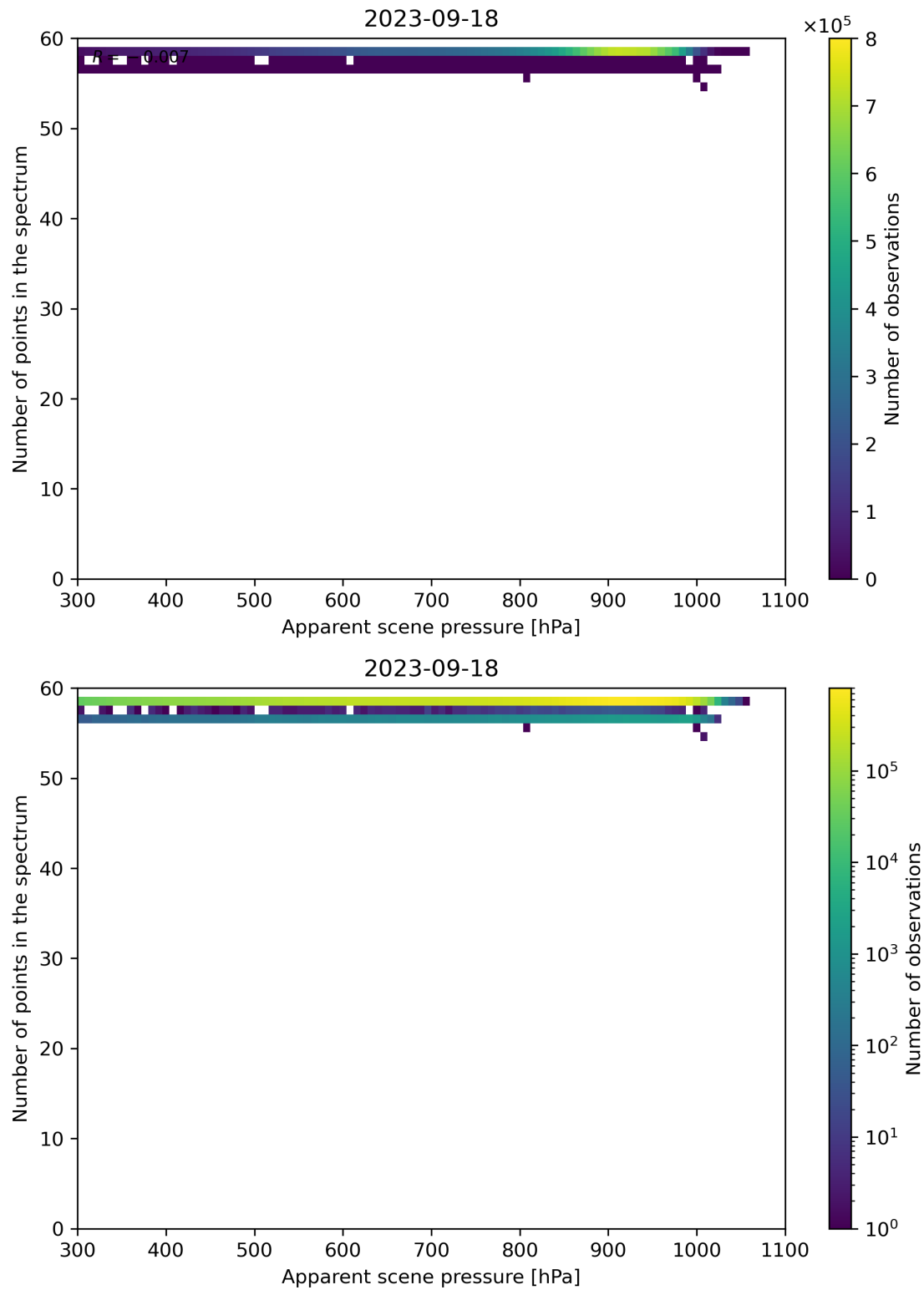
Figure 67: Scatter density plot of “Apparent scene pressure” against “Number of points in the spectrum” for 2023-09-17 to 2023-09-19.
