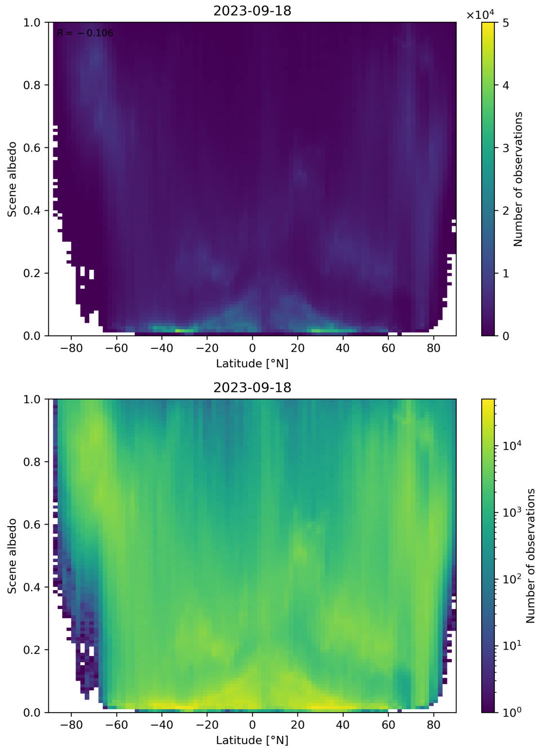
Figure 104: Scatter density plot of “Latitude” against “Scene albedo” for 2023-09-17 to 2023-09-19.
