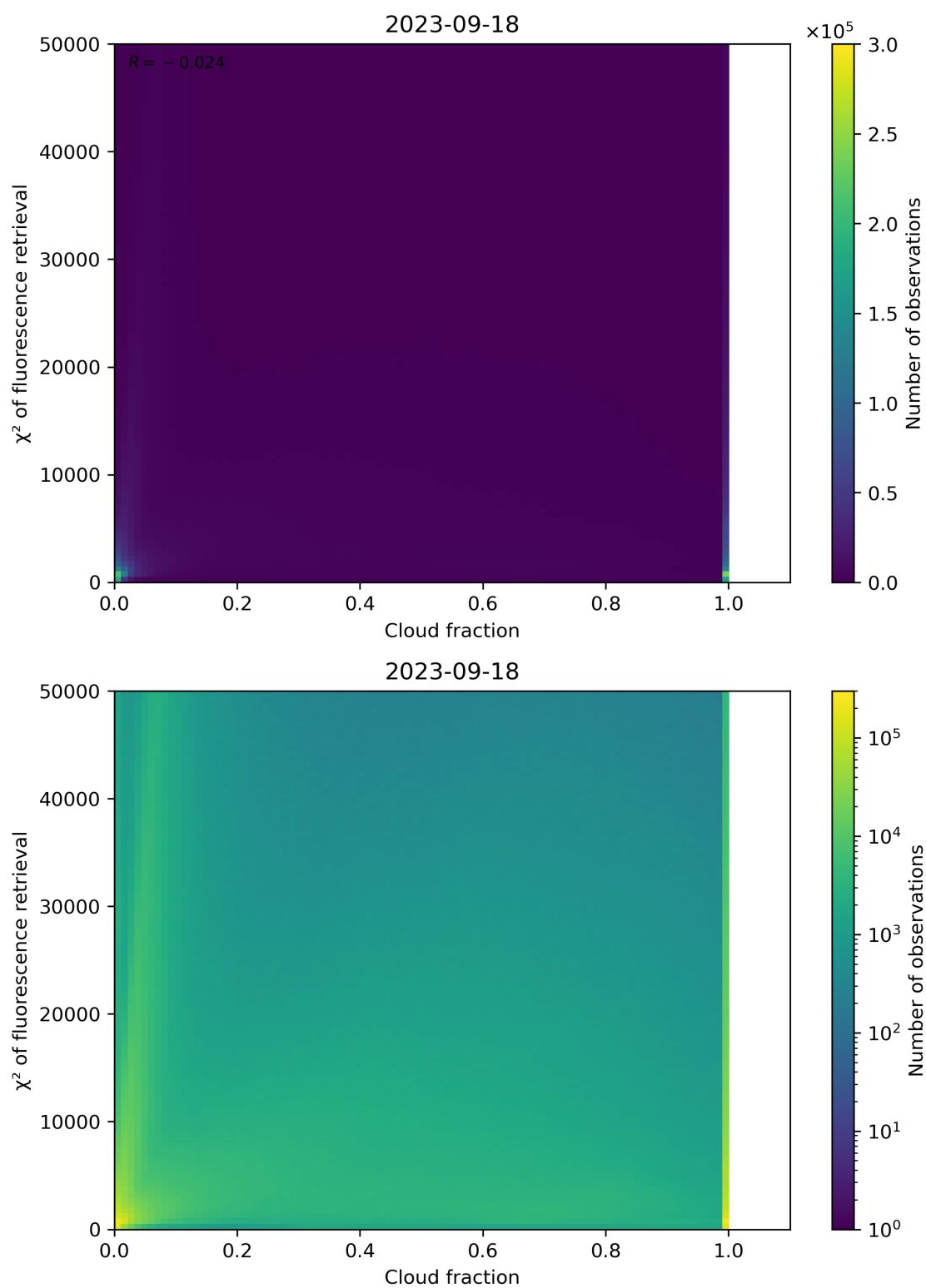
Figure 78: Scatter density plot of “Cloud fraction” against “ \chi^2 of fluorescence retrieval” for 2023-09-17 to 2023-09-19.
