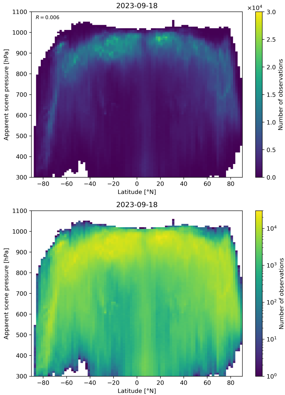
Figure 96: Scatter density plot of “Latitude” against “Apparent scene pressure” for 2023-09-17 to 2023-09-19.
