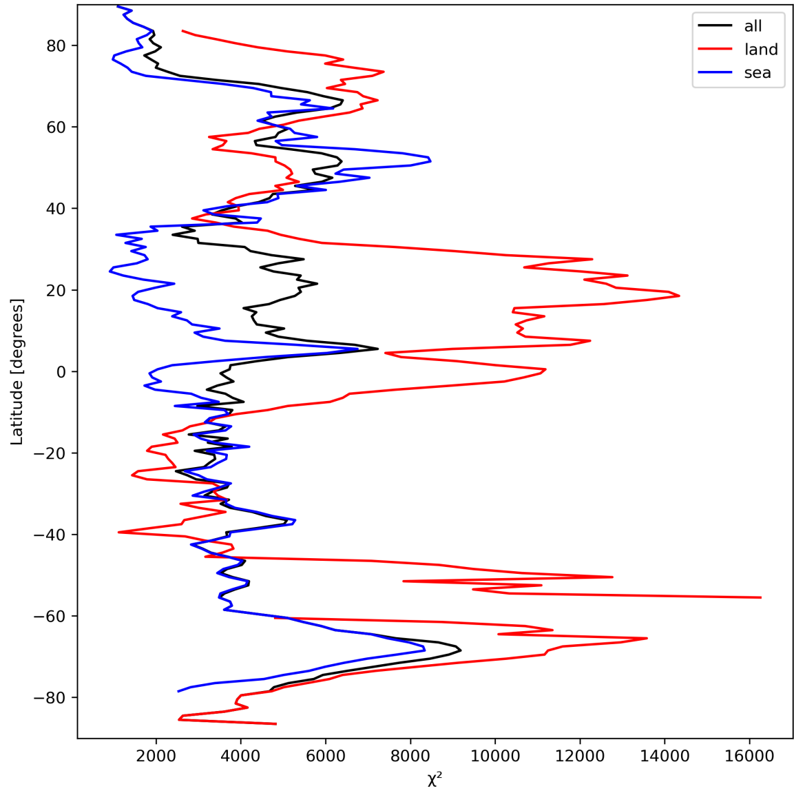
Figure 21: Zonal average of “ \chi^2 ” for 2023-09-17 to 2023-09-19.
