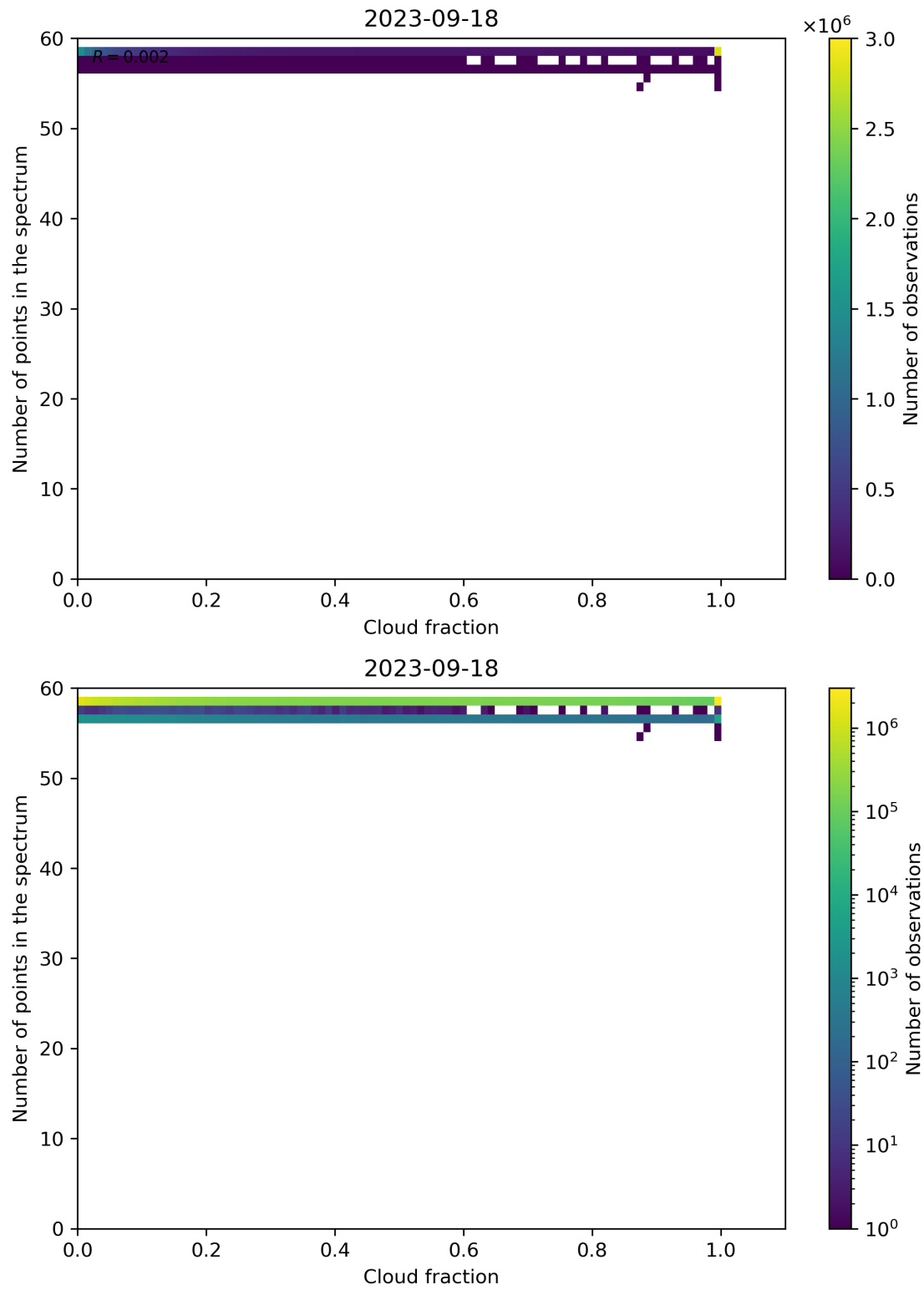
Figure 81: Scatter density plot of “Cloud fraction” against “Number of points in the spectrum” for 2023-09-17 to 2023-09-19.
