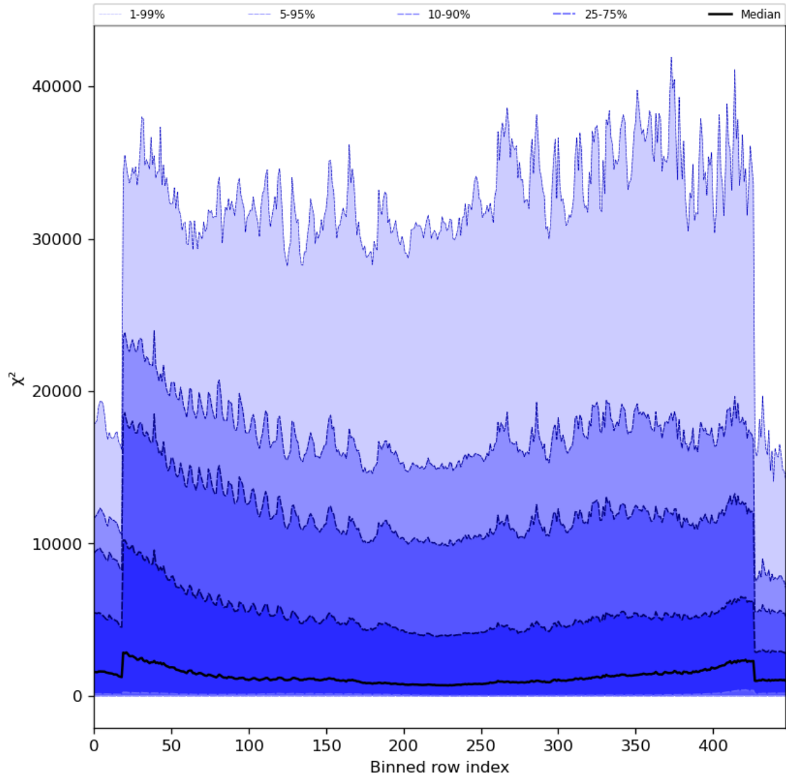
Figure 55: Along track statistics of " \chi^2 " for 2023-09-17 to 2023-09-19
