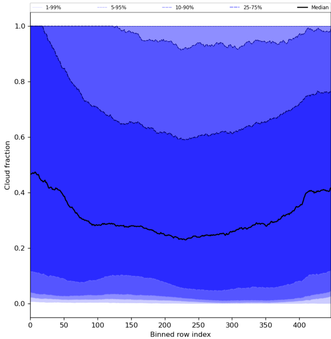
Figure 49: Along track statistics of “Cloud fraction” for 2023-09-17 to 2023-09-19
