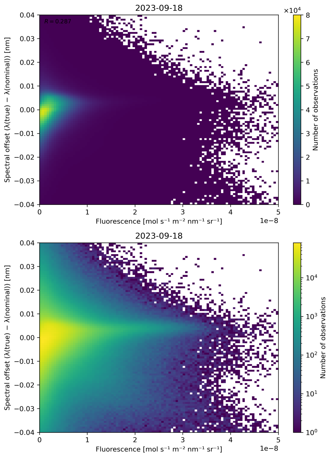
Figure 95: Scatter density plot of “Fluorescence” against “Spectral offset ( \lambda(\text{true}) - \lambda(\text{nominal}) )” for 2023-09-17 to 2023-09-19.
