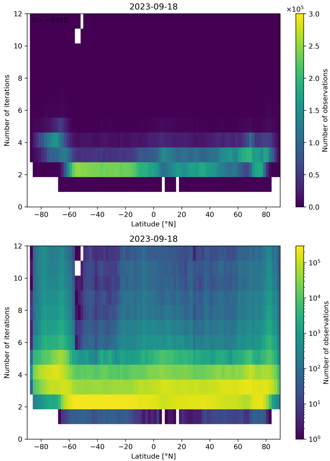
Figure 102: Scatter density plot of “Latitude” against “Number of iterations” for 2023-09-17 to 2023-09-19.
