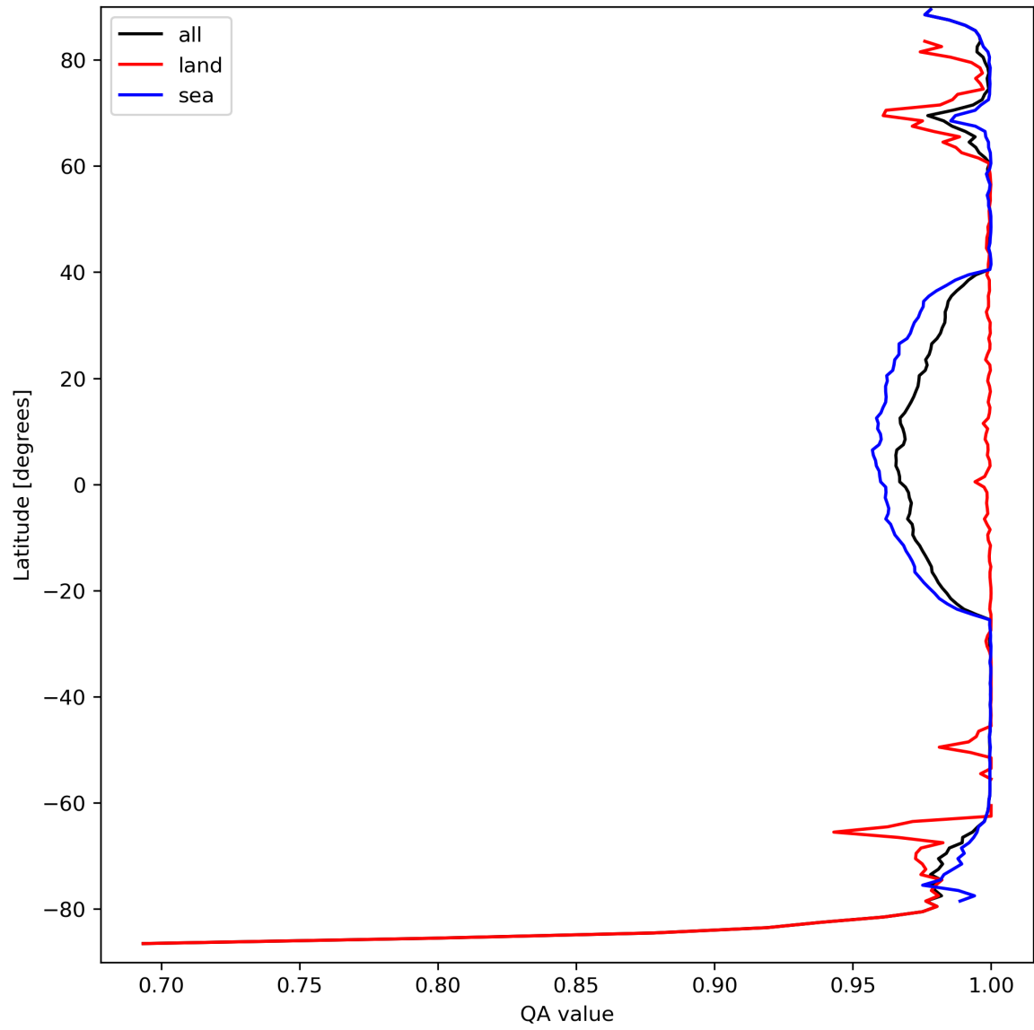
Figure 12: Zonal average of “QA value” for 2023-09-17 to 2023-09-19.
