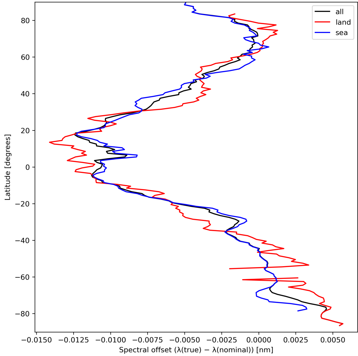
Figure 28: Zonal average of “Spectral offset ( \lambda(\text{true}) - \lambda(\text{nominal}) )” for 2023-09-17 to 2023-09-19.
