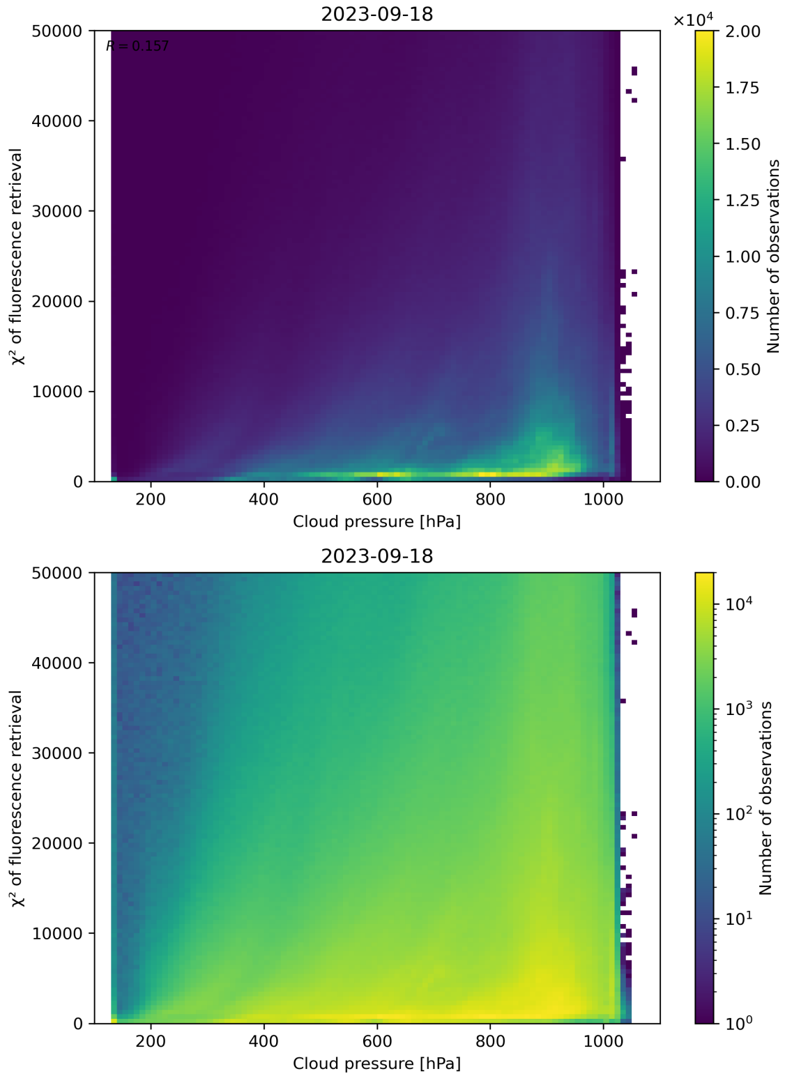
Figure 86: Scatter density plot of “Cloud pressure” against “ \chi^2 of fluorescence retrieval” for 2023-09-17 to 2023-09-19.
