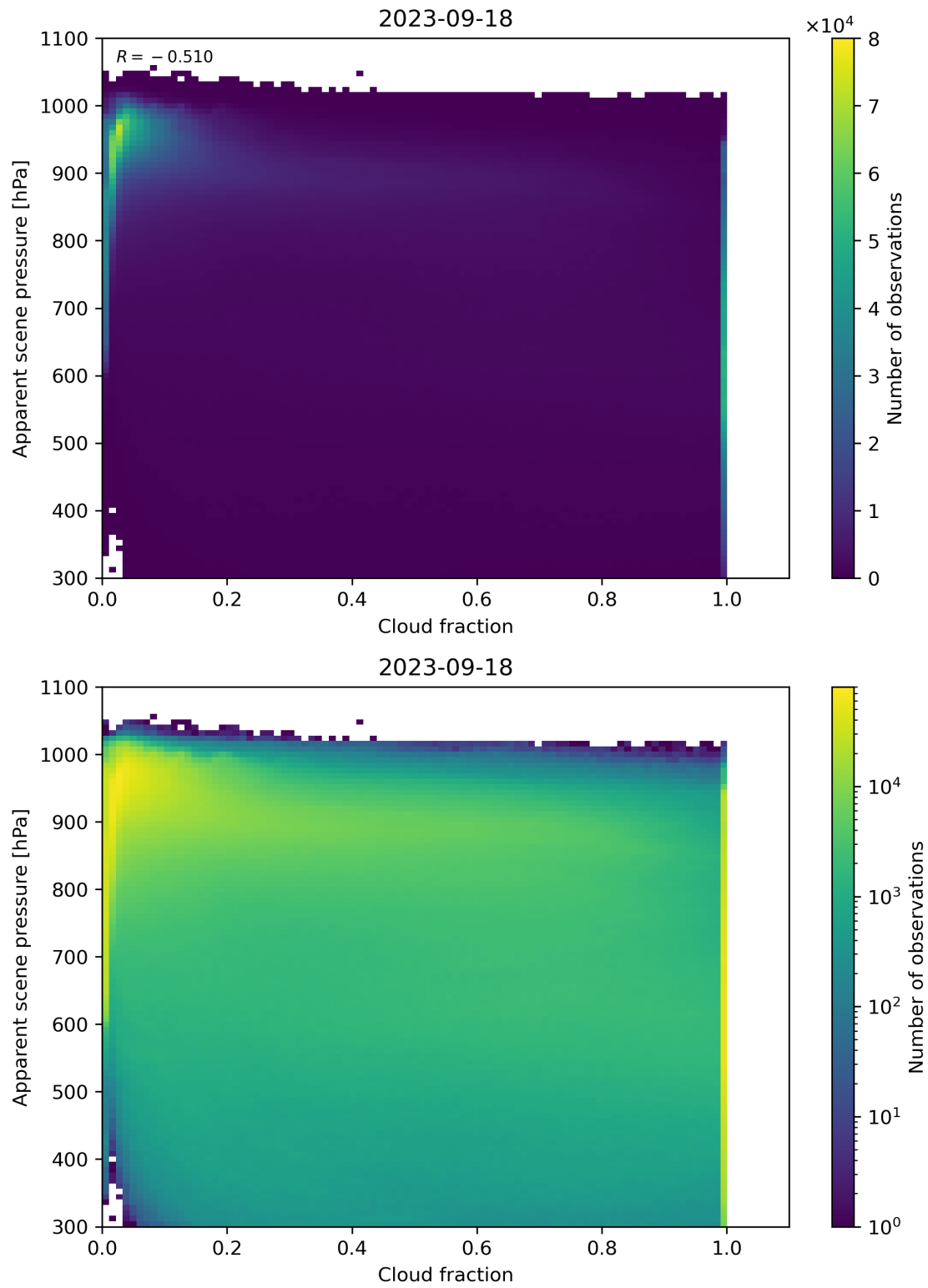
Figure 76: Scatter density plot of “Cloud fraction” against “Apparent scene pressure” for 2023-09-17 to 2023-09-19.
