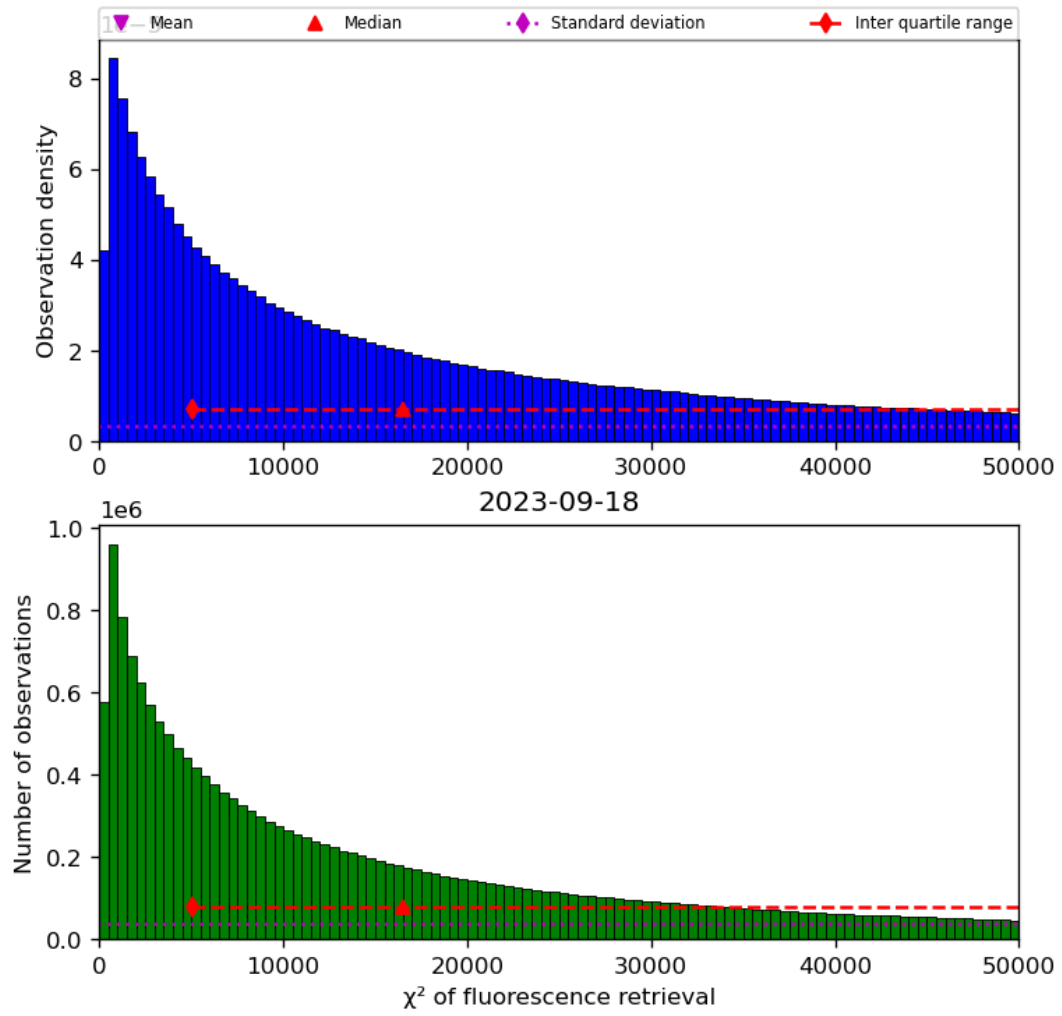
Figure 42: Histogram of “ \chi^2 of fluorescence retrieval” for 2023-09-17 to 2023-09-19
