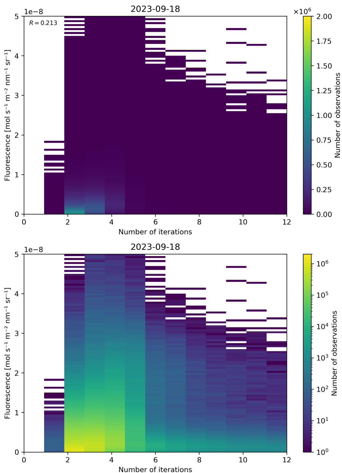
Figure 107: Scatter density plot of “Number of iterations” against “Fluorescence” for 2023-09-17 to 2023-09-19.
