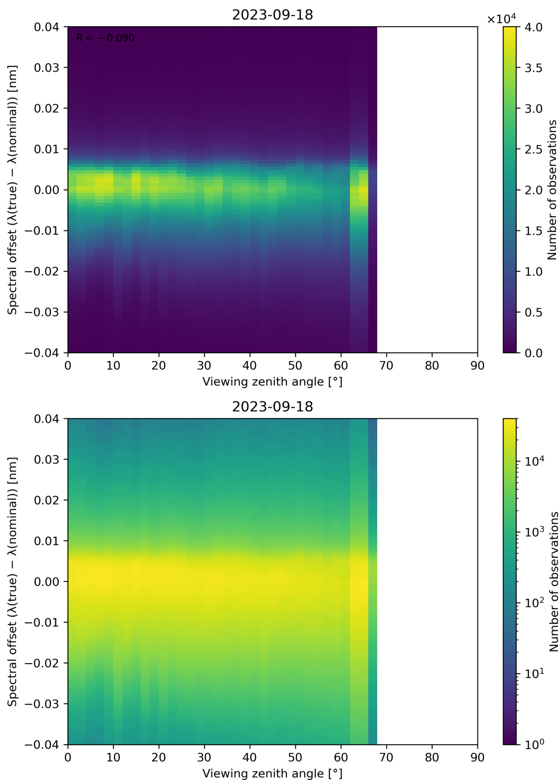
Figure 140: Scatter density plot of “Viewing zenith angle” against “Spectral offset ( \lambda(\text{true}) - \lambda(\text{nominal}) )” for 2023-09-17 to 2023-09-19.
