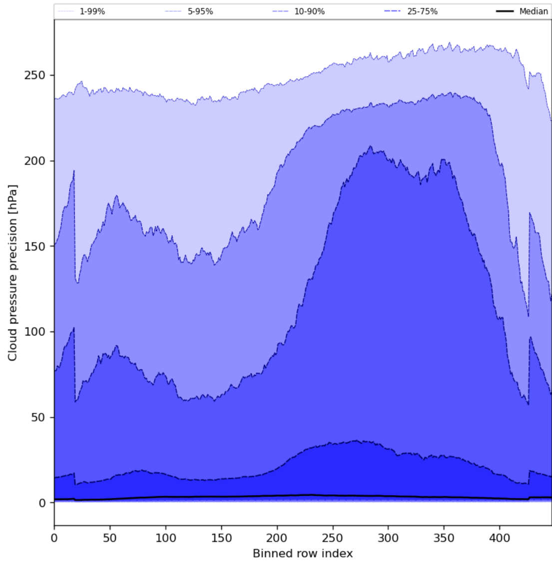
Figure 48: Along track statistics of “Cloud pressure precision” for 2023-09-17 to 2023-09-19
