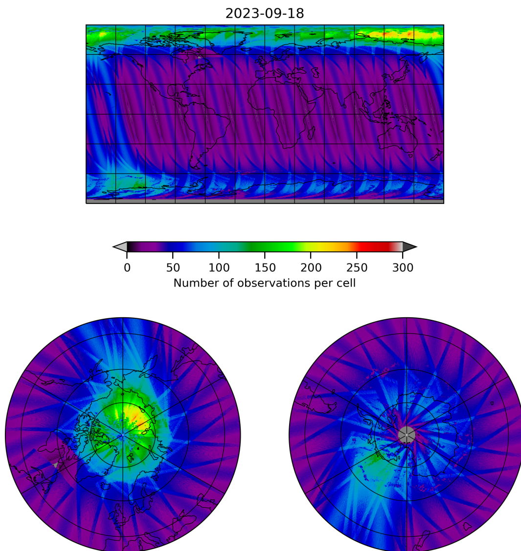
Figure 11: Map of the number of observations for 2023-09-17 to 2023-09-19
