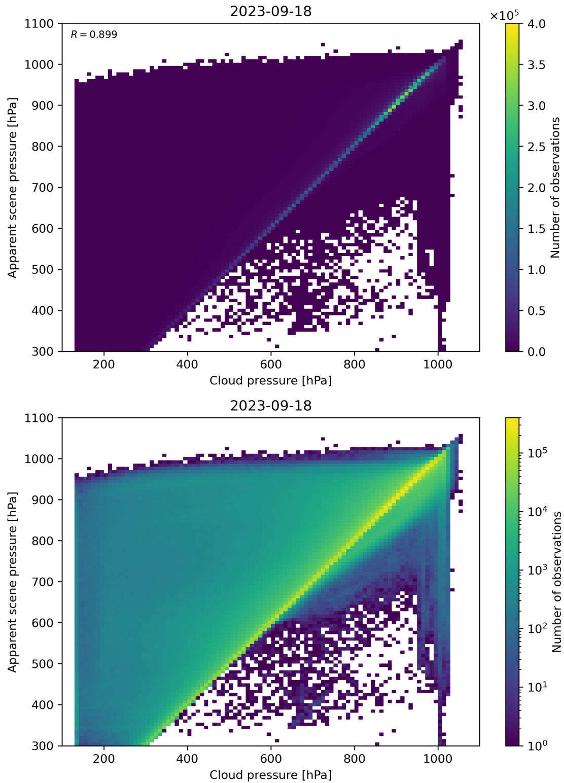
Figure 84: Scatter density plot of “Cloud pressure” against “Apparent scene pressure” for 2023-09-17 to 2023-09-19.
