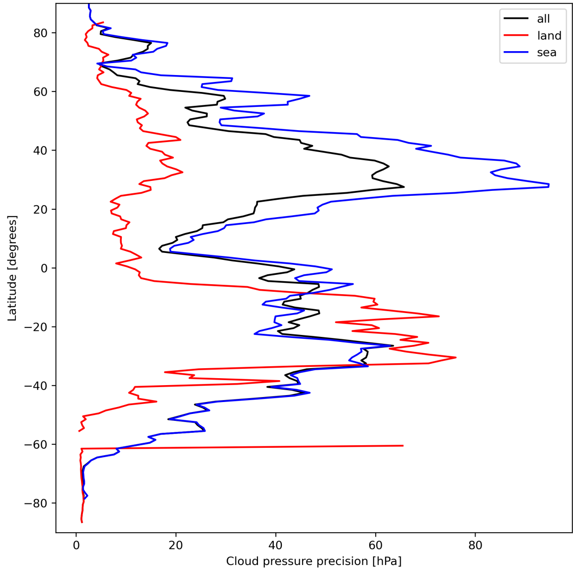
Figure 14: Zonal average of “Cloud pressure precision” for 2023-09-17 to 2023-09-19.
