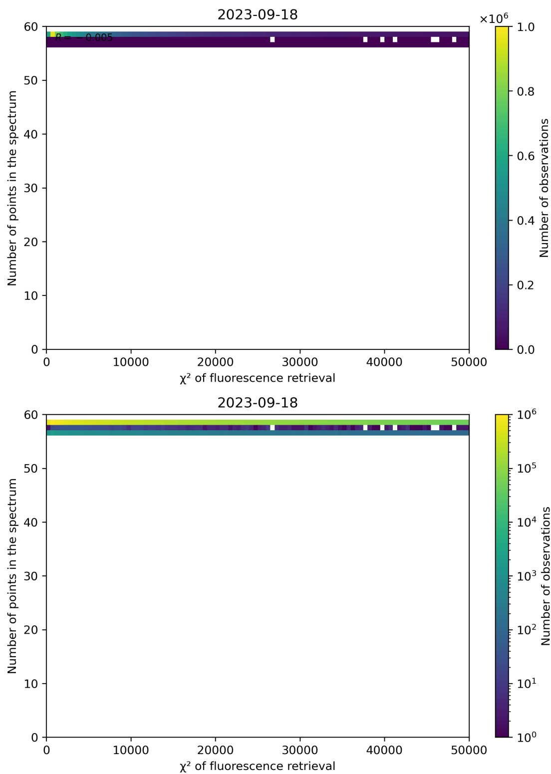
Figure 71: Scatter density plot of “ \chi^2 of fluorescence retrieval” against “Number of points in the spectrum” for 2023-09-17 to 2023-09-19.
