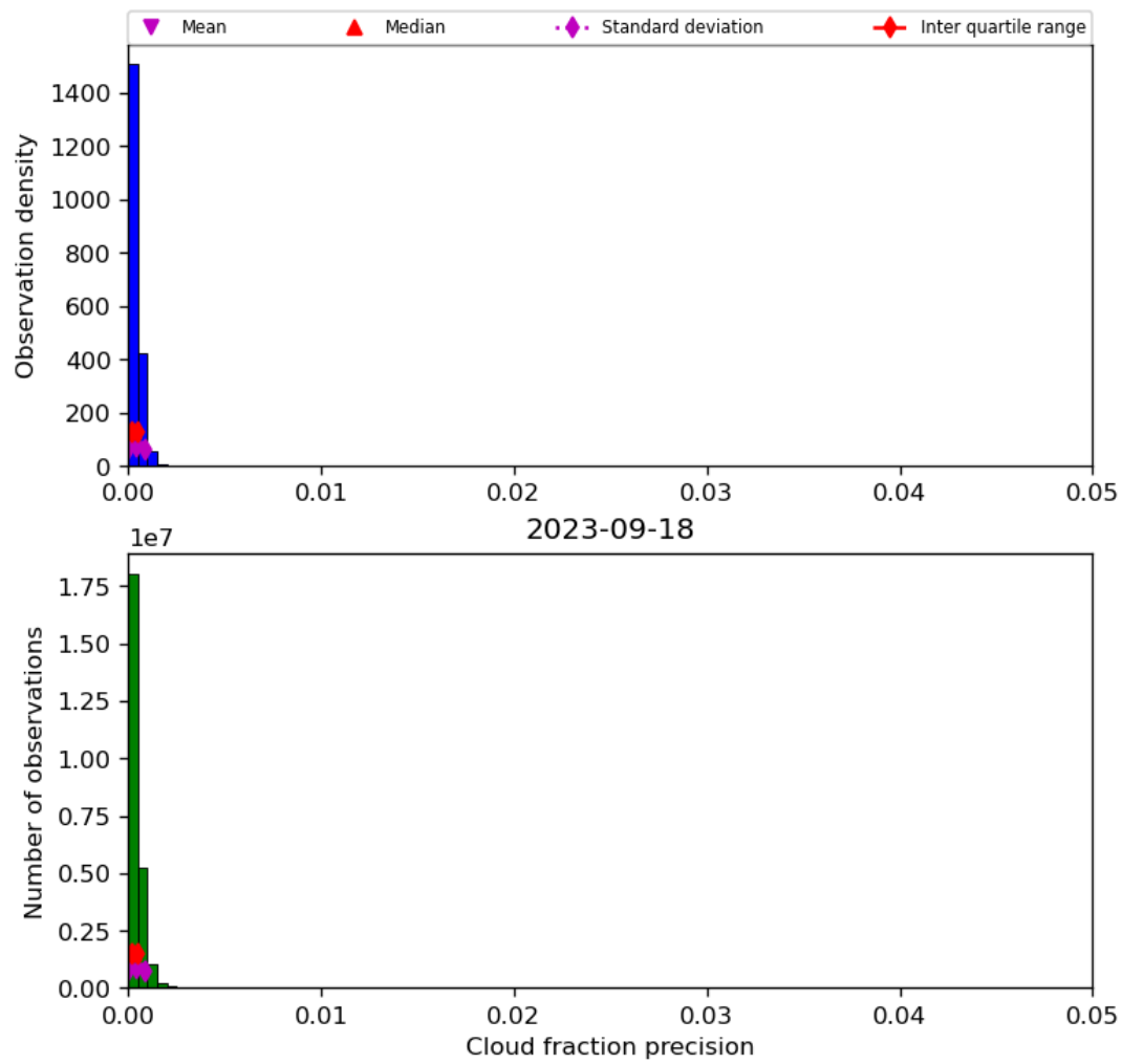
Figure 33: Histogram of “Cloud fraction precision” for 2023-09-17 to 2023-09-19
