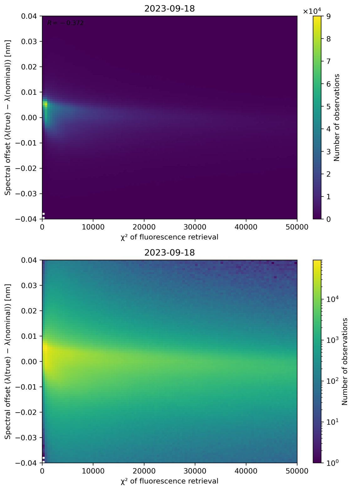
Figure 72: Scatter density plot of " \chi^2 of fluorescence retrieval" against "Spectral offset ( \lambda(\text{true}) - \lambda(\text{nominal}) )" for 2023-09-17 to 2023-09-19.
