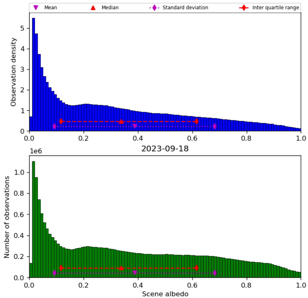
Figure 34: Histogram of “Scene albedo” for 2023-09-17 to 2023-09-19
