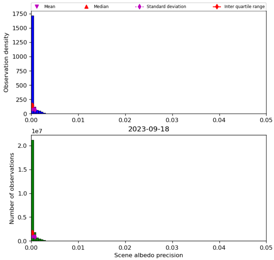
Figure 35: Histogram of “Scene albedo precision” for 2023-09-17 to 2023-09-19
