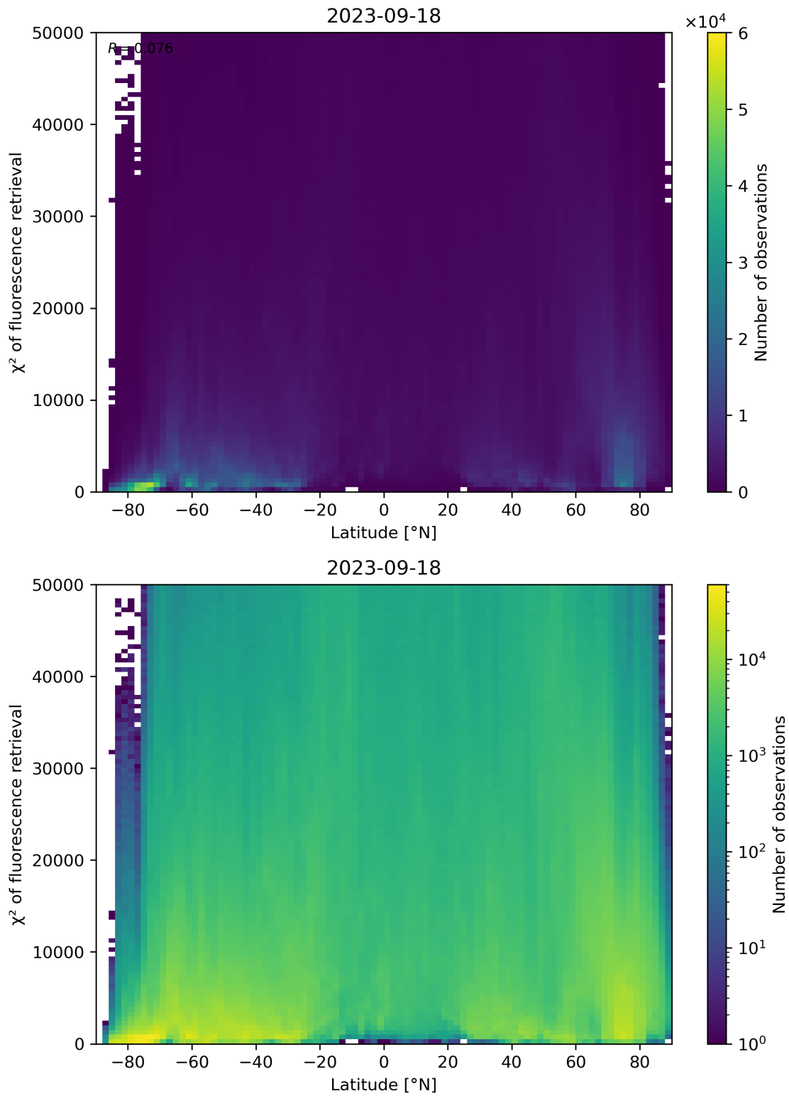
Figure 98: Scatter density plot of “Latitude” against “ \chi^2 of fluorescence retrieval” for 2023-09-17 to 2023-09-19.
