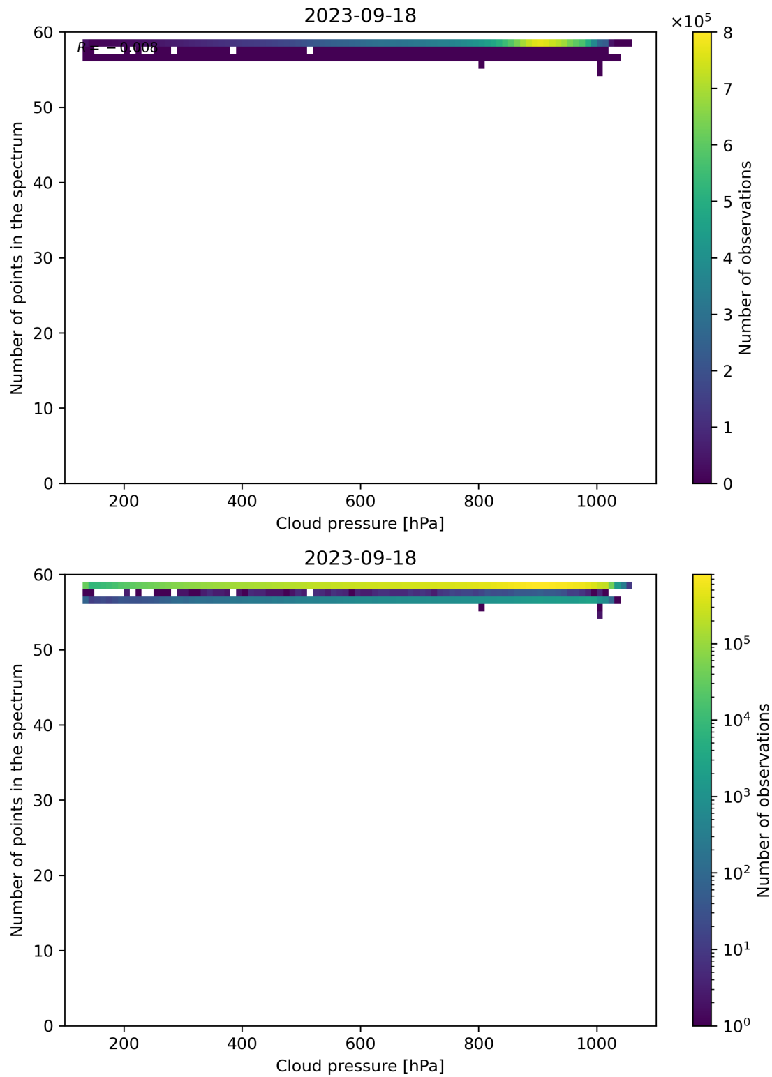
Figure 90: Scatter density plot of “Cloud pressure” against “Number of points in the spectrum” for 2023-09-17 to 2023-09-19.
