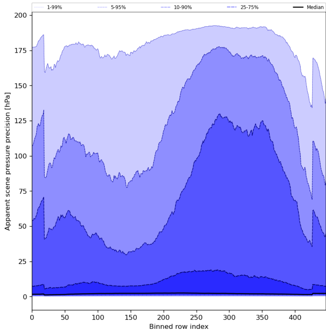
Figure 54: Along track statistics of “Apparent scene pressure precision” for 2023-09-17 to 2023-09-19
