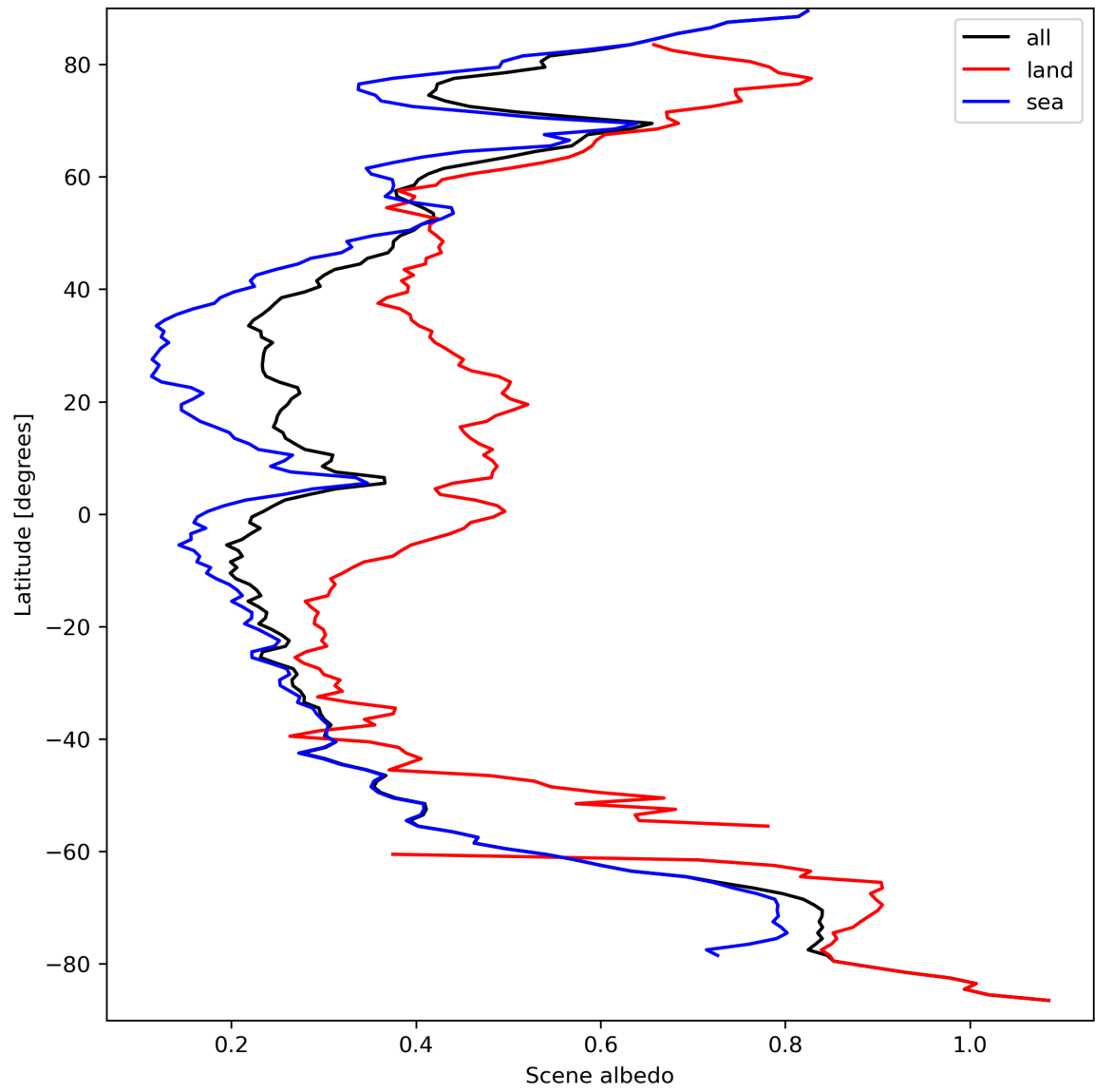
Figure 17: Zonal average of “Scene albedo” for 2023-09-17 to 2023-09-19.
