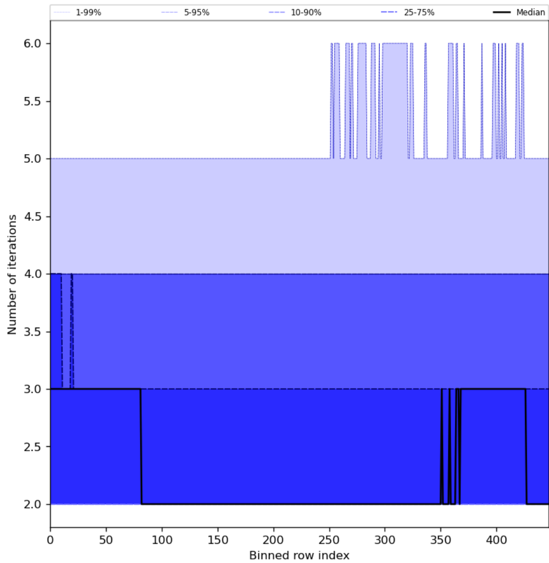
Figure 56: Along track statistics of “Number of iterations” for 2023-09-17 to 2023-09-19
