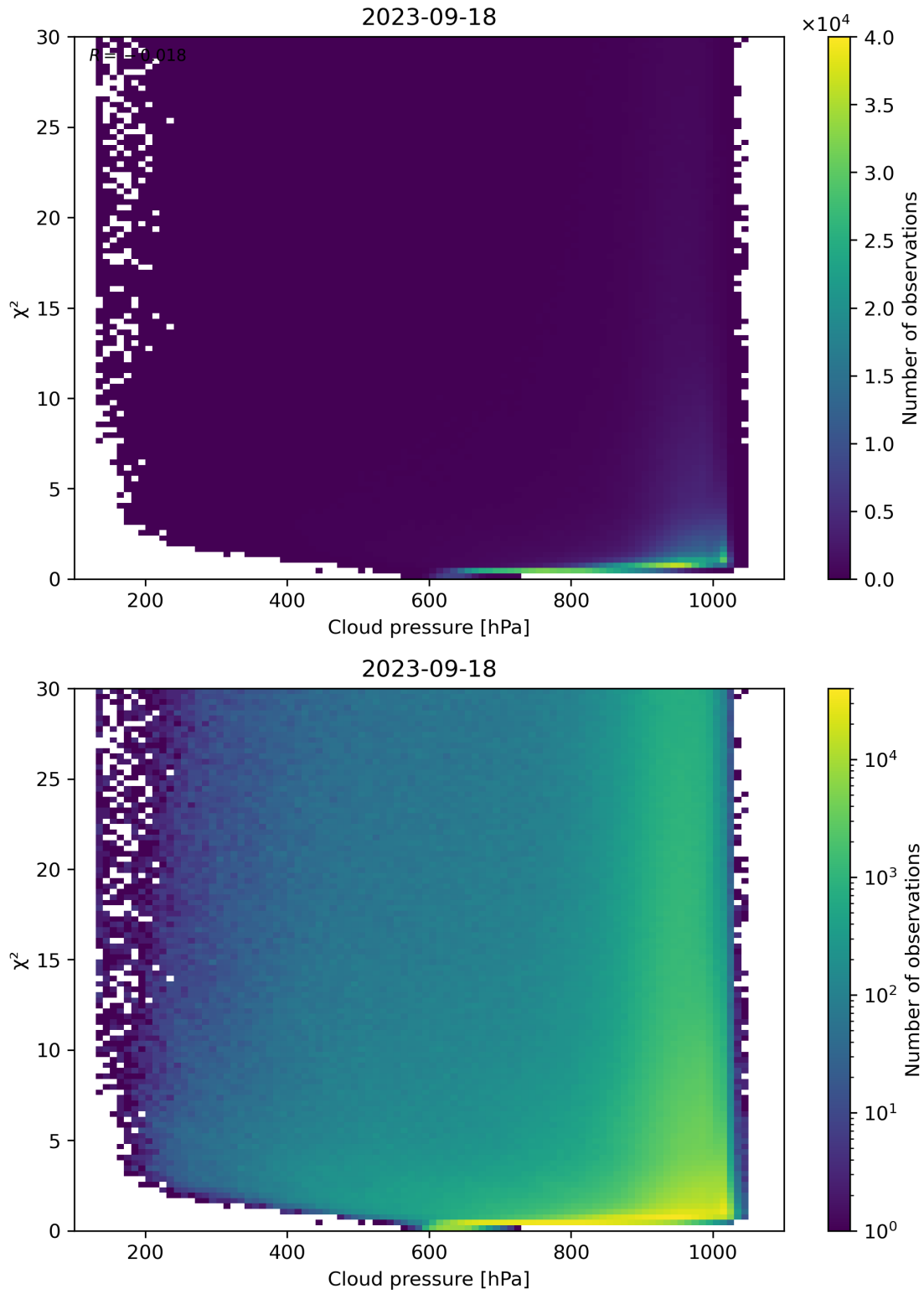
Figure 85: Scatter density plot of “Cloud pressure” against “ \chi^2 ” for 2023-09-17 to 2023-09-19.
