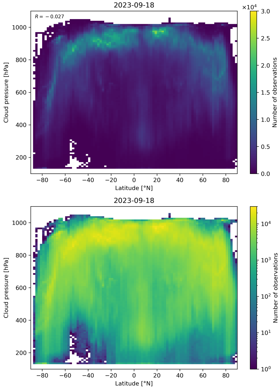
Figure 100: Scatter density plot of “Latitude” against “Cloud pressure” for 2023-09-17 to 2023-09-19.
