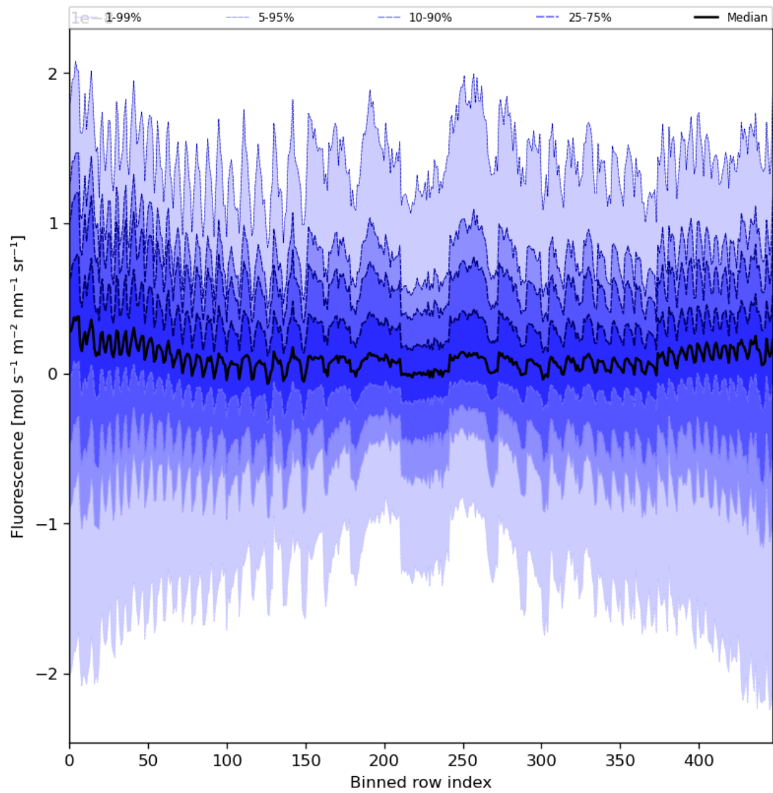
Figure 57: Along track statistics of “Fluorescence” for 2023-09-17 to 2023-09-19
