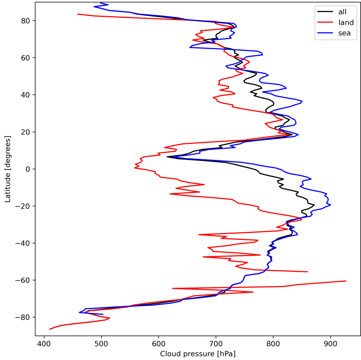
Figure 13: Zonal average of “Cloud pressure” for 2023-09-17 to 2023-09-19.
