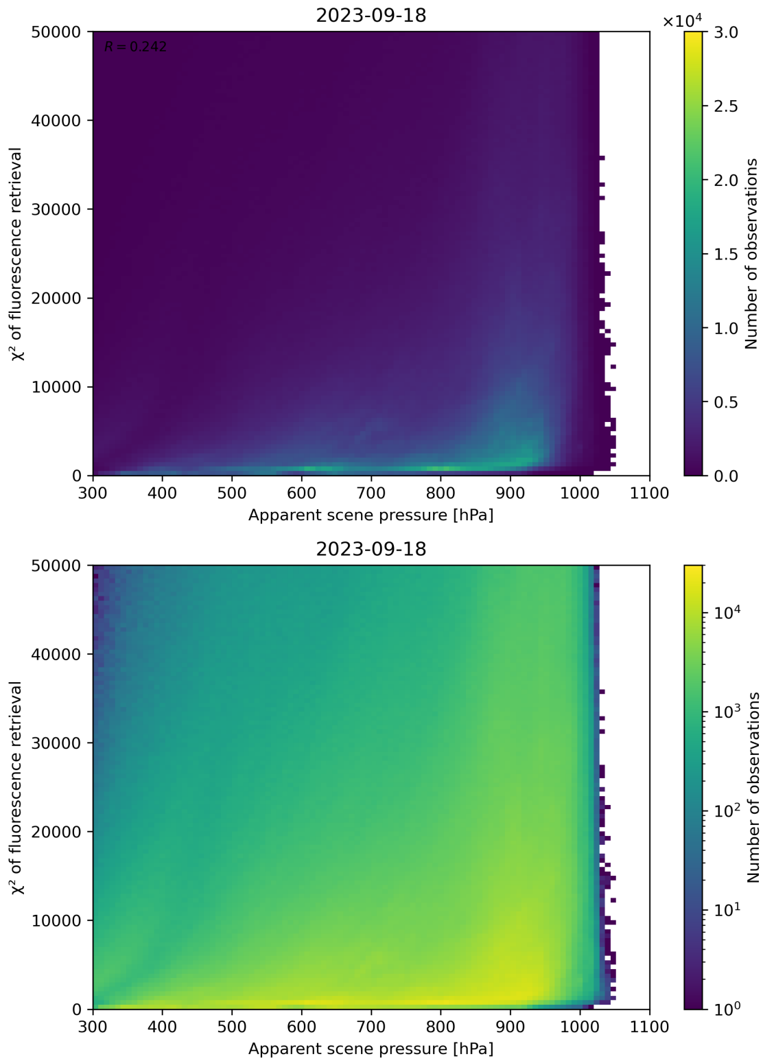
Figure 64: Scatter density plot of “Apparent scene pressure” against “ \chi^2 of fluorescence retrieval” for 2023-09-17 to 2023-09-19.
