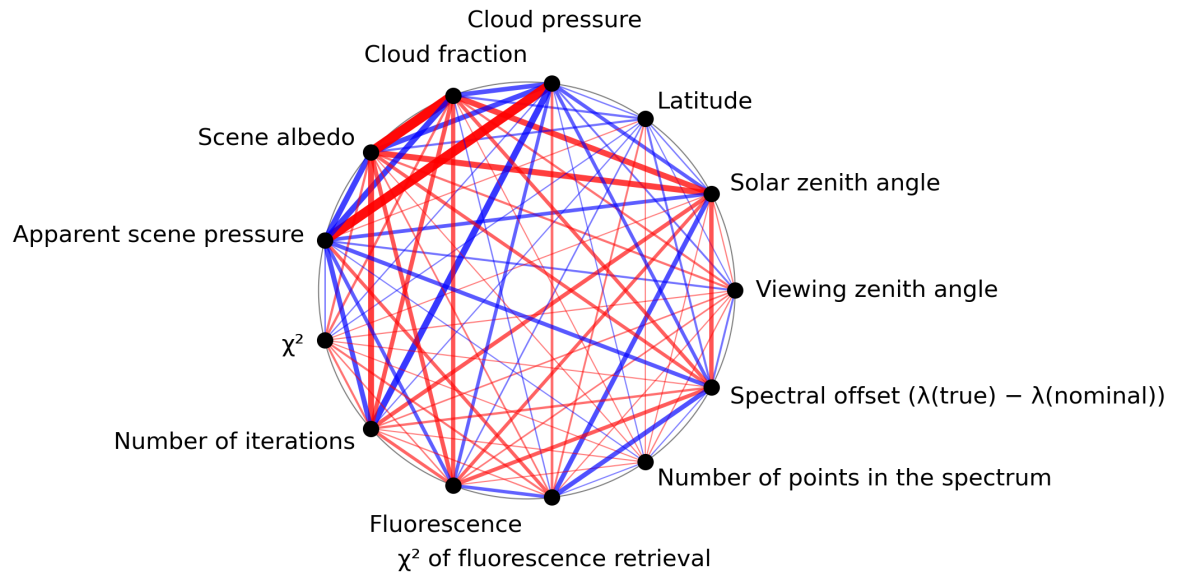
Figure 1: Map of correlation graph for 2023-09-17 to 2023-09-19.
