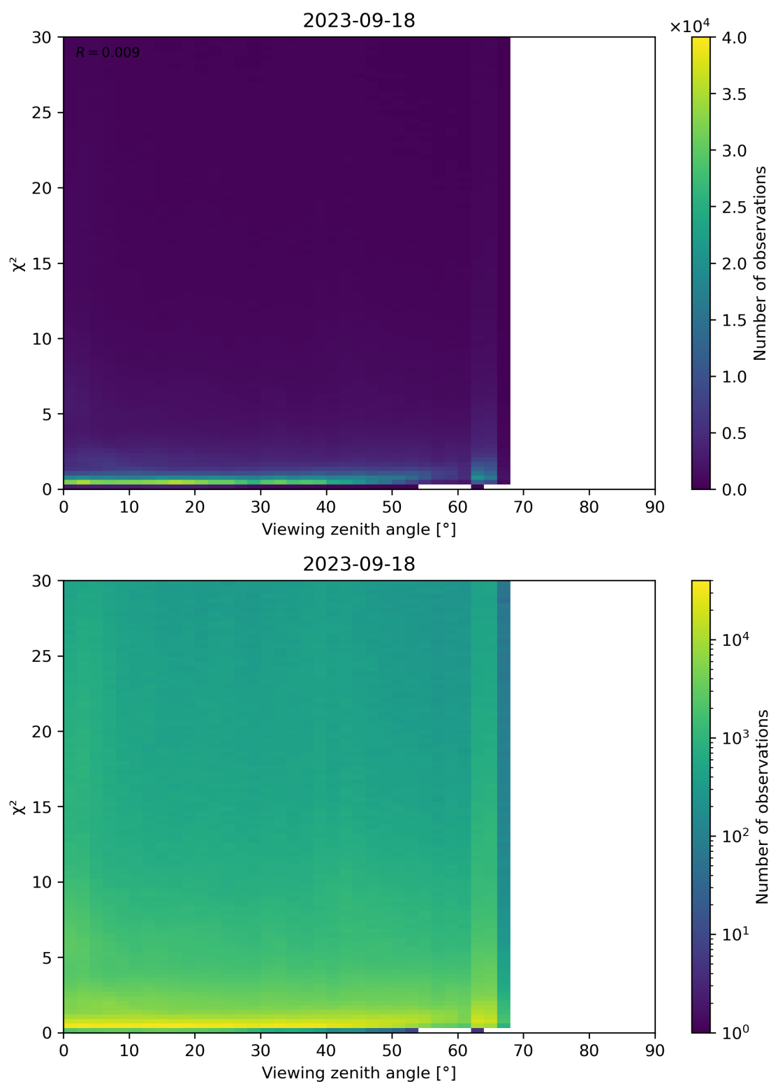
Figure 130: Scatter density plot of “Viewing zenith angle” against “ \chi^2 ” for 2023-09-17 to 2023-09-19.
