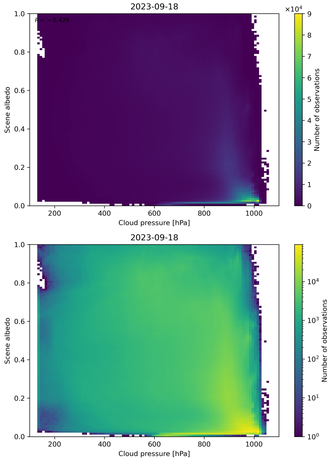
Figure 91: Scatter density plot of “Cloud pressure” against “Scene albedo” for 2023-09-17 to 2023-09-19.
