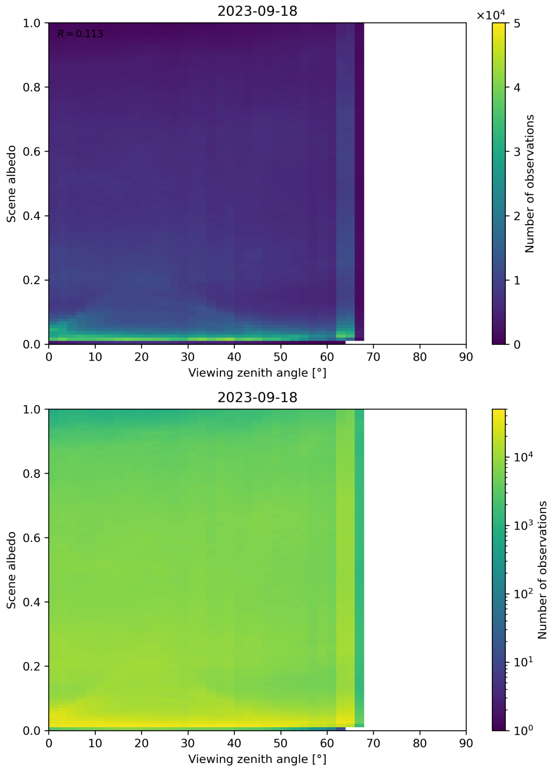
Figure 138: Scatter density plot of “Viewing zenith angle” against “Scene albedo” for 2023-09-17 to 2023-09-19.
