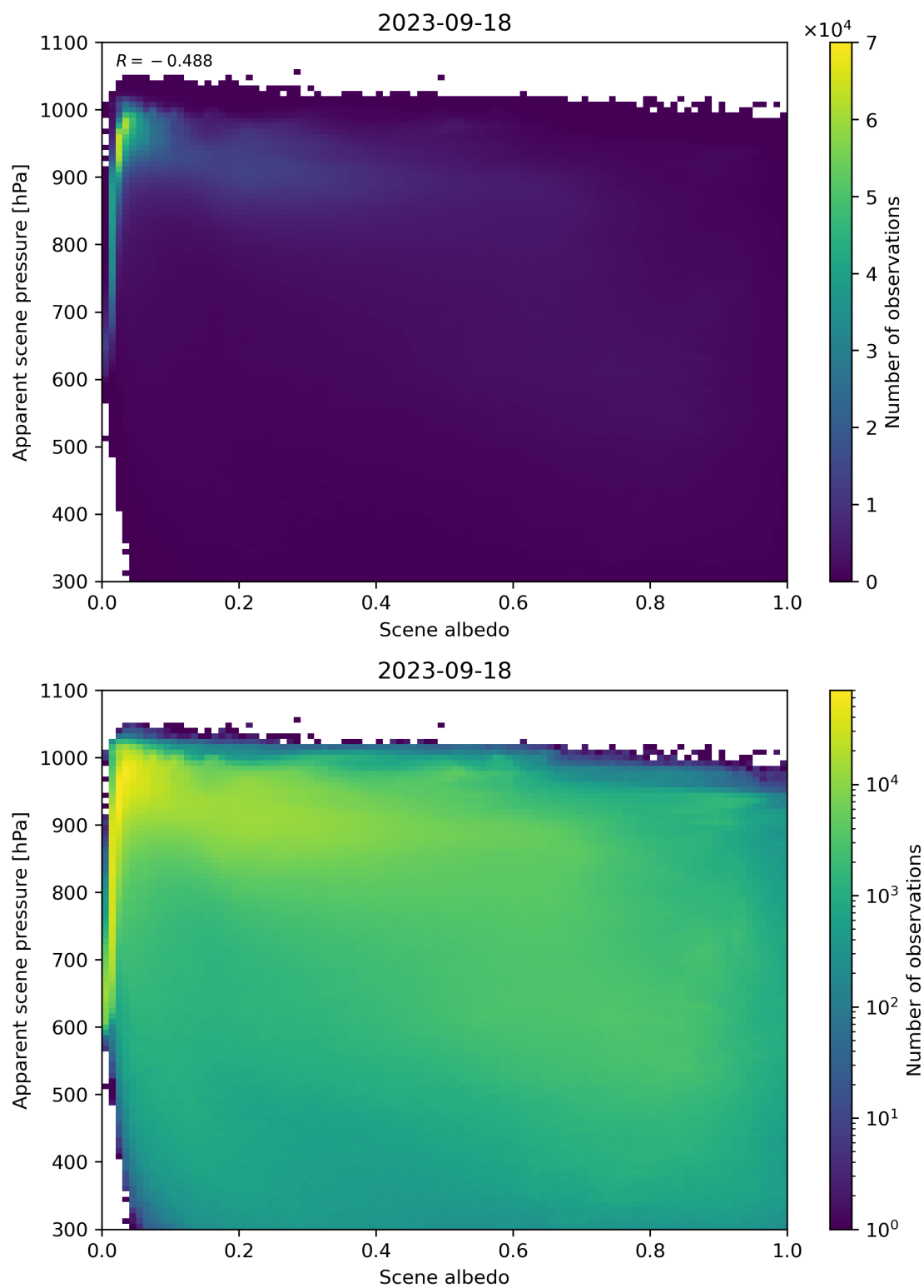
Figure 111: Scatter density plot of “Scene albedo” against “Apparent scene pressure” for 2023-09-17 to 2023-09-19.
