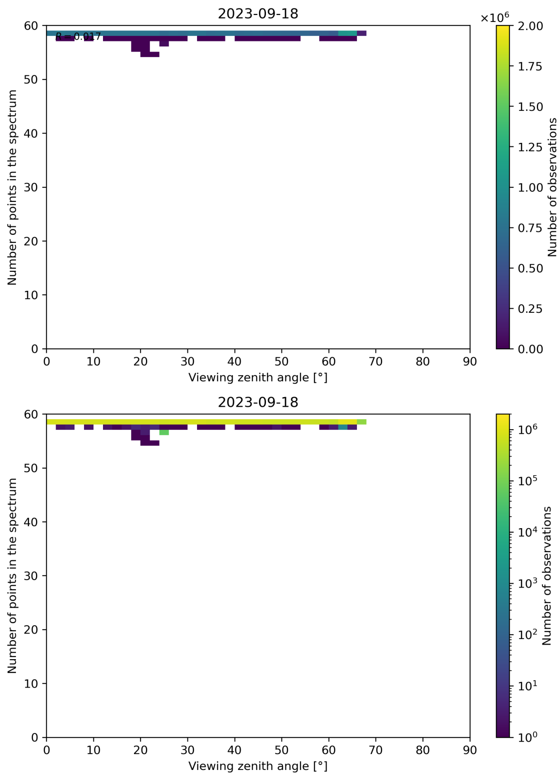
Figure 137: Scatter density plot of “Viewing zenith angle” against “Number of points in the spectrum” for 2023-09-17 to 2023-09-19.
