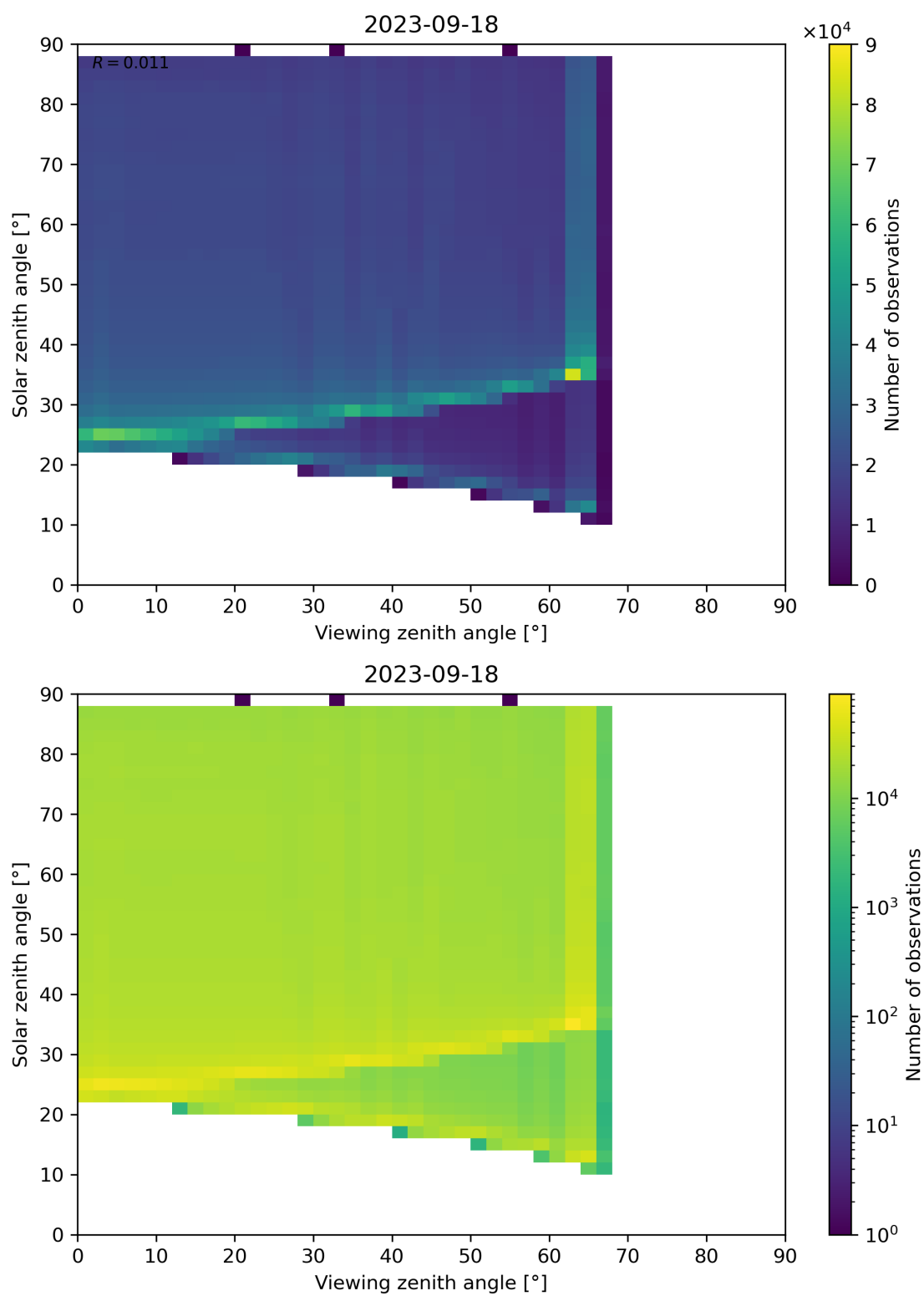
Figure 139: Scatter density plot of “Viewing zenith angle” against “Solar zenith angle” for 2023-09-17 to 2023-09-19.
