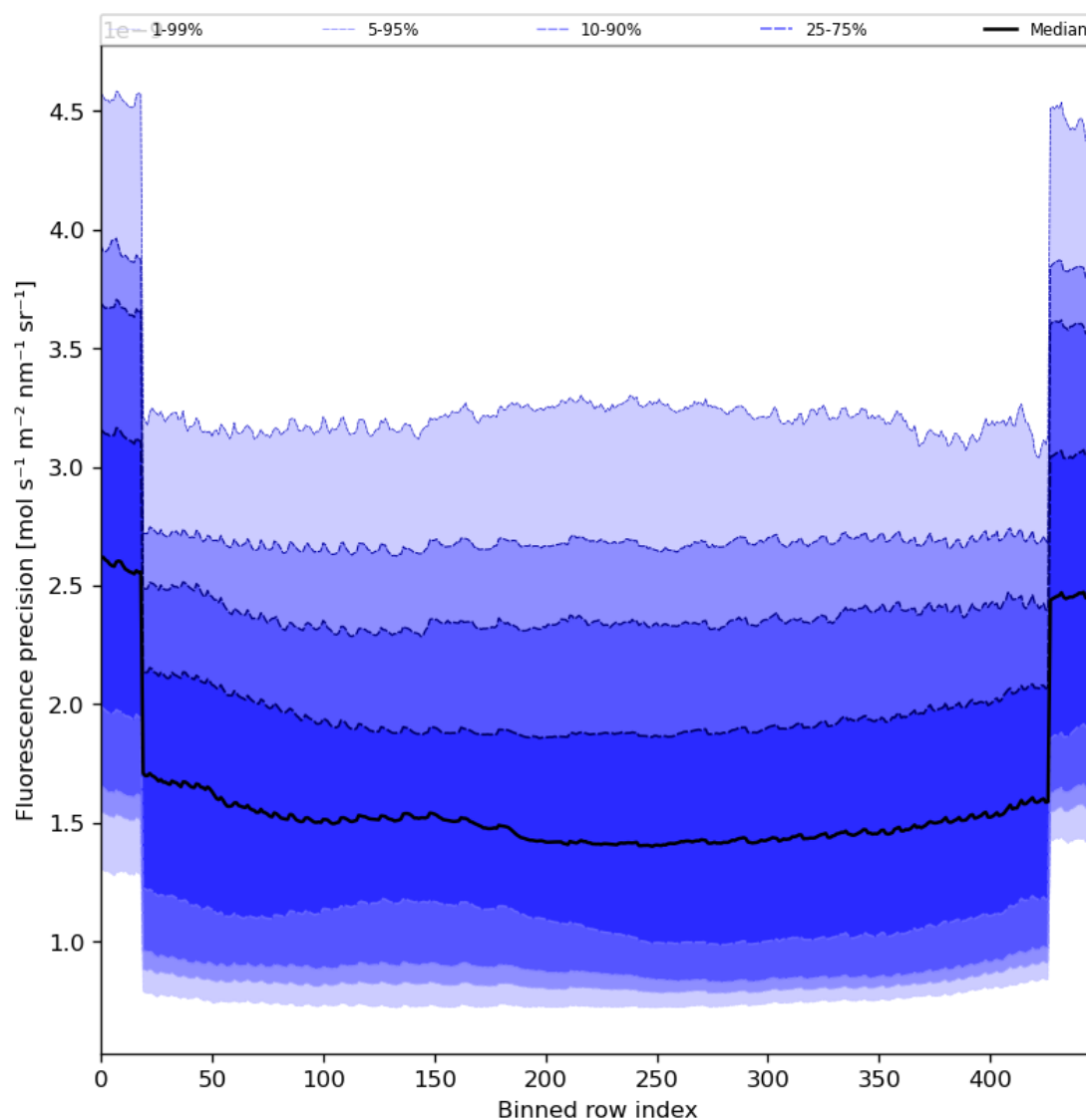
Figure 58: Along track statistics of “Fluorescence precision” for 2023-09-17 to 2023-09-19
