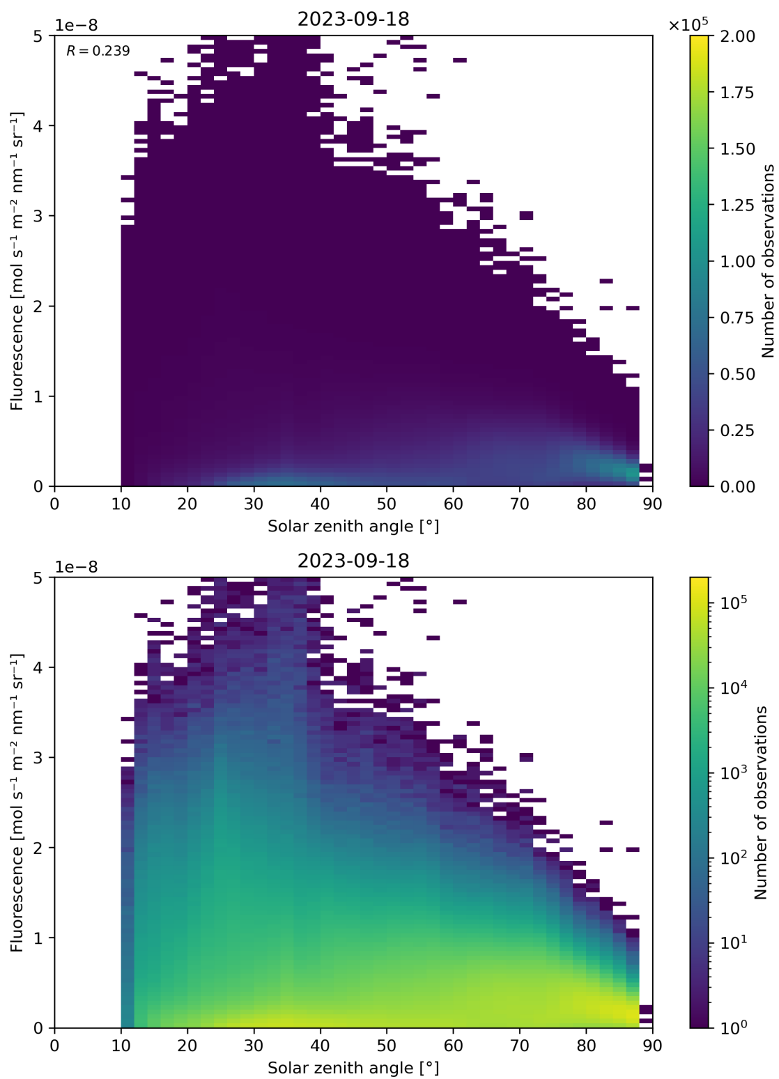
Figure 123: Scatter density plot of “Solar zenith angle” against “Fluorescence” for 2023-09-17 to 2023-09-19.
