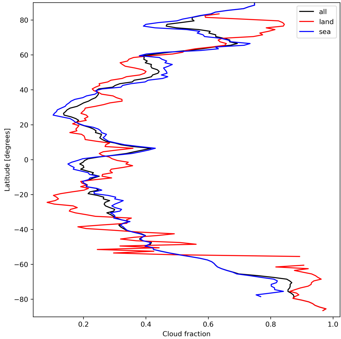
Figure 15: Zonal average of “Cloud fraction” for 2023-09-18 to 2023-09-20.
