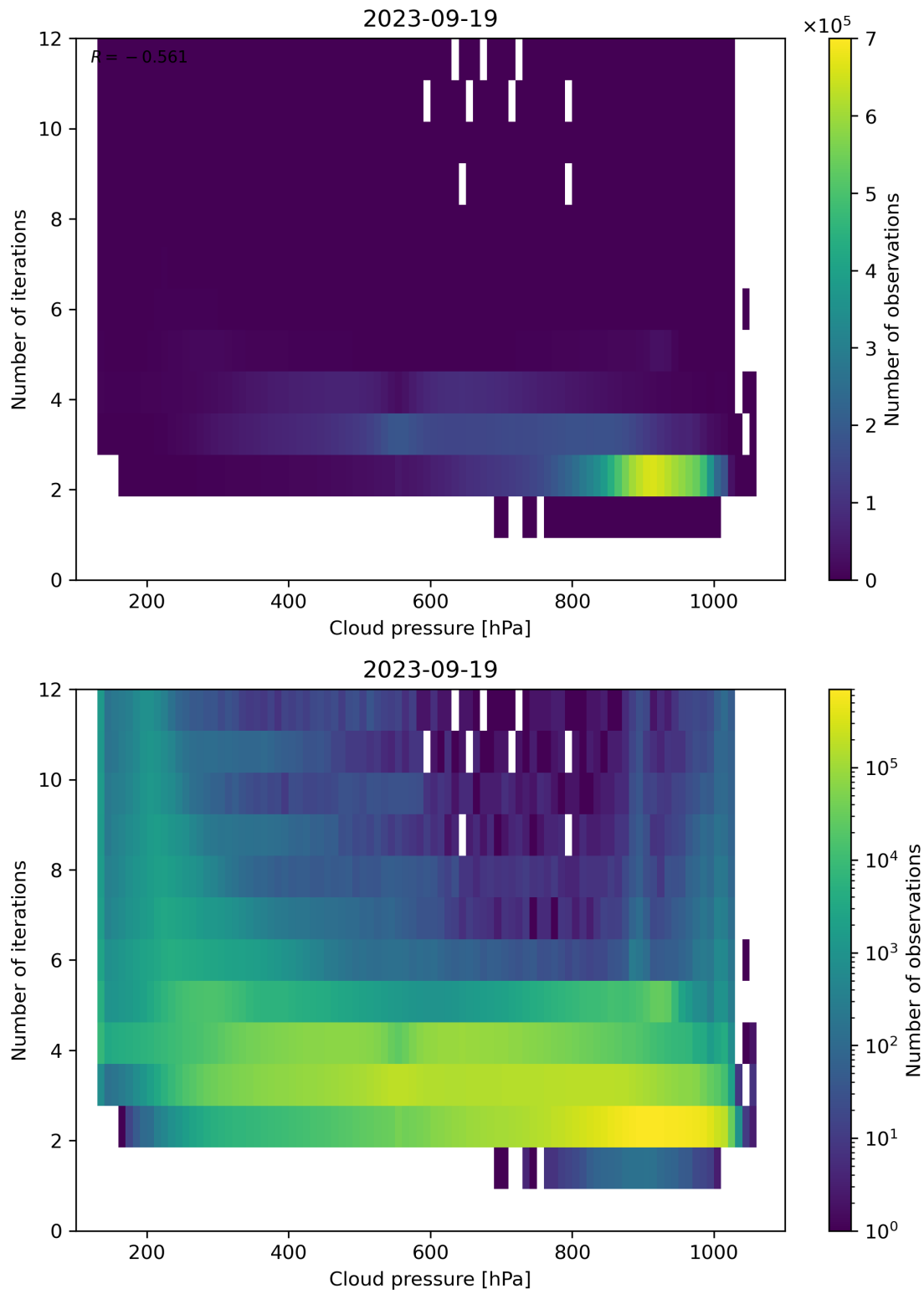
Figure 89: Scatter density plot of “Cloud pressure” against “Number of iterations” for 2023-09-18 to 2023-09-20.
