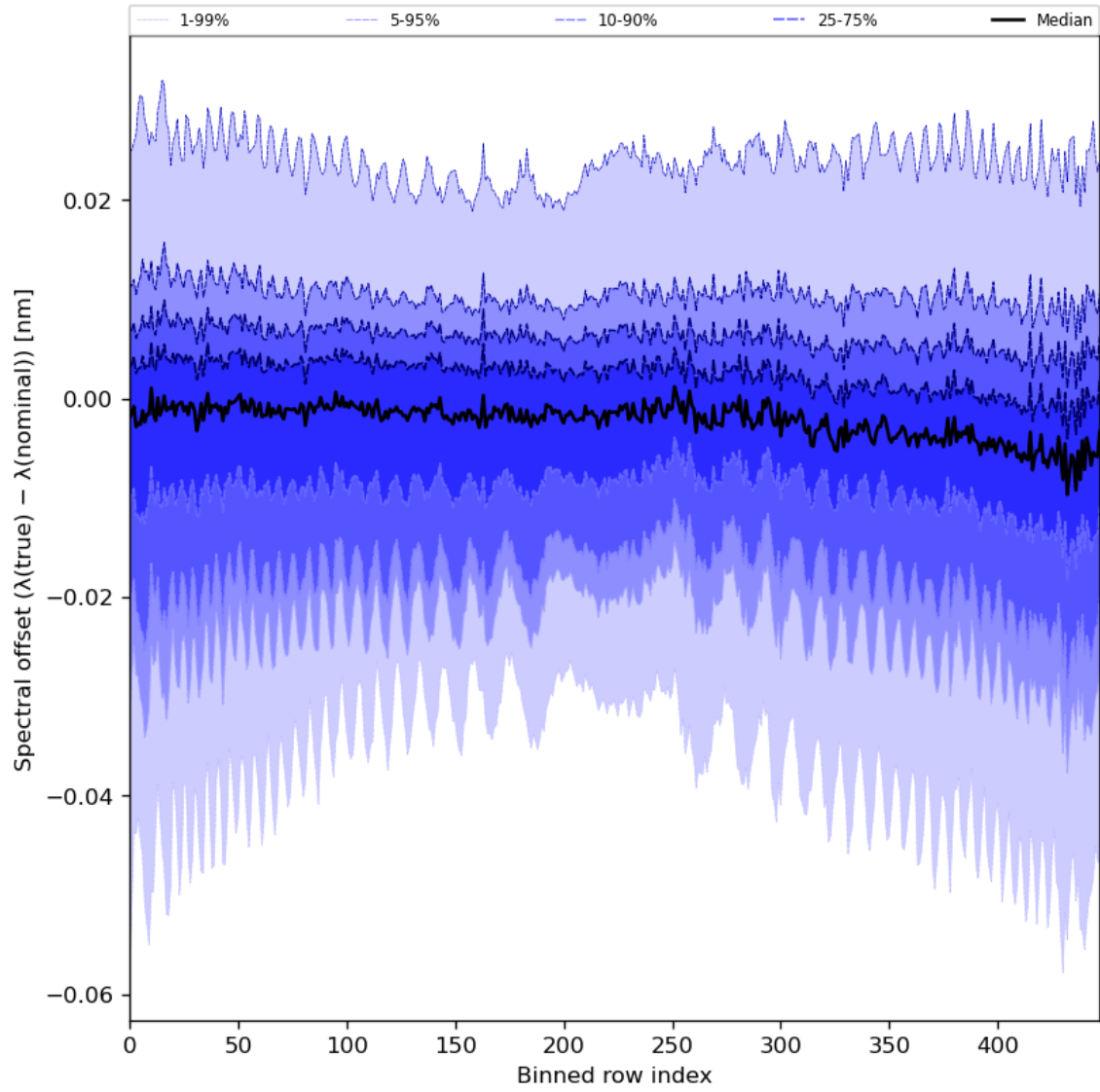
Figure 62: Along track statistics of “Spectral offset ( \lambda(\text{true}) - \lambda(\text{nominal}) )” for 2023-09-18 to 2023-09-20
