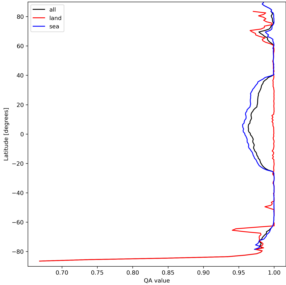
Figure 12: Zonal average of “QA value” for 2023-09-18 to 2023-09-20.
