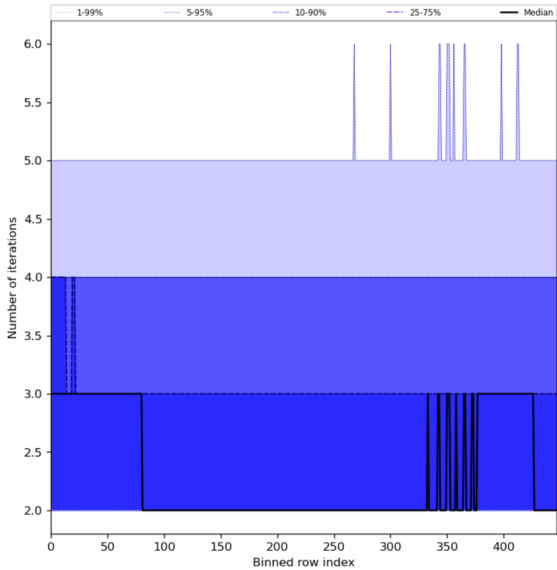
Figure 56: Along track statistics of “Number of iterations” for 2023-09-18 to 2023-09-20
