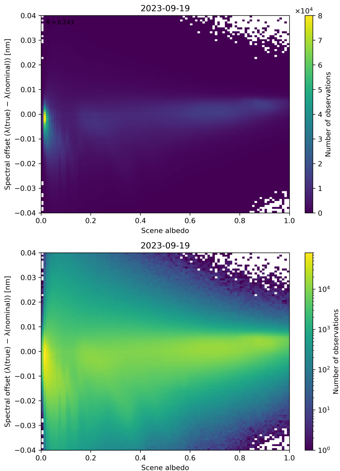
Figure 117: Scatter density plot of “Scene albedo” against “Spectral offset ( \lambda(\text{true}) - \lambda(\text{nominal}) )” for 2023-09-18 to 2023-09-20.
