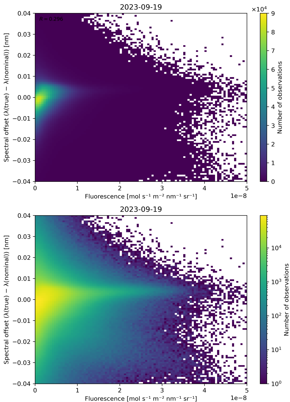
Figure 95: Scatter density plot of “Fluorescence” against “Spectral offset ( \lambda(\text{true}) - \lambda(\text{nominal}) )” for 2023-09-18 to 2023-09-20.
