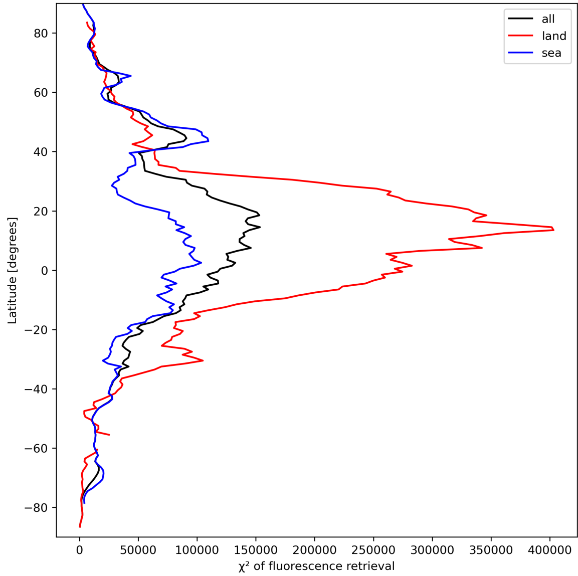
Figure 25: Zonal average of “ \chi^2 of fluorescence retrieval” for 2023-09-18 to 2023-09-20.
