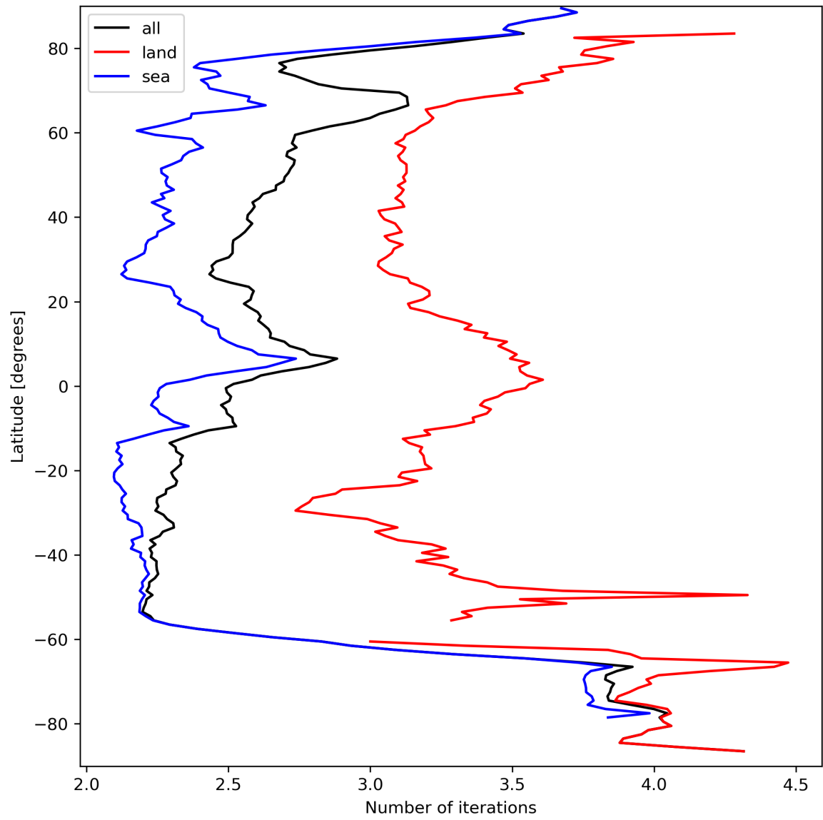
Figure 22: Zonal average of “Number of iterations” for 2023-09-18 to 2023-09-20.
