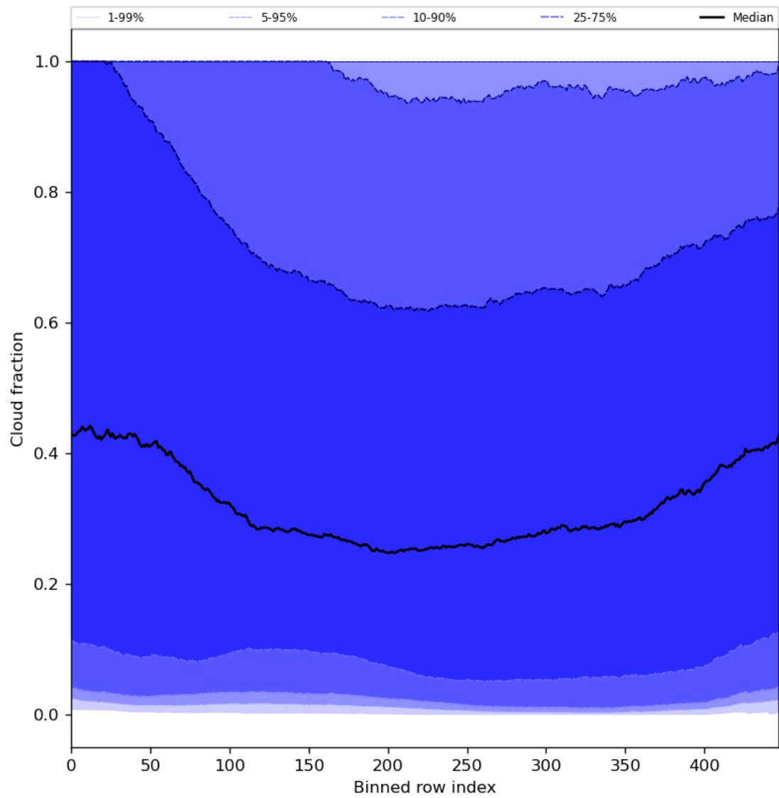
Figure 49: Along track statistics of “Cloud fraction” for 2023-09-18 to 2023-09-20
