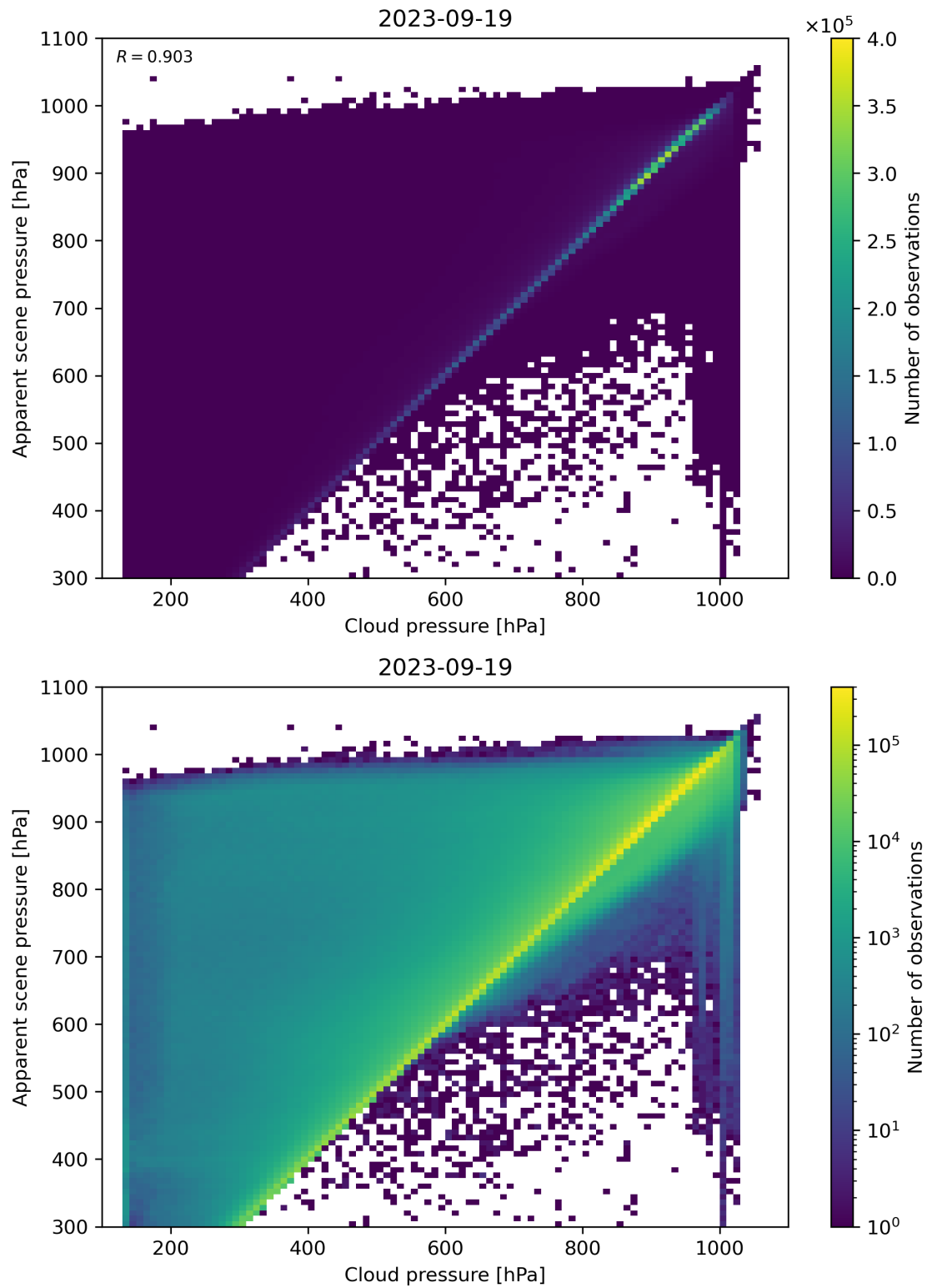
Figure 84: Scatter density plot of “Cloud pressure” against “Apparent scene pressure” for 2023-09-18 to 2023-09-20.
