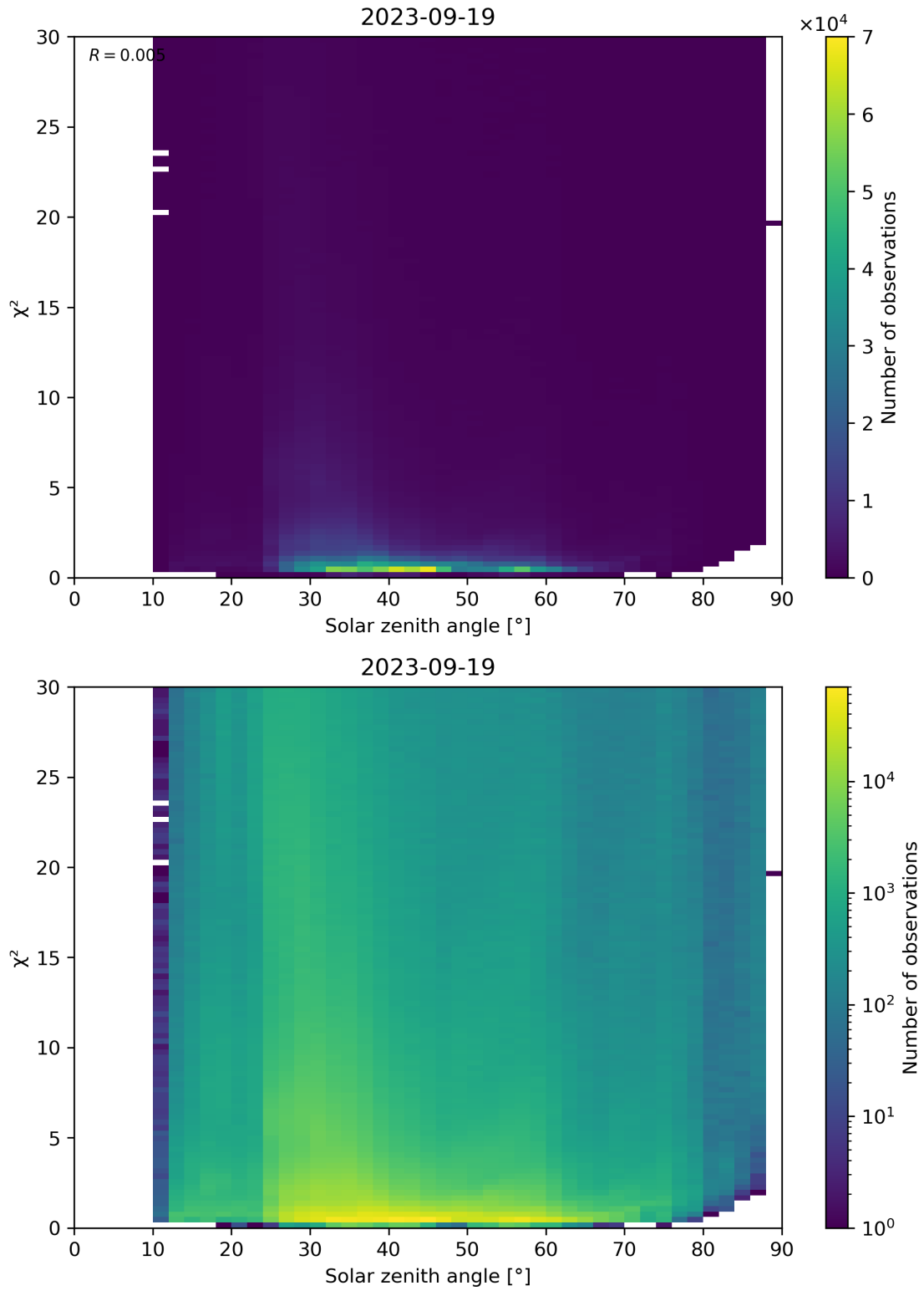
Figure 119: Scatter density plot of “Solar zenith angle” against “ \chi^2 ” for 2023-09-18 to 2023-09-20.
