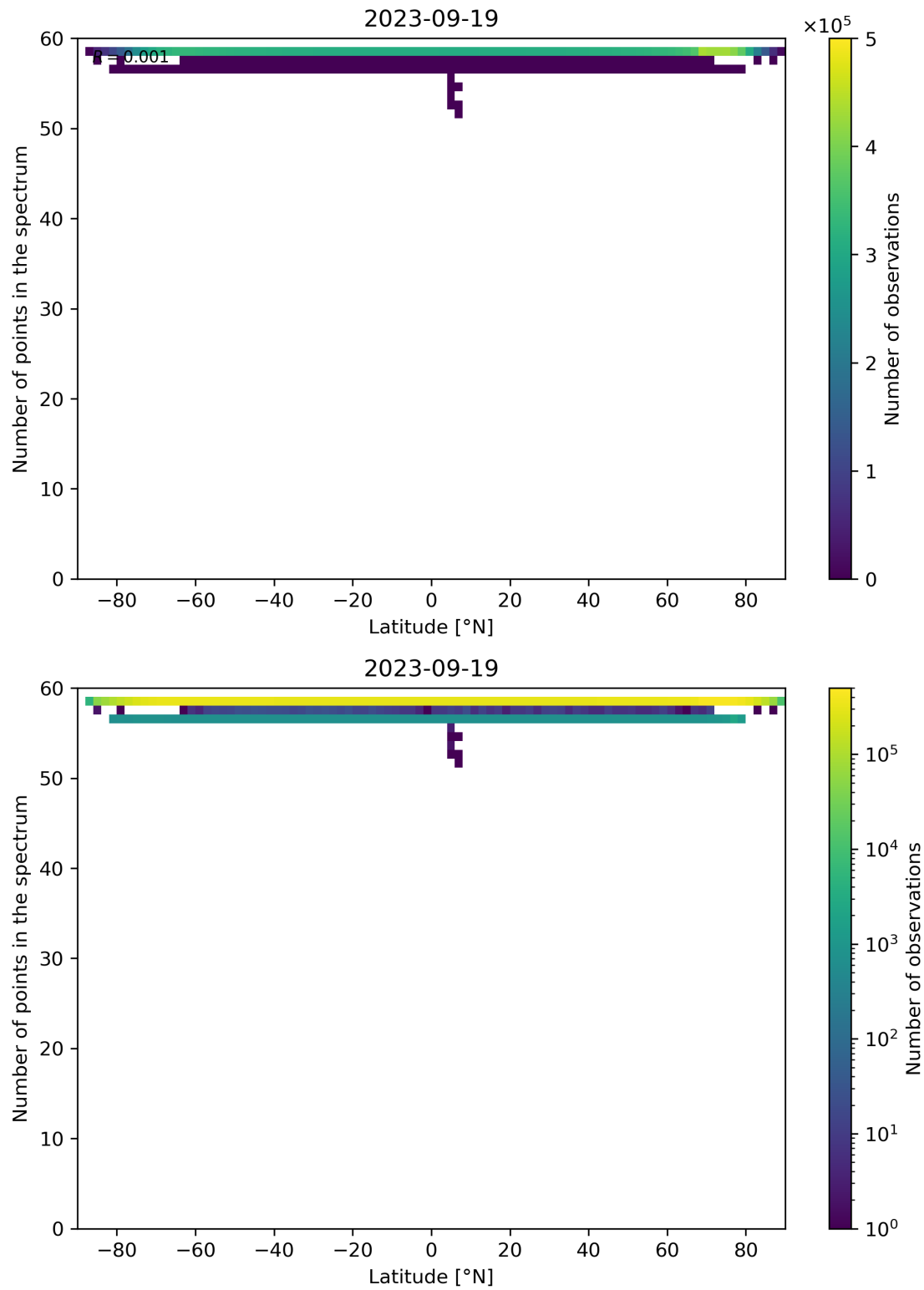
Figure 103: Scatter density plot of “Latitude” against “Number of points in the spectrum” for 2023-09-18 to 2023-09-20.
