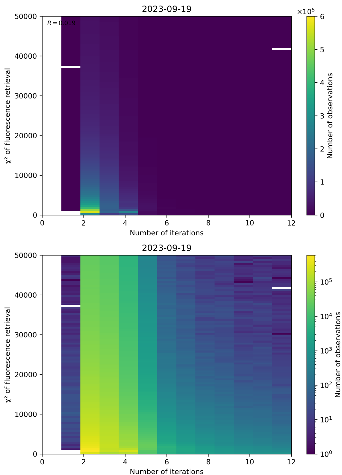
Figure 106: Scatter density plot of “Number of iterations” against “ \chi^2 of fluorescence retrieval” for 2023-09-18 to 2023-09-20.
