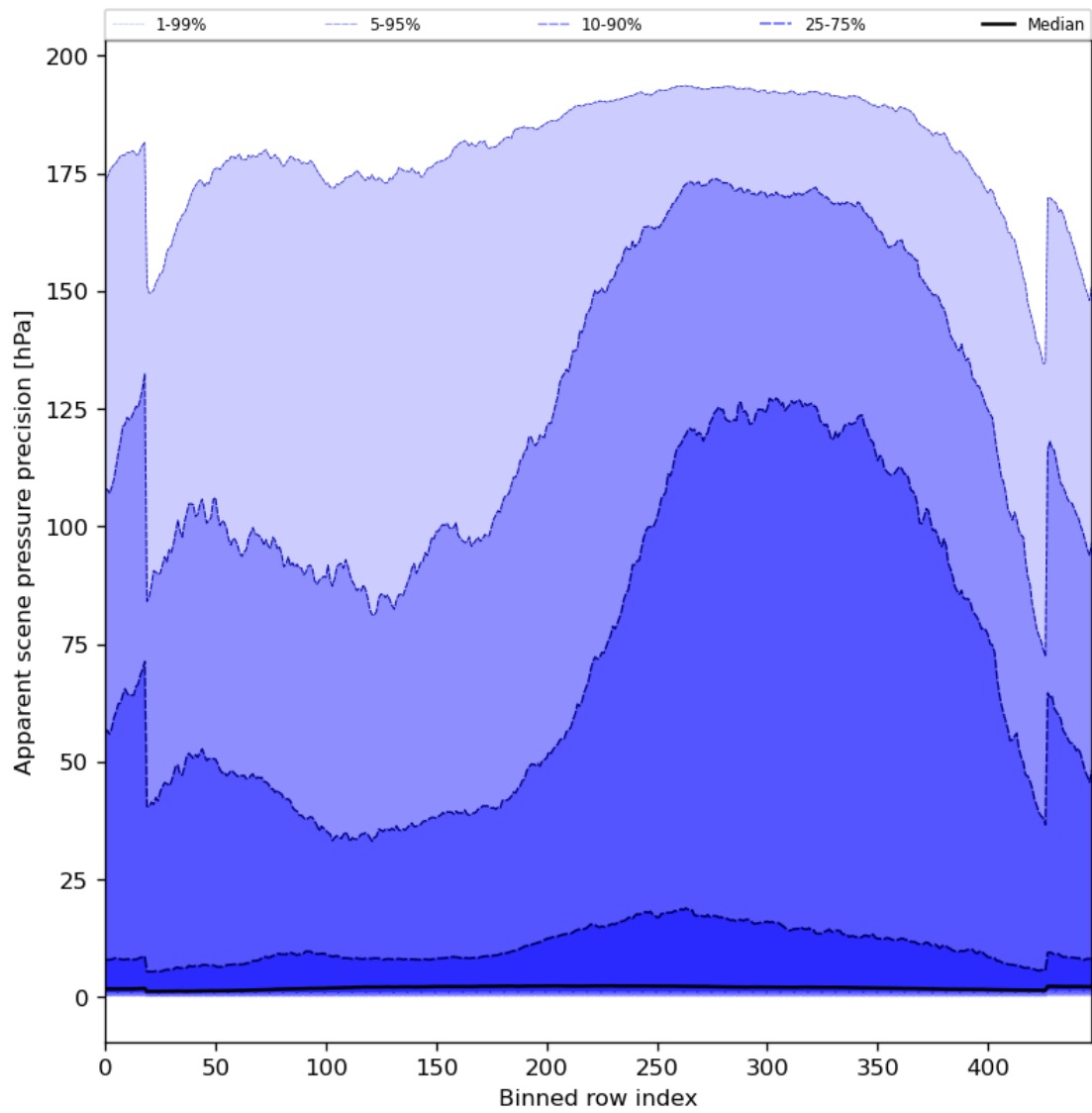
Figure 54: Along track statistics of “Apparent scene pressure precision” for 2023-09-18 to 2023-09-20
