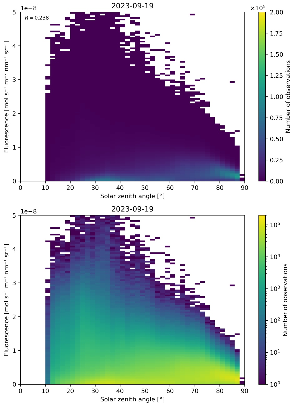
Figure 123: Scatter density plot of “Solar zenith angle” against “Fluorescence” for 2023-09-18 to 2023-09-20.
