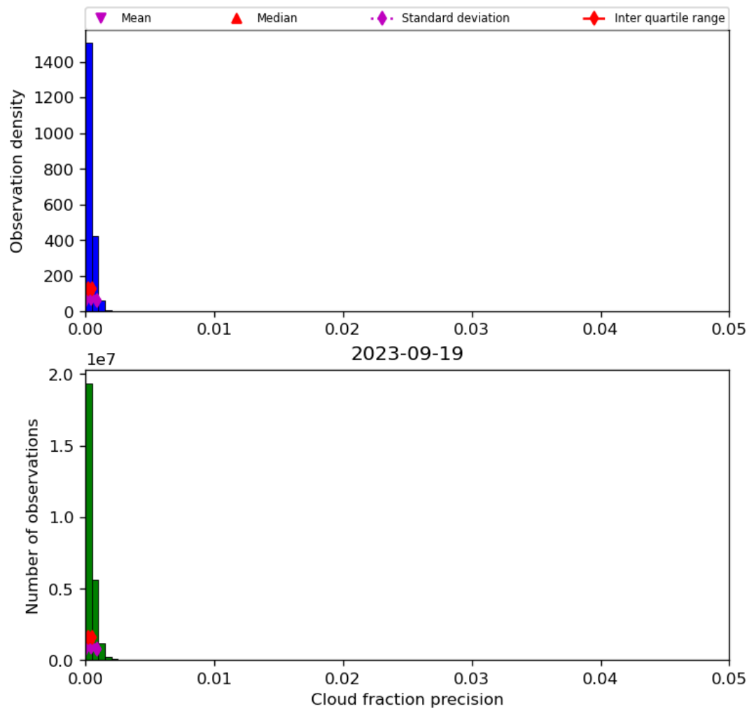
Figure 33: Histogram of “Cloud fraction precision” for 2023-09-18 to 2023-09-20
