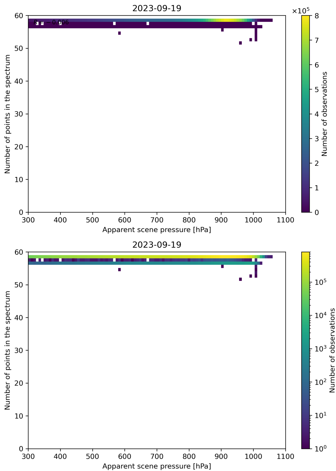
Figure 67: Scatter density plot of “Apparent scene pressure” against “Number of points in the spectrum” for 2023-09-18 to 2023-09-20.
