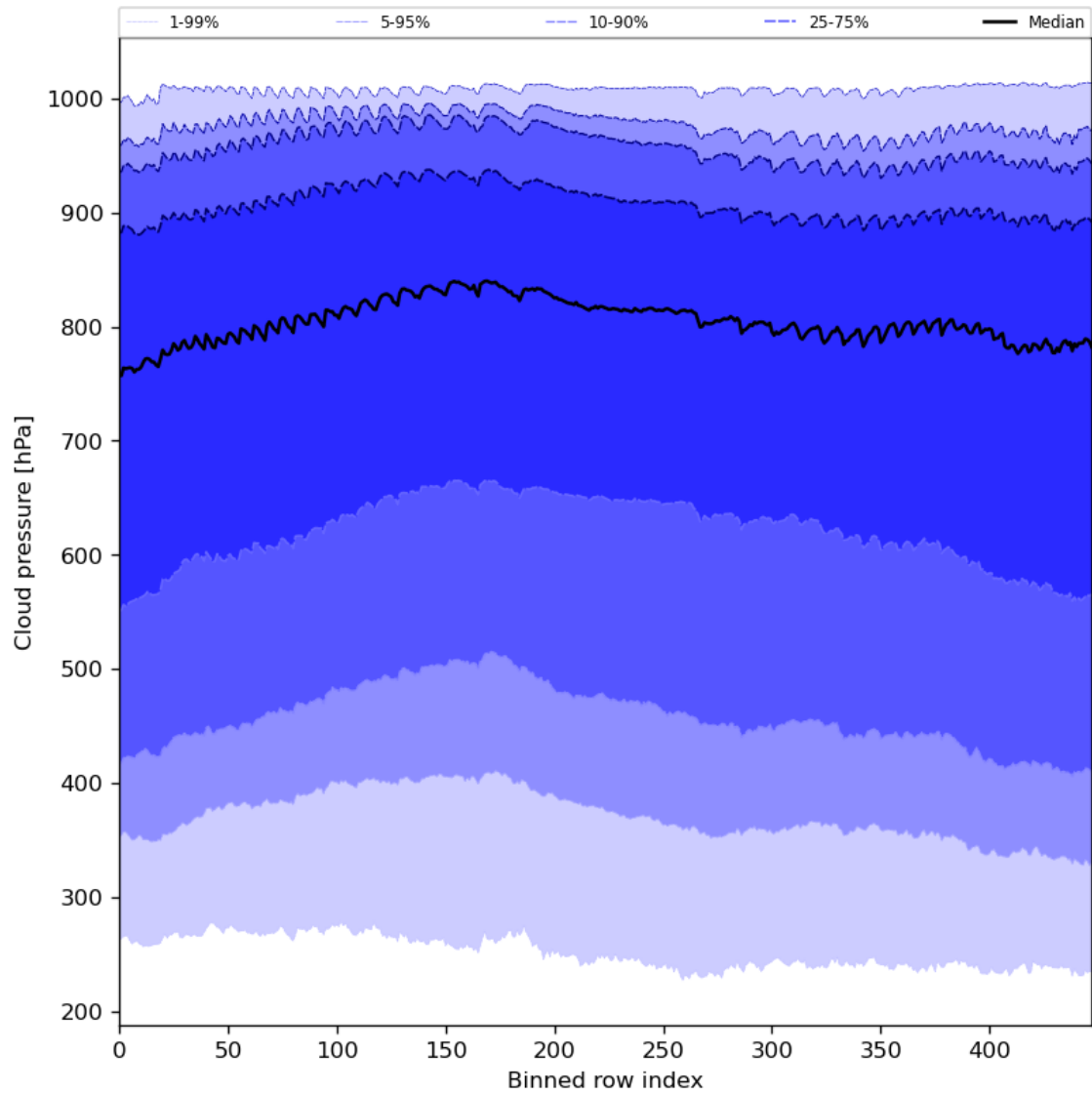
Figure 47: Along track statistics of "Cloud pressure" for 2023-09-18 to 2023-09-20
