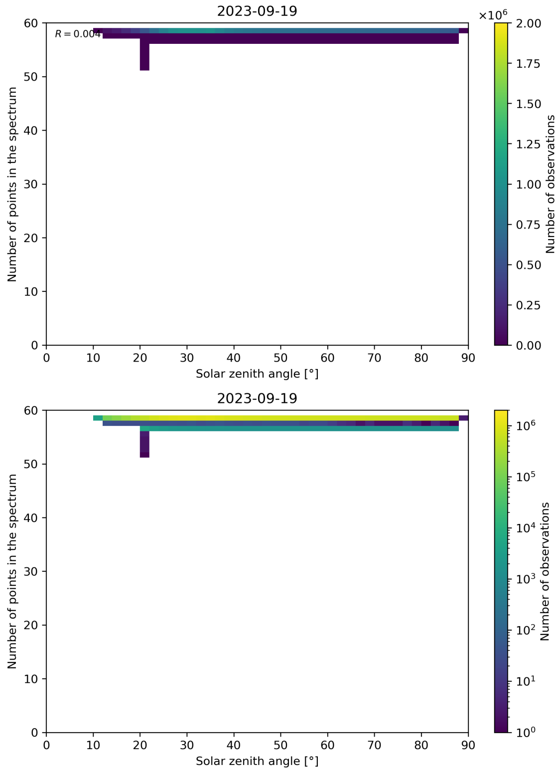
Figure 126: Scatter density plot of “Solar zenith angle” against “Number of points in the spectrum” for 2023-09-18 to 2023-09-20.
