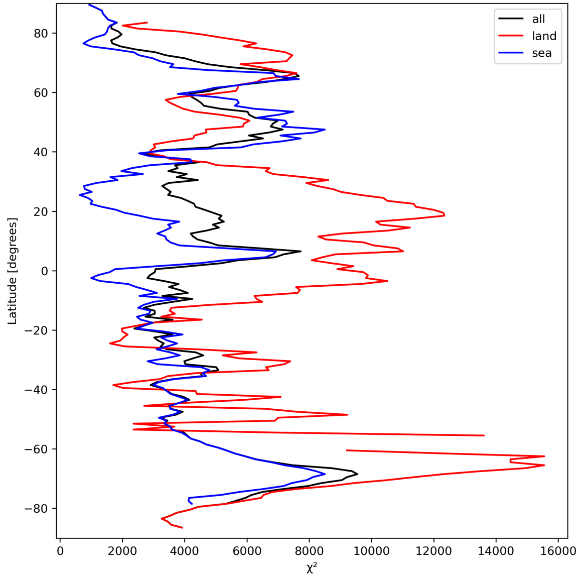
Figure 21: Zonal average of “ \chi^2 ” for 2023-09-18 to 2023-09-20.
