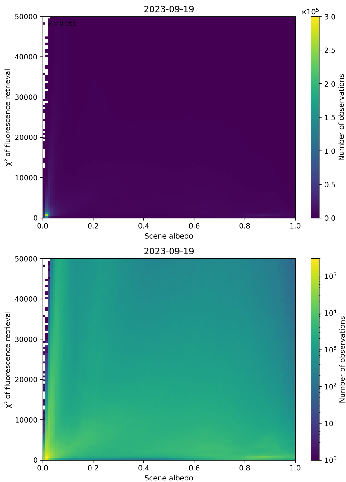
Figure 113: Scatter density plot of “Scene albedo” against “ \chi^2 of fluorescence retrieval” for 2023-09-18 to 2023-09-20.
