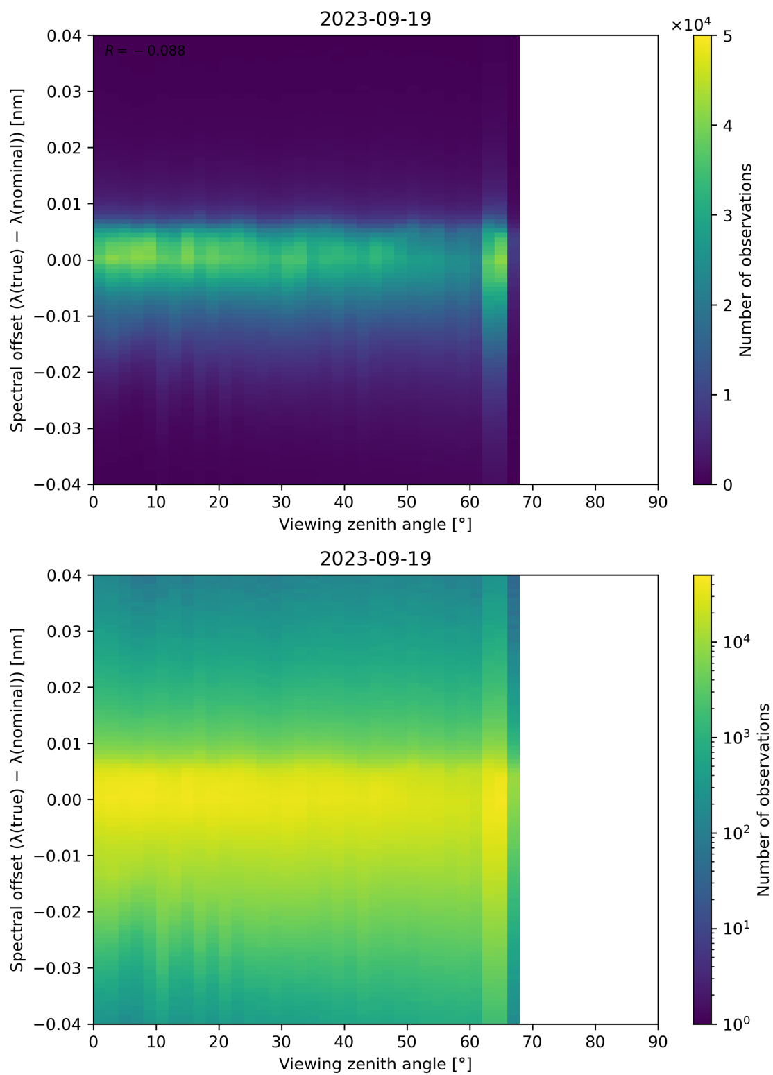
Figure 140: Scatter density plot of “Viewing zenith angle” against “Spectral offset ( \lambda(\text{true}) - \lambda(\text{nominal}) )” for 2023-09-18 to 2023-09-20.
