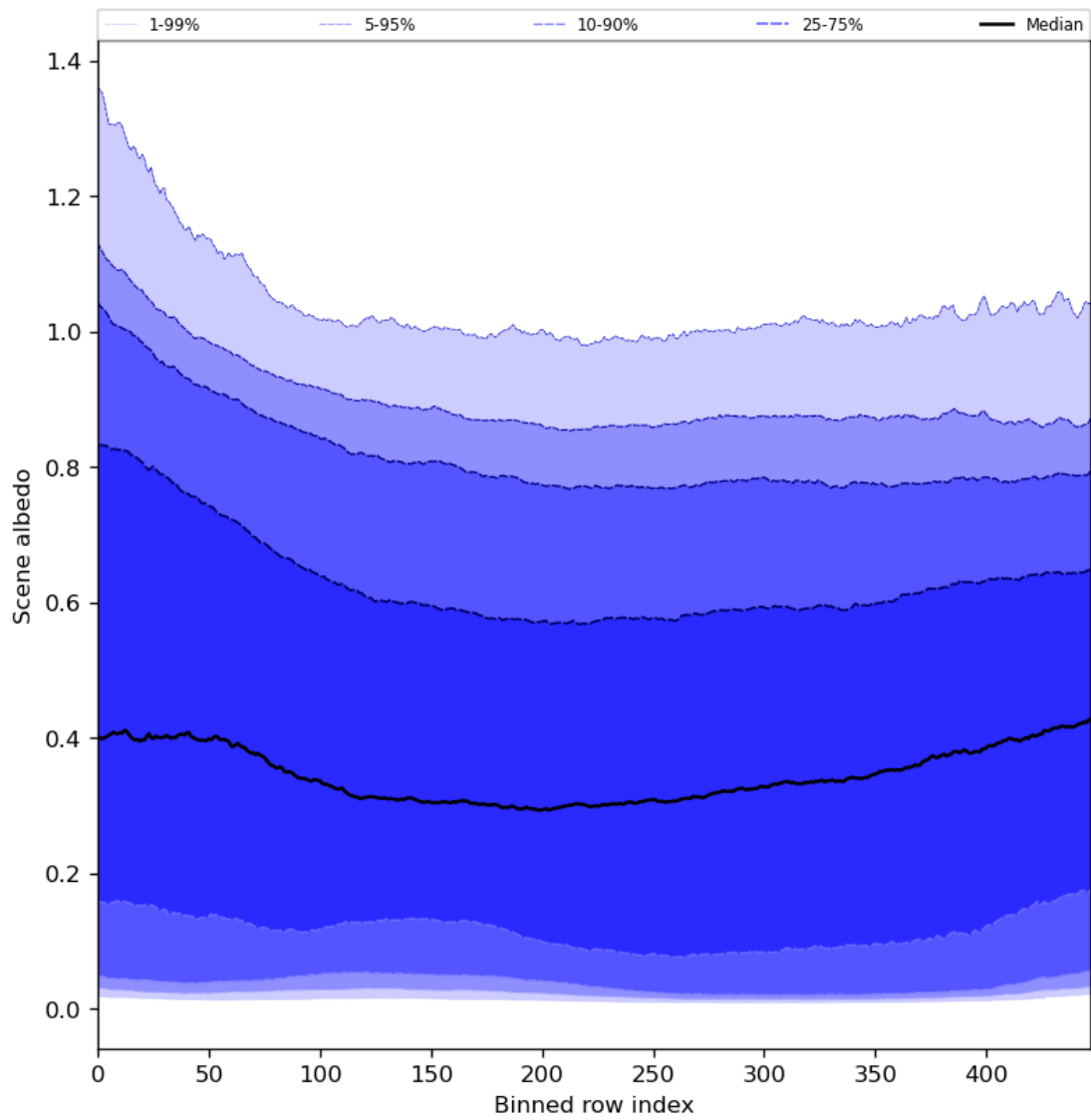
Figure 51: Along track statistics of “Scene albedo” for 2023-09-18 to 2023-09-20
