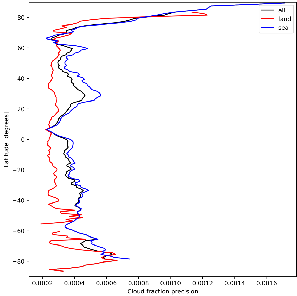
Figure 16: Zonal average of “Cloud fraction precision” for 2023-09-18 to 2023-09-20.
