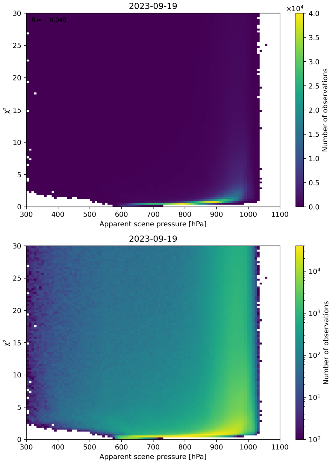
Figure 63: Scatter density plot of “Apparent scene pressure” against “ \chi^2 ” for 2023-09-18 to 2023-09-20.
