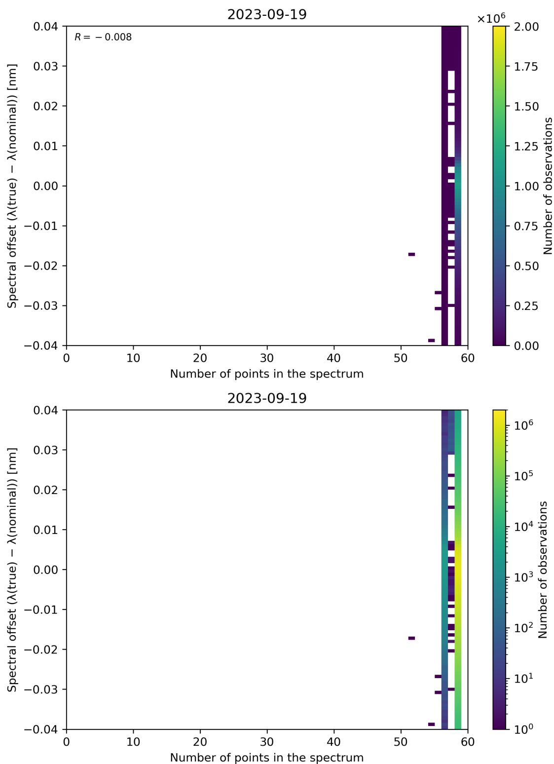
Figure 110: Scatter density plot of “Number of points in the spectrum” against “Spectral offset ( \lambda(\text{true}) - \lambda(\text{nominal}) )” for 2023-09-18 to 2023-09-20.
