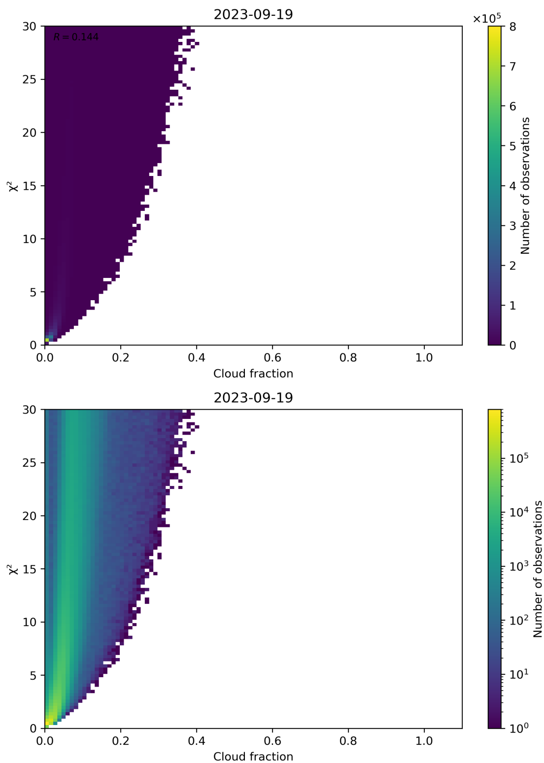
Figure 77: Scatter density plot of “Cloud fraction” against “ \chi^2 ” for 2023-09-18 to 2023-09-20.
