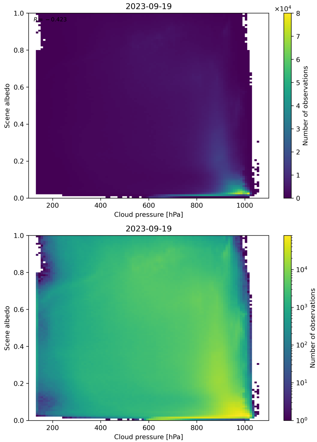
Figure 91: Scatter density plot of “Cloud pressure” against “Scene albedo” for 2023-09-18 to 2023-09-20.
