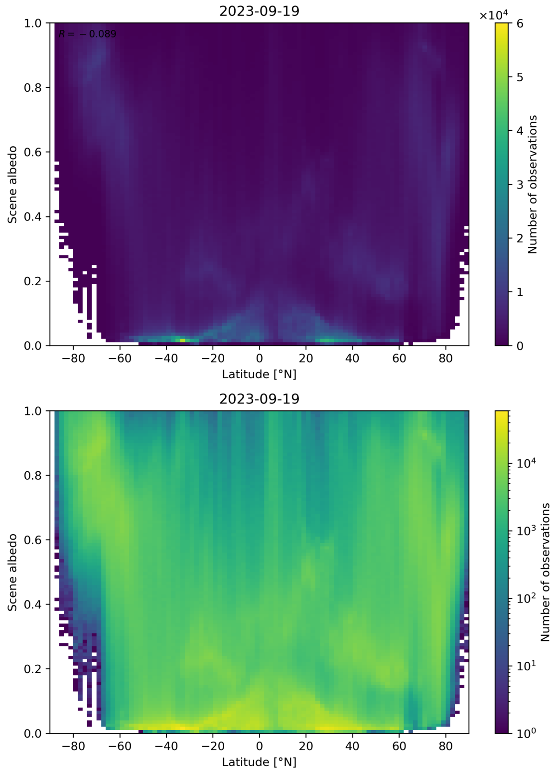
Figure 104: Scatter density plot of “Latitude” against “Scene albedo” for 2023-09-18 to 2023-09-20.
