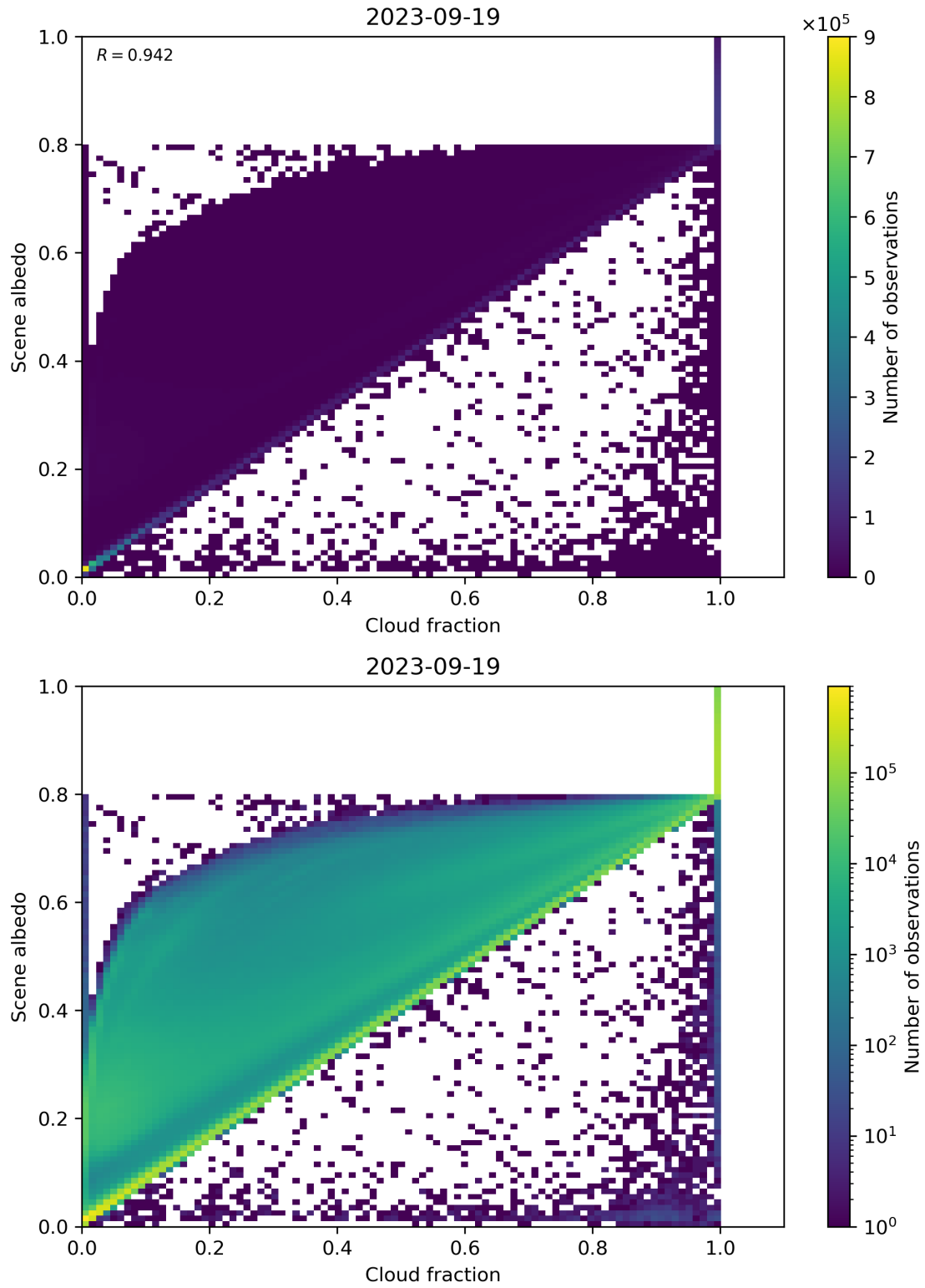
Figure 82: Scatter density plot of “Cloud fraction” against “Scene albedo” for 2023-09-18 to 2023-09-20.
