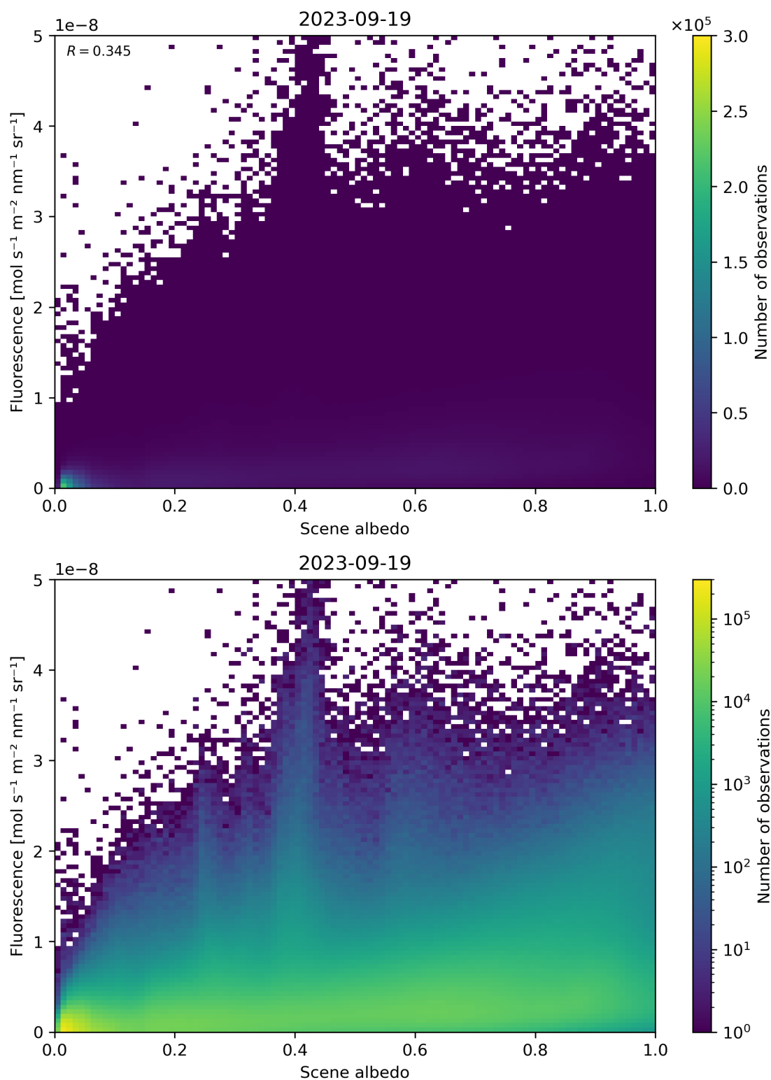
Figure 114: Scatter density plot of “Scene albedo” against “Fluorescence” for 2023-09-18 to 2023-09-20.
