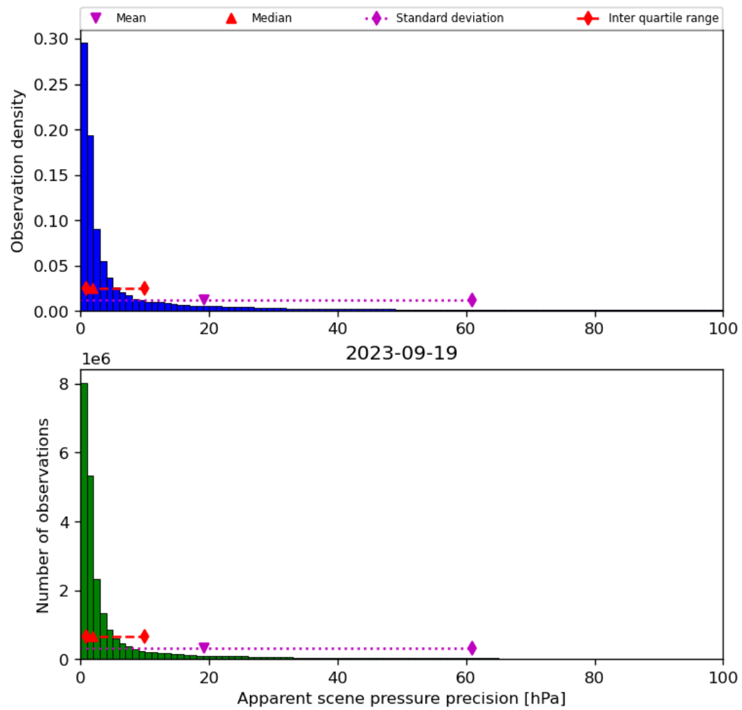
Figure 37: Histogram of “Apparent scene pressure precision” for 2023-09-18 to 2023-09-20
