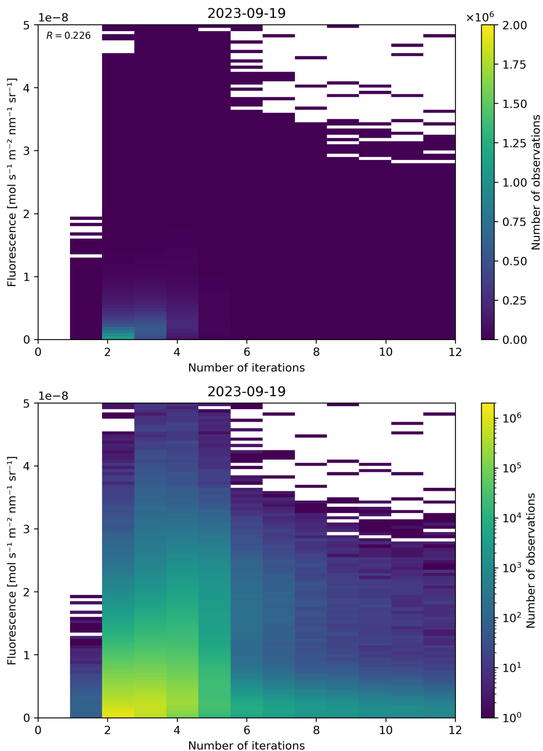
Figure 107: Scatter density plot of "Number of iterations" against "Fluorescence" for 2023-09-18 to 2023-09-20.
