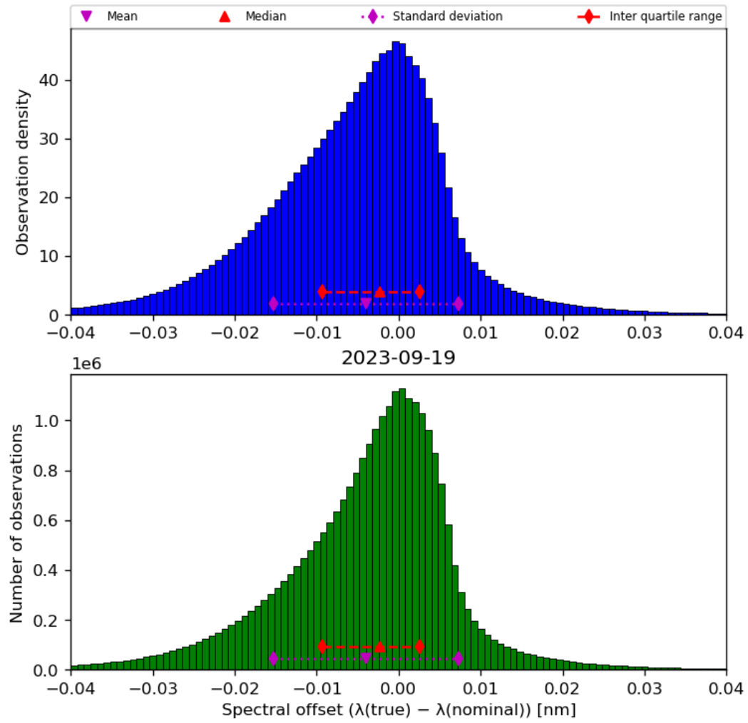
Figure 45: Histogram of “Spectral offset ( \lambda(\text{true}) - \lambda(\text{nominal}) )” for 2023-09-18 to 2023-09-20
