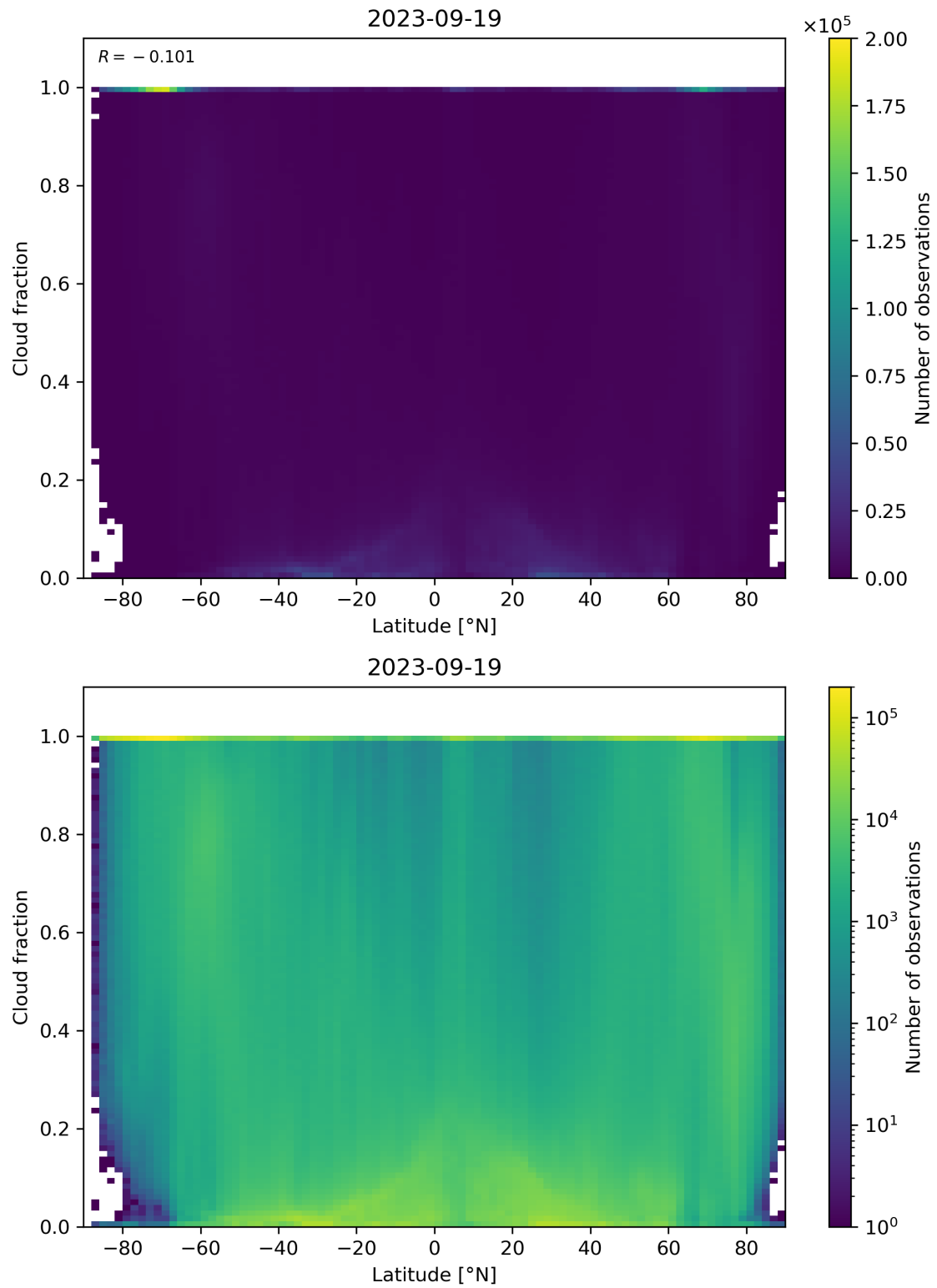
Figure 99: Scatter density plot of “Latitude” against “Cloud fraction” for 2023-09-18 to 2023-09-20.
