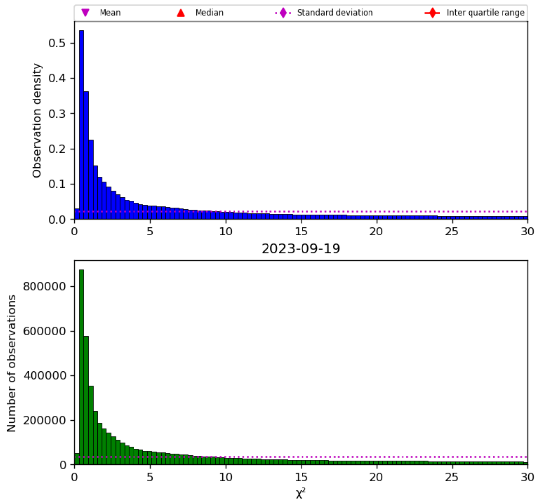
Figure 38: Histogram of “ \chi^2 ” for 2023-09-18 to 2023-09-20
