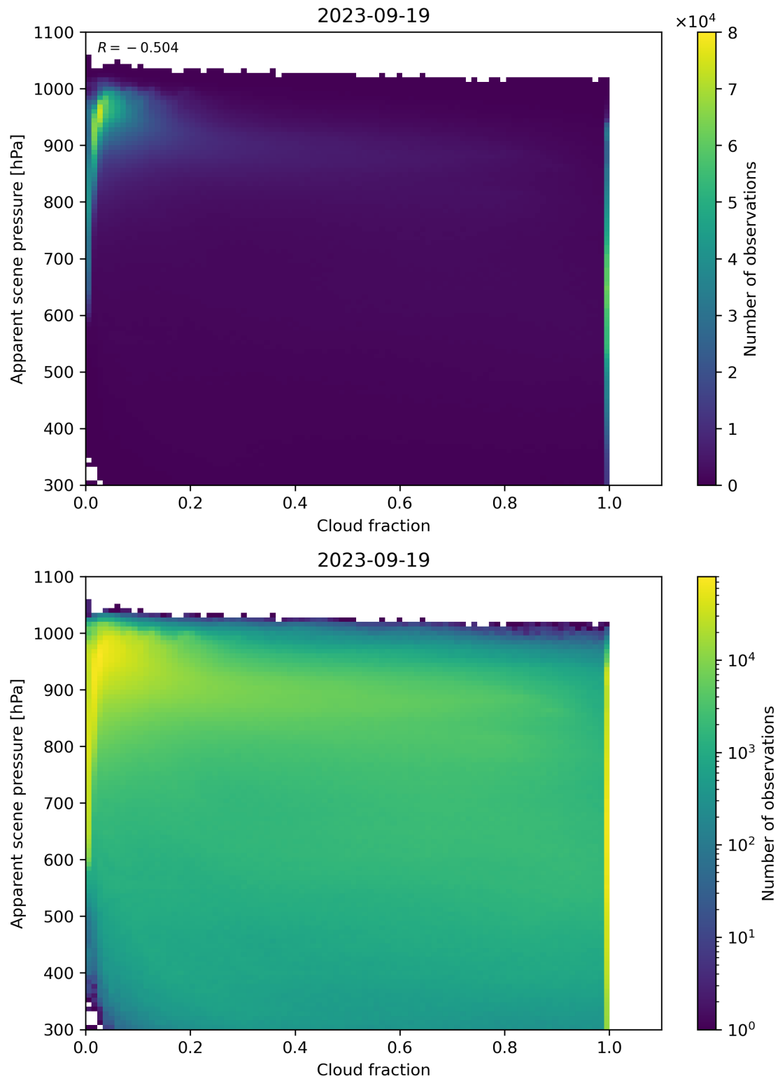
Figure 76: Scatter density plot of “Cloud fraction” against “Apparent scene pressure” for 2023-09-18 to 2023-09-20.
