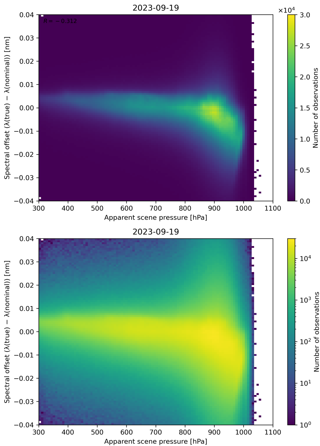
Figure 68: Scatter density plot of “Apparent scene pressure” against “Spectral offset ( \lambda(\text{true}) - \lambda(\text{nominal}) )” for 2023-09-18 to 2023-09-20.
