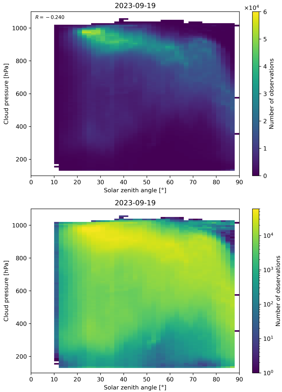
Figure 122: Scatter density plot of “Solar zenith angle” against “Cloud pressure” for 2023-09-18 to 2023-09-20.
