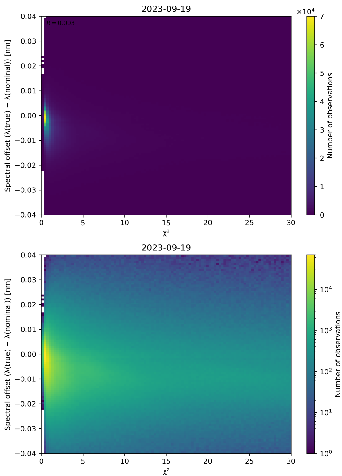
Figure 75: Scatter density plot of “ \chi^2 ” against “Spectral offset ( \lambda(\text{true}) - \lambda(\text{nominal}) )” for 2023-09-18 to 2023-09-20.
