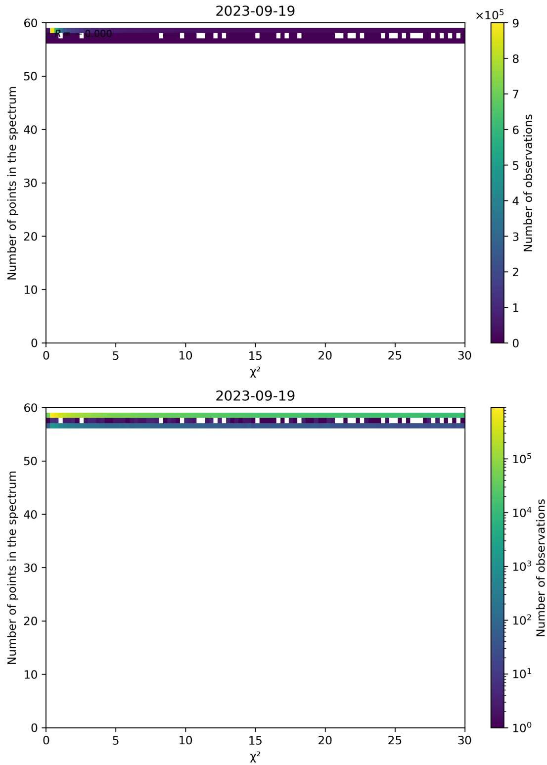
Figure 74: Scatter density plot of “ \chi^2 ” against “Number of points in the spectrum” for 2023-09-18 to 2023-09-20.
