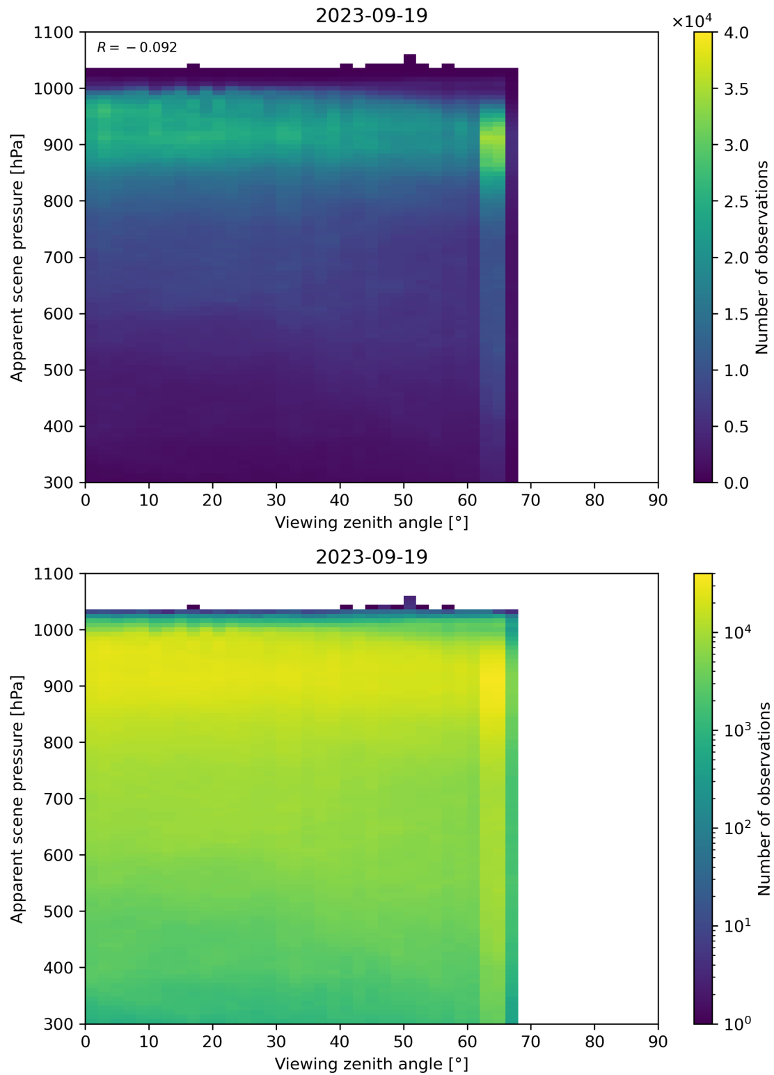
Figure 129: Scatter density plot of “Viewing zenith angle” against “Apparent scene pressure” for 2023-09-18 to 2023-09-20.
