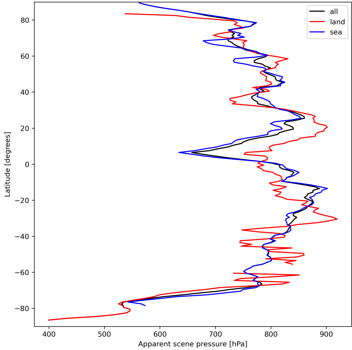
Figure 19: Zonal average of “Apparent scene pressure” for 2023-09-18 to 2023-09-20.
