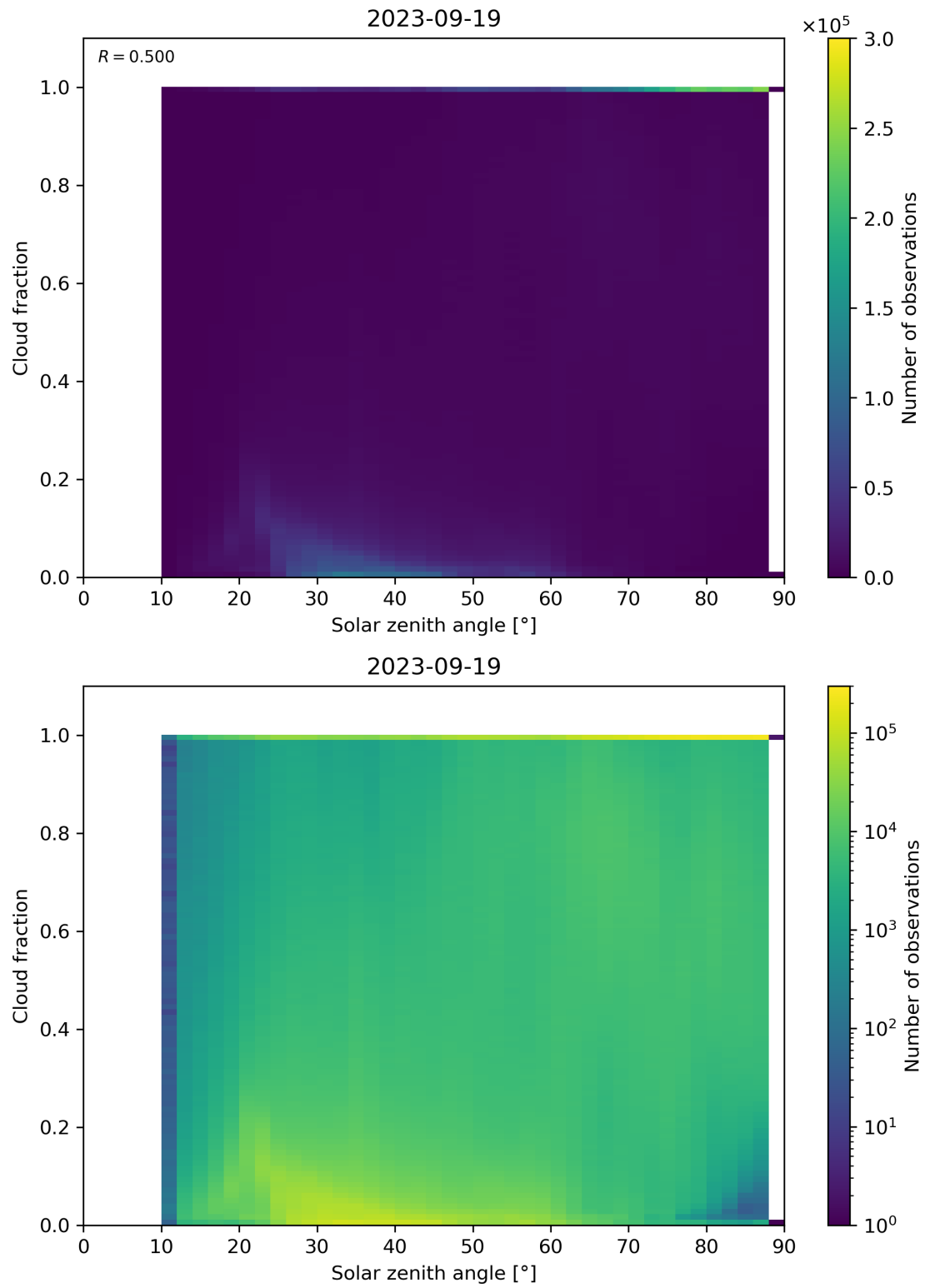
Figure 121: Scatter density plot of “Solar zenith angle” against “Cloud fraction” for 2023-09-18 to 2023-09-20.
