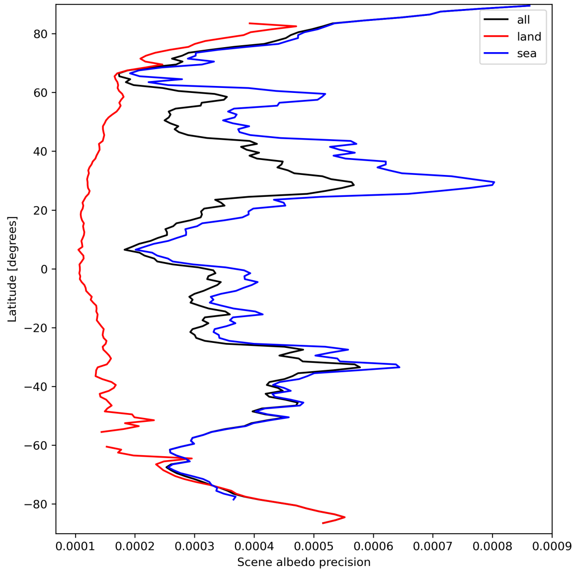
Figure 18: Zonal average of “Scene albedo precision” for 2023-09-18 to 2023-09-20.
