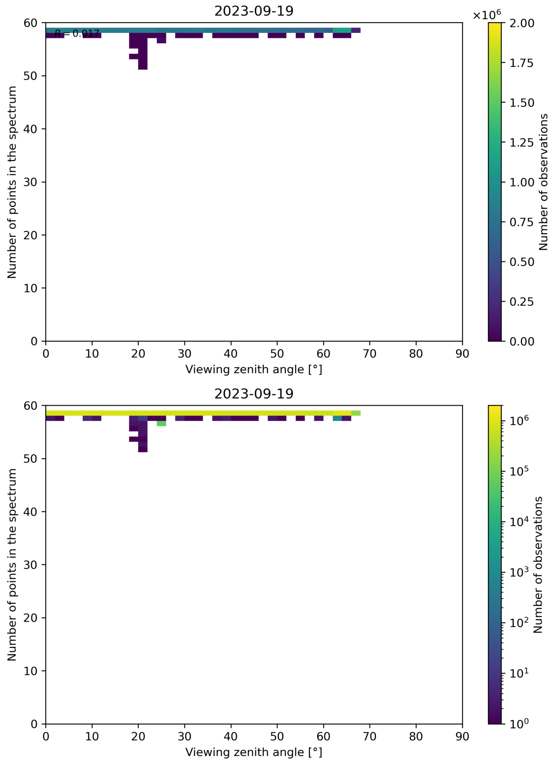
Figure 137: Scatter density plot of “Viewing zenith angle” against “Number of points in the spectrum” for 2023-09-18 to 2023-09-20.
