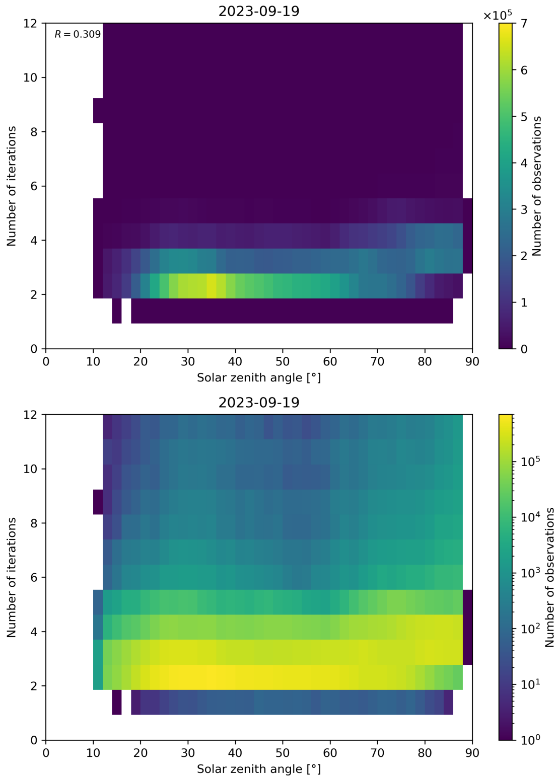
Figure 125: Scatter density plot of “Solar zenith angle” against “Number of iterations” for 2023-09-18 to 2023-09-20.
