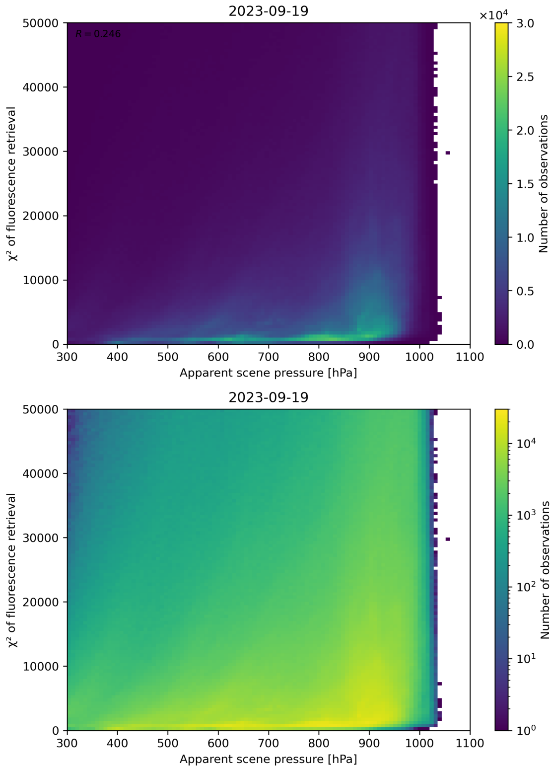
Figure 64: Scatter density plot of “Apparent scene pressure” against “ \chi^2 of fluorescence retrieval” for 2023-09-18 to 2023-09-20.
