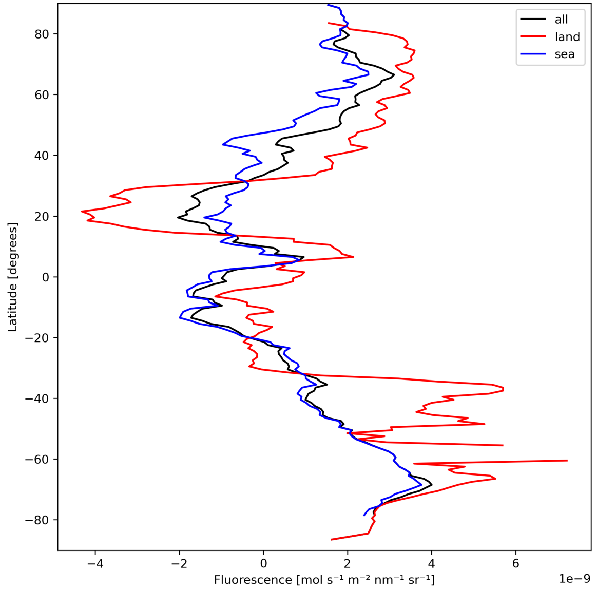
Figure 23: Zonal average of “Fluorescence” for 2023-09-18 to 2023-09-20.
