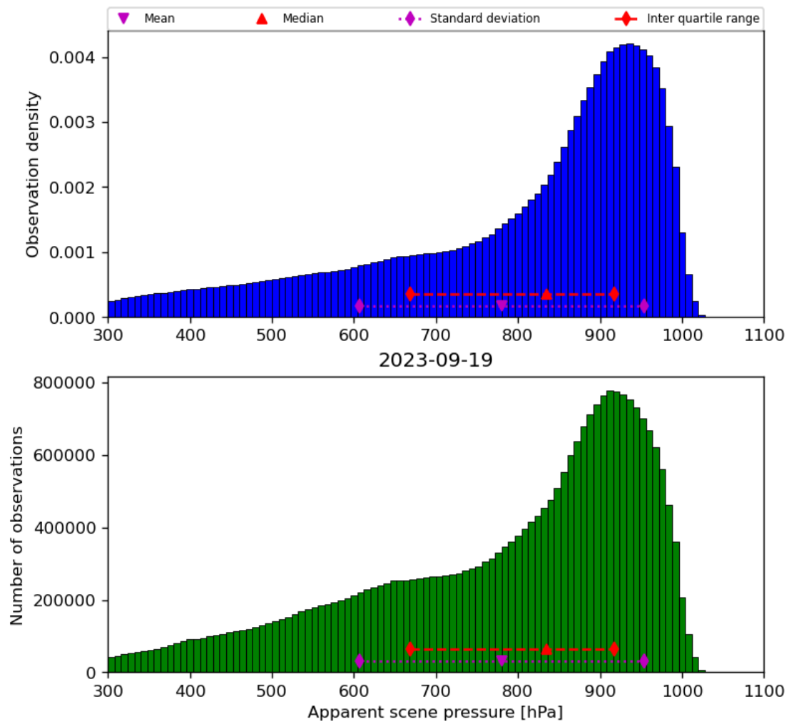
Figure 36: Histogram of “Apparent scene pressure” for 2023-09-18 to 2023-09-20
