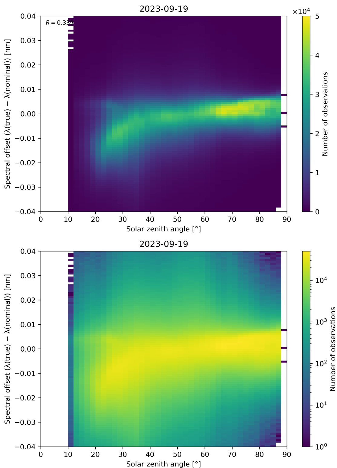
Figure 128: Scatter density plot of “Solar zenith angle” against “Spectral offset ( \lambda(\text{true}) - \lambda(\text{nominal}) )” for 2023-09-18 to 2023-09-20.
