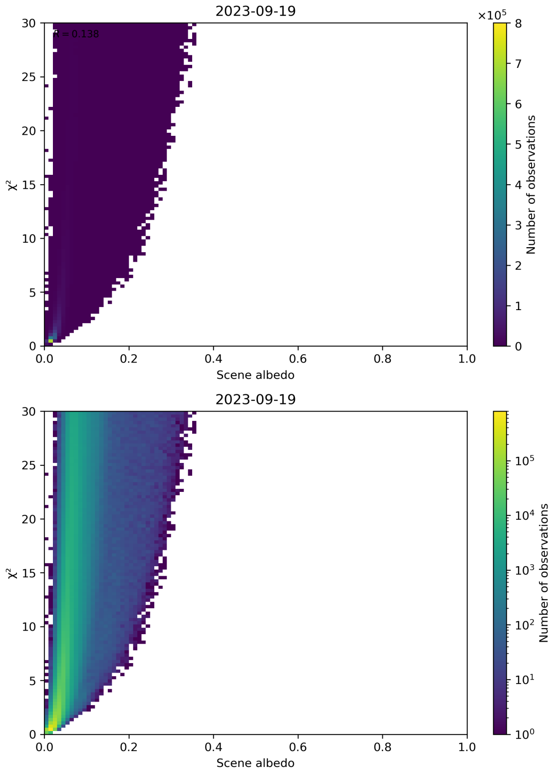
Figure 112: Scatter density plot of “Scene albedo” against “ \chi^2 ” for 2023-09-18 to 2023-09-20.
