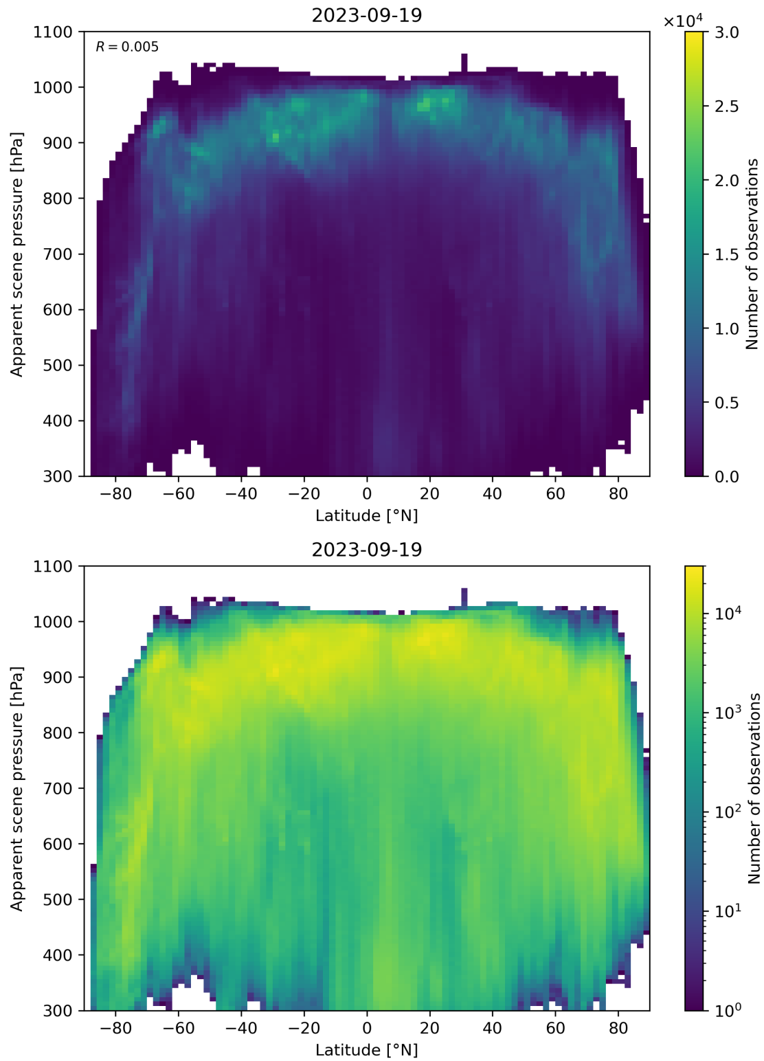
Figure 96: Scatter density plot of “Latitude” against “Apparent scene pressure” for 2023-09-18 to 2023-09-20.
