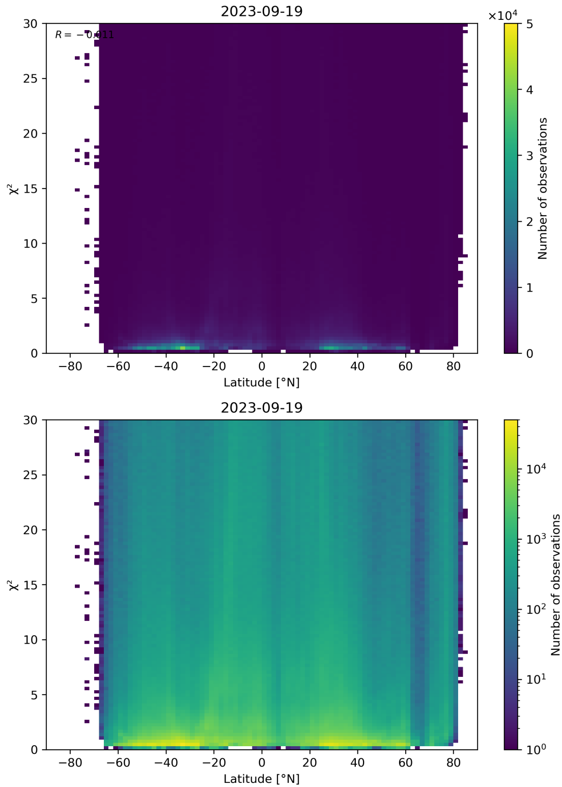
Figure 97: Scatter density plot of “Latitude” against “ \chi^2 ” for 2023-09-18 to 2023-09-20.
