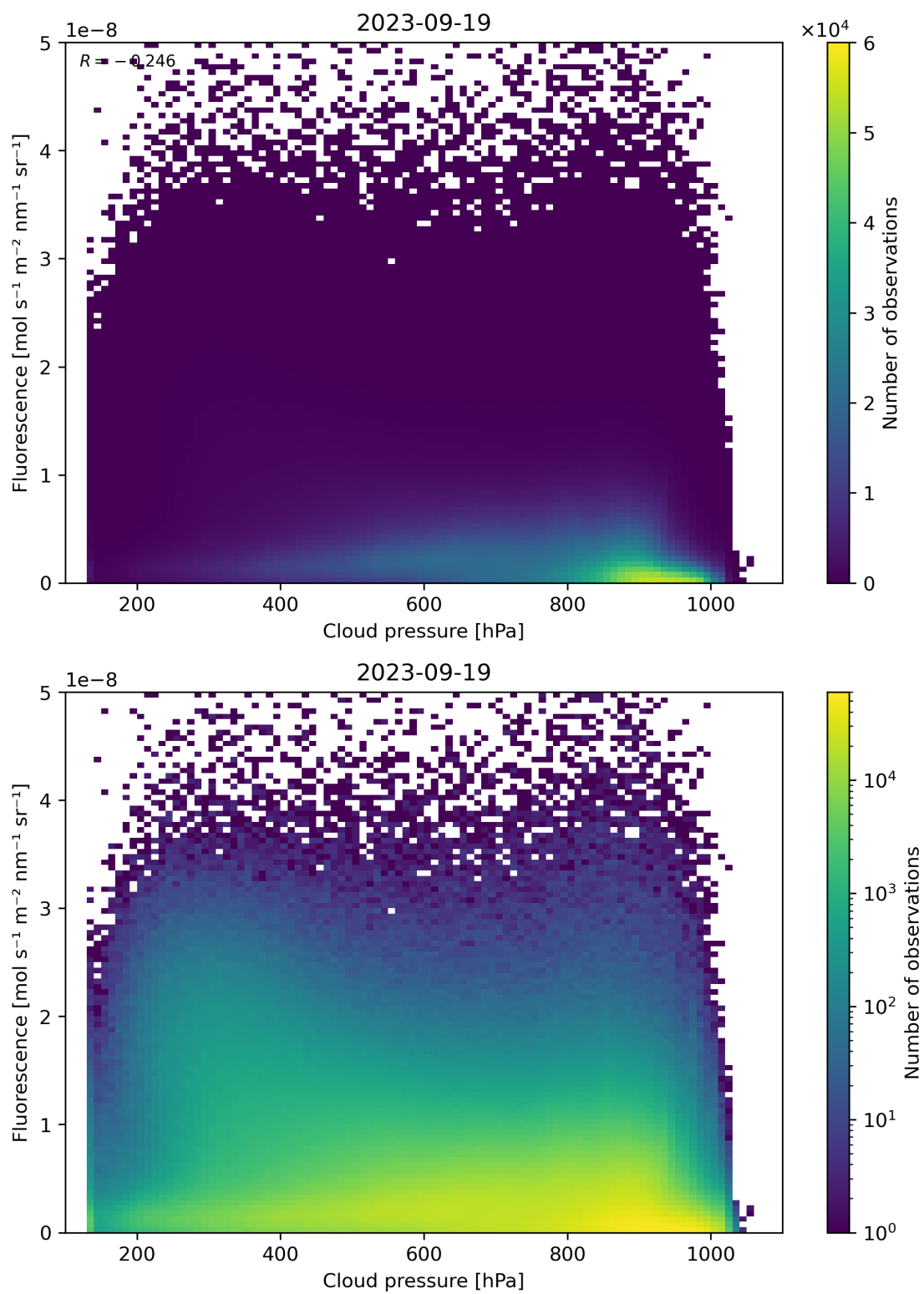
Figure 88: Scatter density plot of “Cloud pressure” against “Fluorescence” for 2023-09-18 to 2023-09-20.
