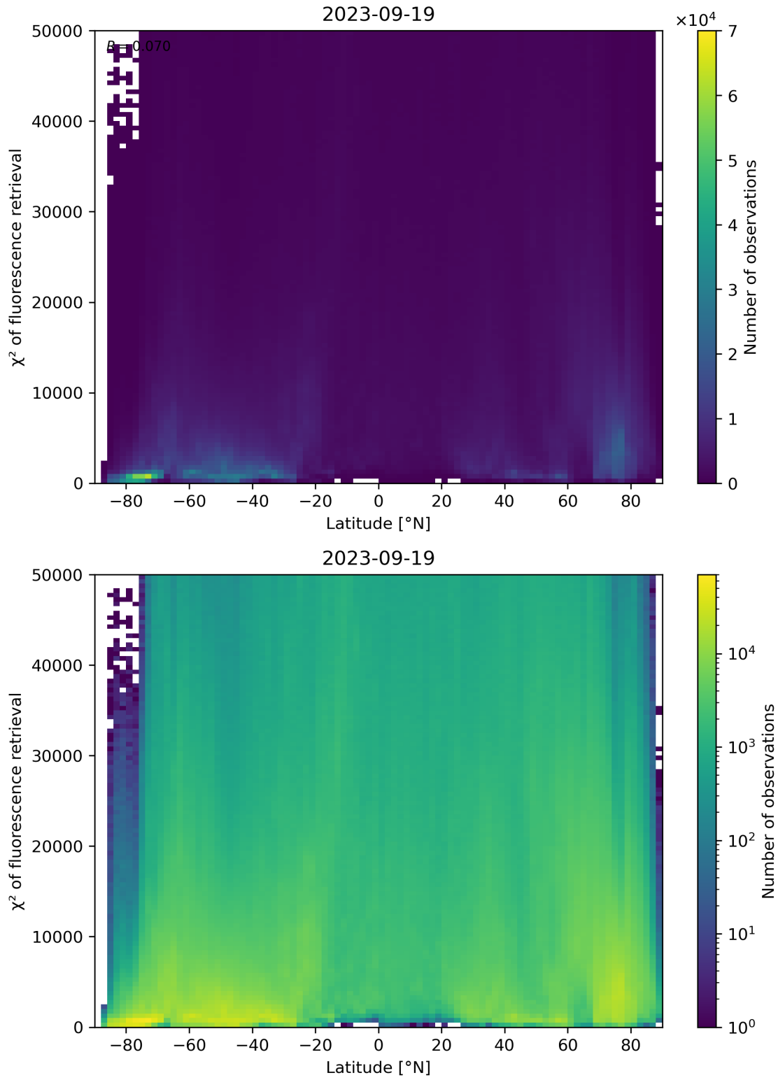
Figure 98: Scatter density plot of “Latitude” against “ \chi^2 of fluorescence retrieval” for 2023-09-18 to 2023-09-20.
