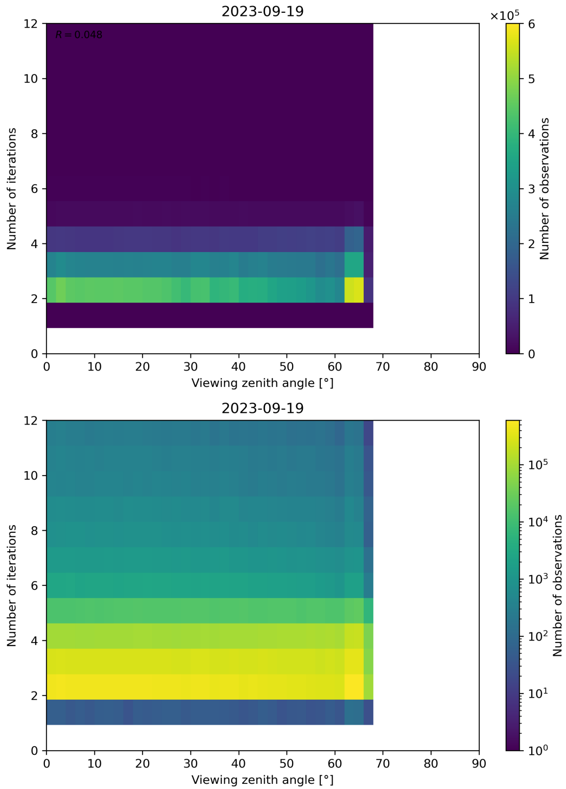
Figure 136: Scatter density plot of “Viewing zenith angle” against “Number of iterations” for 2023-09-18 to 2023-09-20.
