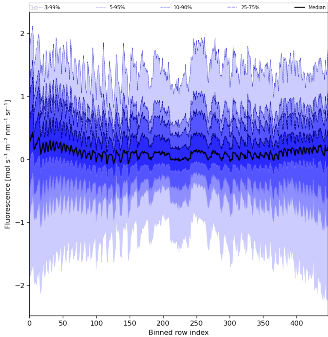
Figure 57: Along track statistics of “Fluorescence” for 2023-09-18 to 2023-09-20
