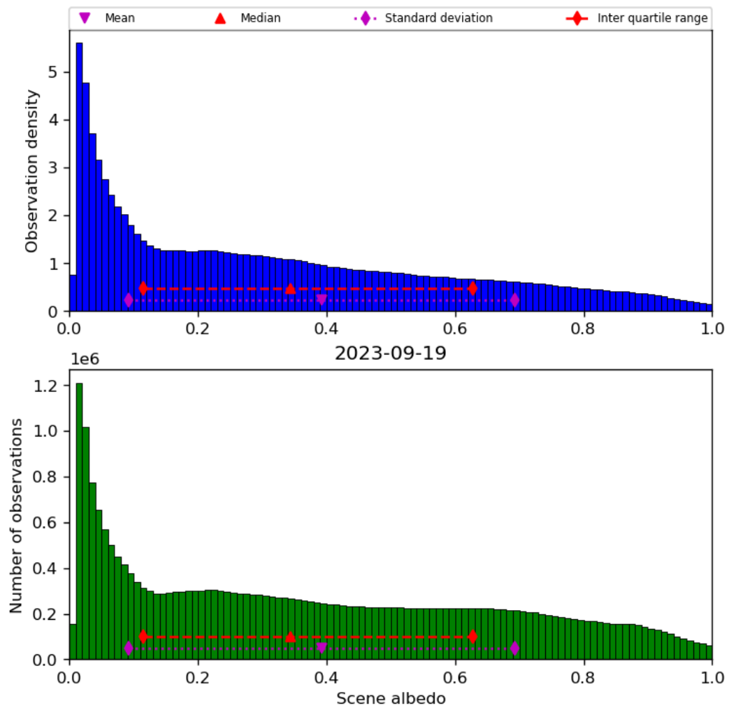
Figure 34: Histogram of “Scene albedo” for 2023-09-18 to 2023-09-20
