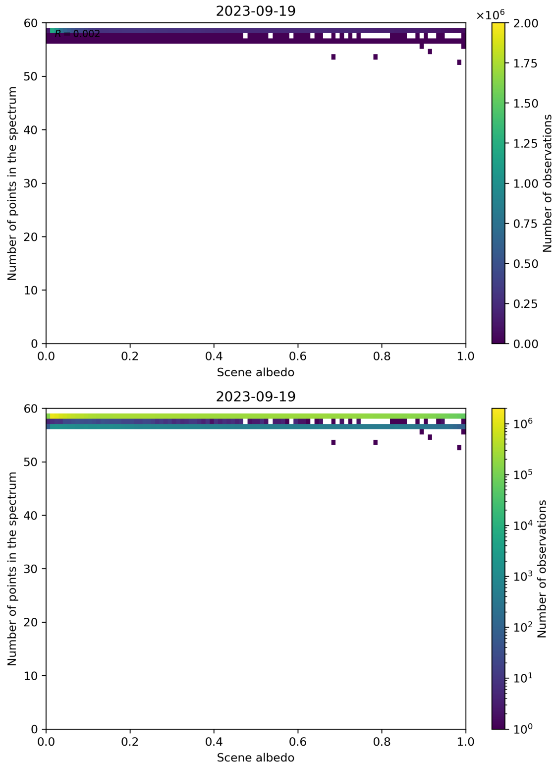
Figure 116: Scatter density plot of “Scene albedo” against “Number of points in the spectrum” for 2023-09-18 to 2023-09-20.
