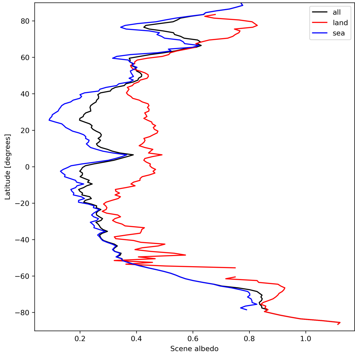
Figure 17: Zonal average of “Scene albedo” for 2023-09-18 to 2023-09-20.
