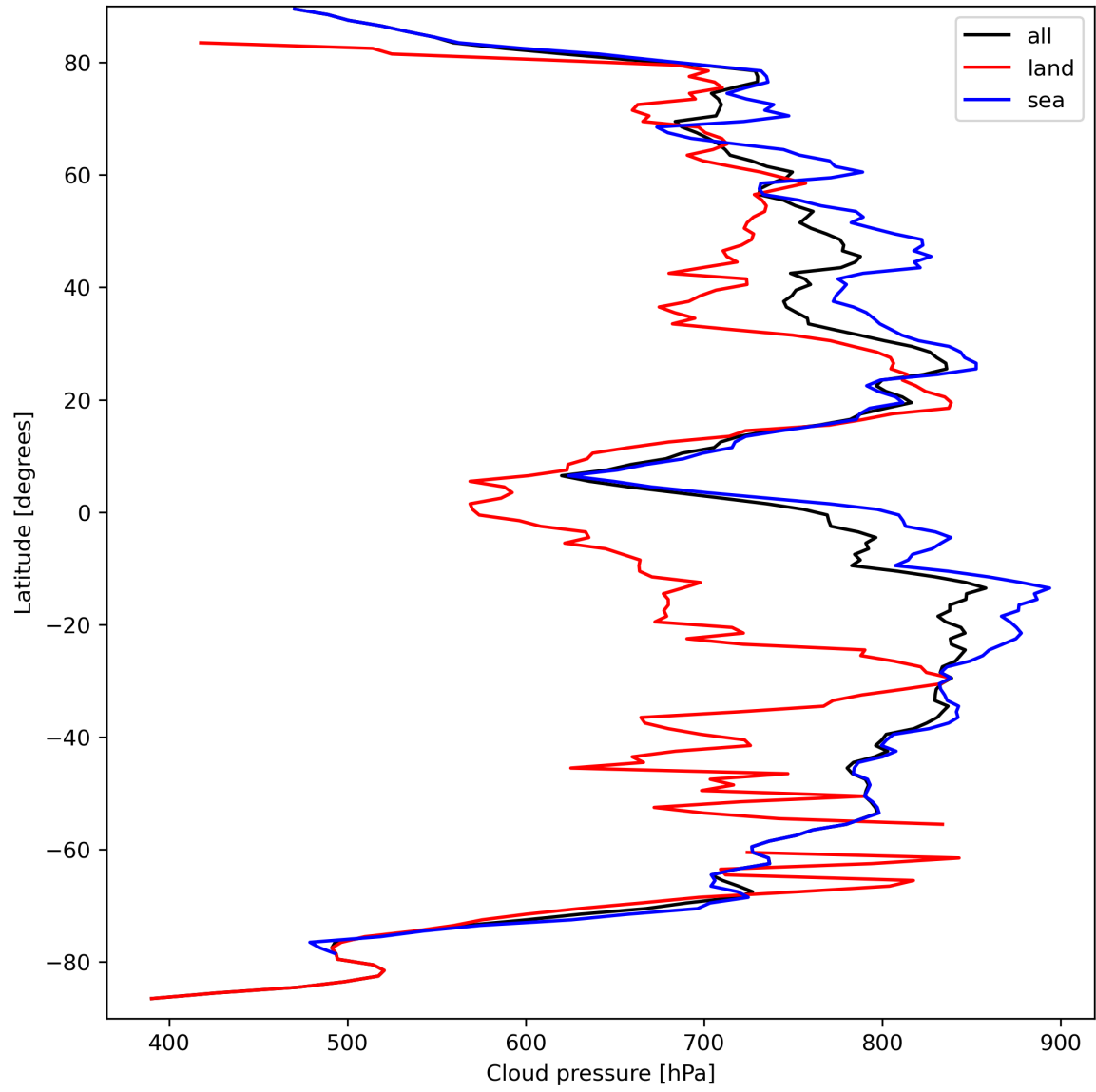
Figure 13: Zonal average of “Cloud pressure” for 2023-09-18 to 2023-09-20.
