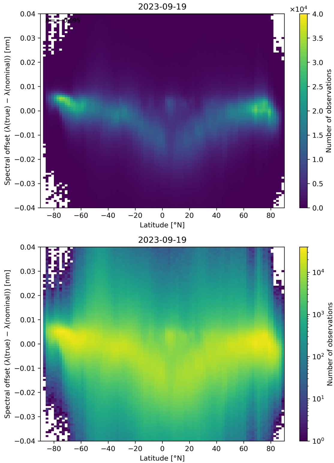
Figure 105: Scatter density plot of “Latitude” against “Spectral offset ( \lambda(\text{true}) - \lambda(\text{nominal}) )” for 2023-09-18 to 2023-09-20.
