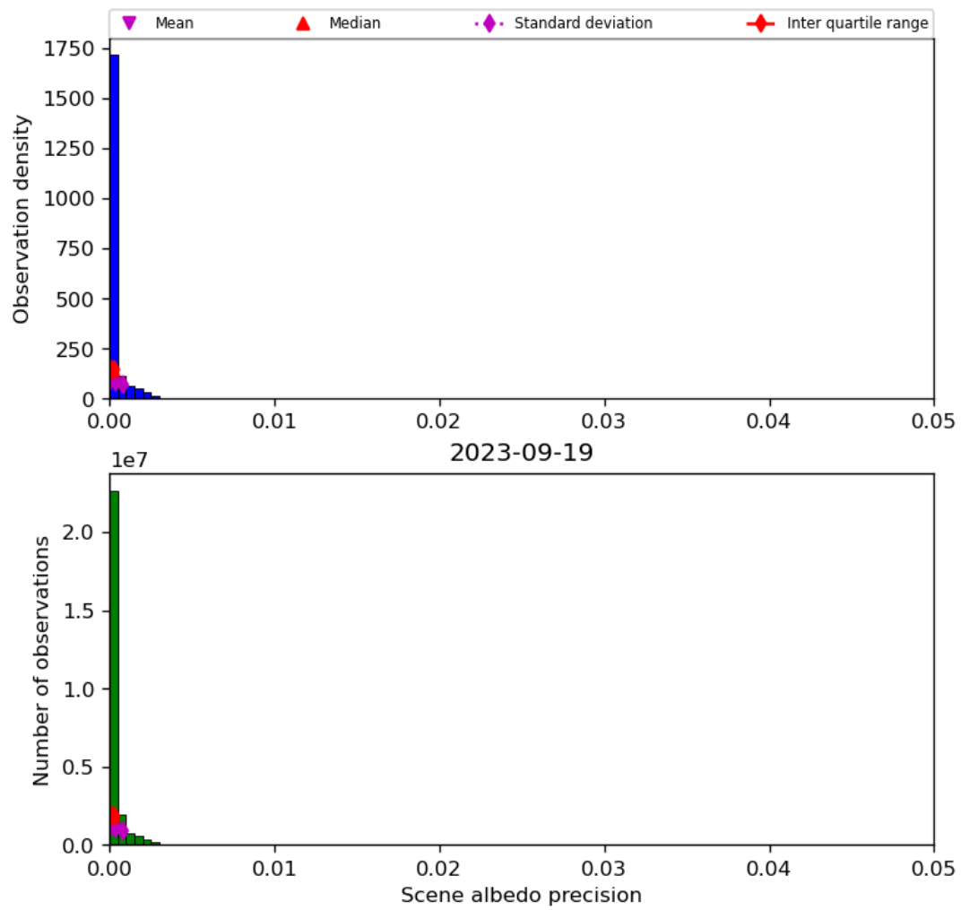
Figure 35: Histogram of “Scene albedo precision” for 2023-09-18 to 2023-09-20
