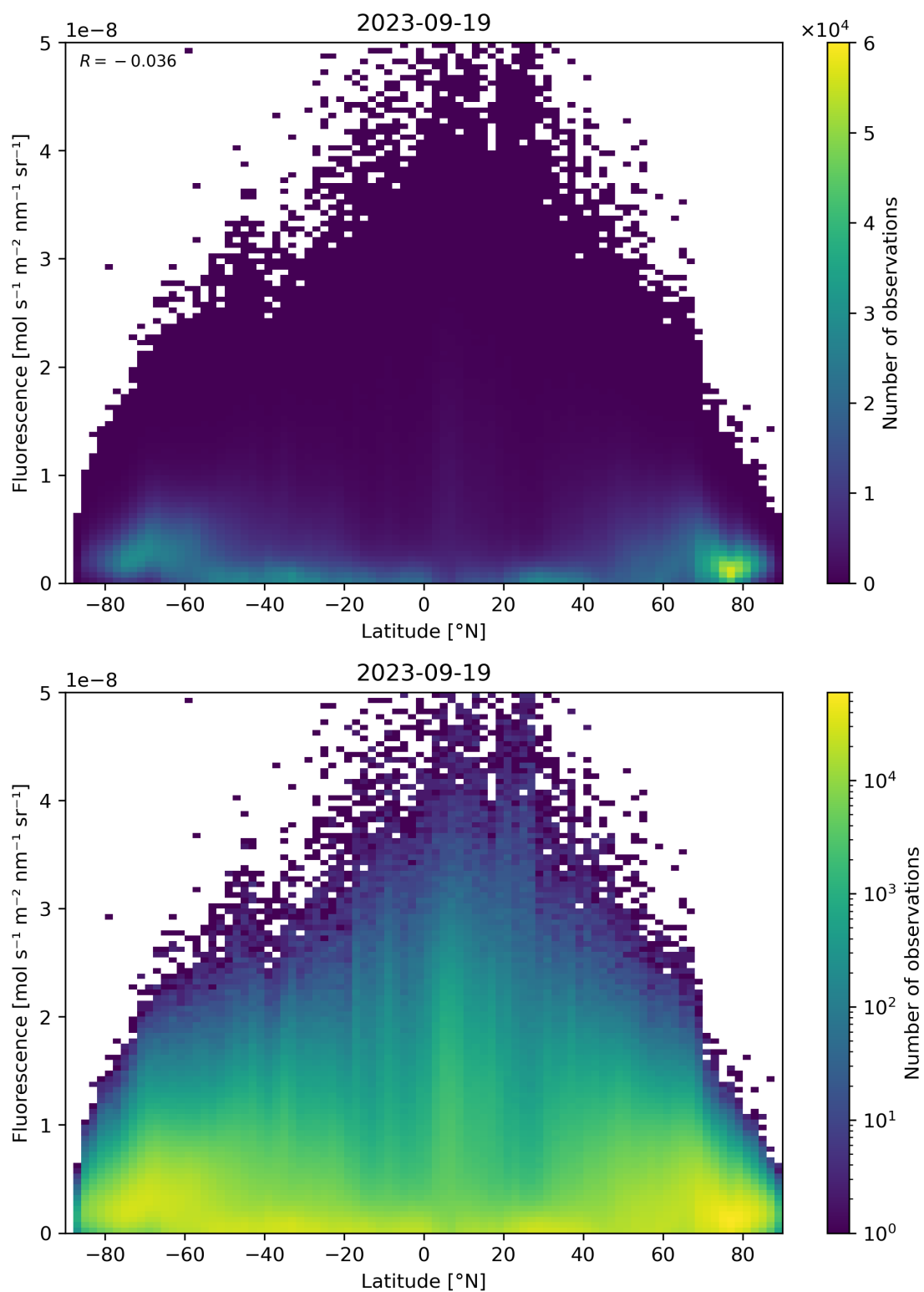
Figure 101: Scatter density plot of “Latitude” against “Fluorescence” for 2023-09-18 to 2023-09-20.
