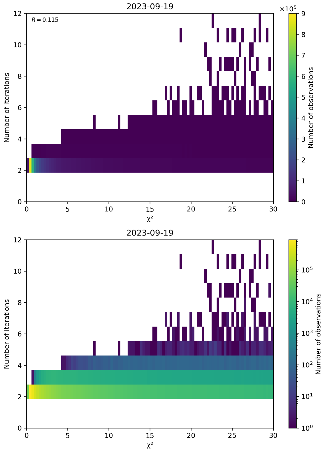
Figure 73: Scatter density plot of “ \chi^2 ” against “Number of iterations” for 2023-09-18 to 2023-09-20.
