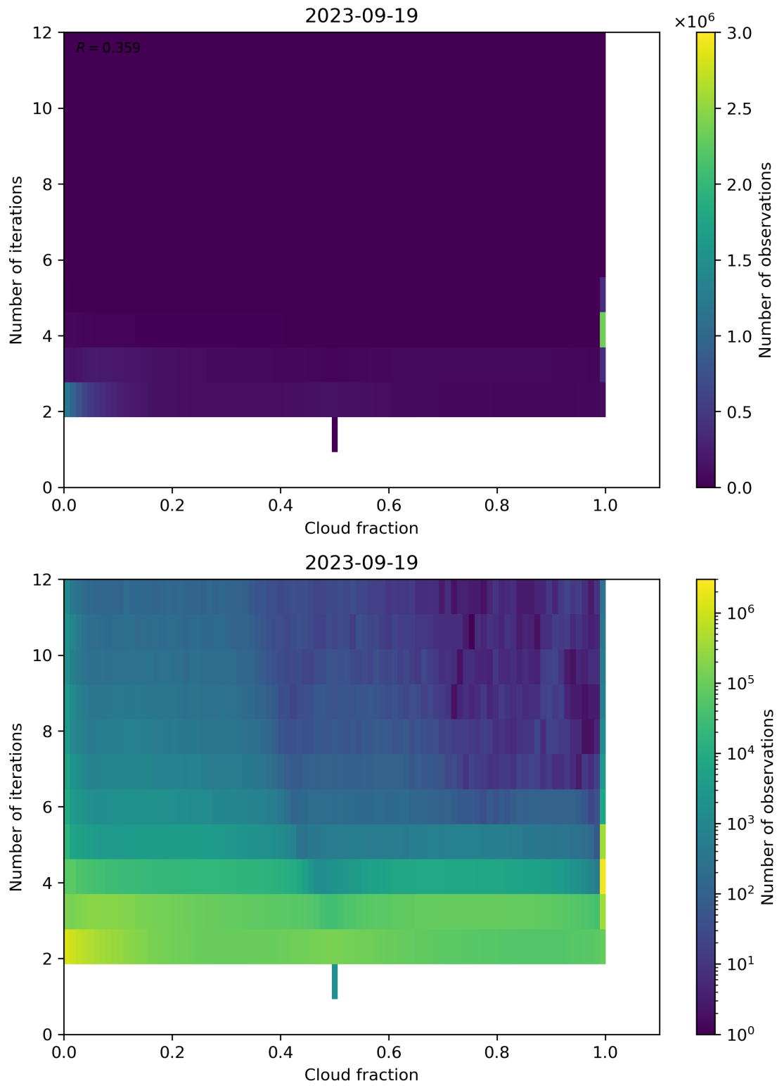
Figure 80: Scatter density plot of “Cloud fraction” against “Number of iterations” for 2023-09-18 to 2023-09-20.
