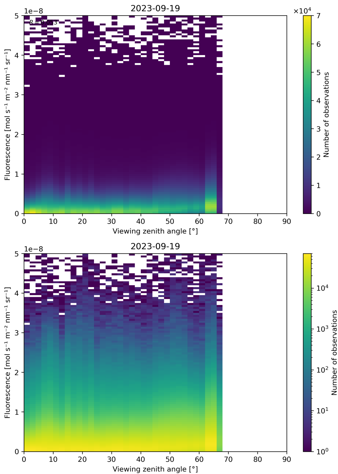
Figure 134: Scatter density plot of “Viewing zenith angle” against “Fluorescence” for 2023-09-18 to 2023-09-20.
