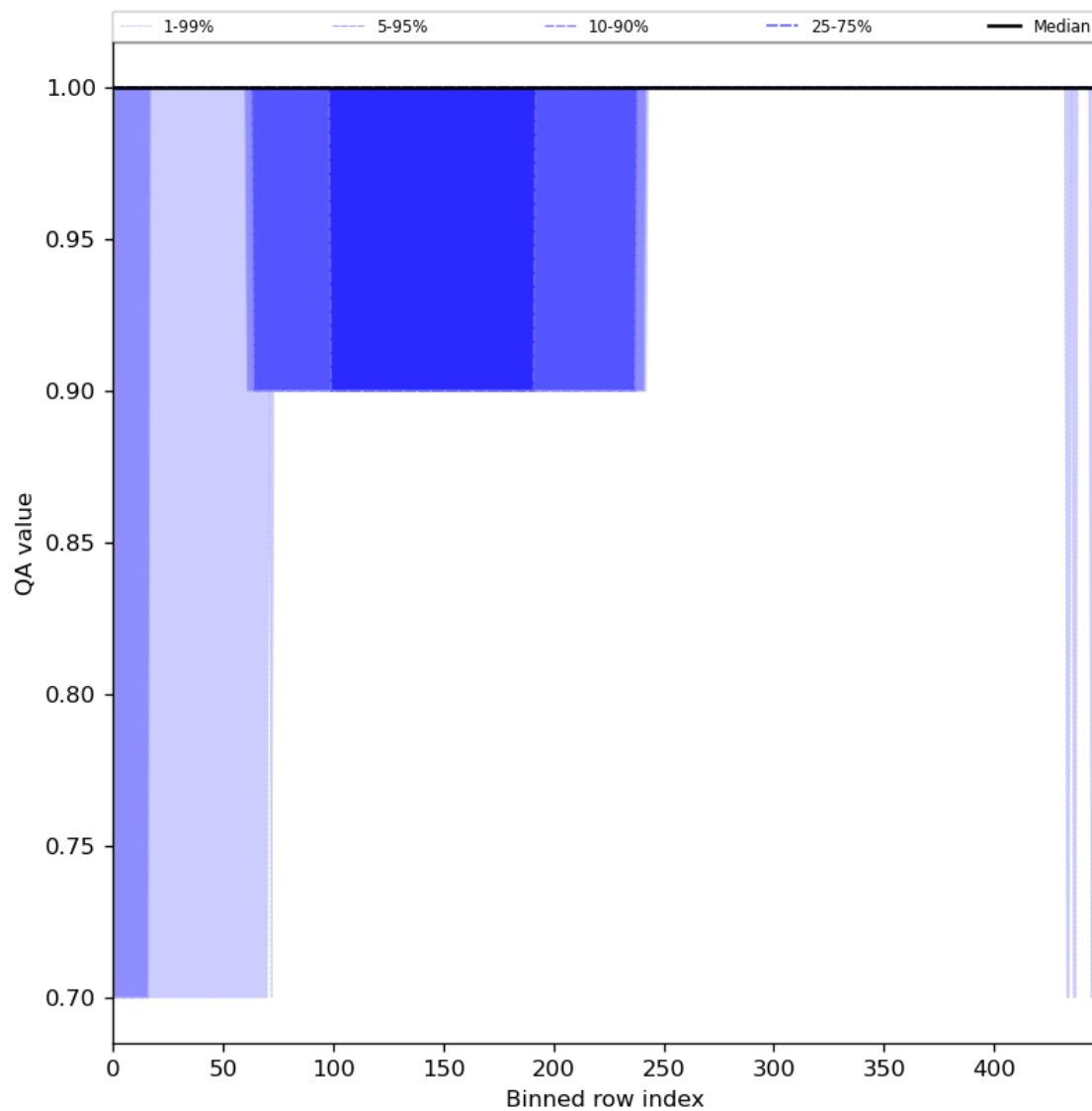
Figure 46: Along track statistics of “QA value” for 2023-09-18 to 2023-09-20
