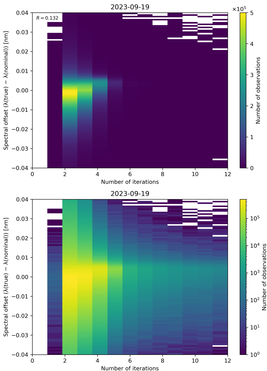
Figure 109: Scatter density plot of “Number of iterations” against “Spectral offset ( \lambda(\text{true}) - \lambda(\text{nominal}) )” for 2023-09-18 to 2023-09-20.
