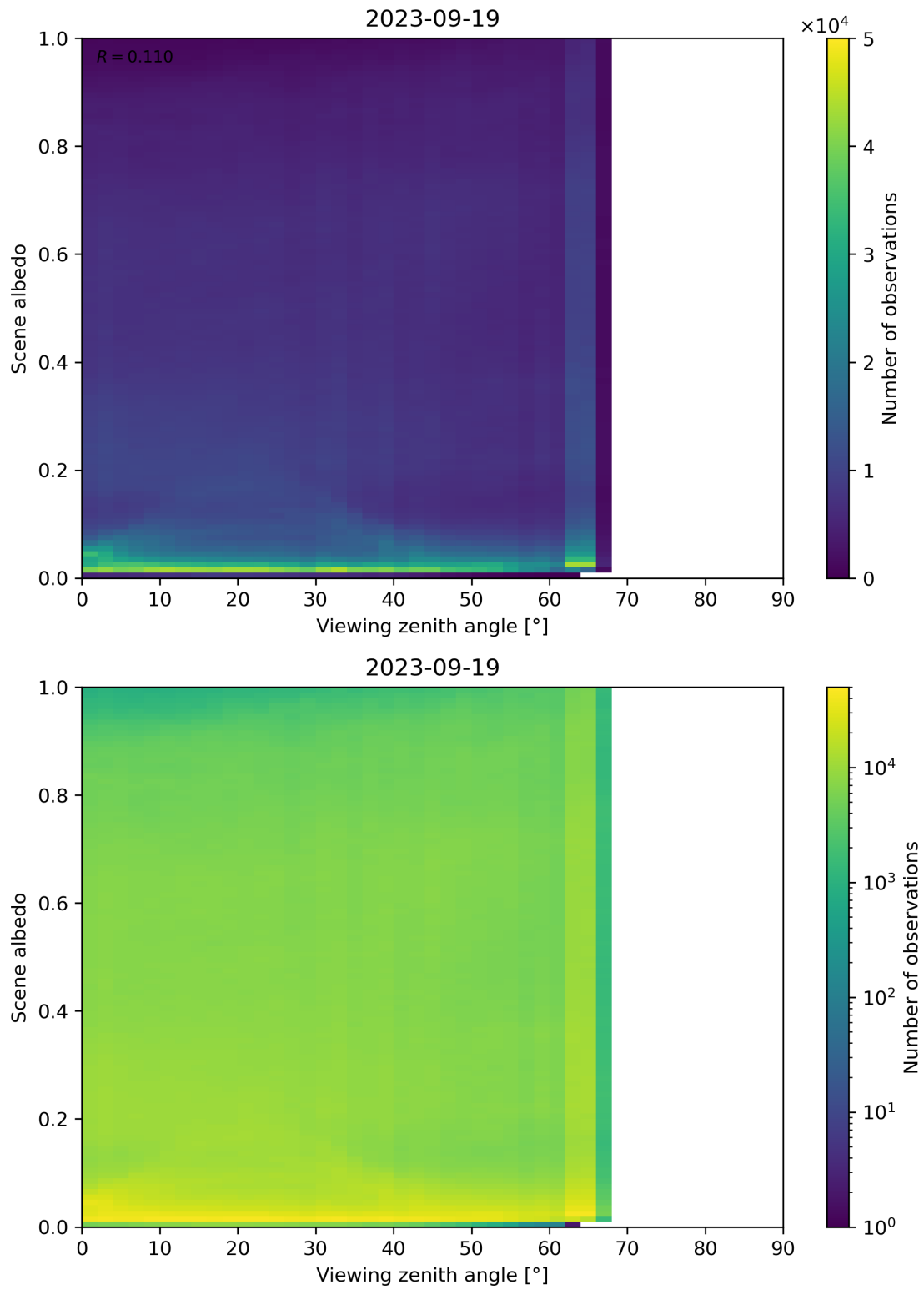
Figure 138: Scatter density plot of “Viewing zenith angle” against “Scene albedo” for 2023-09-18 to 2023-09-20.
