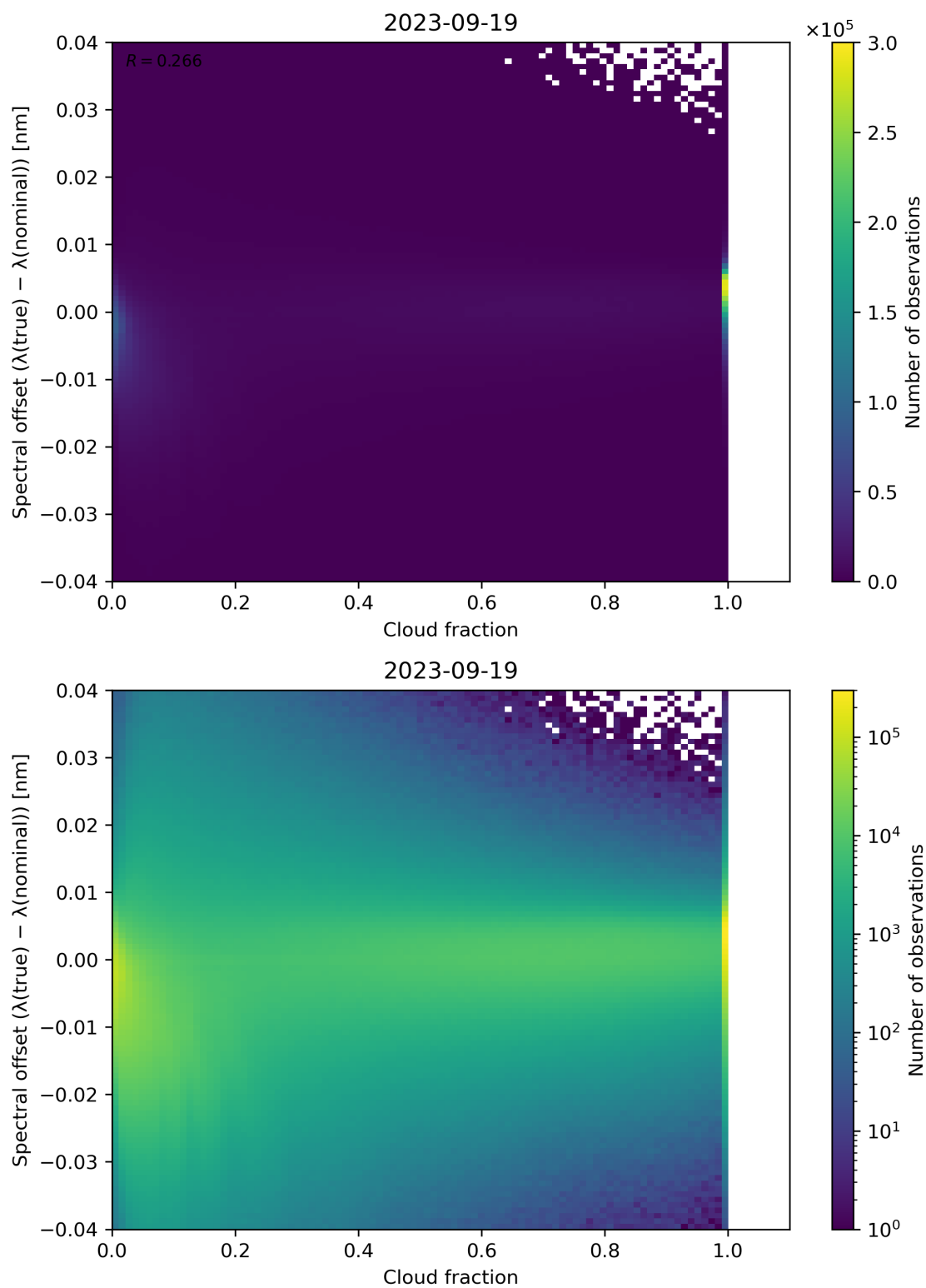
Figure 83: Scatter density plot of “Cloud fraction” against “Spectral offset ( \lambda(\text{true}) - \lambda(\text{nominal}) )” for 2023-09-18 to 2023-09-20.
