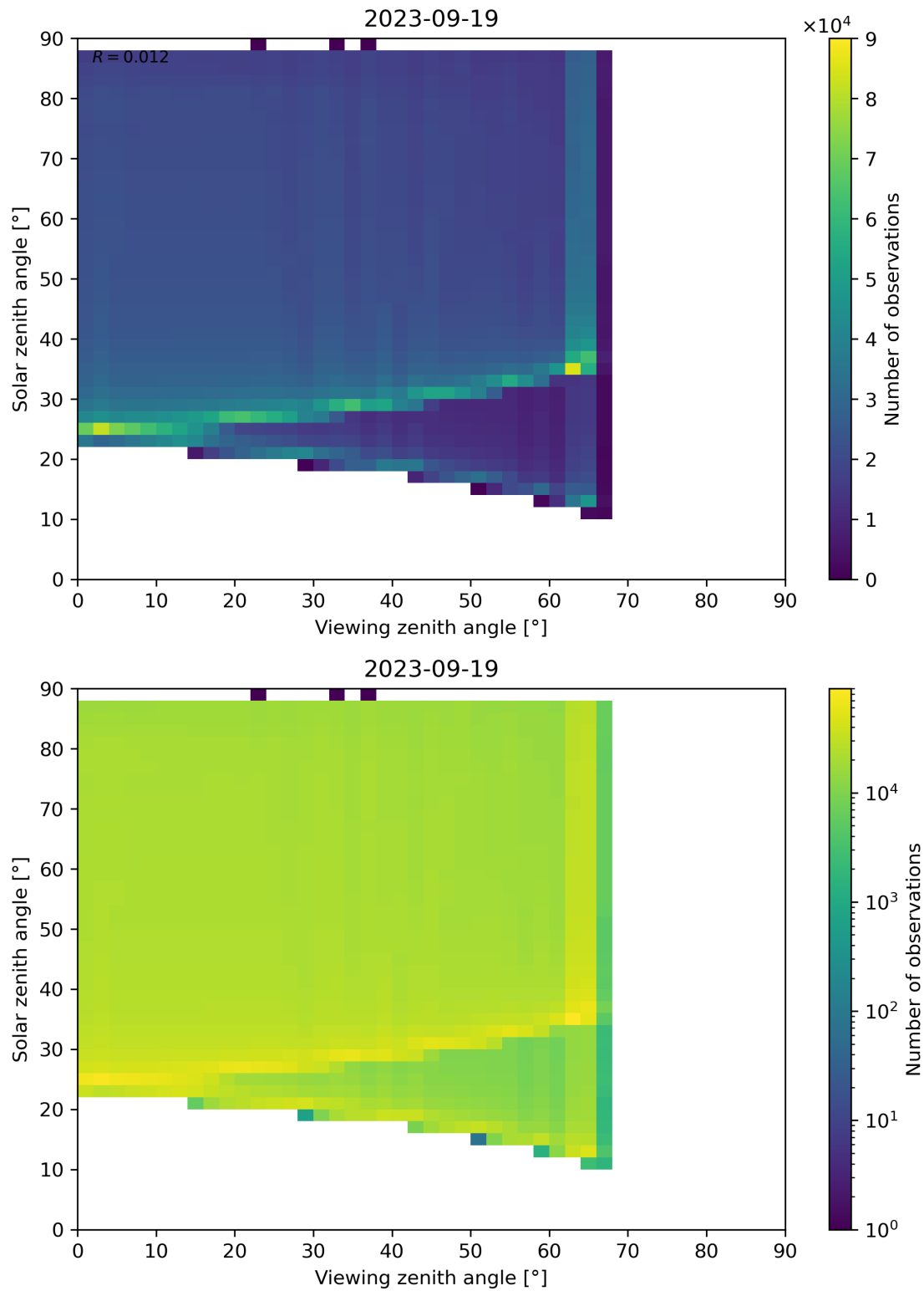
Figure 139: Scatter density plot of “Viewing zenith angle” against “Solar zenith angle” for 2023-09-18 to 2023-09-20.
