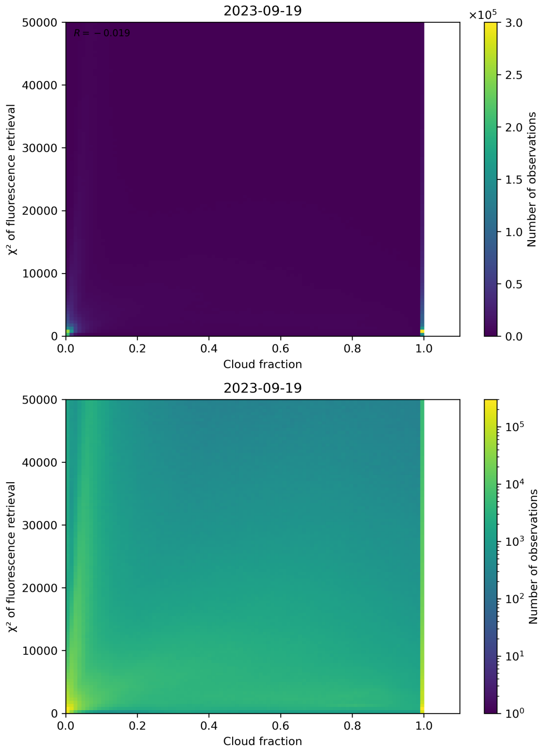
Figure 78: Scatter density plot of “Cloud fraction” against “ \chi^2 of fluorescence retrieval” for 2023-09-18 to 2023-09-20.
