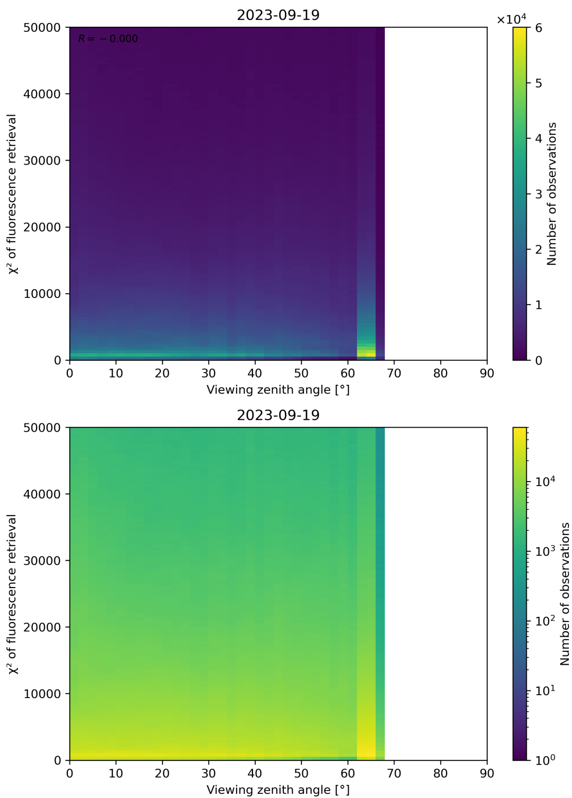
Figure 131: Scatter density plot of “Viewing zenith angle” against “ \chi^2 of fluorescence retrieval” for 2023-09-18 to 2023-09-20.
