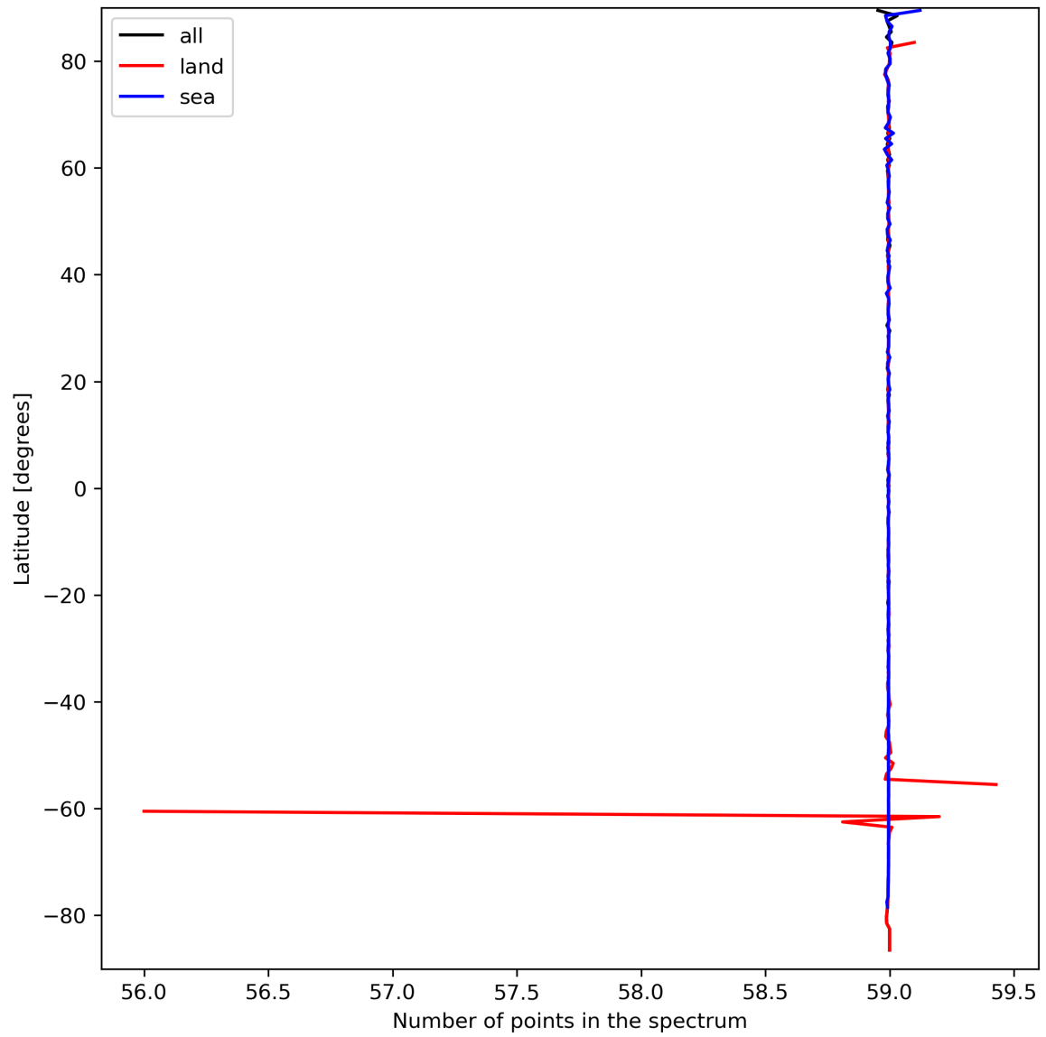
Figure 27: Zonal average of “Number of points in the spectrum” for 2023-09-18 to 2023-09-20.
