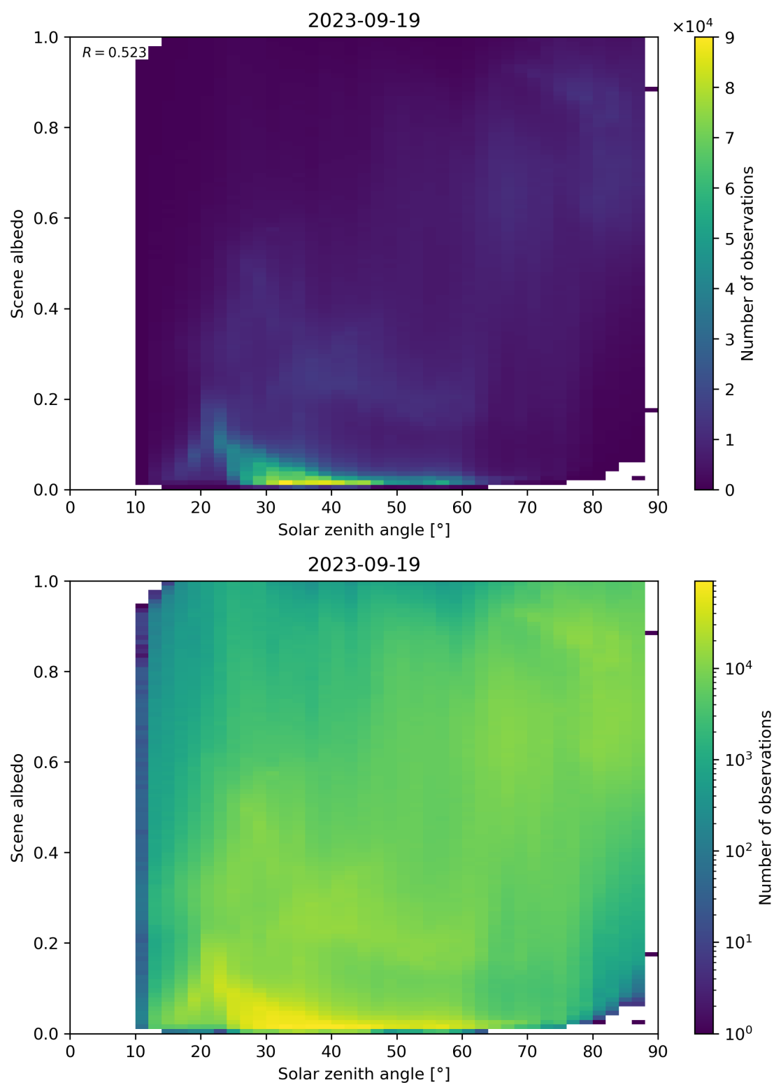
Figure 127: Scatter density plot of “Solar zenith angle” against “Scene albedo” for 2023-09-18 to 2023-09-20.
