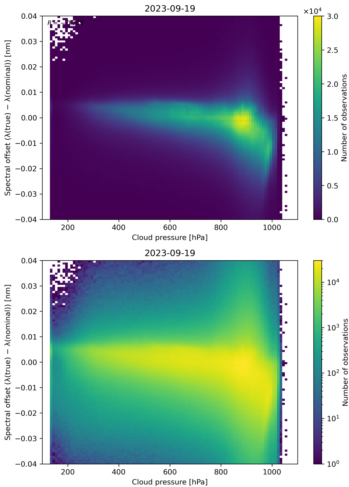
Figure 92: Scatter density plot of “Cloud pressure” against “Spectral offset ( \lambda(\text{true}) - \lambda(\text{nominal}) )” for 2023-09-18 to 2023-09-20.
