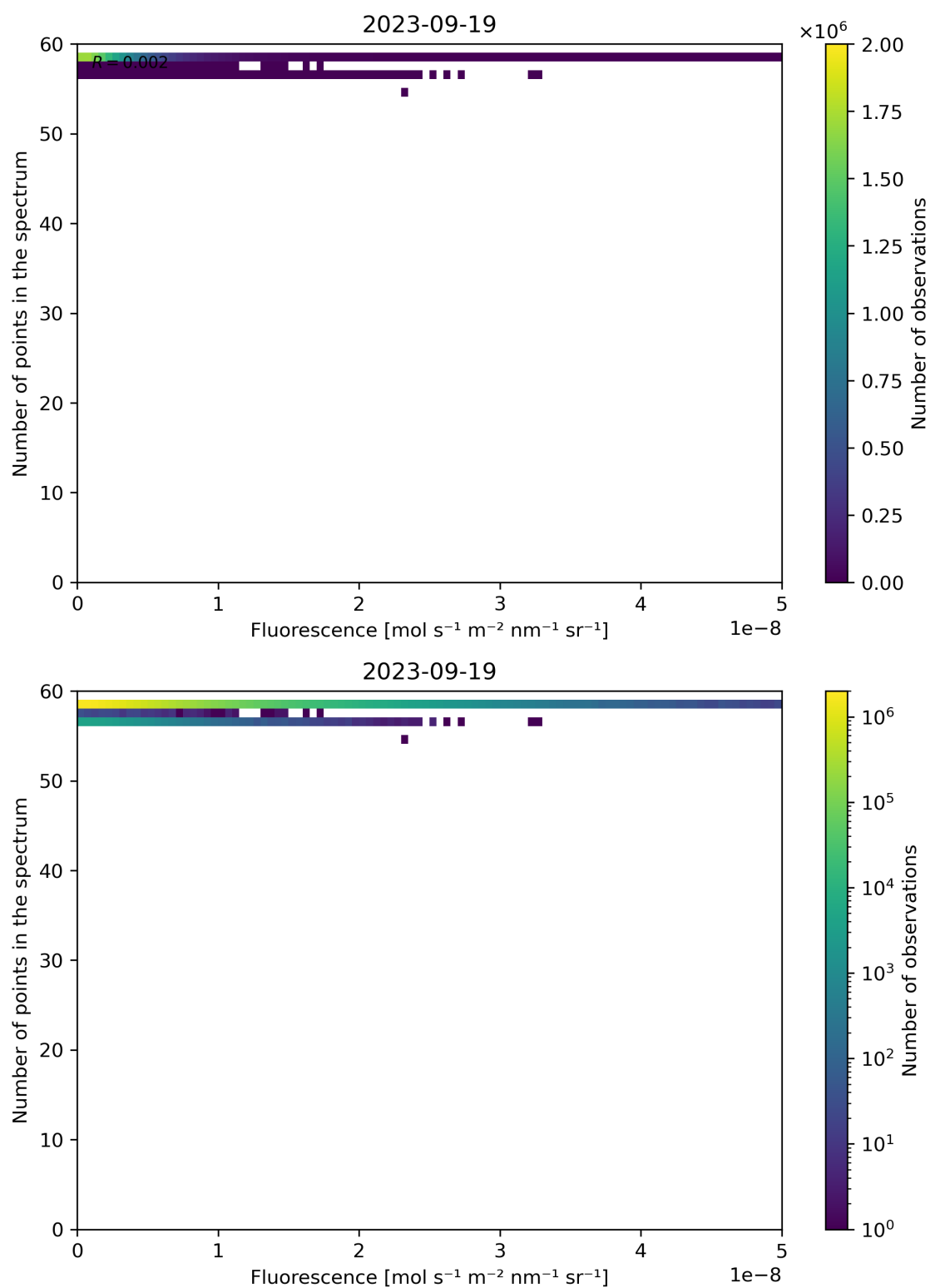
Figure 94: Scatter density plot of “Fluorescence” against “Number of points in the spectrum” for 2023-09-18 to 2023-09-20.
