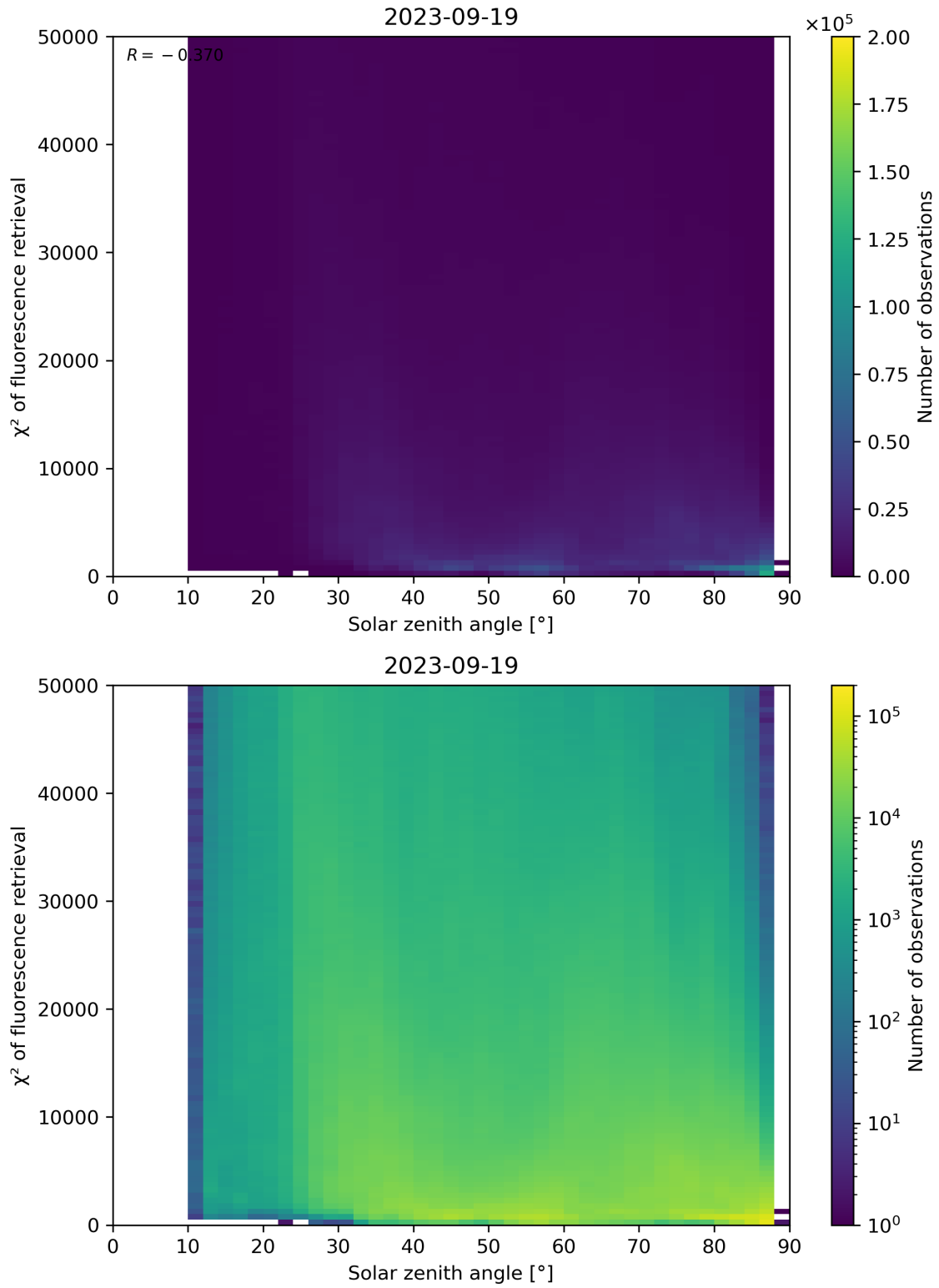
Figure 120: Scatter density plot of “Solar zenith angle” against “ \chi^2 of fluorescence retrieval” for 2023-09-18 to 2023-09-20.
