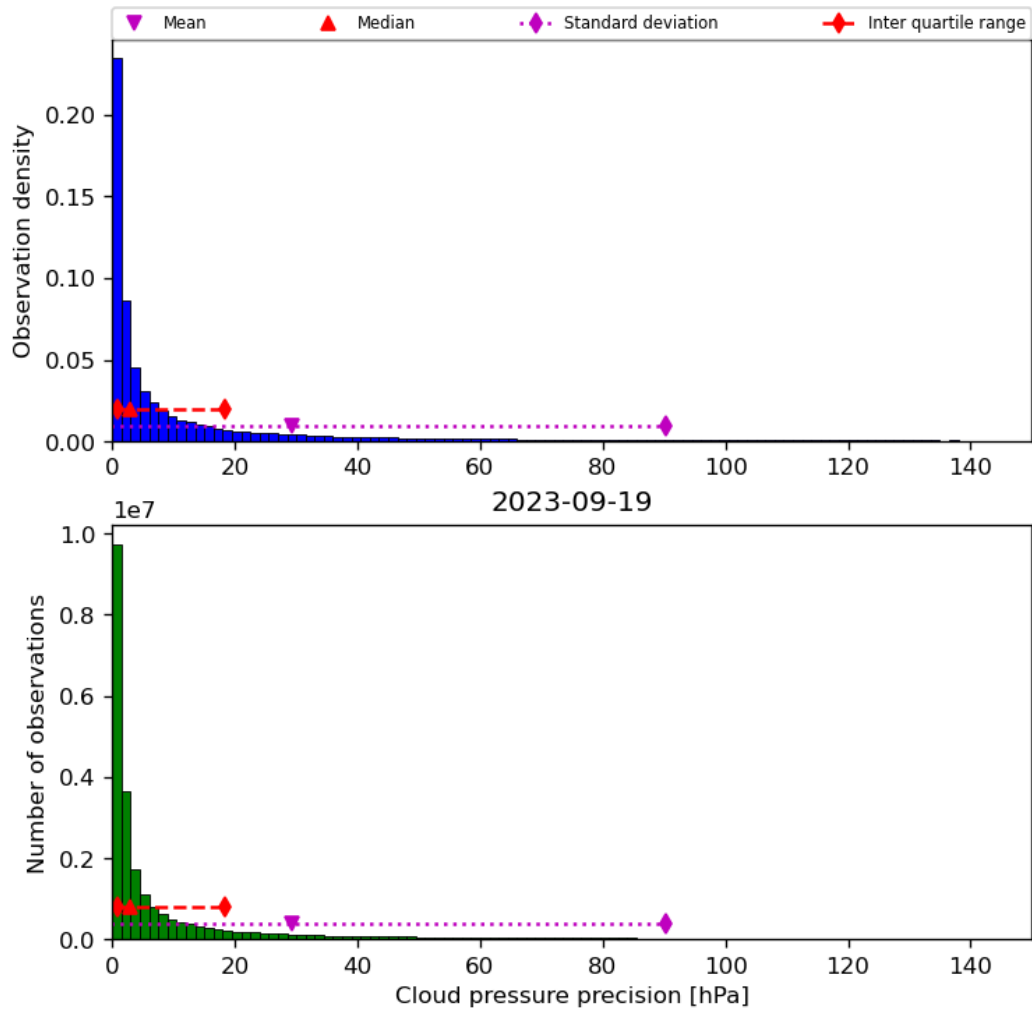
Figure 31: Histogram of “Cloud pressure precision” for 2023-09-18 to 2023-09-20
