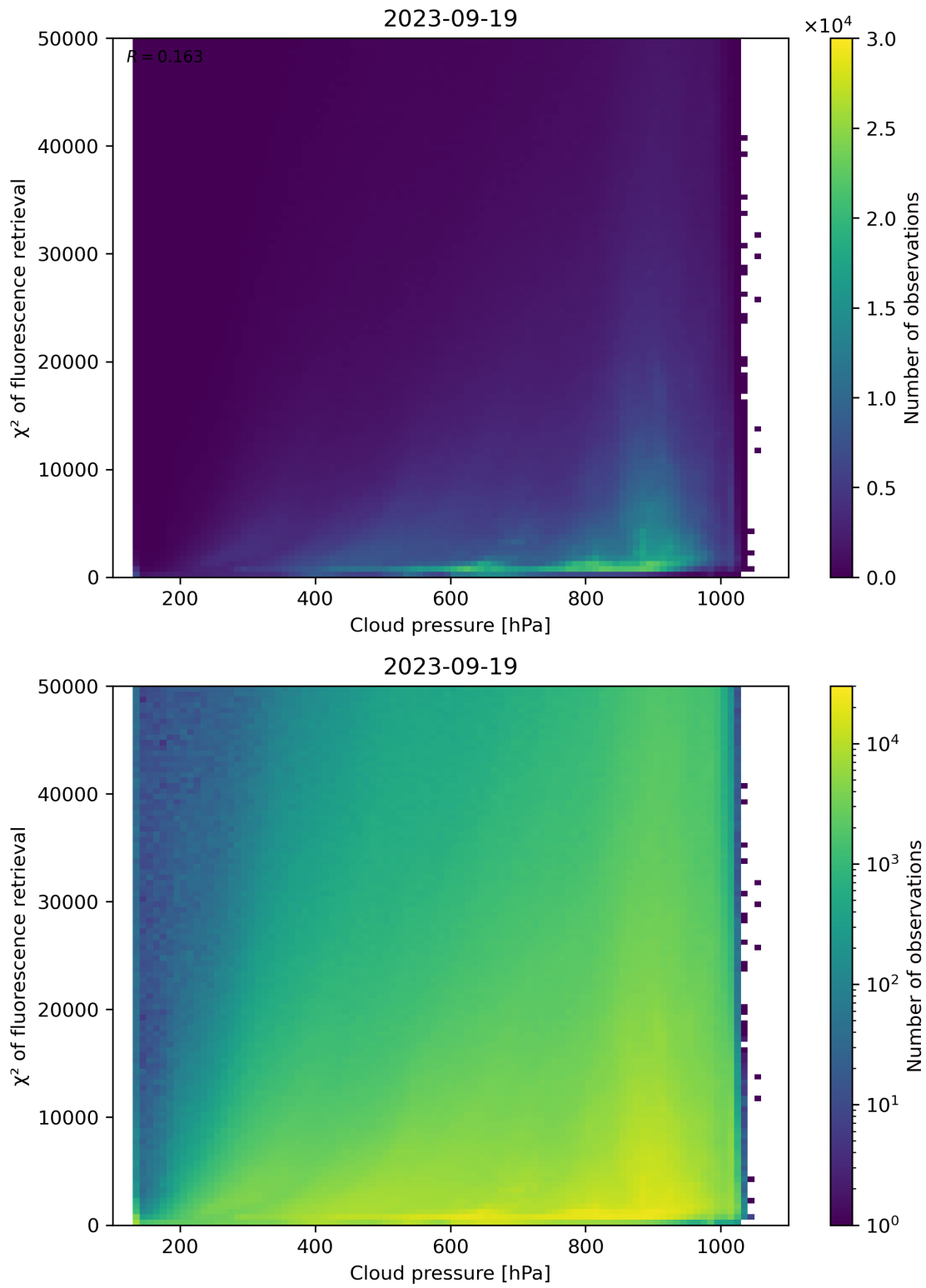
Figure 86: Scatter density plot of “Cloud pressure” against “ \chi^2 of fluorescence retrieval” for 2023-09-18 to 2023-09-20.
