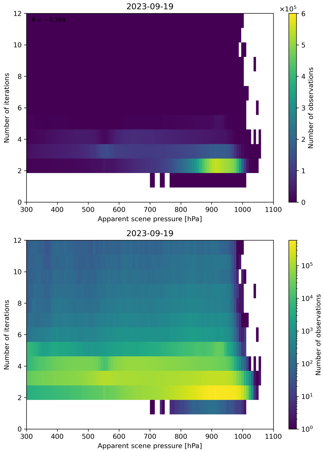
Figure 66: Scatter density plot of “Apparent scene pressure” against “Number of iterations” for 2023-09-18 to 2023-09-20.
