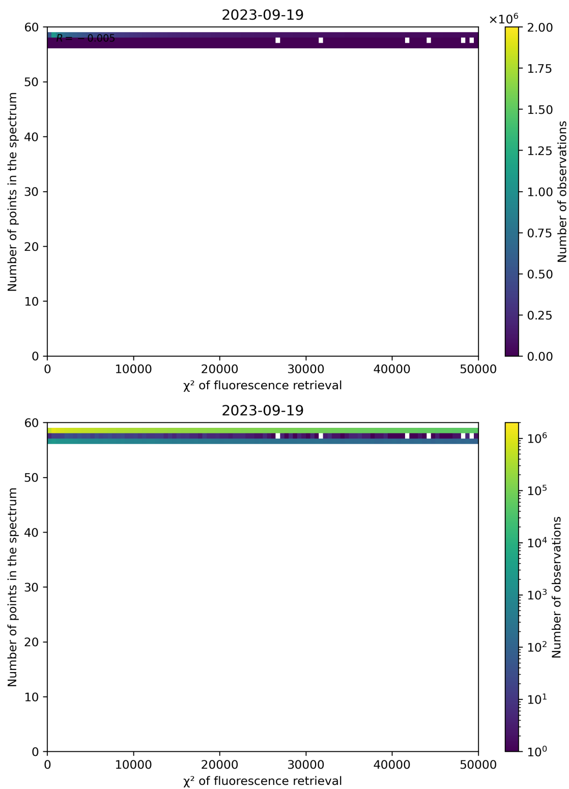
Figure 71: Scatter density plot of " \chi^2 of fluorescence retrieval" against "Number of points in the spectrum" for 2023-09-18 to 2023-09-20.
