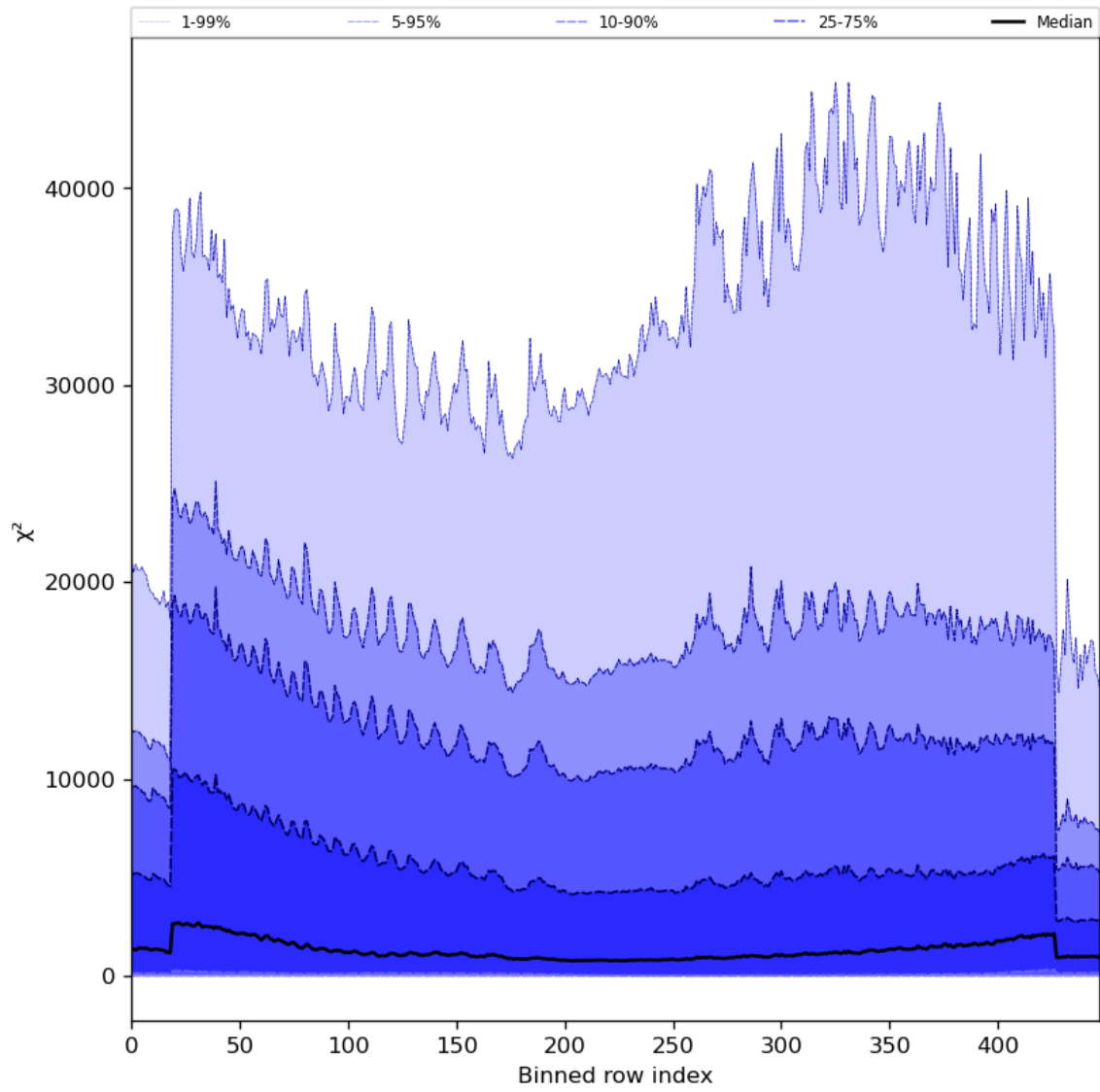
Figure 55: Along track statistics of “ \chi^2 ” for 2023-09-18 to 2023-09-20
