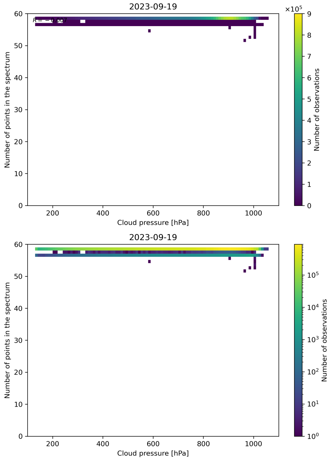
Figure 90: Scatter density plot of “Cloud pressure” against “Number of points in the spectrum” for 2023-09-18 to 2023-09-20.
