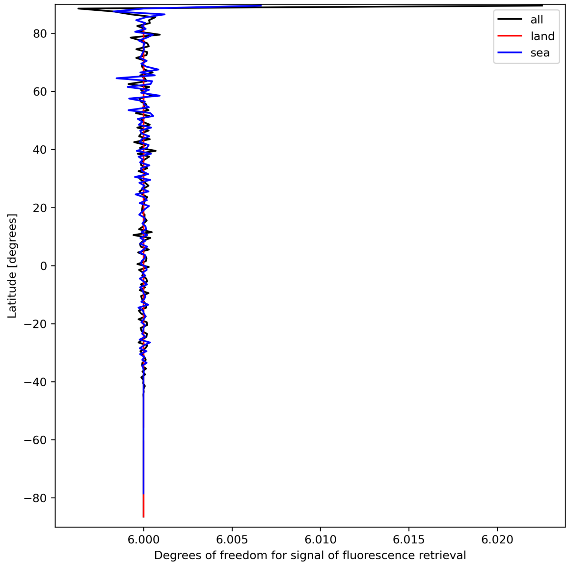
Figure 26: Zonal average of “Degrees of freedom for signal of fluorescence retrieval” for 2023-09-18 to 2023-09-20.
