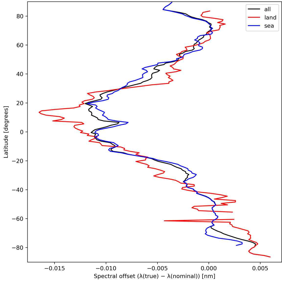
Figure 28: Zonal average of “Spectral offset ( \lambda(\text{true}) - \lambda(\text{nominal}) )” for 2023-09-18 to 2023-09-20.
