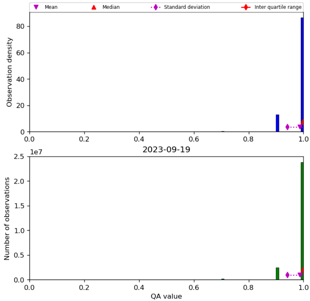
Figure 29: Histogram of “QA value” for 2023-09-18 to 2023-09-20
