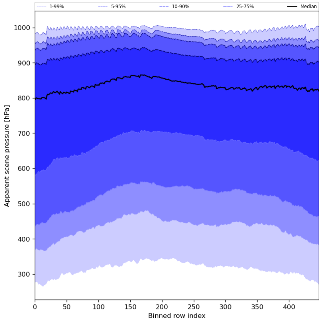
Figure 53: Along track statistics of “Apparent scene pressure” for 2023-09-18 to 2023-09-20
