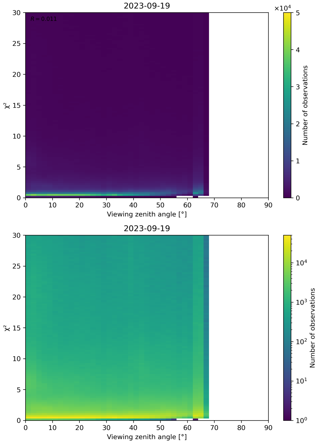
Figure 130: Scatter density plot of “Viewing zenith angle” against “ \chi^2 ” for 2023-09-18 to 2023-09-20.
