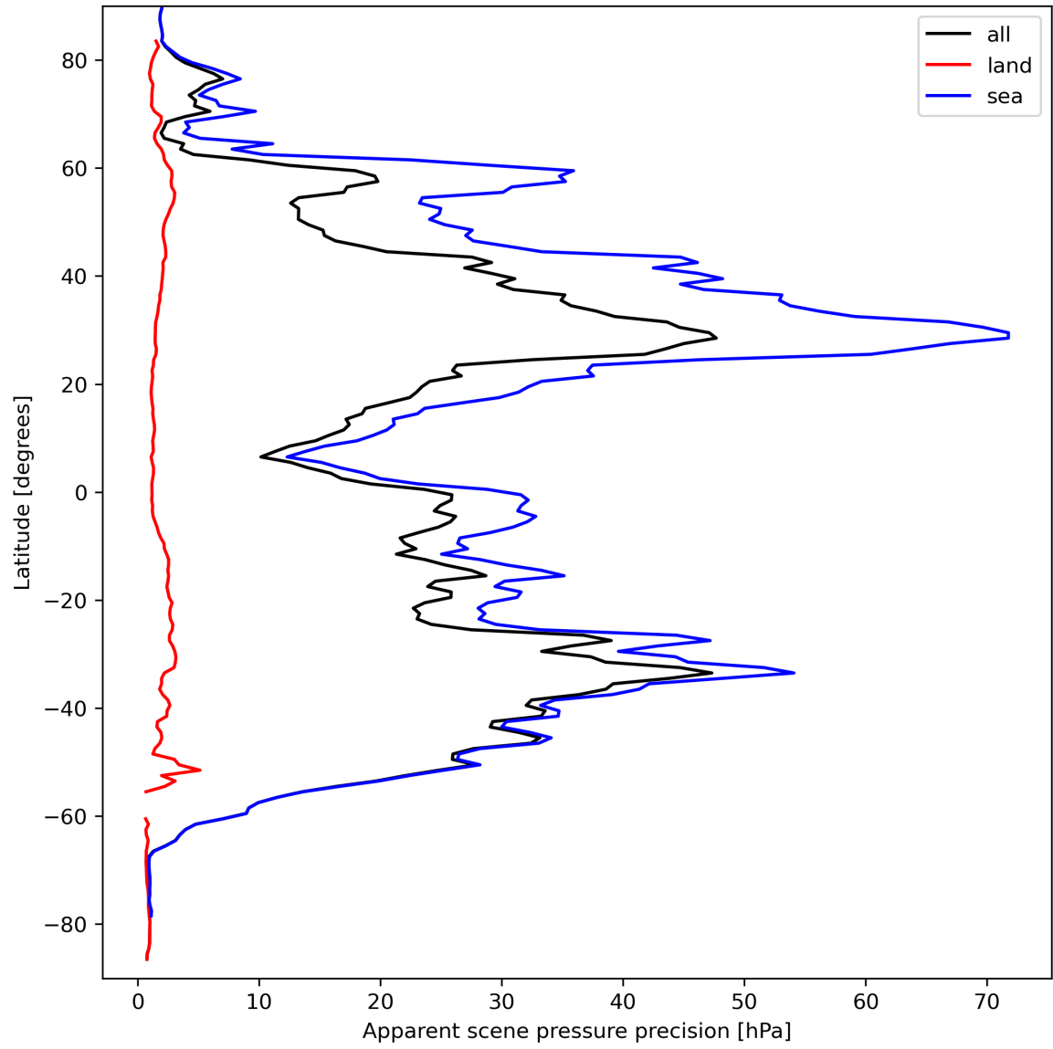
Figure 20: Zonal average of “Apparent scene pressure precision” for 2023-09-18 to 2023-09-20.
