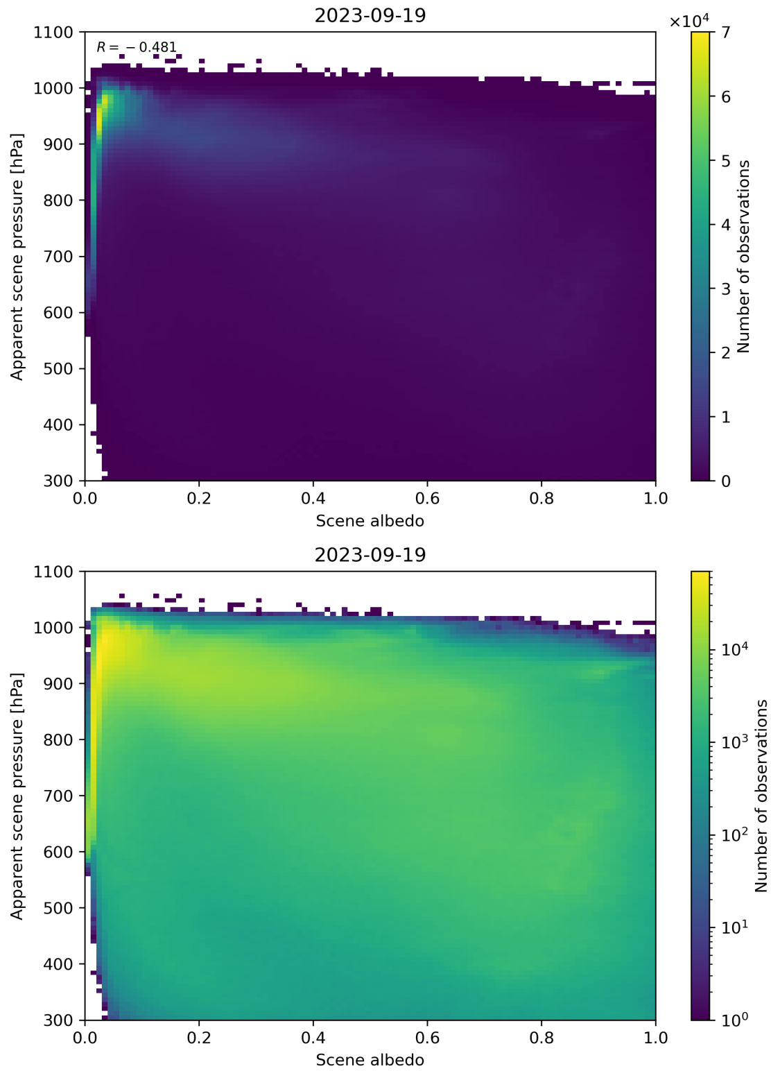
Figure 111: Scatter density plot of “Scene albedo” against “Apparent scene pressure” for 2023-09-18 to 2023-09-20.
