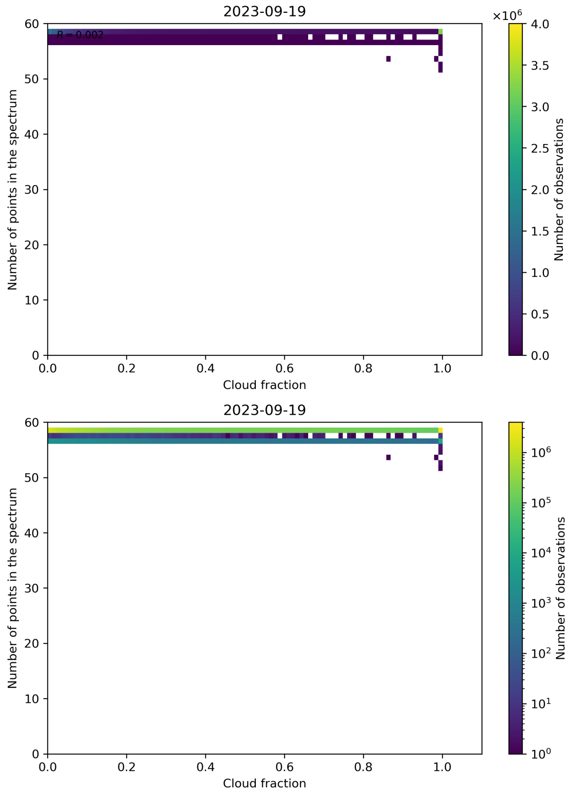
Figure 81: Scatter density plot of “Cloud fraction” against “Number of points in the spectrum” for 2023-09-18 to 2023-09-20.
