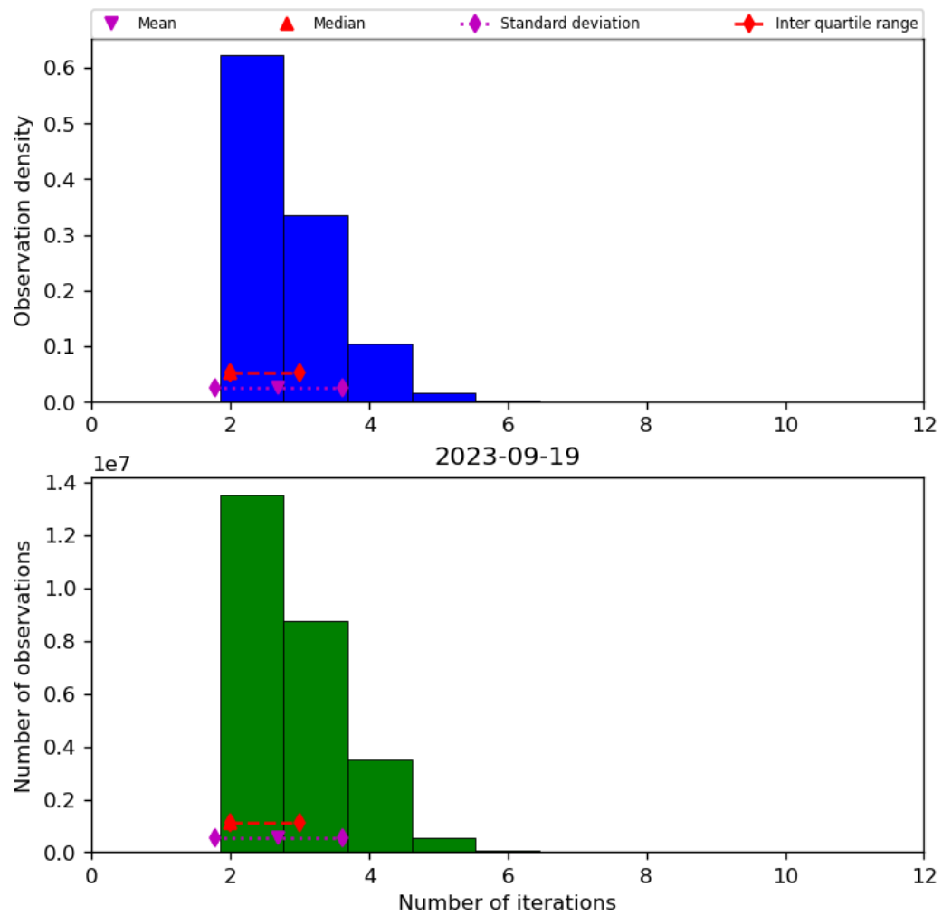
Figure 39: Histogram of “Number of iterations” for 2023-09-18 to 2023-09-20
