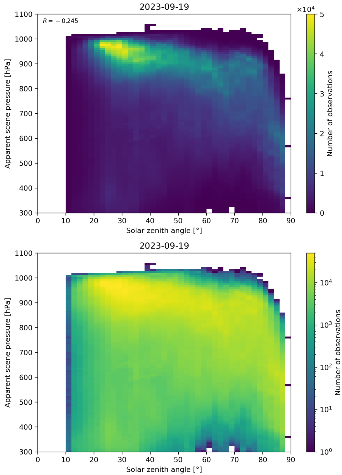
Figure 118: Scatter density plot of “Solar zenith angle” against “Apparent scene pressure” for 2023-09-18 to 2023-09-20.
