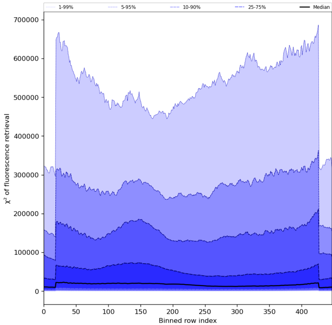
Figure 59: Along track statistics of “ \chi^2 of fluorescence retrieval” for 2023-09-18 to 2023-09-20
