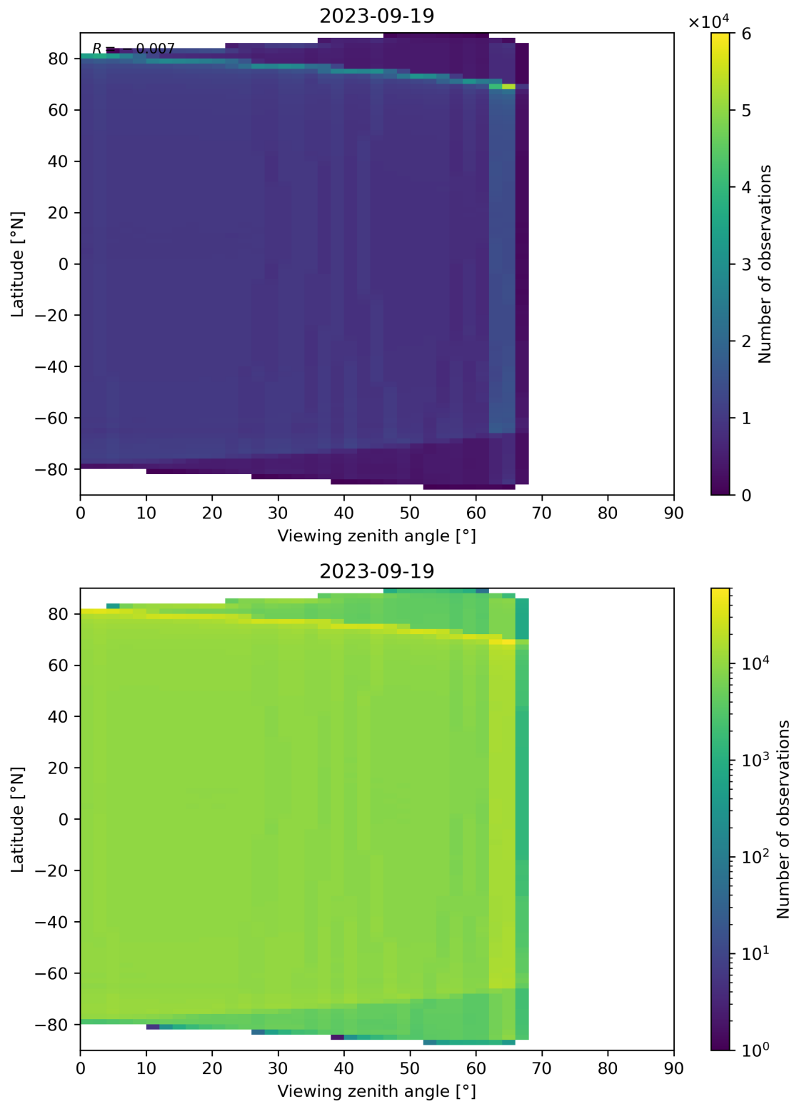
Figure 135: Scatter density plot of “Viewing zenith angle” against “Latitude” for 2023-09-18 to 2023-09-20.
