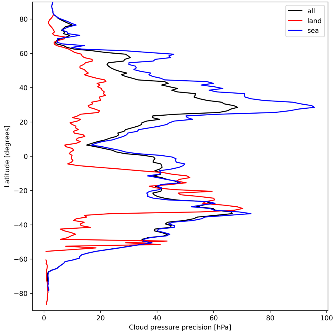
Figure 14: Zonal average of “Cloud pressure precision” for 2023-09-18 to 2023-09-20.
