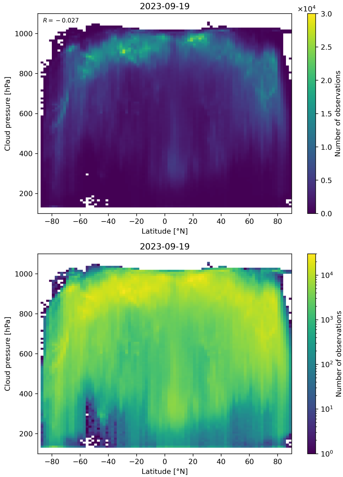
Figure 100: Scatter density plot of “Latitude” against “Cloud pressure” for 2023-09-18 to 2023-09-20.
