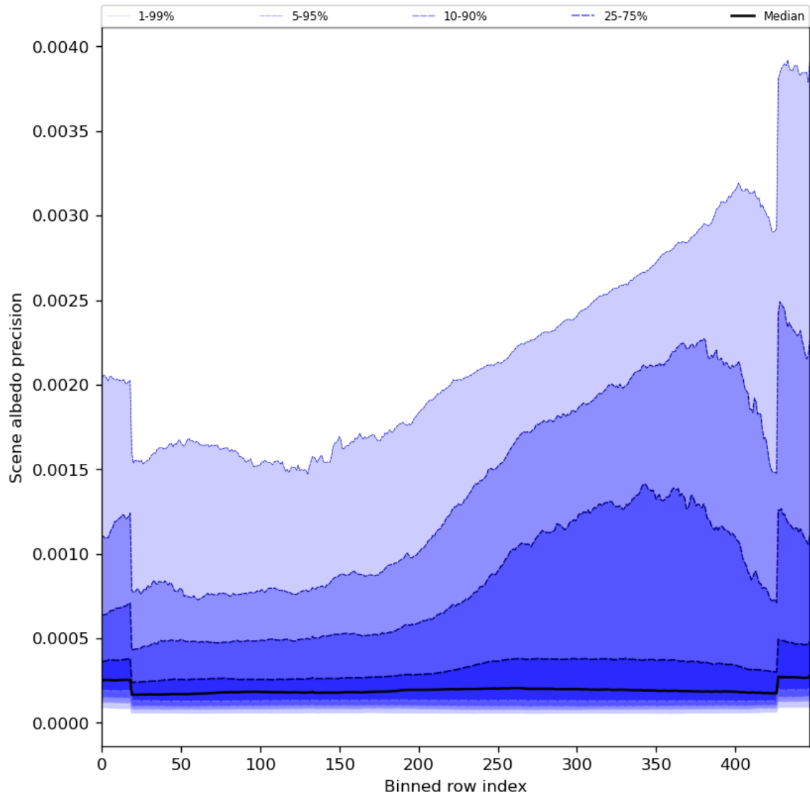
Figure 52: Along track statistics of “Scene albedo precision” for 2023-09-18 to 2023-09-20
