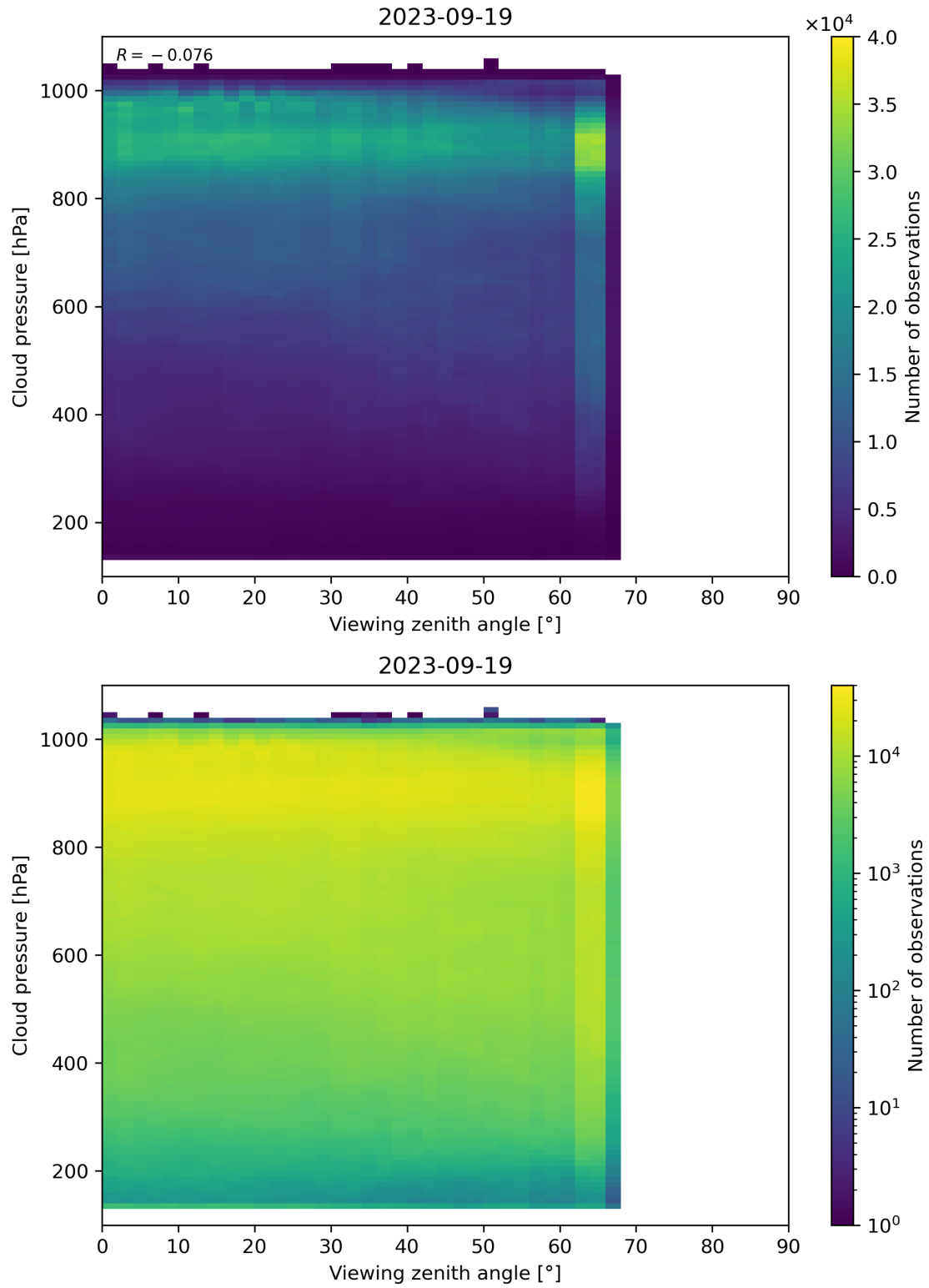
Figure 133: Scatter density plot of “Viewing zenith angle” against “Cloud pressure” for 2023-09-18 to 2023-09-20.
