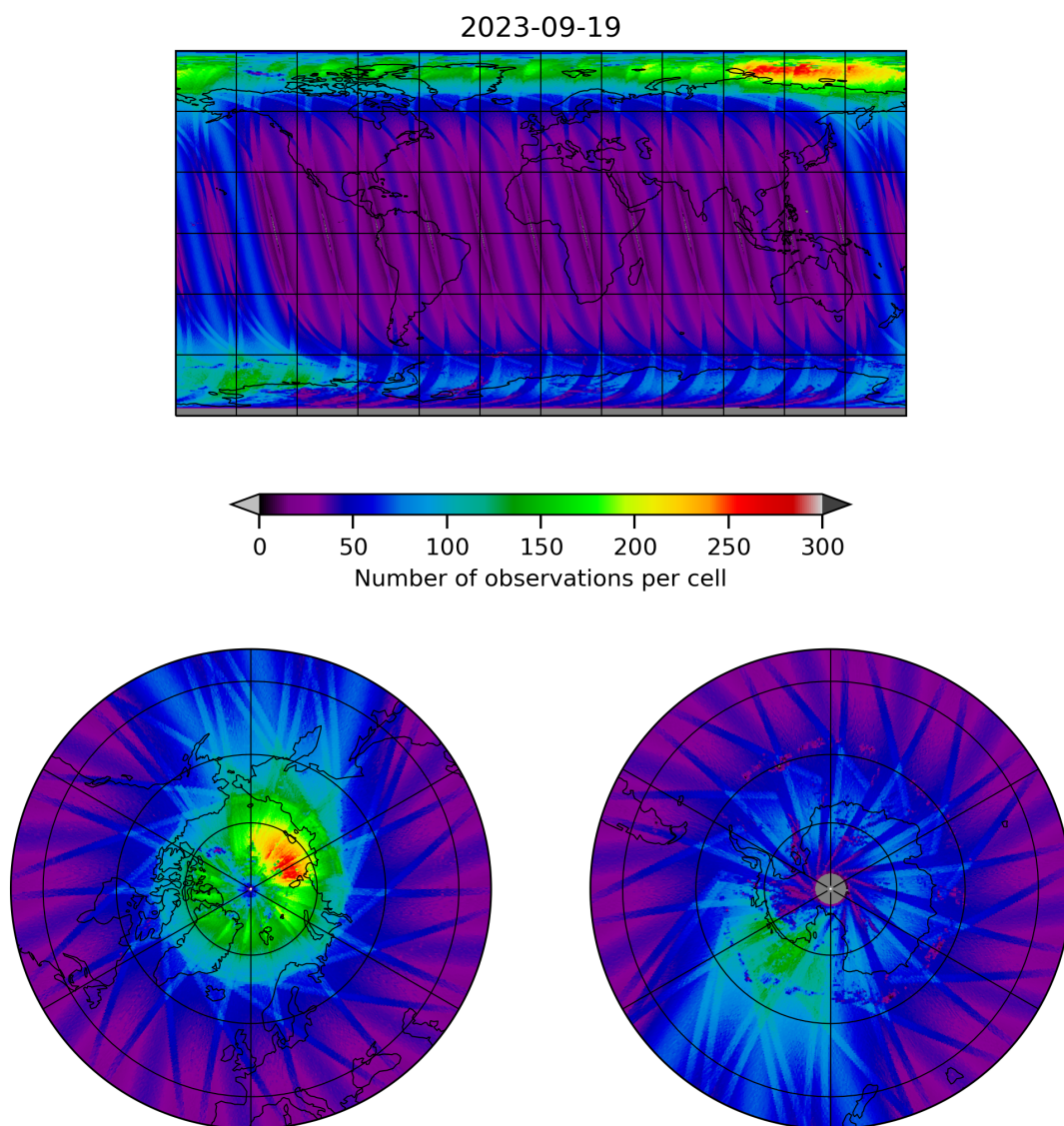
Figure 11: Map of the number of observations for 2023-09-18 to 2023-09-20
