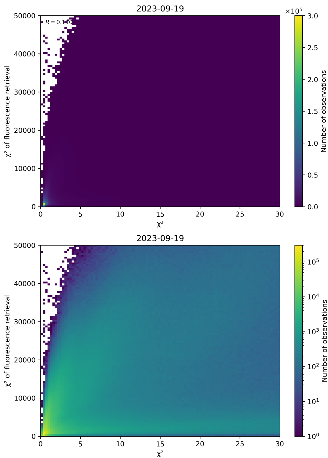
Figure 69: Scatter density plot of “ \chi^2 ” against “ \chi^2 of fluorescence retrieval” for 2023-09-18 to 2023-09-20.
