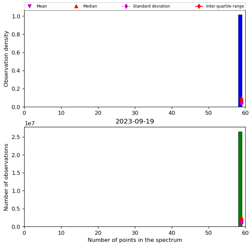
Figure 44: Histogram of "Number of points in the spectrum" for 2023-09-18 to 2023-09-20
