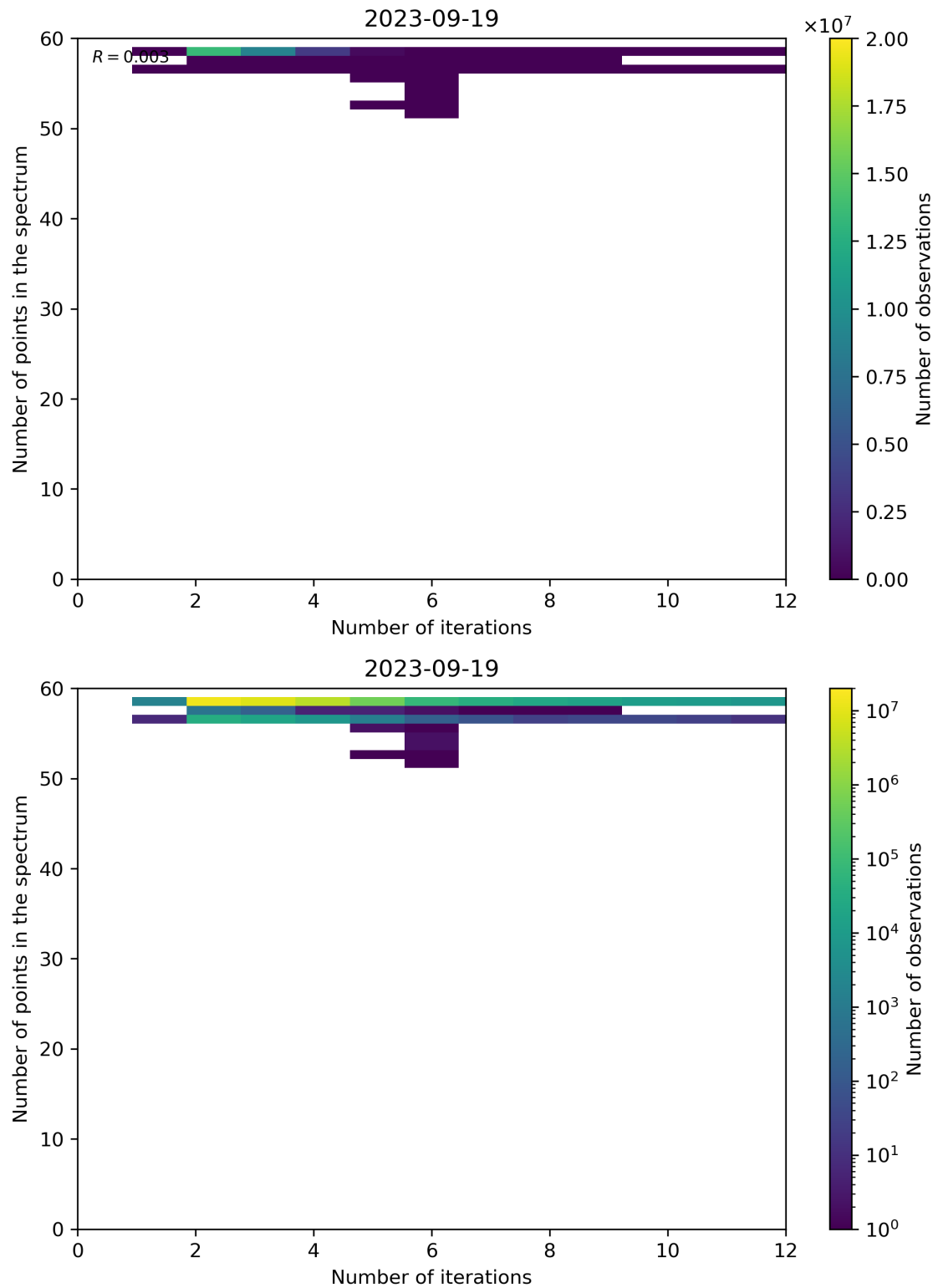
Figure 108: Scatter density plot of “Number of iterations” against “Number of points in the spectrum” for 2023-09-18 to 2023-09-20.
