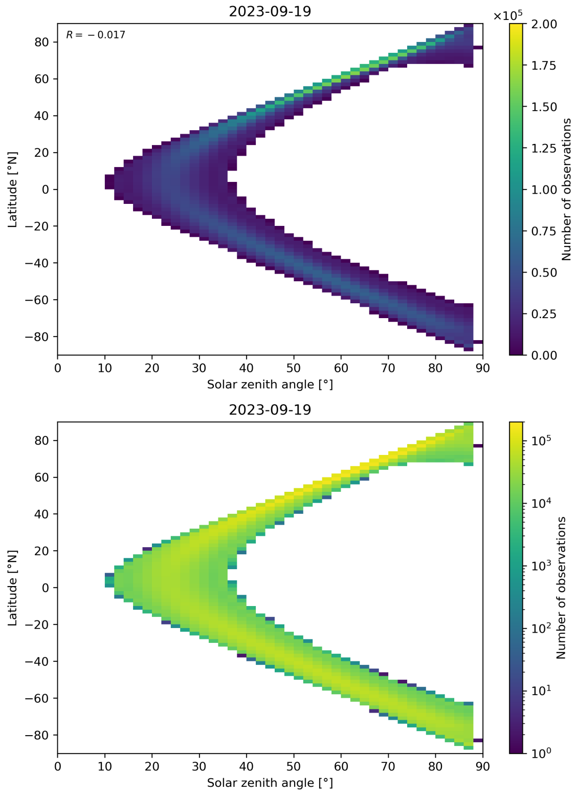
Figure 124: Scatter density plot of “Solar zenith angle” against “Latitude” for 2023-09-18 to 2023-09-20.
