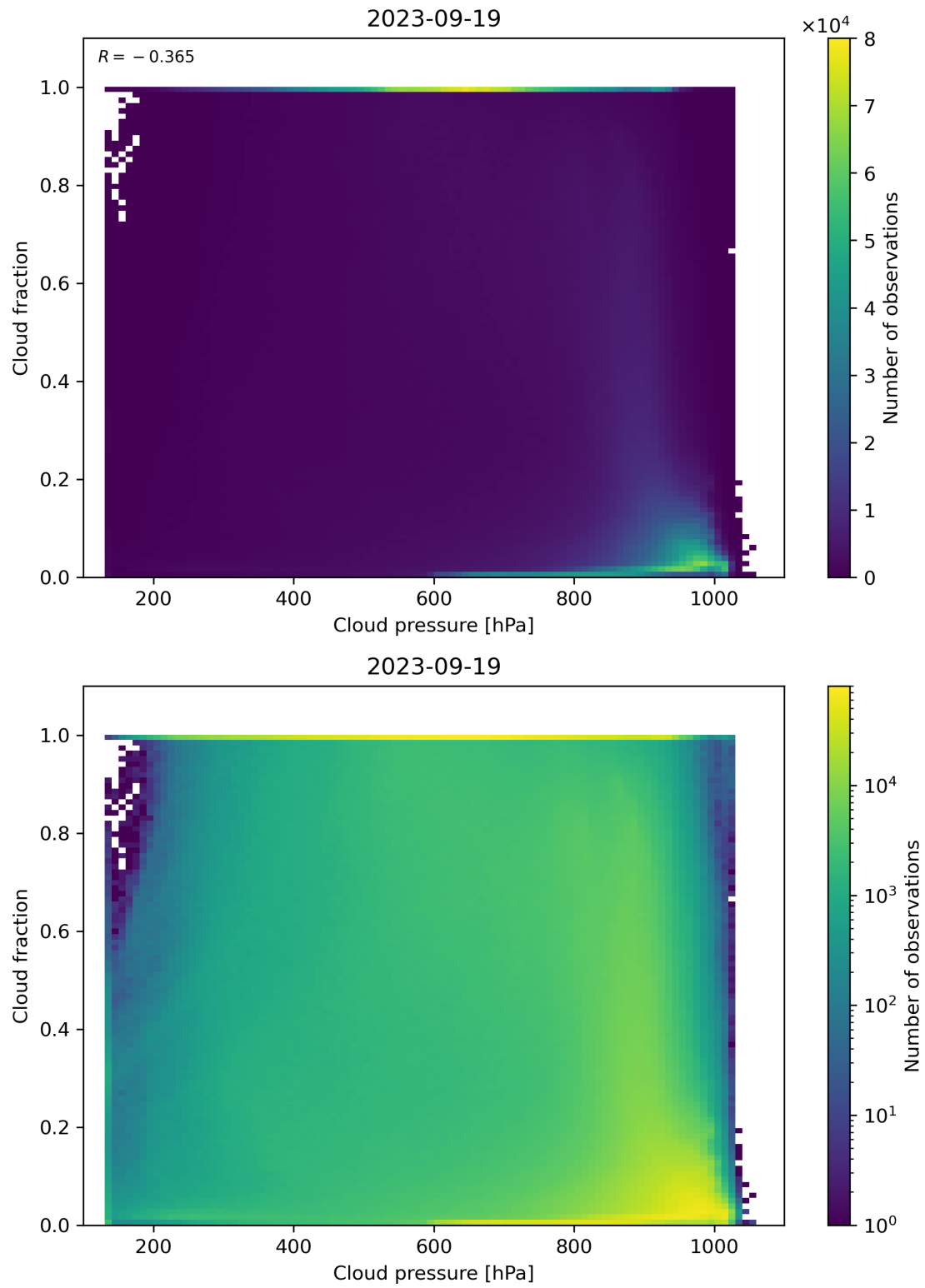
Figure 87: Scatter density plot of “Cloud pressure” against “Cloud fraction” for 2023-09-18 to 2023-09-20.
