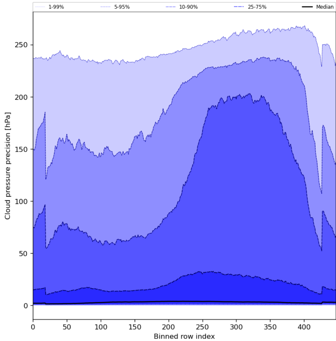
Figure 48: Along track statistics of “Cloud pressure precision” for 2023-09-18 to 2023-09-20
