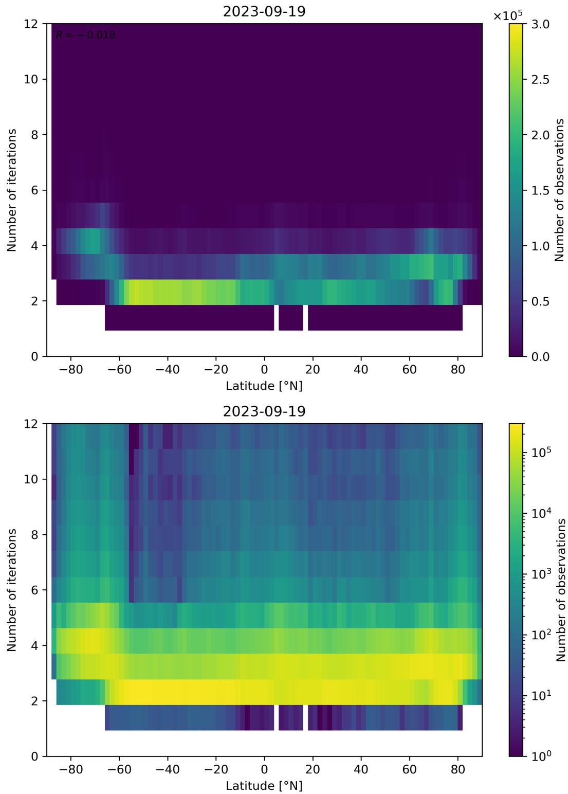
Figure 102: Scatter density plot of “Latitude” against “Number of iterations” for 2023-09-18 to 2023-09-20.
