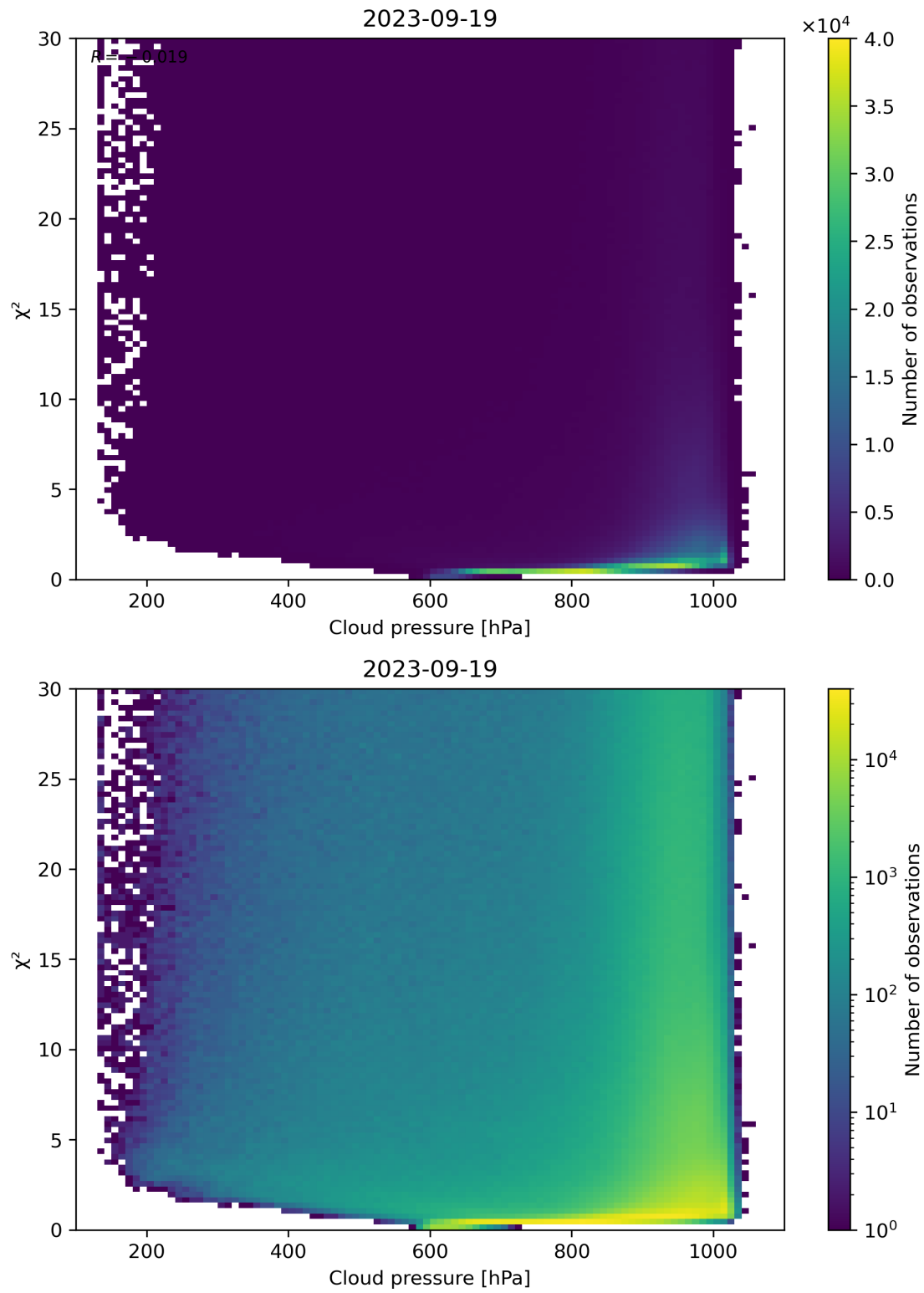
Figure 85: Scatter density plot of “Cloud pressure” against “ \chi^2 ” for 2023-09-18 to 2023-09-20.
