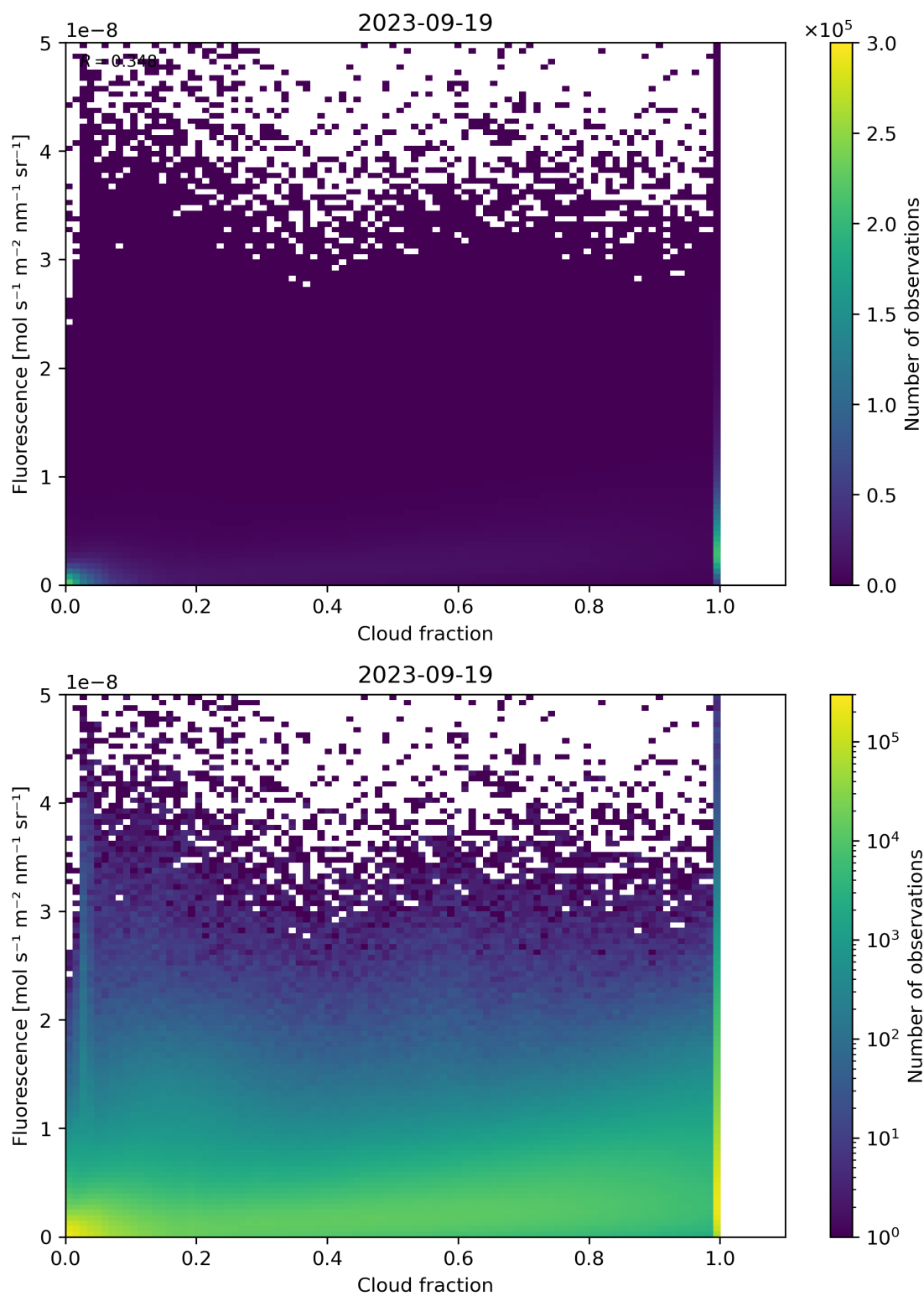
Figure 79: Scatter density plot of “Cloud fraction” against “Fluorescence” for 2023-09-18 to 2023-09-20.
