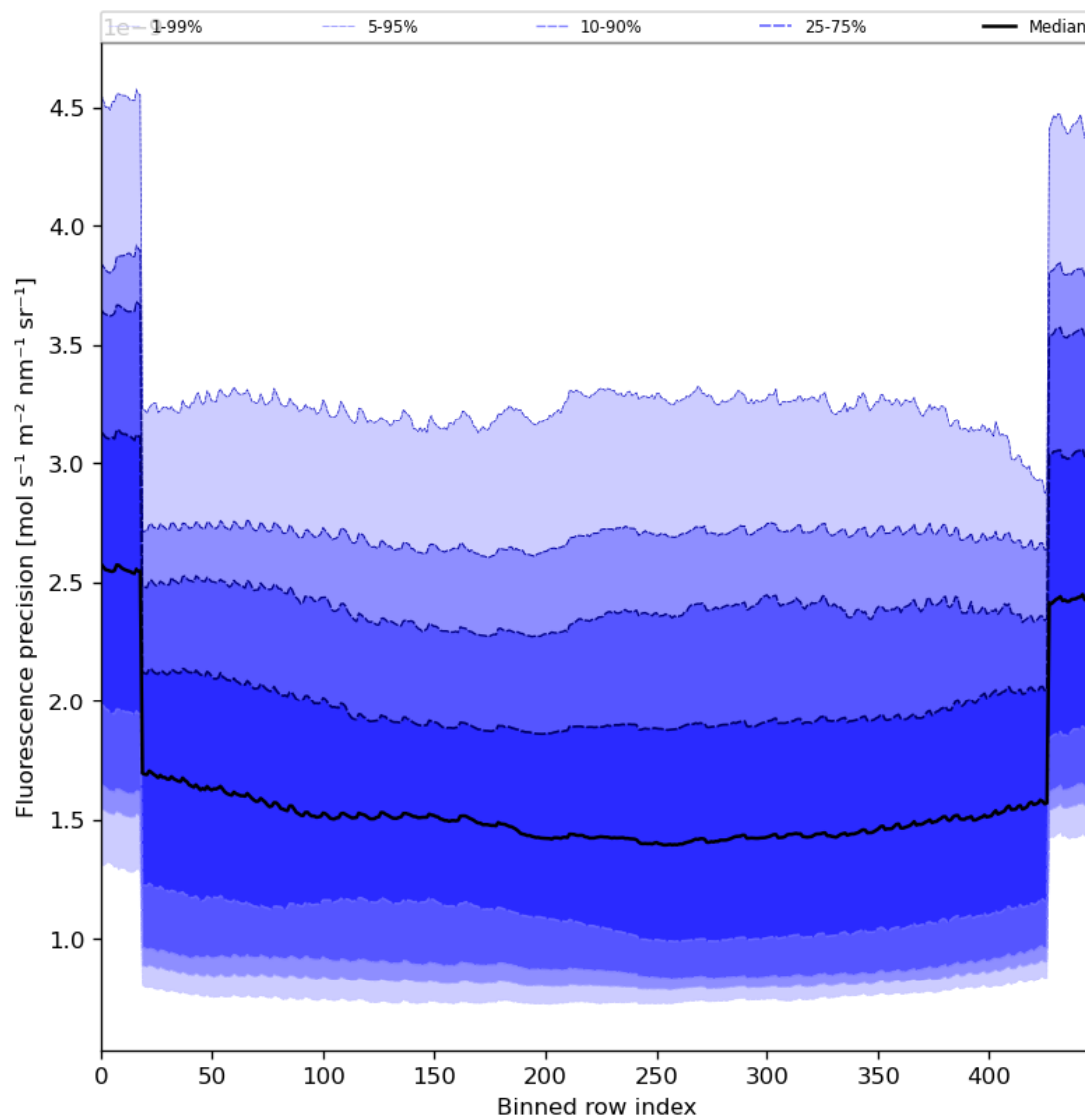
Figure 58: Along track statistics of “Fluorescence precision” for 2023-09-18 to 2023-09-20
