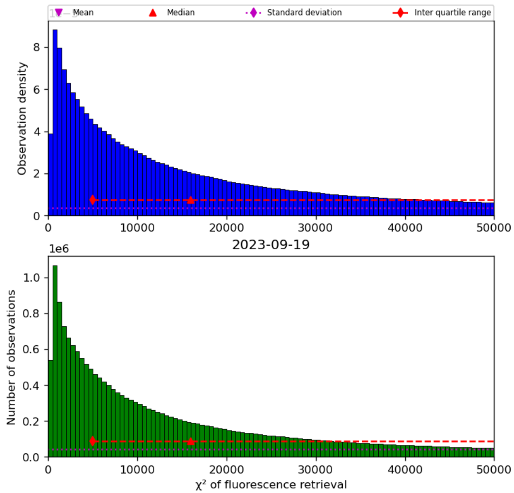
Figure 42: Histogram of “ \chi^2 of fluorescence retrieval” for 2023-09-18 to 2023-09-20
