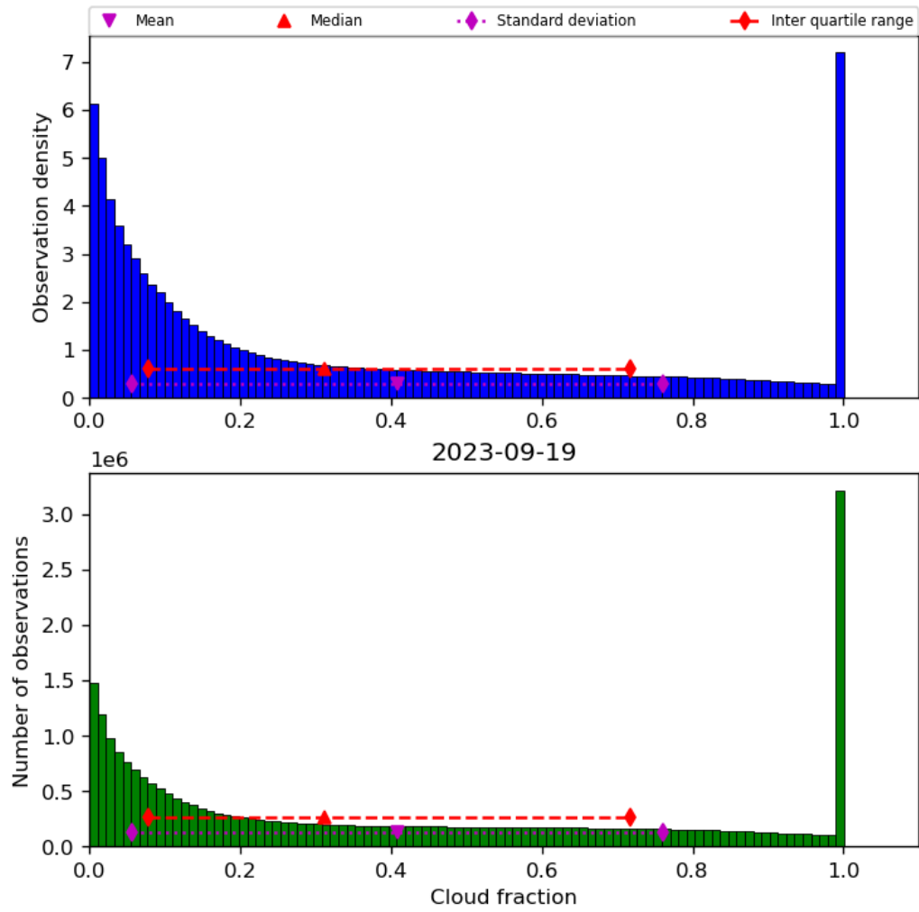
Figure 32: Histogram of “Cloud fraction” for 2023-09-18 to 2023-09-20
