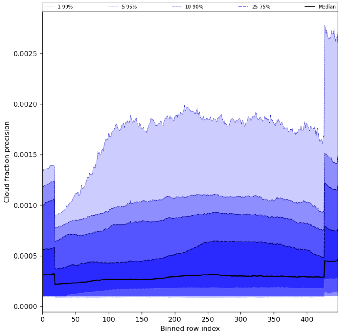
Figure 50: Along track statistics of “Cloud fraction precision” for 2023-09-18 to 2023-09-20
