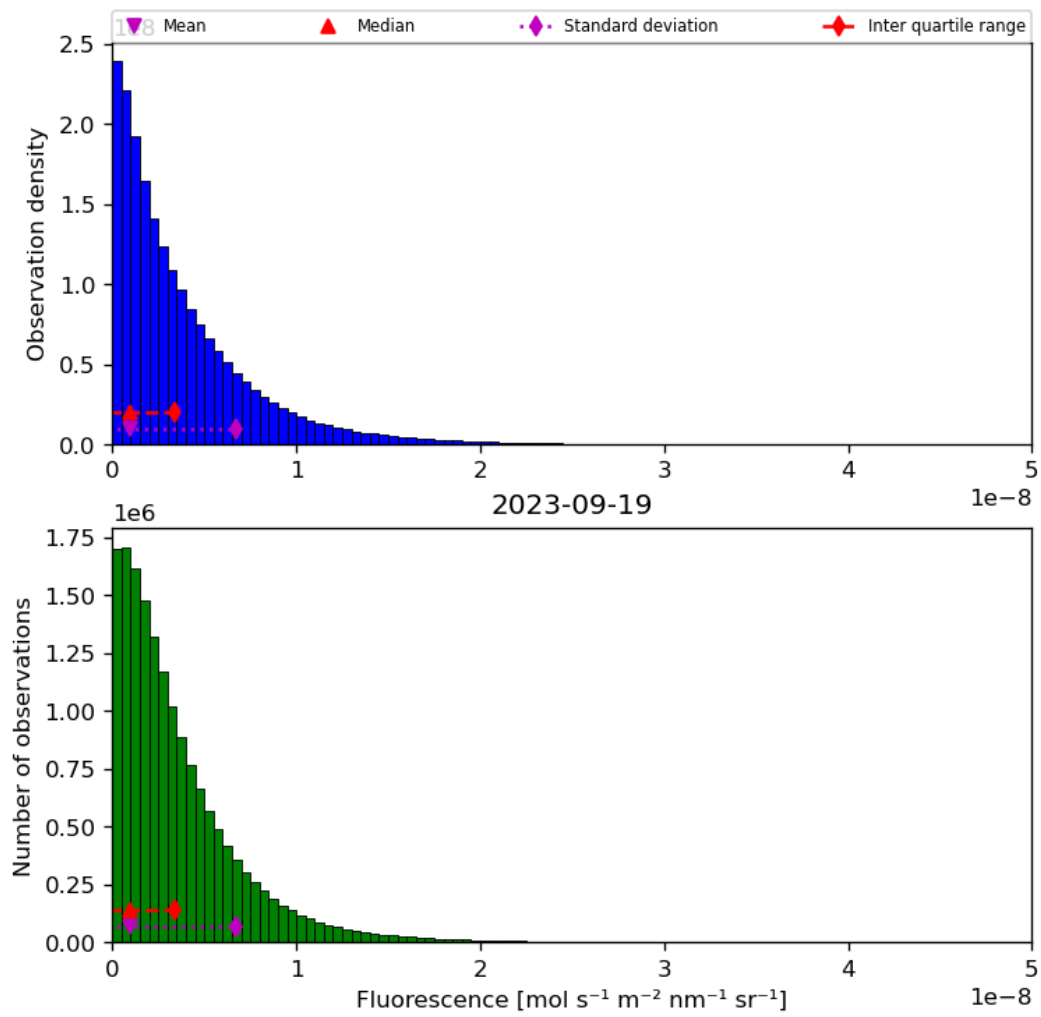
Figure 40: Histogram of “Fluorescence” for 2023-09-18 to 2023-09-20
