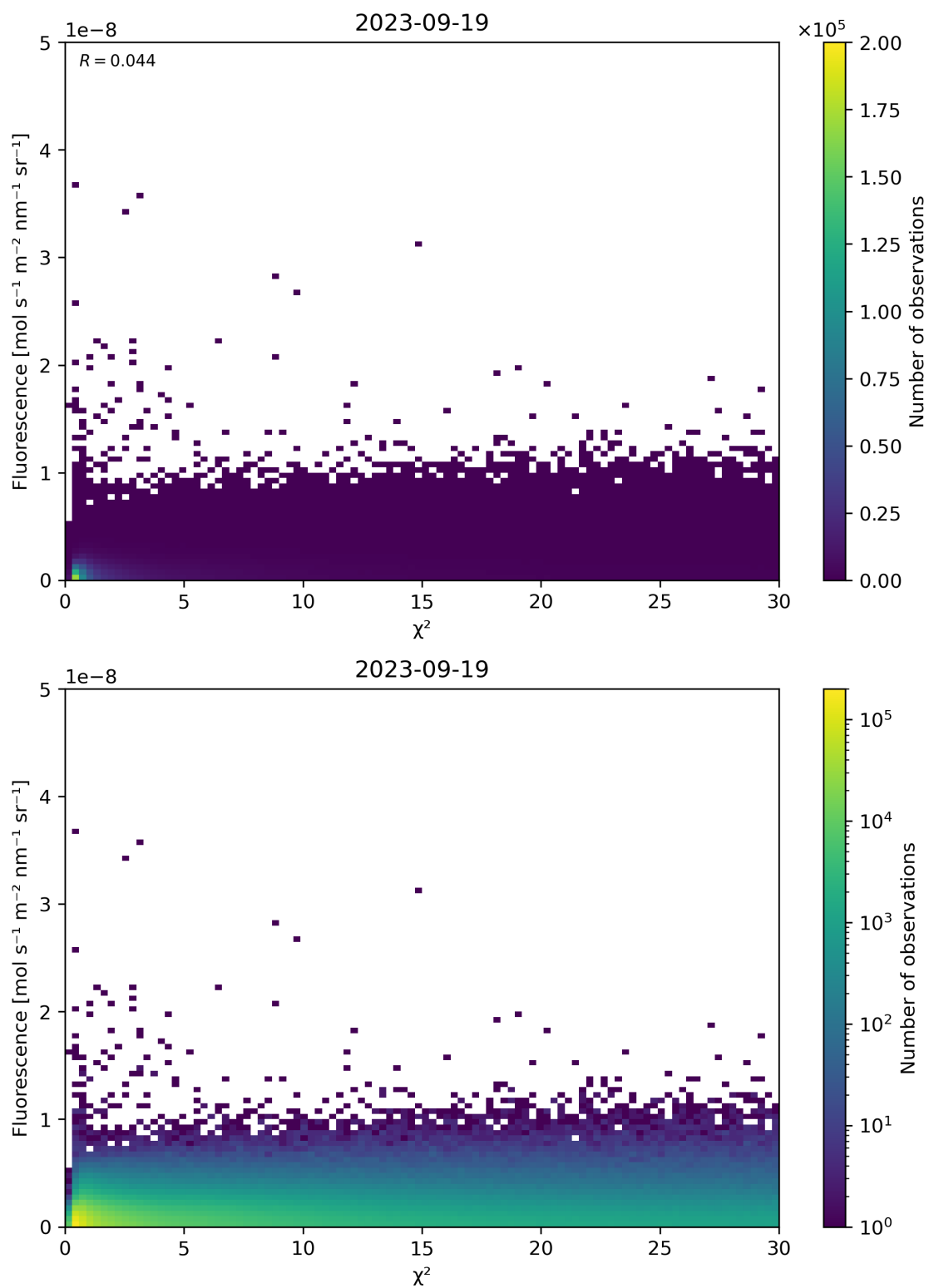
Figure 70: Scatter density plot of “ \chi^2 ” against “Fluorescence” for 2023-09-18 to 2023-09-20.
