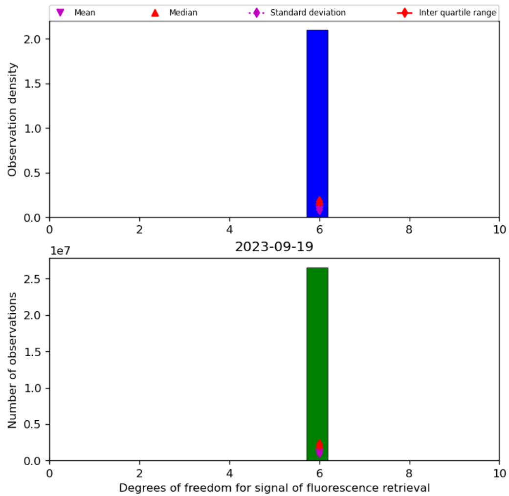
Figure 43: Histogram of “Degrees of freedom for signal of fluorescence retrieval” for 2023-09-18 to 2023-09-20
