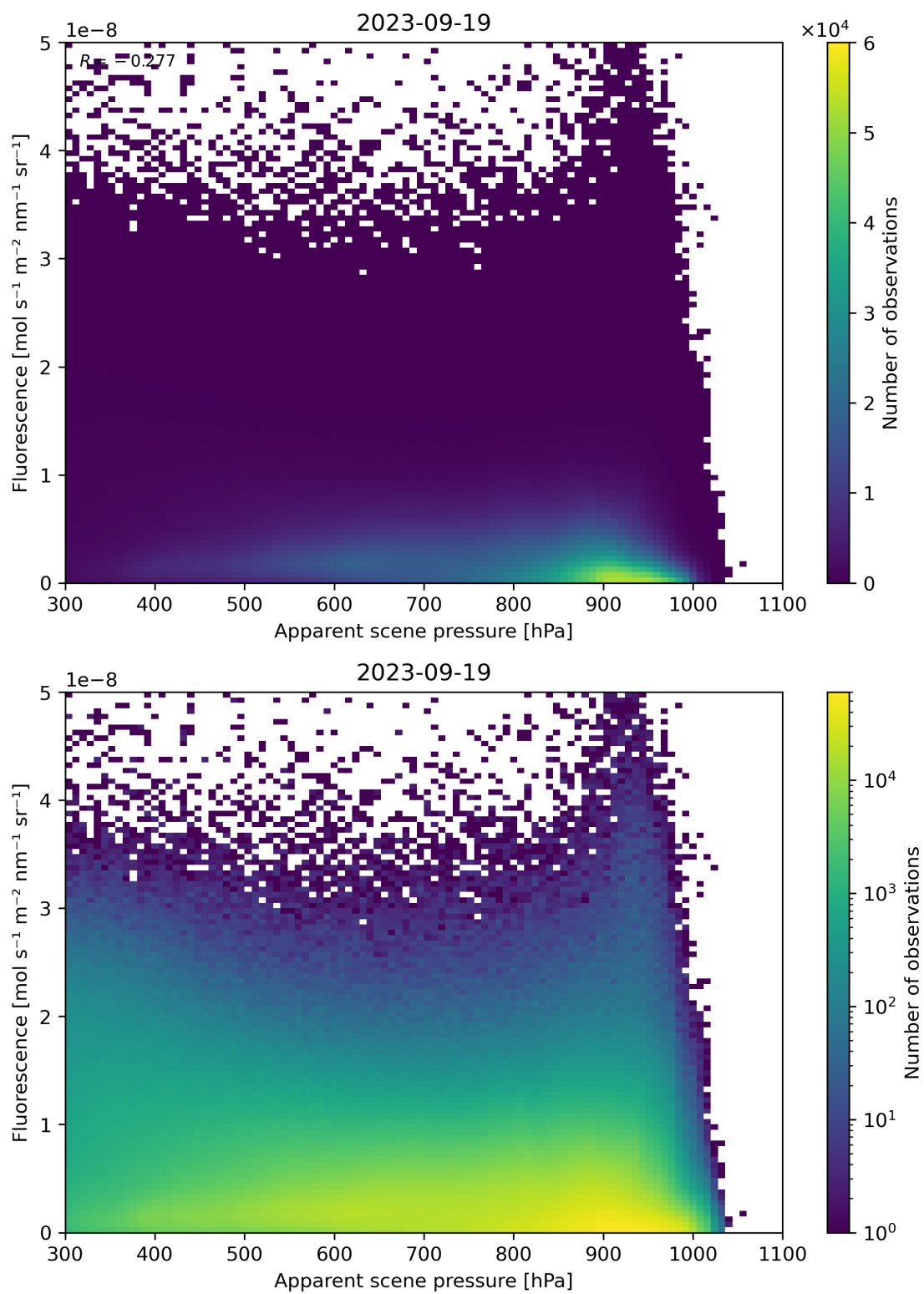
Figure 65: Scatter density plot of “Apparent scene pressure” against “Fluorescence” for 2023-09-18 to 2023-09-20.
