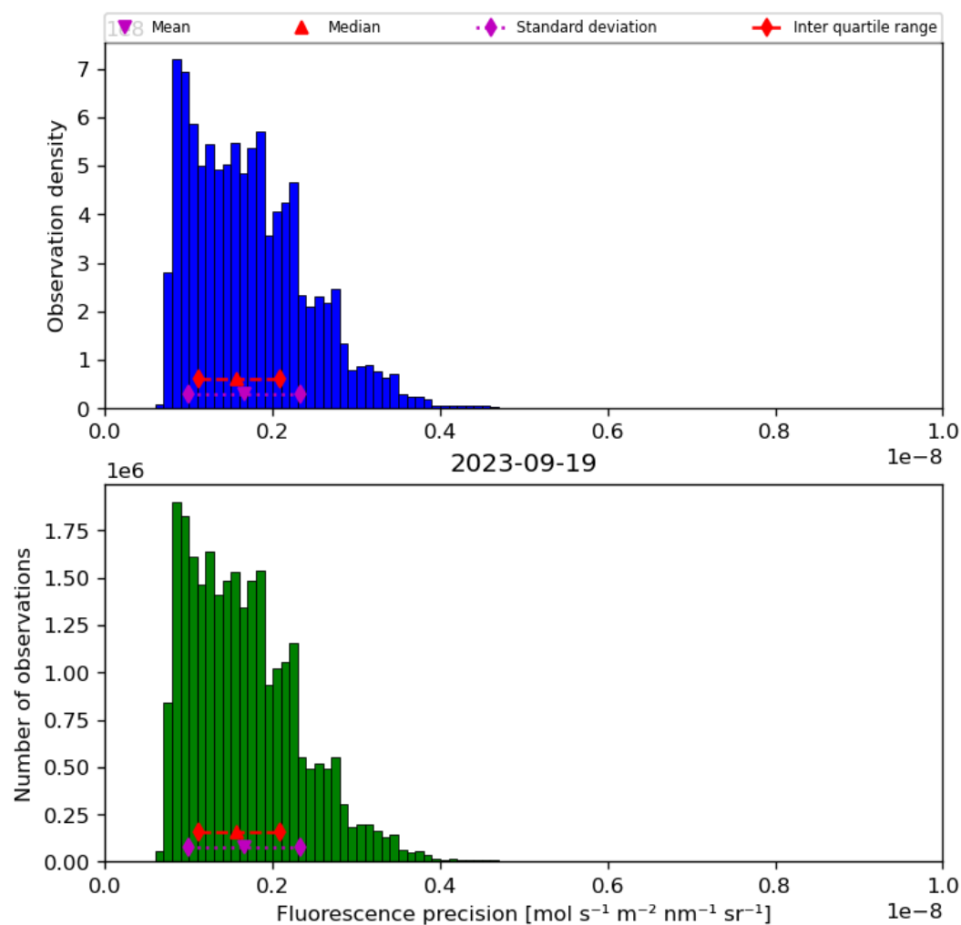
Figure 41: Histogram of “Fluorescence precision” for 2023-09-18 to 2023-09-20
