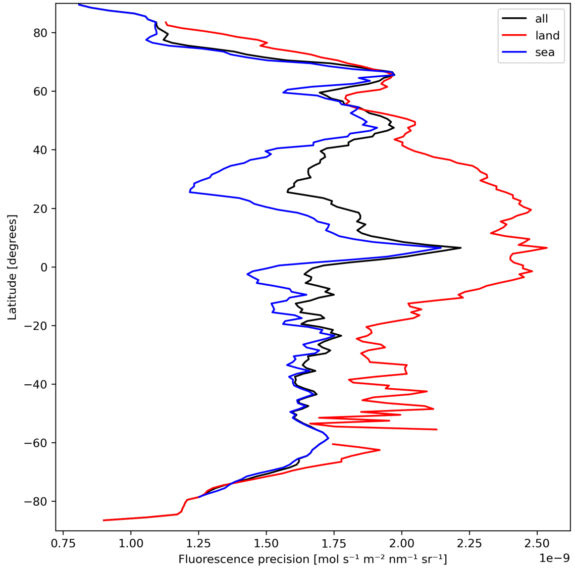
Figure 24: Zonal average of “Fluorescence precision” for 2023-09-18 to 2023-09-20.
