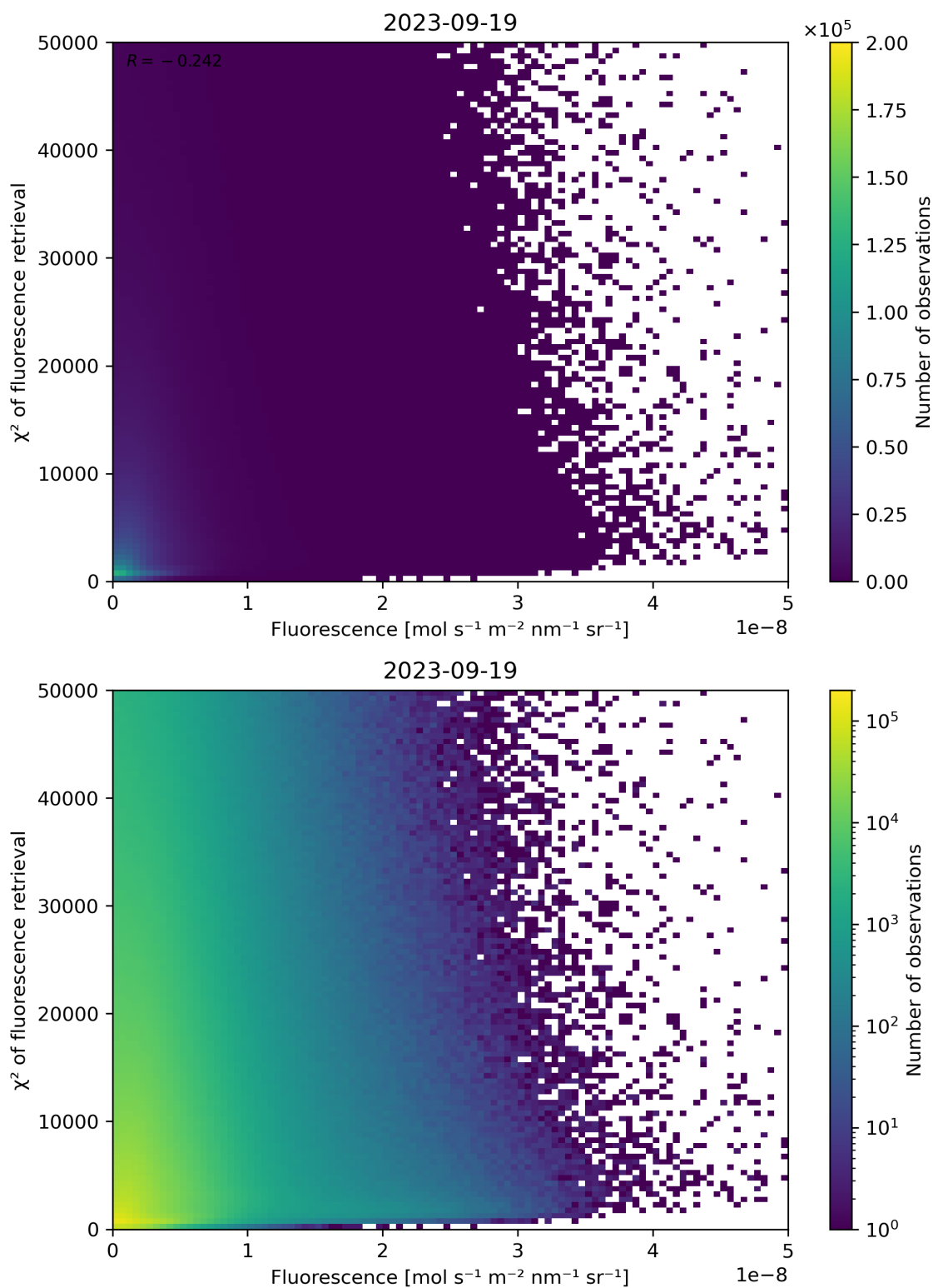
Figure 93: Scatter density plot of “Fluorescence” against “ \chi^2 of fluorescence retrieval” for 2023-09-18 to 2023-09-20.
