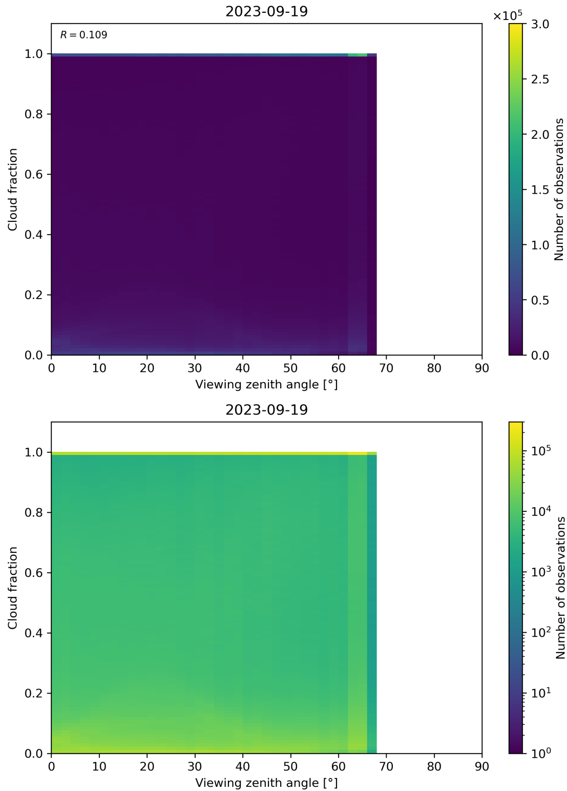
Figure 132: Scatter density plot of “Viewing zenith angle” against “Cloud fraction” for 2023-09-18 to 2023-09-20.
