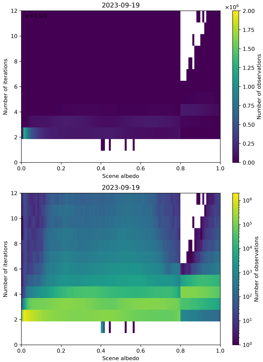
Figure 115: Scatter density plot of “Scene albedo” against “Number of iterations” for 2023-09-18 to 2023-09-20.
