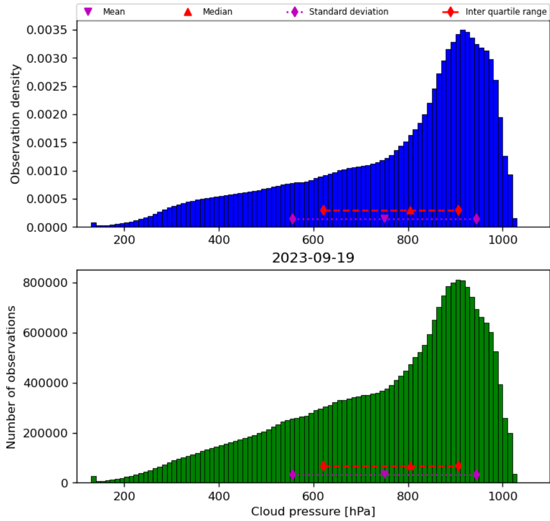
Figure 30: Histogram of “Cloud pressure” for 2023-09-18 to 2023-09-20
