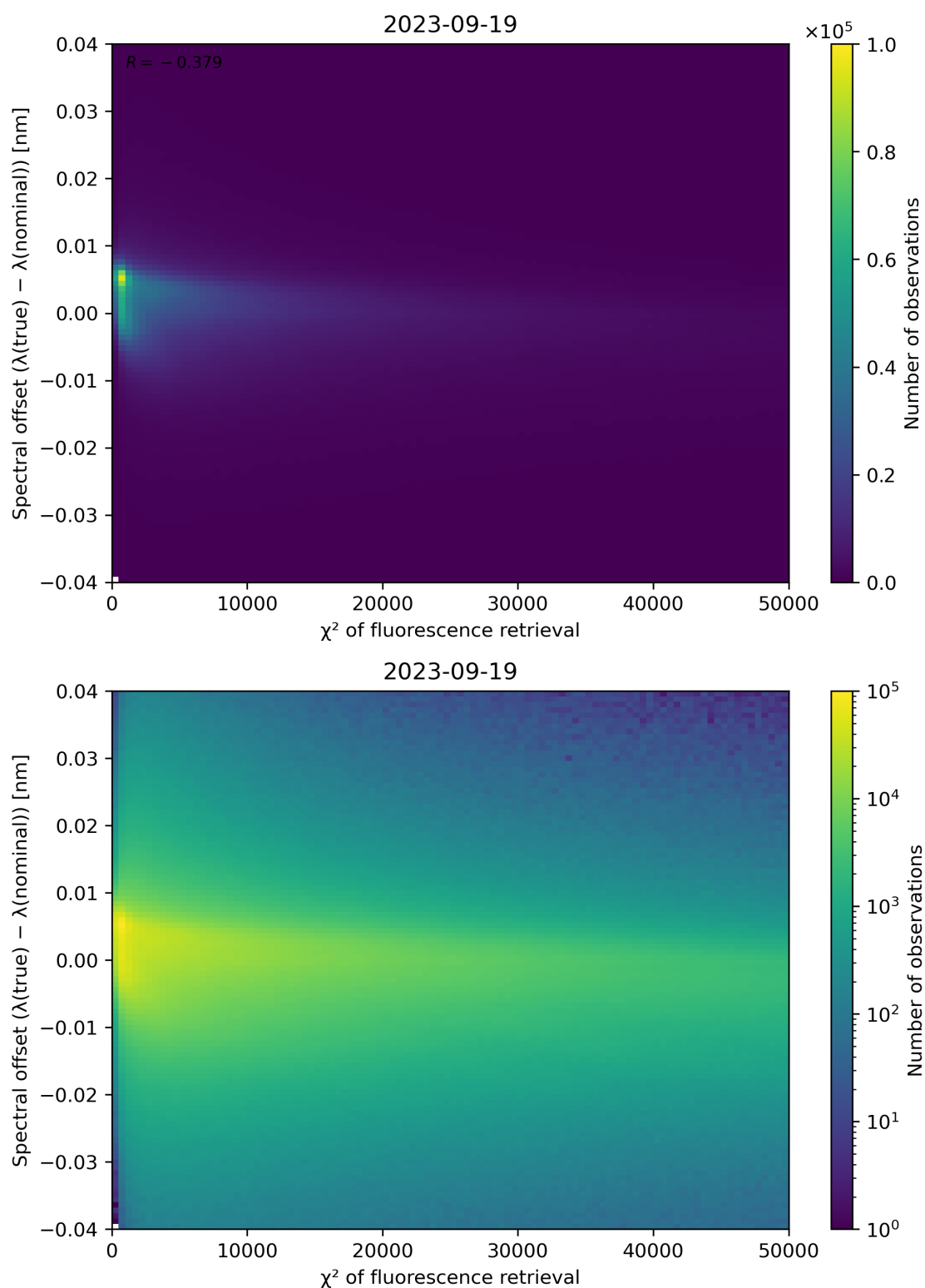
Figure 72: Scatter density plot of " \chi^2 of fluorescence retrieval" against "Spectral offset ( \lambda(\text{true}) - \lambda(\text{nominal}) )" for 2023-09-18 to 2023-09-20.
