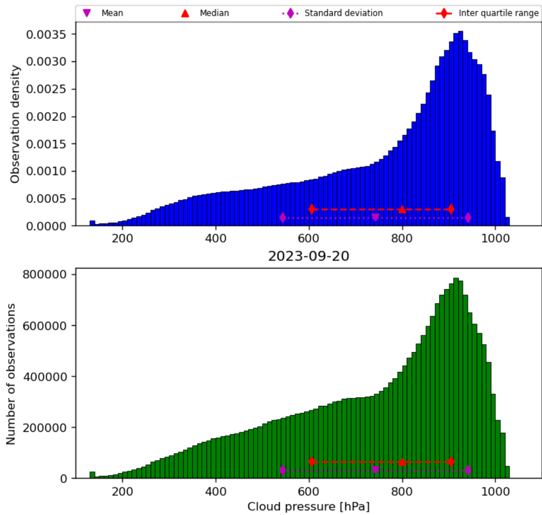
Figure 30: Histogram of “Cloud pressure” for 2023-09-20 to 2023-09-21
