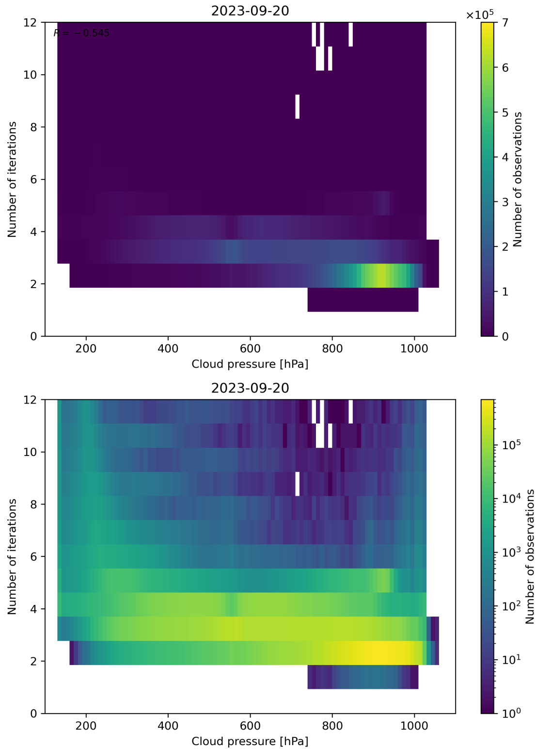
Figure 89: Scatter density plot of “Cloud pressure” against “Number of iterations” for 2023-09-20 to 2023-09-21.
