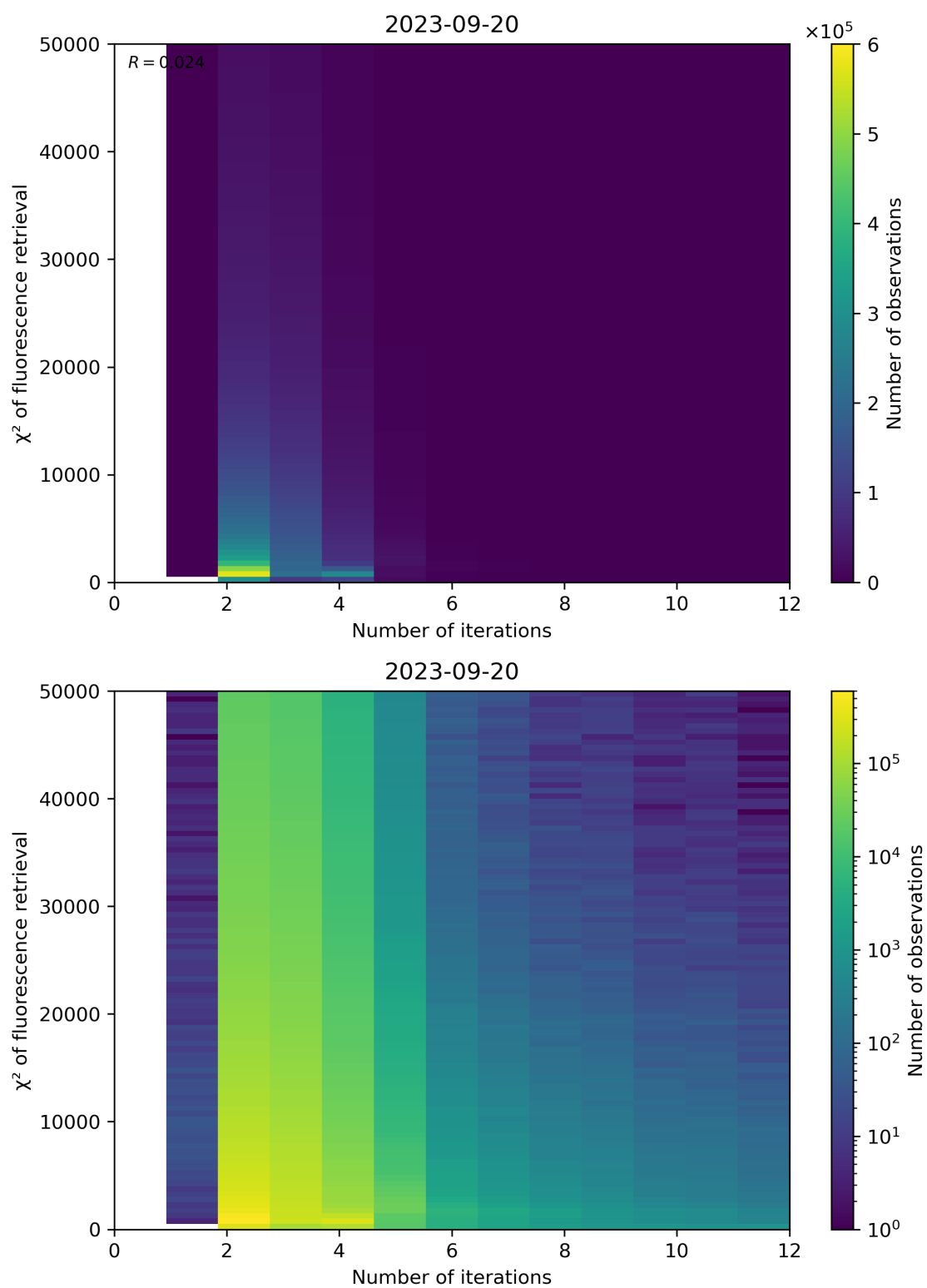
Figure 106: Scatter density plot of “Number of iterations” against “ \chi^2 of fluorescence retrieval” for 2023-09-20 to 2023-09-21.
