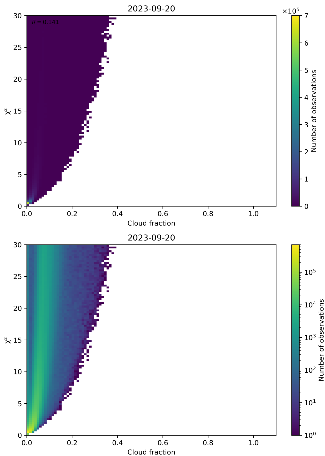
Figure 77: Scatter density plot of “Cloud fraction” against “ \chi^2 ” for 2023-09-20 to 2023-09-21.
