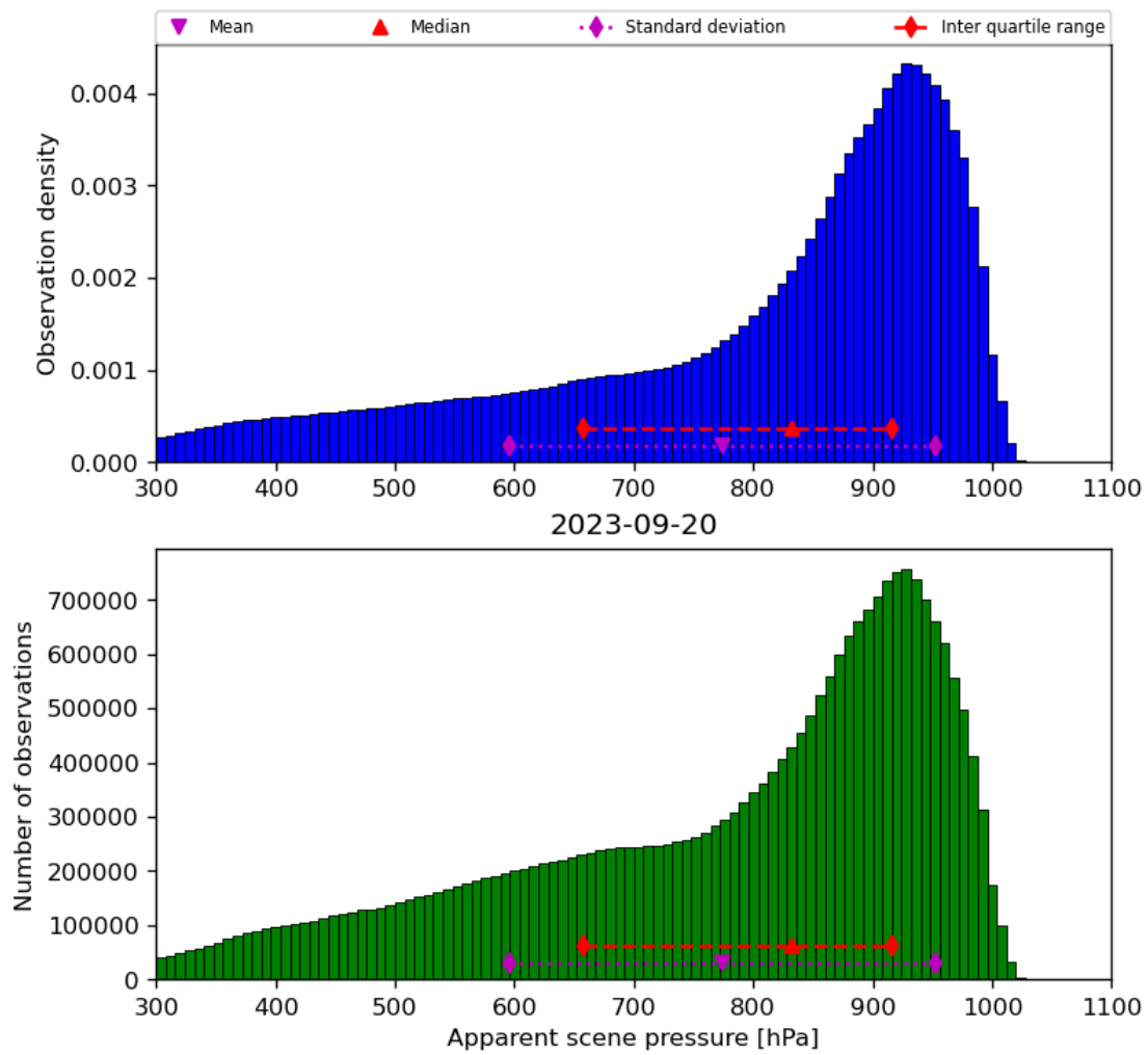
Figure 36: Histogram of “Apparent scene pressure” for 2023-09-20 to 2023-09-21
