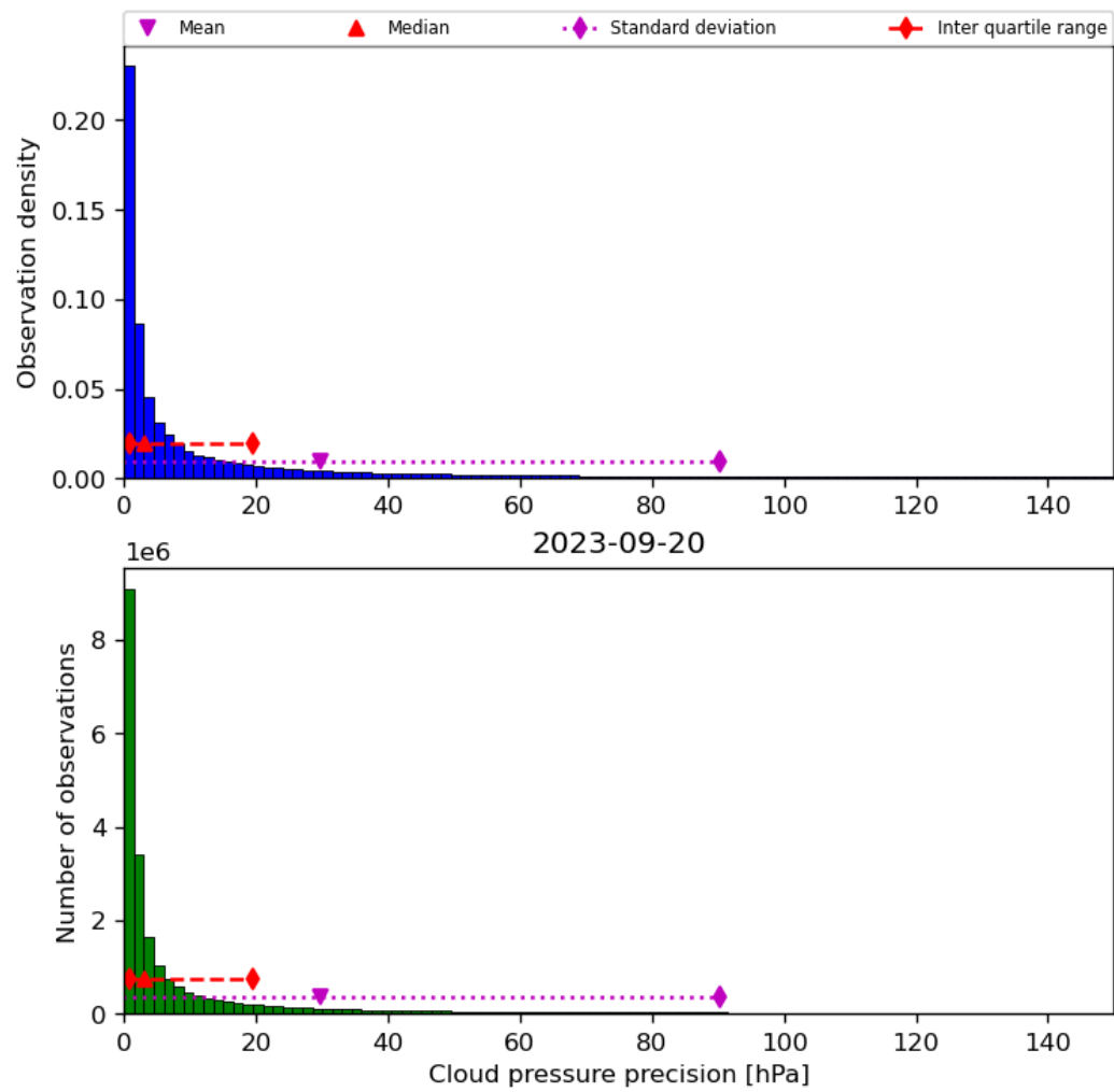
Figure 31: Histogram of “Cloud pressure precision” for 2023-09-20 to 2023-09-21
