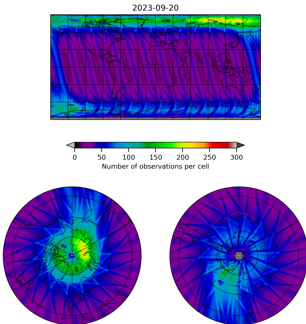
Figure 11: Map of the number of observations for 2023-09-20 to 2023-09-21
