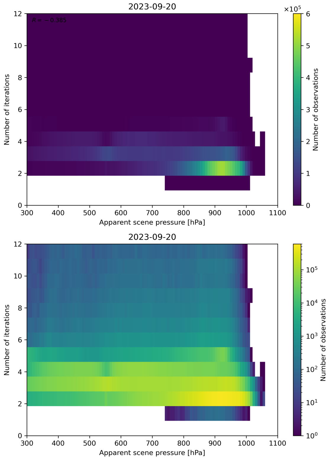
Figure 66: Scatter density plot of “Apparent scene pressure” against “Number of iterations” for 2023-09-20 to 2023-09-21.
