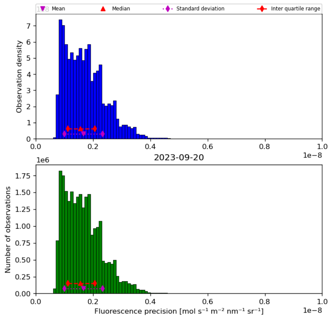
Figure 41: Histogram of “Fluorescence precision” for 2023-09-20 to 2023-09-21
