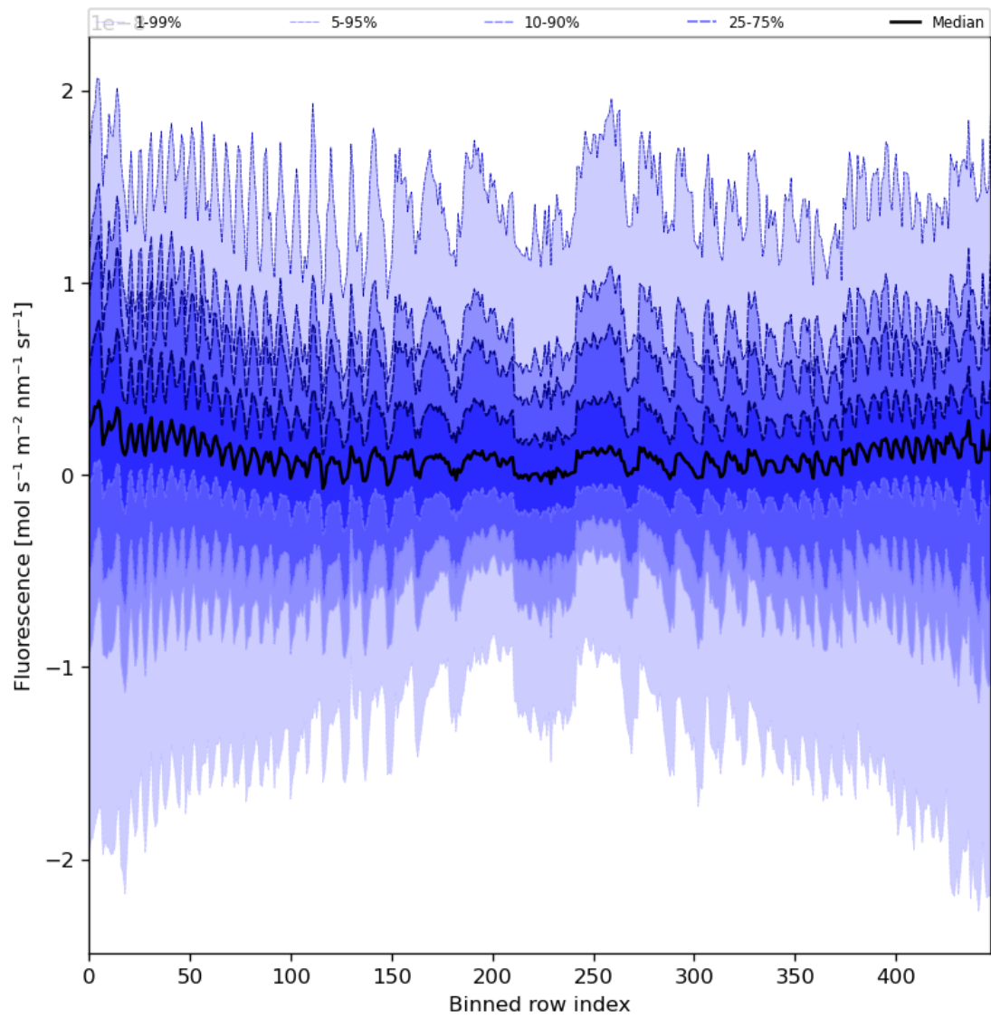
Figure 57: Along track statistics of “Fluorescence” for 2023-09-20 to 2023-09-21
