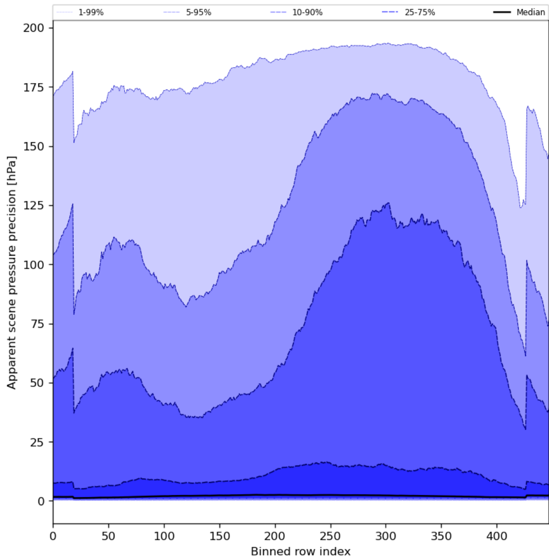
Figure 54: Along track statistics of “Apparent scene pressure precision” for 2023-09-20 to 2023-09-21
