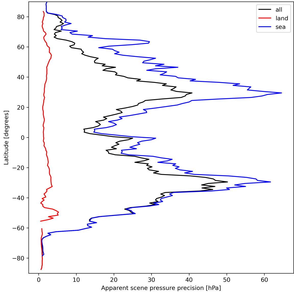
Figure 20: Zonal average of “Apparent scene pressure precision” for 2023-09-20 to 2023-09-21.
