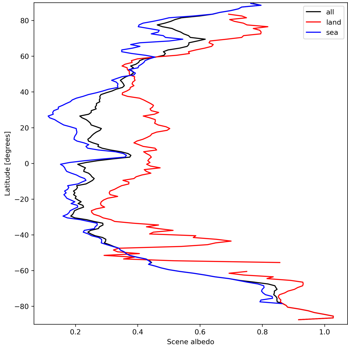
Figure 17: Zonal average of “Scene albedo” for 2023-09-20 to 2023-09-21.
