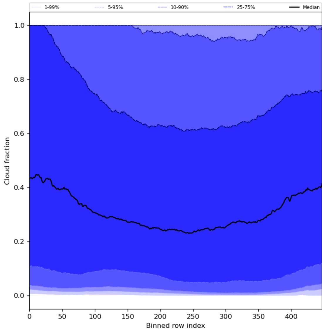
Figure 49: Along track statistics of “Cloud fraction” for 2023-09-20 to 2023-09-21
