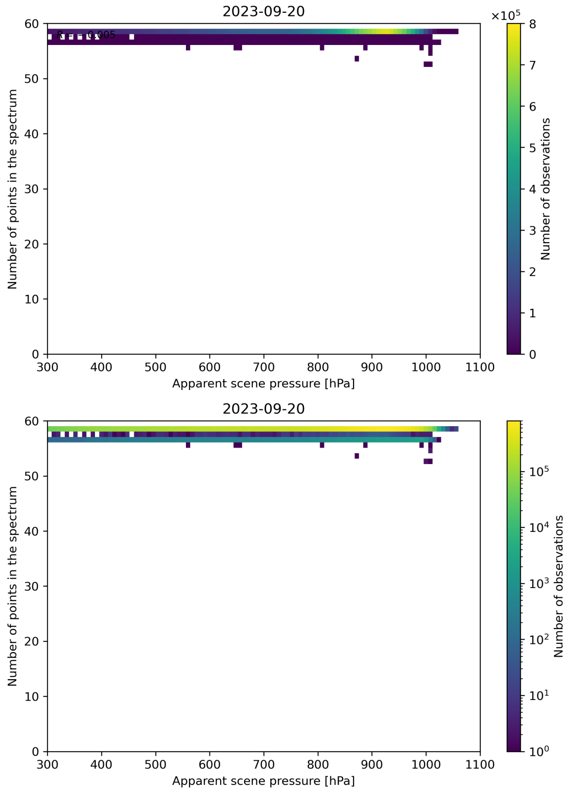
Figure 67: Scatter density plot of “Apparent scene pressure” against “Number of points in the spectrum” for 2023-09-20 to 2023-09-21.
