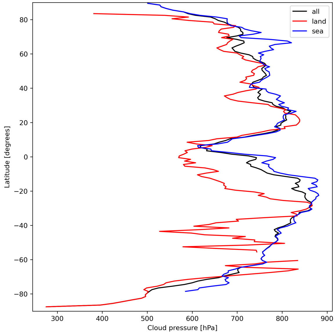
Figure 13: Zonal average of “Cloud pressure” for 2023-09-20 to 2023-09-21.
