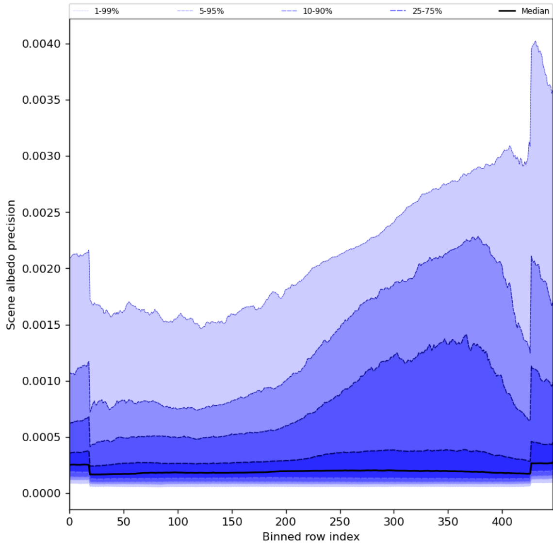
Figure 52: Along track statistics of “Scene albedo precision” for 2023-09-20 to 2023-09-21
