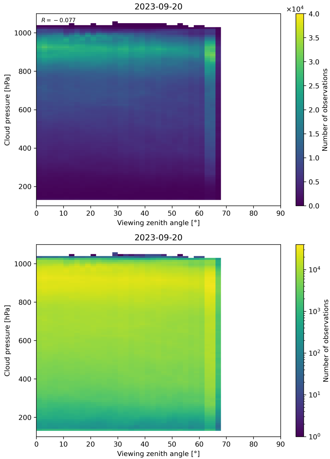
Figure 133: Scatter density plot of “Viewing zenith angle” against “Cloud pressure” for 2023-09-20 to 2023-09-21.
