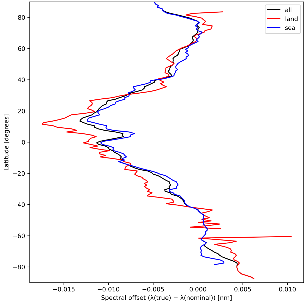
Figure 28: Zonal average of “Spectral offset ( \lambda(\text{true}) - \lambda(\text{nominal}) )” for 2023-09-20 to 2023-09-21.
