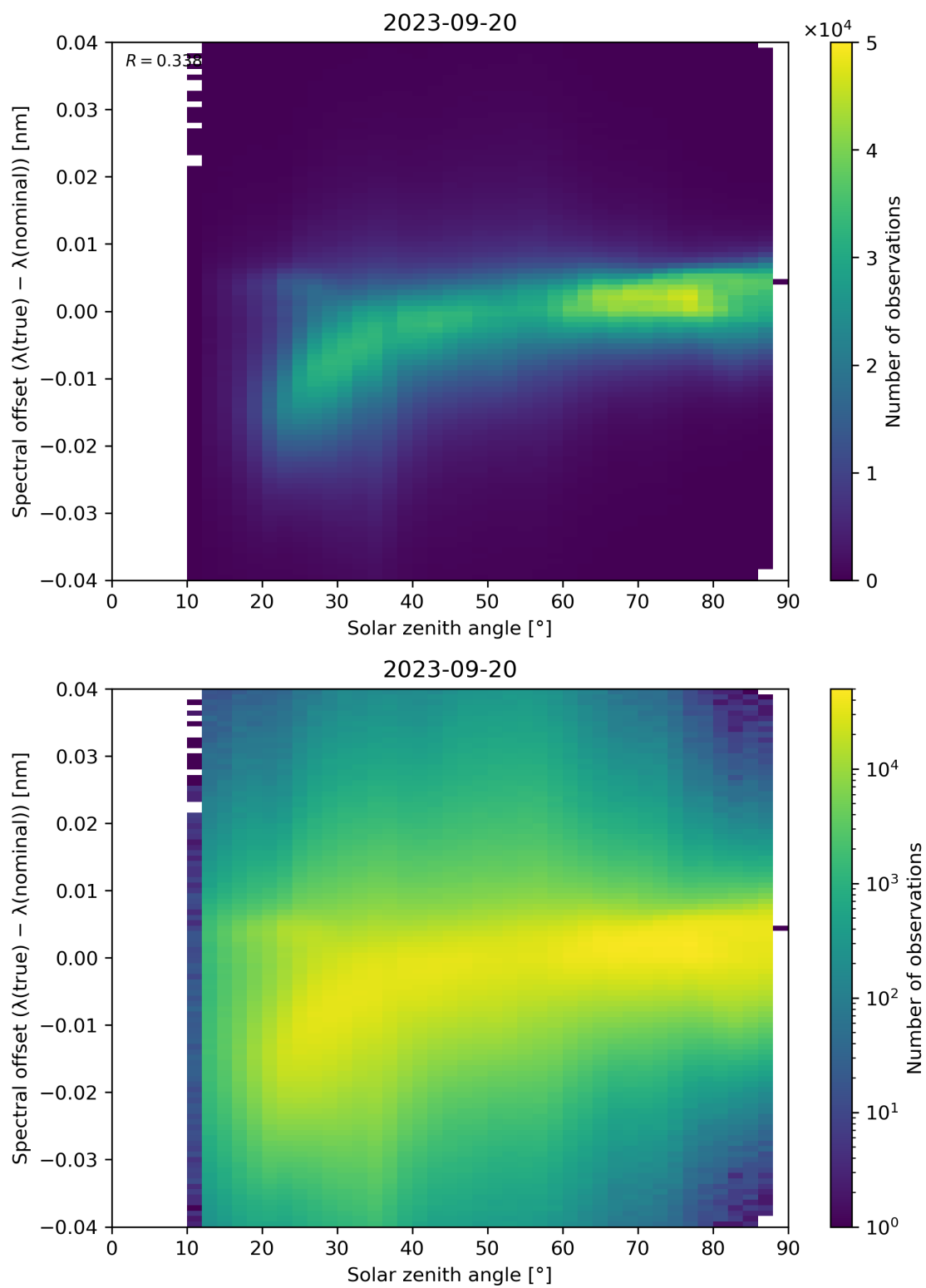
Figure 128: Scatter density plot of “Solar zenith angle” against “Spectral offset ( \lambda(\text{true}) - \lambda(\text{nominal}) )” for 2023-09-20 to 2023-09-21.
