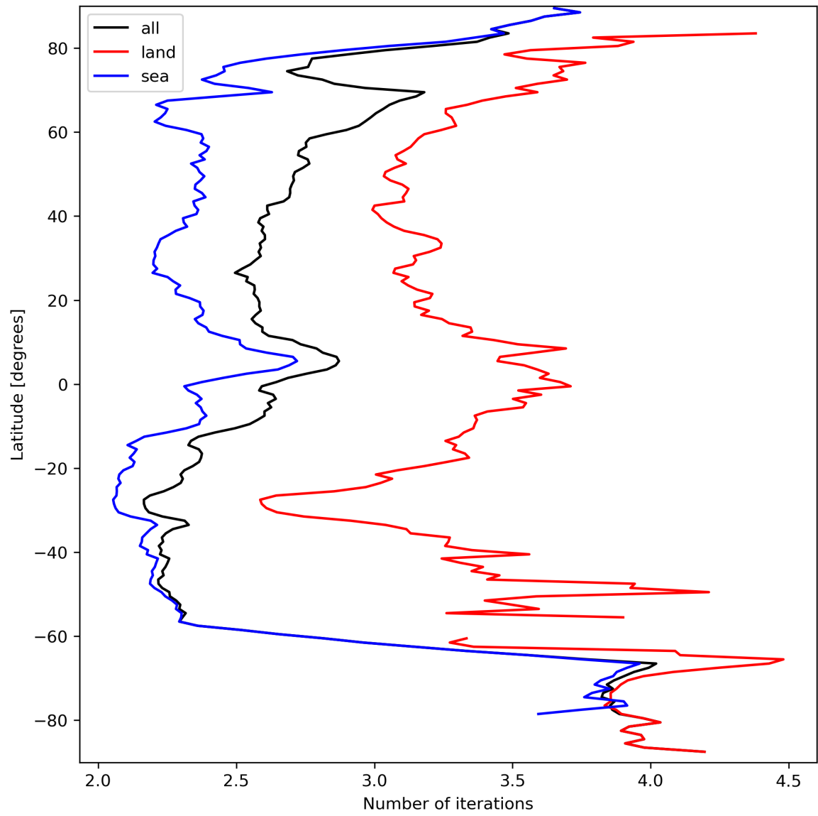
Figure 22: Zonal average of “Number of iterations” for 2023-09-20 to 2023-09-21.
