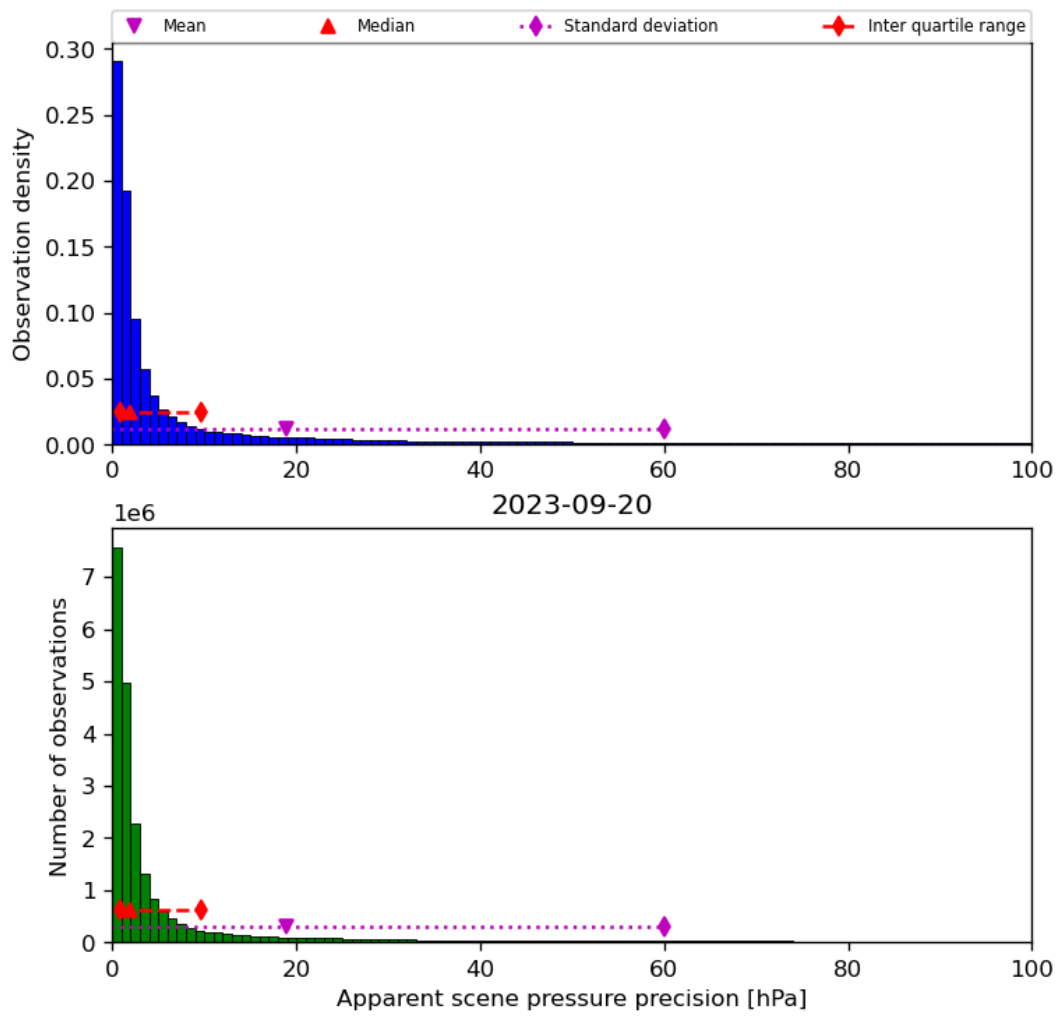
Figure 37: Histogram of “Apparent scene pressure precision” for 2023-09-20 to 2023-09-21
