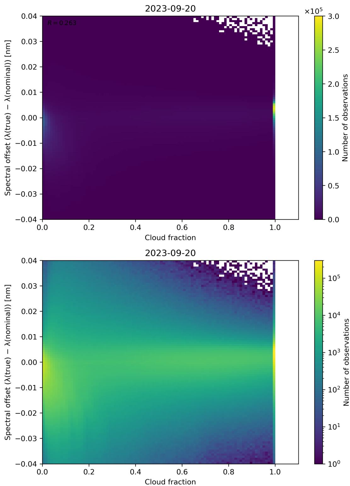
Figure 83: Scatter density plot of “Cloud fraction” against “Spectral offset ( \lambda(\text{true}) - \lambda(\text{nominal}) )” for 2023-09-20 to 2023-09-21.
