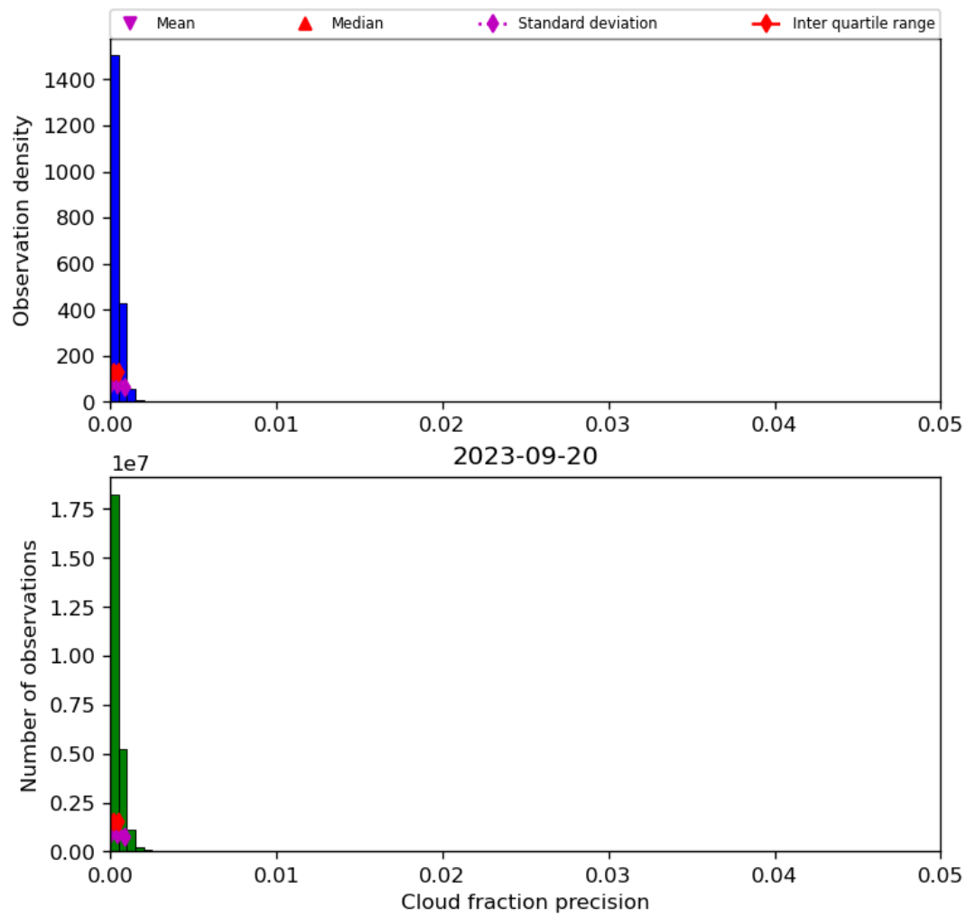
Figure 33: Histogram of “Cloud fraction precision” for 2023-09-20 to 2023-09-21
