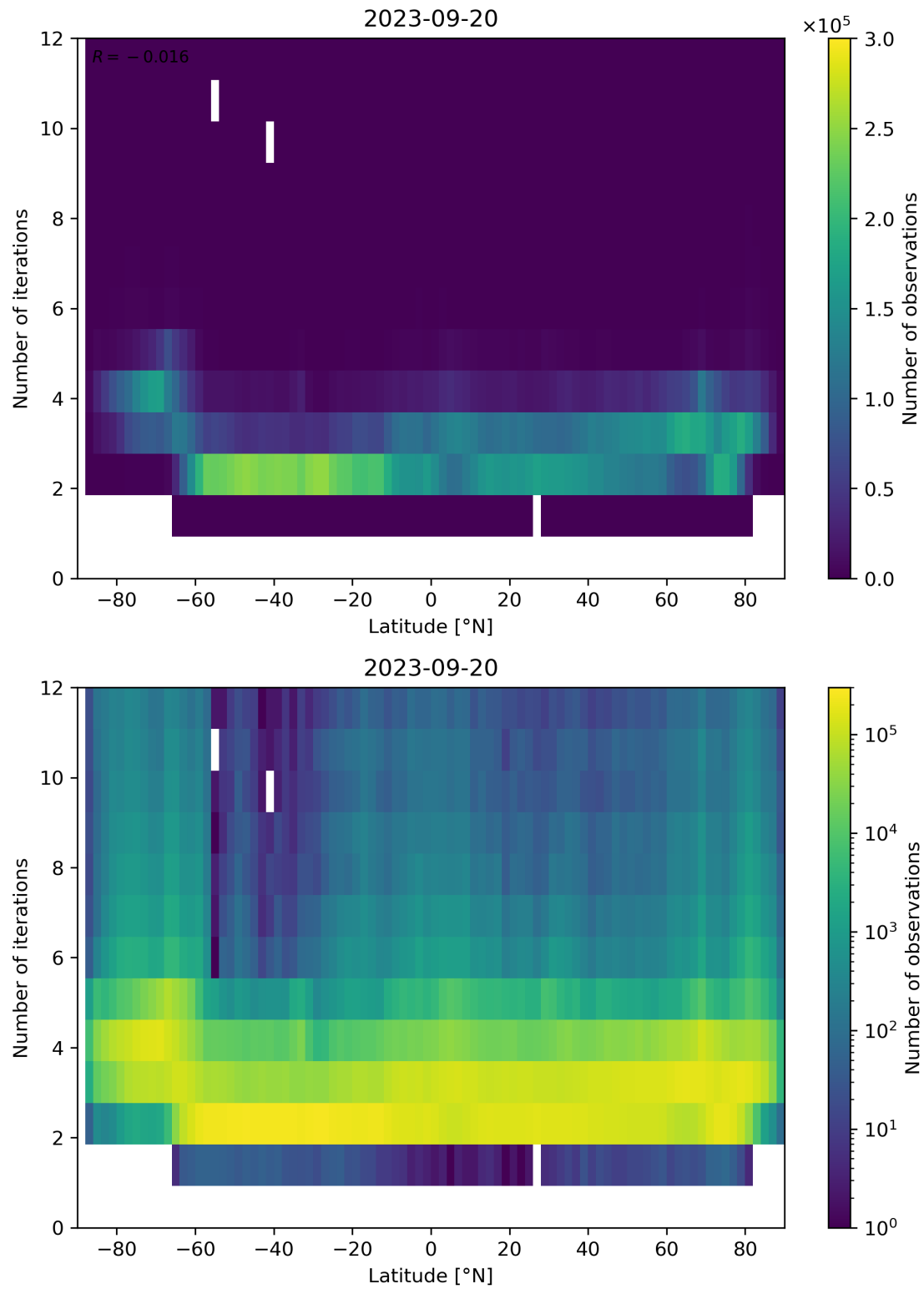
Figure 102: Scatter density plot of “Latitude” against “Number of iterations” for 2023-09-20 to 2023-09-21.
