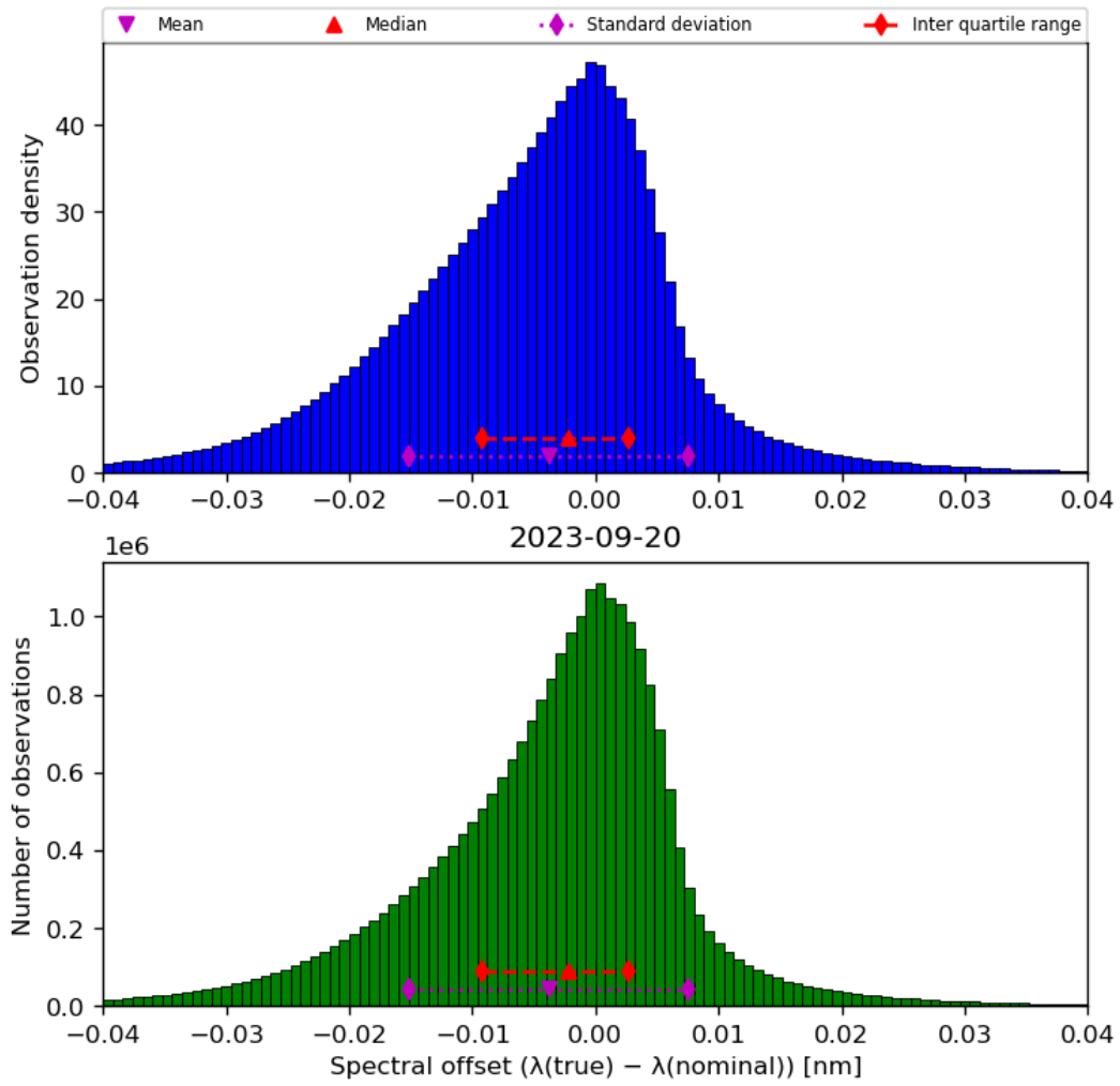
Figure 45: Histogram of “Spectral offset ( \lambda(\text{true}) - \lambda(\text{nominal}) )” for 2023-09-20 to 2023-09-21
