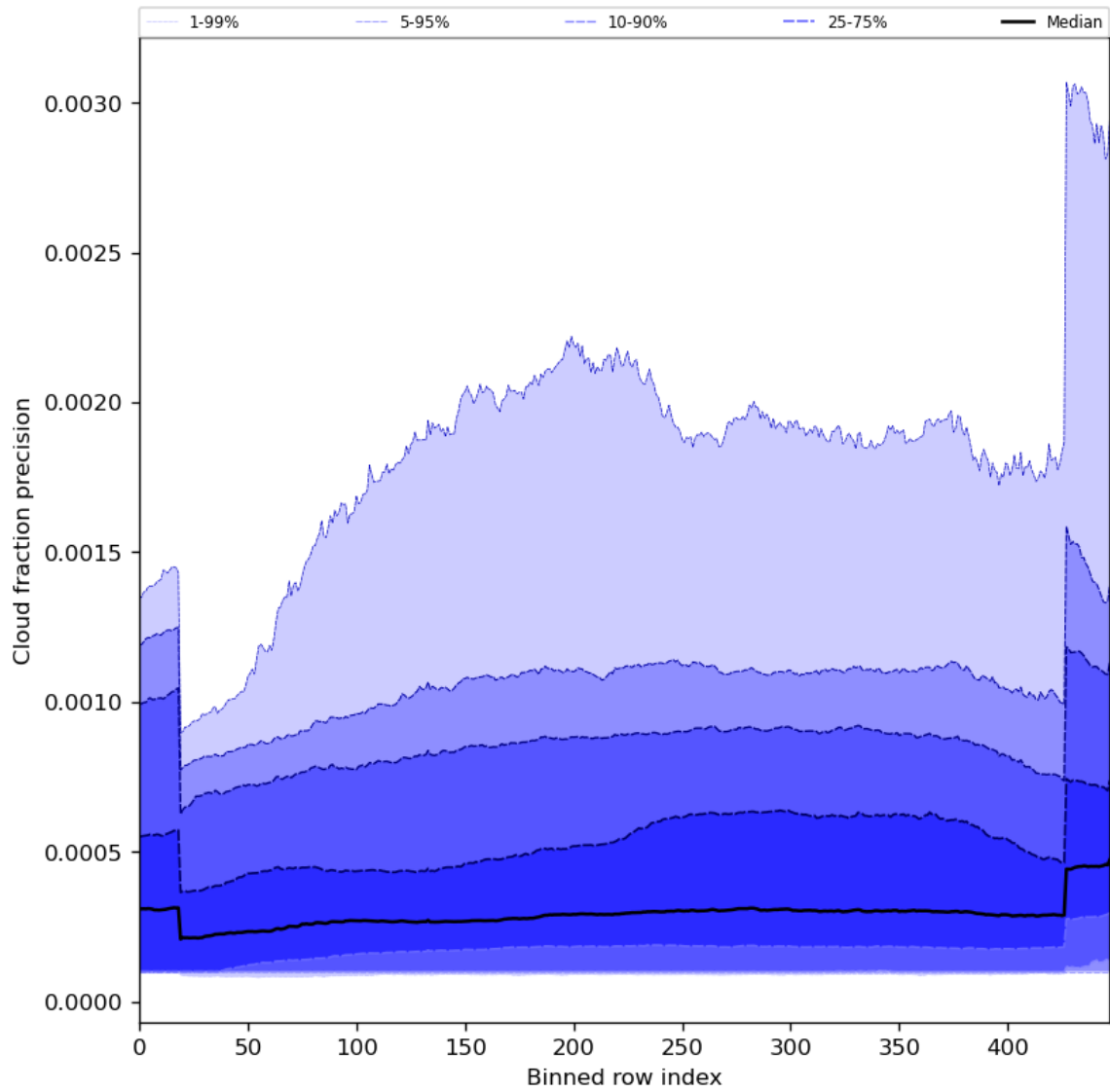
Figure 50: Along track statistics of “Cloud fraction precision” for 2023-09-20 to 2023-09-21
