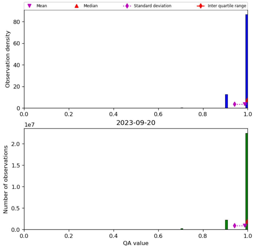
Figure 29: Histogram of “QA value” for 2023-09-20 to 2023-09-21
