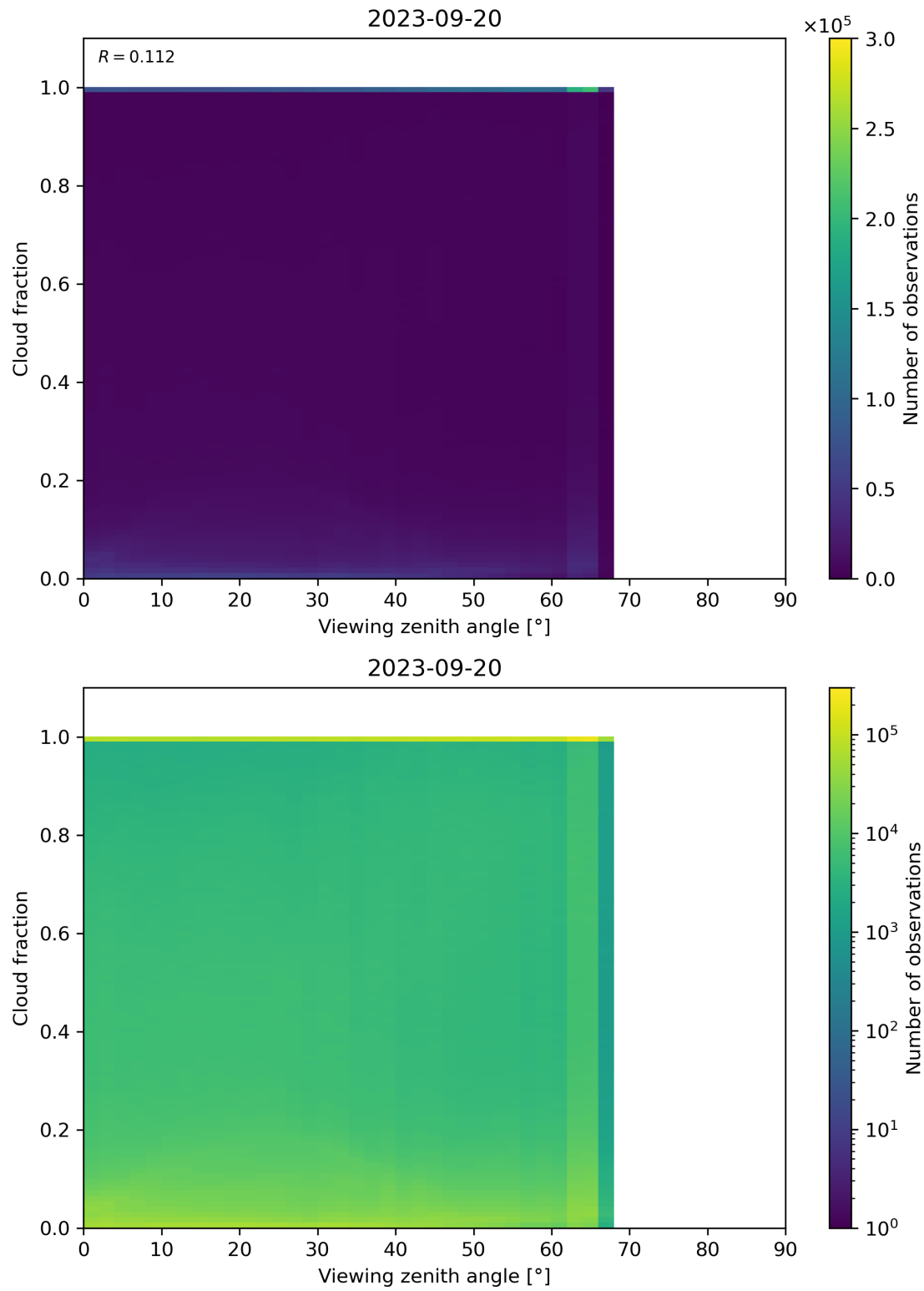
Figure 132: Scatter density plot of “Viewing zenith angle” against “Cloud fraction” for 2023-09-20 to 2023-09-21.
