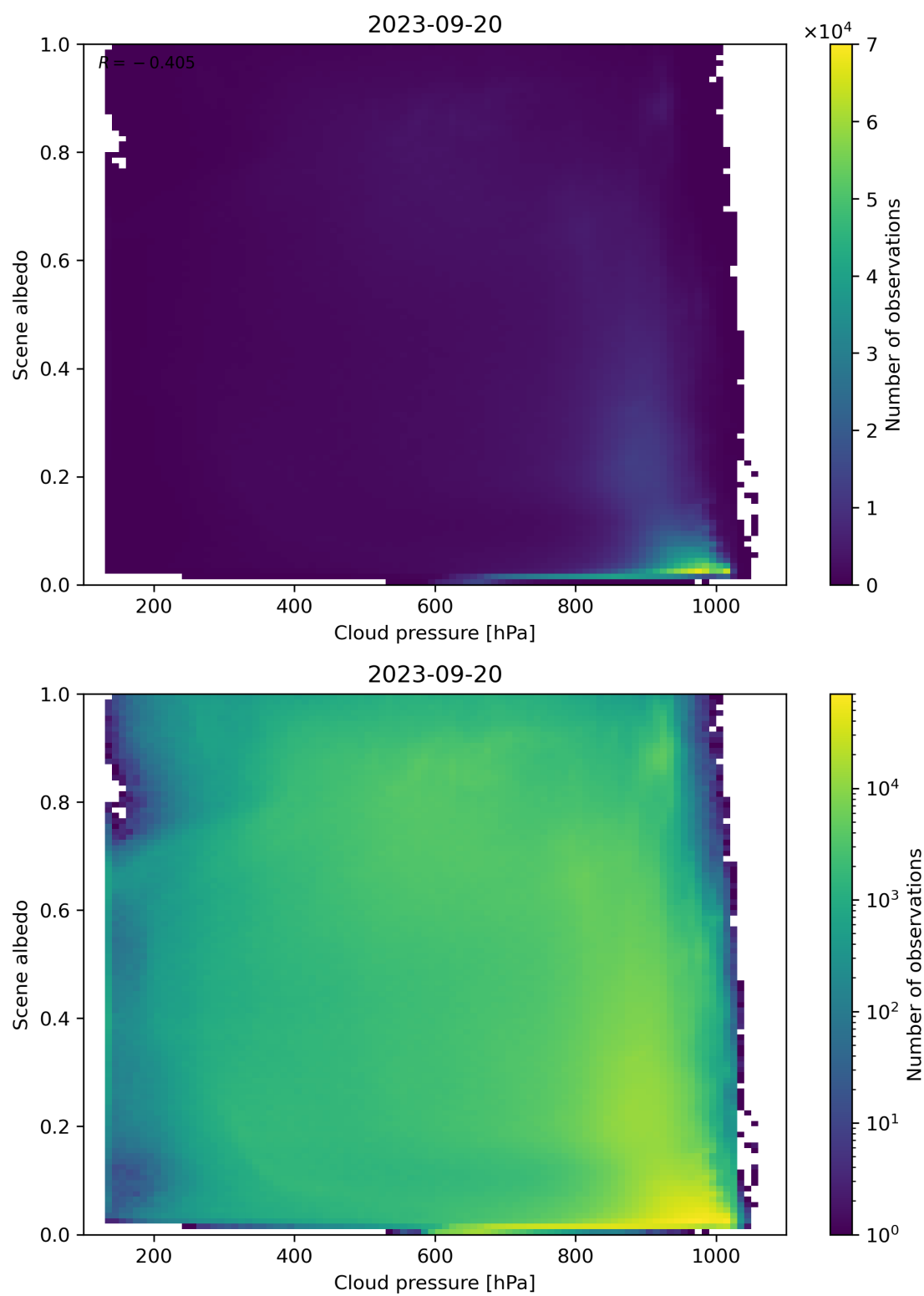
Figure 91: Scatter density plot of “Cloud pressure” against “Scene albedo” for 2023-09-20 to 2023-09-21.
