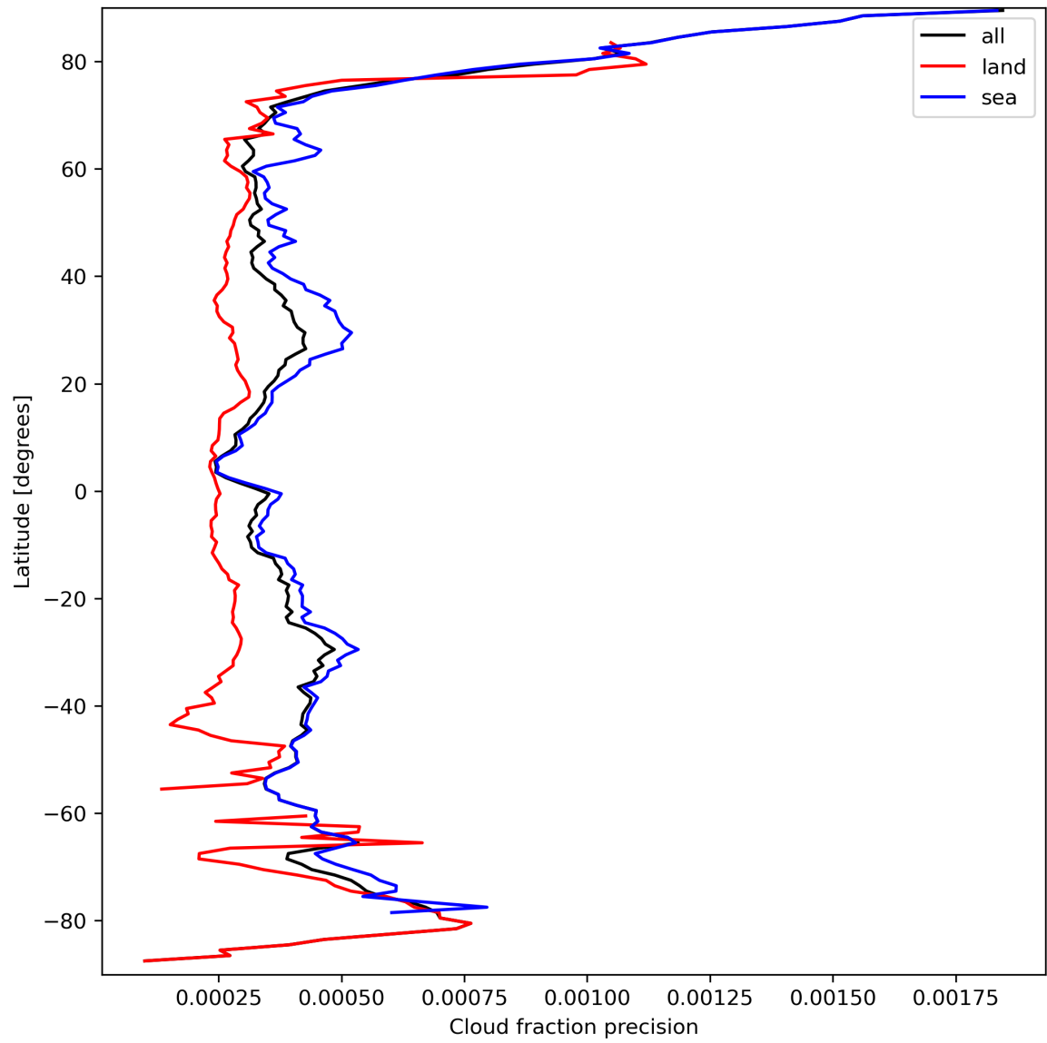
Figure 16: Zonal average of “Cloud fraction precision” for 2023-09-20 to 2023-09-21.
