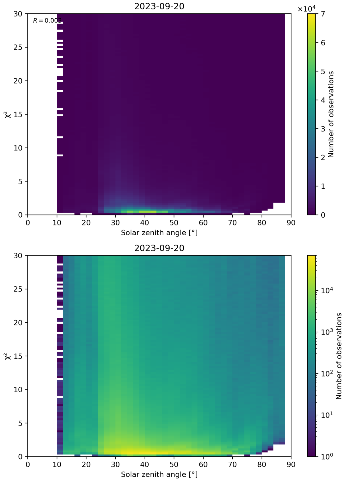
Figure 119: Scatter density plot of “Solar zenith angle” against “ \chi^2 ” for 2023-09-20 to 2023-09-21.
