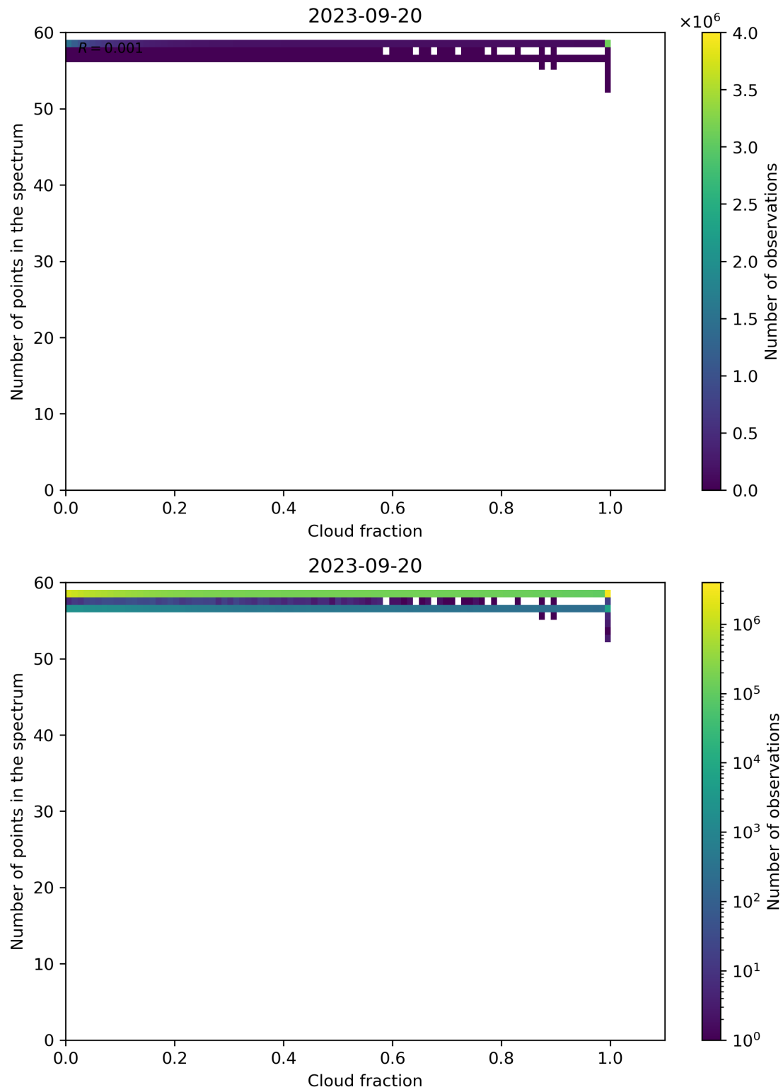
Figure 81: Scatter density plot of “Cloud fraction” against “Number of points in the spectrum” for 2023-09-20 to 2023-09-21.
