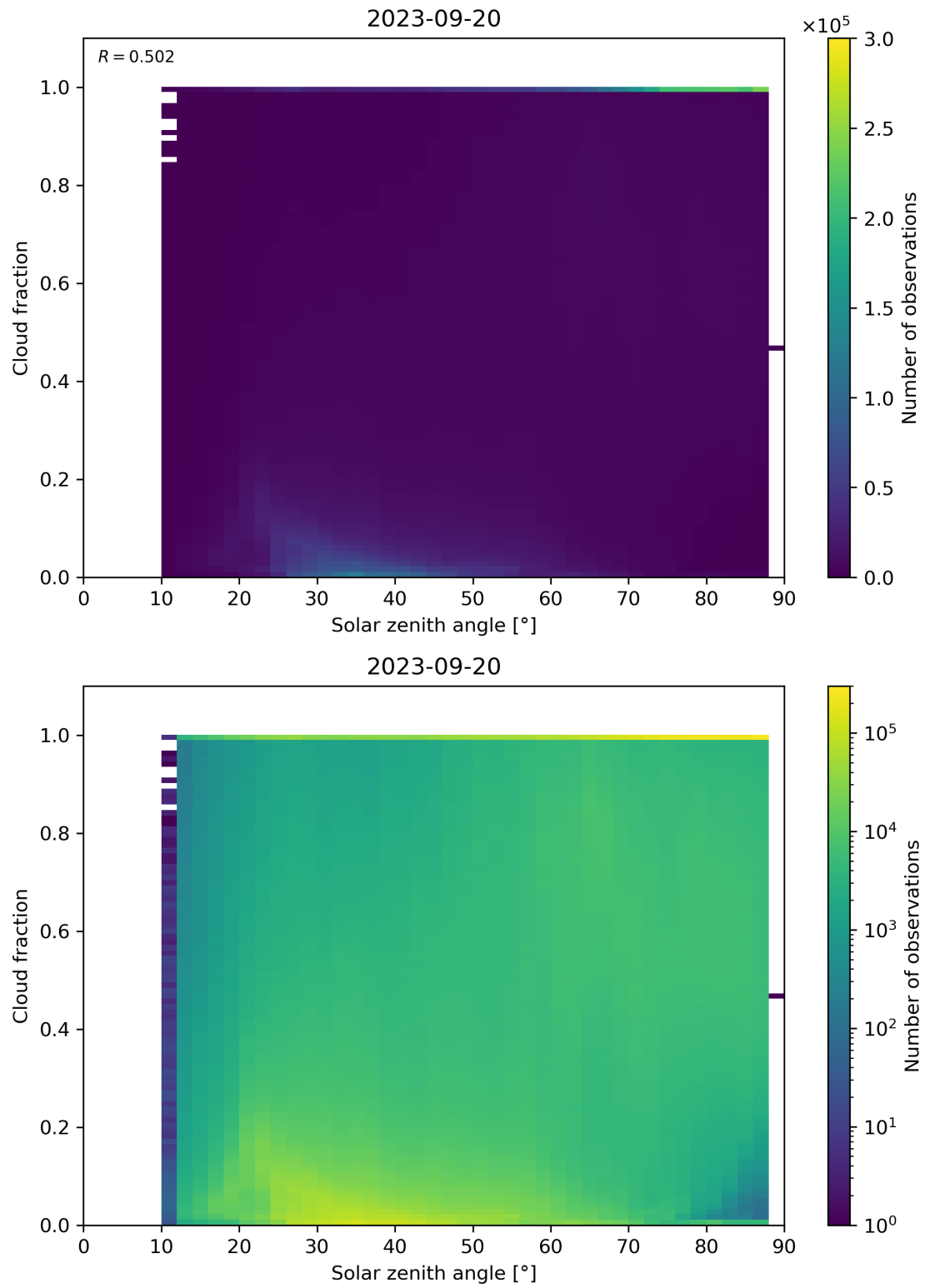
Figure 121: Scatter density plot of “Solar zenith angle” against “Cloud fraction” for 2023-09-20 to 2023-09-21.
