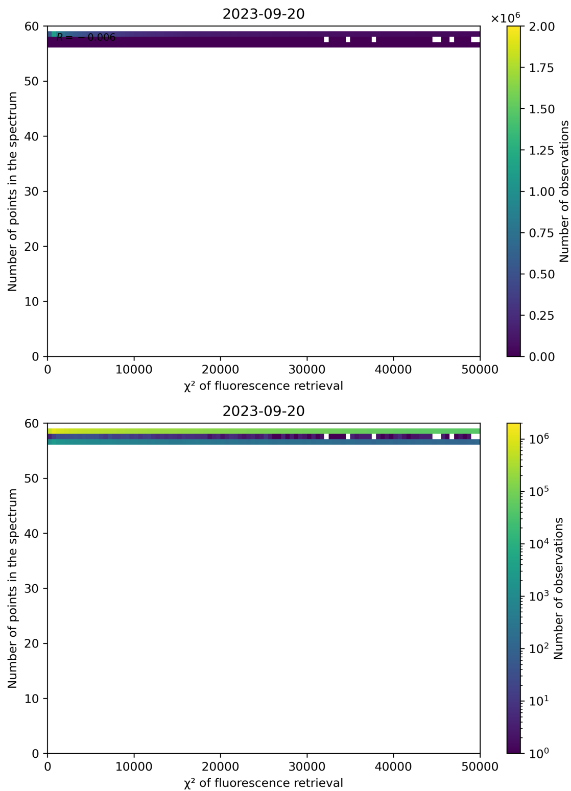
Figure 71: Scatter density plot of " \chi^2 of fluorescence retrieval" against "Number of points in the spectrum" for 2023-09-20 to 2023-09-21.
