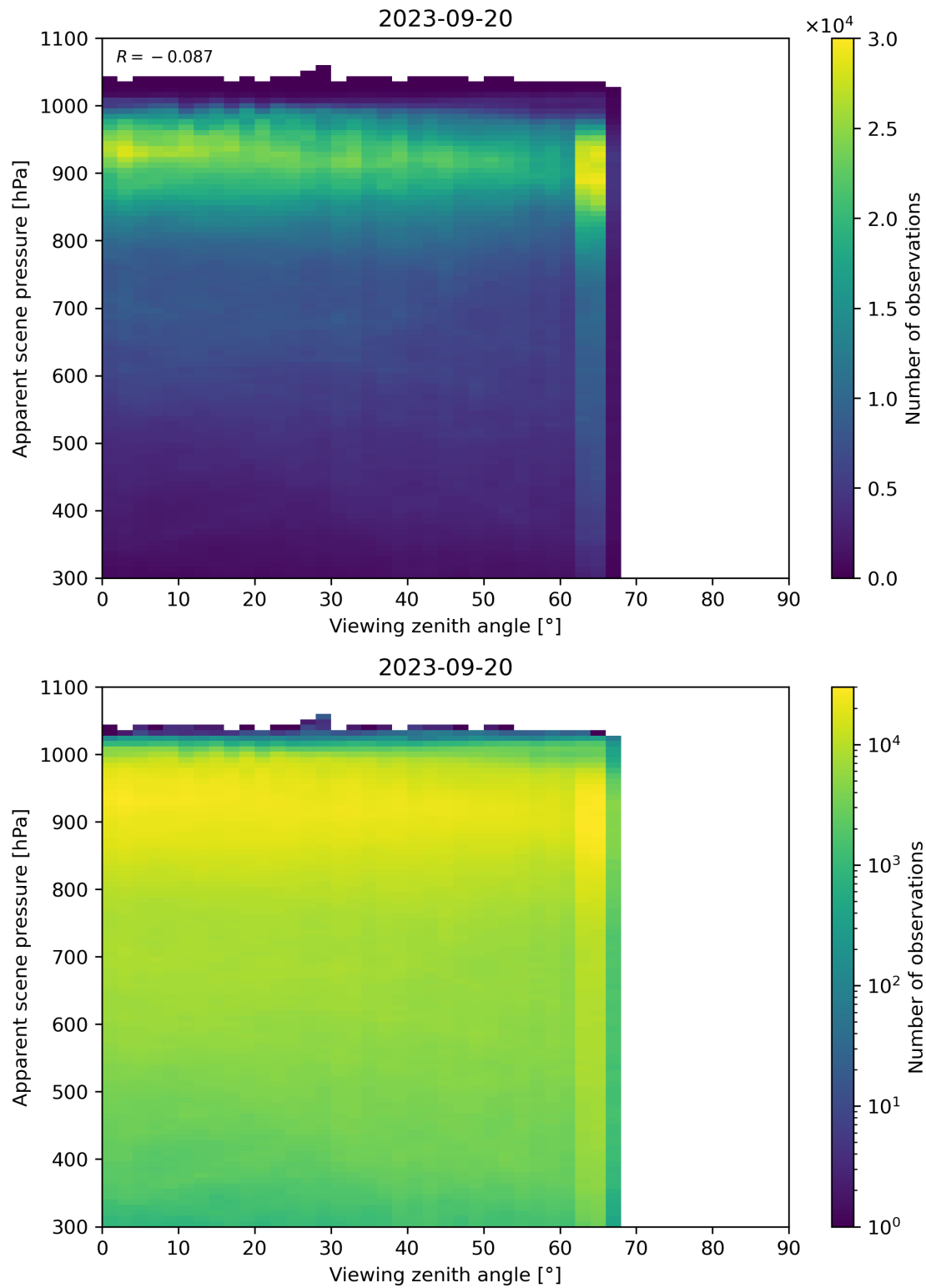
Figure 129: Scatter density plot of “Viewing zenith angle” against “Apparent scene pressure” for 2023-09-20 to 2023-09-21.
