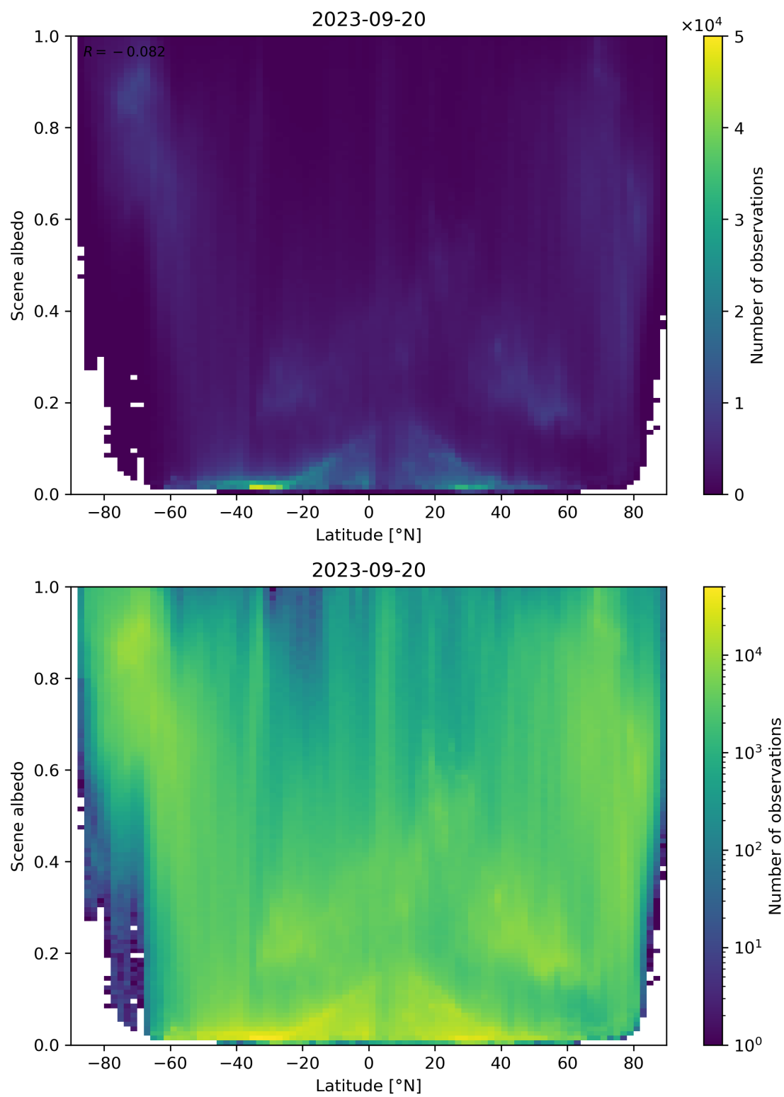
Figure 104: Scatter density plot of “Latitude” against “Scene albedo” for 2023-09-20 to 2023-09-21.
