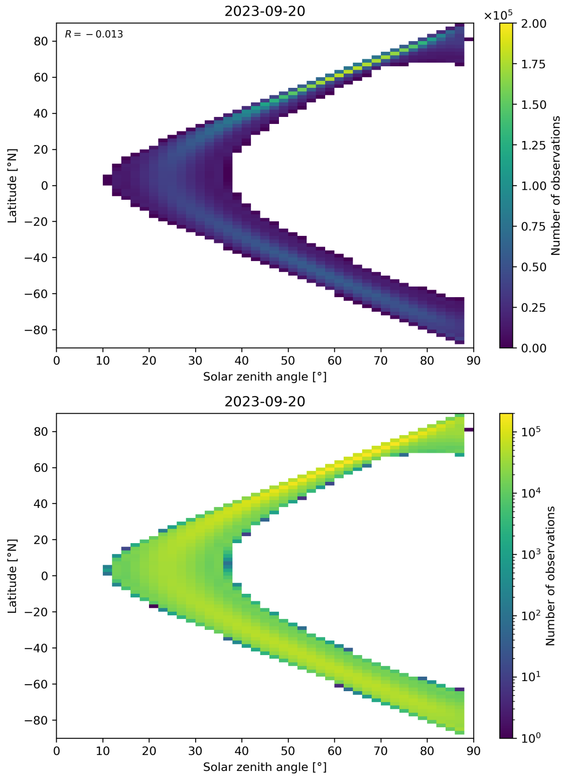
Figure 124: Scatter density plot of “Solar zenith angle” against “Latitude” for 2023-09-20 to 2023-09-21.
