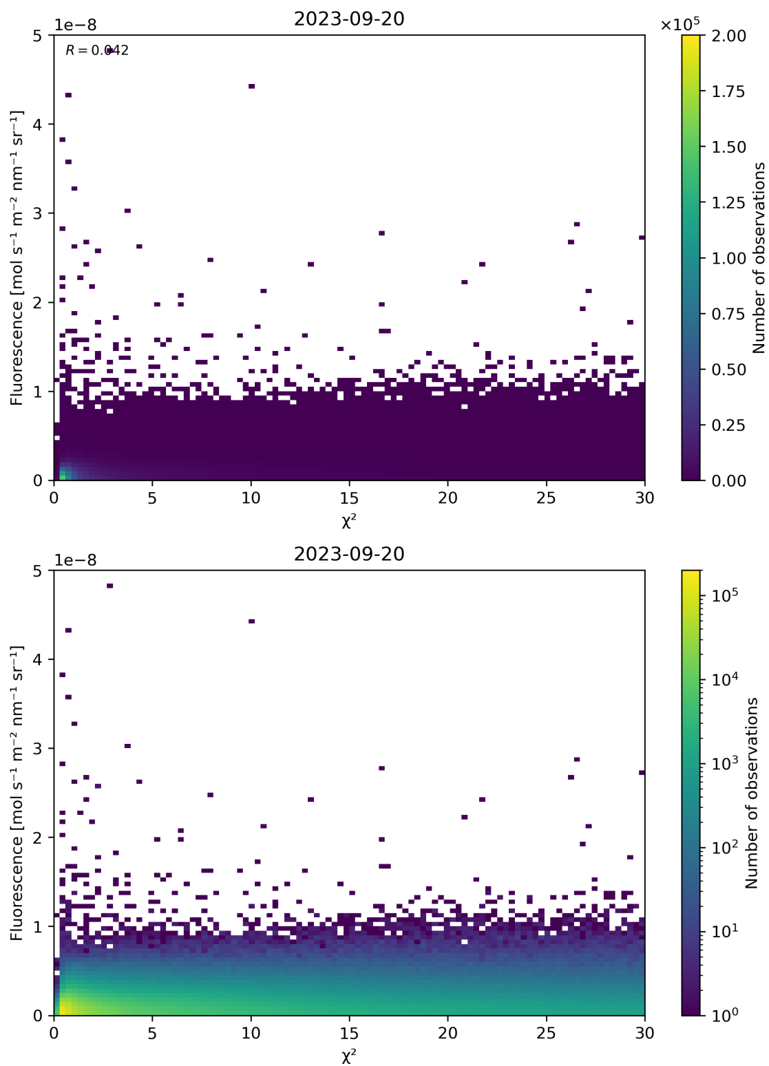
Figure 70: Scatter density plot of “ \chi^2 ” against “Fluorescence” for 2023-09-20 to 2023-09-21.
