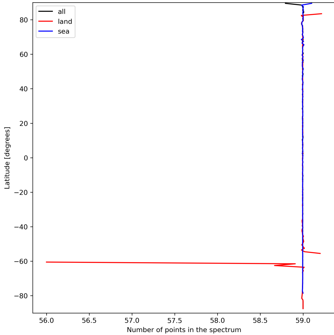
Figure 27: Zonal average of “Number of points in the spectrum” for 2023-09-20 to 2023-09-21.
