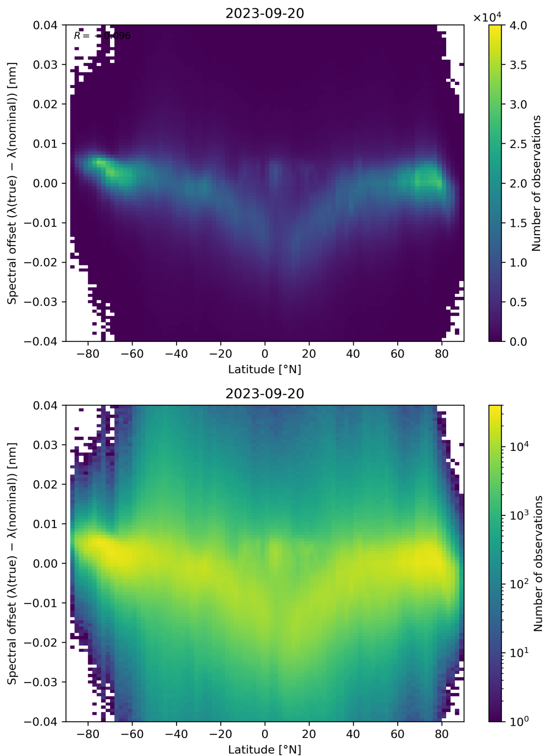
Figure 105: Scatter density plot of “Latitude” against “Spectral offset ( \lambda(\text{true}) - \lambda(\text{nominal}) )” for 2023-09-20 to 2023-09-21.
