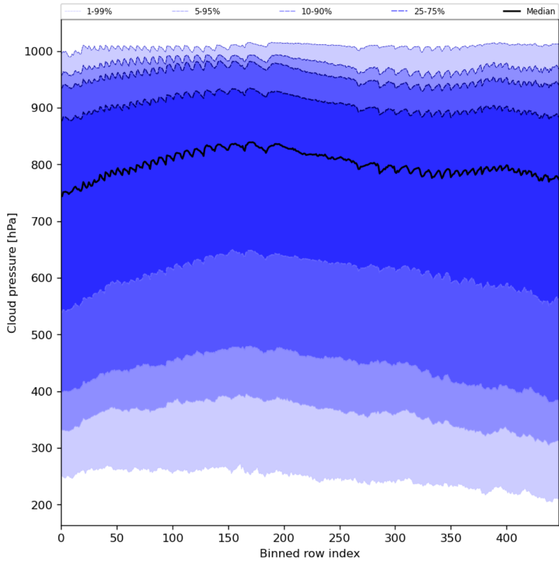
Figure 47: Along track statistics of “Cloud pressure” for 2023-09-20 to 2023-09-21
