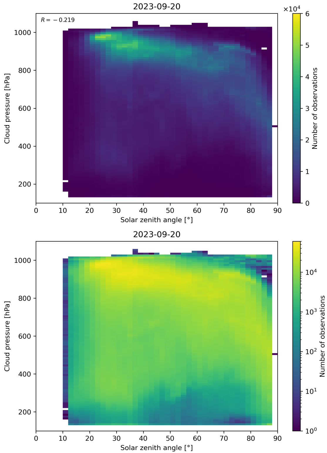
Figure 122: Scatter density plot of “Solar zenith angle” against “Cloud pressure” for 2023-09-20 to 2023-09-21.
