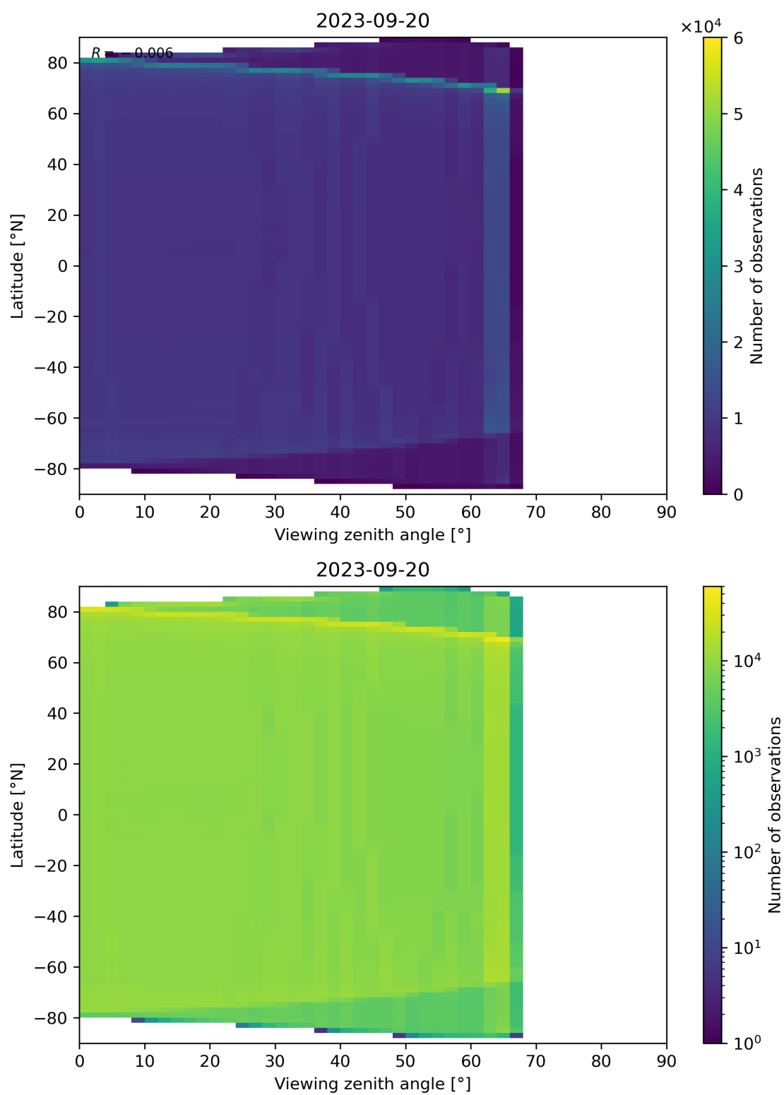
Figure 135: Scatter density plot of “Viewing zenith angle” against “Latitude” for 2023-09-20 to 2023-09-21.
