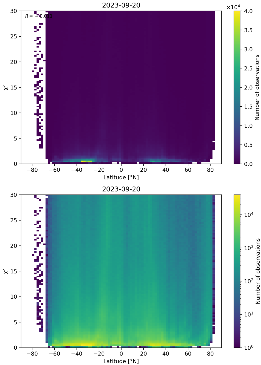
Figure 97: Scatter density plot of “Latitude” against “ \chi^2 ” for 2023-09-20 to 2023-09-21.
