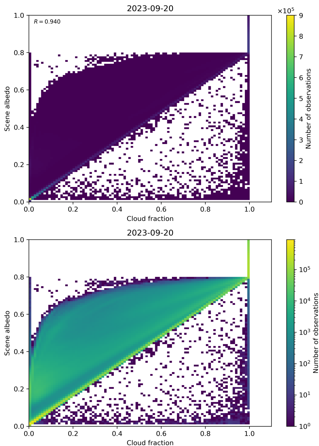
Figure 82: Scatter density plot of “Cloud fraction” against “Scene albedo” for 2023-09-20 to 2023-09-21.
