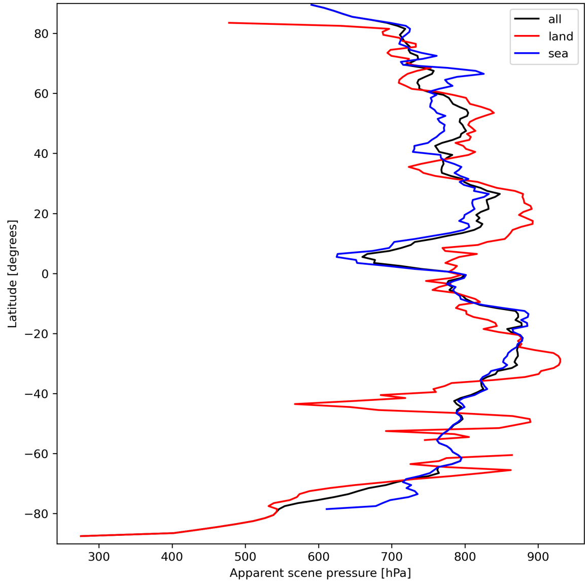
Figure 19: Zonal average of “Apparent scene pressure” for 2023-09-20 to 2023-09-21.
