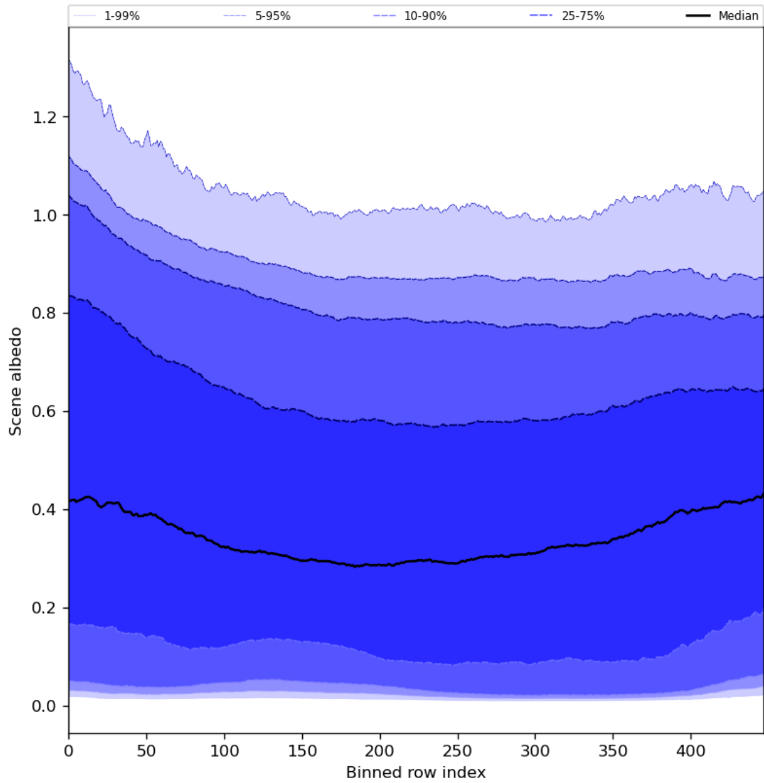
Figure 51: Along track statistics of “Scene albedo” for 2023-09-20 to 2023-09-21
