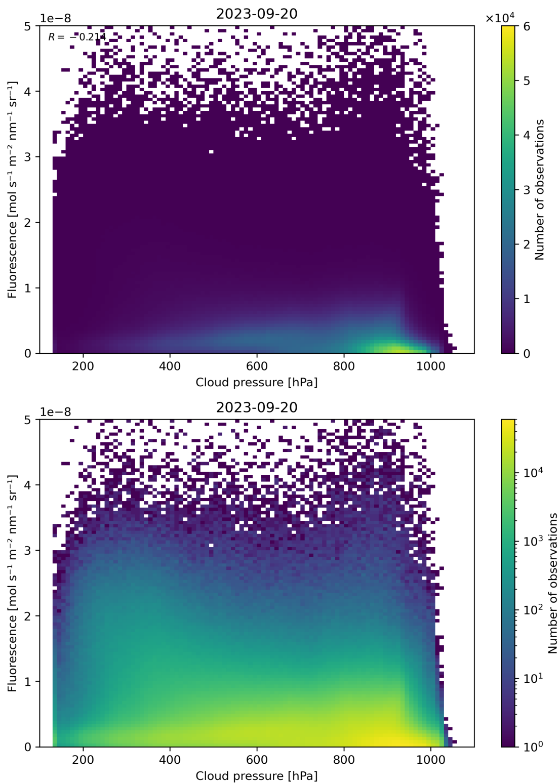
Figure 88: Scatter density plot of “Cloud pressure” against “Fluorescence” for 2023-09-20 to 2023-09-21.
