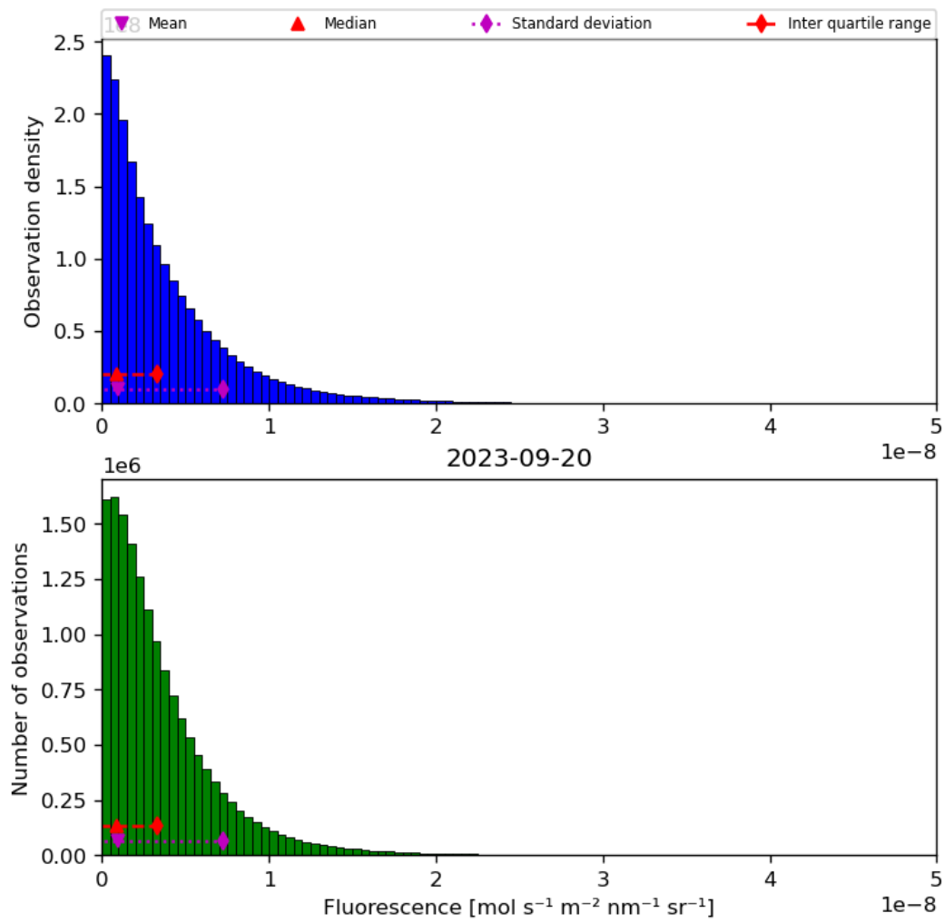
Figure 40: Histogram of “Fluorescence” for 2023-09-20 to 2023-09-21
