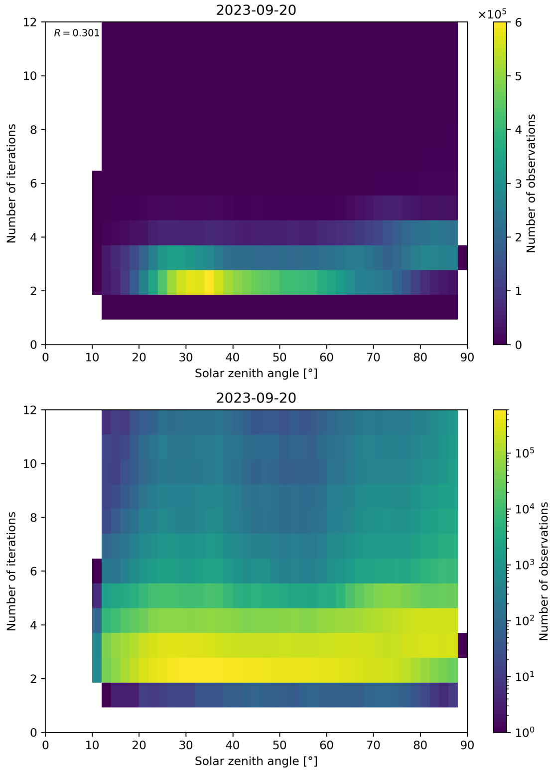
Figure 125: Scatter density plot of “Solar zenith angle” against “Number of iterations” for 2023-09-20 to 2023-09-21.
