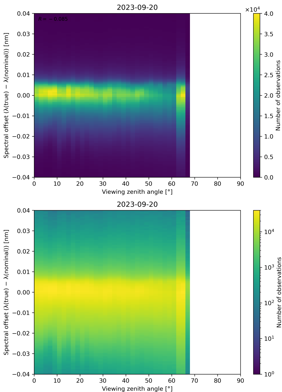
Figure 140: Scatter density plot of “Viewing zenith angle” against “Spectral offset ( \lambda(\text{true}) - \lambda(\text{nominal}) )” for 2023-09-20 to 2023-09-21.
