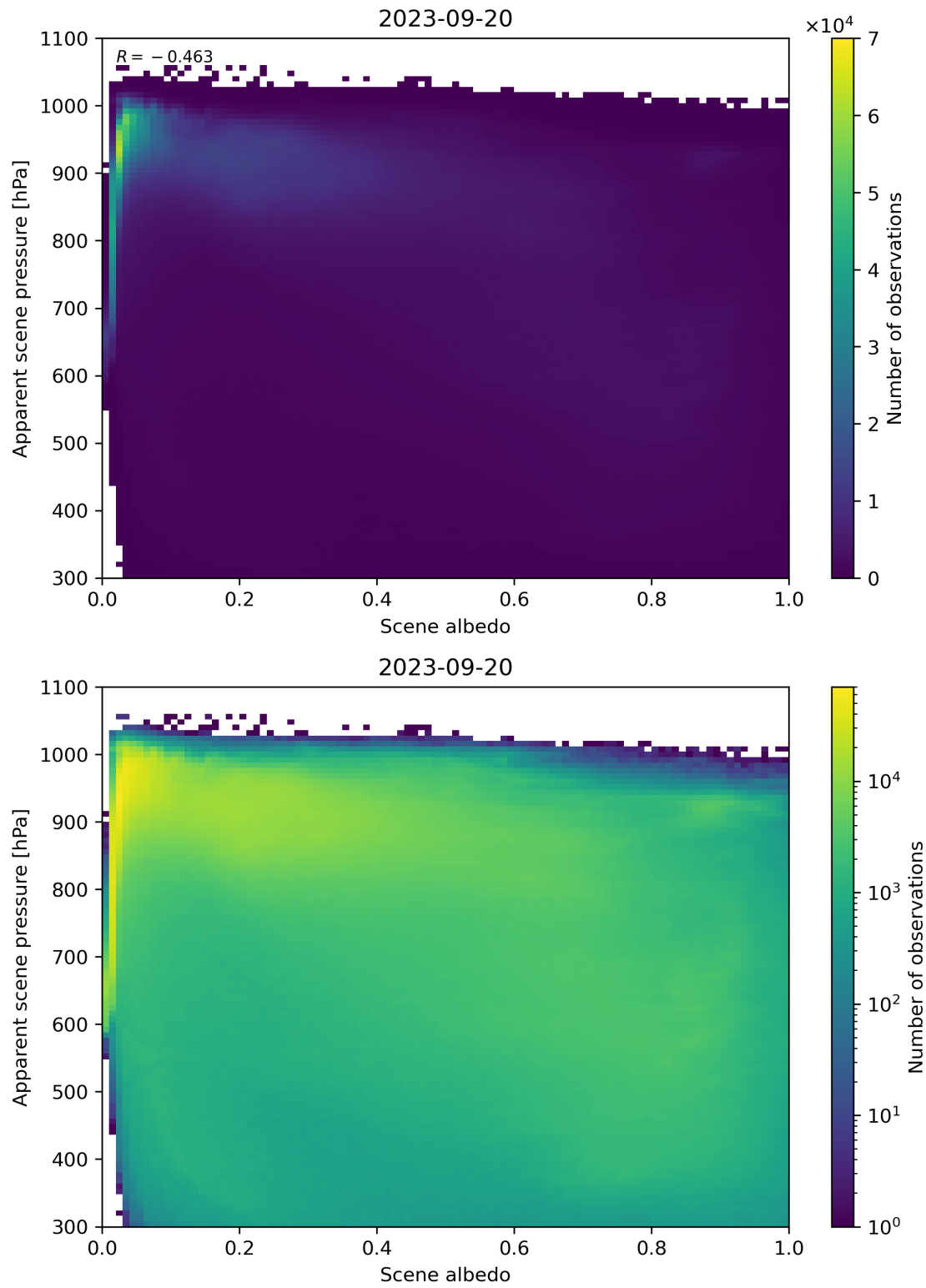
Figure 111: Scatter density plot of “Scene albedo” against “Apparent scene pressure” for 2023-09-20 to 2023-09-21.
