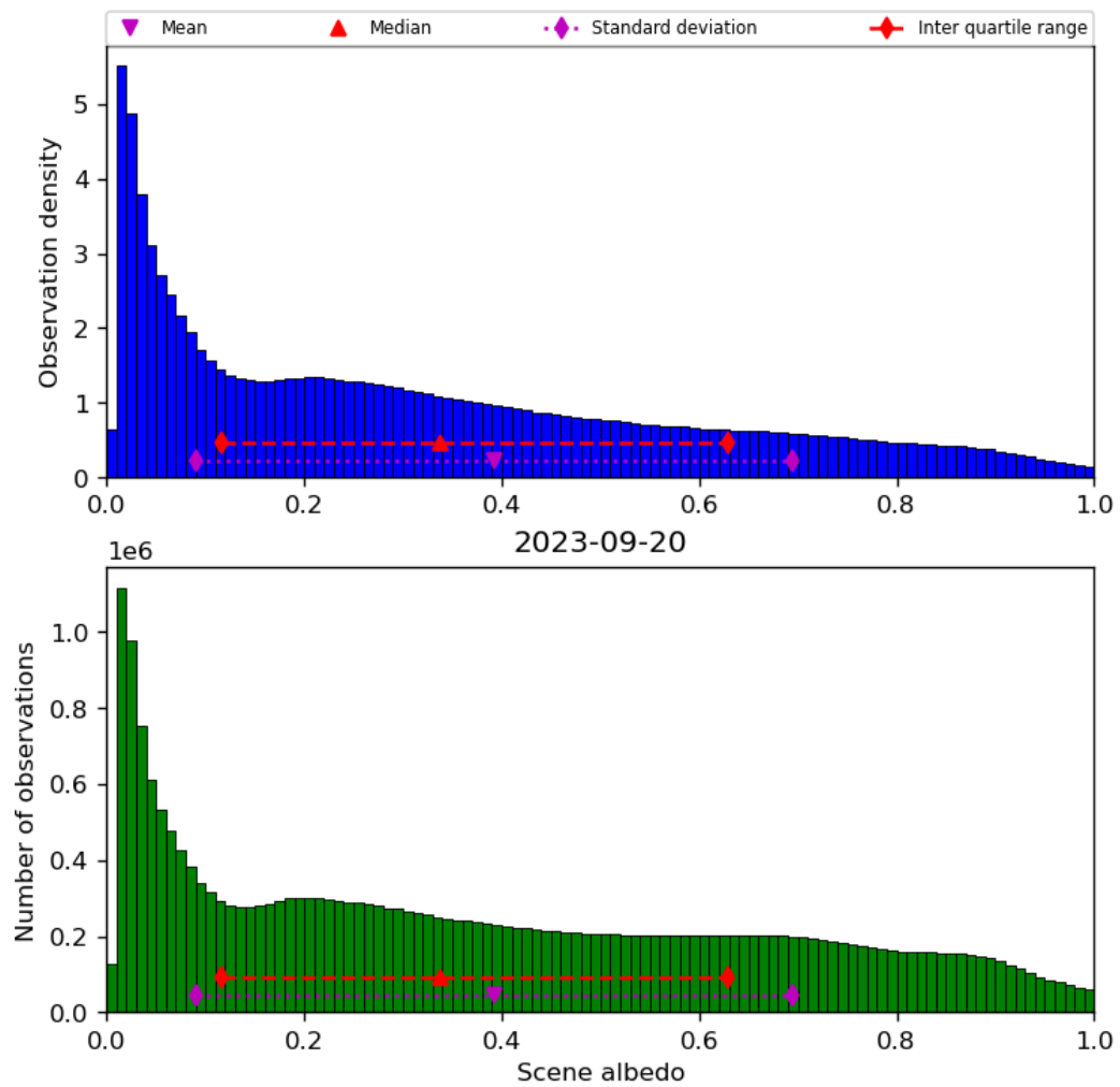
Figure 34: Histogram of “Scene albedo” for 2023-09-20 to 2023-09-21
