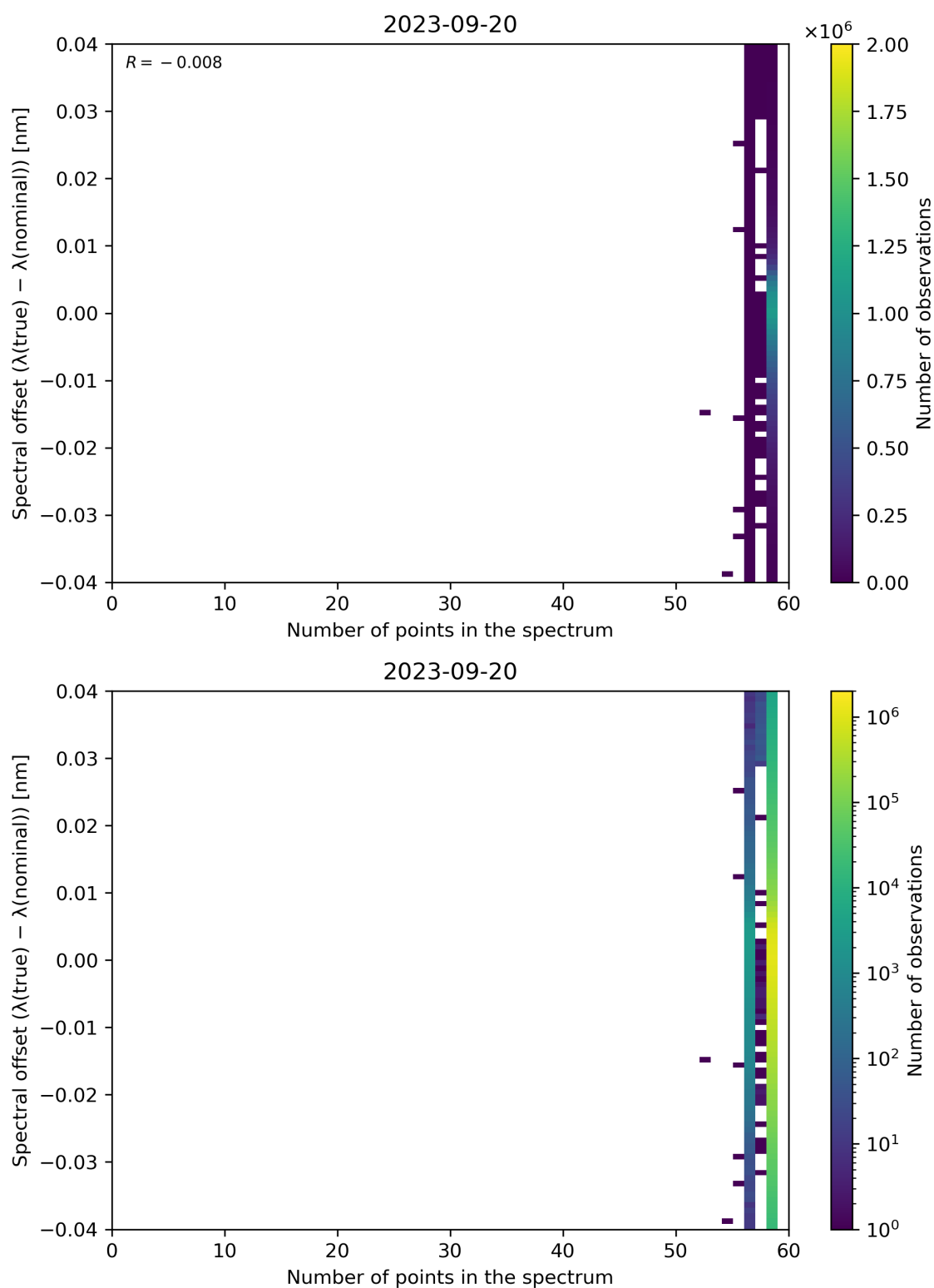
Figure 110: Scatter density plot of “Number of points in the spectrum” against “Spectral offset ( \lambda(\text{true}) - \lambda(\text{nominal}) )” for 2023-09-20 to 2023-09-21.
