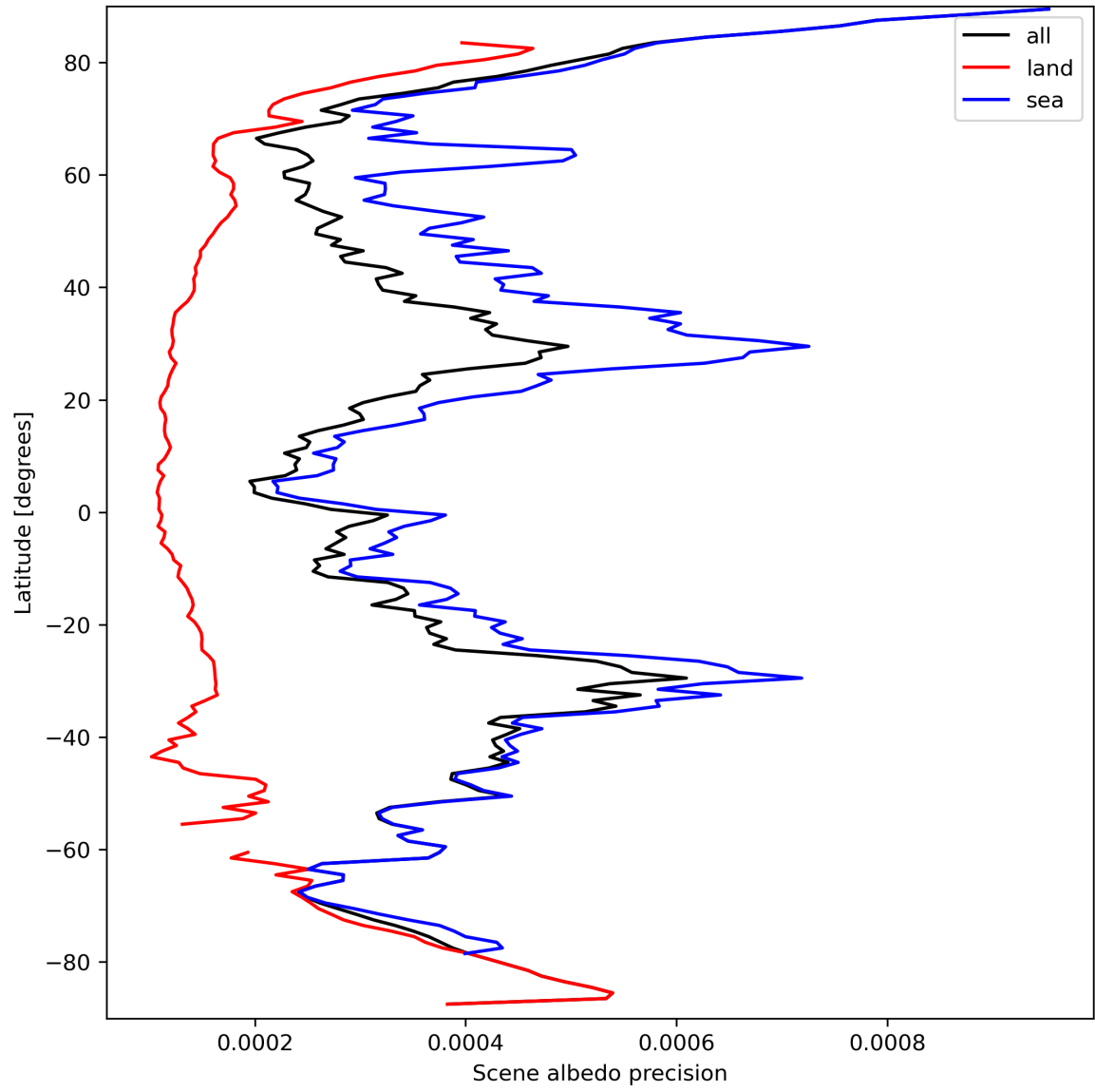
Figure 18: Zonal average of “Scene albedo precision” for 2023-09-20 to 2023-09-21.
