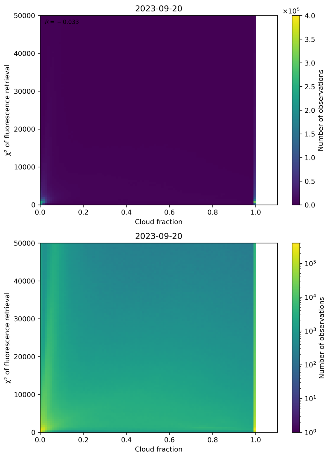
Figure 78: Scatter density plot of “Cloud fraction” against “ \chi^2 of fluorescence retrieval” for 2023-09-20 to 2023-09-21.
