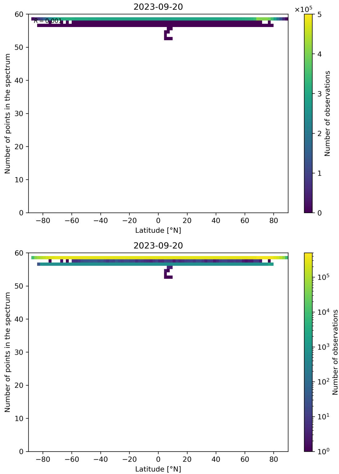
Figure 103: Scatter density plot of “Latitude” against “Number of points in the spectrum” for 2023-09-20 to 2023-09-21.
