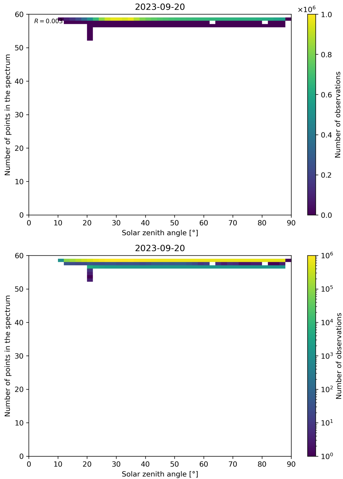
Figure 126: Scatter density plot of “Solar zenith angle” against “Number of points in the spectrum” for 2023-09-20 to 2023-09-21.
