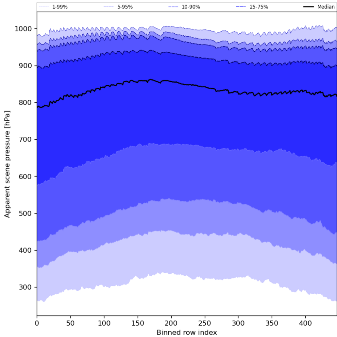
Figure 53: Along track statistics of “Apparent scene pressure” for 2023-09-20 to 2023-09-21
