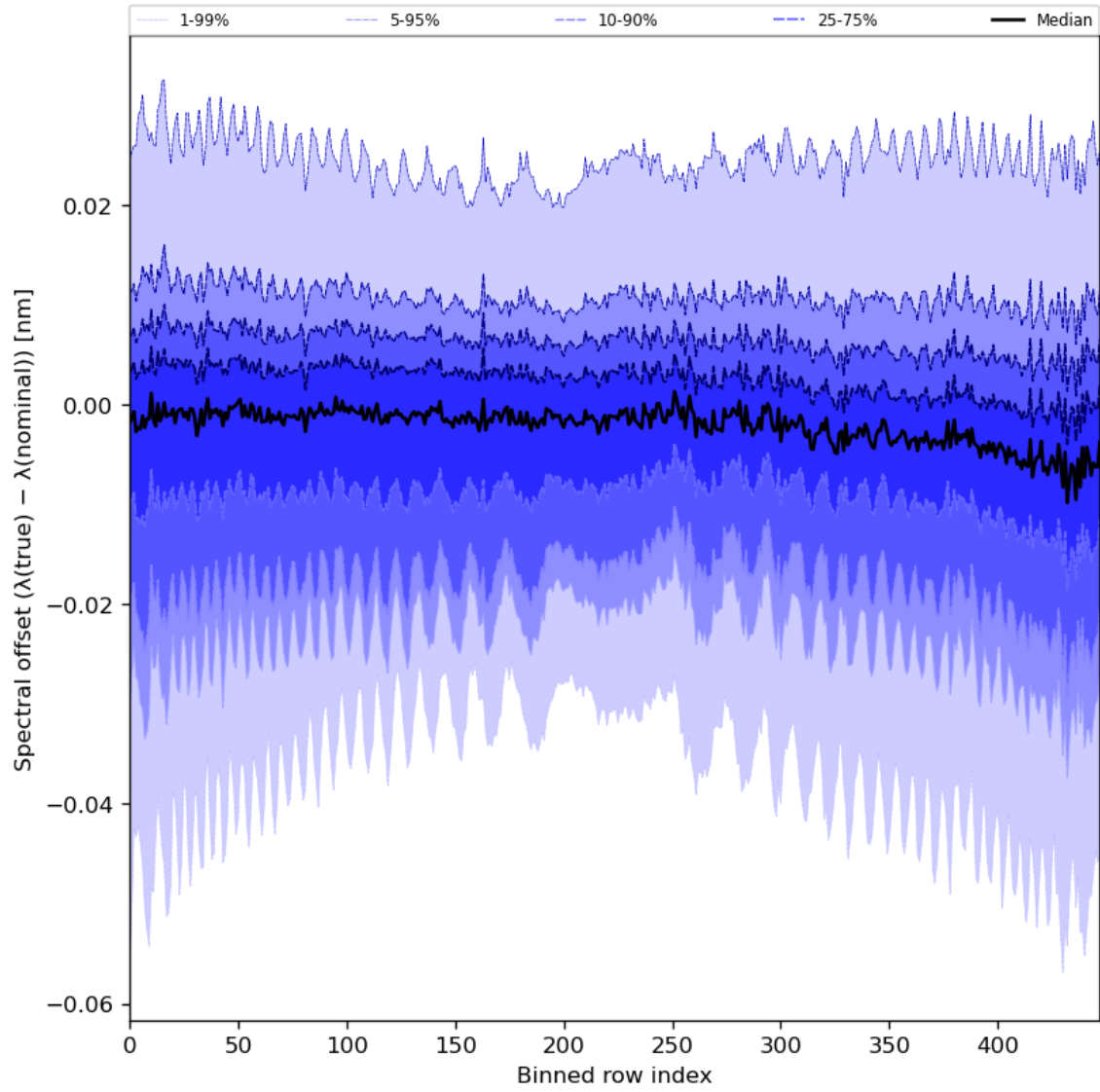
Figure 62: Along track statistics of “Spectral offset ( \lambda(\text{true}) - \lambda(\text{nominal}) )” for 2023-09-20 to 2023-09-21
