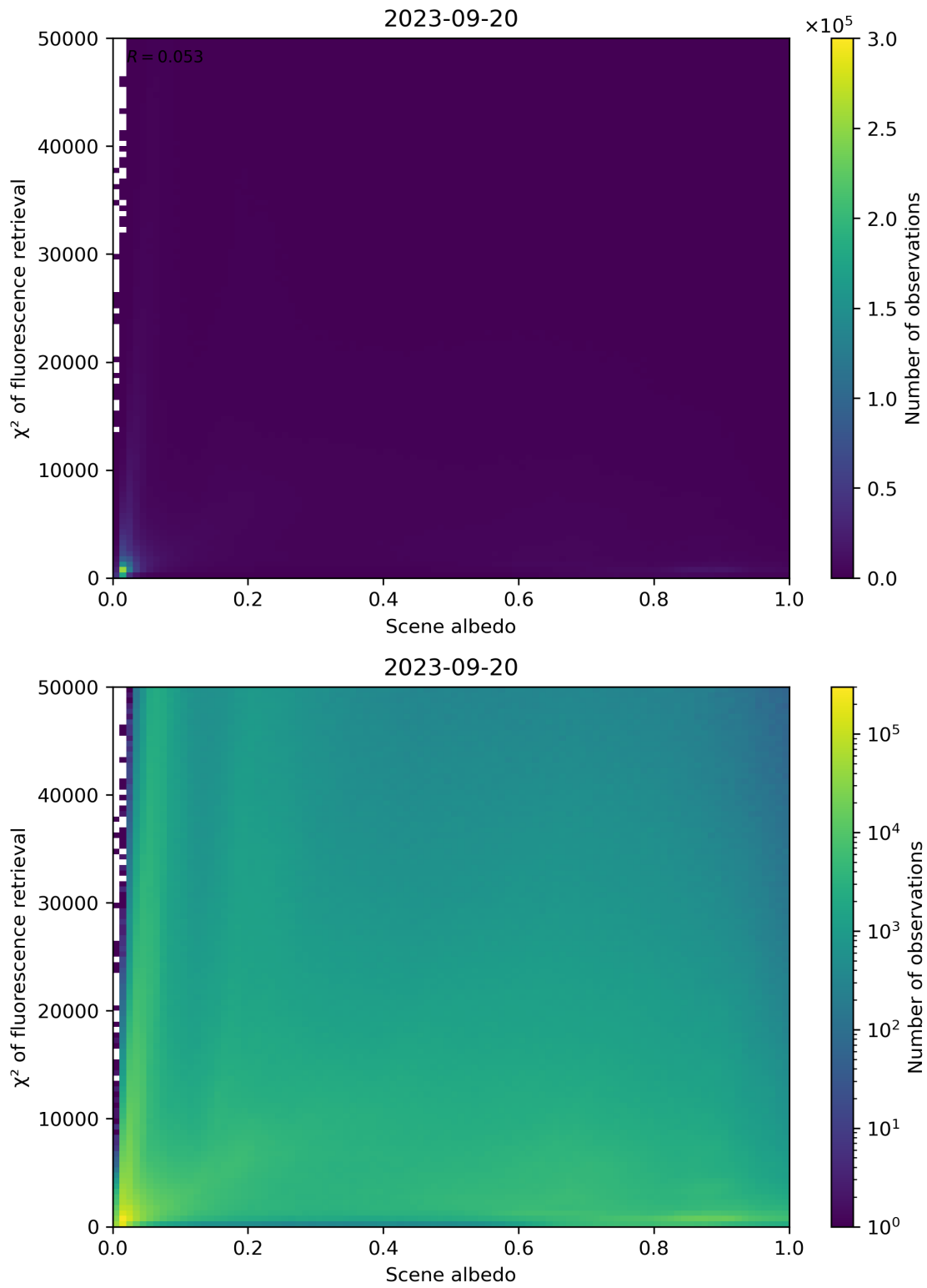
Figure 113: Scatter density plot of “Scene albedo” against “ \chi^2 of fluorescence retrieval” for 2023-09-20 to 2023-09-21.
