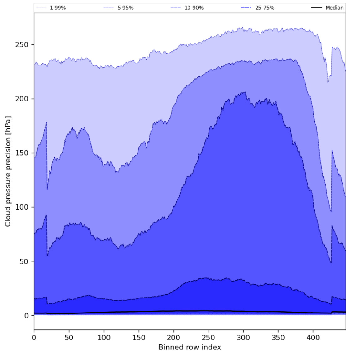
Figure 48: Along track statistics of “Cloud pressure precision” for 2023-09-20 to 2023-09-21
