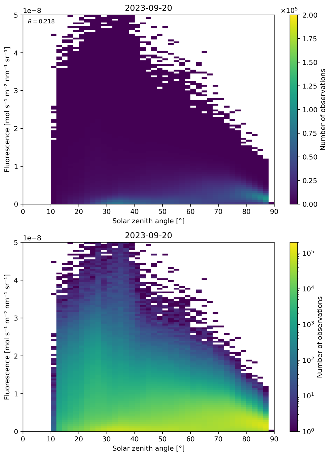
Figure 123: Scatter density plot of “Solar zenith angle” against “Fluorescence” for 2023-09-20 to 2023-09-21.
