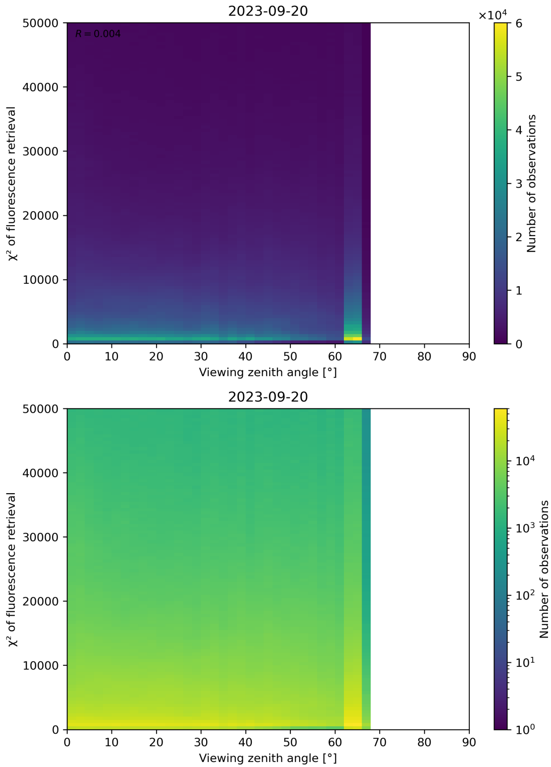
Figure 131: Scatter density plot of “Viewing zenith angle” against “ \chi^2 of fluorescence retrieval” for 2023-09-20 to 2023-09-21.
