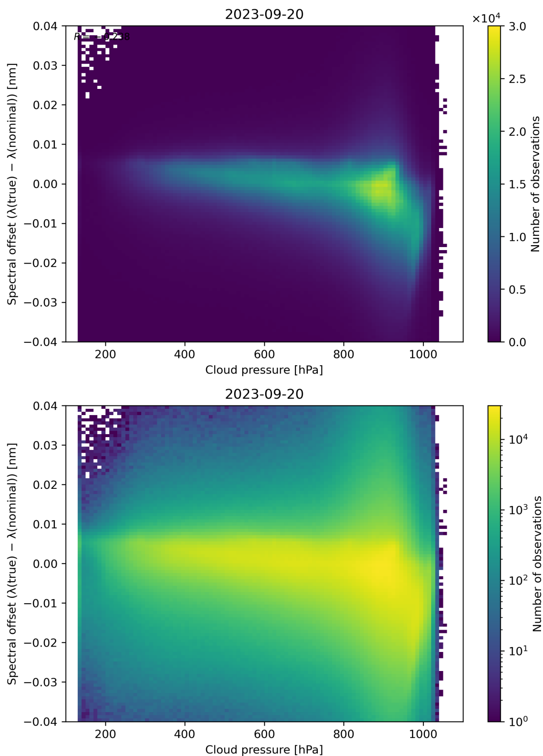
Figure 92: Scatter density plot of “Cloud pressure” against “Spectral offset ( \lambda(\text{true}) - \lambda(\text{nominal}) )” for 2023-09-20 to 2023-09-21.
