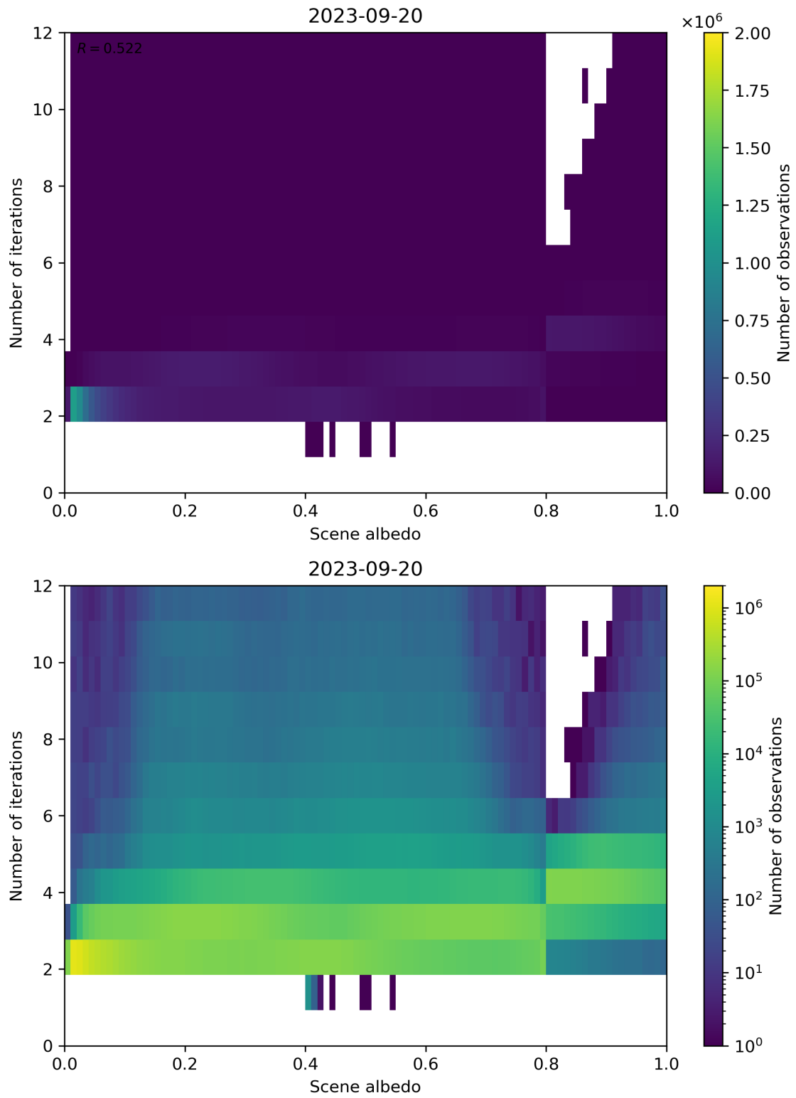
Figure 115: Scatter density plot of “Scene albedo” against “Number of iterations” for 2023-09-20 to 2023-09-21.
