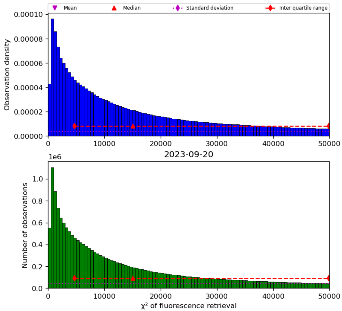
Figure 42: Histogram of “ \chi^2 of fluorescence retrieval” for 2023-09-20 to 2023-09-21
