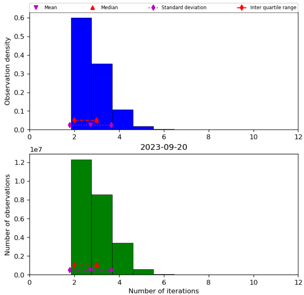
Figure 39: Histogram of “Number of iterations” for 2023-09-20 to 2023-09-21
