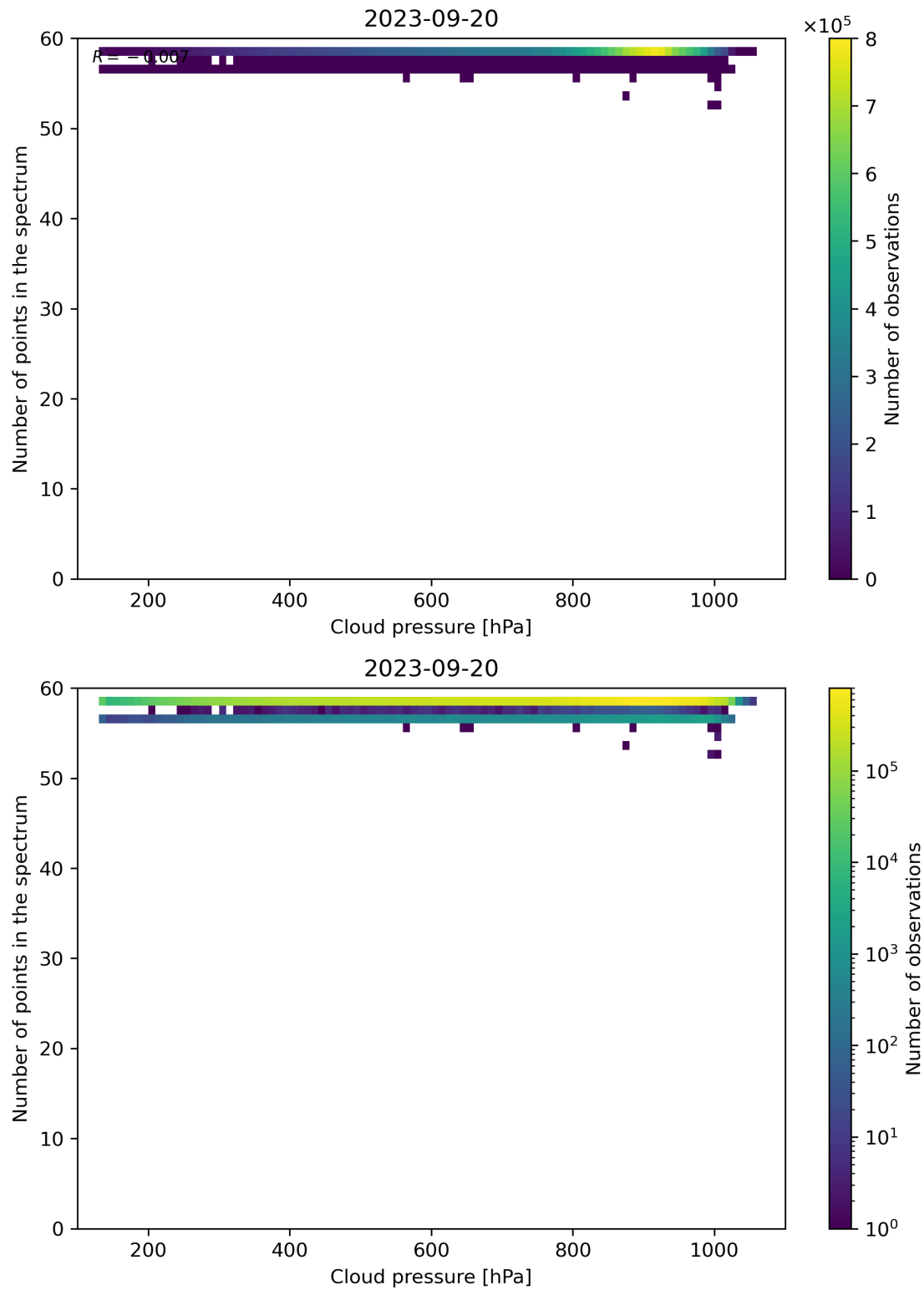
Figure 90: Scatter density plot of “Cloud pressure” against “Number of points in the spectrum” for 2023-09-20 to 2023-09-21.
