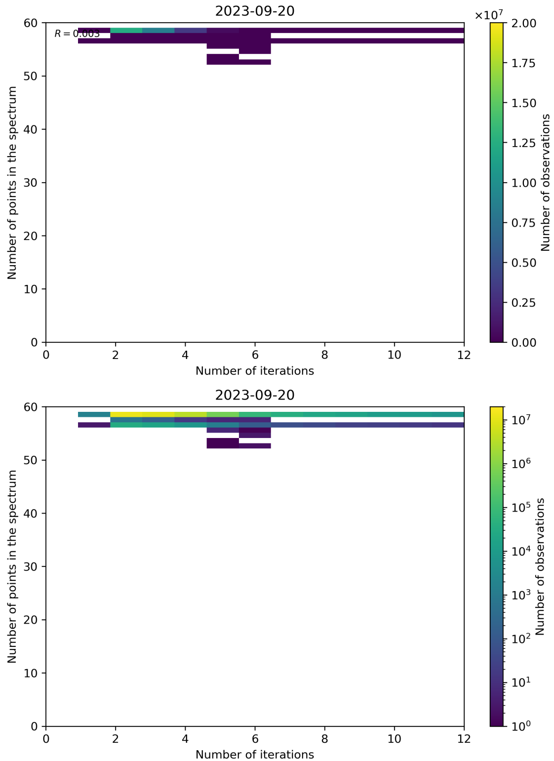
Figure 108: Scatter density plot of “Number of iterations” against “Number of points in the spectrum” for 2023-09-20 to 2023-09-21.
