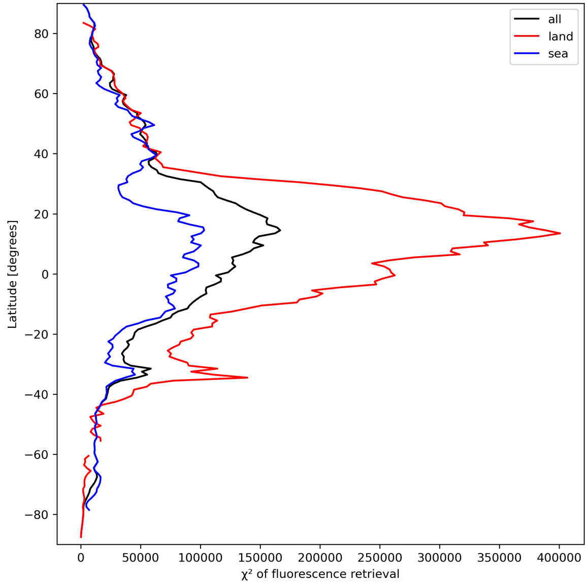
Figure 25: Zonal average of “ \chi^2 of fluorescence retrieval” for 2023-09-20 to 2023-09-21.
