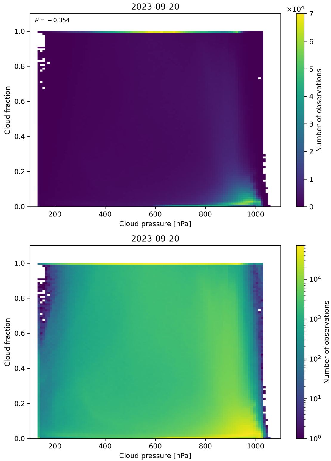
Figure 87: Scatter density plot of “Cloud pressure” against “Cloud fraction” for 2023-09-20 to 2023-09-21.
