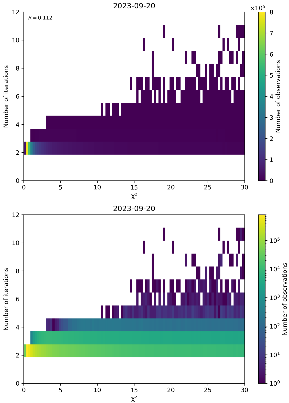
Figure 73: Scatter density plot of “ \chi^2 ” against “Number of iterations” for 2023-09-20 to 2023-09-21.
