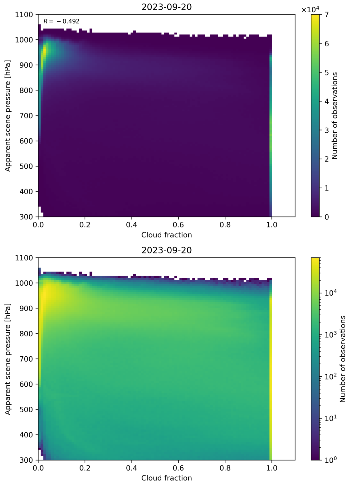
Figure 76: Scatter density plot of “Cloud fraction” against “Apparent scene pressure” for 2023-09-20 to 2023-09-21.
