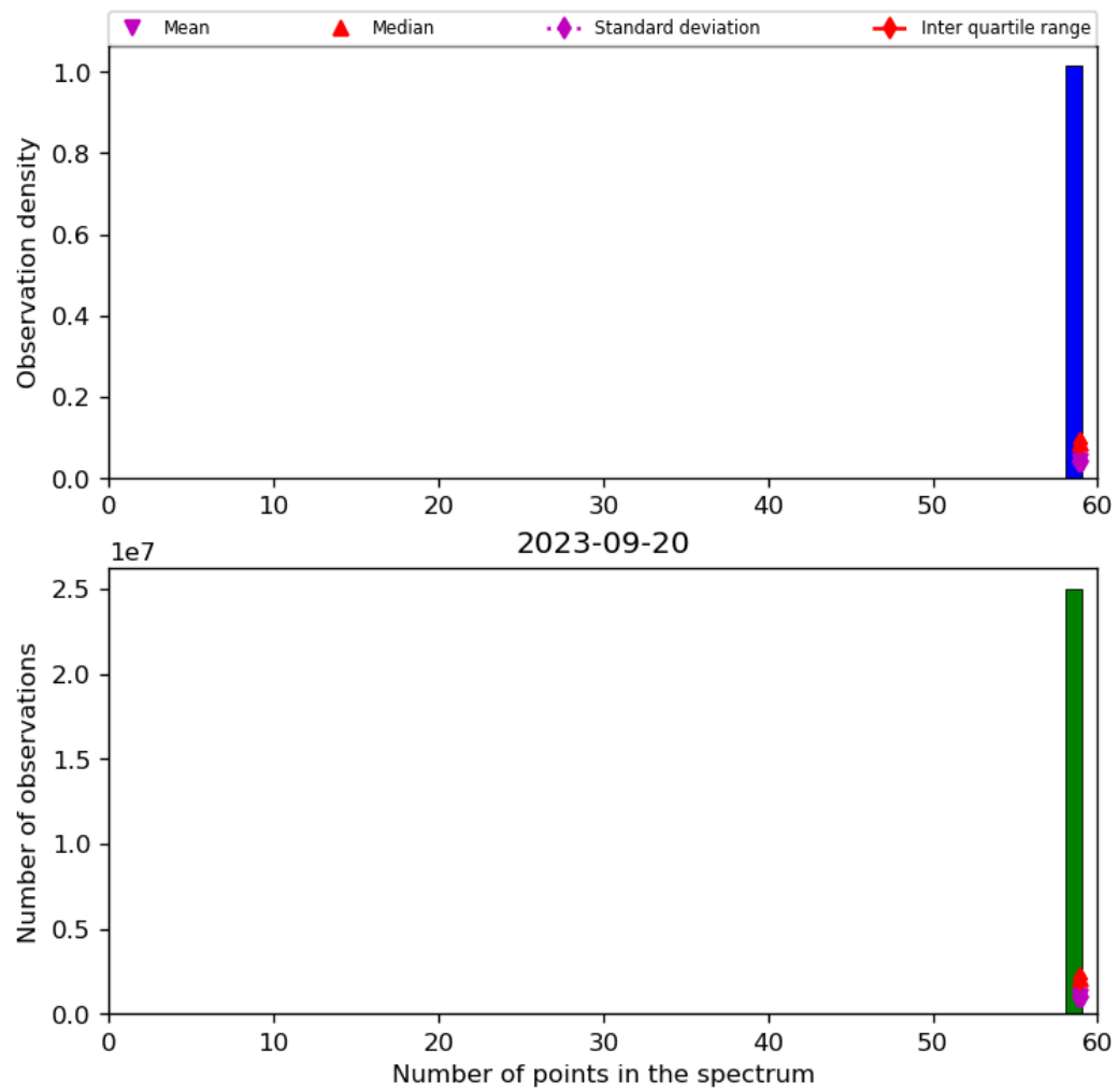
Figure 44: Histogram of “Number of points in the spectrum” for 2023-09-20 to 2023-09-21
