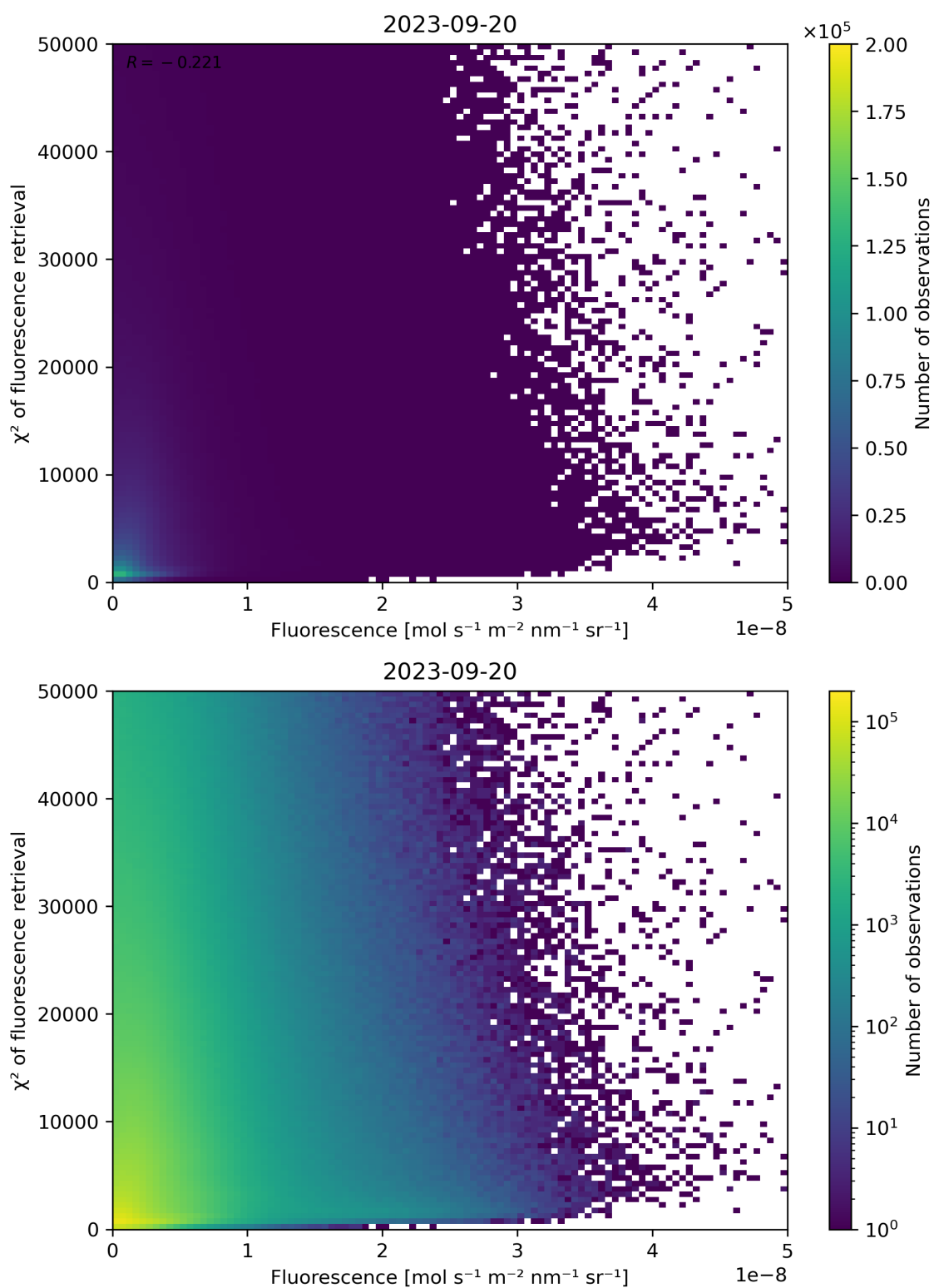
Figure 93: Scatter density plot of “Fluorescence” against “ \chi^2 of fluorescence retrieval” for 2023-09-20 to 2023-09-21.
