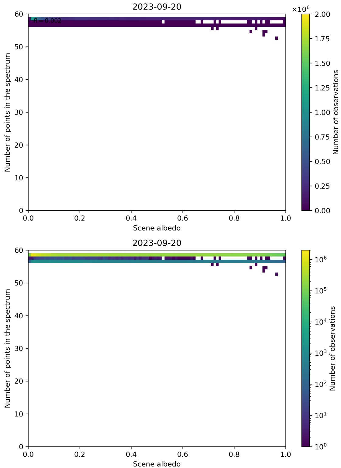
Figure 116: Scatter density plot of “Scene albedo” against “Number of points in the spectrum” for 2023-09-20 to 2023-09-21.
