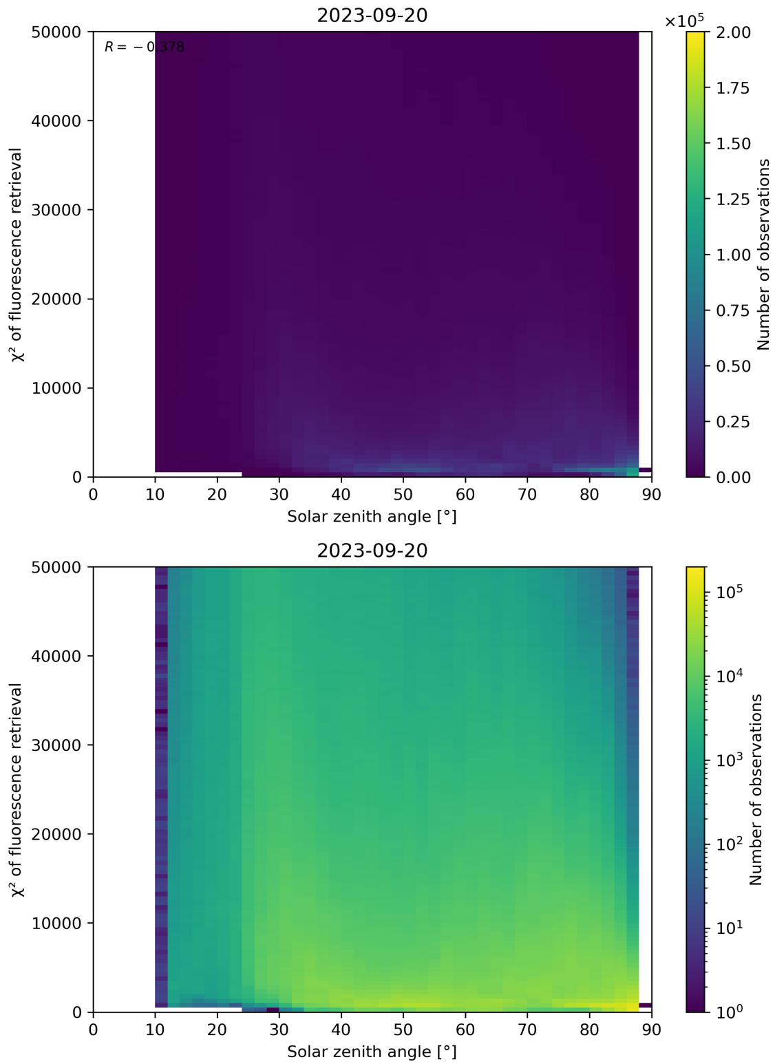
Figure 120: Scatter density plot of “Solar zenith angle” against “ \chi^2 of fluorescence retrieval” for 2023-09-20 to 2023-09-21.
