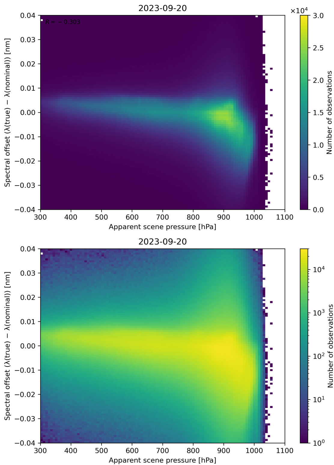
Figure 68: Scatter density plot of “Apparent scene pressure” against “Spectral offset ( \lambda(\text{true}) - \lambda(\text{nominal}) )” for 2023-09-20 to 2023-09-21.
