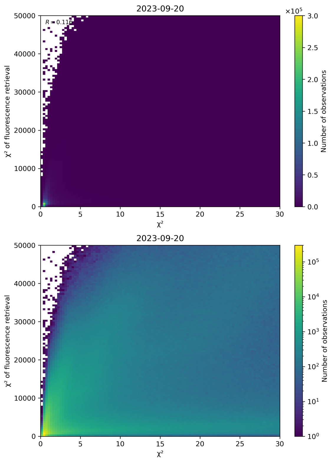
Figure 69: Scatter density plot of “ \chi^2 ” against “ \chi^2 of fluorescence retrieval” for 2023-09-20 to 2023-09-21.
