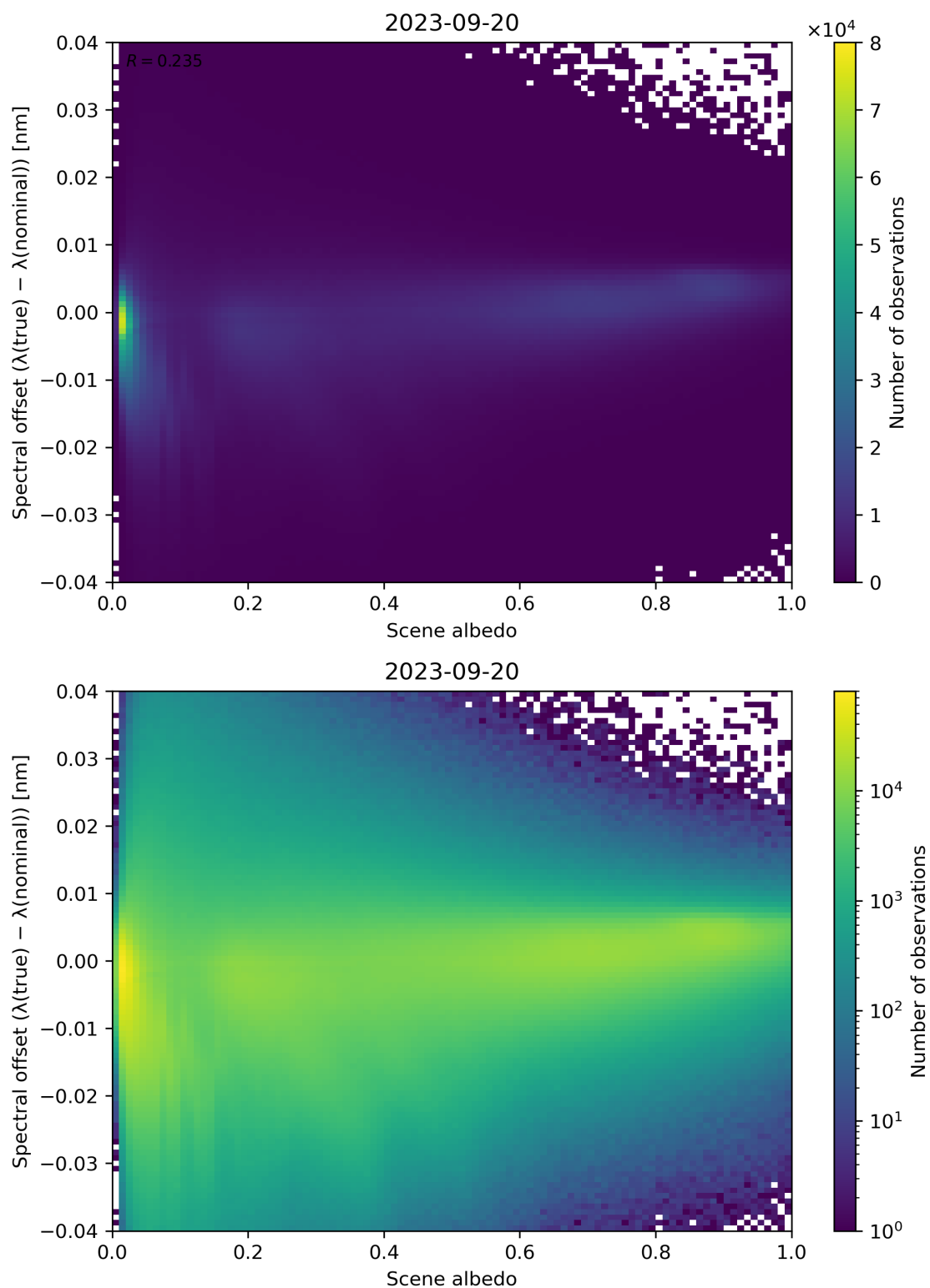
Figure 117: Scatter density plot of “Scene albedo” against “Spectral offset ( \lambda(\text{true}) - \lambda(\text{nominal}) )” for 2023-09-20 to 2023-09-21.
