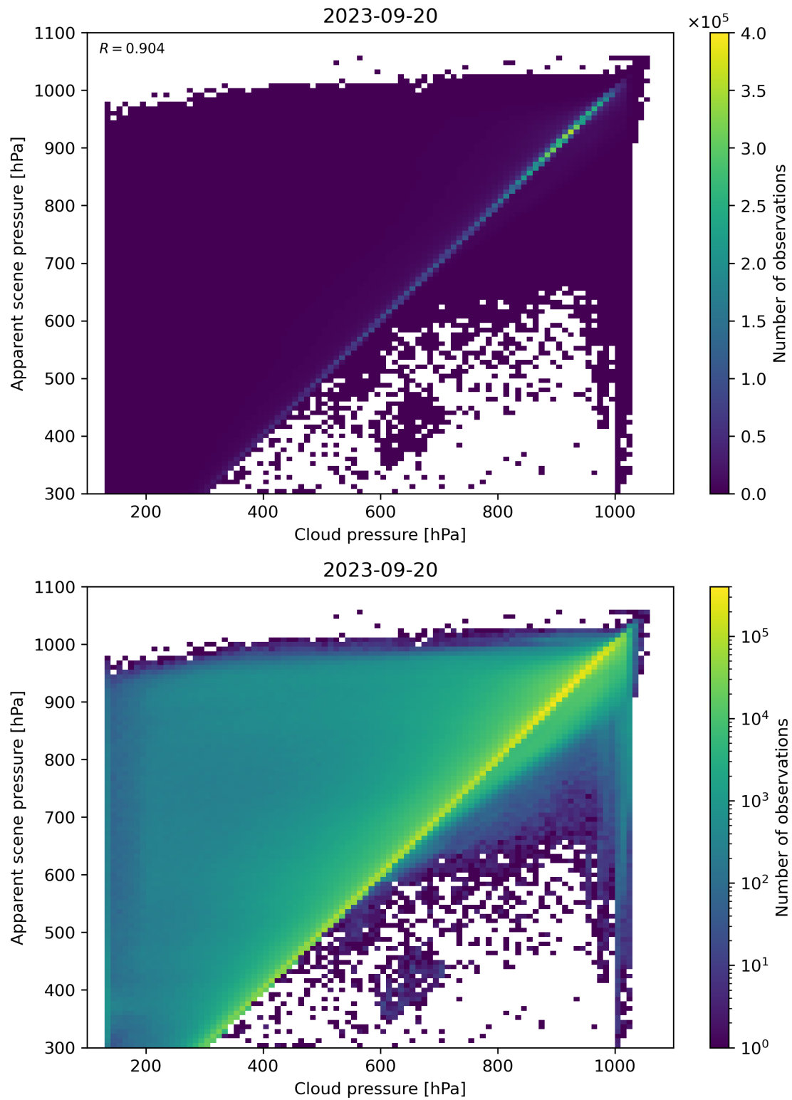
Figure 84: Scatter density plot of “Cloud pressure” against “Apparent scene pressure” for 2023-09-20 to 2023-09-21.
