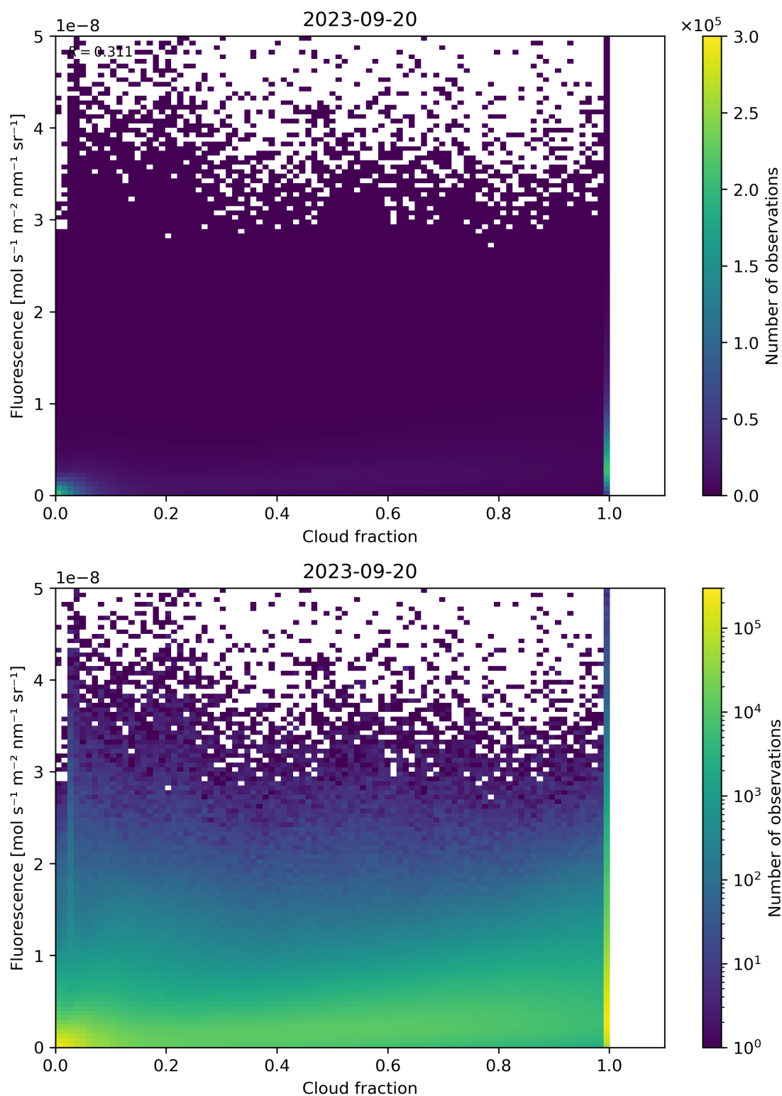
Figure 79: Scatter density plot of “Cloud fraction” against “Fluorescence” for 2023-09-20 to 2023-09-21.
