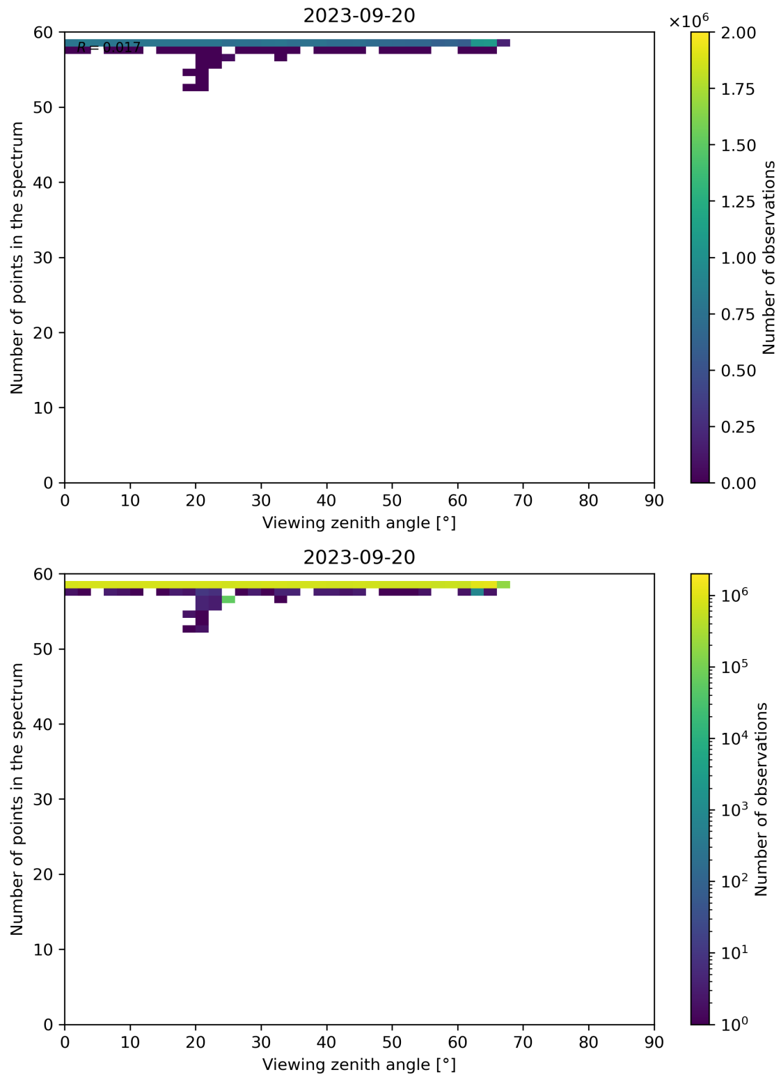
Figure 137: Scatter density plot of “Viewing zenith angle” against “Number of points in the spectrum” for 2023-09-20 to 2023-09-21.
