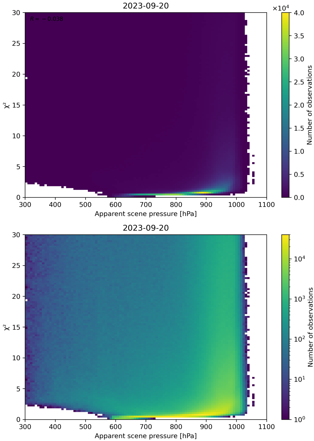
Figure 63: Scatter density plot of “Apparent scene pressure” against “ \chi^2 ” for 2023-09-20 to 2023-09-21.
