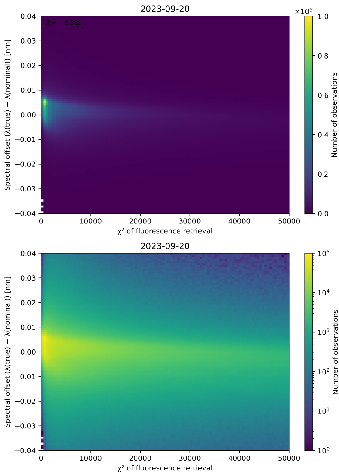
Figure 72: Scatter density plot of " \chi^2 of fluorescence retrieval" against "Spectral offset ( \lambda(\text{true}) - \lambda(\text{nominal}) )" for 2023-09-20 to 2023-09-21.
