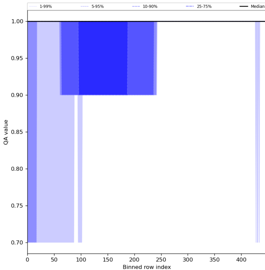
Figure 46: Along track statistics of “QA value” for 2023-09-20 to 2023-09-21
