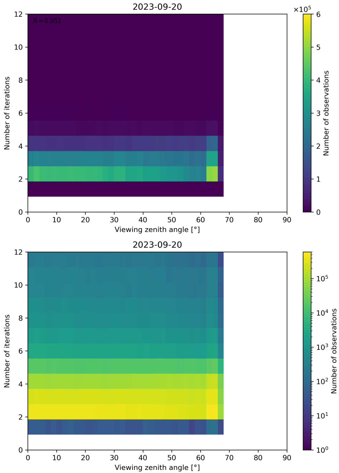
Figure 136: Scatter density plot of “Viewing zenith angle” against “Number of iterations” for 2023-09-20 to 2023-09-21.
