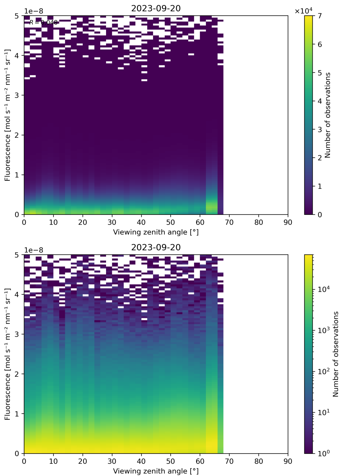
Figure 134: Scatter density plot of “Viewing zenith angle” against “Fluorescence” for 2023-09-20 to 2023-09-21.
