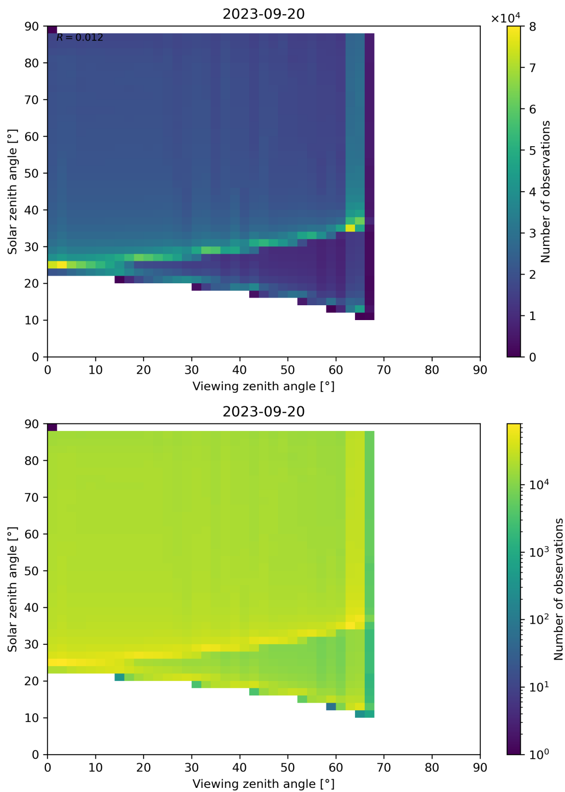
Figure 139: Scatter density plot of “Viewing zenith angle” against “Solar zenith angle” for 2023-09-20 to 2023-09-21.
