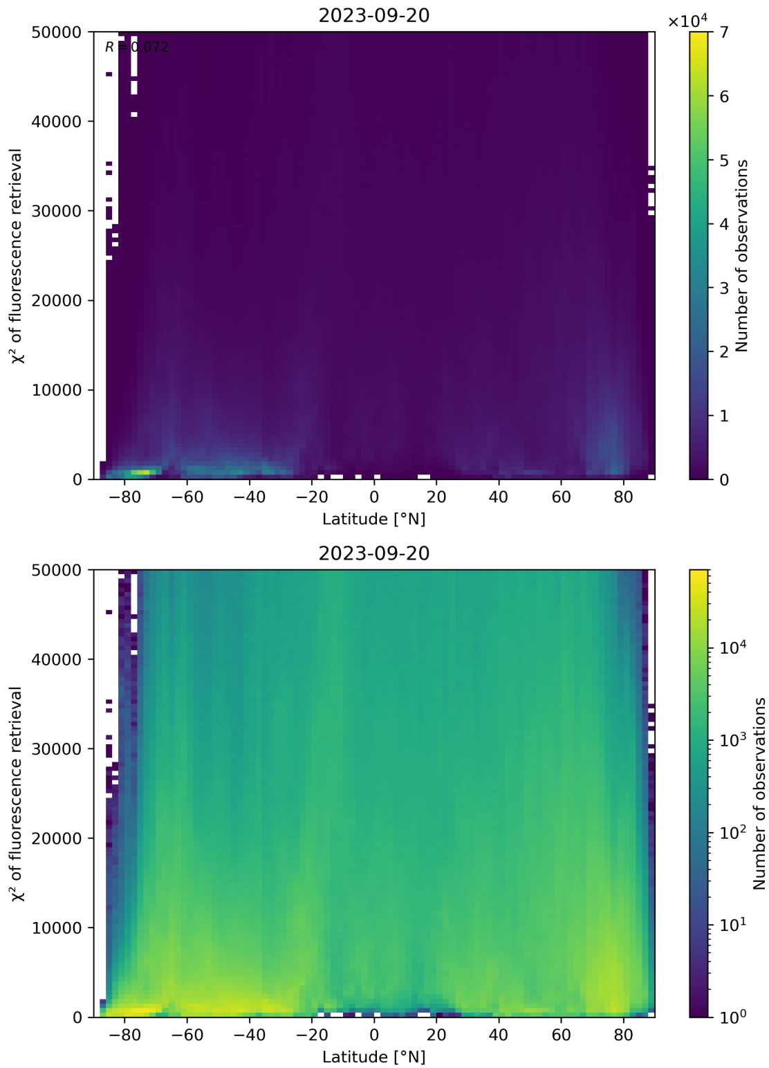
Figure 98: Scatter density plot of “Latitude” against “ \chi^2 of fluorescence retrieval” for 2023-09-20 to 2023-09-21.
