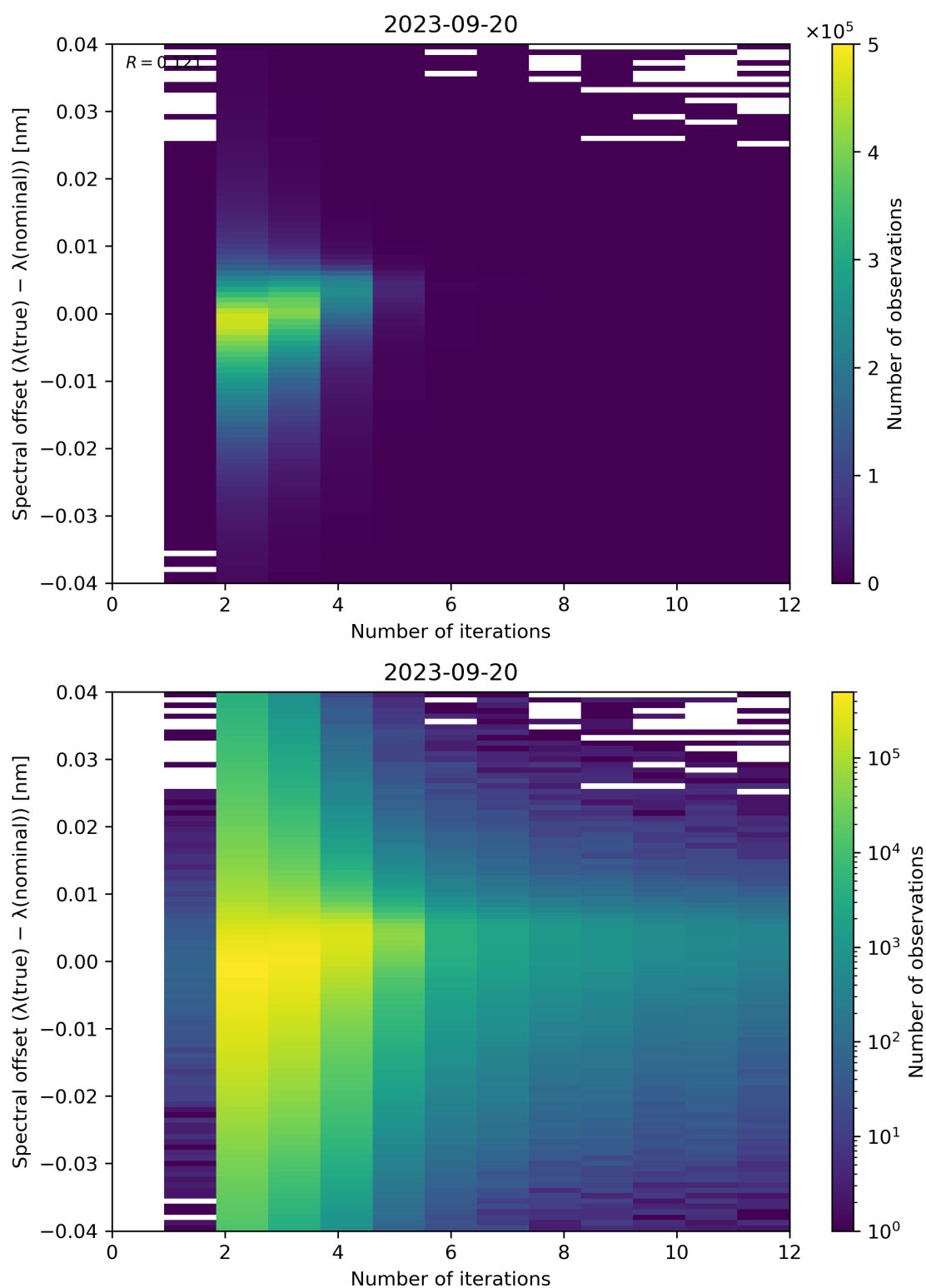
Figure 109: Scatter density plot of “Number of iterations” against “Spectral offset ( \lambda(\text{true}) - \lambda(\text{nominal}) )” for 2023-09-20 to 2023-09-21.
