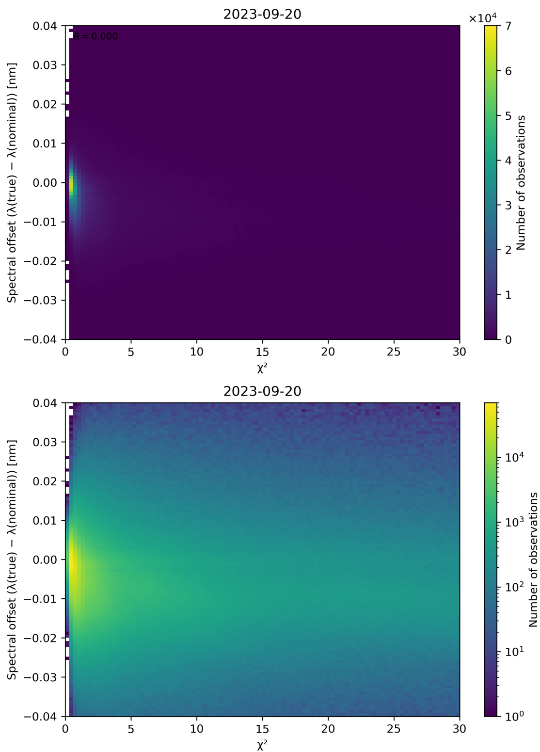
Figure 75: Scatter density plot of " \chi^2 " against "Spectral offset ( \lambda(\text{true}) - \lambda(\text{nominal}) )" for 2023-09-20 to 2023-09-21.
