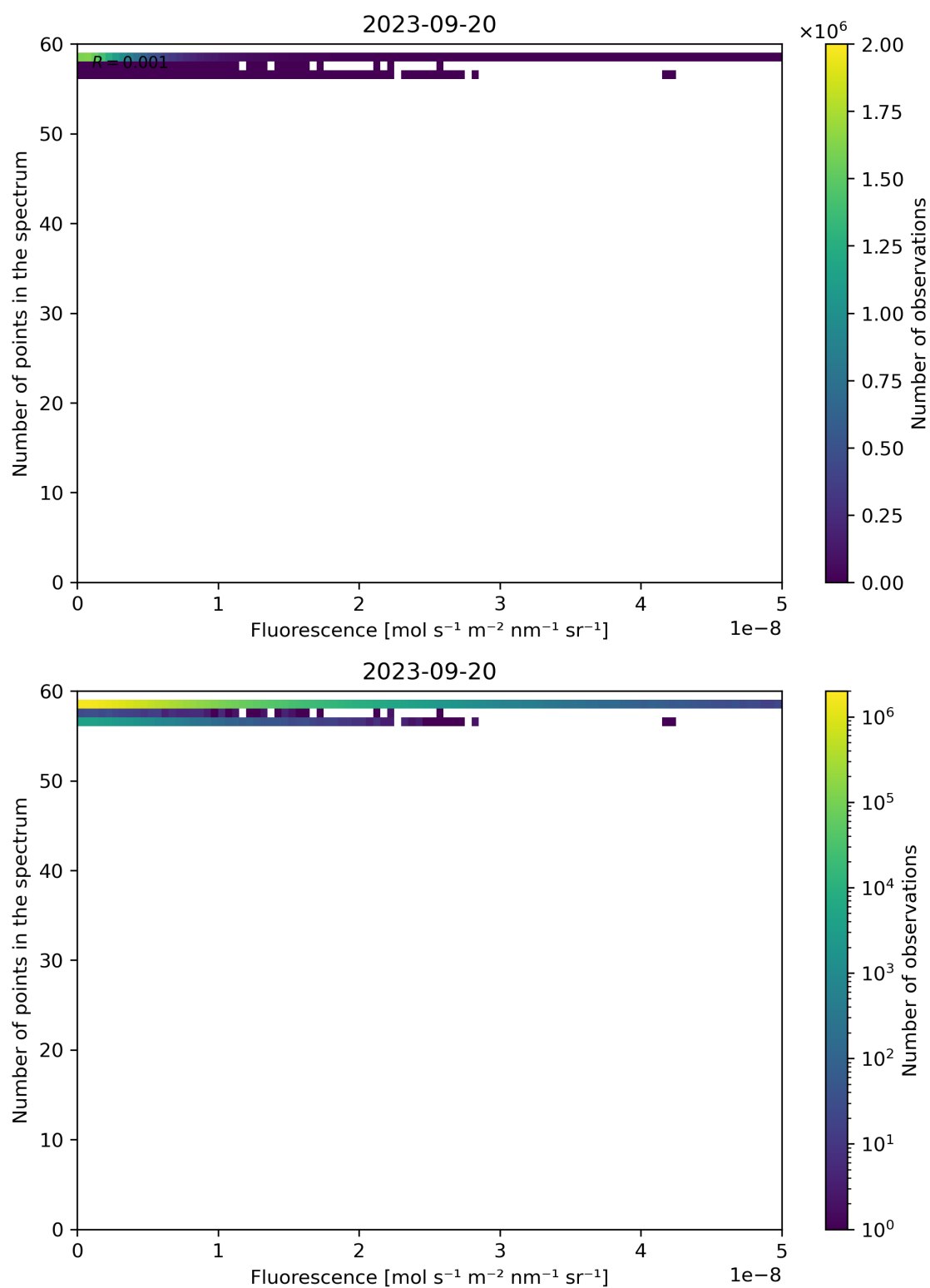
Figure 94: Scatter density plot of “Fluorescence” against “Number of points in the spectrum” for 2023-09-20 to 2023-09-21.
