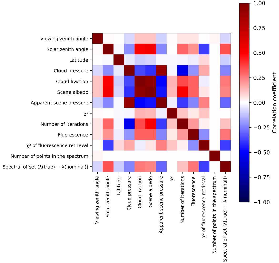
Figure 2: Map of correlation matrix for 2023-09-20 to 2023-09-21.
