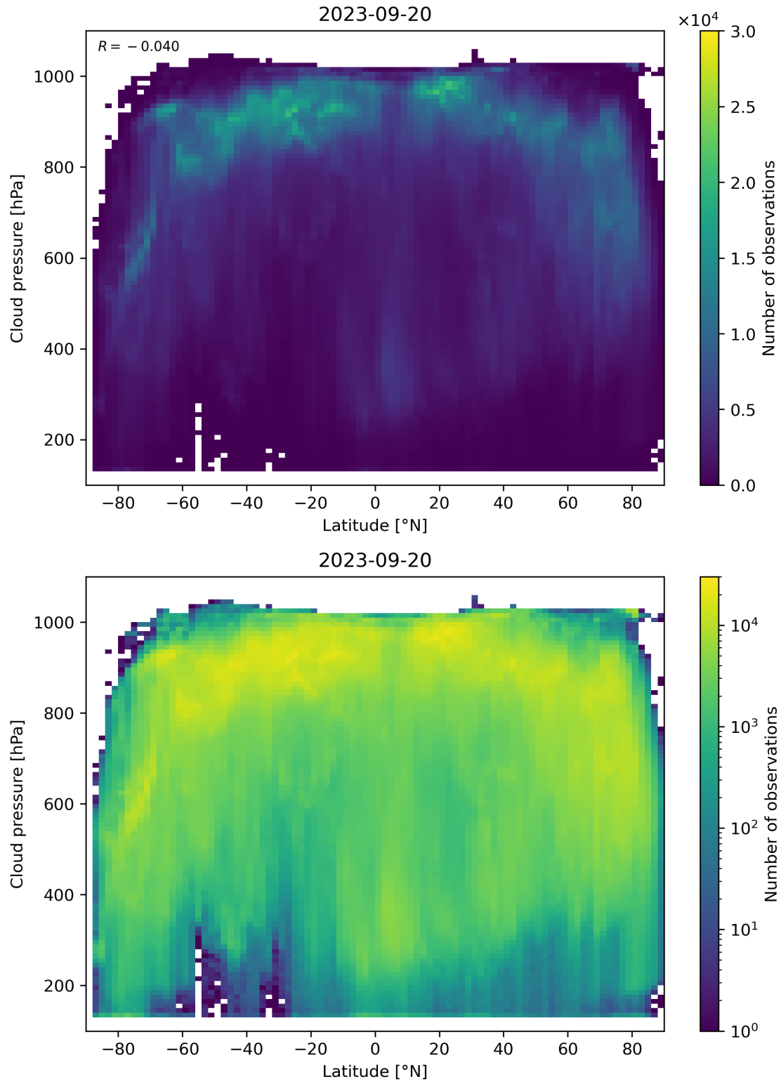
Figure 100: Scatter density plot of “Latitude” against “Cloud pressure” for 2023-09-20 to 2023-09-21.
