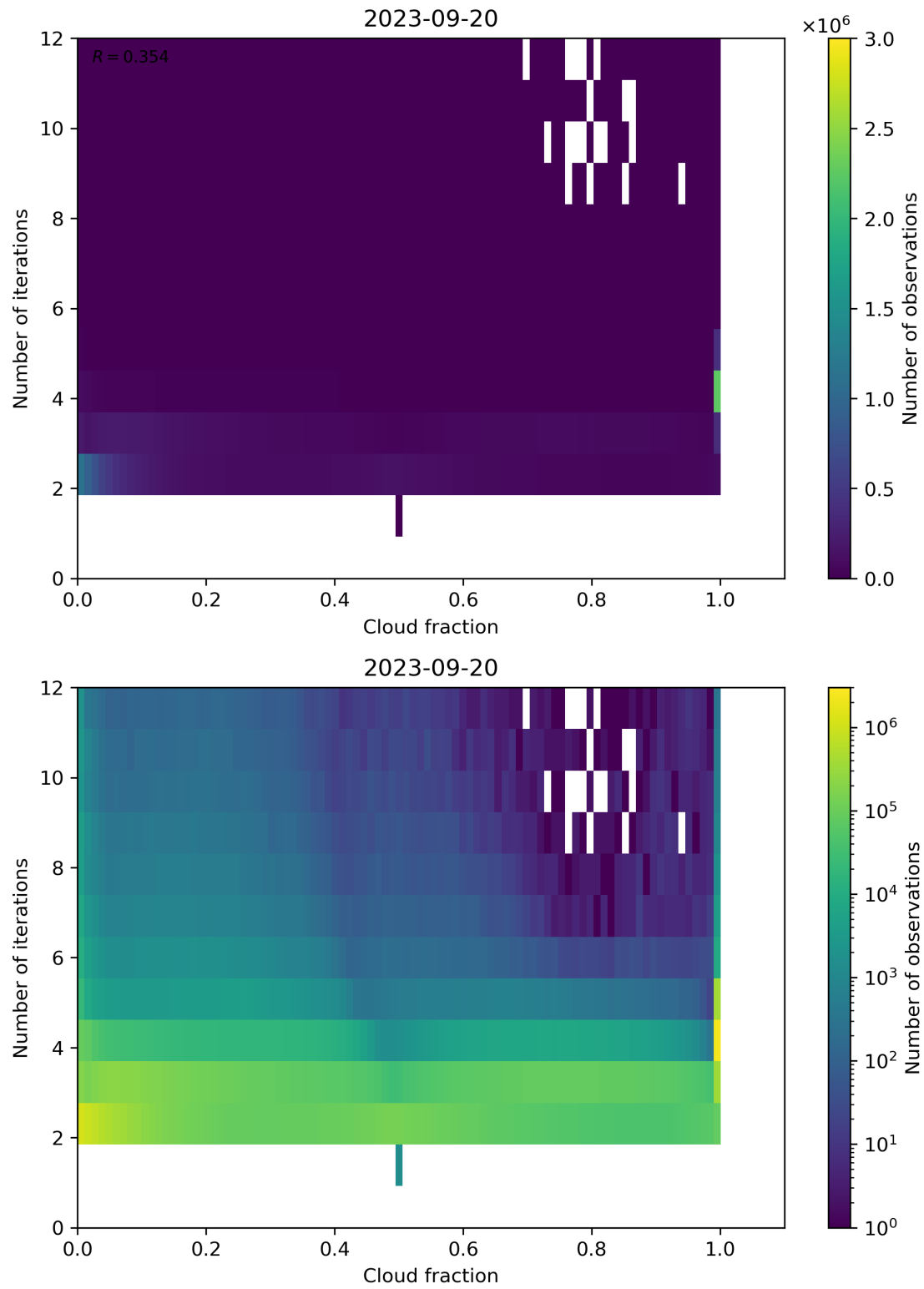
Figure 80: Scatter density plot of “Cloud fraction” against “Number of iterations” for 2023-09-20 to 2023-09-21.
