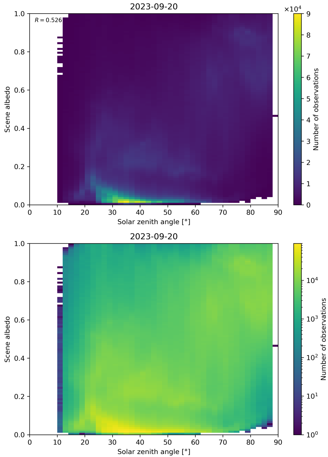
Figure 127: Scatter density plot of “Solar zenith angle” against “Scene albedo” for 2023-09-20 to 2023-09-21.
