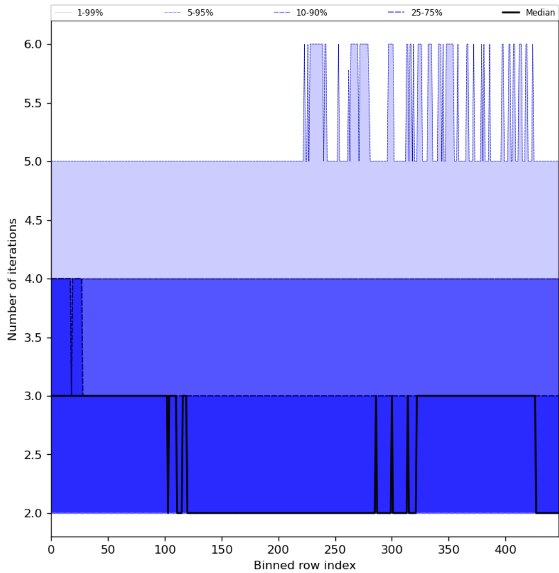
Figure 56: Along track statistics of “Number of iterations” for 2023-09-20 to 2023-09-21
