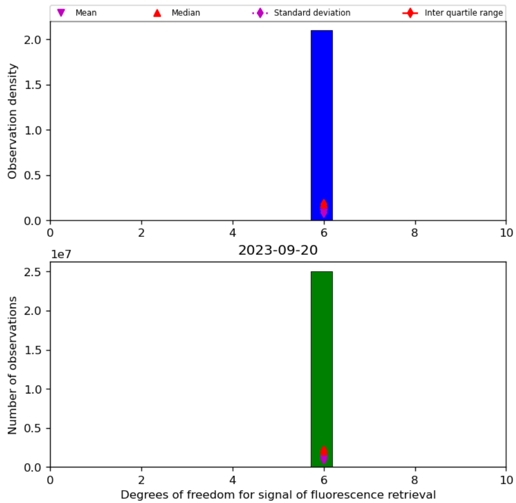
Figure 43: Histogram of “Degrees of freedom for signal of fluorescence retrieval” for 2023-09-20 to 2023-09-21
