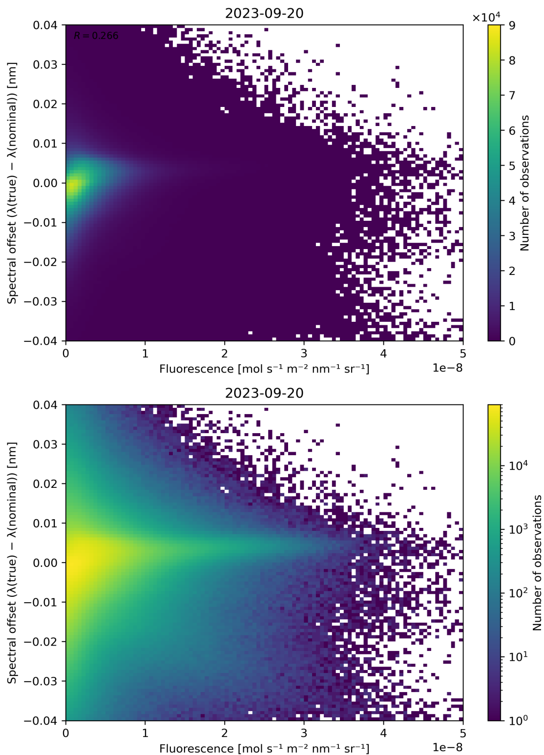
Figure 95: Scatter density plot of “Fluorescence” against “Spectral offset ( \lambda(\text{true}) - \lambda(\text{nominal}) )” for 2023-09-20 to 2023-09-21.
