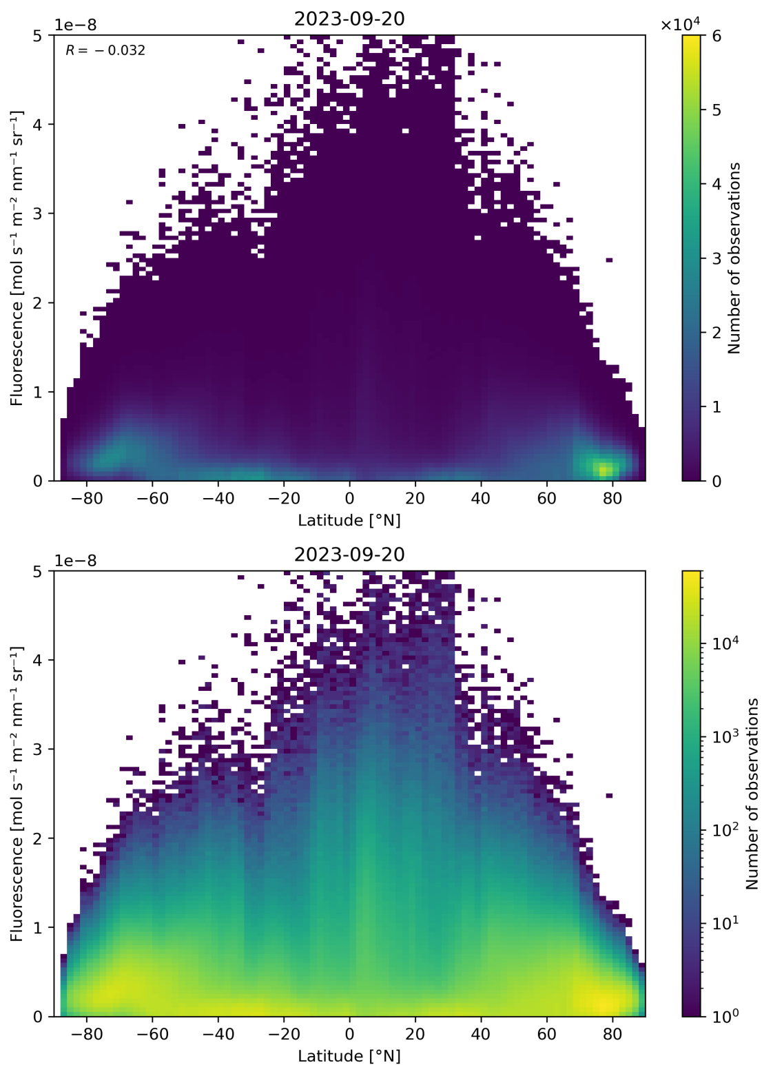
Figure 101: Scatter density plot of “Latitude” against “Fluorescence” for 2023-09-20 to 2023-09-21.
