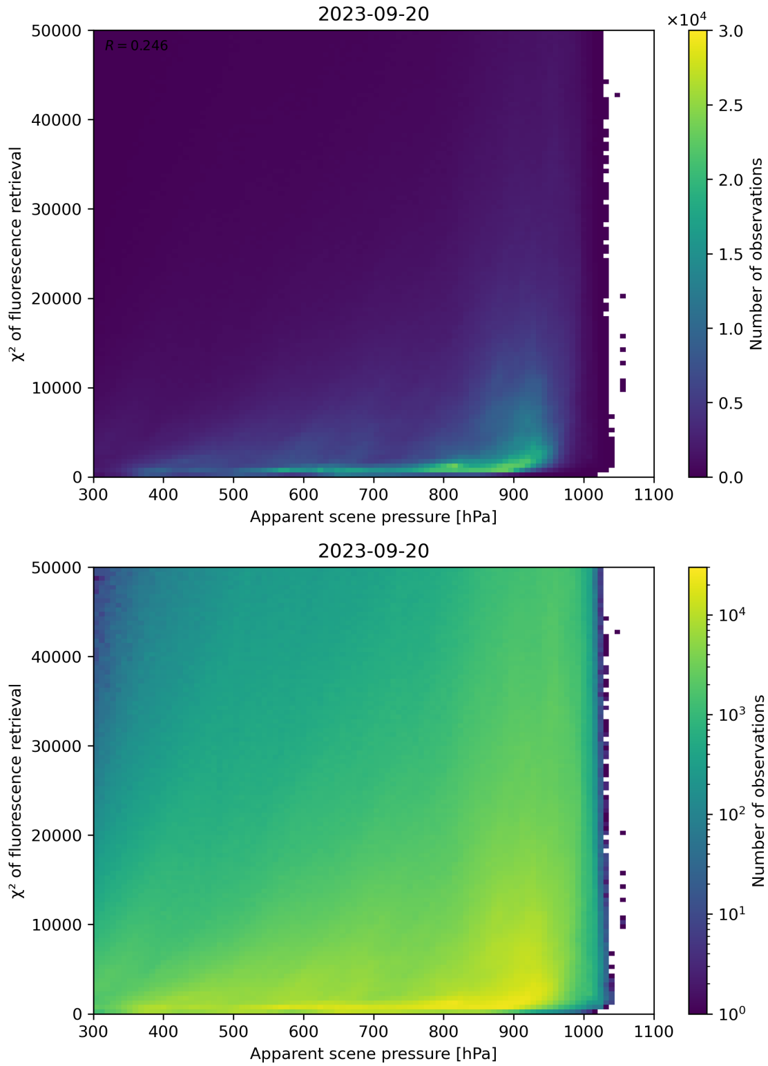
Figure 64: Scatter density plot of “Apparent scene pressure” against “ \chi^2 of fluorescence retrieval” for 2023-09-20 to 2023-09-21.
