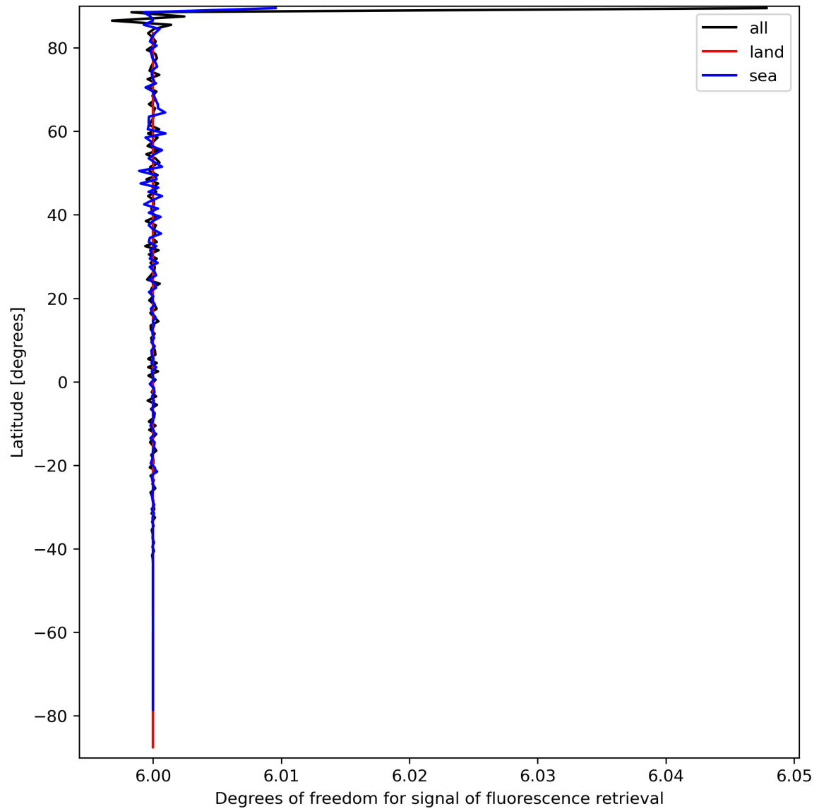
Figure 26: Zonal average of “Degrees of freedom for signal of fluorescence retrieval” for 2023-09-20 to 2023-09-21.
