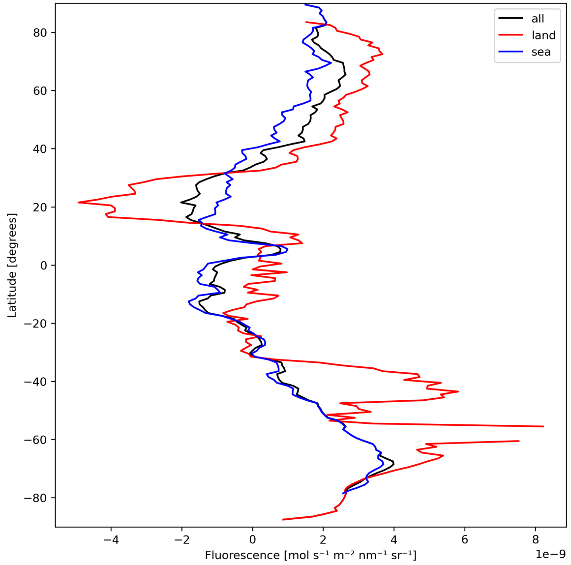
Figure 23: Zonal average of “Fluorescence” for 2023-09-20 to 2023-09-21.
