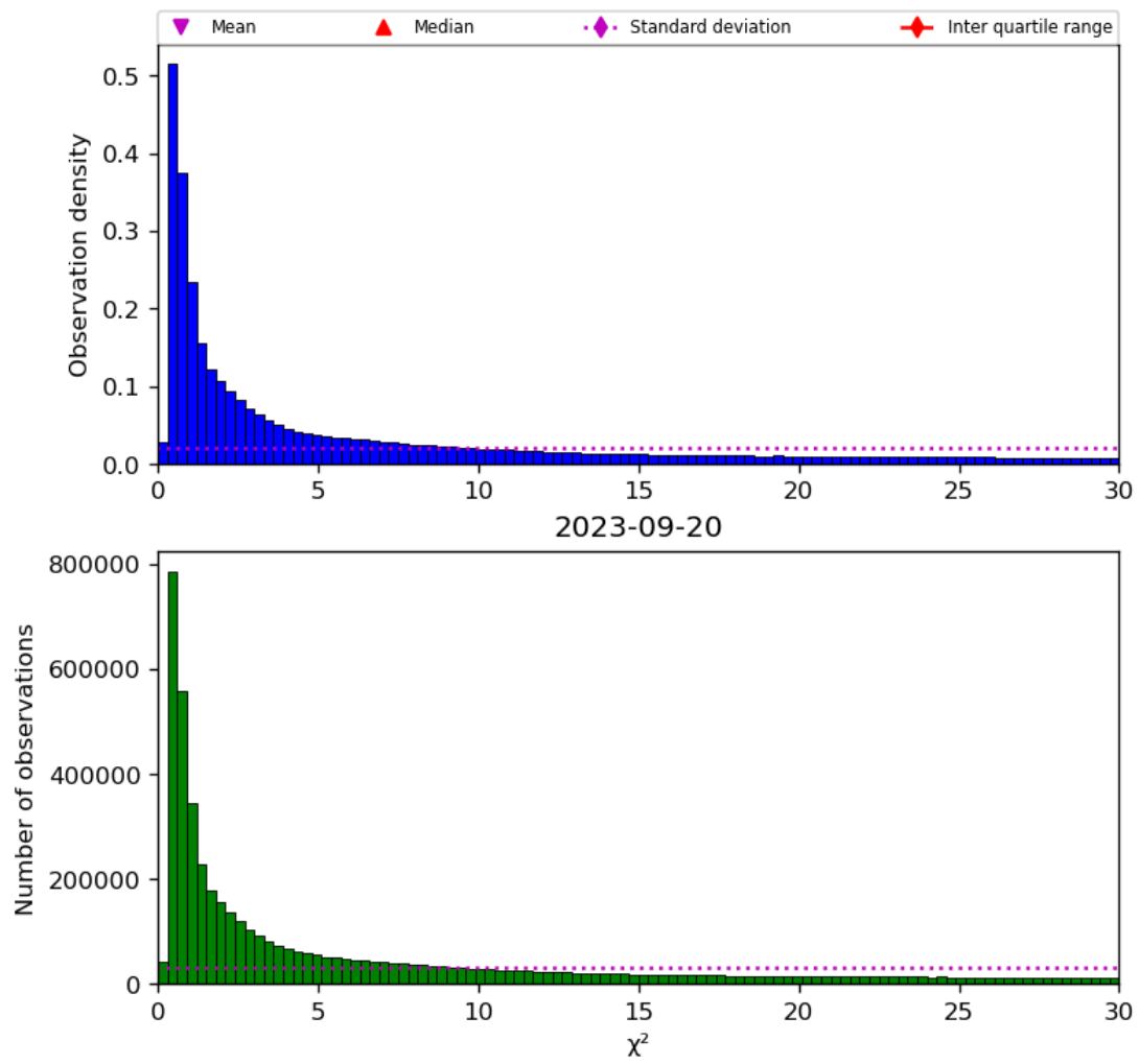
Figure 38: Histogram of “ \chi^2 ” for 2023-09-20 to 2023-09-21
