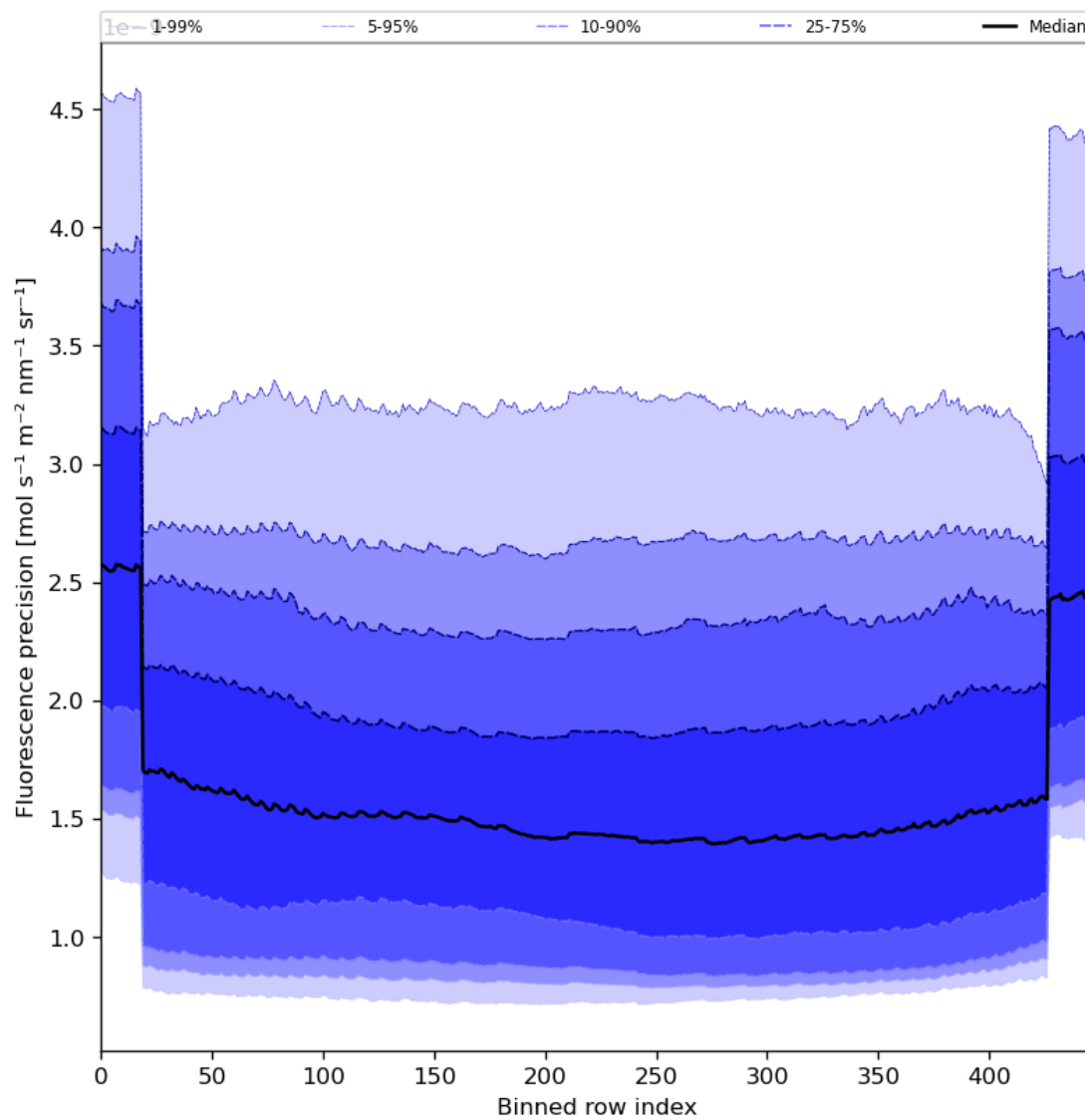
Figure 58: Along track statistics of “Fluorescence precision” for 2023-09-20 to 2023-09-21
