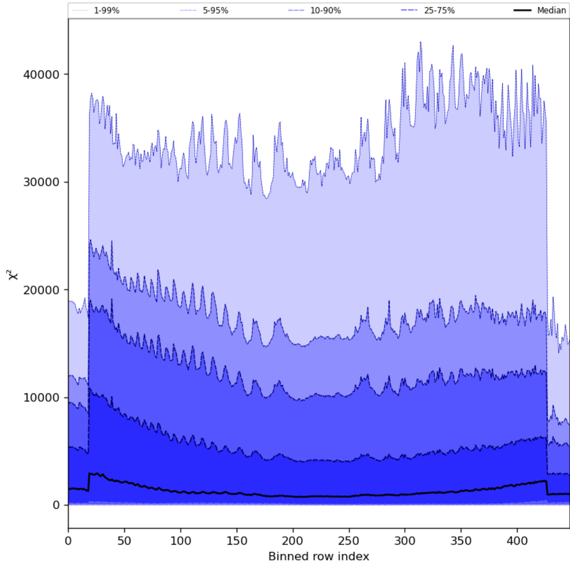
Figure 55: Along track statistics of “ \chi^2 ” for 2023-09-20 to 2023-09-21
