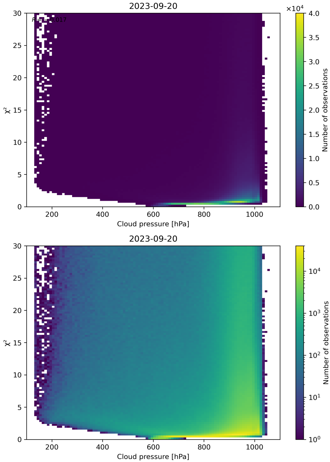
Figure 85: Scatter density plot of “Cloud pressure” against “ \chi^2 ” for 2023-09-20 to 2023-09-21.
