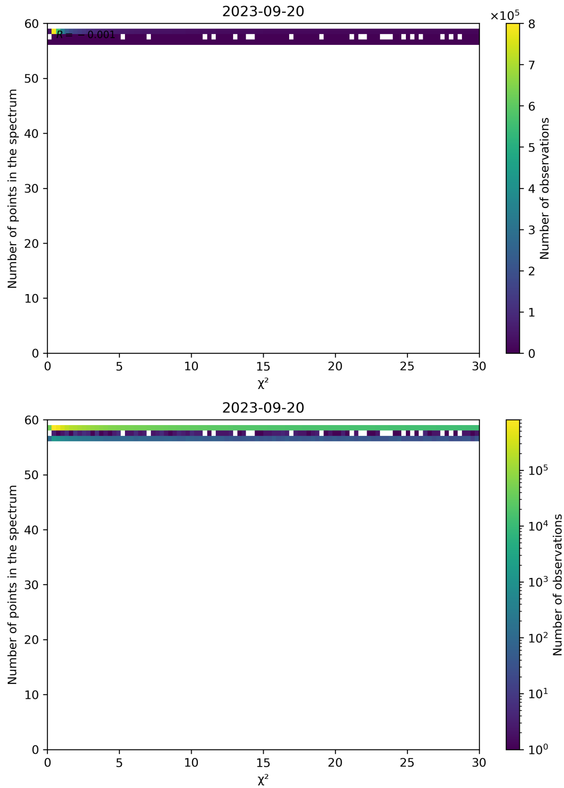
Figure 74: Scatter density plot of " \chi^2 " against "Number of points in the spectrum" for 2023-09-20 to 2023-09-21.
