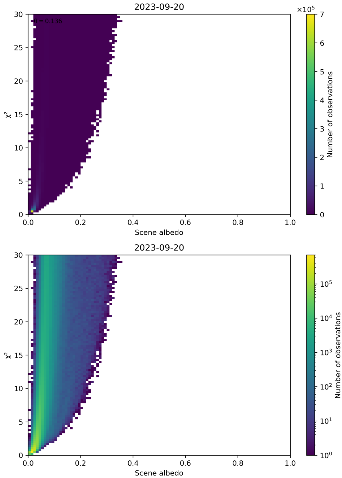
Figure 112: Scatter density plot of “Scene albedo” against “ \chi^2 ” for 2023-09-20 to 2023-09-21.
