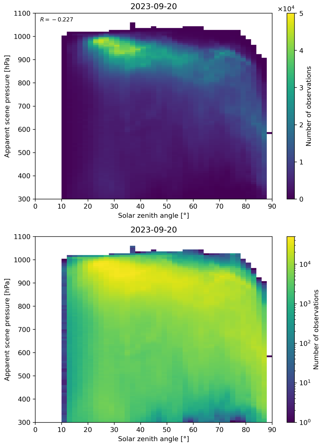
Figure 118: Scatter density plot of “Solar zenith angle” against “Apparent scene pressure” for 2023-09-20 to 2023-09-21.
