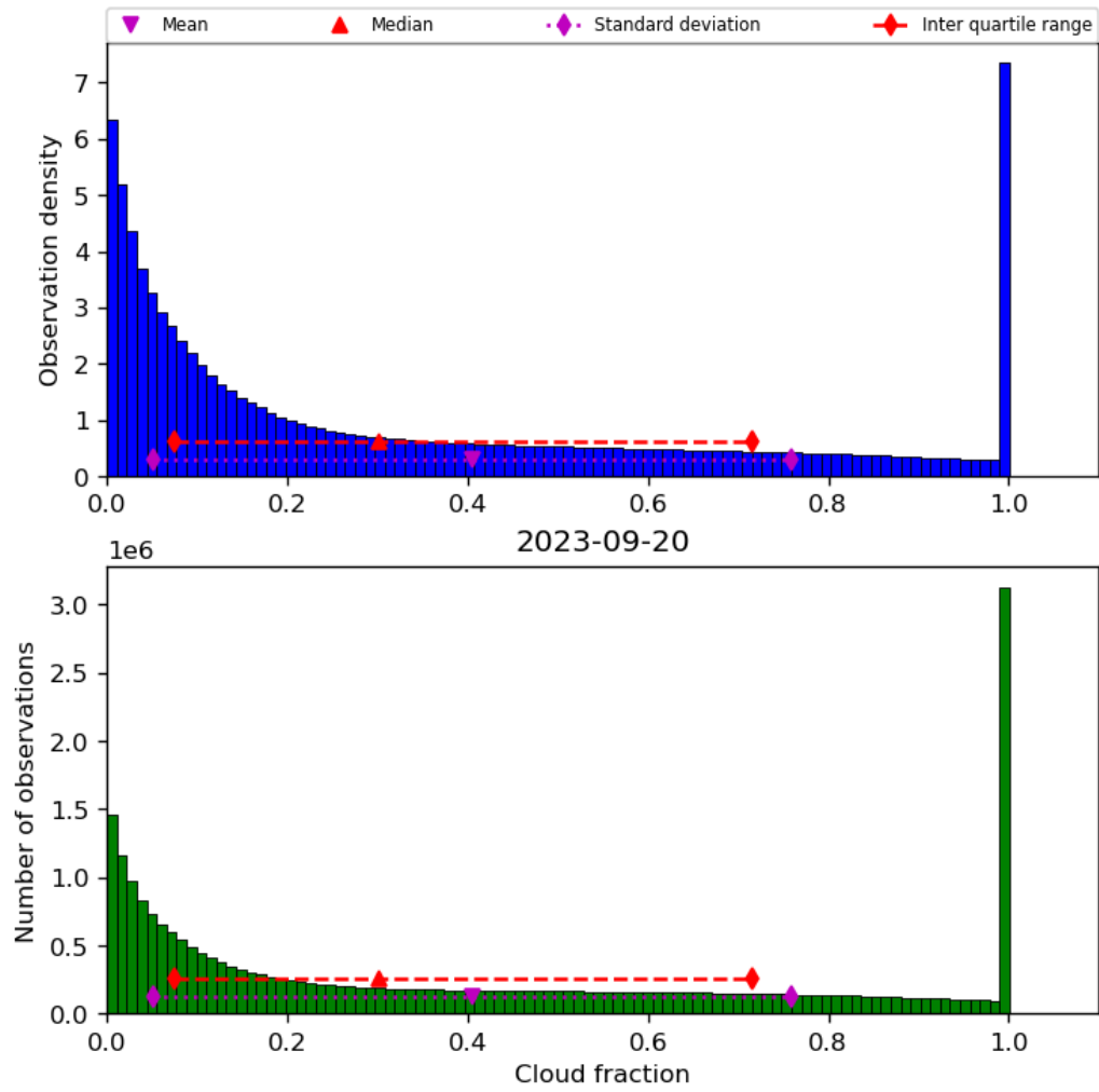
Figure 32: Histogram of “Cloud fraction” for 2023-09-20 to 2023-09-21
