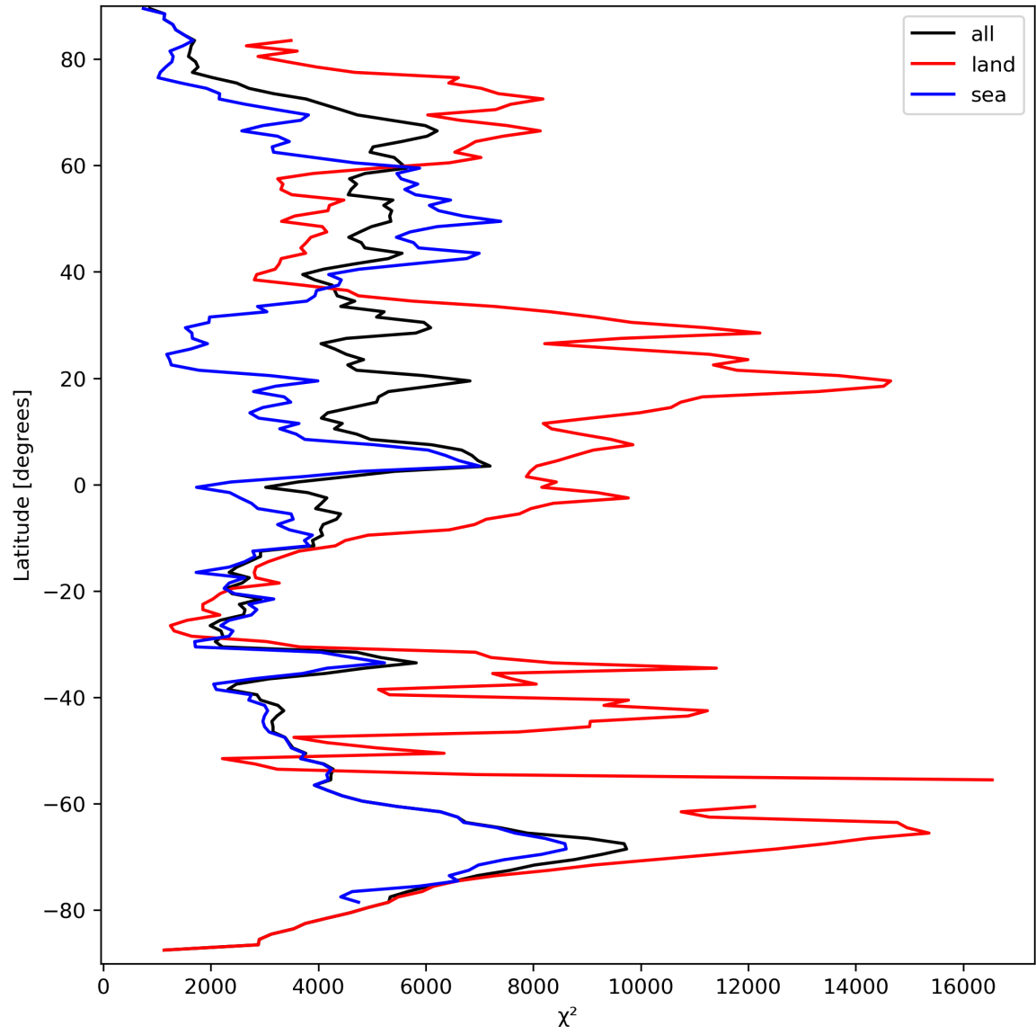
Figure 21: Zonal average of “ \chi^2 ” for 2023-09-20 to 2023-09-21.
