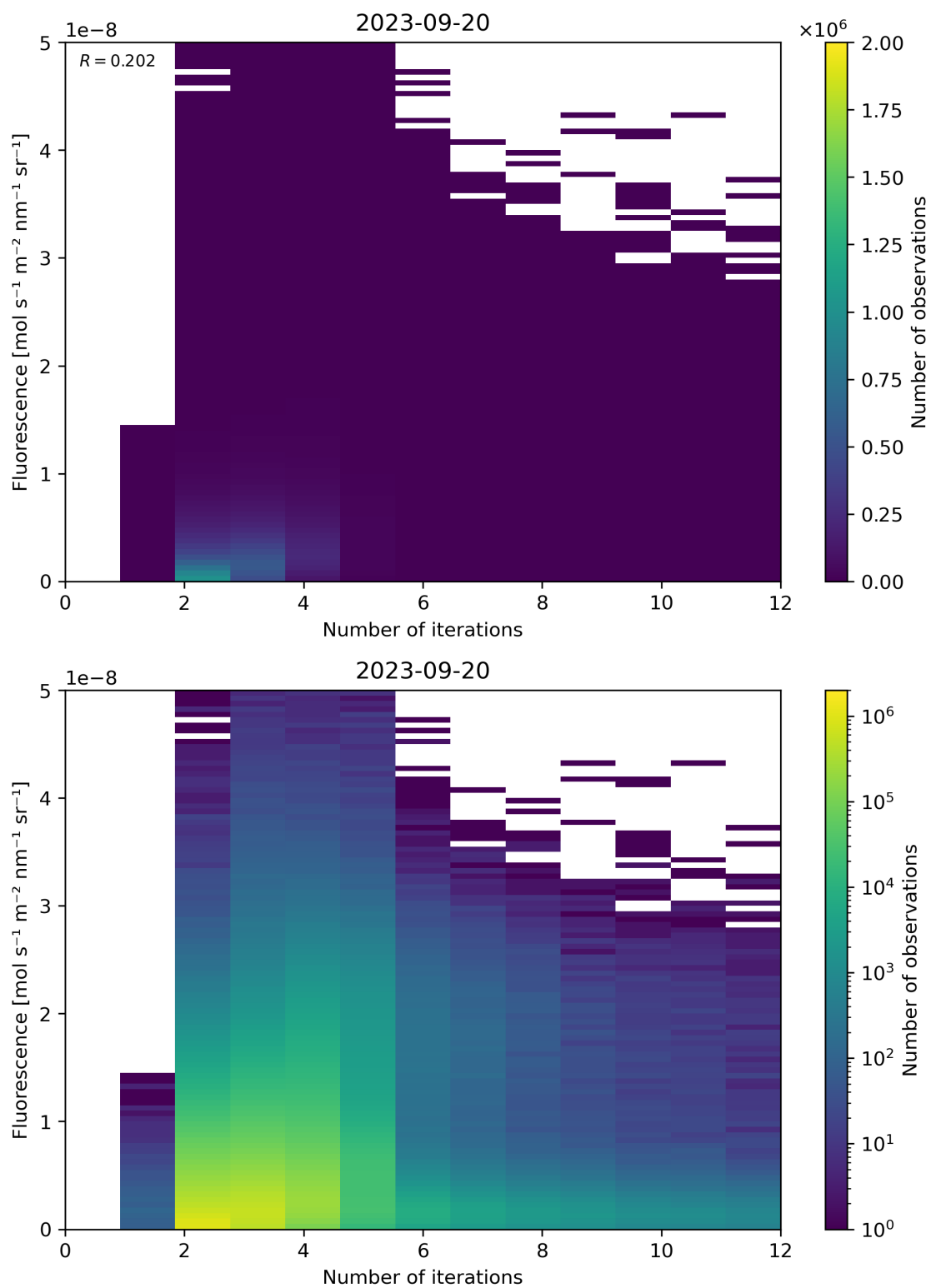
Figure 107: Scatter density plot of “Number of iterations” against “Fluorescence” for 2023-09-20 to 2023-09-21.
