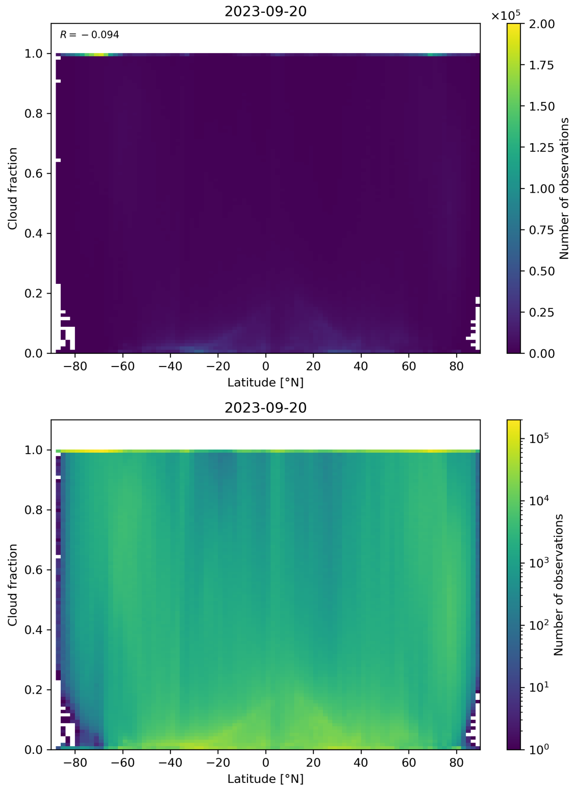
Figure 99: Scatter density plot of “Latitude” against “Cloud fraction” for 2023-09-20 to 2023-09-21.
