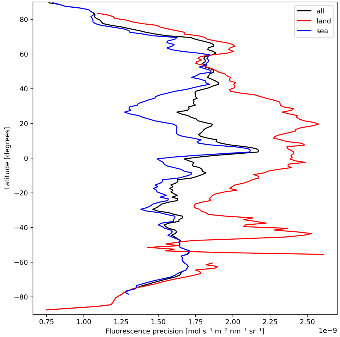
Figure 24: Zonal average of “Fluorescence precision” for 2023-09-20 to 2023-09-21.
