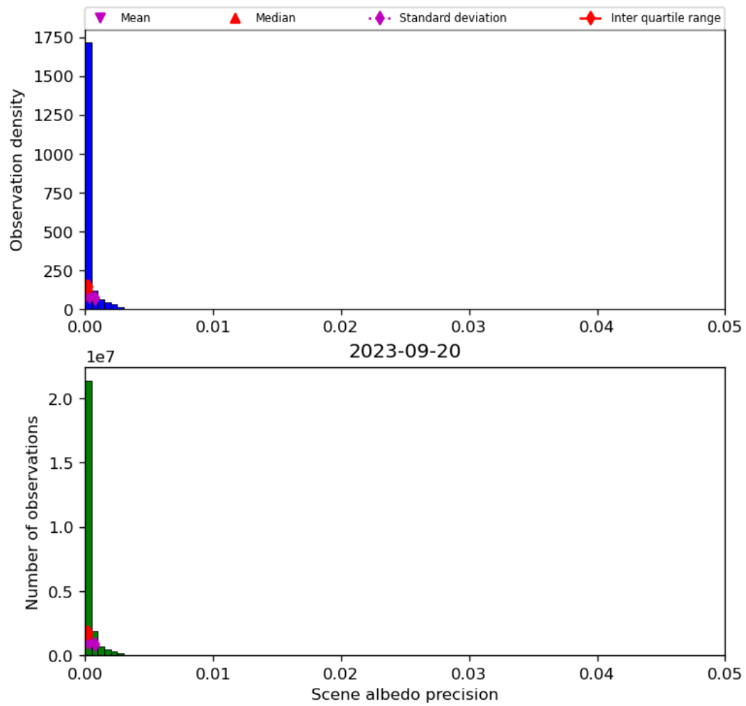
Figure 35: Histogram of “Scene albedo precision” for 2023-09-20 to 2023-09-21
