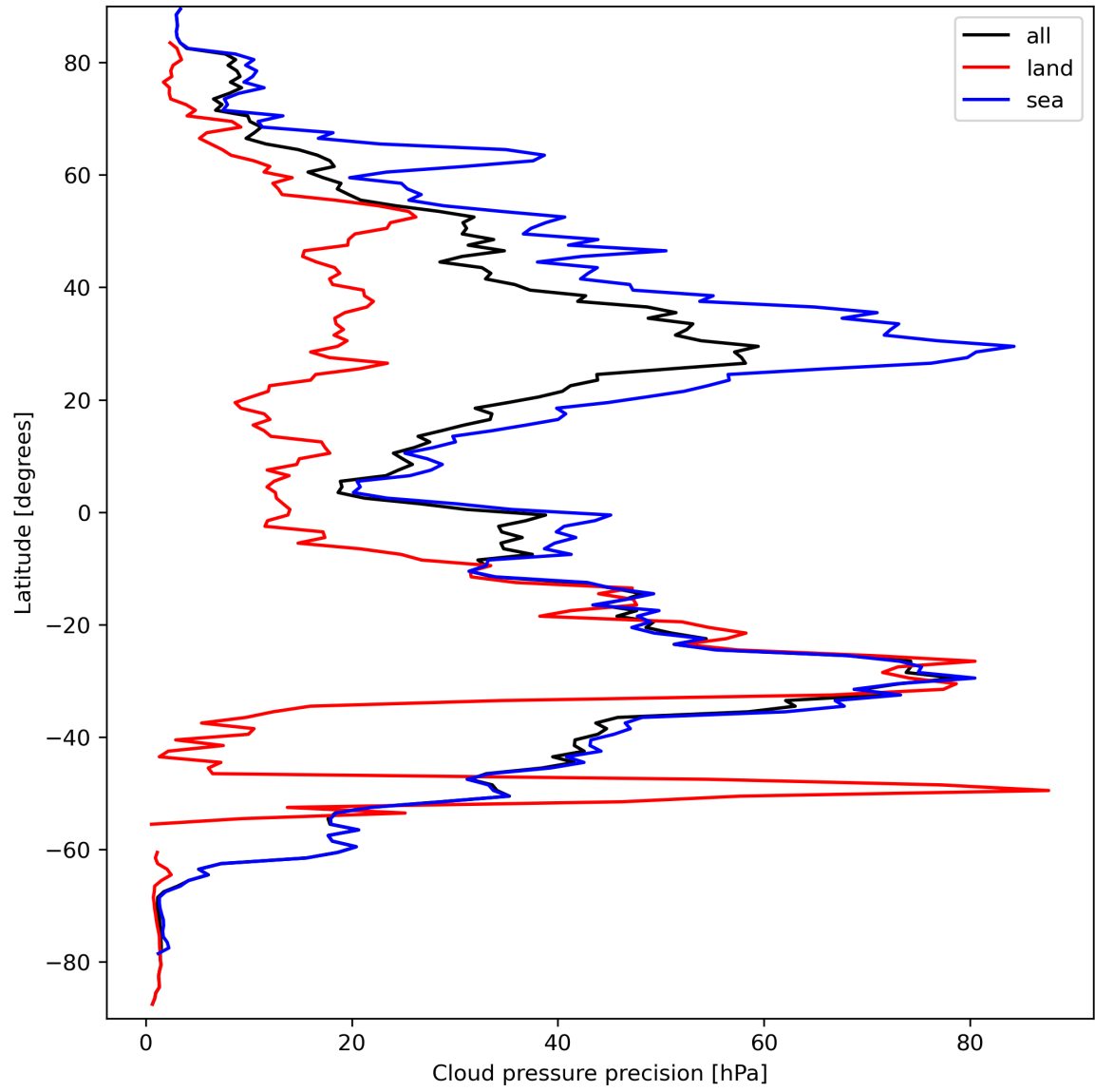
Figure 14: Zonal average of “Cloud pressure precision” for 2023-09-20 to 2023-09-21.
