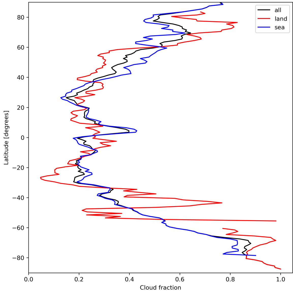
Figure 15: Zonal average of “Cloud fraction” for 2023-09-20 to 2023-09-21.
