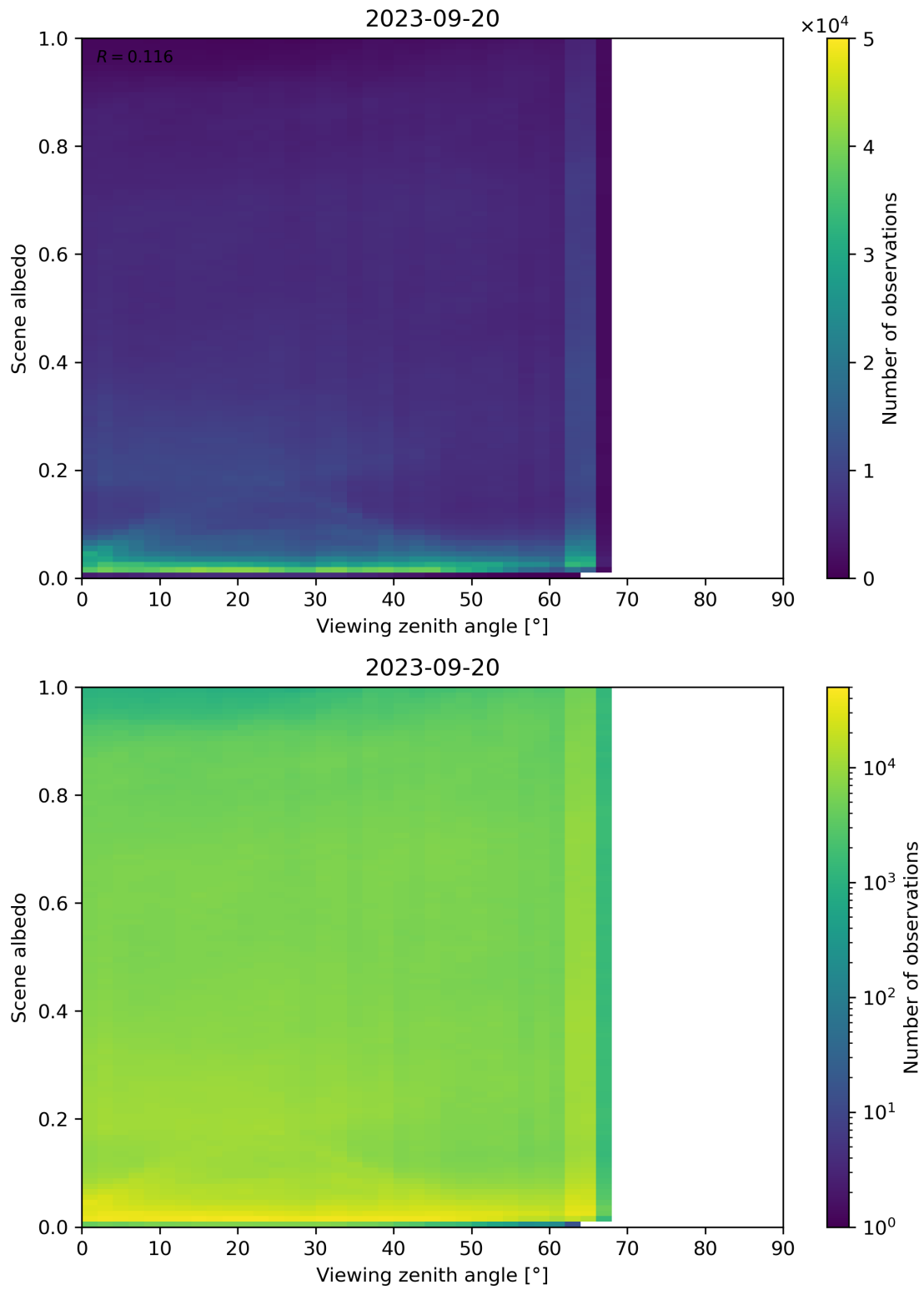
Figure 138: Scatter density plot of “Viewing zenith angle” against “Scene albedo” for 2023-09-20 to 2023-09-21.
