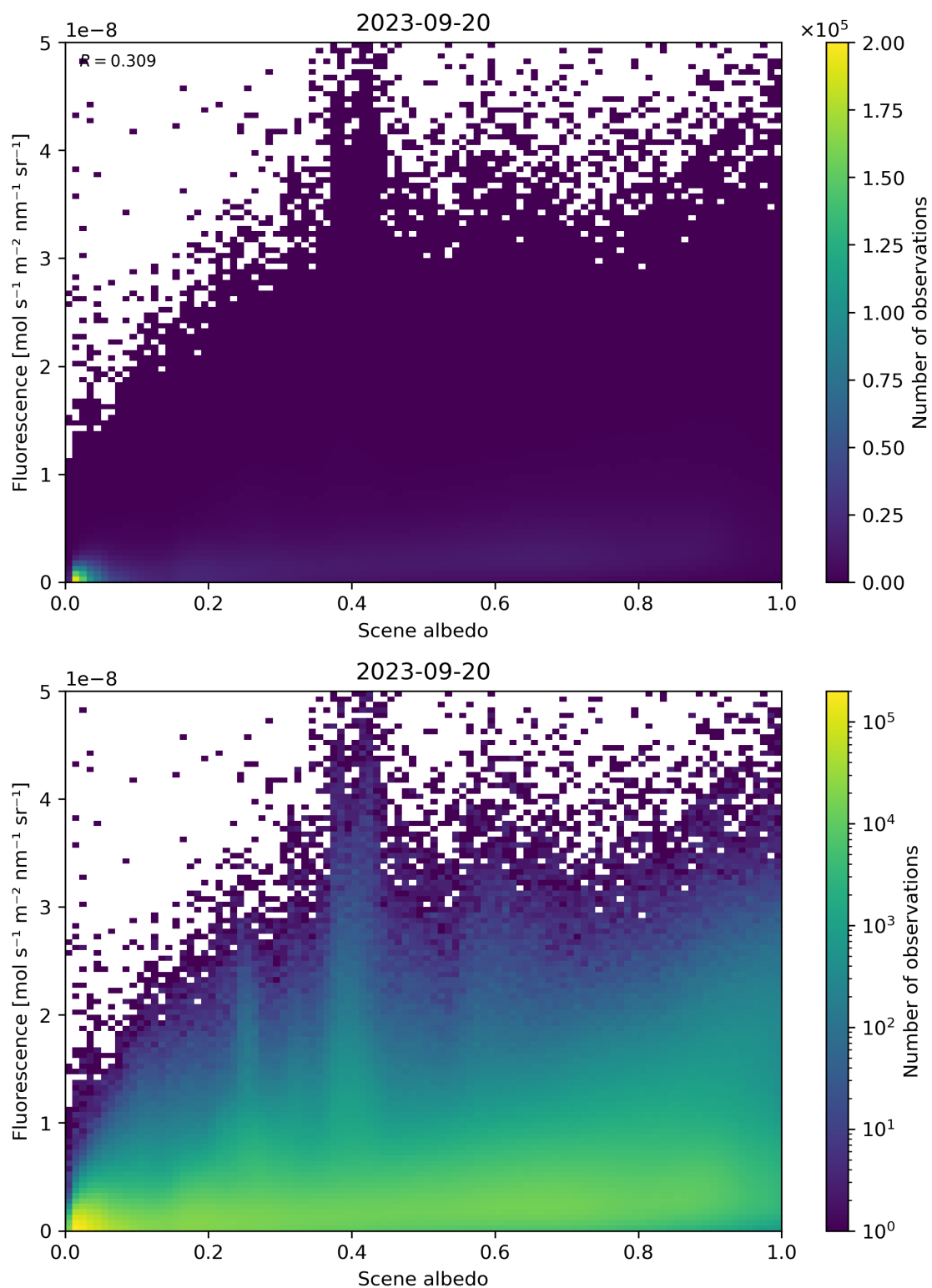
Figure 114: Scatter density plot of “Scene albedo” against “Fluorescence” for 2023-09-20 to 2023-09-21.
