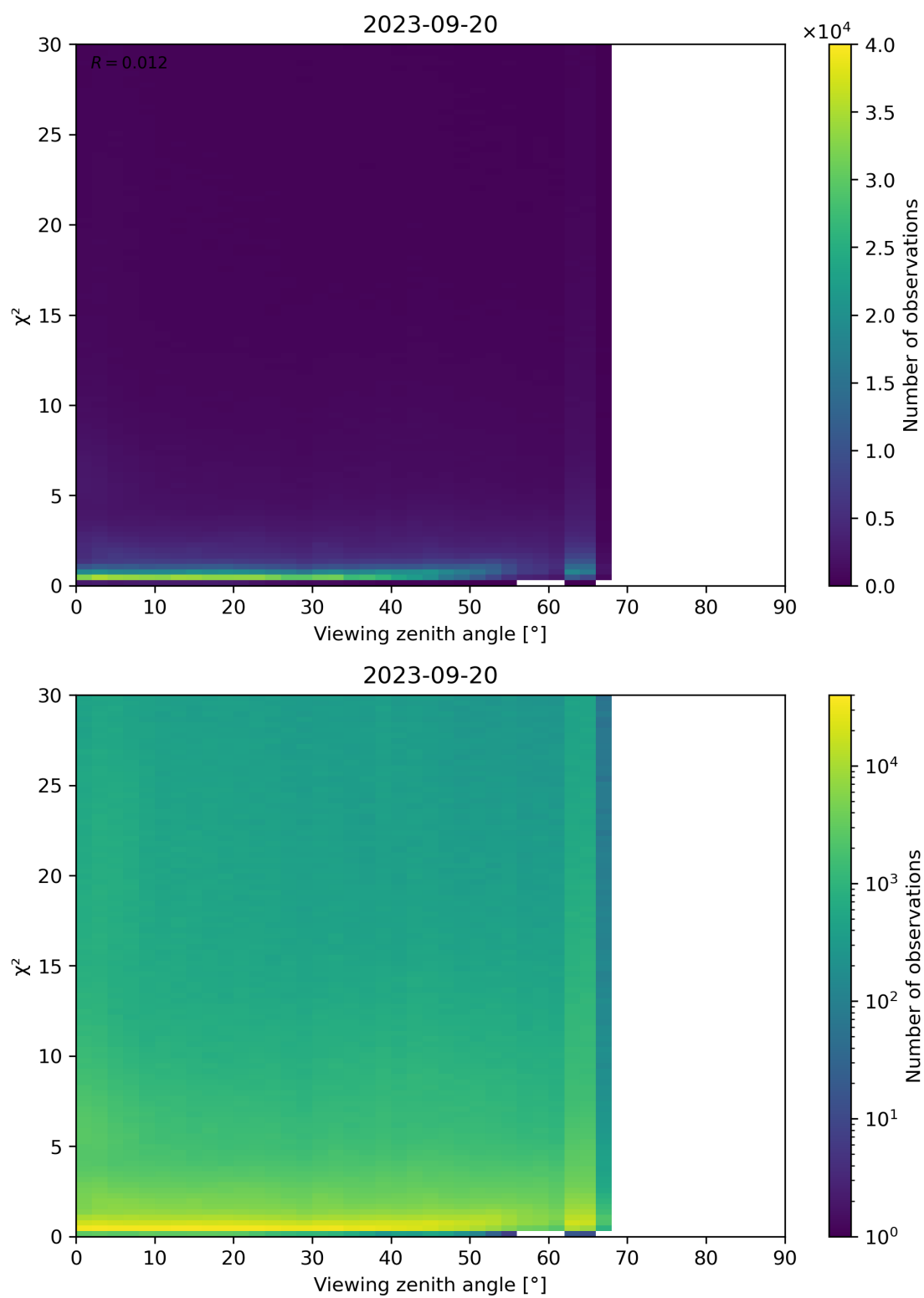
Figure 130: Scatter density plot of “Viewing zenith angle” against “ \chi^2 ” for 2023-09-20 to 2023-09-21.
