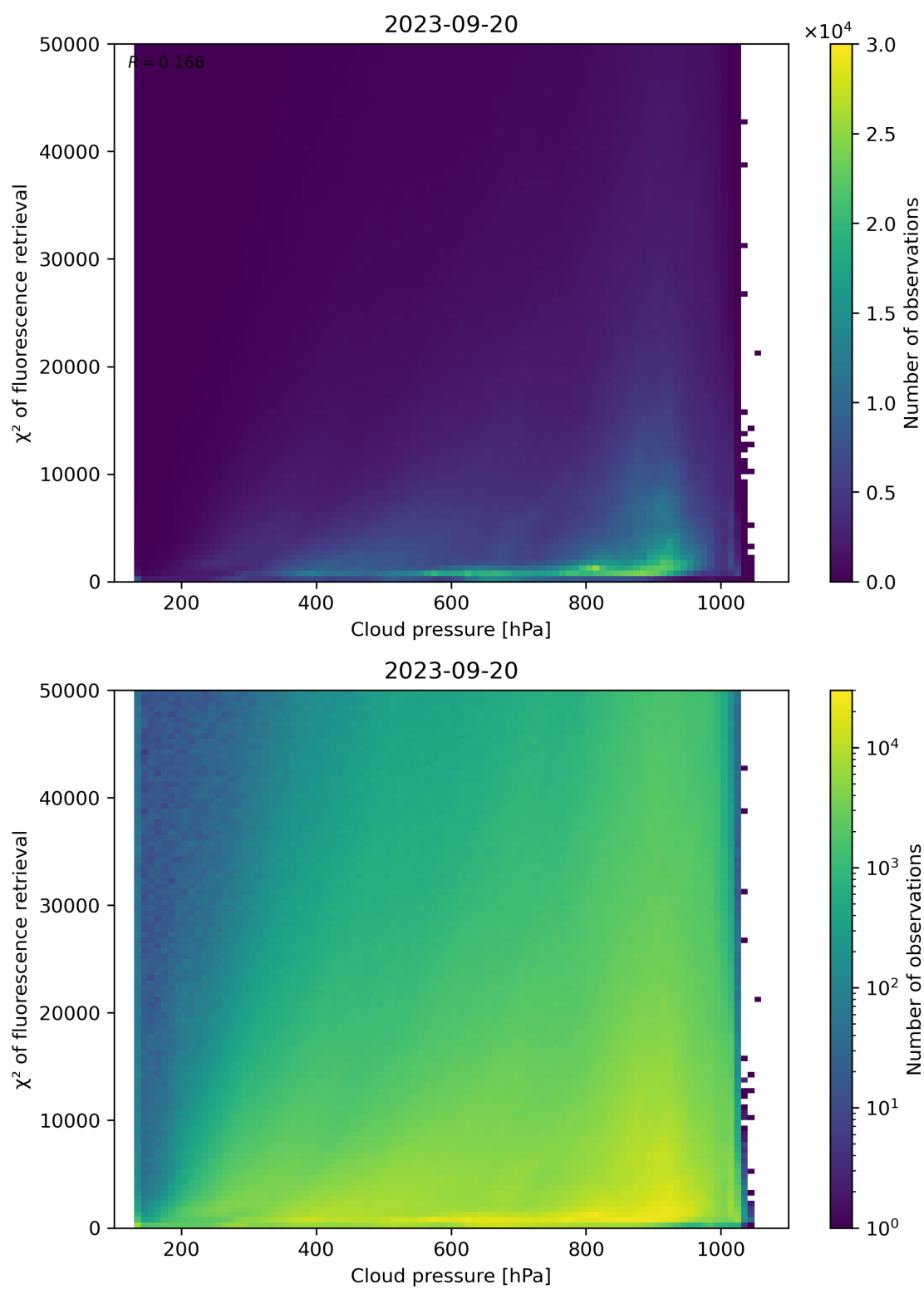
Figure 86: Scatter density plot of “Cloud pressure” against “ \chi^2 of fluorescence retrieval” for 2023-09-20 to 2023-09-21.
