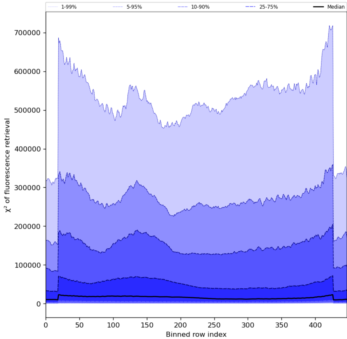
Figure 59: Along track statistics of “ \chi^2 of fluorescence retrieval” for 2023-09-20 to 2023-09-21
