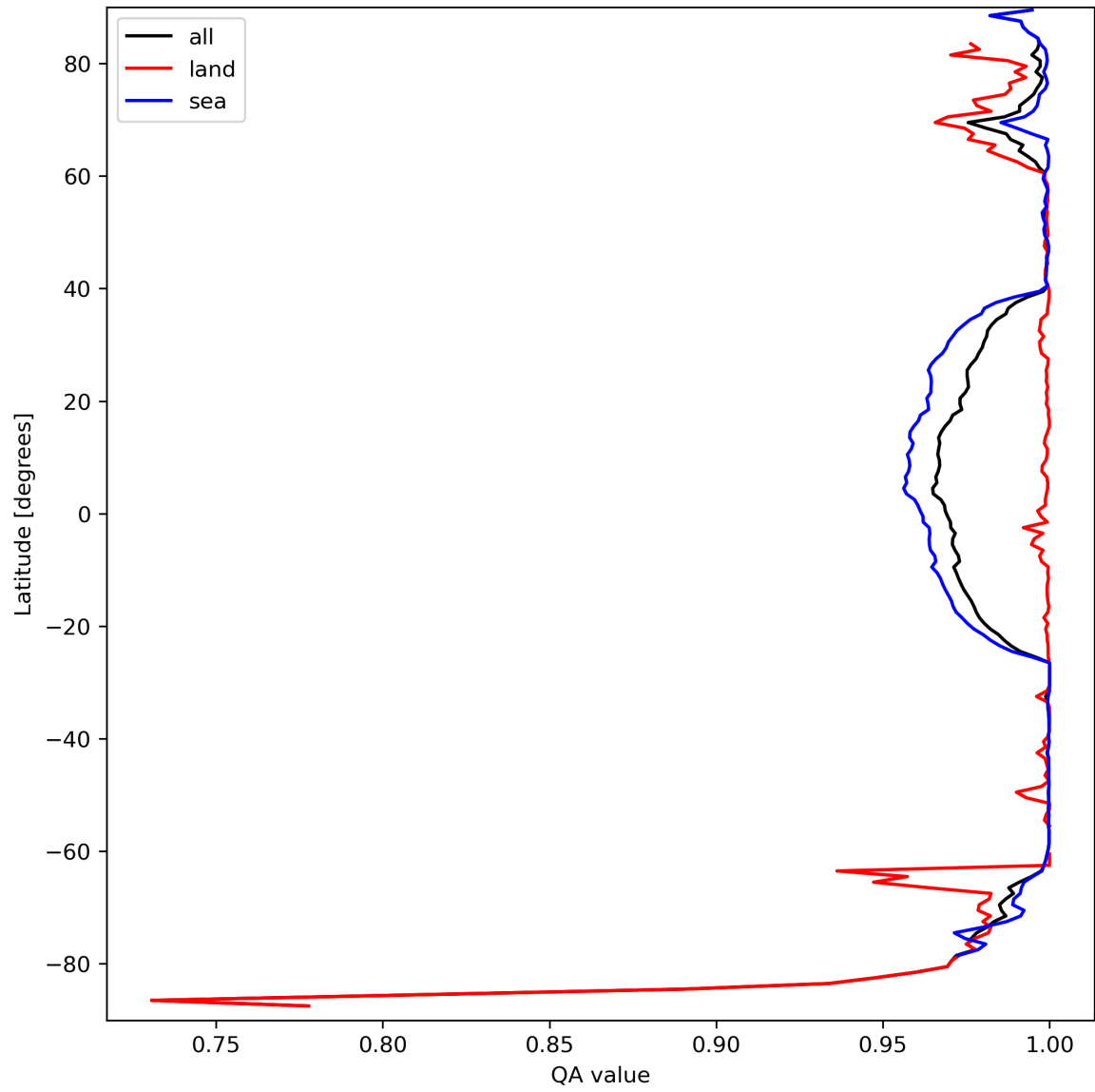
Figure 12: Zonal average of “QA value” for 2023-09-20 to 2023-09-21.
