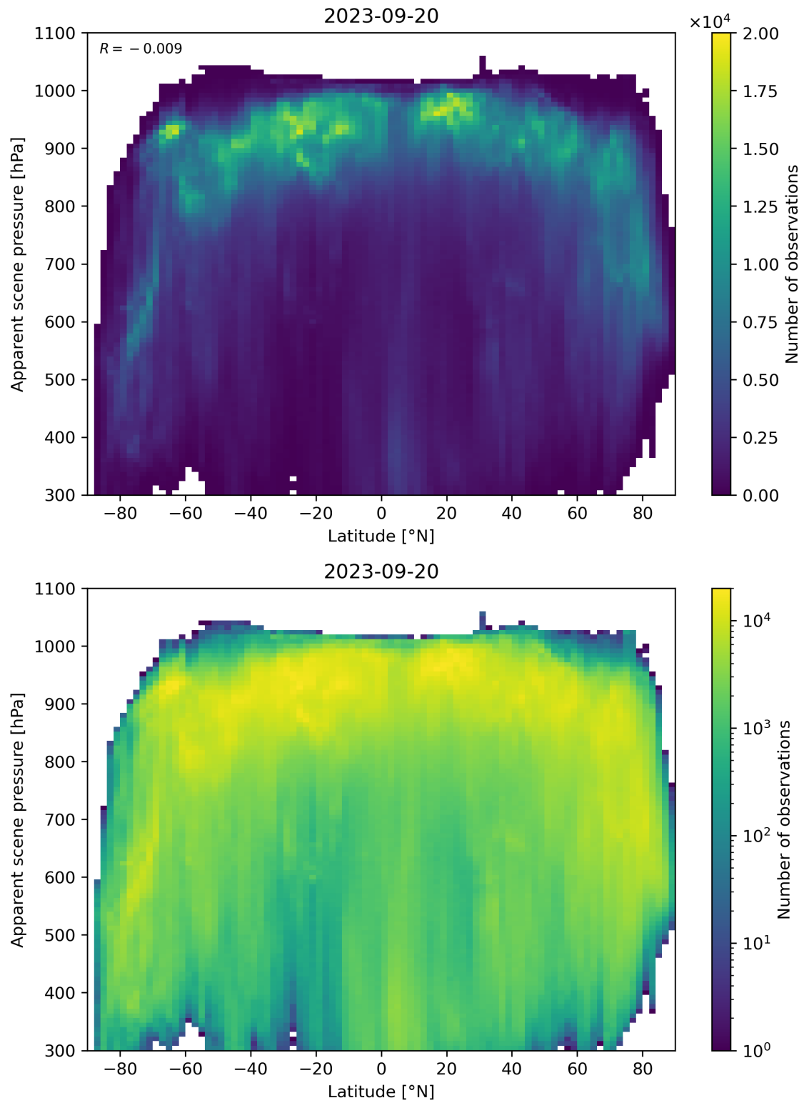
Figure 96: Scatter density plot of “Latitude” against “Apparent scene pressure” for 2023-09-20 to 2023-09-21.
