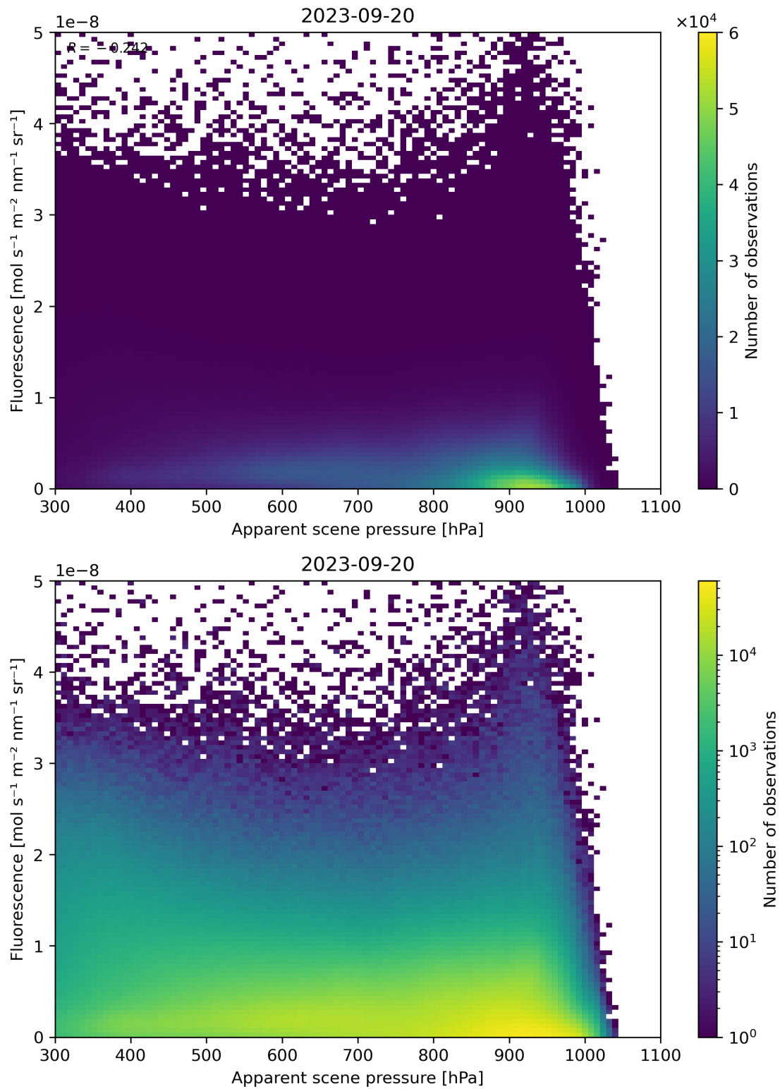
Figure 65: Scatter density plot of “Apparent scene pressure” against “Fluorescence” for 2023-09-20 to 2023-09-21.
