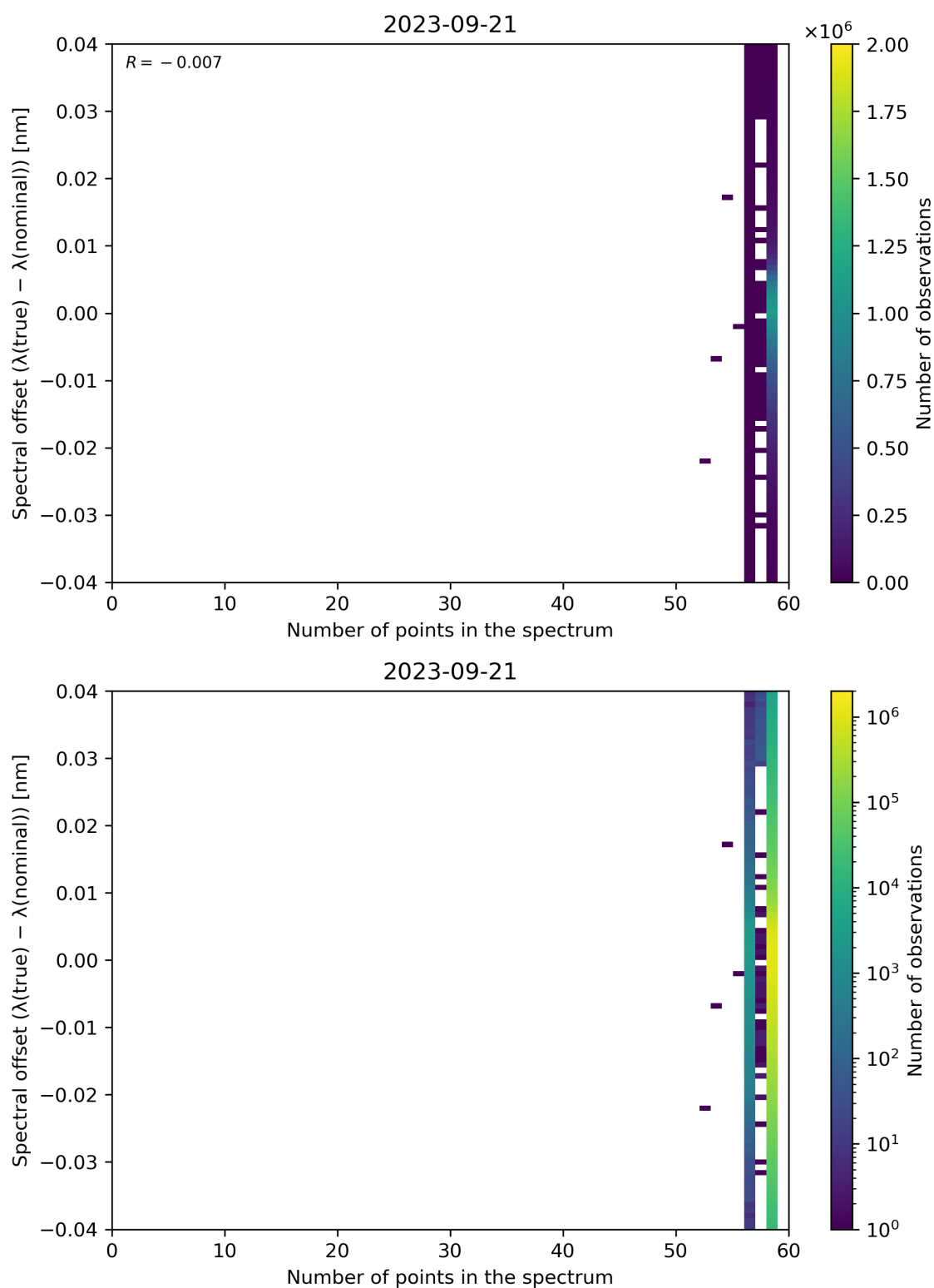
Figure 110: Scatter density plot of “Number of points in the spectrum” against “Spectral offset ( \lambda(\text{true}) - \lambda(\text{nominal}) )” for 2023-09-20 to 2023-09-22.
