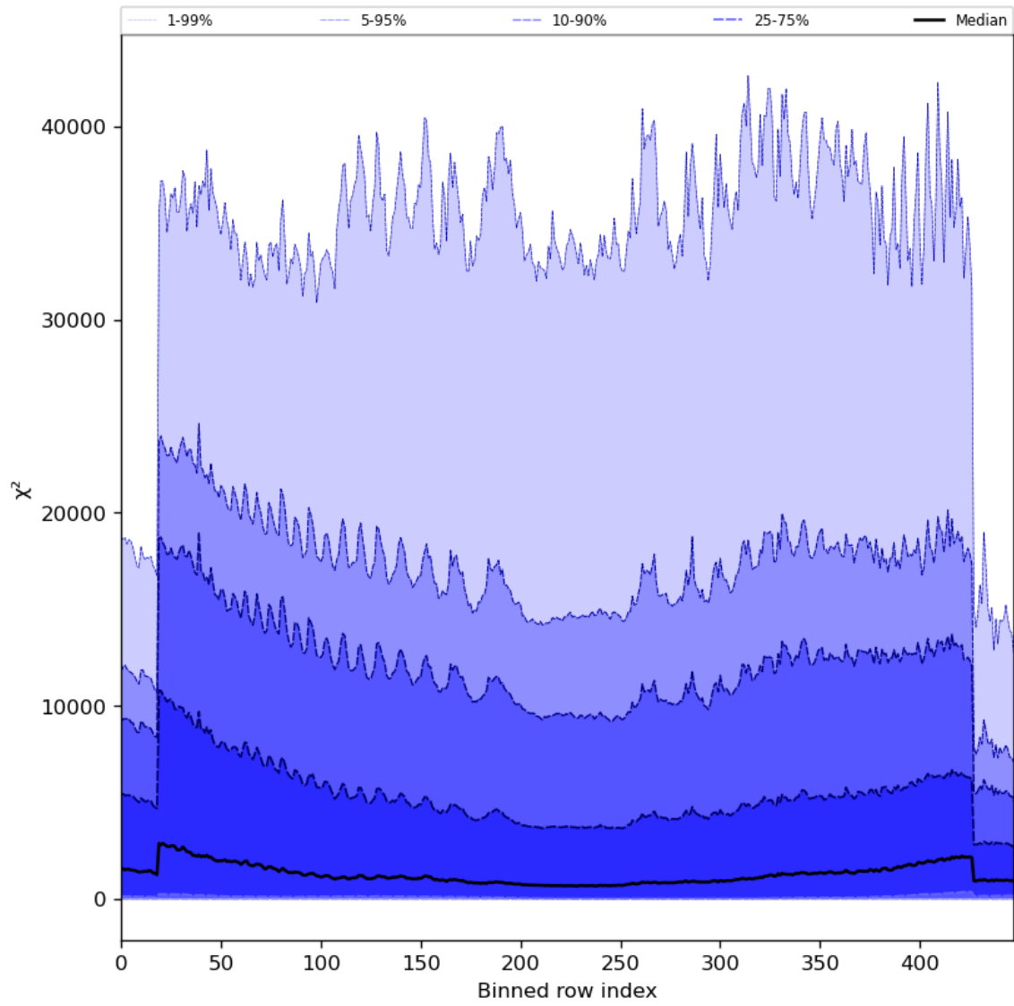
Figure 55: Along track statistics of “ \chi^2 ” for 2023-09-20 to 2023-09-22
