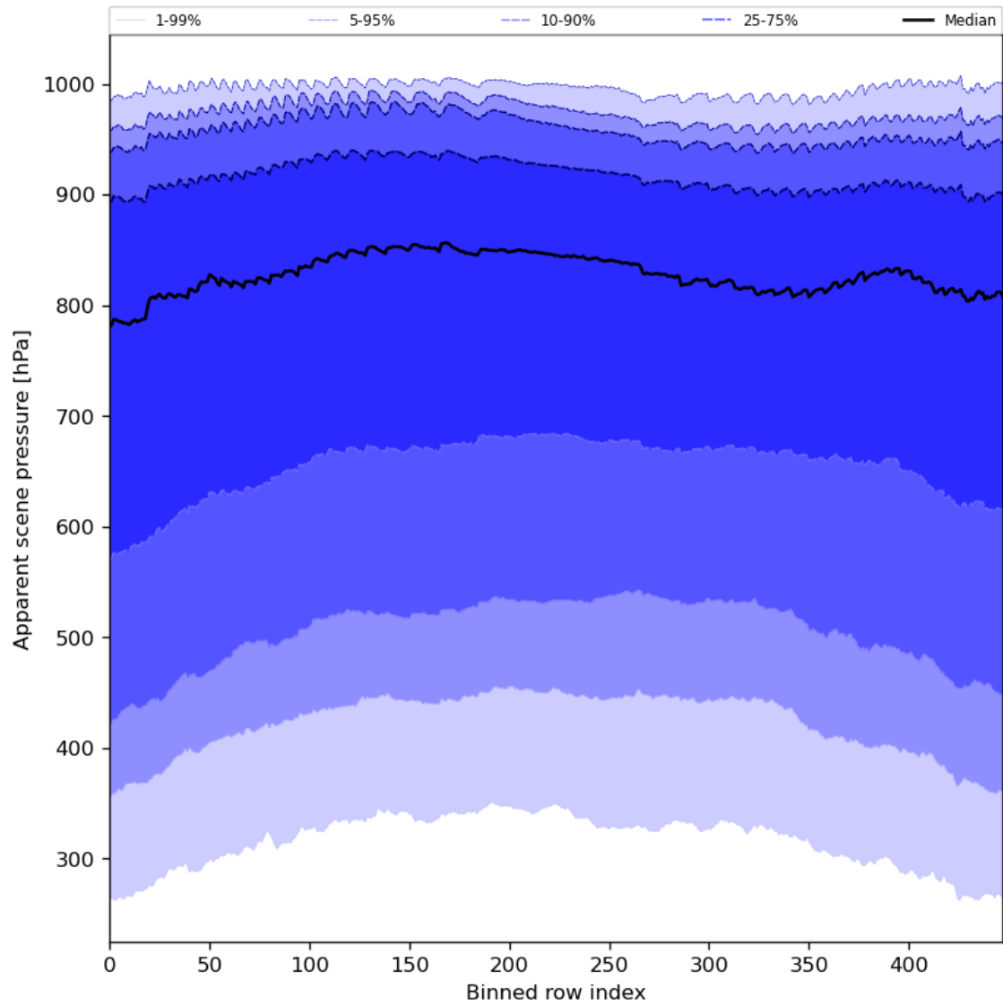
Figure 53: Along track statistics of “Apparent scene pressure” for 2023-09-20 to 2023-09-22
