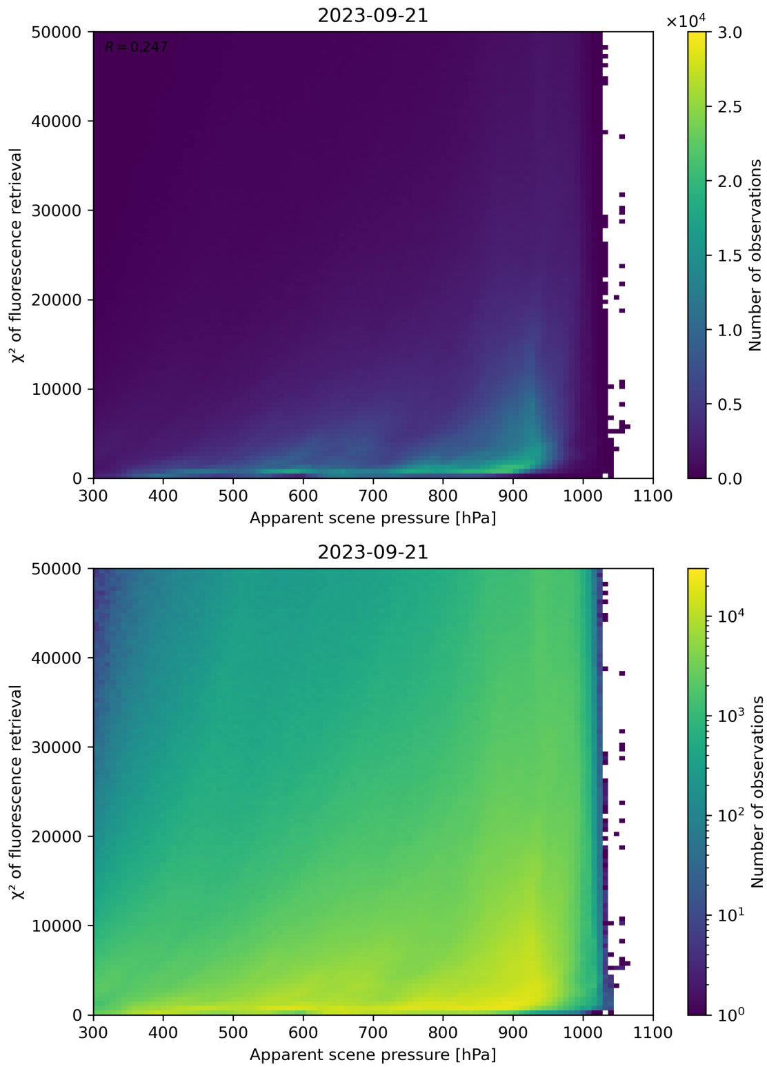
Figure 64: Scatter density plot of “Apparent scene pressure” against “ \chi^2 of fluorescence retrieval” for 2023-09-20 to 2023-09-22.
