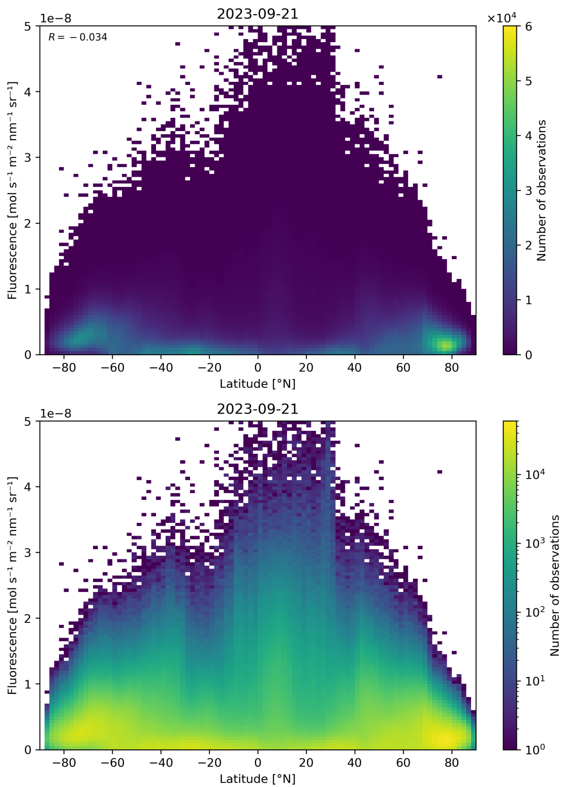
Figure 101: Scatter density plot of “Latitude” against “Fluorescence” for 2023-09-20 to 2023-09-22.
