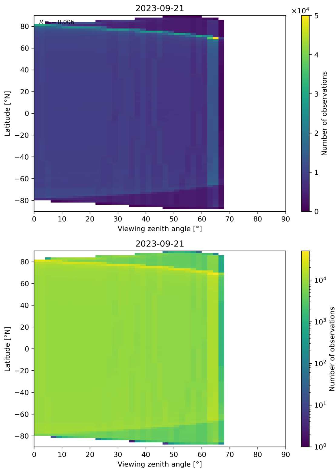
Figure 135: Scatter density plot of “Viewing zenith angle” against “Latitude” for 2023-09-20 to 2023-09-22.
