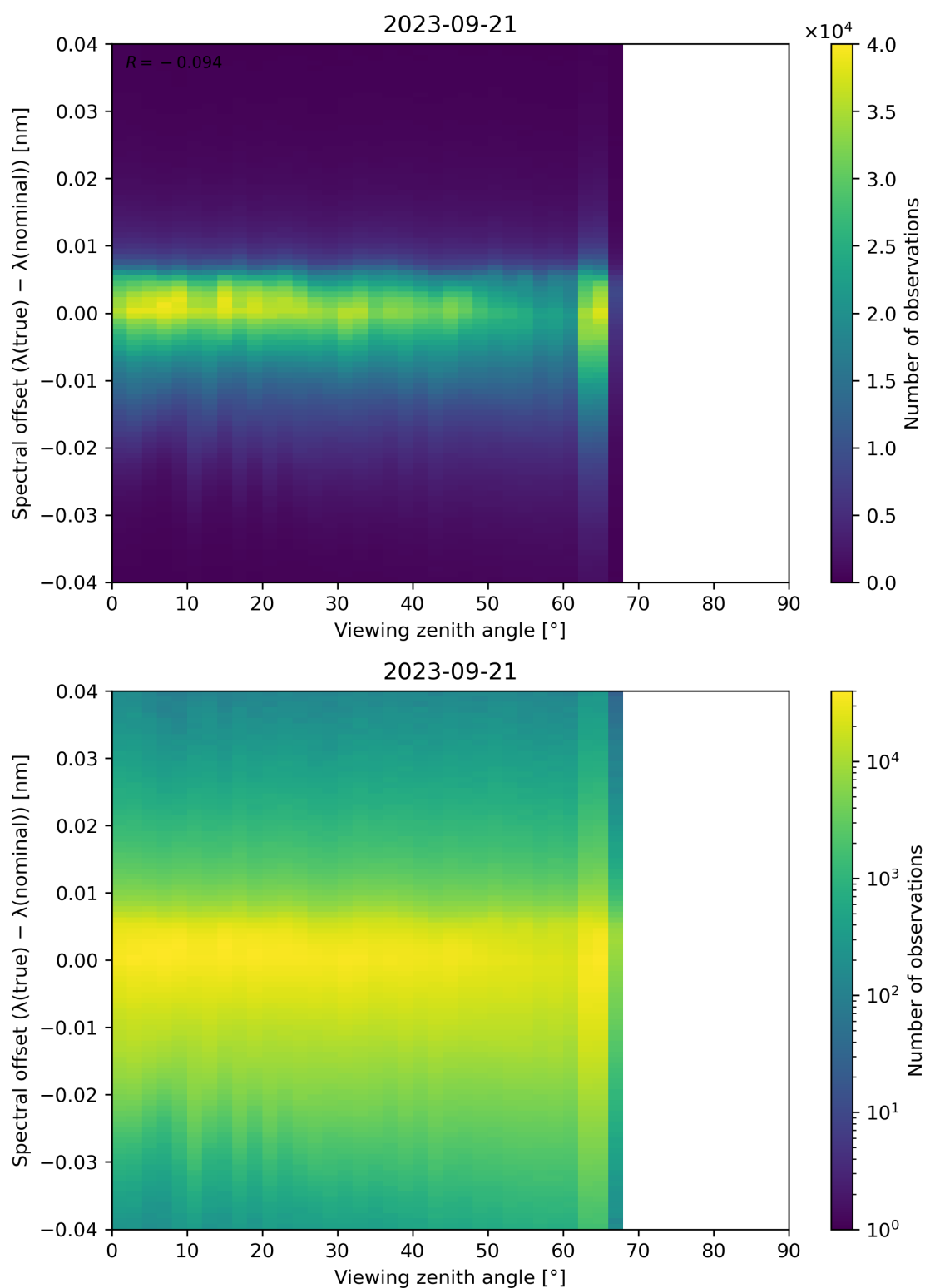
Figure 140: Scatter density plot of “Viewing zenith angle” against “Spectral offset ( \lambda(\text{true}) - \lambda(\text{nominal}) )” for 2023-09-20 to 2023-09-22.
