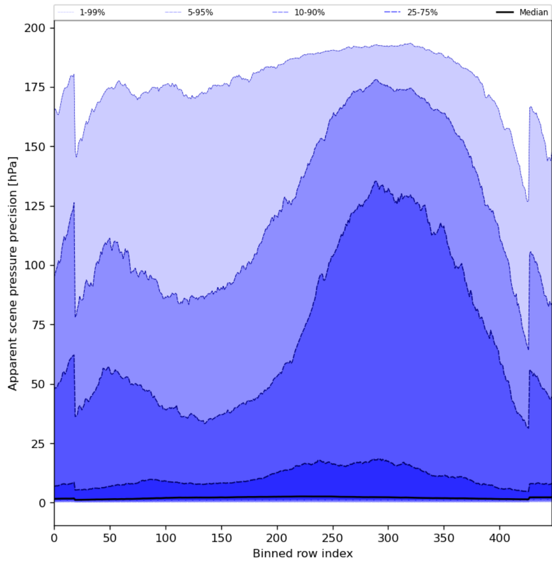
Figure 54: Along track statistics of “Apparent scene pressure precision” for 2023-09-20 to 2023-09-22
