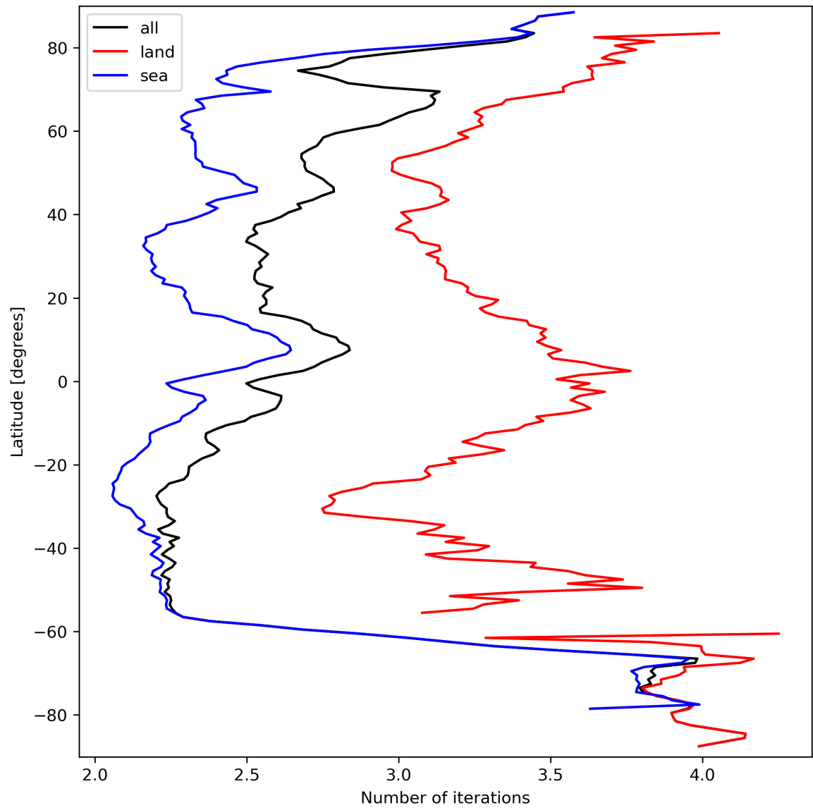
Figure 22: Zonal average of “Number of iterations” for 2023-09-20 to 2023-09-22.
