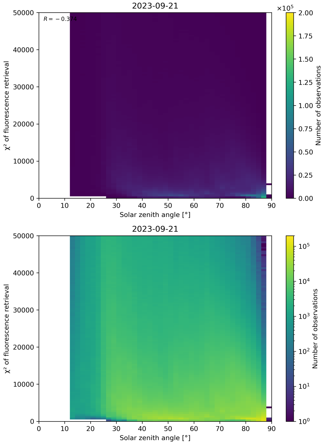
Figure 120: Scatter density plot of “Solar zenith angle” against “ \chi^2 of fluorescence retrieval” for 2023-09-20 to 2023-09-22.
