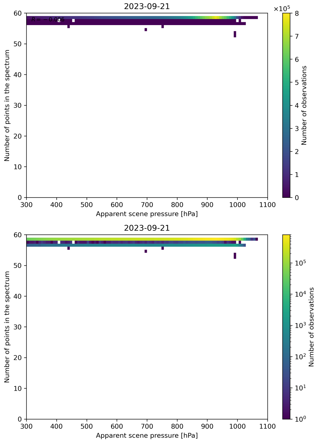
Figure 67: Scatter density plot of “Apparent scene pressure” against “Number of points in the spectrum” for 2023-09-20 to 2023-09-22.
