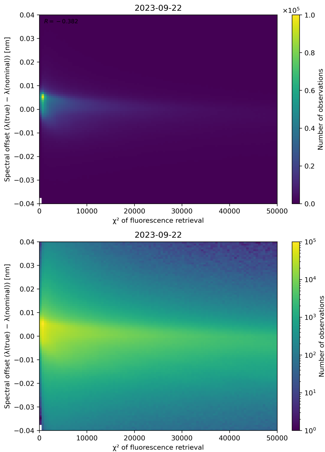
Figure 72: Scatter density plot of “ \chi^2 of fluorescence retrieval” against “Spectral offset ( \lambda(\text{true}) - \lambda(\text{nominal}) )” for 2023-09-21 to 2023-09-23.
