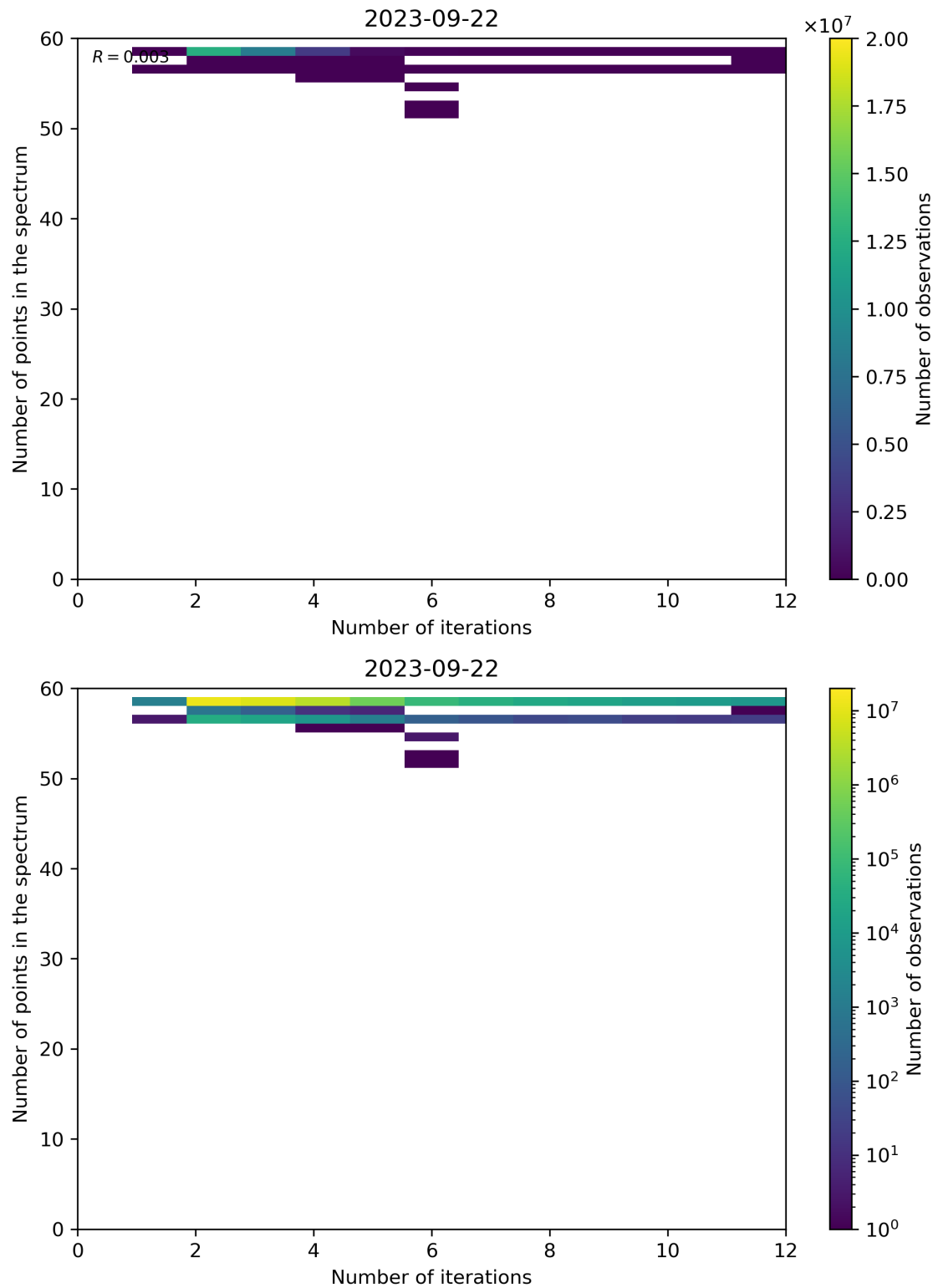
Figure 108: Scatter density plot of “Number of iterations” against “Number of points in the spectrum” for 2023-09-21 to 2023-09-23.
