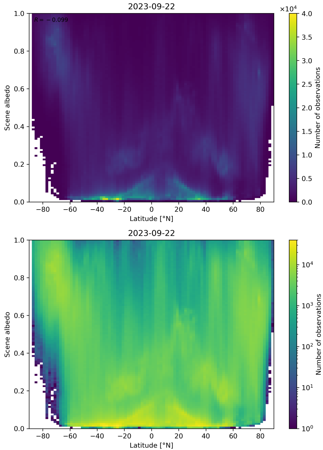
Figure 104: Scatter density plot of “Latitude” against “Scene albedo” for 2023-09-21 to 2023-09-23.
