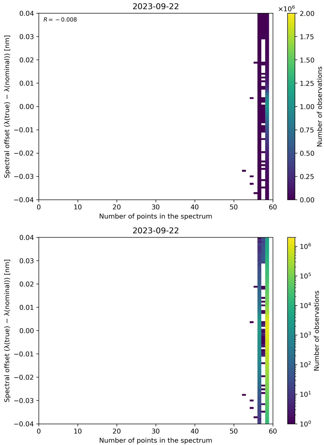
Figure 110: Scatter density plot of “Number of points in the spectrum” against “Spectral offset ( \lambda(\text{true}) - \lambda(\text{nominal}) )” for 2023-09-21 to 2023-09-23.
