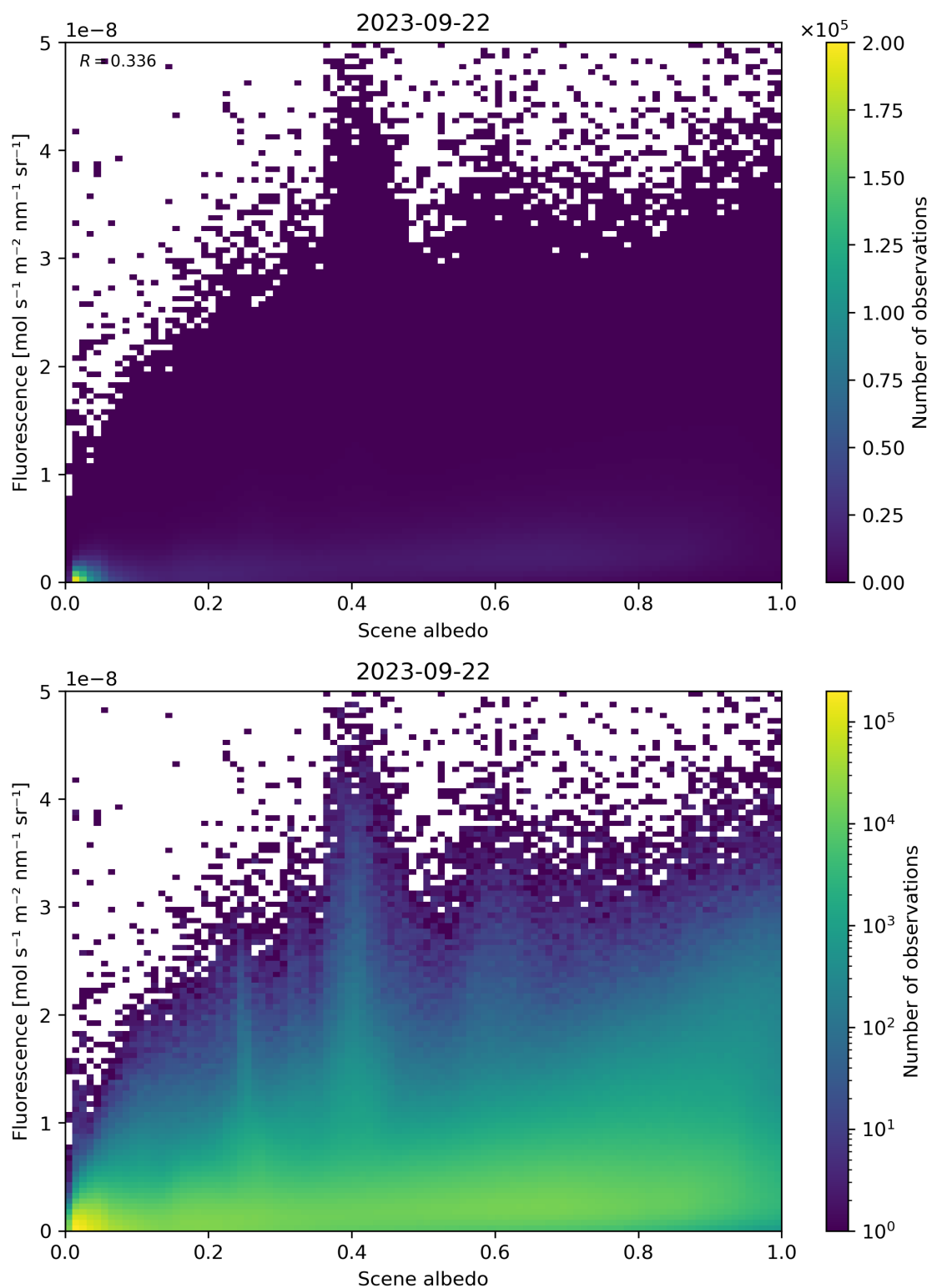
Figure 114: Scatter density plot of “Scene albedo” against “Fluorescence” for 2023-09-21 to 2023-09-23.
