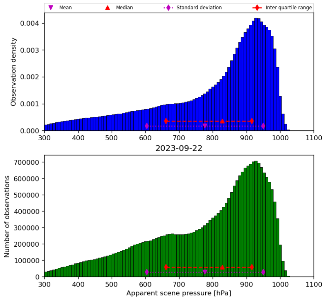
Figure 36: Histogram of “Apparent scene pressure” for 2023-09-21 to 2023-09-23
