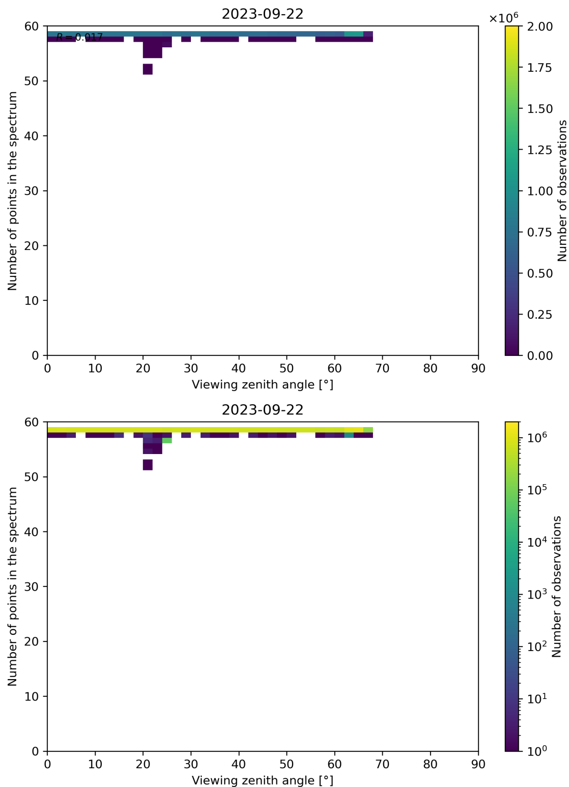
Figure 137: Scatter density plot of “Viewing zenith angle” against “Number of points in the spectrum” for 2023-09-21 to 2023-09-23.
