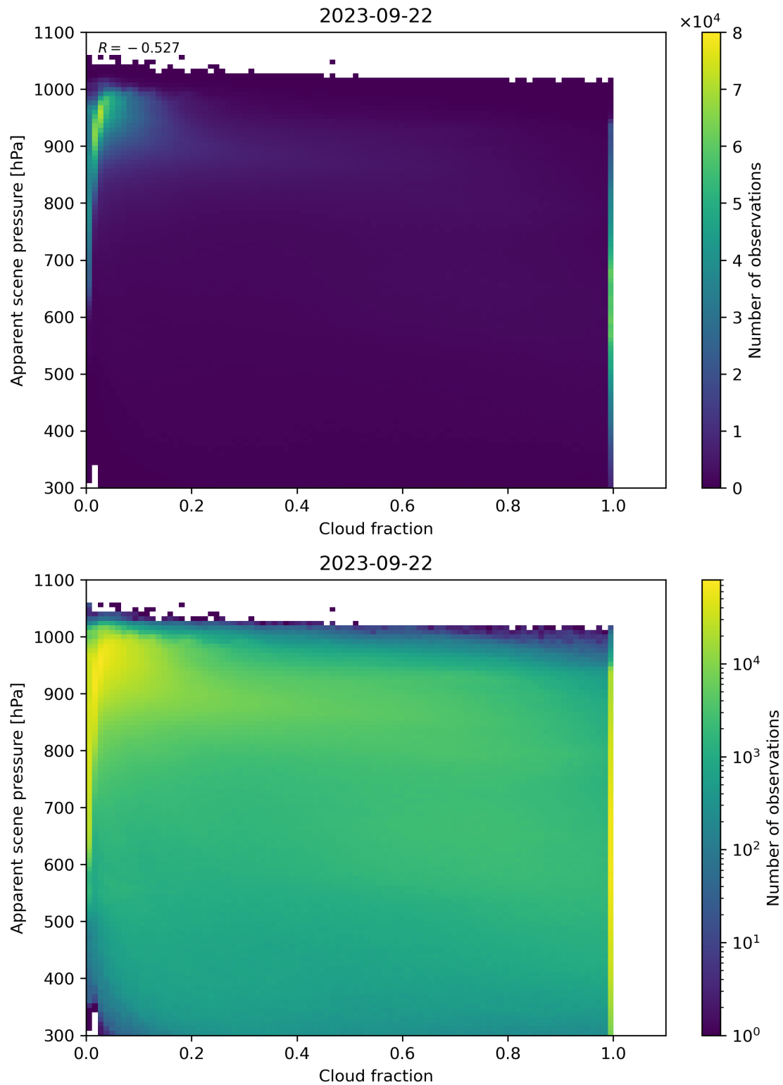
Figure 76: Scatter density plot of “Cloud fraction” against “Apparent scene pressure” for 2023-09-21 to 2023-09-23.
