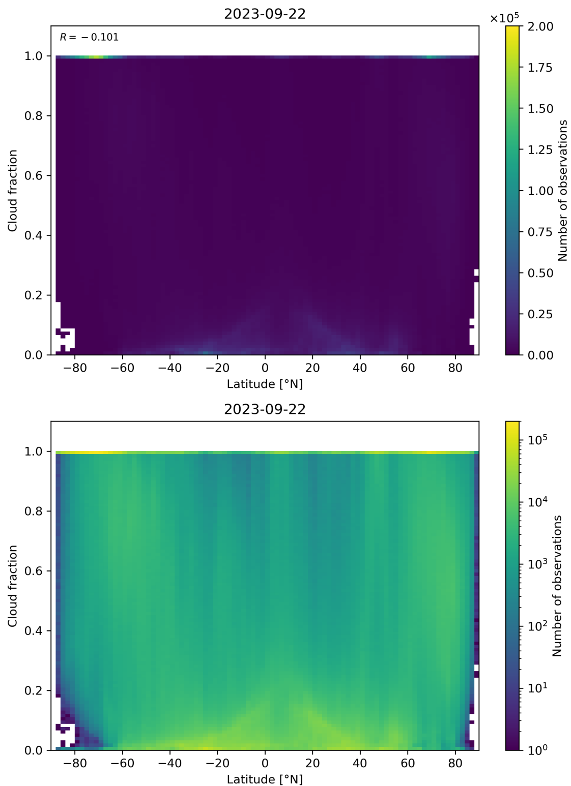
Figure 99: Scatter density plot of “Latitude” against “Cloud fraction” for 2023-09-21 to 2023-09-23.
