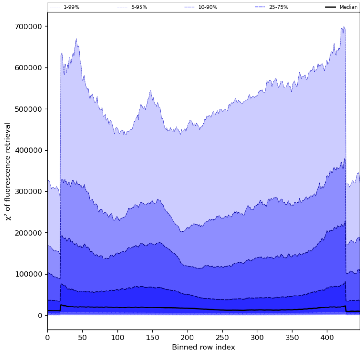
Figure 59: Along track statistics of “ \chi^2 of fluorescence retrieval” for 2023-09-21 to 2023-09-23
