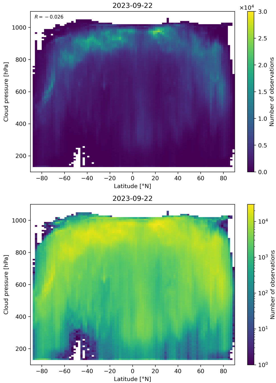
Figure 100: Scatter density plot of “Latitude” against “Cloud pressure” for 2023-09-21 to 2023-09-23.
