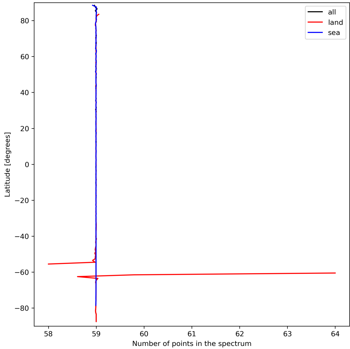
Figure 27: Zonal average of “Number of points in the spectrum” for 2023-09-21 to 2023-09-23.
