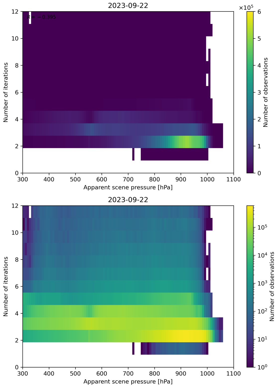
Figure 66: Scatter density plot of “Apparent scene pressure” against “Number of iterations” for 2023-09-21 to 2023-09-23.
