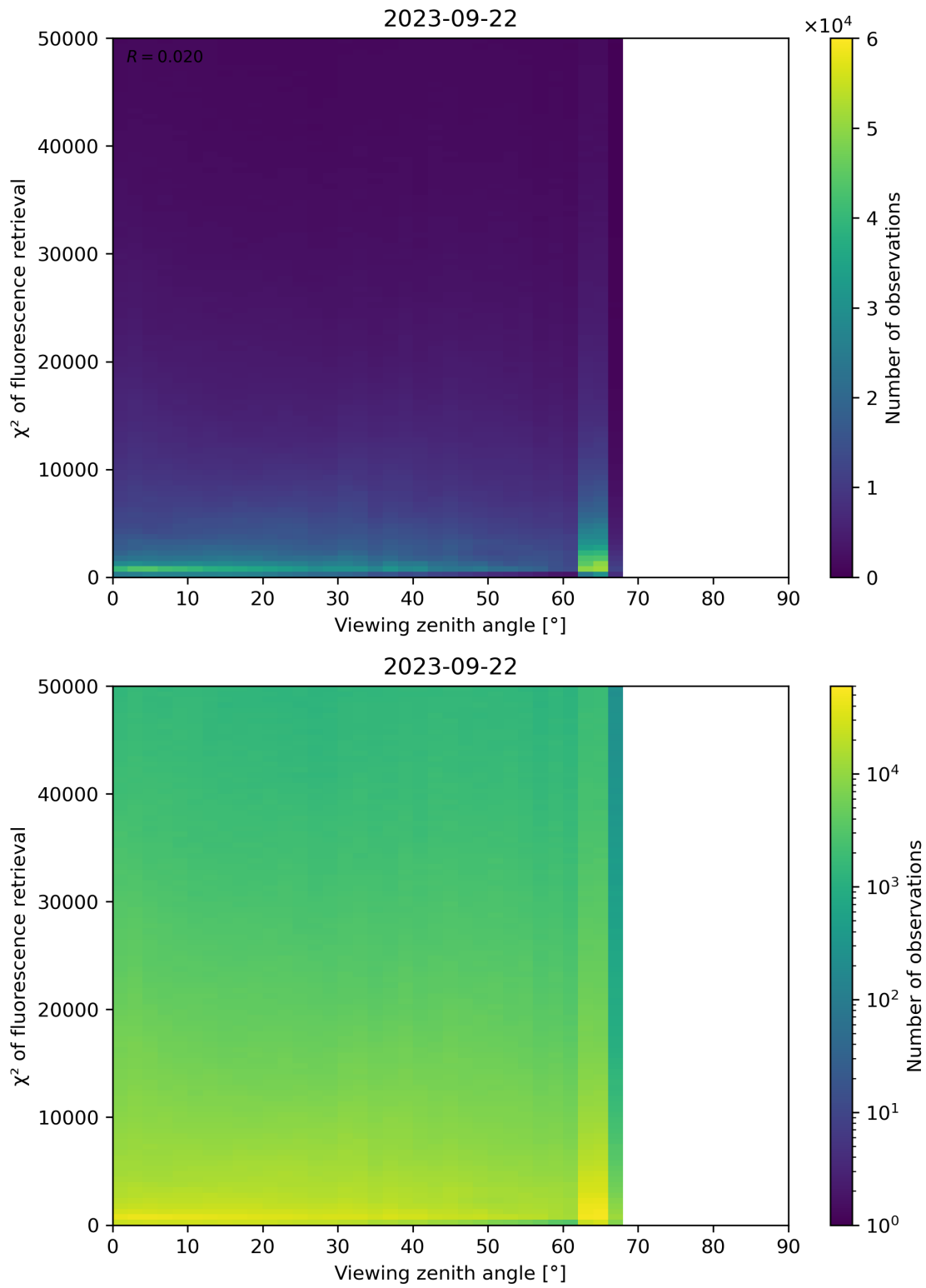
Figure 131: Scatter density plot of “Viewing zenith angle” against “ \chi^2 of fluorescence retrieval” for 2023-09-21 to 2023-09-23.
