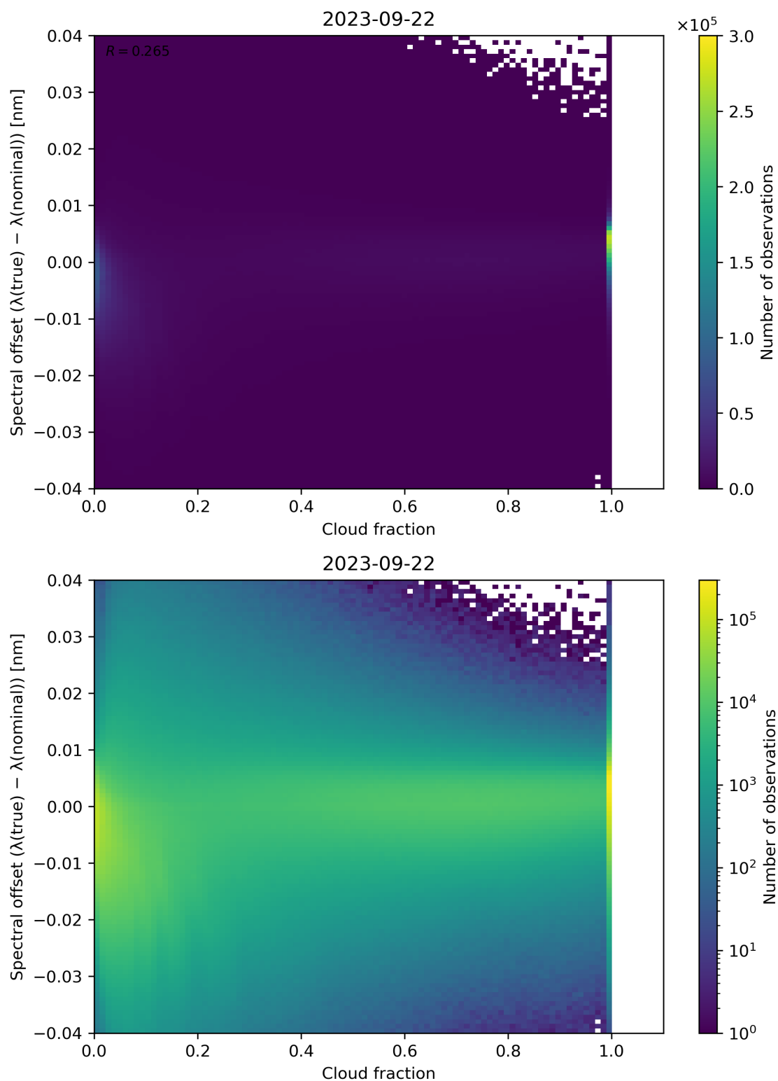
Figure 83: Scatter density plot of “Cloud fraction” against “Spectral offset ( \lambda(\text{true}) - \lambda(\text{nominal}) )” for 2023-09-21 to 2023-09-23.
