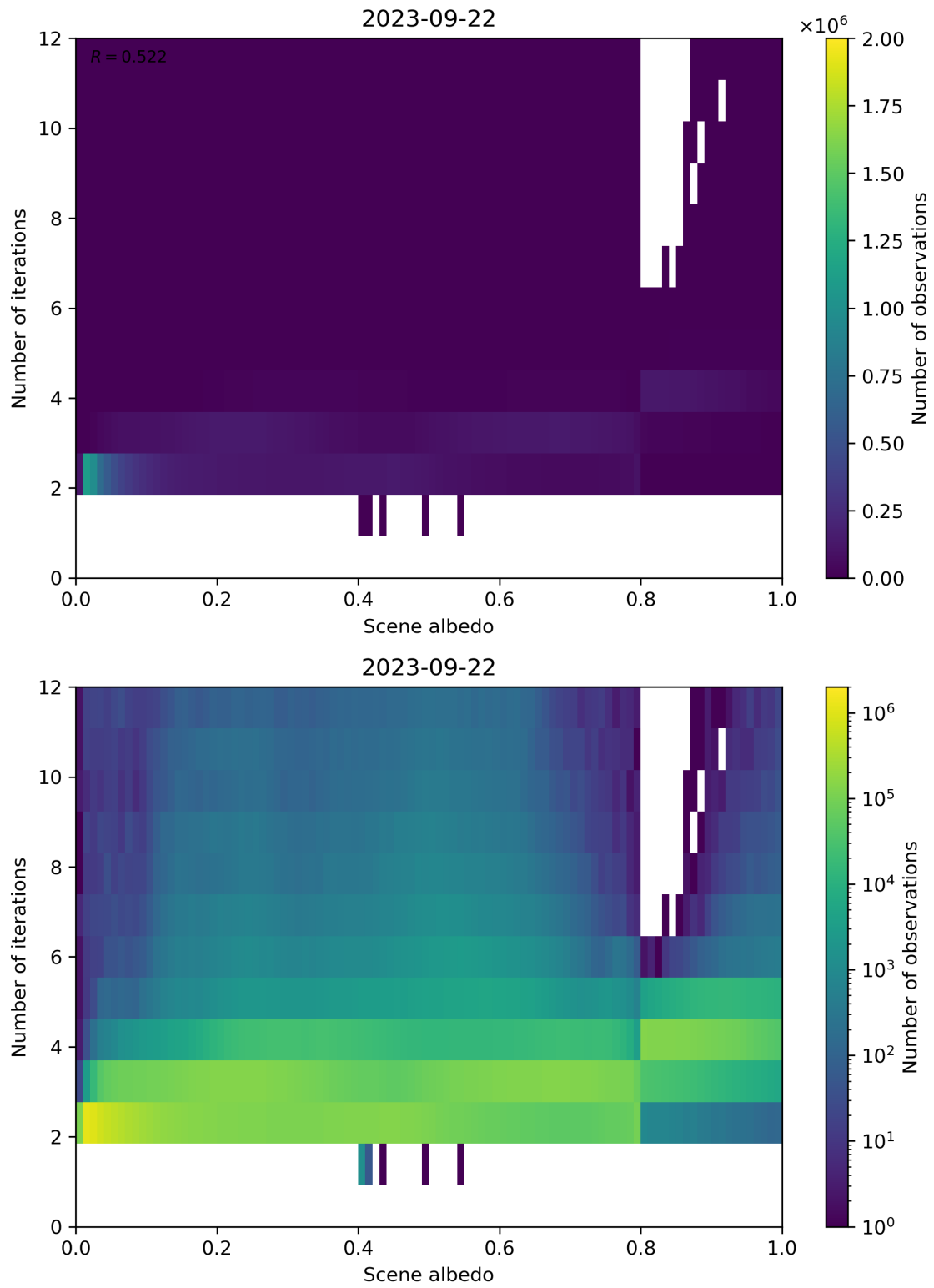
Figure 115: Scatter density plot of “Scene albedo” against “Number of iterations” for 2023-09-21 to 2023-09-23.
