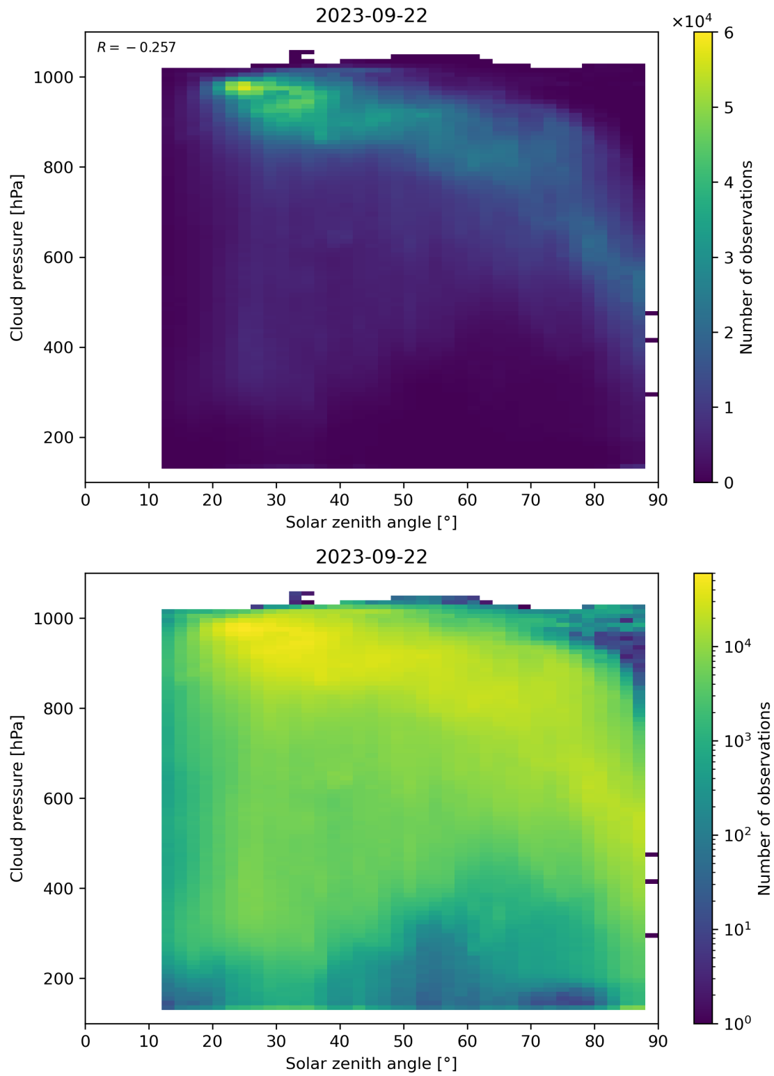
Figure 122: Scatter density plot of “Solar zenith angle” against “Cloud pressure” for 2023-09-21 to 2023-09-23.
