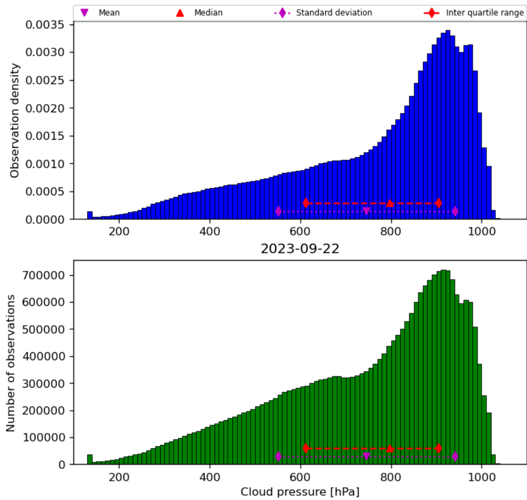
Figure 30: Histogram of “Cloud pressure” for 2023-09-21 to 2023-09-23
