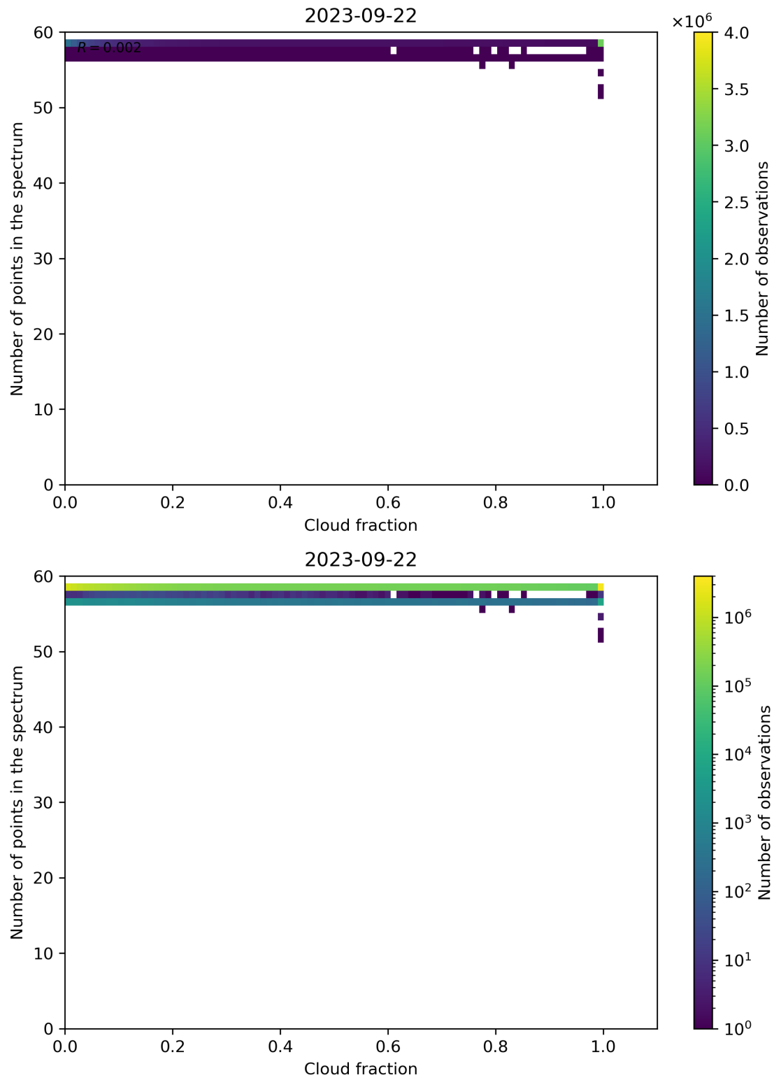
Figure 81: Scatter density plot of “Cloud fraction” against “Number of points in the spectrum” for 2023-09-21 to 2023-09-23.
