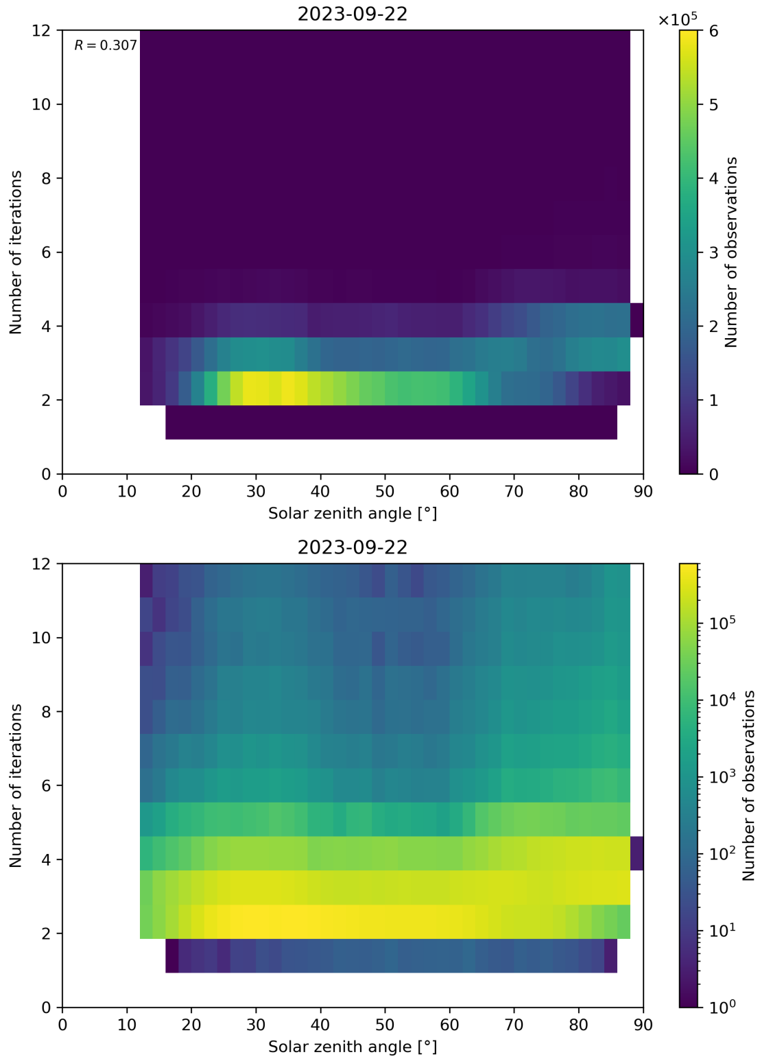
Figure 125: Scatter density plot of “Solar zenith angle” against “Number of iterations” for 2023-09-21 to 2023-09-23.
