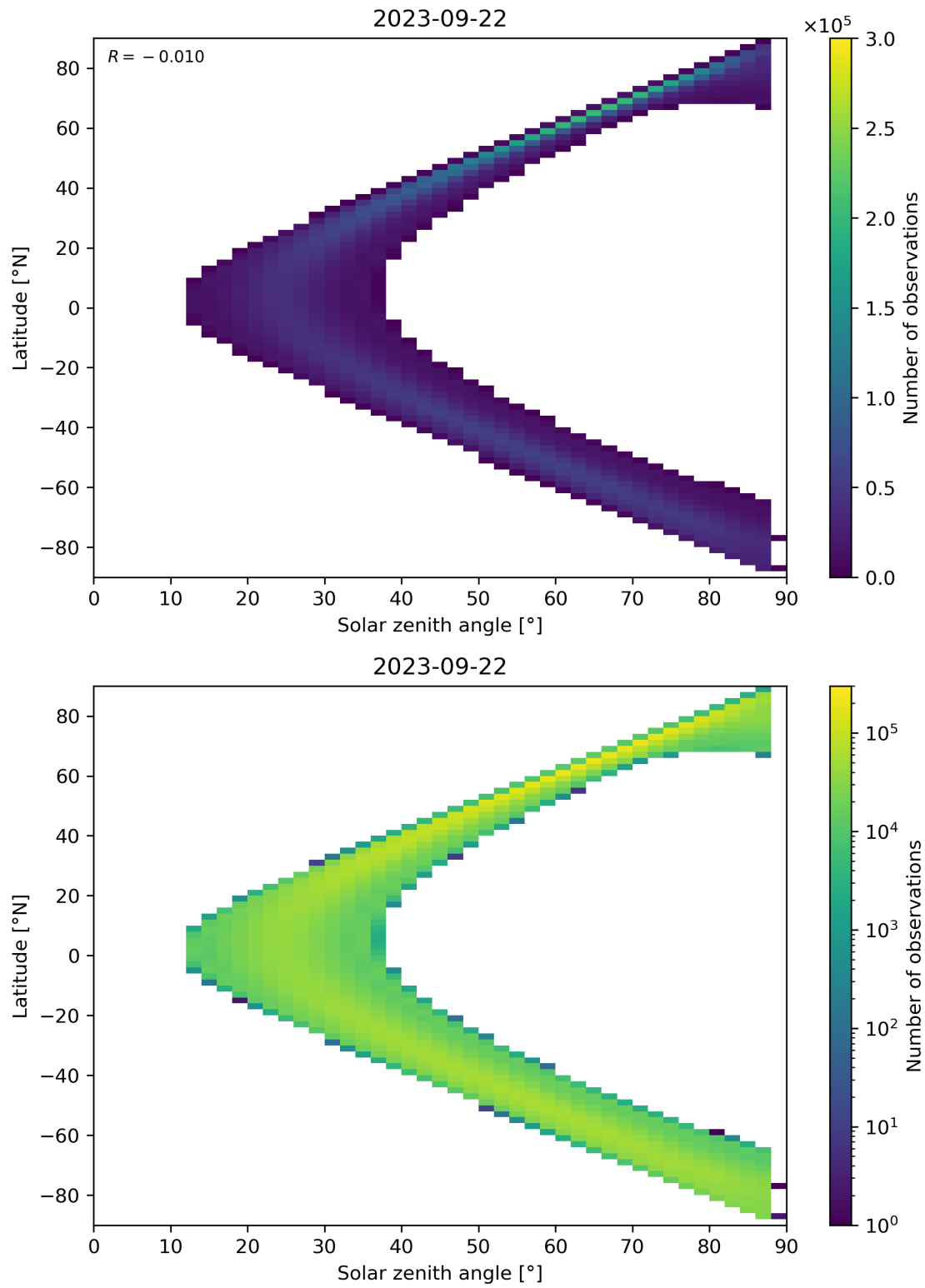
Figure 124: Scatter density plot of “Solar zenith angle” against “Latitude” for 2023-09-21 to 2023-09-23.
