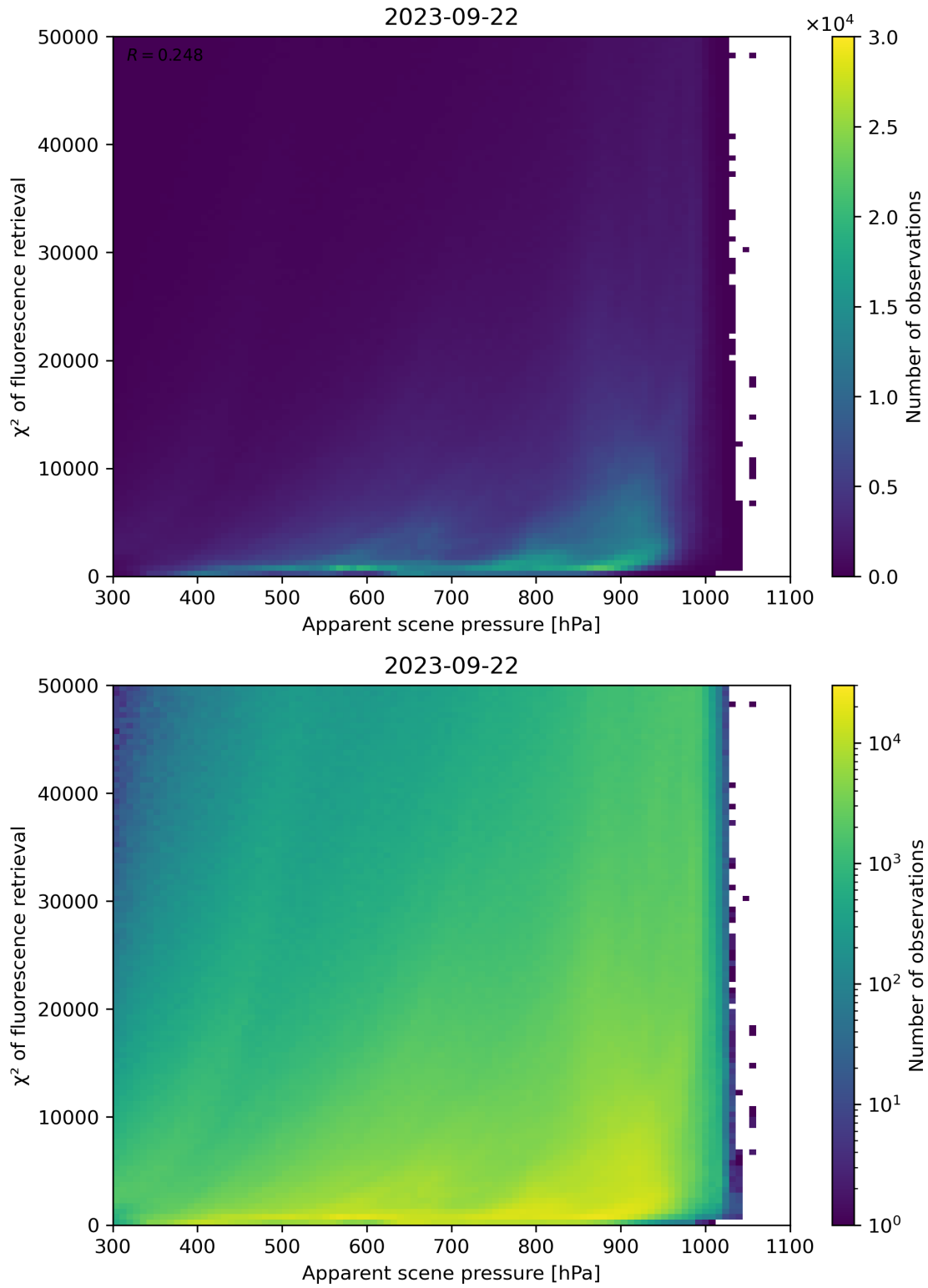
Figure 64: Scatter density plot of “Apparent scene pressure” against “ \chi^2 of fluorescence retrieval” for 2023-09-21 to 2023-09-23.
