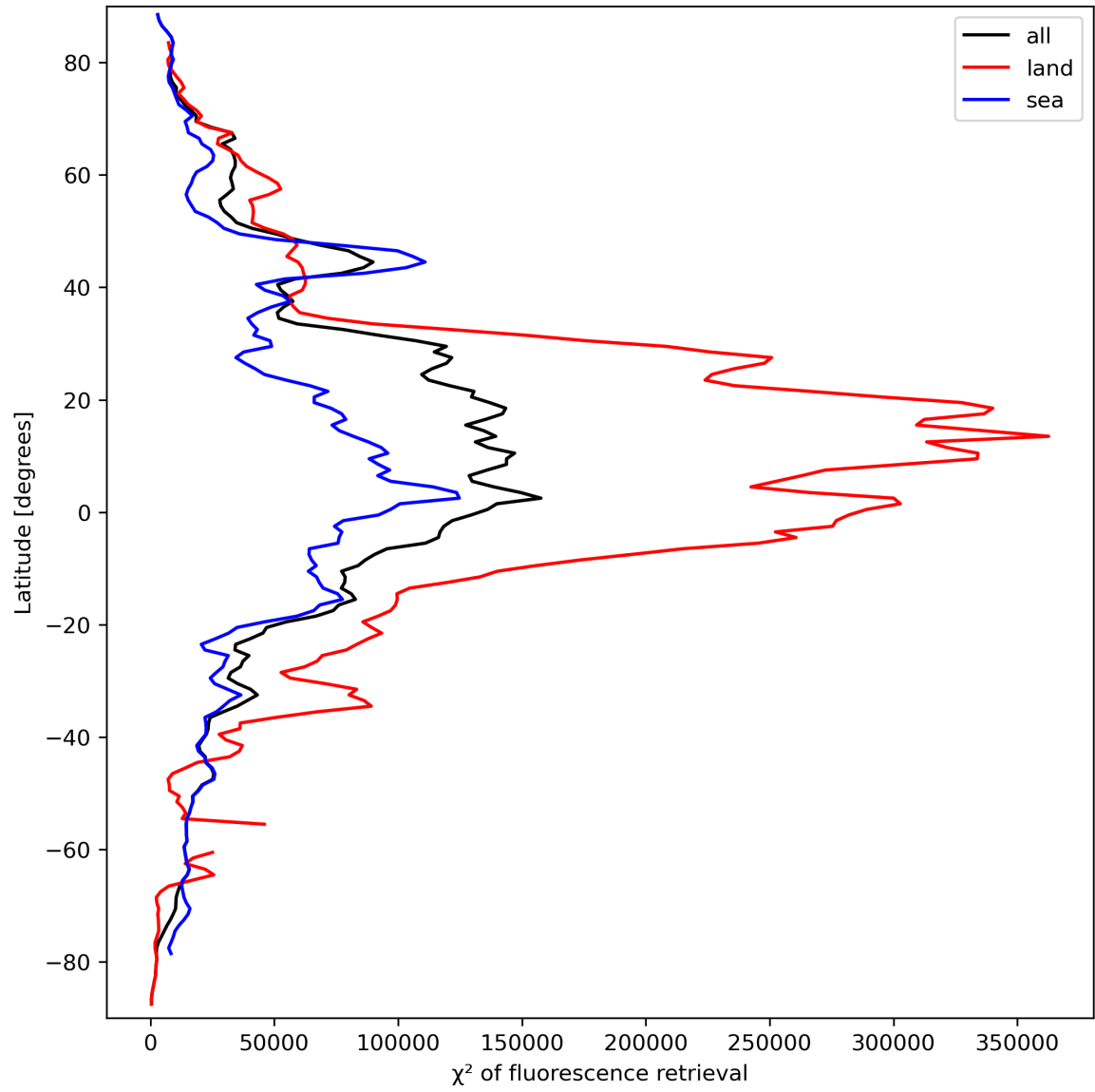
Figure 25: Zonal average of “ \chi^2 of fluorescence retrieval” for 2023-09-21 to 2023-09-23.
