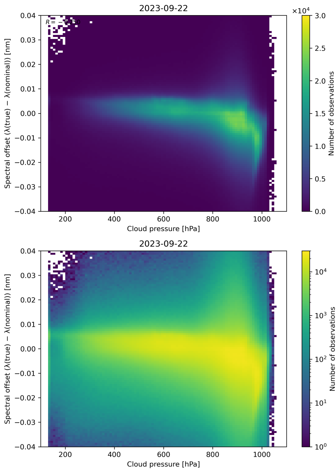
Figure 92: Scatter density plot of “Cloud pressure” against “Spectral offset ( \lambda(\text{true}) - \lambda(\text{nominal}) )” for 2023-09-21 to 2023-09-23.
