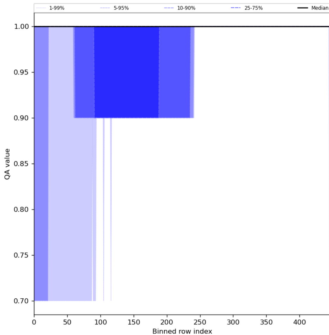
Figure 46: Along track statistics of “QA value” for 2023-09-21 to 2023-09-23
