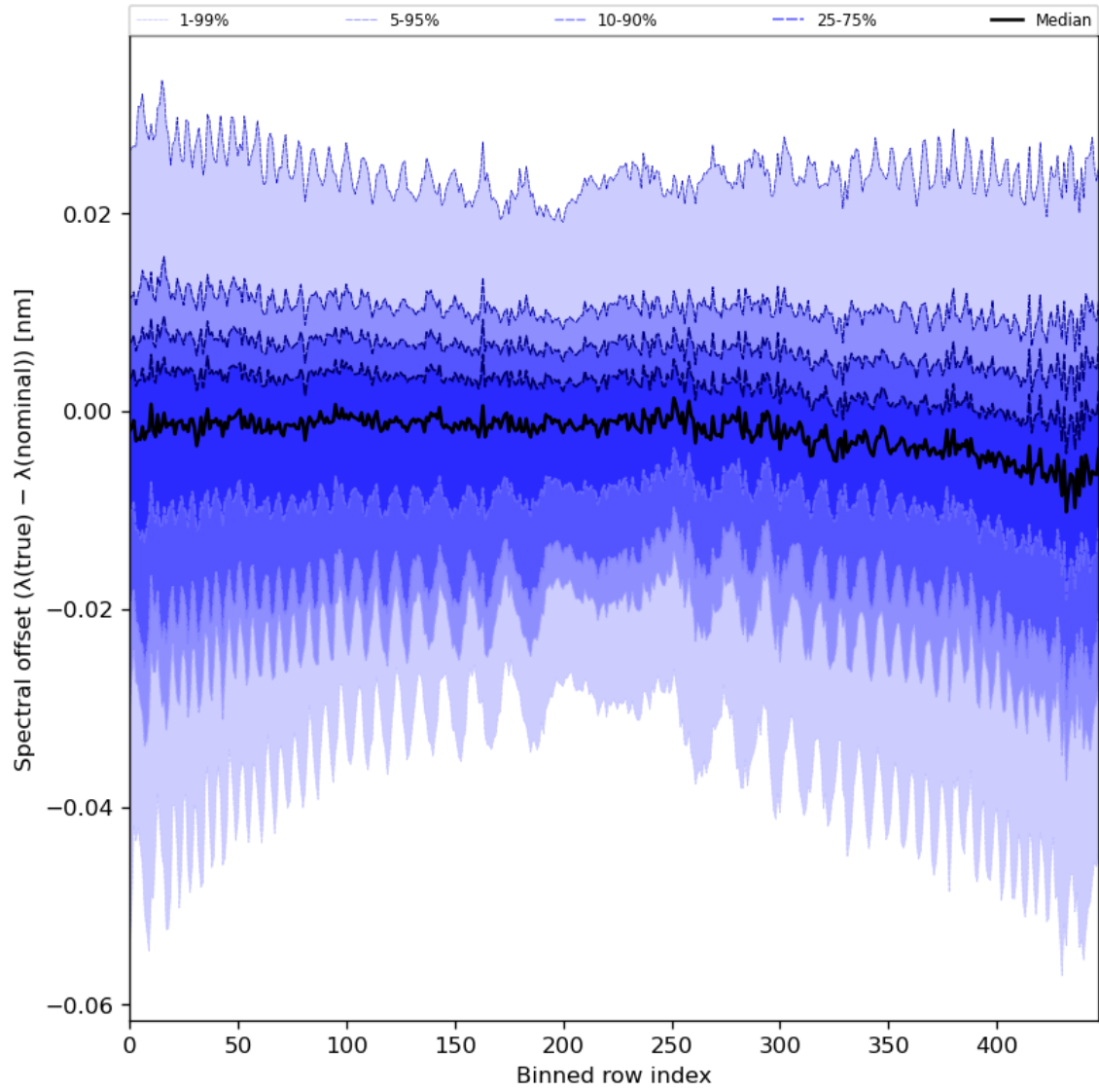
Figure 62: Along track statistics of “Spectral offset ( \lambda(\text{true}) - \lambda(\text{nominal}) )” for 2023-09-21 to 2023-09-23
