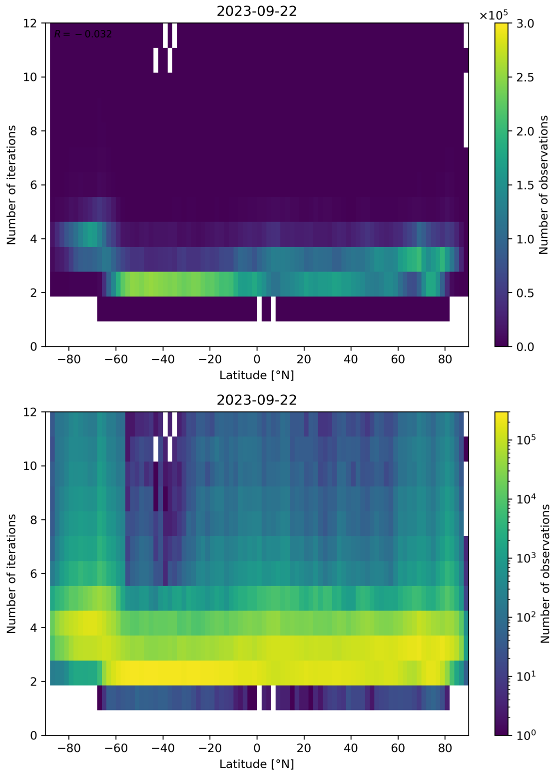
Figure 102: Scatter density plot of “Latitude” against “Number of iterations” for 2023-09-21 to 2023-09-23.
