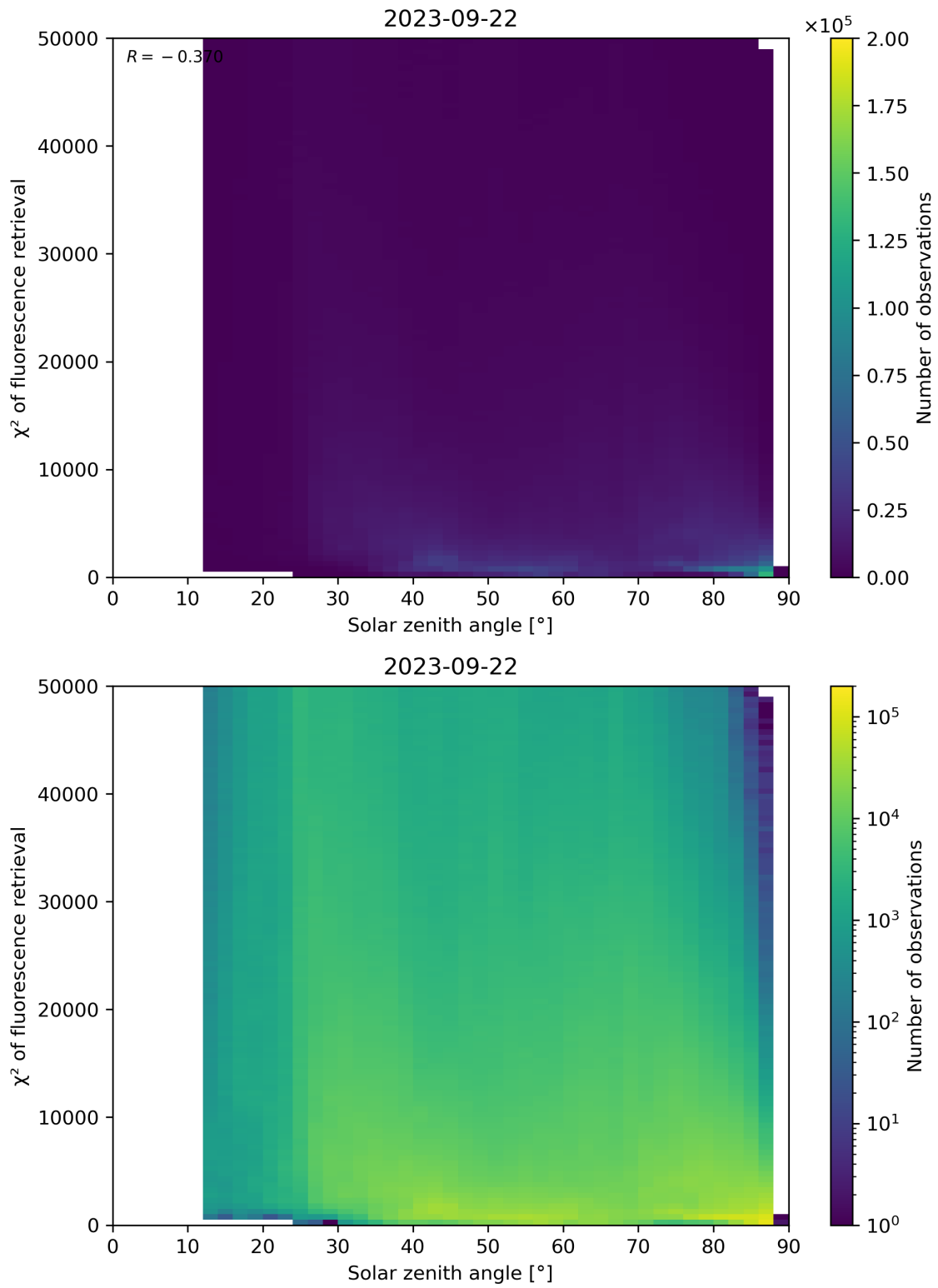
Figure 120: Scatter density plot of “Solar zenith angle” against “ \chi^2 of fluorescence retrieval” for 2023-09-21 to 2023-09-23.
