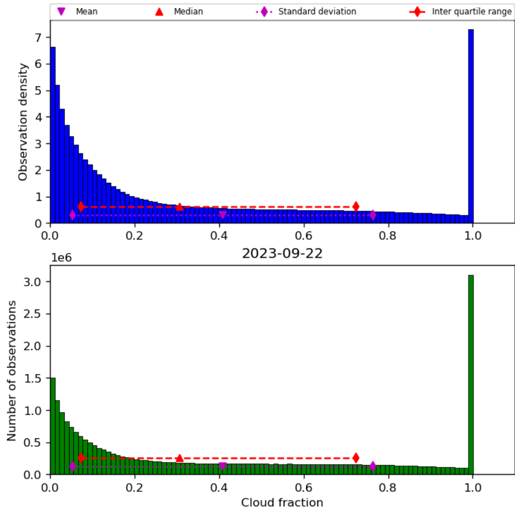
Figure 32: Histogram of “Cloud fraction” for 2023-09-21 to 2023-09-23
