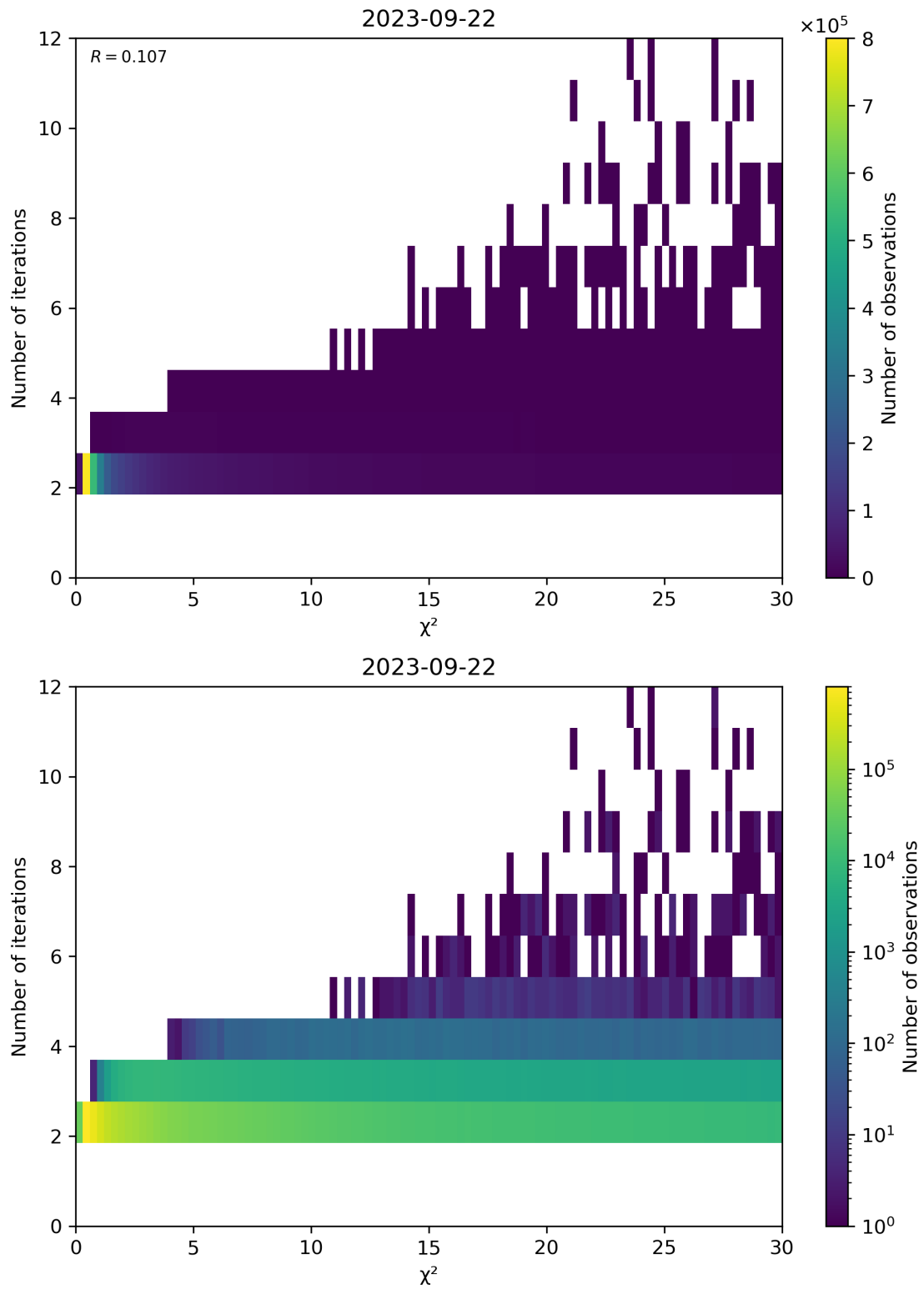
Figure 73: Scatter density plot of “ \chi^2 ” against “Number of iterations” for 2023-09-21 to 2023-09-23.
