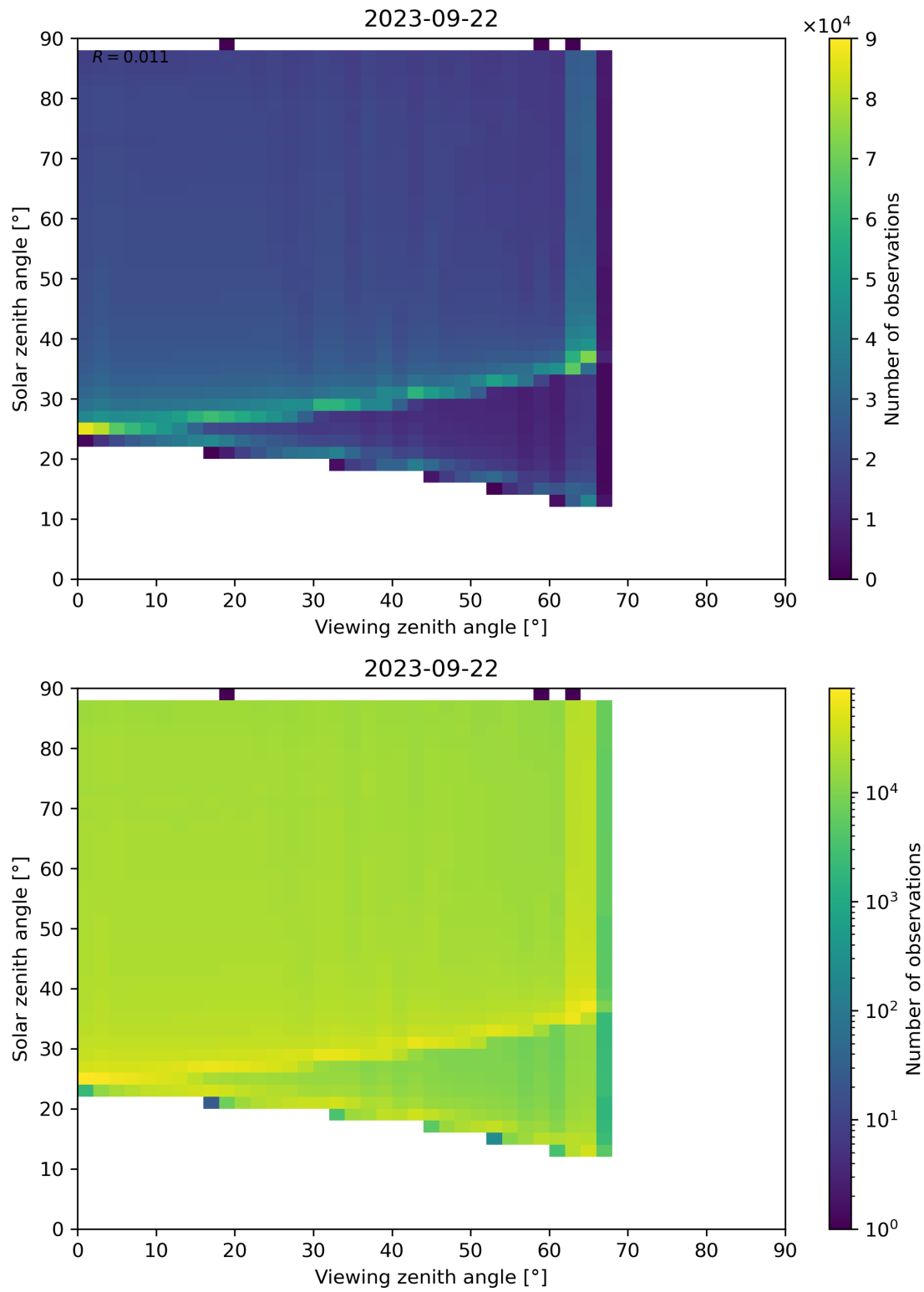
Figure 139: Scatter density plot of “Viewing zenith angle” against “Solar zenith angle” for 2023-09-21 to 2023-09-23.
