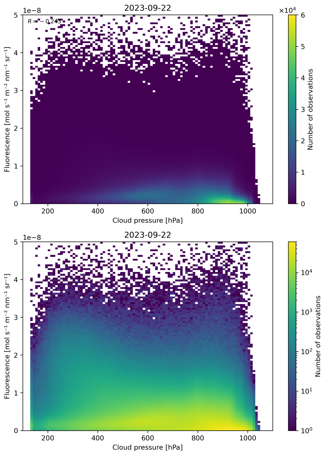
Figure 88: Scatter density plot of “Cloud pressure” against “Fluorescence” for 2023-09-21 to 2023-09-23.
