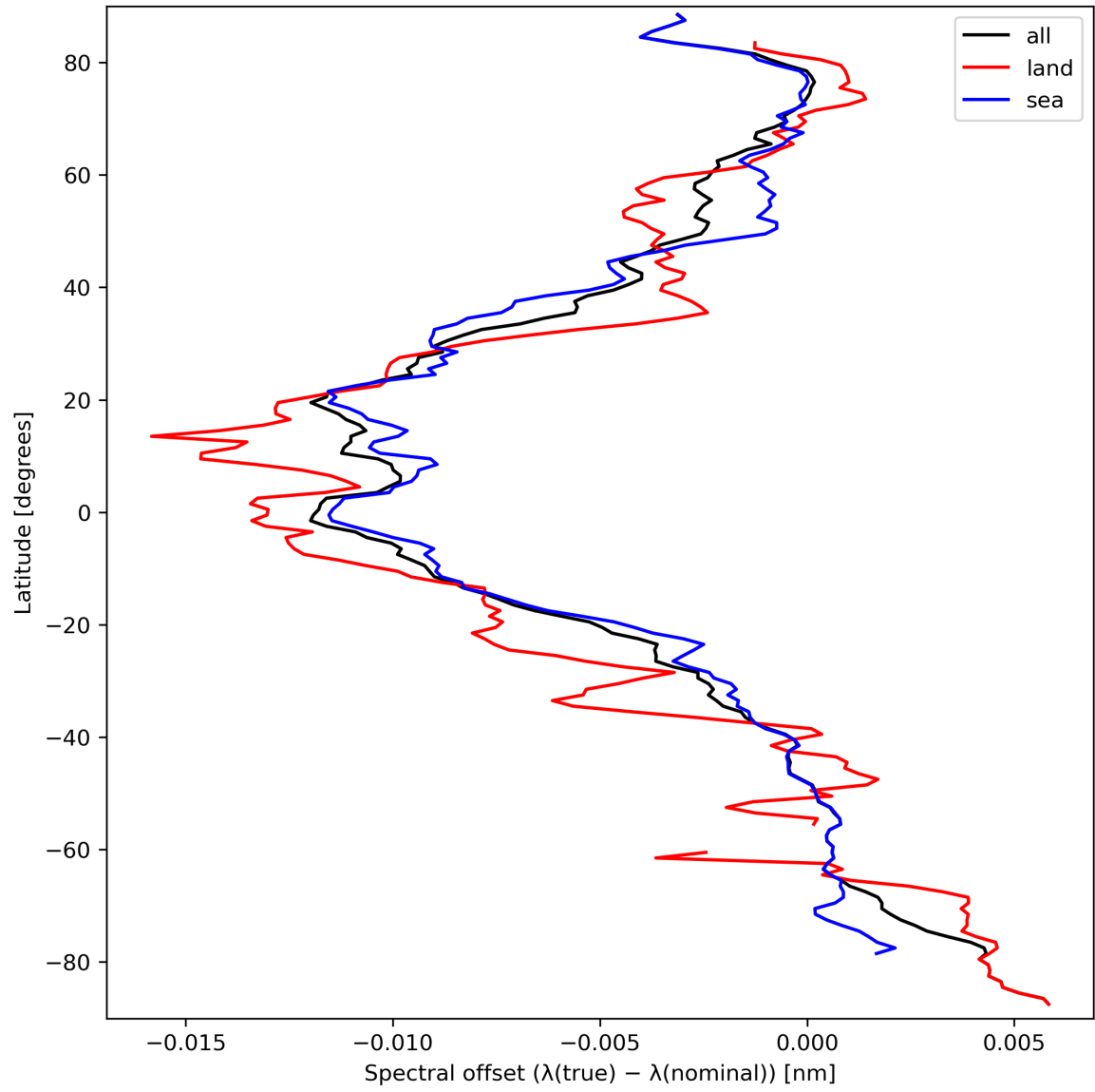
Figure 28: Zonal average of “Spectral offset ( \lambda(\text{true}) - \lambda(\text{nominal}) )” for 2023-09-21 to 2023-09-23.
