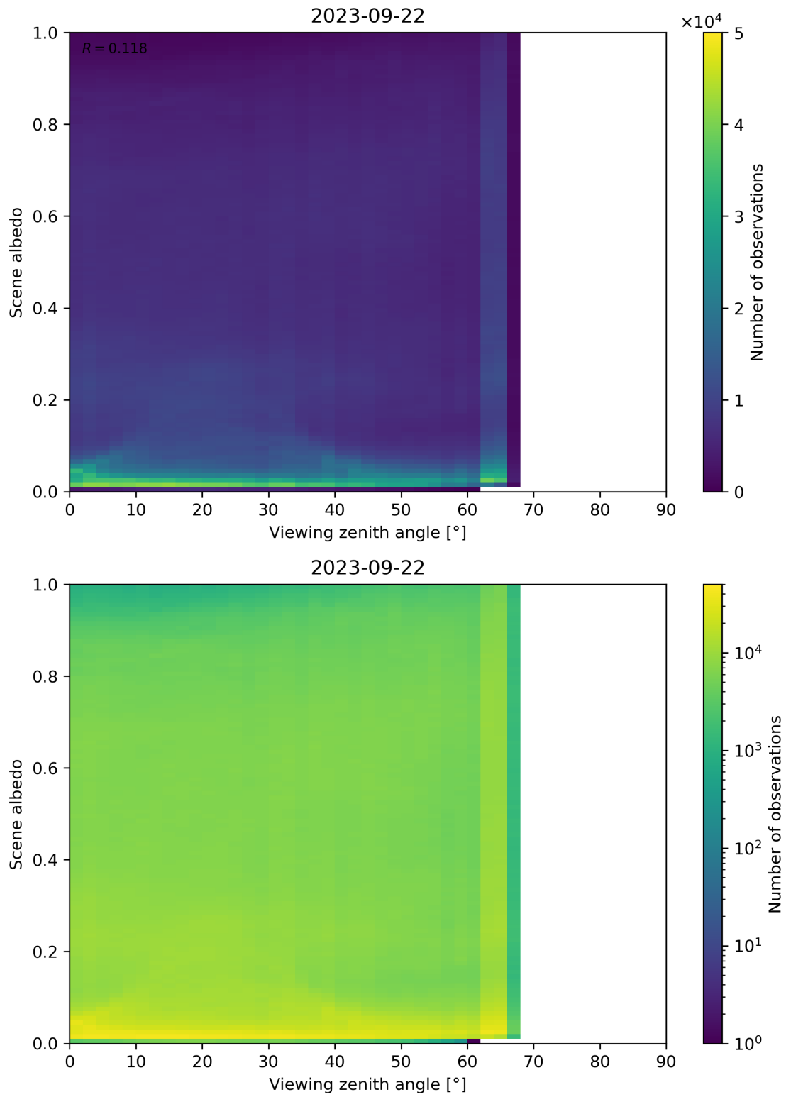
Figure 138: Scatter density plot of “Viewing zenith angle” against “Scene albedo” for 2023-09-21 to 2023-09-23.
