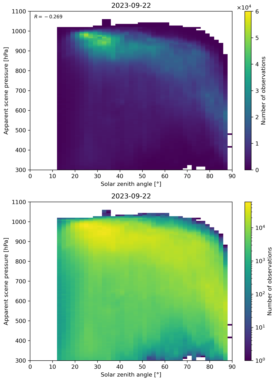
Figure 118: Scatter density plot of “Solar zenith angle” against “Apparent scene pressure” for 2023-09-21 to 2023-09-23.
