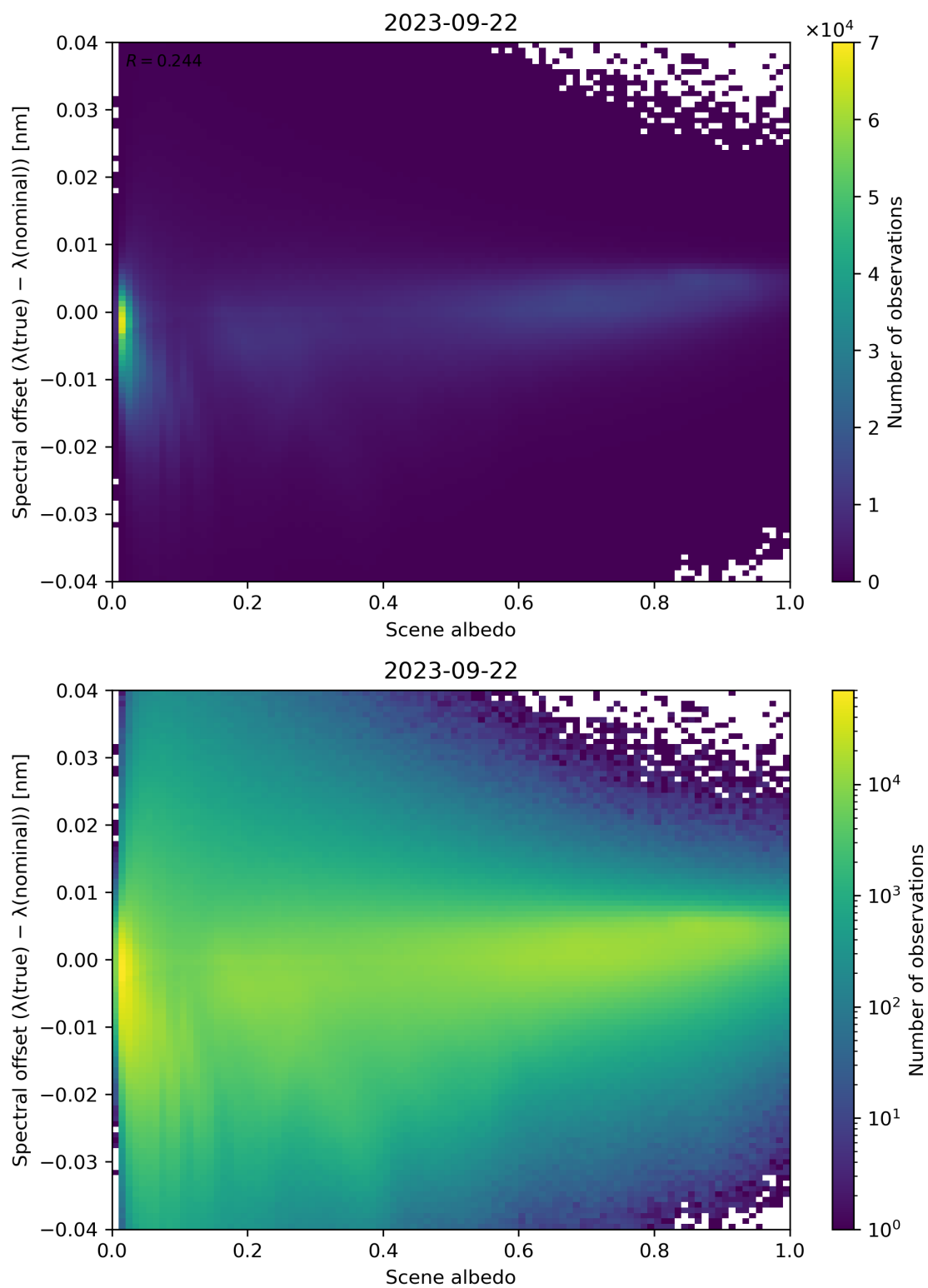
Figure 117: Scatter density plot of “Scene albedo” against “Spectral offset ( \lambda(\text{true}) - \lambda(\text{nominal}) )” for 2023-09-21 to 2023-09-23.
