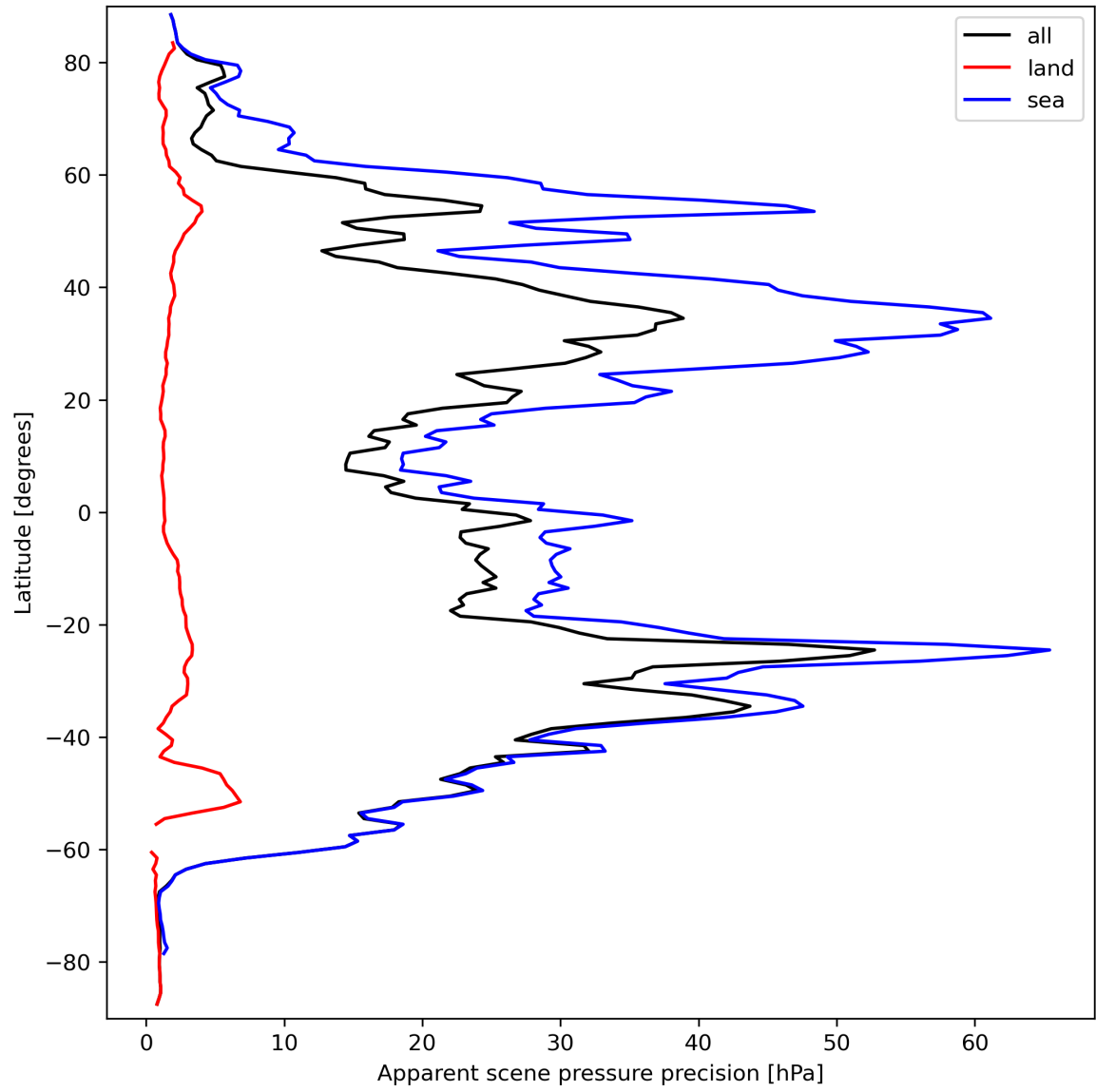
Figure 20: Zonal average of “Apparent scene pressure precision” for 2023-09-21 to 2023-09-23.
