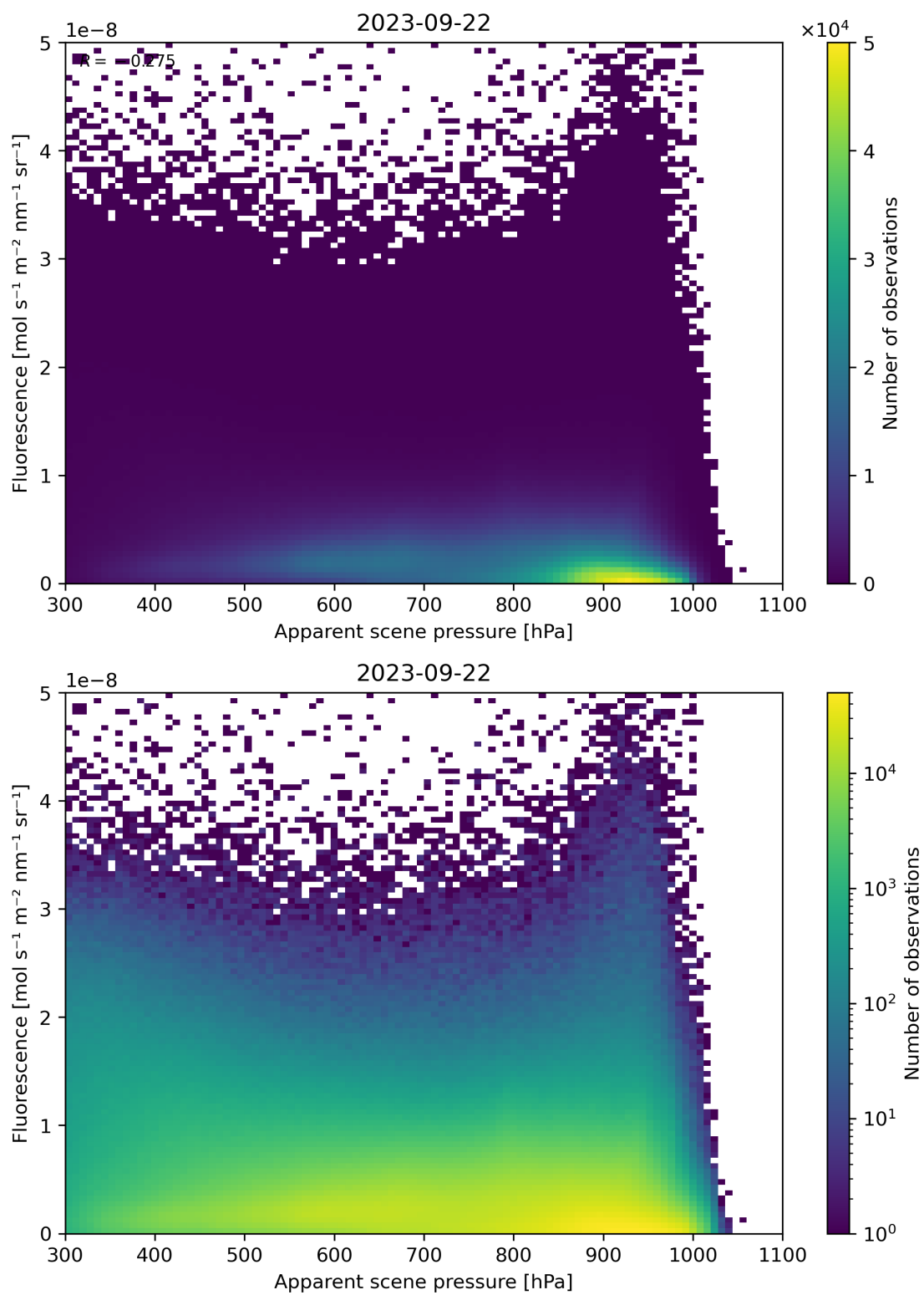
Figure 65: Scatter density plot of “Apparent scene pressure” against “Fluorescence” for 2023-09-21 to 2023-09-23.
