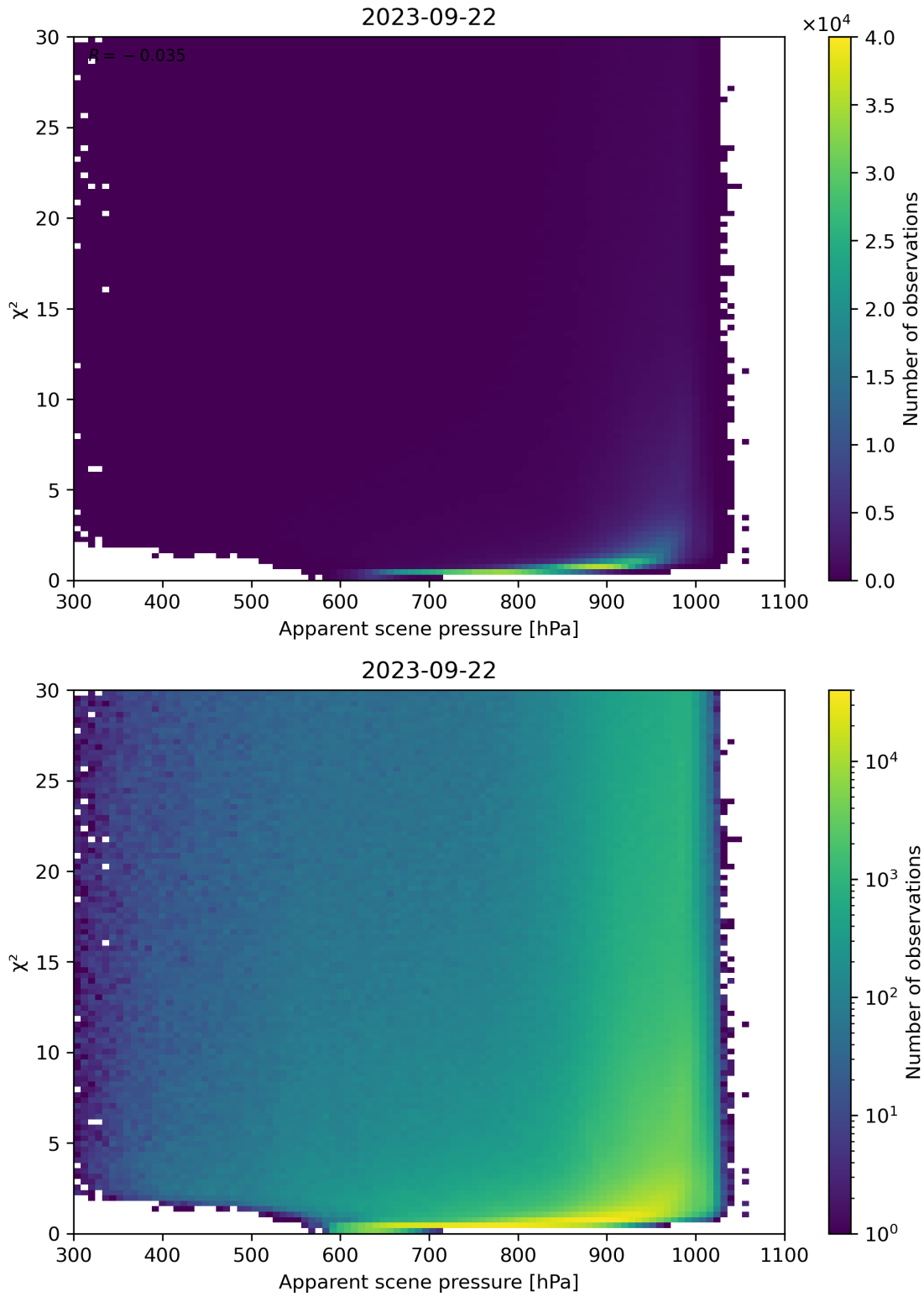
Figure 63: Scatter density plot of “Apparent scene pressure” against “ \chi^2 ” for 2023-09-21 to 2023-09-23.
