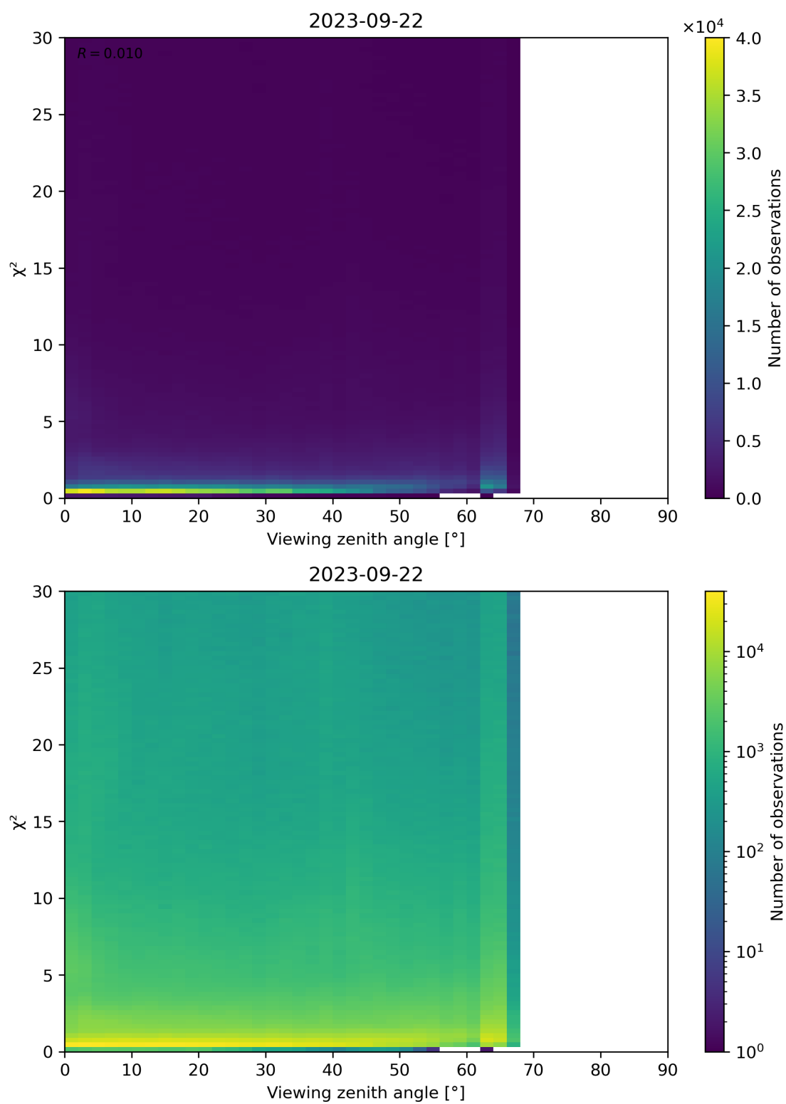
Figure 130: Scatter density plot of “Viewing zenith angle” against “ \chi^2 ” for 2023-09-21 to 2023-09-23.
