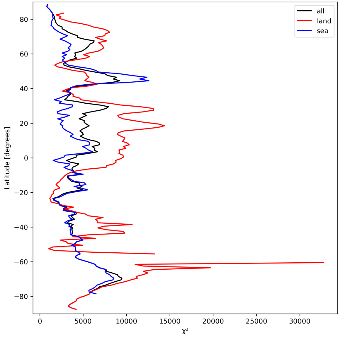
Figure 21: Zonal average of “ \chi^2 ” for 2023-09-21 to 2023-09-23.
