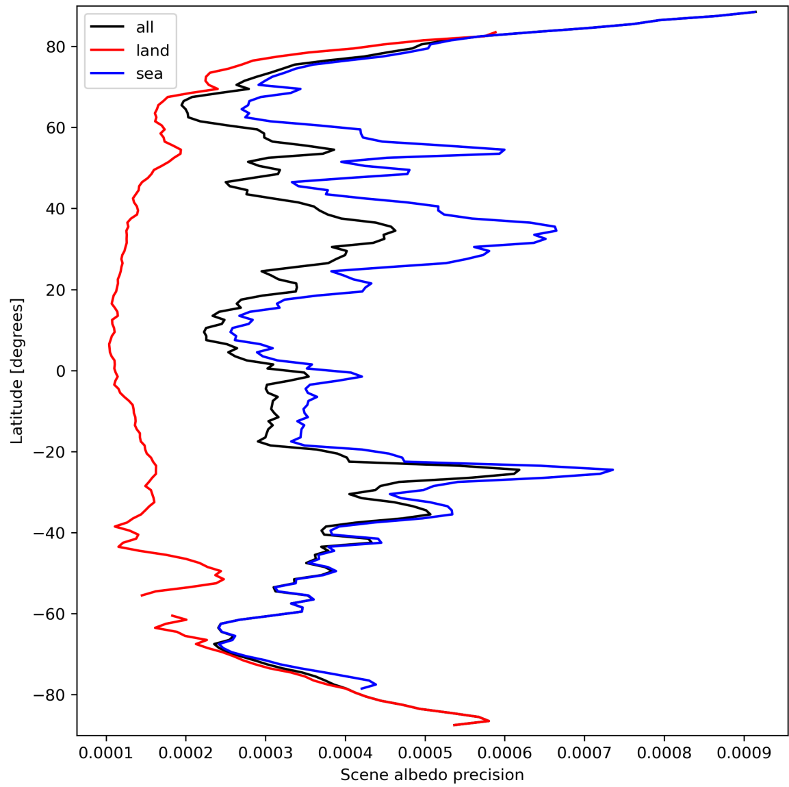
Figure 18: Zonal average of “Scene albedo precision” for 2023-09-21 to 2023-09-23.
