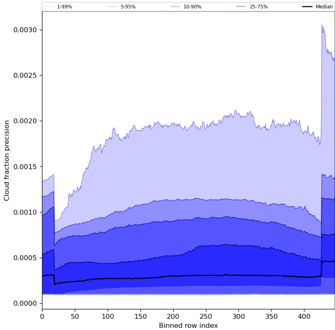
Figure 50: Along track statistics of “Cloud fraction precision” for 2023-09-21 to 2023-09-23
