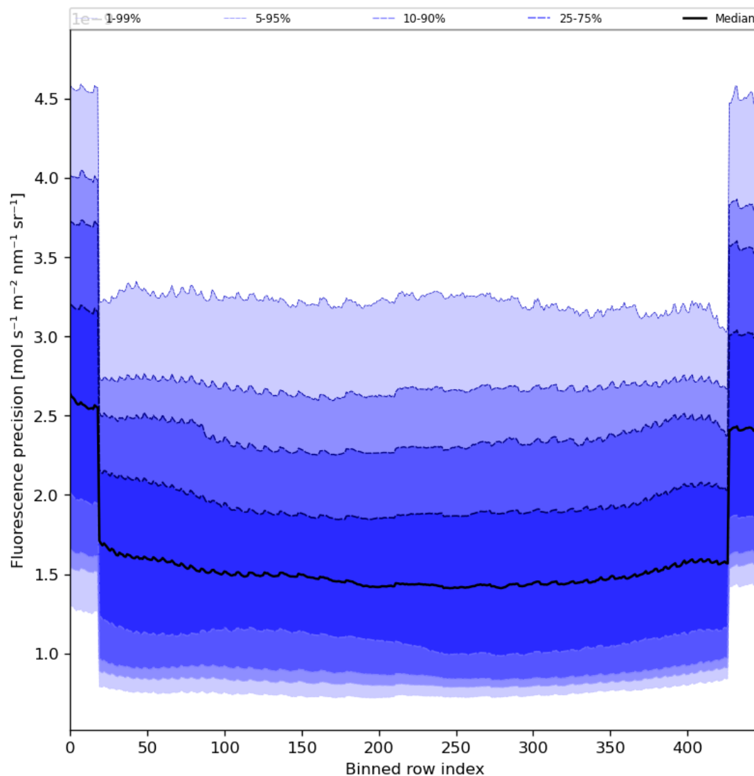
Figure 58: Along track statistics of “Fluorescence precision” for 2023-09-21 to 2023-09-23
