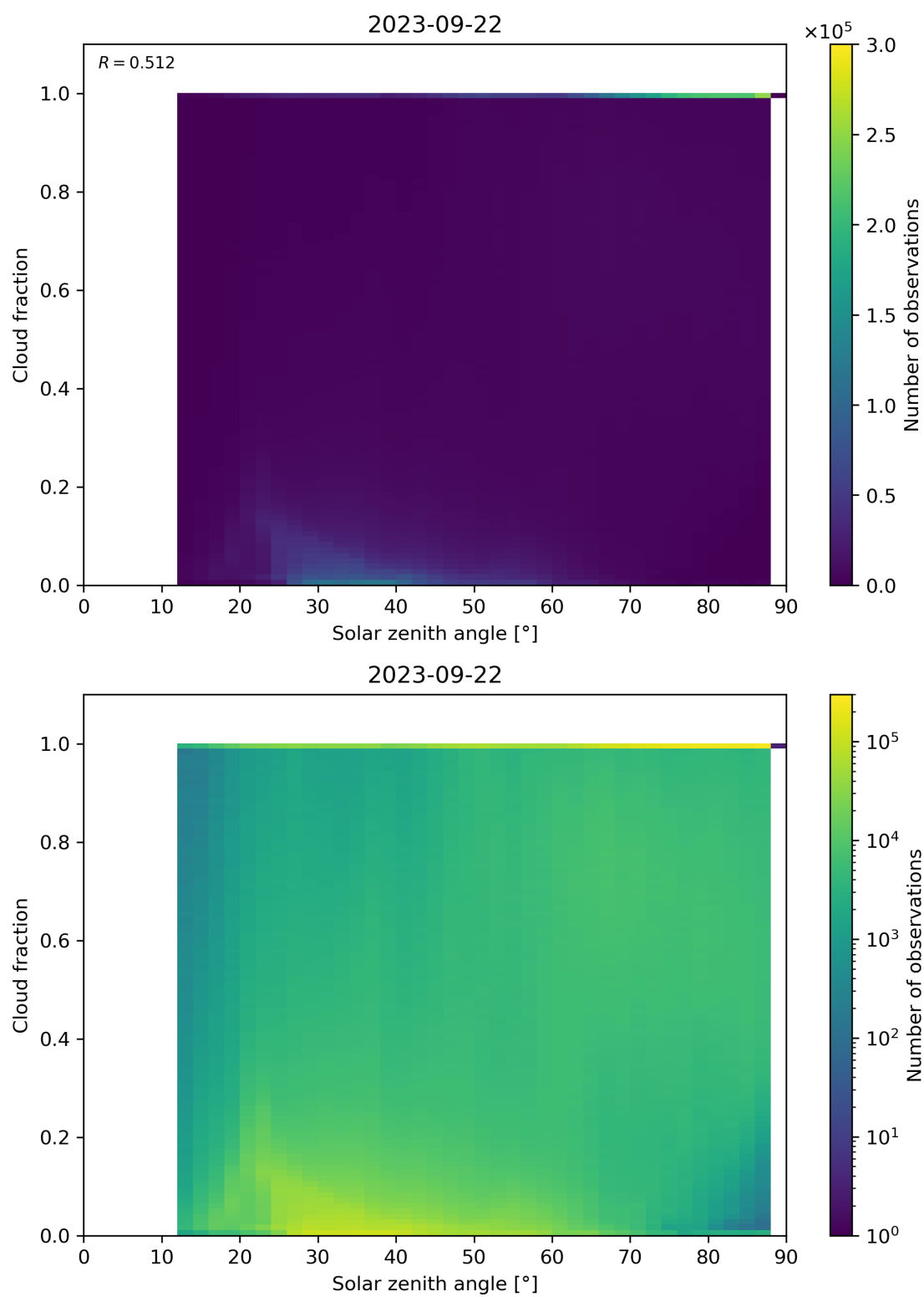
Figure 121: Scatter density plot of “Solar zenith angle” against “Cloud fraction” for 2023-09-21 to 2023-09-23.
