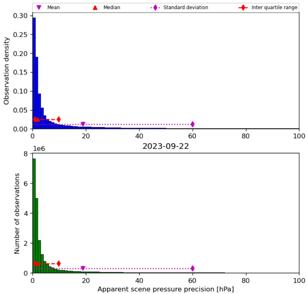
Figure 37: Histogram of “Apparent scene pressure precision” for 2023-09-21 to 2023-09-23
