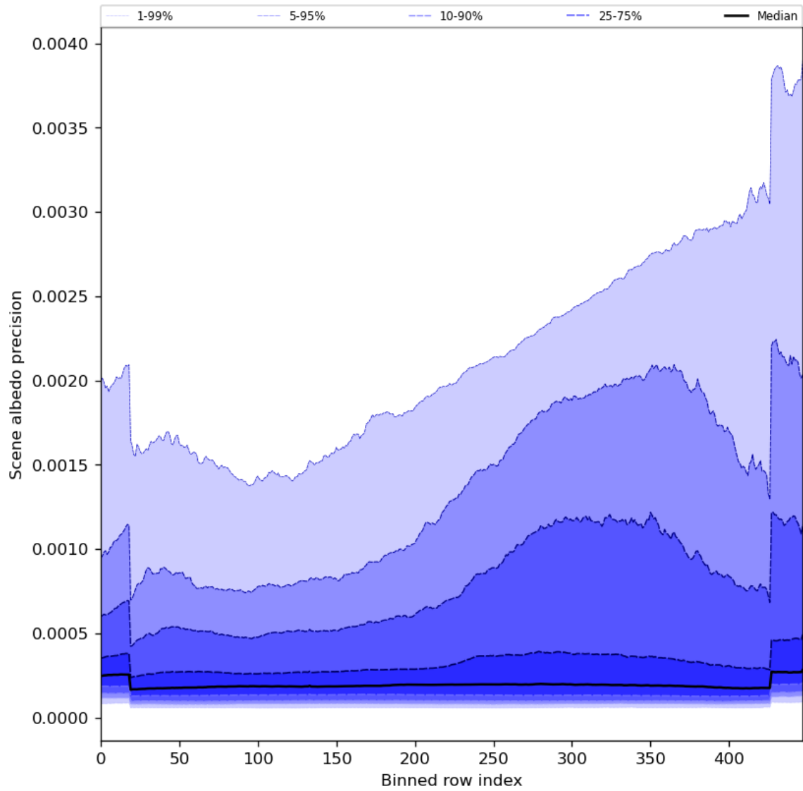
Figure 52: Along track statistics of “Scene albedo precision” for 2023-09-21 to 2023-09-23
