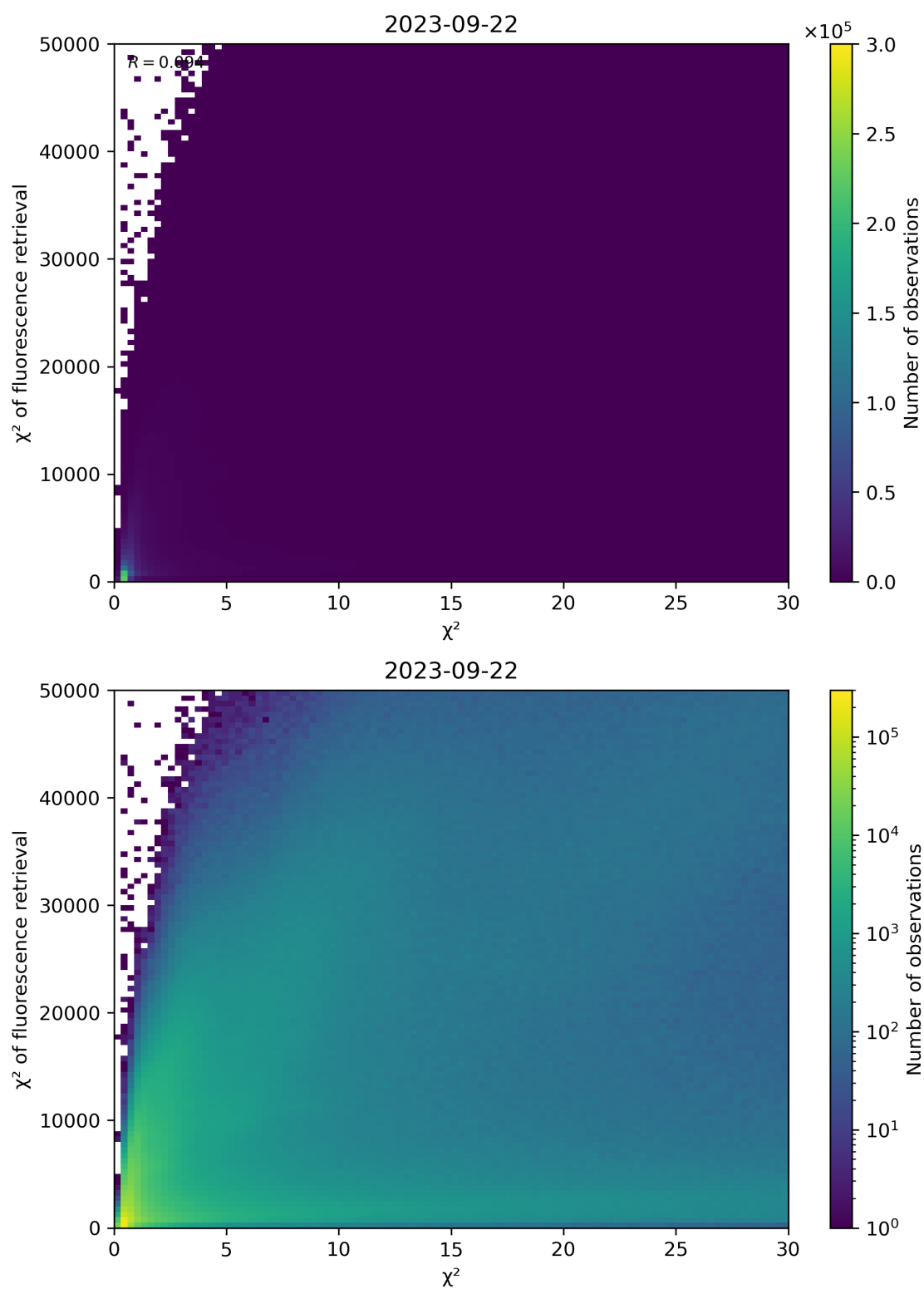
Figure 69: Scatter density plot of “ \chi^2 ” against “ \chi^2 of fluorescence retrieval” for 2023-09-21 to 2023-09-23.
