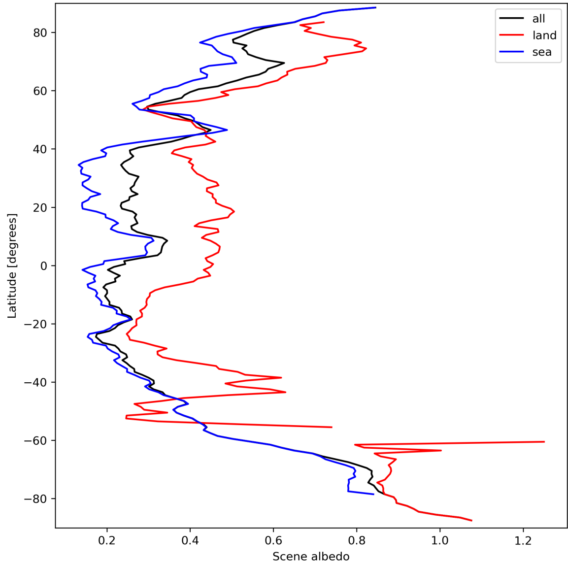
Figure 17: Zonal average of “Scene albedo” for 2023-09-21 to 2023-09-23.
