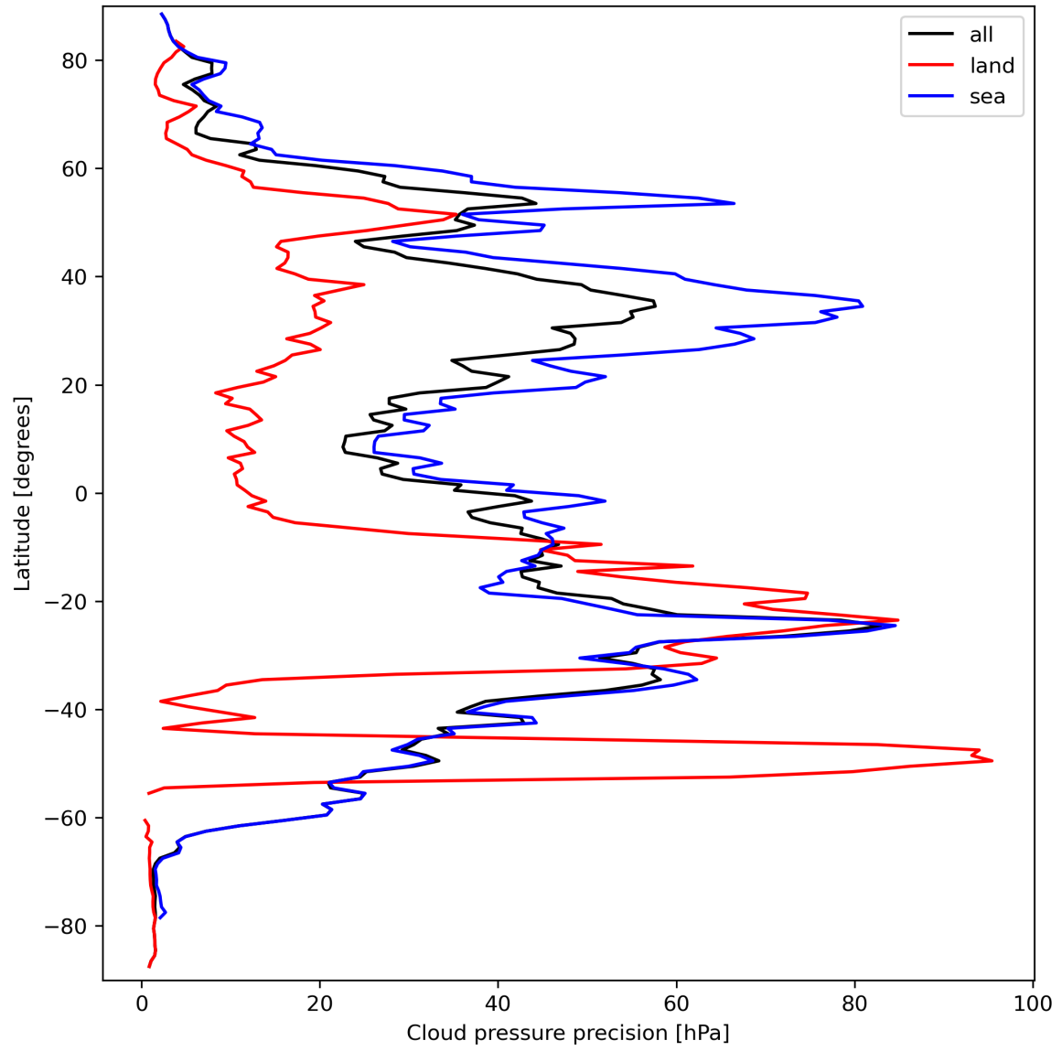
Figure 14: Zonal average of “Cloud pressure precision” for 2023-09-21 to 2023-09-23.
