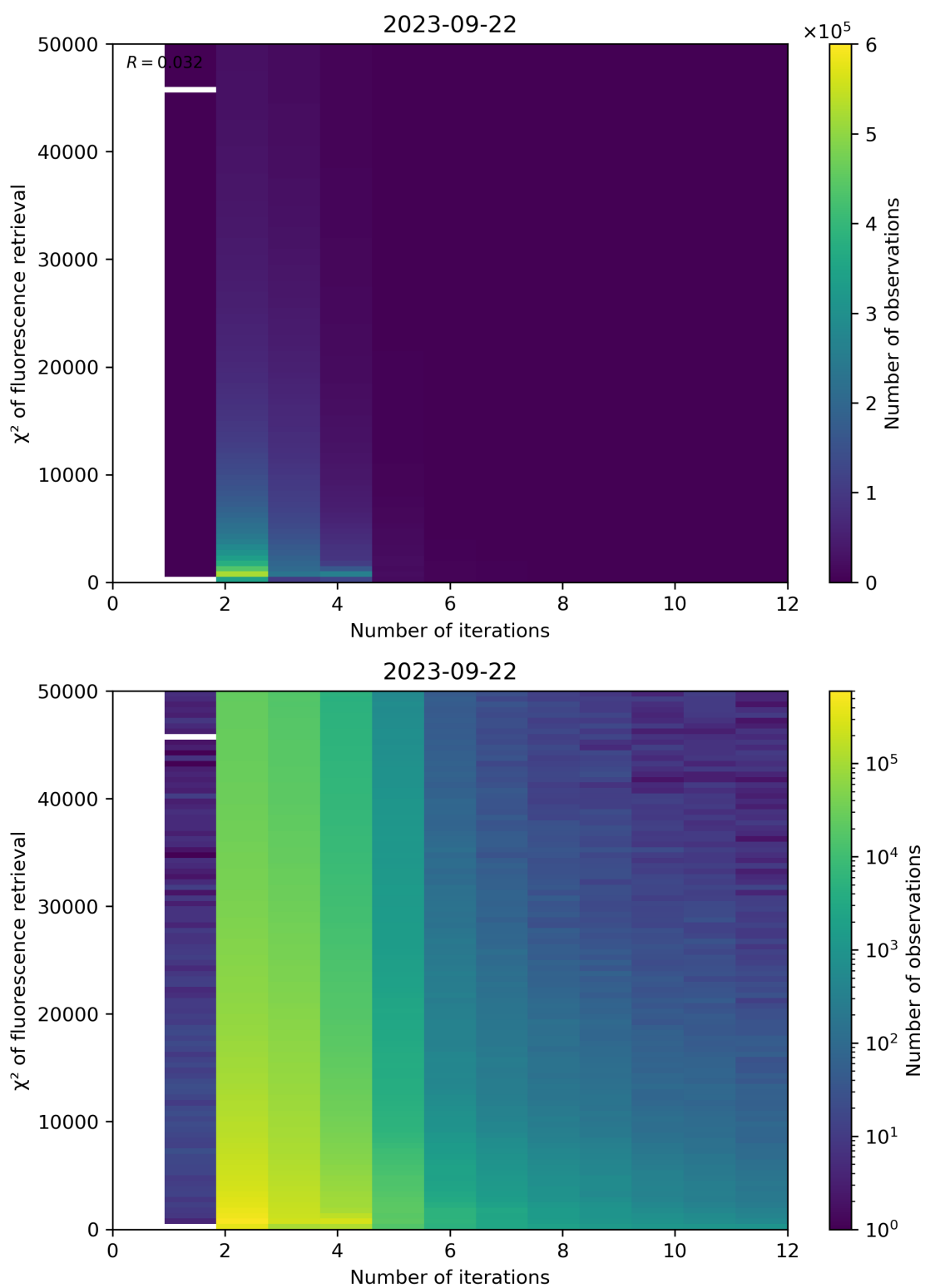
Figure 106: Scatter density plot of “Number of iterations” against “ \chi^2 of fluorescence retrieval” for 2023-09-21 to 2023-09-23.
