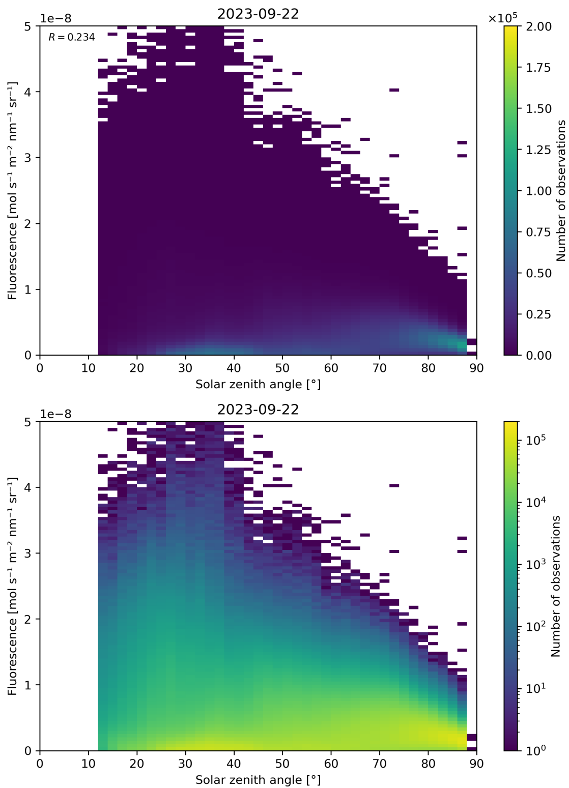
Figure 123: Scatter density plot of “Solar zenith angle” against “Fluorescence” for 2023-09-21 to 2023-09-23.
