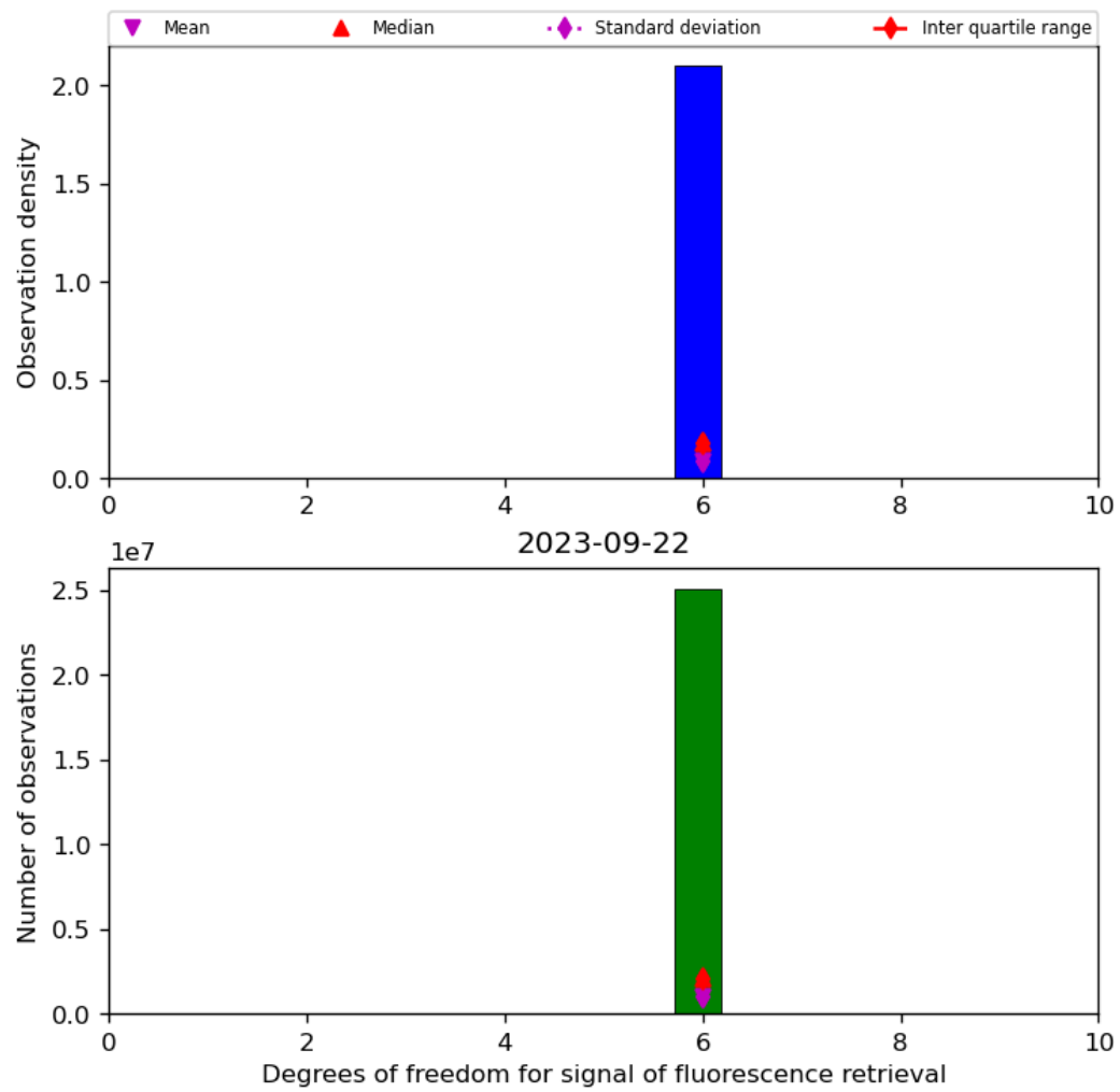
Figure 43: Histogram of “Degrees of freedom for signal of fluorescence retrieval” for 2023-09-21 to 2023-09-23
