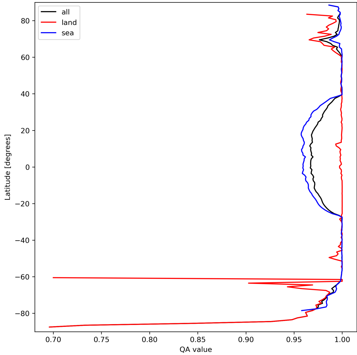
Figure 12: Zonal average of "QA value" for 2023-09-21 to 2023-09-23.
