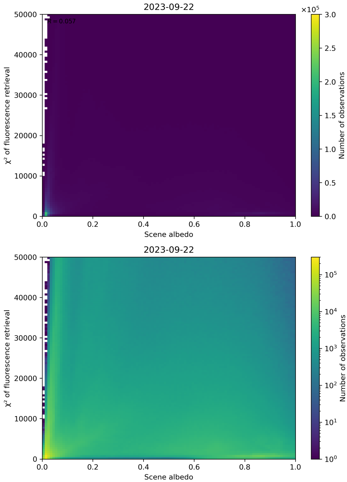
Figure 113: Scatter density plot of “Scene albedo” against “ \chi^2 of fluorescence retrieval” for 2023-09-21 to 2023-09-23.
