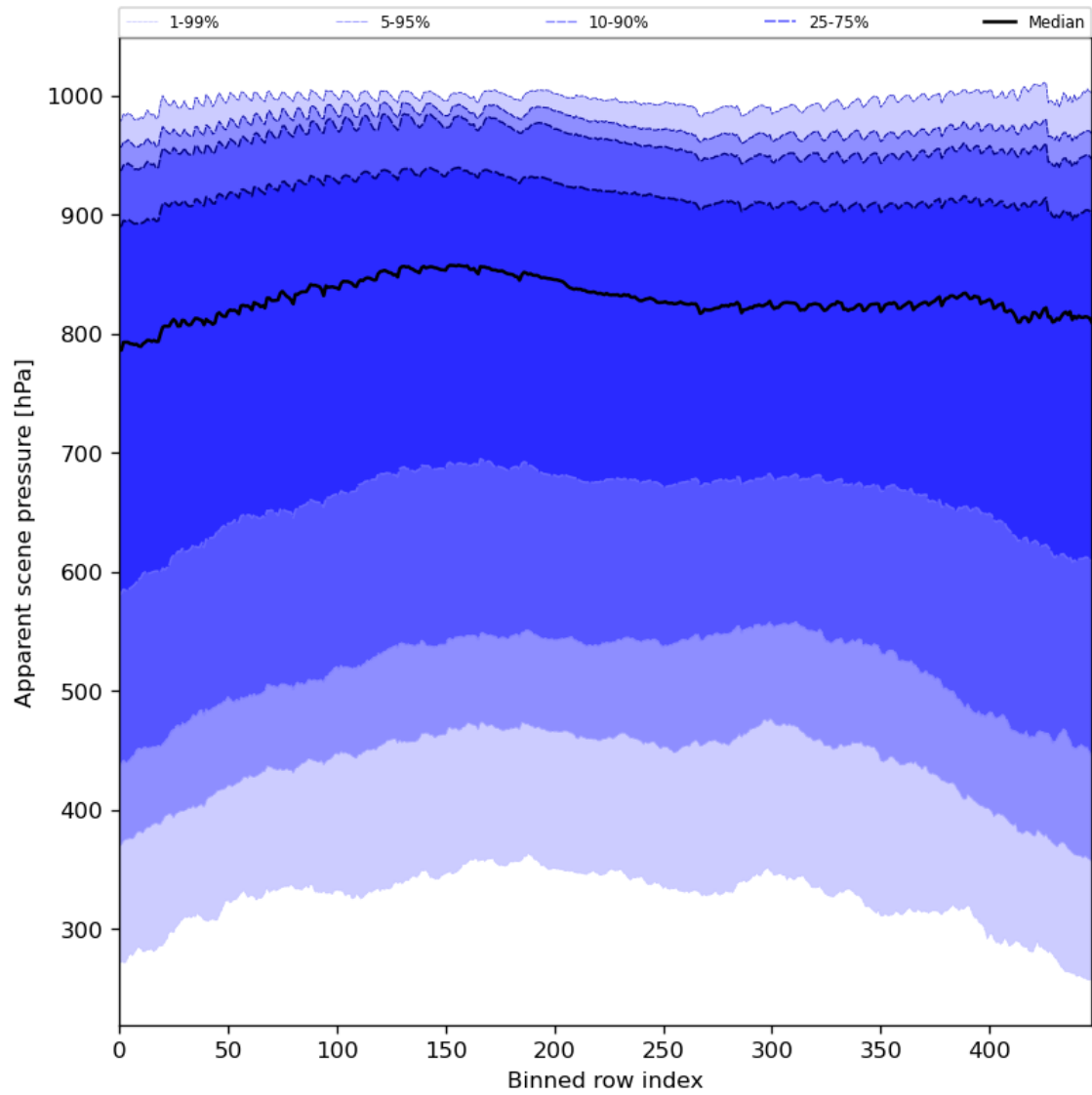
Figure 53: Along track statistics of “Apparent scene pressure” for 2023-09-21 to 2023-09-23
