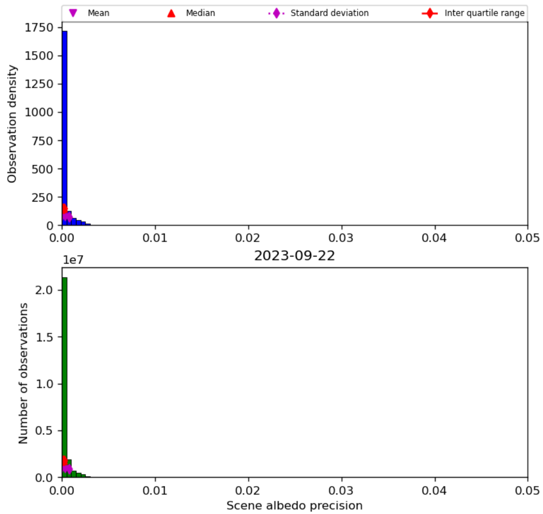
Figure 35: Histogram of “Scene albedo precision” for 2023-09-21 to 2023-09-23
