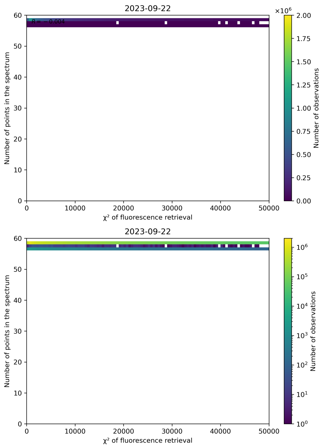
Figure 71: Scatter density plot of “ \chi^2 of fluorescence retrieval” against “Number of points in the spectrum” for 2023-09-21 to 2023-09-23.
