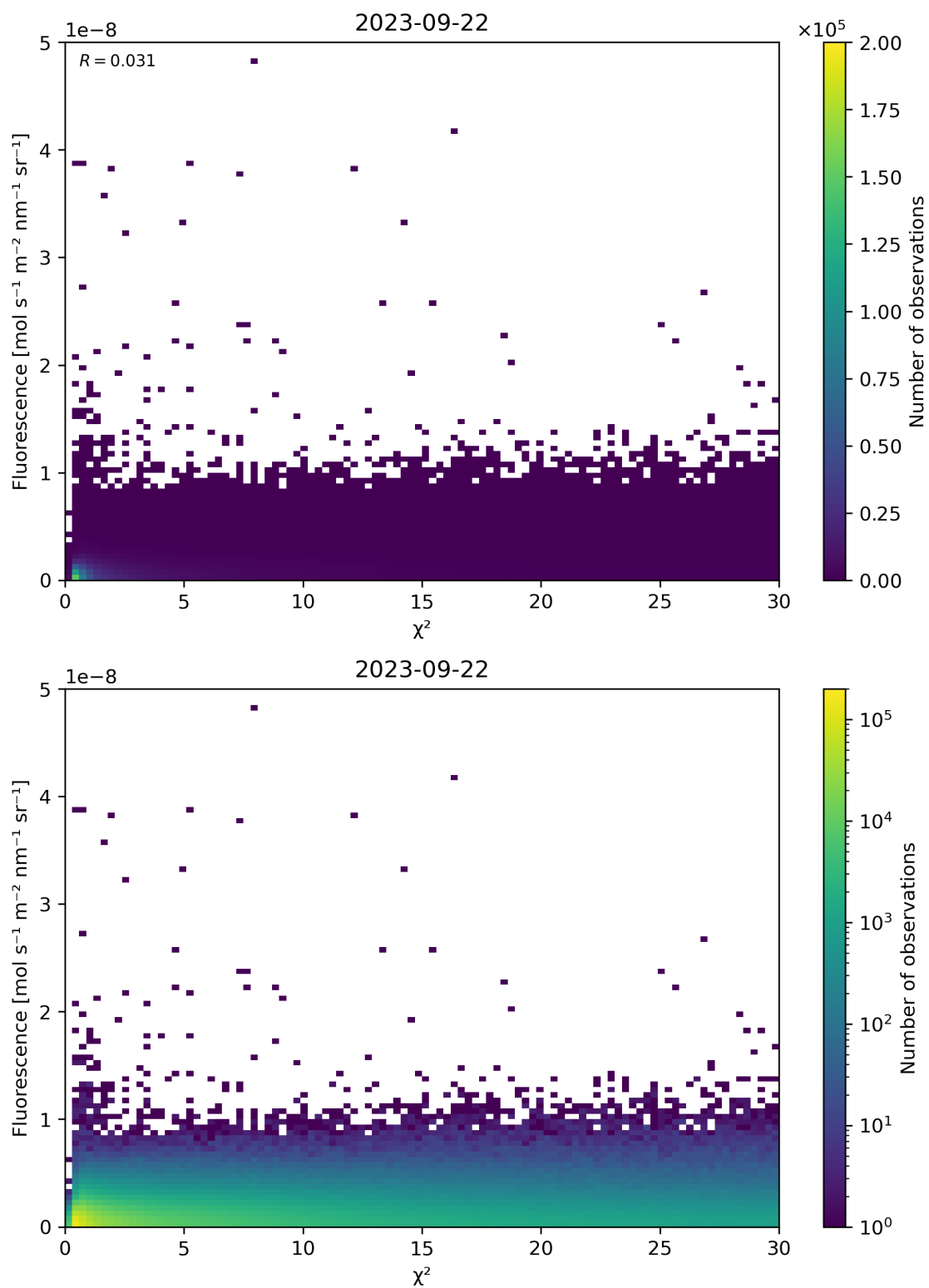
Figure 70: Scatter density plot of “ \chi^2 ” against “Fluorescence” for 2023-09-21 to 2023-09-23.
