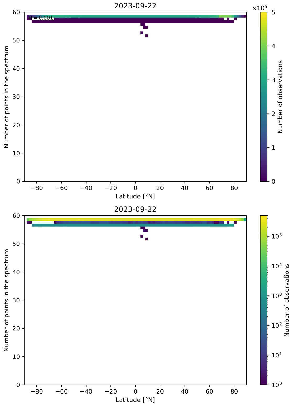
Figure 103: Scatter density plot of “Latitude” against “Number of points in the spectrum” for 2023-09-21 to 2023-09-23.
