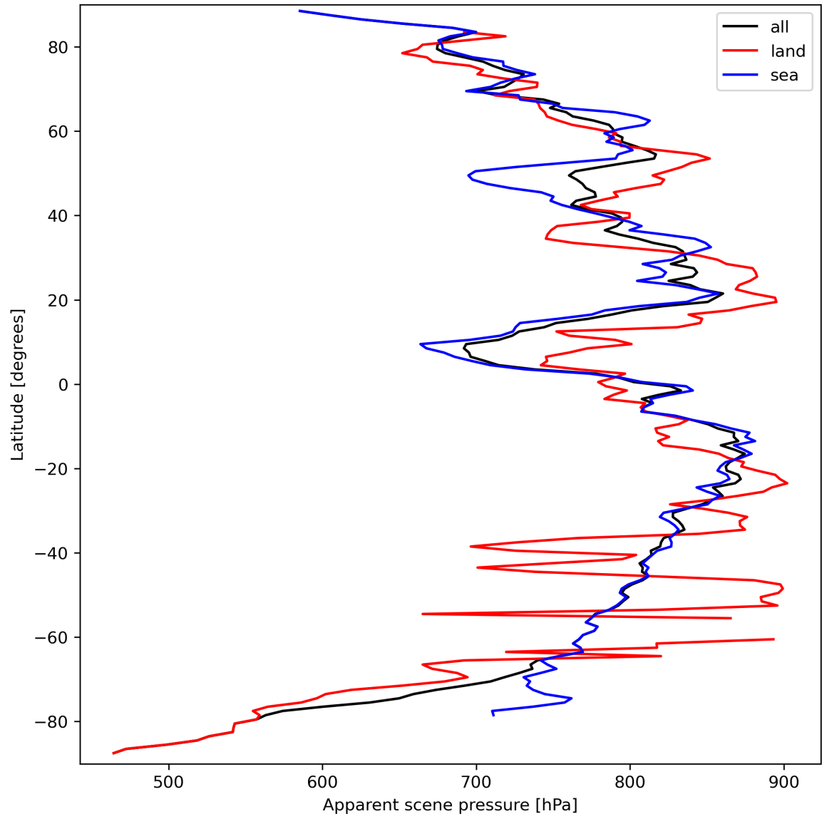
Figure 19: Zonal average of “Apparent scene pressure” for 2023-09-21 to 2023-09-23.
