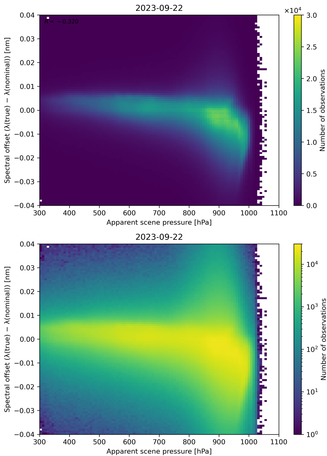
Figure 68: Scatter density plot of “Apparent scene pressure” against “Spectral offset ( \lambda(\text{true}) - \lambda(\text{nominal}) )” for 2023-09-21 to 2023-09-23.
