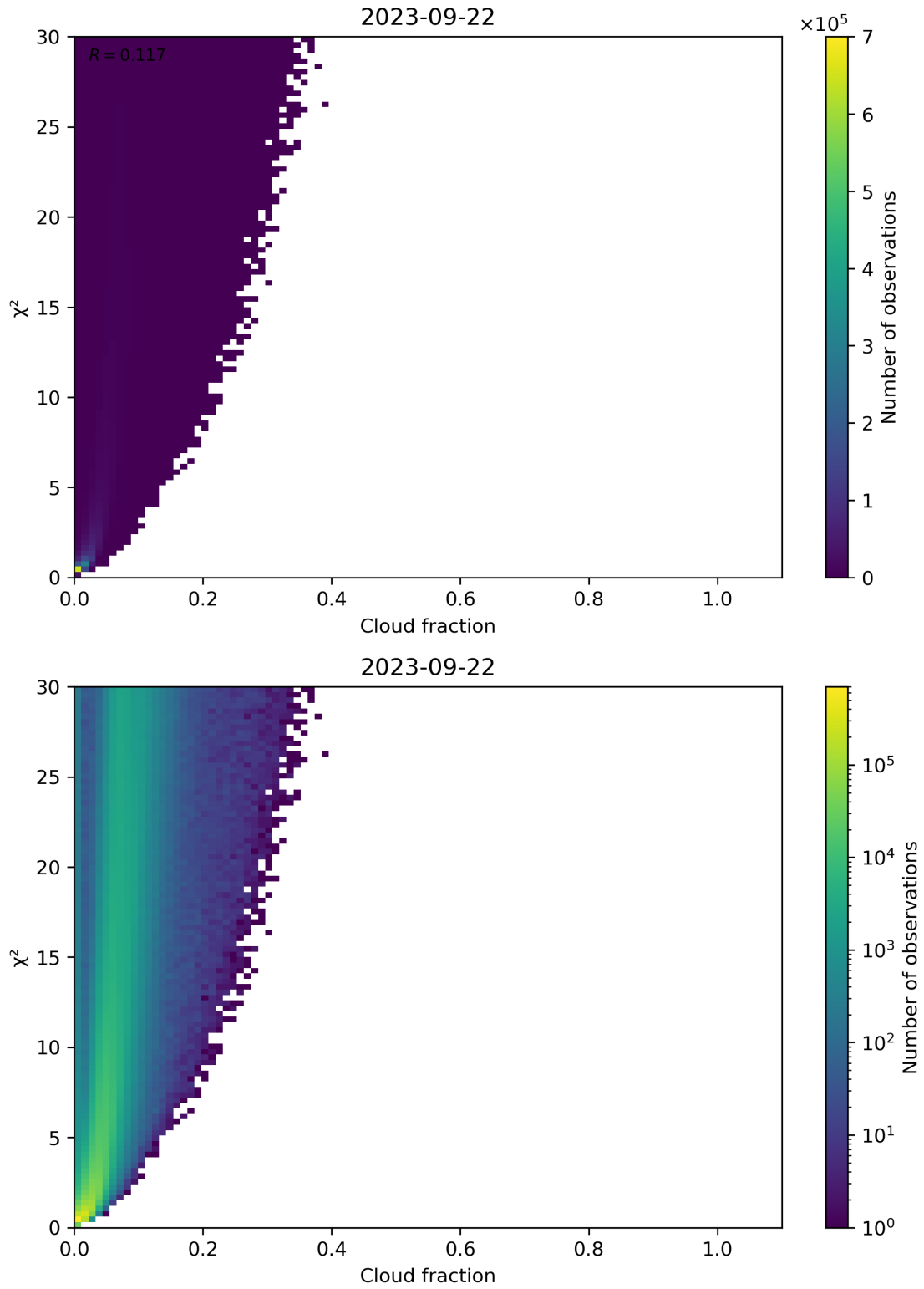
Figure 77: Scatter density plot of “Cloud fraction” against “ \chi^2 ” for 2023-09-21 to 2023-09-23.
