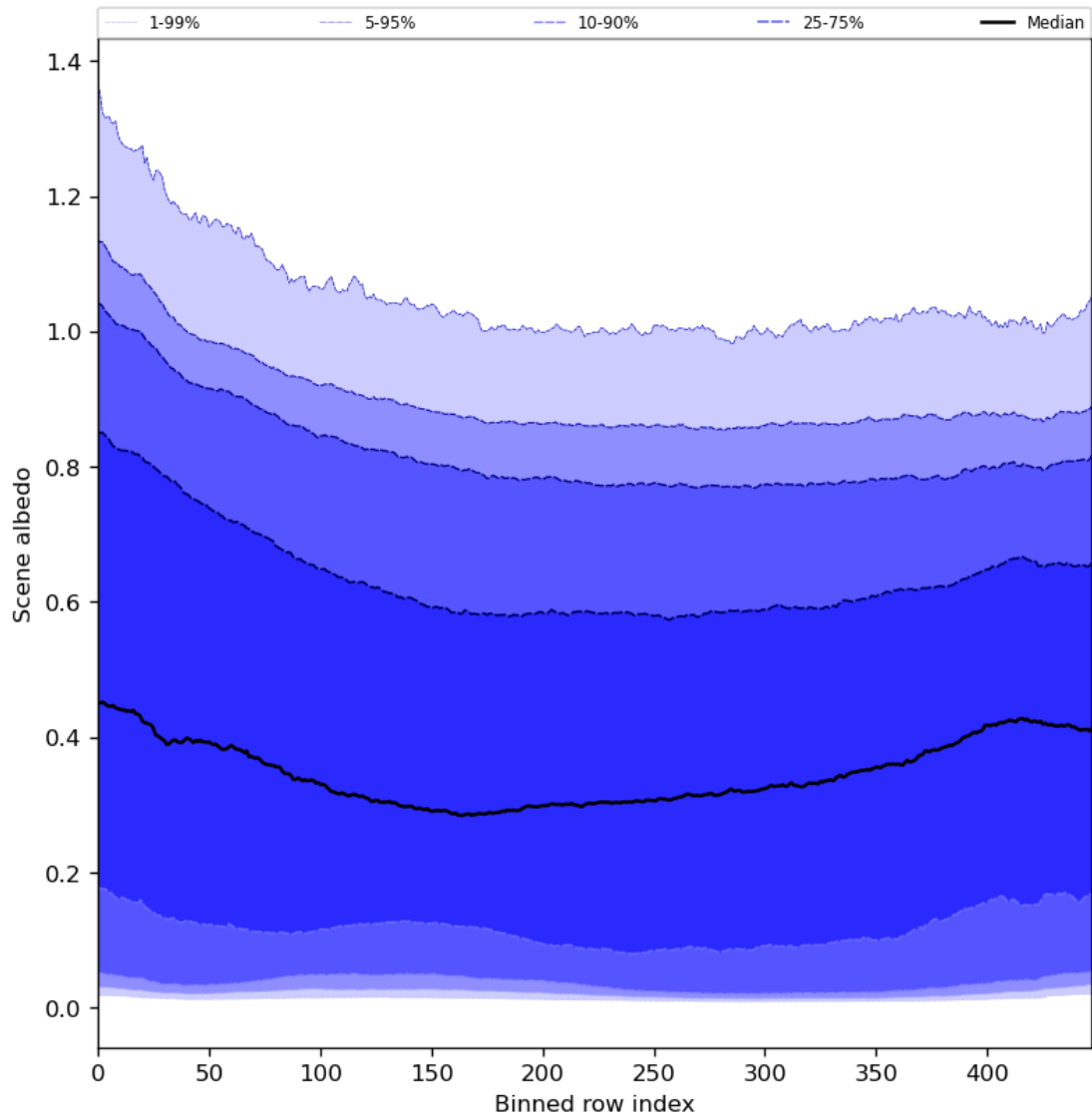
Figure 51: Along track statistics of “Scene albedo” for 2023-09-21 to 2023-09-23
