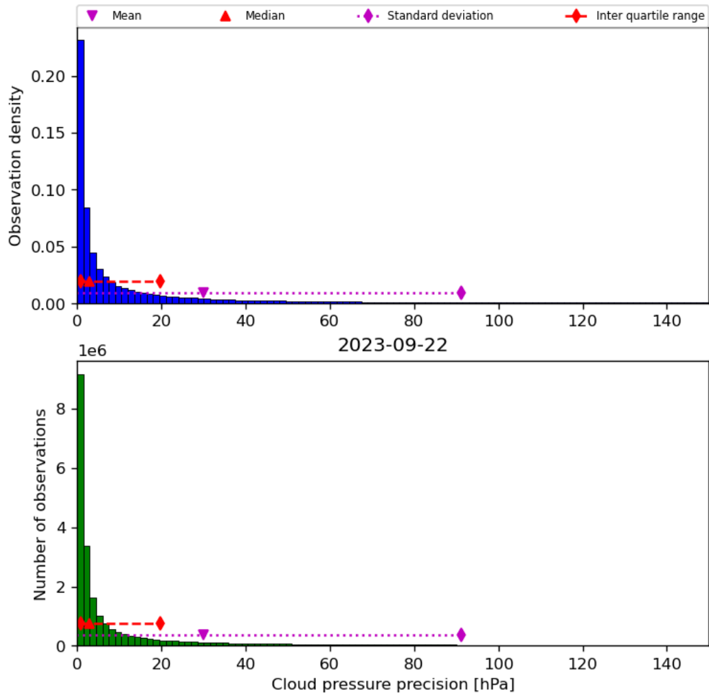
Figure 31: Histogram of “Cloud pressure precision” for 2023-09-21 to 2023-09-23
