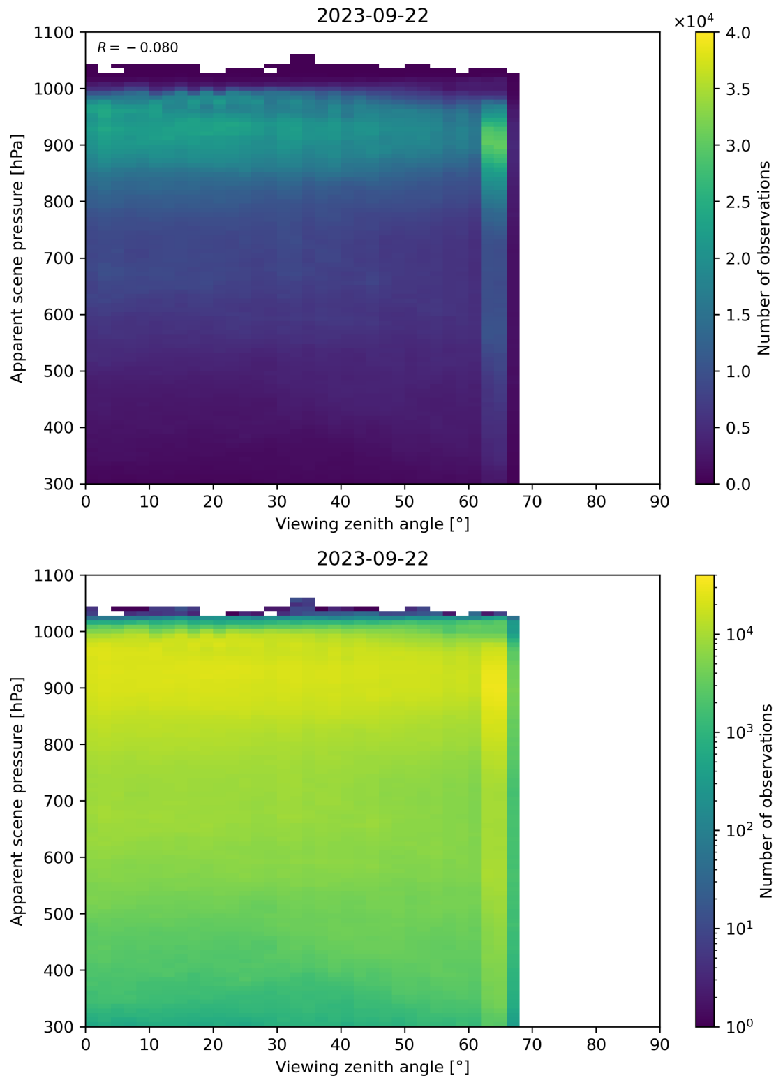
Figure 129: Scatter density plot of “Viewing zenith angle” against “Apparent scene pressure” for 2023-09-21 to 2023-09-23.
