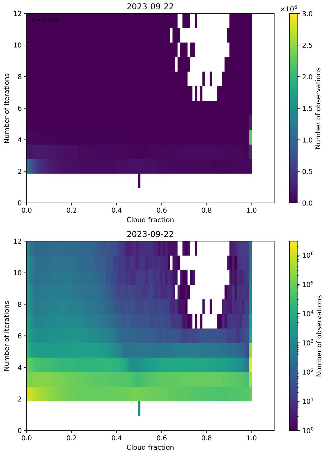
Figure 80: Scatter density plot of “Cloud fraction” against “Number of iterations” for 2023-09-21 to 2023-09-23.
