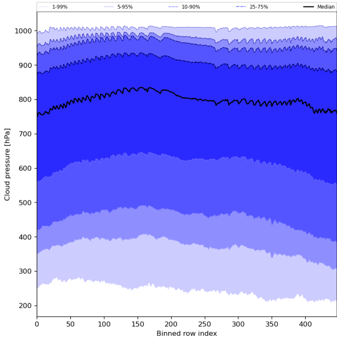
Figure 47: Along track statistics of “Cloud pressure” for 2023-09-21 to 2023-09-23
