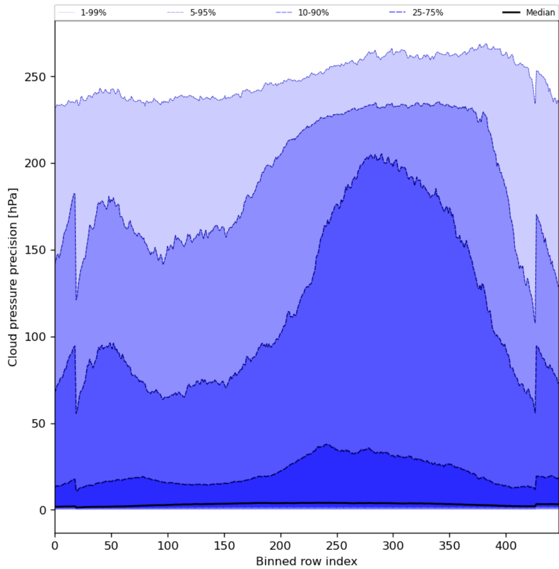
Figure 48: Along track statistics of “Cloud pressure precision” for 2023-09-21 to 2023-09-23
