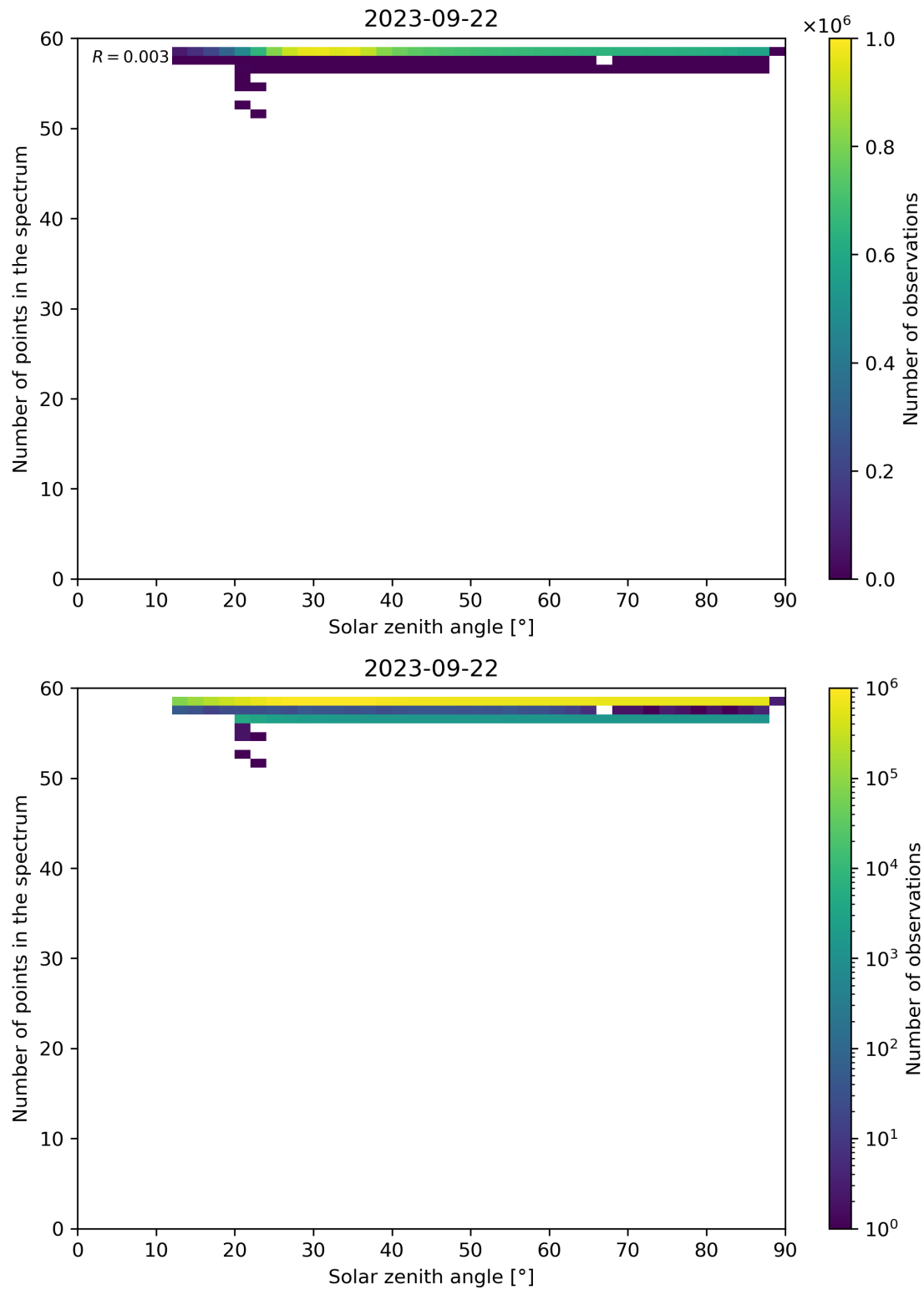
Figure 126: Scatter density plot of “Solar zenith angle” against “Number of points in the spectrum” for 2023-09-21 to 2023-09-23.
