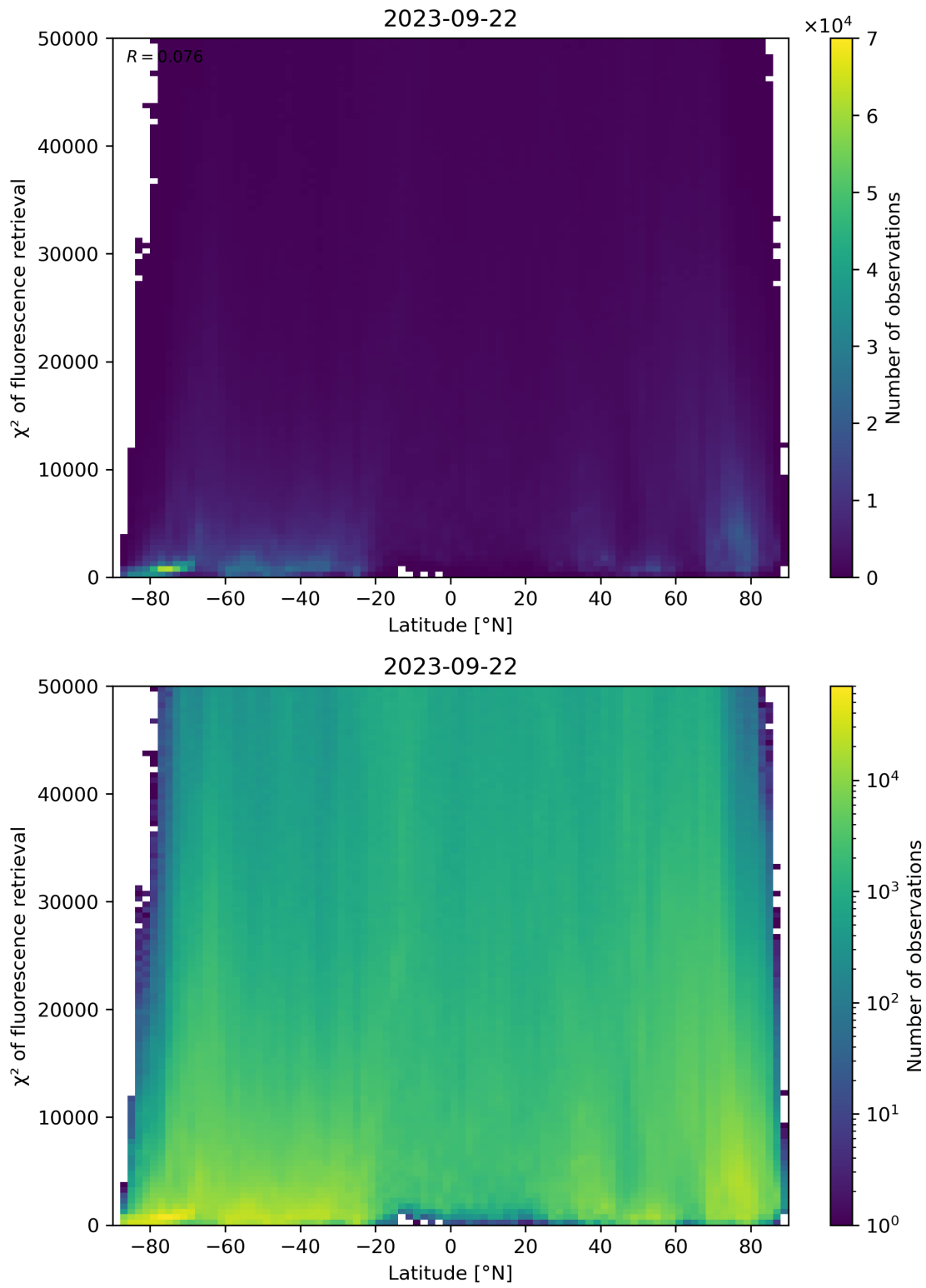
Figure 98: Scatter density plot of “Latitude” against “ \chi^2 of fluorescence retrieval” for 2023-09-21 to 2023-09-23.
