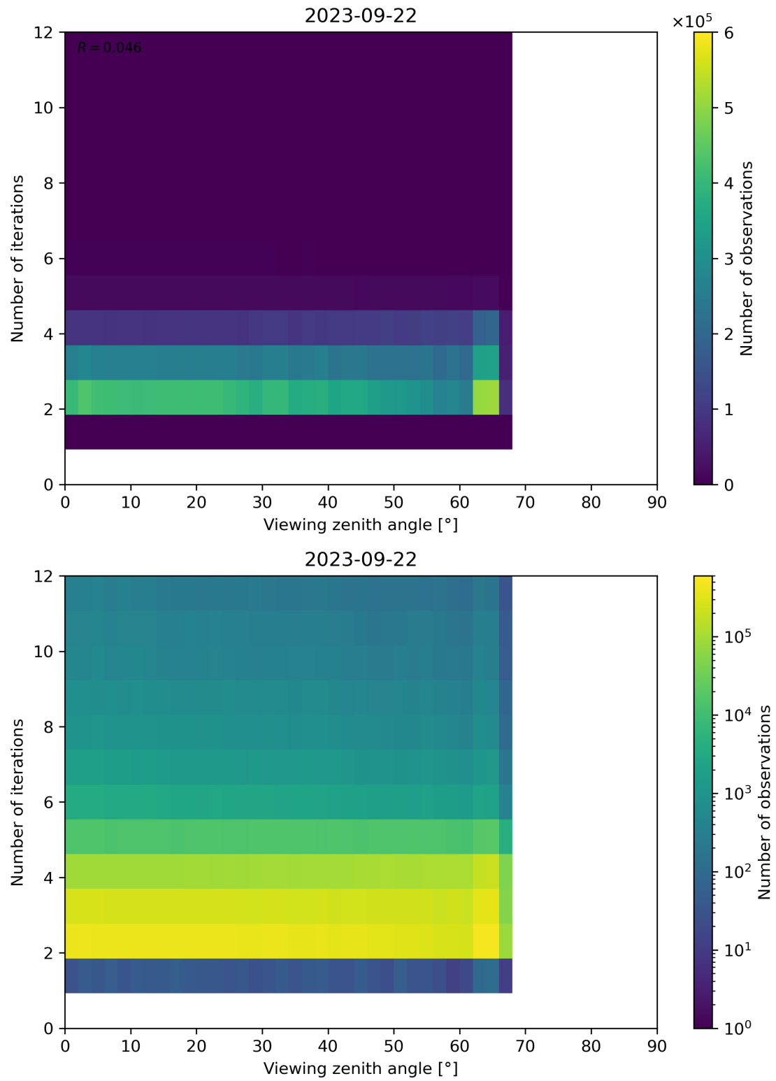
Figure 136: Scatter density plot of “Viewing zenith angle” against “Number of iterations” for 2023-09-21 to 2023-09-23.
