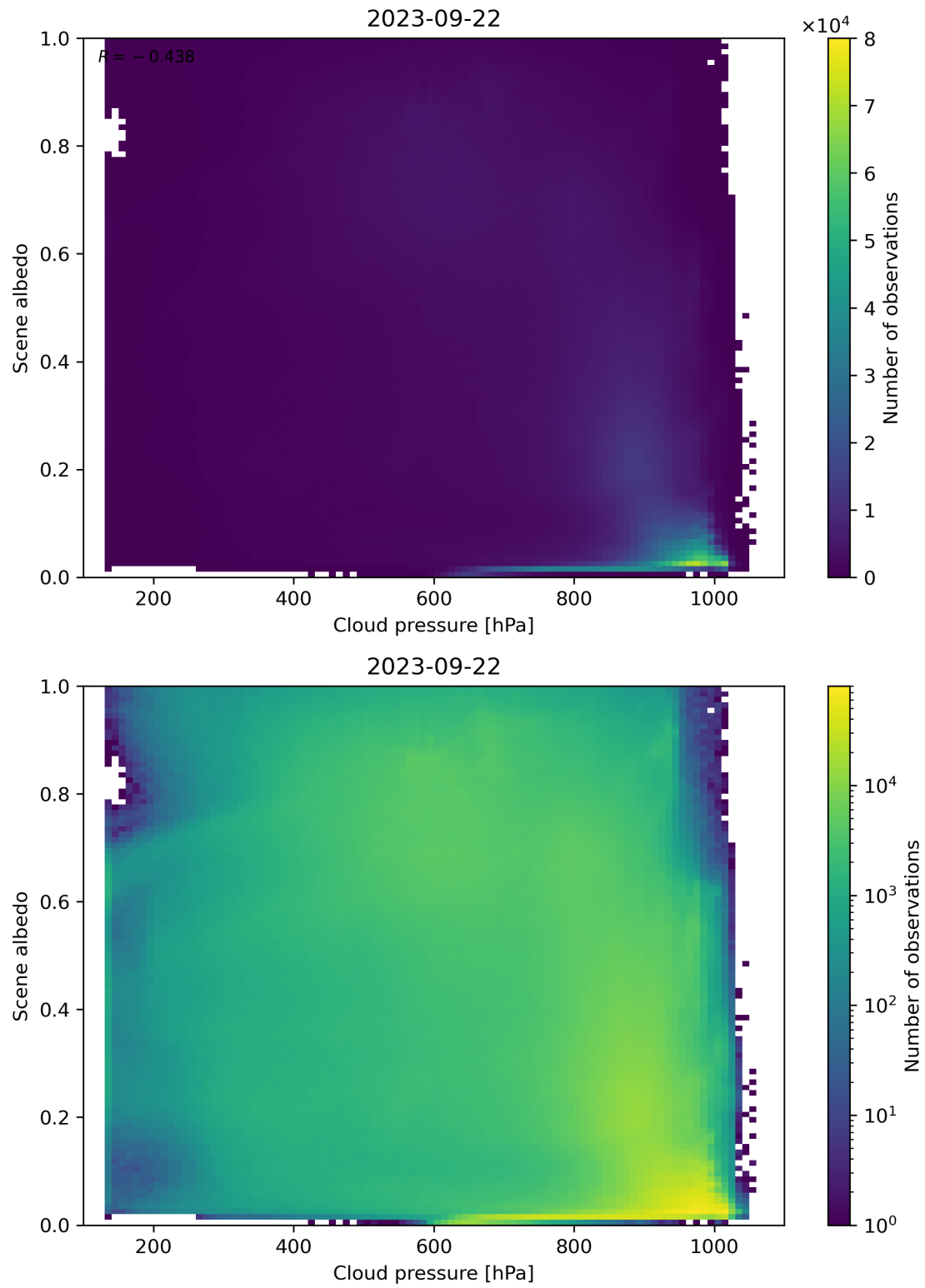
Figure 91: Scatter density plot of “Cloud pressure” against “Scene albedo” for 2023-09-21 to 2023-09-23.
