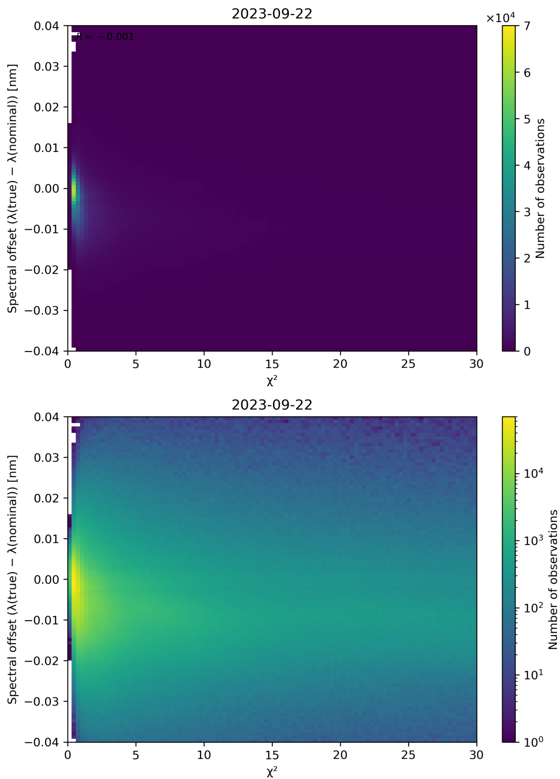
Figure 75: Scatter density plot of “ \chi^2 ” against “Spectral offset ( \lambda(\text{true}) - \lambda(\text{nominal}) )” for 2023-09-21 to 2023-09-23.
