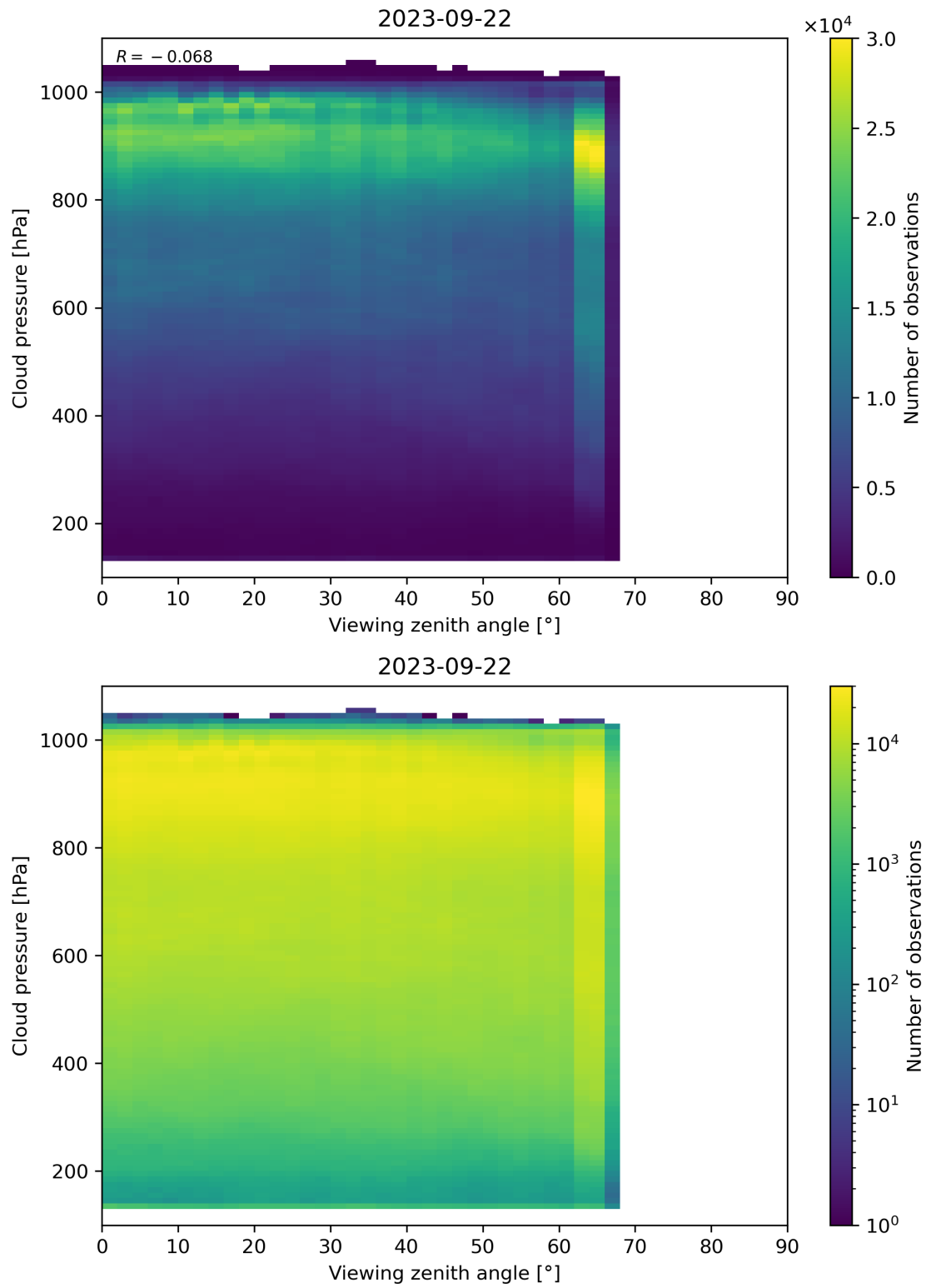
Figure 133: Scatter density plot of “Viewing zenith angle” against “Cloud pressure” for 2023-09-21 to 2023-09-23.
