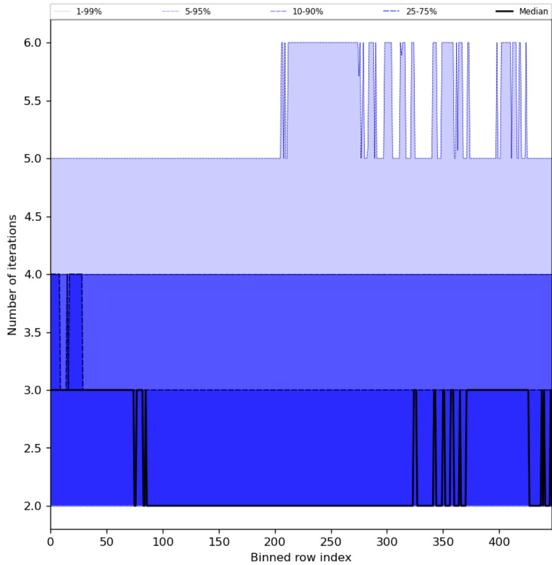
Figure 56: Along track statistics of “Number of iterations” for 2023-09-21 to 2023-09-23
