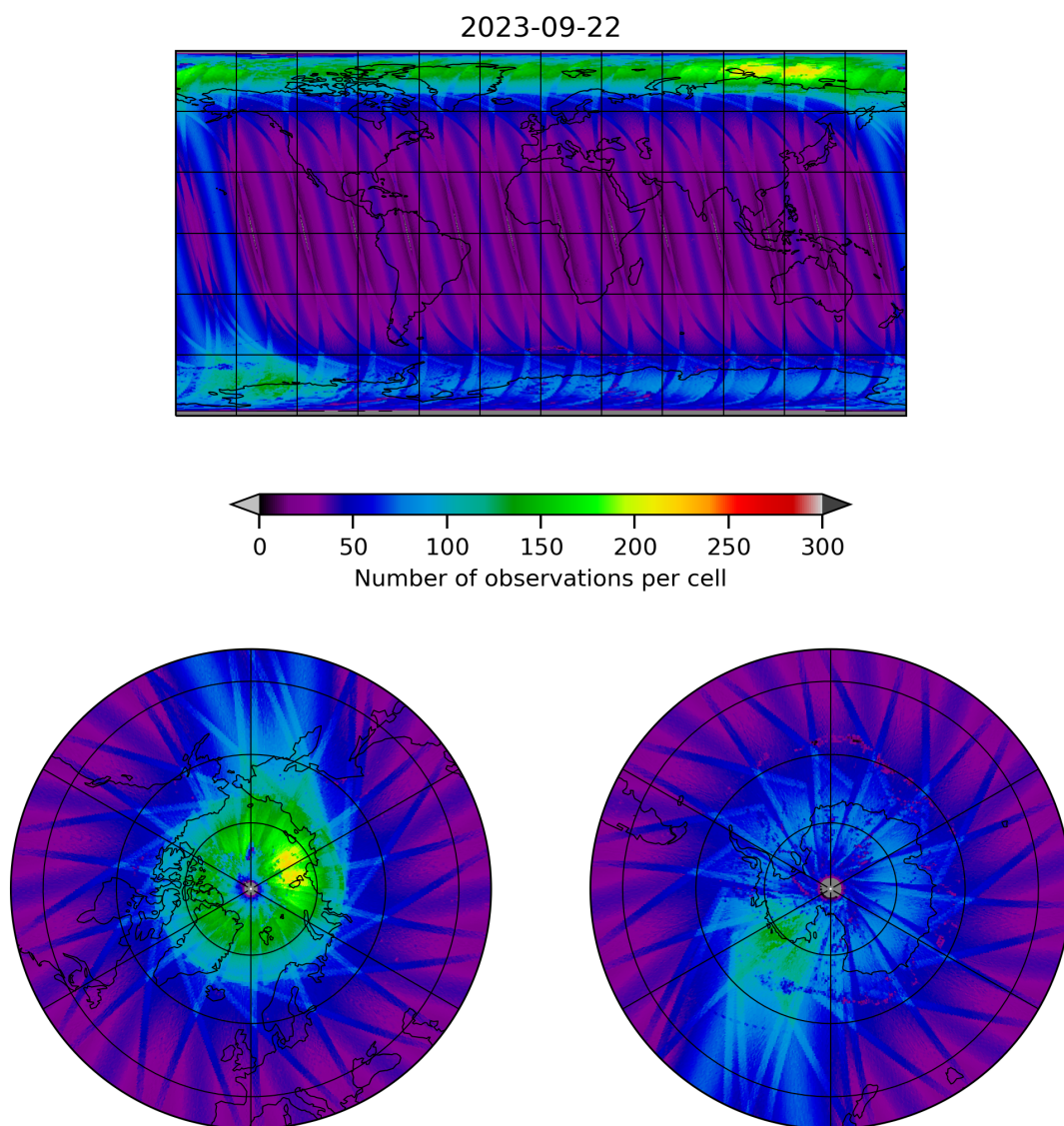
Figure 11: Map of the number of observations for 2023-09-21 to 2023-09-23
