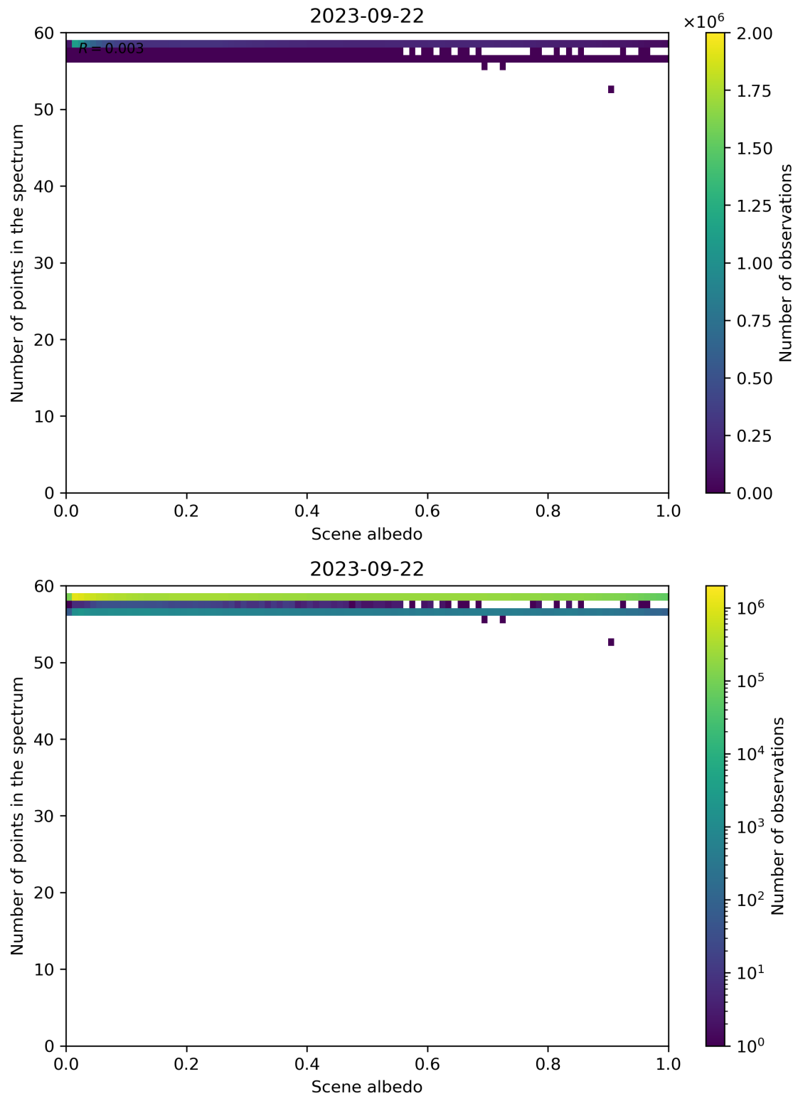
Figure 116: Scatter density plot of “Scene albedo” against “Number of points in the spectrum” for 2023-09-21 to 2023-09-23.
