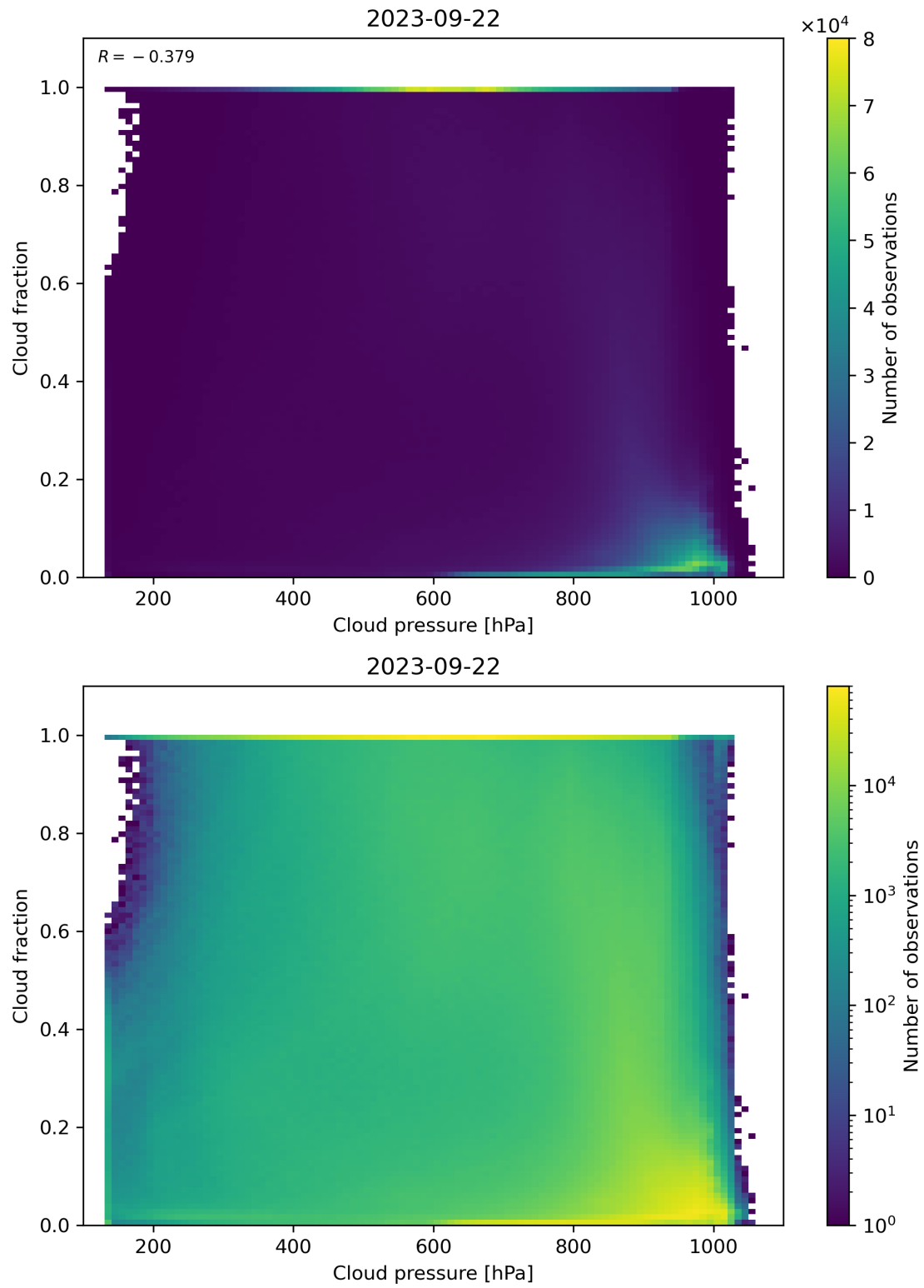
Figure 87: Scatter density plot of “Cloud pressure” against “Cloud fraction” for 2023-09-21 to 2023-09-23.
