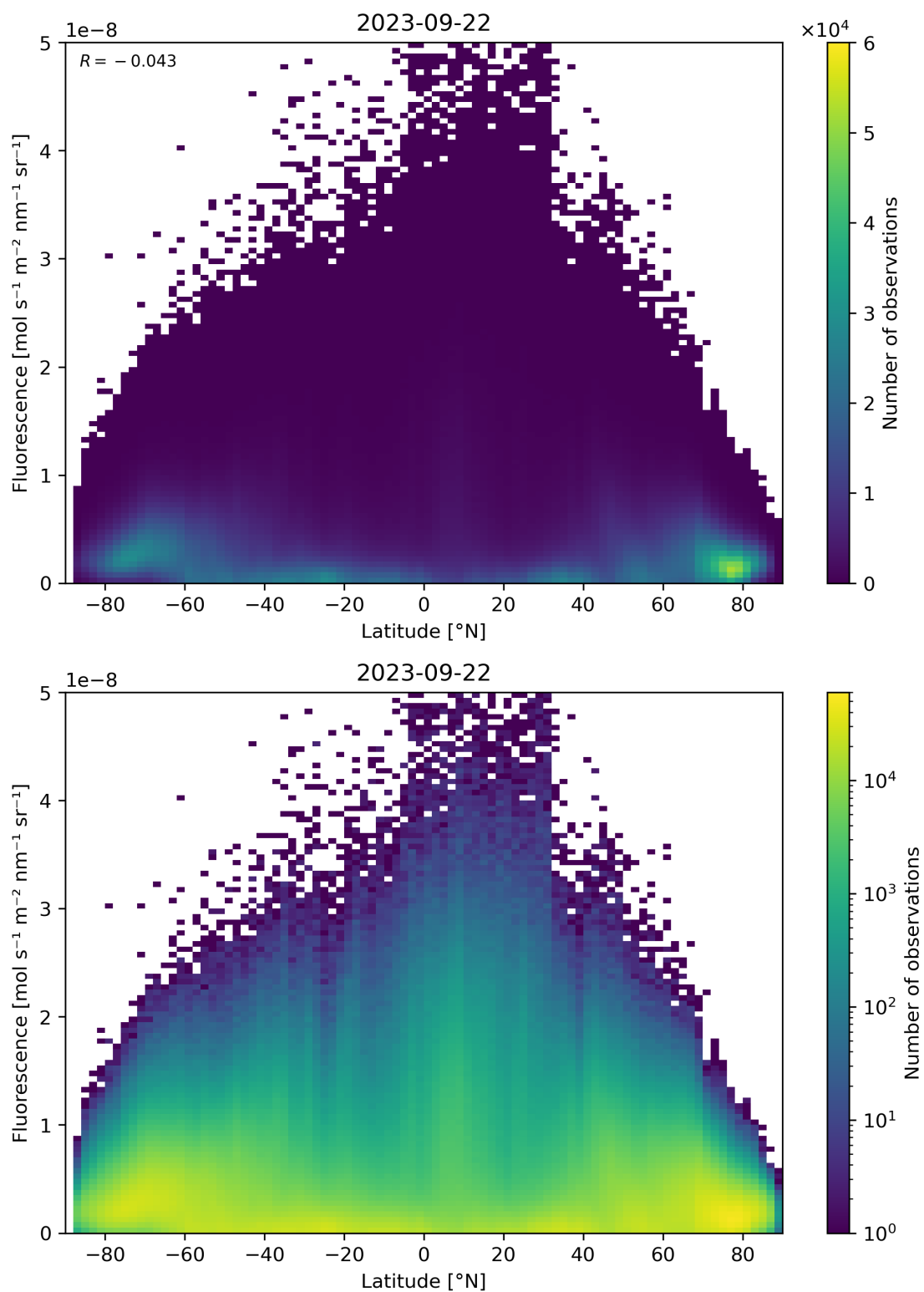
Figure 101: Scatter density plot of “Latitude” against “Fluorescence” for 2023-09-21 to 2023-09-23.
