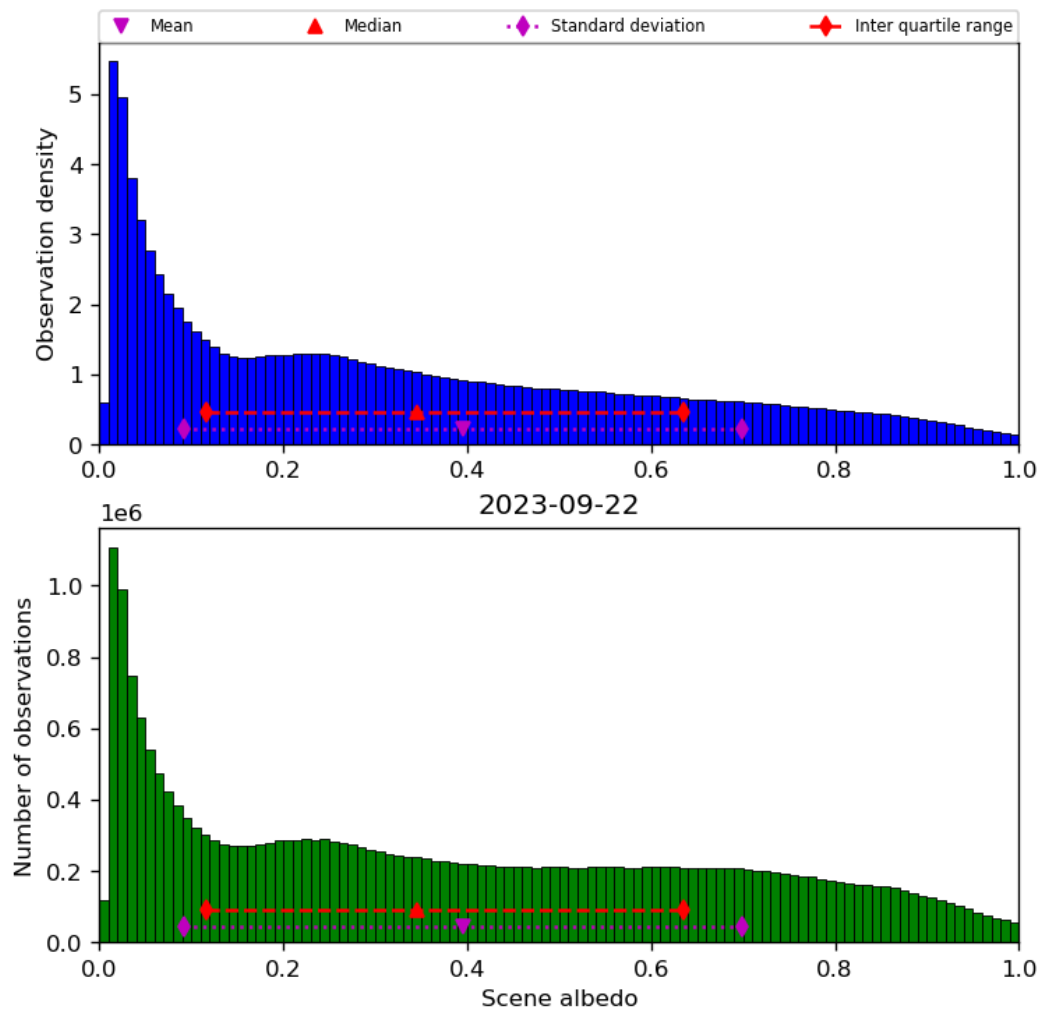
Figure 34: Histogram of “Scene albedo” for 2023-09-21 to 2023-09-23
