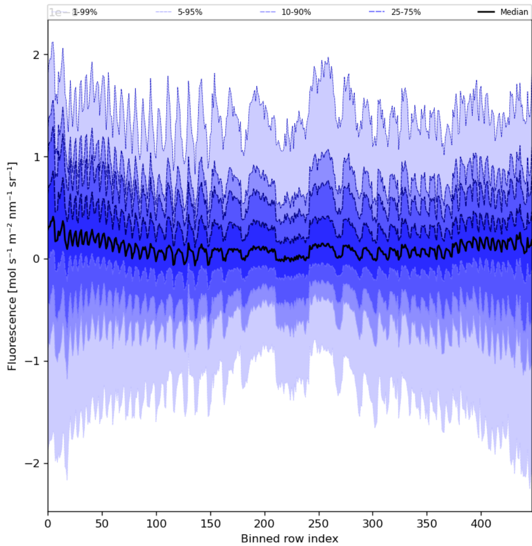
Figure 57: Along track statistics of “Fluorescence” for 2023-09-21 to 2023-09-23
