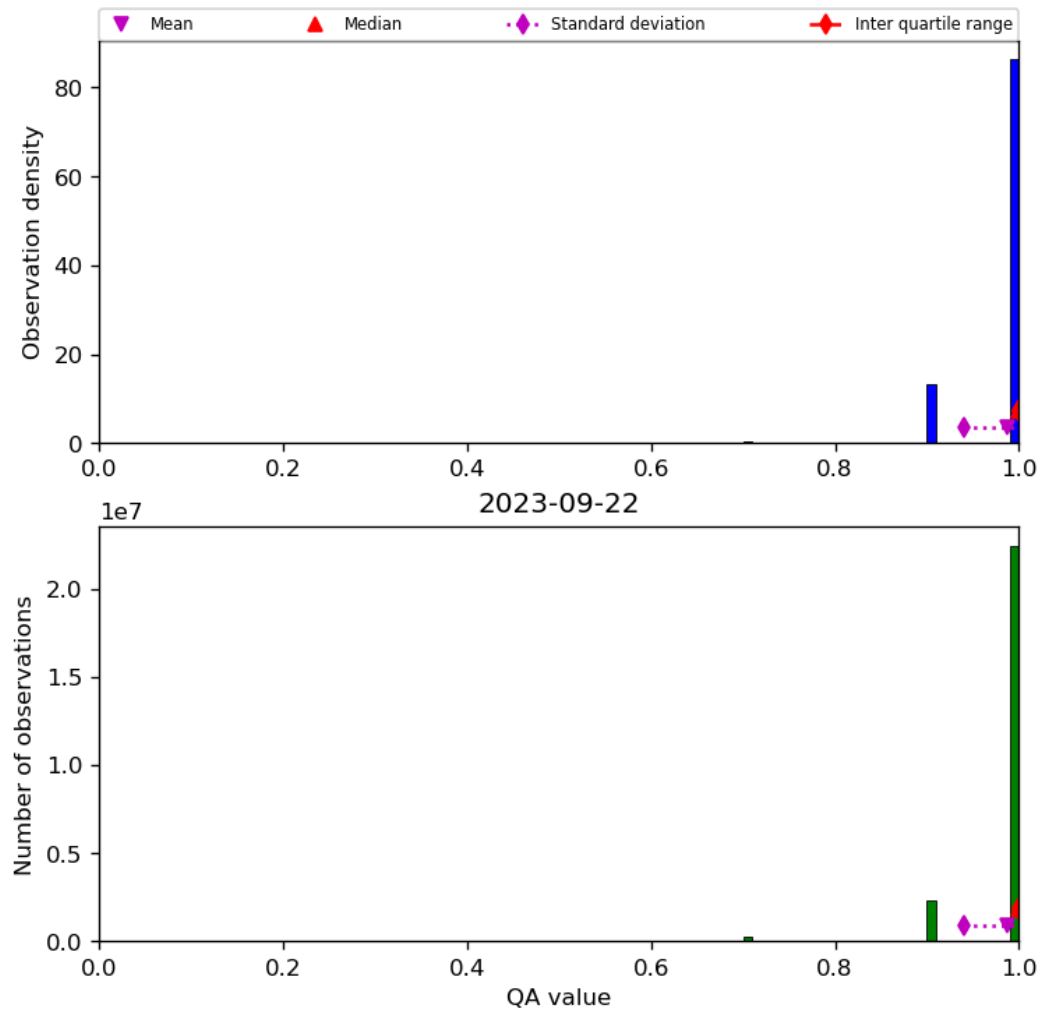
Figure 29: Histogram of “QA value” for 2023-09-21 to 2023-09-23
