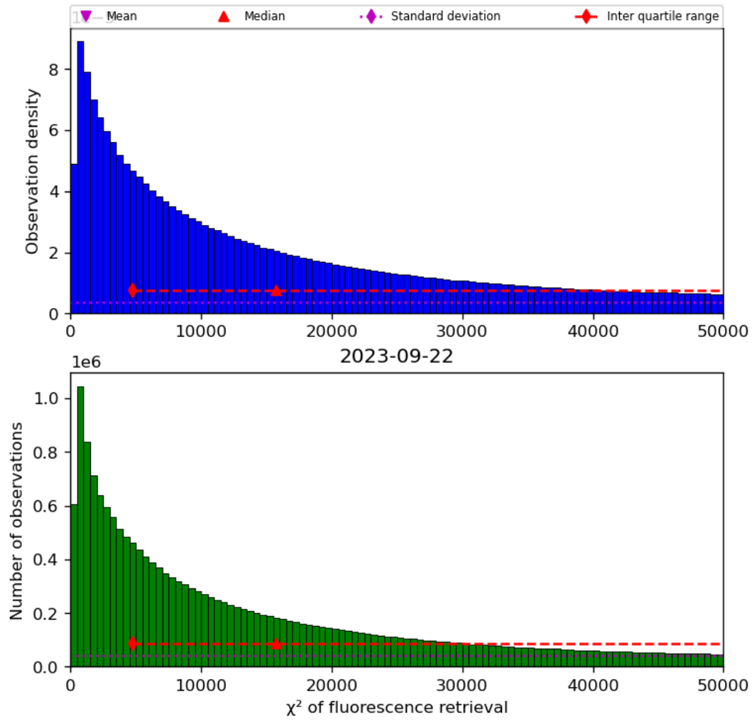
Figure 42: Histogram of “ \chi^2 of fluorescence retrieval” for 2023-09-21 to 2023-09-23
