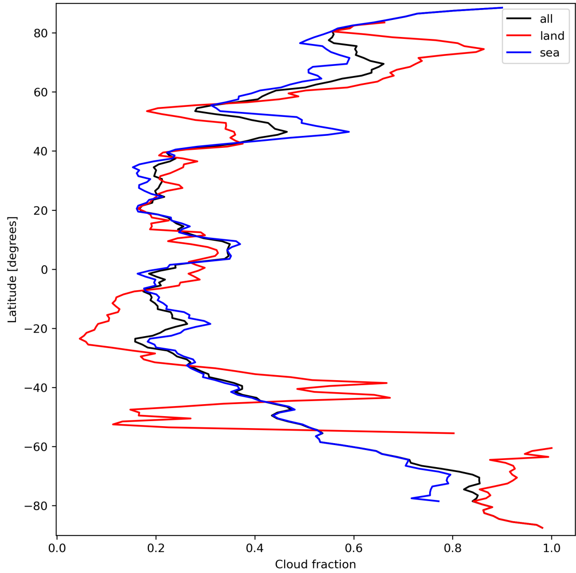
Figure 15: Zonal average of “Cloud fraction” for 2023-09-21 to 2023-09-23.
