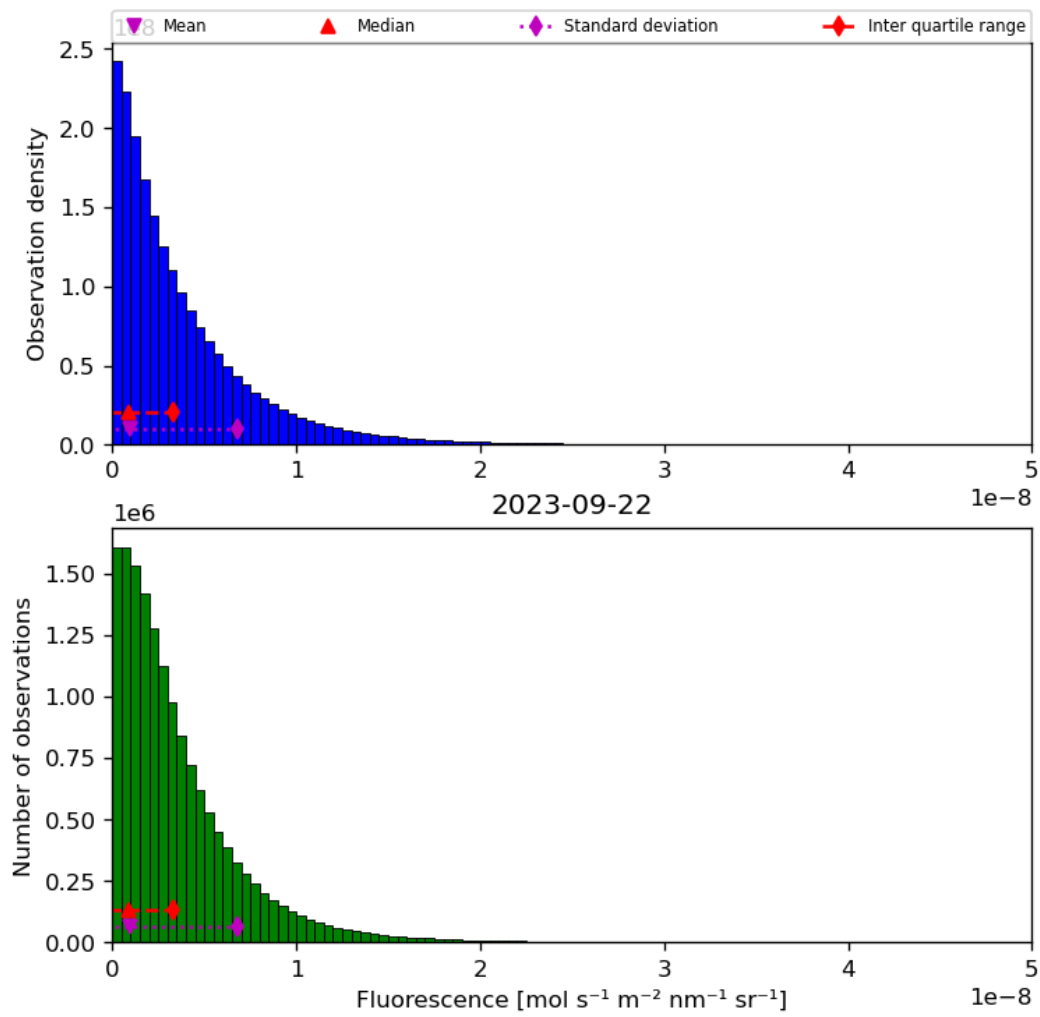
Figure 40: Histogram of “Fluorescence” for 2023-09-21 to 2023-09-23
