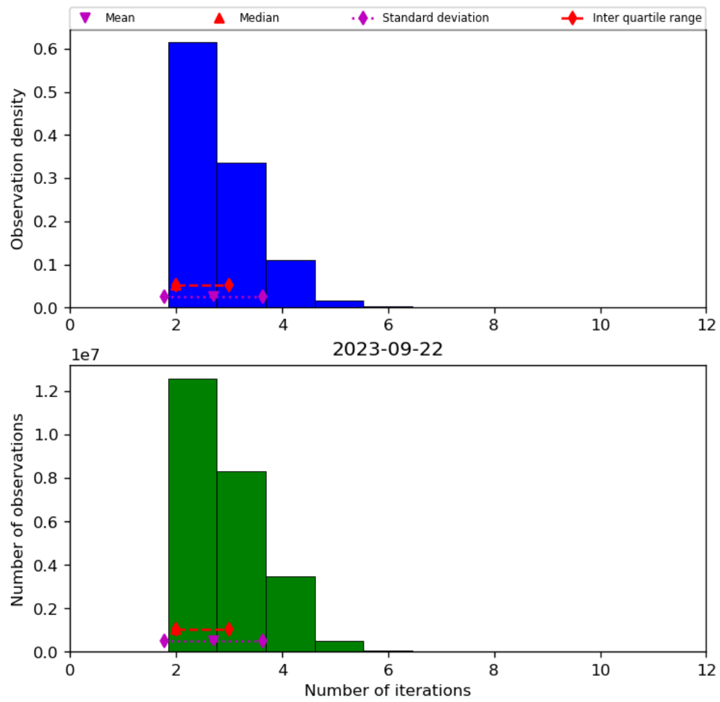
Figure 39: Histogram of “Number of iterations” for 2023-09-21 to 2023-09-23
