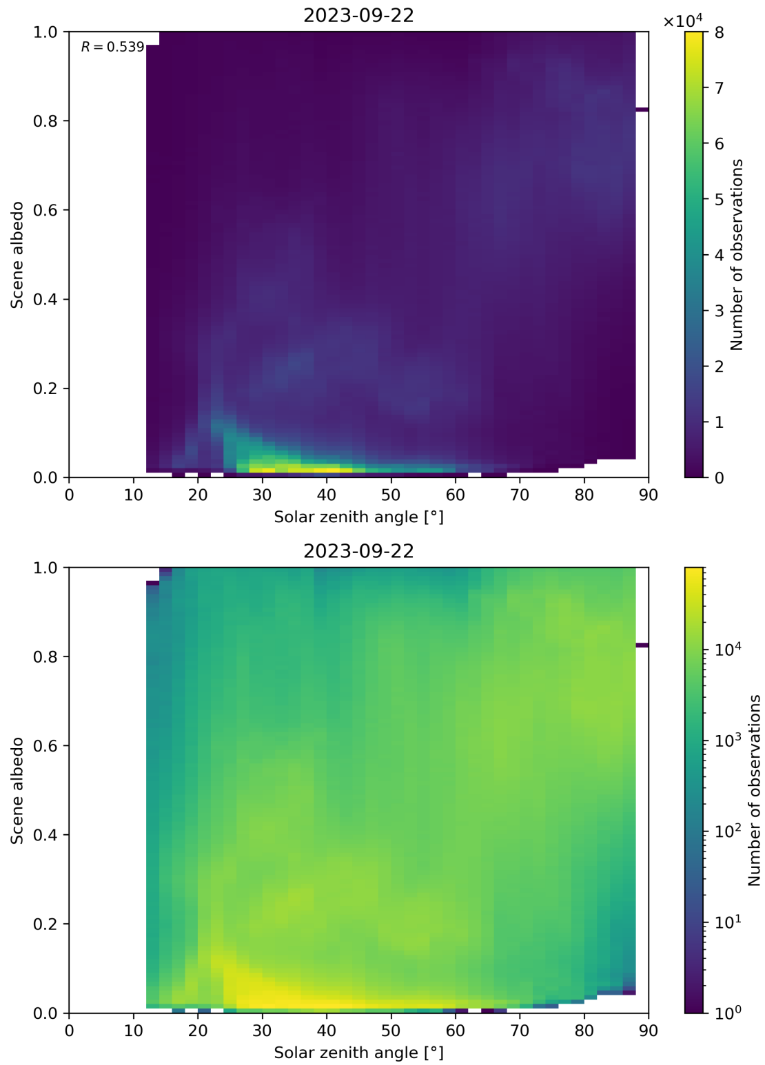
Figure 127: Scatter density plot of “Solar zenith angle” against “Scene albedo” for 2023-09-21 to 2023-09-23.
