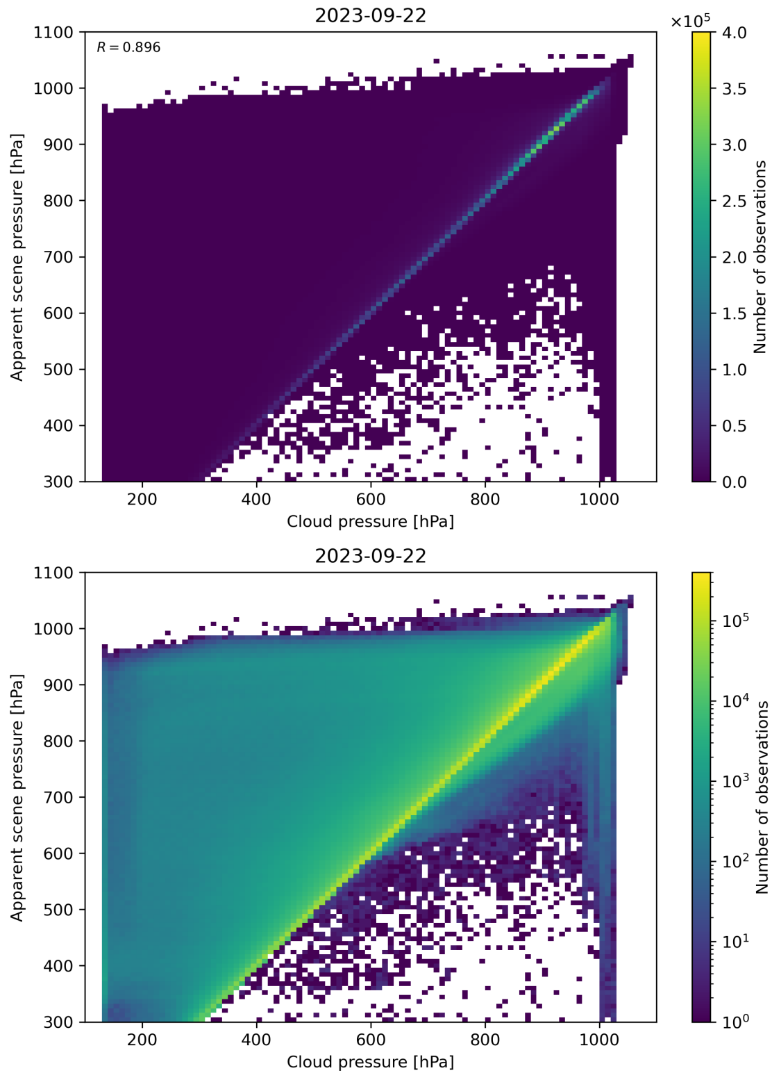
Figure 84: Scatter density plot of “Cloud pressure” against “Apparent scene pressure” for 2023-09-21 to 2023-09-23.
