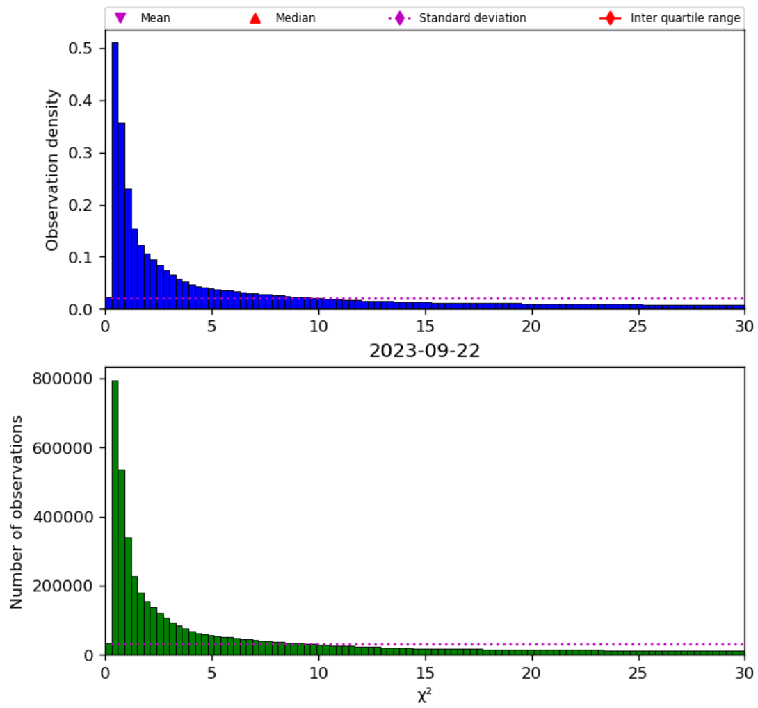
Figure 38: Histogram of " \chi^2 " for 2023-09-21 to 2023-09-23
