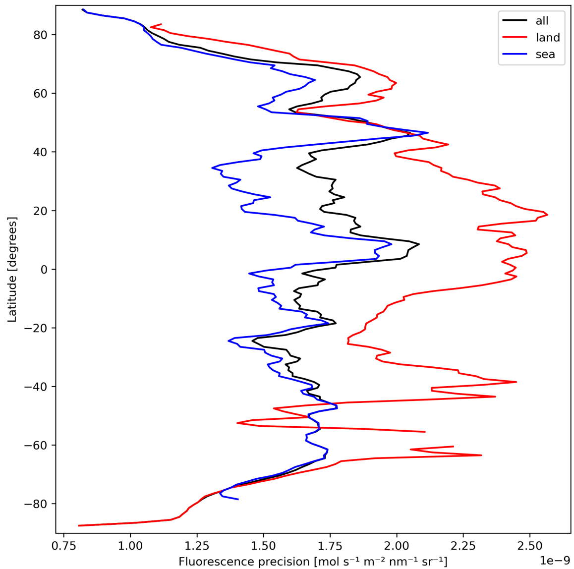
Figure 24: Zonal average of “Fluorescence precision” for 2023-09-21 to 2023-09-23.
