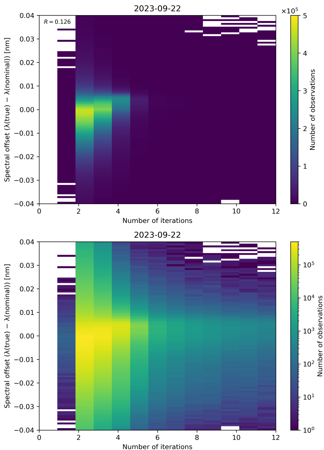
Figure 109: Scatter density plot of “Number of iterations” against “Spectral offset ( \lambda(\text{true}) - \lambda(\text{nominal}) )” for 2023-09-21 to 2023-09-23.
