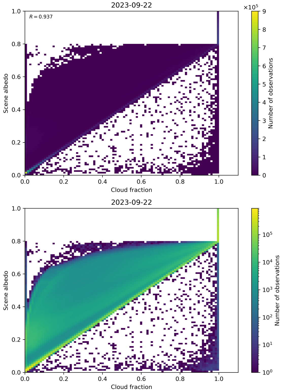
Figure 82: Scatter density plot of “Cloud fraction” against “Scene albedo” for 2023-09-21 to 2023-09-23.
