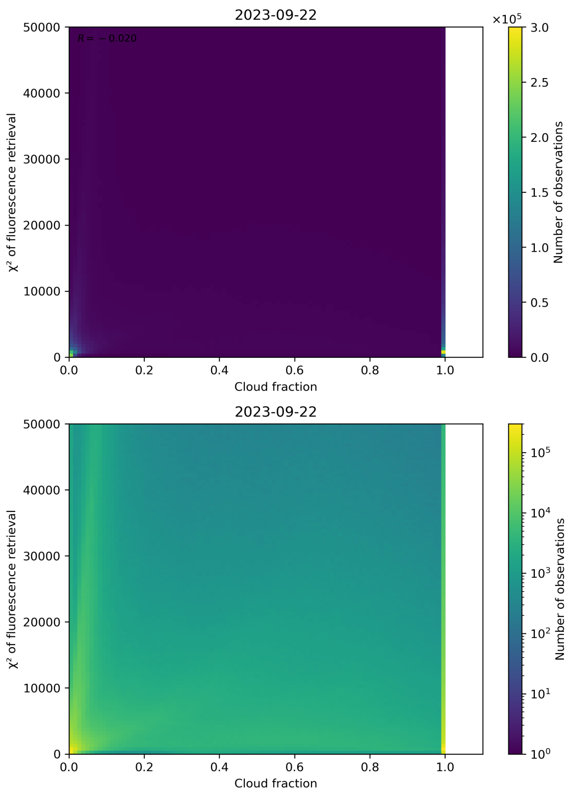
Figure 78: Scatter density plot of “Cloud fraction” against “ \chi^2 of fluorescence retrieval” for 2023-09-21 to 2023-09-23.
