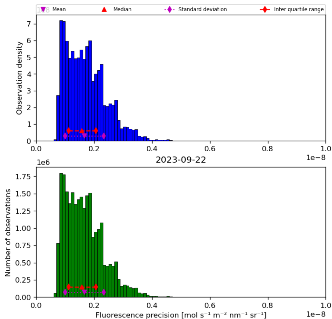
Figure 41: Histogram of “Fluorescence precision” for 2023-09-21 to 2023-09-23
