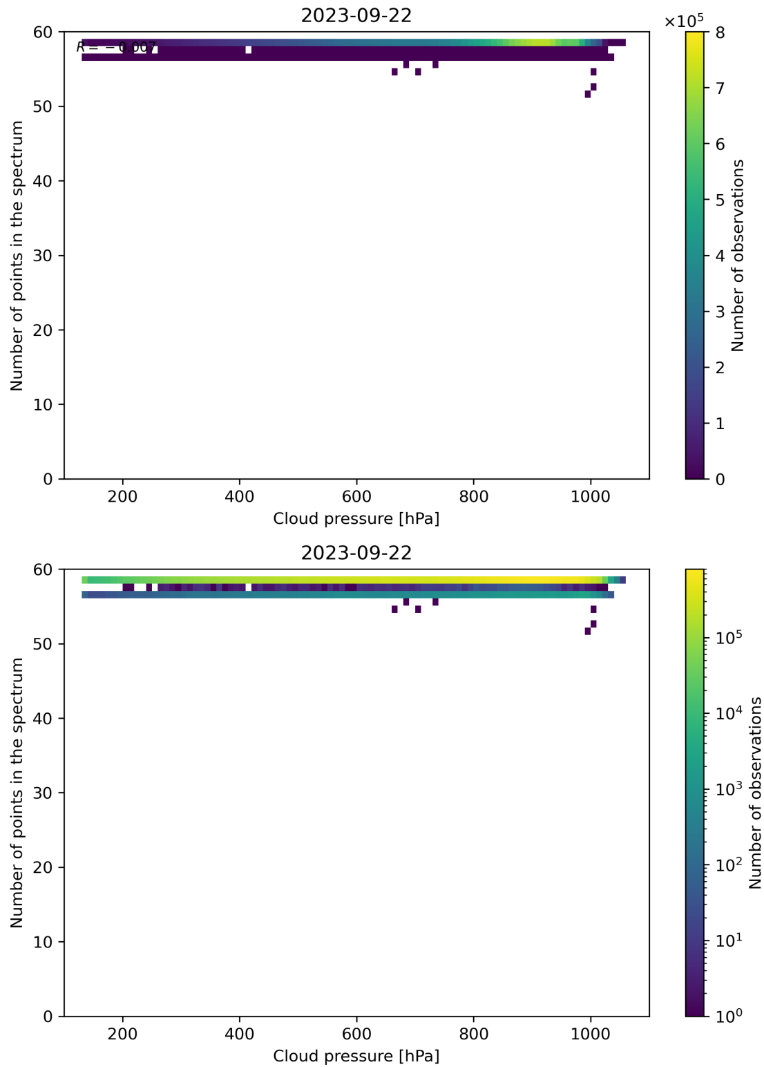
Figure 90: Scatter density plot of “Cloud pressure” against “Number of points in the spectrum” for 2023-09-21 to 2023-09-23.
