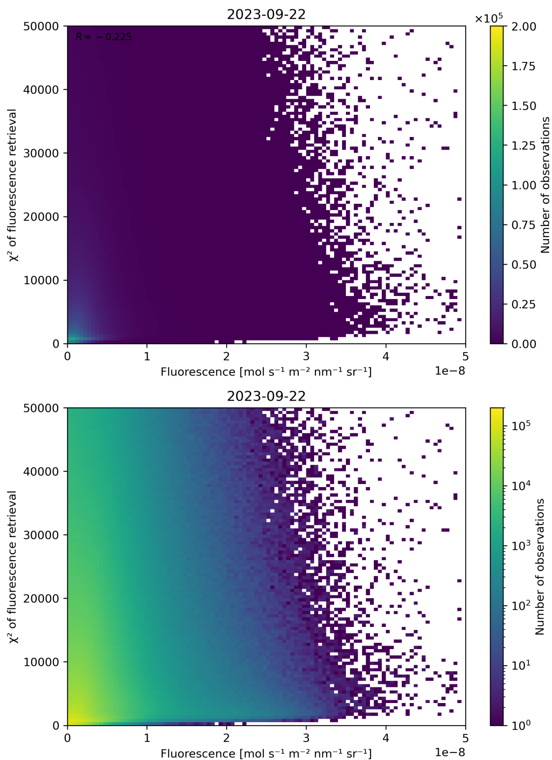
Figure 93: Scatter density plot of “Fluorescence” against “ \chi^2 of fluorescence retrieval” for 2023-09-21 to 2023-09-23.
