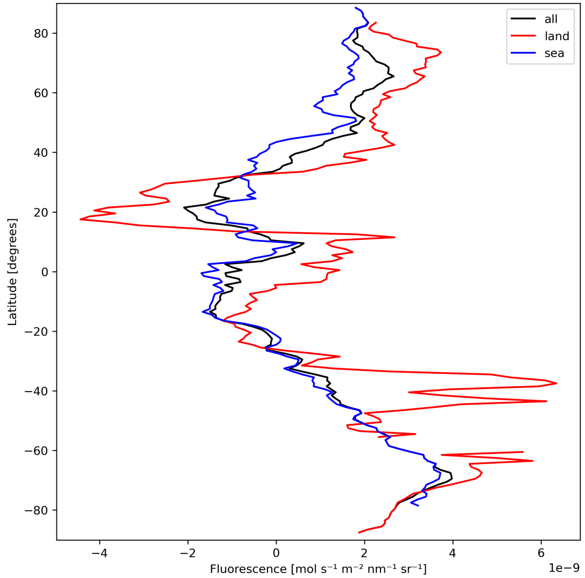
Figure 23: Zonal average of “Fluorescence” for 2023-09-21 to 2023-09-23.
