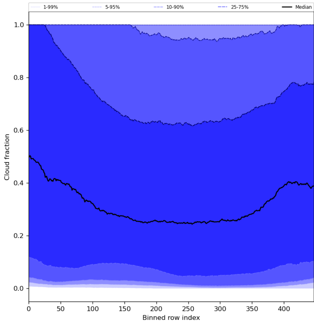
Figure 49: Along track statistics of “Cloud fraction” for 2023-09-21 to 2023-09-23
