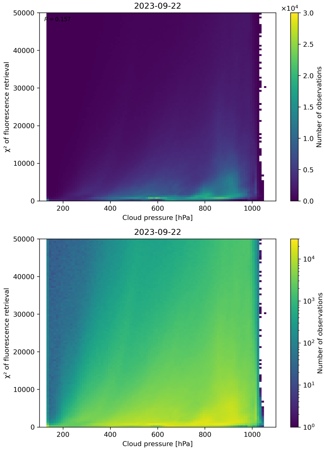
Figure 86: Scatter density plot of “Cloud pressure” against “ \chi^2 of fluorescence retrieval” for 2023-09-21 to 2023-09-23.
