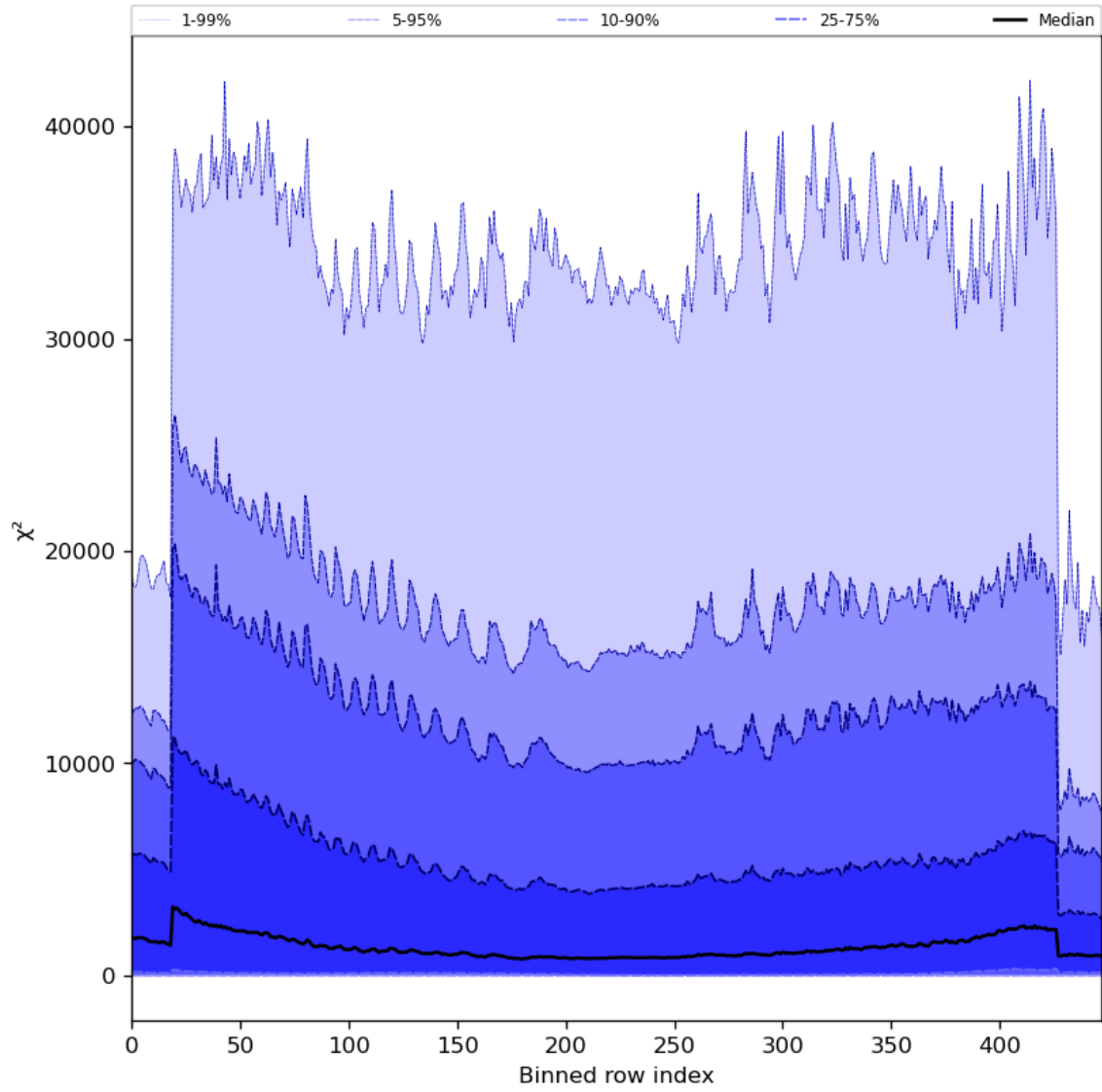
Figure 55: Along track statistics of “ \chi^2 ” for 2023-09-21 to 2023-09-23
