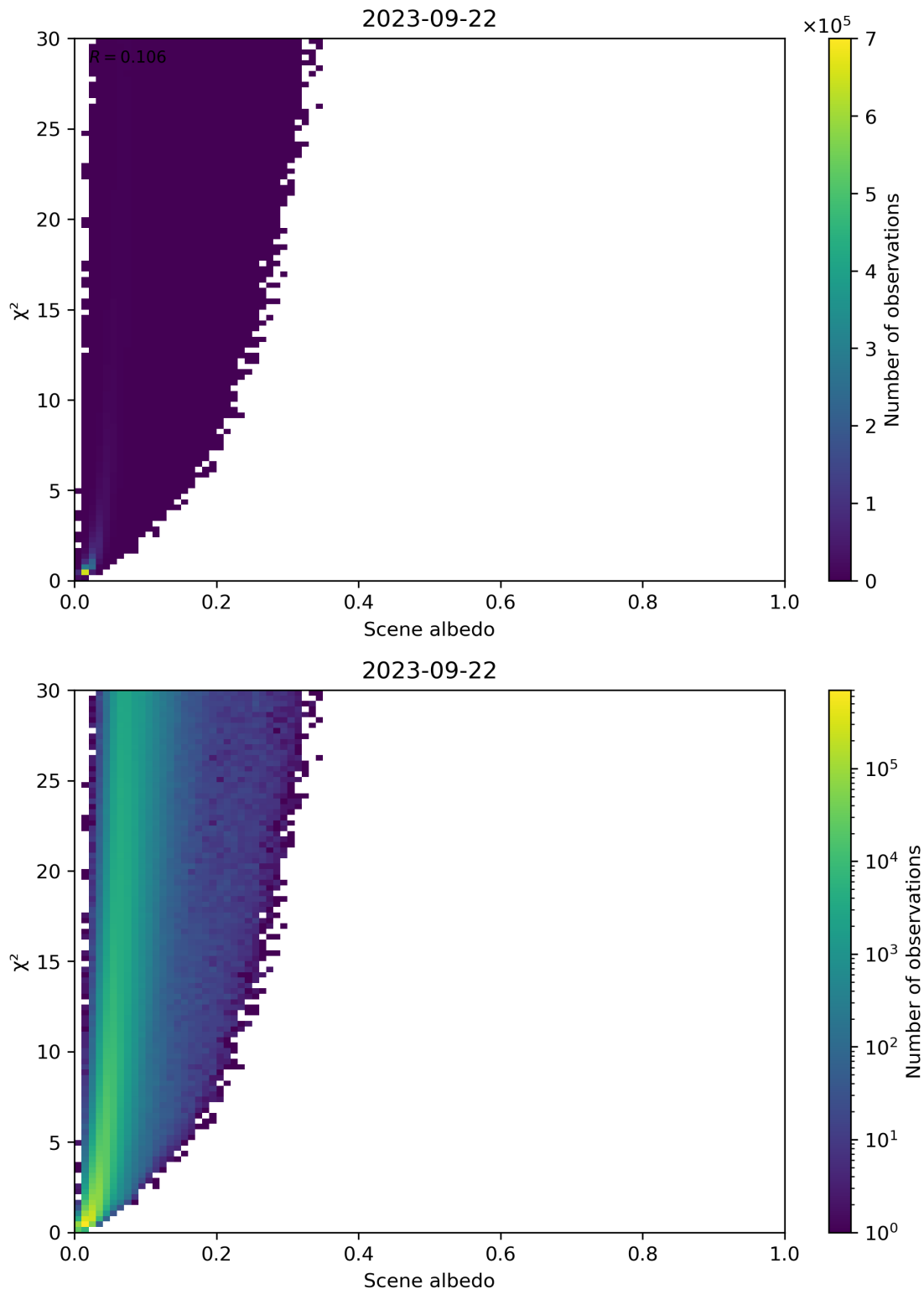
Figure 112: Scatter density plot of “Scene albedo” against “ \chi^2 ” for 2023-09-21 to 2023-09-23.
