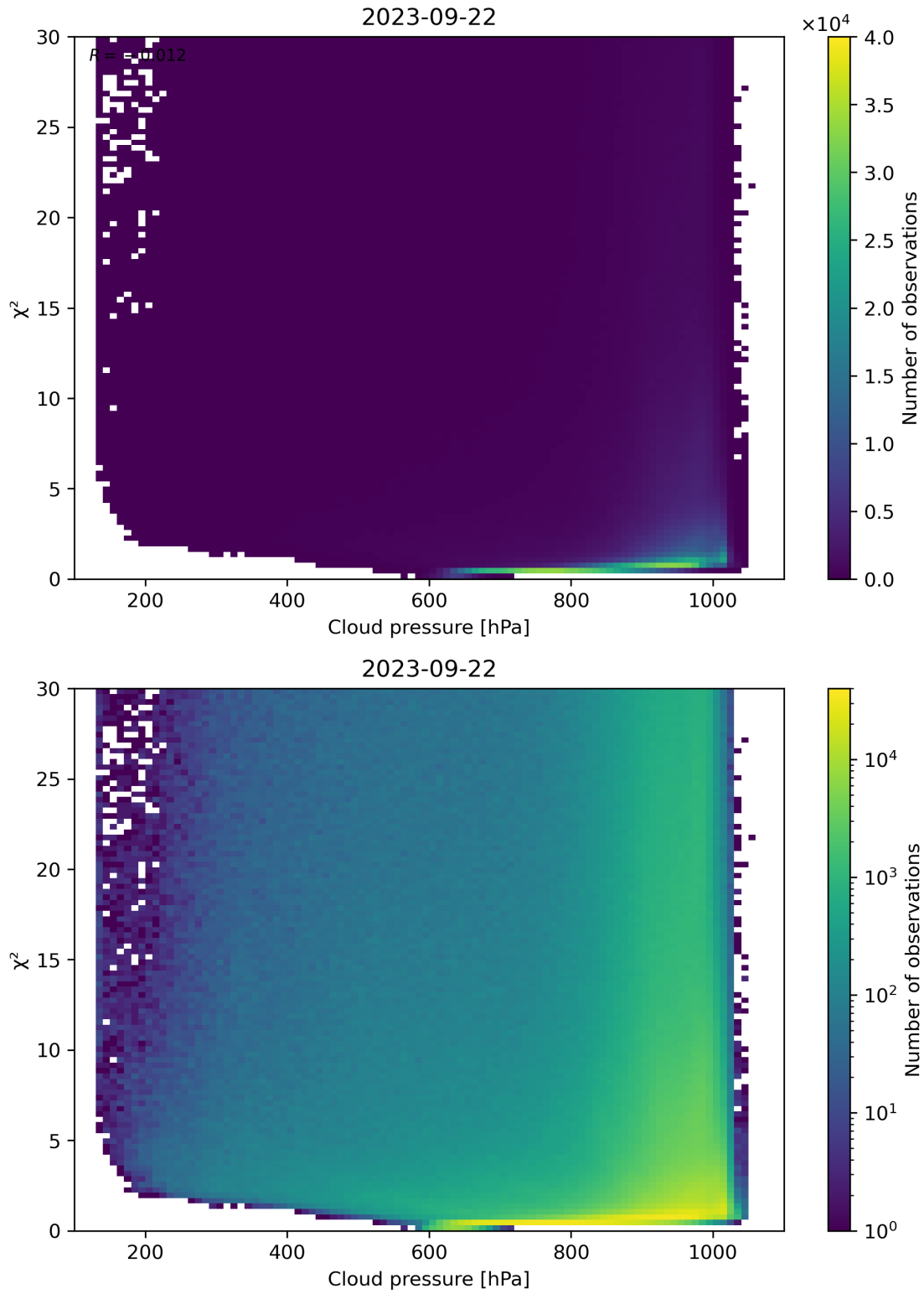
Figure 85: Scatter density plot of “Cloud pressure” against “ \chi^2 ” for 2023-09-21 to 2023-09-23.
