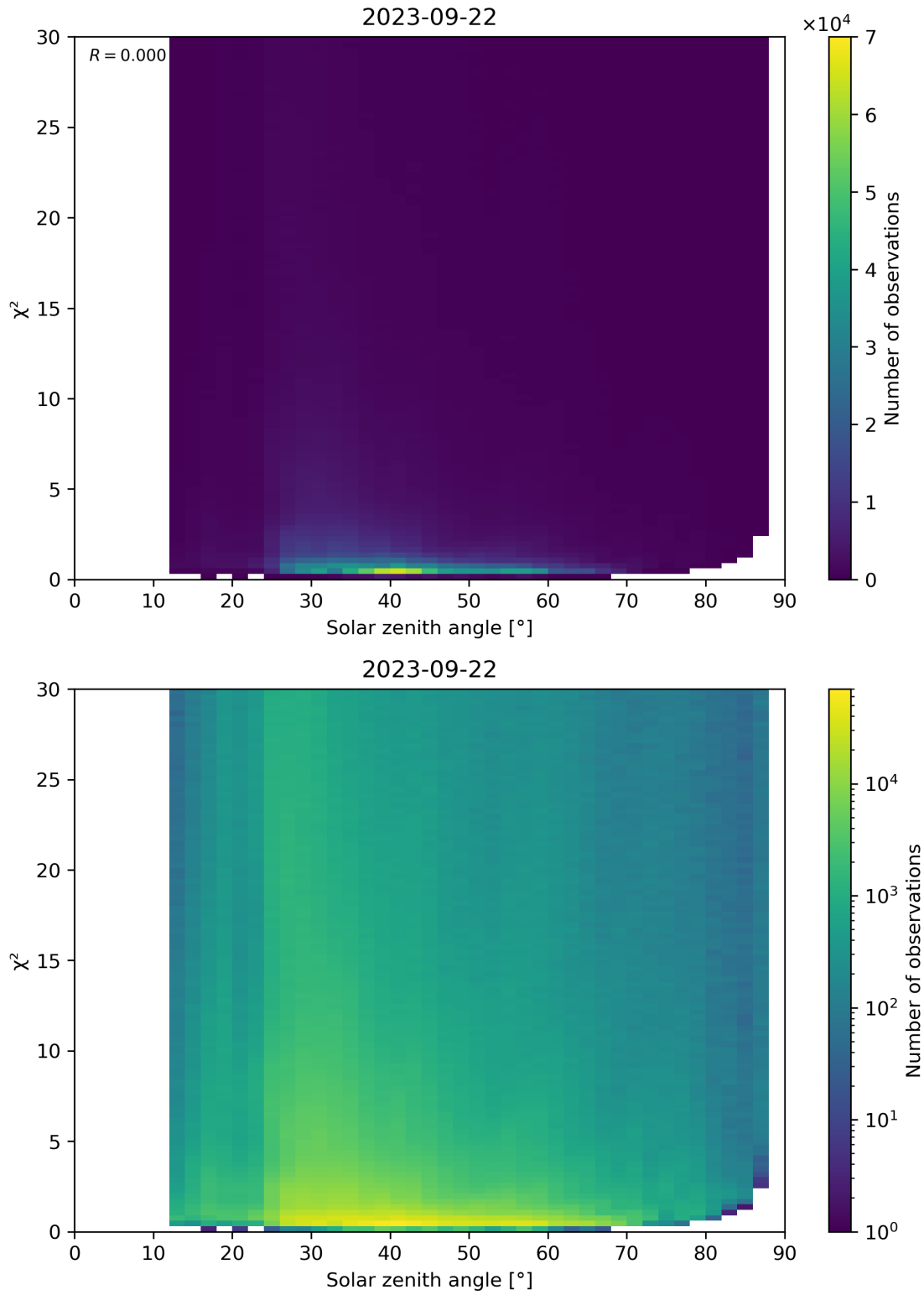
Figure 119: Scatter density plot of “Solar zenith angle” against “ \chi^2 ” for 2023-09-21 to 2023-09-23.
