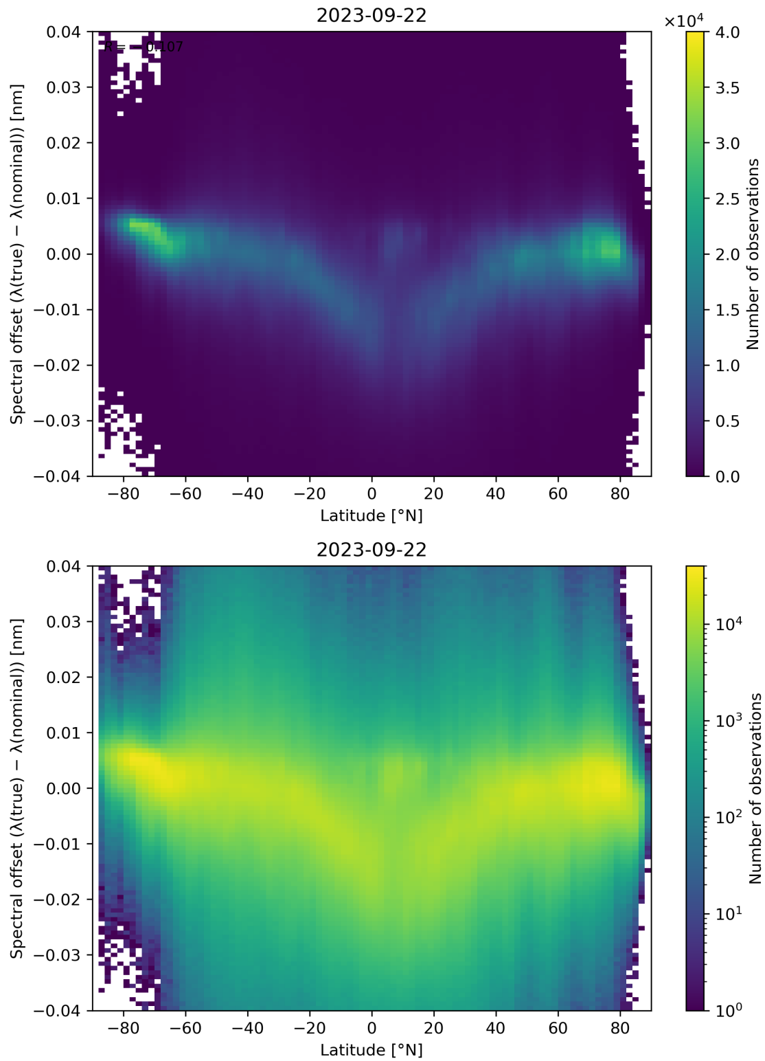
Figure 105: Scatter density plot of “Latitude” against “Spectral offset ( \lambda(\text{true}) - \lambda(\text{nominal}) )” for 2023-09-21 to 2023-09-23.
