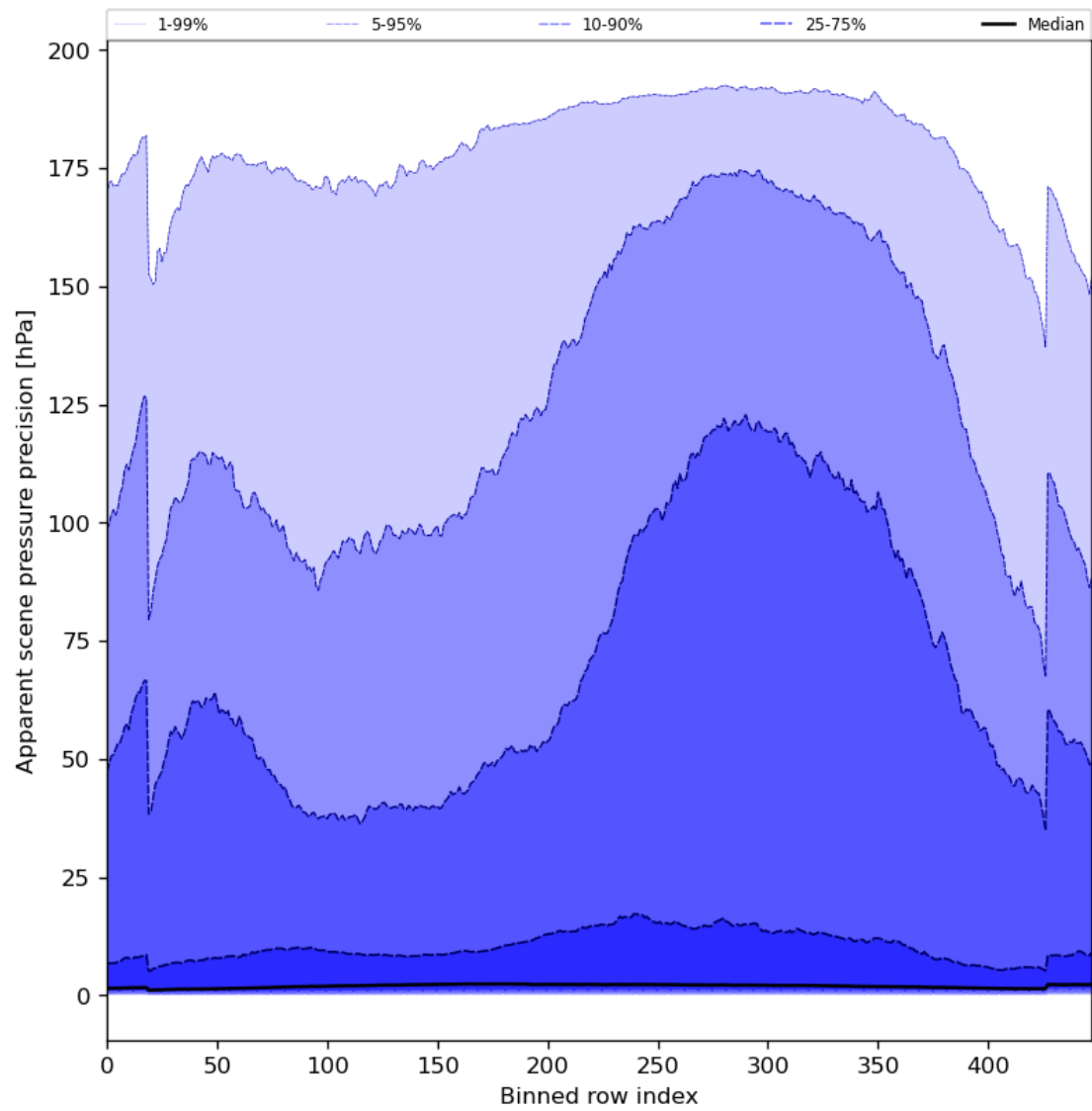
Figure 54: Along track statistics of “Apparent scene pressure precision” for 2023-09-21 to 2023-09-23
