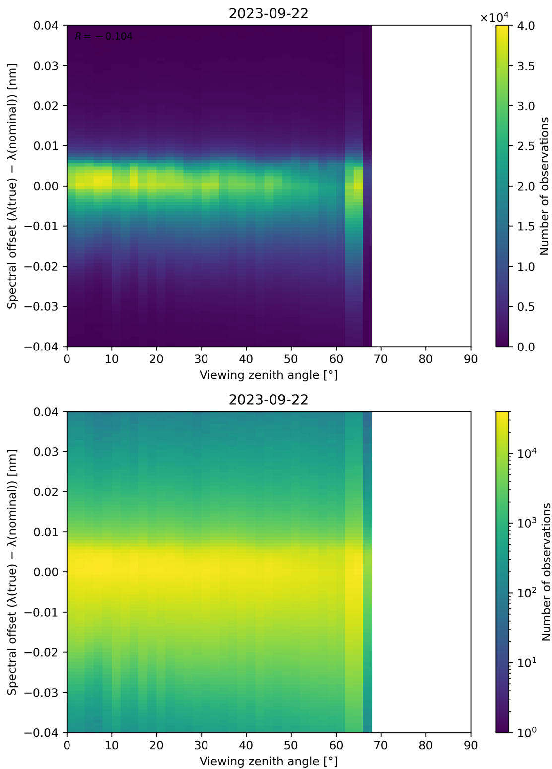
Figure 140: Scatter density plot of “Viewing zenith angle” against “Spectral offset ( \lambda(\text{true}) - \lambda(\text{nominal}) )” for 2023-09-21 to 2023-09-23.
