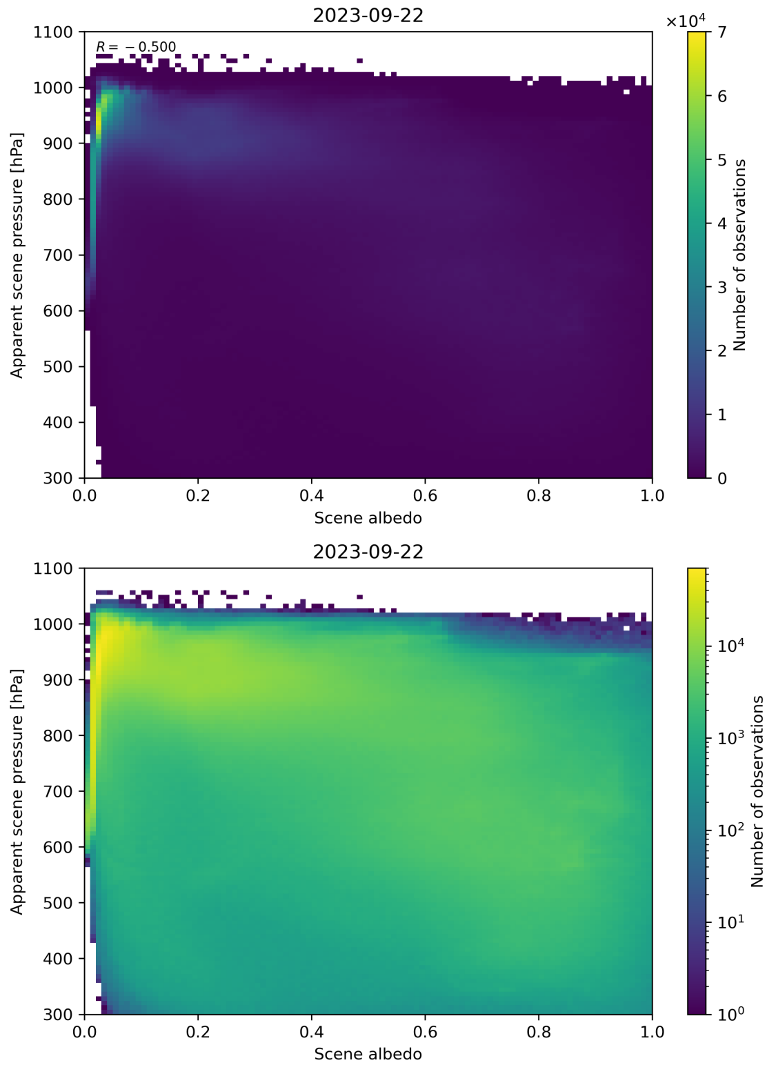
Figure 111: Scatter density plot of “Scene albedo” against “Apparent scene pressure” for 2023-09-21 to 2023-09-23.
