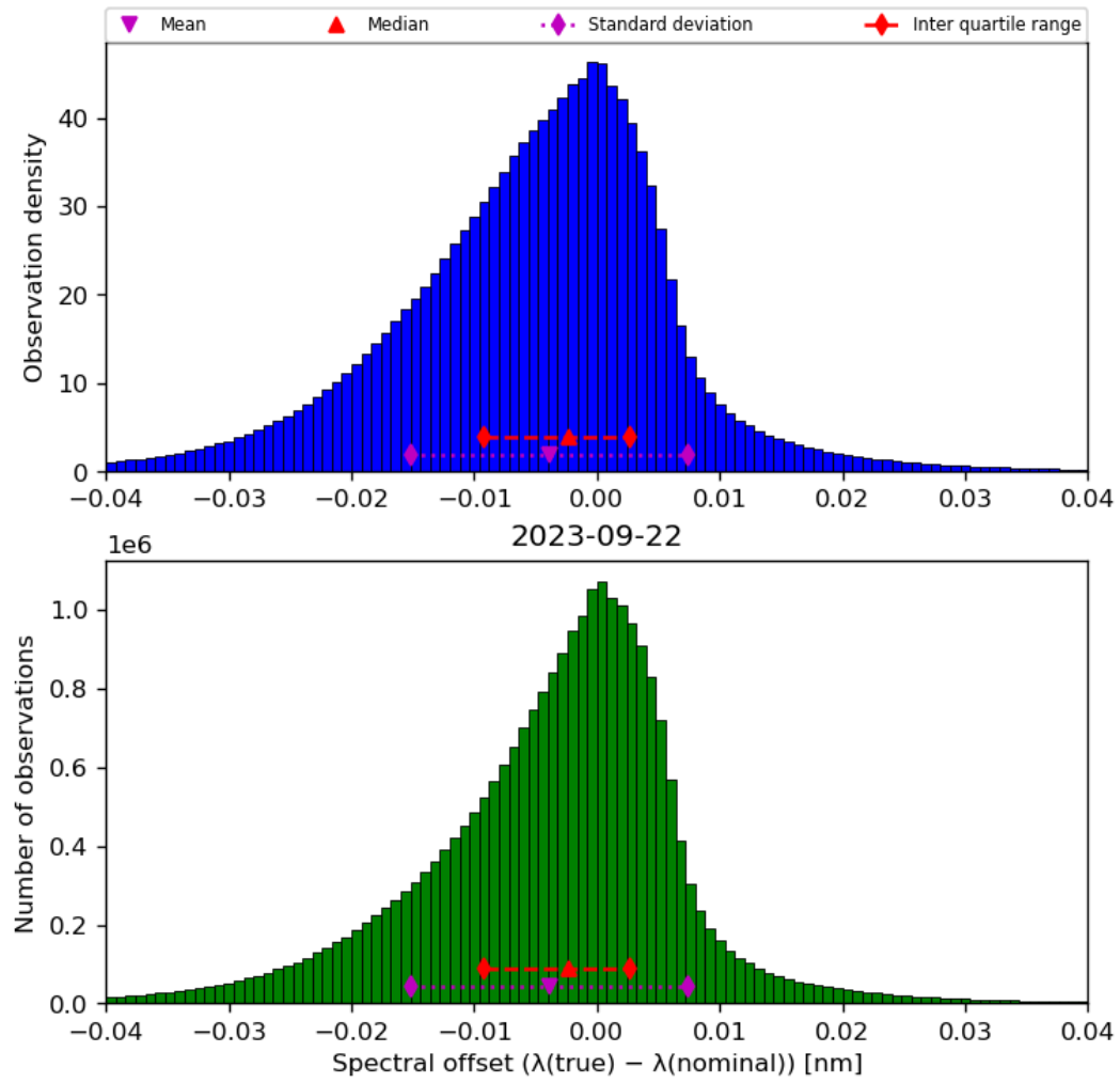
Figure 45: Histogram of “Spectral offset ( \lambda(\text{true}) - \lambda(\text{nominal}) )” for 2023-09-21 to 2023-09-23
