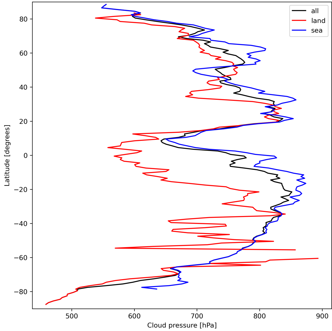
Figure 13: Zonal average of “Cloud pressure” for 2023-09-21 to 2023-09-23.
