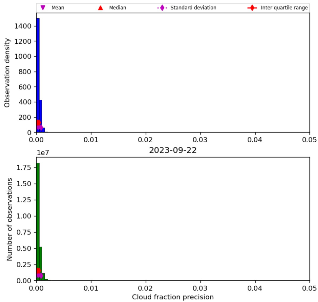
Figure 33: Histogram of “Cloud fraction precision” for 2023-09-21 to 2023-09-23
