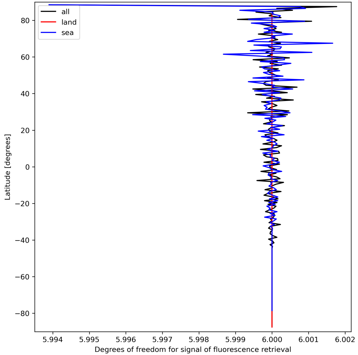
Figure 26: Zonal average of “Degrees of freedom for signal of fluorescence retrieval” for 2023-09-21 to 2023-09-23.
