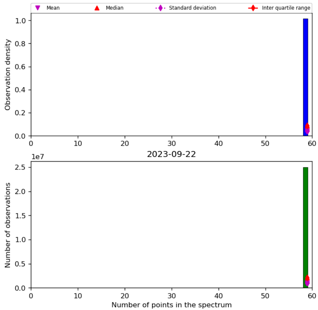
Figure 44: Histogram of “Number of points in the spectrum” for 2023-09-21 to 2023-09-23
