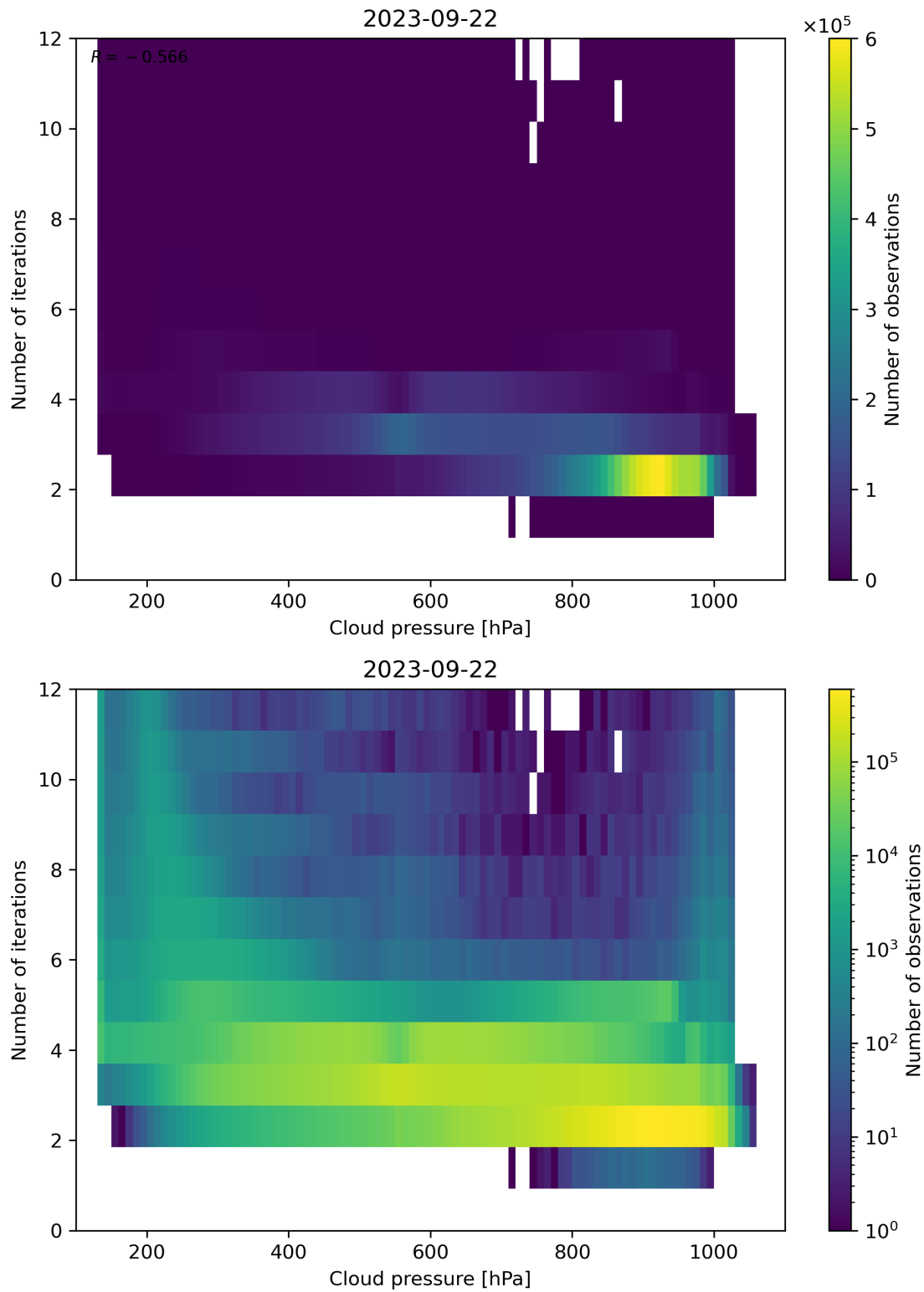
Figure 89: Scatter density plot of “Cloud pressure” against “Number of iterations” for 2023-09-21 to 2023-09-23.
