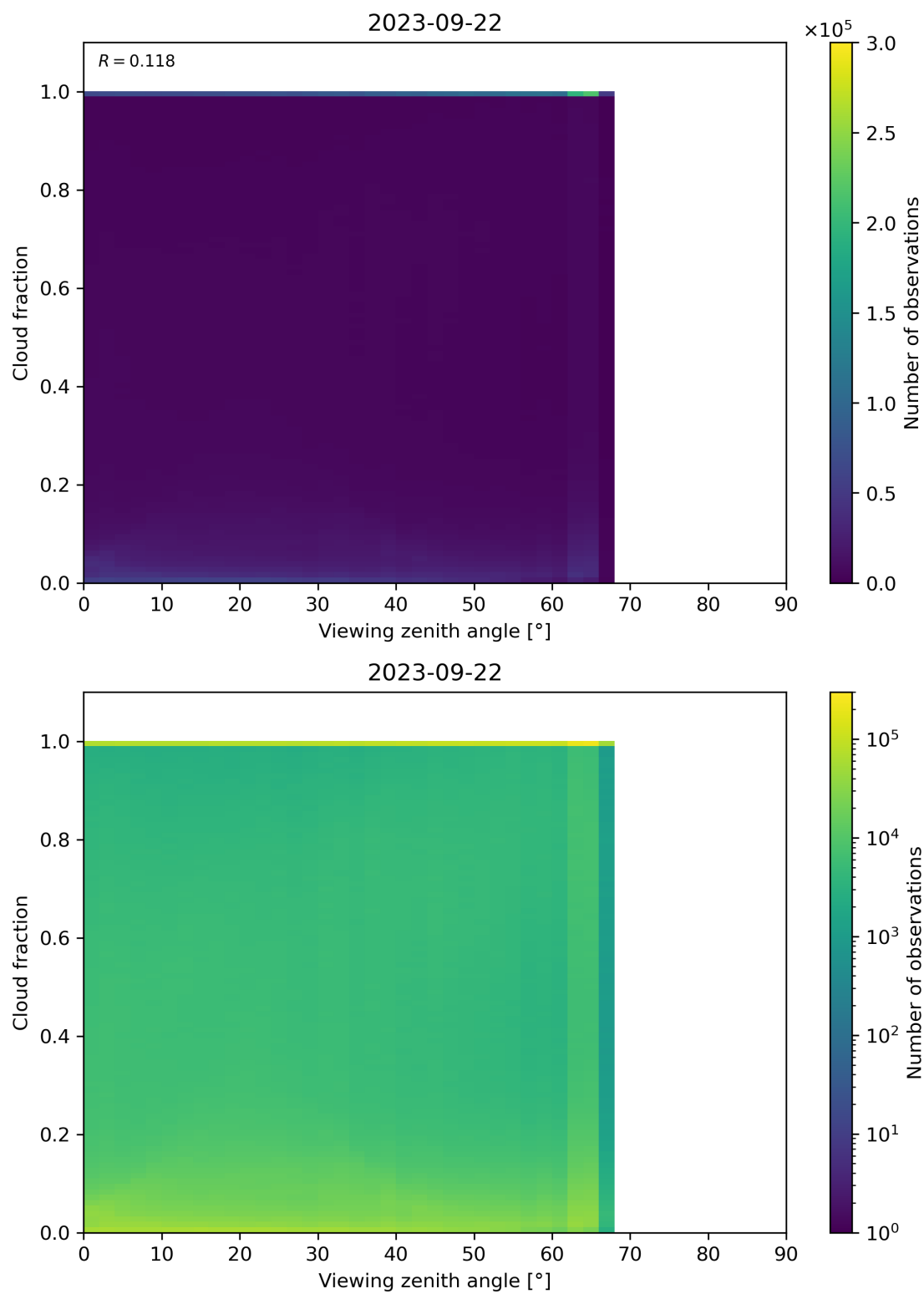
Figure 132: Scatter density plot of “Viewing zenith angle” against “Cloud fraction” for 2023-09-21 to 2023-09-23.
