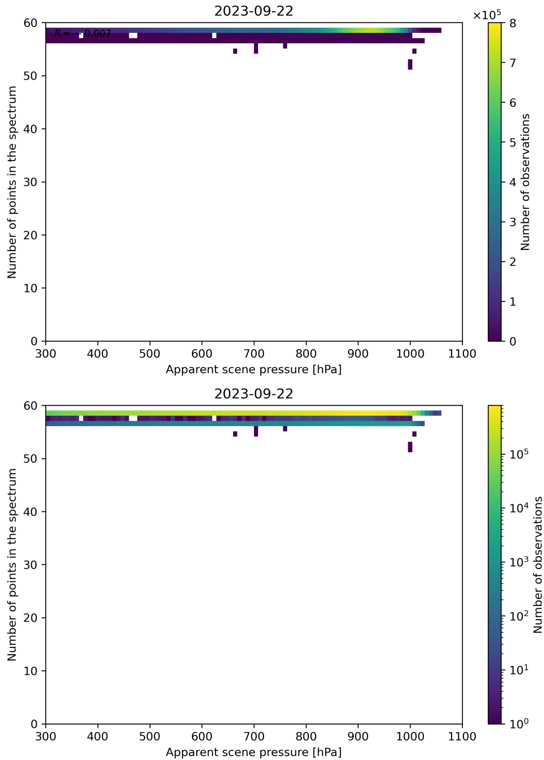
Figure 67: Scatter density plot of “Apparent scene pressure” against “Number of points in the spectrum” for 2023-09-21 to 2023-09-23.
