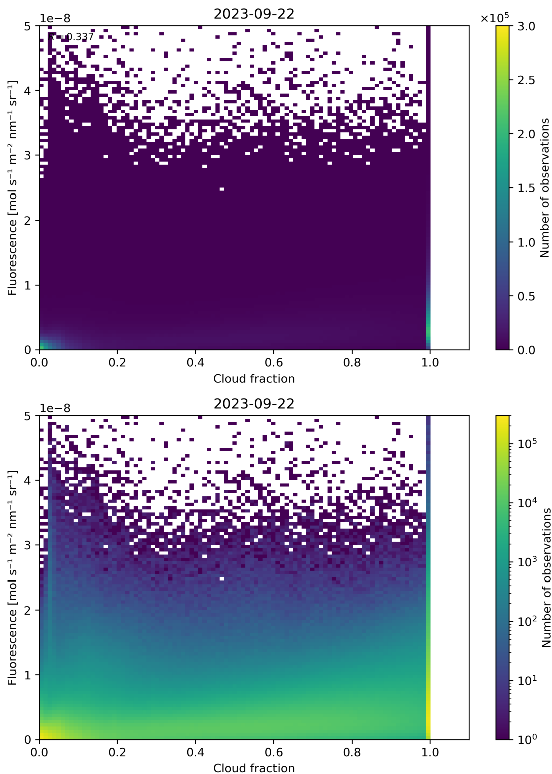
Figure 79: Scatter density plot of “Cloud fraction” against “Fluorescence” for 2023-09-21 to 2023-09-23.
