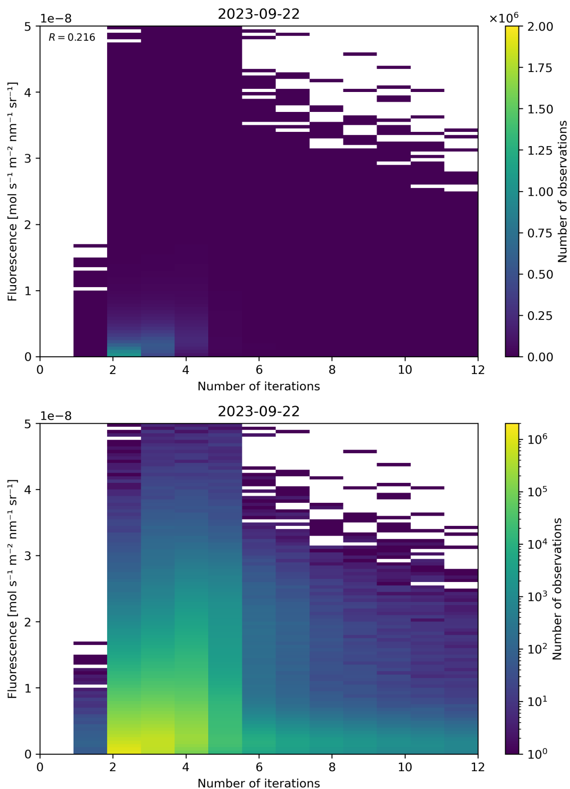
Figure 107: Scatter density plot of “Number of iterations” against “Fluorescence” for 2023-09-21 to 2023-09-23.
