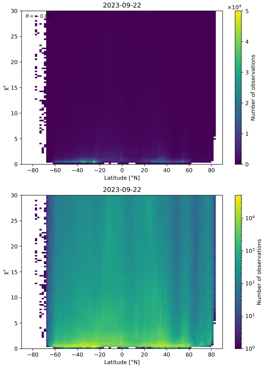
Figure 97: Scatter density plot of “Latitude” against “ \chi^2 ” for 2023-09-21 to 2023-09-23.
