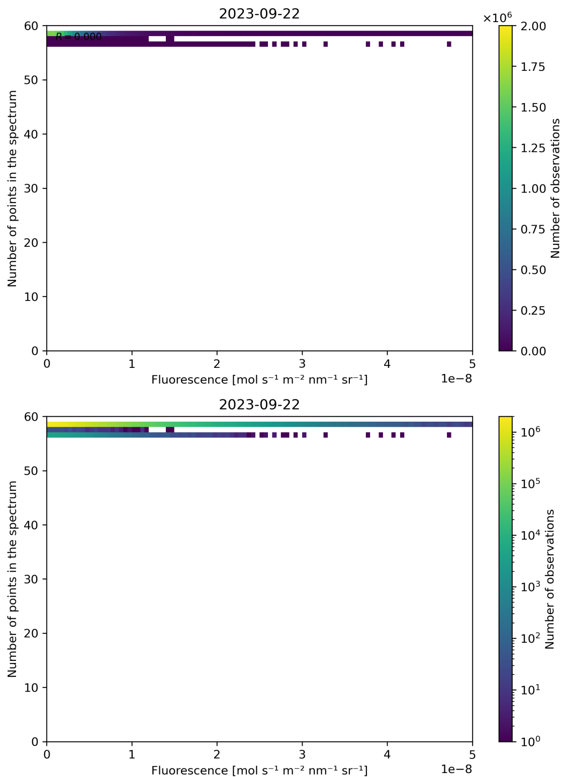
Figure 94: Scatter density plot of “Fluorescence” against “Number of points in the spectrum” for 2023-09-21 to 2023-09-23.
