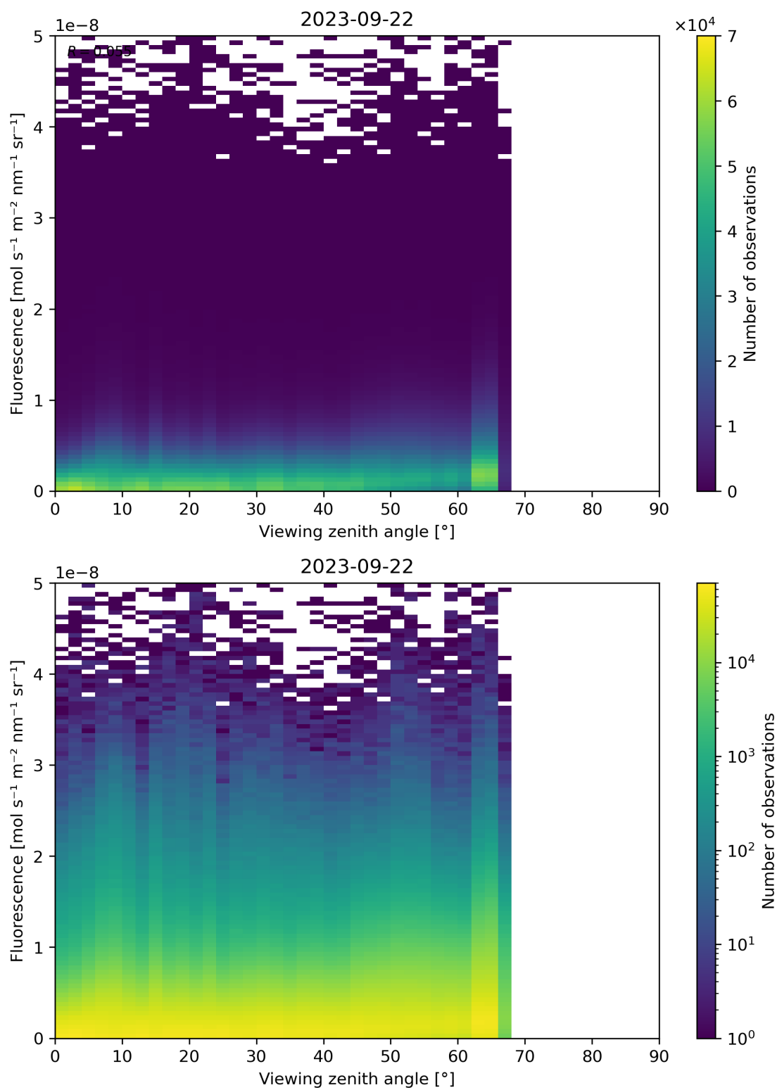
Figure 134: Scatter density plot of “Viewing zenith angle” against “Fluorescence” for 2023-09-21 to 2023-09-23.
