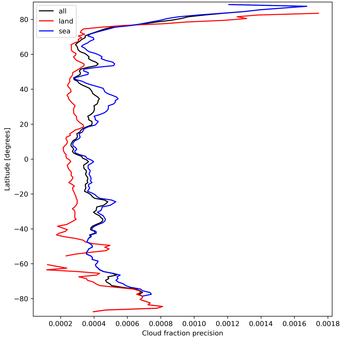
Figure 16: Zonal average of “Cloud fraction precision” for 2023-09-21 to 2023-09-23.
