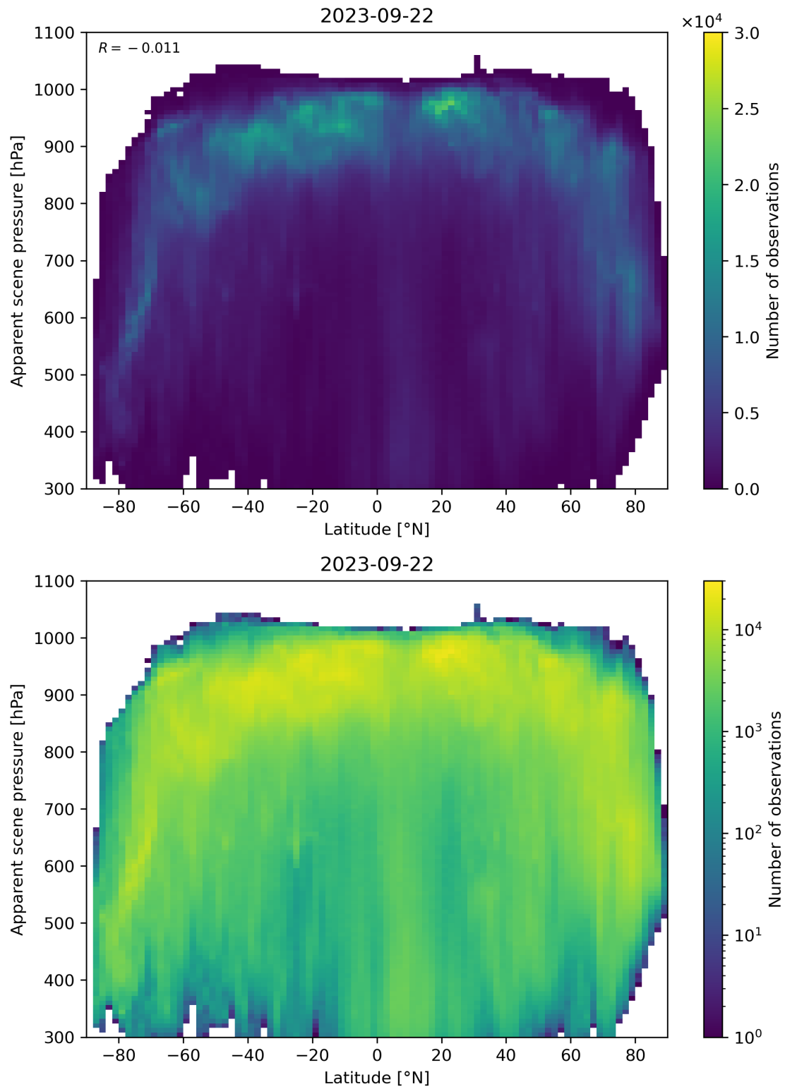
Figure 96: Scatter density plot of “Latitude” against “Apparent scene pressure” for 2023-09-21 to 2023-09-23.
