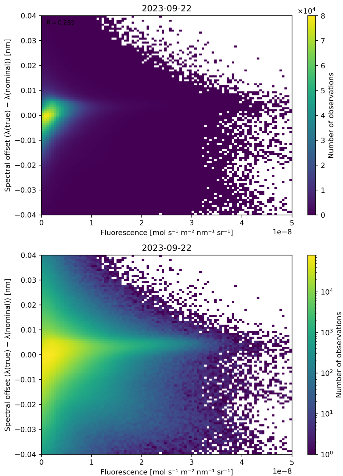
Figure 95: Scatter density plot of “Fluorescence” against “Spectral offset ( \lambda(\text{true}) - \lambda(\text{nominal}) )” for 2023-09-21 to 2023-09-23.
