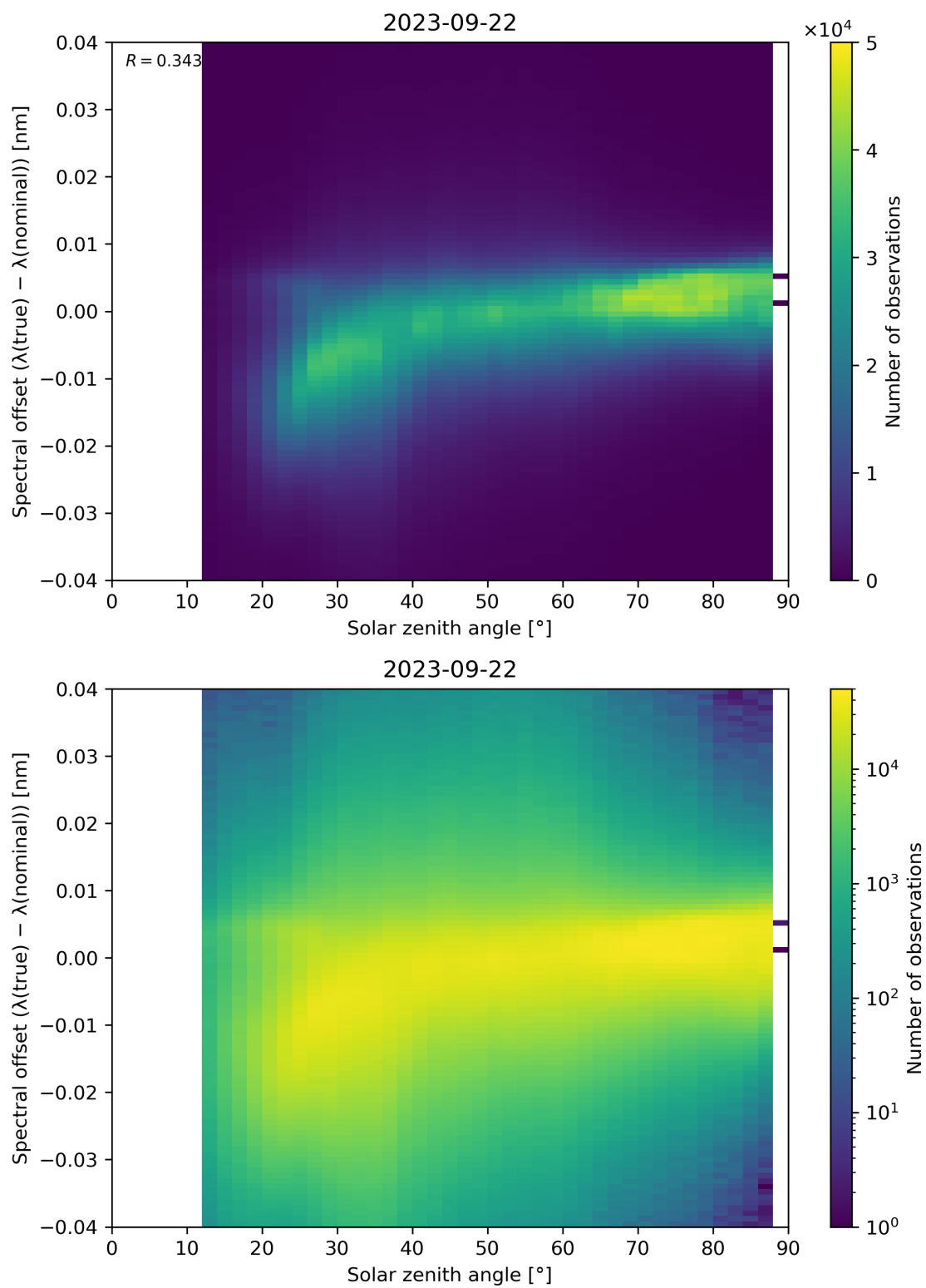
Figure 128: Scatter density plot of “Solar zenith angle” against “Spectral offset ( \lambda(\text{true}) - \lambda(\text{nominal}) )” for 2023-09-21 to 2023-09-23.
