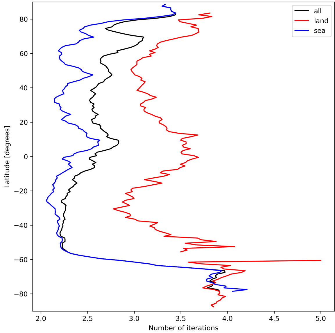
Figure 22: Zonal average of “Number of iterations” for 2023-09-21 to 2023-09-23.
