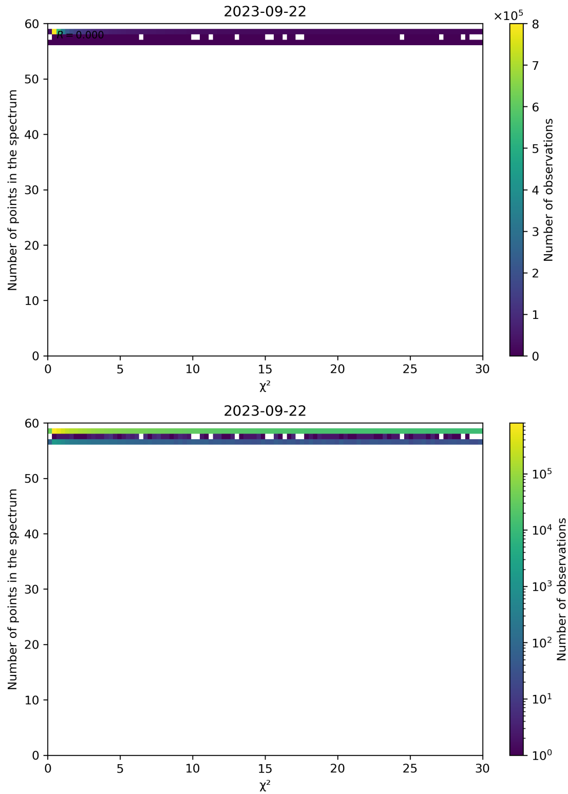
Figure 74: Scatter density plot of “ \chi^2 ” against “Number of points in the spectrum” for 2023-09-21 to 2023-09-23.
