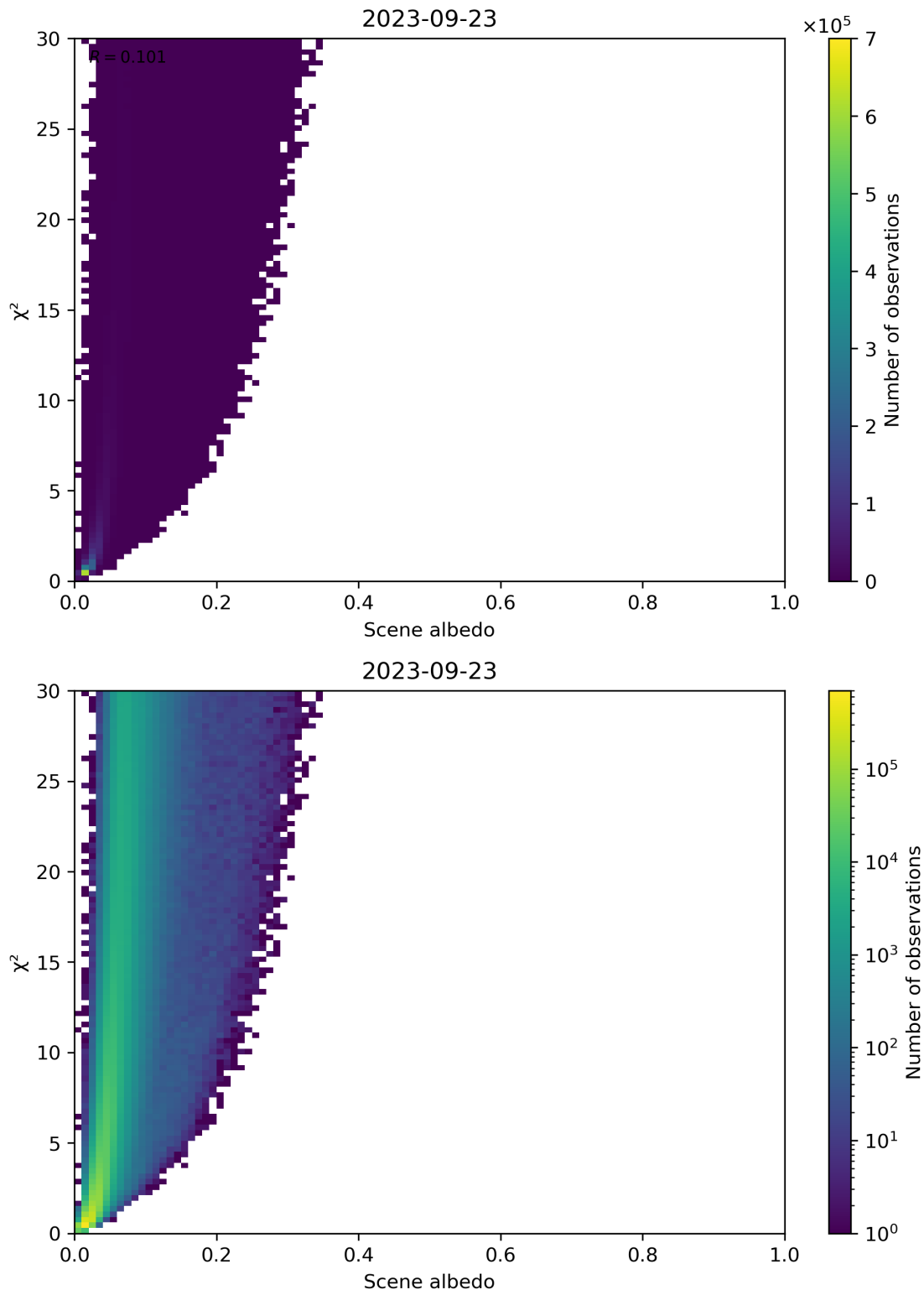
Figure 112: Scatter density plot of “Scene albedo” against “ \chi^2 ” for 2023-09-22 to 2023-09-24.
