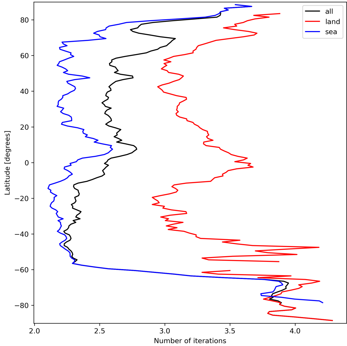
Figure 22: Zonal average of “Number of iterations” for 2023-09-22 to 2023-09-24.
