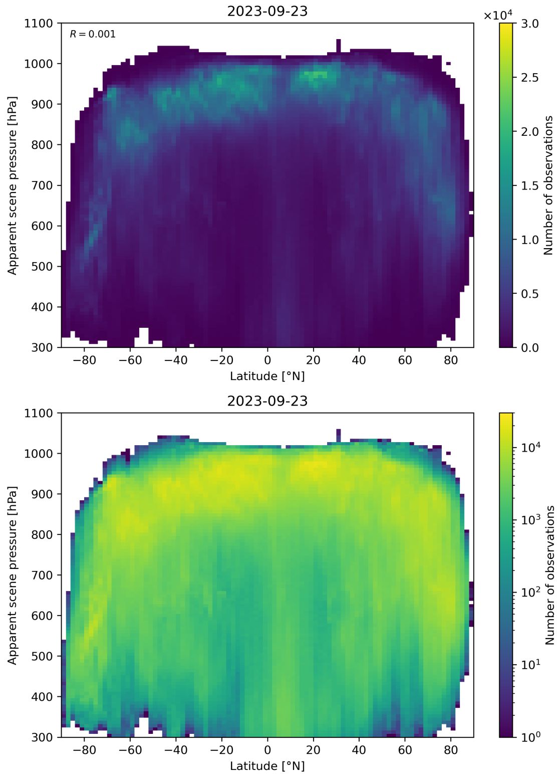
Figure 96: Scatter density plot of “Latitude” against “Apparent scene pressure” for 2023-09-22 to 2023-09-24.
