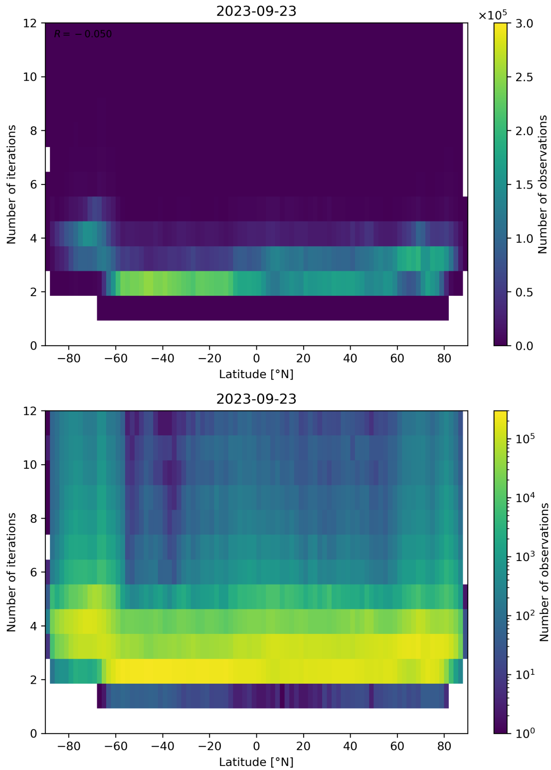
Figure 102: Scatter density plot of “Latitude” against “Number of iterations” for 2023-09-22 to 2023-09-24.
