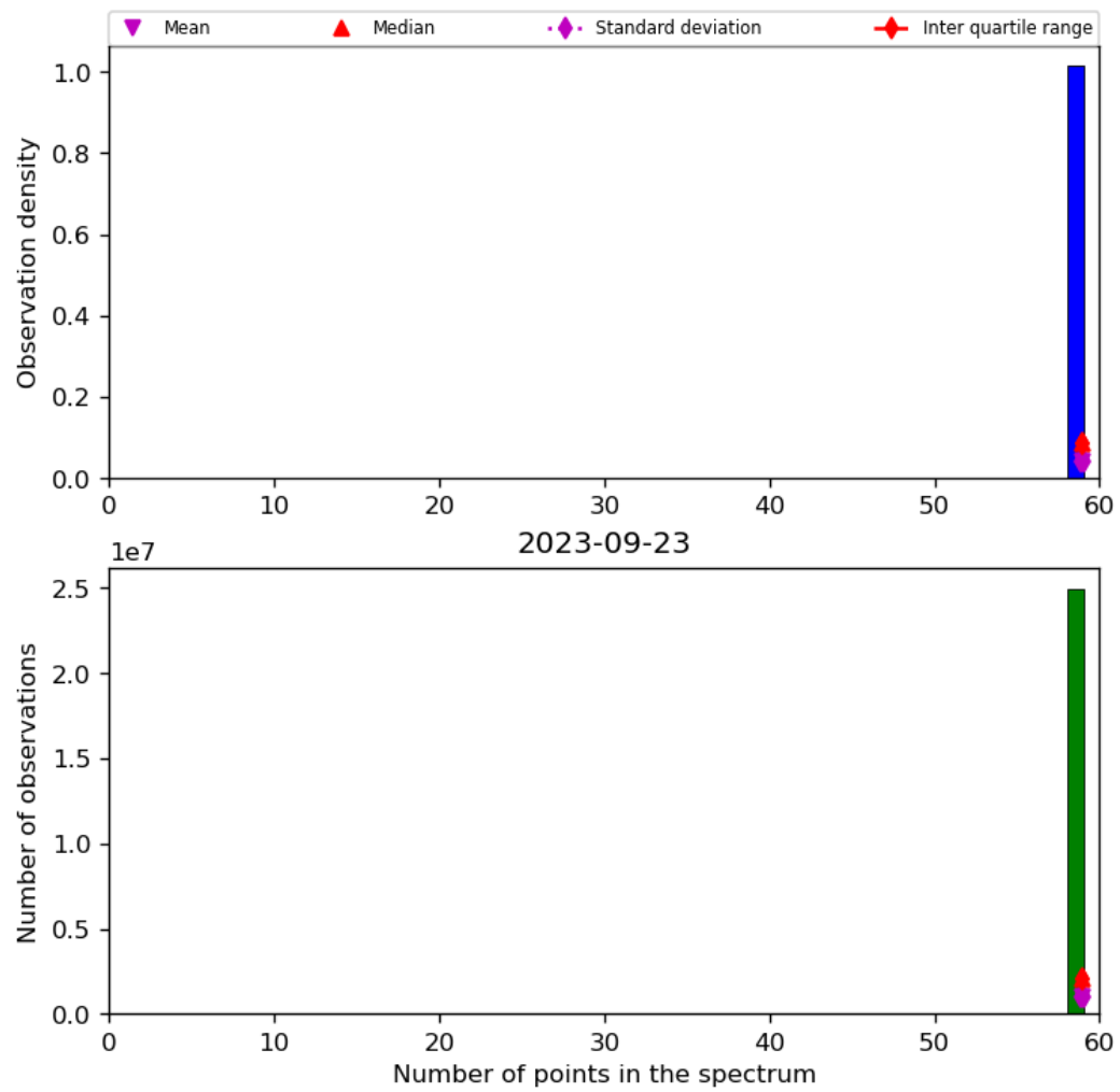
Figure 44: Histogram of “Number of points in the spectrum” for 2023-09-22 to 2023-09-24
