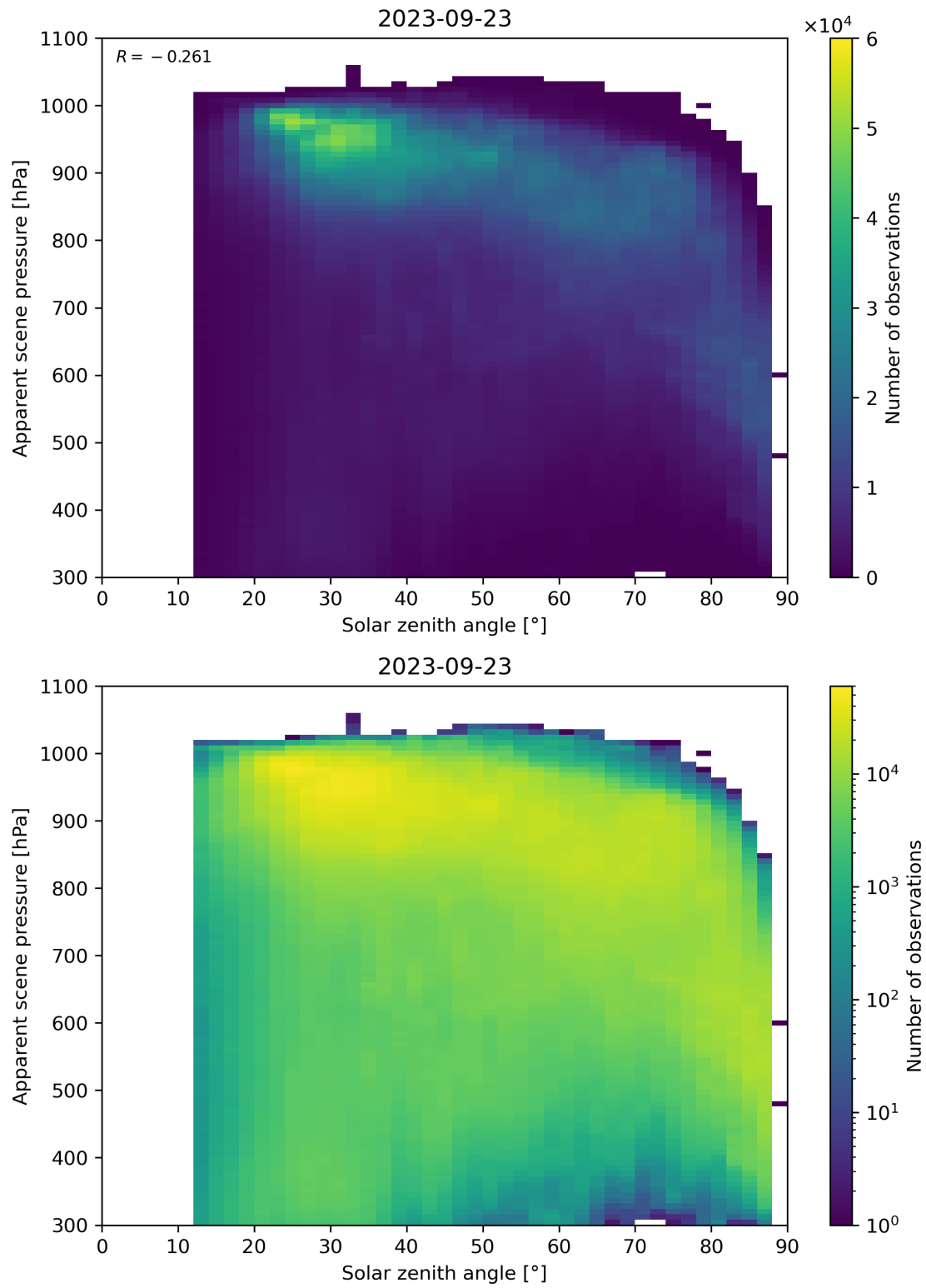
Figure 118: Scatter density plot of “Solar zenith angle” against “Apparent scene pressure” for 2023-09-22 to 2023-09-24.
