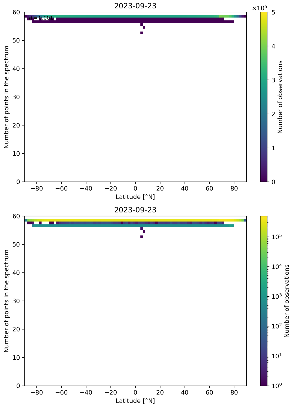
Figure 103: Scatter density plot of “Latitude” against “Number of points in the spectrum” for 2023-09-22 to 2023-09-24.
