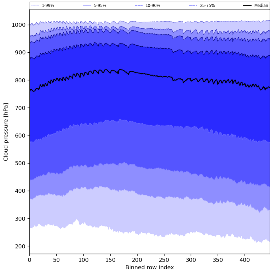
Figure 47: Along track statistics of “Cloud pressure” for 2023-09-22 to 2023-09-24
