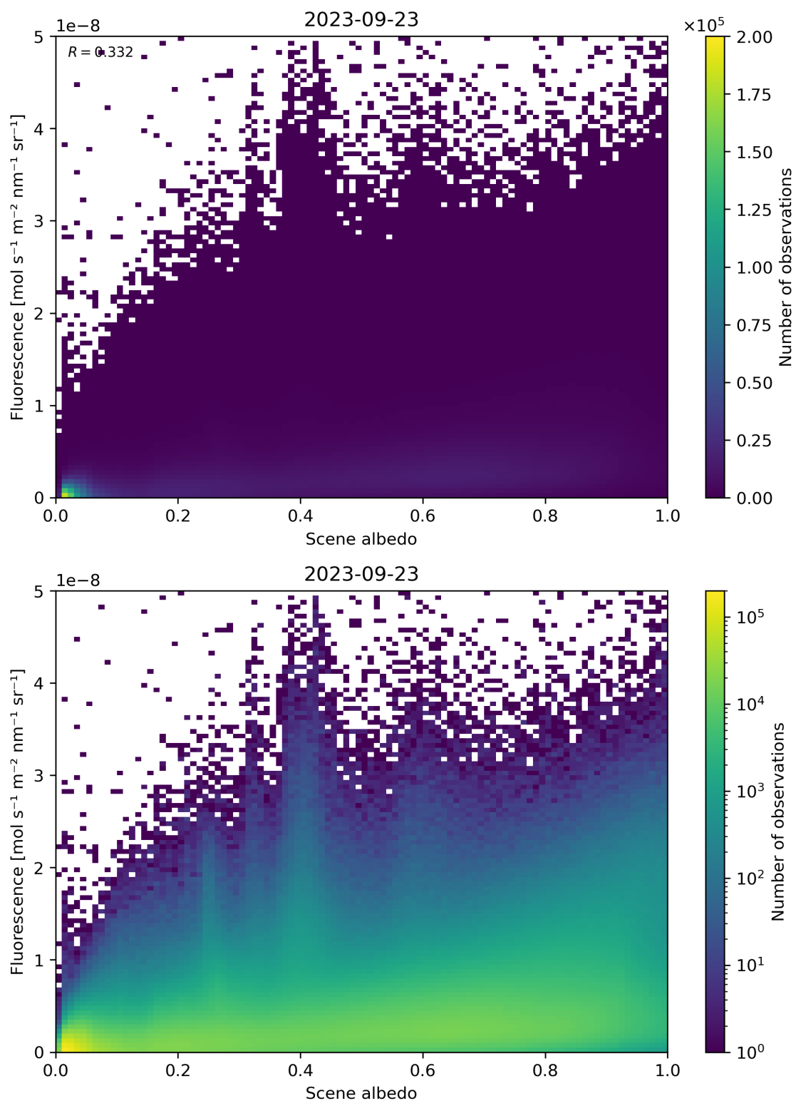
Figure 114: Scatter density plot of “Scene albedo” against “Fluorescence” for 2023-09-22 to 2023-09-24.
