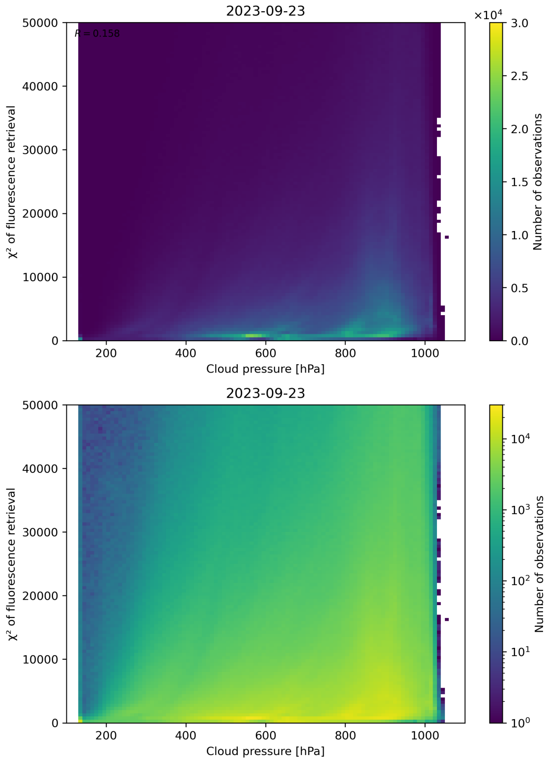
Figure 86: Scatter density plot of “Cloud pressure” against “ \chi^2 of fluorescence retrieval” for 2023-09-22 to 2023-09-24.
