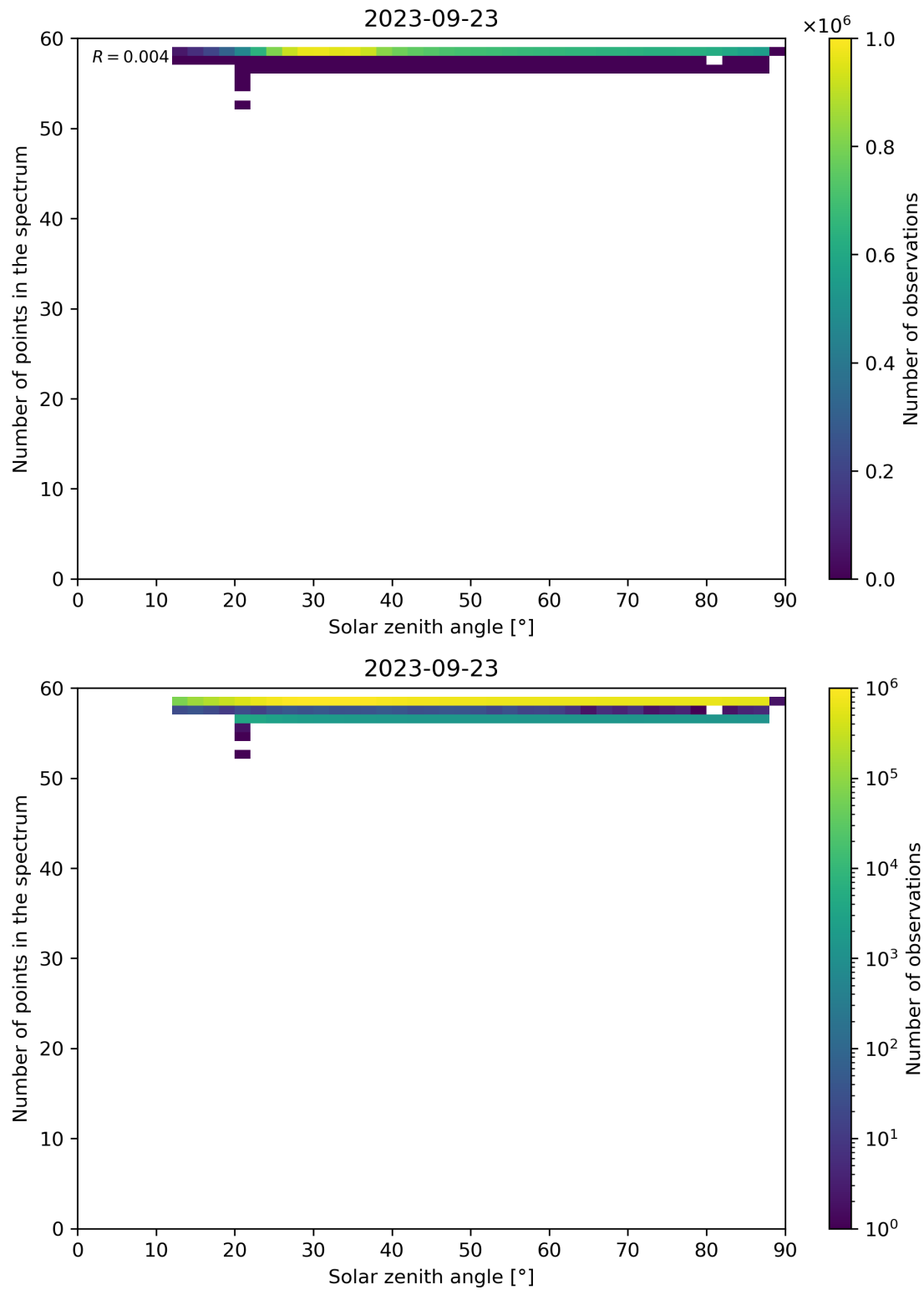
Figure 126: Scatter density plot of “Solar zenith angle” against “Number of points in the spectrum” for 2023-09-22 to 2023-09-24.
