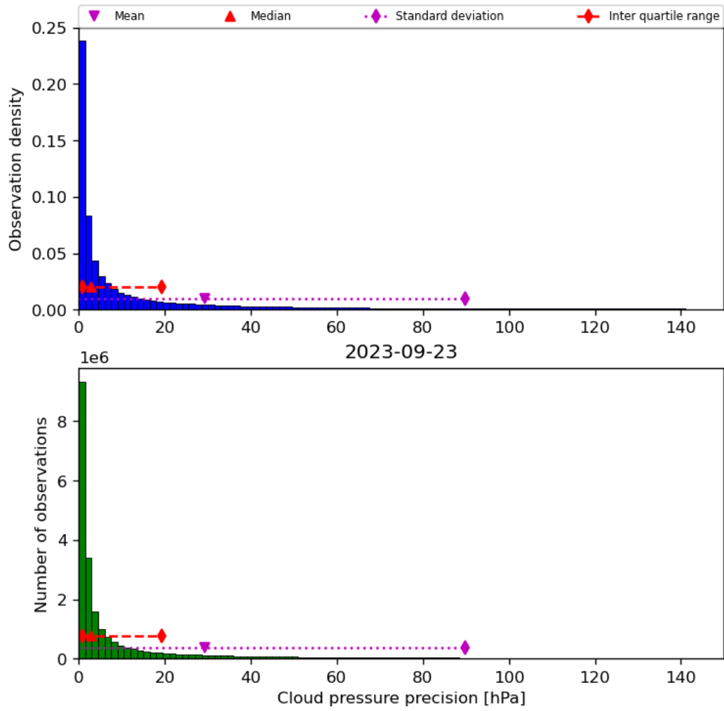
Figure 31: Histogram of “Cloud pressure precision” for 2023-09-22 to 2023-09-24
