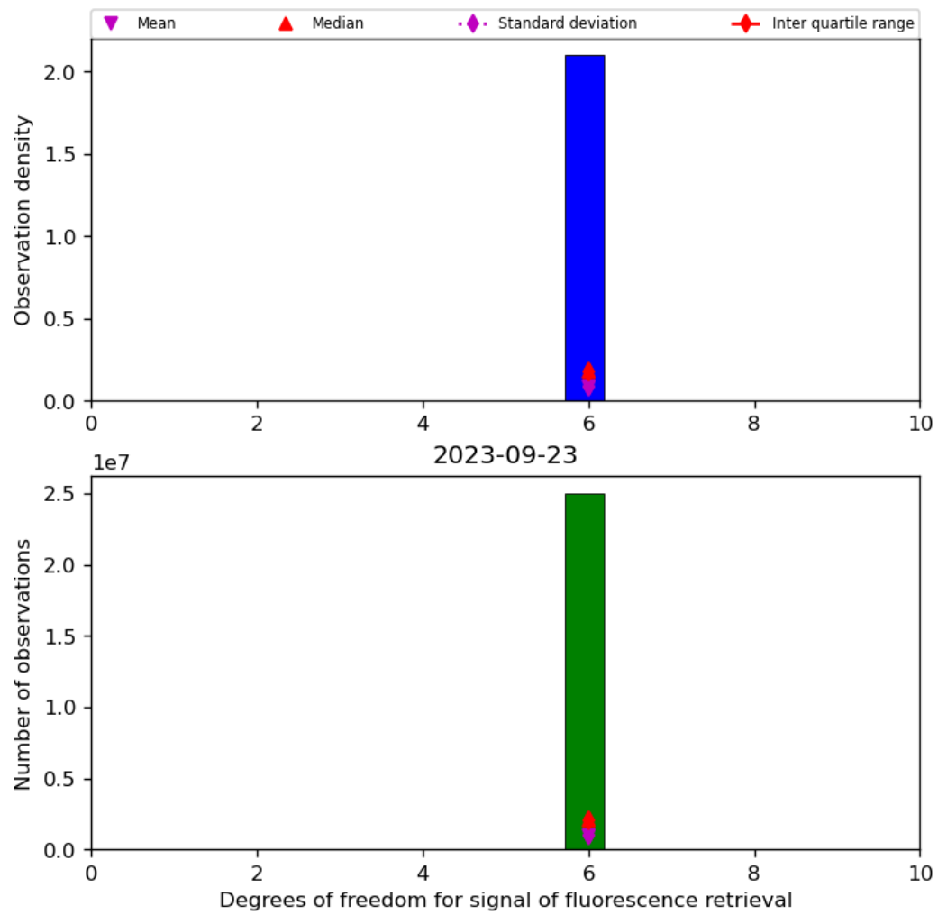
Figure 43: Histogram of “Degrees of freedom for signal of fluorescence retrieval” for 2023-09-22 to 2023-09-24
