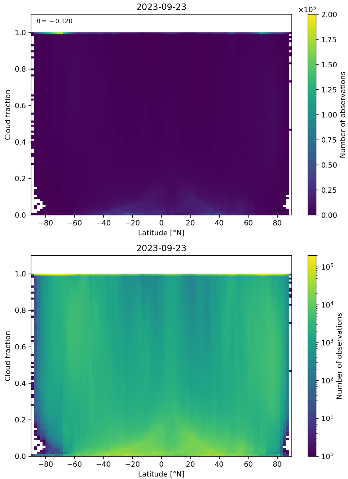
Figure 99: Scatter density plot of “Latitude” against “Cloud fraction” for 2023-09-22 to 2023-09-24.
