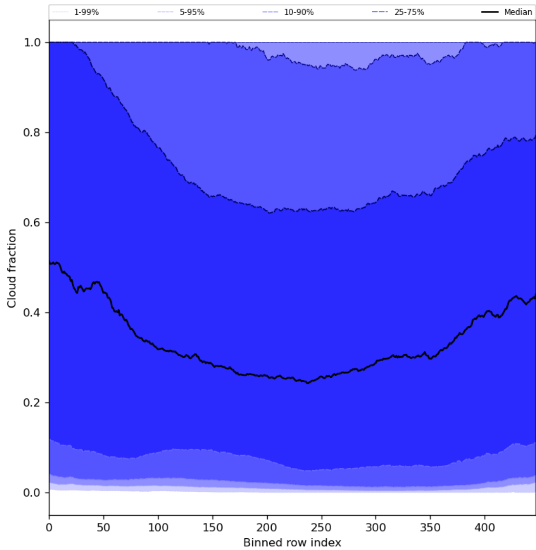
Figure 49: Along track statistics of “Cloud fraction” for 2023-09-22 to 2023-09-24
