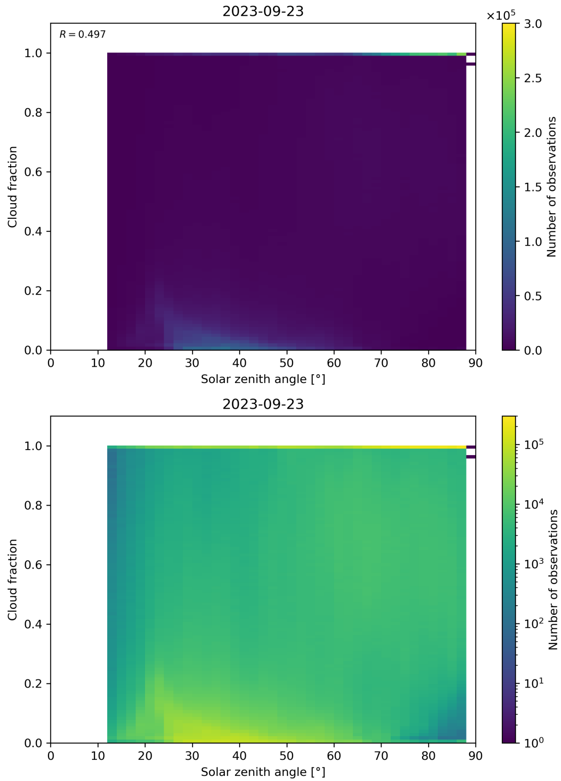
Figure 121: Scatter density plot of “Solar zenith angle” against “Cloud fraction” for 2023-09-22 to 2023-09-24.
