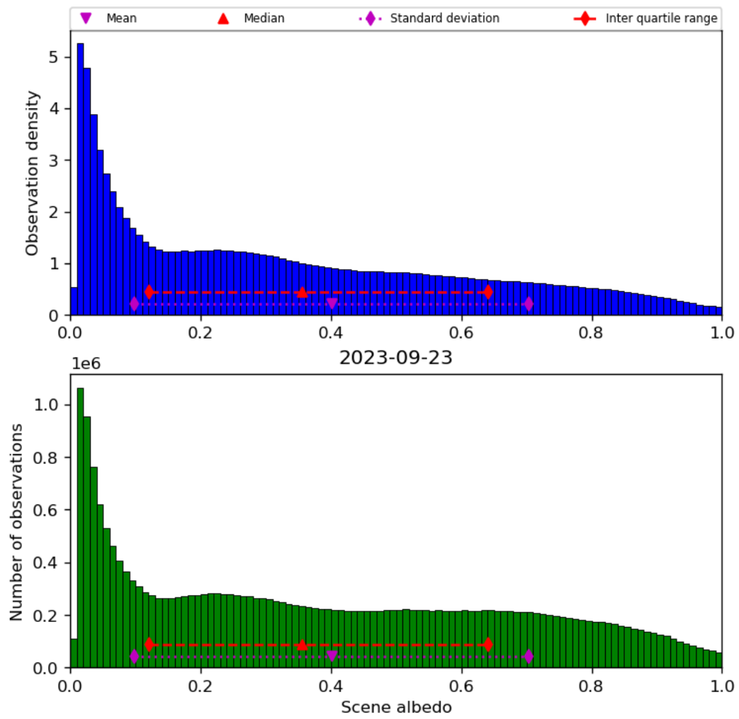
Figure 34: Histogram of “Scene albedo” for 2023-09-22 to 2023-09-24
