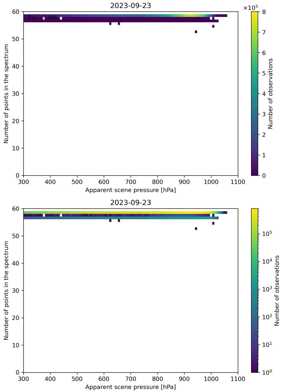
Figure 67: Scatter density plot of “Apparent scene pressure” against “Number of points in the spectrum” for 2023-09-22 to 2023-09-24.
