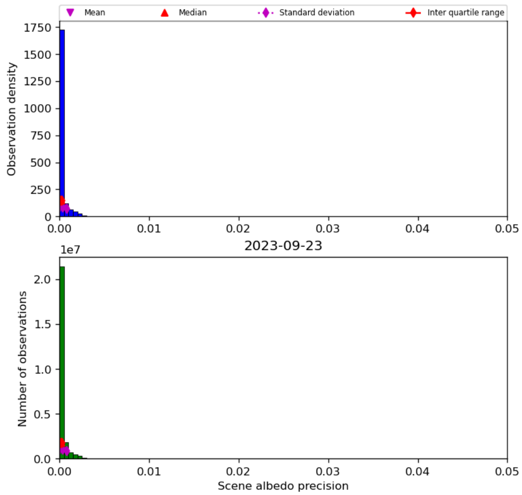
Figure 35: Histogram of “Scene albedo precision” for 2023-09-22 to 2023-09-24
