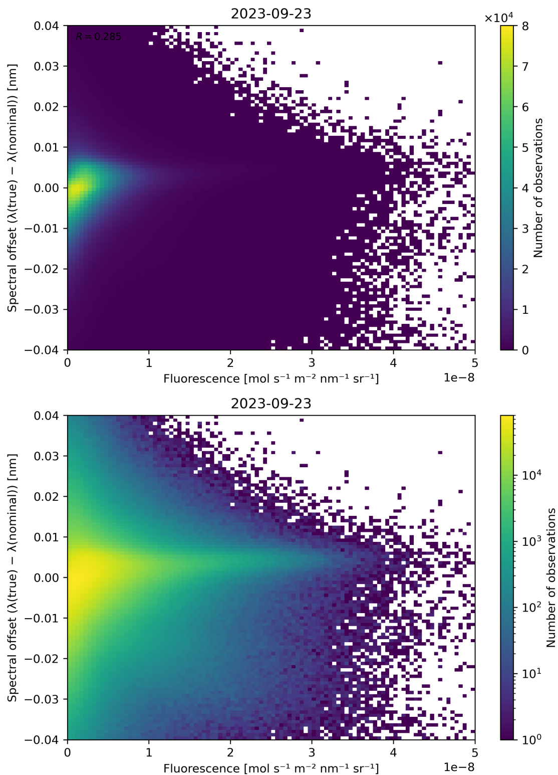
Figure 95: Scatter density plot of “Fluorescence” against “Spectral offset ( \lambda(\text{true}) - \lambda(\text{nominal}) )” for 2023-09-22 to 2023-09-24.
