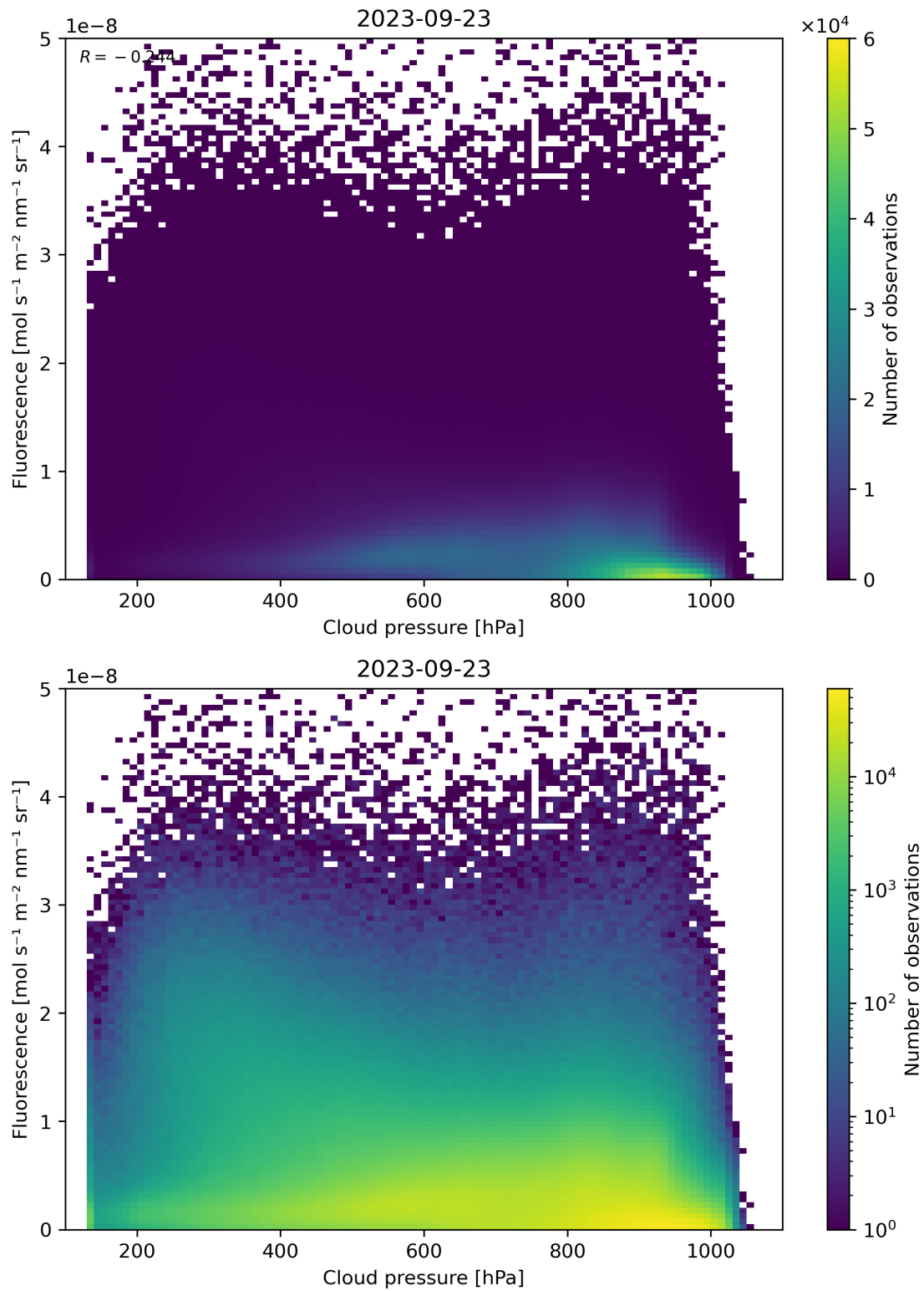
Figure 88: Scatter density plot of “Cloud pressure” against “Fluorescence” for 2023-09-22 to 2023-09-24.
