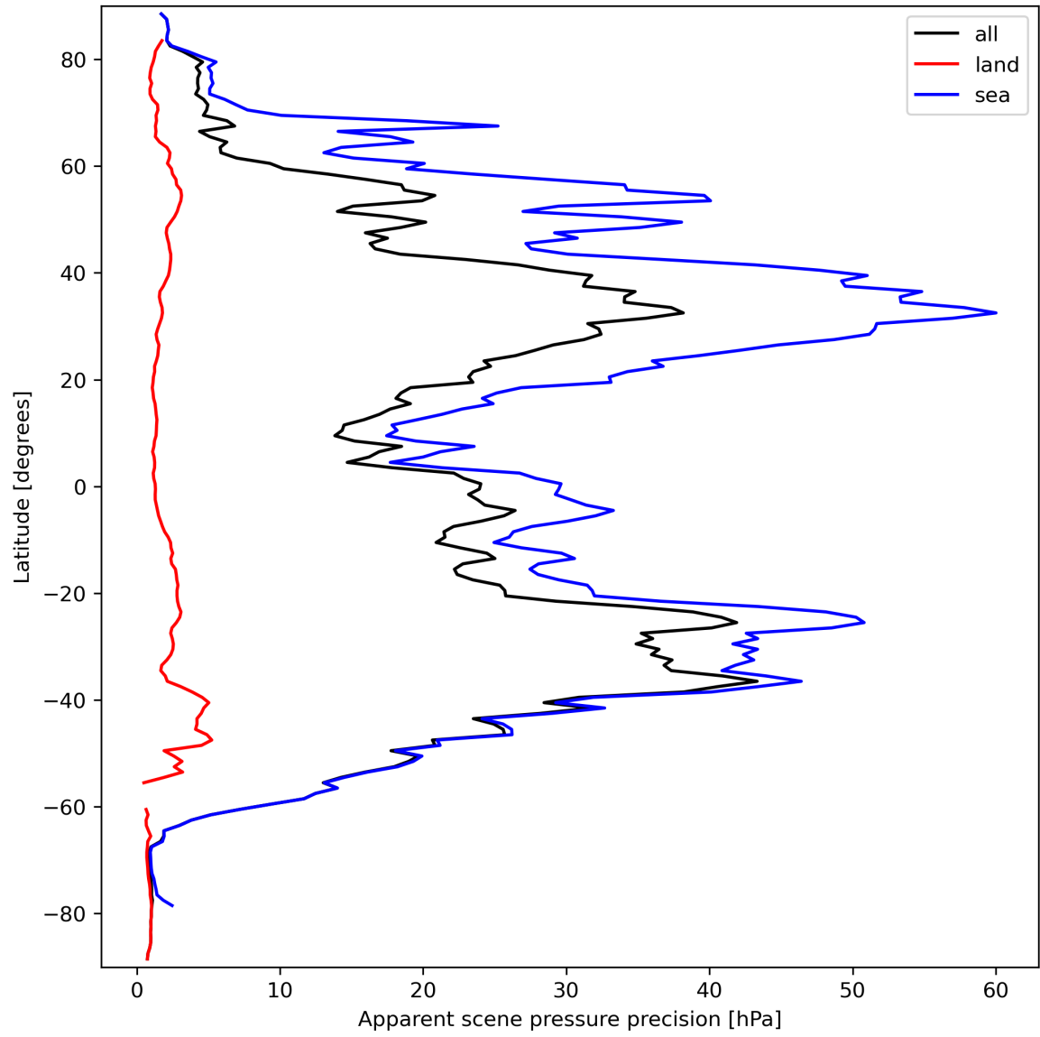
Figure 20: Zonal average of “Apparent scene pressure precision” for 2023-09-22 to 2023-09-24.
