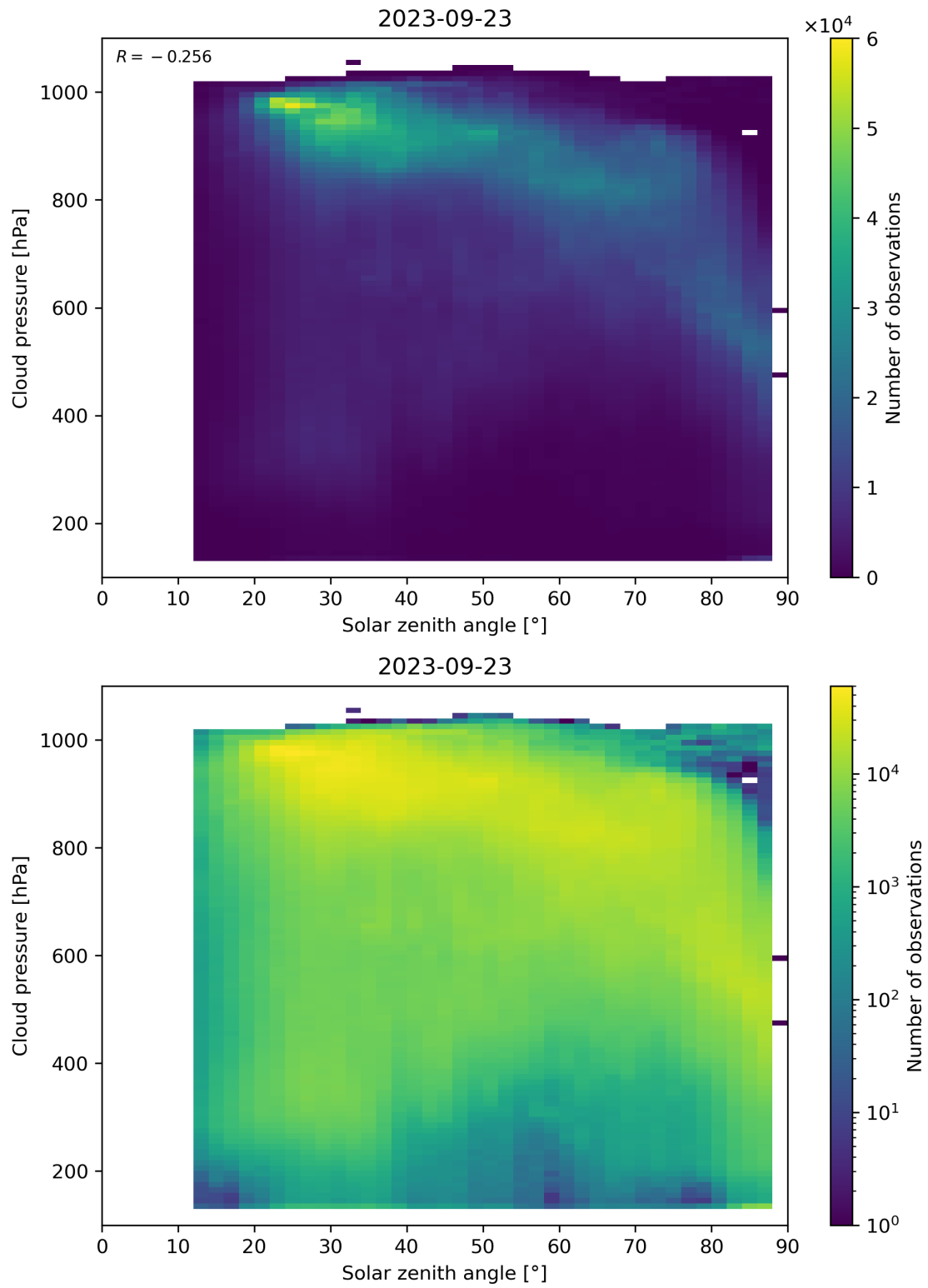
Figure 122: Scatter density plot of “Solar zenith angle” against “Cloud pressure” for 2023-09-22 to 2023-09-24.
