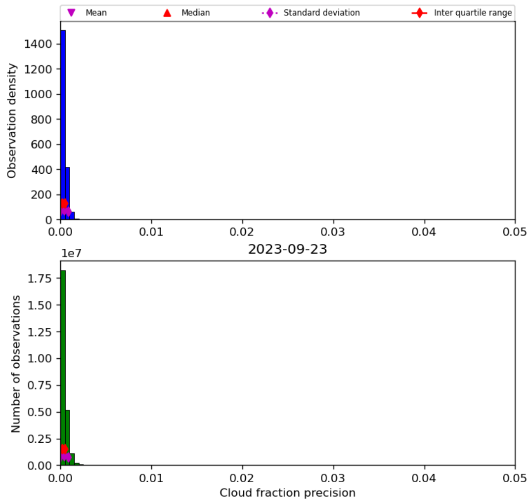
Figure 33: Histogram of “Cloud fraction precision” for 2023-09-22 to 2023-09-24
