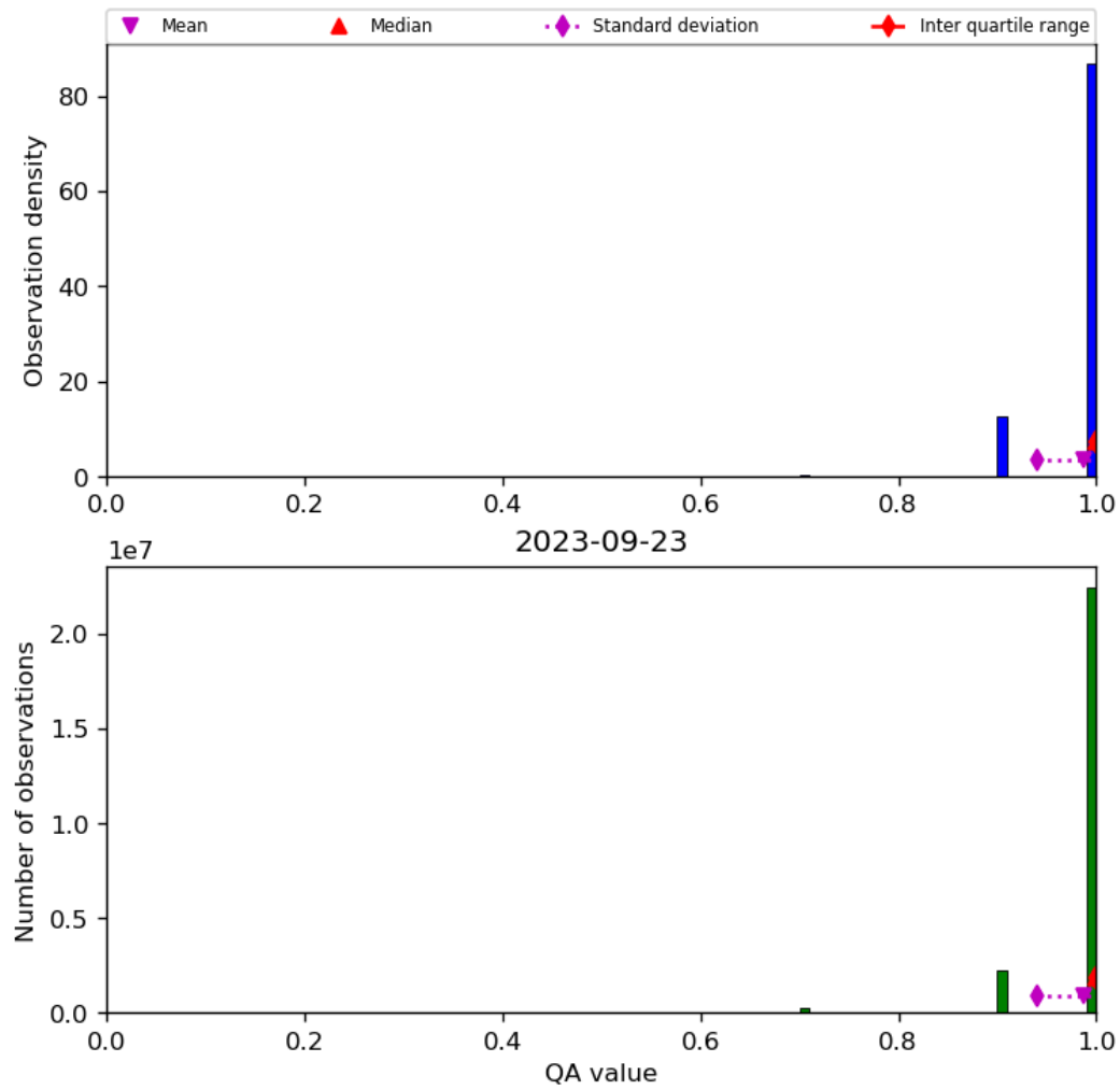
Figure 29: Histogram of “QA value” for 2023-09-22 to 2023-09-24
