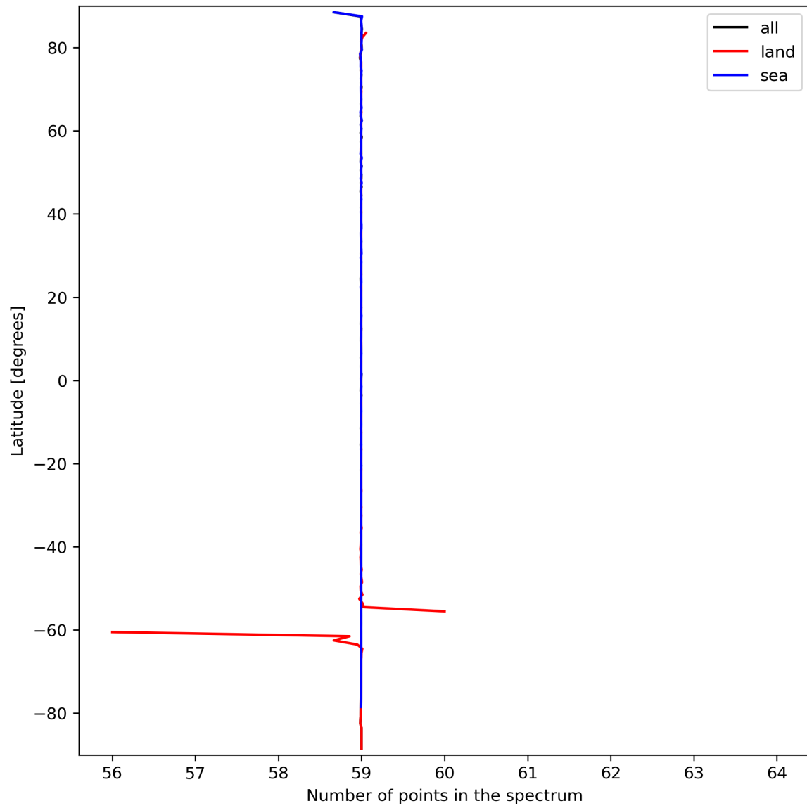
Figure 27: Zonal average of “Number of points in the spectrum” for 2023-09-22 to 2023-09-24.
