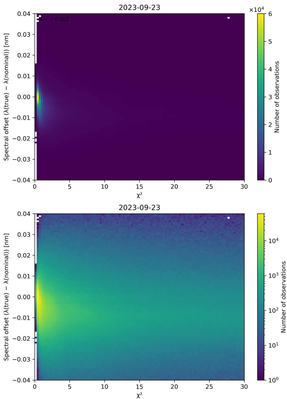
Figure 75: Scatter density plot of “ \chi^2 ” against “Spectral offset ( \lambda(\text{true}) - \lambda(\text{nominal}) )” for 2023-09-22 to 2023-09-24.
