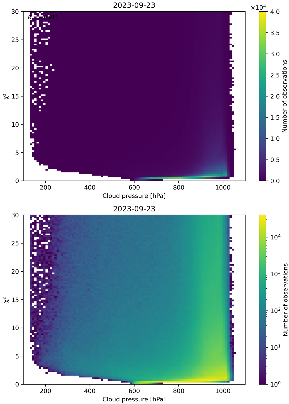
Figure 85: Scatter density plot of “Cloud pressure” against “ \chi^2 ” for 2023-09-22 to 2023-09-24.
