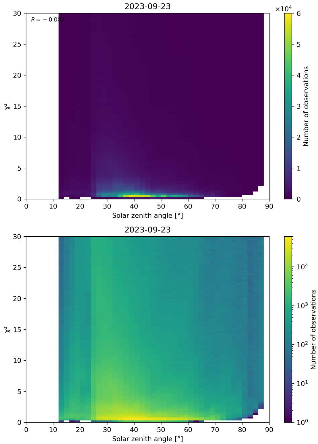
Figure 119: Scatter density plot of “Solar zenith angle” against “ \chi^2 ” for 2023-09-22 to 2023-09-24.
