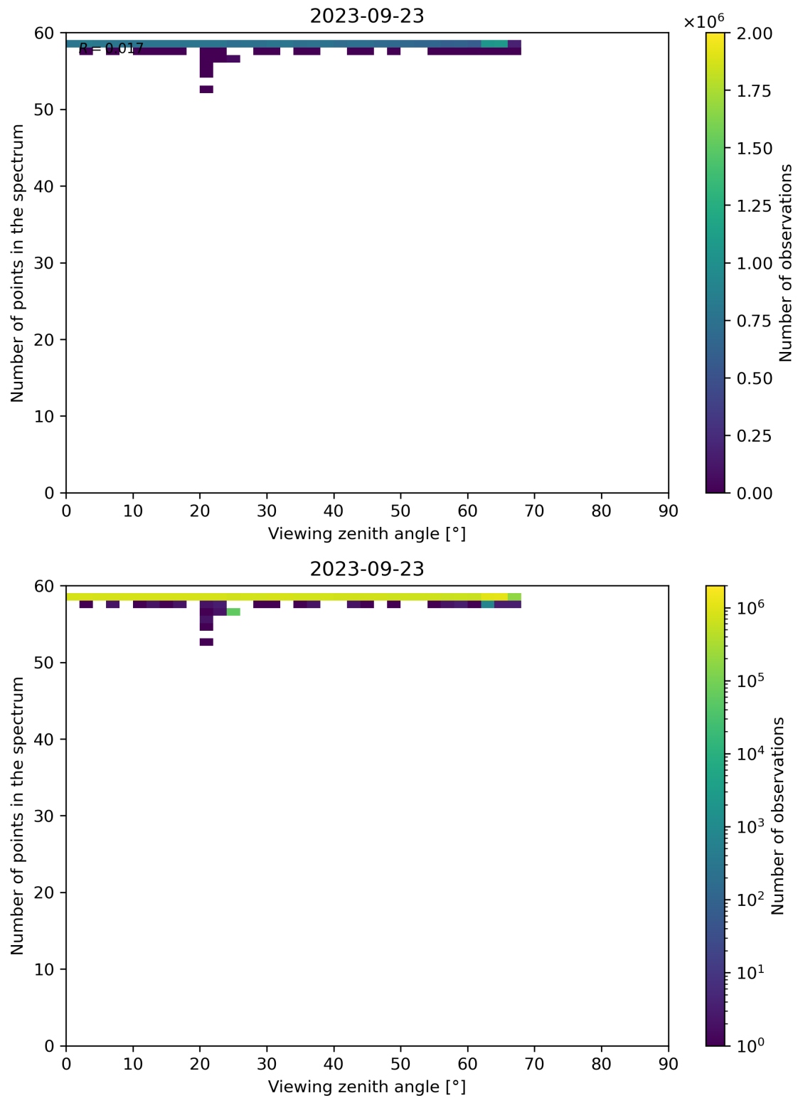
Figure 137: Scatter density plot of “Viewing zenith angle” against “Number of points in the spectrum” for 2023-09-22 to 2023-09-24.
