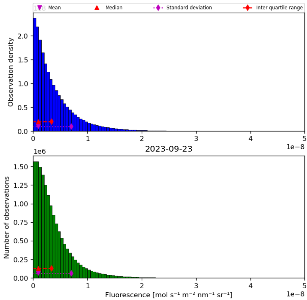
Figure 40: Histogram of “Fluorescence” for 2023-09-22 to 2023-09-24
