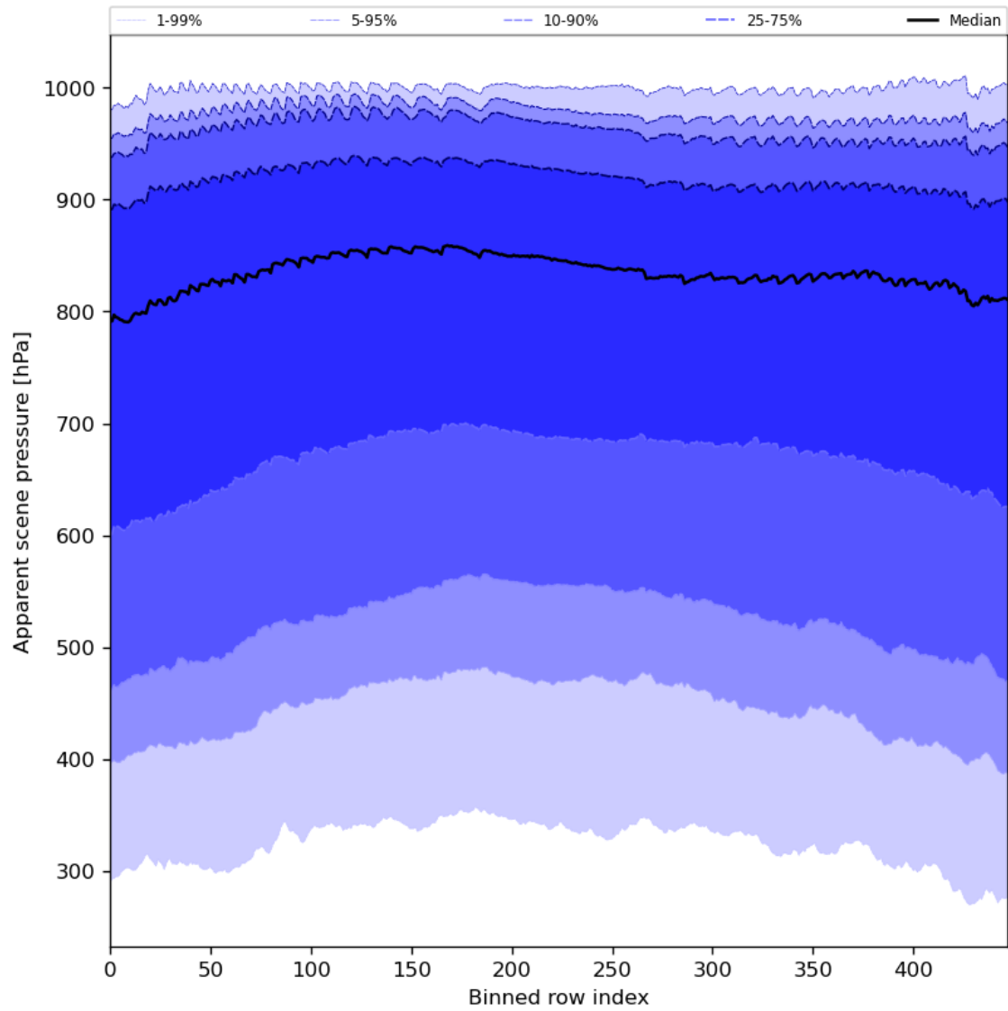
Figure 53: Along track statistics of “Apparent scene pressure” for 2023-09-22 to 2023-09-24
