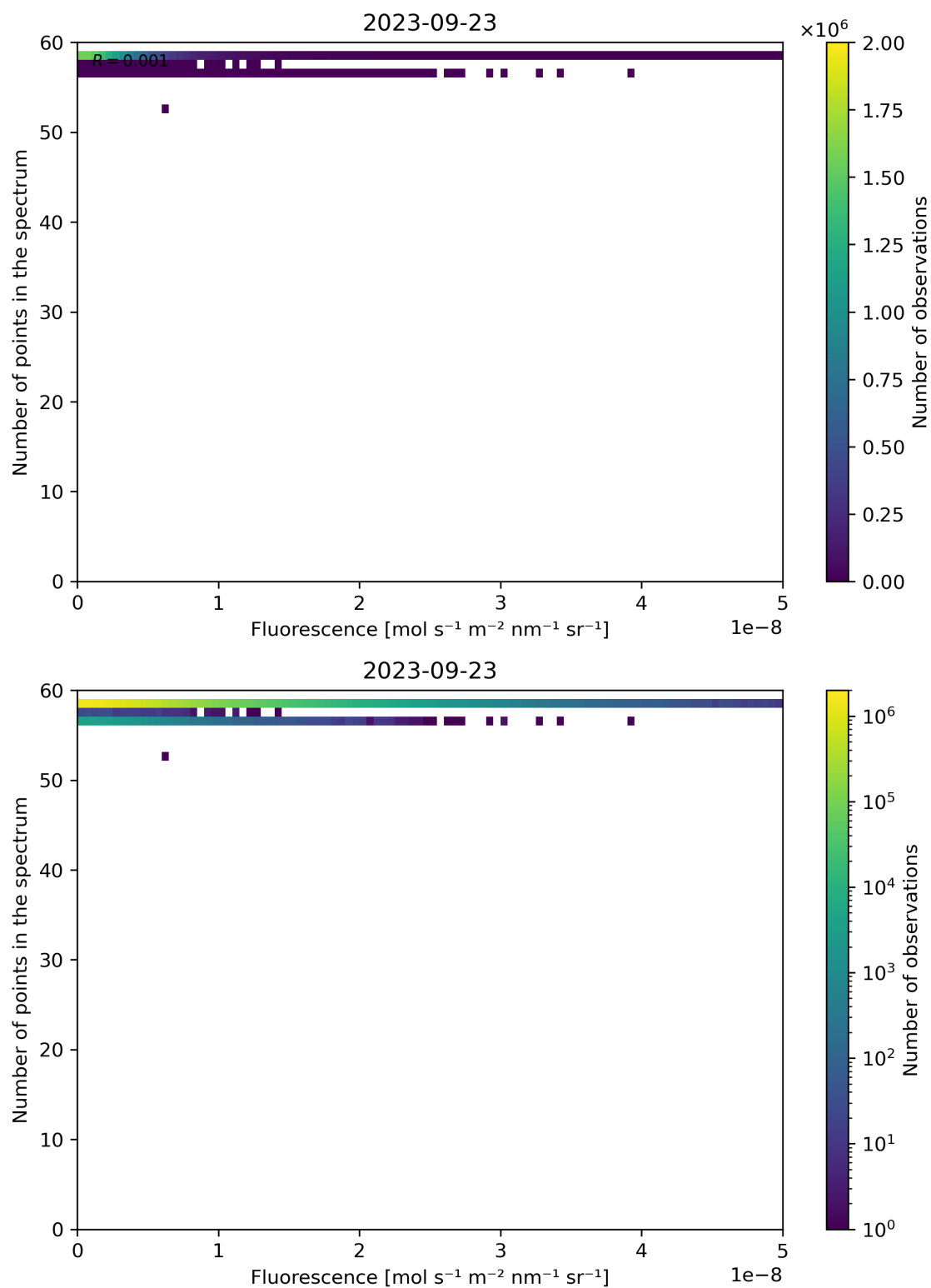
Figure 94: Scatter density plot of “Fluorescence” against “Number of points in the spectrum” for 2023-09-22 to 2023-09-24.
