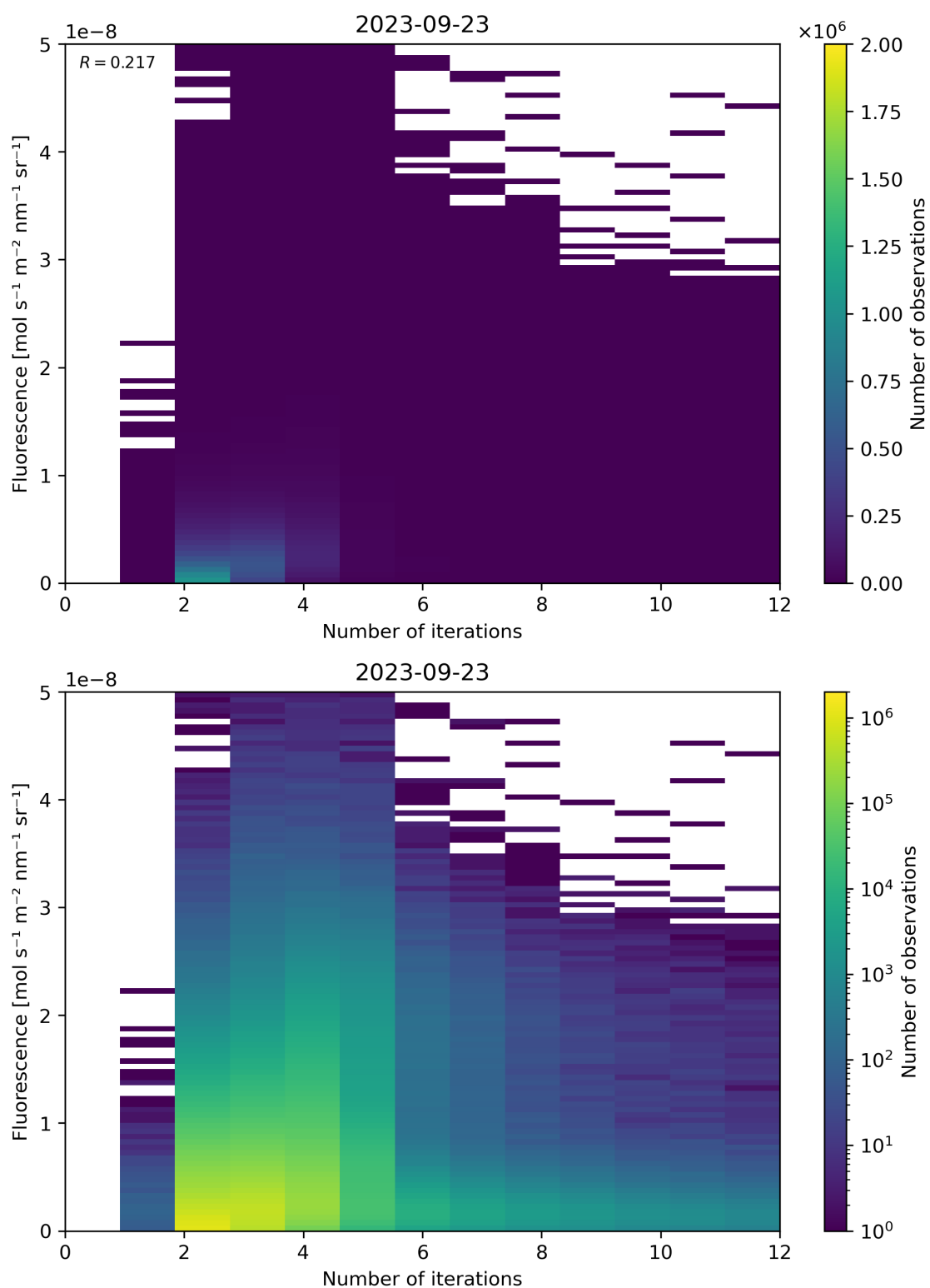
Figure 107: Scatter density plot of “Number of iterations” against “Fluorescence” for 2023-09-22 to 2023-09-24.
