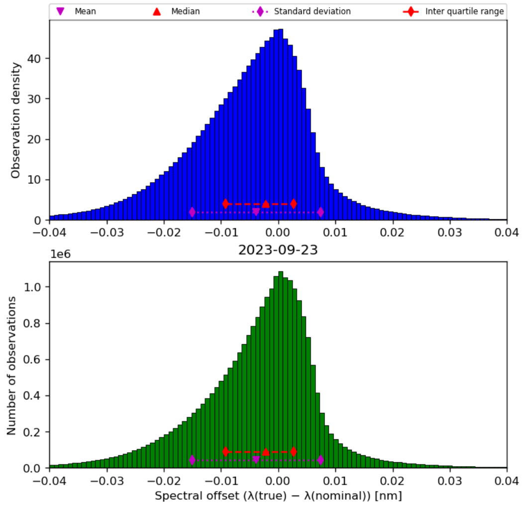
Figure 45: Histogram of “Spectral offset ( \lambda(\text{true}) - \lambda(\text{nominal}) )” for 2023-09-22 to 2023-09-24
