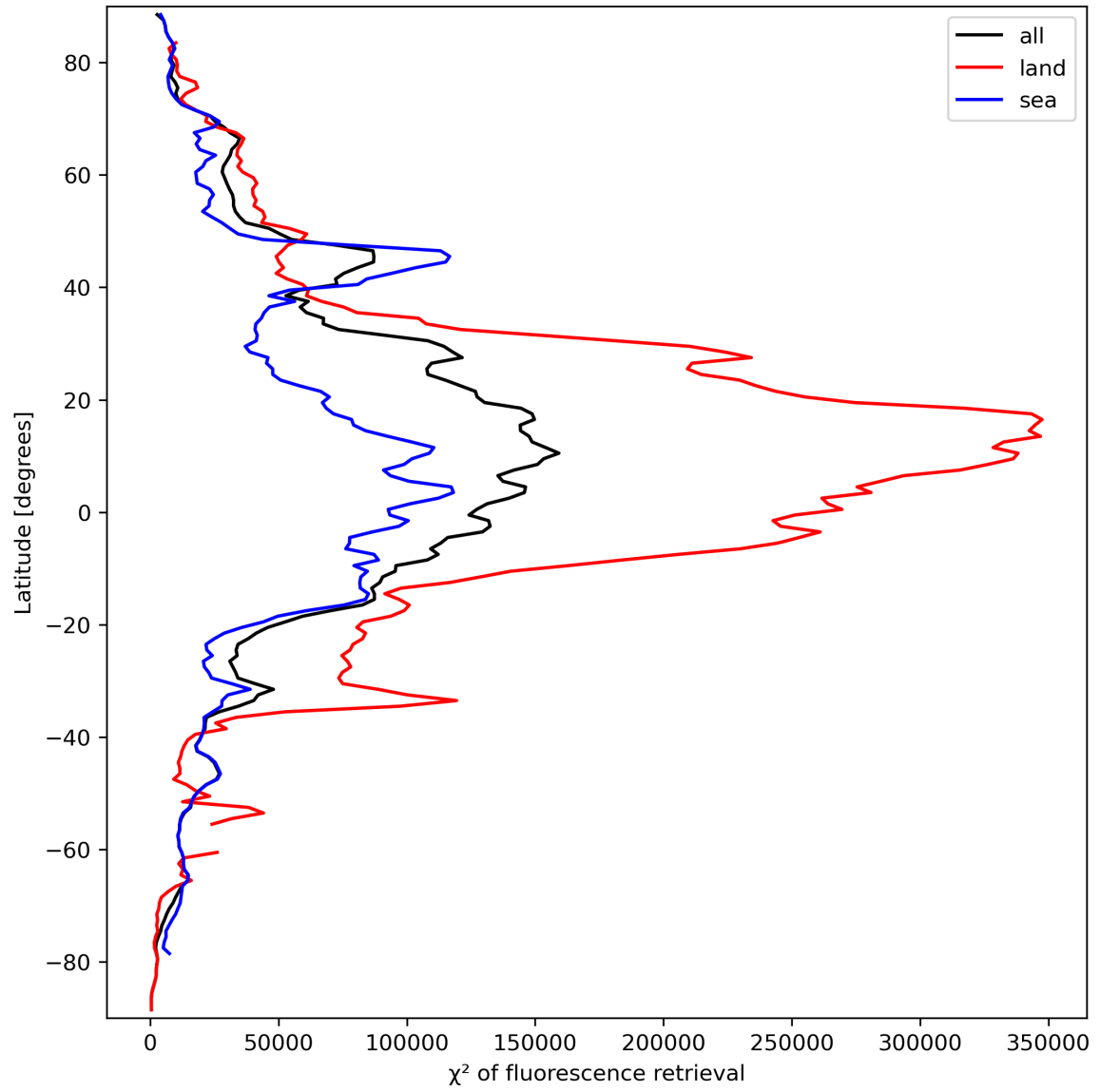
Figure 25: Zonal average of “ \chi^2 of fluorescence retrieval” for 2023-09-22 to 2023-09-24.
