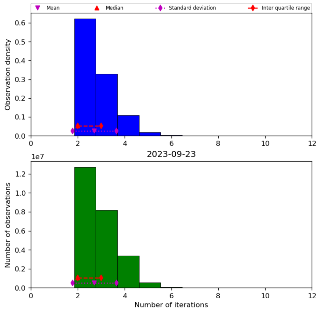
Figure 39: Histogram of “Number of iterations” for 2023-09-22 to 2023-09-24
