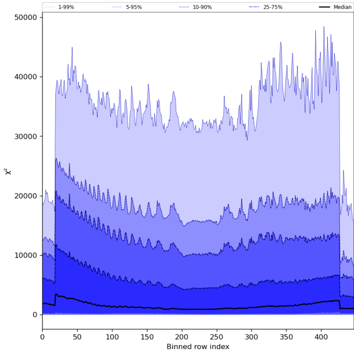
Figure 55: Along track statistics of “ \chi^2 ” for 2023-09-22 to 2023-09-24
