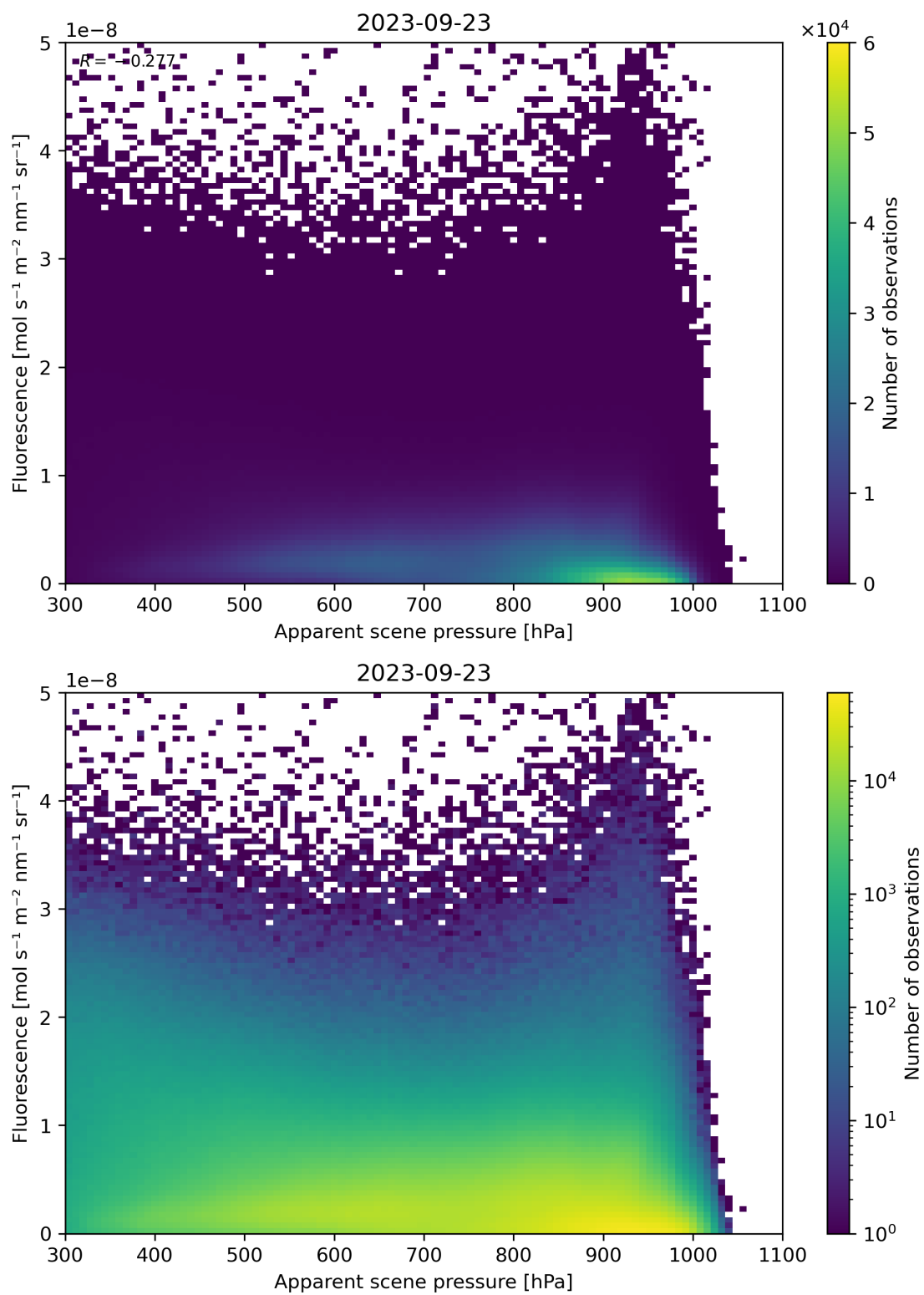
Figure 65: Scatter density plot of “Apparent scene pressure” against “Fluorescence” for 2023-09-22 to 2023-09-24.
