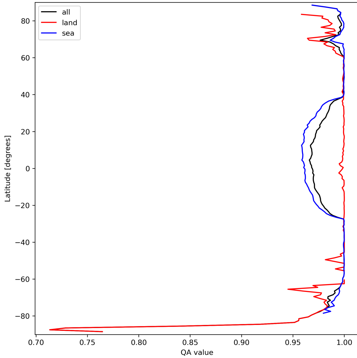
Figure 12: Zonal average of “QA value” for 2023-09-22 to 2023-09-24.
