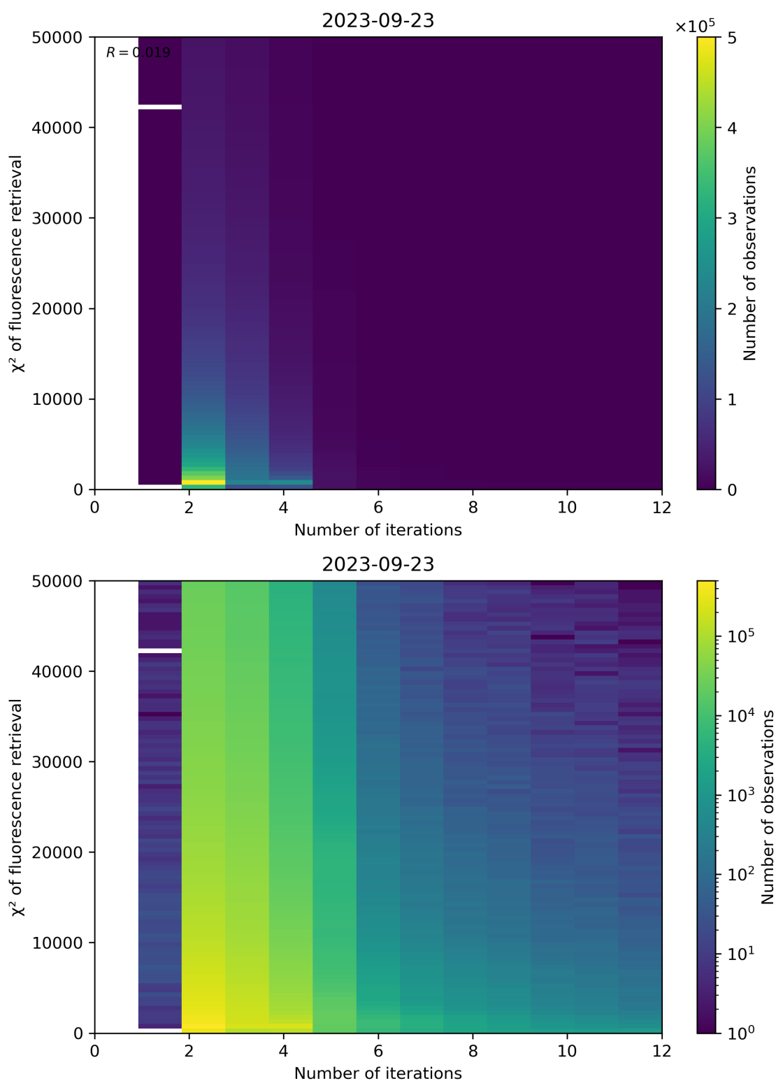
Figure 106: Scatter density plot of “Number of iterations” against “ \chi^2 of fluorescence retrieval” for 2023-09-22 to 2023-09-24.
