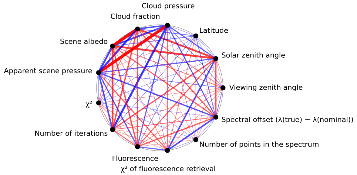
Figure 1: Map of correlation graph for 2023-09-22 to 2023-09-24.
