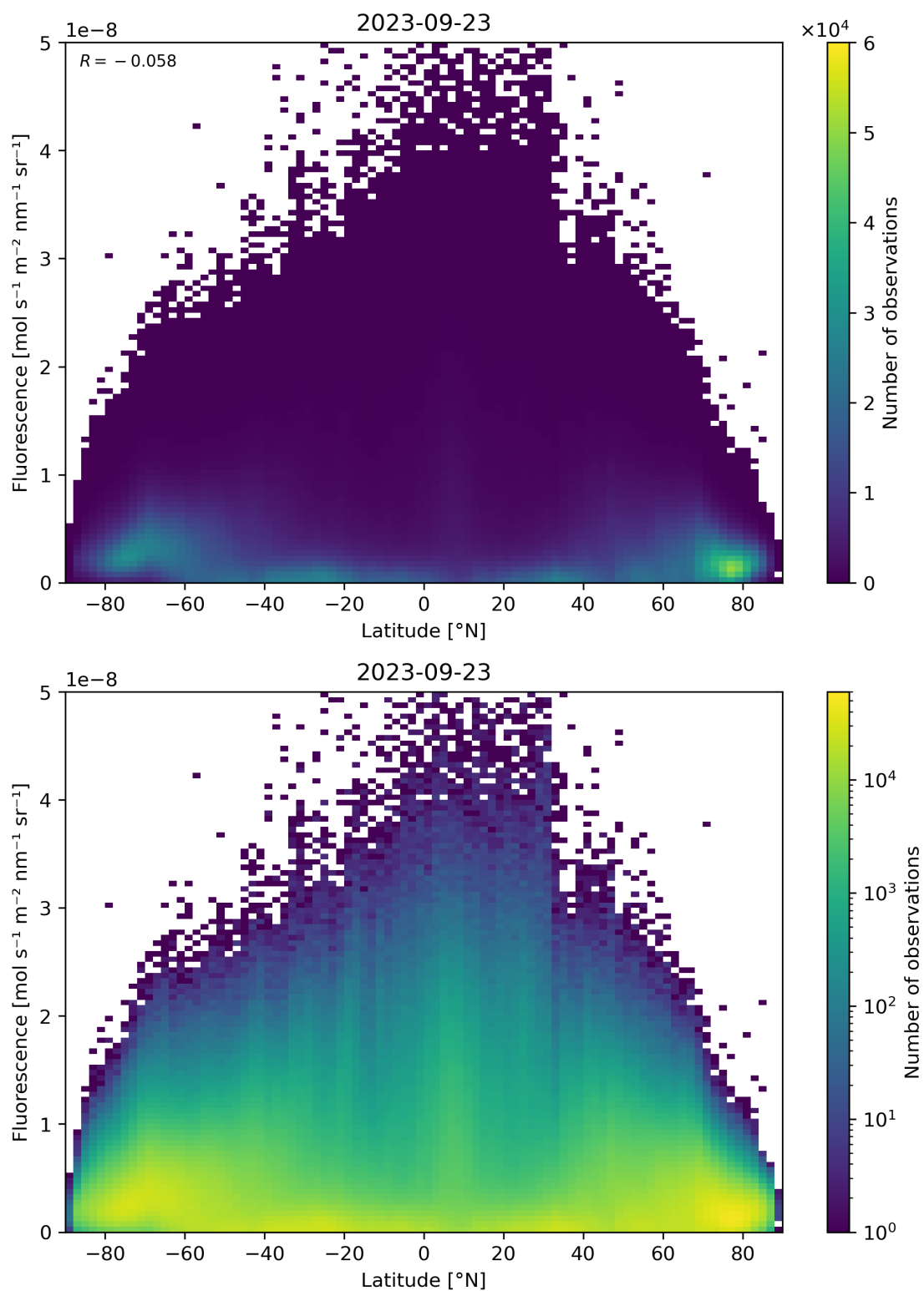
Figure 101: Scatter density plot of “Latitude” against “Fluorescence” for 2023-09-22 to 2023-09-24.
