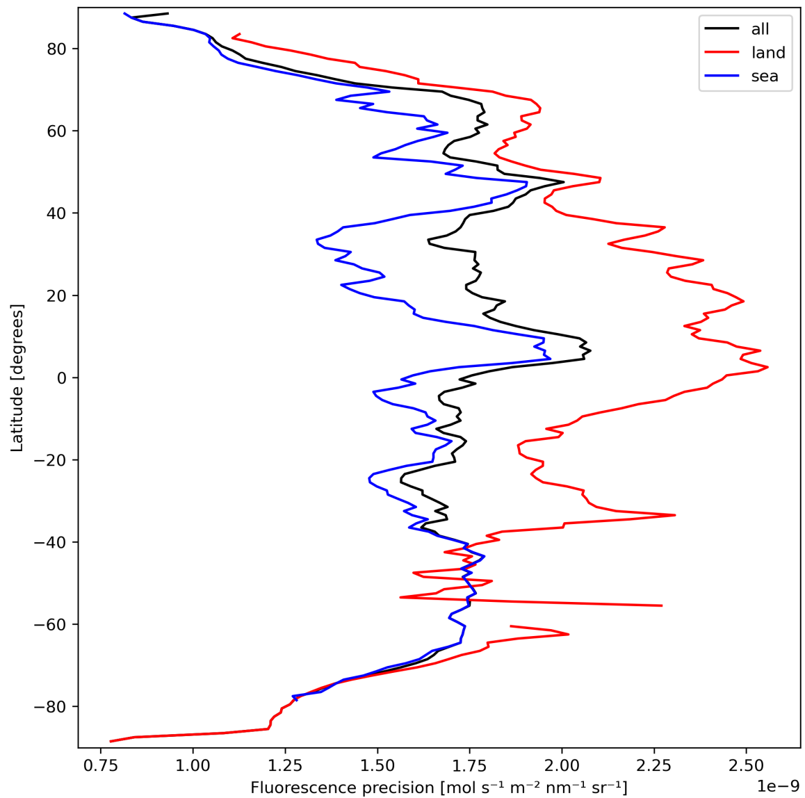
Figure 24: Zonal average of “Fluorescence precision” for 2023-09-22 to 2023-09-24.
