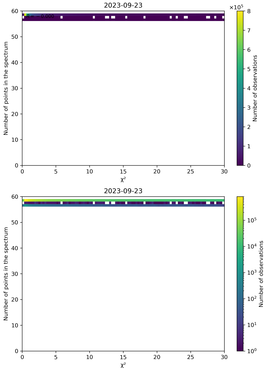
Figure 74: Scatter density plot of " \chi^2 " against "Number of points in the spectrum" for 2023-09-22 to 2023-09-24.
