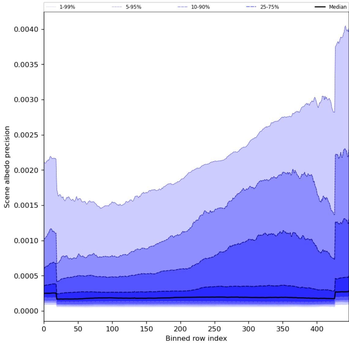
Figure 52: Along track statistics of “Scene albedo precision” for 2023-09-22 to 2023-09-24
