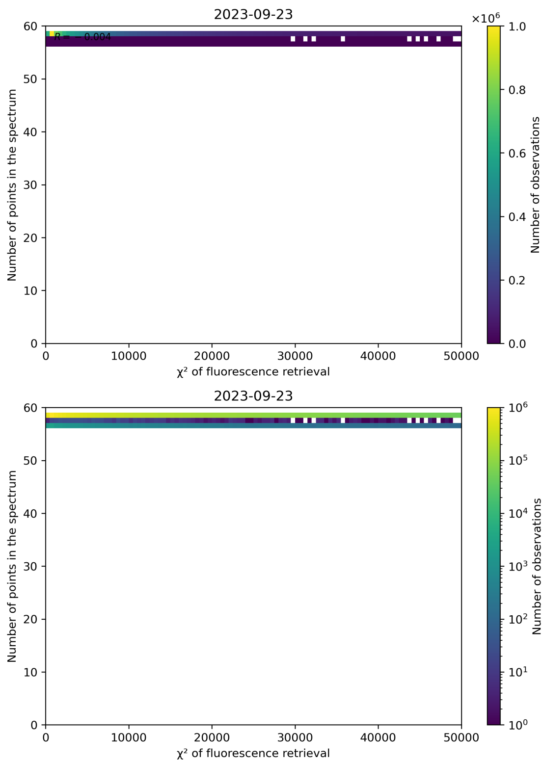
Figure 71: Scatter density plot of “ \chi^2 of fluorescence retrieval” against “Number of points in the spectrum” for 2023-09-22 to 2023-09-24.
