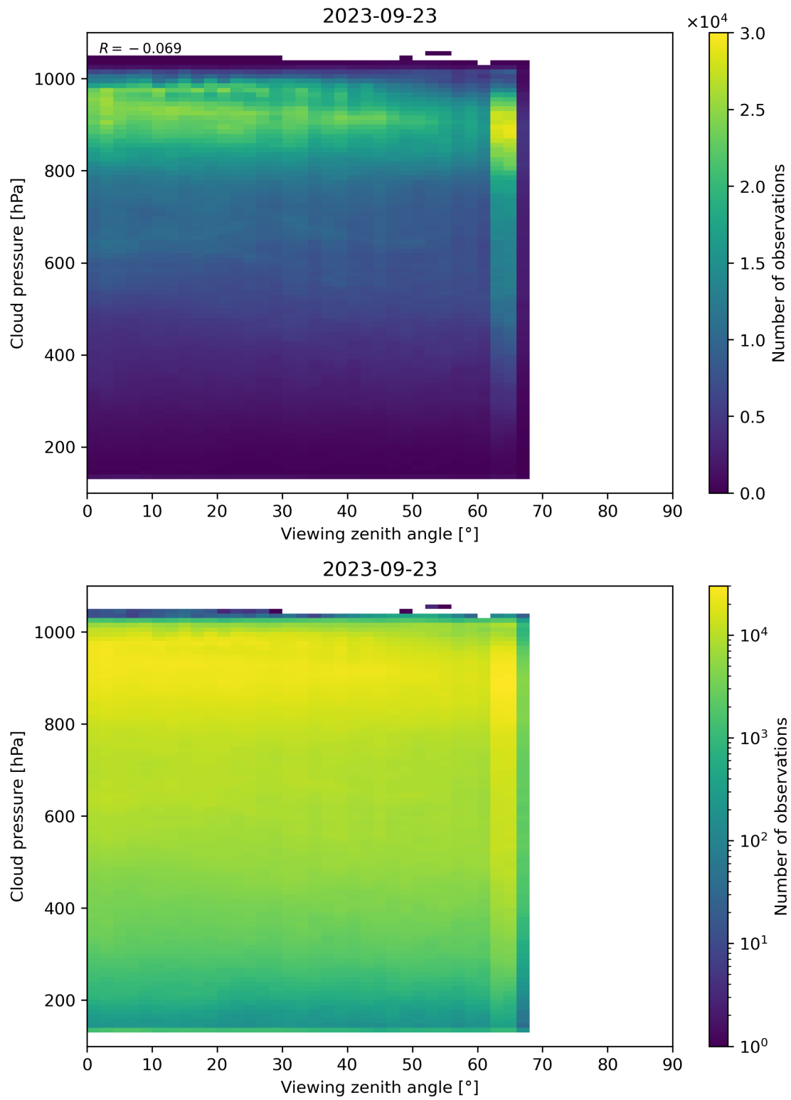
Figure 133: Scatter density plot of “Viewing zenith angle” against “Cloud pressure” for 2023-09-22 to 2023-09-24.
