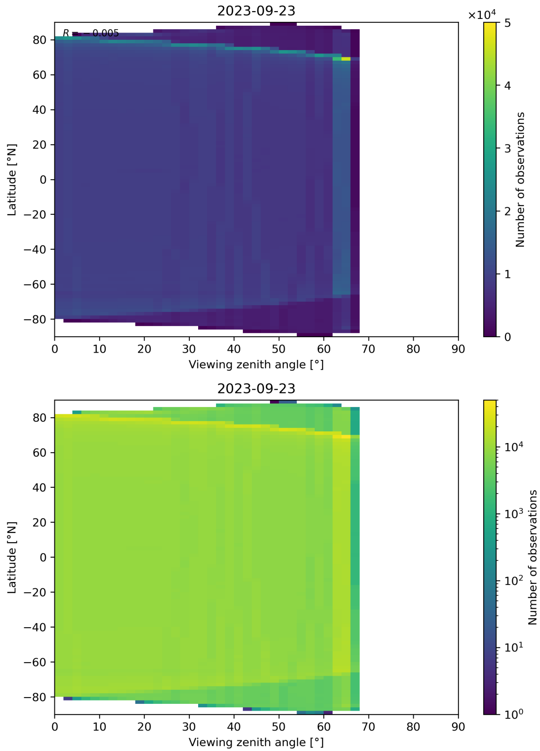
Figure 135: Scatter density plot of “Viewing zenith angle” against “Latitude” for 2023-09-22 to 2023-09-24.
