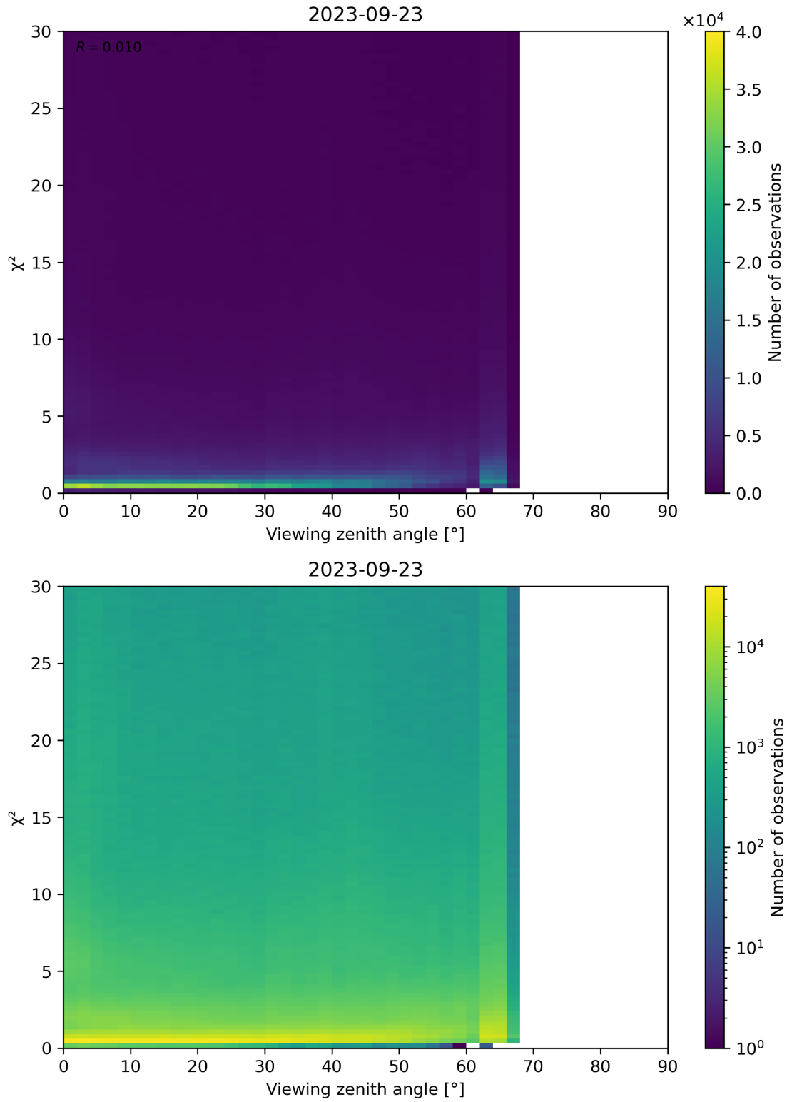
Figure 130: Scatter density plot of “Viewing zenith angle” against “ \chi^2 ” for 2023-09-22 to 2023-09-24.
