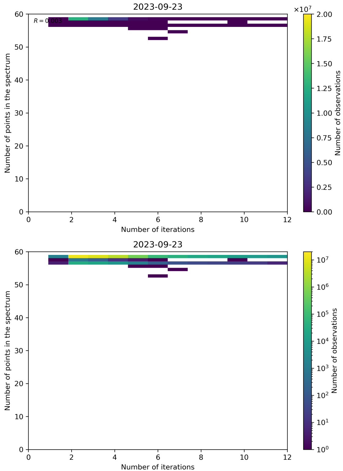
Figure 108: Scatter density plot of “Number of iterations” against “Number of points in the spectrum” for 2023-09-22 to 2023-09-24.
