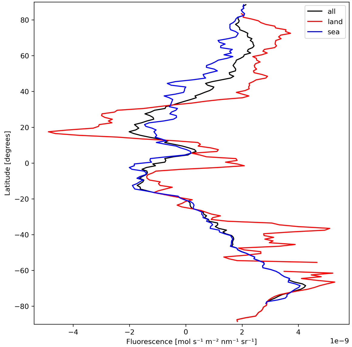
Figure 23: Zonal average of “Fluorescence” for 2023-09-22 to 2023-09-24.
