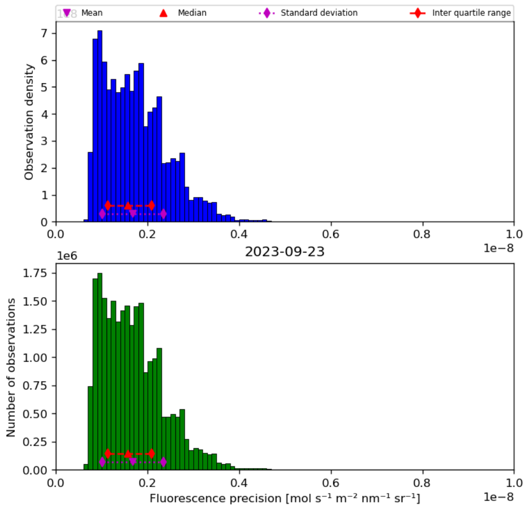
Figure 41: Histogram of “Fluorescence precision” for 2023-09-22 to 2023-09-24
