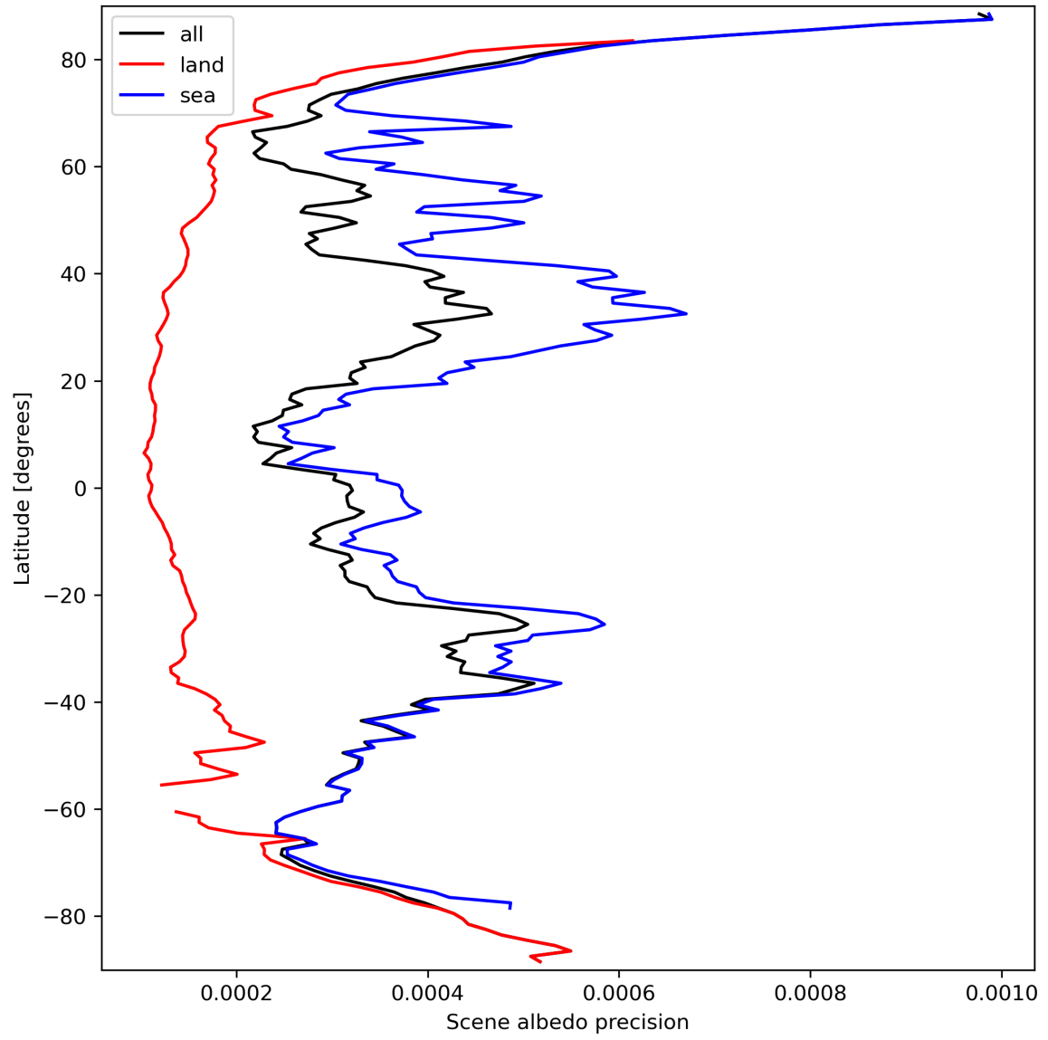
Figure 18: Zonal average of “Scene albedo precision” for 2023-09-22 to 2023-09-24.
