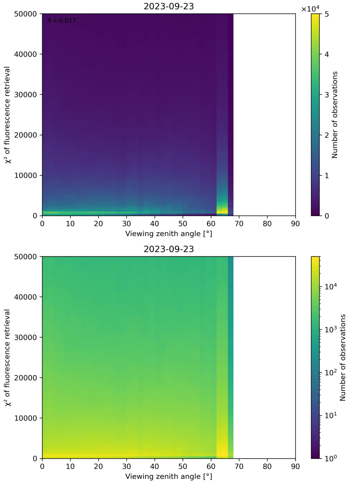
Figure 131: Scatter density plot of “Viewing zenith angle” against “ \chi^2 of fluorescence retrieval” for 2023-09-22 to 2023-09-24.
