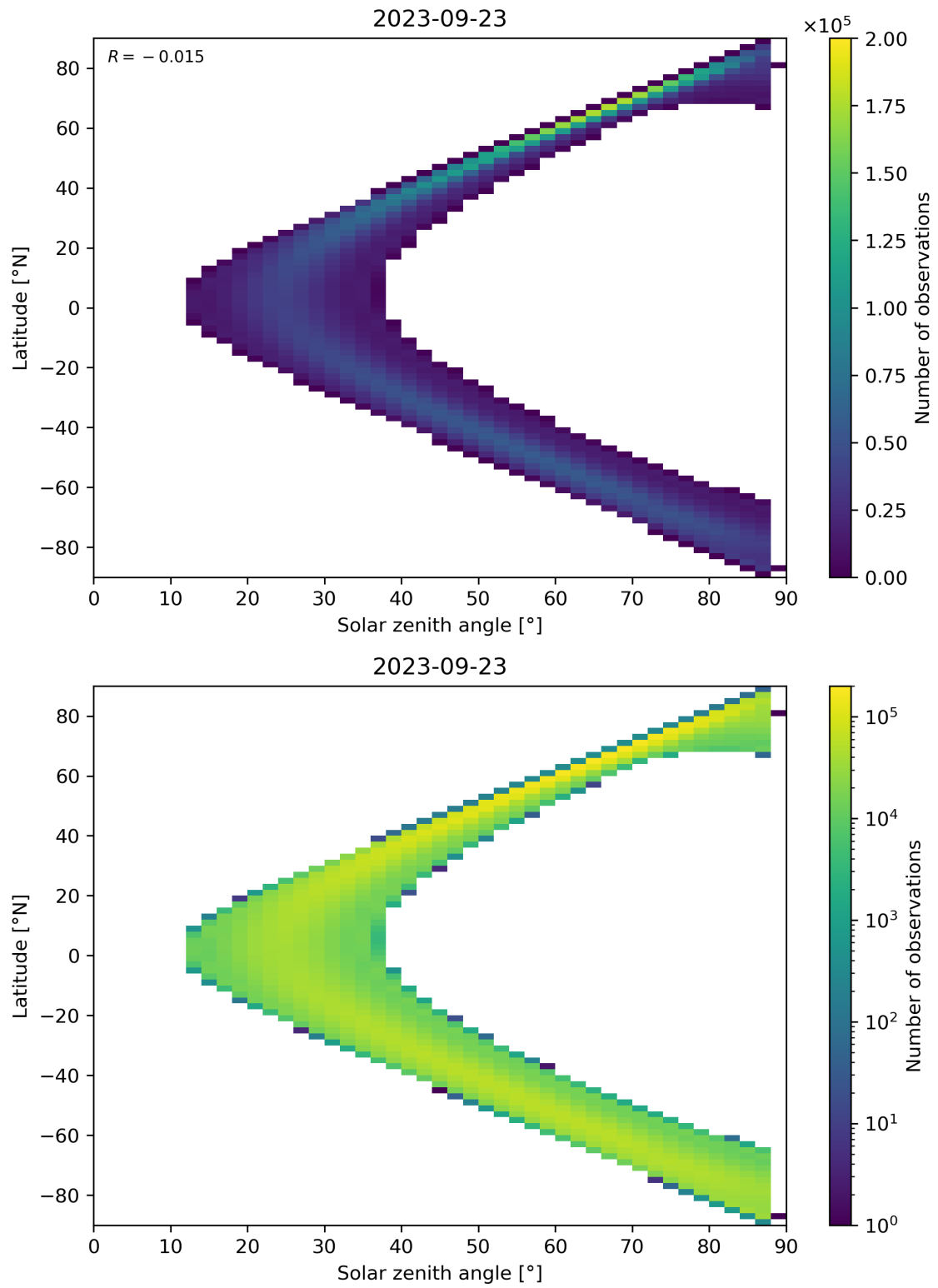
Figure 124: Scatter density plot of “Solar zenith angle” against “Latitude” for 2023-09-22 to 2023-09-24.
