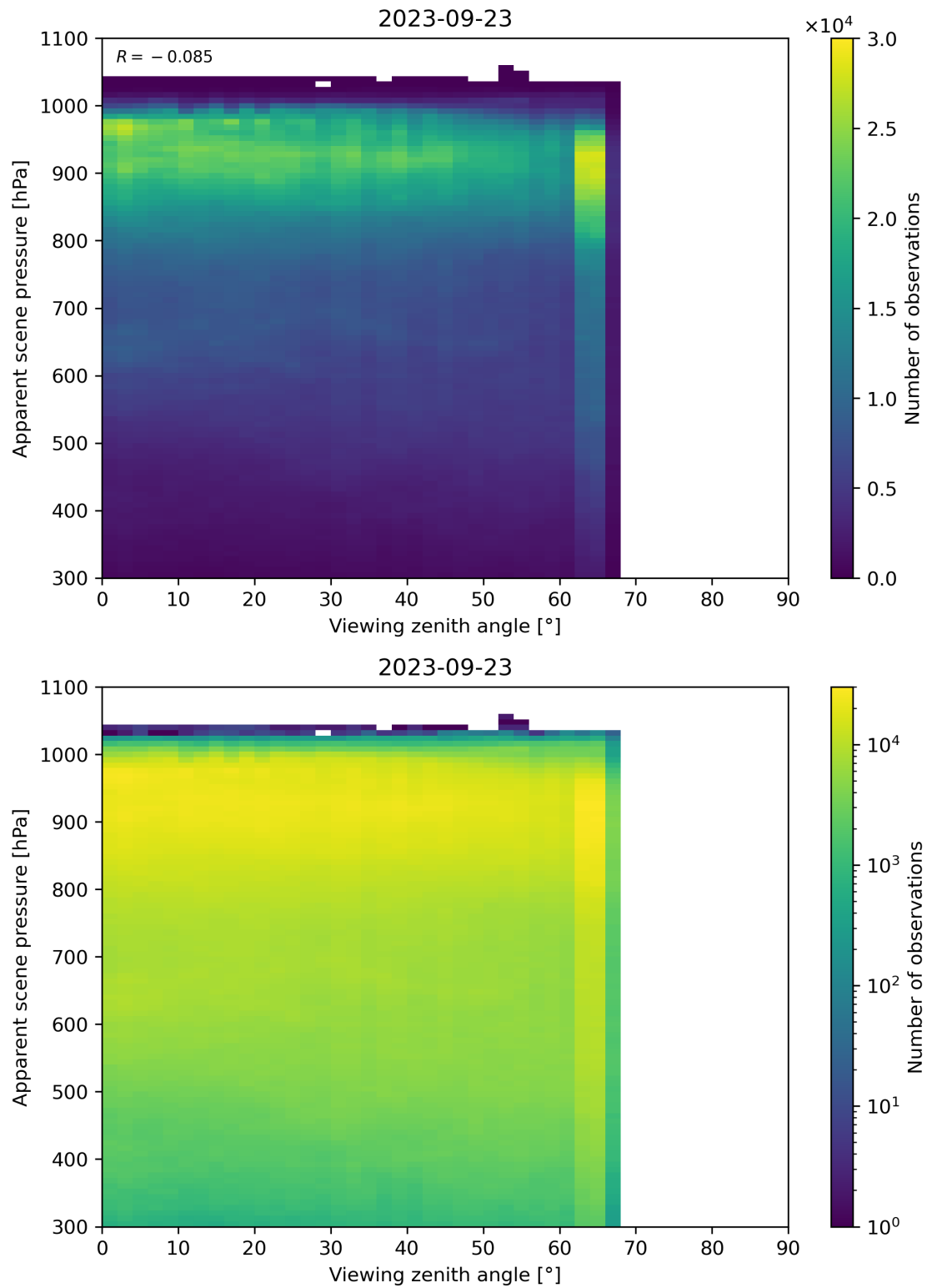
Figure 129: Scatter density plot of “Viewing zenith angle” against “Apparent scene pressure” for 2023-09-22 to 2023-09-24.
