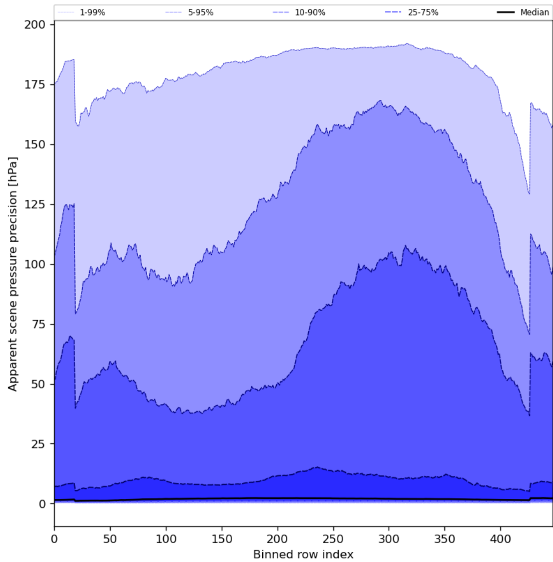
Figure 54: Along track statistics of “Apparent scene pressure precision” for 2023-09-22 to 2023-09-24
