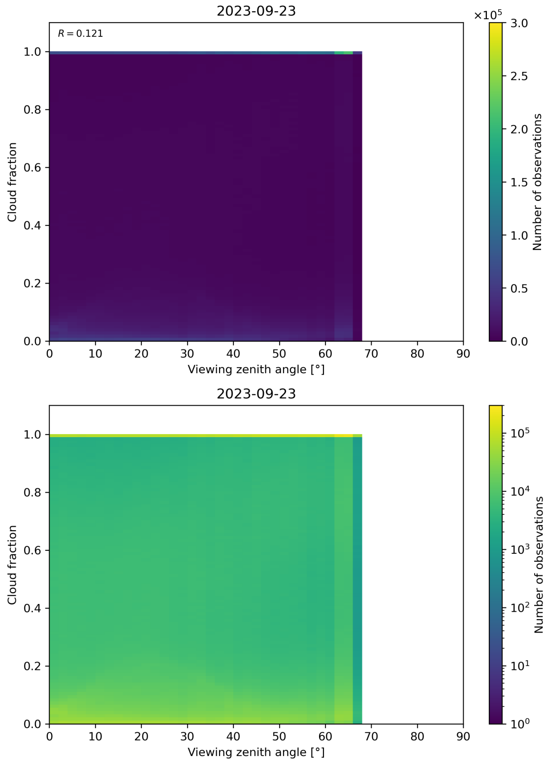
Figure 132: Scatter density plot of “Viewing zenith angle” against “Cloud fraction” for 2023-09-22 to 2023-09-24.
