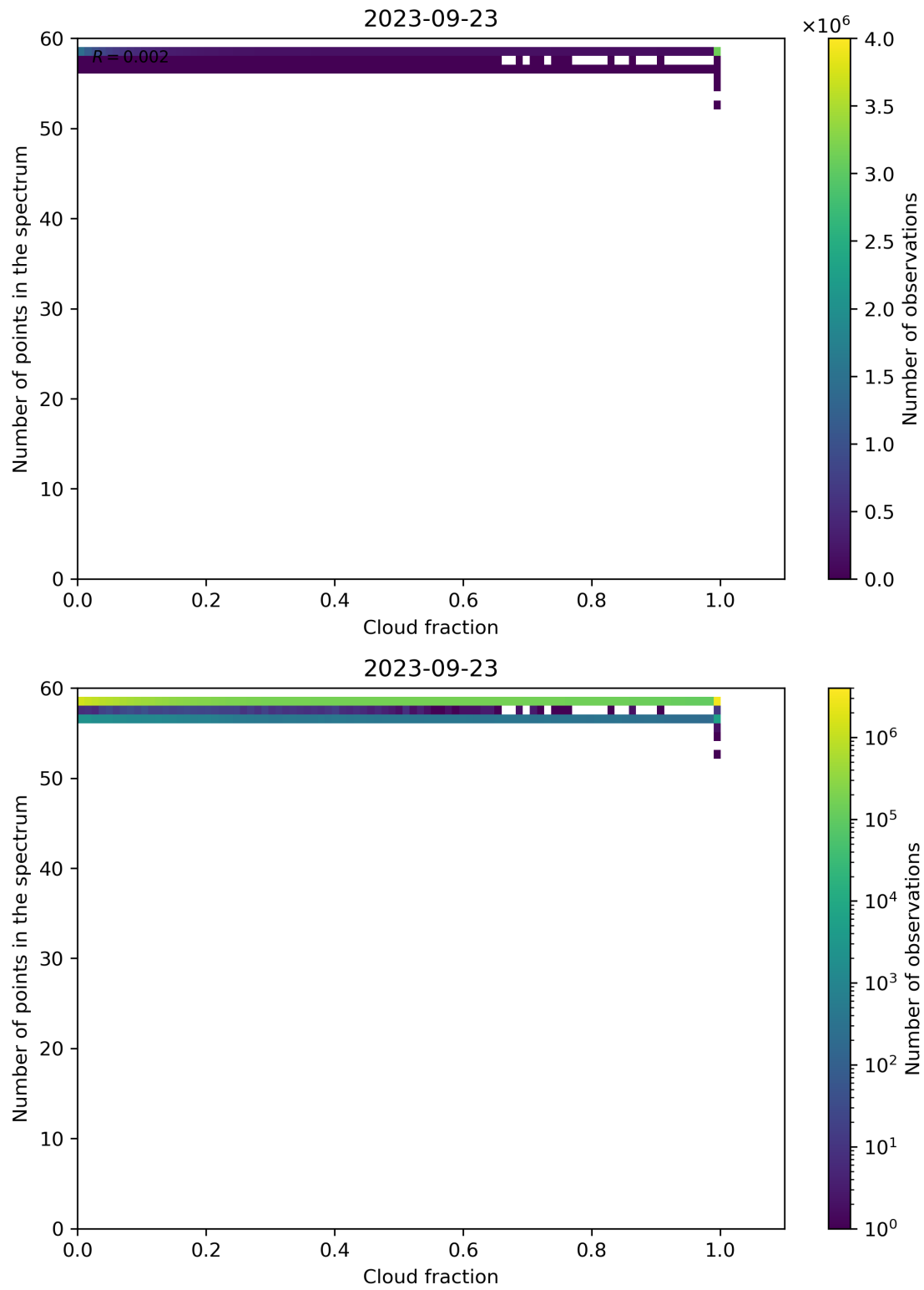
Figure 81: Scatter density plot of “Cloud fraction” against “Number of points in the spectrum” for 2023-09-22 to 2023-09-24.
