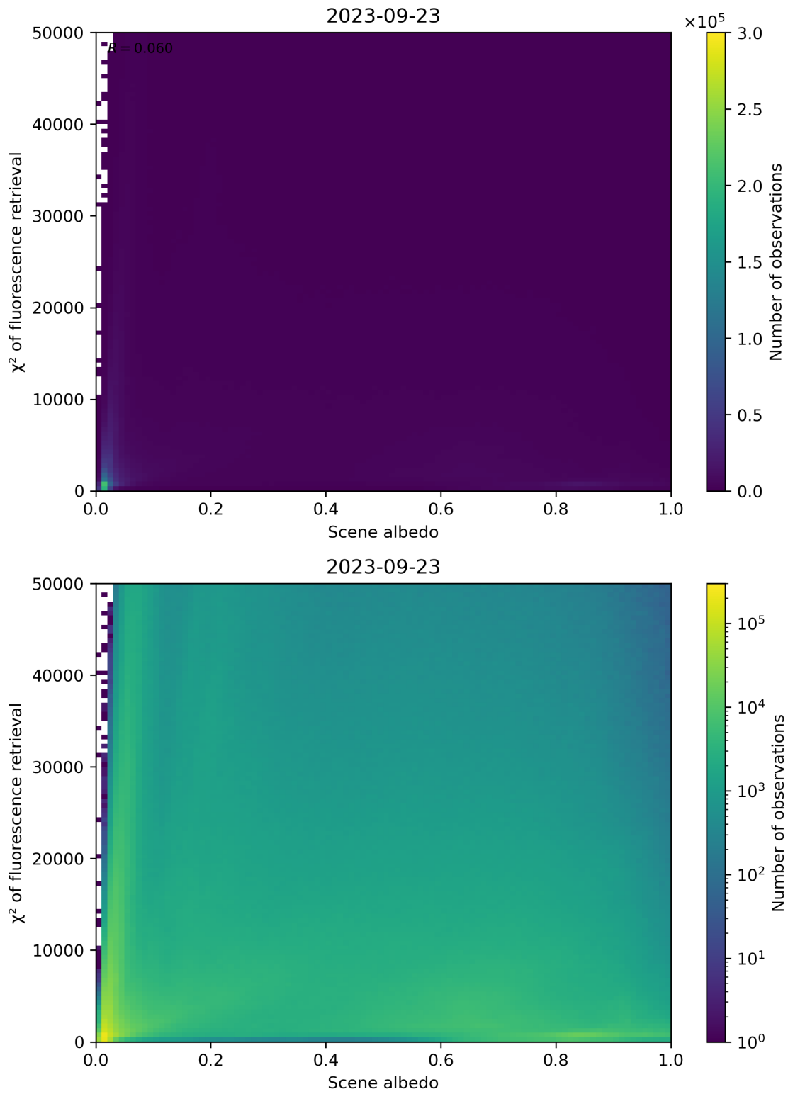
Figure 113: Scatter density plot of “Scene albedo” against “ \chi^2 of fluorescence retrieval” for 2023-09-22 to 2023-09-24.
