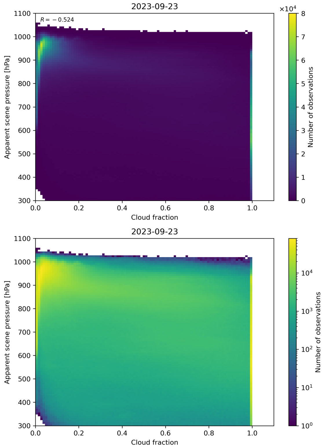
Figure 76: Scatter density plot of “Cloud fraction” against “Apparent scene pressure” for 2023-09-22 to 2023-09-24.
