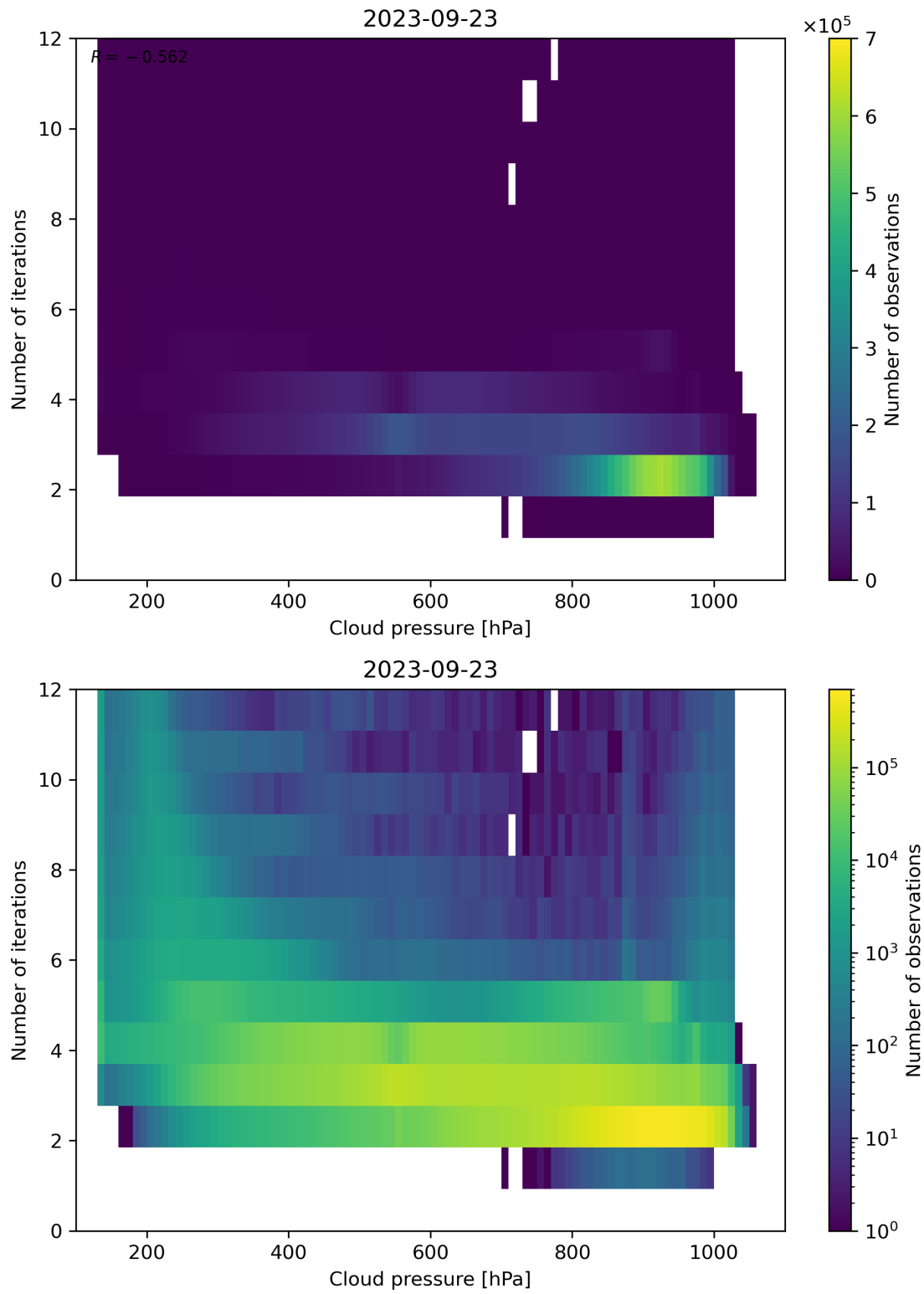
Figure 89: Scatter density plot of “Cloud pressure” against “Number of iterations” for 2023-09-22 to 2023-09-24.
