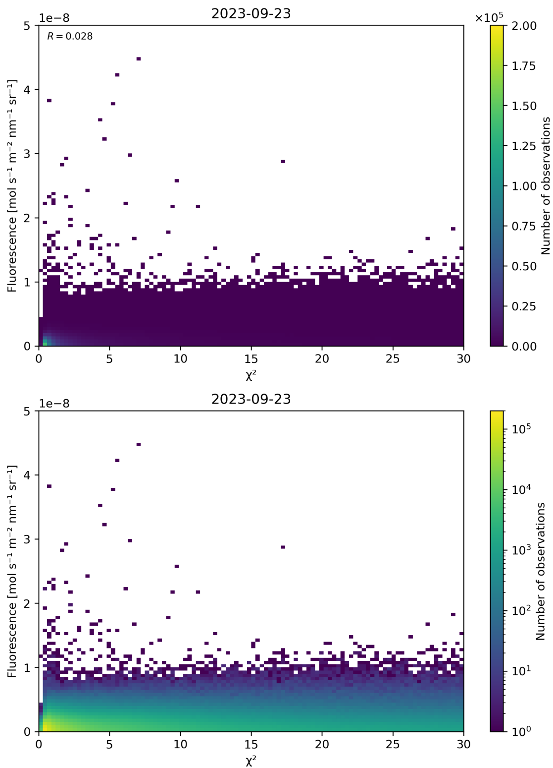
Figure 70: Scatter density plot of “ \chi^2 ” against “Fluorescence” for 2023-09-22 to 2023-09-24.
