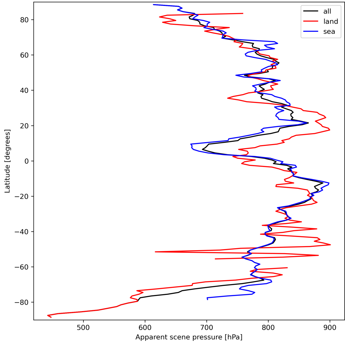
Figure 19: Zonal average of “Apparent scene pressure” for 2023-09-22 to 2023-09-24.
