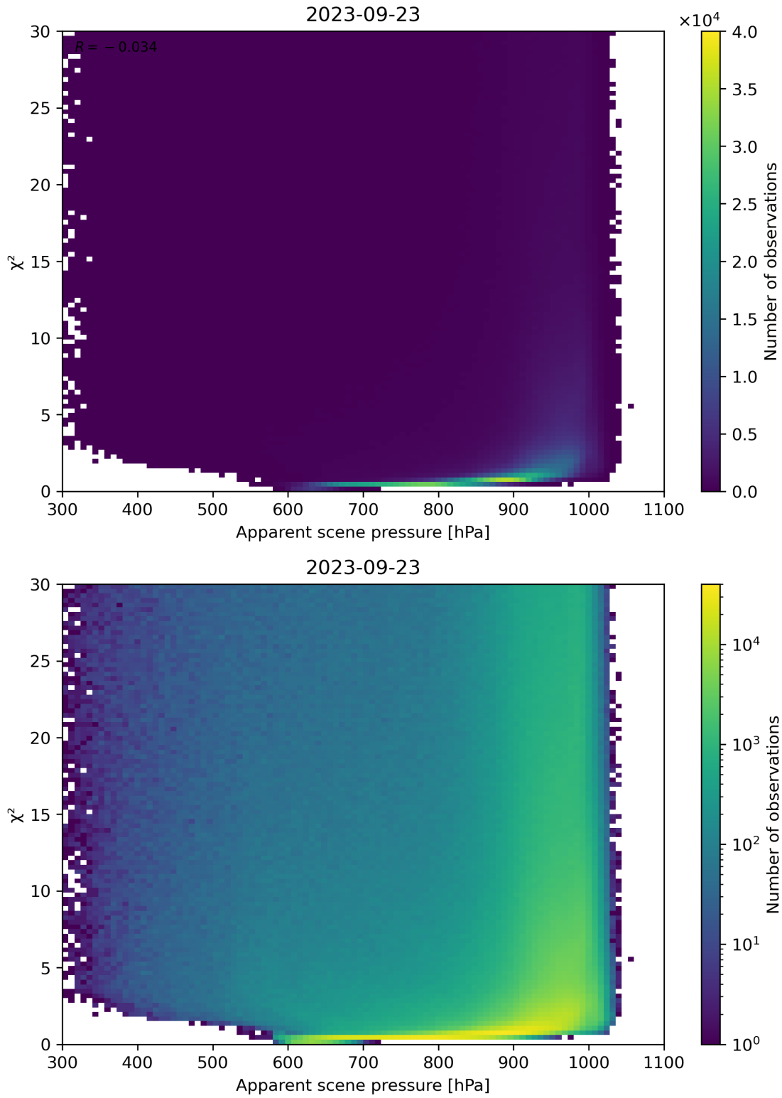
Figure 63: Scatter density plot of “Apparent scene pressure” against “ \chi^2 ” for 2023-09-22 to 2023-09-24.
