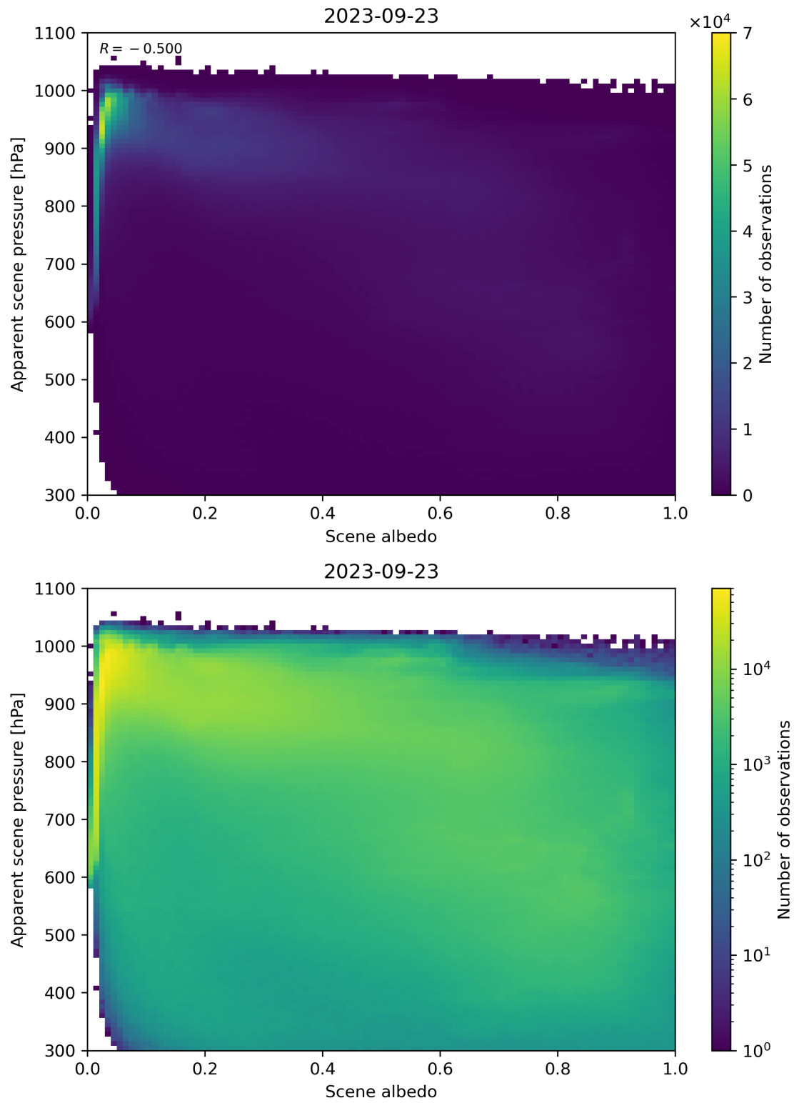
Figure 111: Scatter density plot of “Scene albedo” against “Apparent scene pressure” for 2023-09-22 to 2023-09-24.
