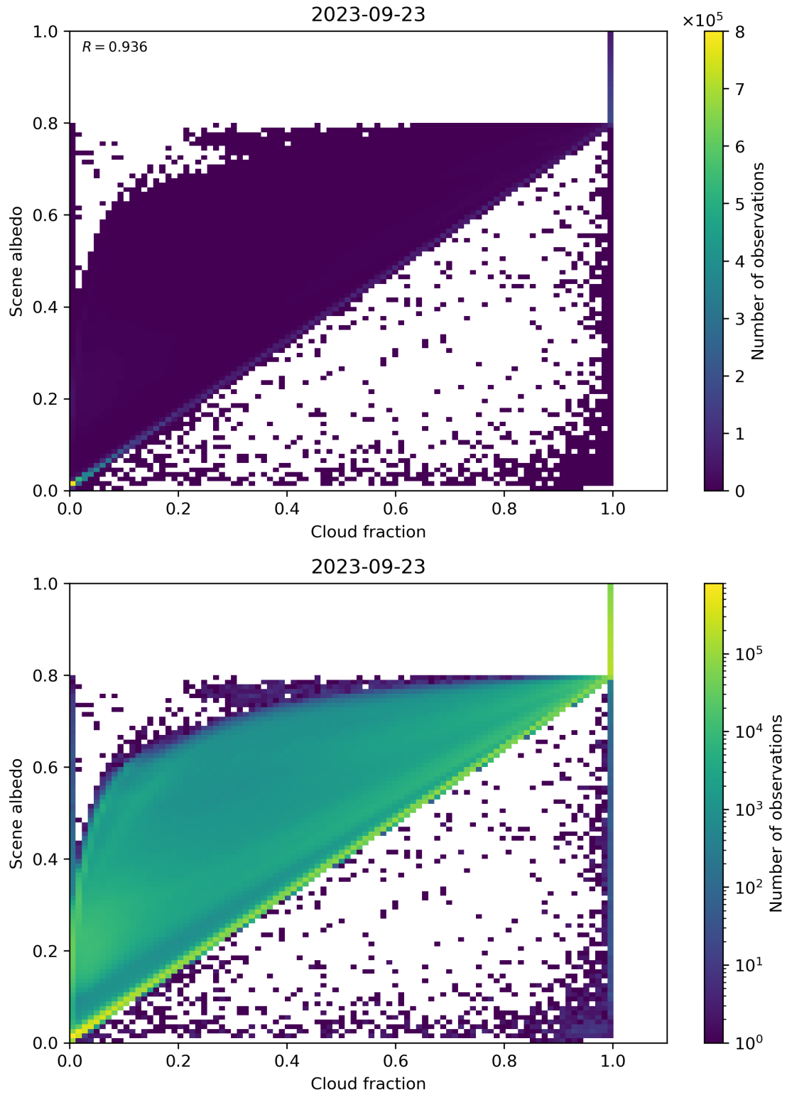
Figure 82: Scatter density plot of “Cloud fraction” against “Scene albedo” for 2023-09-22 to 2023-09-24.
