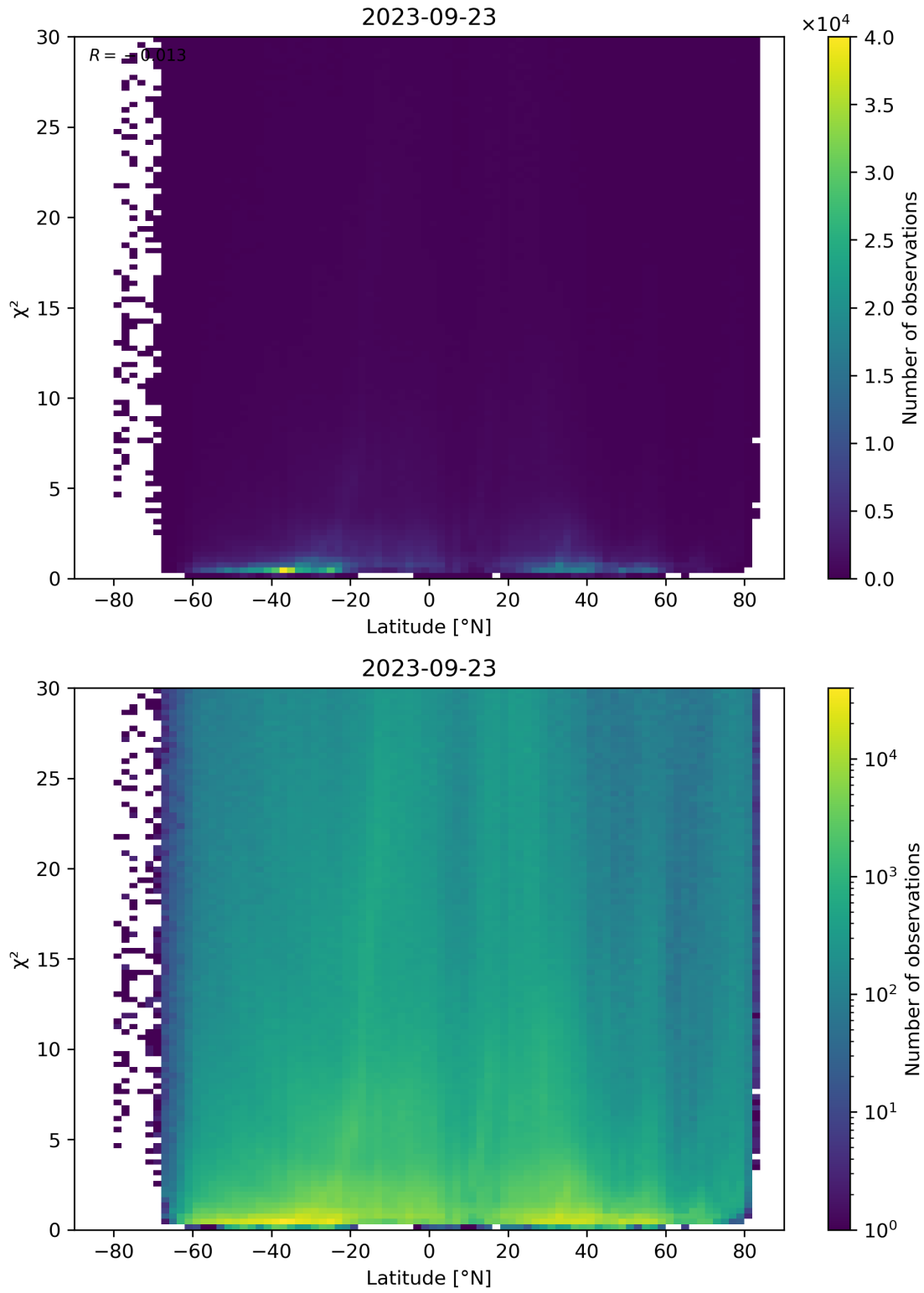
Figure 97: Scatter density plot of “Latitude” against “ \chi^2 ” for 2023-09-22 to 2023-09-24.
