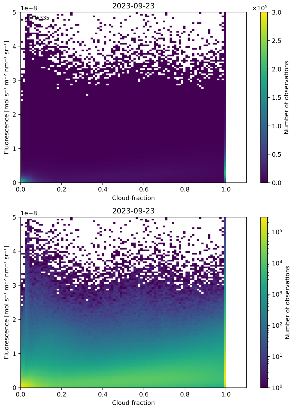
Figure 79: Scatter density plot of “Cloud fraction” against “Fluorescence” for 2023-09-22 to 2023-09-24.
