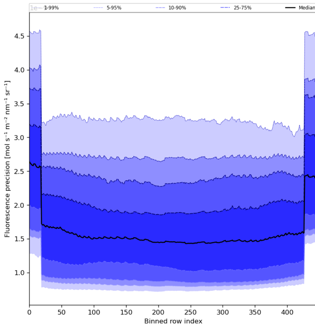
Figure 58: Along track statistics of “Fluorescence precision” for 2023-09-22 to 2023-09-24
