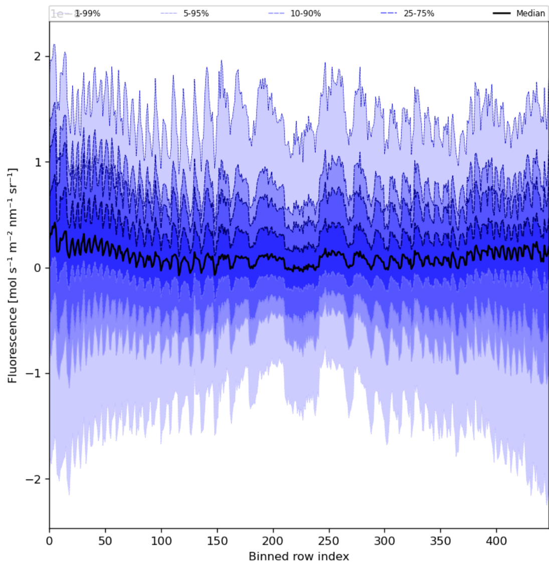
Figure 57: Along track statistics of "Fluorescence" for 2023-09-22 to 2023-09-24
