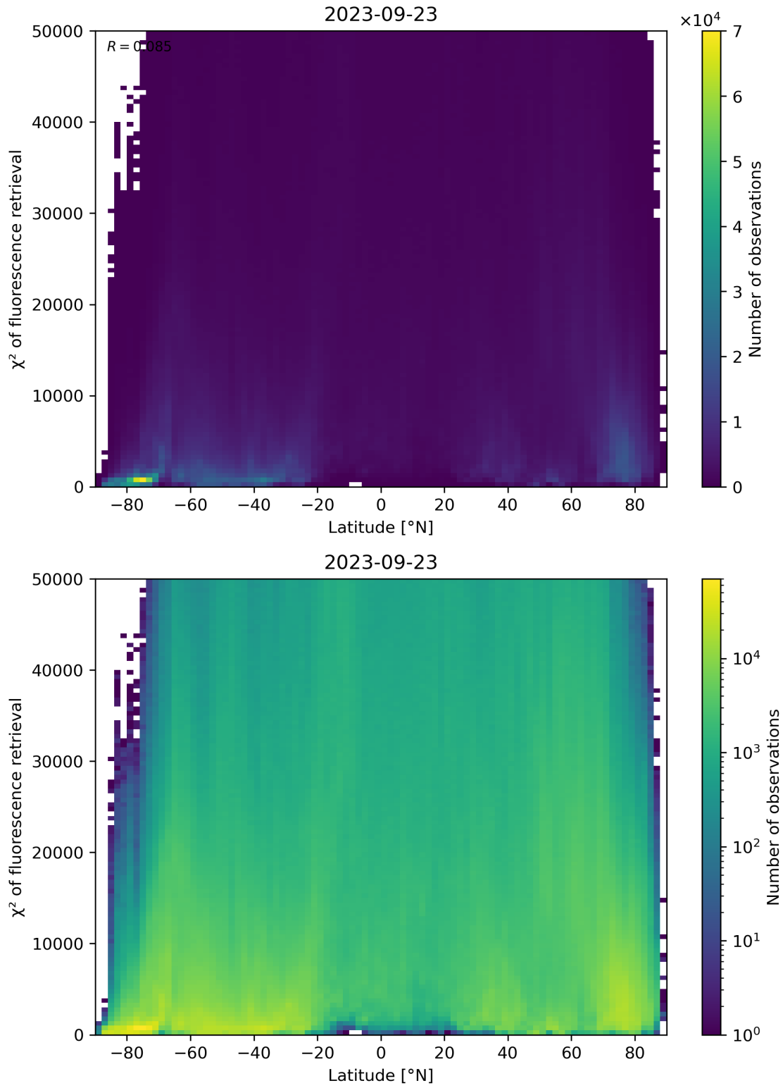
Figure 98: Scatter density plot of “Latitude” against “ \chi^2 of fluorescence retrieval” for 2023-09-22 to 2023-09-24.
