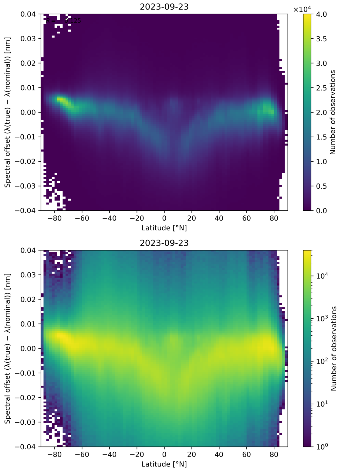
Figure 105: Scatter density plot of “Latitude” against “Spectral offset ( \lambda(\text{true}) - \lambda(\text{nominal}) )” for 2023-09-22 to 2023-09-24.
