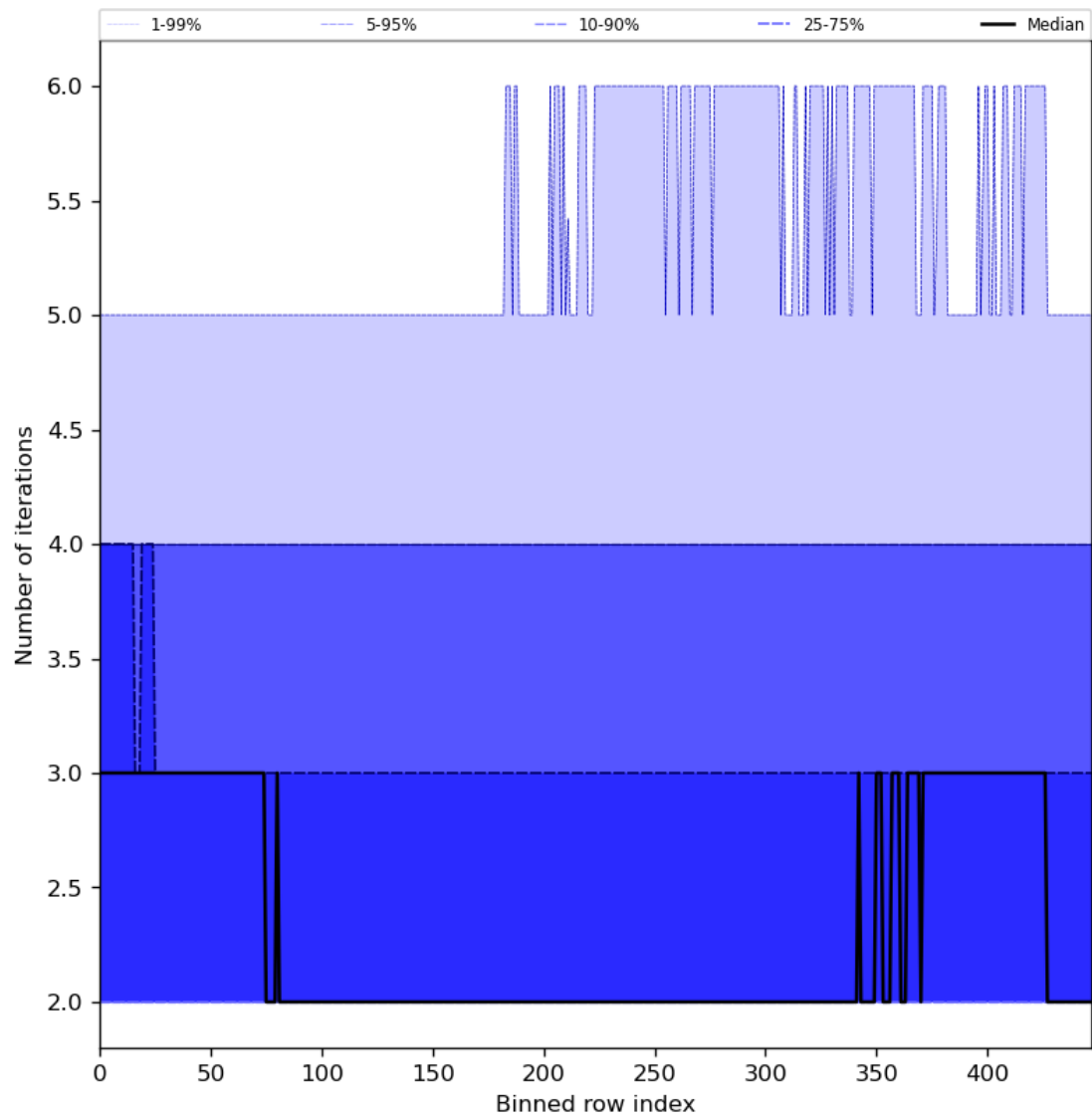
Figure 56: Along track statistics of “Number of iterations” for 2023-09-22 to 2023-09-24
