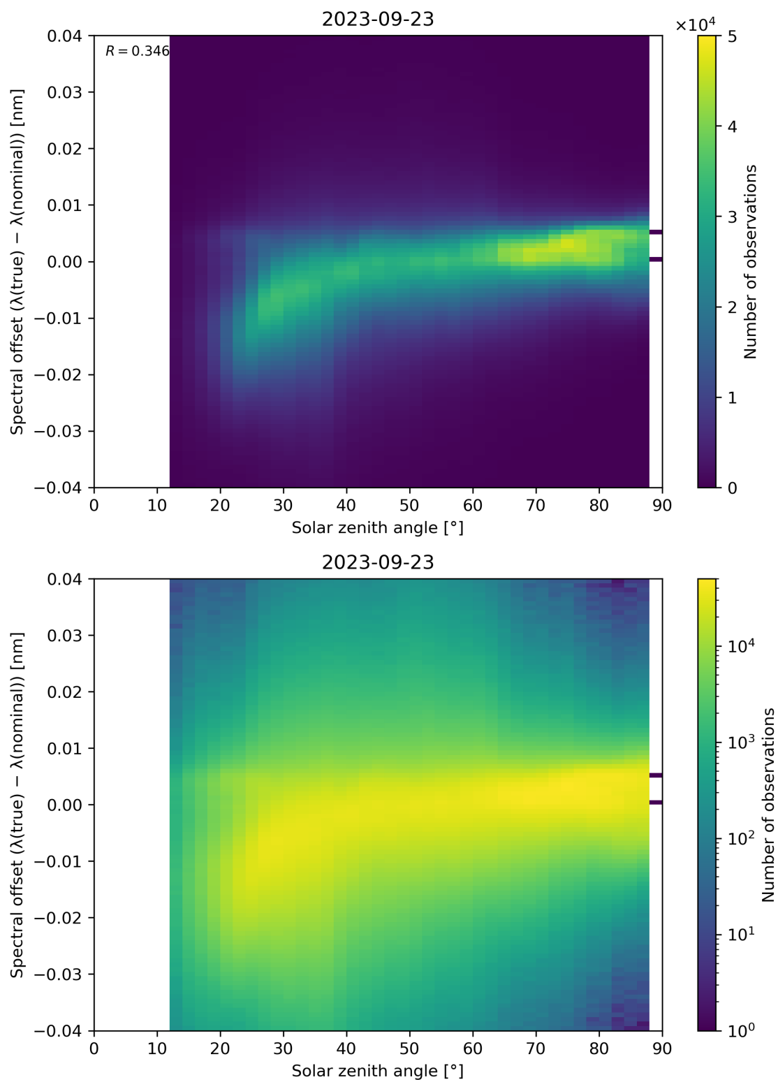
Figure 128: Scatter density plot of “Solar zenith angle” against “Spectral offset ( \lambda(\text{true}) - \lambda(\text{nominal}) )” for 2023-09-22 to 2023-09-24.
