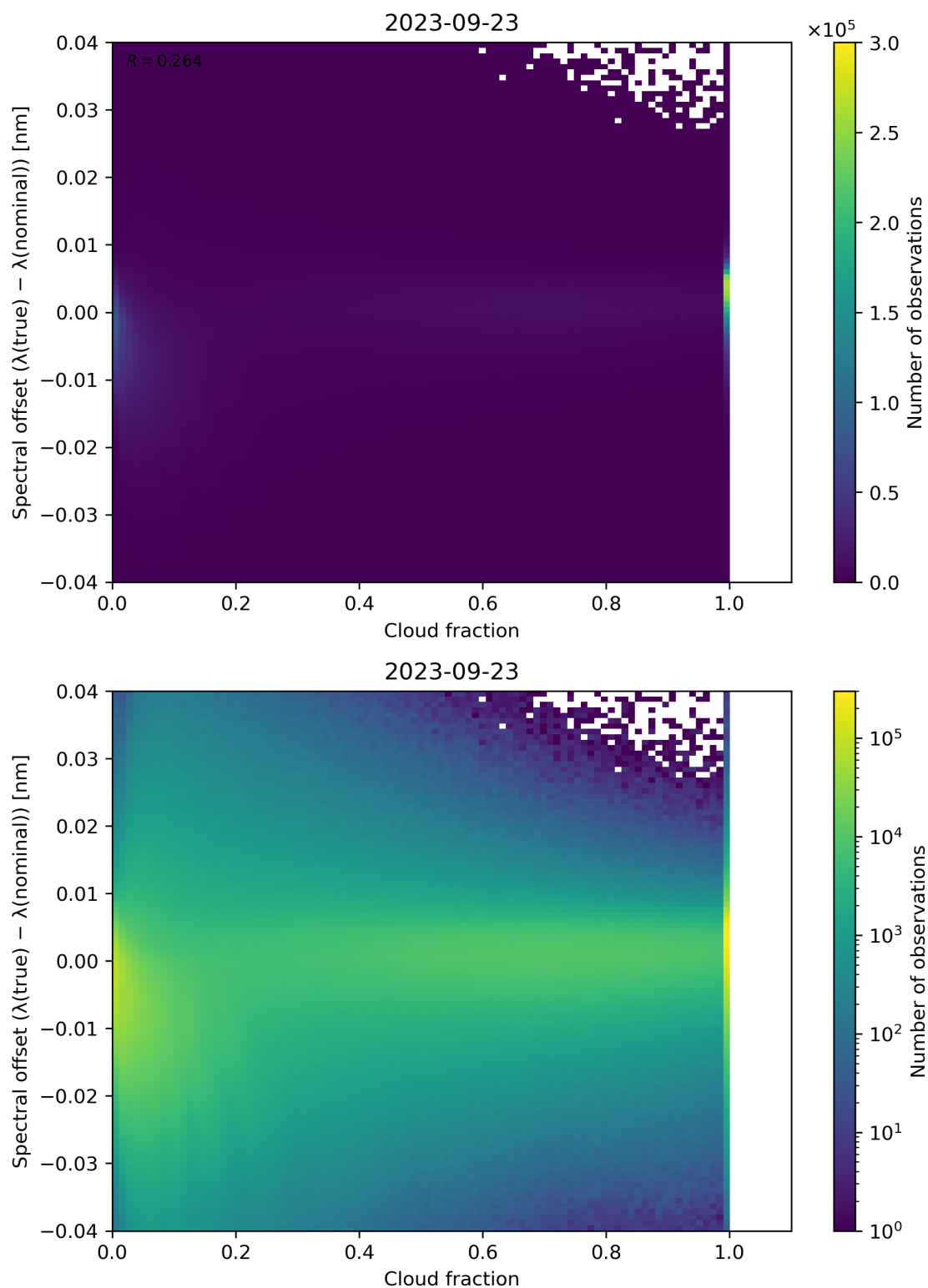
Figure 83: Scatter density plot of “Cloud fraction” against “Spectral offset ( \lambda(\text{true}) - \lambda(\text{nominal}) )” for 2023-09-22 to 2023-09-24.
