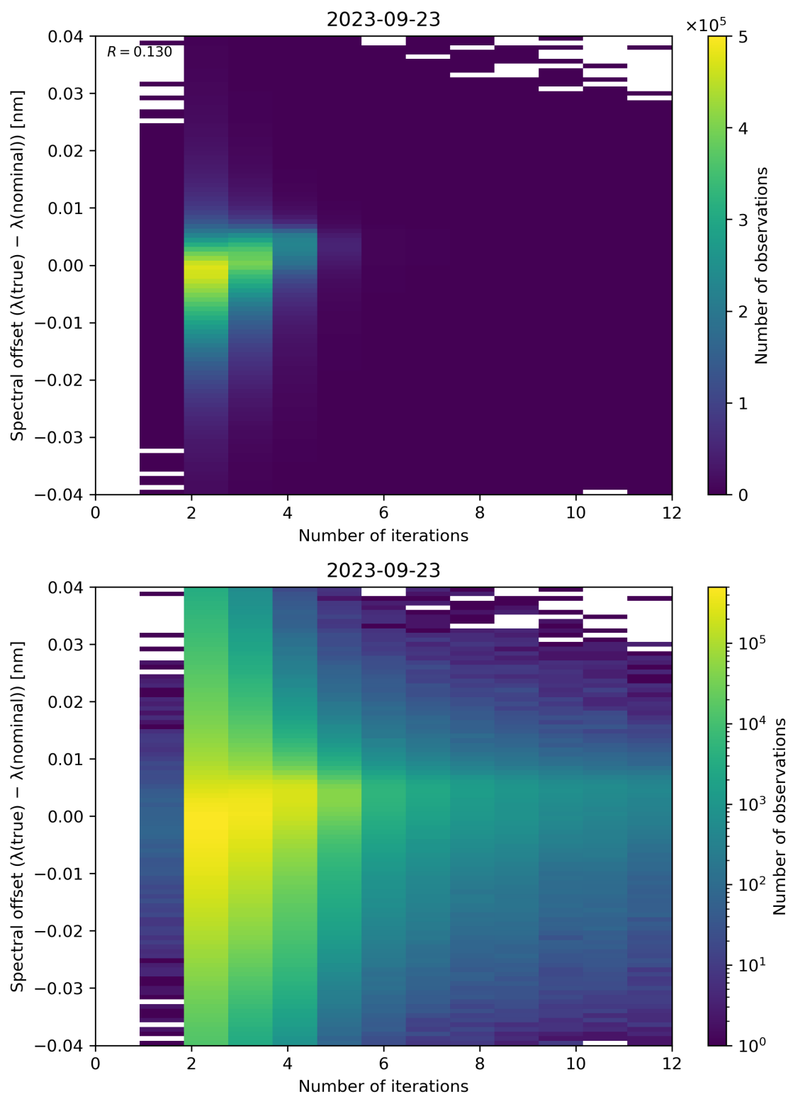
Figure 109: Scatter density plot of “Number of iterations” against “Spectral offset ( \lambda(\text{true}) - \lambda(\text{nominal}) )” for 2023-09-22 to 2023-09-24.
