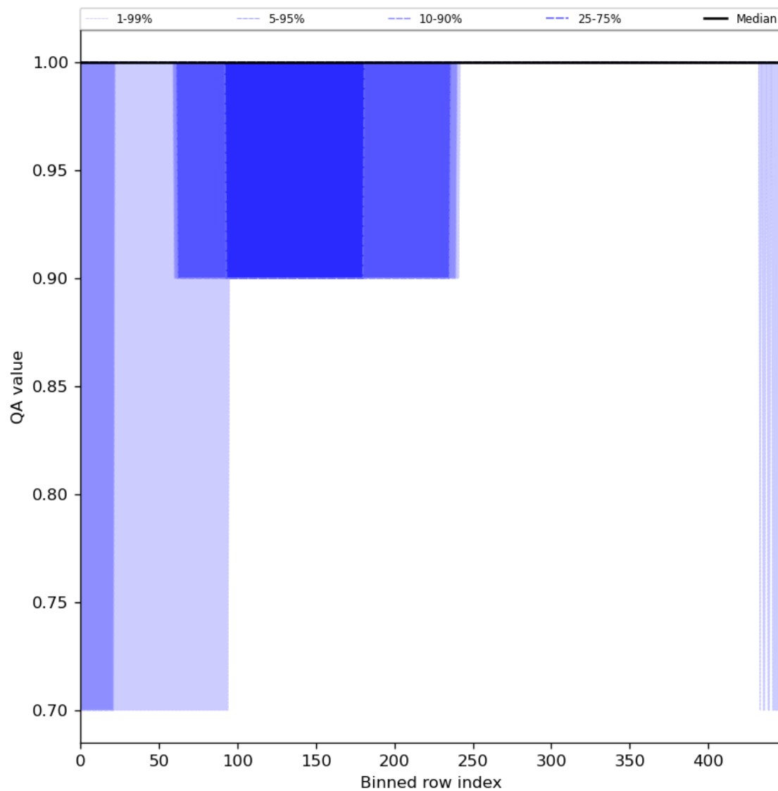
Figure 46: Along track statistics of “QA value” for 2023-09-22 to 2023-09-24
