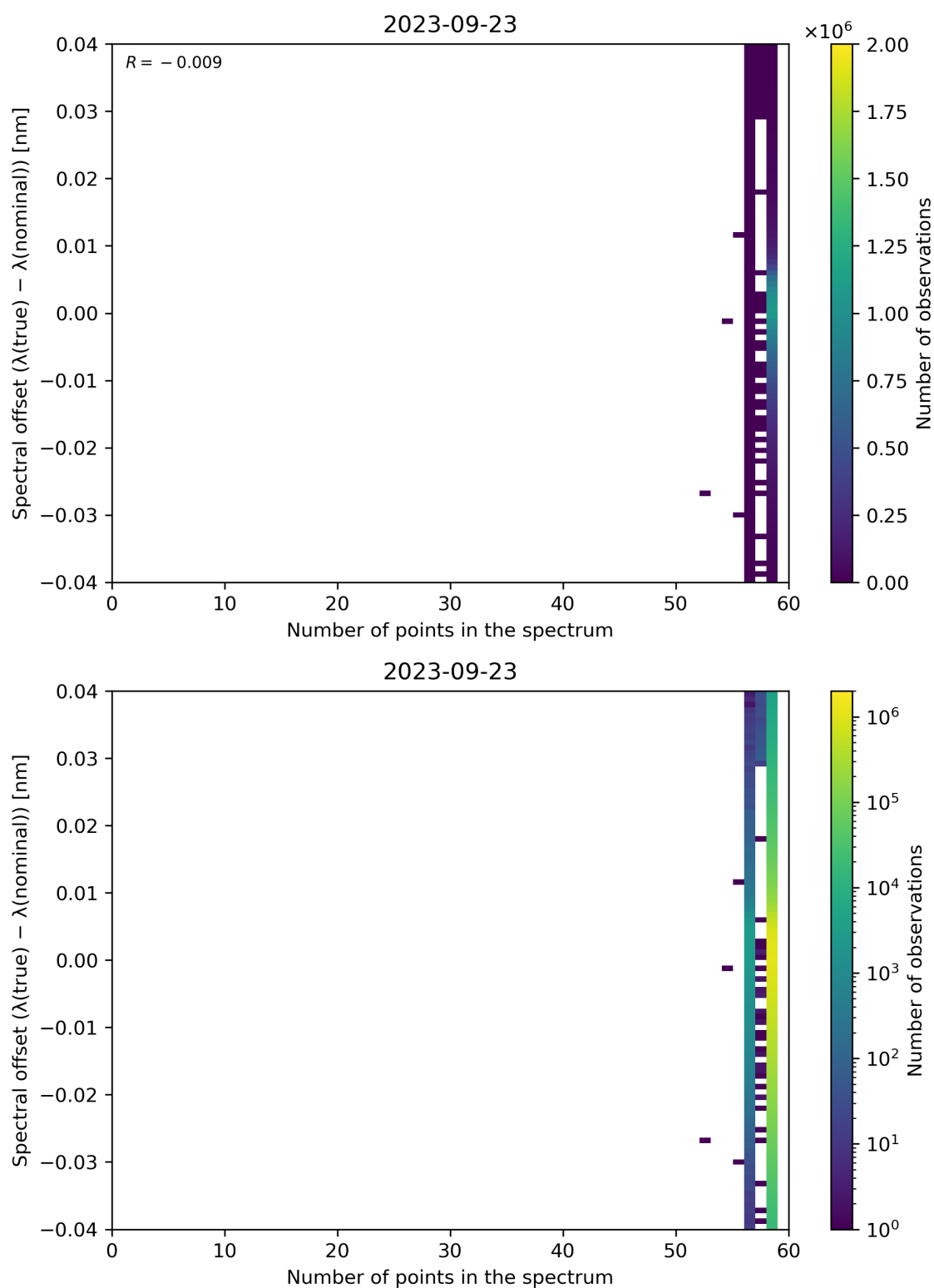
Figure 110: Scatter density plot of “Number of points in the spectrum” against “Spectral offset ( \lambda(\text{true}) - \lambda(\text{nominal}) )” for 2023-09-22 to 2023-09-24.
