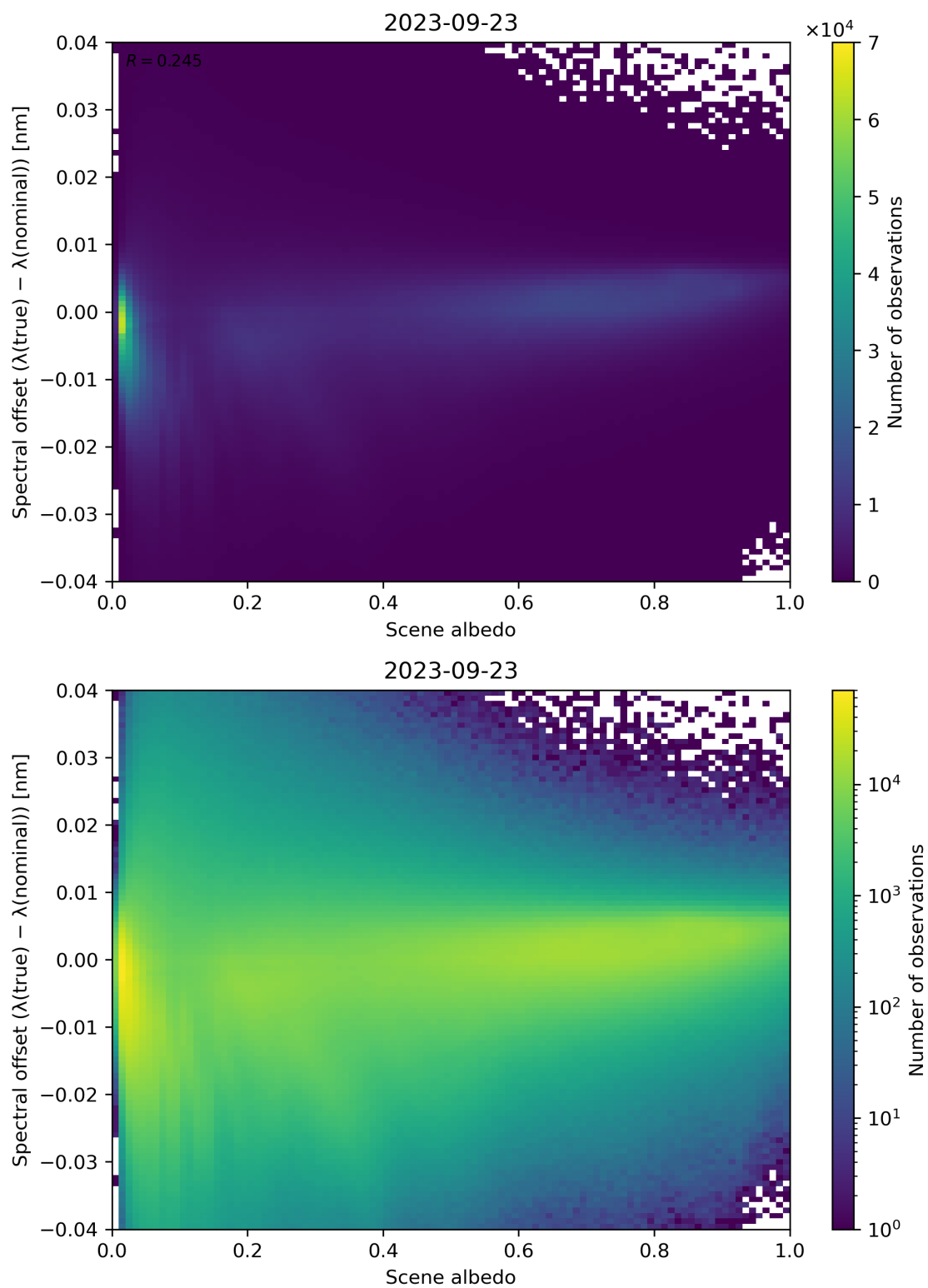
Figure 117: Scatter density plot of “Scene albedo” against “Spectral offset ( \lambda(\text{true}) - \lambda(\text{nominal}) )” for 2023-09-22 to 2023-09-24.
