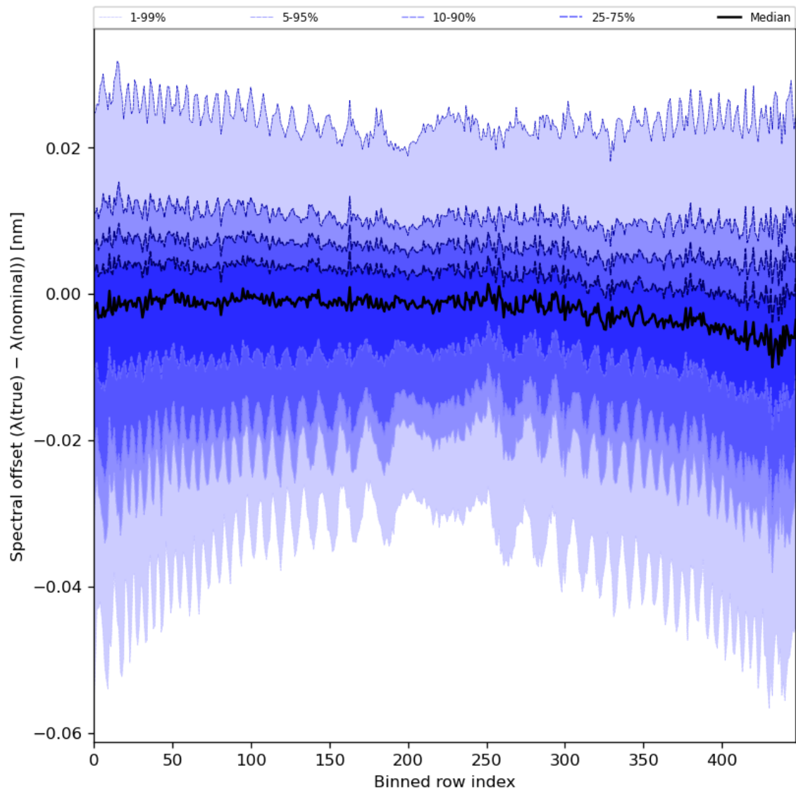
Figure 62: Along track statistics of “Spectral offset ( \lambda(\text{true}) - \lambda(\text{nominal}) )” for 2023-09-22 to 2023-09-24
