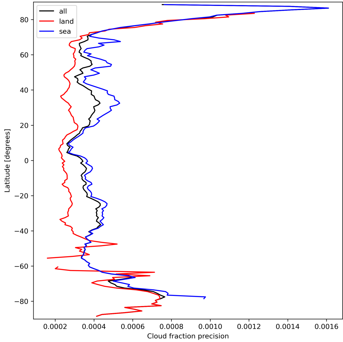
Figure 16: Zonal average of “Cloud fraction precision” for 2023-09-22 to 2023-09-24.
