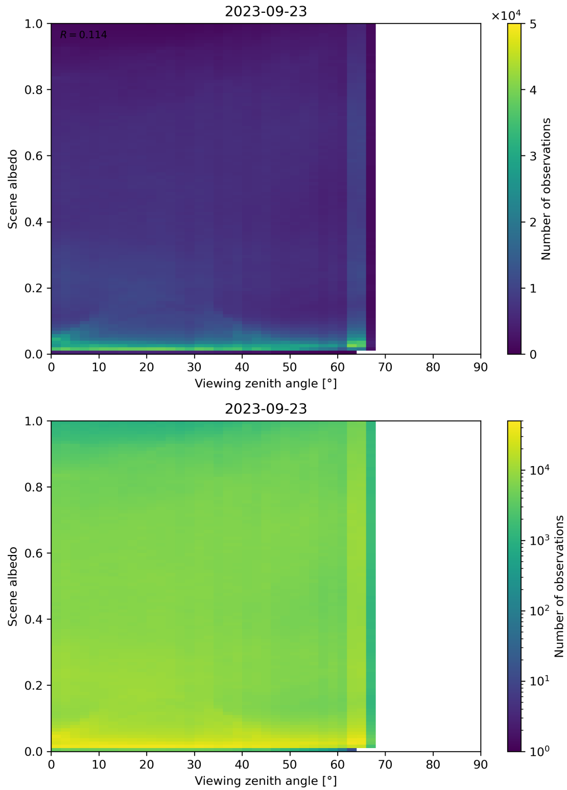
Figure 138: Scatter density plot of “Viewing zenith angle” against “Scene albedo” for 2023-09-22 to 2023-09-24.
