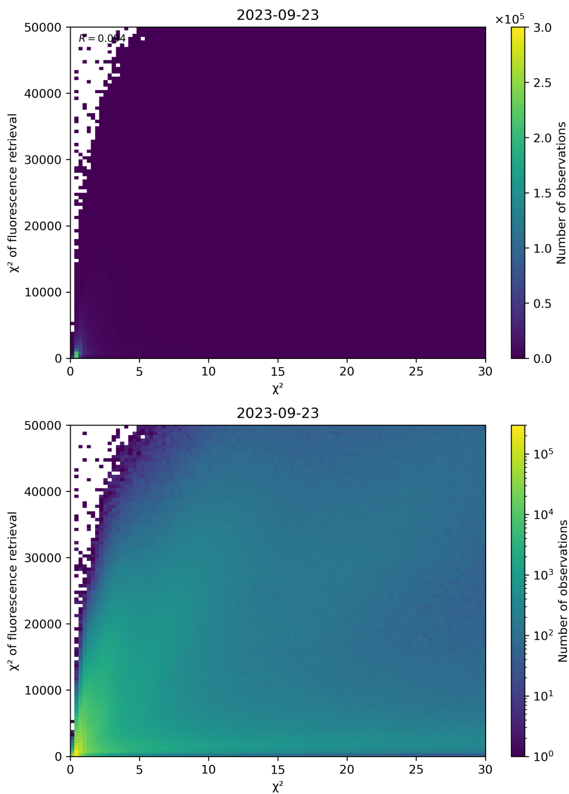
Figure 69: Scatter density plot of “ \chi^2 ” against “ \chi^2 of fluorescence retrieval” for 2023-09-22 to 2023-09-24.
