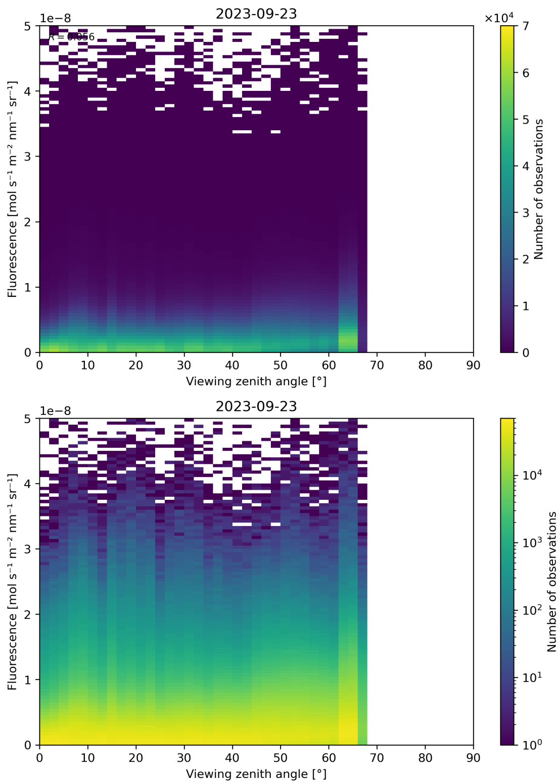
Figure 134: Scatter density plot of “Viewing zenith angle” against “Fluorescence” for 2023-09-22 to 2023-09-24.
