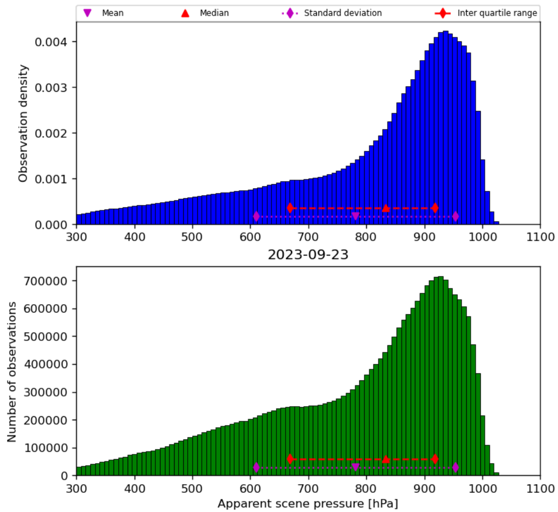
Figure 36: Histogram of “Apparent scene pressure” for 2023-09-22 to 2023-09-24
