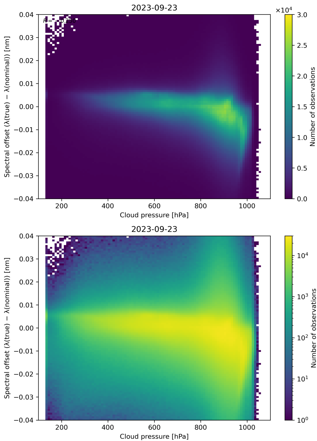
Figure 92: Scatter density plot of “Cloud pressure” against “Spectral offset ( \lambda(\text{true}) - \lambda(\text{nominal}) )” for 2023-09-22 to 2023-09-24.
