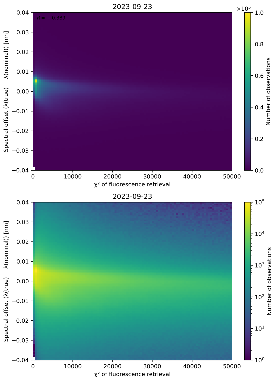
Figure 72: Scatter density plot of " \chi^2 of fluorescence retrieval" against "Spectral offset ( \lambda(\text{true}) - \lambda(\text{nominal}) )" for 2023-09-22 to 2023-09-24.
