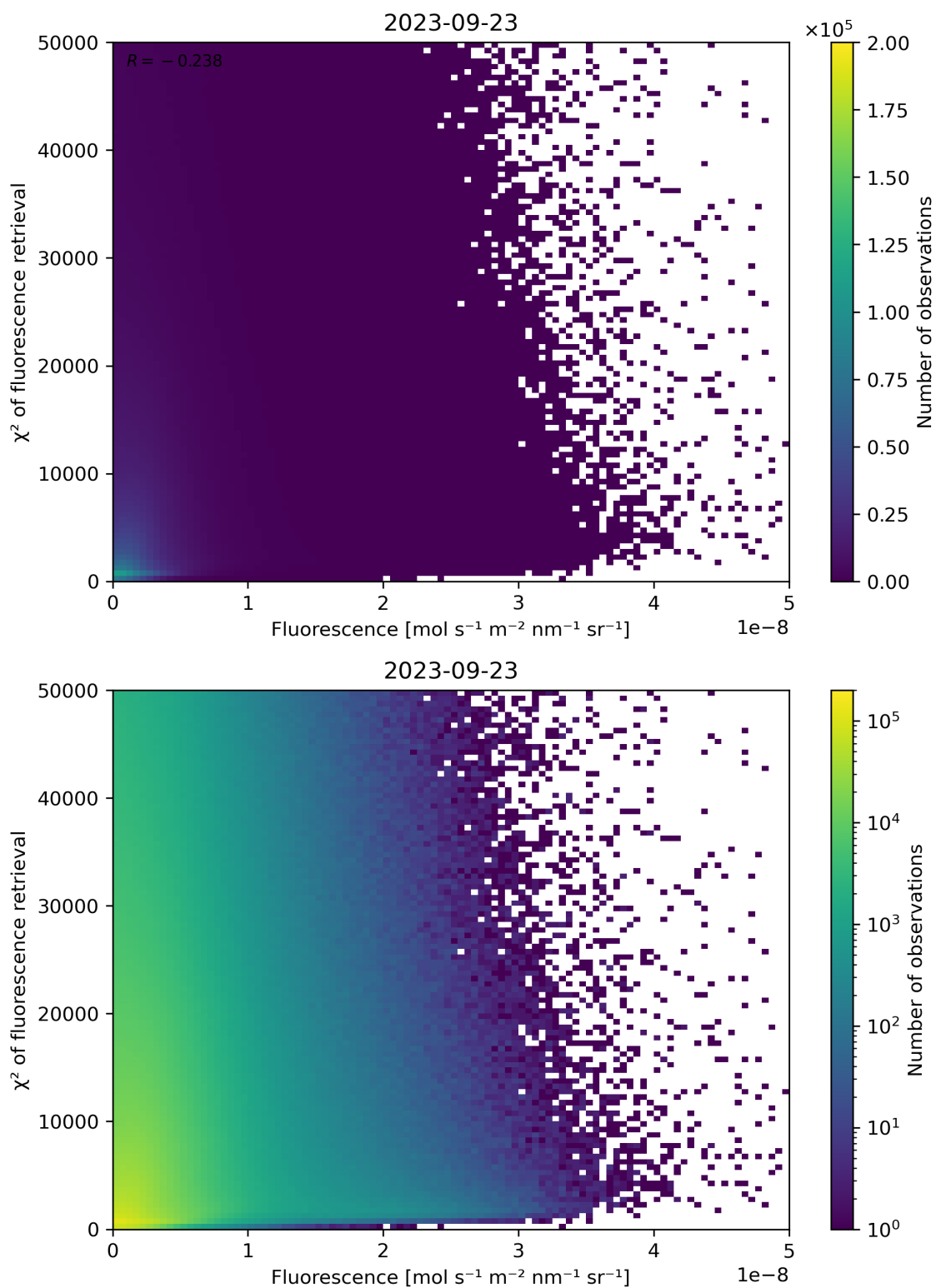
Figure 93: Scatter density plot of “Fluorescence” against “ \chi^2 of fluorescence retrieval” for 2023-09-22 to 2023-09-24.
