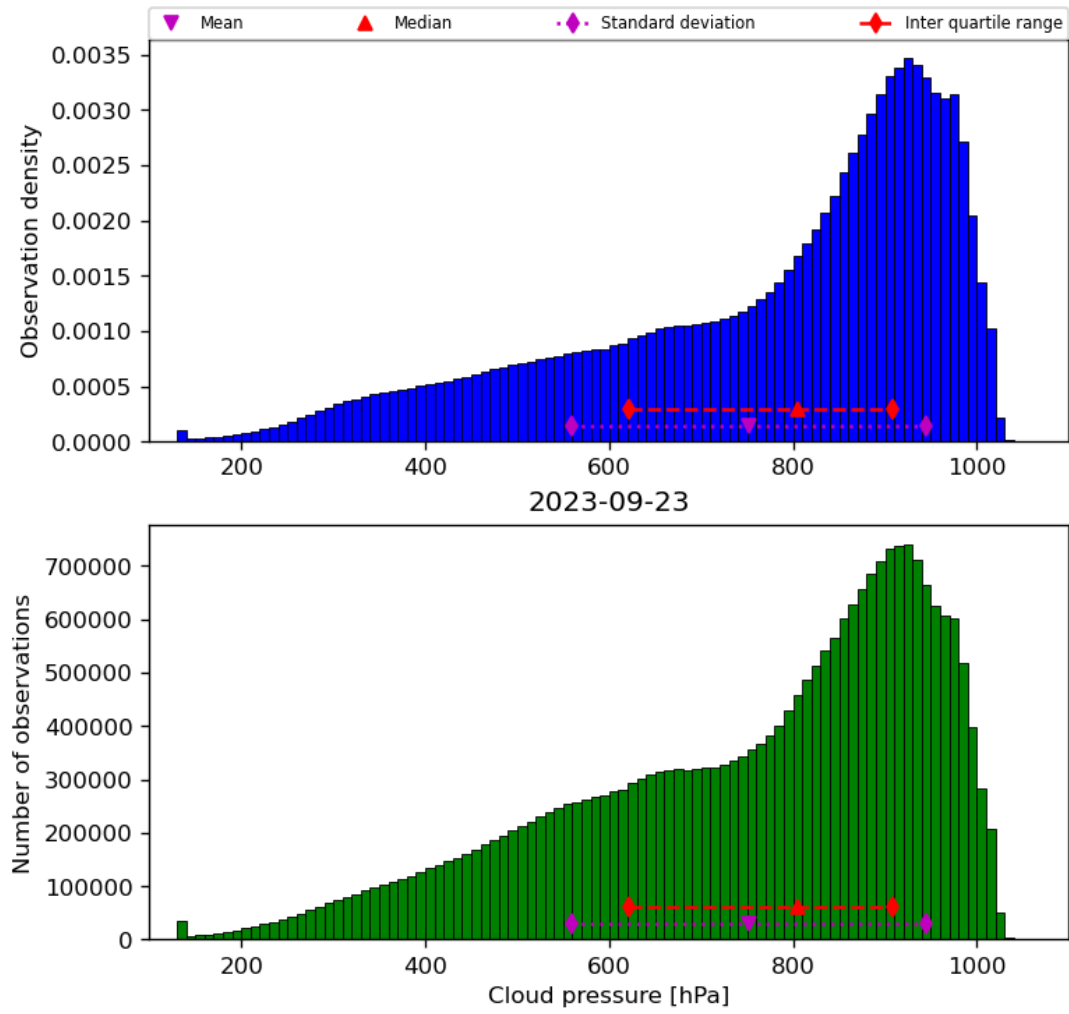
Figure 30: Histogram of “Cloud pressure” for 2023-09-22 to 2023-09-24
