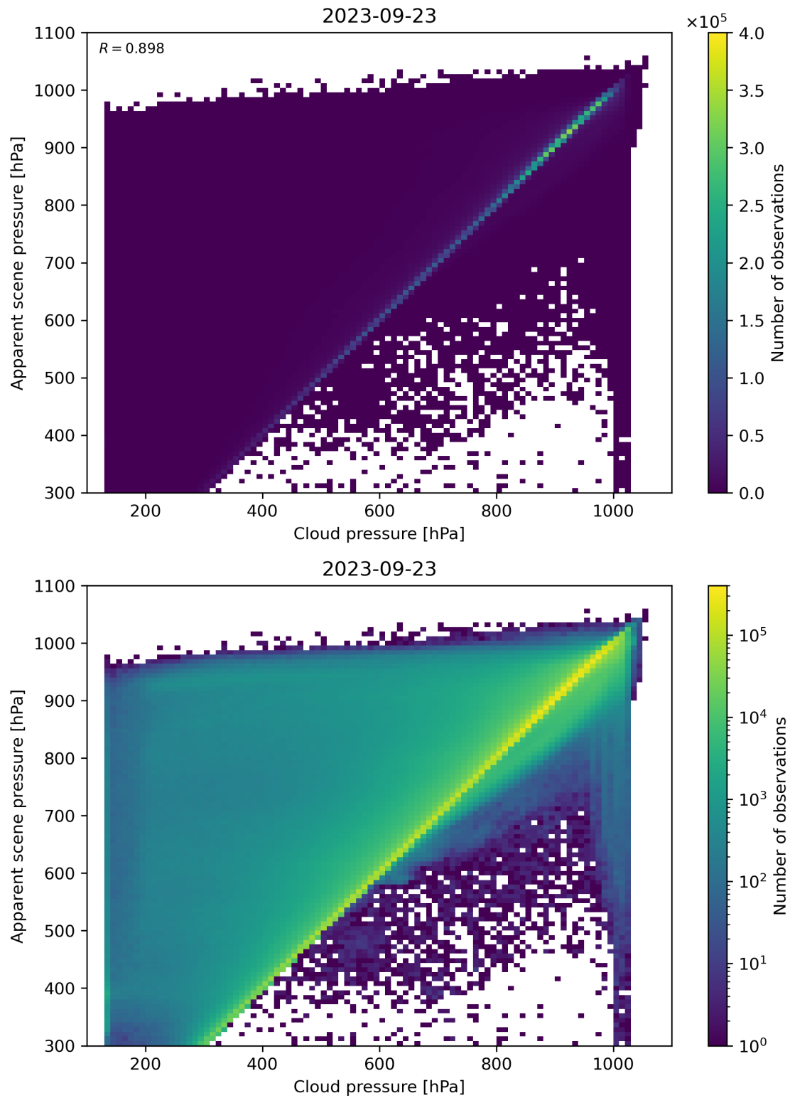
Figure 84: Scatter density plot of “Cloud pressure” against “Apparent scene pressure” for 2023-09-22 to 2023-09-24.
