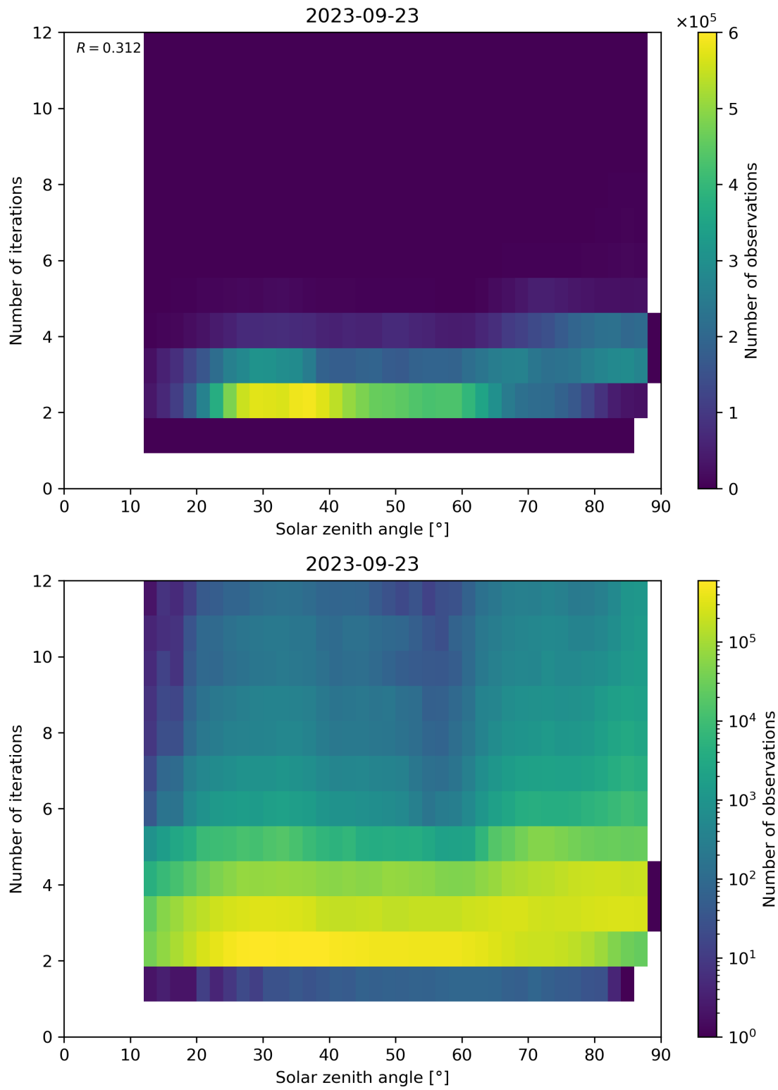
Figure 125: Scatter density plot of “Solar zenith angle” against “Number of iterations” for 2023-09-22 to 2023-09-24.
