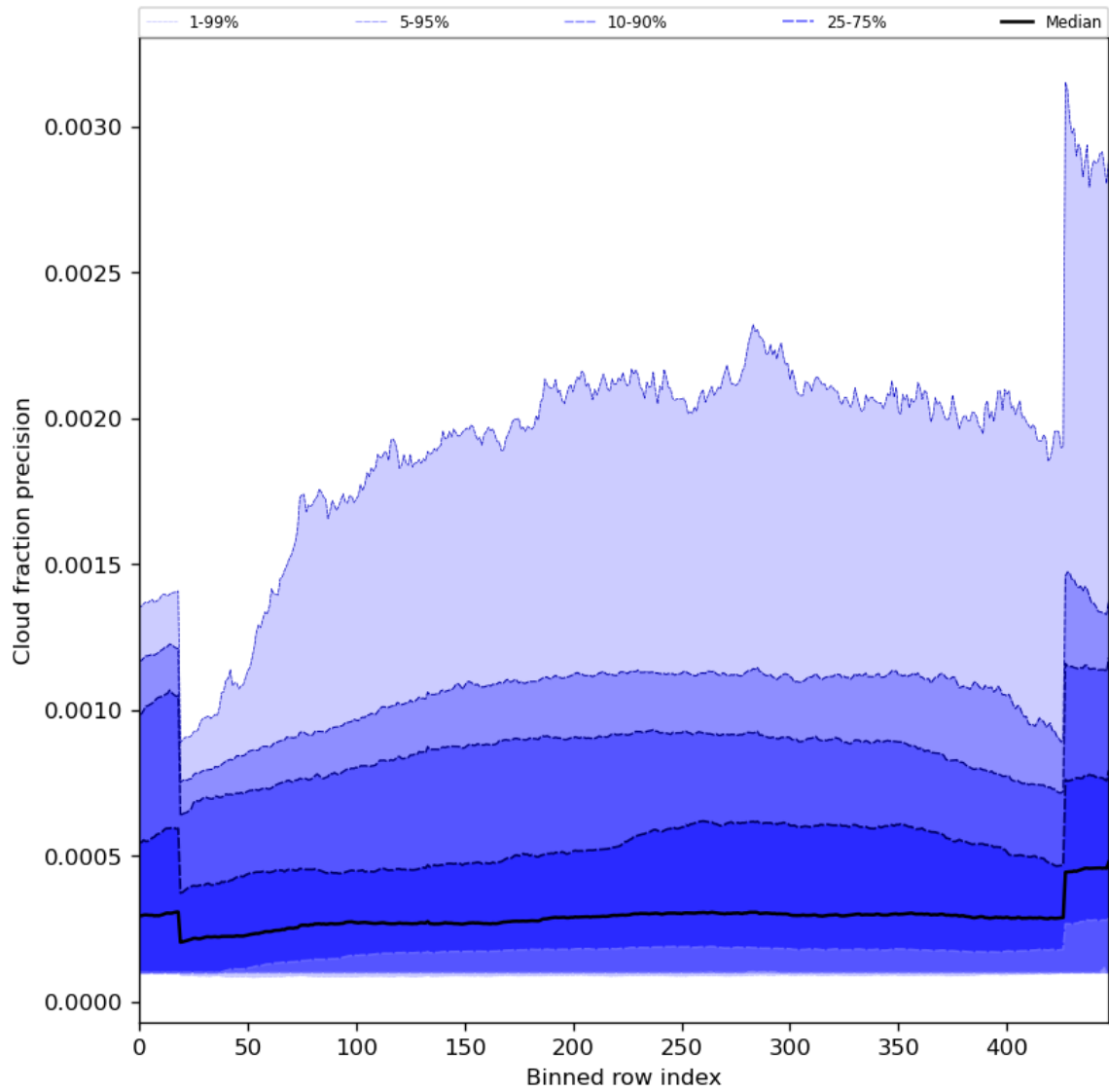
Figure 50: Along track statistics of “Cloud fraction precision” for 2023-09-22 to 2023-09-24
