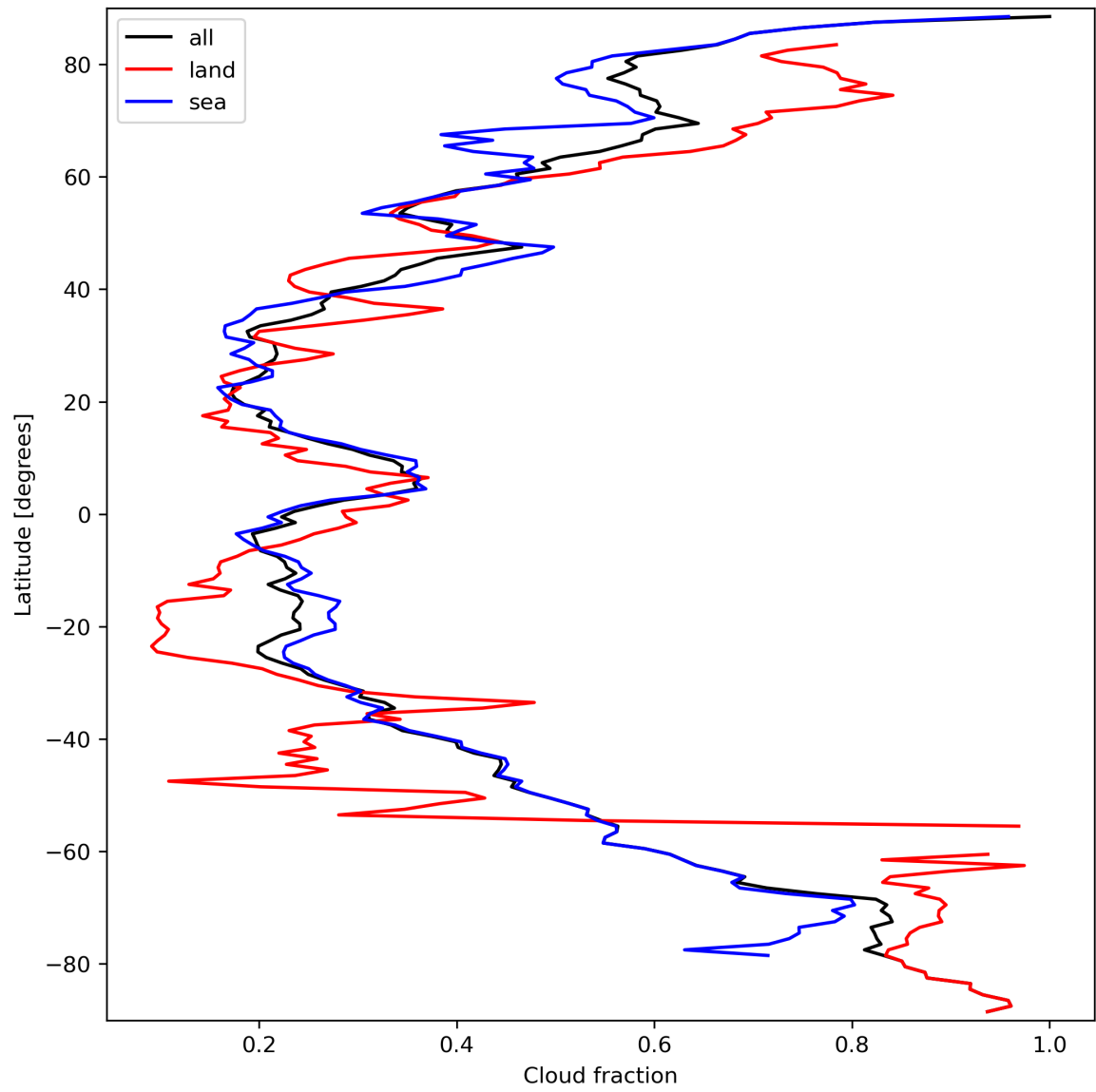
Figure 15: Zonal average of “Cloud fraction” for 2023-09-22 to 2023-09-24.
