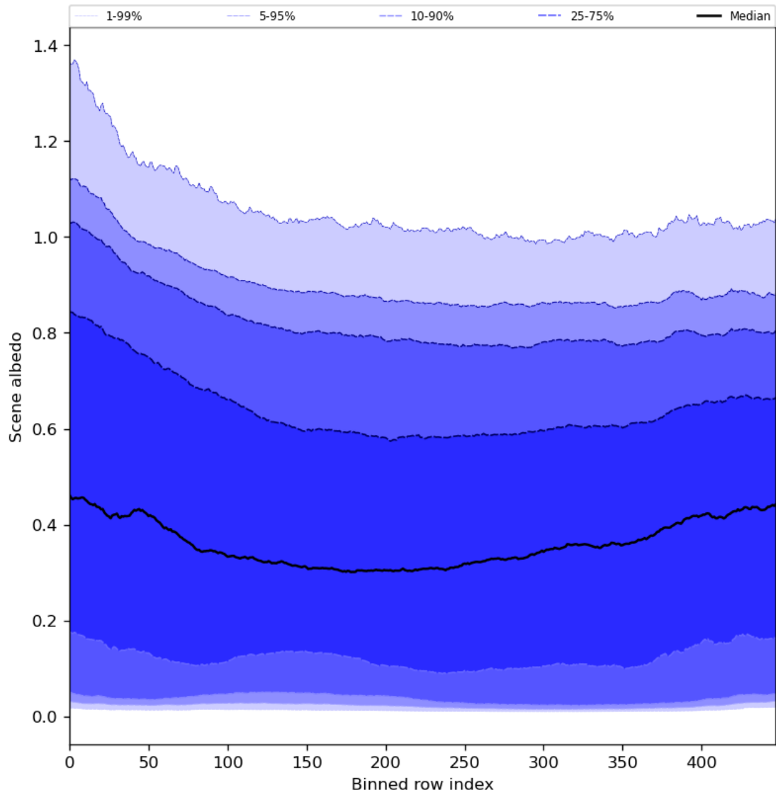
Figure 51: Along track statistics of “Scene albedo” for 2023-09-22 to 2023-09-24
