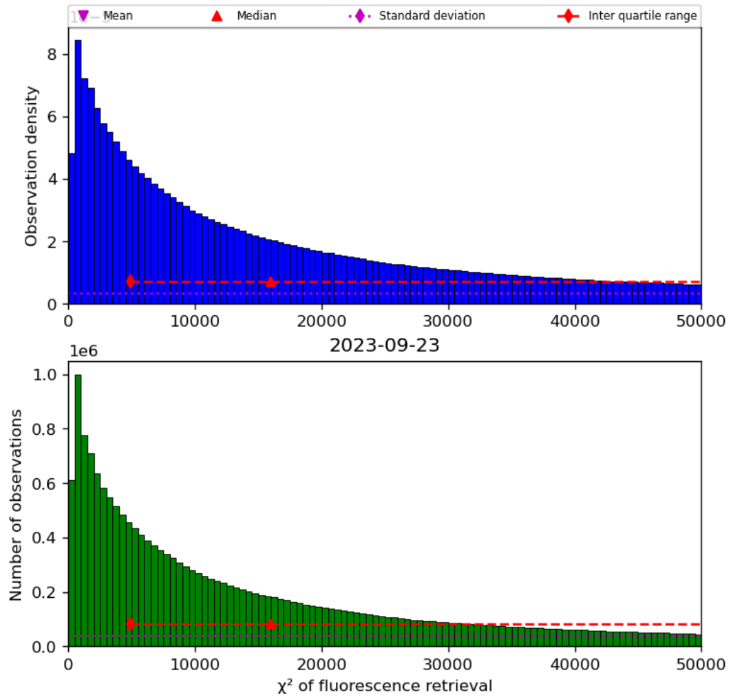
Figure 42: Histogram of “ \chi^2 of fluorescence retrieval” for 2023-09-22 to 2023-09-24
