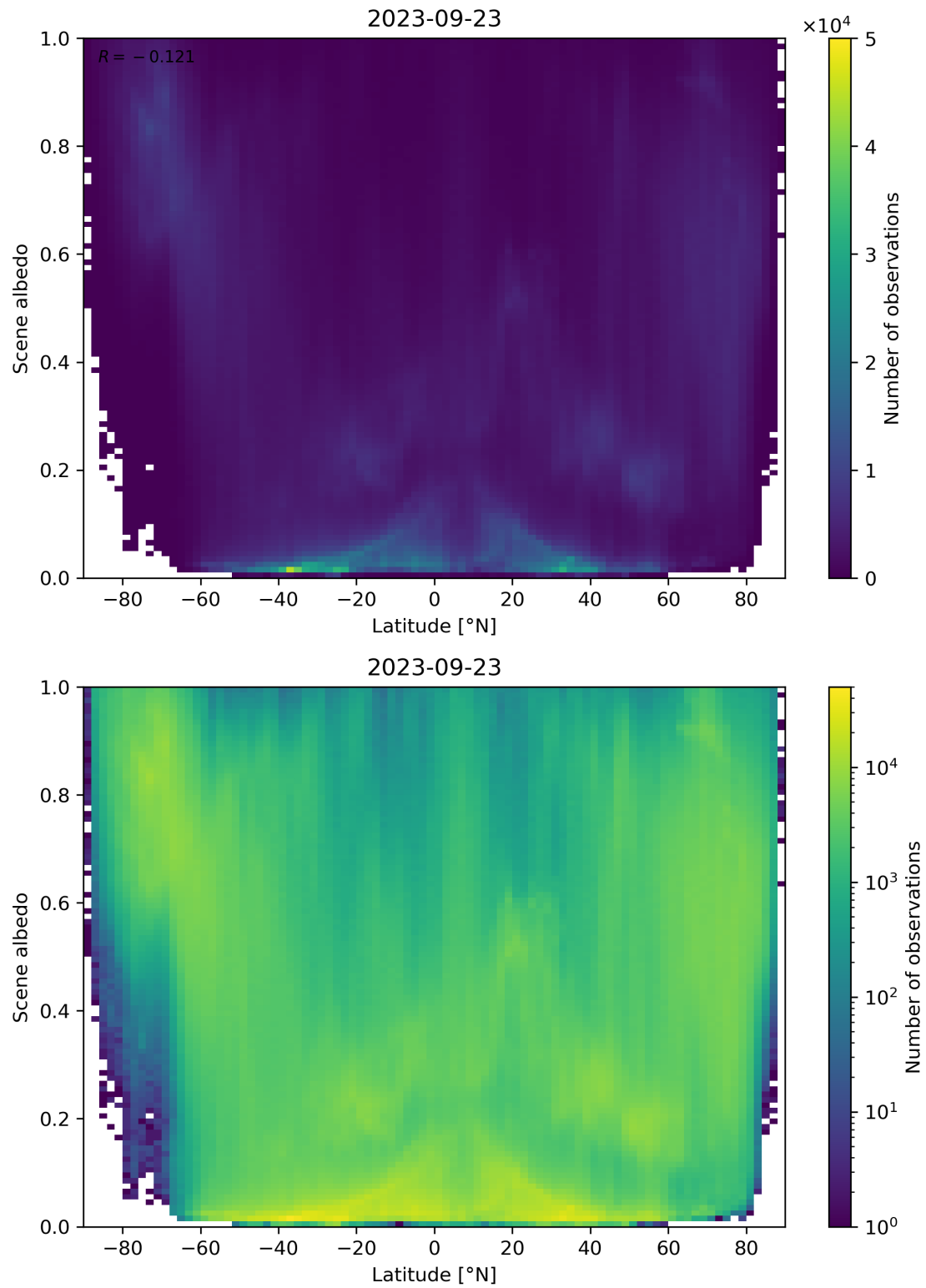
Figure 104: Scatter density plot of “Latitude” against “Scene albedo” for 2023-09-22 to 2023-09-24.
