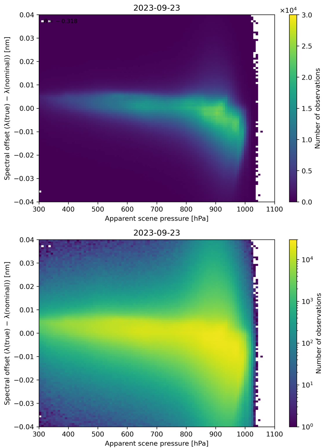
Figure 68: Scatter density plot of “Apparent scene pressure” against “Spectral offset ( \lambda(\text{true}) - \lambda(\text{nominal}) )” for 2023-09-22 to 2023-09-24.
