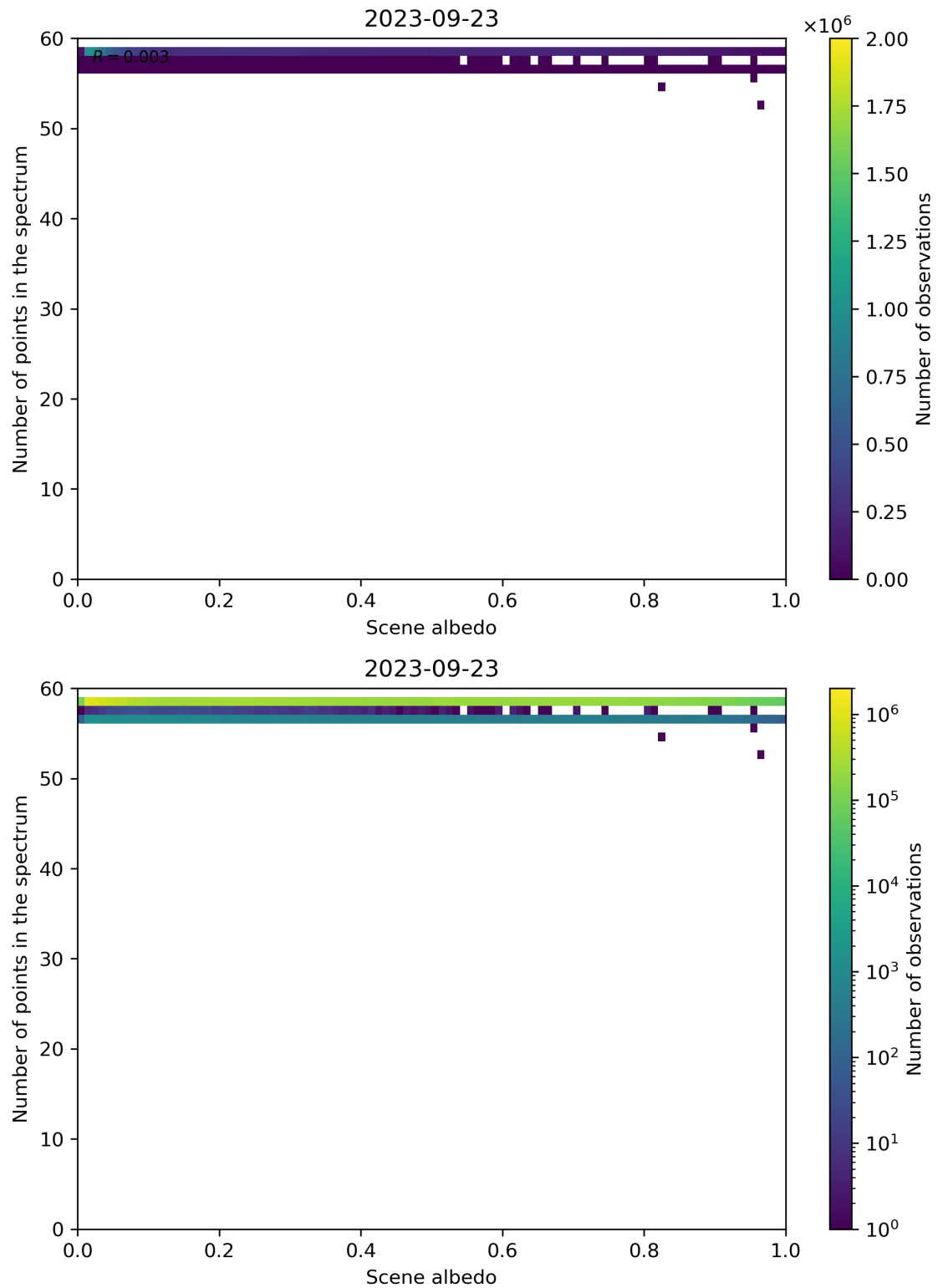
Figure 116: Scatter density plot of “Scene albedo” against “Number of points in the spectrum” for 2023-09-22 to 2023-09-24.
