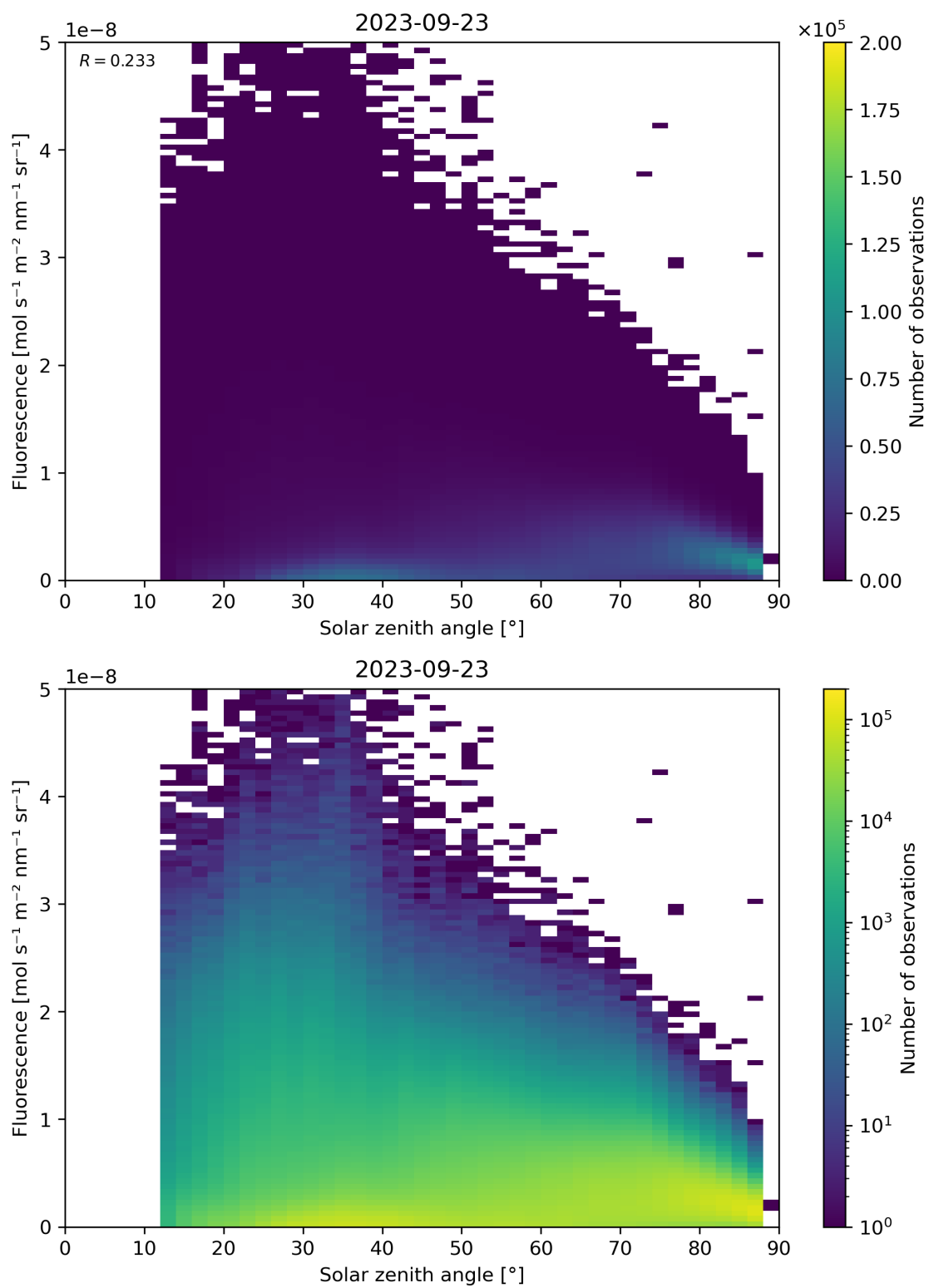
Figure 123: Scatter density plot of “Solar zenith angle” against “Fluorescence” for 2023-09-22 to 2023-09-24.
