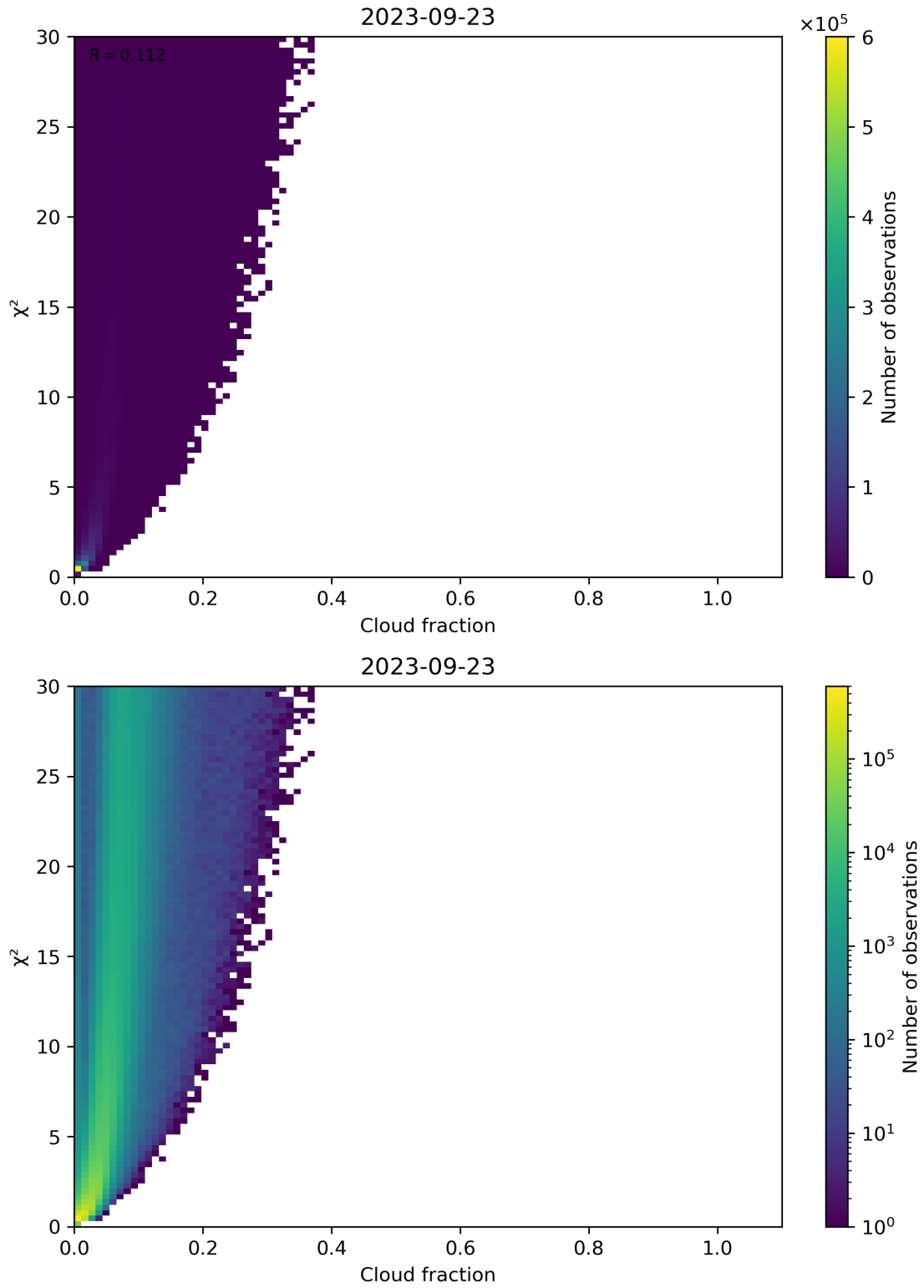
Figure 77: Scatter density plot of “Cloud fraction” against “ \chi^2 ” for 2023-09-22 to 2023-09-24.
