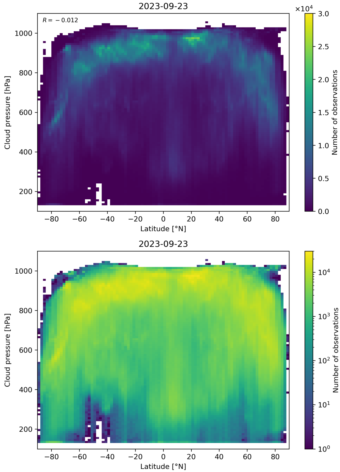
Figure 100: Scatter density plot of “Latitude” against “Cloud pressure” for 2023-09-22 to 2023-09-24.
