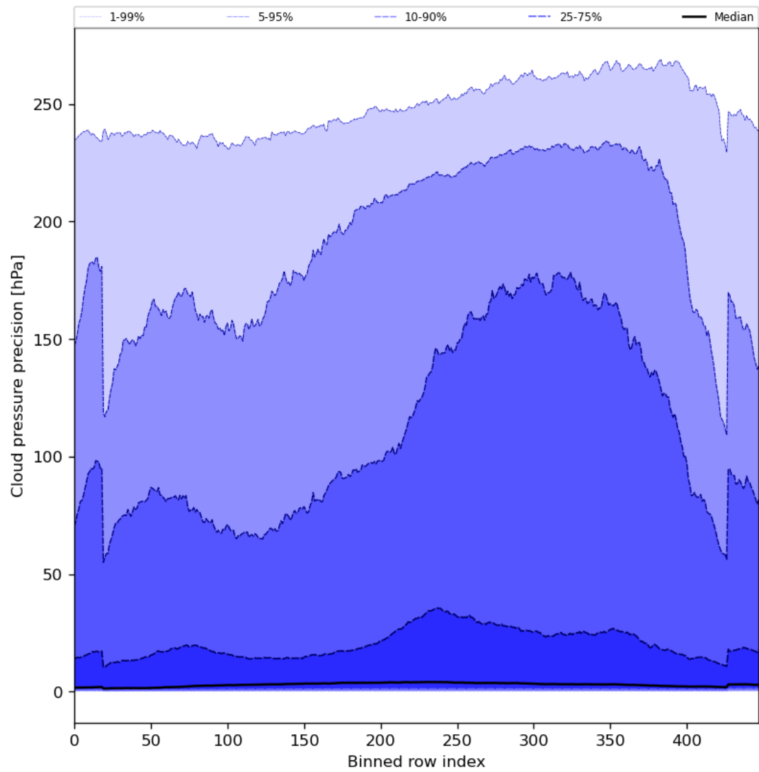
Figure 48: Along track statistics of “Cloud pressure precision” for 2023-09-22 to 2023-09-24
