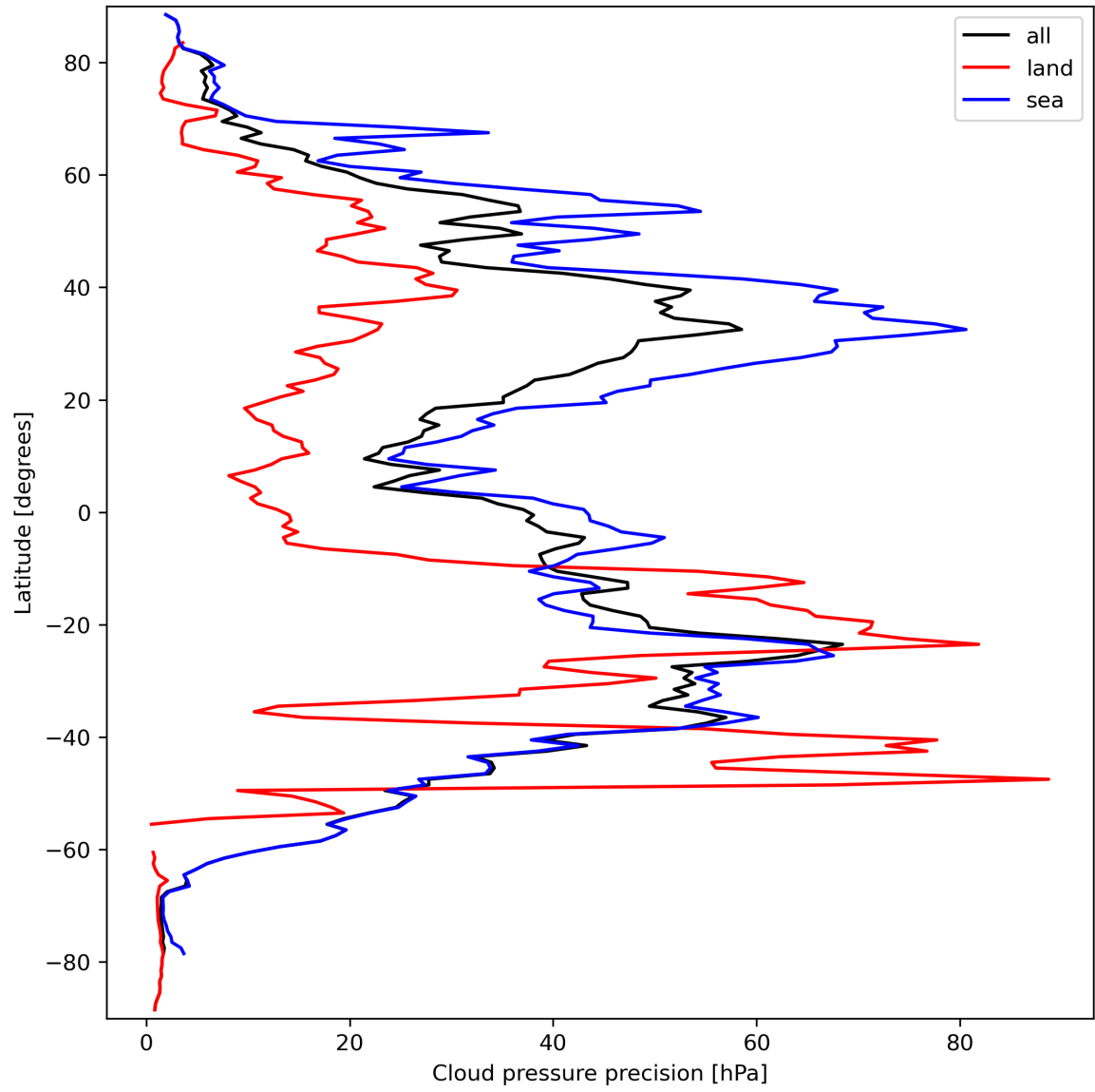
Figure 14: Zonal average of “Cloud pressure precision” for 2023-09-22 to 2023-09-24.
