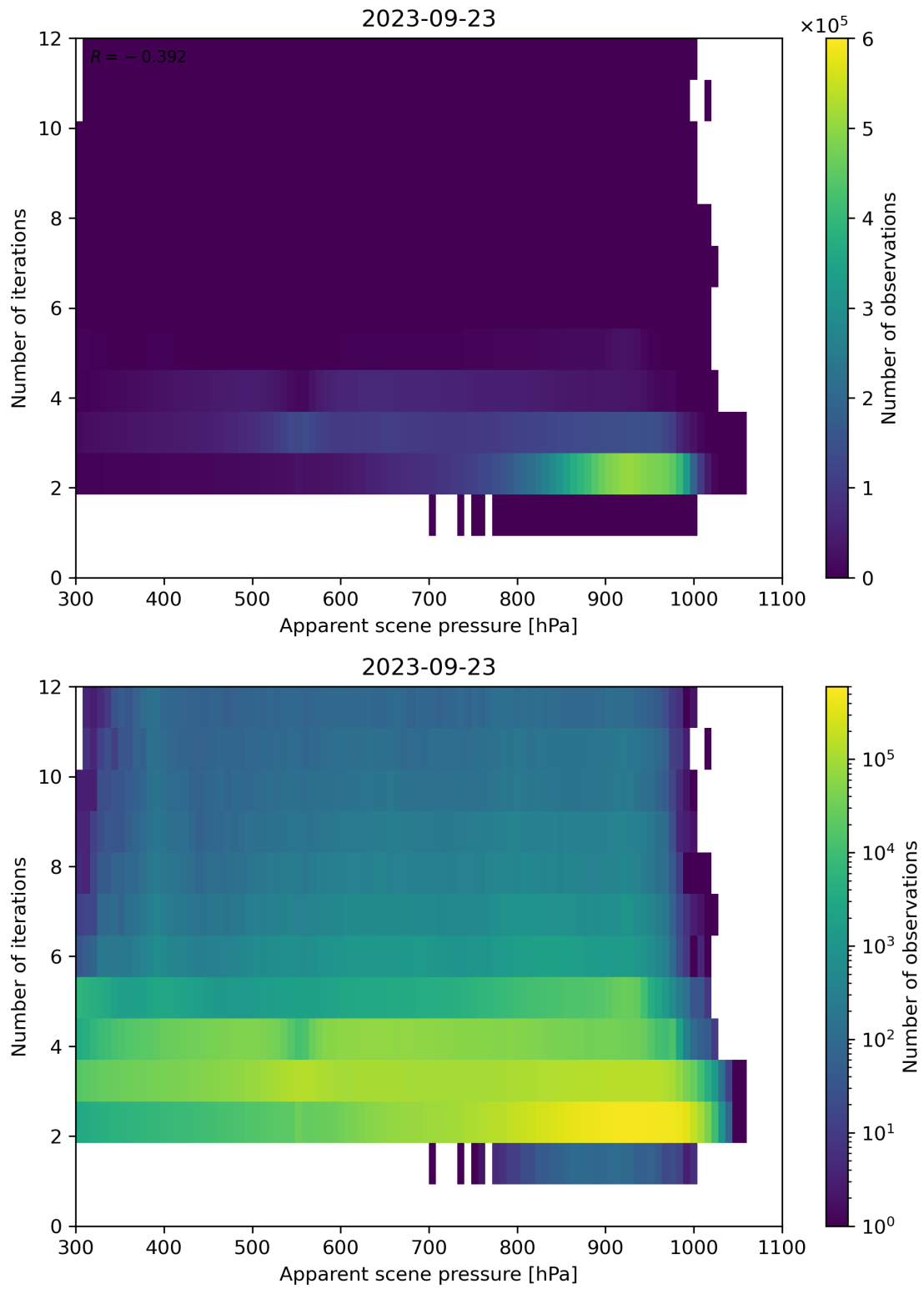
Figure 66: Scatter density plot of “Apparent scene pressure” against “Number of iterations” for 2023-09-22 to 2023-09-24.
