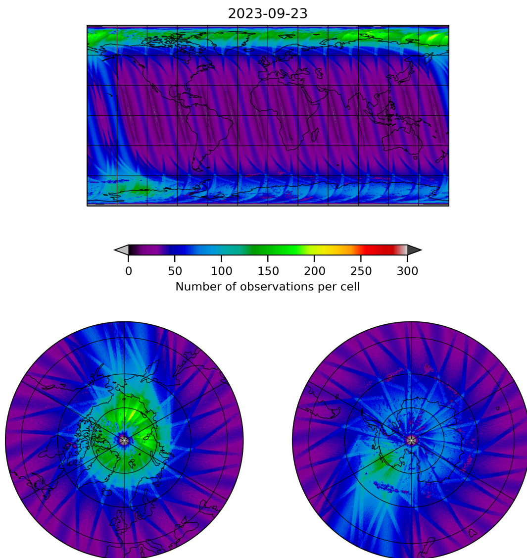
Figure 11: Map of the number of observations for 2023-09-22 to 2023-09-24
