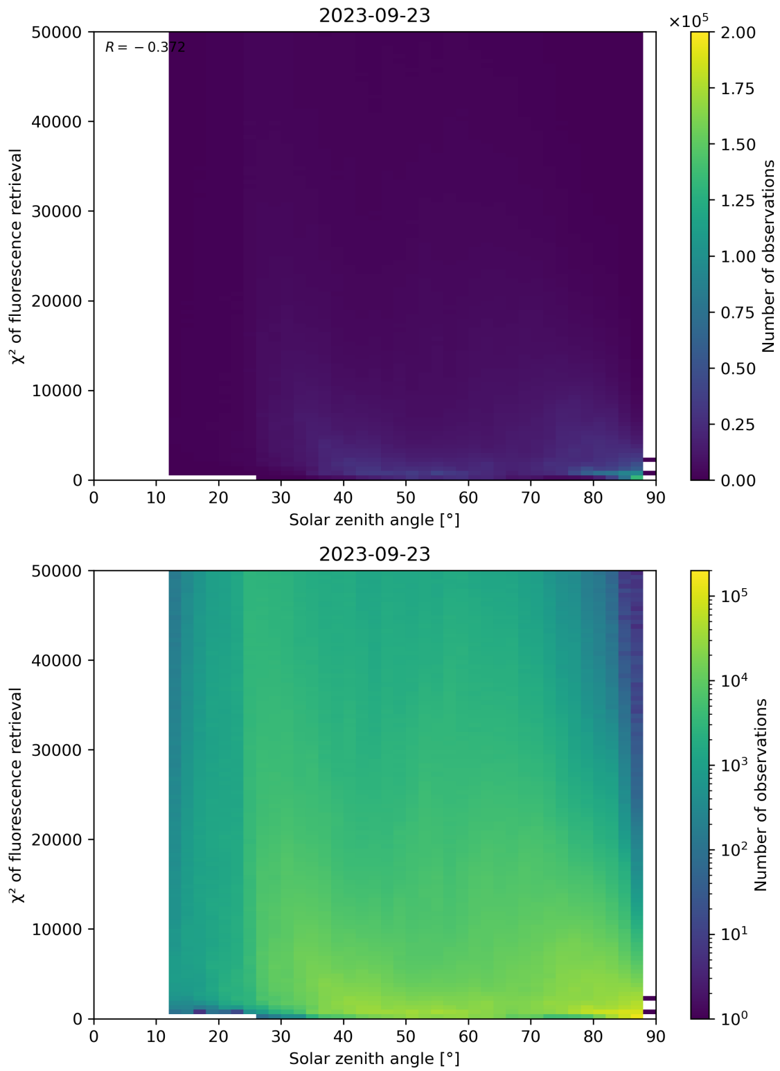
Figure 120: Scatter density plot of “Solar zenith angle” against “ \chi^2 of fluorescence retrieval” for 2023-09-22 to 2023-09-24.
