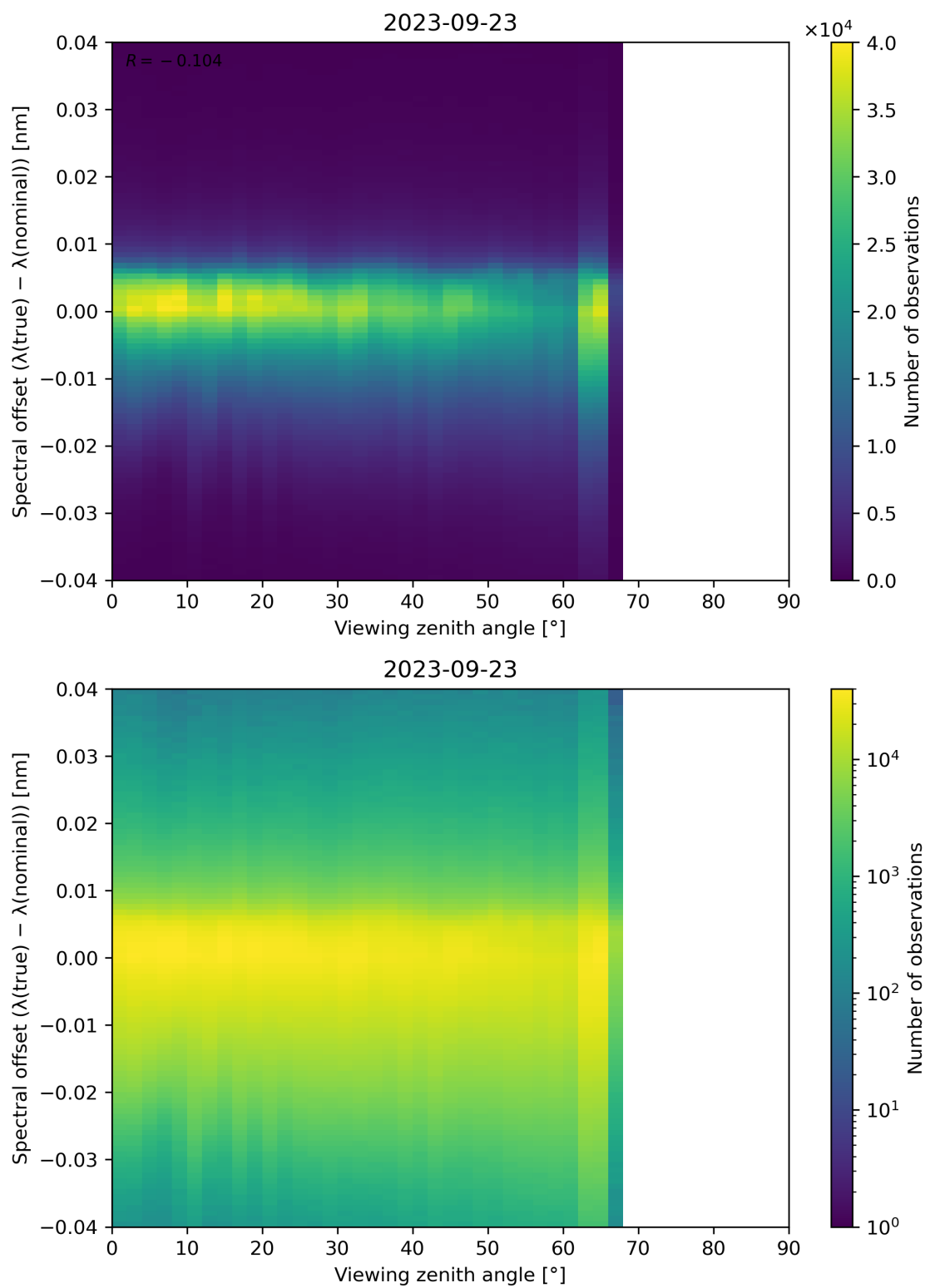
Figure 140: Scatter density plot of “Viewing zenith angle” against “Spectral offset ( \lambda(\text{true}) - \lambda(\text{nominal}) )” for 2023-09-22 to 2023-09-24.
