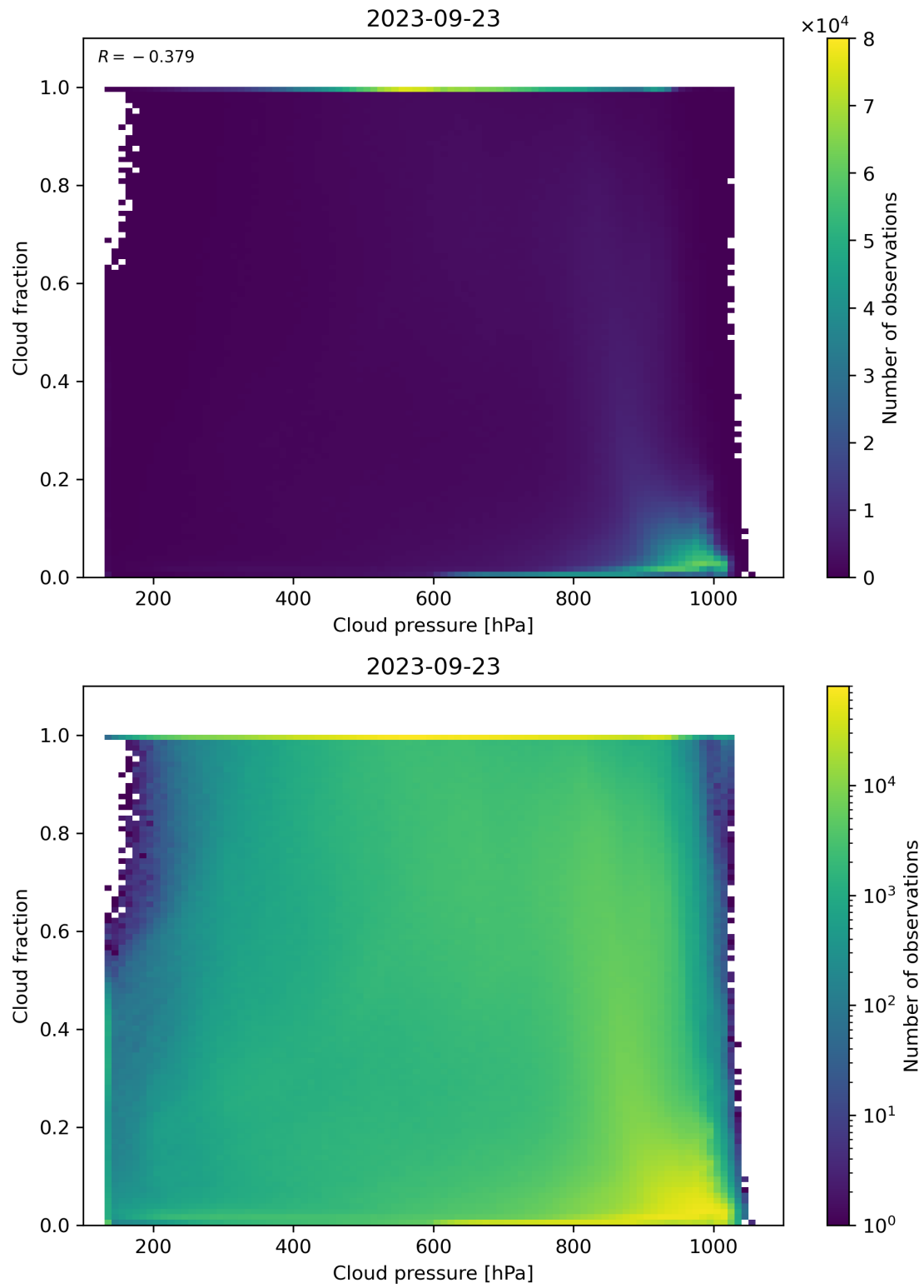
Figure 87: Scatter density plot of “Cloud pressure” against “Cloud fraction” for 2023-09-22 to 2023-09-24.
