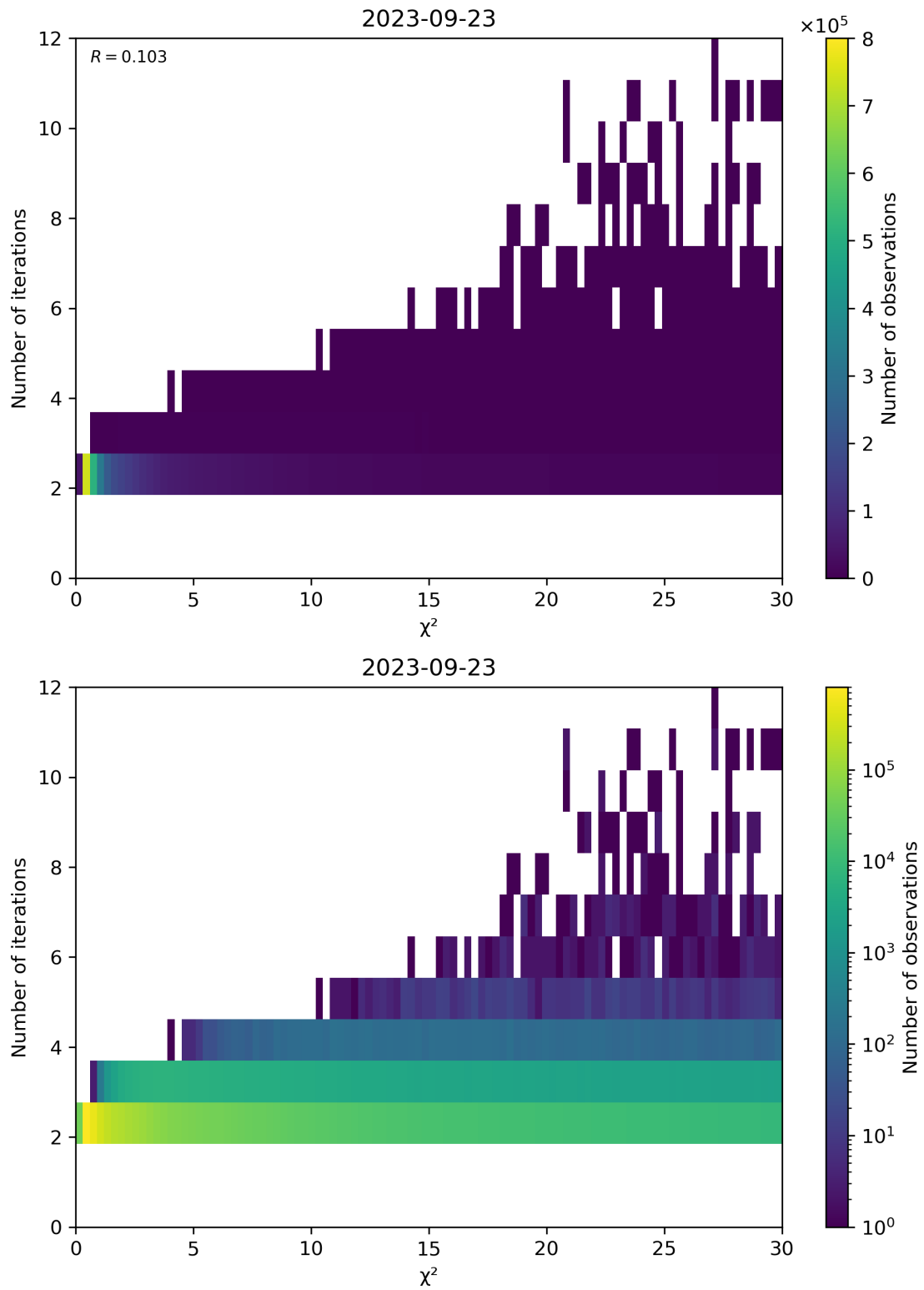
Figure 73: Scatter density plot of “ \chi^2 ” against “Number of iterations” for 2023-09-22 to 2023-09-24.
