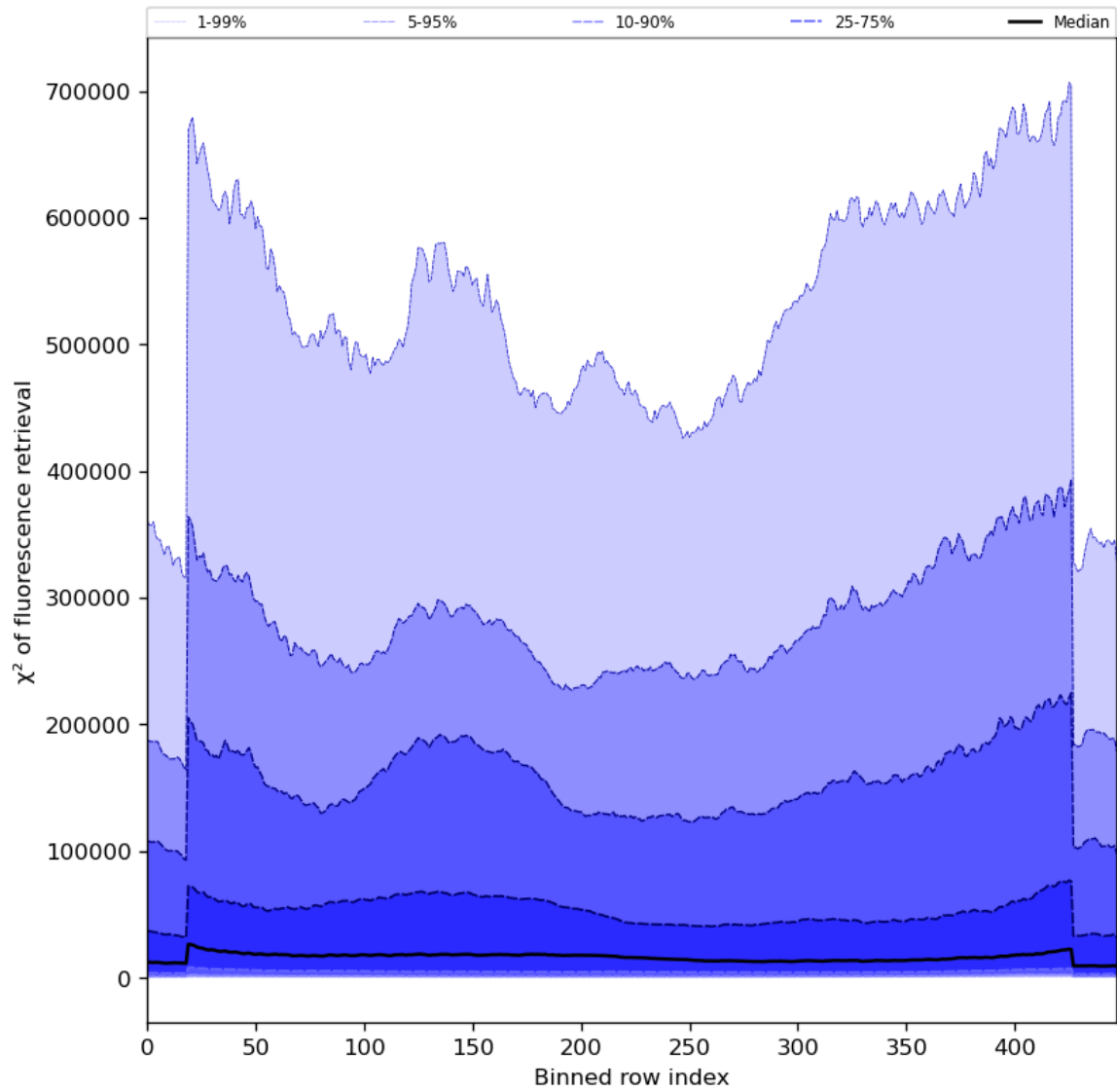
Figure 59: Along track statistics of “ \chi^2 of fluorescence retrieval” for 2023-09-22 to 2023-09-24
