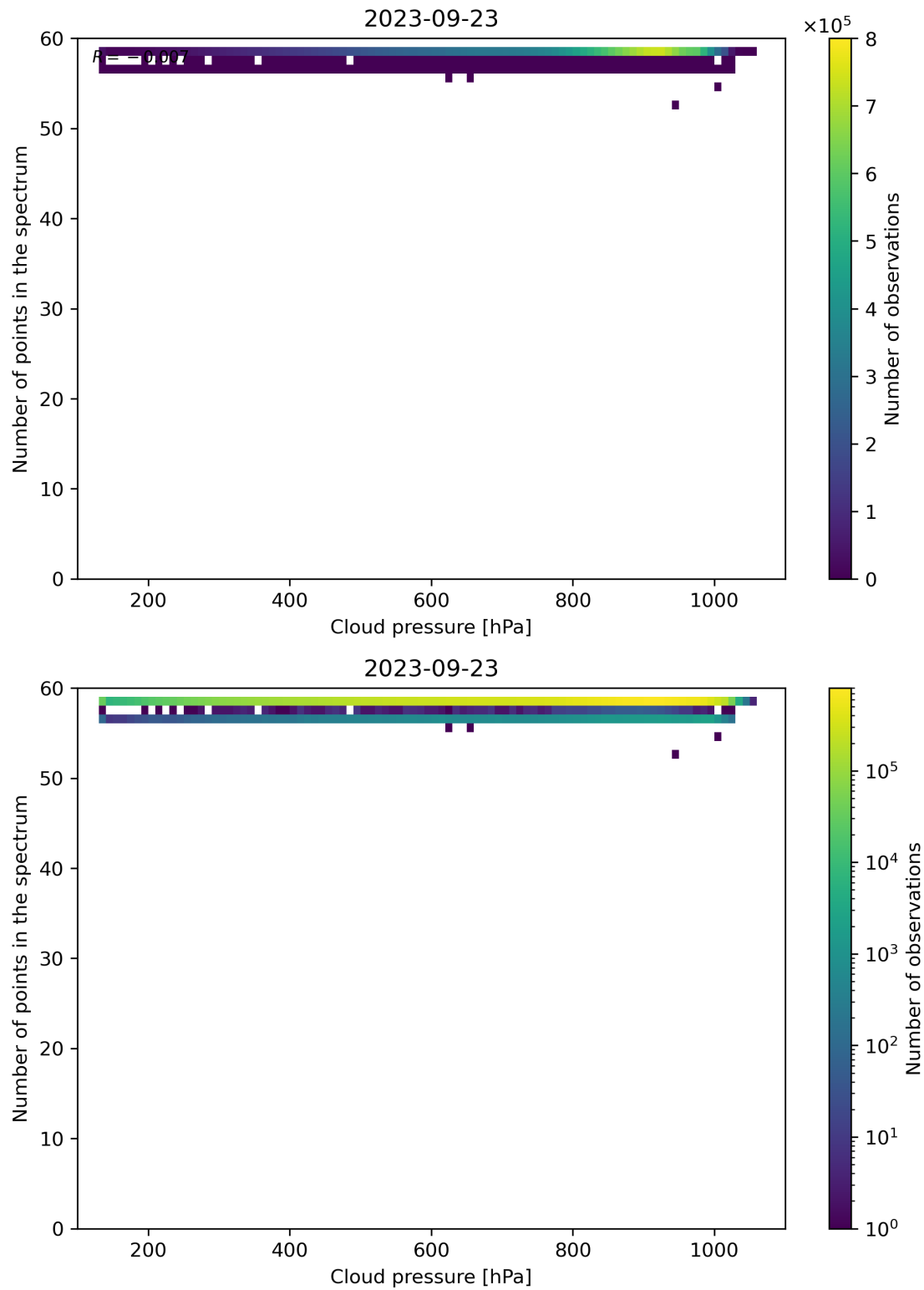
Figure 90: Scatter density plot of “Cloud pressure” against “Number of points in the spectrum” for 2023-09-22 to 2023-09-24.
