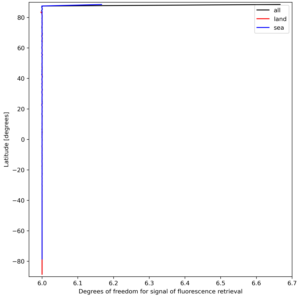
Figure 26: Zonal average of “Degrees of freedom for signal of fluorescence retrieval” for 2023-09-22 to 2023-09-24.
