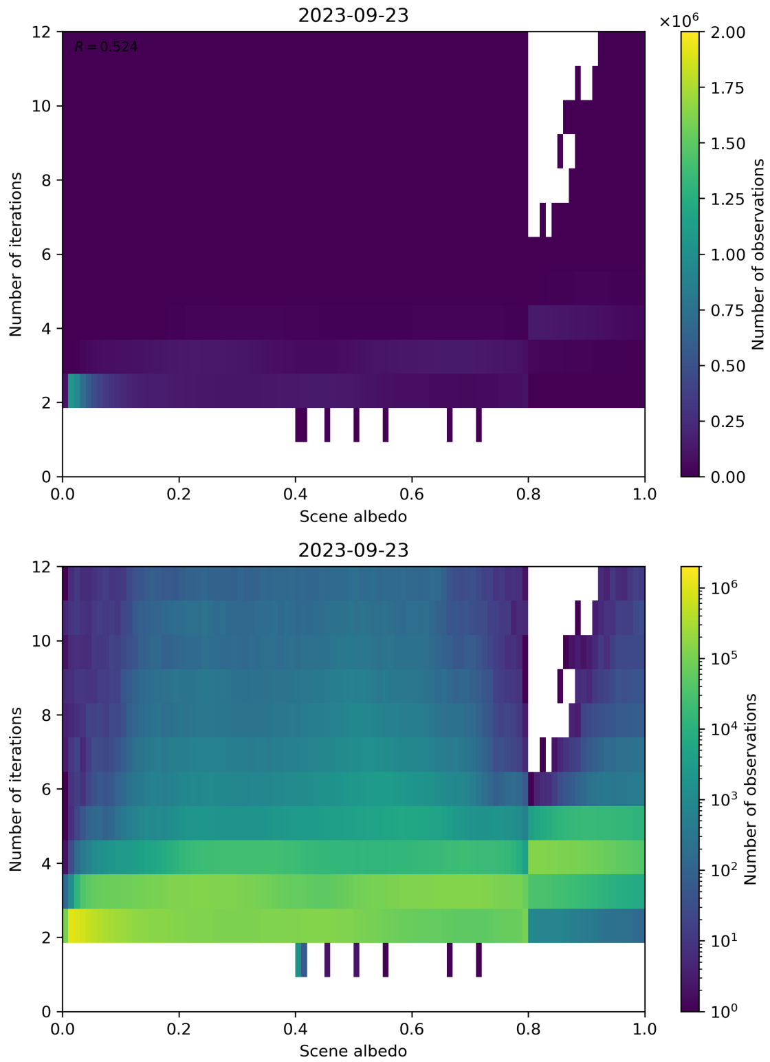
Figure 115: Scatter density plot of “Scene albedo” against “Number of iterations” for 2023-09-22 to 2023-09-24.
