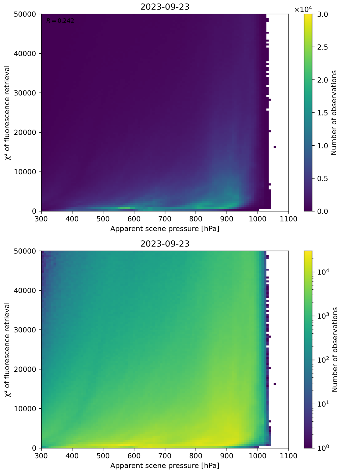
Figure 64: Scatter density plot of “Apparent scene pressure” against “ \chi^2 of fluorescence retrieval” for 2023-09-22 to 2023-09-24.
