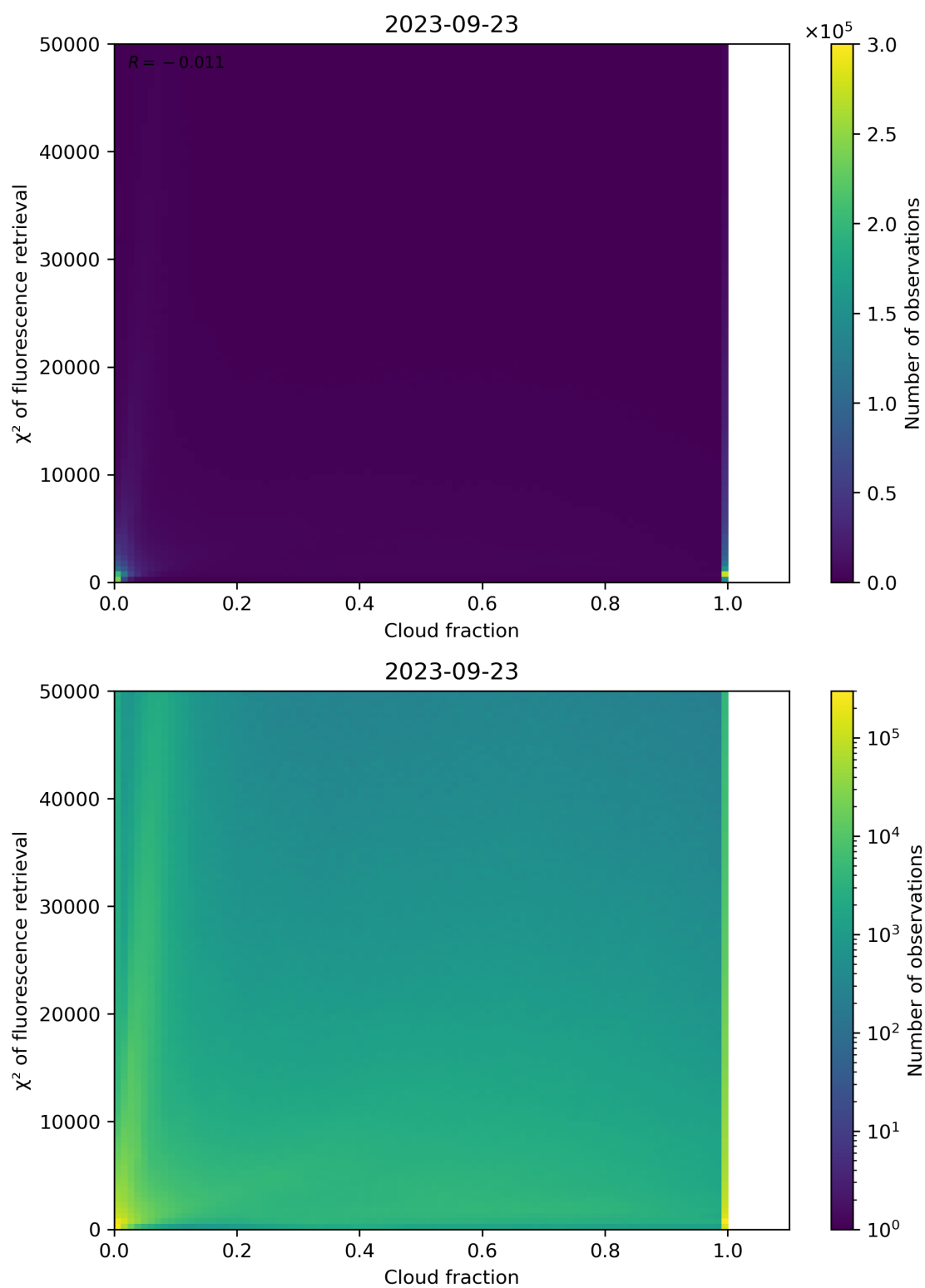
Figure 78: Scatter density plot of “Cloud fraction” against “ \chi^2 of fluorescence retrieval” for 2023-09-22 to 2023-09-24.
