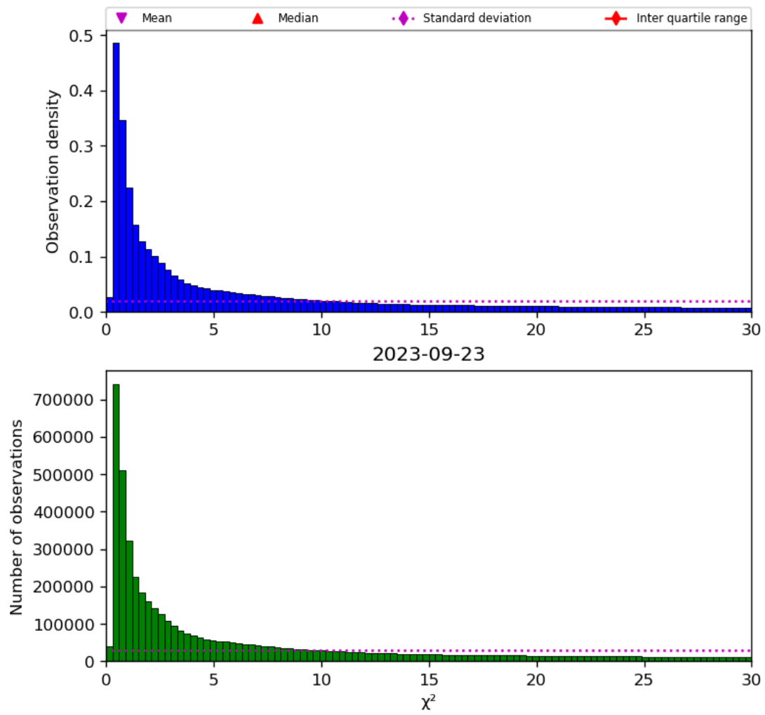
Figure 38: Histogram of " \chi^2 " for 2023-09-22 to 2023-09-24
