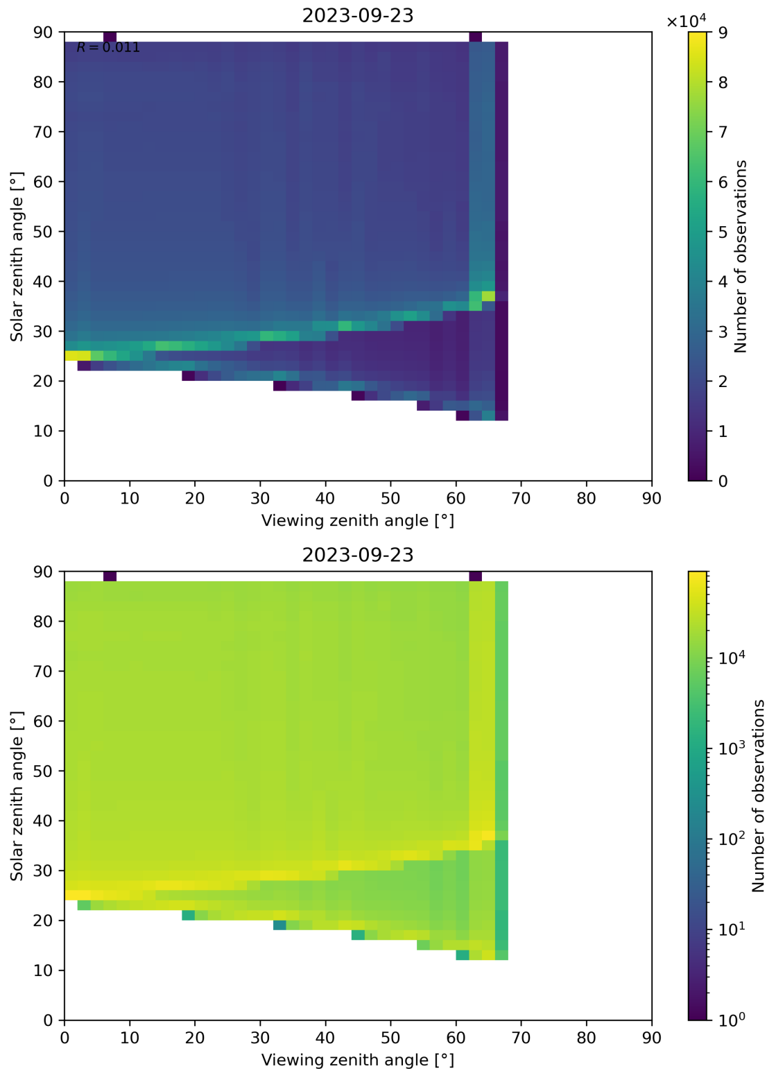
Figure 139: Scatter density plot of “Viewing zenith angle” against “Solar zenith angle” for 2023-09-22 to 2023-09-24.
