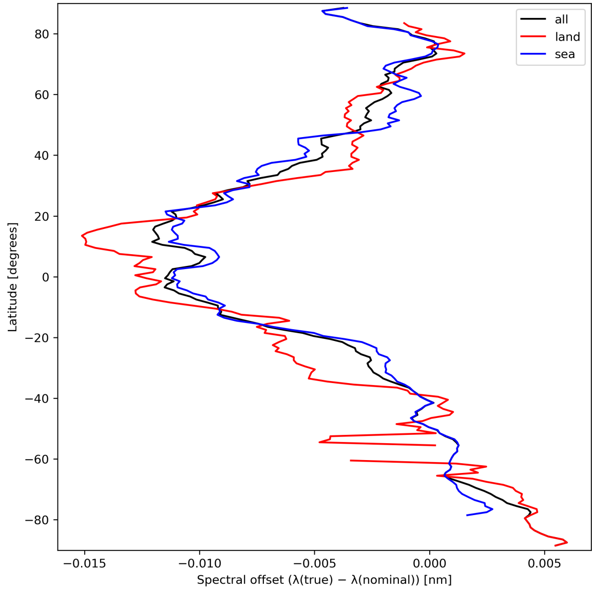
Figure 28: Zonal average of “Spectral offset ( \lambda(\text{true}) - \lambda(\text{nominal}) )” for 2023-09-22 to 2023-09-24.
