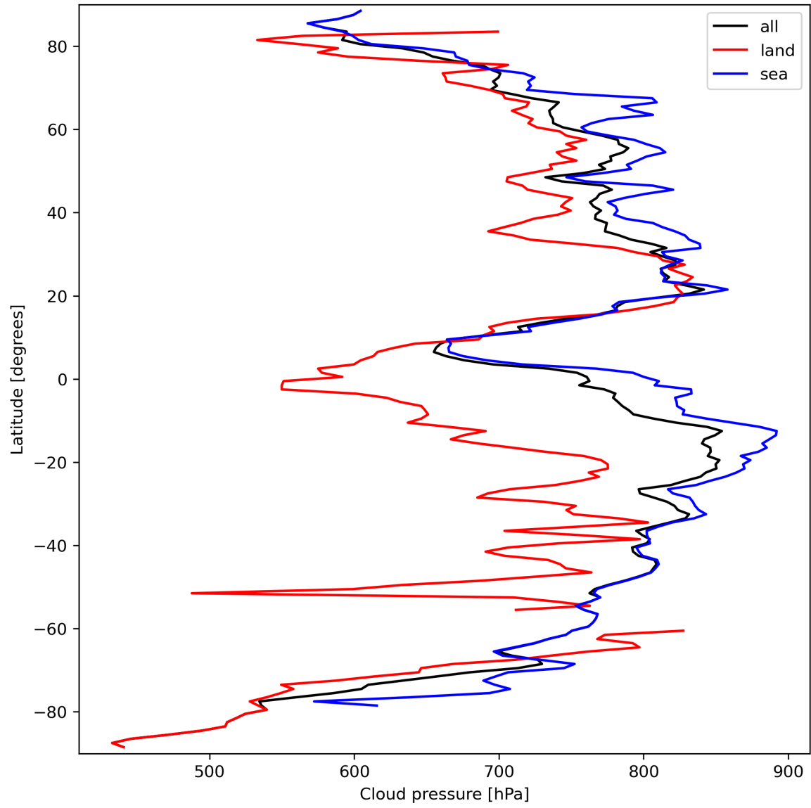
Figure 13: Zonal average of “Cloud pressure” for 2023-09-22 to 2023-09-24.
