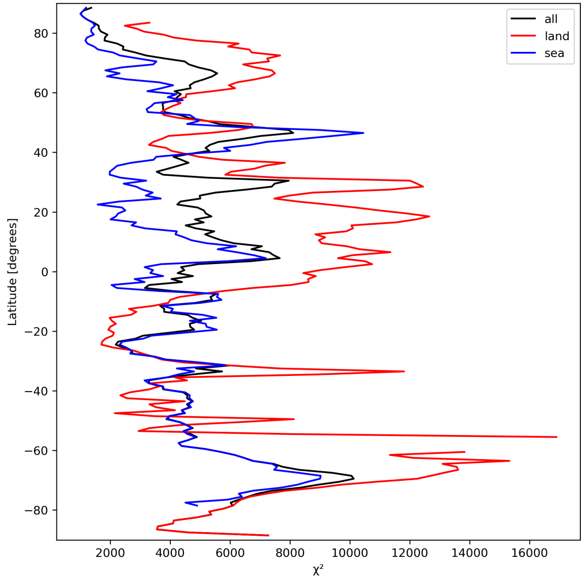
Figure 21: Zonal average of “ \chi^2 ” for 2023-09-22 to 2023-09-24.
