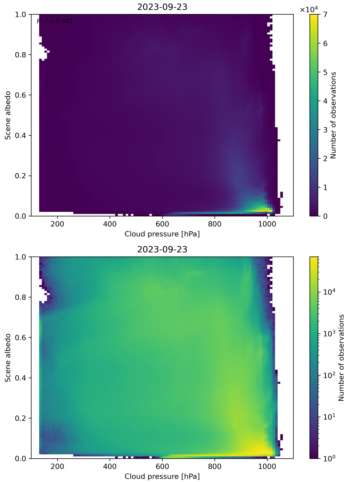
Figure 91: Scatter density plot of “Cloud pressure” against “Scene albedo” for 2023-09-22 to 2023-09-24.
