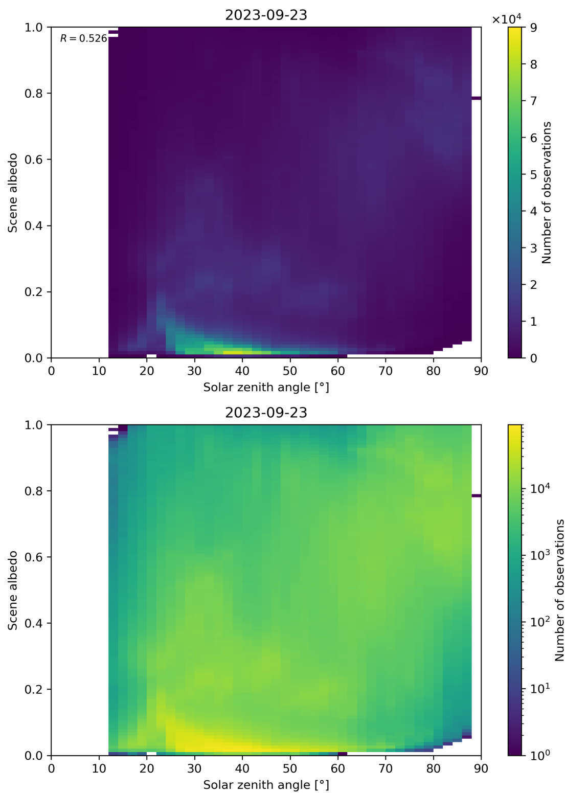
Figure 127: Scatter density plot of “Solar zenith angle” against “Scene albedo” for 2023-09-22 to 2023-09-24.
