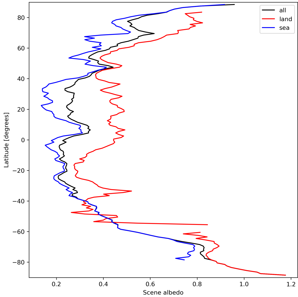
Figure 17: Zonal average of “Scene albedo” for 2023-09-22 to 2023-09-24.
