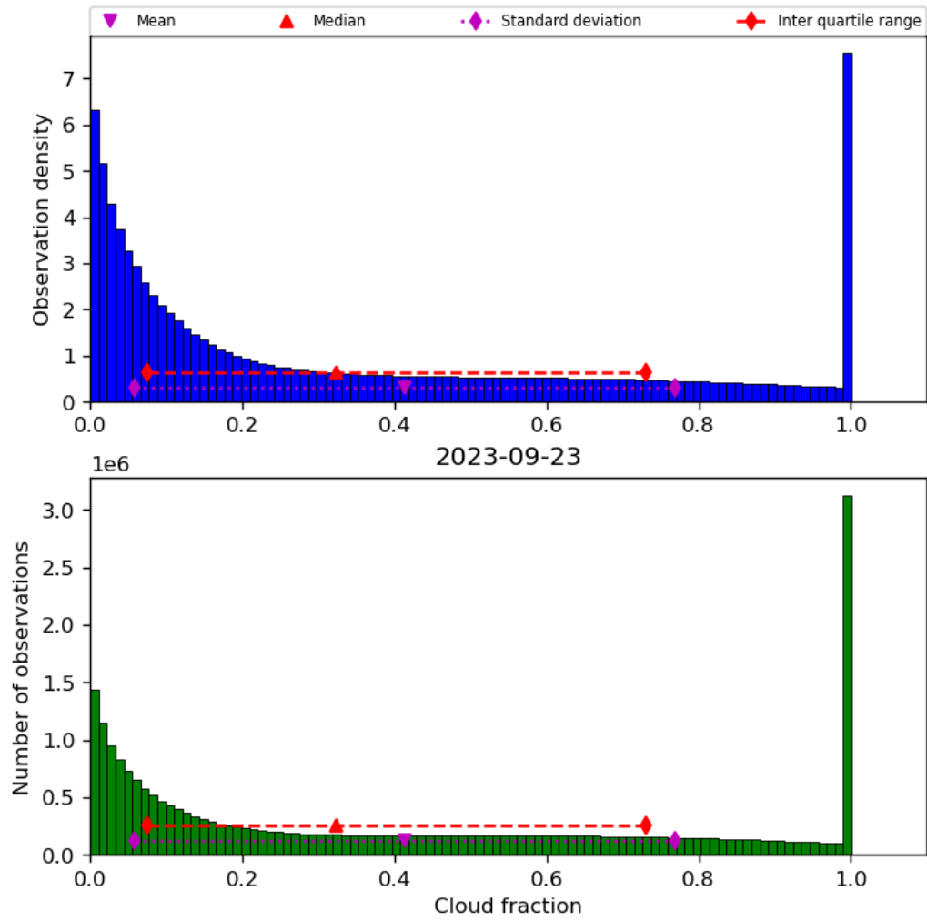
Figure 32: Histogram of “Cloud fraction” for 2023-09-22 to 2023-09-24
