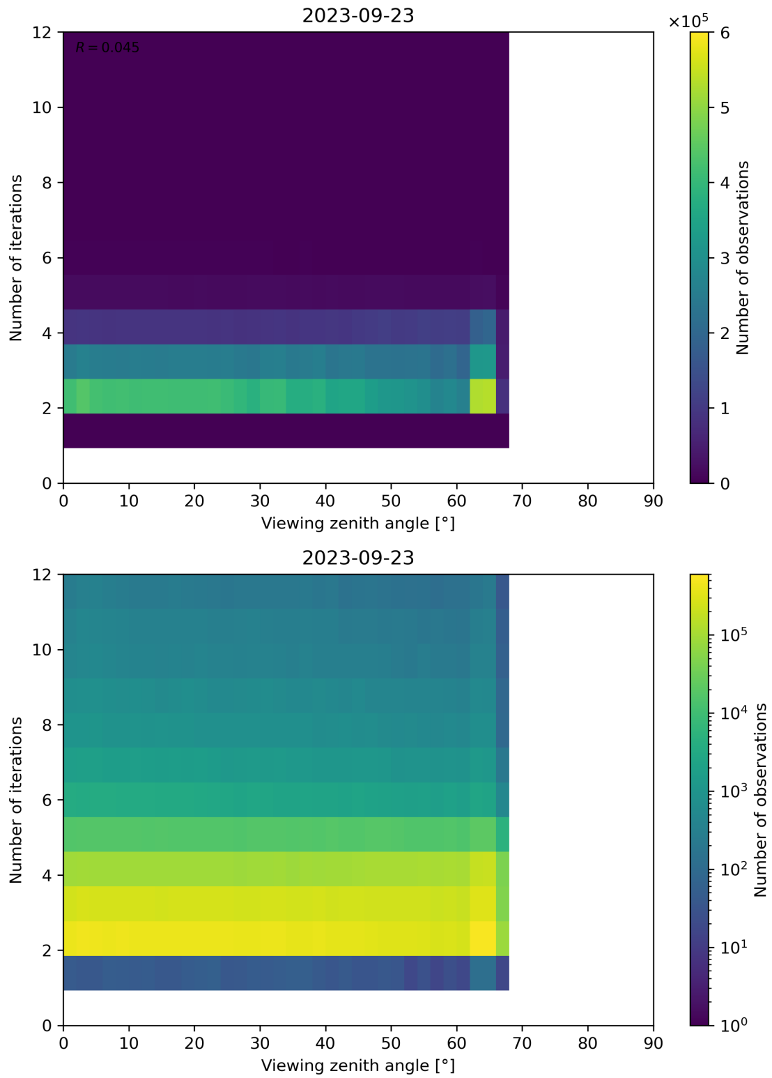
Figure 136: Scatter density plot of “Viewing zenith angle” against “Number of iterations” for 2023-09-22 to 2023-09-24.
