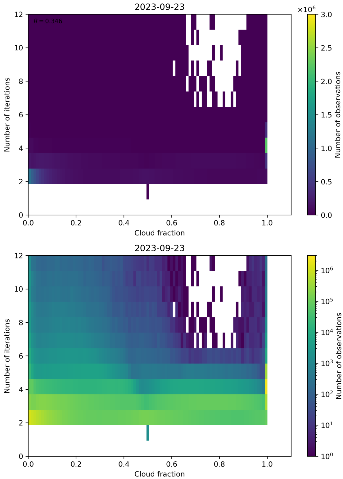
Figure 80: Scatter density plot of “Cloud fraction” against “Number of iterations” for 2023-09-22 to 2023-09-24.
