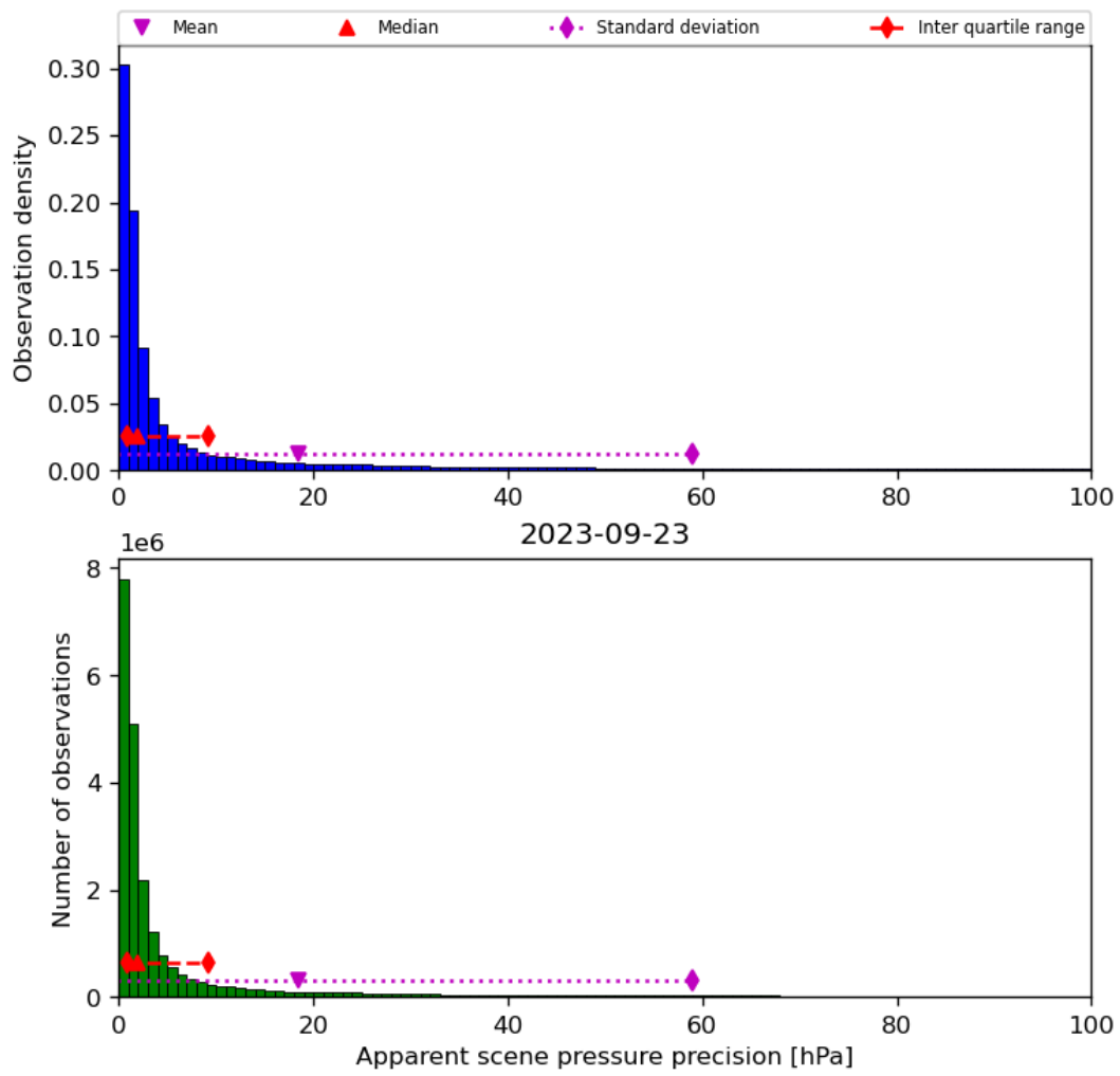
Figure 37: Histogram of “Apparent scene pressure precision” for 2023-09-22 to 2023-09-24
