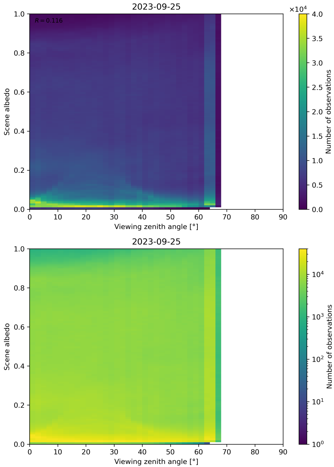
Figure 138: Scatter density plot of “Viewing zenith angle” against “Scene albedo” for 2023-09-24 to 2023-09-26.
