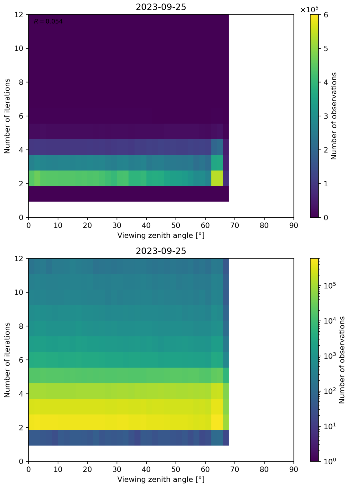
Figure 136: Scatter density plot of “Viewing zenith angle” against “Number of iterations” for 2023-09-24 to 2023-09-26.
