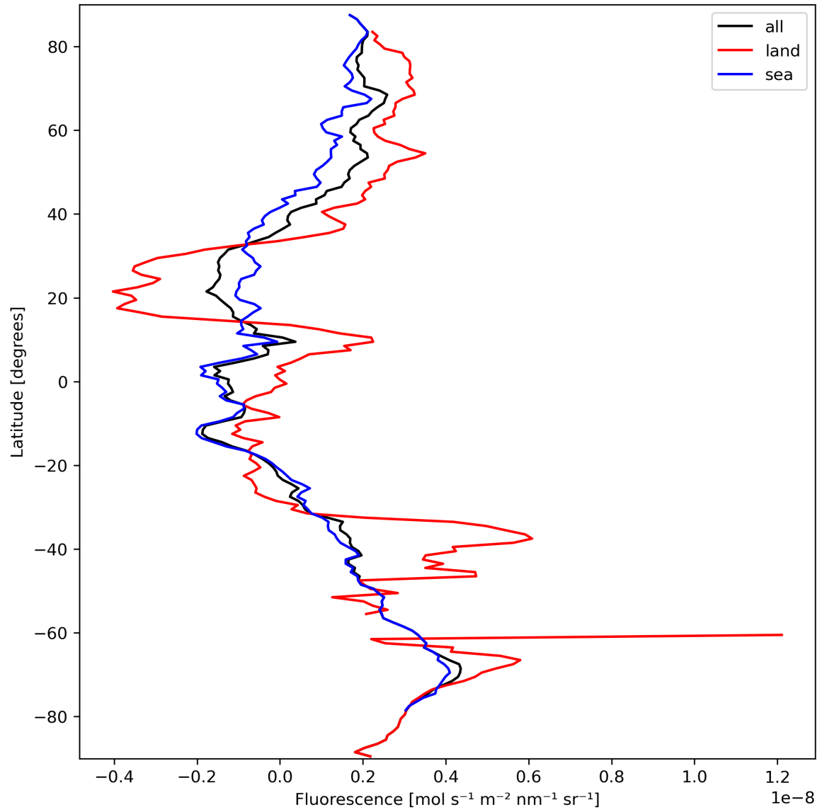
Figure 23: Zonal average of “Fluorescence” for 2023-09-24 to 2023-09-26.
