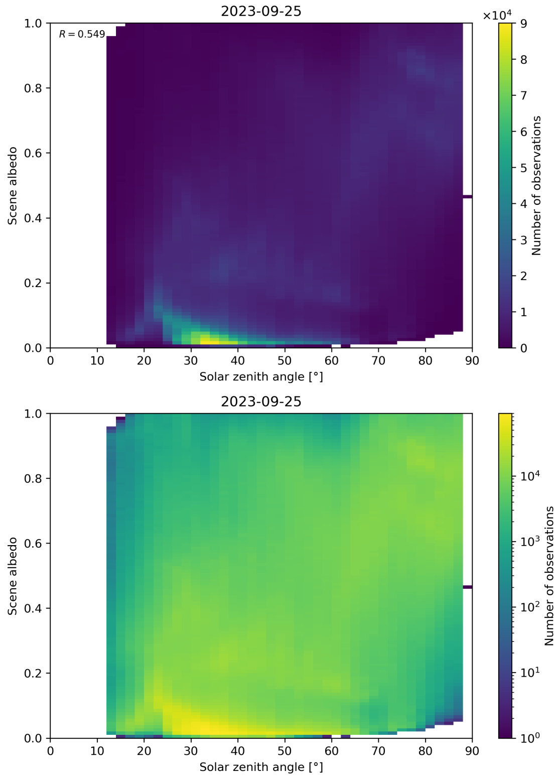
Figure 127: Scatter density plot of “Solar zenith angle” against “Scene albedo” for 2023-09-24 to 2023-09-26.
