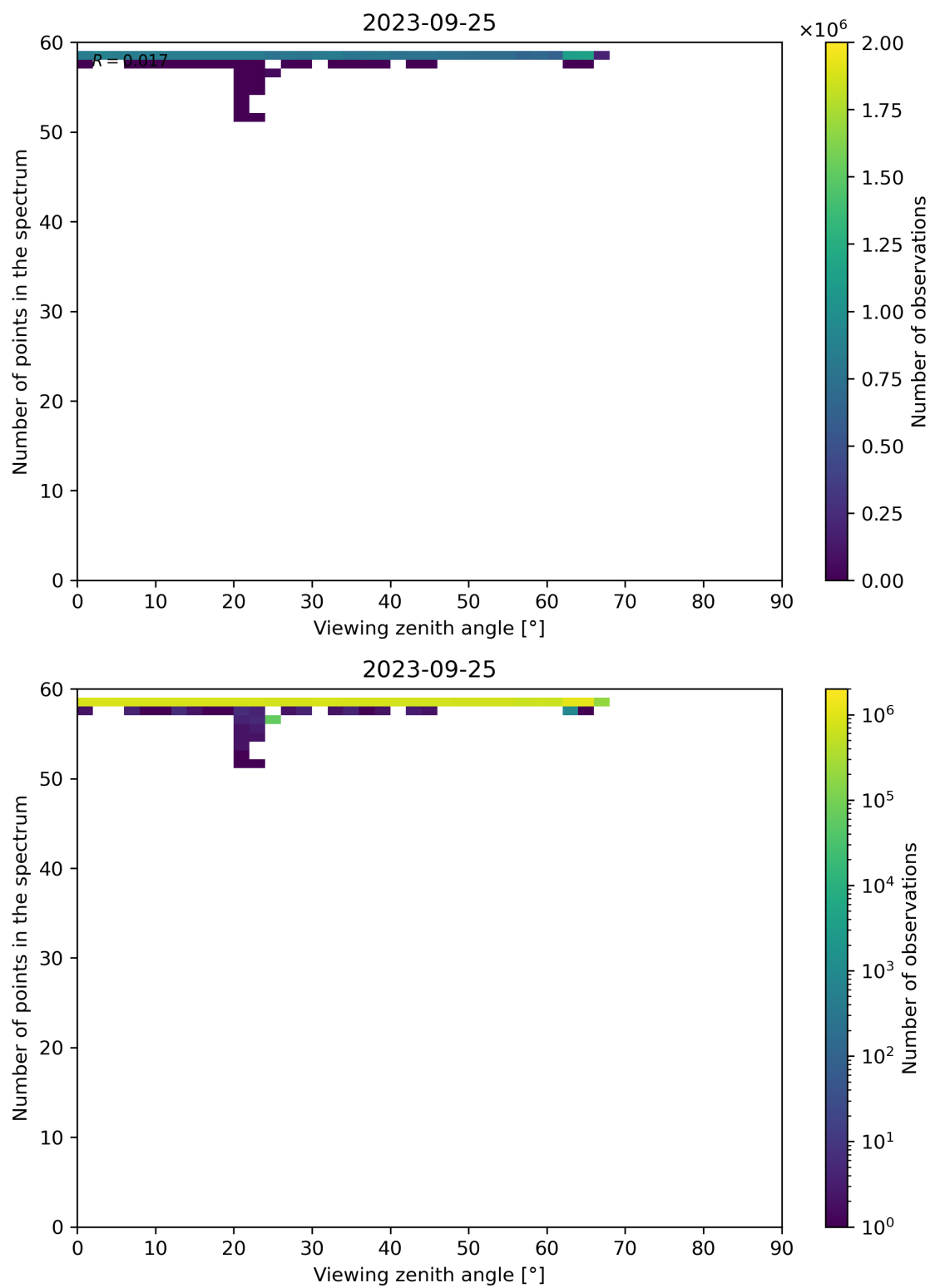
Figure 137: Scatter density plot of “Viewing zenith angle” against “Number of points in the spectrum” for 2023-09-24 to 2023-09-26.
