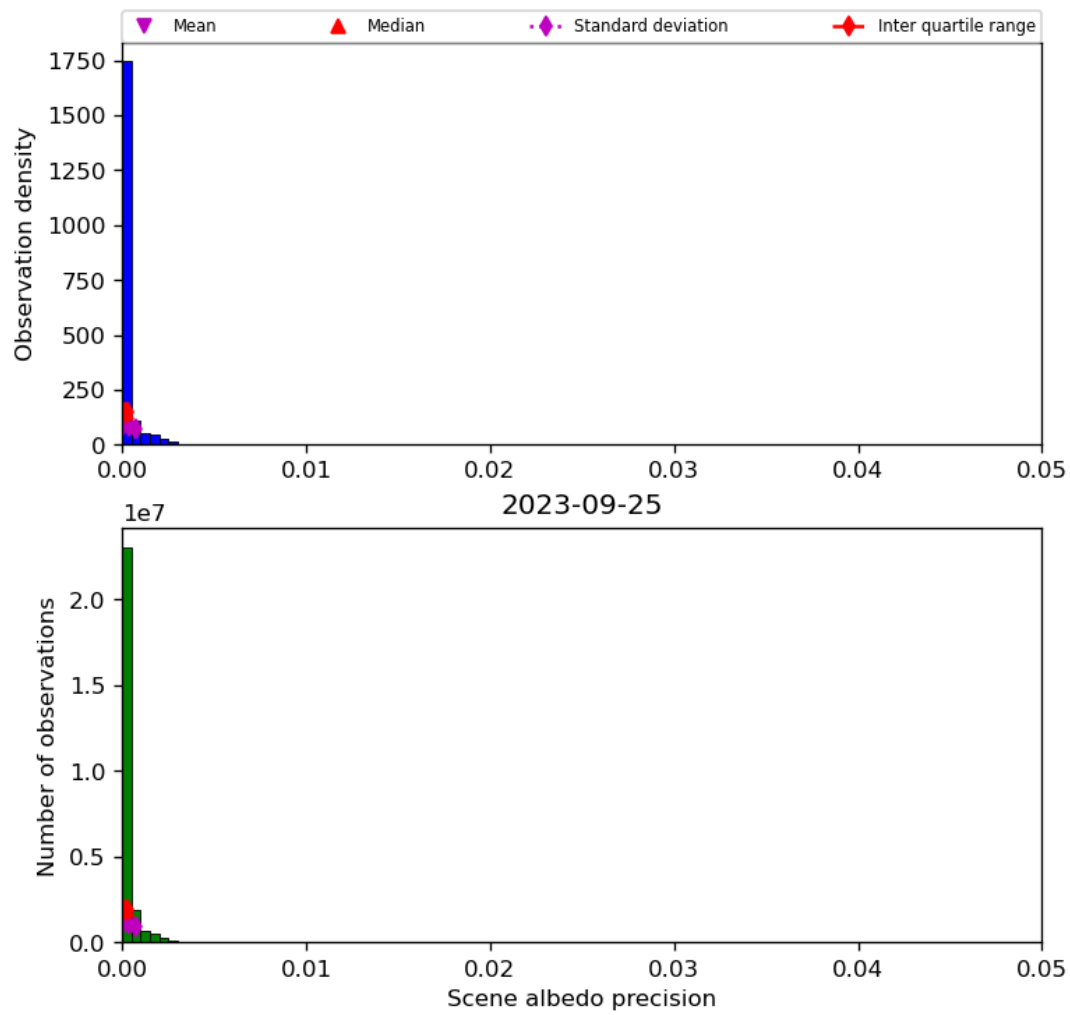
Figure 35: Histogram of “Scene albedo precision” for 2023-09-24 to 2023-09-26
