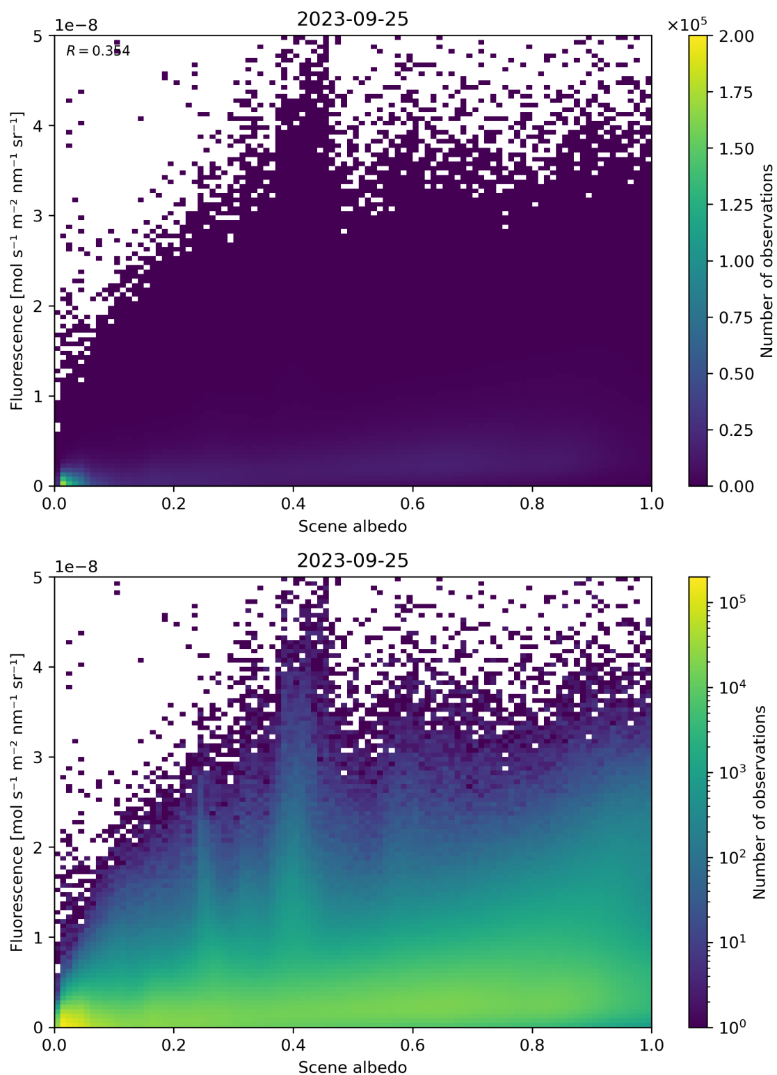
Figure 114: Scatter density plot of “Scene albedo” against “Fluorescence” for 2023-09-24 to 2023-09-26.
