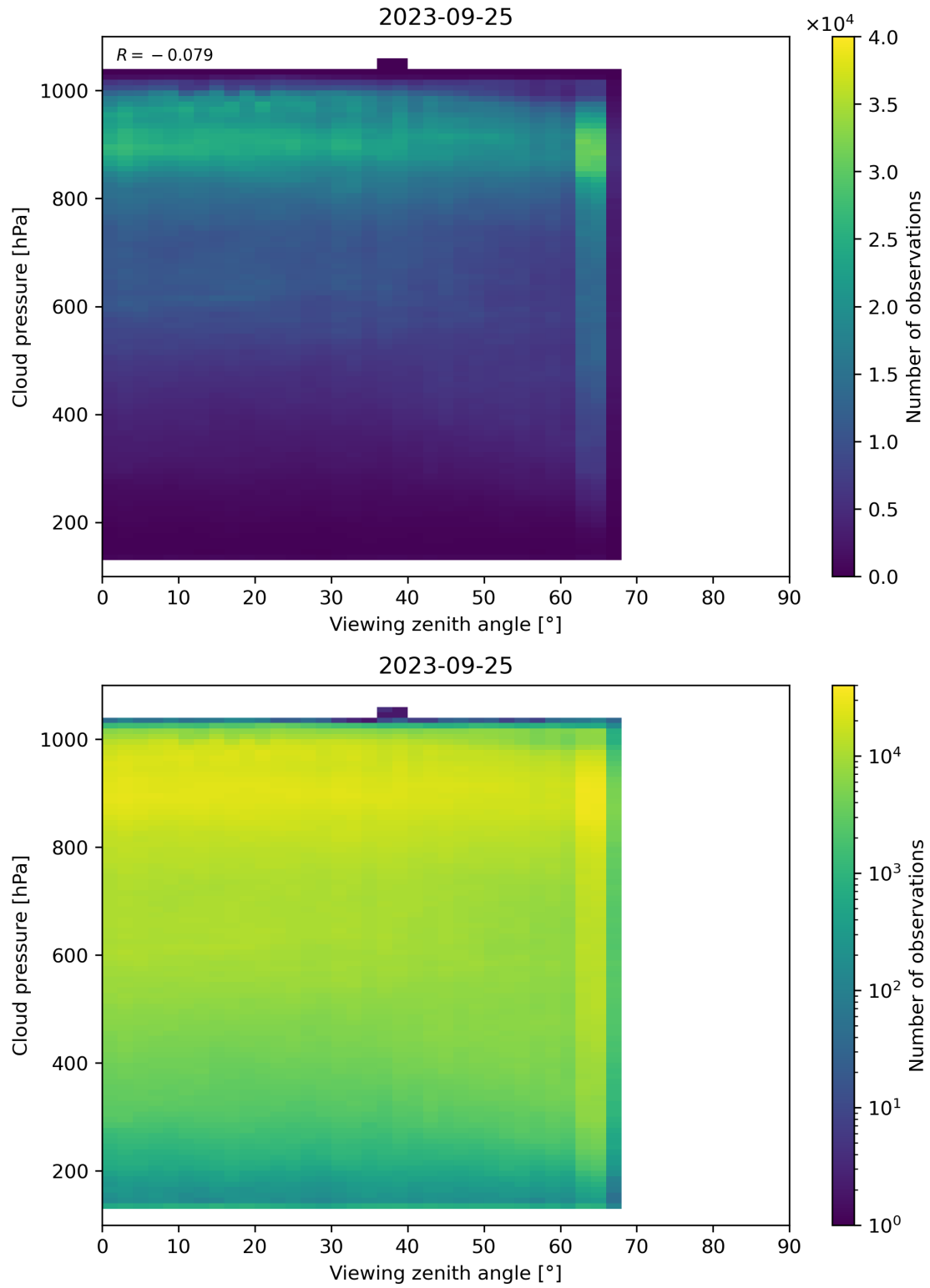
Figure 133: Scatter density plot of “Viewing zenith angle” against “Cloud pressure” for 2023-09-24 to 2023-09-26.
