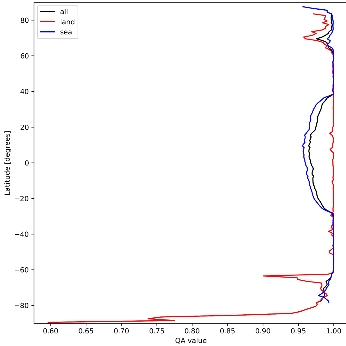
Figure 12: Zonal average of "QA value" for 2023-09-24 to 2023-09-26.
