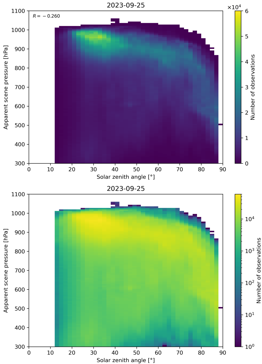
Figure 118: Scatter density plot of “Solar zenith angle” against “Apparent scene pressure” for 2023-09-24 to 2023-09-26.
