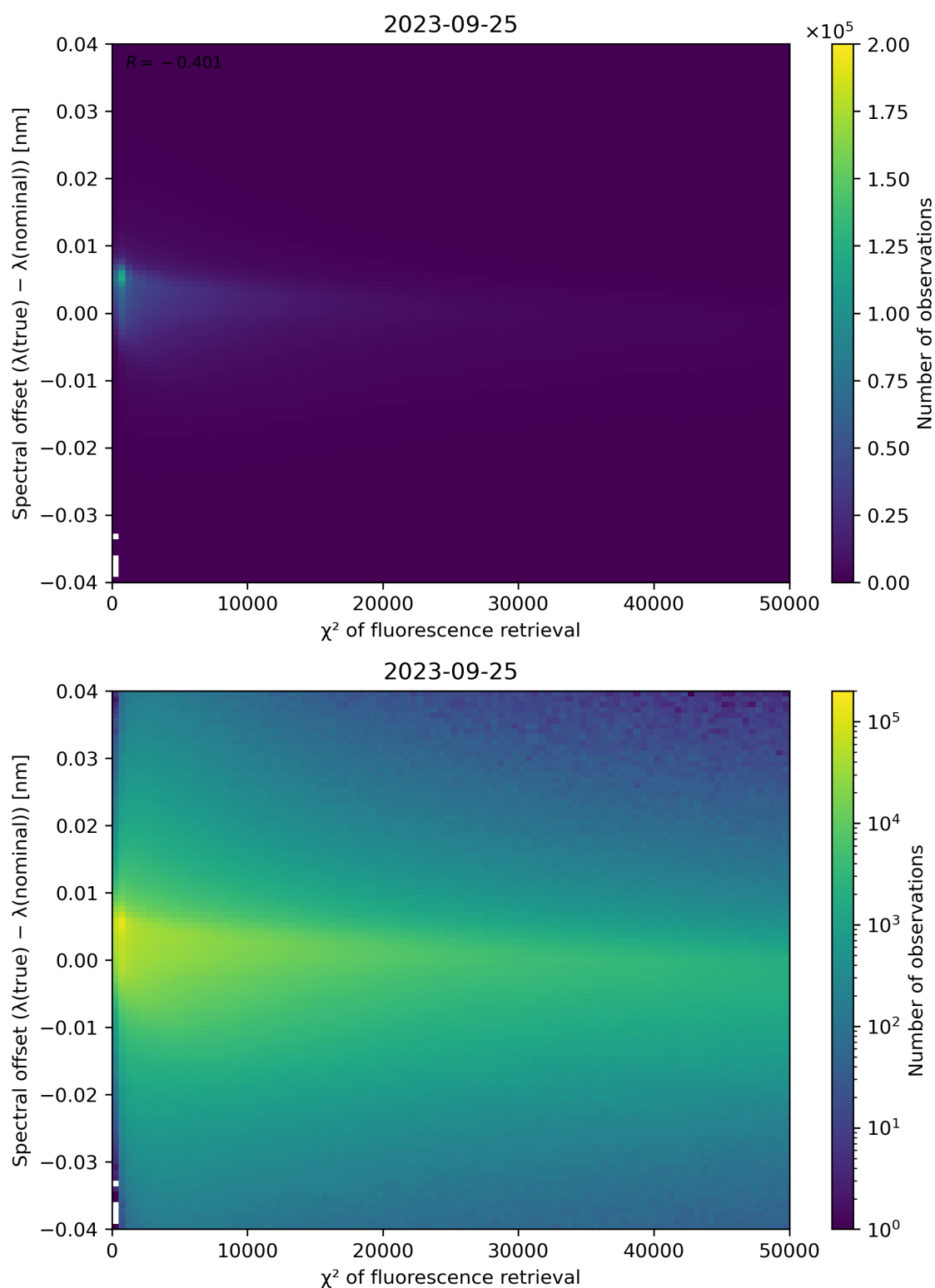
Figure 72: Scatter density plot of " \chi^2 of fluorescence retrieval" against "Spectral offset ( \lambda(\text{true}) - \lambda(\text{nominal}) )" for 2023-09-24 to 2023-09-26.
