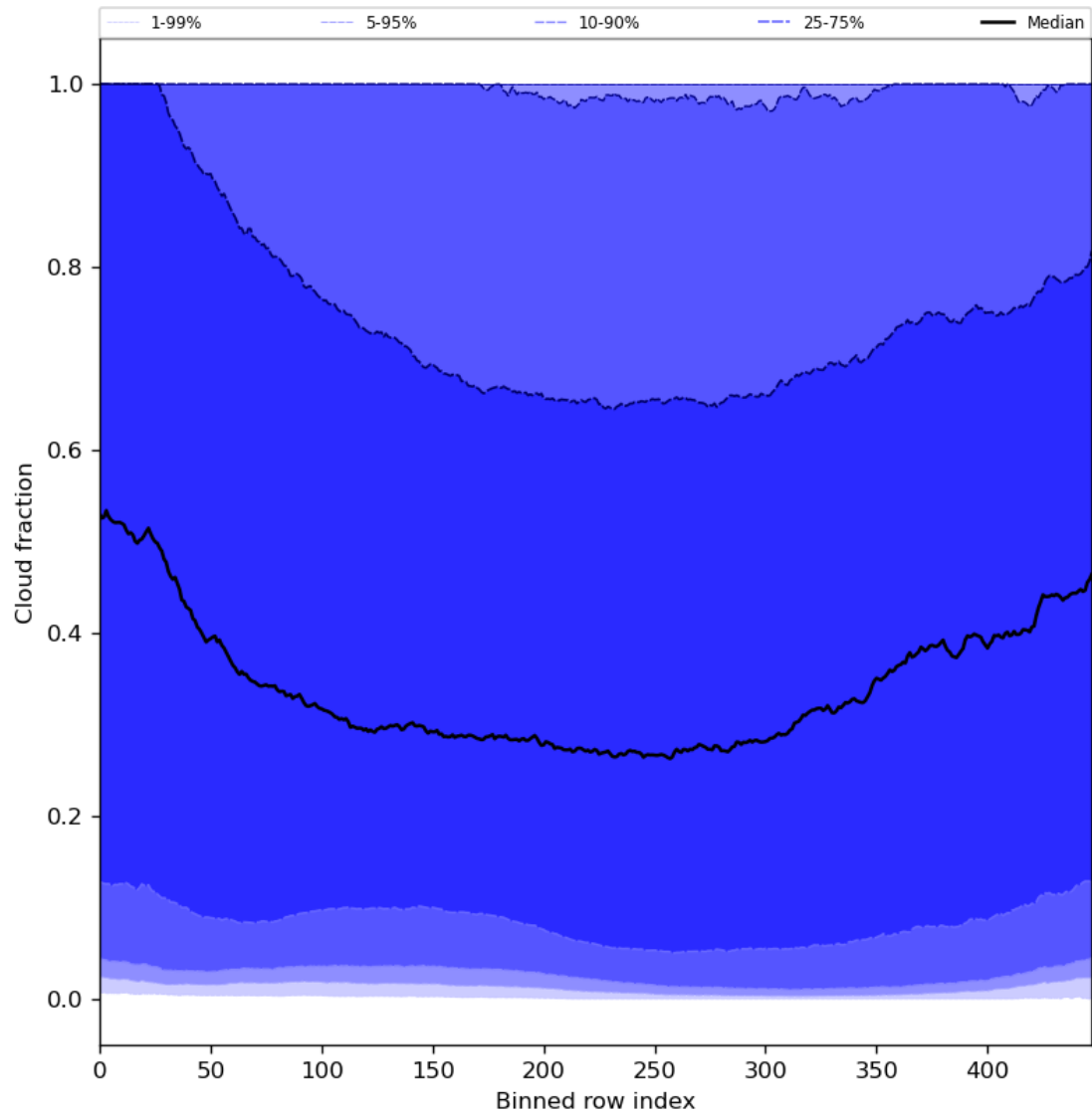
Figure 49: Along track statistics of “Cloud fraction” for 2023-09-24 to 2023-09-26
