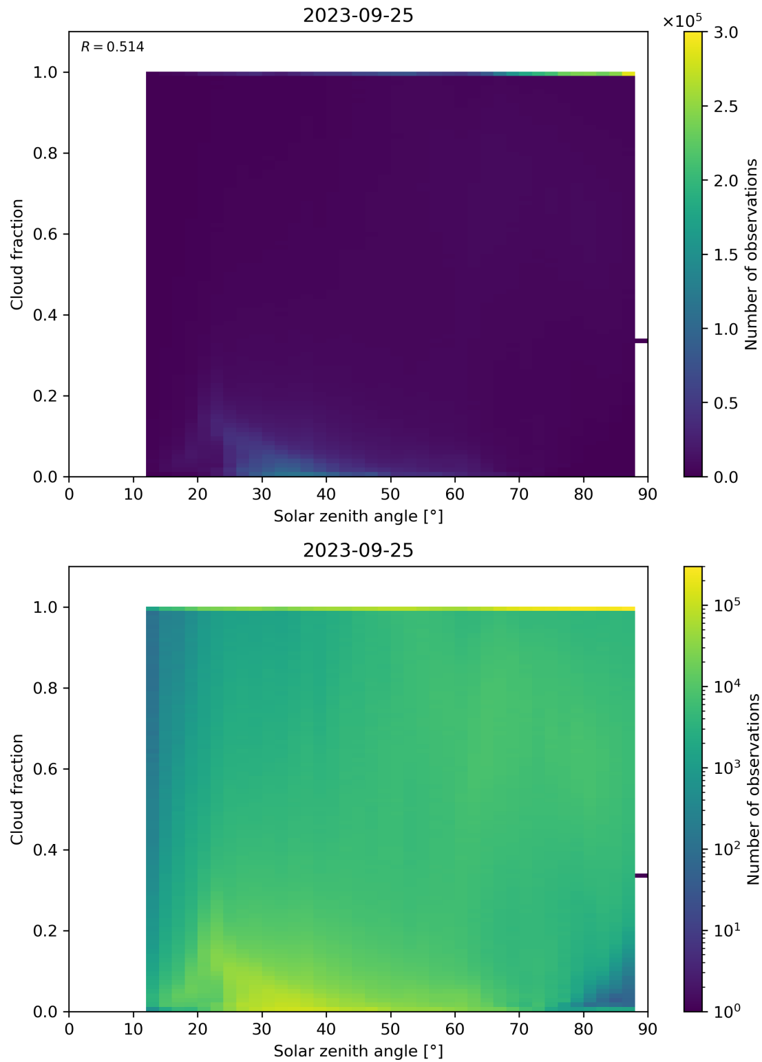
Figure 121: Scatter density plot of “Solar zenith angle” against “Cloud fraction” for 2023-09-24 to 2023-09-26.
