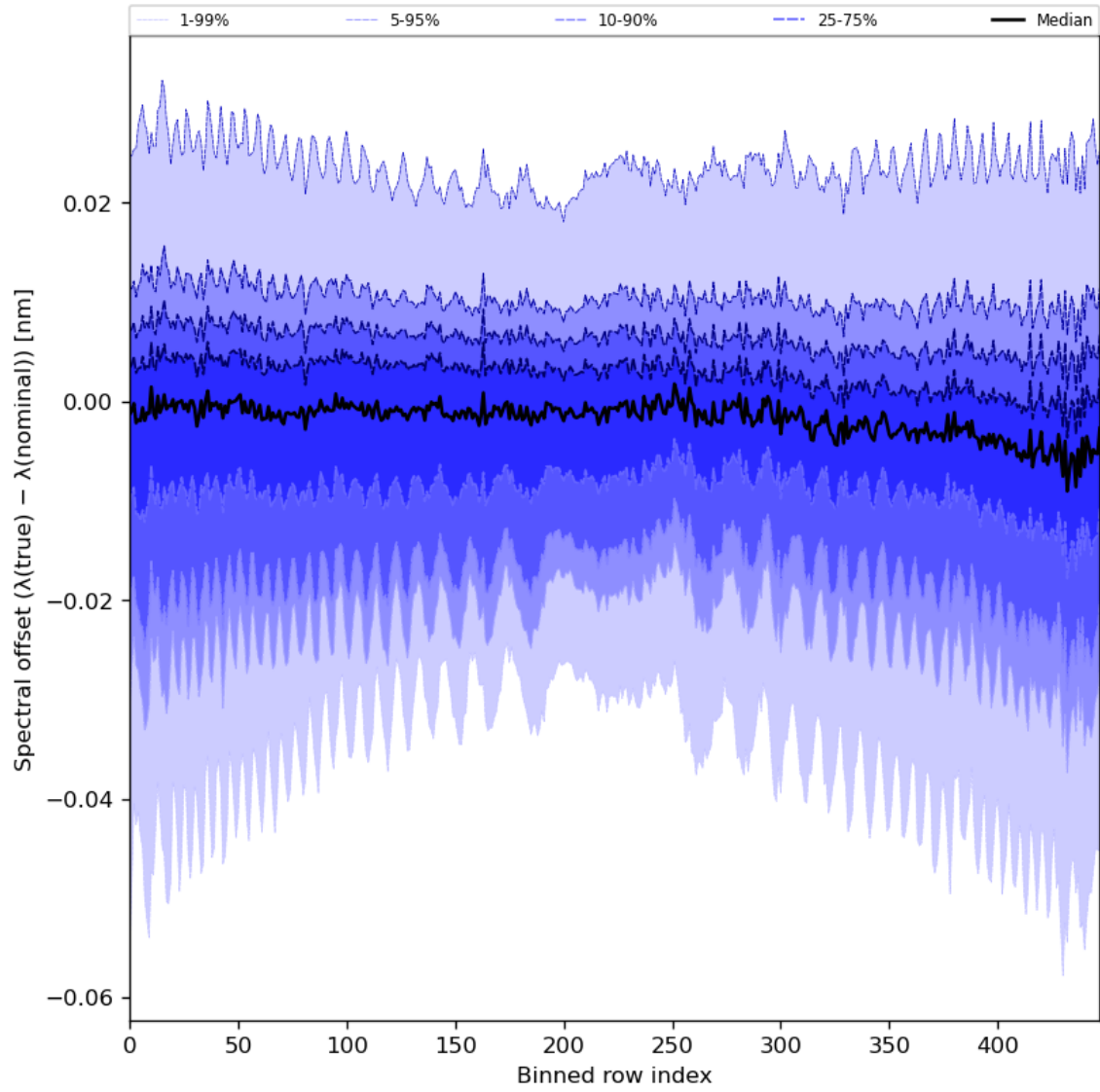
Figure 62: Along track statistics of “Spectral offset ( \lambda(\text{true}) - \lambda(\text{nominal}) )” for 2023-09-24 to 2023-09-26
