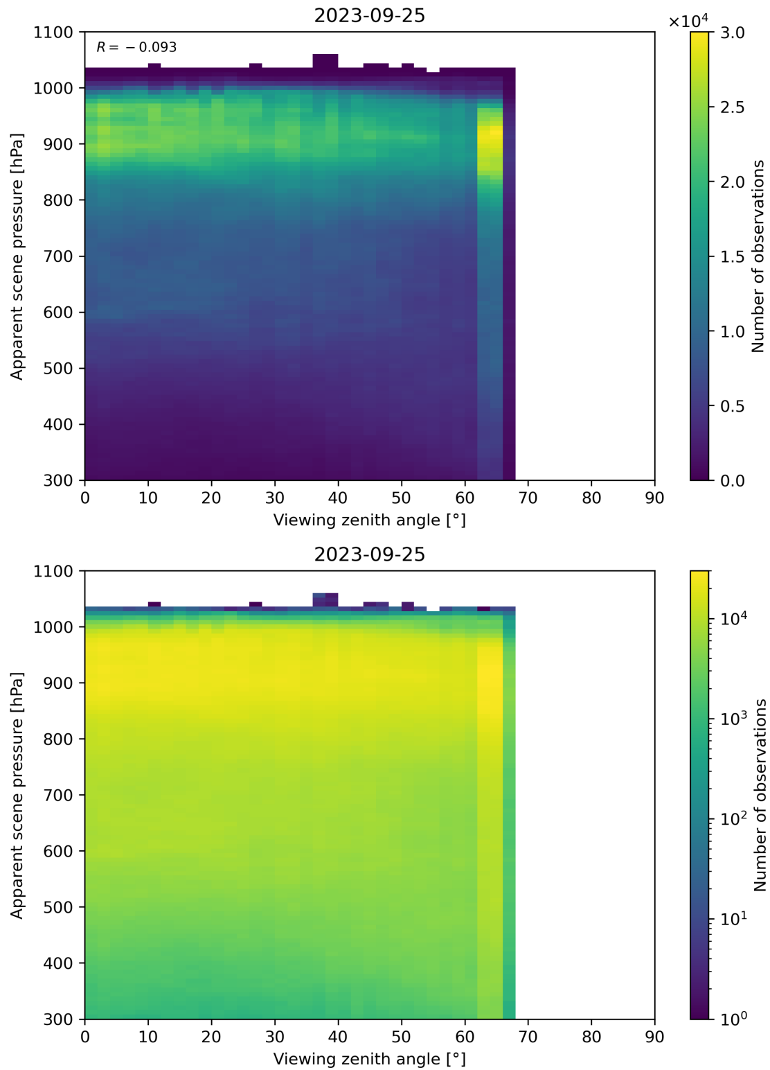
Figure 129: Scatter density plot of “Viewing zenith angle” against “Apparent scene pressure” for 2023-09-24 to 2023-09-26.
