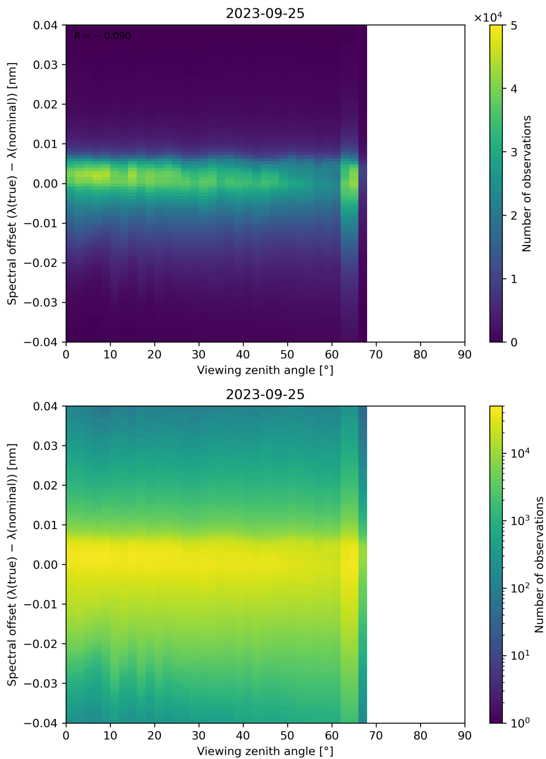
Figure 140: Scatter density plot of “Viewing zenith angle” against “Spectral offset ( \lambda(\text{true}) - \lambda(\text{nominal}) )” for 2023-09-24 to 2023-09-26.
