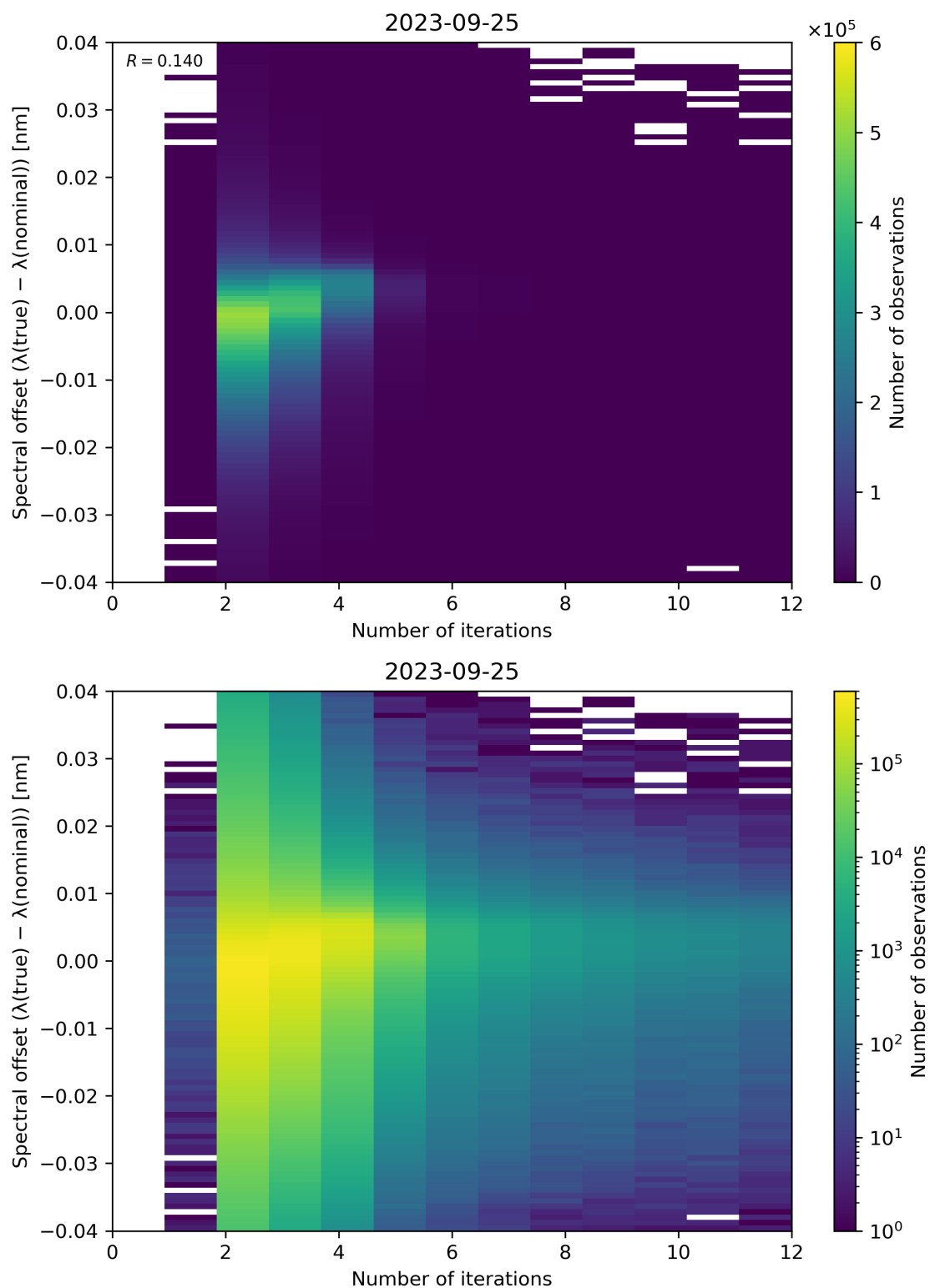
Figure 109: Scatter density plot of “Number of iterations” against “Spectral offset ( \lambda(\text{true}) - \lambda(\text{nominal}) )” for 2023-09-24 to 2023-09-26.
