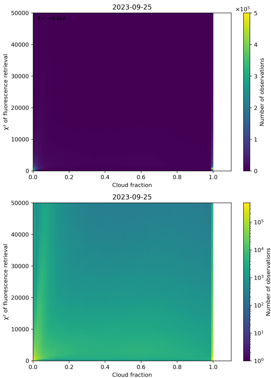
Figure 78: Scatter density plot of “Cloud fraction” against “ \chi^2 of fluorescence retrieval” for 2023-09-24 to 2023-09-26.
