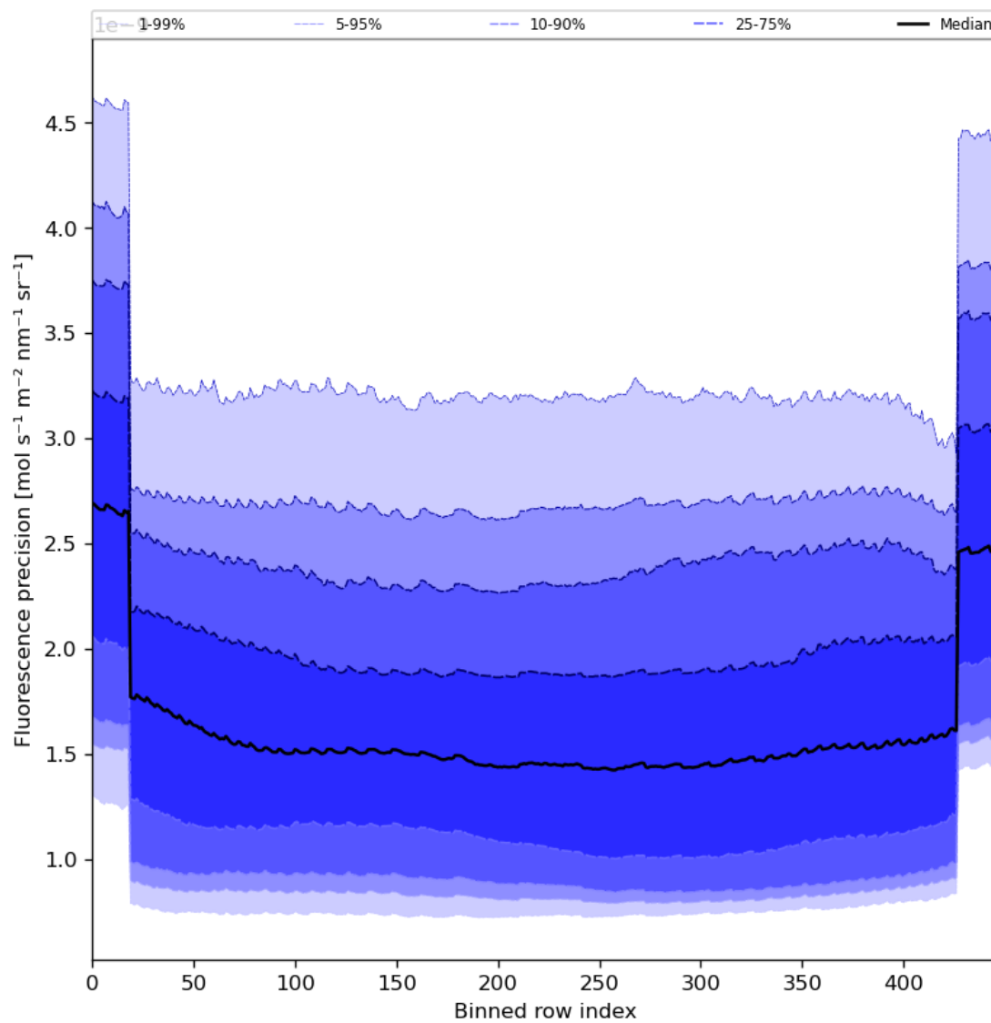
Figure 58: Along track statistics of “Fluorescence precision” for 2023-09-24 to 2023-09-26
