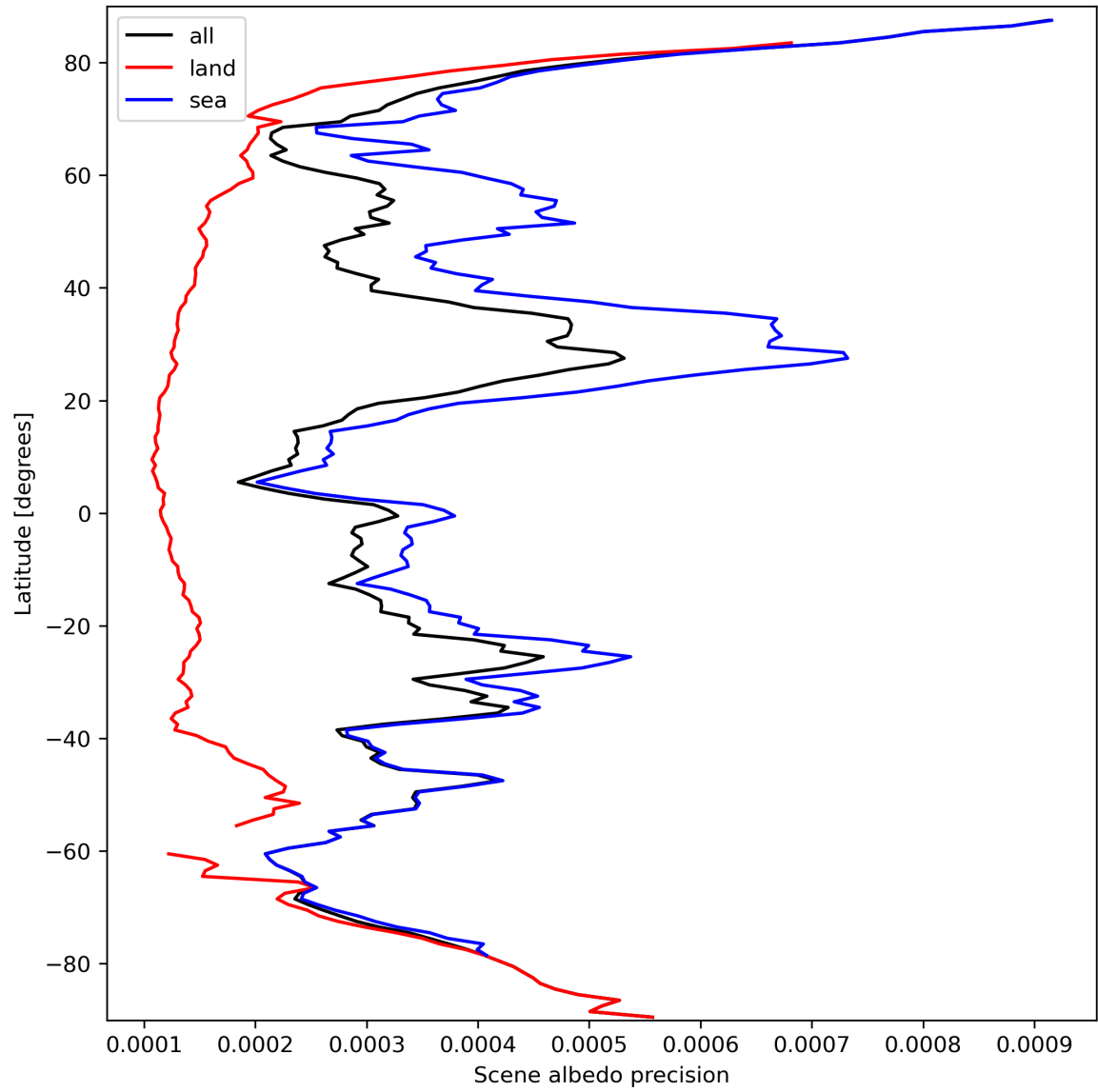
Figure 18: Zonal average of “Scene albedo precision” for 2023-09-24 to 2023-09-26.
