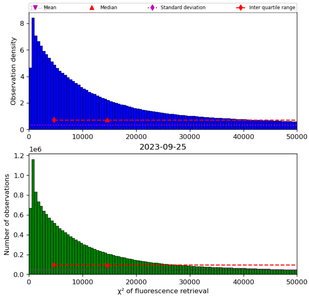
Figure 42: Histogram of “ \chi^2 of fluorescence retrieval” for 2023-09-24 to 2023-09-26
