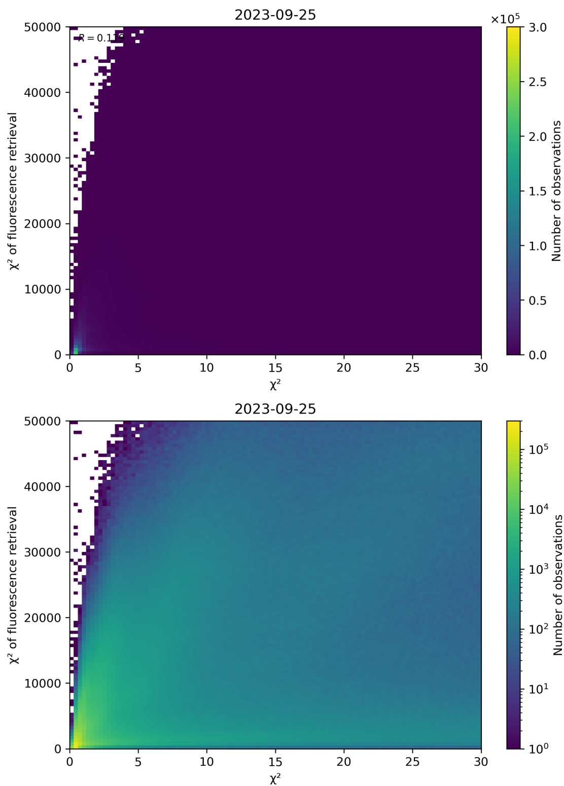
Figure 69: Scatter density plot of “ \chi^2 ” against “ \chi^2 of fluorescence retrieval” for 2023-09-24 to 2023-09-26.
