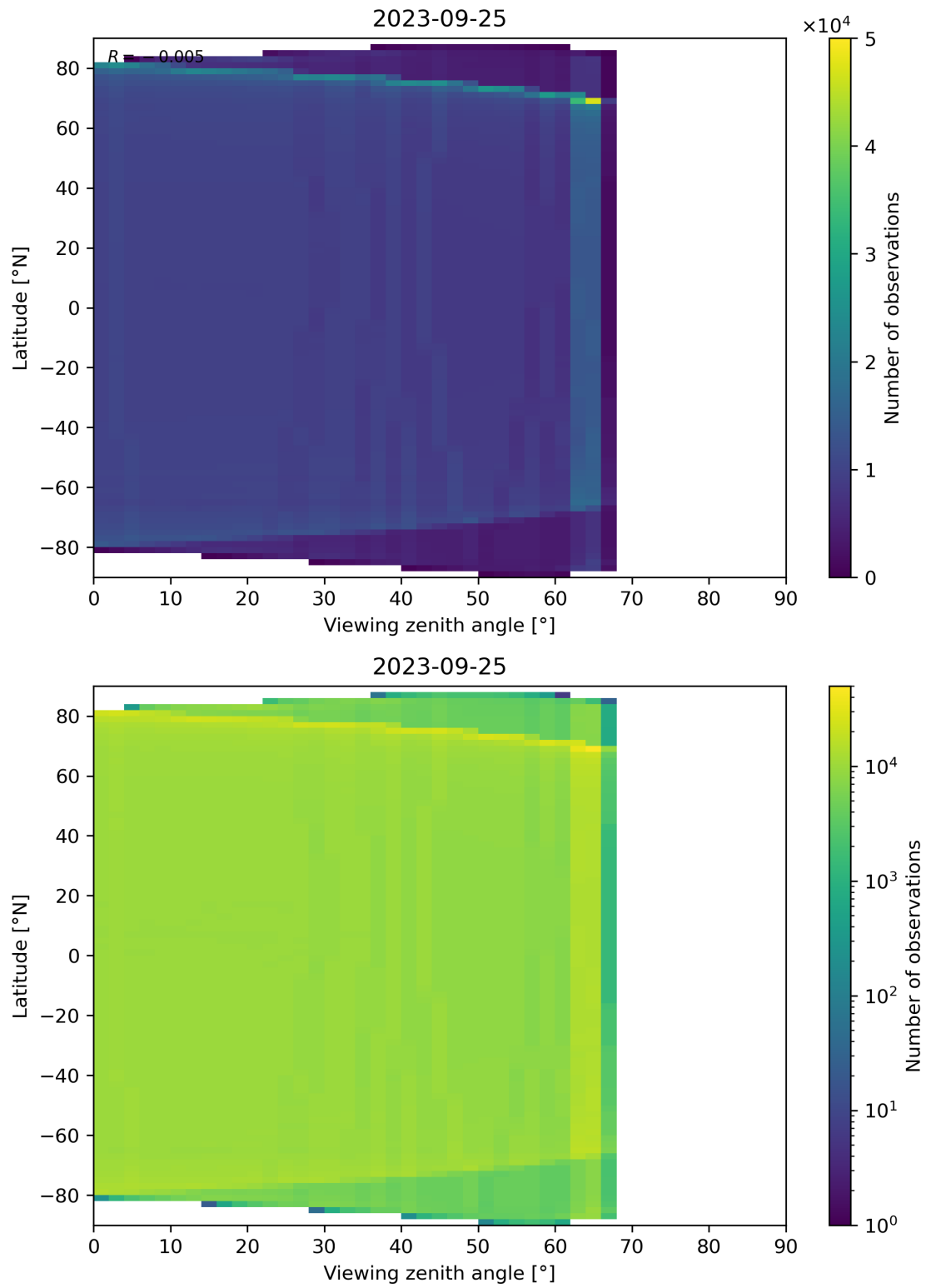
Figure 135: Scatter density plot of “Viewing zenith angle” against “Latitude” for 2023-09-24 to 2023-09-26.
