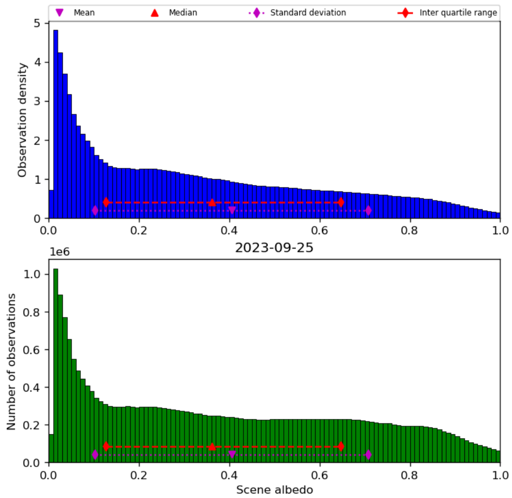
Figure 34: Histogram of “Scene albedo” for 2023-09-24 to 2023-09-26
