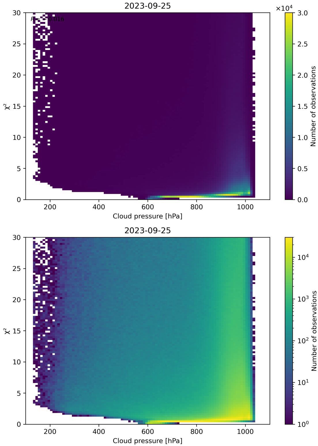
Figure 85: Scatter density plot of “Cloud pressure” against “ \chi^2 ” for 2023-09-24 to 2023-09-26.
