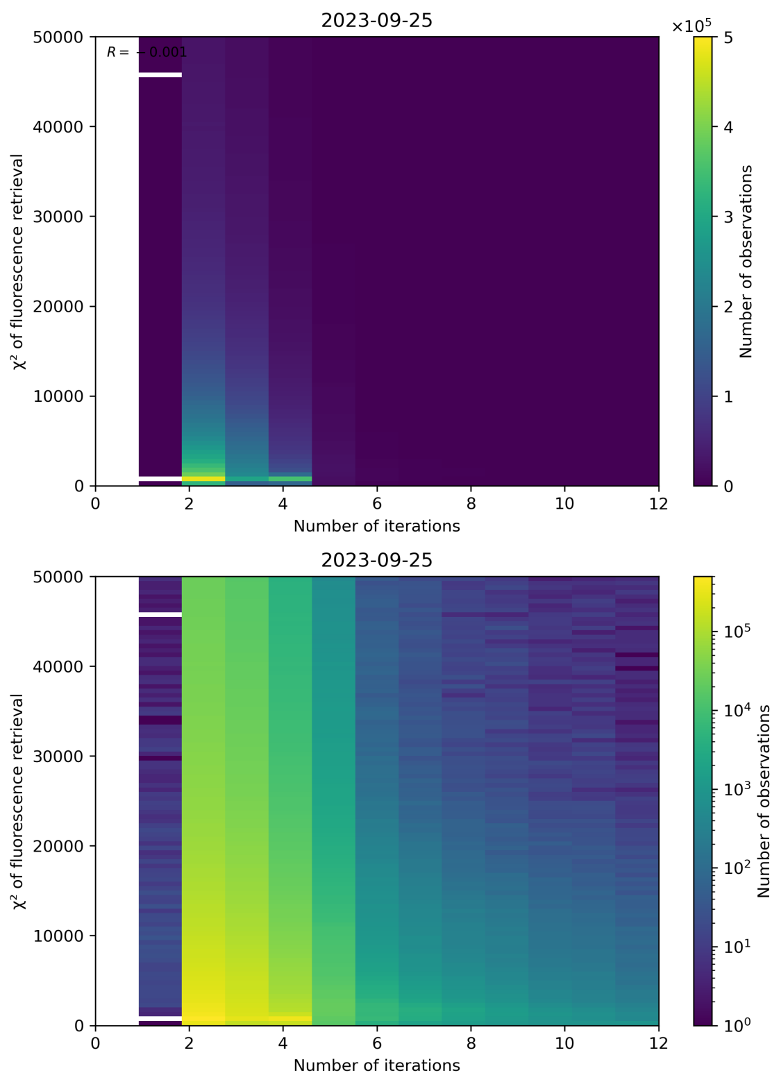
Figure 106: Scatter density plot of “Number of iterations” against “ \chi^2 of fluorescence retrieval” for 2023-09-24 to 2023-09-26.
