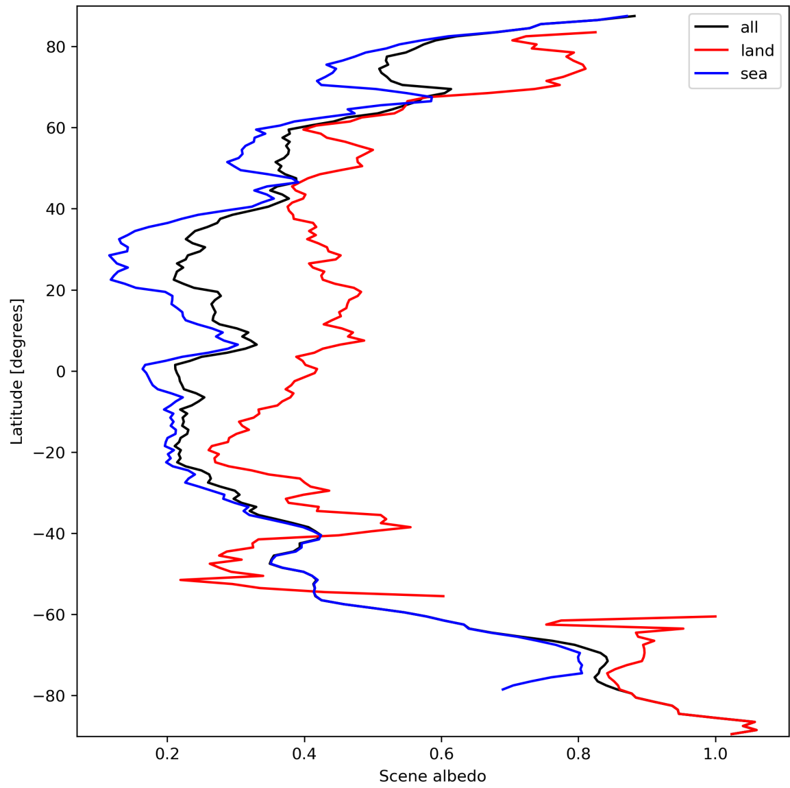
Figure 17: Zonal average of “Scene albedo” for 2023-09-24 to 2023-09-26.
