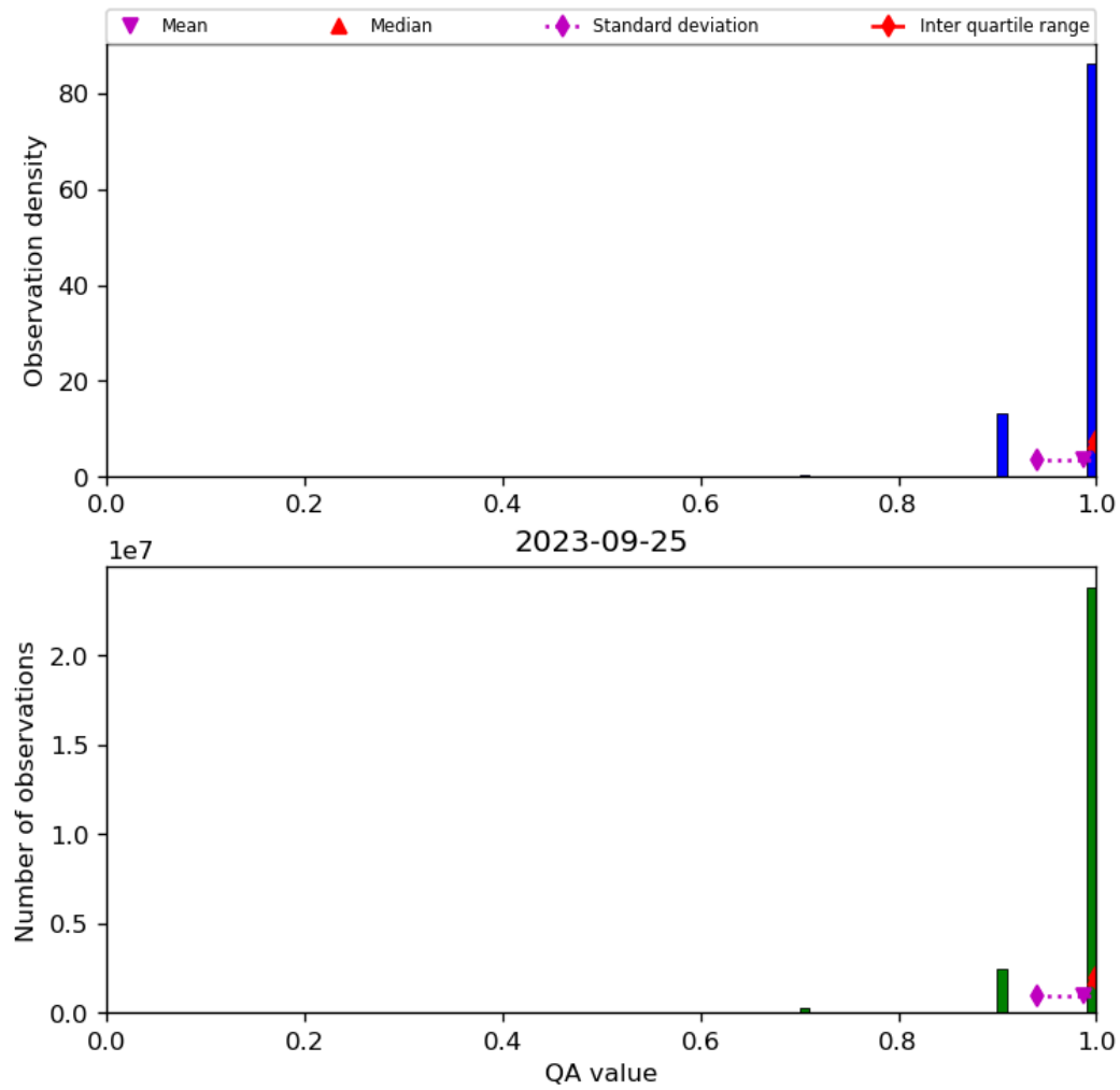
Figure 29: Histogram of “QA value” for 2023-09-24 to 2023-09-26
