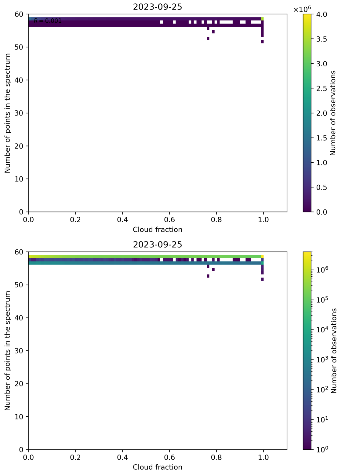
Figure 81: Scatter density plot of “Cloud fraction” against “Number of points in the spectrum” for 2023-09-24 to 2023-09-26.
