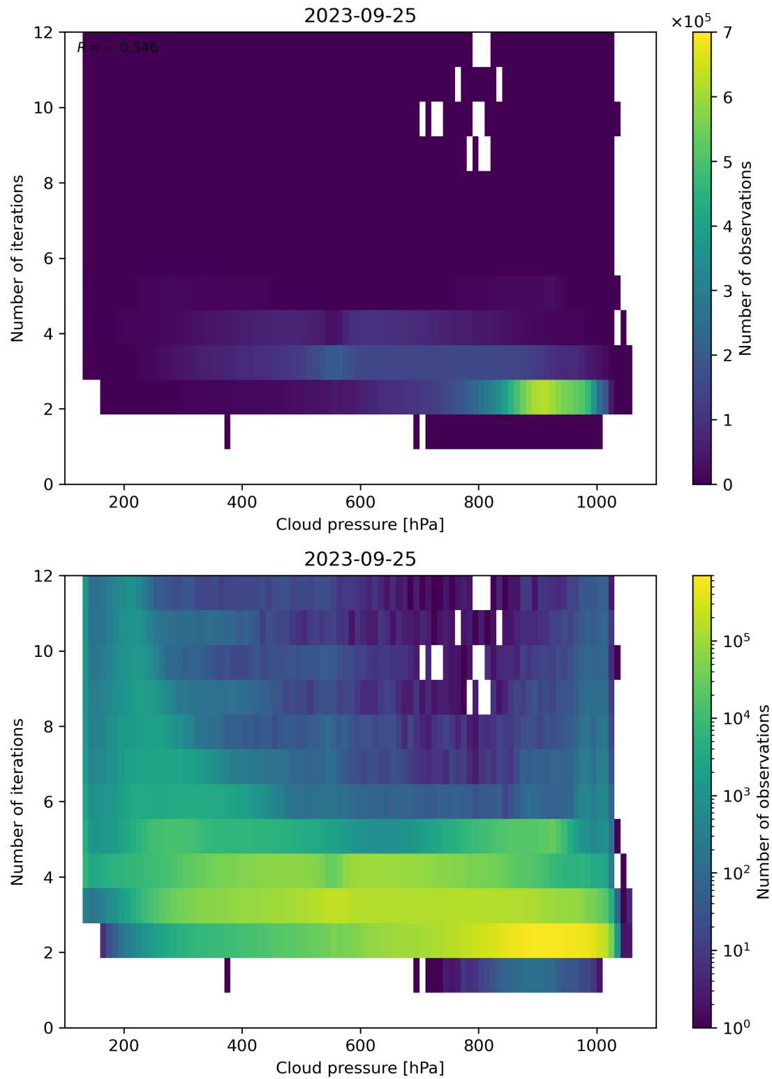
Figure 89: Scatter density plot of “Cloud pressure” against “Number of iterations” for 2023-09-24 to 2023-09-26.
