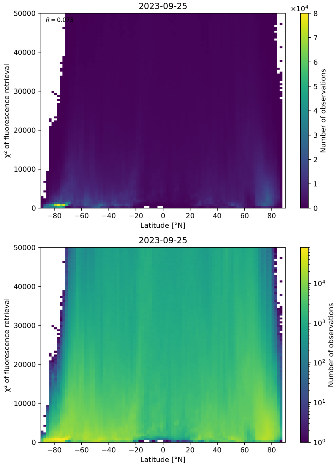
Figure 98: Scatter density plot of “Latitude” against “ \chi^2 of fluorescence retrieval” for 2023-09-24 to 2023-09-26.
