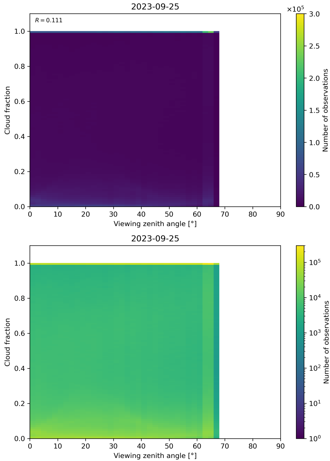
Figure 132: Scatter density plot of “Viewing zenith angle” against “Cloud fraction” for 2023-09-24 to 2023-09-26.
