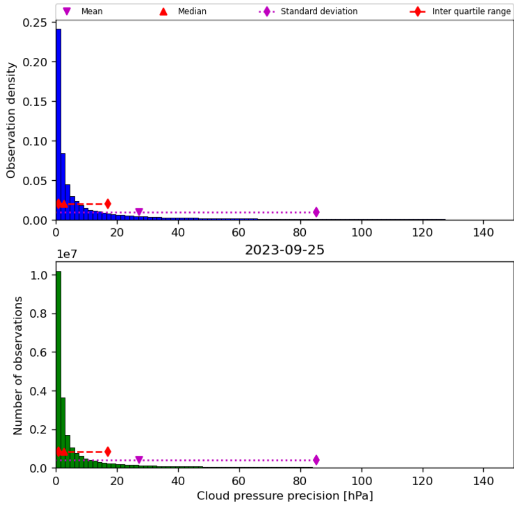
Figure 31: Histogram of “Cloud pressure precision” for 2023-09-24 to 2023-09-26
