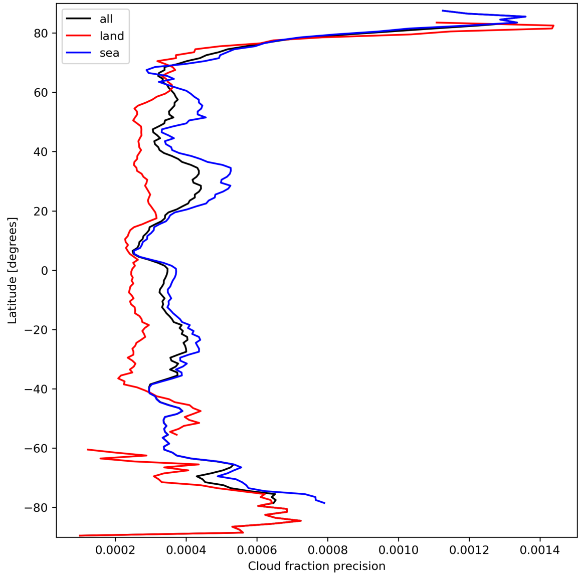
Figure 16: Zonal average of “Cloud fraction precision” for 2023-09-24 to 2023-09-26.
