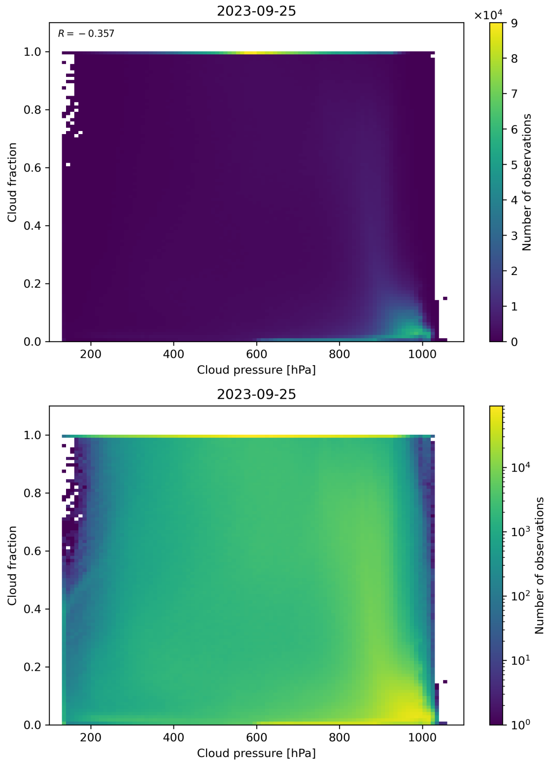
Figure 87: Scatter density plot of “Cloud pressure” against “Cloud fraction” for 2023-09-24 to 2023-09-26.
