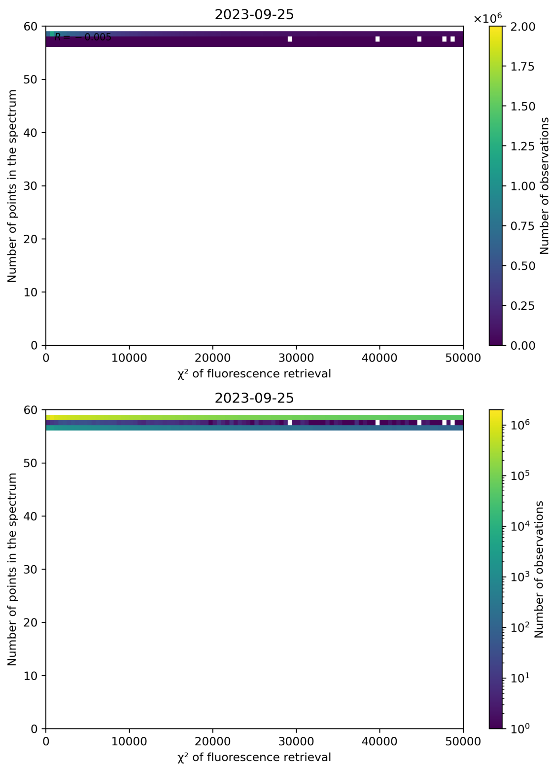
Figure 71: Scatter density plot of “ \chi^2 of fluorescence retrieval” against “Number of points in the spectrum” for 2023-09-24 to 2023-09-26.
