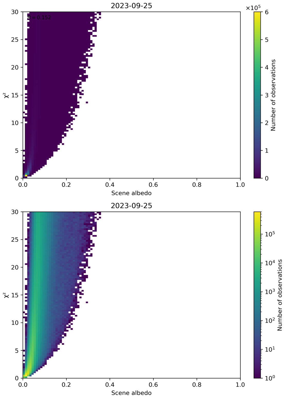
Figure 112: Scatter density plot of “Scene albedo” against “ \chi^2 ” for 2023-09-24 to 2023-09-26.
