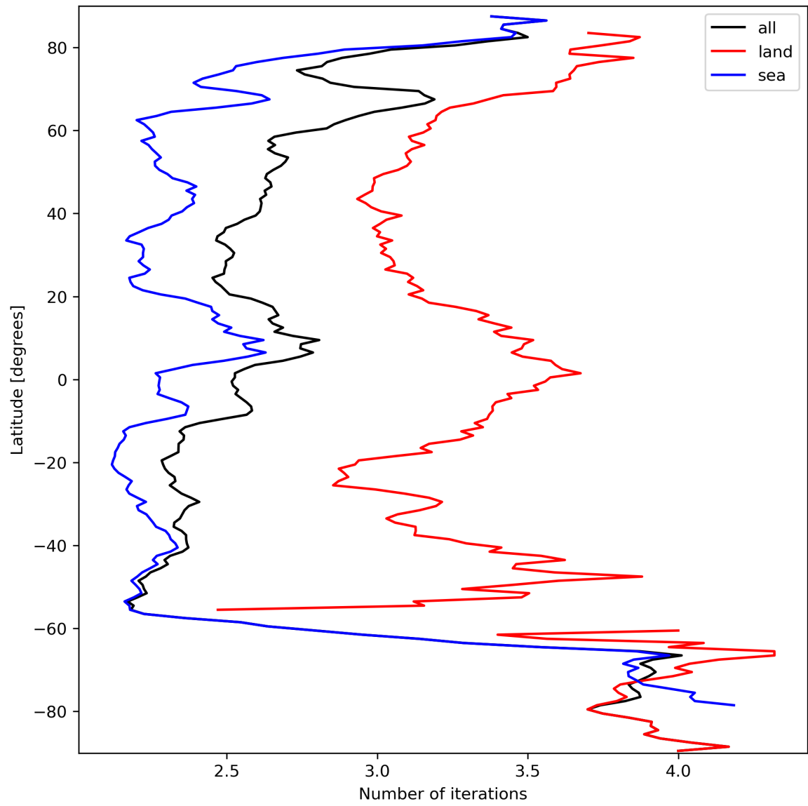
Figure 22: Zonal average of “Number of iterations” for 2023-09-24 to 2023-09-26.
