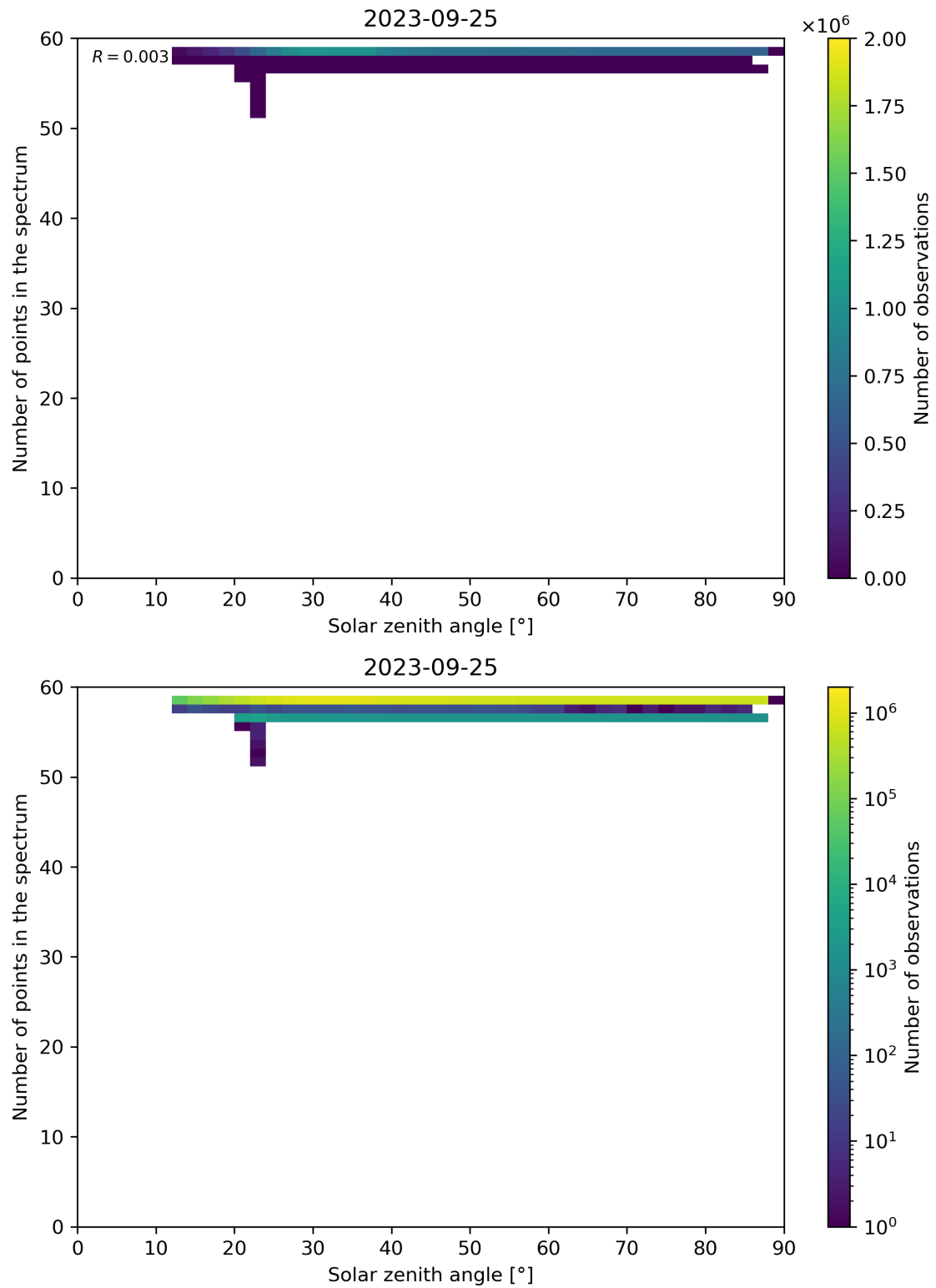
Figure 126: Scatter density plot of “Solar zenith angle” against “Number of points in the spectrum” for 2023-09-24 to 2023-09-26.
