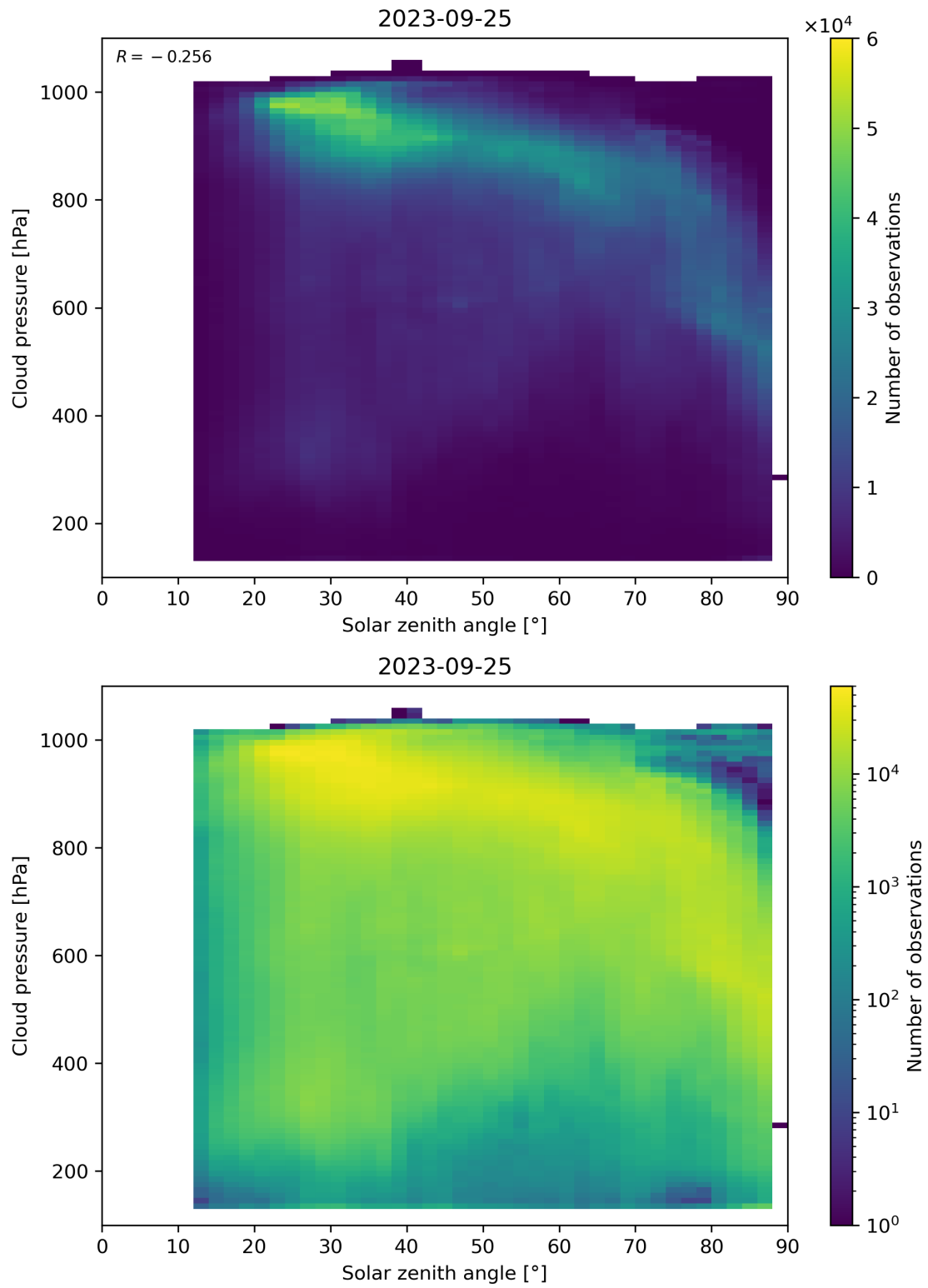
Figure 122: Scatter density plot of “Solar zenith angle” against “Cloud pressure” for 2023-09-24 to 2023-09-26.
