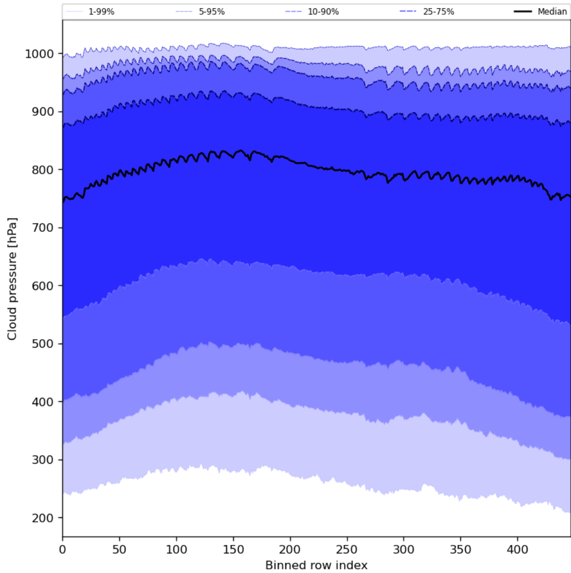
Figure 47: Along track statistics of “Cloud pressure” for 2023-09-24 to 2023-09-26
