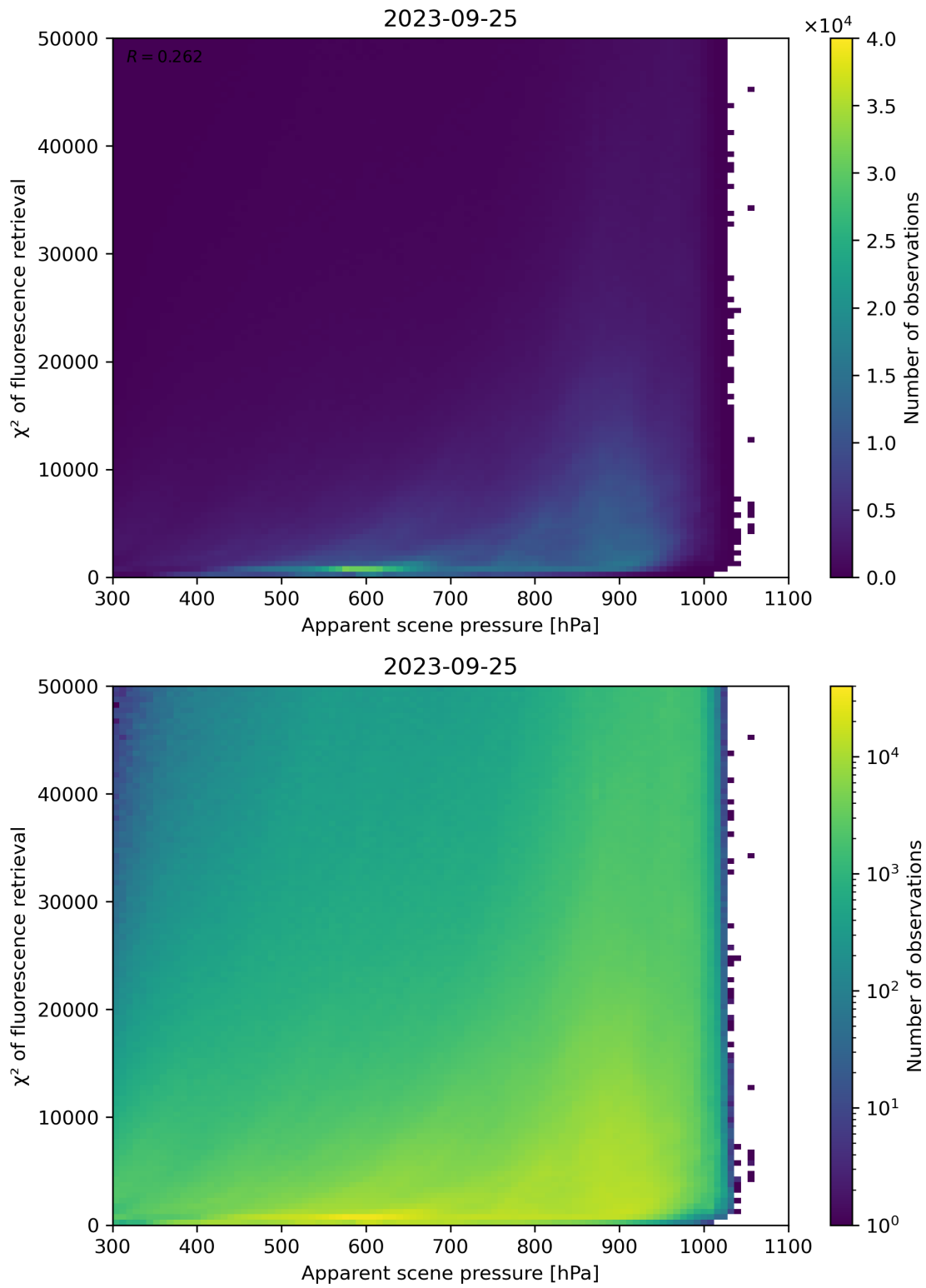
Figure 64: Scatter density plot of “Apparent scene pressure” against “ \chi^2 of fluorescence retrieval” for 2023-09-24 to 2023-09-26.
