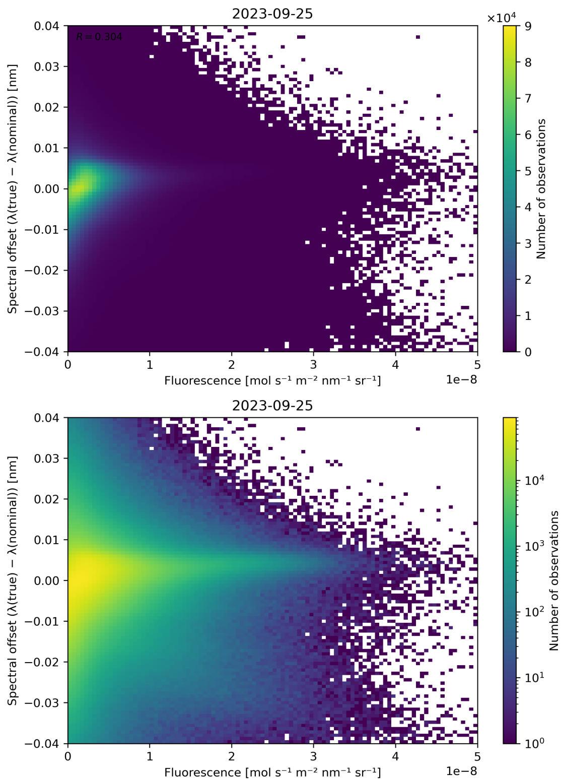
Figure 95: Scatter density plot of “Fluorescence” against “Spectral offset ( \lambda(\text{true}) - \lambda(\text{nominal}) )” for 2023-09-24 to 2023-09-26.
