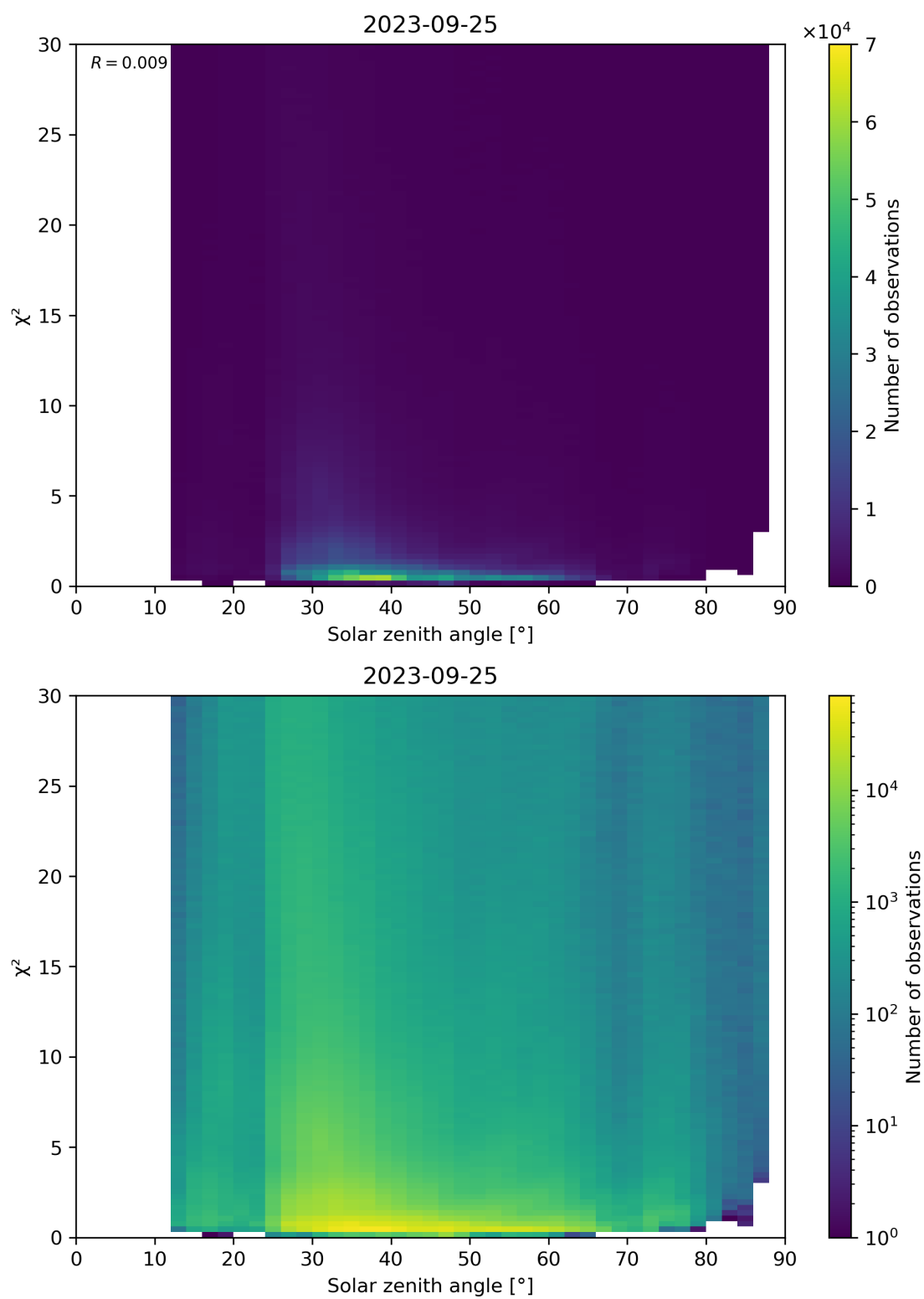
Figure 119: Scatter density plot of “Solar zenith angle” against “ \chi^2 ” for 2023-09-24 to 2023-09-26.
