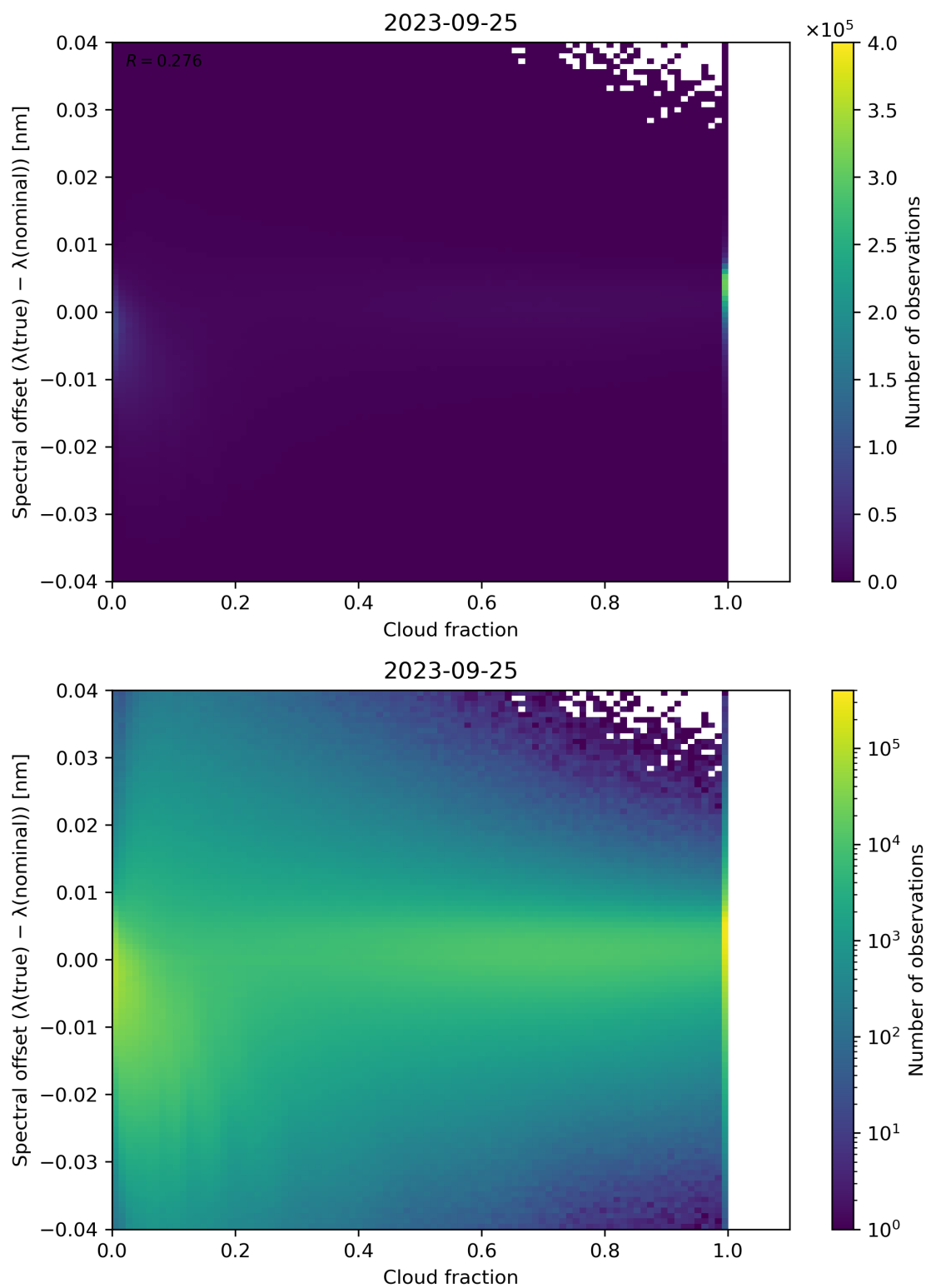
Figure 83: Scatter density plot of “Cloud fraction” against “Spectral offset ( \lambda(\text{true}) - \lambda(\text{nominal}) )” for 2023-09-24 to 2023-09-26.
