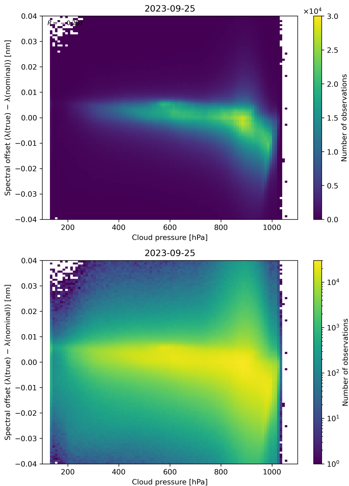
Figure 92: Scatter density plot of “Cloud pressure” against “Spectral offset ( \lambda(\text{true}) - \lambda(\text{nominal}) )” for 2023-09-24 to 2023-09-26.
