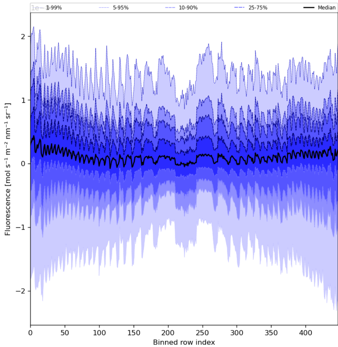
Figure 57: Along track statistics of “Fluorescence” for 2023-09-24 to 2023-09-26
