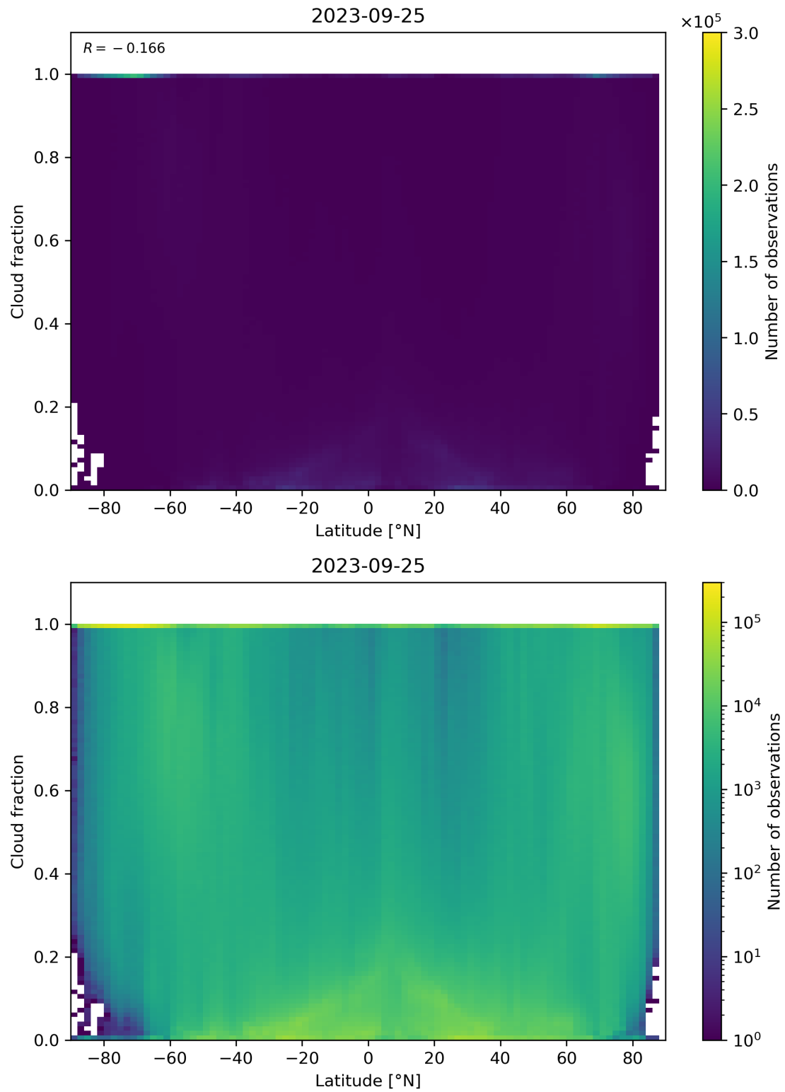
Figure 99: Scatter density plot of “Latitude” against “Cloud fraction” for 2023-09-24 to 2023-09-26.
