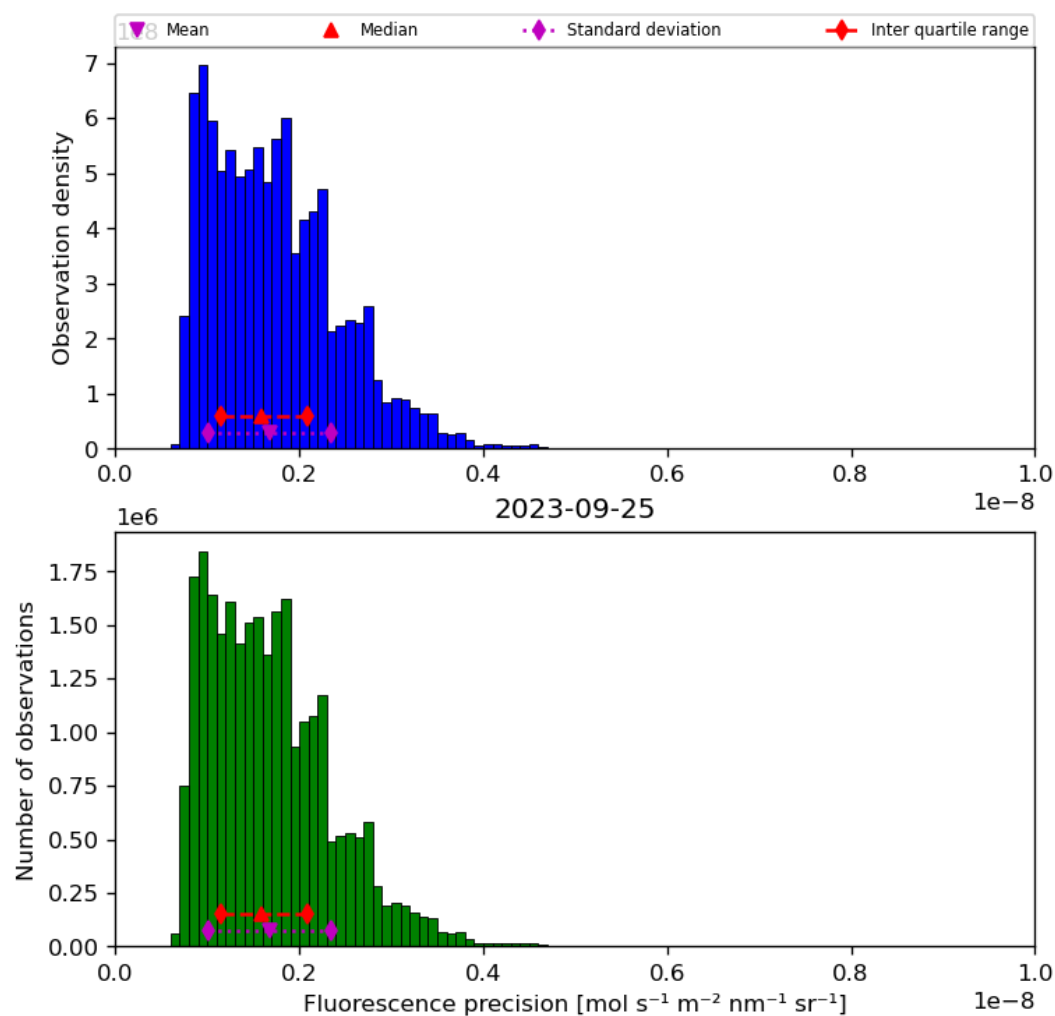
Figure 41: Histogram of “Fluorescence precision” for 2023-09-24 to 2023-09-26
