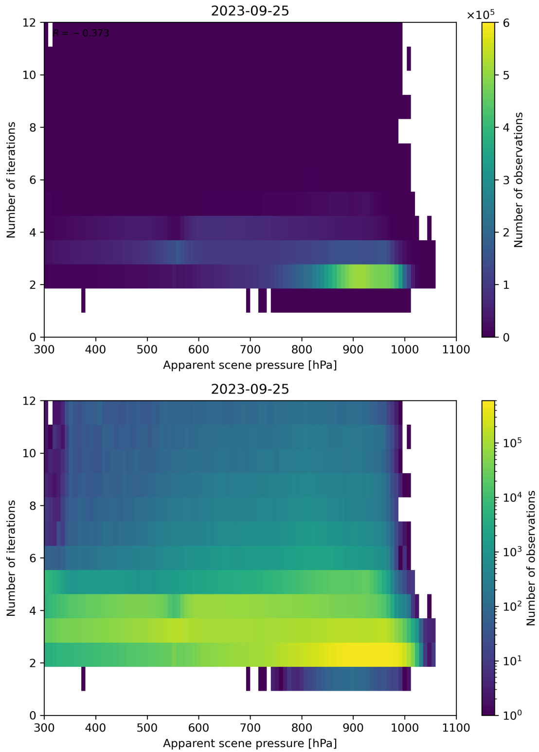
Figure 66: Scatter density plot of “Apparent scene pressure” against “Number of iterations” for 2023-09-24 to 2023-09-26.
