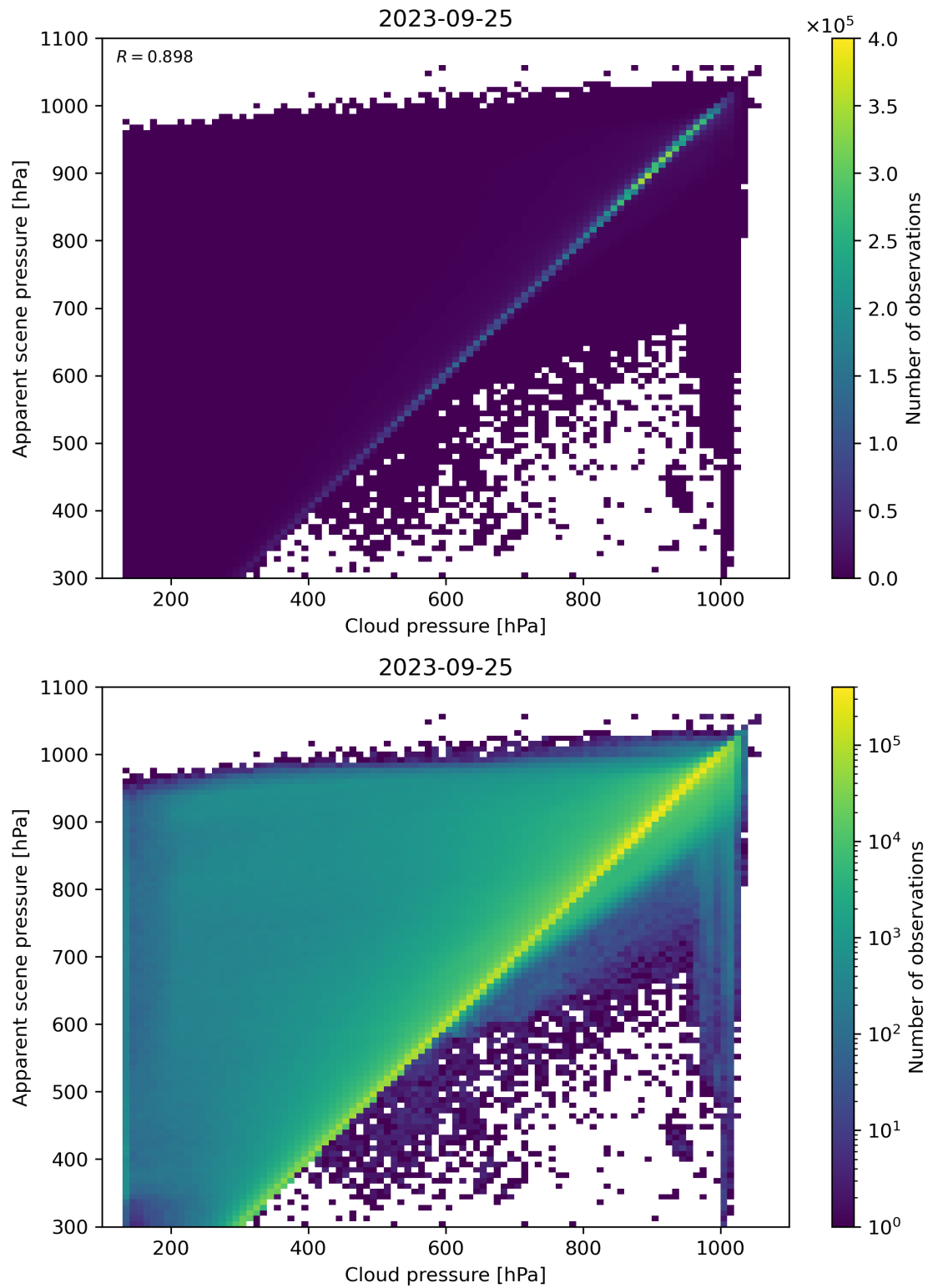
Figure 84: Scatter density plot of “Cloud pressure” against “Apparent scene pressure” for 2023-09-24 to 2023-09-26.
