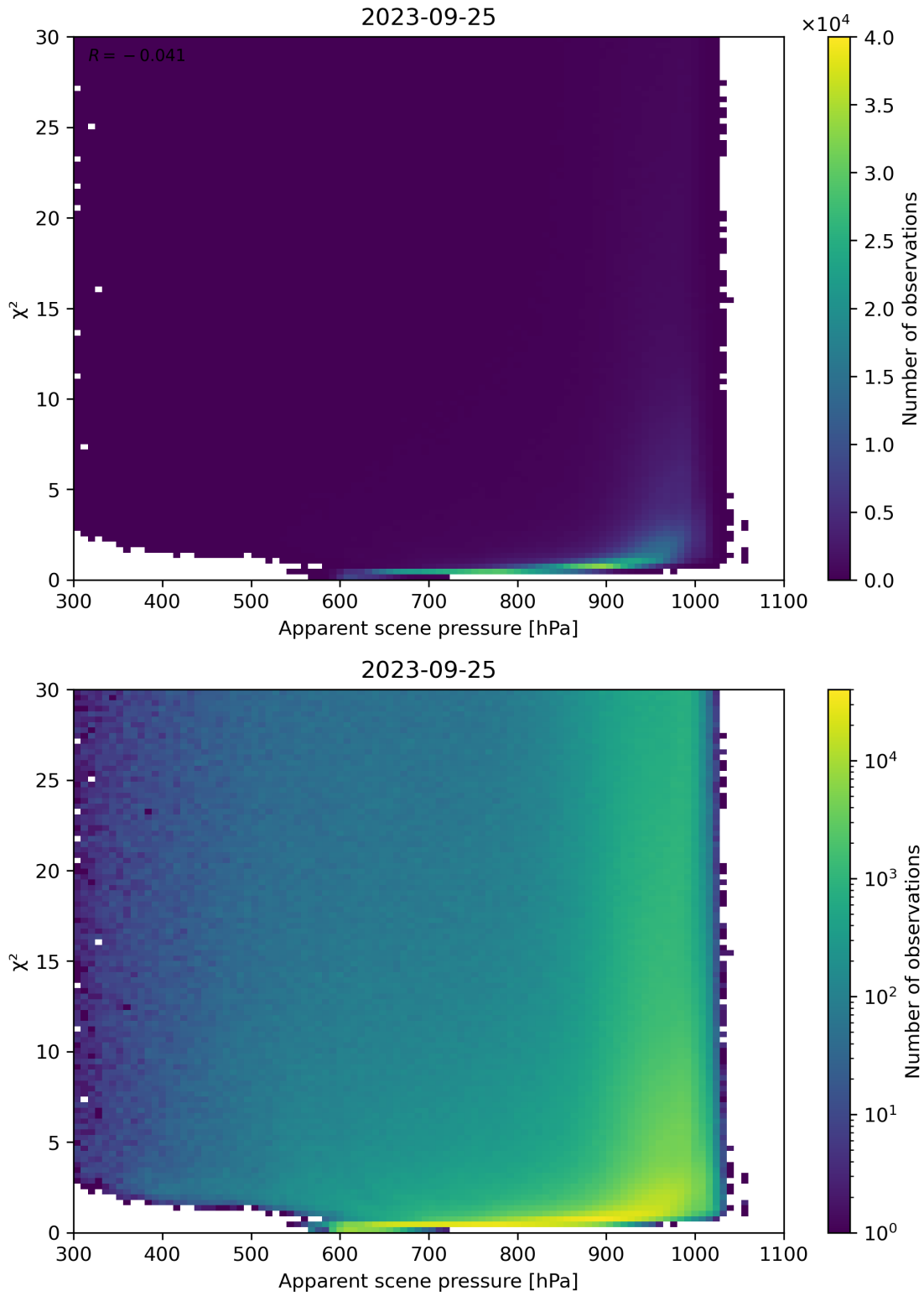
Figure 63: Scatter density plot of “Apparent scene pressure” against “ \chi^2 ” for 2023-09-24 to 2023-09-26.
