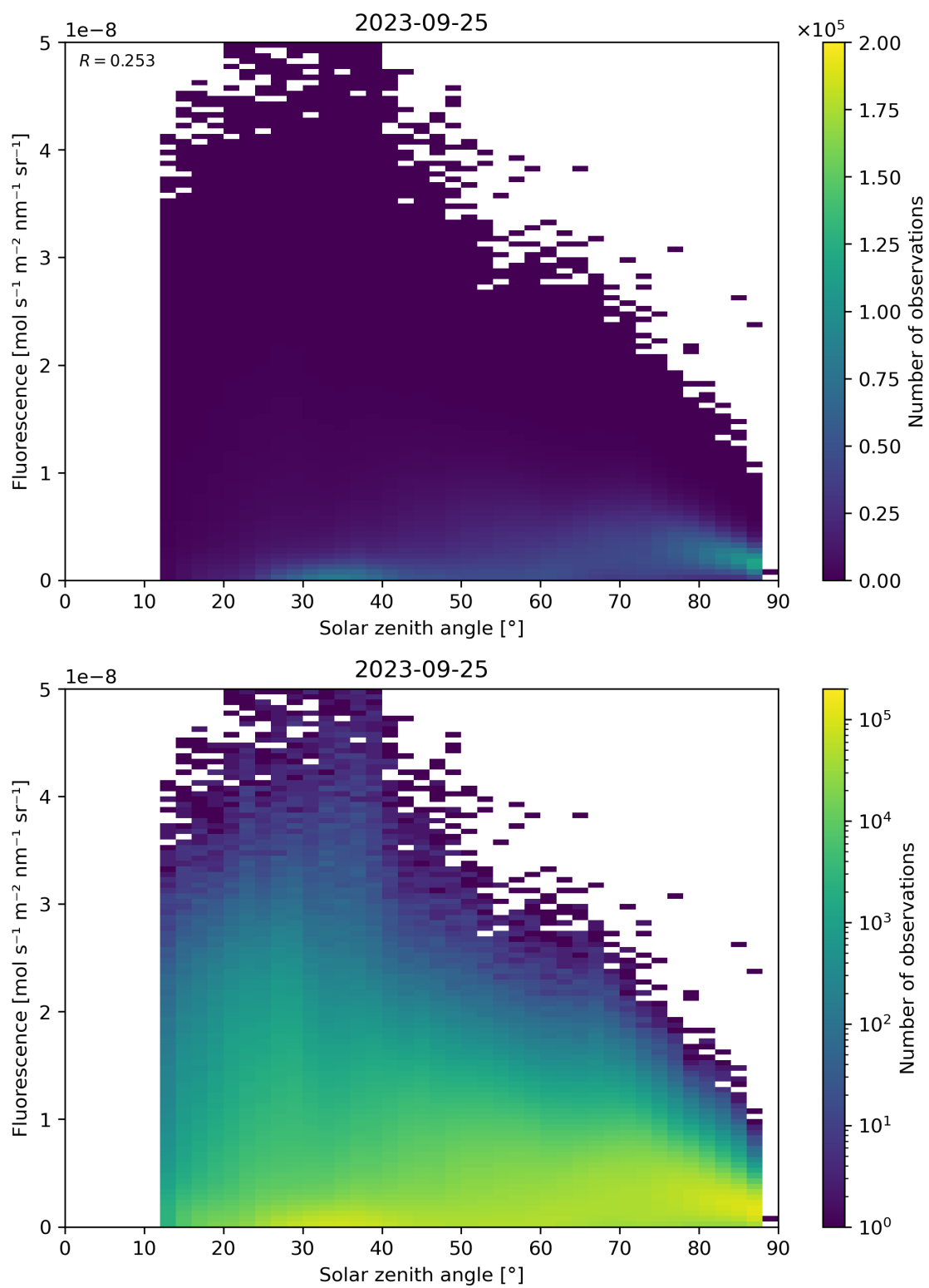
Figure 123: Scatter density plot of “Solar zenith angle” against “Fluorescence” for 2023-09-24 to 2023-09-26.
