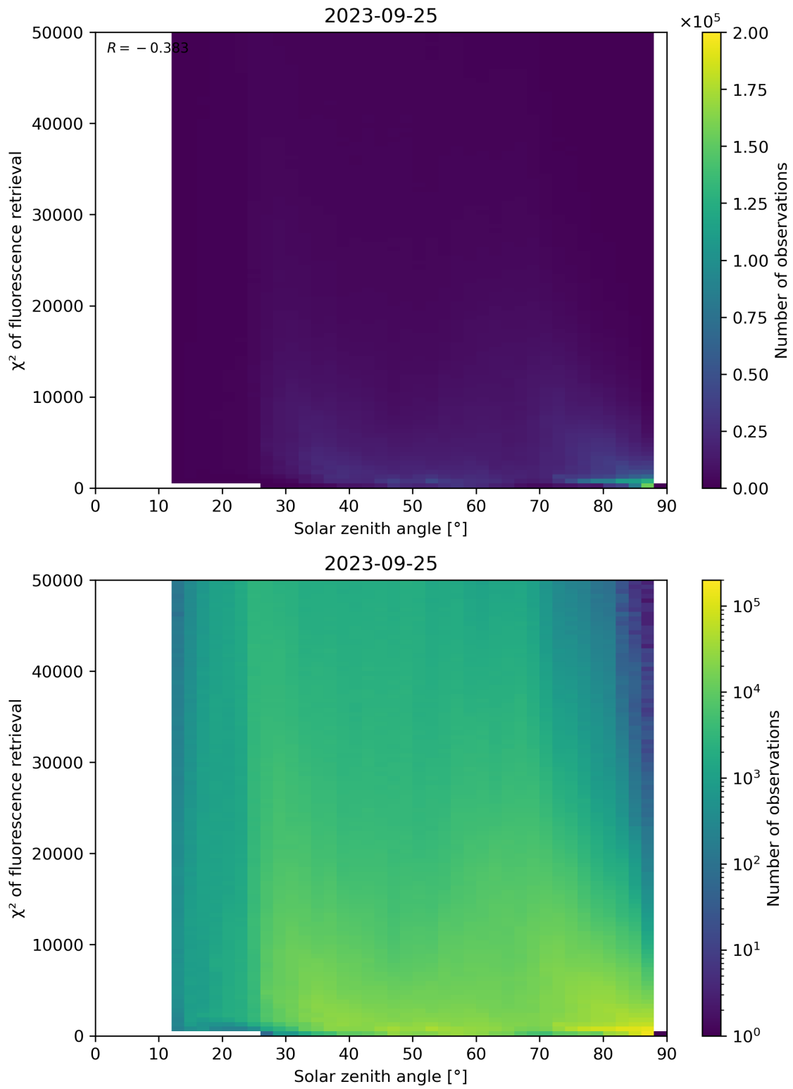
Figure 120: Scatter density plot of “Solar zenith angle” against “ \chi^2 of fluorescence retrieval” for 2023-09-24 to 2023-09-26.
