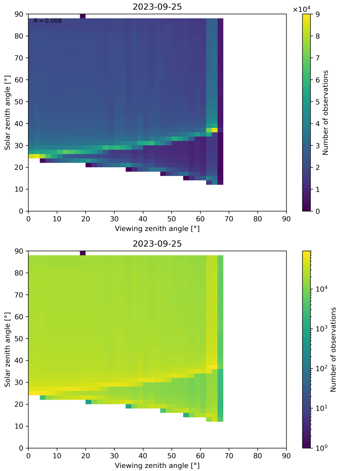
Figure 139: Scatter density plot of “Viewing zenith angle” against “Solar zenith angle” for 2023-09-24 to 2023-09-26.
