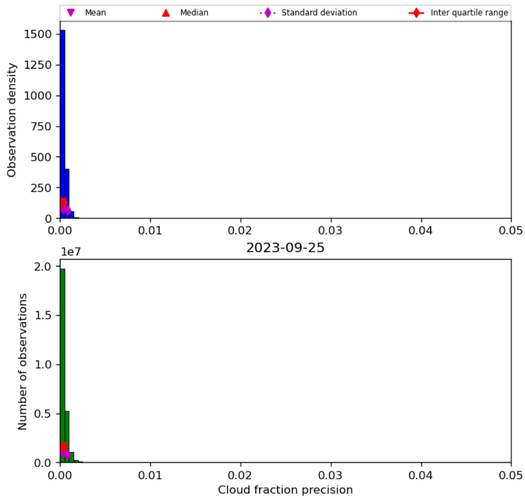
Figure 33: Histogram of “Cloud fraction precision” for 2023-09-24 to 2023-09-26
