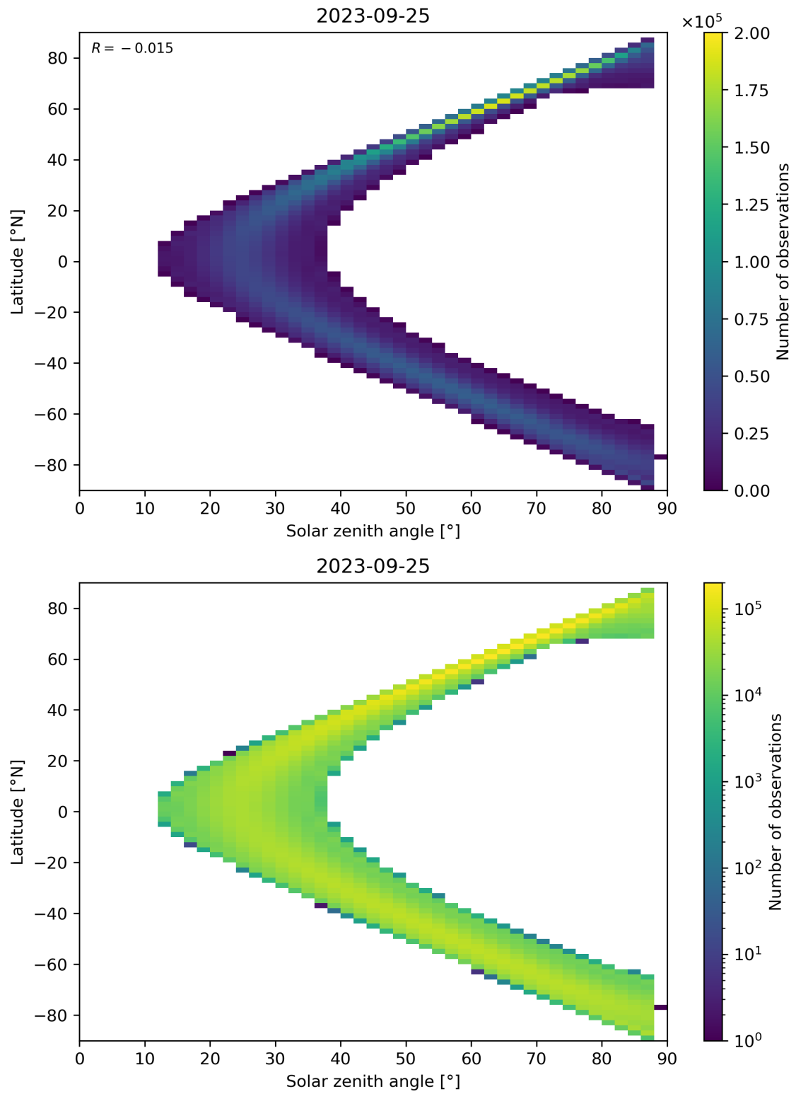
Figure 124: Scatter density plot of “Solar zenith angle” against “Latitude” for 2023-09-24 to 2023-09-26.
