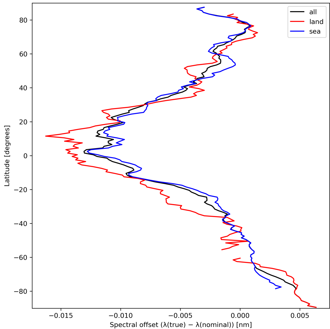
Figure 28: Zonal average of “Spectral offset ( \lambda(\text{true}) - \lambda(\text{nominal}) )” for 2023-09-24 to 2023-09-26.
