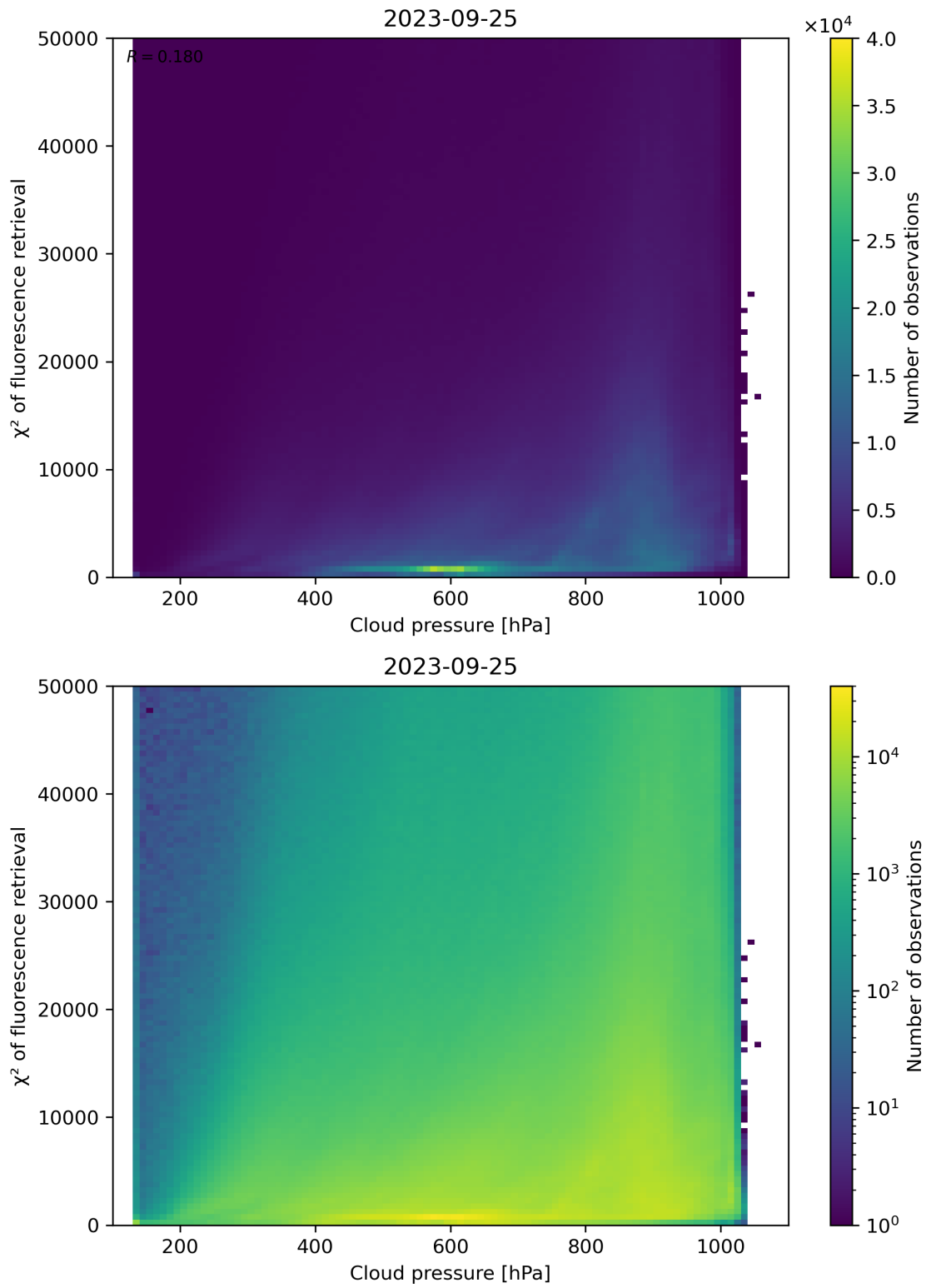
Figure 86: Scatter density plot of “Cloud pressure” against “ \chi^2 of fluorescence retrieval” for 2023-09-24 to 2023-09-26.
