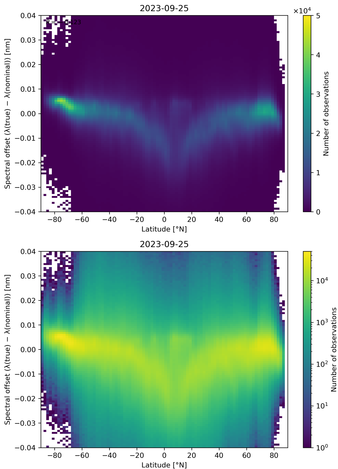
Figure 105: Scatter density plot of “Latitude” against “Spectral offset ( \lambda(\text{true}) - \lambda(\text{nominal}) )” for 2023-09-24 to 2023-09-26.
