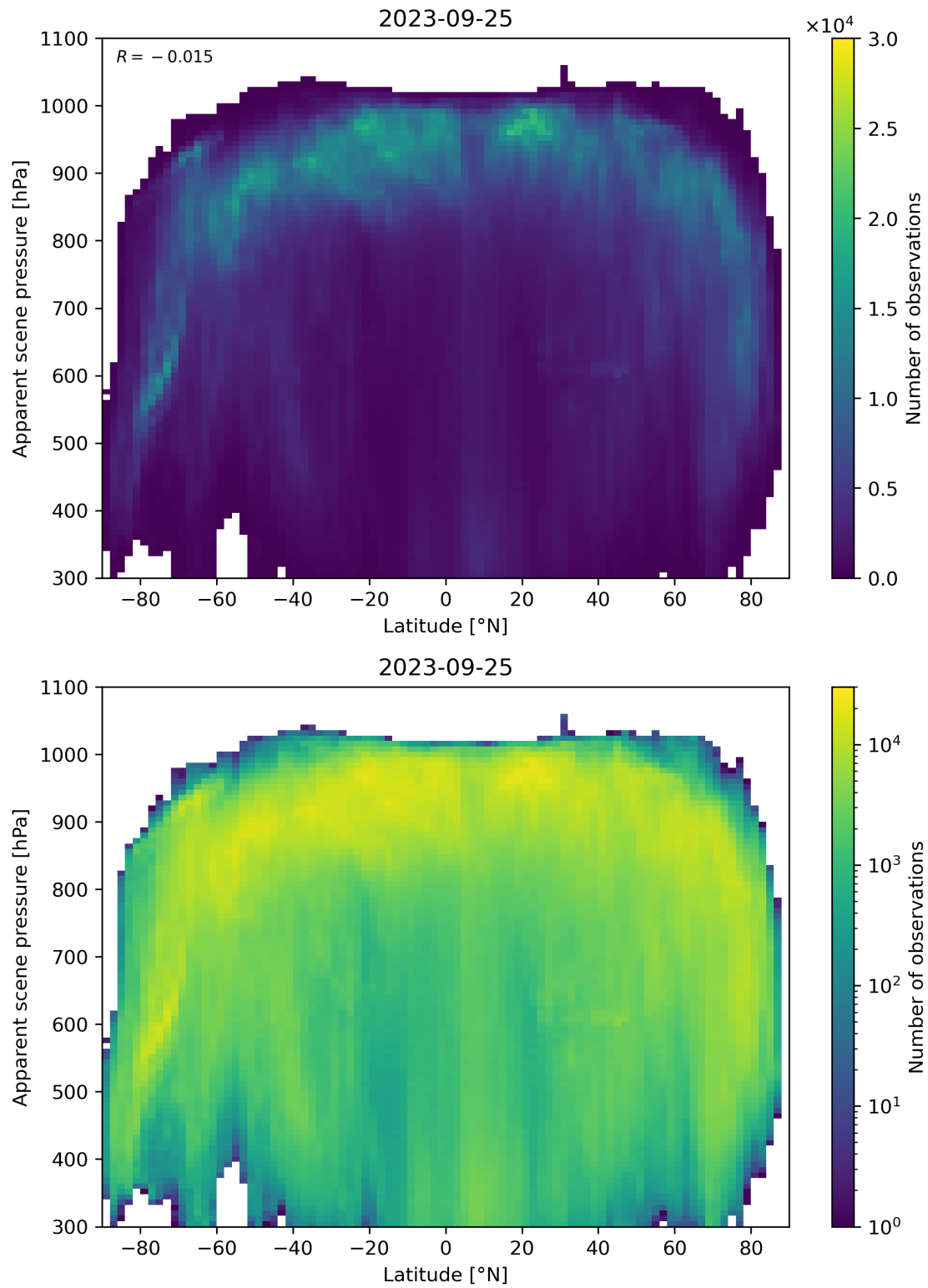
Figure 96: Scatter density plot of “Latitude” against “Apparent scene pressure” for 2023-09-24 to 2023-09-26.
