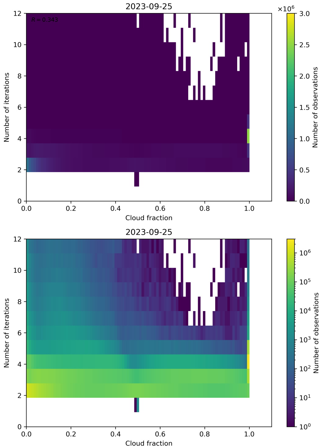
Figure 80: Scatter density plot of “Cloud fraction” against “Number of iterations” for 2023-09-24 to 2023-09-26.
