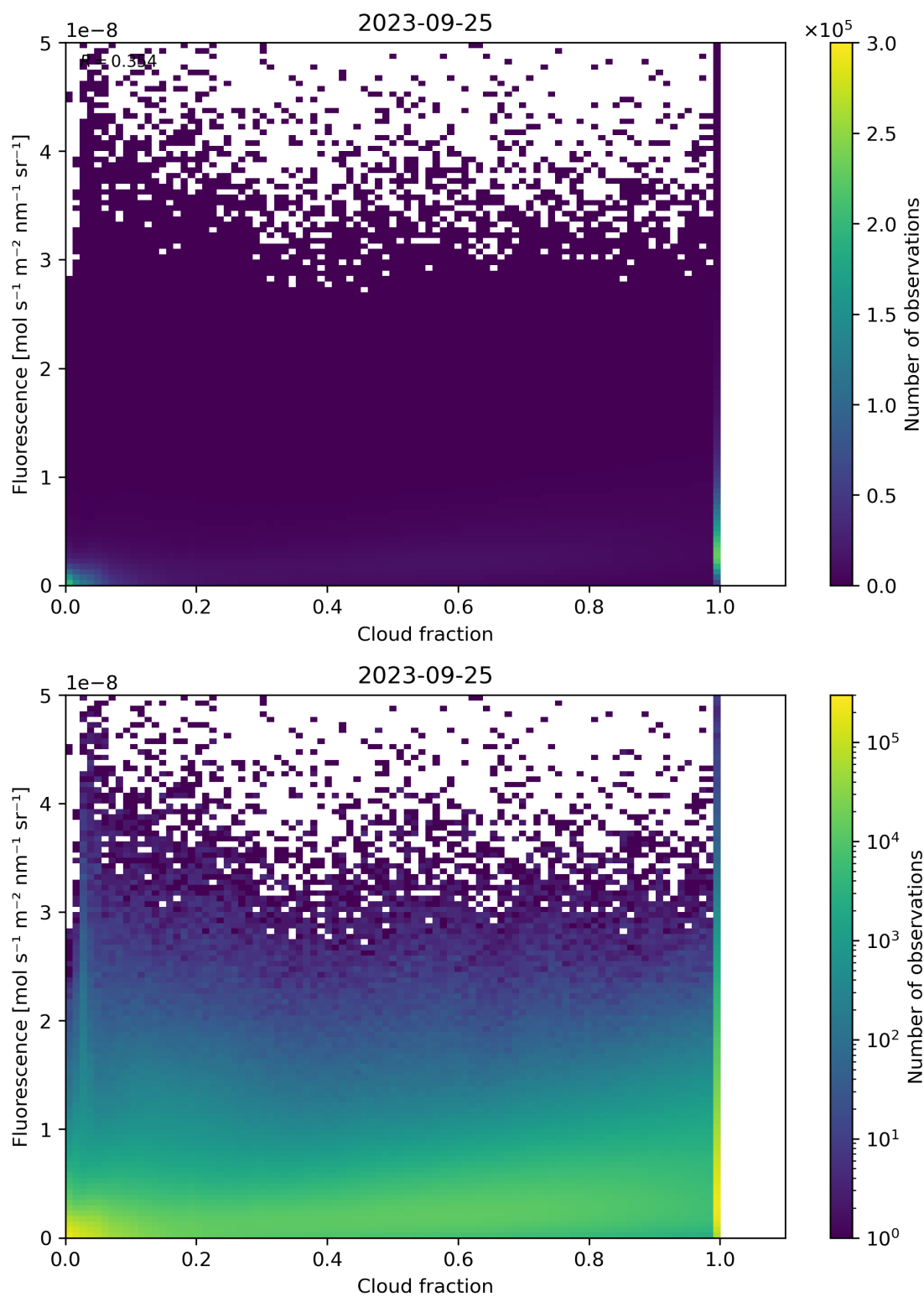
Figure 79: Scatter density plot of “Cloud fraction” against “Fluorescence” for 2023-09-24 to 2023-09-26.
