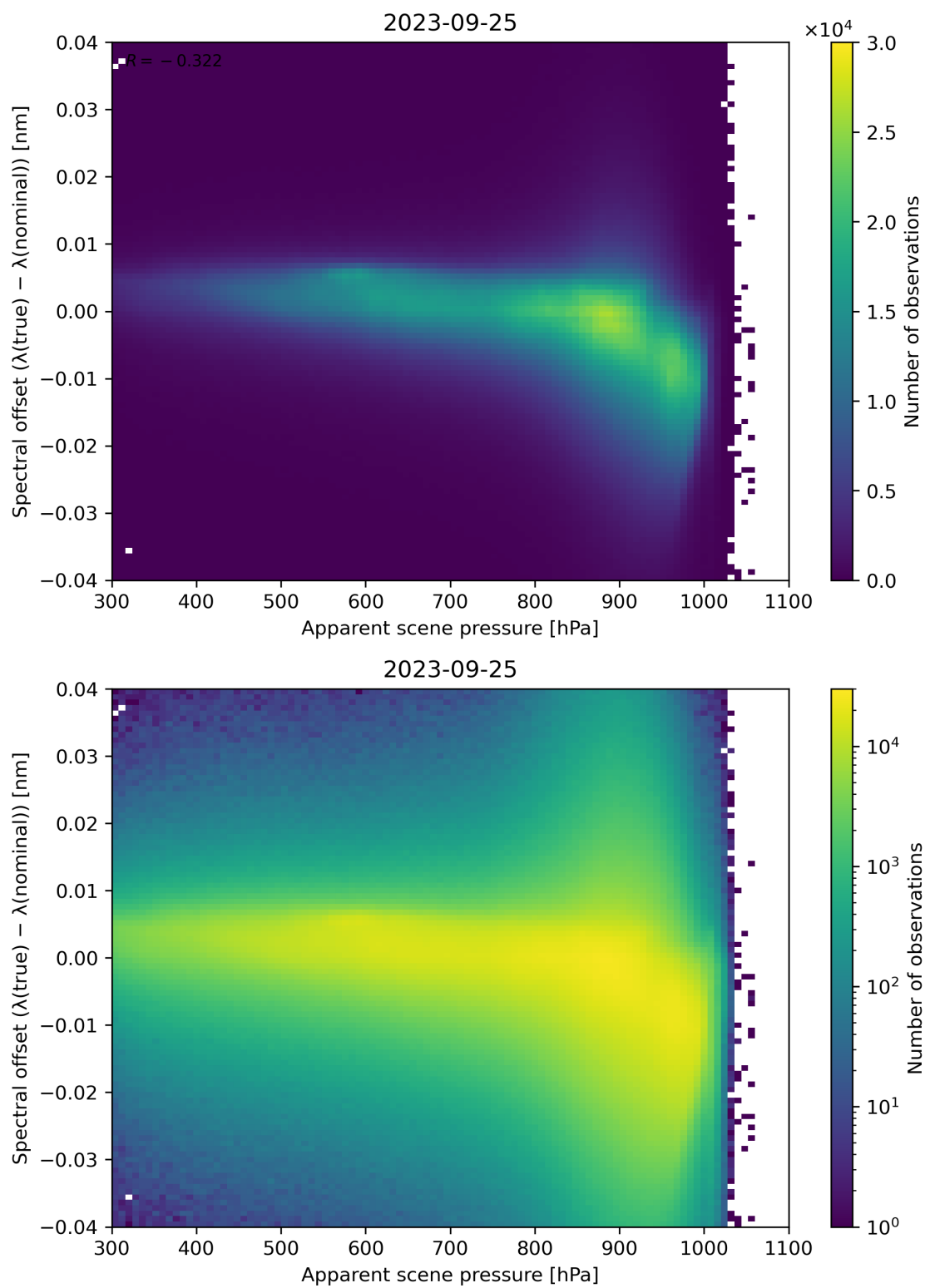
Figure 68: Scatter density plot of “Apparent scene pressure” against “Spectral offset ( \lambda(\text{true}) - \lambda(\text{nominal}) )” for 2023-09-24 to 2023-09-26.
