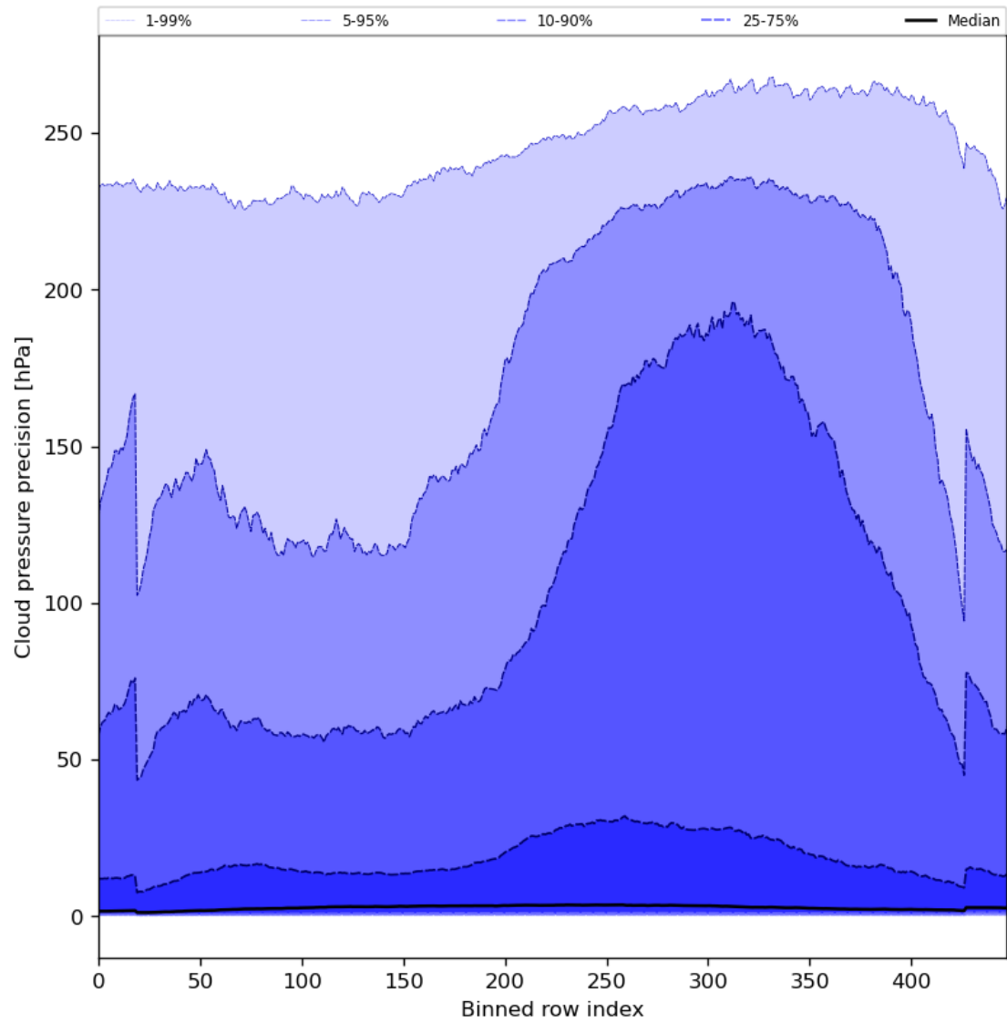
Figure 48: Along track statistics of “Cloud pressure precision” for 2023-09-24 to 2023-09-26
