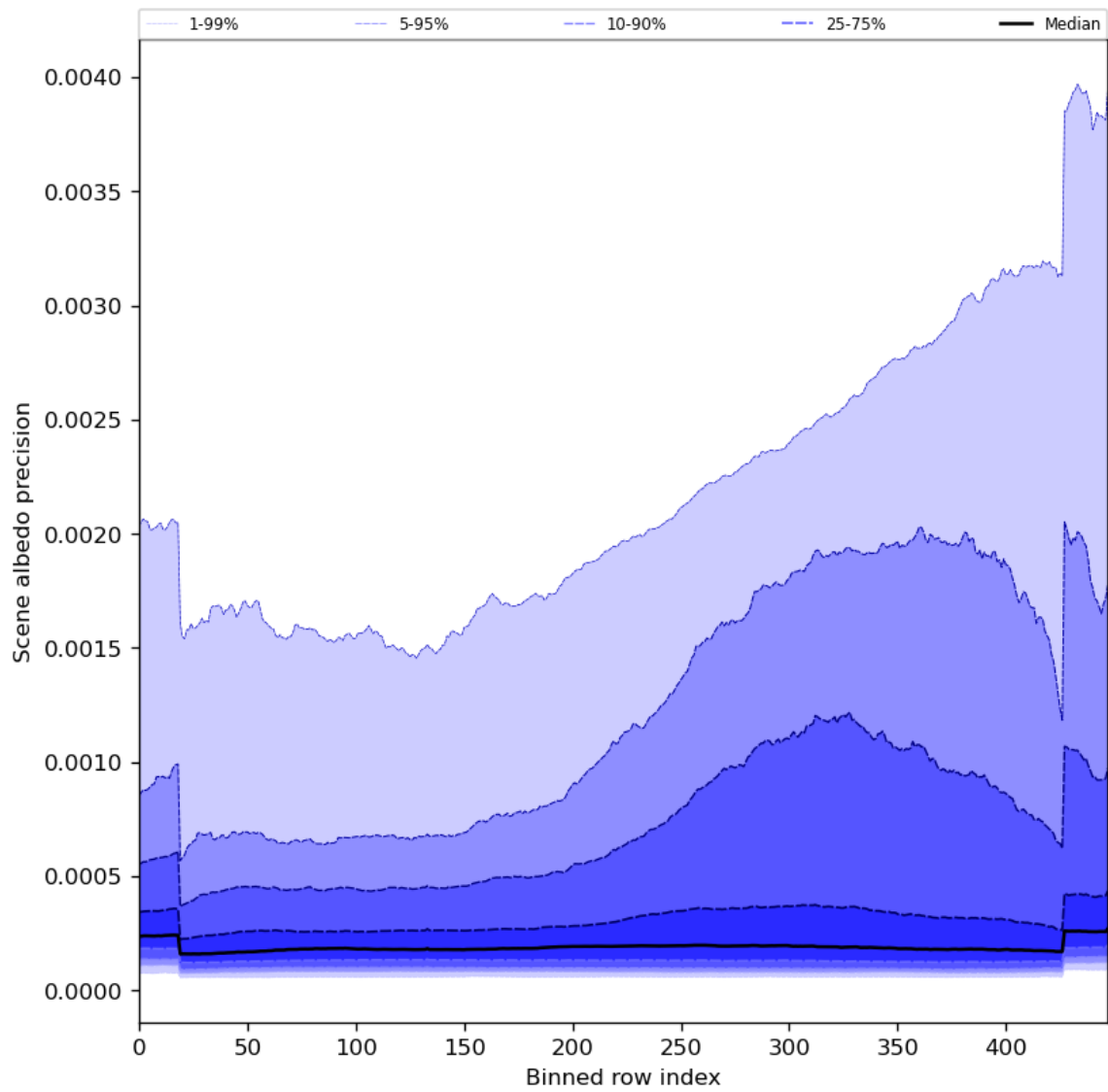
Figure 52: Along track statistics of “Scene albedo precision” for 2023-09-24 to 2023-09-26
