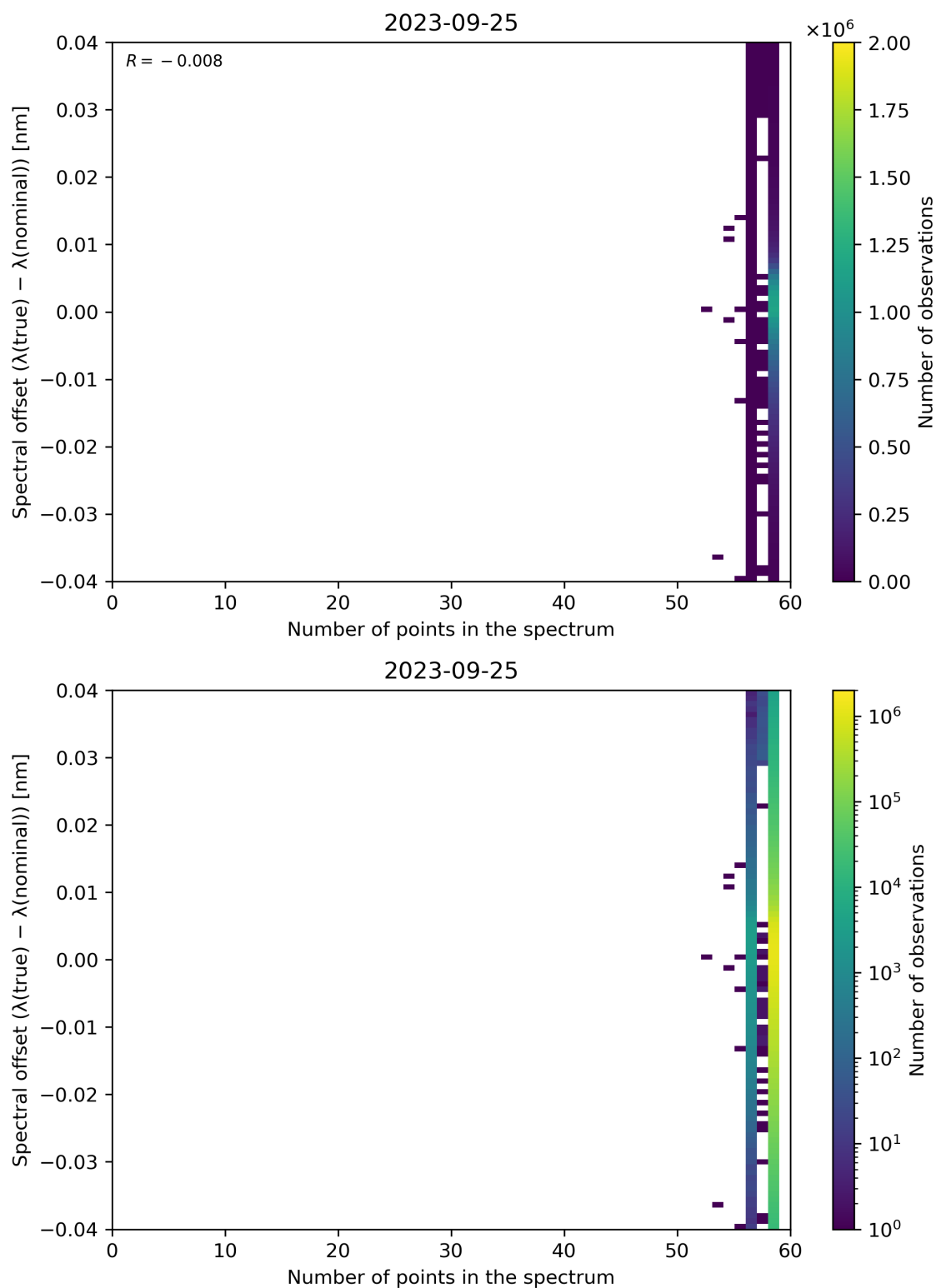
Figure 110: Scatter density plot of “Number of points in the spectrum” against “Spectral offset ( \lambda(\text{true}) - \lambda(\text{nominal}) )” for 2023-09-24 to 2023-09-26.
