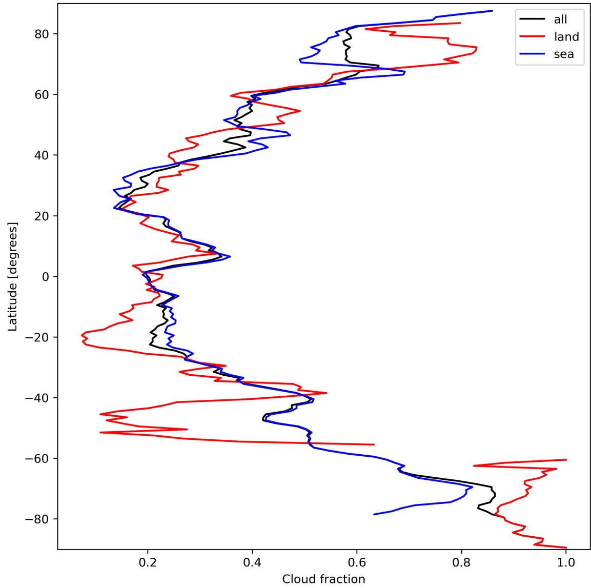
Figure 15: Zonal average of “Cloud fraction” for 2023-09-24 to 2023-09-26.
