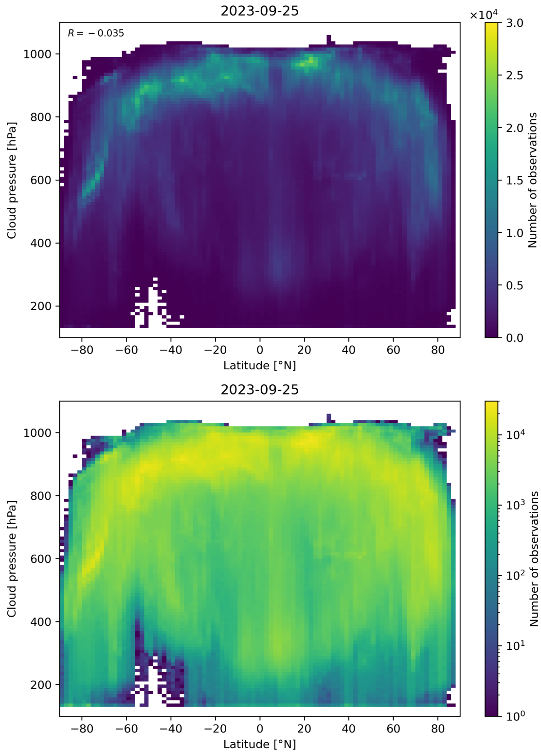
Figure 100: Scatter density plot of “Latitude” against “Cloud pressure” for 2023-09-24 to 2023-09-26.
