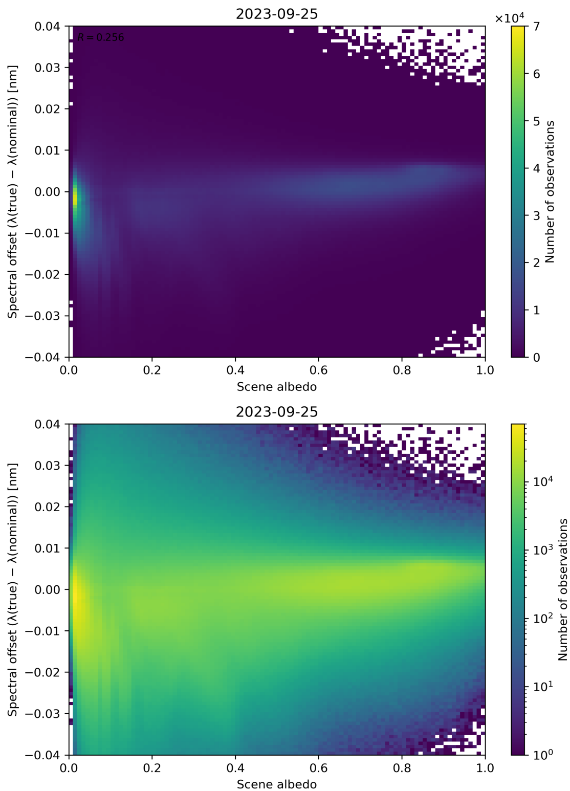
Figure 117: Scatter density plot of “Scene albedo” against “Spectral offset ( \lambda(\text{true}) - \lambda(\text{nominal}) )” for 2023-09-24 to 2023-09-26.
