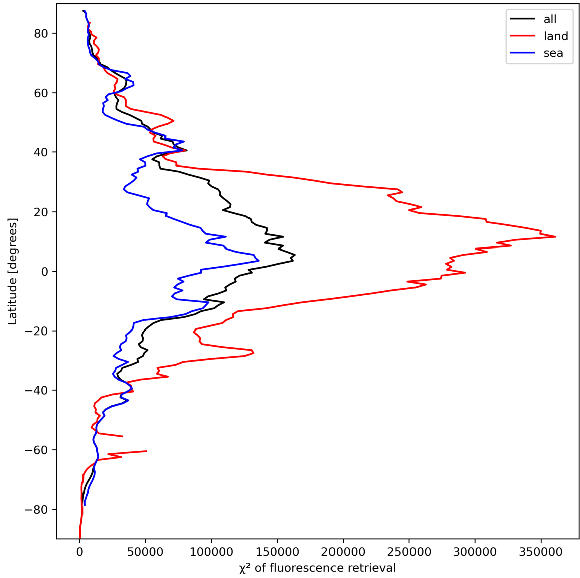
Figure 25: Zonal average of “ \chi^2 of fluorescence retrieval” for 2023-09-24 to 2023-09-26.
