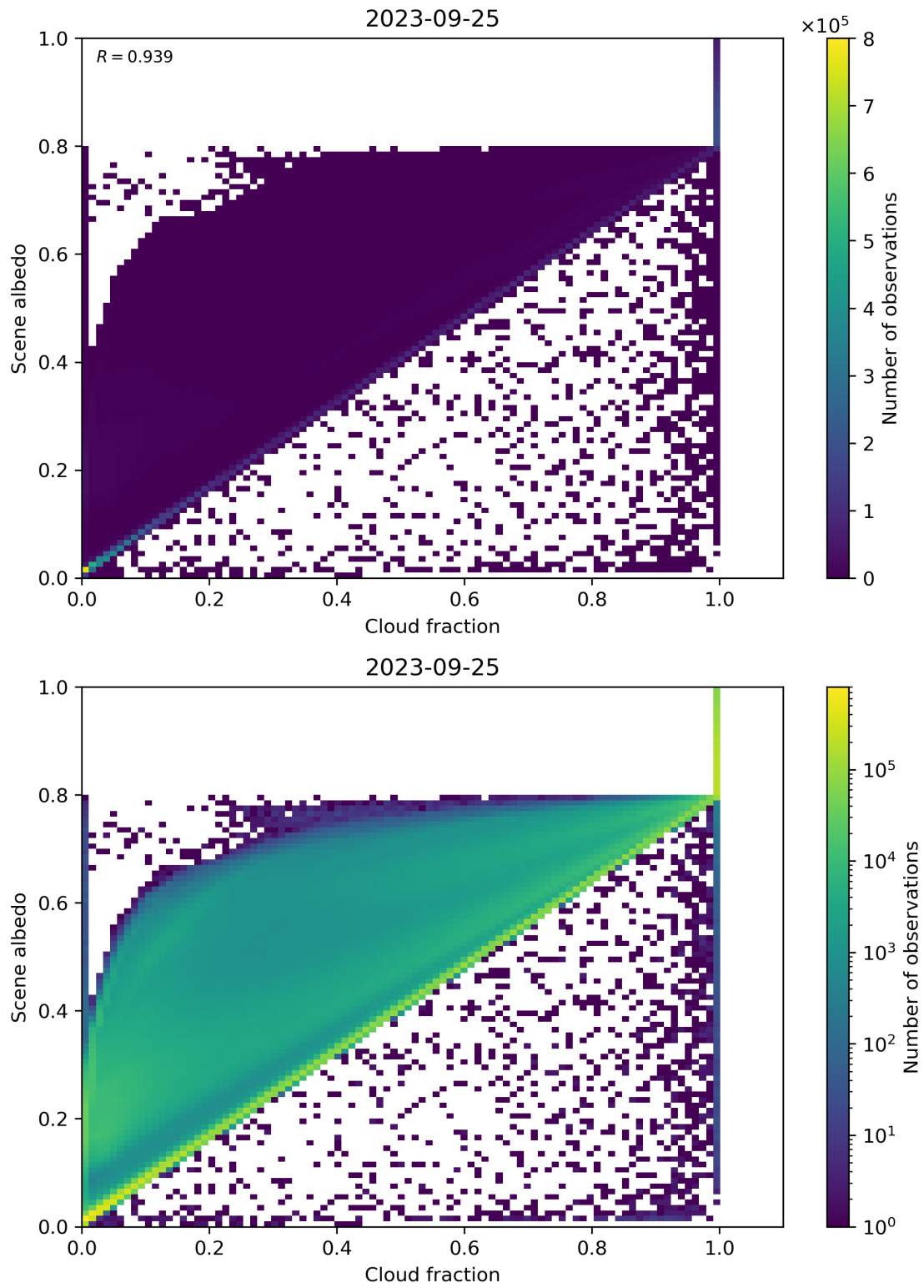
Figure 82: Scatter density plot of “Cloud fraction” against “Scene albedo” for 2023-09-24 to 2023-09-26.
