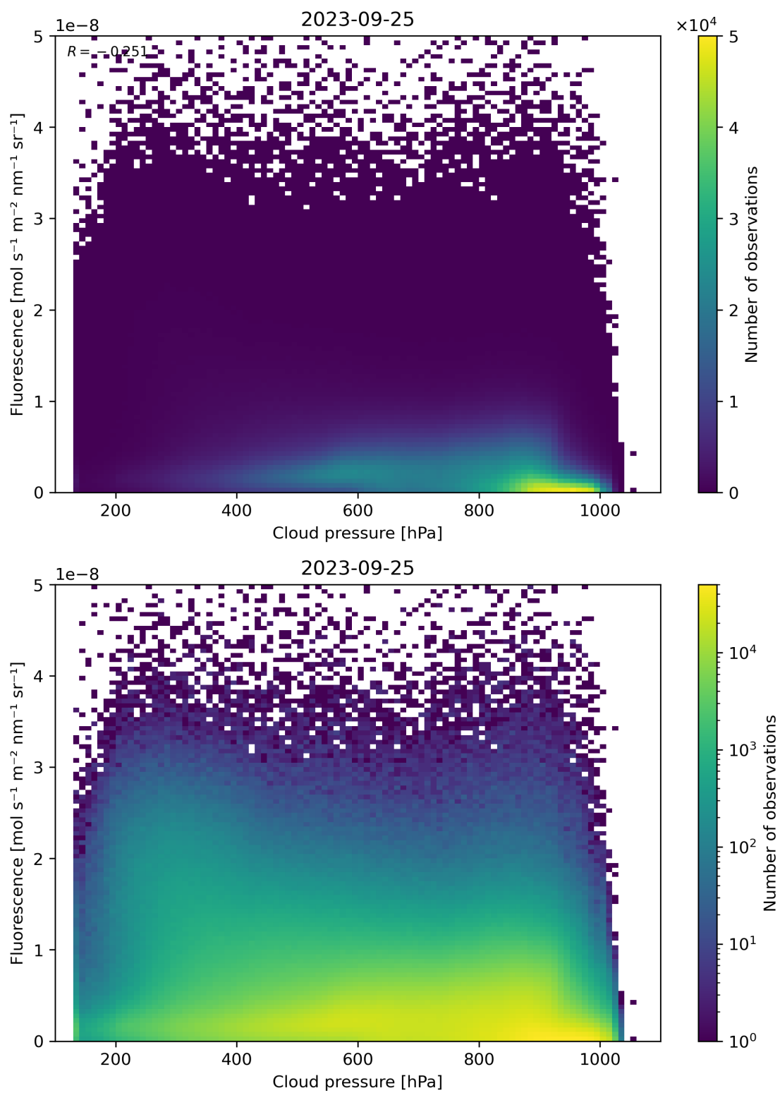
Figure 88: Scatter density plot of “Cloud pressure” against “Fluorescence” for 2023-09-24 to 2023-09-26.
