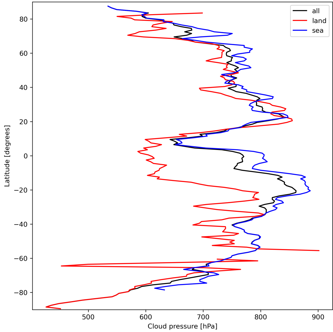
Figure 13: Zonal average of “Cloud pressure” for 2023-09-24 to 2023-09-26.
