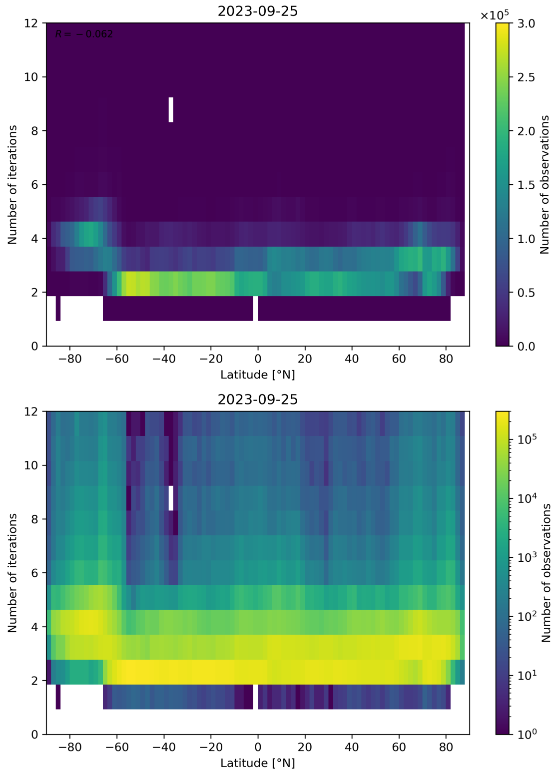
Figure 102: Scatter density plot of “Latitude” against “Number of iterations” for 2023-09-24 to 2023-09-26.
