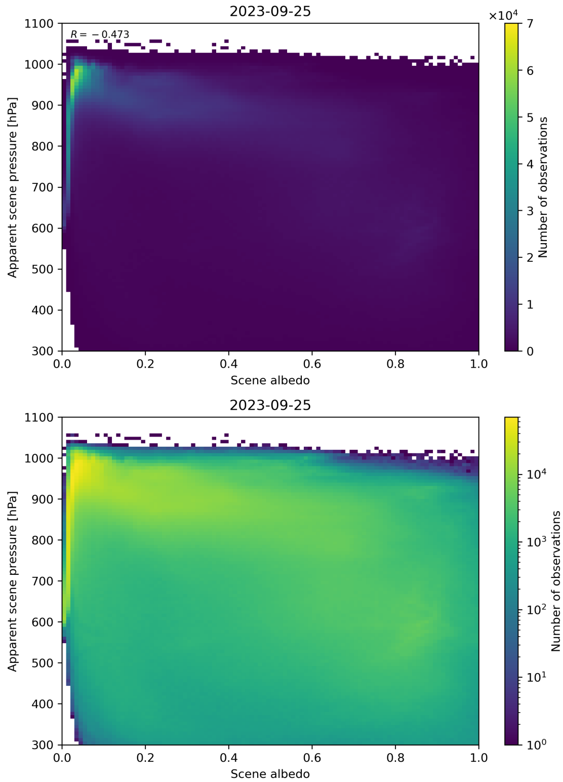
Figure 111: Scatter density plot of “Scene albedo” against “Apparent scene pressure” for 2023-09-24 to 2023-09-26.
