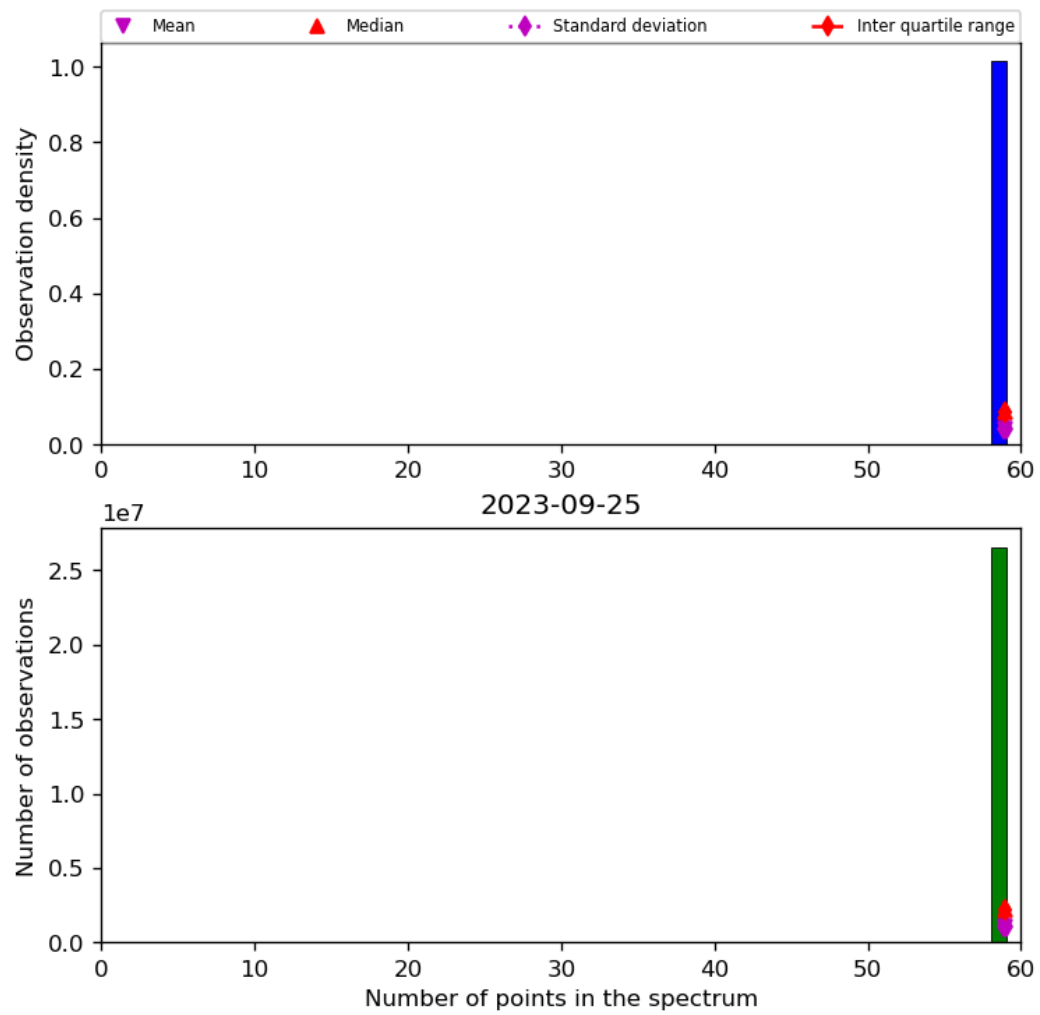
Figure 44: Histogram of "Number of points in the spectrum" for 2023-09-24 to 2023-09-26
