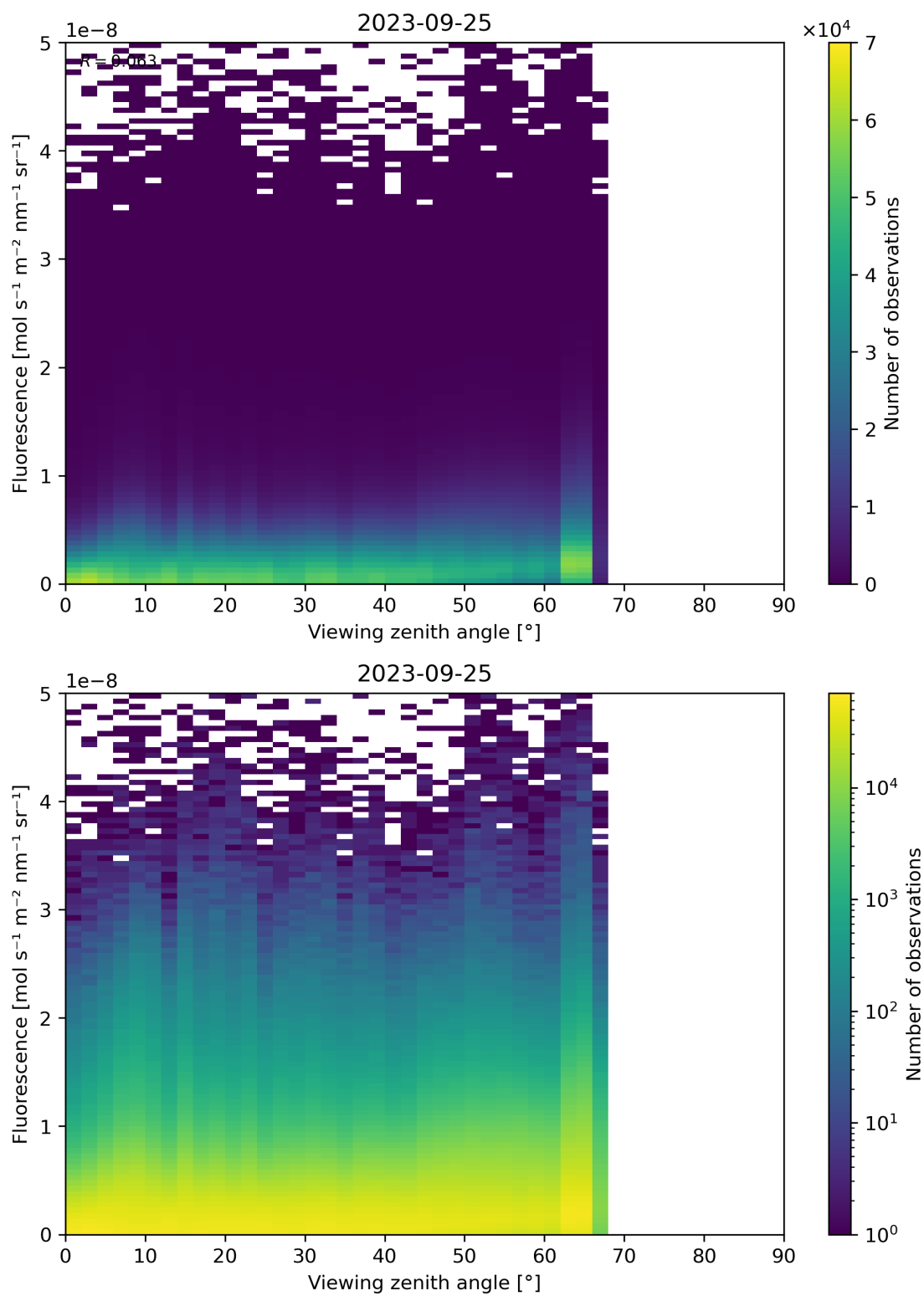
Figure 134: Scatter density plot of “Viewing zenith angle” against “Fluorescence” for 2023-09-24 to 2023-09-26.
