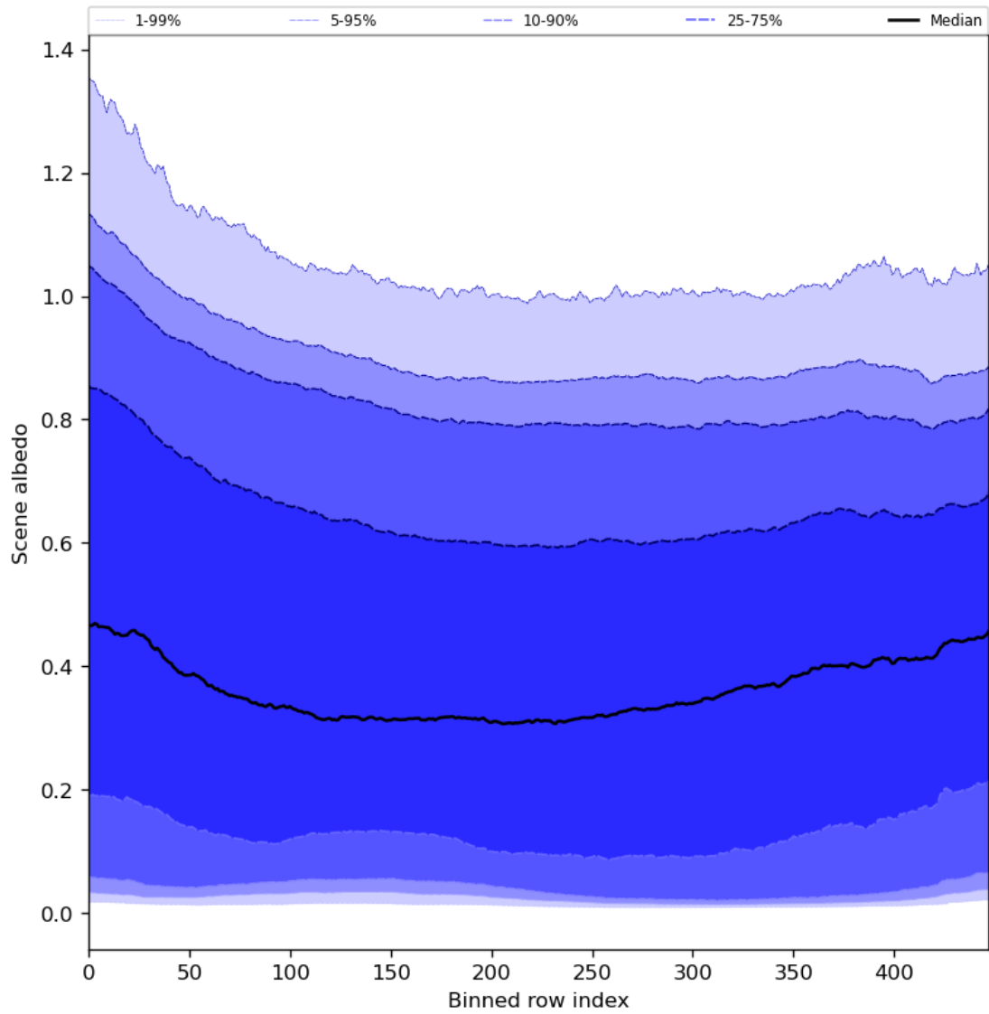
Figure 51: Along track statistics of “Scene albedo” for 2023-09-24 to 2023-09-26
