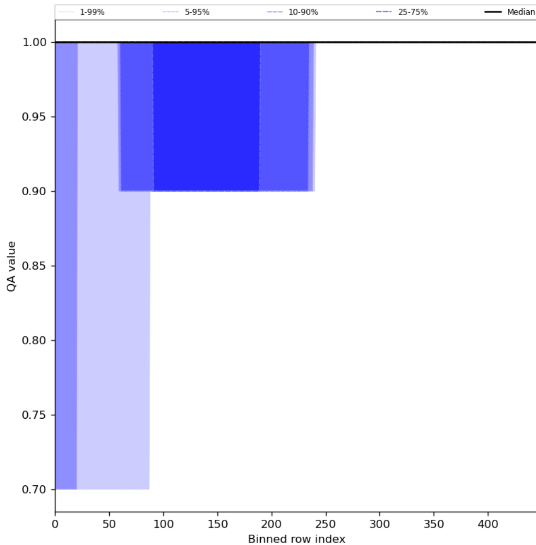
Figure 46: Along track statistics of “QA value” for 2023-09-24 to 2023-09-26
