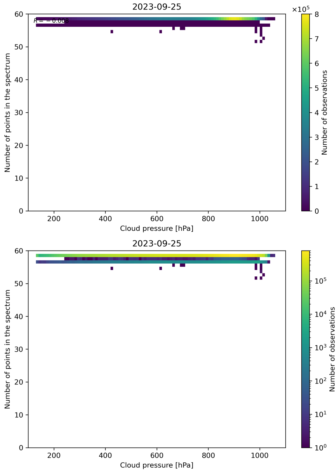
Figure 90: Scatter density plot of “Cloud pressure” against “Number of points in the spectrum” for 2023-09-24 to 2023-09-26.
