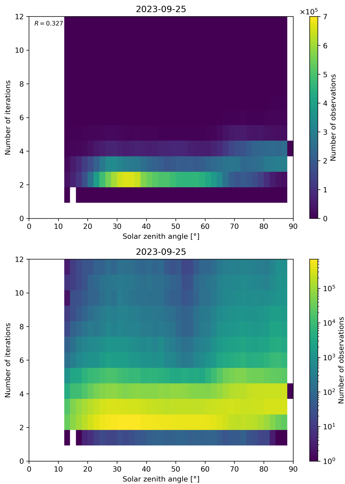
Figure 125: Scatter density plot of “Solar zenith angle” against “Number of iterations” for 2023-09-24 to 2023-09-26.
