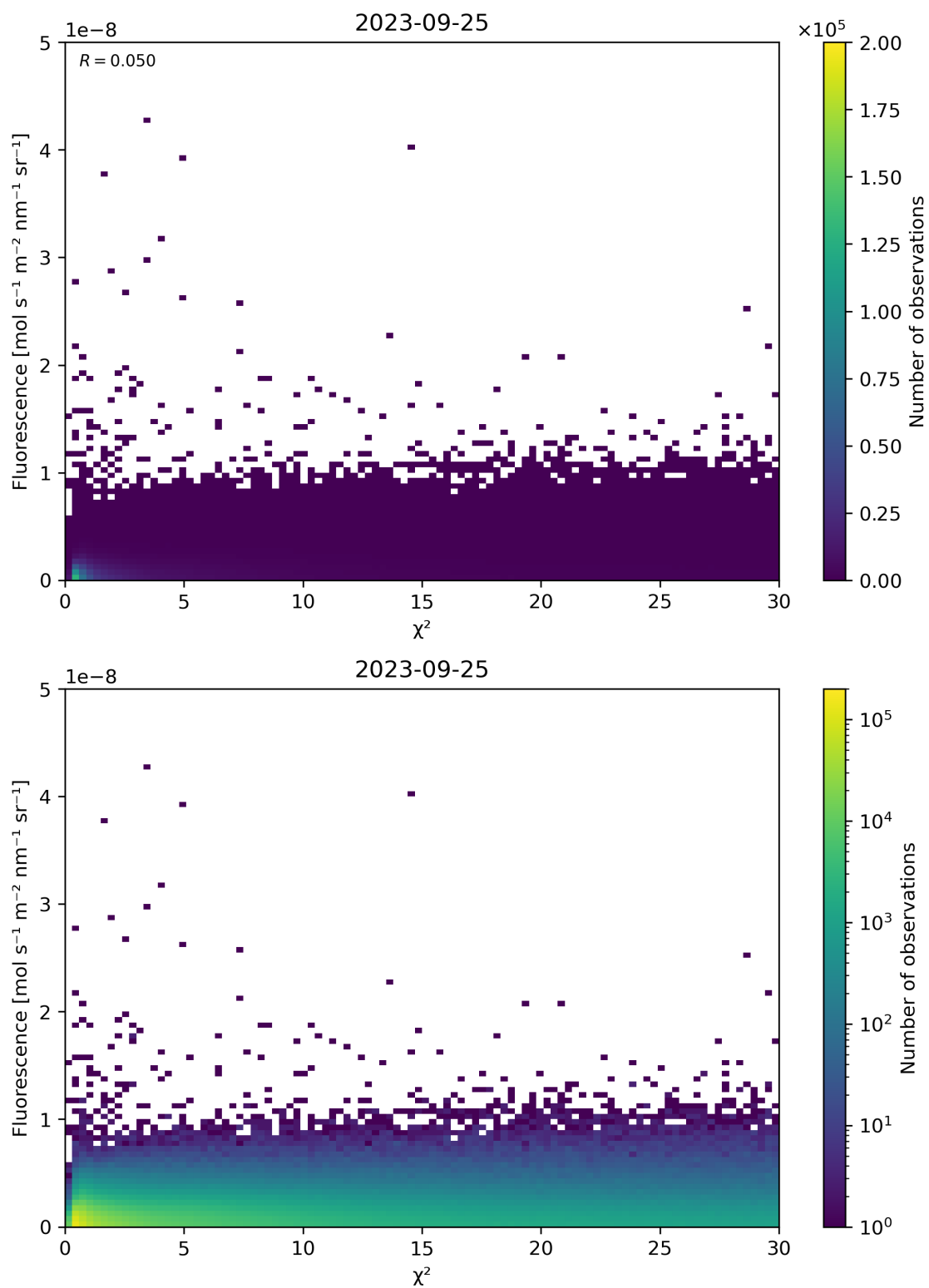
Figure 70: Scatter density plot of “ \chi^2 ” against “Fluorescence” for 2023-09-24 to 2023-09-26.
