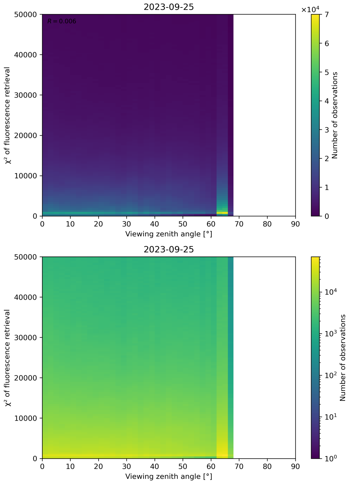
Figure 131: Scatter density plot of “Viewing zenith angle” against “ \chi^2 of fluorescence retrieval” for 2023-09-24 to 2023-09-26.
