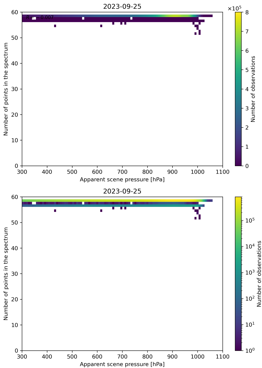
Figure 67: Scatter density plot of “Apparent scene pressure” against “Number of points in the spectrum” for 2023-09-24 to 2023-09-26.
