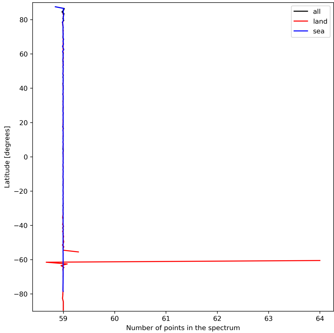
Figure 27: Zonal average of “Number of points in the spectrum” for 2023-09-24 to 2023-09-26.
