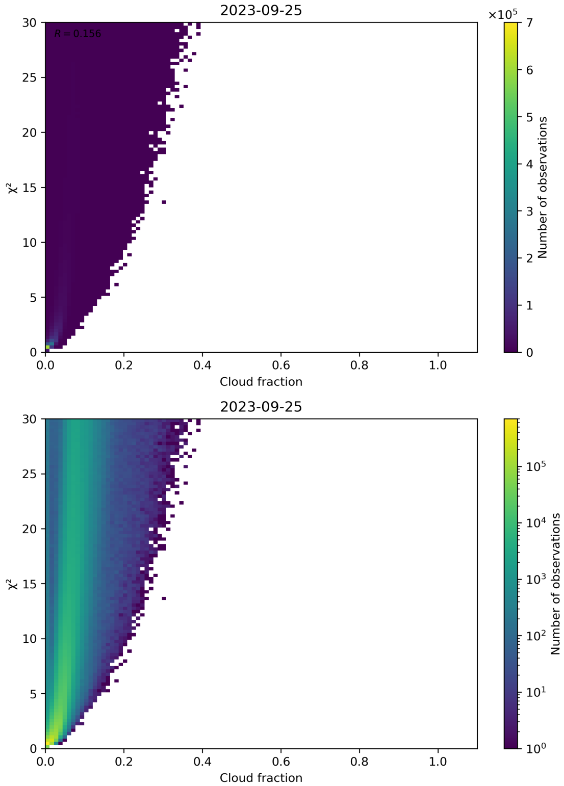
Figure 77: Scatter density plot of “Cloud fraction” against “ \chi^2 ” for 2023-09-24 to 2023-09-26.
