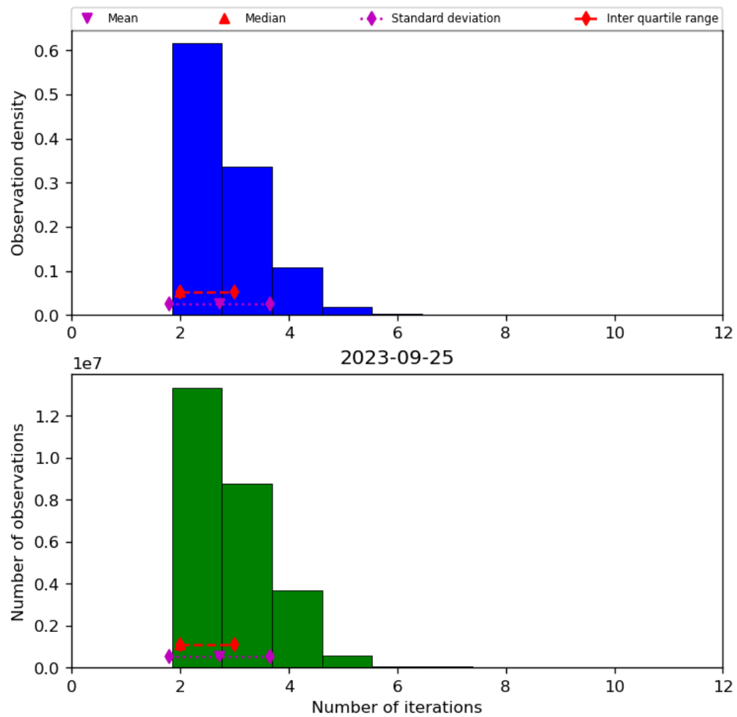
Figure 39: Histogram of “Number of iterations” for 2023-09-24 to 2023-09-26
