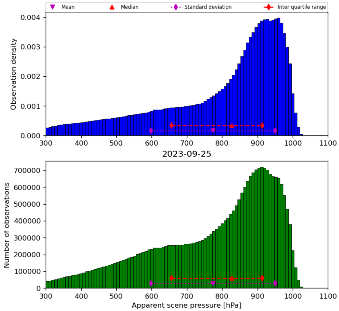
Figure 36: Histogram of “Apparent scene pressure” for 2023-09-24 to 2023-09-26
