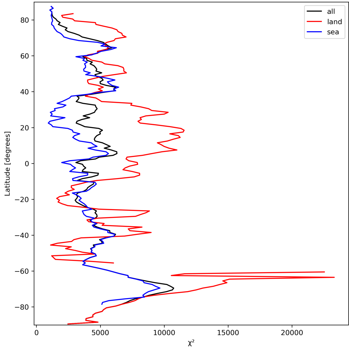
Figure 21: Zonal average of “ \chi^2 ” for 2023-09-24 to 2023-09-26.
