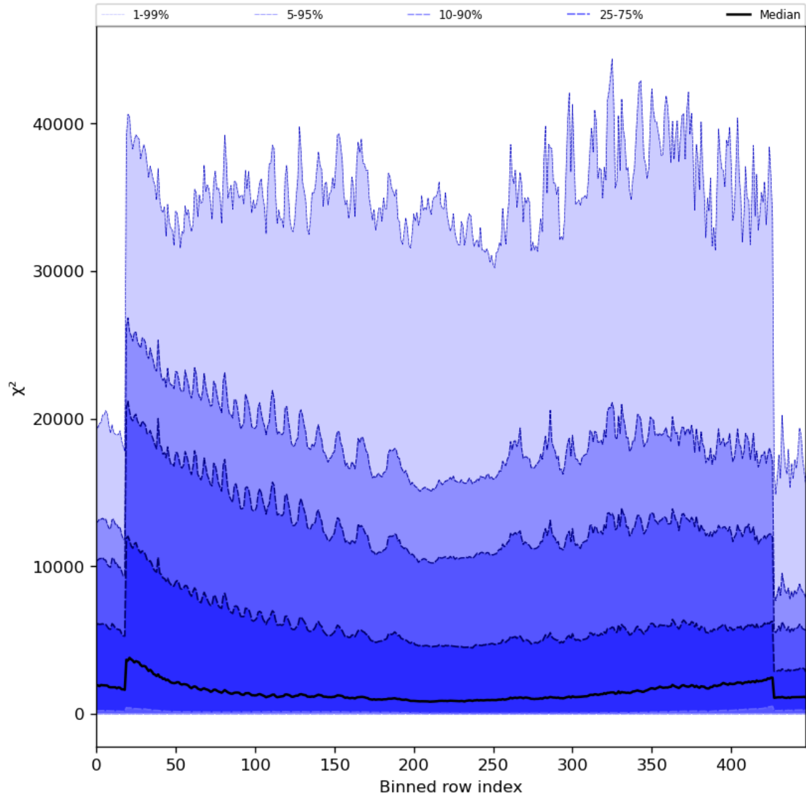
Figure 55: Along track statistics of “ \chi^2 ” for 2023-09-24 to 2023-09-26
