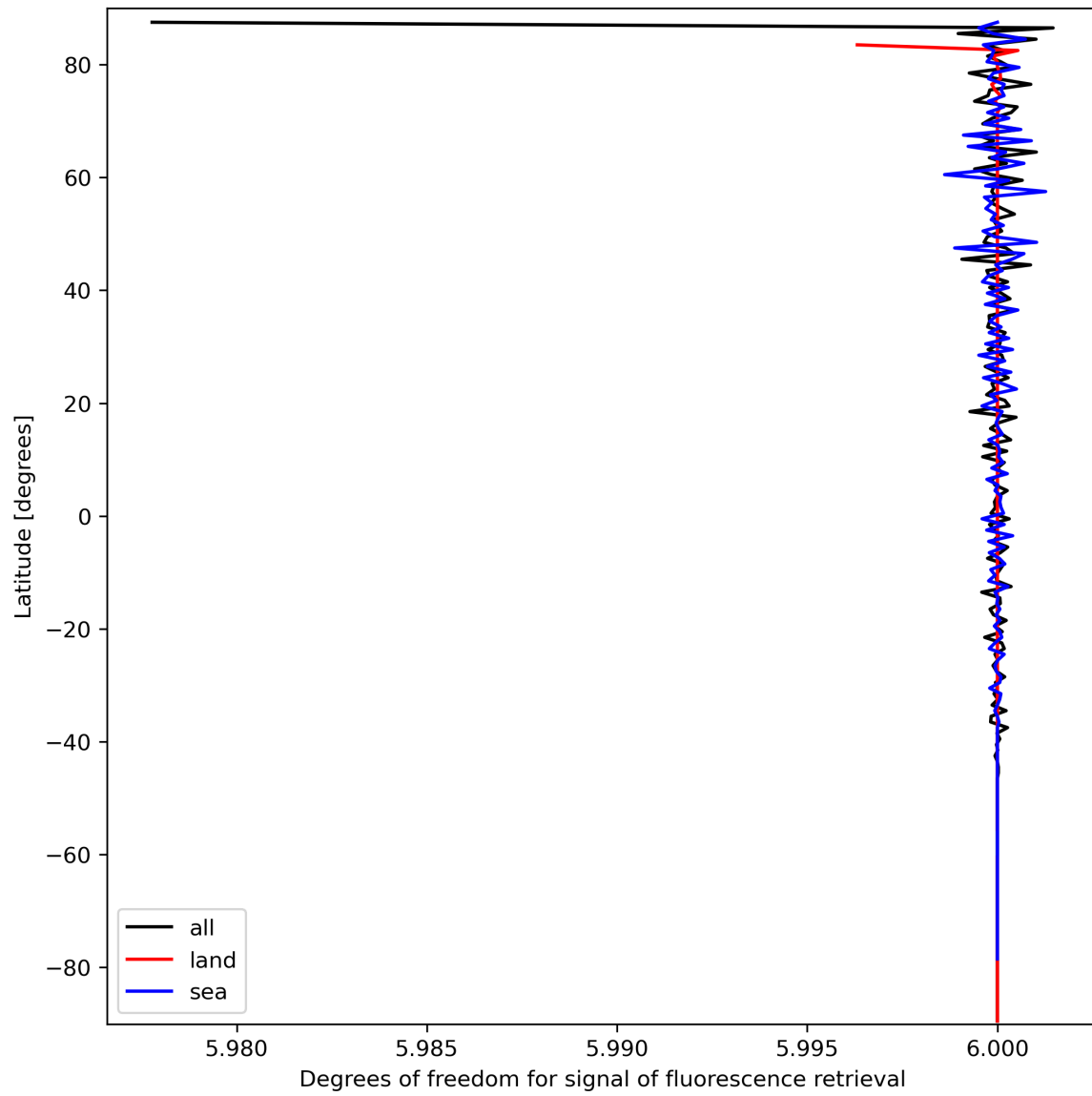
Figure 26: Zonal average of “Degrees of freedom for signal of fluorescence retrieval” for 2023-09-24 to 2023-09-26.
