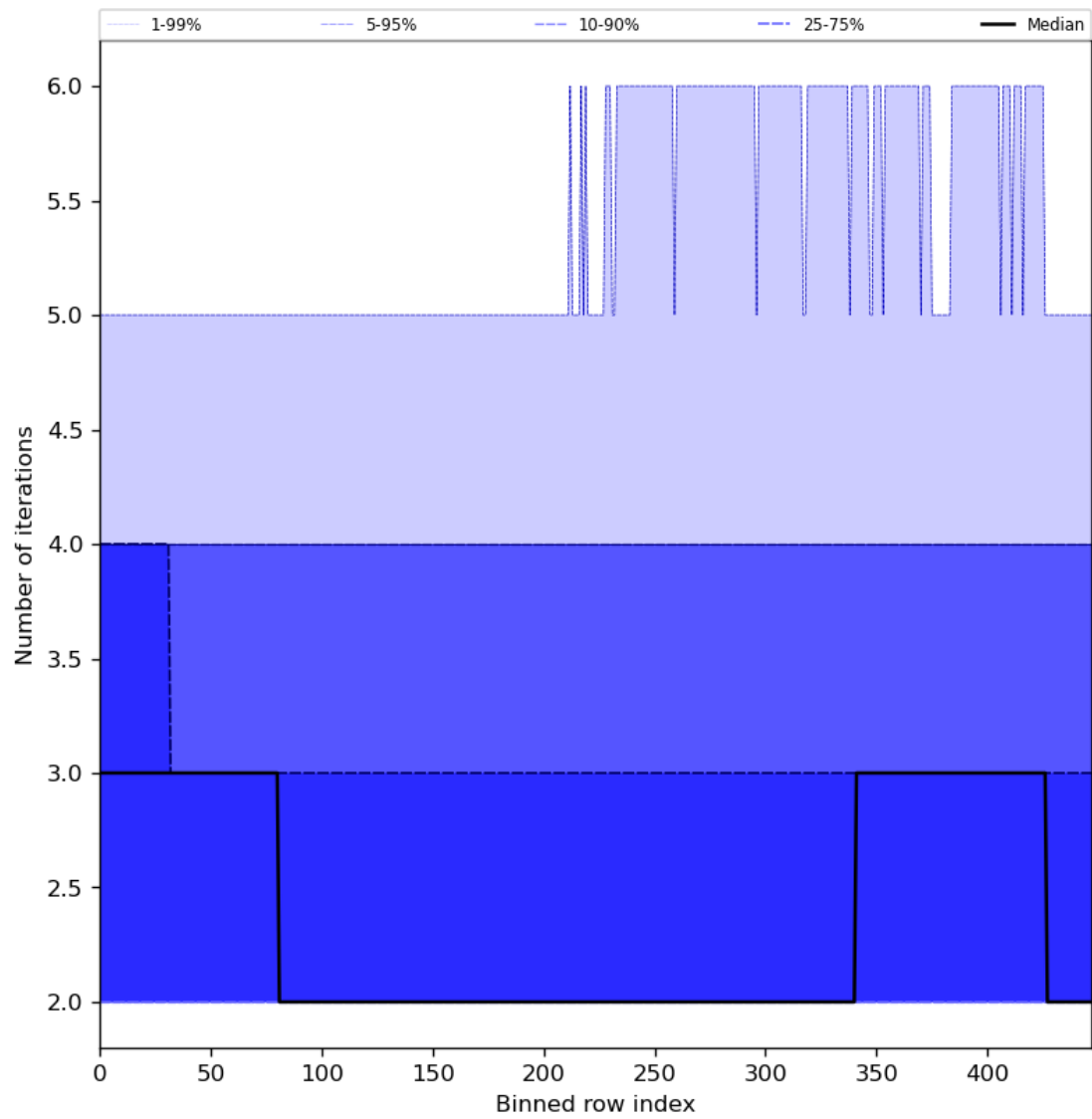
Figure 56: Along track statistics of “Number of iterations” for 2023-09-24 to 2023-09-26
