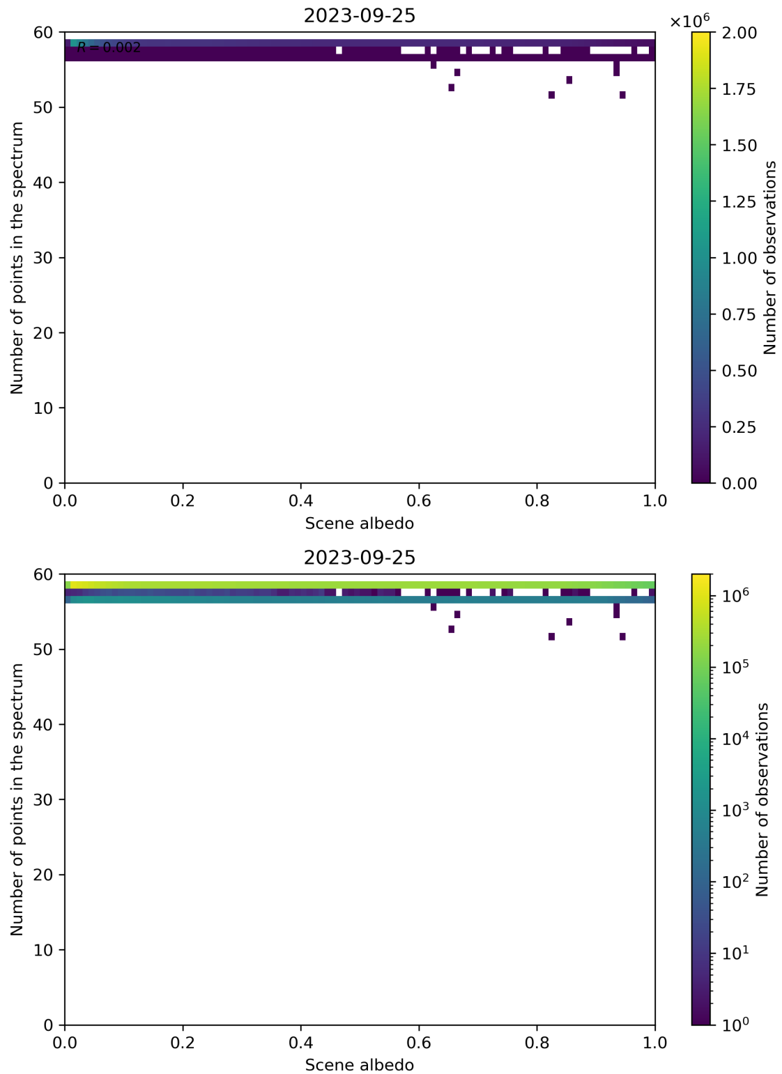
Figure 116: Scatter density plot of “Scene albedo” against “Number of points in the spectrum” for 2023-09-24 to 2023-09-26.
