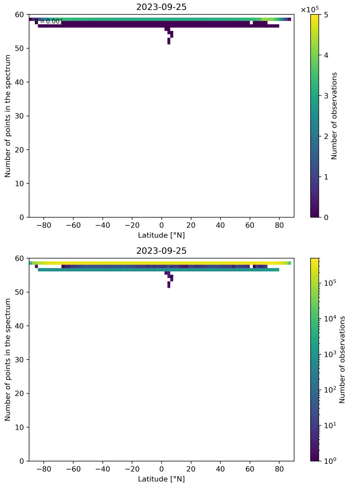
Figure 103: Scatter density plot of “Latitude” against “Number of points in the spectrum” for 2023-09-24 to 2023-09-26.
