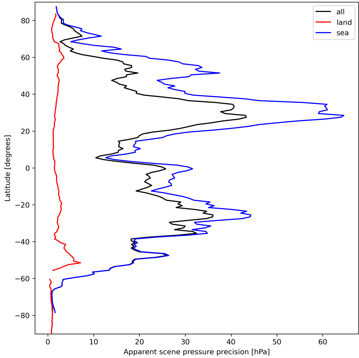
Figure 20: Zonal average of “Apparent scene pressure precision” for 2023-09-24 to 2023-09-26.
