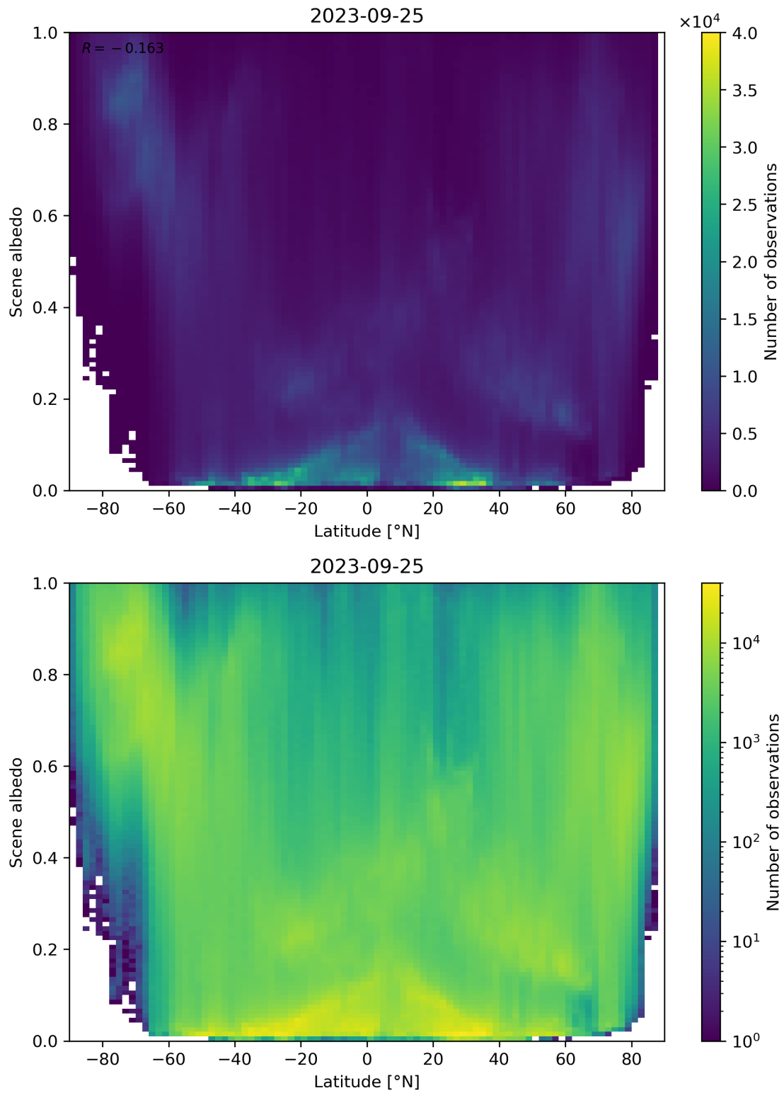
Figure 104: Scatter density plot of “Latitude” against “Scene albedo” for 2023-09-24 to 2023-09-26.
