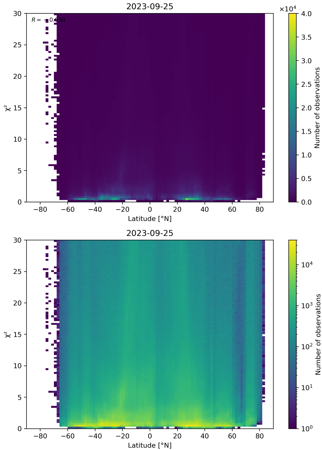
Figure 97: Scatter density plot of “Latitude” against “ \chi^2 ” for 2023-09-24 to 2023-09-26.
