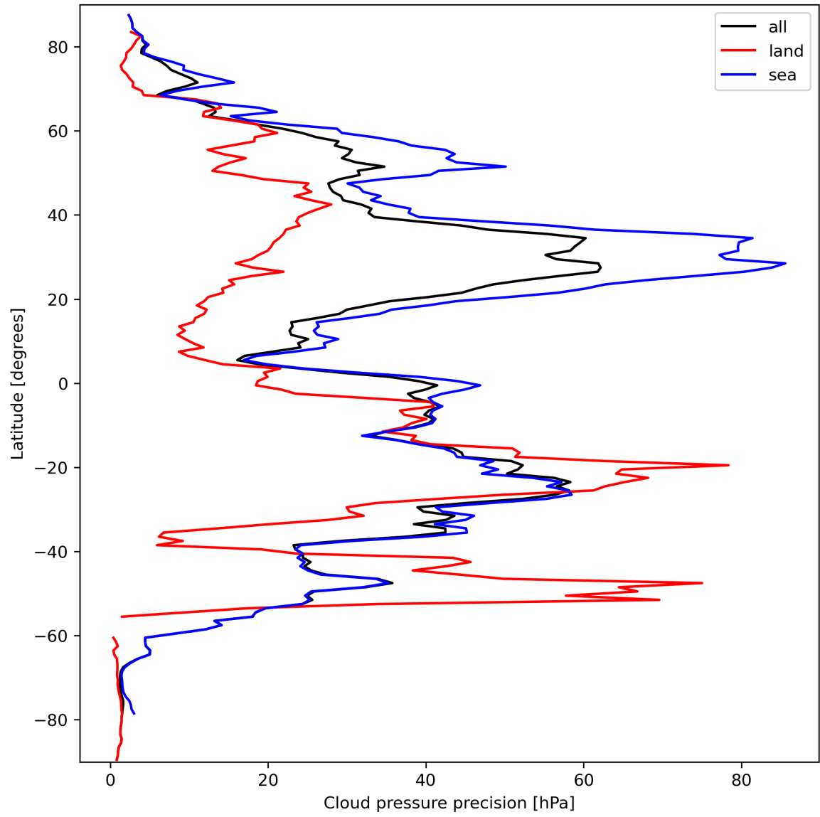
Figure 14: Zonal average of “Cloud pressure precision” for 2023-09-24 to 2023-09-26.
