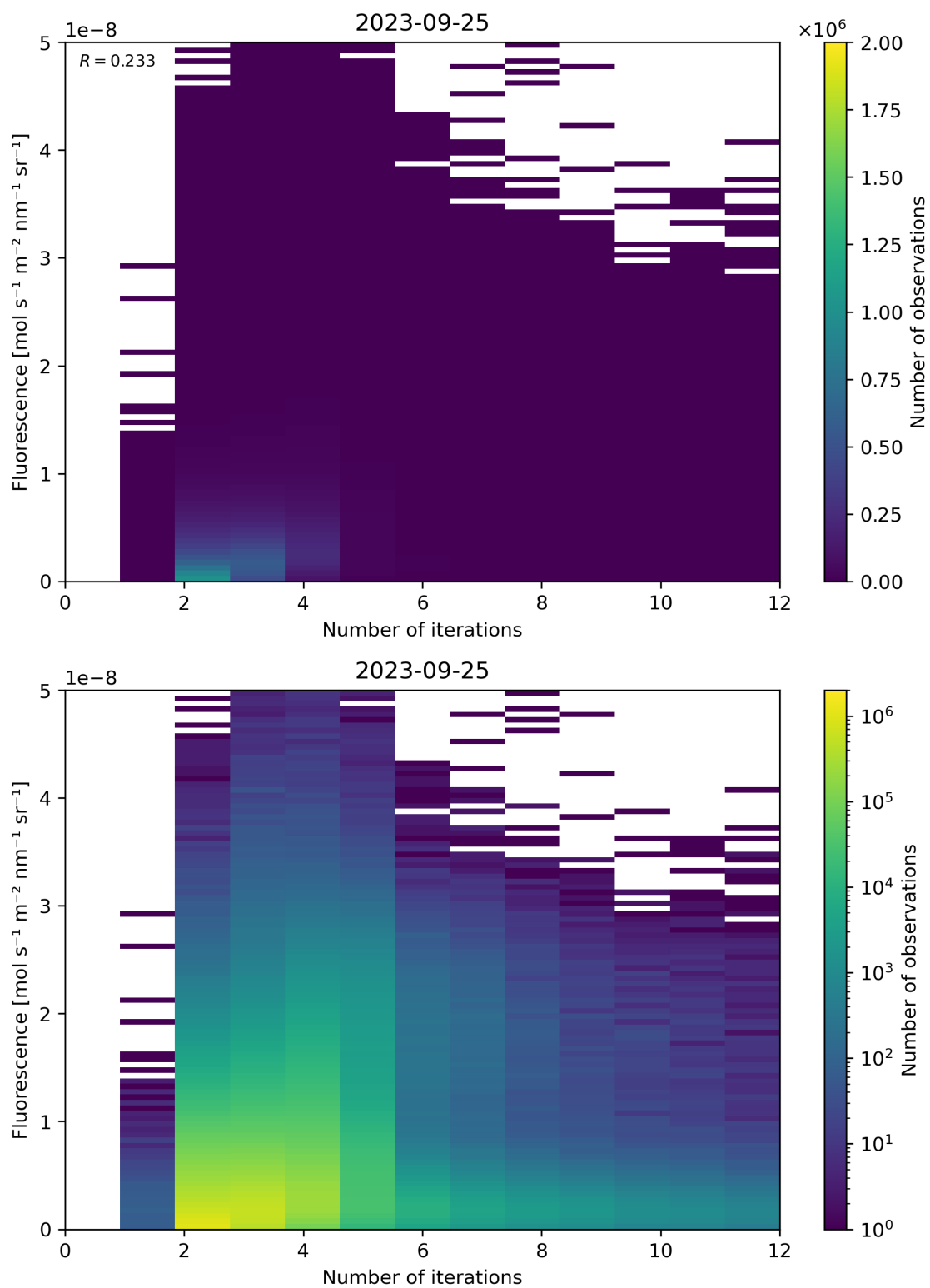
Figure 107: Scatter density plot of “Number of iterations” against “Fluorescence” for 2023-09-24 to 2023-09-26.
