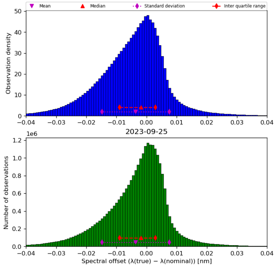
Figure 45: Histogram of “Spectral offset ( \lambda(\text{true}) - \lambda(\text{nominal}) )” for 2023-09-24 to 2023-09-26
