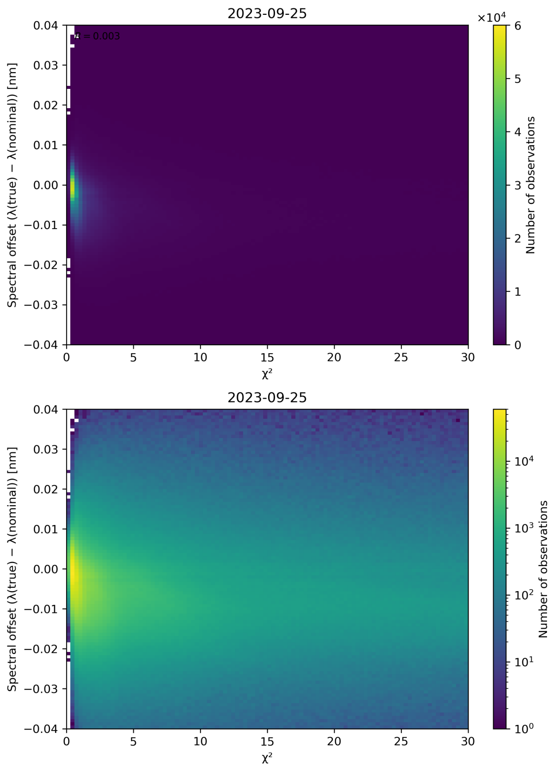
Figure 75: Scatter density plot of “ \chi^2 ” against “Spectral offset ( \lambda(\text{true}) - \lambda(\text{nominal}) )” for 2023-09-24 to 2023-09-26.
