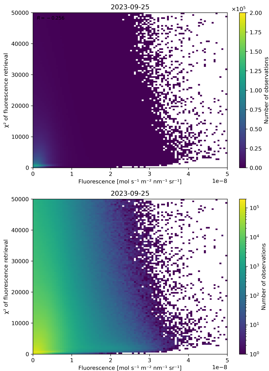
Figure 93: Scatter density plot of “Fluorescence” against “ \chi^2 of fluorescence retrieval” for 2023-09-24 to 2023-09-26.
