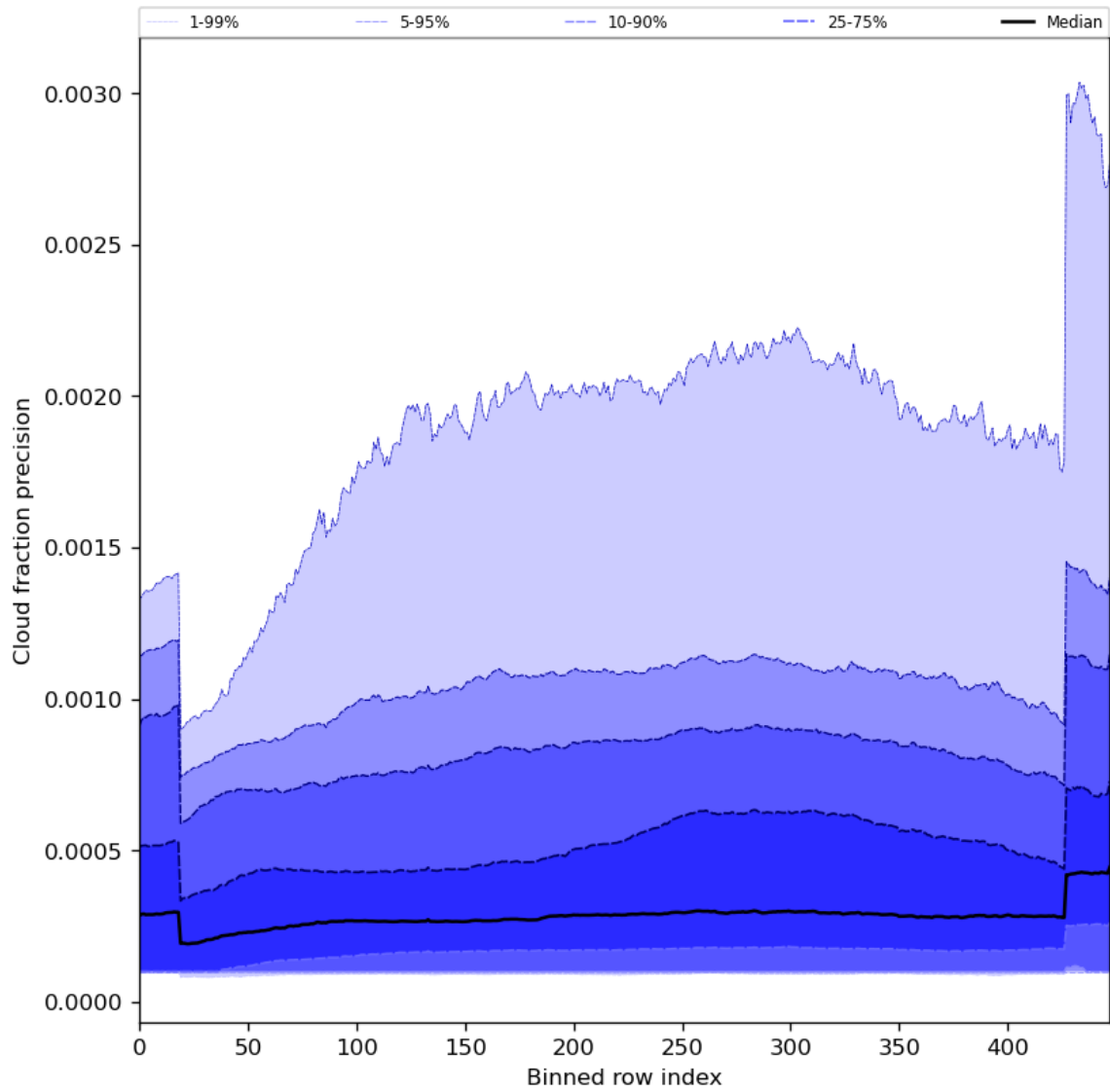
Figure 50: Along track statistics of “Cloud fraction precision” for 2023-09-24 to 2023-09-26
