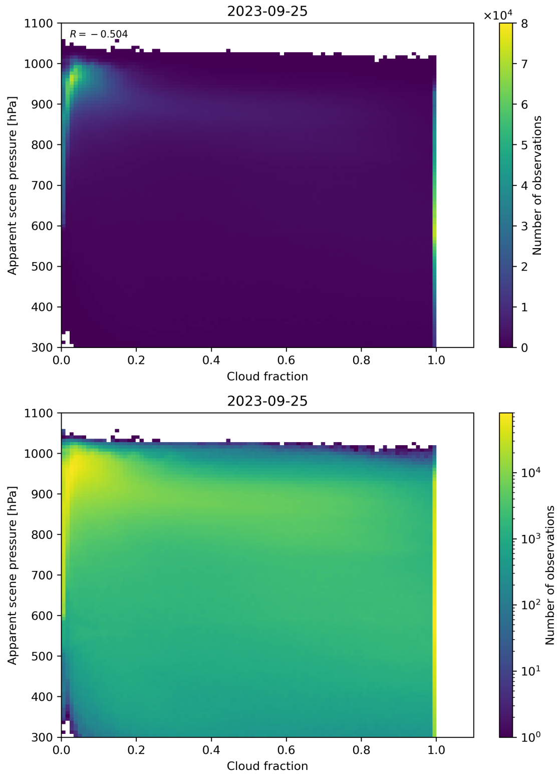
Figure 76: Scatter density plot of “Cloud fraction” against “Apparent scene pressure” for 2023-09-24 to 2023-09-26.
