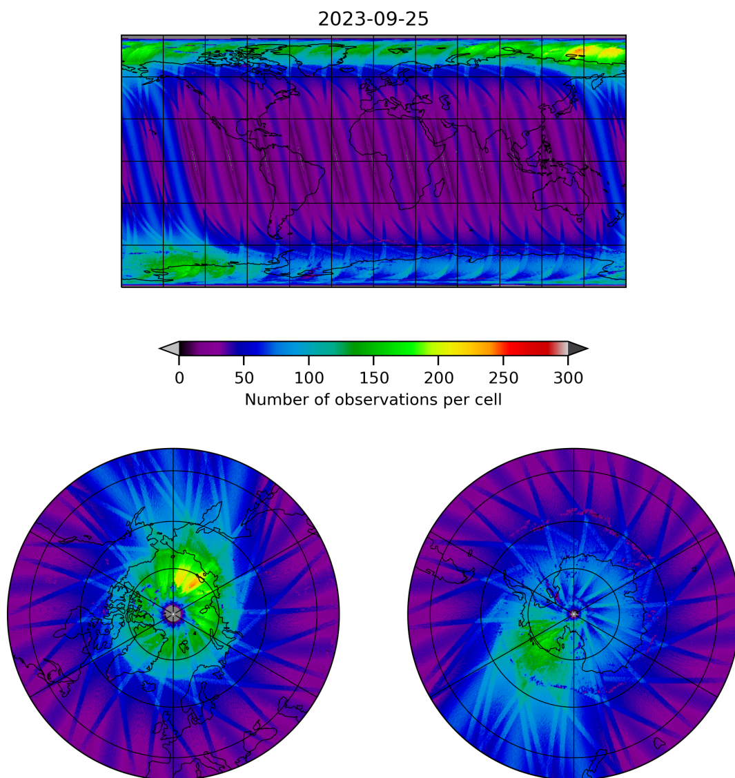
Figure 11: Map of the number of observations for 2023-09-24 to 2023-09-26
