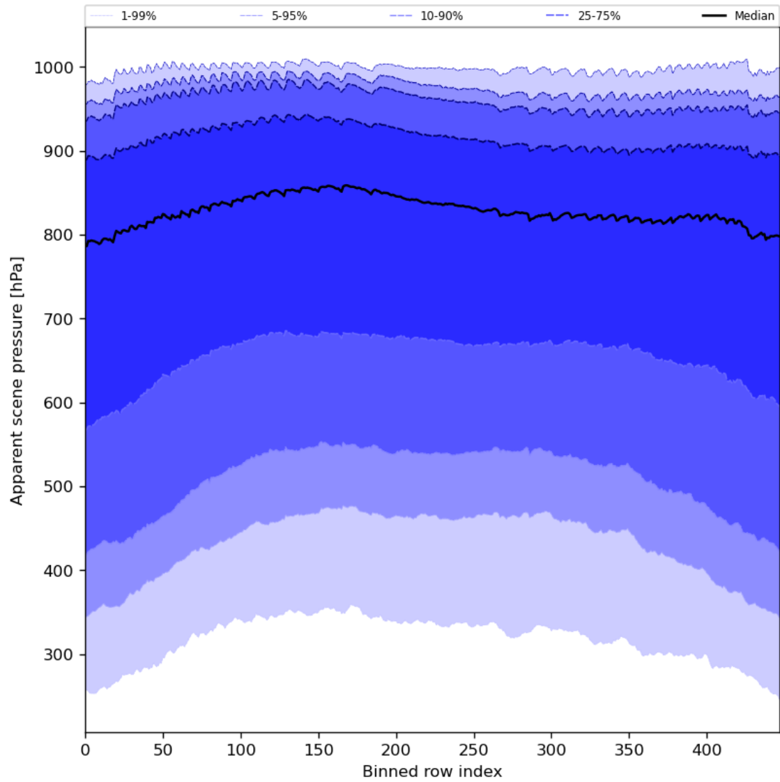
Figure 53: Along track statistics of “Apparent scene pressure” for 2023-09-24 to 2023-09-26
