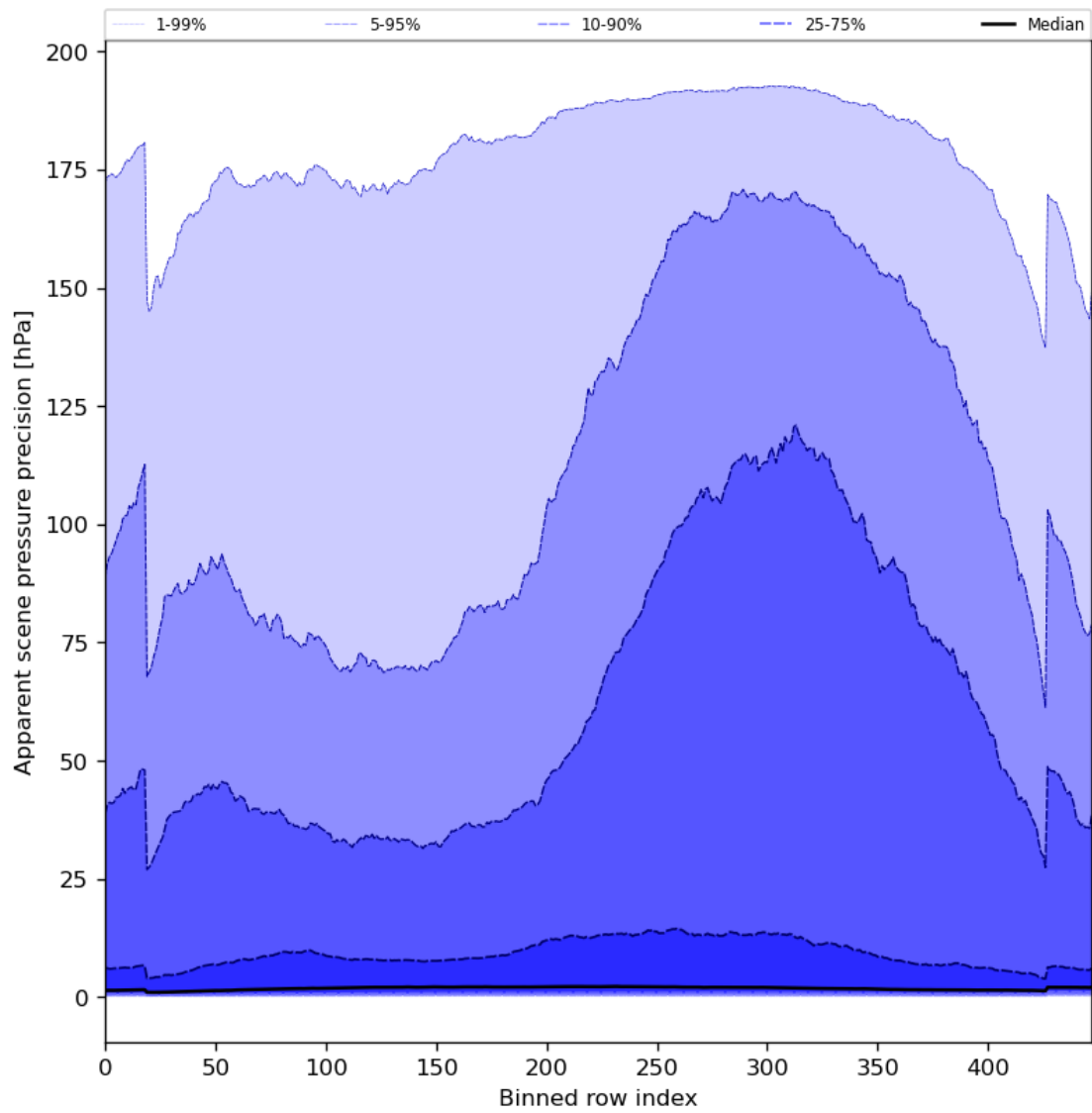
Figure 54: Along track statistics of “Apparent scene pressure precision” for 2023-09-24 to 2023-09-26
