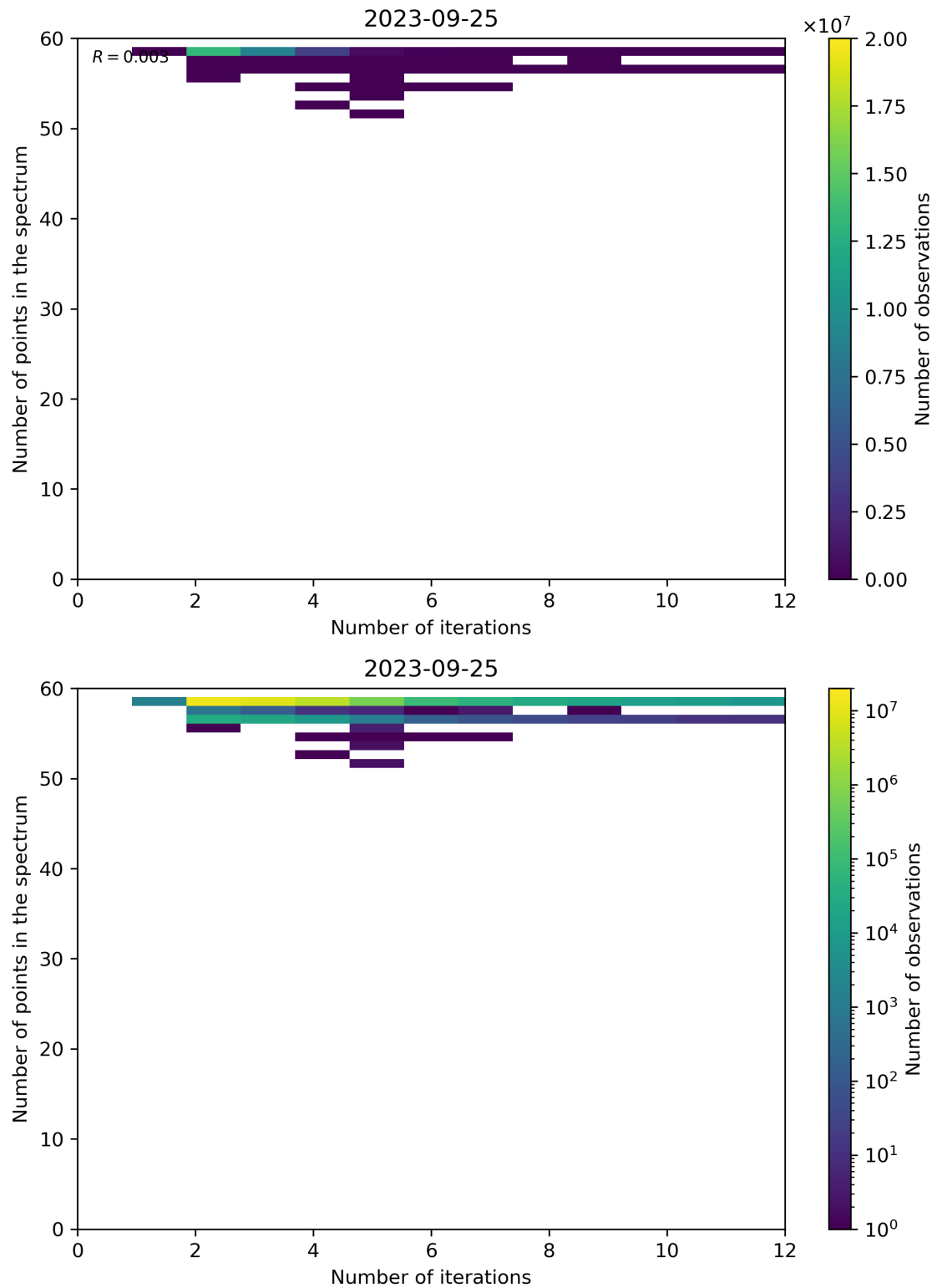
Figure 108: Scatter density plot of “Number of iterations” against “Number of points in the spectrum” for 2023-09-24 to 2023-09-26.
