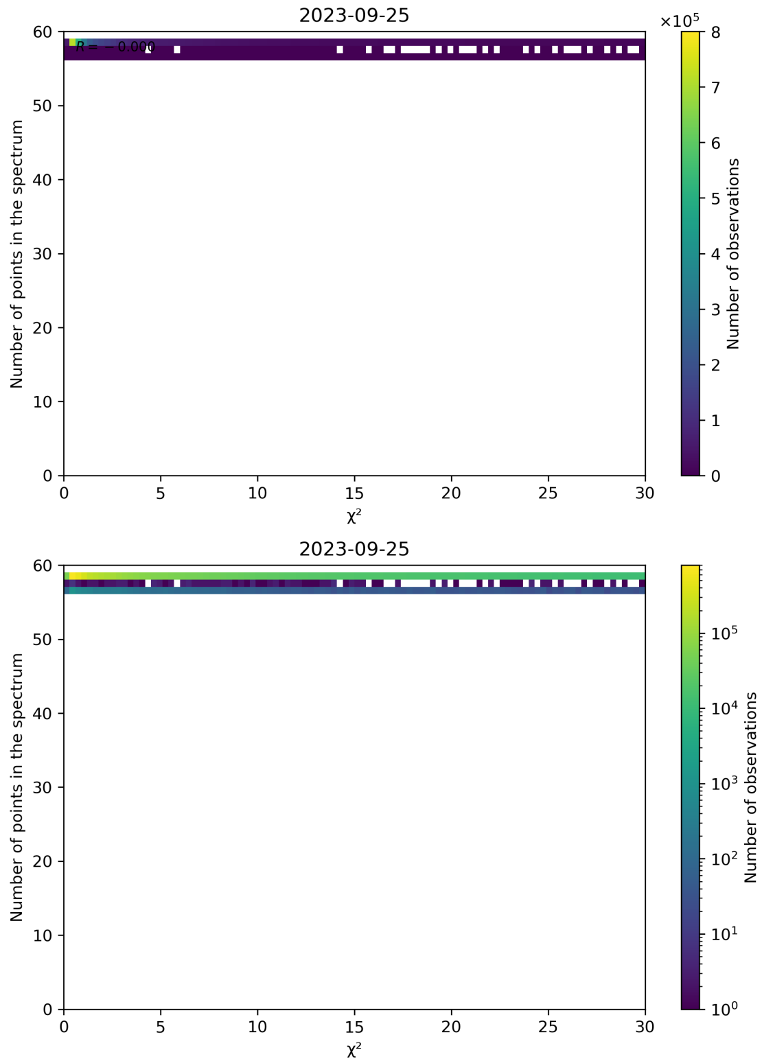
Figure 74: Scatter density plot of " \chi^2 " against "Number of points in the spectrum" for 2023-09-24 to 2023-09-26.
