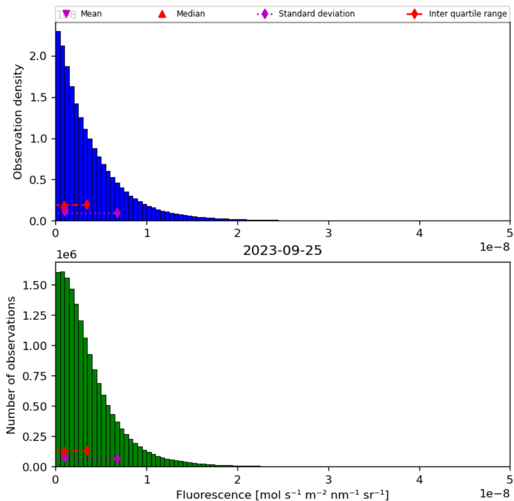
Figure 40: Histogram of “Fluorescence” for 2023-09-24 to 2023-09-26
