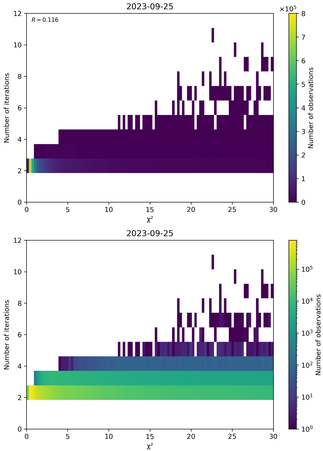
Figure 73: Scatter density plot of “ \chi^2 ” against “Number of iterations” for 2023-09-24 to 2023-09-26.
