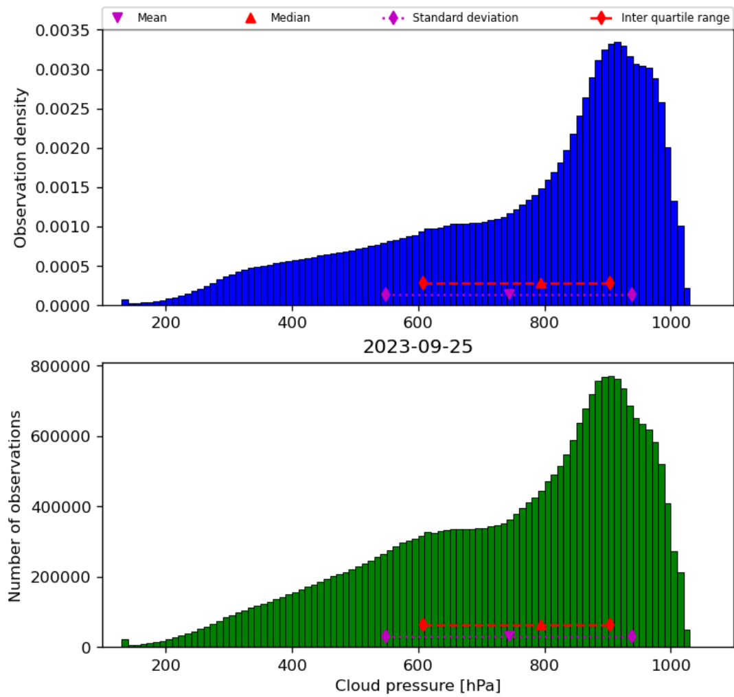
Figure 30: Histogram of “Cloud pressure” for 2023-09-24 to 2023-09-26
