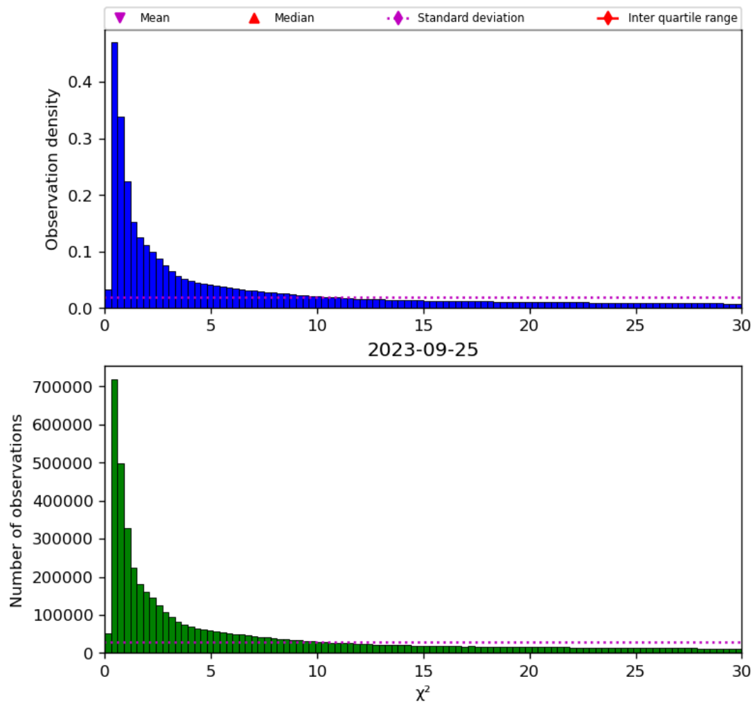
Figure 38: Histogram of “ \chi^2 ” for 2023-09-24 to 2023-09-26
