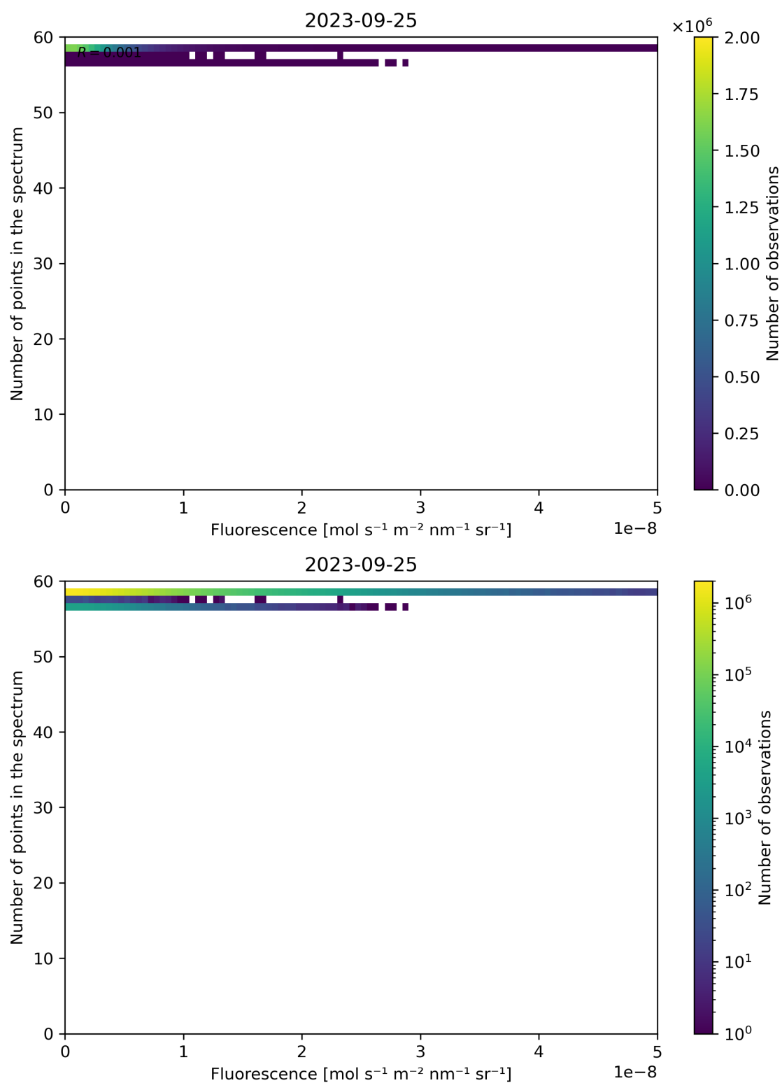
Figure 94: Scatter density plot of “Fluorescence” against “Number of points in the spectrum” for 2023-09-24 to 2023-09-26.
