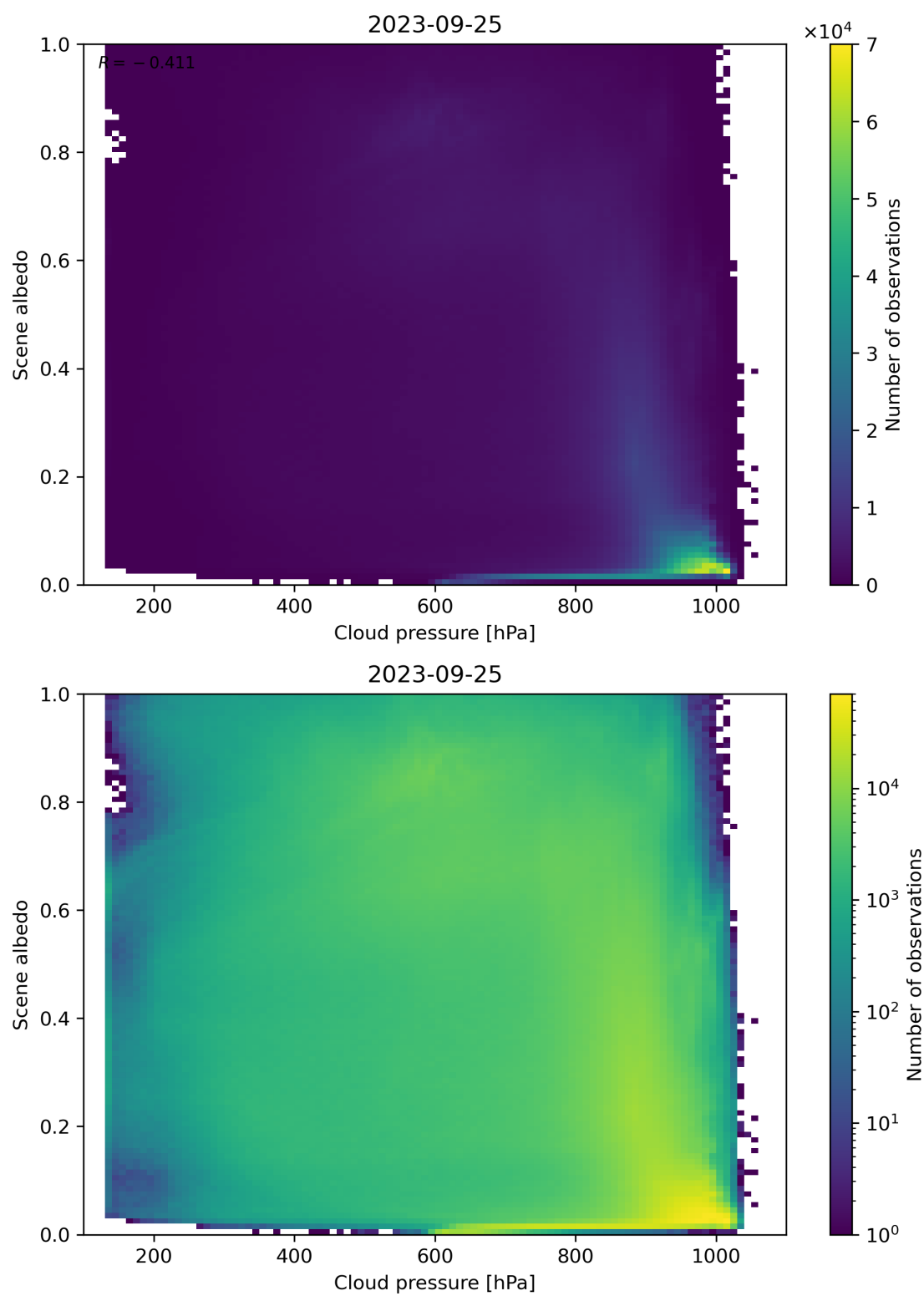
Figure 91: Scatter density plot of “Cloud pressure” against “Scene albedo” for 2023-09-24 to 2023-09-26.
