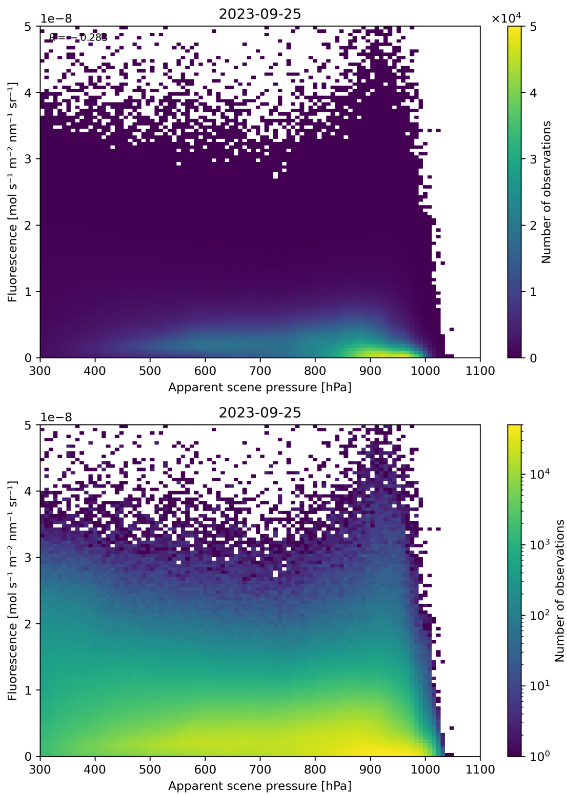
Figure 65: Scatter density plot of “Apparent scene pressure” against “Fluorescence” for 2023-09-24 to 2023-09-26.
