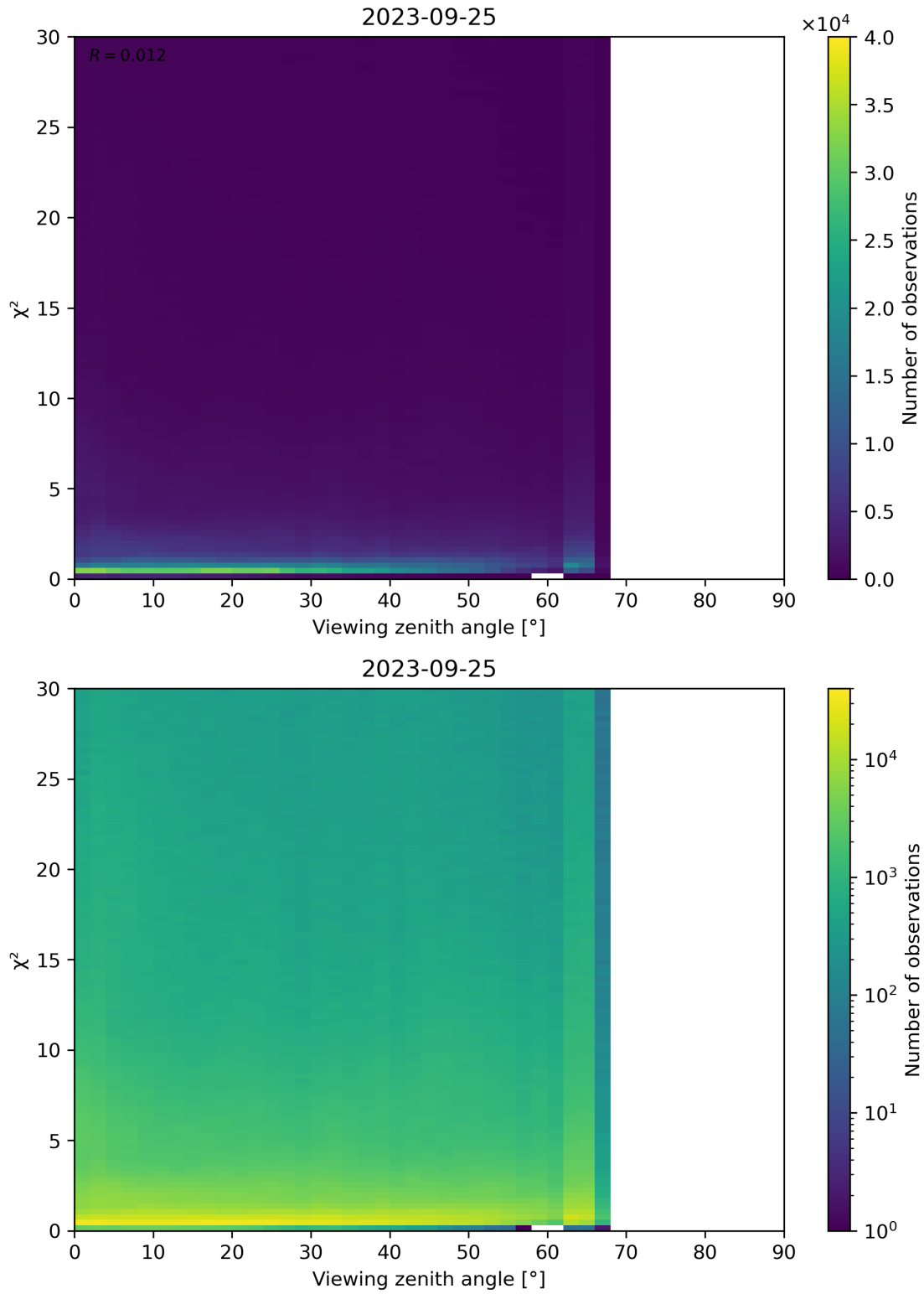
Figure 130: Scatter density plot of “Viewing zenith angle” against “ \chi^2 ” for 2023-09-24 to 2023-09-26.
