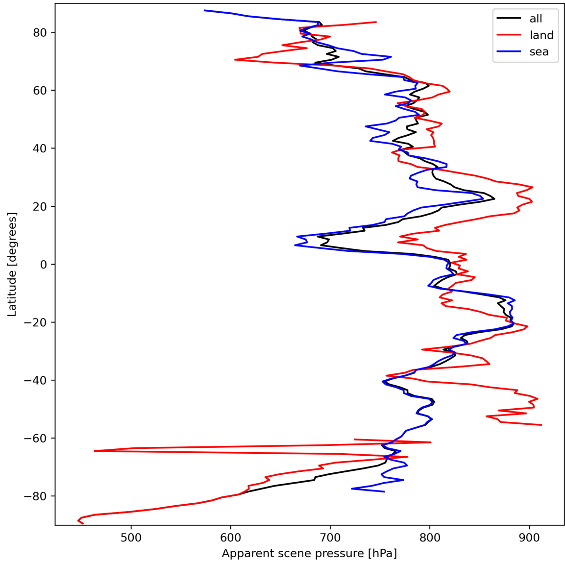
Figure 19: Zonal average of “Apparent scene pressure” for 2023-09-24 to 2023-09-26.
