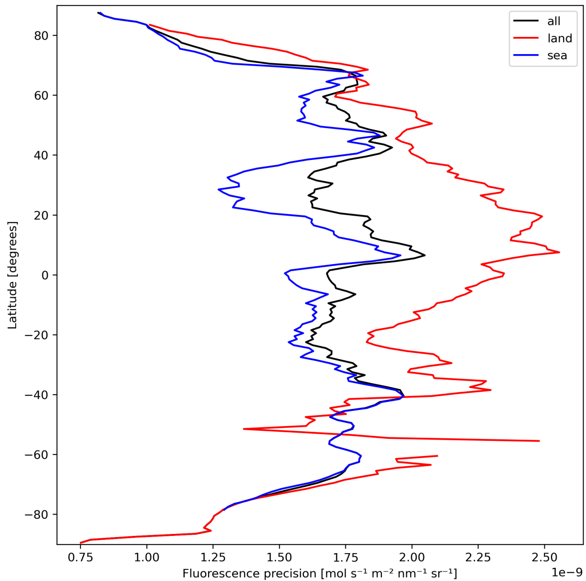
Figure 24: Zonal average of “Fluorescence precision” for 2023-09-24 to 2023-09-26.
