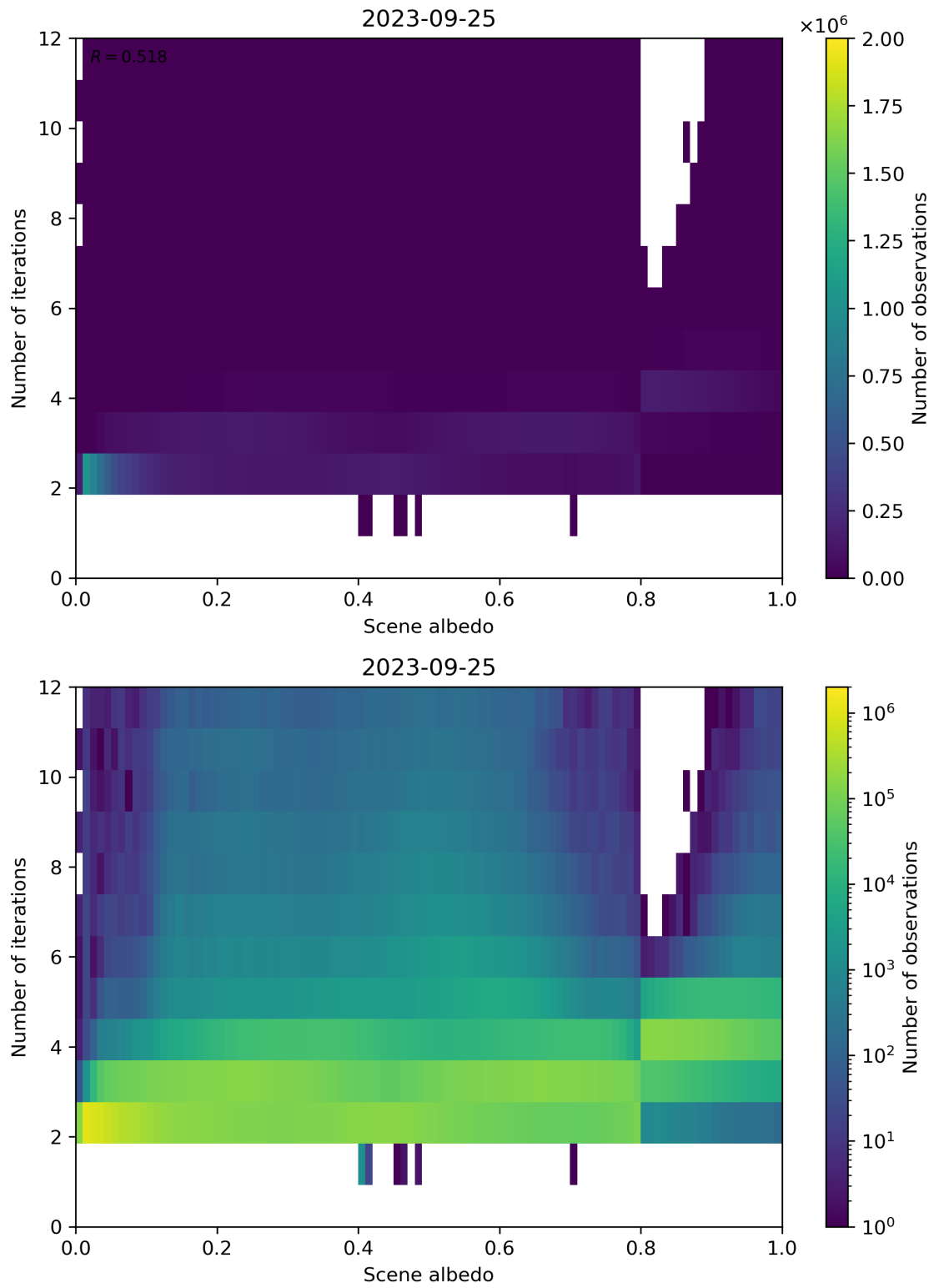
Figure 115: Scatter density plot of “Scene albedo” against “Number of iterations” for 2023-09-24 to 2023-09-26.
