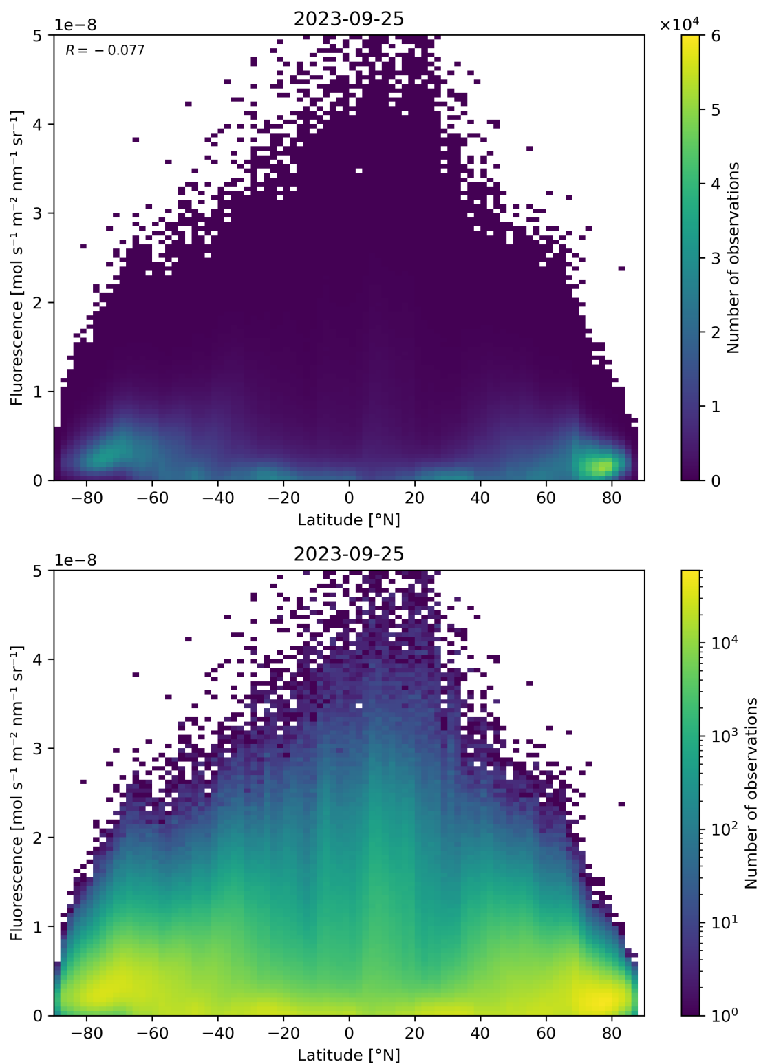
Figure 101: Scatter density plot of “Latitude” against “Fluorescence” for 2023-09-24 to 2023-09-26.
