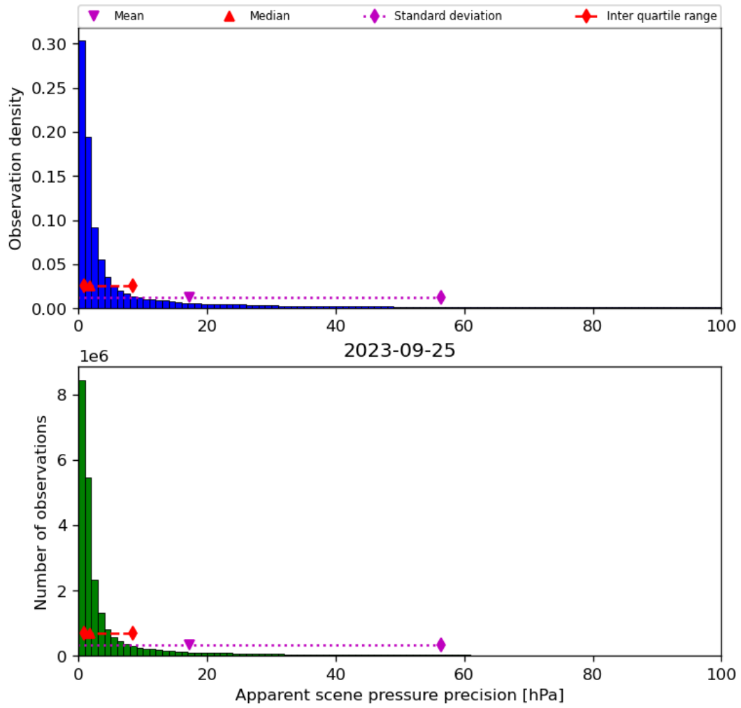
Figure 37: Histogram of “Apparent scene pressure precision” for 2023-09-24 to 2023-09-26
