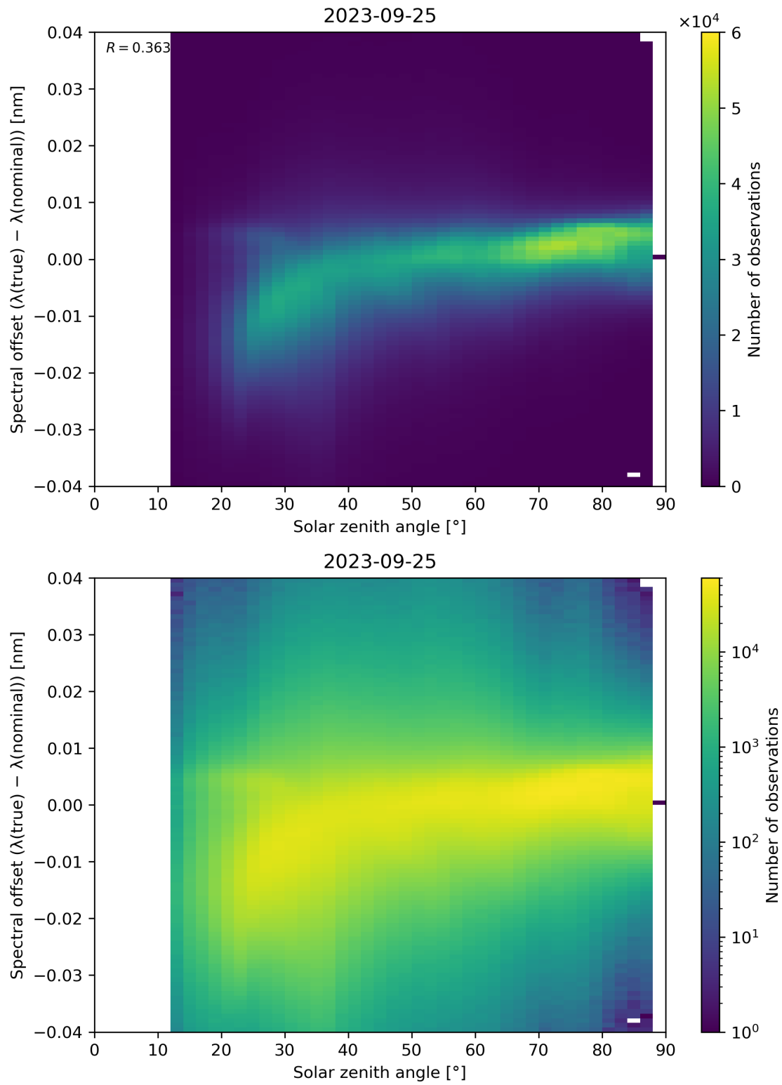
Figure 128: Scatter density plot of “Solar zenith angle” against “Spectral offset ( \lambda(\text{true}) - \lambda(\text{nominal}) )” for 2023-09-24 to 2023-09-26.
