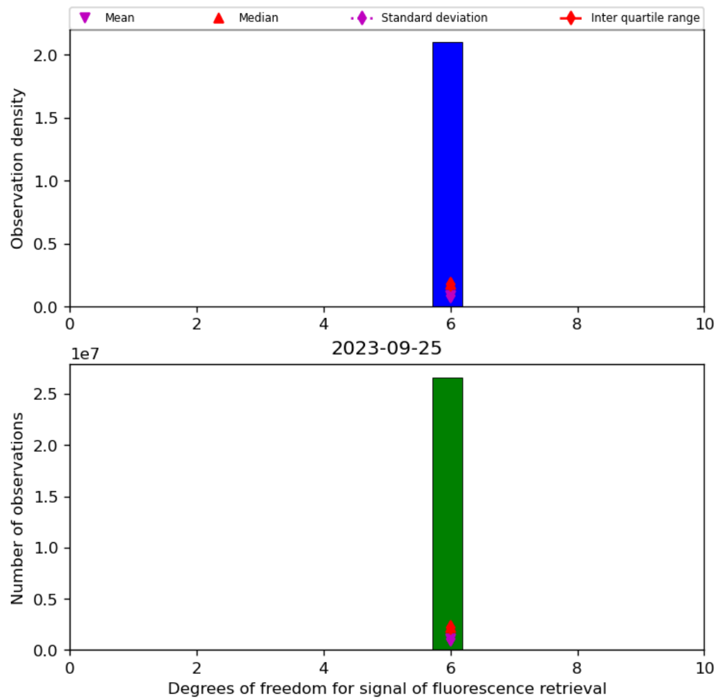
Figure 43: Histogram of “Degrees of freedom for signal of fluorescence retrieval” for 2023-09-24 to 2023-09-26
