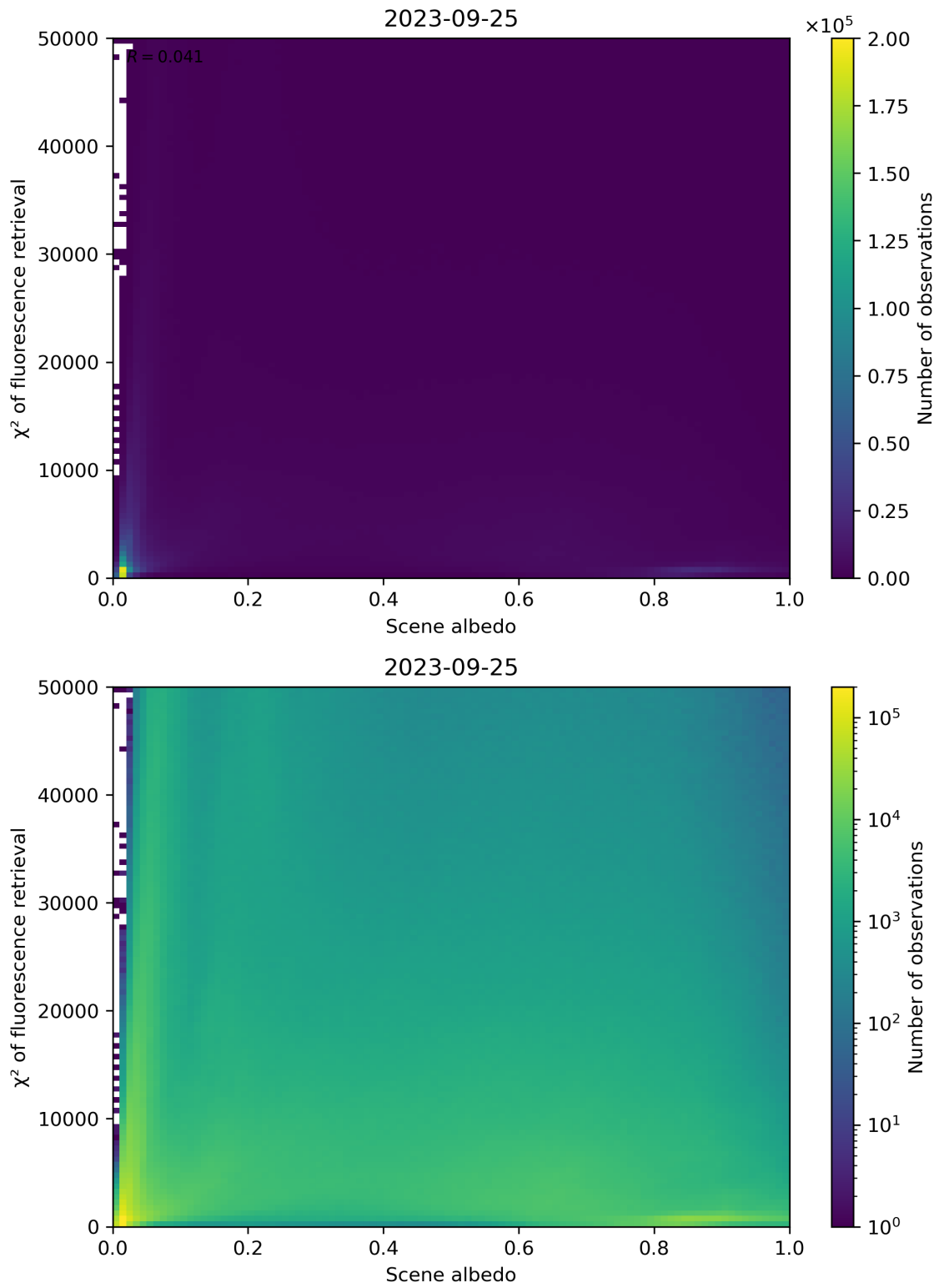
Figure 113: Scatter density plot of “Scene albedo” against “ \chi^2 of fluorescence retrieval” for 2023-09-24 to 2023-09-26.
