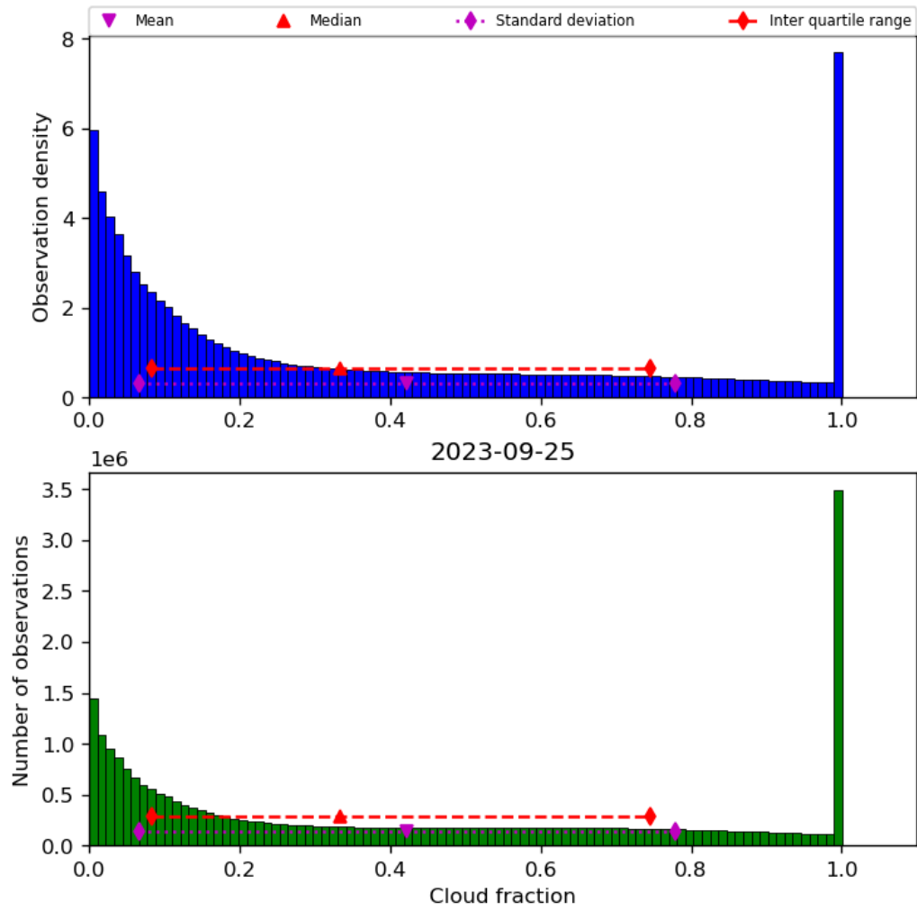
Figure 32: Histogram of “Cloud fraction” for 2023-09-24 to 2023-09-26
