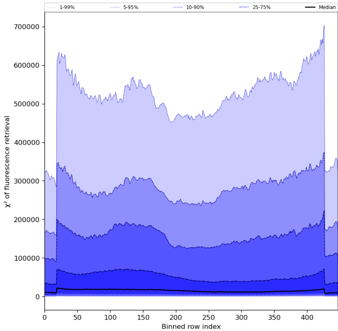
Figure 59: Along track statistics of “ \chi^2 of fluorescence retrieval” for 2023-09-24 to 2023-09-26
