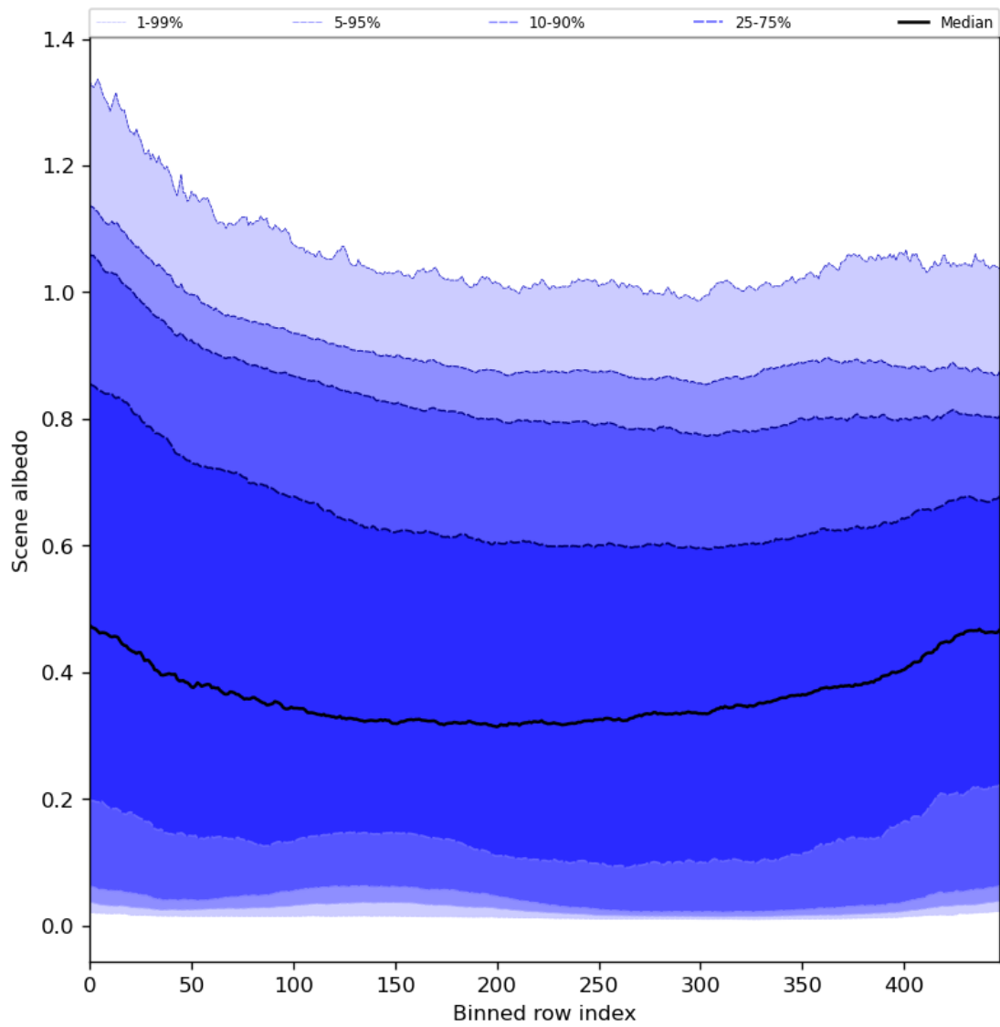
Figure 51: Along track statistics of “Scene albedo” for 2023-09-26 to 2023-09-27
