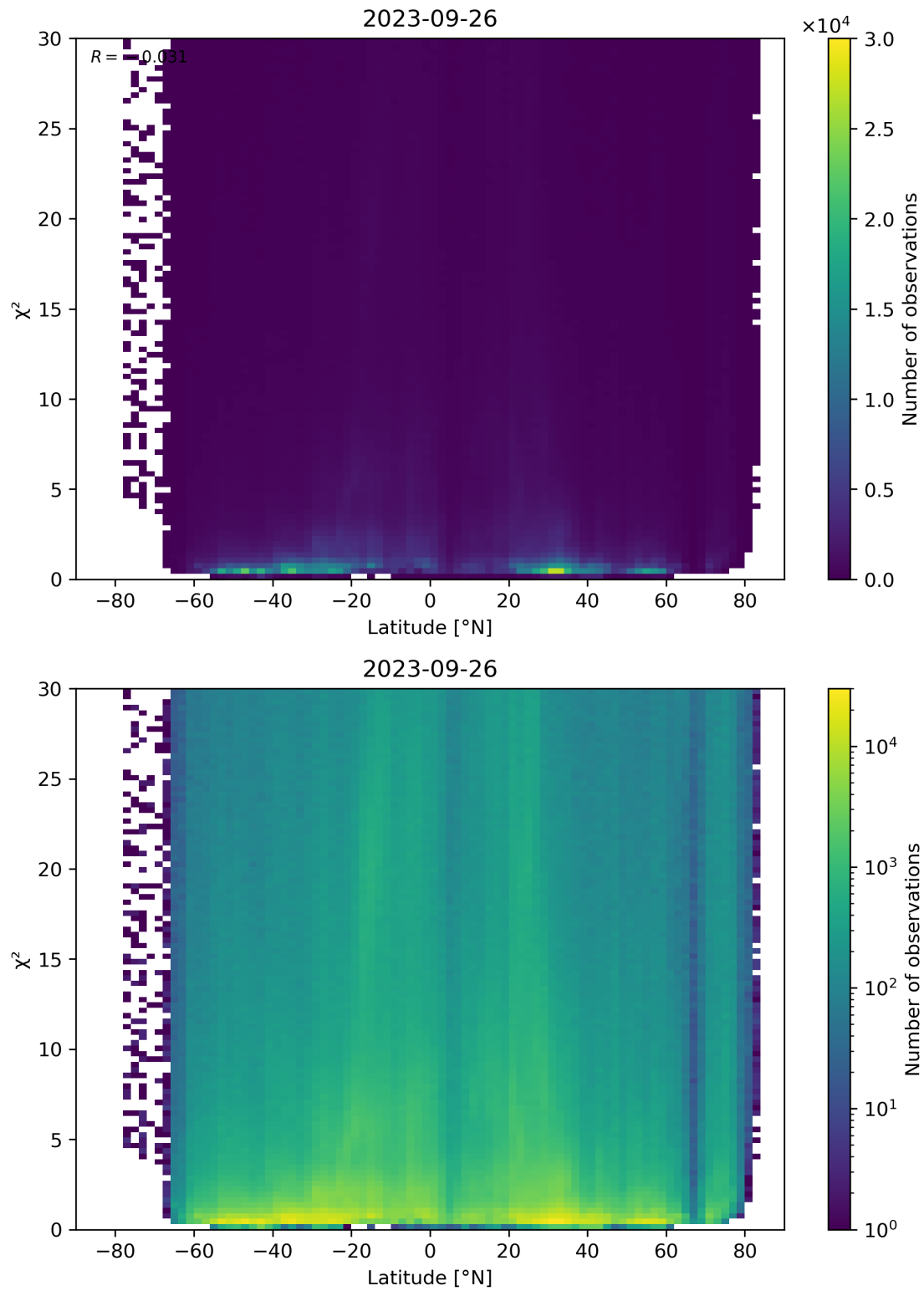
Figure 97: Scatter density plot of “Latitude” against “ \chi^2 ” for 2023-09-26 to 2023-09-27.
