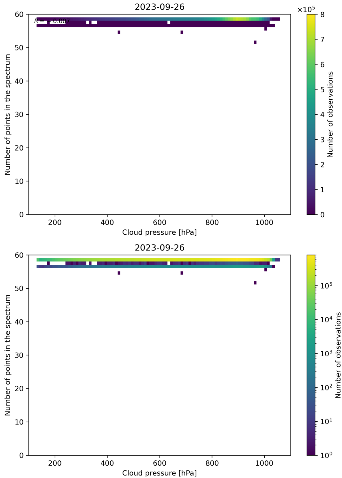
Figure 90: Scatter density plot of “Cloud pressure” against “Number of points in the spectrum” for 2023-09-26 to 2023-09-27.
