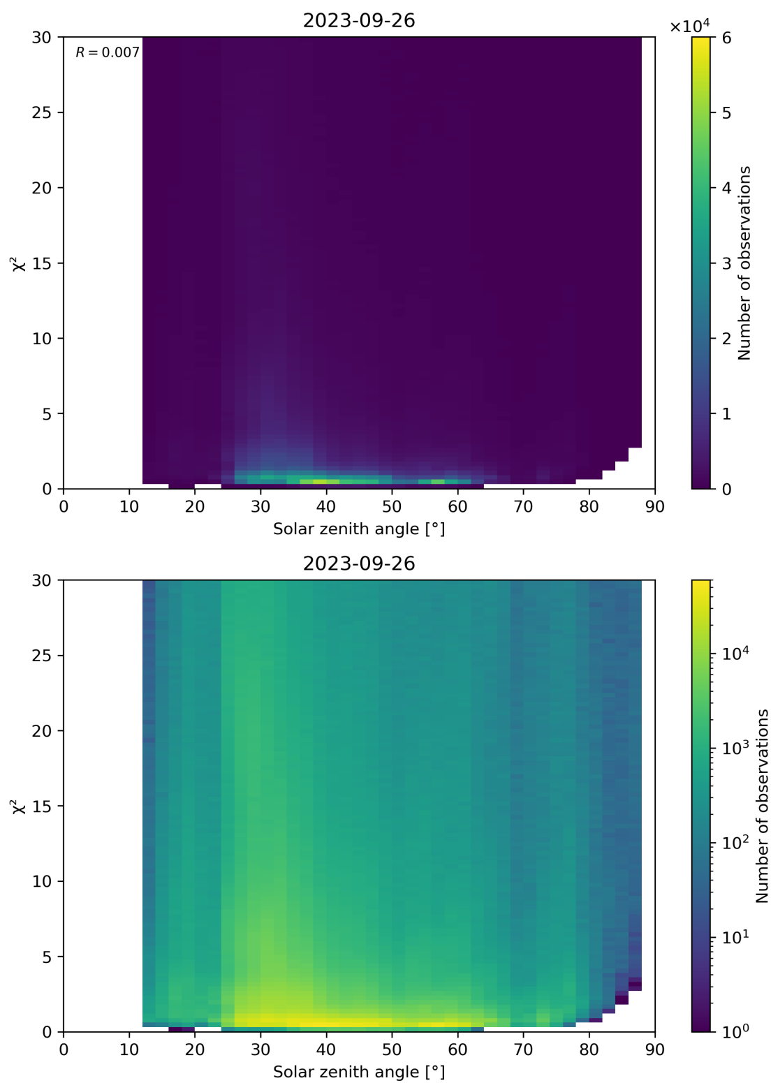
Figure 119: Scatter density plot of “Solar zenith angle” against “ \chi^2 ” for 2023-09-26 to 2023-09-27.
