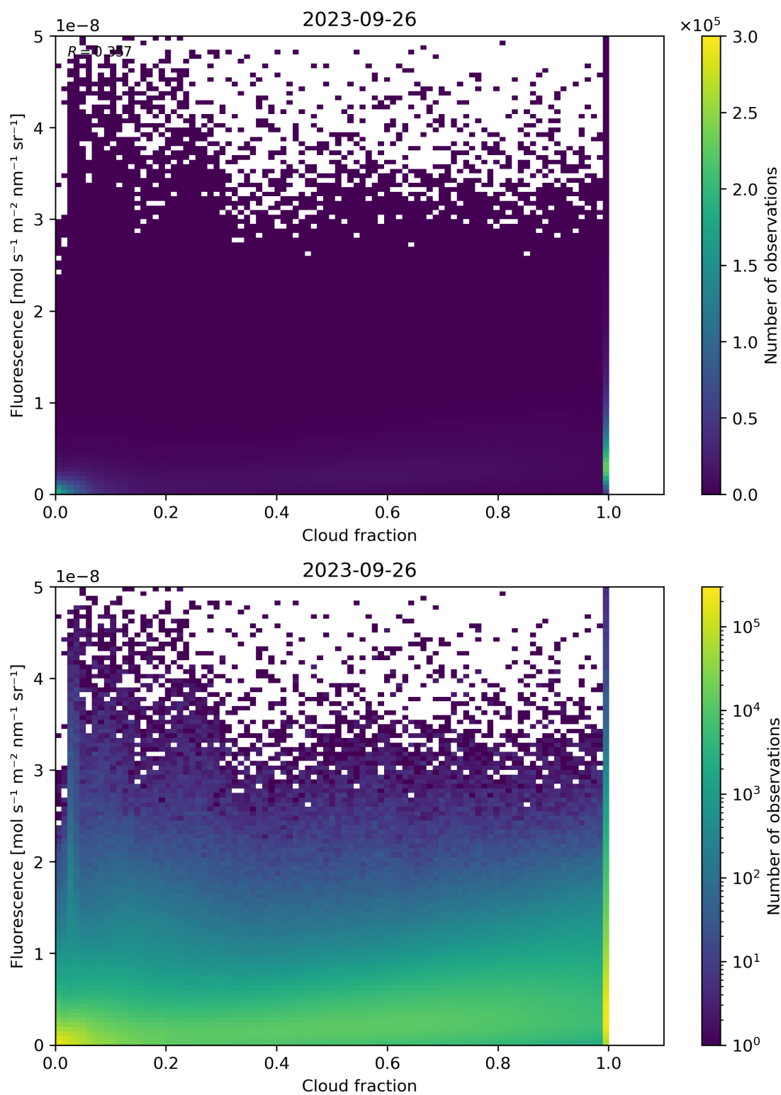
Figure 79: Scatter density plot of “Cloud fraction” against “Fluorescence” for 2023-09-26 to 2023-09-27.
