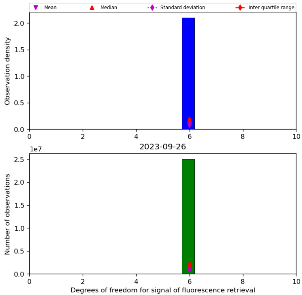
Figure 43: Histogram of “Degrees of freedom for signal of fluorescence retrieval” for 2023-09-26 to 2023-09-27
