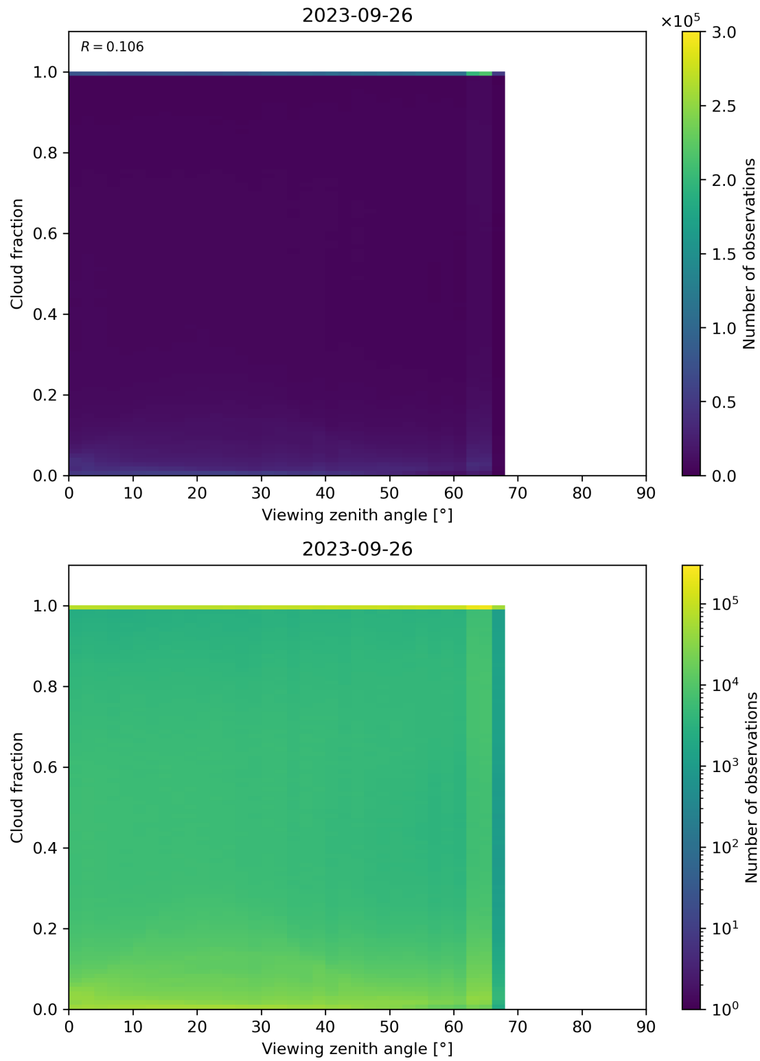
Figure 132: Scatter density plot of “Viewing zenith angle” against “Cloud fraction” for 2023-09-26 to 2023-09-27.
