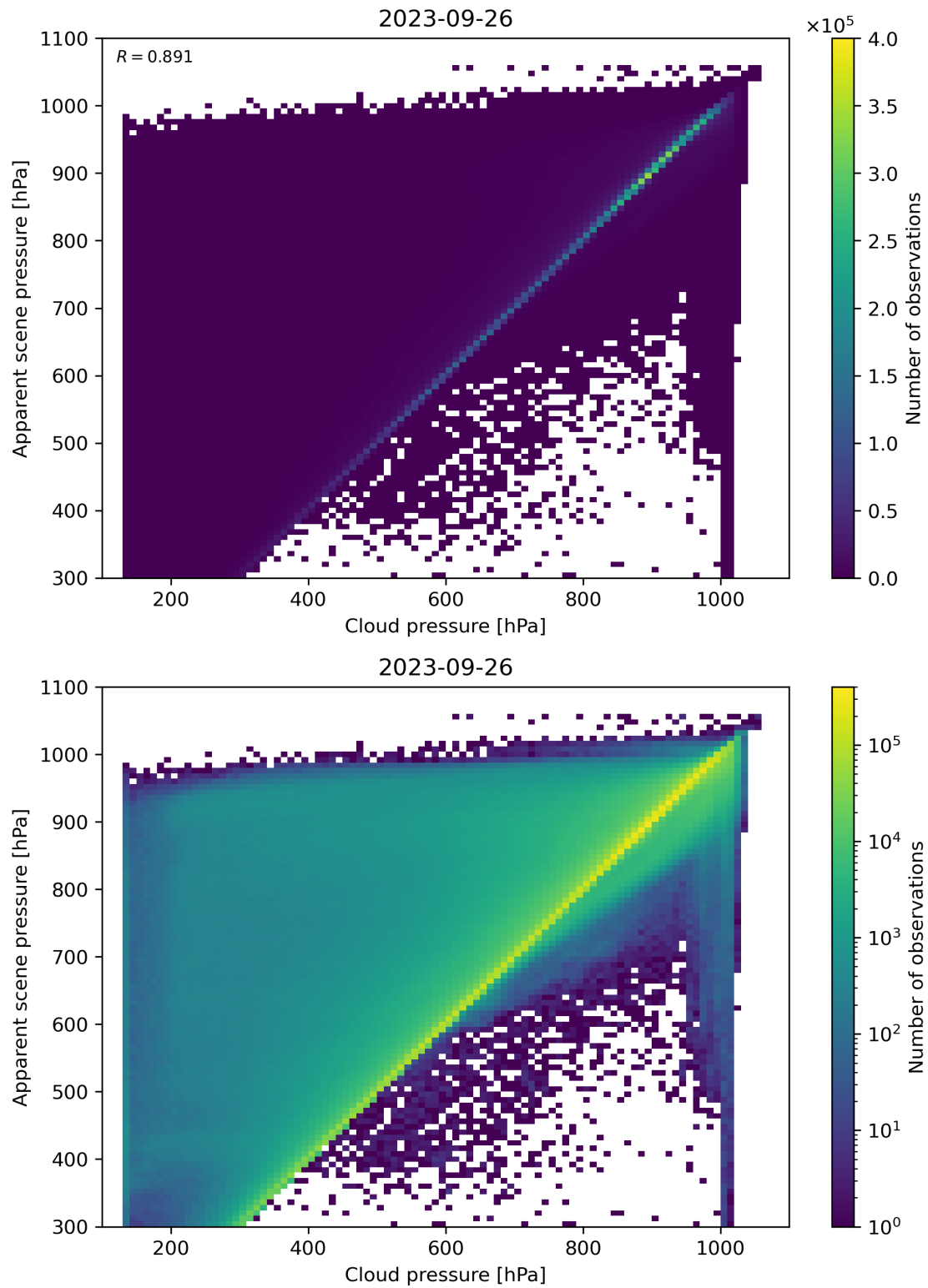
Figure 84: Scatter density plot of “Cloud pressure” against “Apparent scene pressure” for 2023-09-26 to 2023-09-27.
