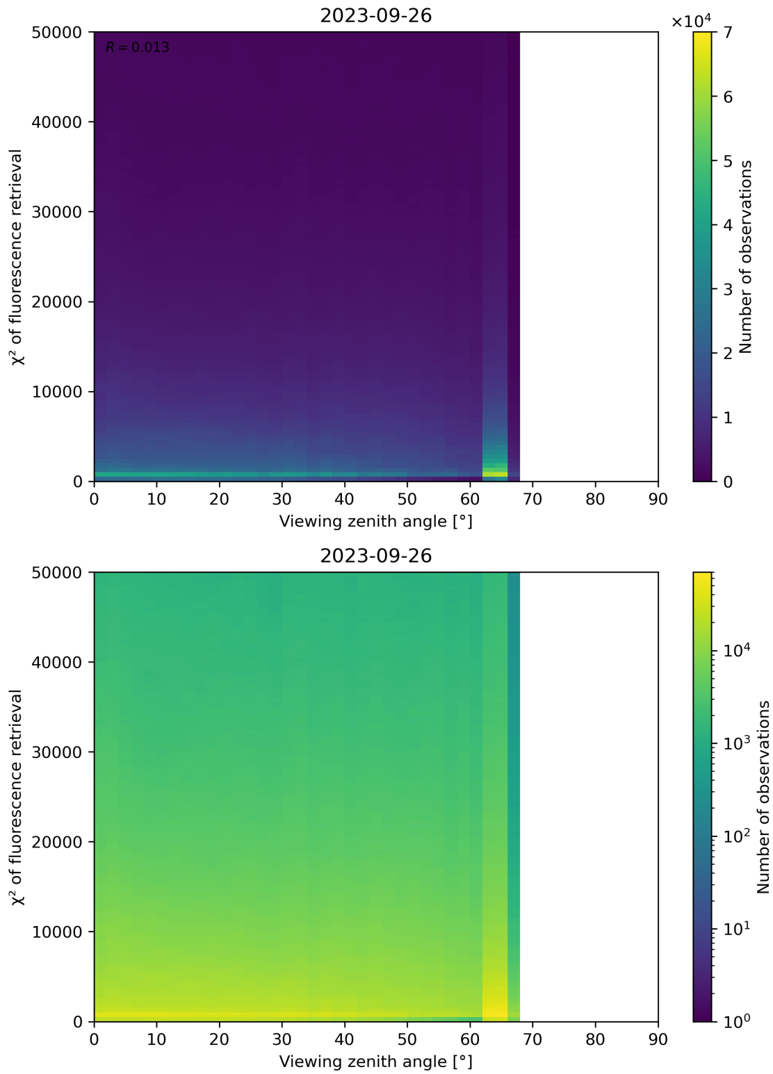
Figure 131: Scatter density plot of “Viewing zenith angle” against “ \chi^2 of fluorescence retrieval” for 2023-09-26 to 2023-09-27.
