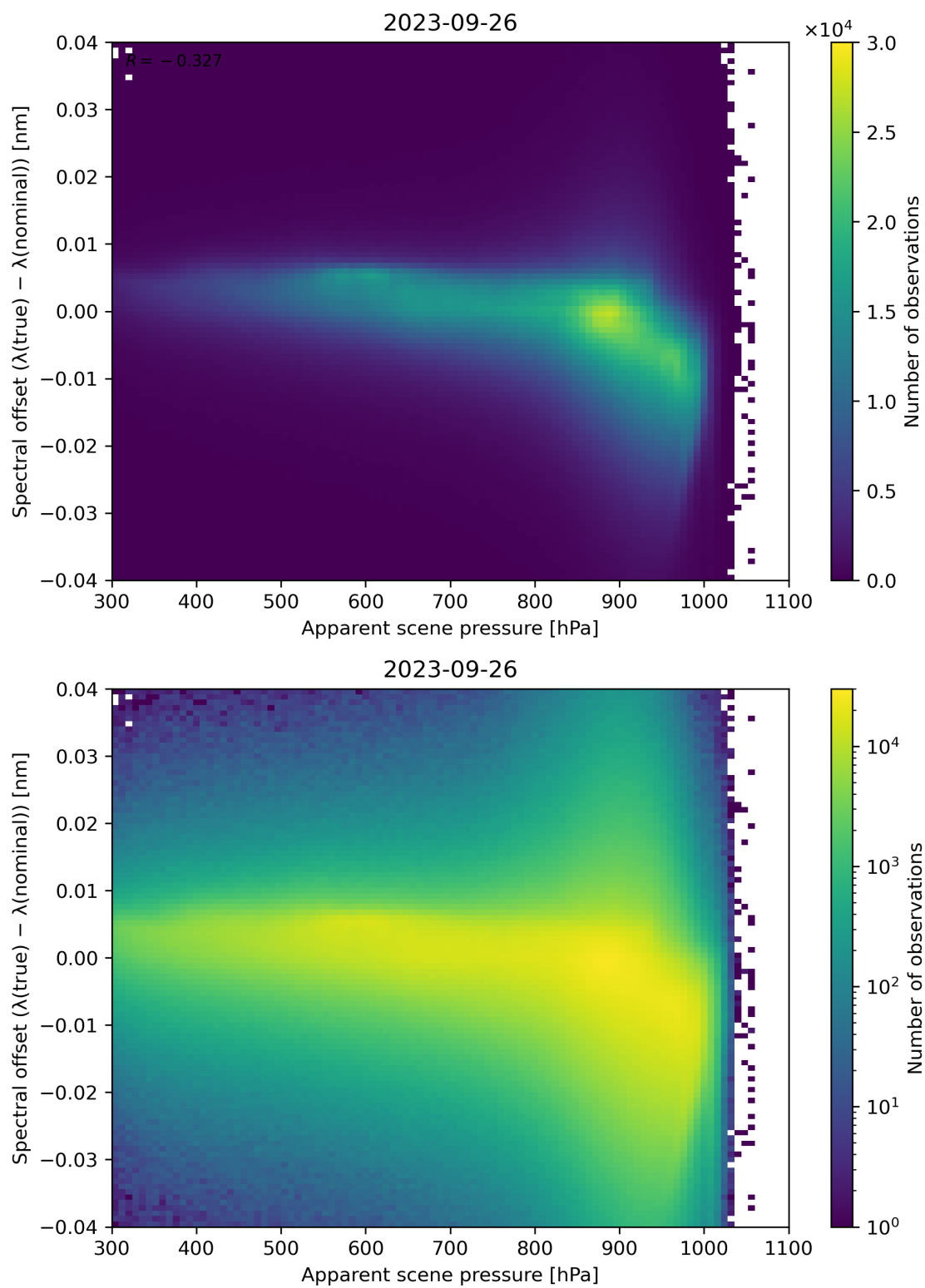
Figure 68: Scatter density plot of “Apparent scene pressure” against “Spectral offset ( \lambda(\text{true}) - \lambda(\text{nominal}) )” for 2023-09-26 to 2023-09-27.
