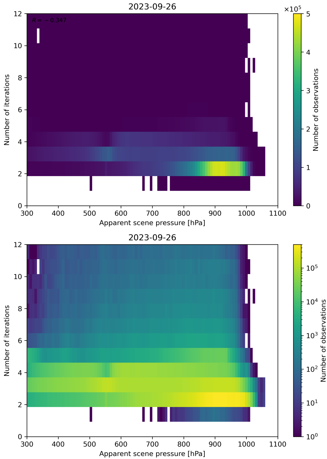
Figure 66: Scatter density plot of “Apparent scene pressure” against “Number of iterations” for 2023-09-26 to 2023-09-27.
