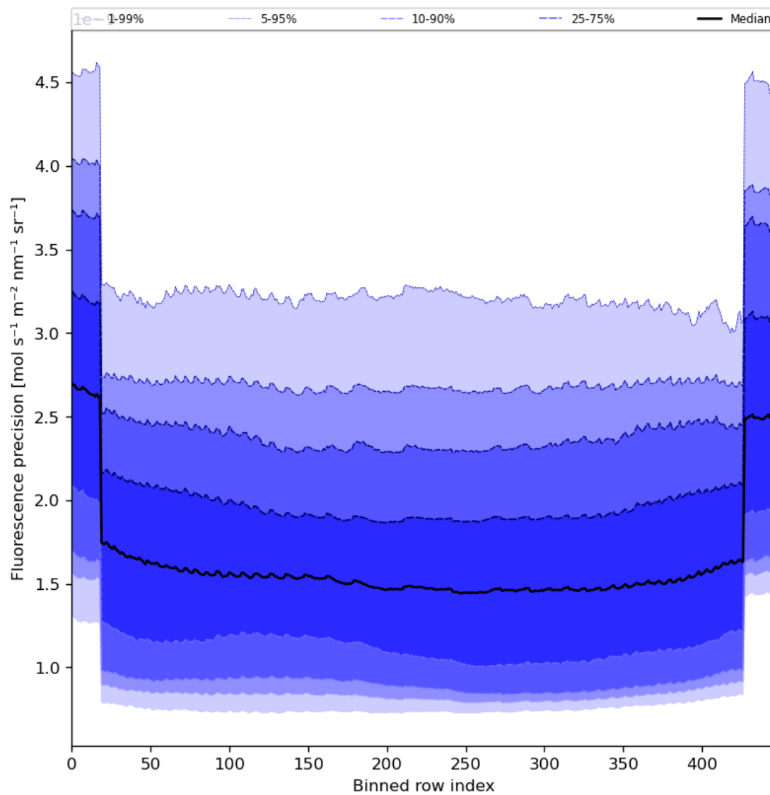
Figure 58: Along track statistics of “Fluorescence precision” for 2023-09-26 to 2023-09-27
