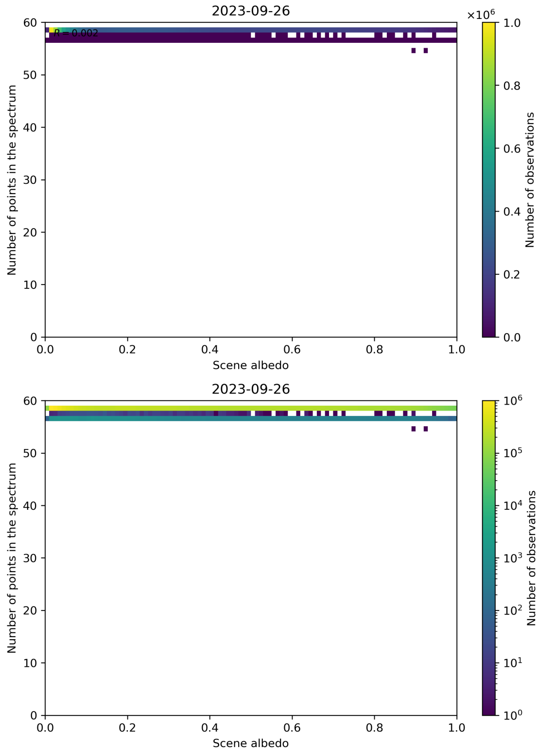
Figure 116: Scatter density plot of “Scene albedo” against “Number of points in the spectrum” for 2023-09-26 to 2023-09-27.
