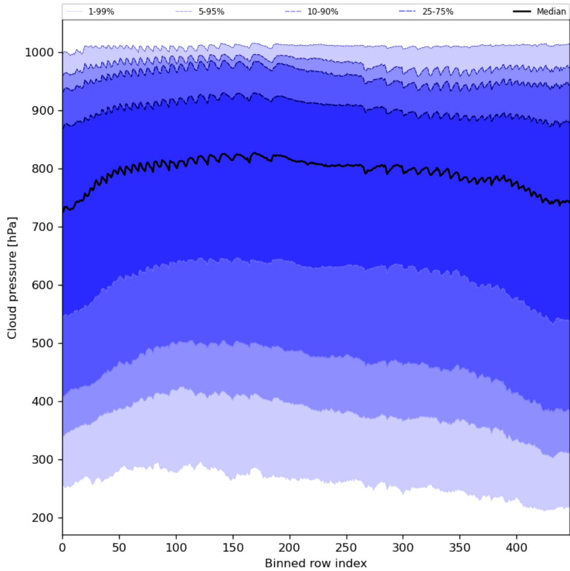
Figure 47: Along track statistics of “Cloud pressure” for 2023-09-26 to 2023-09-27
