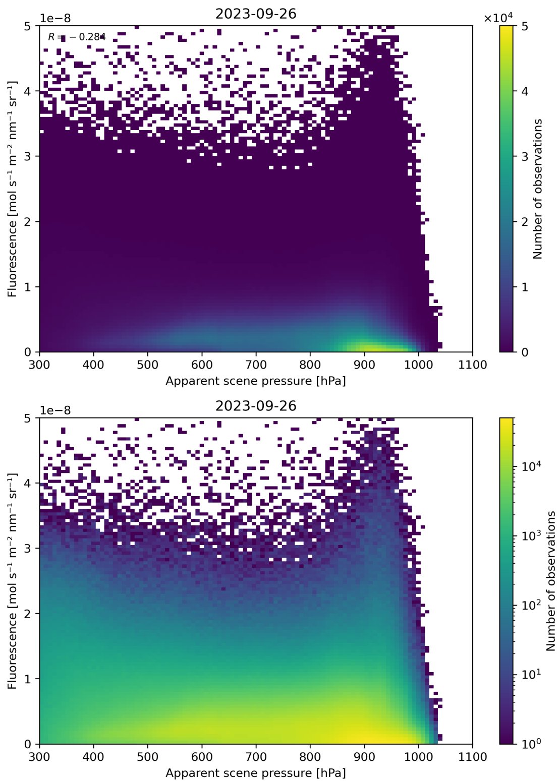
Figure 65: Scatter density plot of “Apparent scene pressure” against “Fluorescence” for 2023-09-26 to 2023-09-27.
