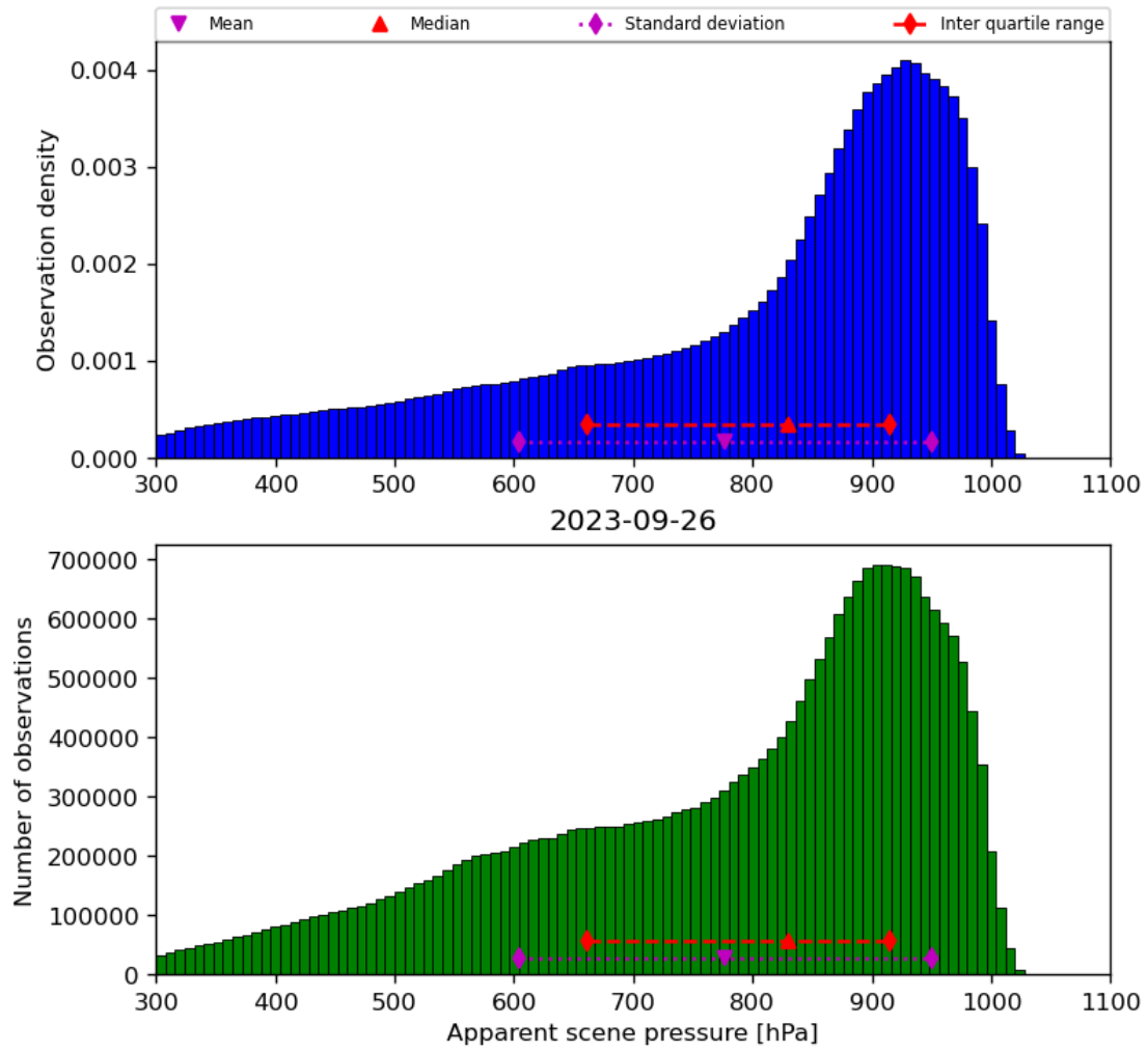
Figure 36: Histogram of “Apparent scene pressure” for 2023-09-26 to 2023-09-27
