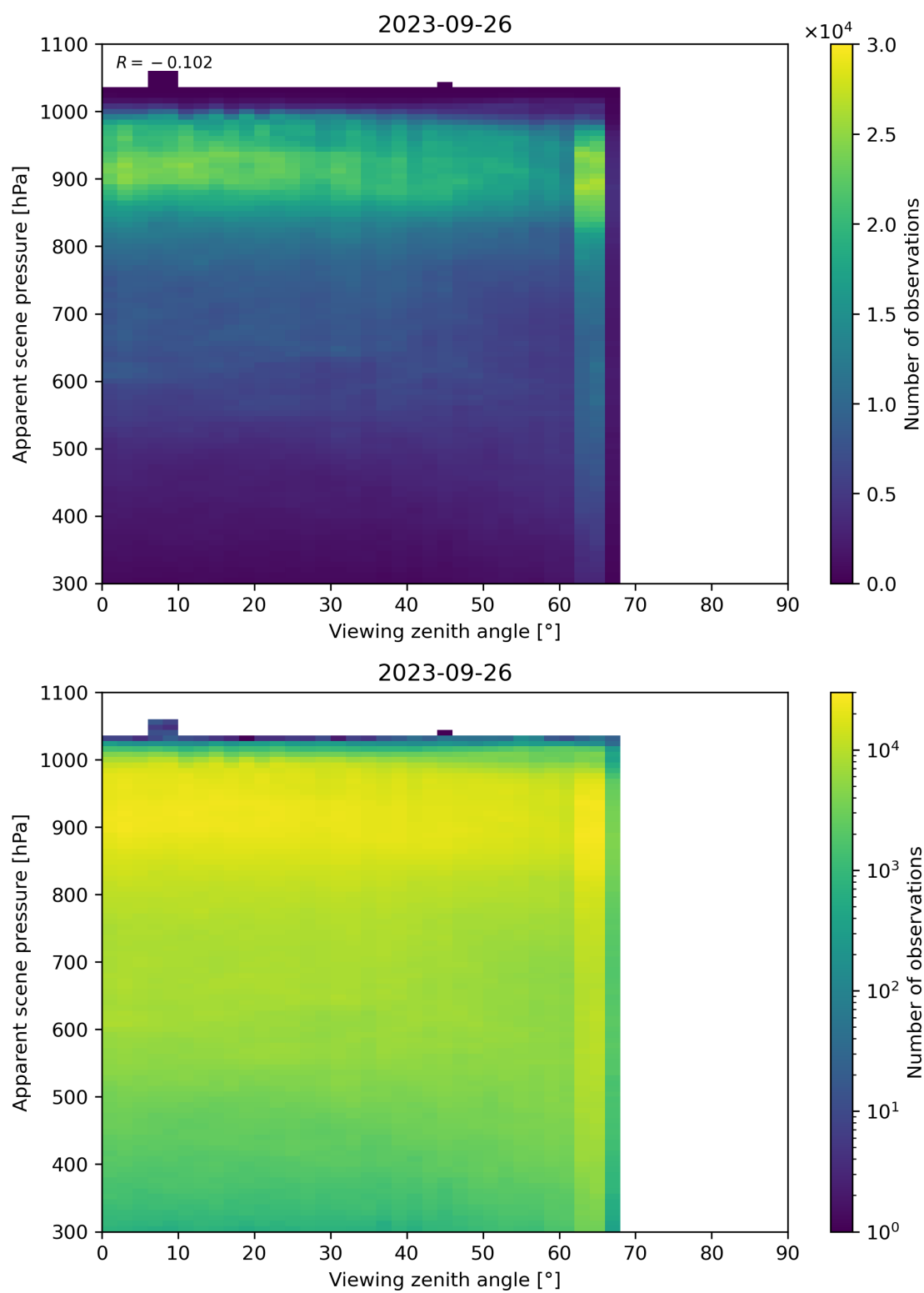
Figure 129: Scatter density plot of “Viewing zenith angle” against “Apparent scene pressure” for 2023-09-26 to 2023-09-27.
