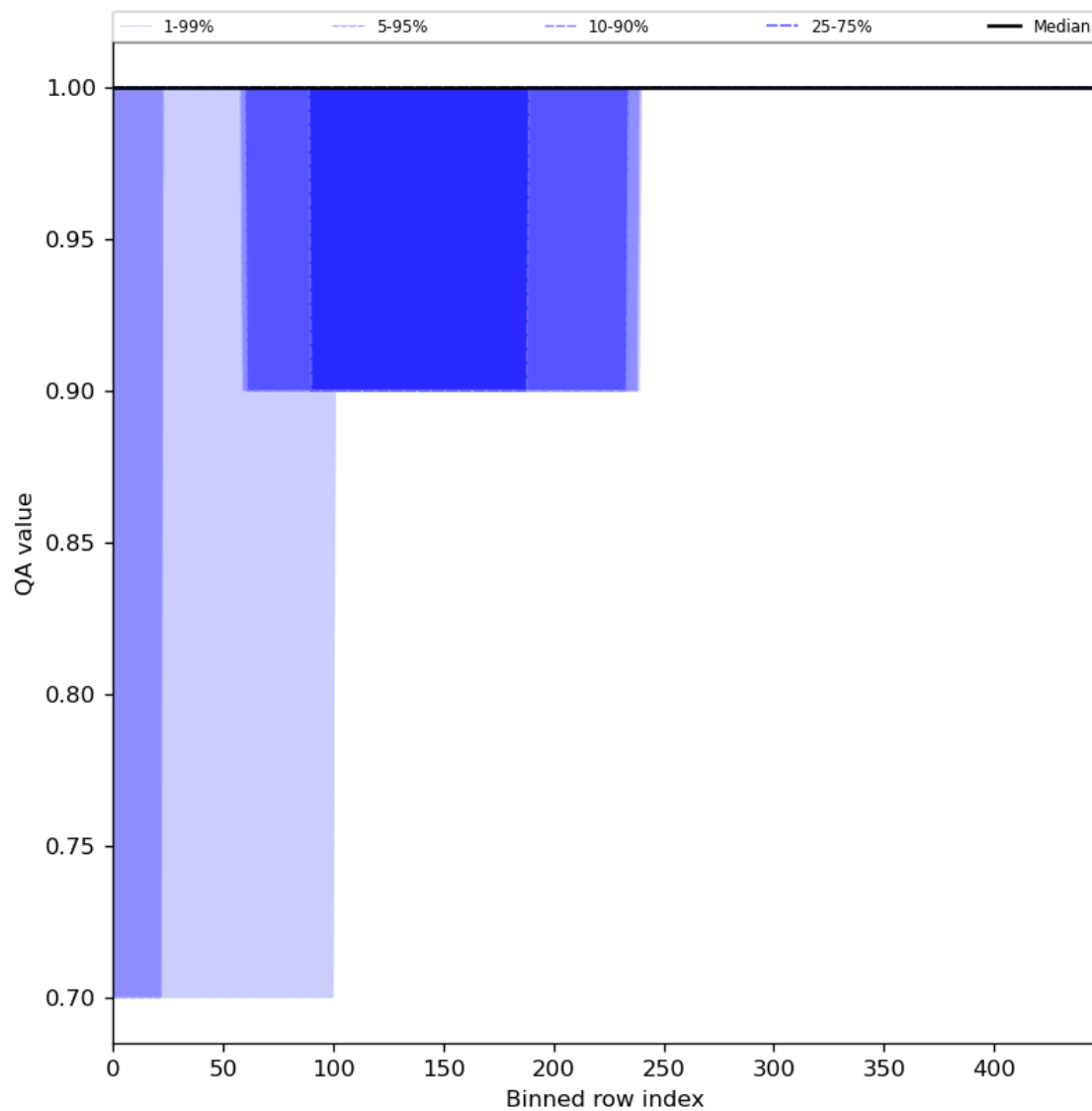
Figure 46: Along track statistics of “QA value” for 2023-09-26 to 2023-09-27
