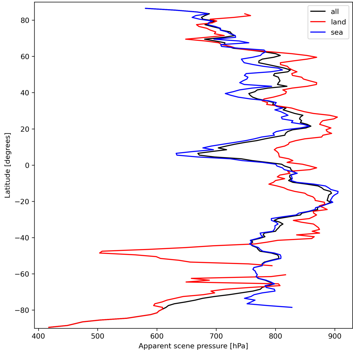
Figure 19: Zonal average of “Apparent scene pressure” for 2023-09-26 to 2023-09-27.
