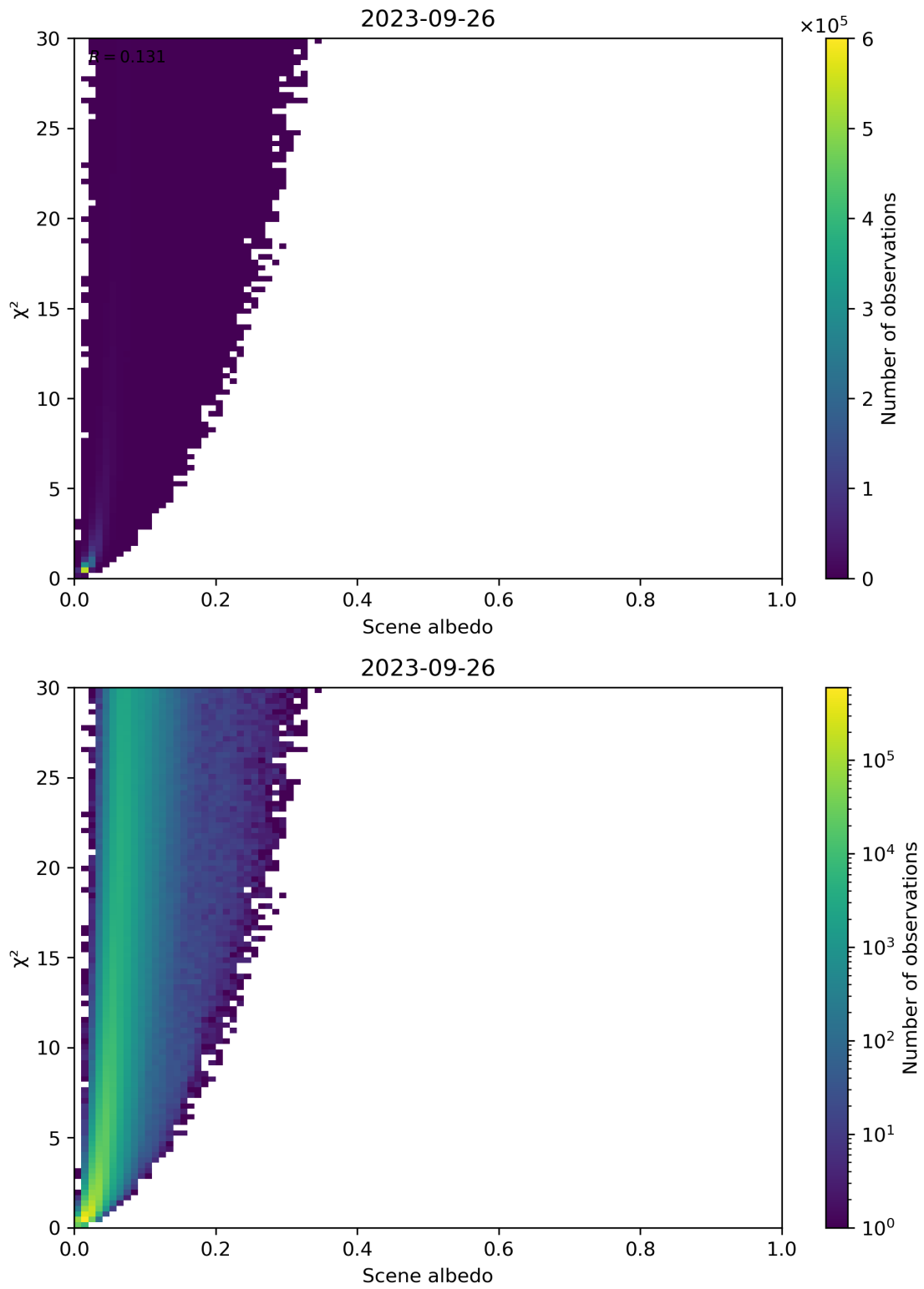
Figure 112: Scatter density plot of “Scene albedo” against “ \chi^2 ” for 2023-09-26 to 2023-09-27.
