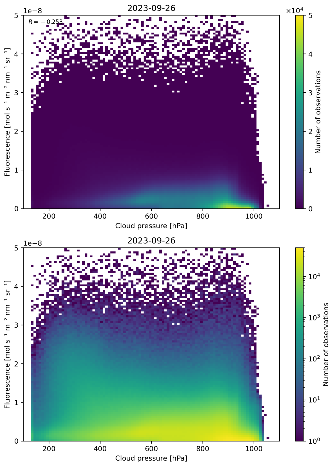
Figure 88: Scatter density plot of “Cloud pressure” against “Fluorescence” for 2023-09-26 to 2023-09-27.
