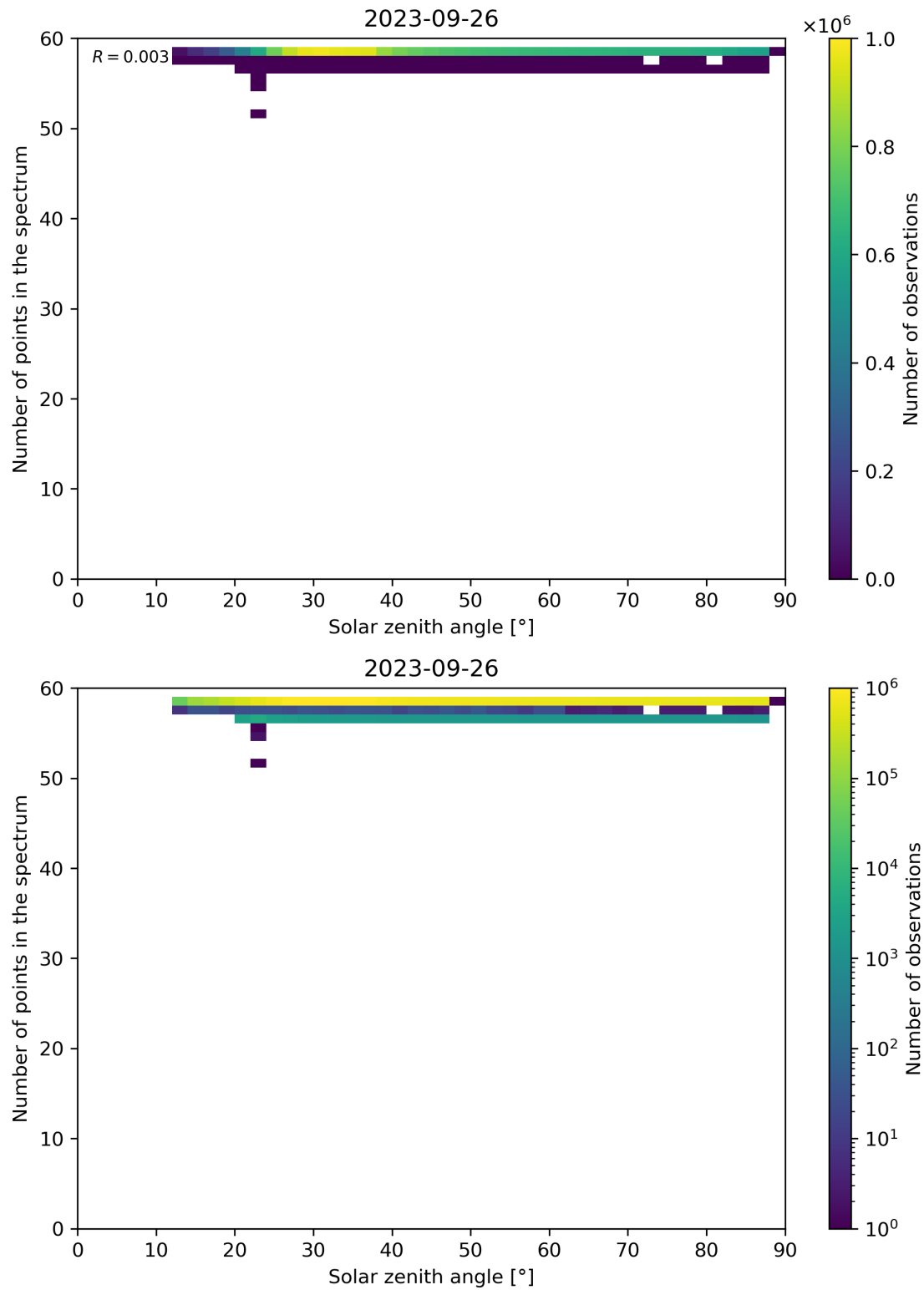
Figure 126: Scatter density plot of “Solar zenith angle” against “Number of points in the spectrum” for 2023-09-26 to 2023-09-27.
