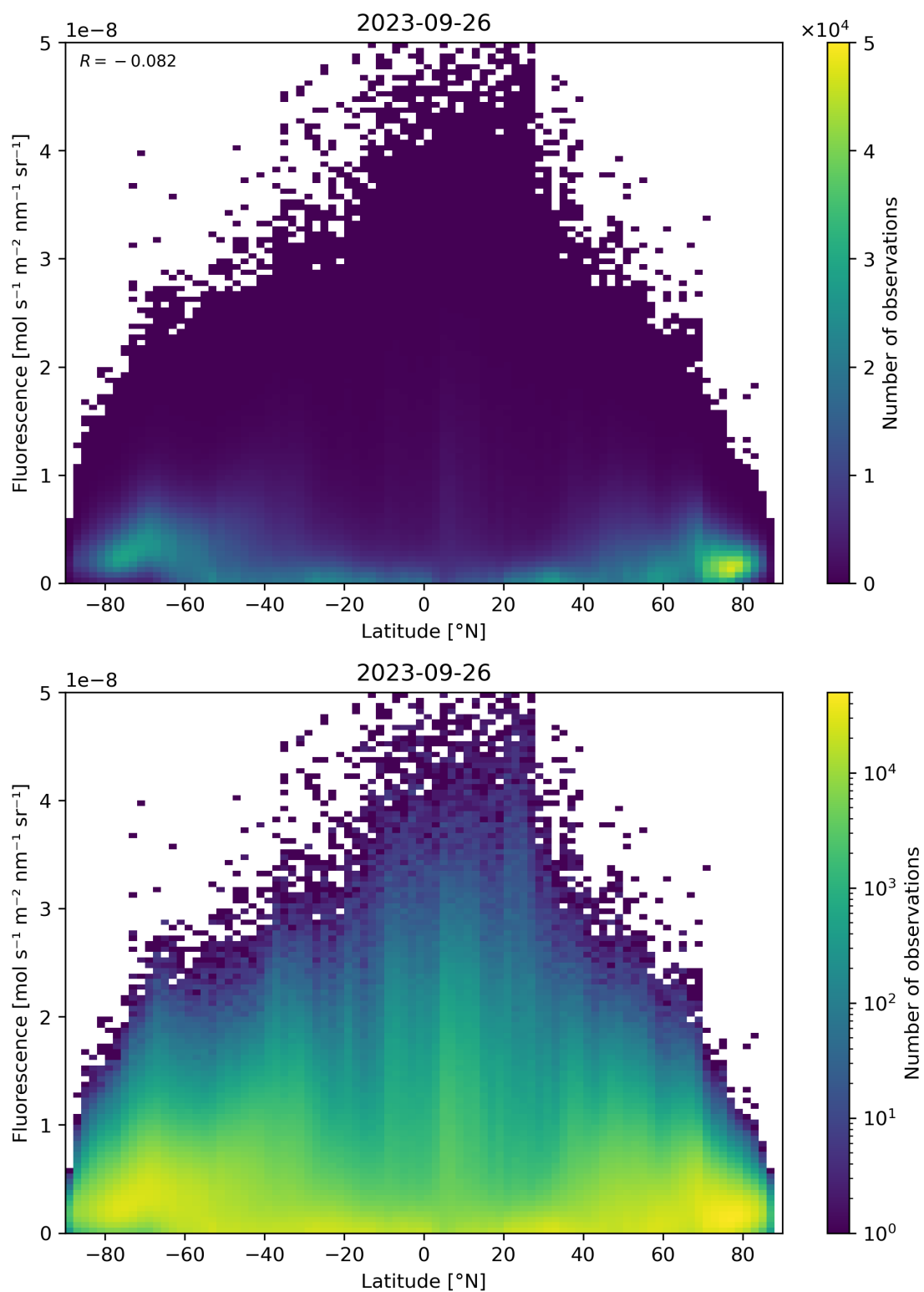
Figure 101: Scatter density plot of “Latitude” against “Fluorescence” for 2023-09-26 to 2023-09-27.
