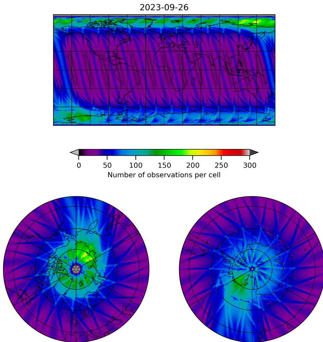
Figure 11: Map of the number of observations for 2023-09-26 to 2023-09-27
