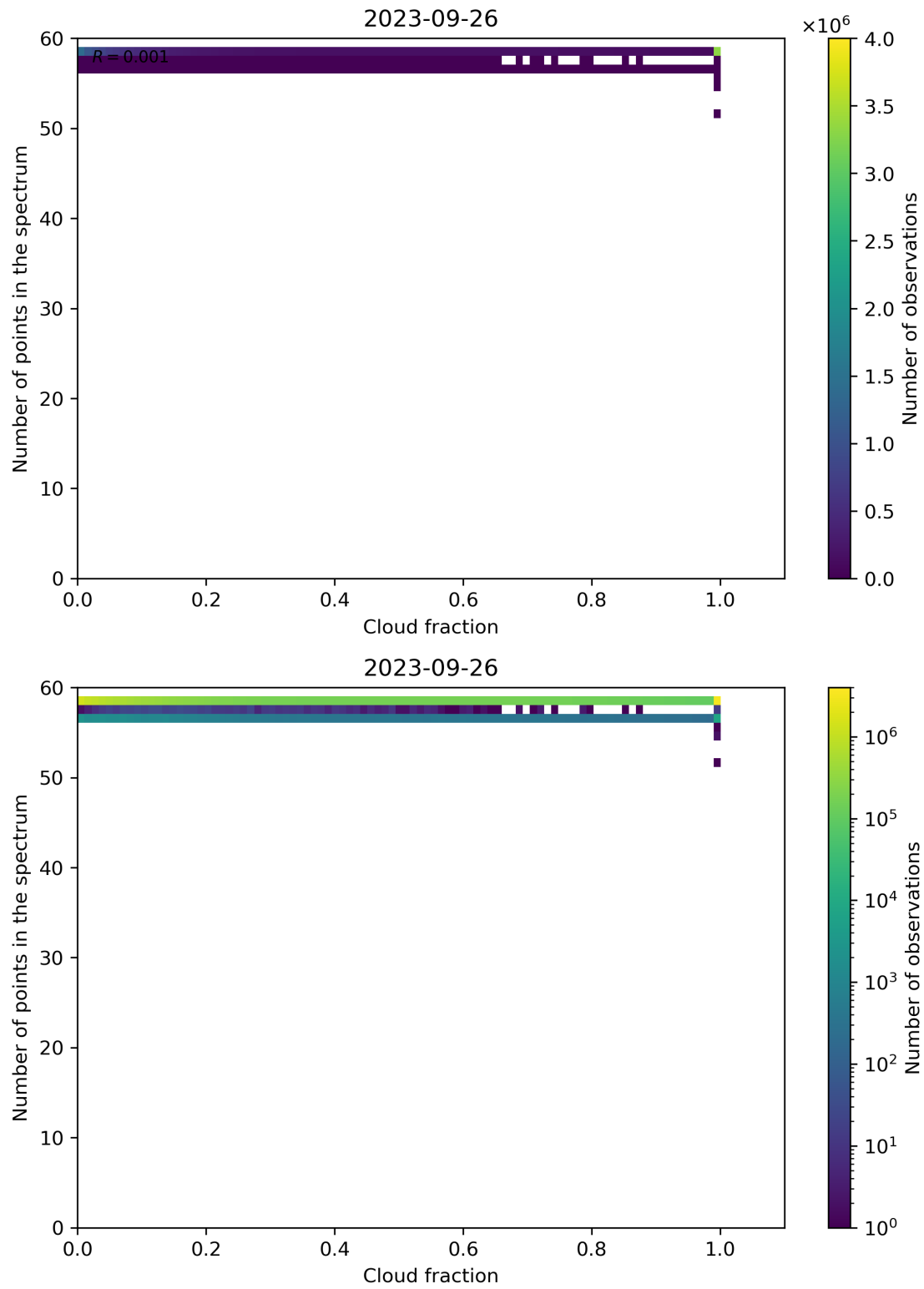
Figure 81: Scatter density plot of “Cloud fraction” against “Number of points in the spectrum” for 2023-09-26 to 2023-09-27.
