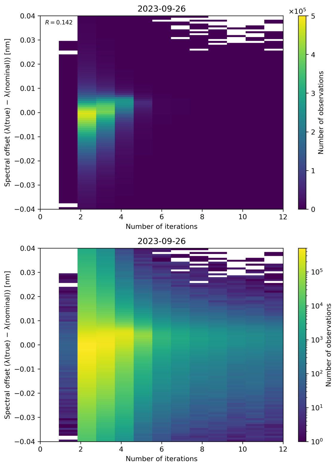
Figure 109: Scatter density plot of “Number of iterations” against “Spectral offset ( \lambda(\text{true}) - \lambda(\text{nominal}) )” for 2023-09-26 to 2023-09-27.
