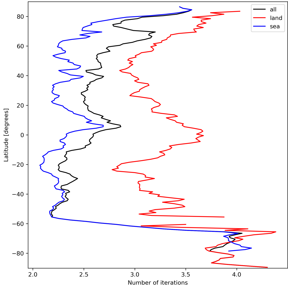
Figure 22: Zonal average of “Number of iterations” for 2023-09-26 to 2023-09-27.
