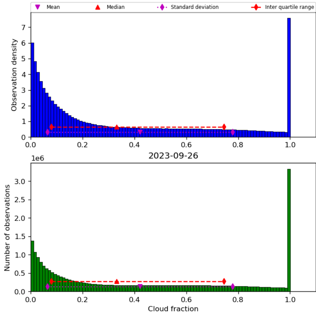
Figure 32: Histogram of “Cloud fraction” for 2023-09-26 to 2023-09-27
