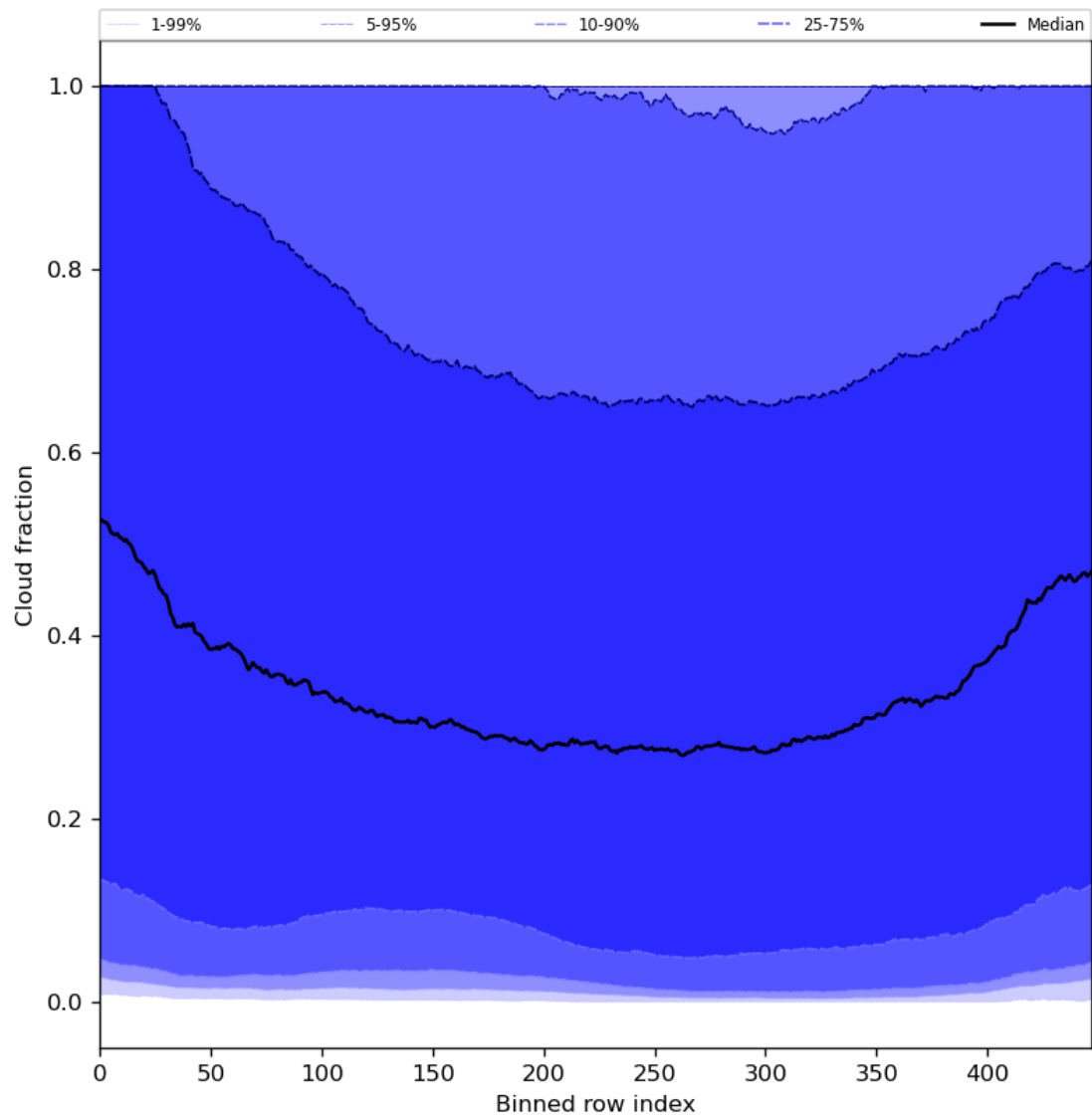
Figure 49: Along track statistics of “Cloud fraction” for 2023-09-26 to 2023-09-27
