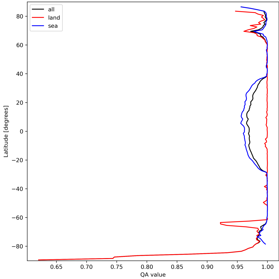
Figure 12: Zonal average of “QA value” for 2023-09-26 to 2023-09-27.
