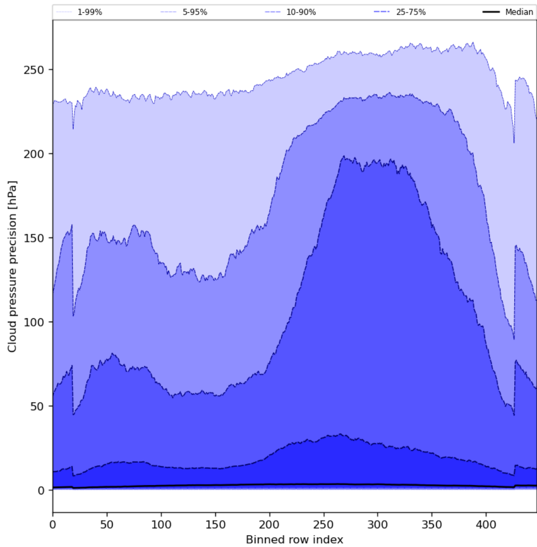
Figure 48: Along track statistics of “Cloud pressure precision” for 2023-09-26 to 2023-09-27
