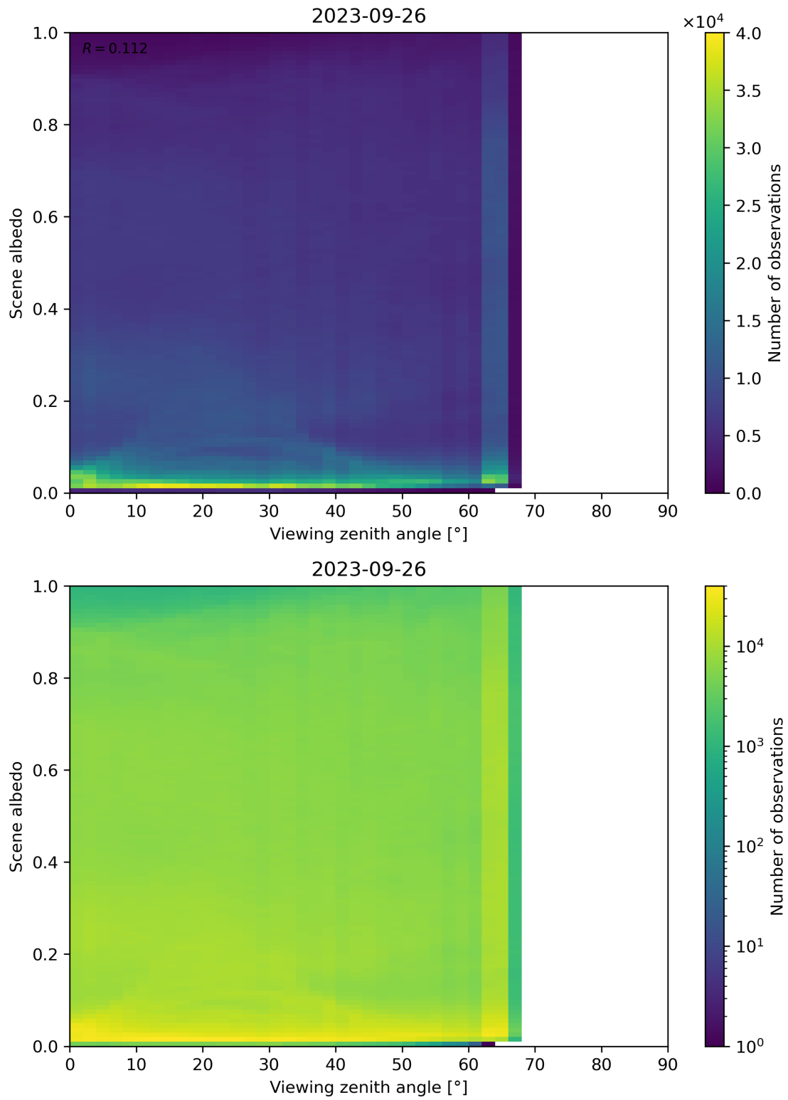
Figure 138: Scatter density plot of “Viewing zenith angle” against “Scene albedo” for 2023-09-26 to 2023-09-27.
