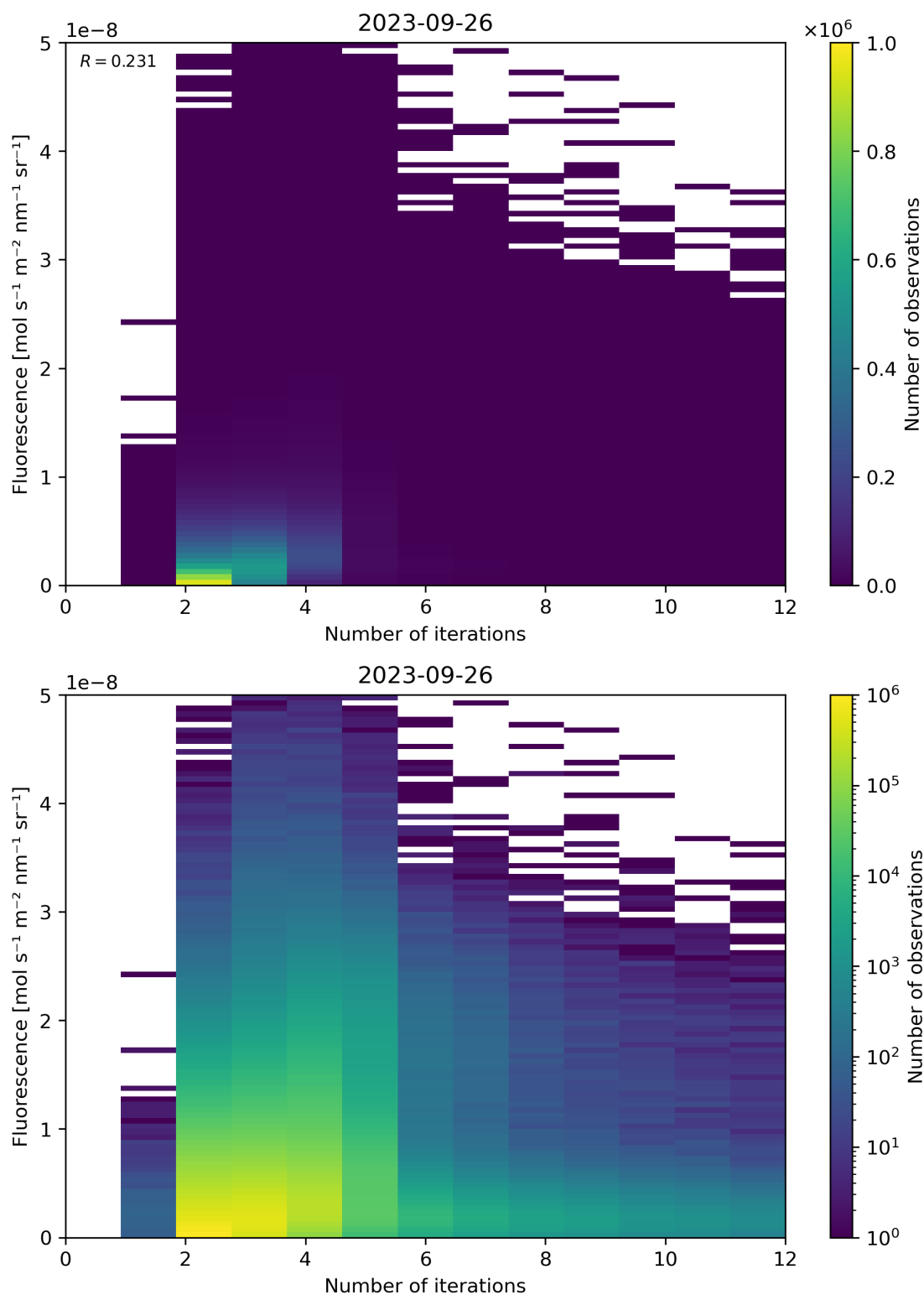
Figure 107: Scatter density plot of “Number of iterations” against “Fluorescence” for 2023-09-26 to 2023-09-27.
