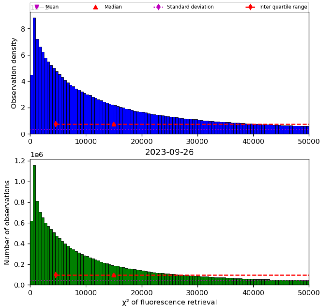
Figure 42: Histogram of “ \chi^2 of fluorescence retrieval” for 2023-09-26 to 2023-09-27
