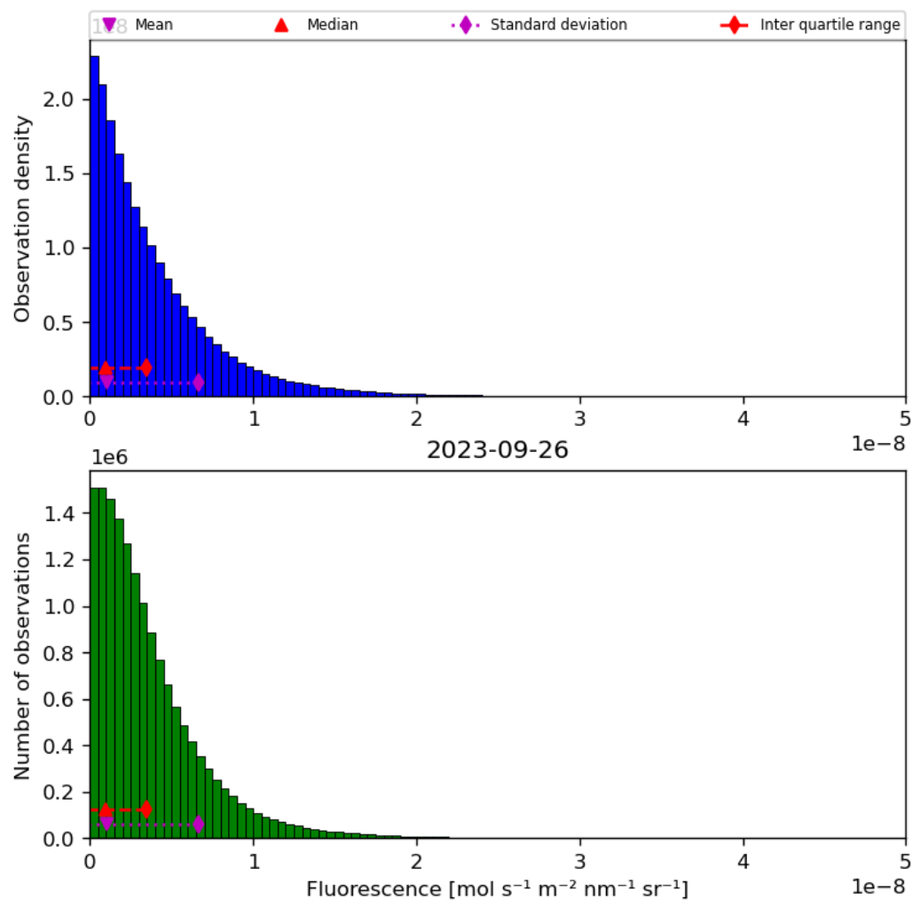
Figure 40: Histogram of “Fluorescence” for 2023-09-26 to 2023-09-27
