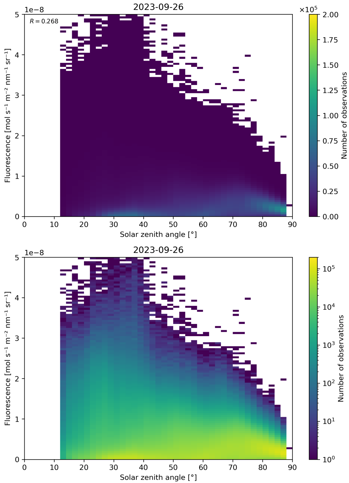
Figure 123: Scatter density plot of “Solar zenith angle” against “Fluorescence” for 2023-09-26 to 2023-09-27.
