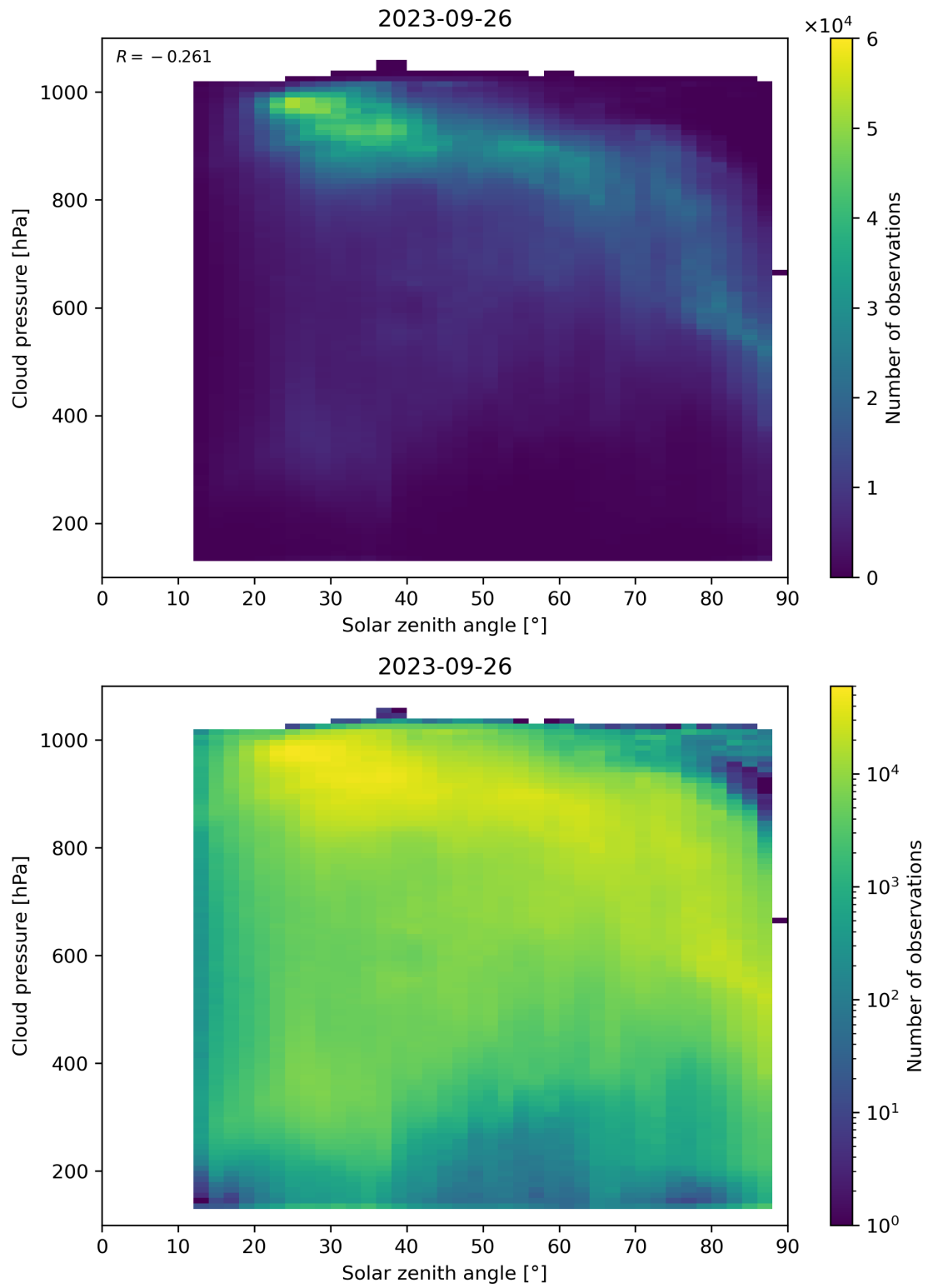
Figure 122: Scatter density plot of “Solar zenith angle” against “Cloud pressure” for 2023-09-26 to 2023-09-27.
