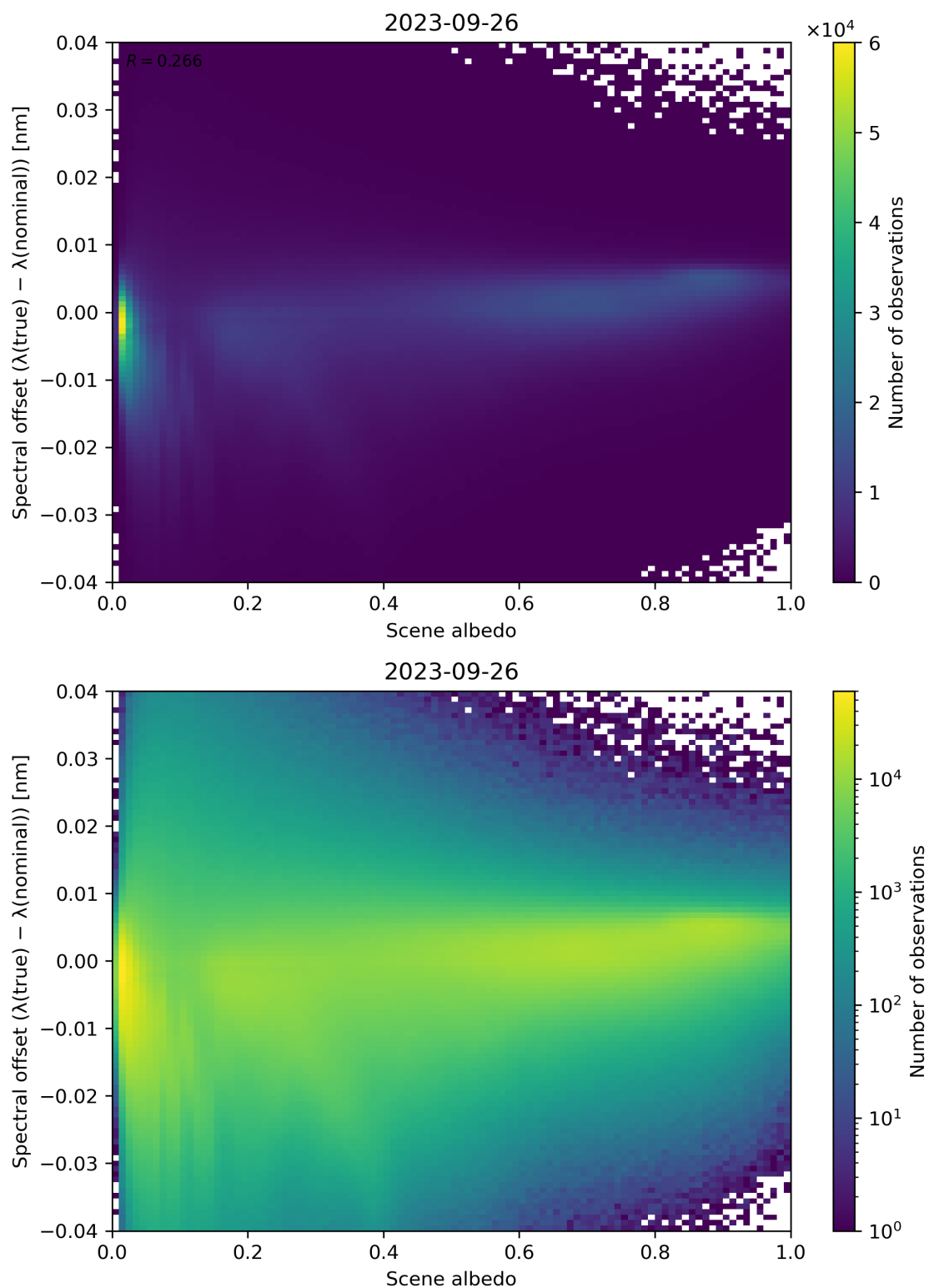
Figure 117: Scatter density plot of “Scene albedo” against “Spectral offset ( \lambda(\text{true}) - \lambda(\text{nominal}) )” for 2023-09-26 to 2023-09-27.
