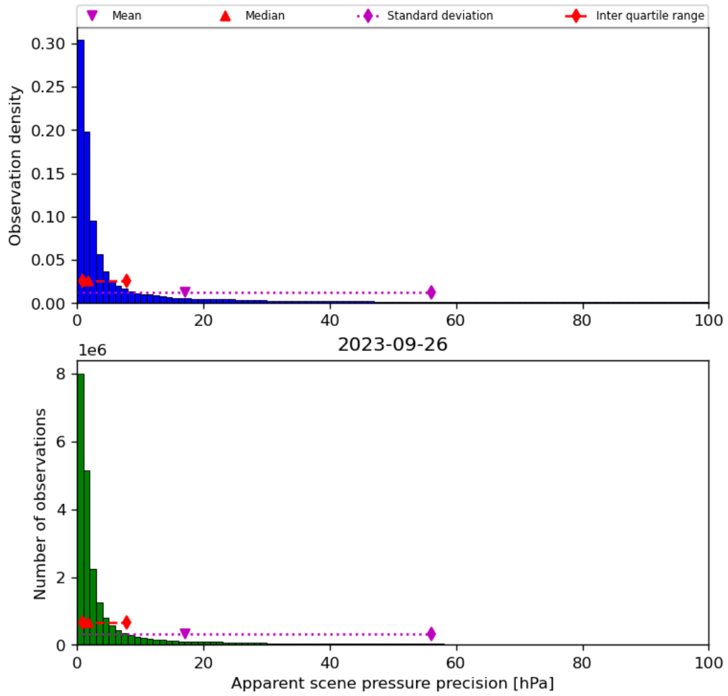
Figure 37: Histogram of “Apparent scene pressure precision” for 2023-09-26 to 2023-09-27
