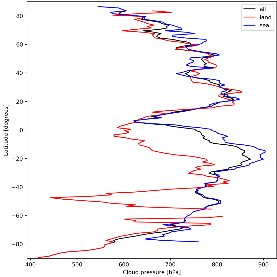
Figure 13: Zonal average of “Cloud pressure” for 2023-09-26 to 2023-09-27.
