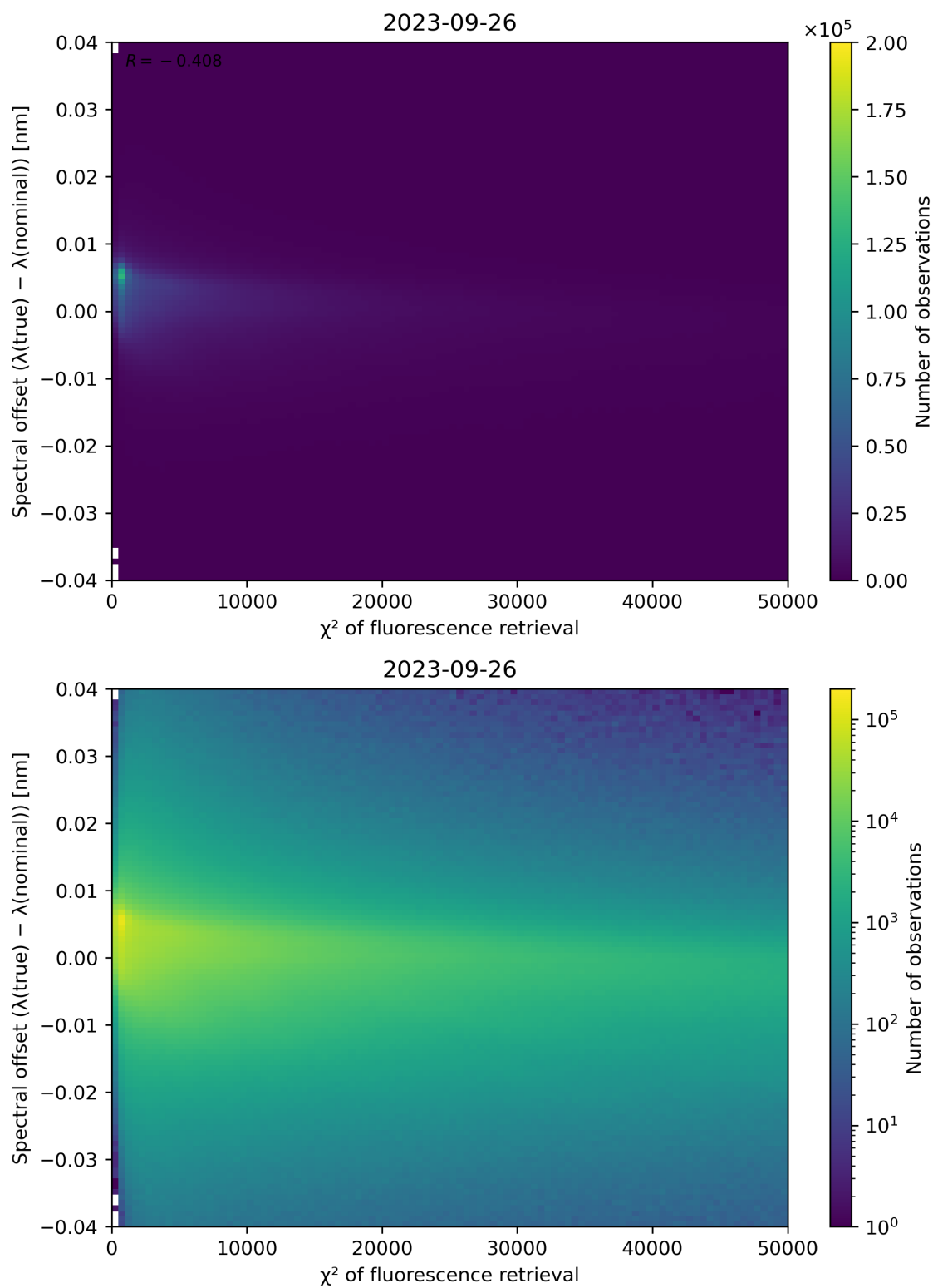
Figure 72: Scatter density plot of " \chi^2 of fluorescence retrieval" against "Spectral offset ( \lambda(\text{true}) - \lambda(\text{nominal}) )" for 2023-09-26 to 2023-09-27.
