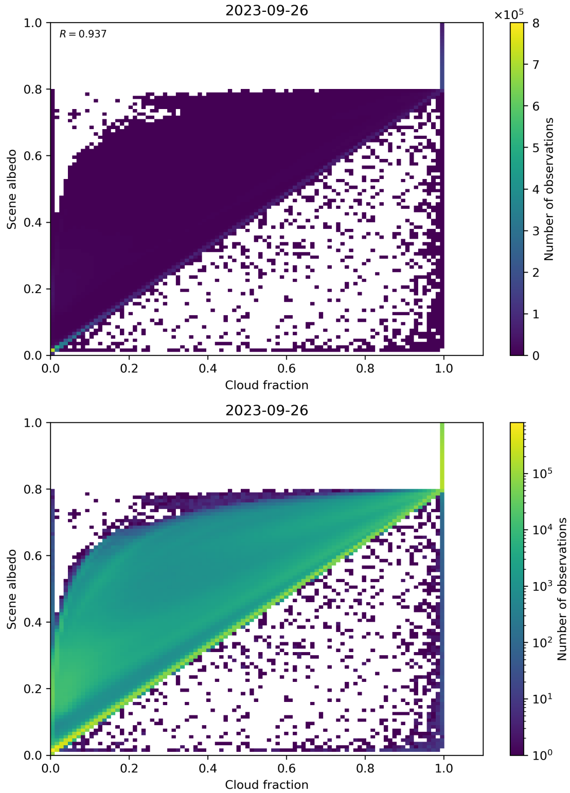
Figure 82: Scatter density plot of “Cloud fraction” against “Scene albedo” for 2023-09-26 to 2023-09-27.
