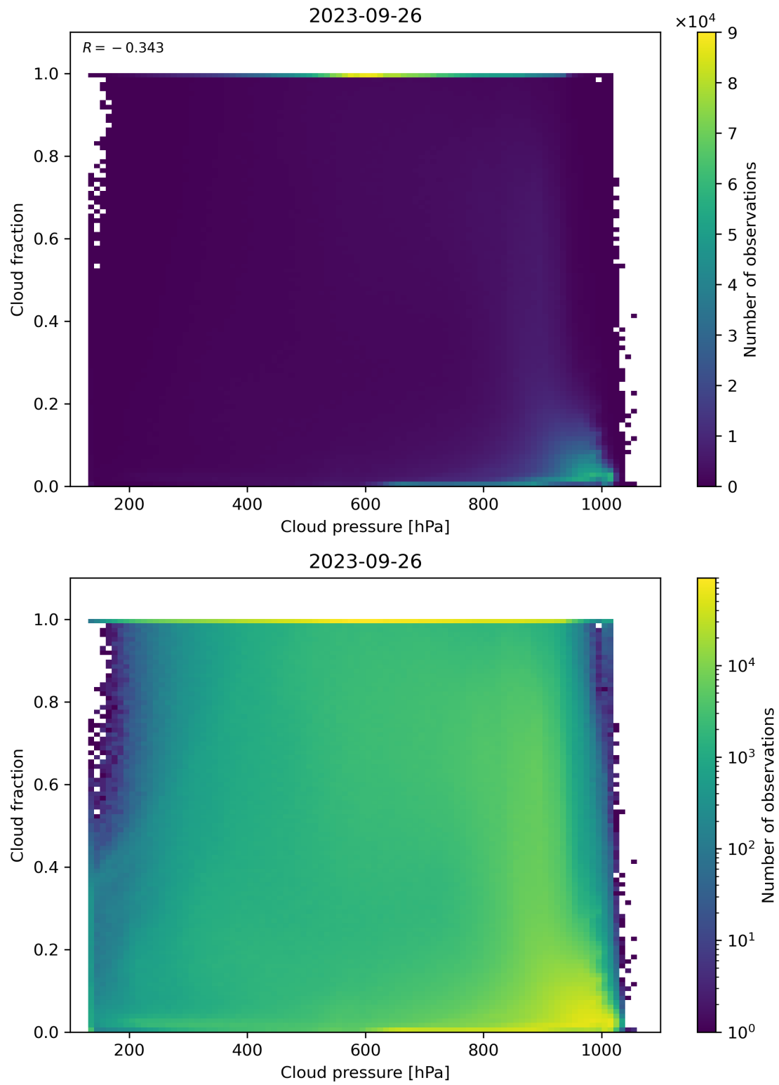
Figure 87: Scatter density plot of “Cloud pressure” against “Cloud fraction” for 2023-09-26 to 2023-09-27.
