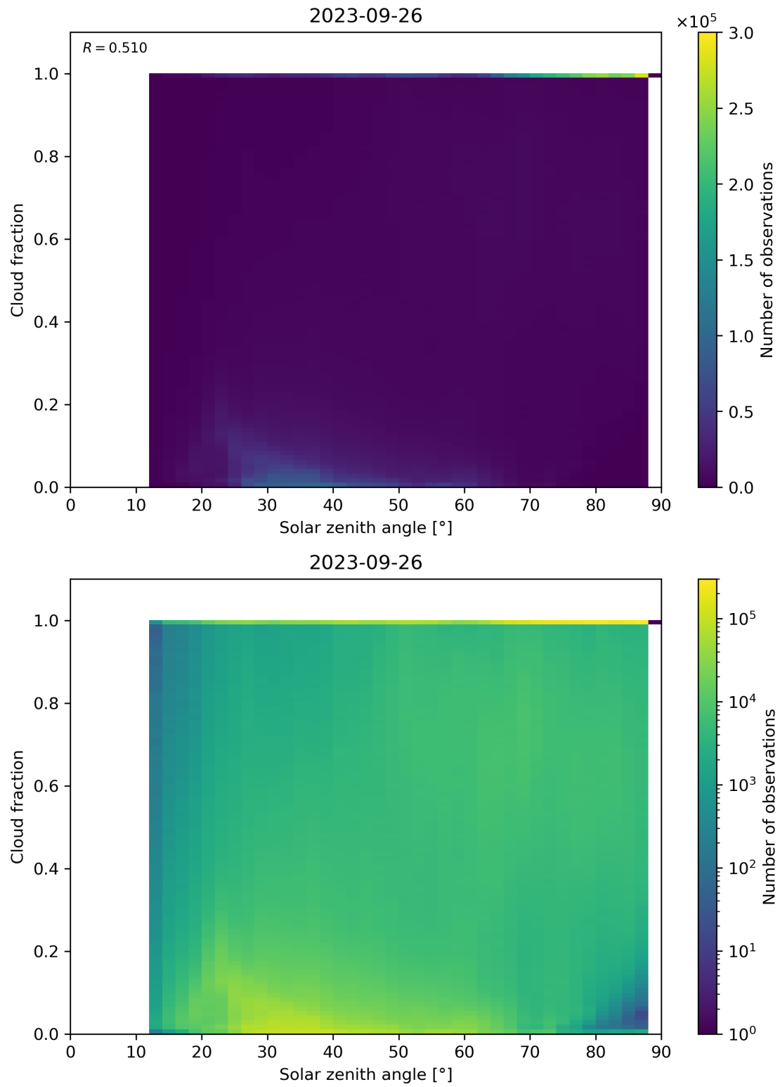
Figure 121: Scatter density plot of “Solar zenith angle” against “Cloud fraction” for 2023-09-26 to 2023-09-27.
