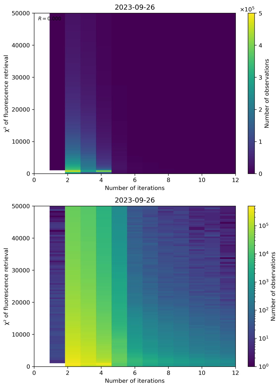
Figure 106: Scatter density plot of “Number of iterations” against “ \chi^2 of fluorescence retrieval” for 2023-09-26 to 2023-09-27.
