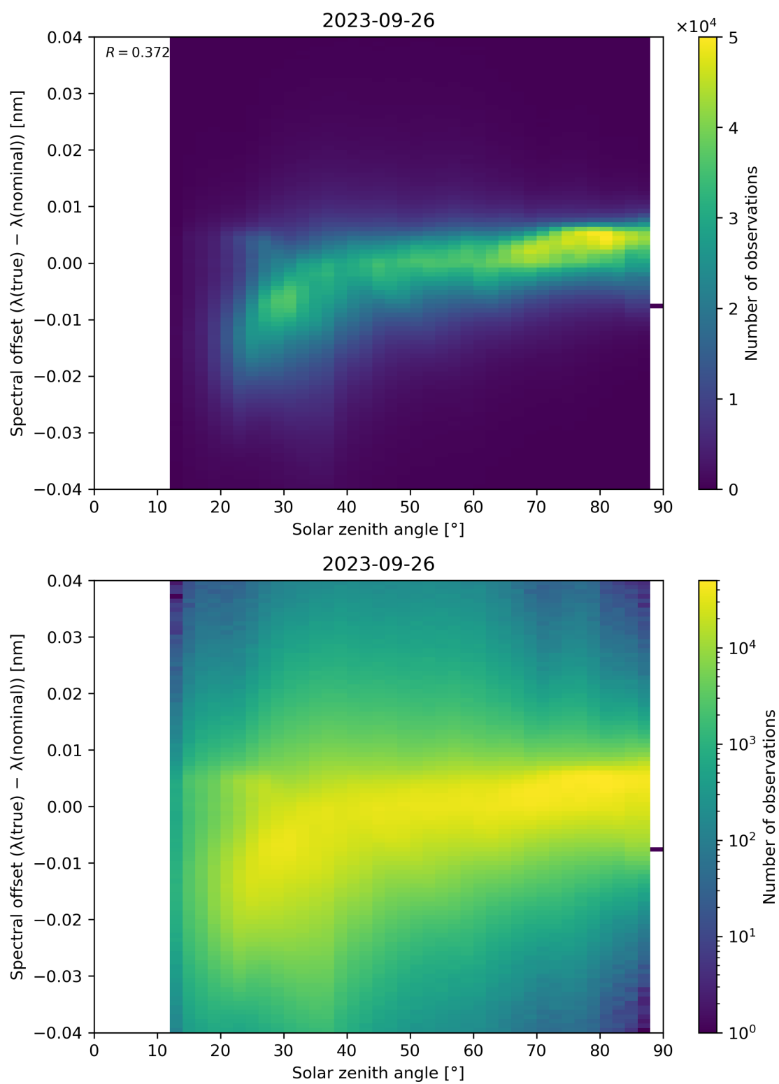
Figure 128: Scatter density plot of “Solar zenith angle” against “Spectral offset ( \lambda(\text{true}) - \lambda(\text{nominal}) )” for 2023-09-26 to 2023-09-27.
