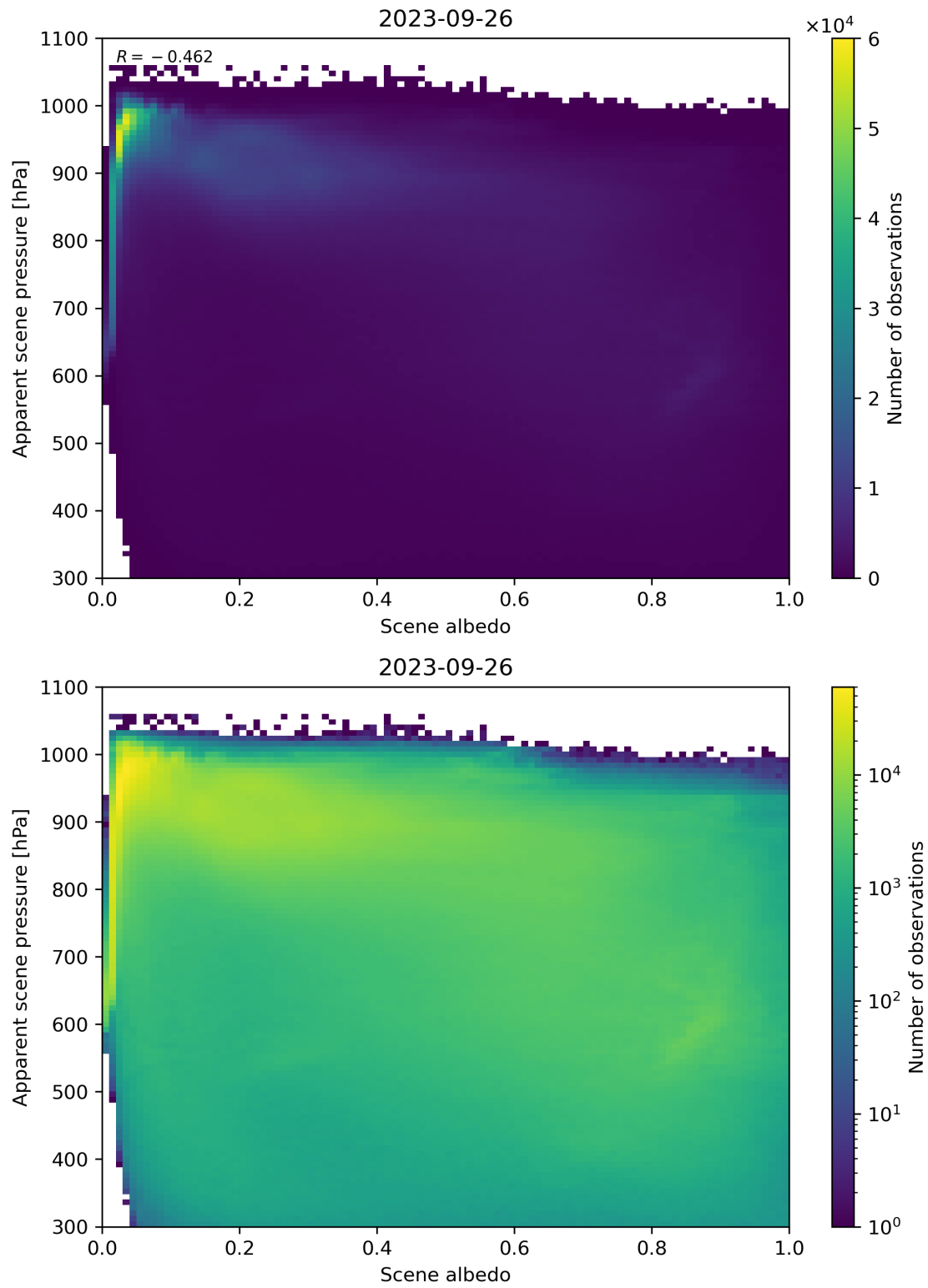
Figure 111: Scatter density plot of “Scene albedo” against “Apparent scene pressure” for 2023-09-26 to 2023-09-27.
