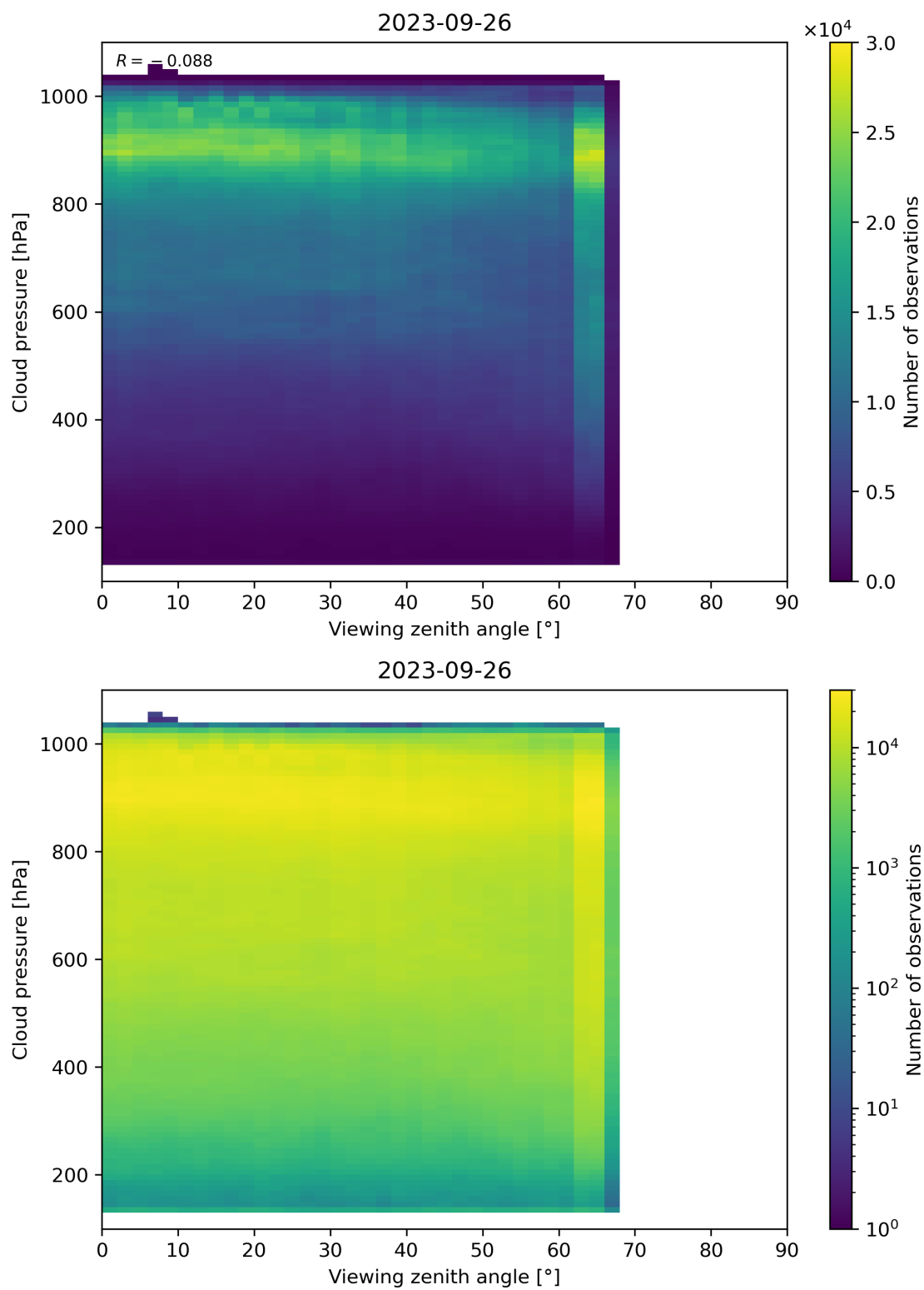
Figure 133: Scatter density plot of “Viewing zenith angle” against “Cloud pressure” for 2023-09-26 to 2023-09-27.
