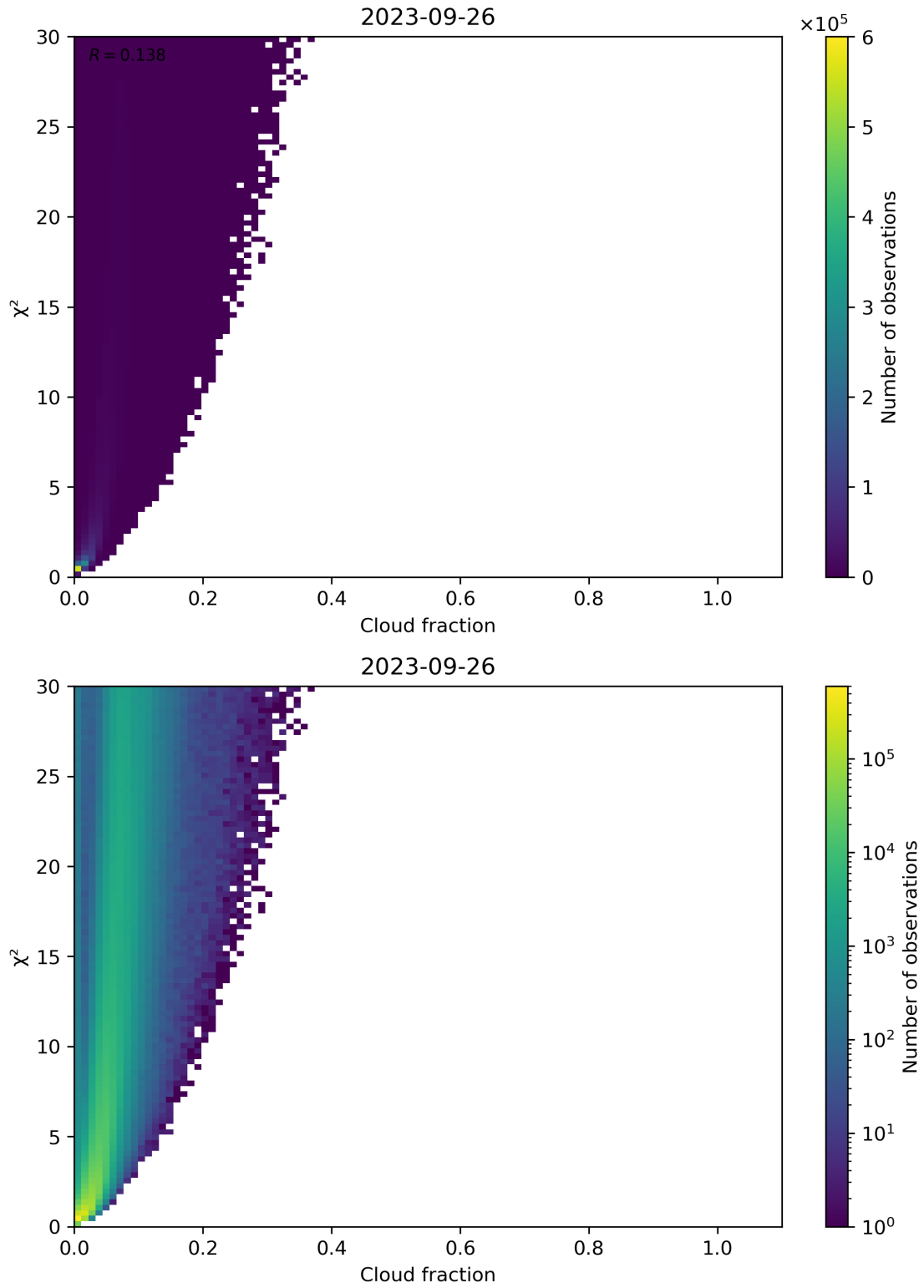
Figure 77: Scatter density plot of “Cloud fraction” against “ \chi^2 ” for 2023-09-26 to 2023-09-27.
