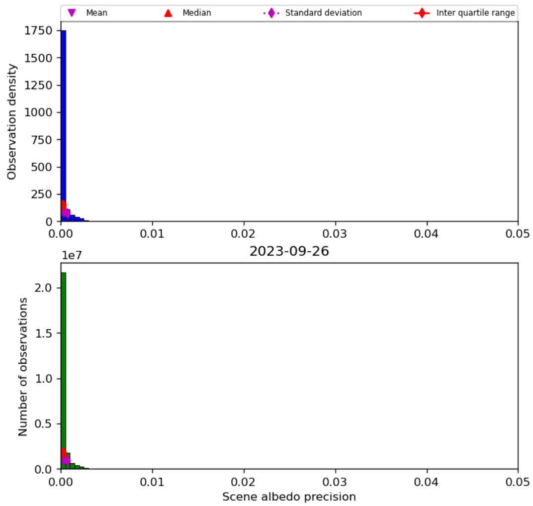
Figure 35: Histogram of “Scene albedo precision” for 2023-09-26 to 2023-09-27
