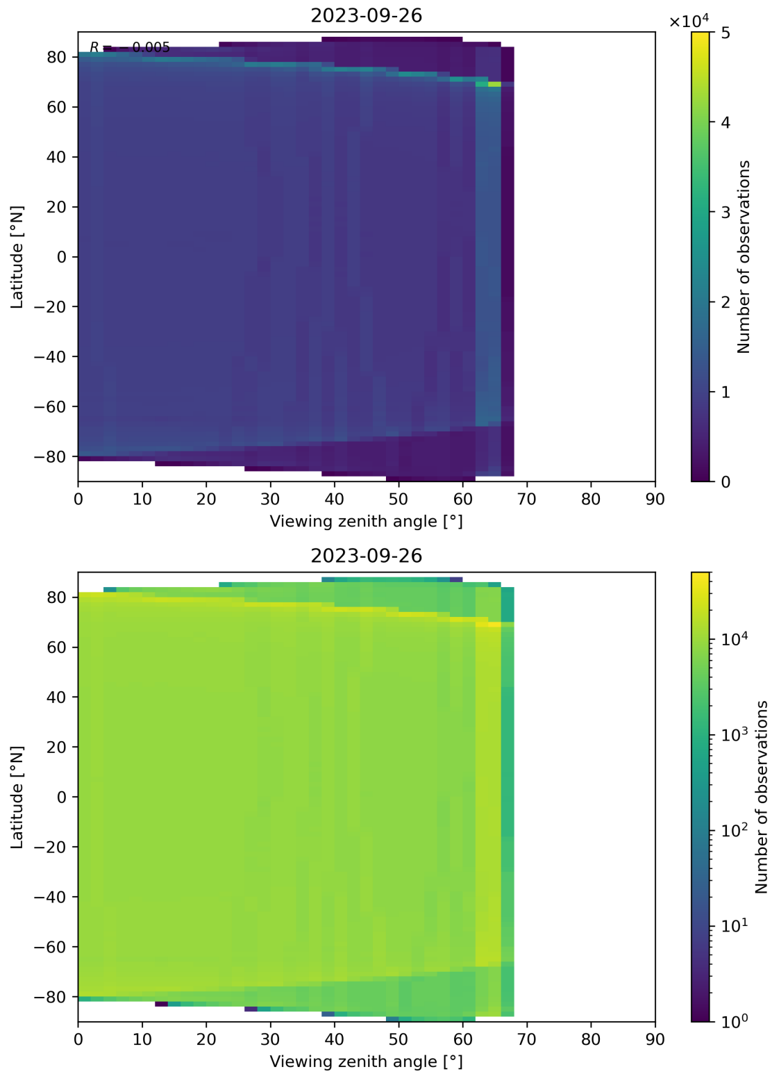
Figure 135: Scatter density plot of “Viewing zenith angle” against “Latitude” for 2023-09-26 to 2023-09-27.
