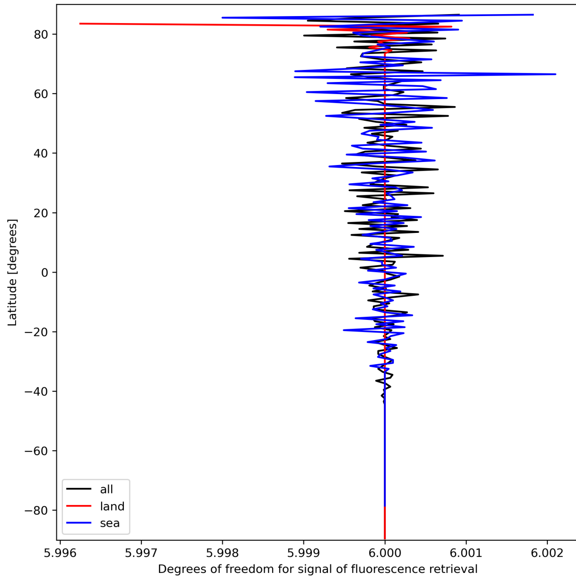
Figure 26: Zonal average of “Degrees of freedom for signal of fluorescence retrieval” for 2023-09-26 to 2023-09-27.
