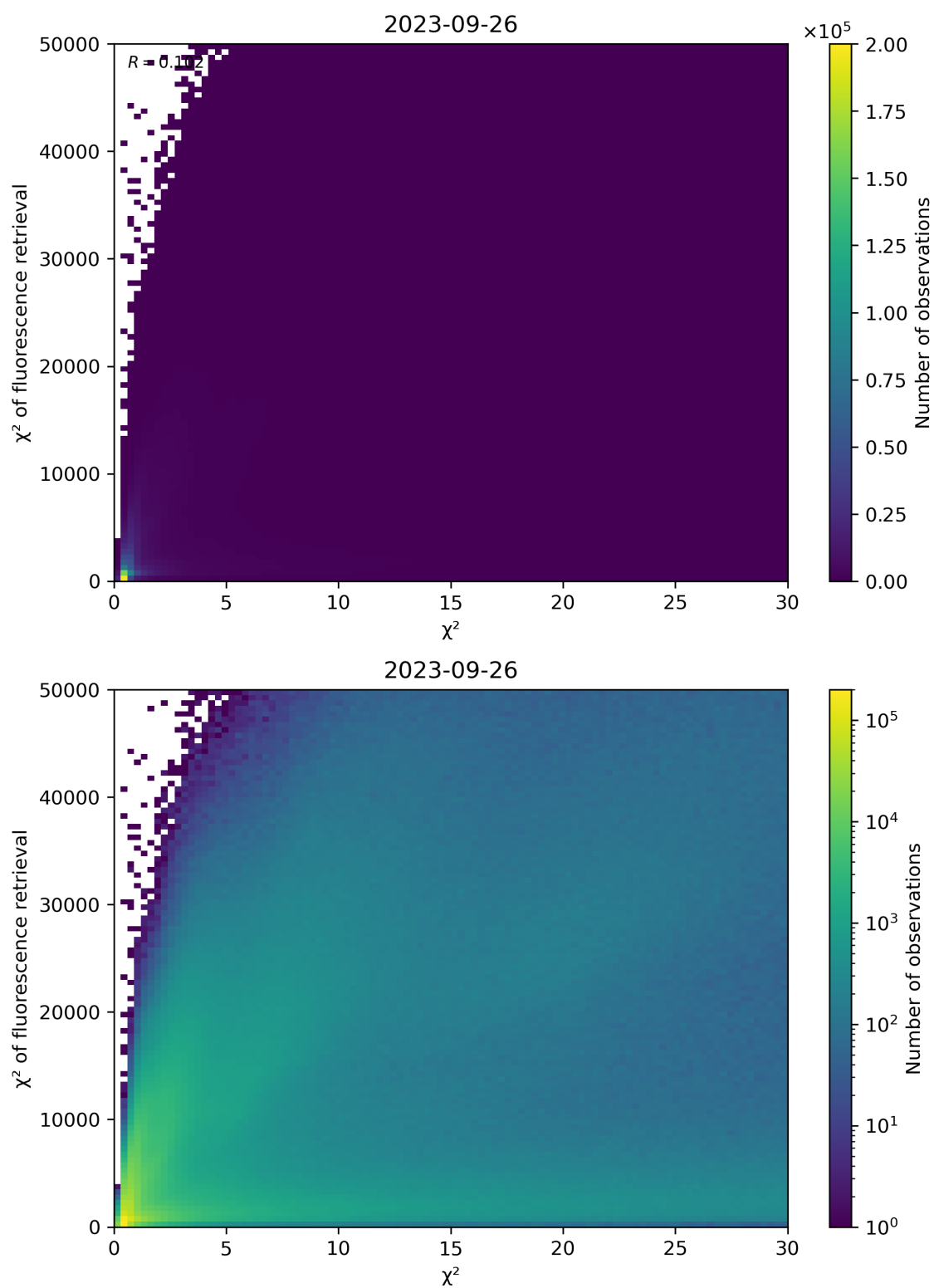
Figure 69: Scatter density plot of “ \chi^2 ” against “ \chi^2 of fluorescence retrieval” for 2023-09-26 to 2023-09-27.
