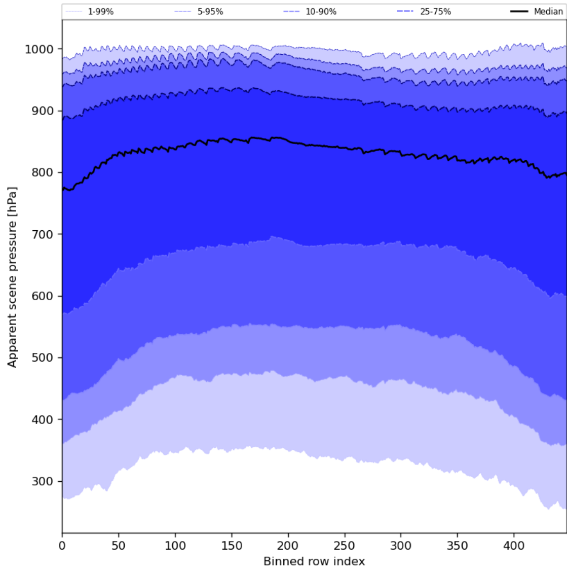
Figure 53: Along track statistics of “Apparent scene pressure” for 2023-09-26 to 2023-09-27
