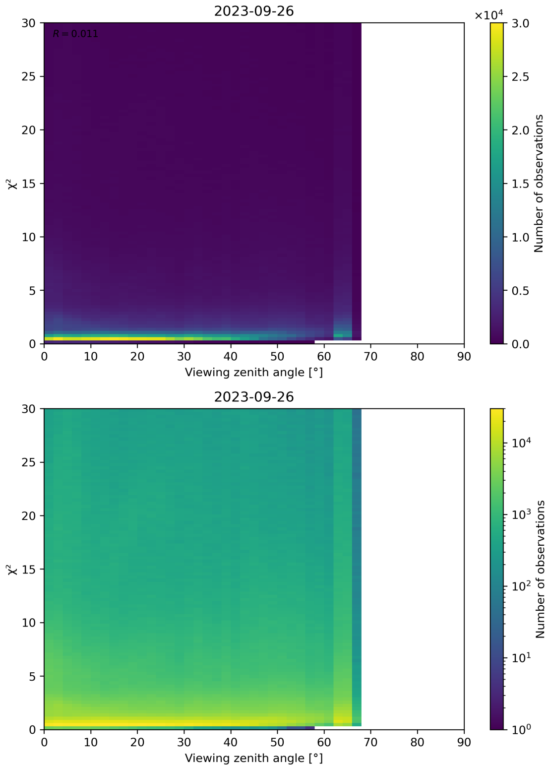
Figure 130: Scatter density plot of “Viewing zenith angle” against “ \chi^2 ” for 2023-09-26 to 2023-09-27.
