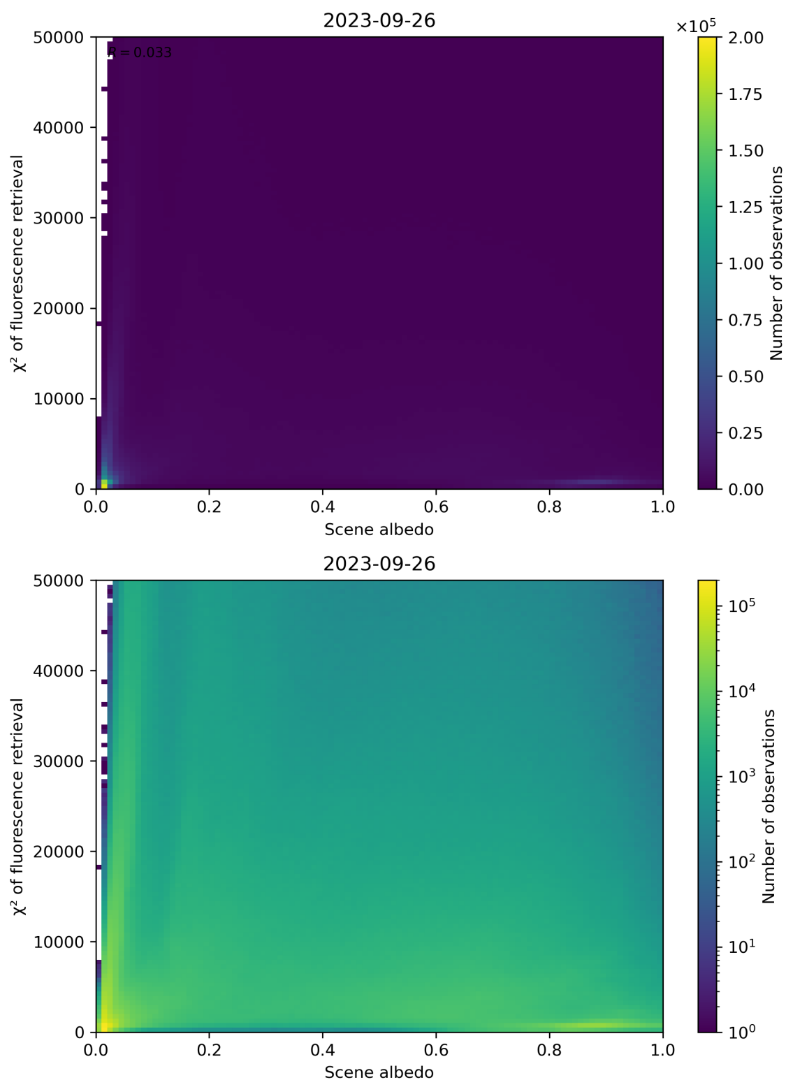
Figure 113: Scatter density plot of “Scene albedo” against “ \chi^2 of fluorescence retrieval” for 2023-09-26 to 2023-09-27.
