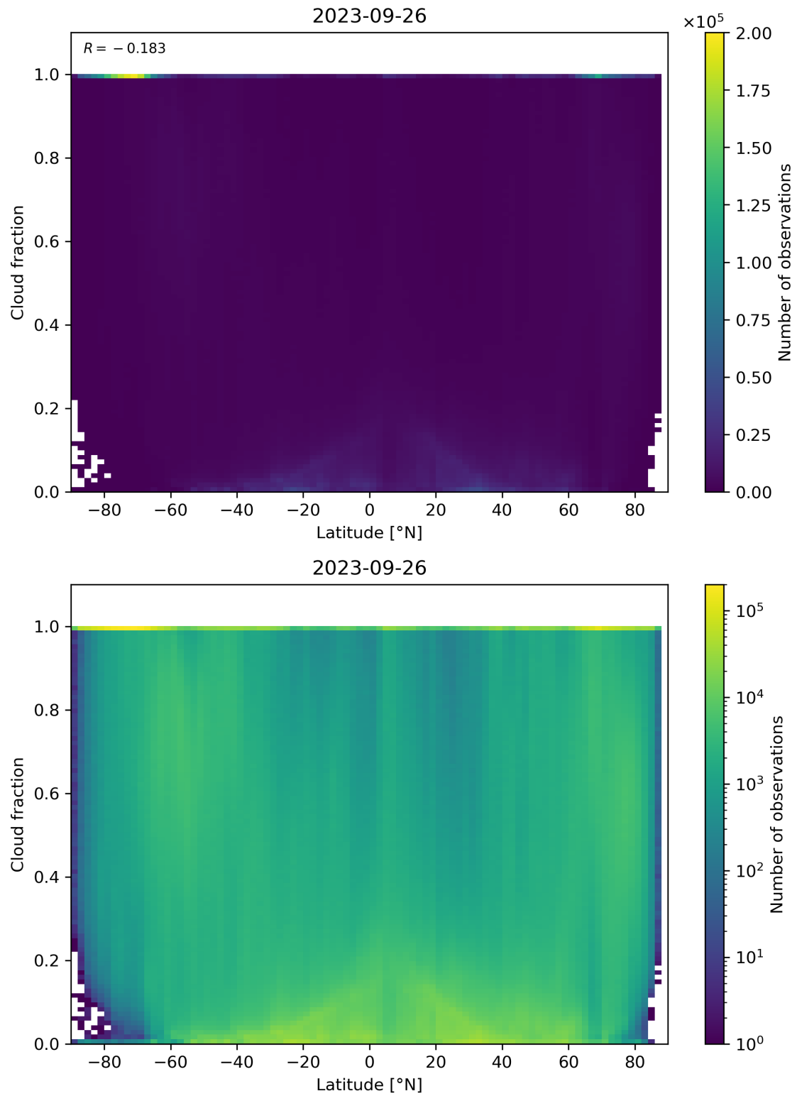
Figure 99: Scatter density plot of “Latitude” against “Cloud fraction” for 2023-09-26 to 2023-09-27.
