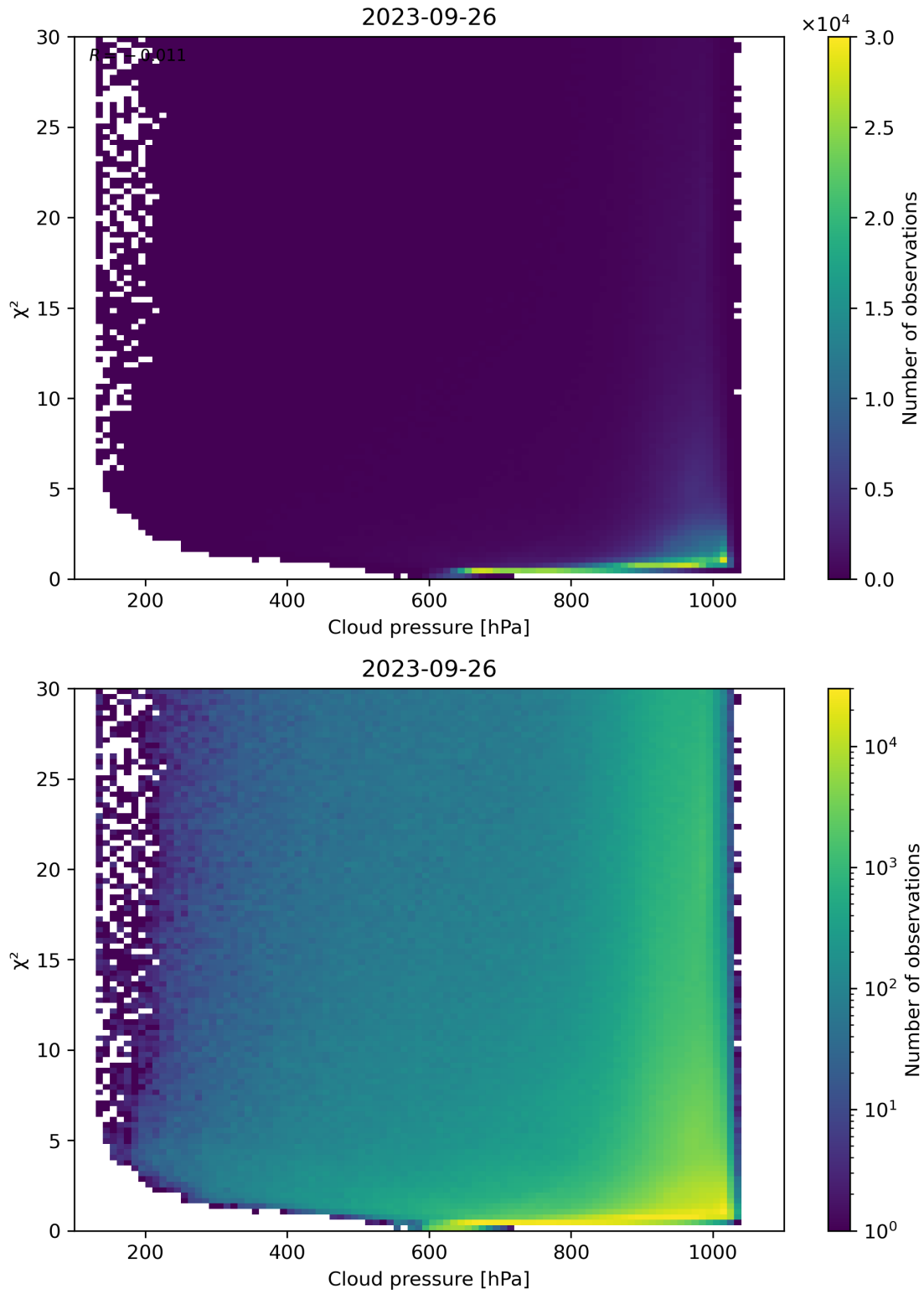
Figure 85: Scatter density plot of “Cloud pressure” against “ \chi^2 ” for 2023-09-26 to 2023-09-27.
