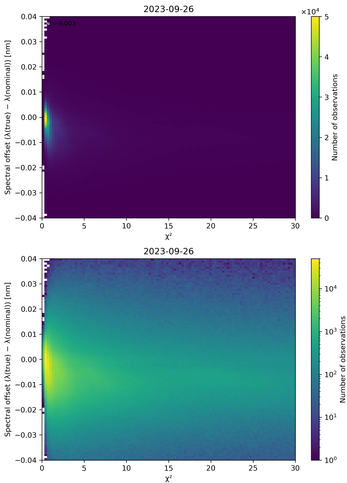
Figure 75: Scatter density plot of “ \chi^2 ” against “Spectral offset ( \lambda(\text{true}) - \lambda(\text{nominal}) )” for 2023-09-26 to 2023-09-27.
