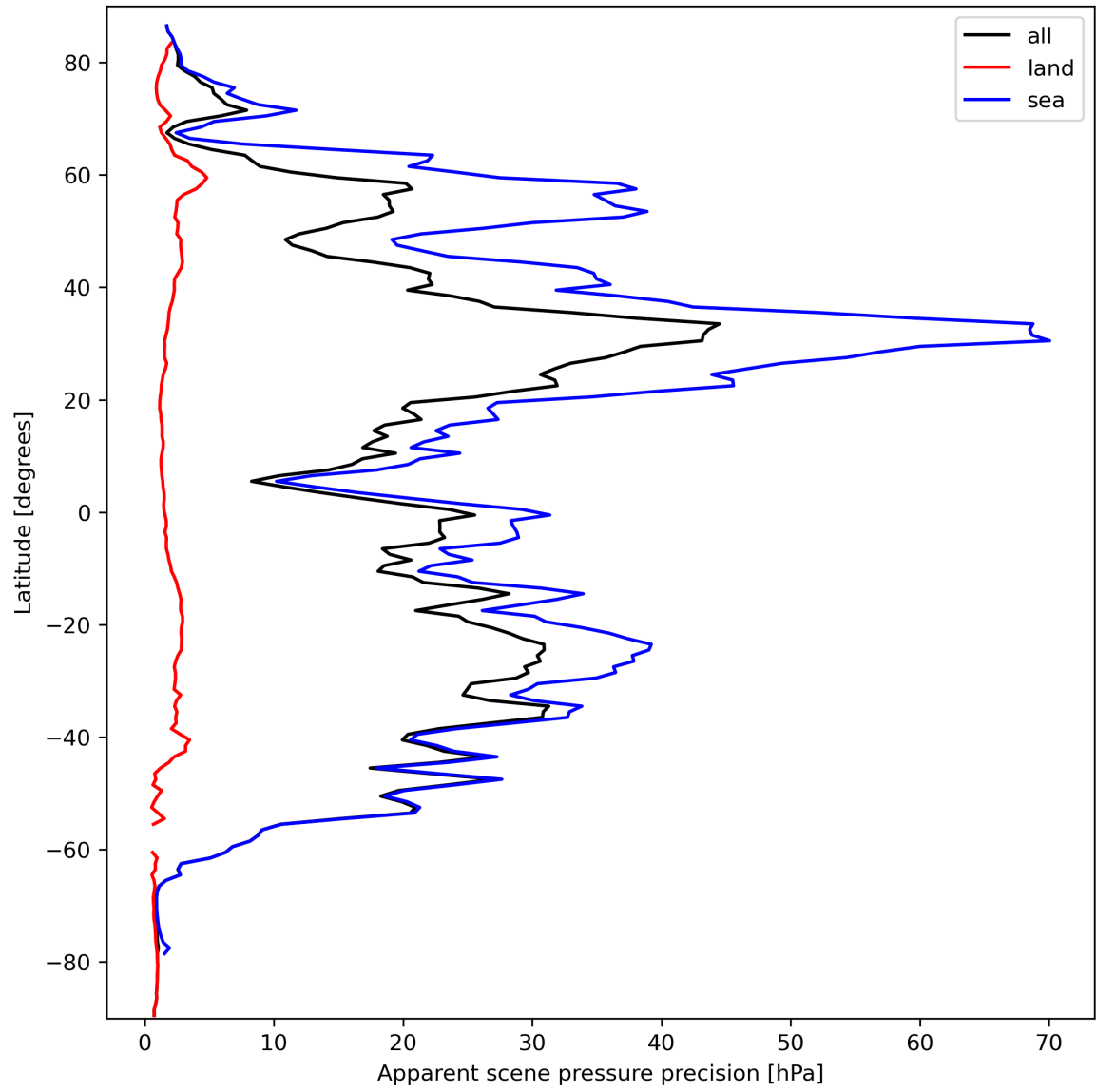
Figure 20: Zonal average of “Apparent scene pressure precision” for 2023-09-26 to 2023-09-27.
