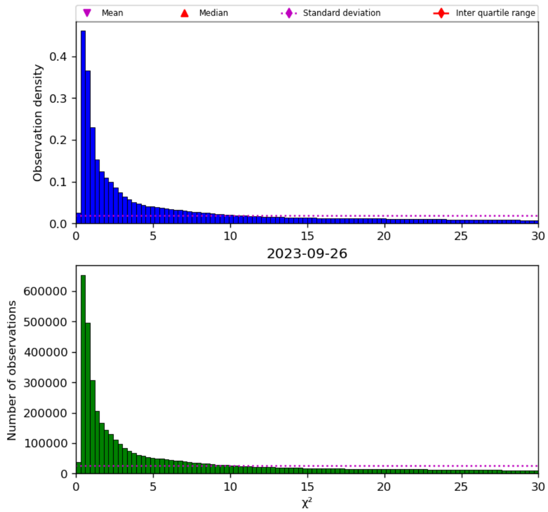
Figure 38: Histogram of “ \chi^2 ” for 2023-09-26 to 2023-09-27
