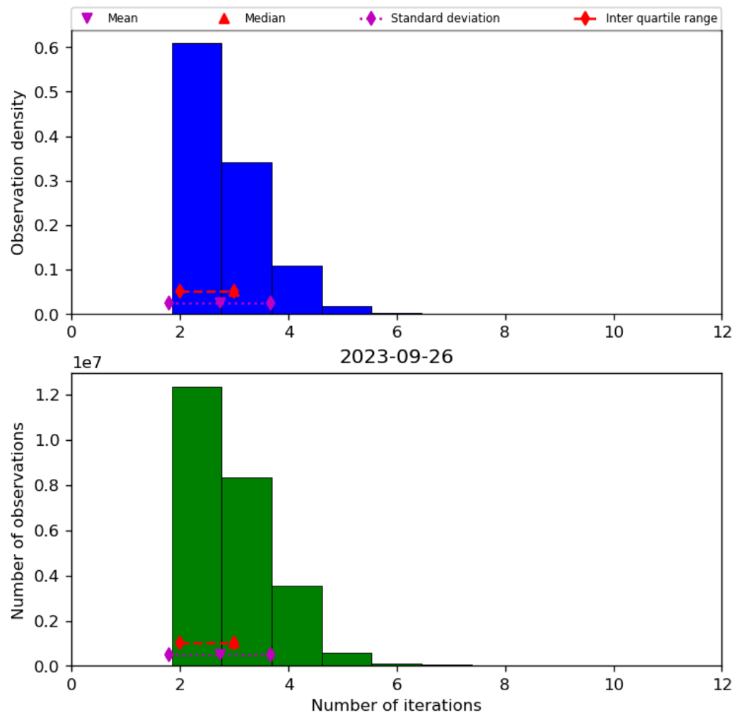
Figure 39: Histogram of “Number of iterations” for 2023-09-26 to 2023-09-27
