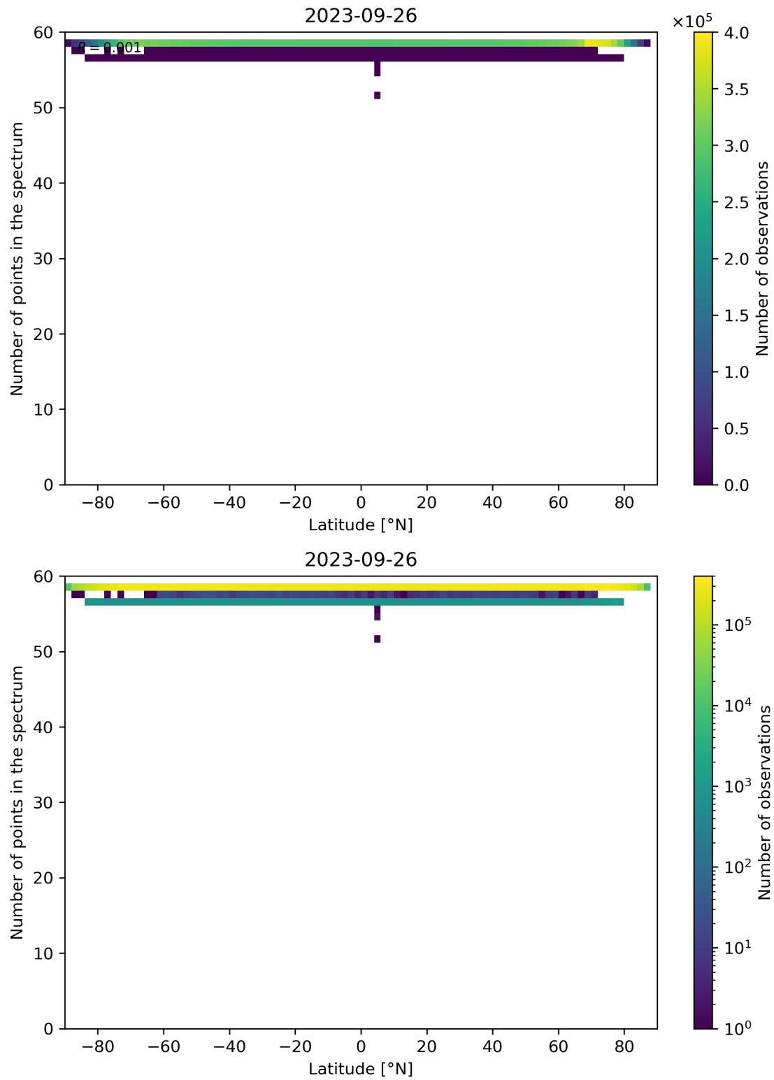
Figure 103: Scatter density plot of “Latitude” against “Number of points in the spectrum” for 2023-09-26 to 2023-09-27.
