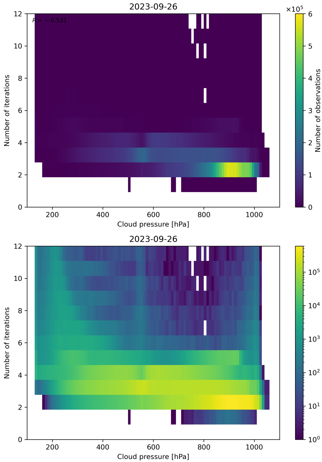
Figure 89: Scatter density plot of “Cloud pressure” against “Number of iterations” for 2023-09-26 to 2023-09-27.
