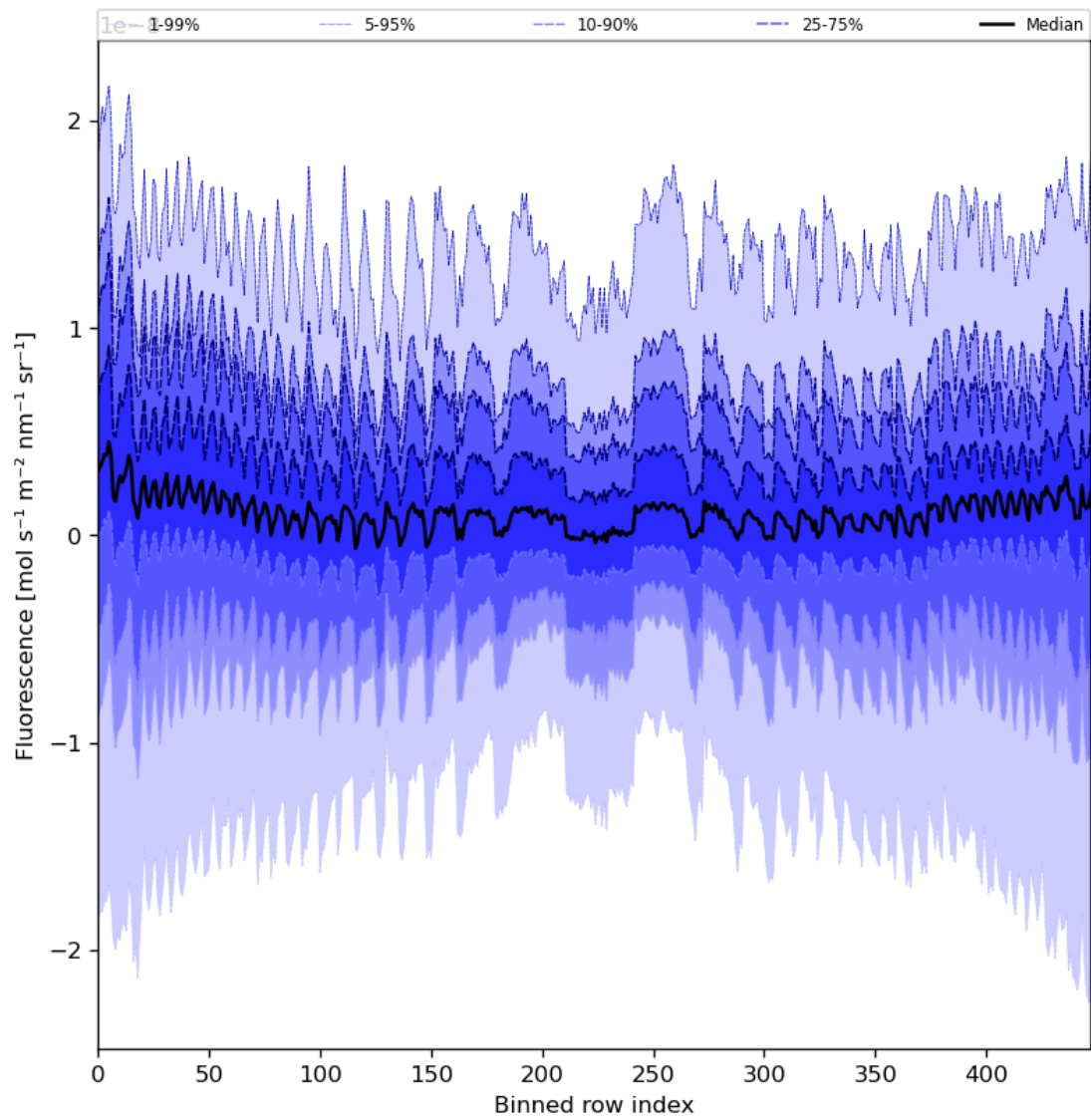
Figure 57: Along track statistics of “Fluorescence” for 2023-09-26 to 2023-09-27
