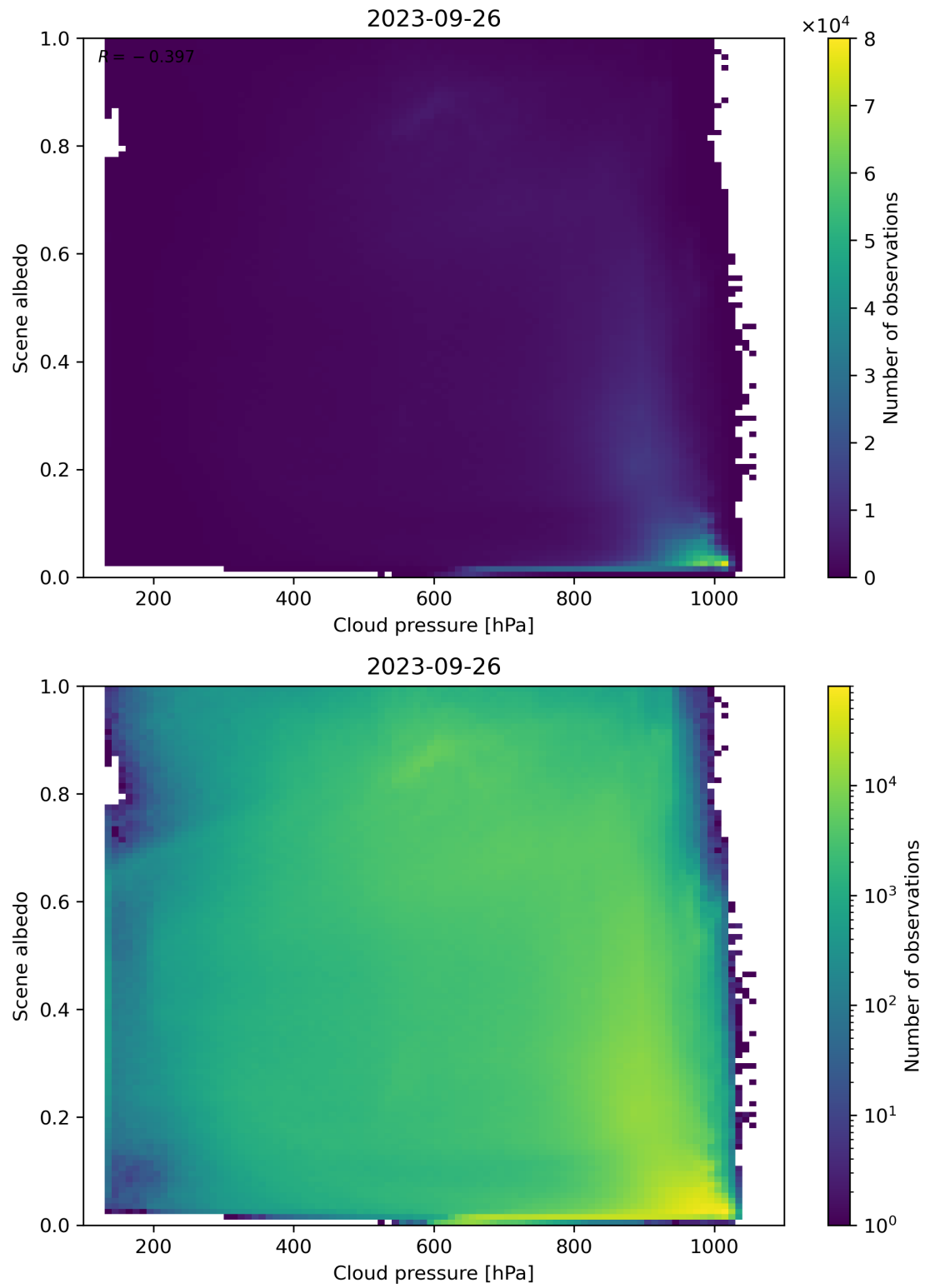
Figure 91: Scatter density plot of “Cloud pressure” against “Scene albedo” for 2023-09-26 to 2023-09-27.
