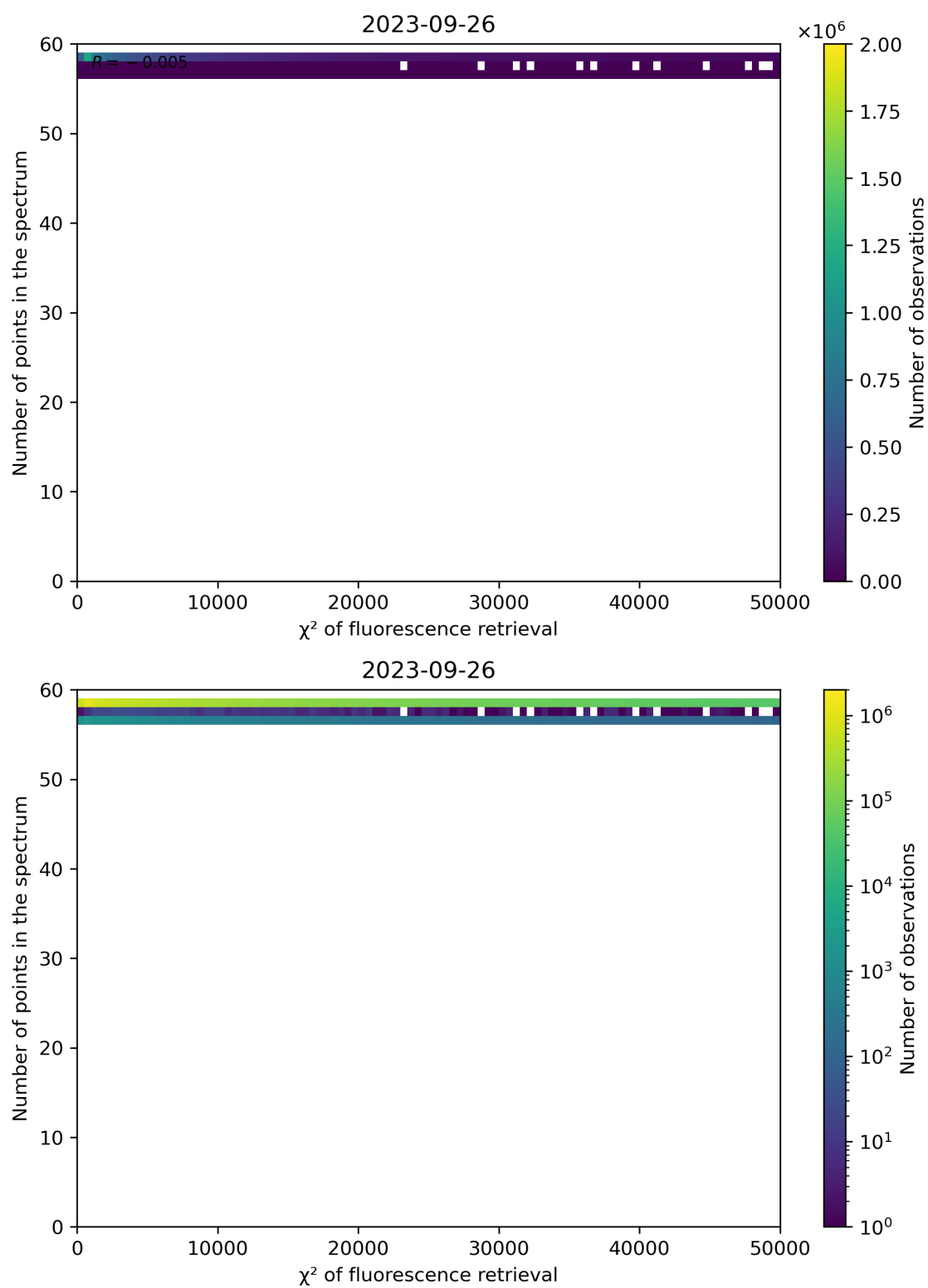
Figure 71: Scatter density plot of “ \chi^2 of fluorescence retrieval” against “Number of points in the spectrum” for 2023-09-26 to 2023-09-27.
