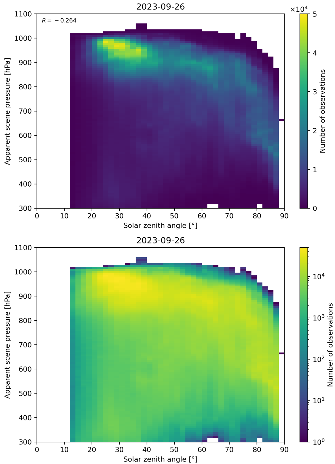
Figure 118: Scatter density plot of “Solar zenith angle” against “Apparent scene pressure” for 2023-09-26 to 2023-09-27.
