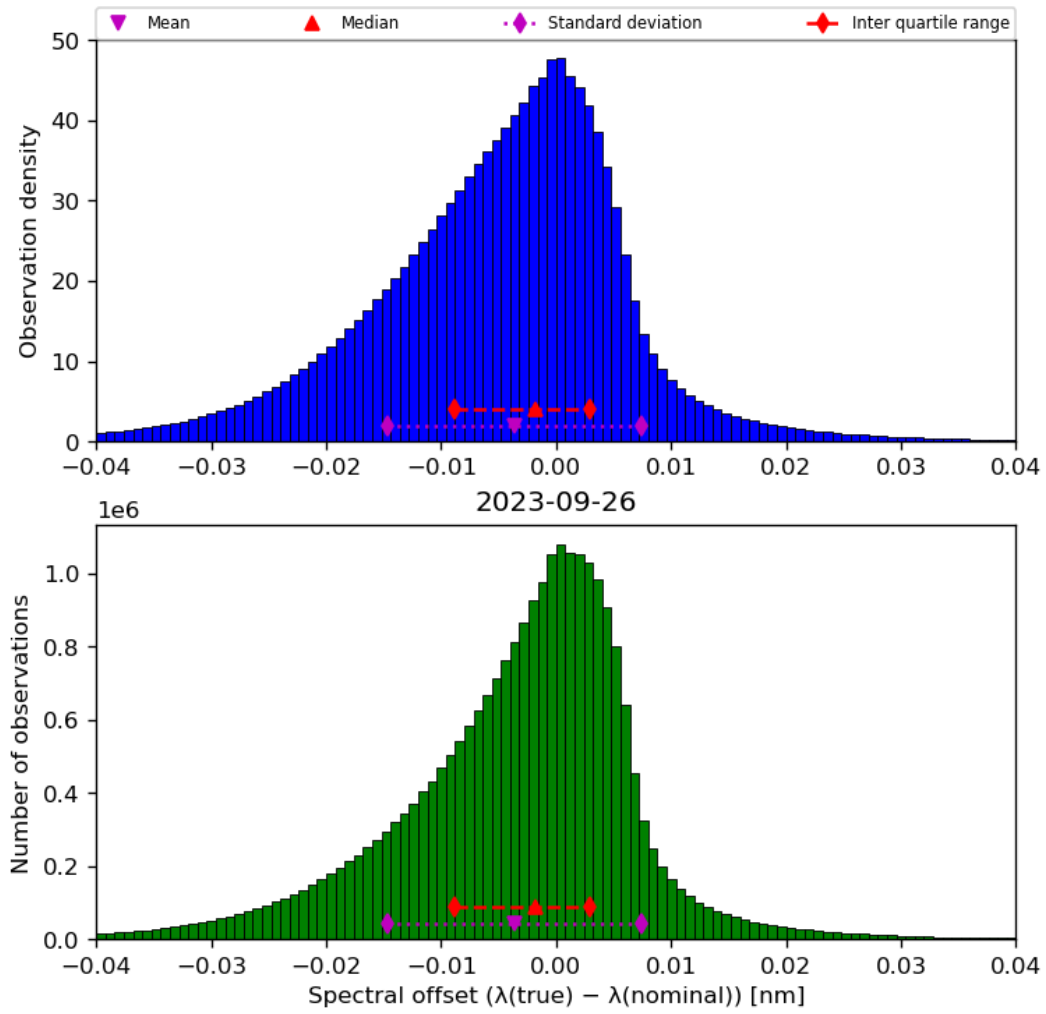
Figure 45: Histogram of “Spectral offset ( \lambda(\text{true}) - \lambda(\text{nominal}) )” for 2023-09-26 to 2023-09-27
