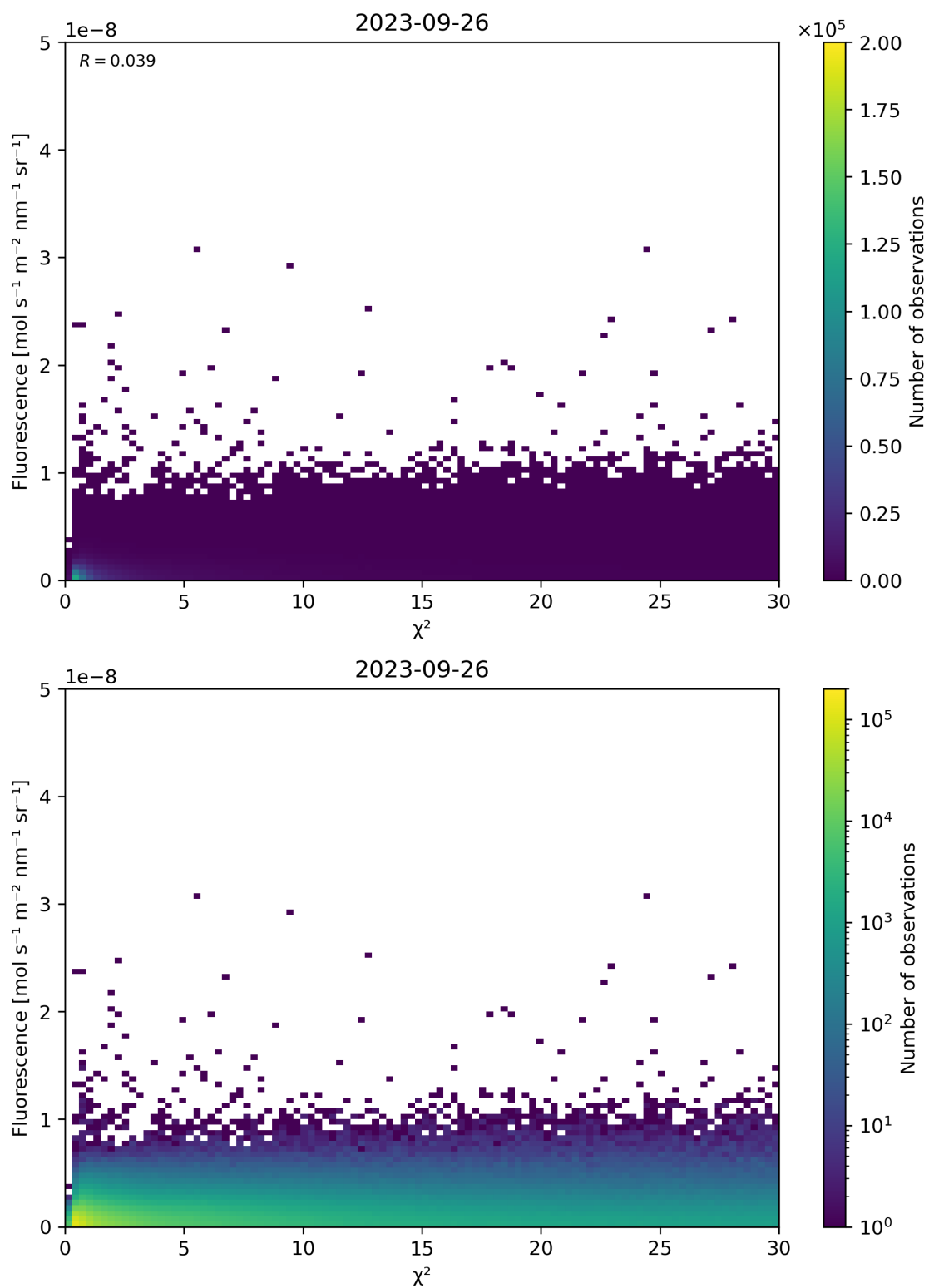
Figure 70: Scatter density plot of “ \chi^2 ” against “Fluorescence” for 2023-09-26 to 2023-09-27.
