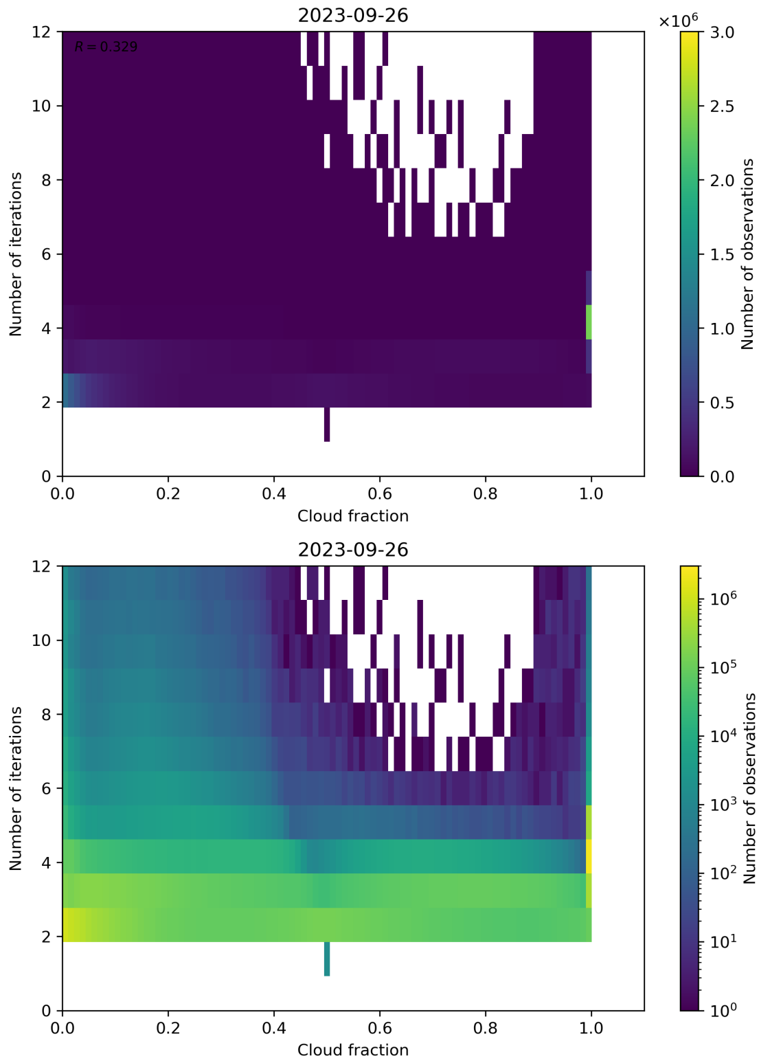
Figure 80: Scatter density plot of “Cloud fraction” against “Number of iterations” for 2023-09-26 to 2023-09-27.
