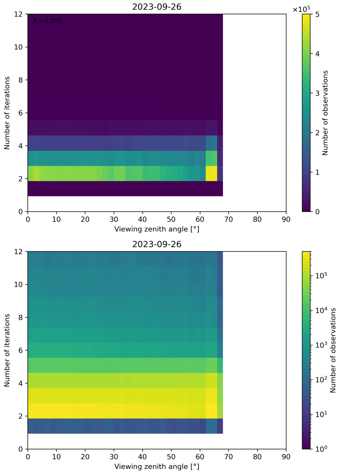
Figure 136: Scatter density plot of “Viewing zenith angle” against “Number of iterations” for 2023-09-26 to 2023-09-27.
