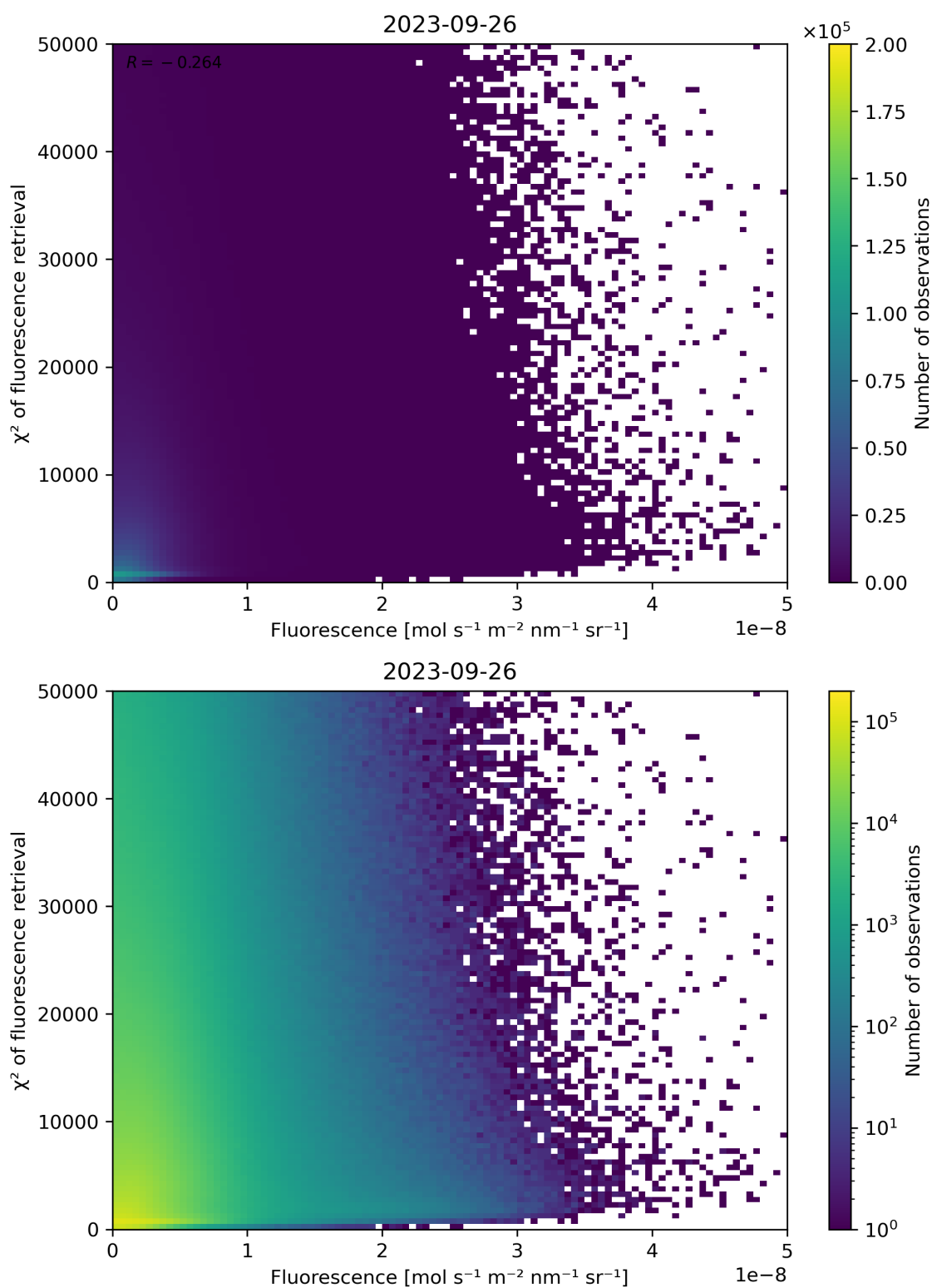
Figure 93: Scatter density plot of “Fluorescence” against “ \chi^2 of fluorescence retrieval” for 2023-09-26 to 2023-09-27.
