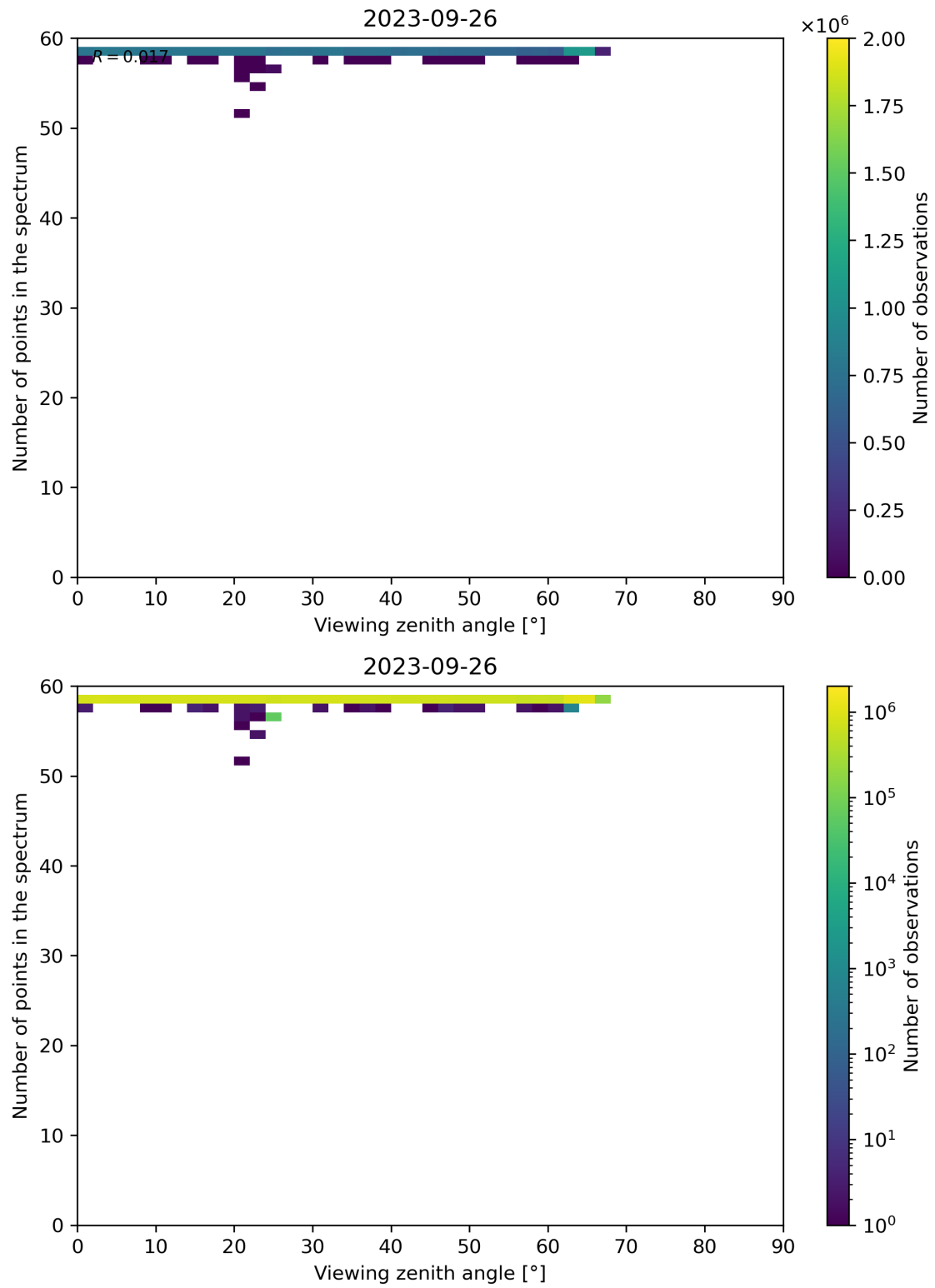
Figure 137: Scatter density plot of “Viewing zenith angle” against “Number of points in the spectrum” for 2023-09-26 to 2023-09-27.
