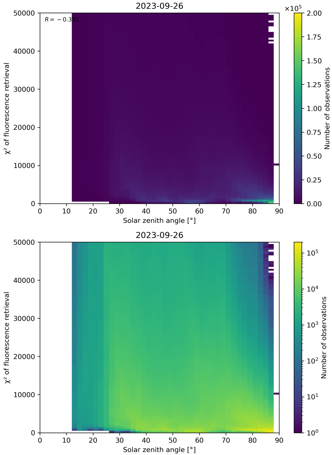
Figure 120: Scatter density plot of “Solar zenith angle” against “ \chi^2 of fluorescence retrieval” for 2023-09-26 to 2023-09-27.
