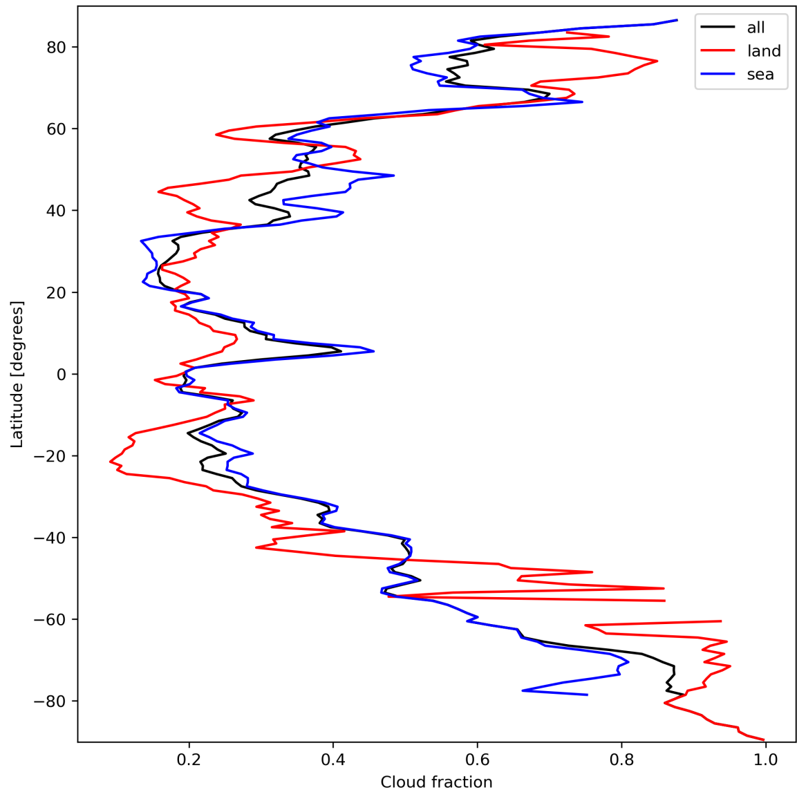
Figure 15: Zonal average of “Cloud fraction” for 2023-09-26 to 2023-09-27.
