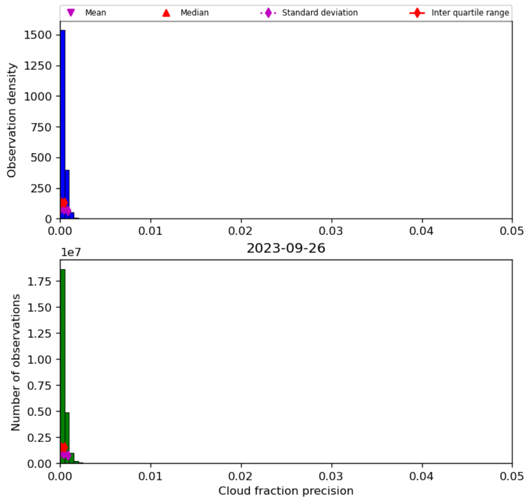
Figure 33: Histogram of “Cloud fraction precision” for 2023-09-26 to 2023-09-27
