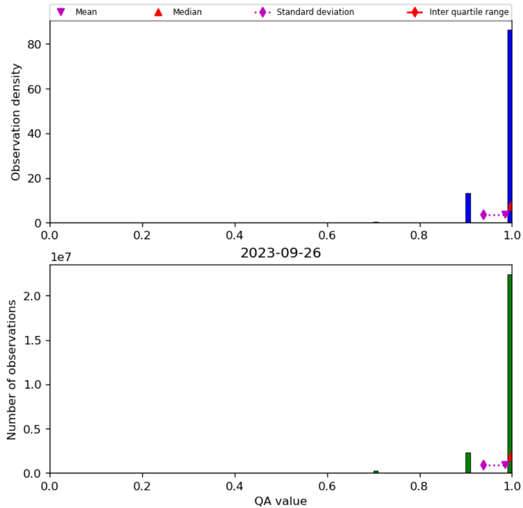
Figure 29: Histogram of “QA value” for 2023-09-26 to 2023-09-27
