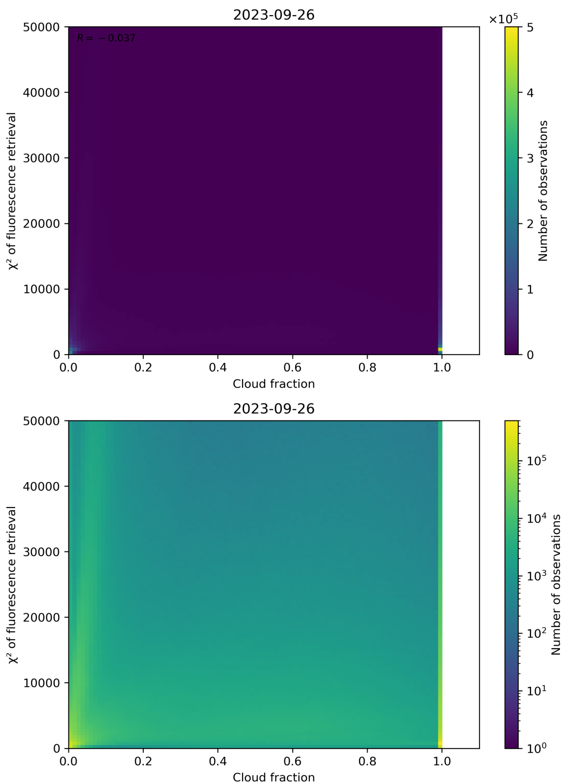
Figure 78: Scatter density plot of “Cloud fraction” against “ \chi^2 of fluorescence retrieval” for 2023-09-26 to 2023-09-27.
