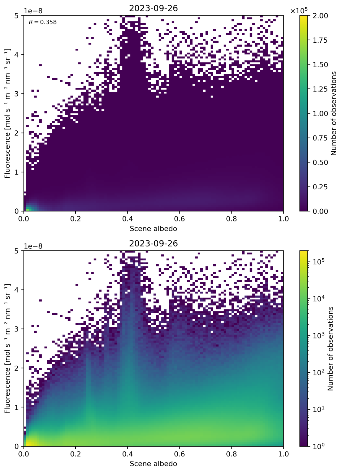
Figure 114: Scatter density plot of “Scene albedo” against “Fluorescence” for 2023-09-26 to 2023-09-27.
