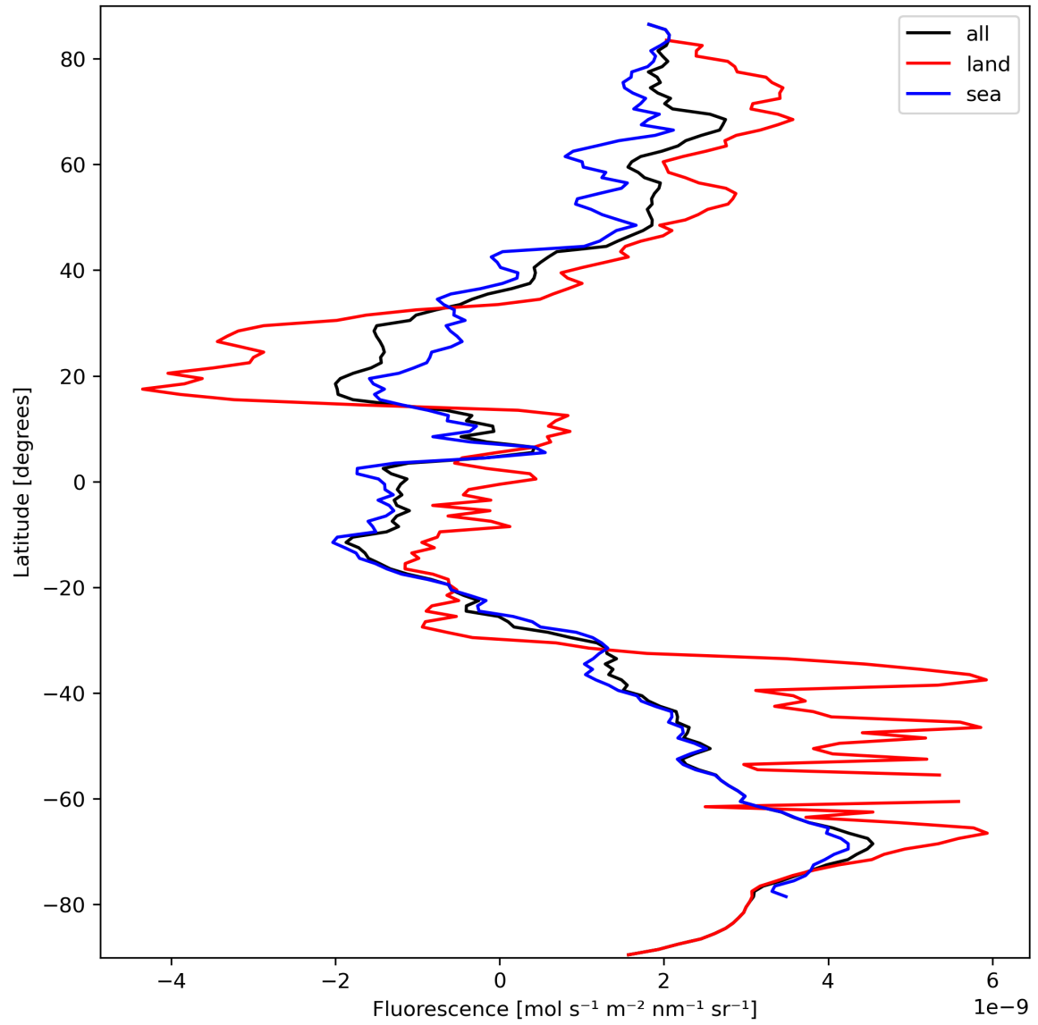
Figure 23: Zonal average of “Fluorescence” for 2023-09-26 to 2023-09-27.
