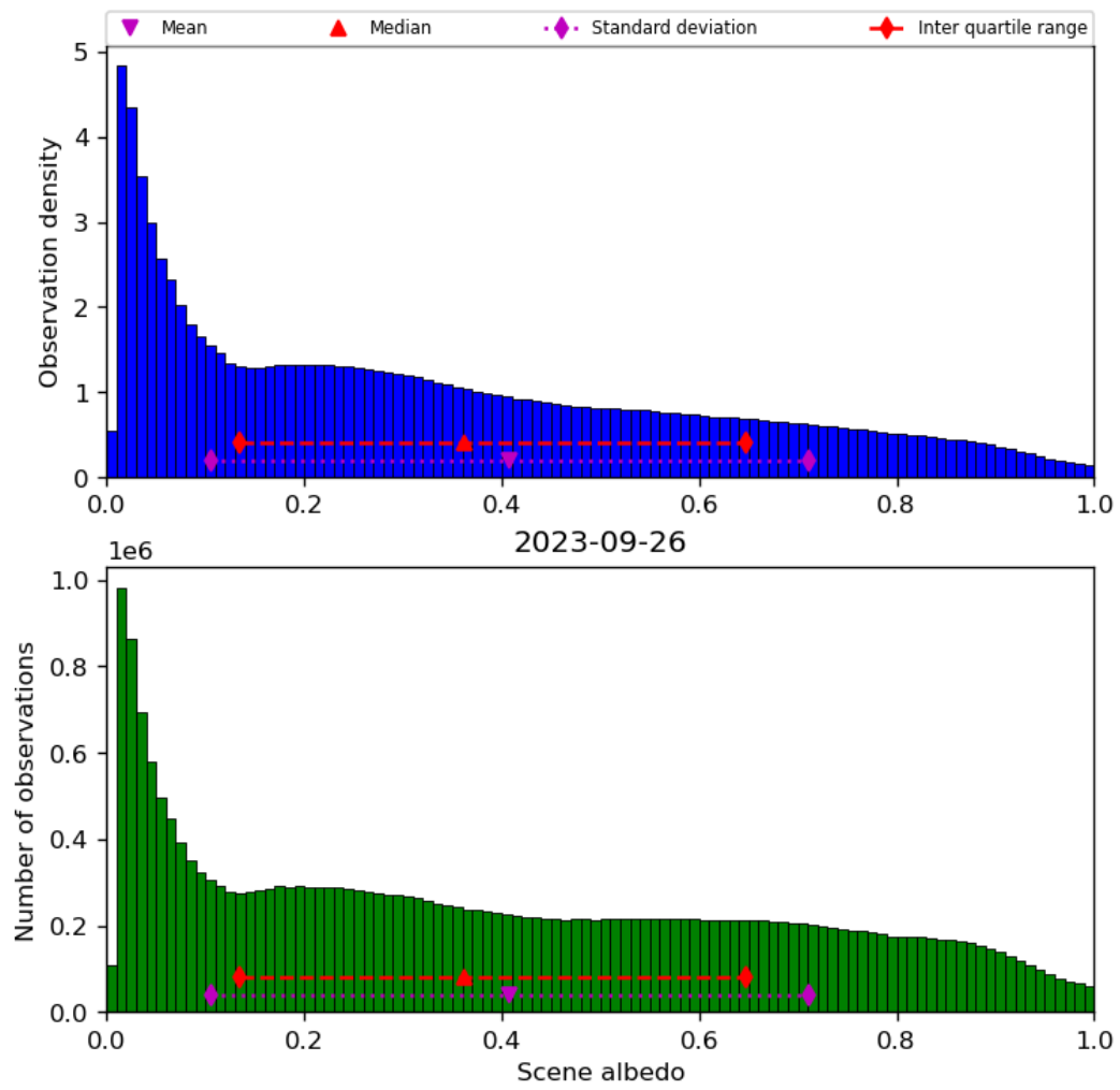
Figure 34: Histogram of “Scene albedo” for 2023-09-26 to 2023-09-27
