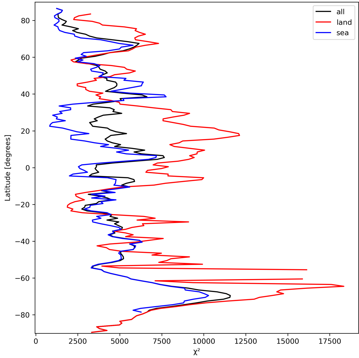
Figure 21: Zonal average of “ \chi^2 ” for 2023-09-26 to 2023-09-27.
