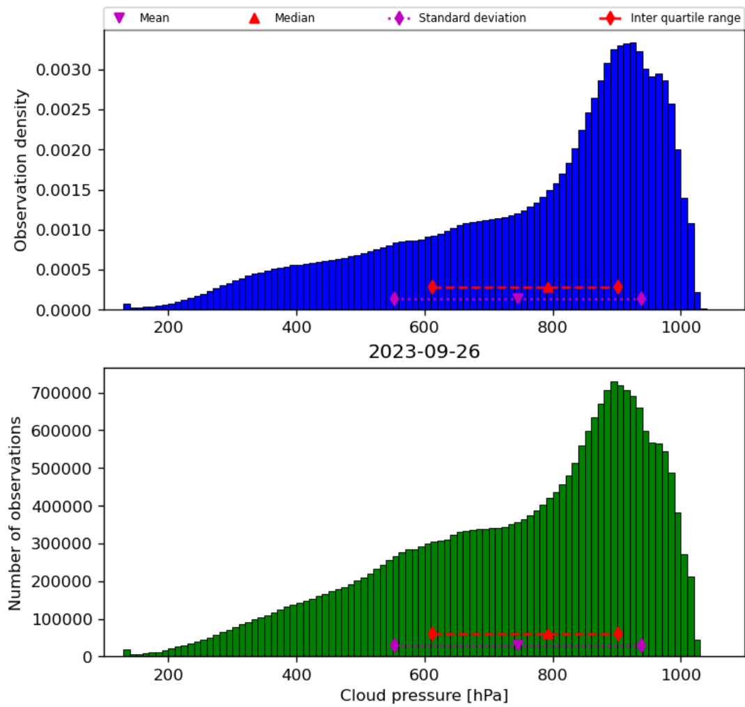
Figure 30: Histogram of “Cloud pressure” for 2023-09-26 to 2023-09-27
