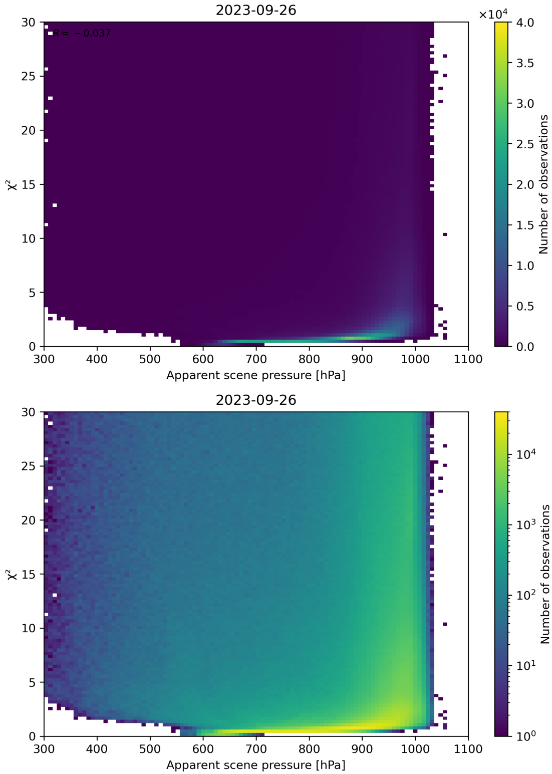
Figure 63: Scatter density plot of “Apparent scene pressure” against “ \chi^2 ” for 2023-09-26 to 2023-09-27.
