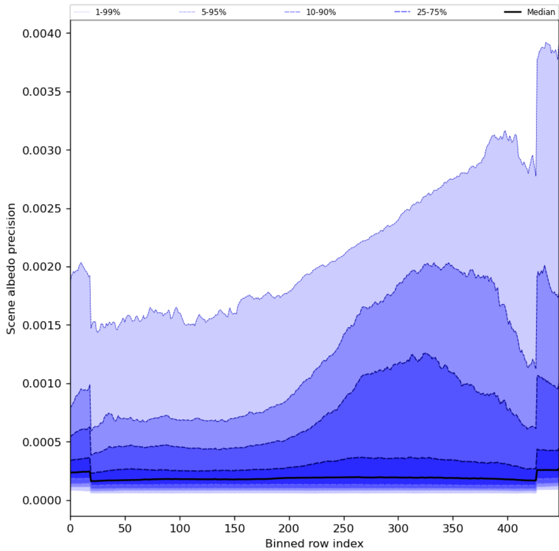
Figure 52: Along track statistics of “Scene albedo precision” for 2023-09-26 to 2023-09-27
