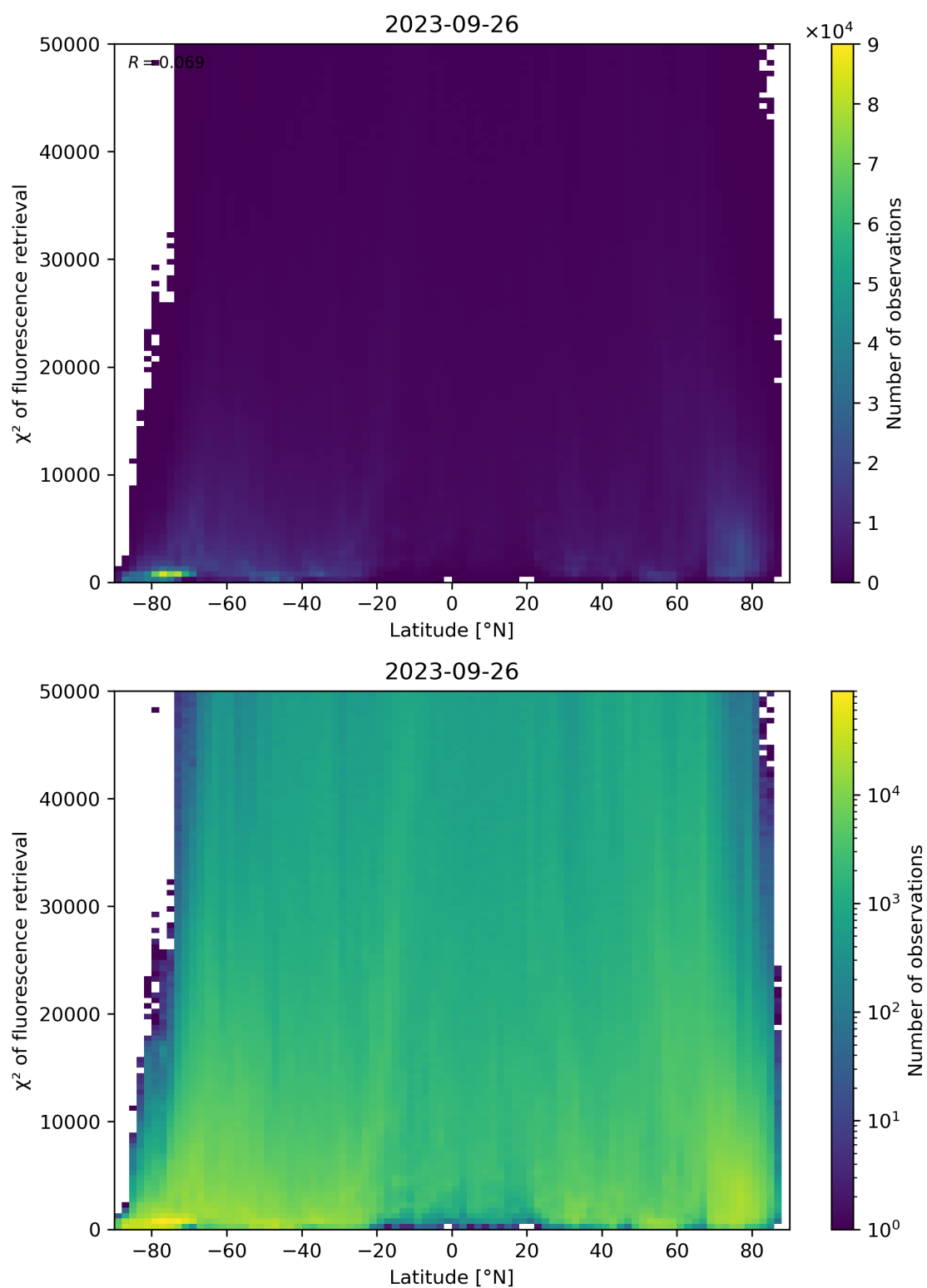
Figure 98: Scatter density plot of “Latitude” against “ \chi^2 of fluorescence retrieval” for 2023-09-26 to 2023-09-27.
