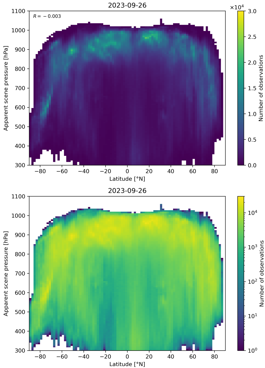
Figure 96: Scatter density plot of “Latitude” against “Apparent scene pressure” for 2023-09-26 to 2023-09-27.
