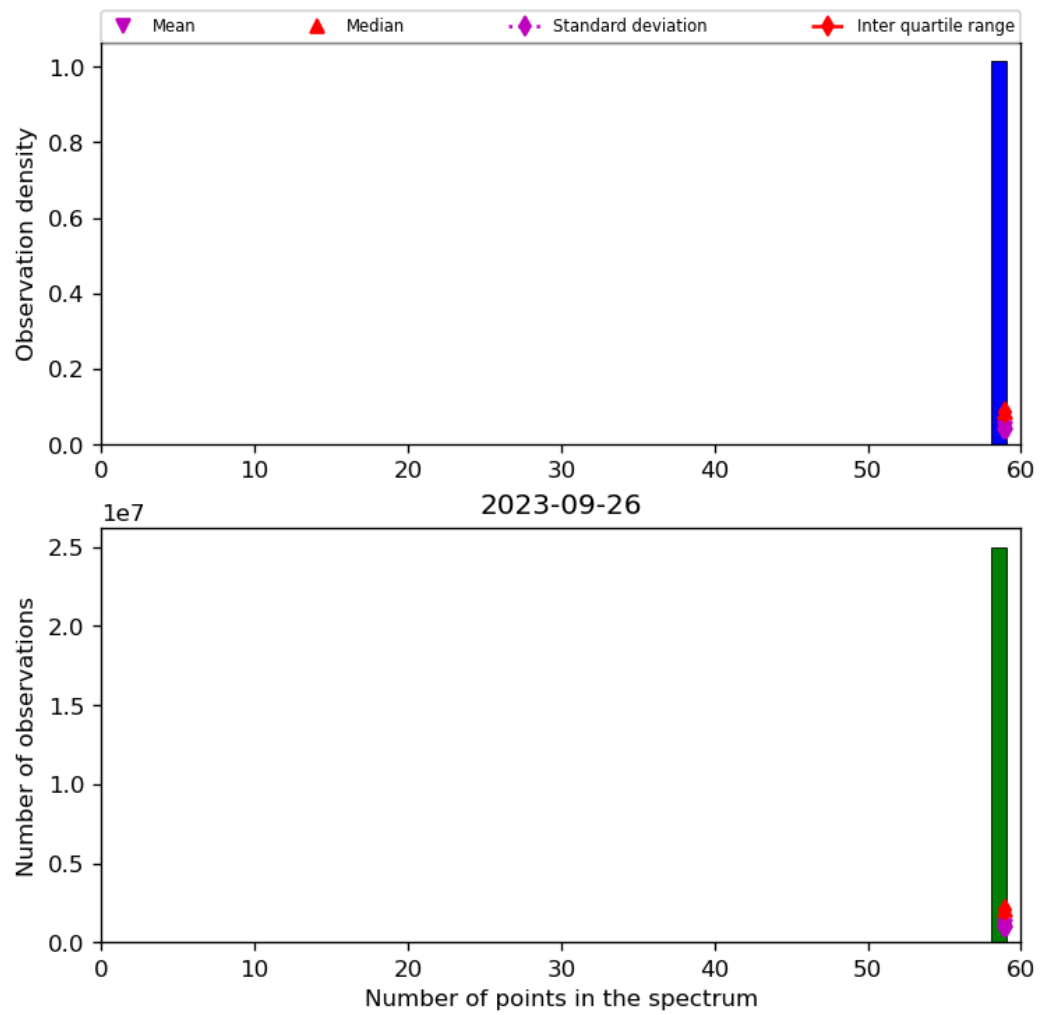
Figure 44: Histogram of “Number of points in the spectrum” for 2023-09-26 to 2023-09-27
