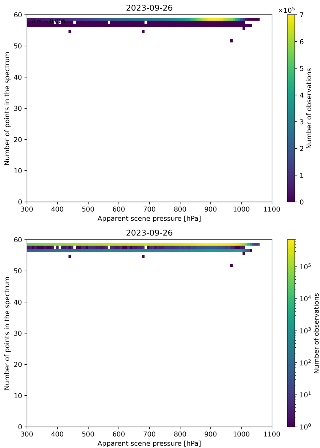
Figure 67: Scatter density plot of “Apparent scene pressure” against “Number of points in the spectrum” for 2023-09-26 to 2023-09-27.
