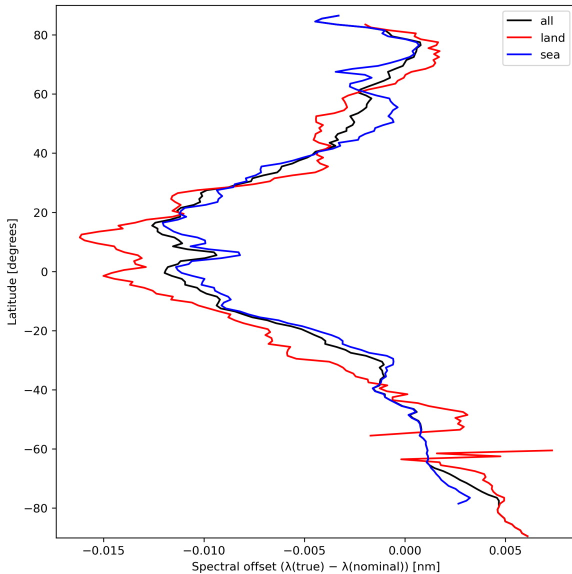
Figure 28: Zonal average of “Spectral offset ( \lambda(\text{true}) - \lambda(\text{nominal}) )” for 2023-09-26 to 2023-09-27.
