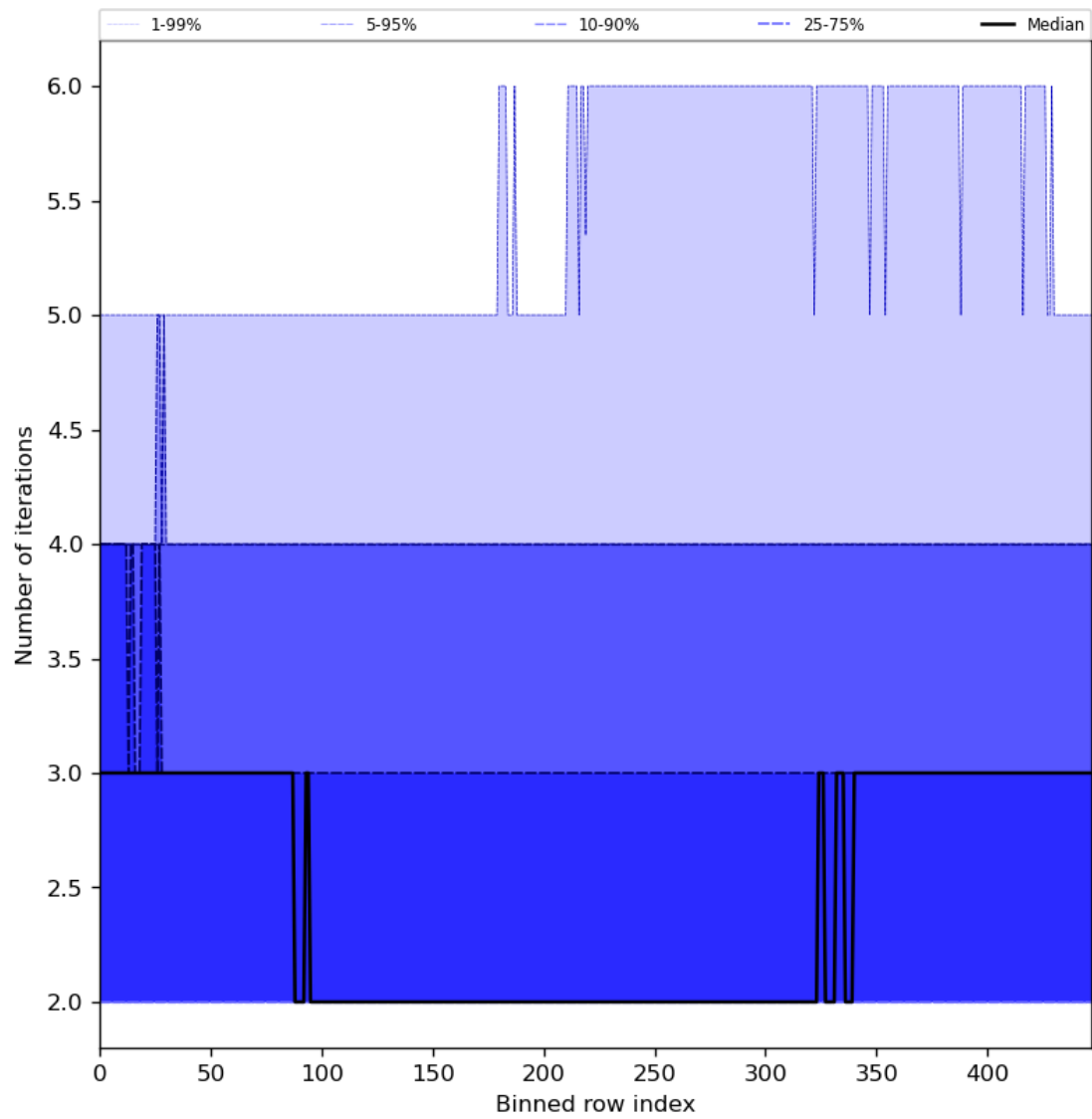
Figure 56: Along track statistics of “Number of iterations” for 2023-09-26 to 2023-09-27
