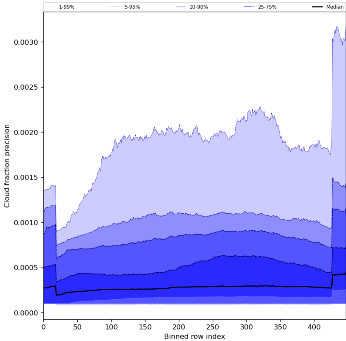
Figure 50: Along track statistics of “Cloud fraction precision” for 2023-09-26 to 2023-09-27
