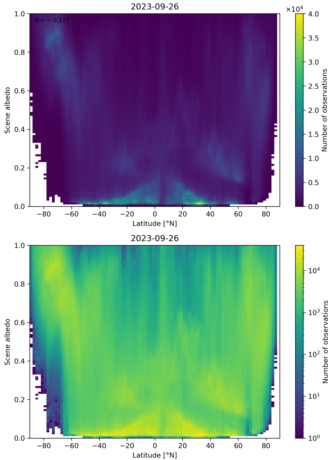
Figure 104: Scatter density plot of “Latitude” against “Scene albedo” for 2023-09-26 to 2023-09-27.
