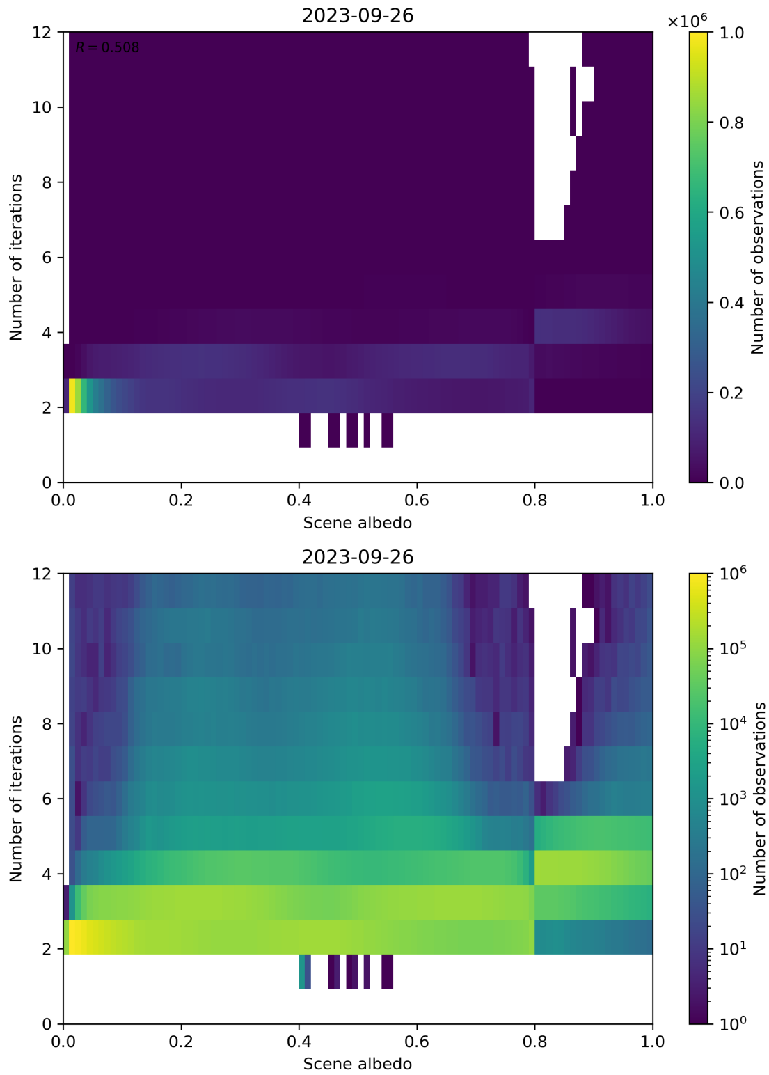
Figure 115: Scatter density plot of “Scene albedo” against “Number of iterations” for 2023-09-26 to 2023-09-27.
