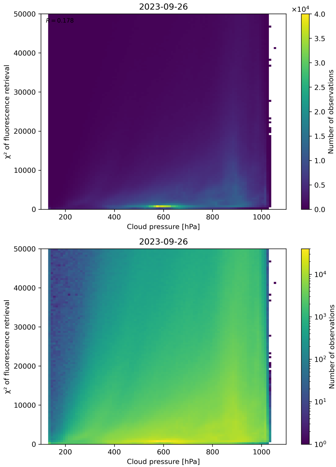
Figure 86: Scatter density plot of “Cloud pressure” against “ \chi^2 of fluorescence retrieval” for 2023-09-26 to 2023-09-27.
