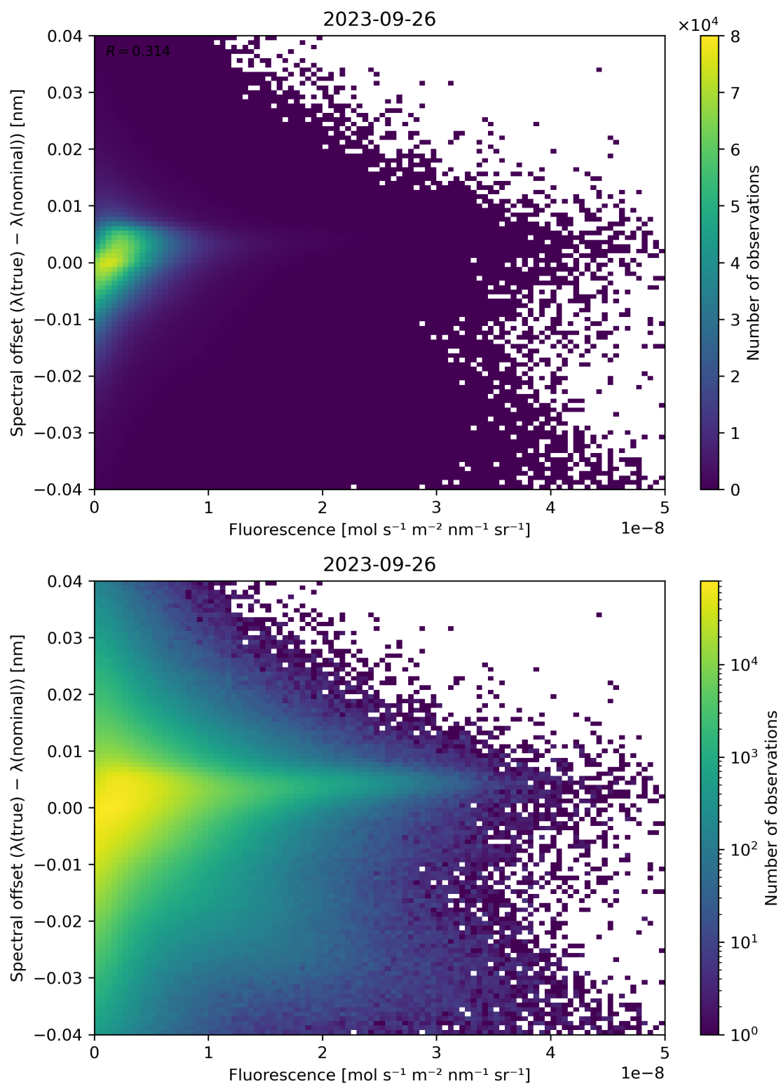
Figure 95: Scatter density plot of “Fluorescence” against “Spectral offset ( \lambda(\text{true}) - \lambda(\text{nominal}) )” for 2023-09-26 to 2023-09-27.
