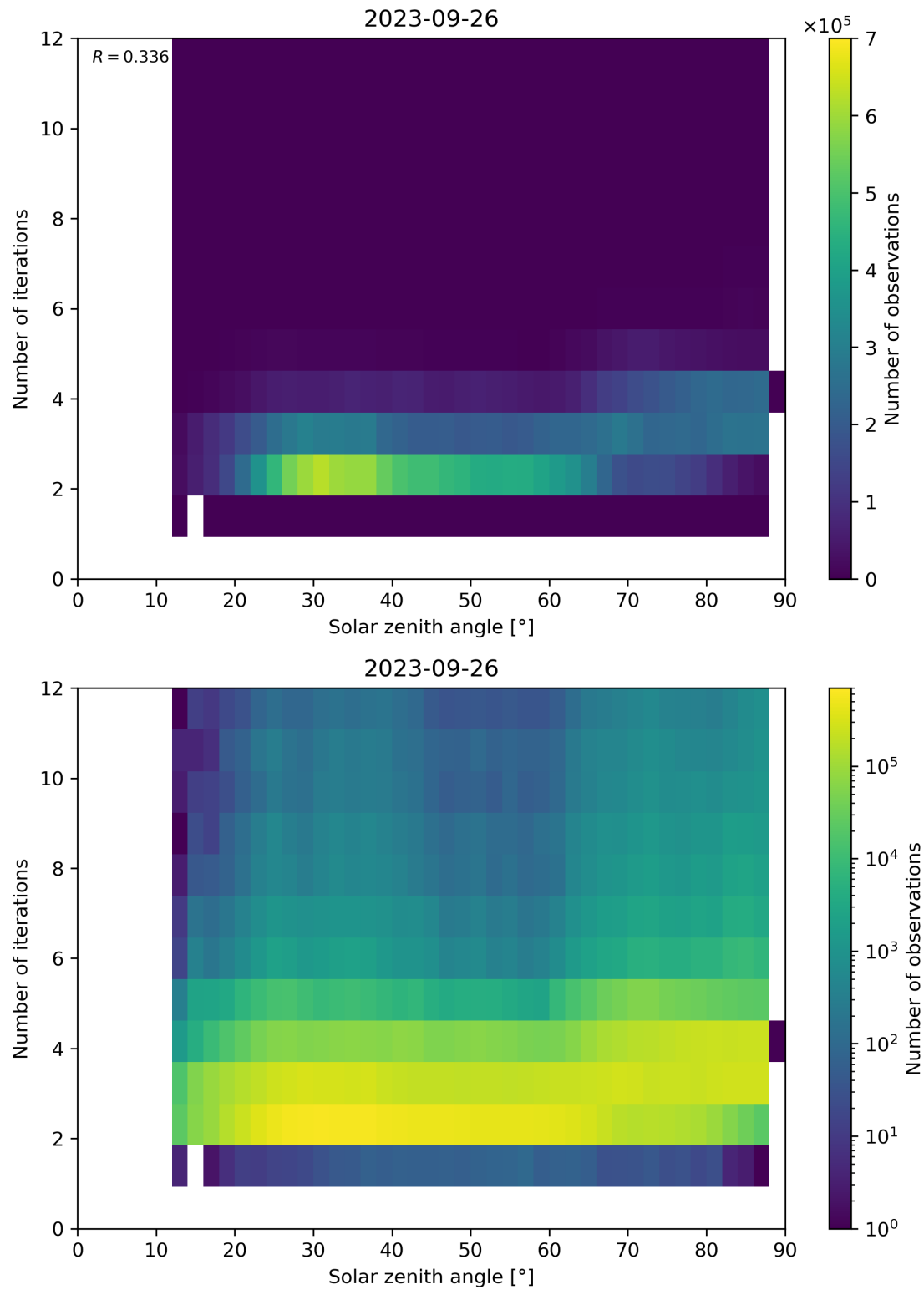
Figure 125: Scatter density plot of “Solar zenith angle” against “Number of iterations” for 2023-09-26 to 2023-09-27.
