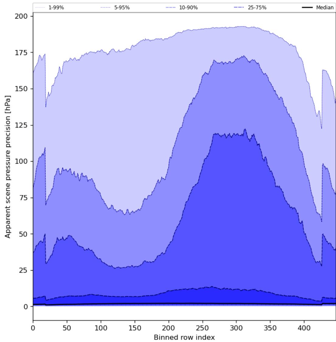
Figure 54: Along track statistics of “Apparent scene pressure precision” for 2023-09-26 to 2023-09-27
