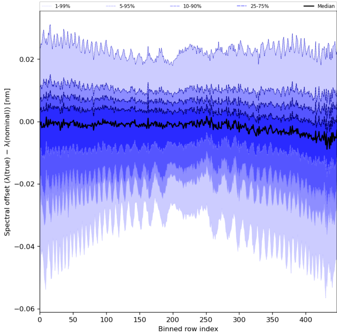
Figure 62: Along track statistics of “Spectral offset ( \lambda(\text{true}) - \lambda(\text{nominal}) )” for 2023-09-26 to 2023-09-27
