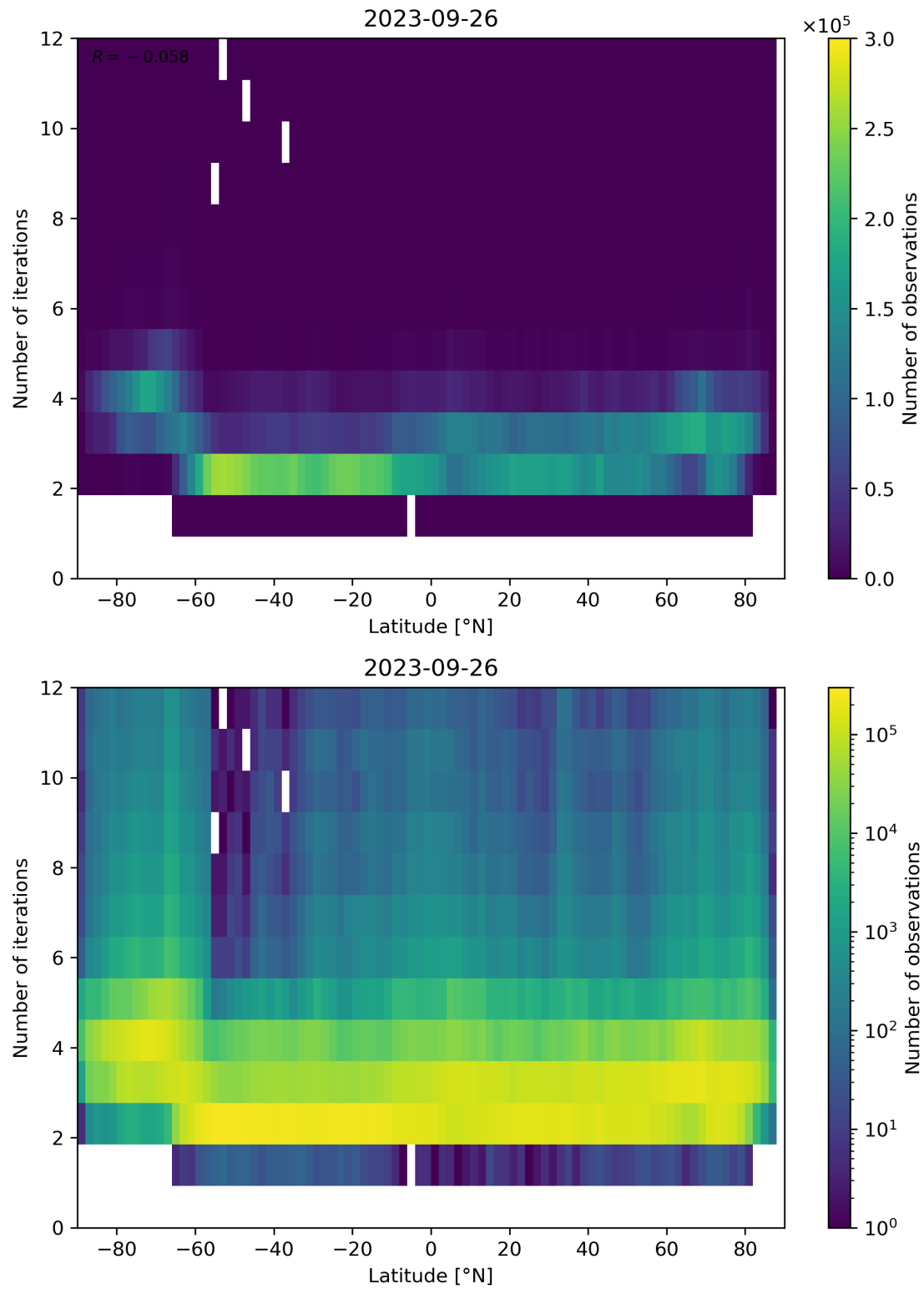
Figure 102: Scatter density plot of “Latitude” against “Number of iterations” for 2023-09-26 to 2023-09-27.
