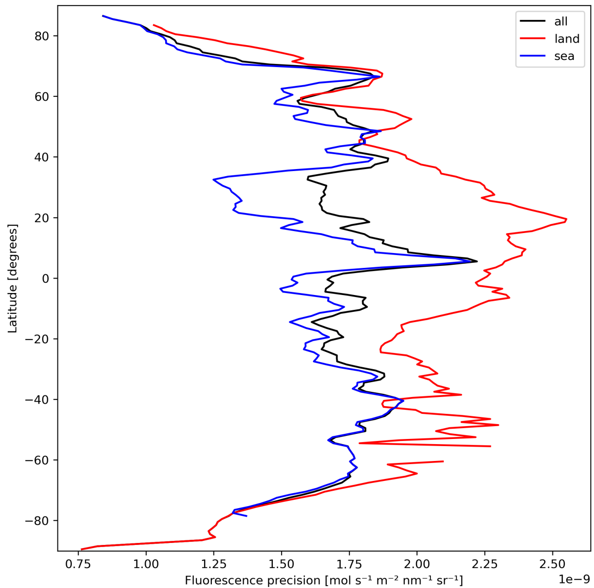
Figure 24: Zonal average of “Fluorescence precision” for 2023-09-26 to 2023-09-27.
