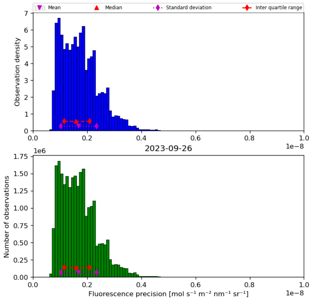
Figure 41: Histogram of “Fluorescence precision” for 2023-09-26 to 2023-09-27
