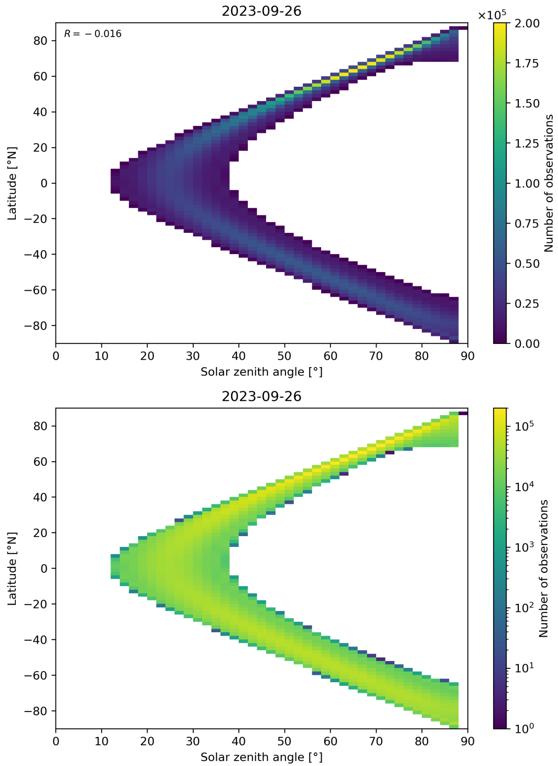
Figure 124: Scatter density plot of “Solar zenith angle” against “Latitude” for 2023-09-26 to 2023-09-27.
