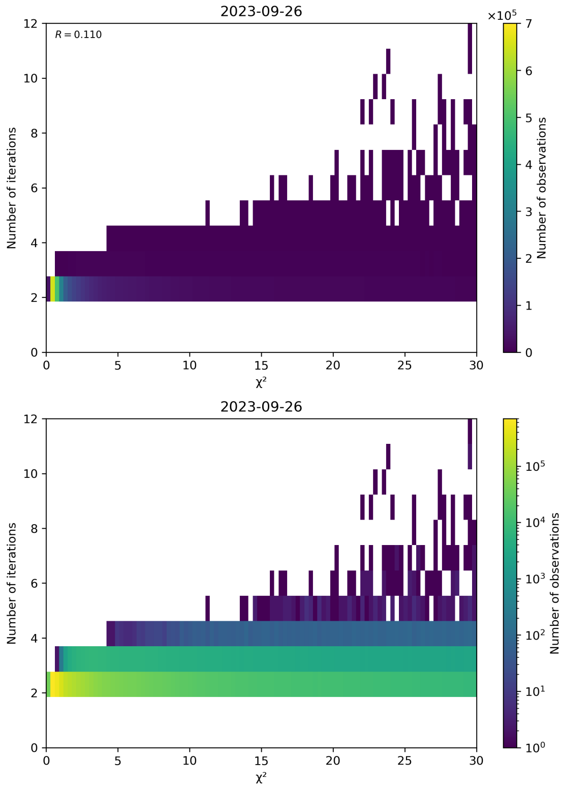
Figure 73: Scatter density plot of “ \chi^2 ” against “Number of iterations” for 2023-09-26 to 2023-09-27.
