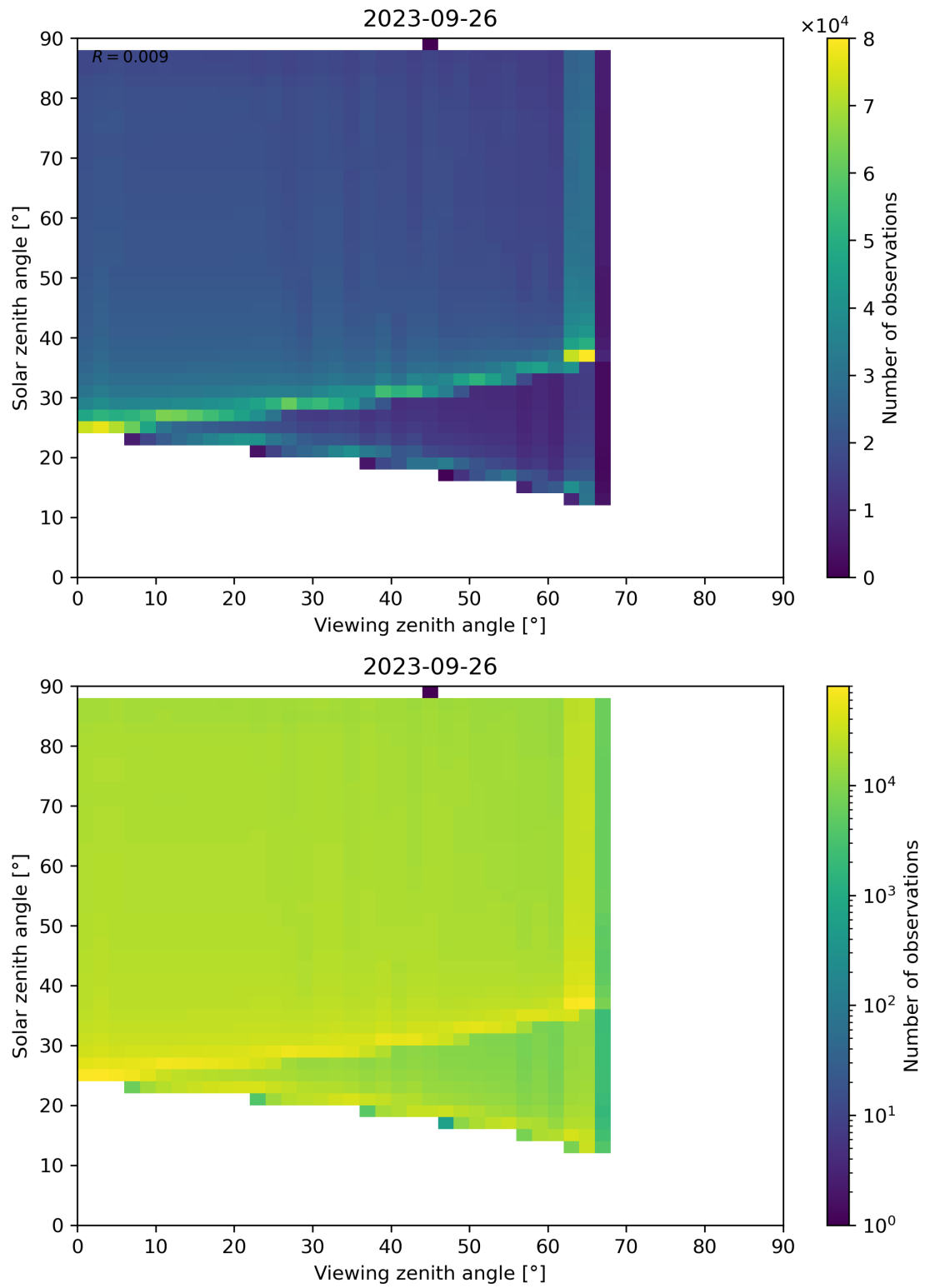
Figure 139: Scatter density plot of “Viewing zenith angle” against “Solar zenith angle” for 2023-09-26 to 2023-09-27.
