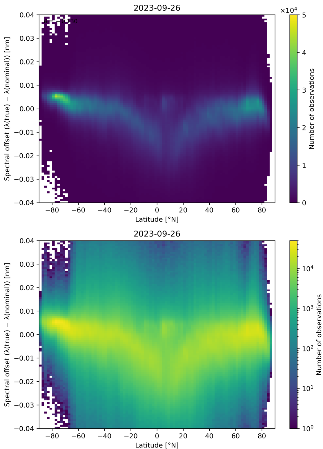
Figure 105: Scatter density plot of “Latitude” against “Spectral offset ( \lambda(\text{true}) - \lambda(\text{nominal}) )” for 2023-09-26 to 2023-09-27.
