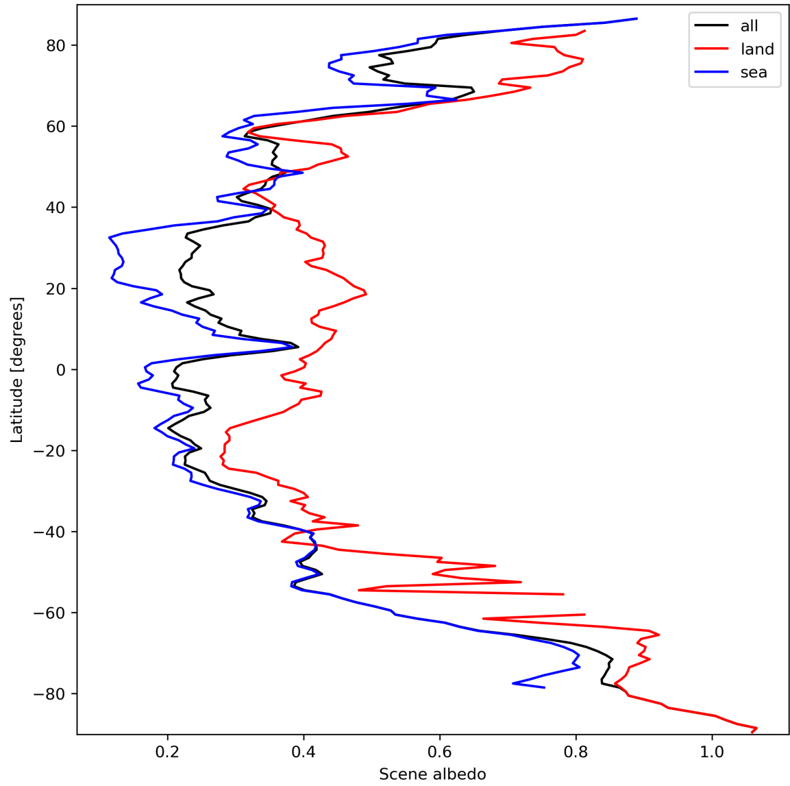
Figure 17: Zonal average of “Scene albedo” for 2023-09-26 to 2023-09-27.
