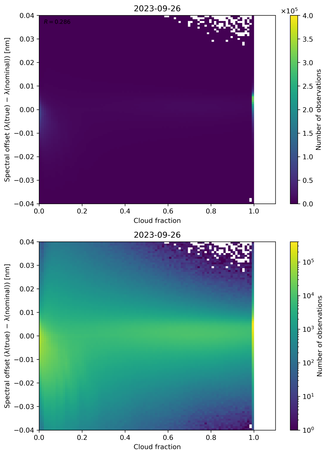
Figure 83: Scatter density plot of “Cloud fraction” against “Spectral offset ( \lambda(\text{true}) - \lambda(\text{nominal}) )” for 2023-09-26 to 2023-09-27.
