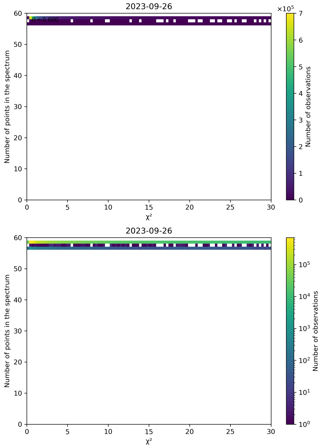
Figure 74: Scatter density plot of " \chi^2 " against "Number of points in the spectrum" for 2023-09-26 to 2023-09-27.
