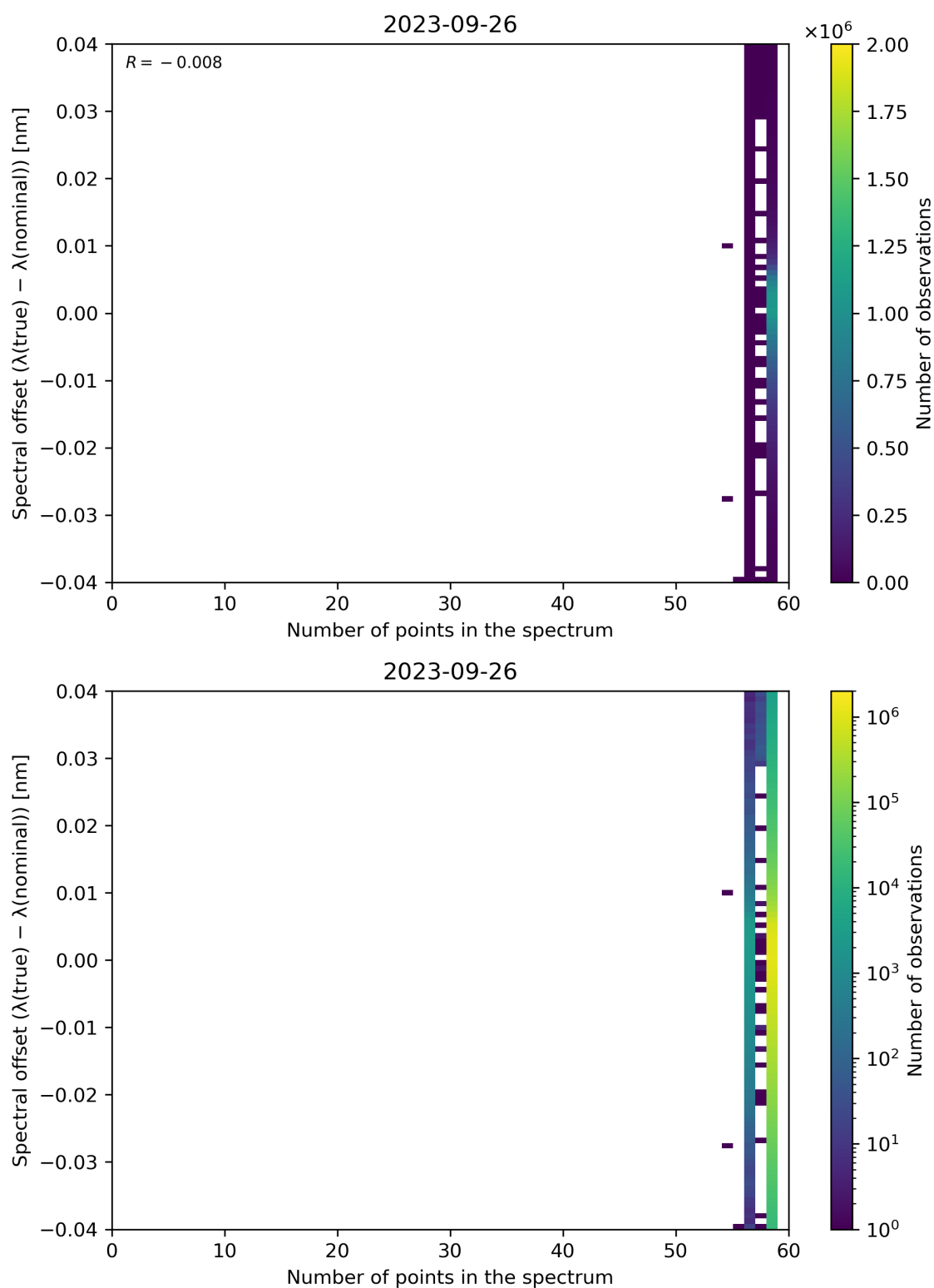
Figure 110: Scatter density plot of “Number of points in the spectrum” against “Spectral offset ( \lambda(\text{true}) - \lambda(\text{nominal}) )” for 2023-09-26 to 2023-09-27.
