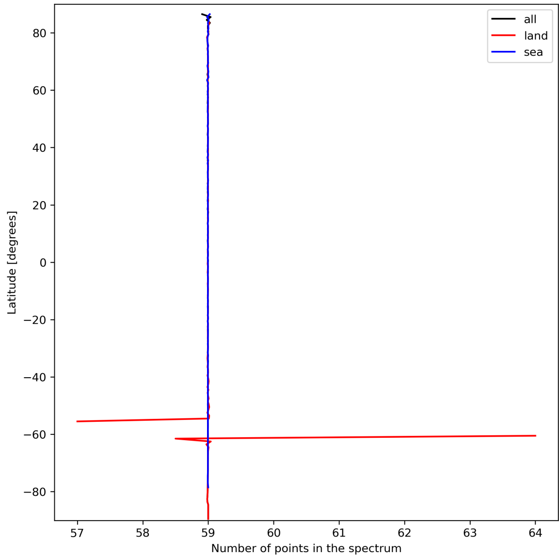
Figure 27: Zonal average of “Number of points in the spectrum” for 2023-09-26 to 2023-09-27.
