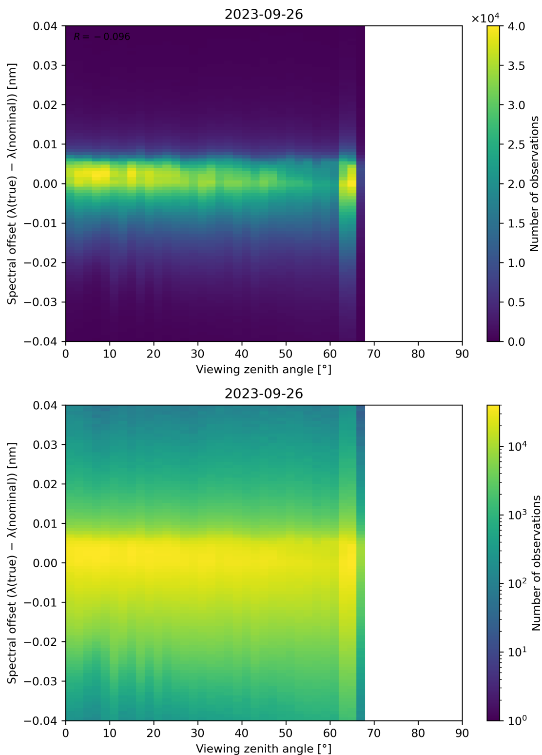
Figure 140: Scatter density plot of “Viewing zenith angle” against “Spectral offset ( \lambda(\text{true}) - \lambda(\text{nominal}) )” for 2023-09-26 to 2023-09-27.
