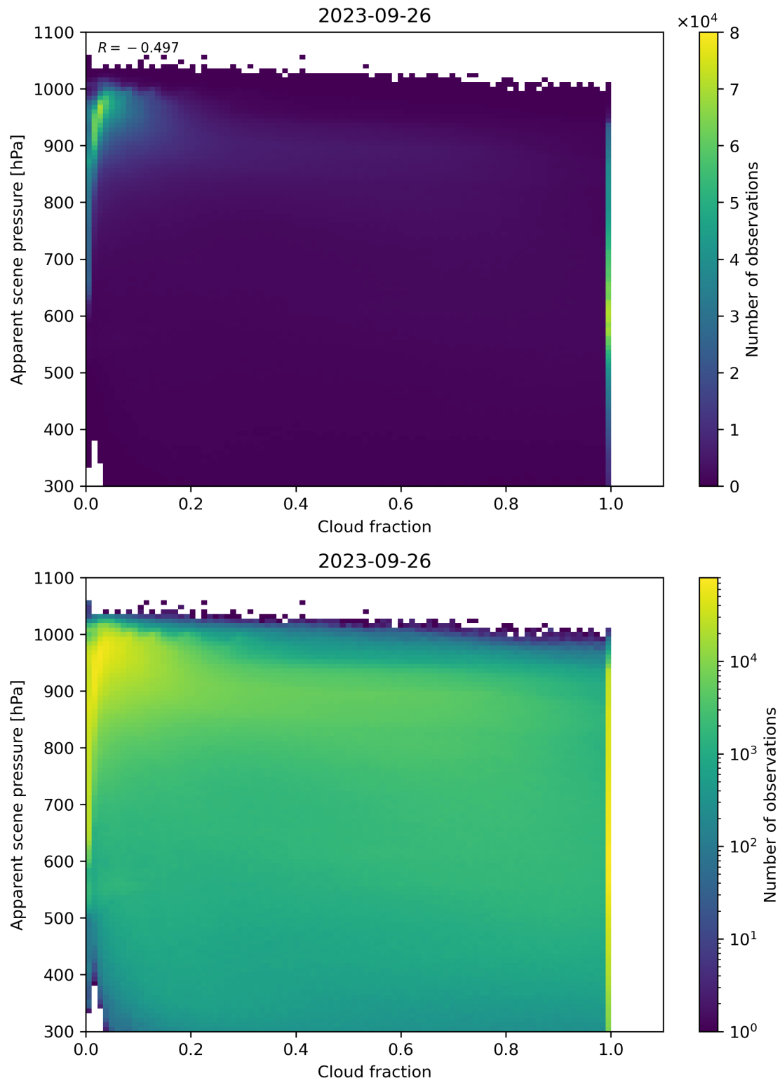
Figure 76: Scatter density plot of “Cloud fraction” against “Apparent scene pressure” for 2023-09-26 to 2023-09-27.
