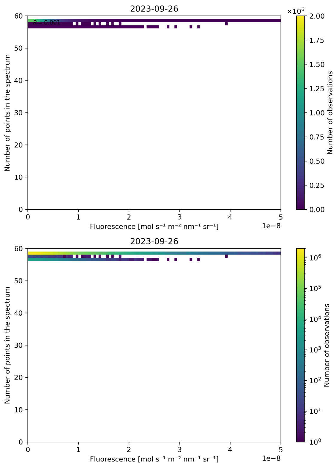
Figure 94: Scatter density plot of “Fluorescence” against “Number of points in the spectrum” for 2023-09-26 to 2023-09-27.
