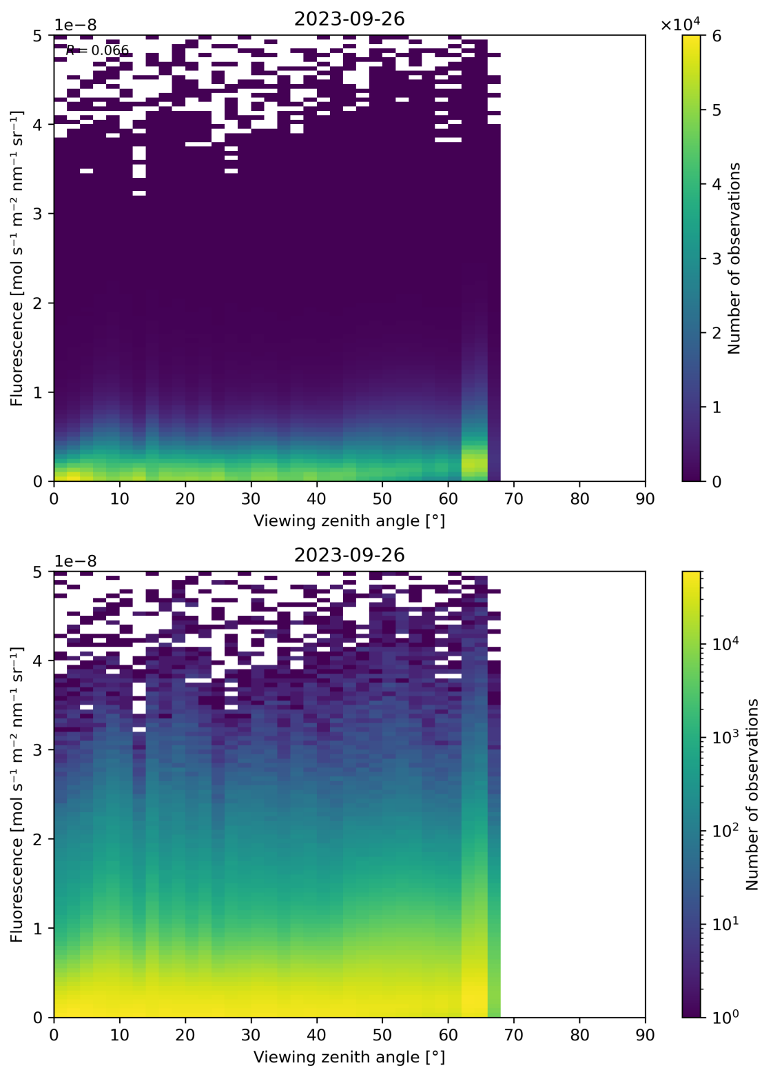
Figure 134: Scatter density plot of “Viewing zenith angle” against “Fluorescence” for 2023-09-26 to 2023-09-27.
