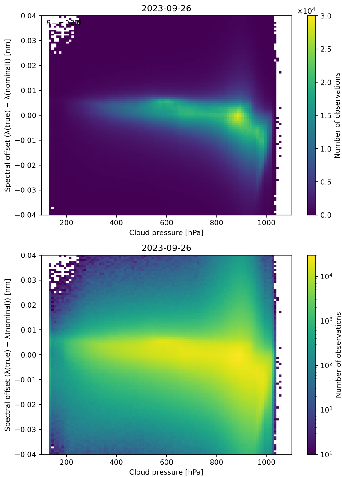
Figure 92: Scatter density plot of “Cloud pressure” against “Spectral offset ( \lambda(\text{true}) - \lambda(\text{nominal}) )” for 2023-09-26 to 2023-09-27.
