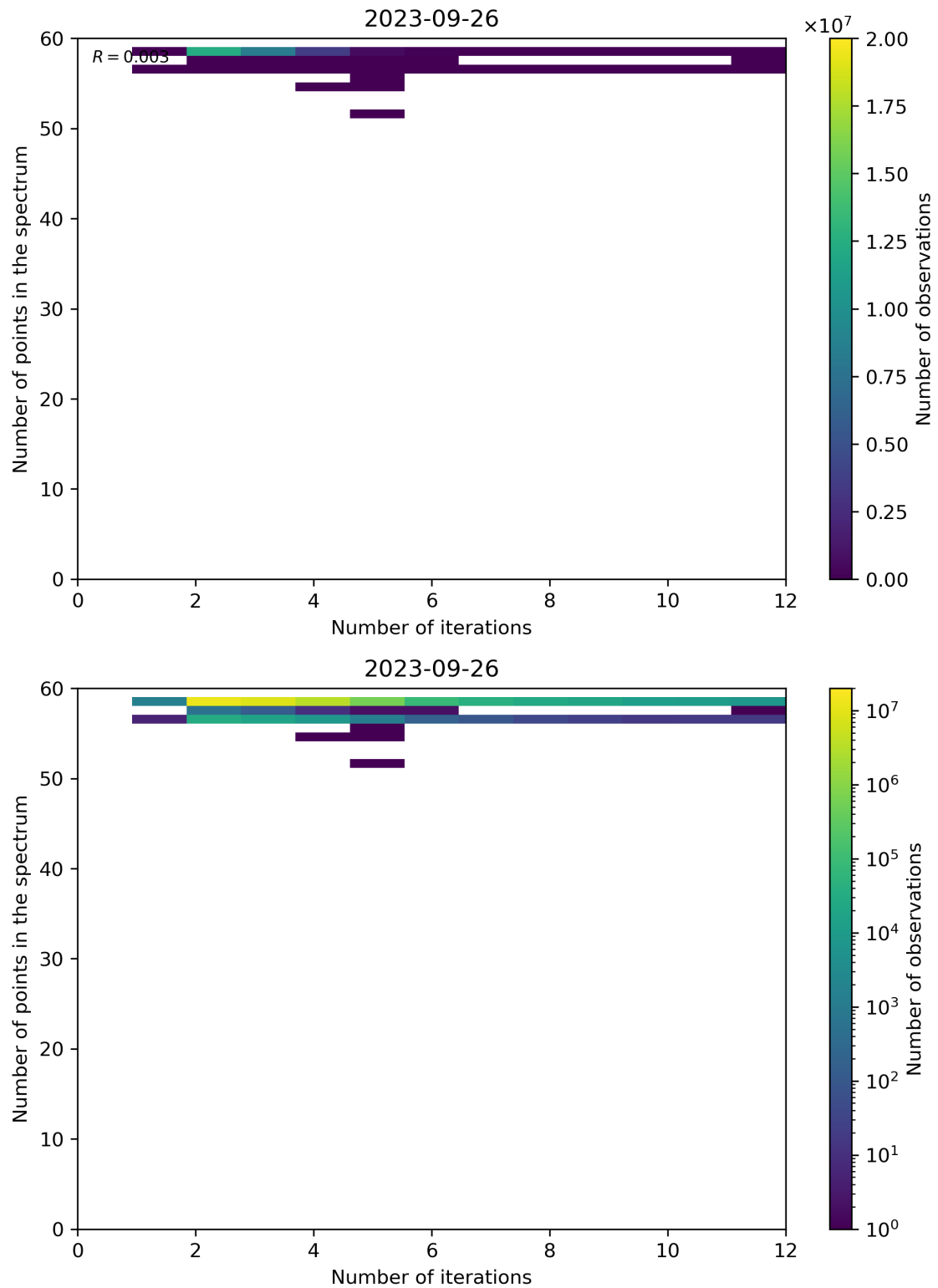
Figure 108: Scatter density plot of “Number of iterations” against “Number of points in the spectrum” for 2023-09-26 to 2023-09-27.
