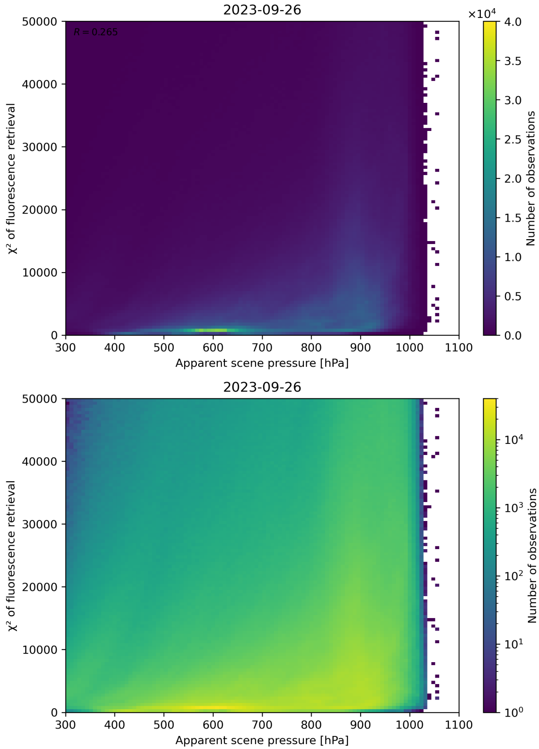
Figure 64: Scatter density plot of “Apparent scene pressure” against “ \chi^2 of fluorescence retrieval” for 2023-09-26 to 2023-09-27.
