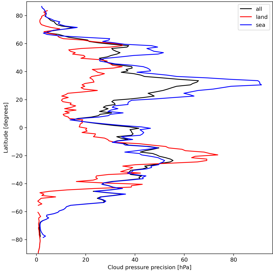
Figure 14: Zonal average of “Cloud pressure precision” for 2023-09-26 to 2023-09-27.
