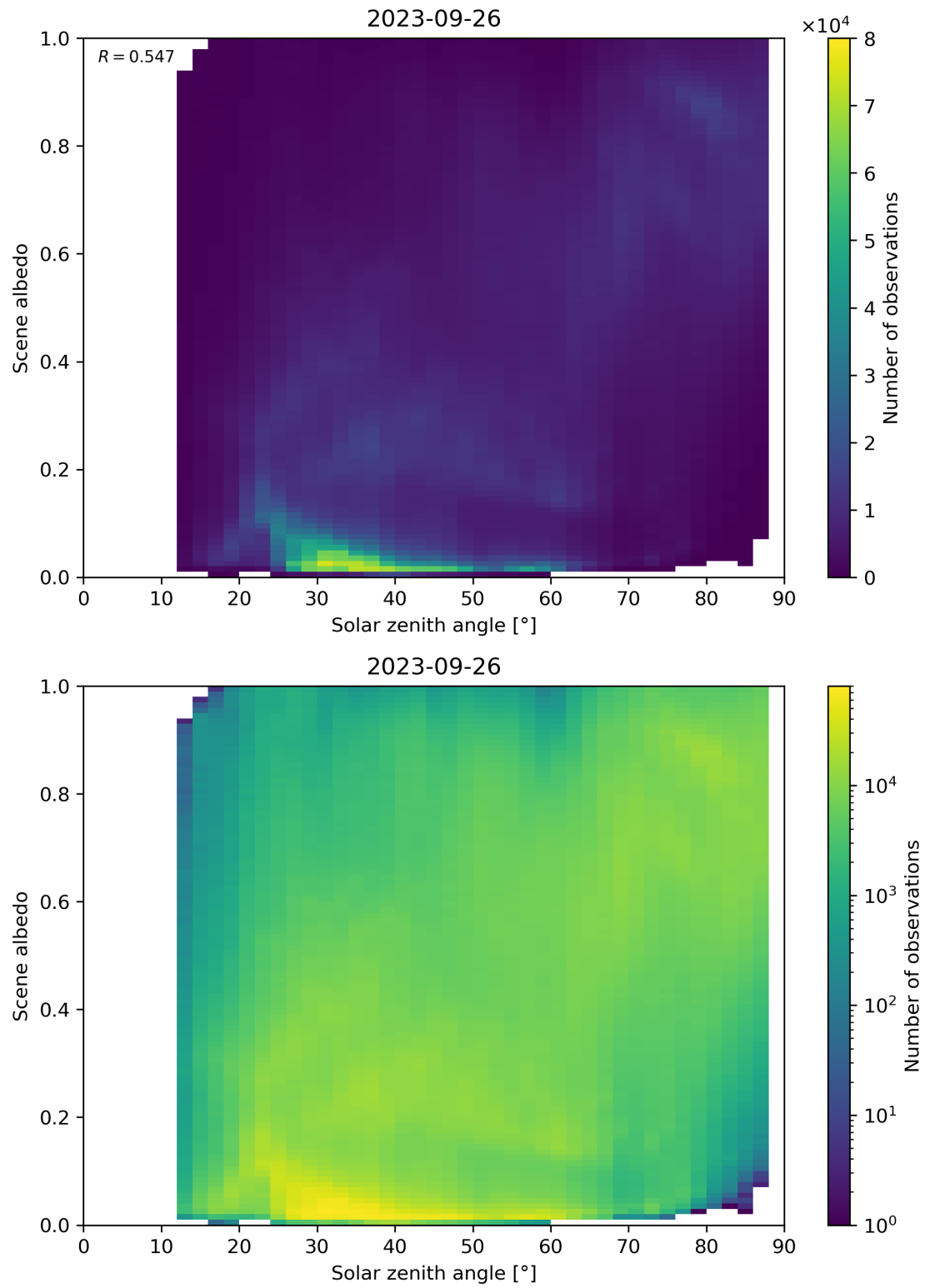
Figure 127: Scatter density plot of “Solar zenith angle” against “Scene albedo” for 2023-09-26 to 2023-09-27.
