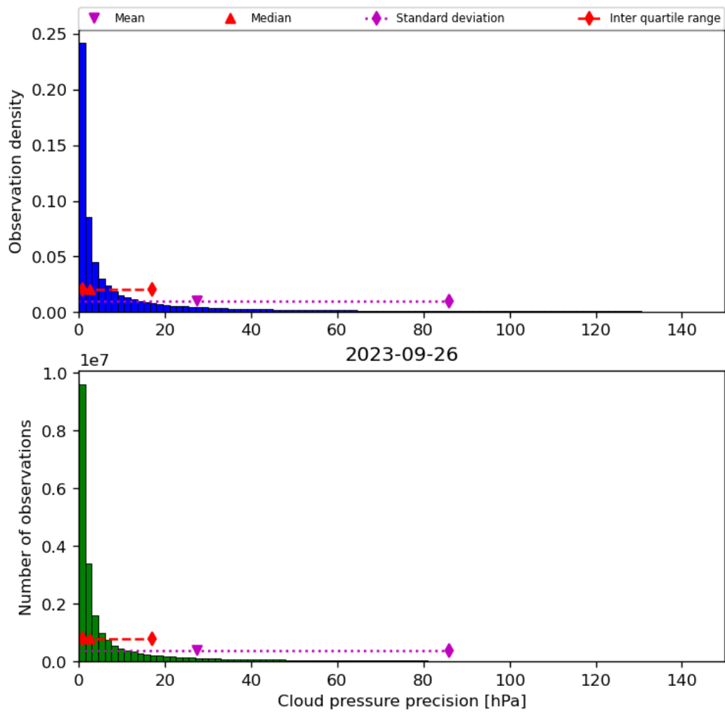
Figure 31: Histogram of “Cloud pressure precision” for 2023-09-26 to 2023-09-27
