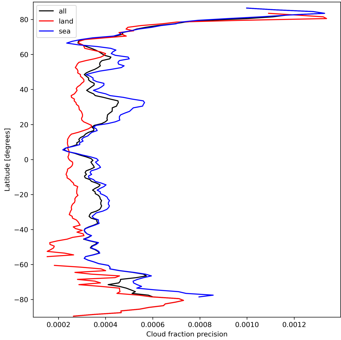
Figure 16: Zonal average of “Cloud fraction precision” for 2023-09-26 to 2023-09-27.
