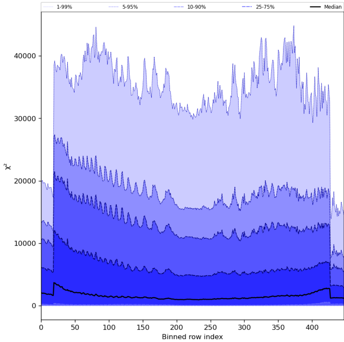
Figure 55: Along track statistics of “ \chi^2 ” for 2023-09-26 to 2023-09-27
