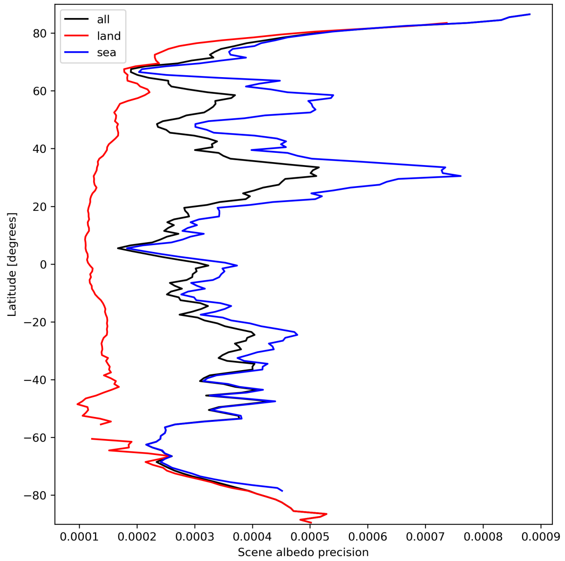
Figure 18: Zonal average of “Scene albedo precision” for 2023-09-26 to 2023-09-27.
