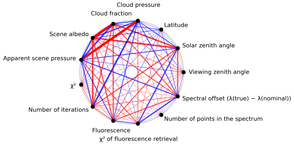
Figure 1: Map of correlation graph for 2023-09-26 to 2023-09-27.
