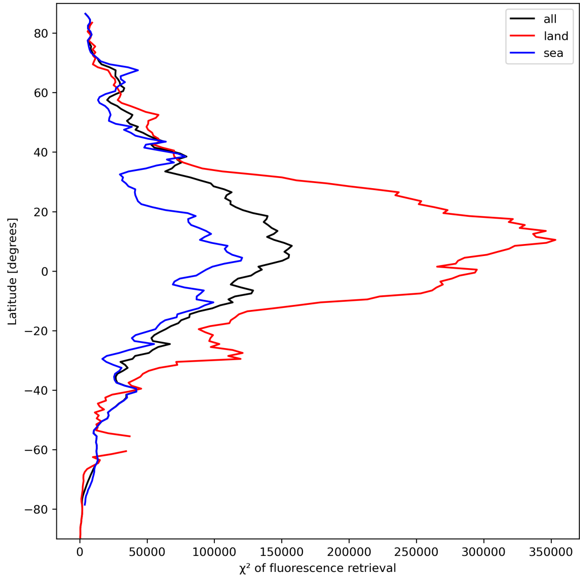
Figure 25: Zonal average of “ \chi^2 of fluorescence retrieval” for 2023-09-26 to 2023-09-27.
