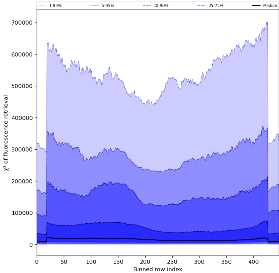
Figure 59: Along track statistics of “ \chi^2 of fluorescence retrieval” for 2023-09-26 to 2023-09-27
