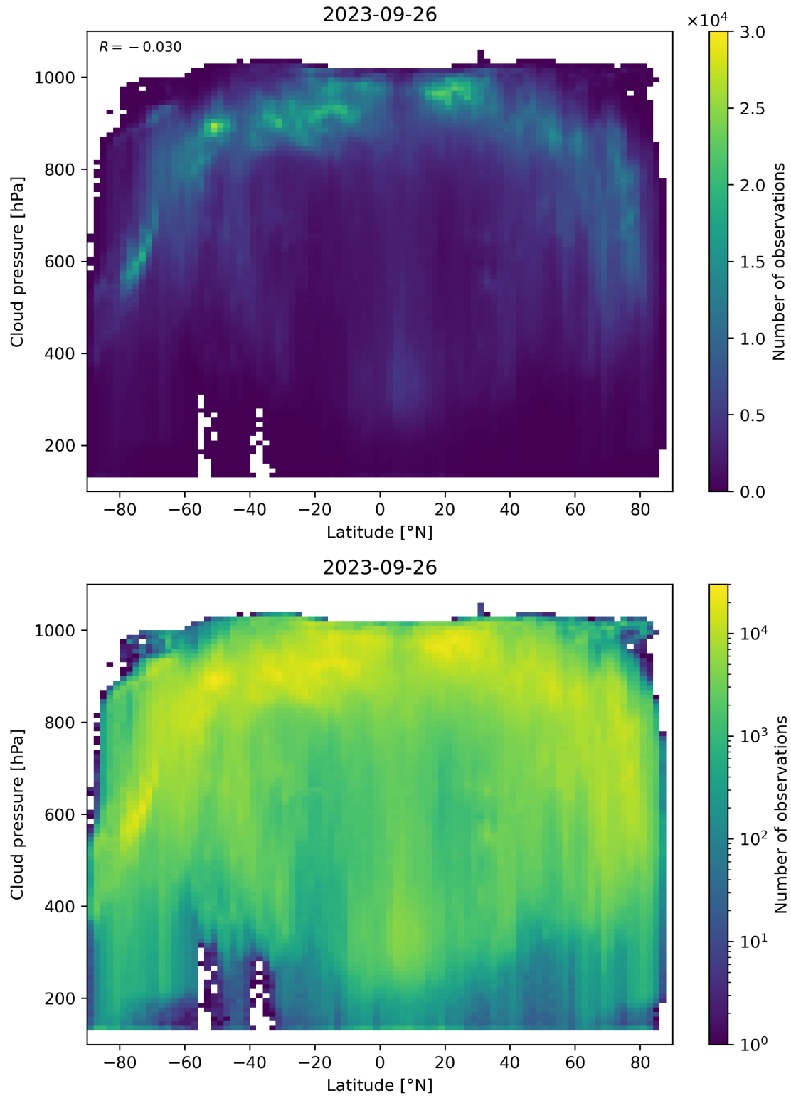
Figure 100: Scatter density plot of “Latitude” against “Cloud pressure” for 2023-09-26 to 2023-09-27.
