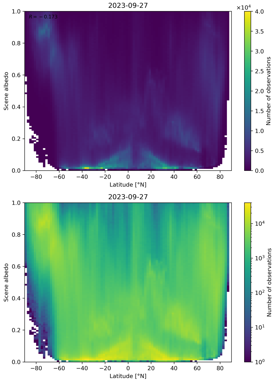
Figure 104: Scatter density plot of “Latitude” against “Scene albedo” for 2023-09-26 to 2023-09-28.
