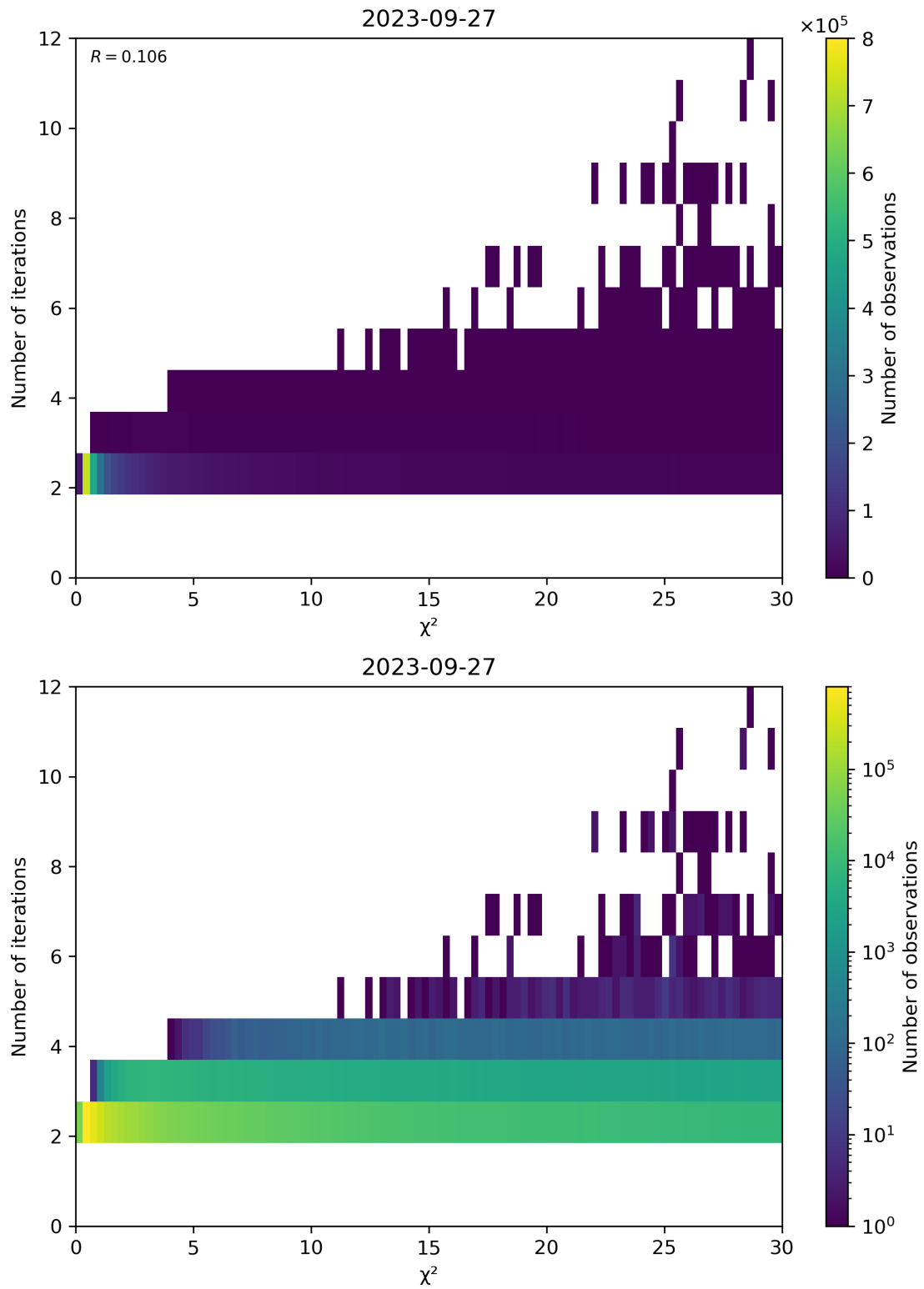
Figure 73: Scatter density plot of “ \chi^2 ” against “Number of iterations” for 2023-09-26 to 2023-09-28.
