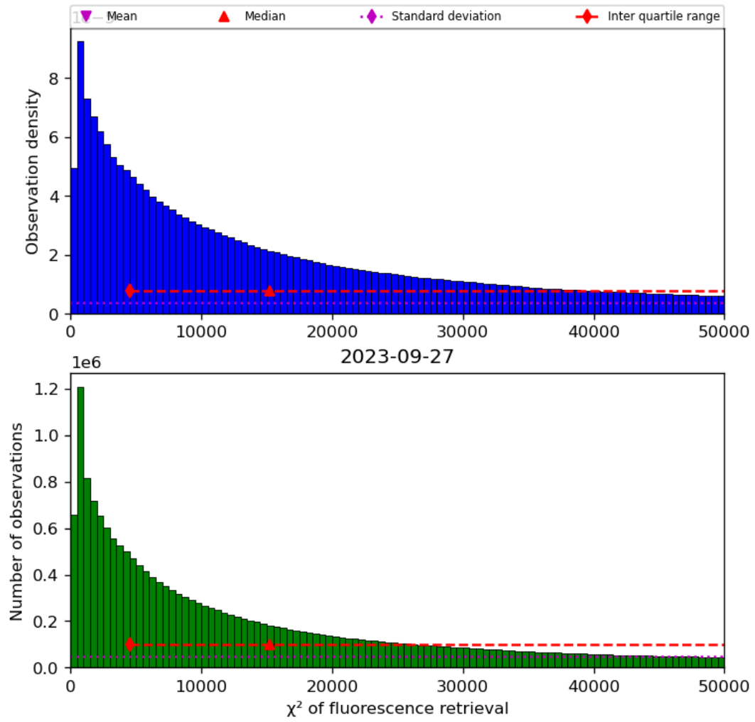
Figure 42: Histogram of “ \chi^2 of fluorescence retrieval” for 2023-09-26 to 2023-09-28
