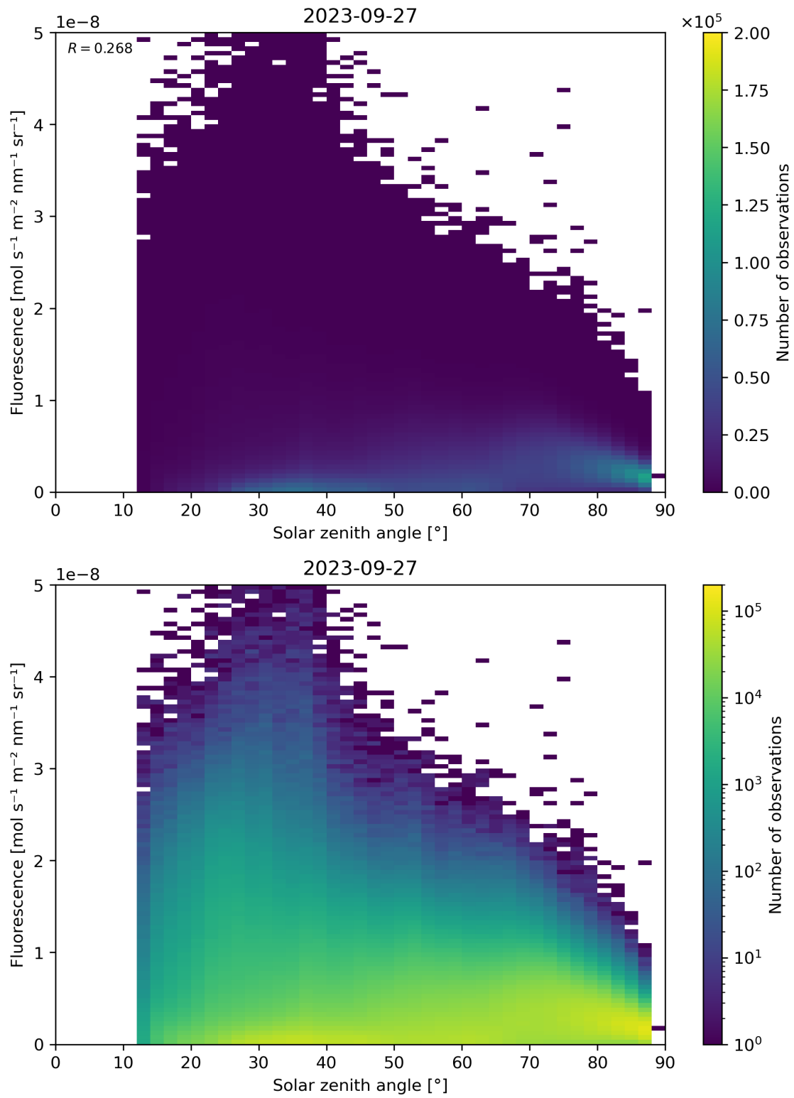
Figure 123: Scatter density plot of “Solar zenith angle” against “Fluorescence” for 2023-09-26 to 2023-09-28.
