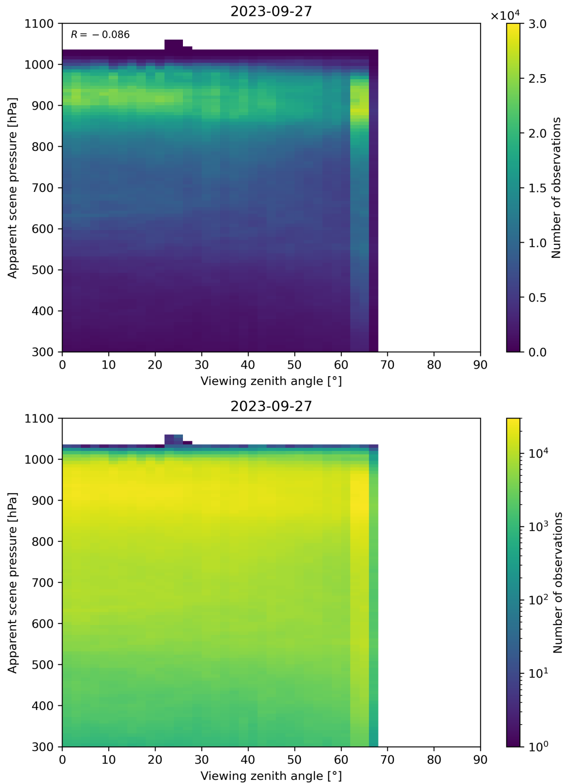
Figure 129: Scatter density plot of “Viewing zenith angle” against “Apparent scene pressure” for 2023-09-26 to 2023-09-28.
