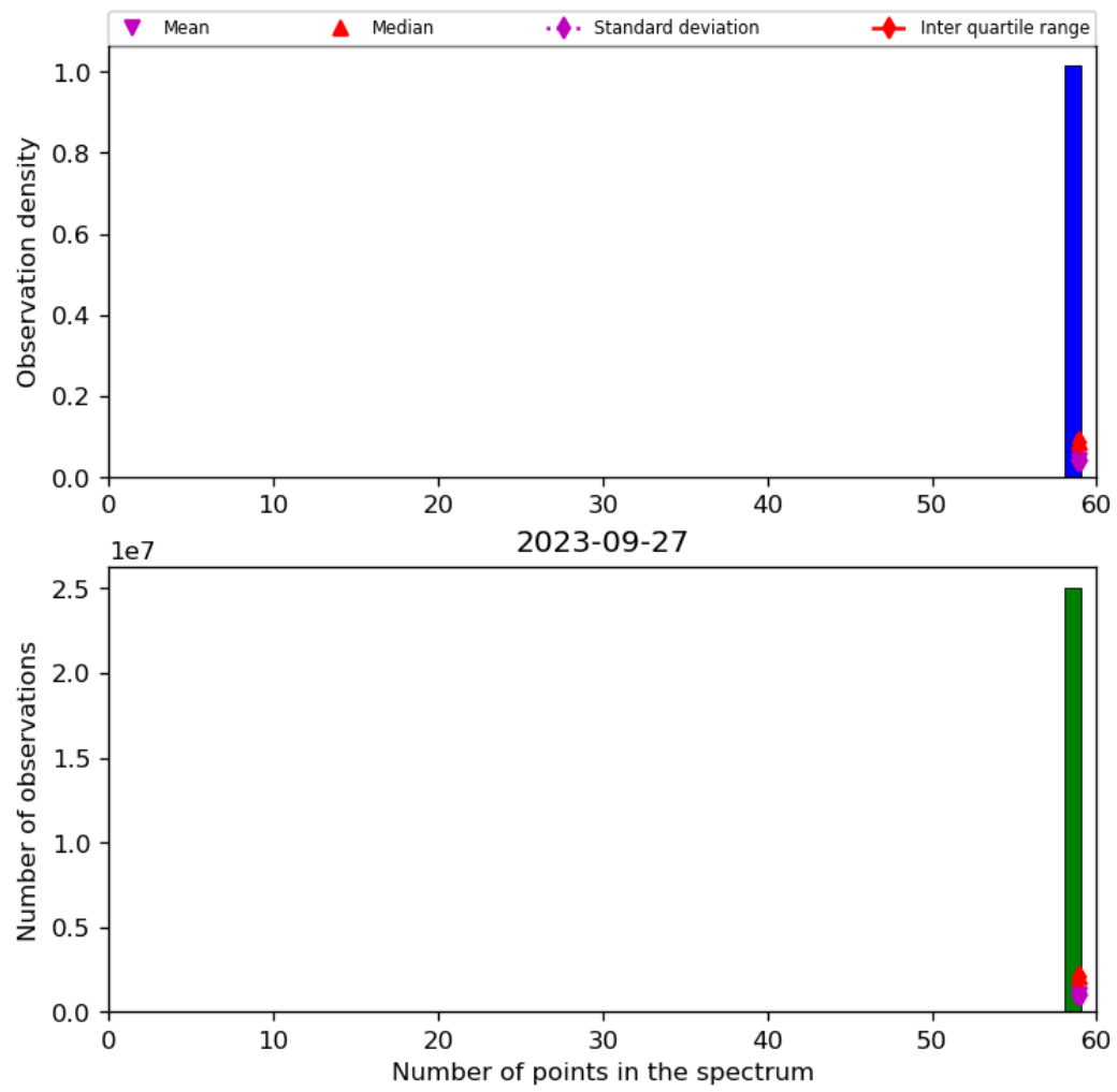
Figure 44: Histogram of “Number of points in the spectrum” for 2023-09-26 to 2023-09-28
