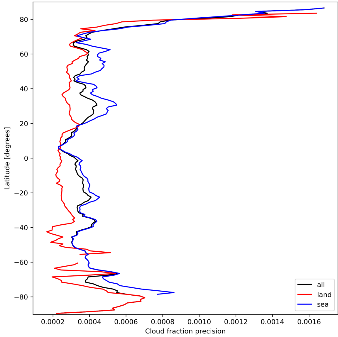
Figure 16: Zonal average of "Cloud fraction precision" for 2023-09-26 to 2023-09-28.
