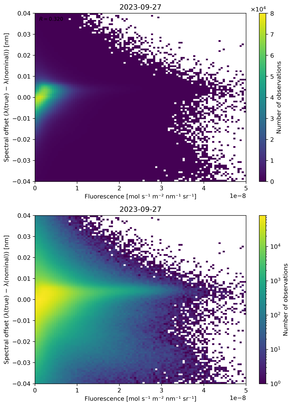
Figure 95: Scatter density plot of “Fluorescence” against “Spectral offset ( \lambda(\text{true}) - \lambda(\text{nominal}) )” for 2023-09-26 to 2023-09-28.
