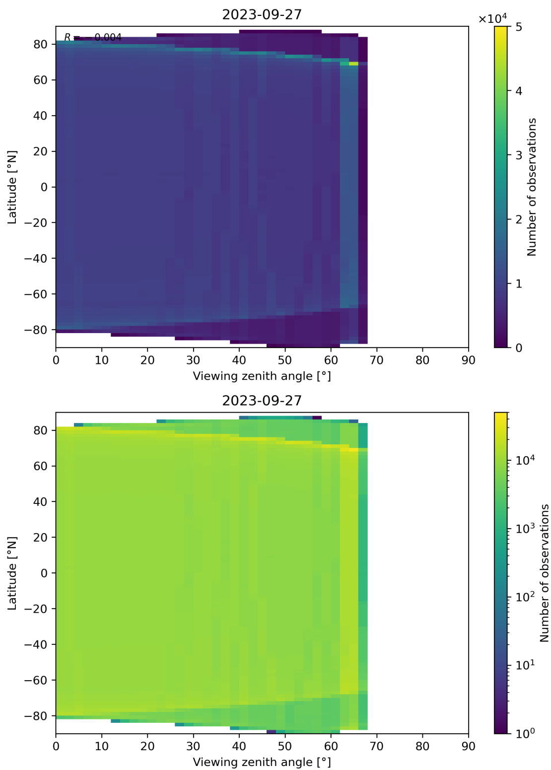
Figure 135: Scatter density plot of “Viewing zenith angle” against “Latitude” for 2023-09-26 to 2023-09-28.
