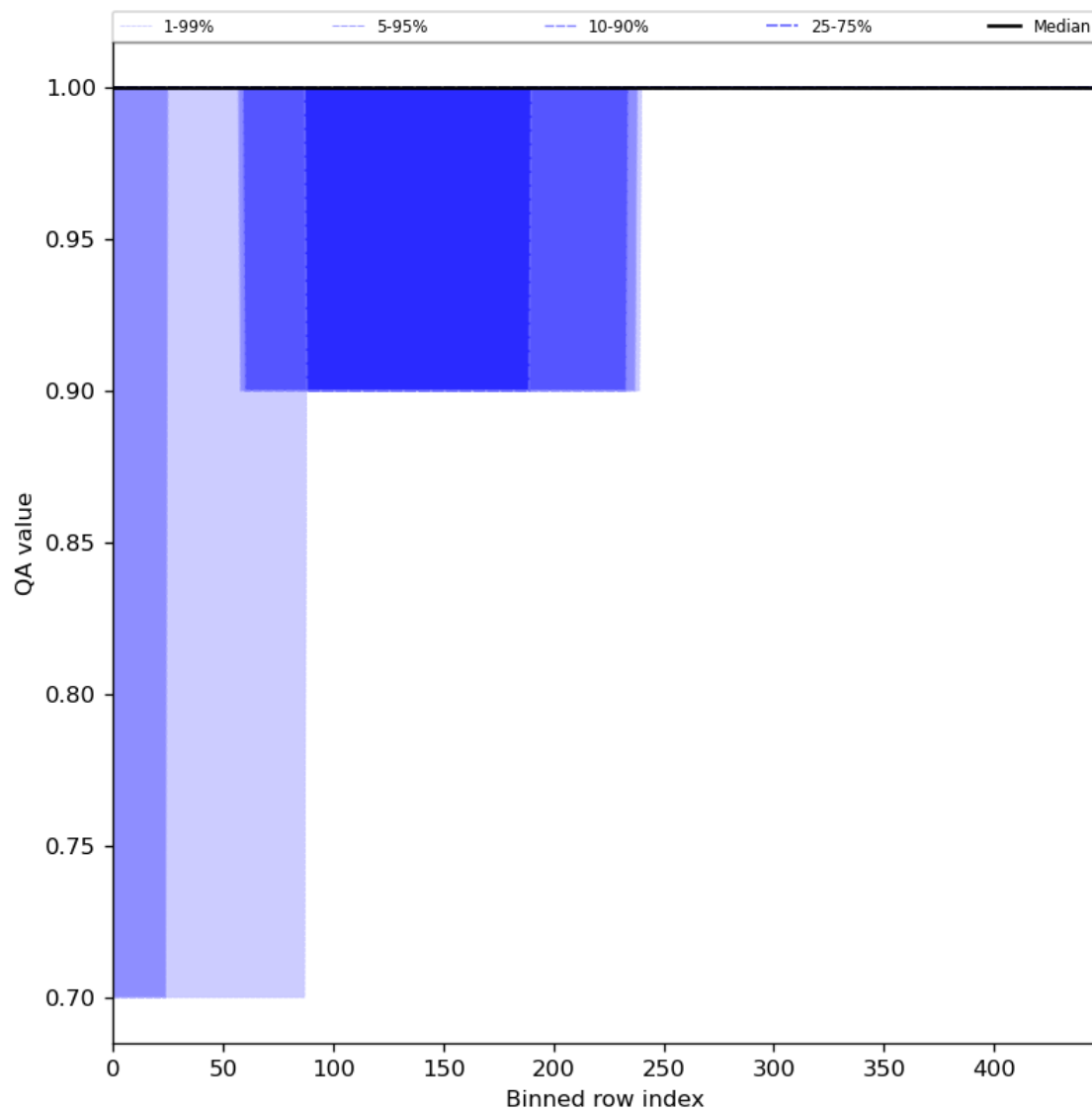
Figure 46: Along track statistics of “QA value” for 2023-09-26 to 2023-09-28
