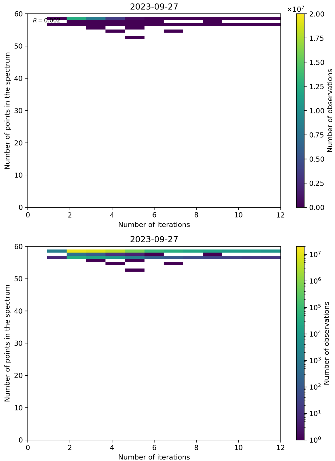
Figure 108: Scatter density plot of “Number of iterations” against “Number of points in the spectrum” for 2023-09-26 to 2023-09-28.
