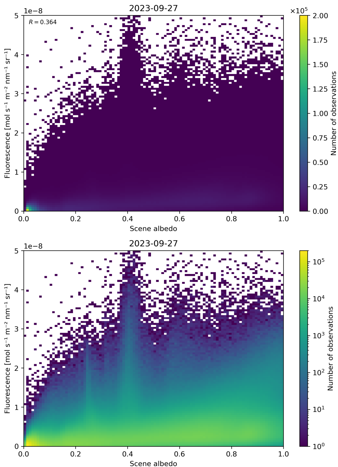
Figure 114: Scatter density plot of “Scene albedo” against “Fluorescence” for 2023-09-26 to 2023-09-28.
