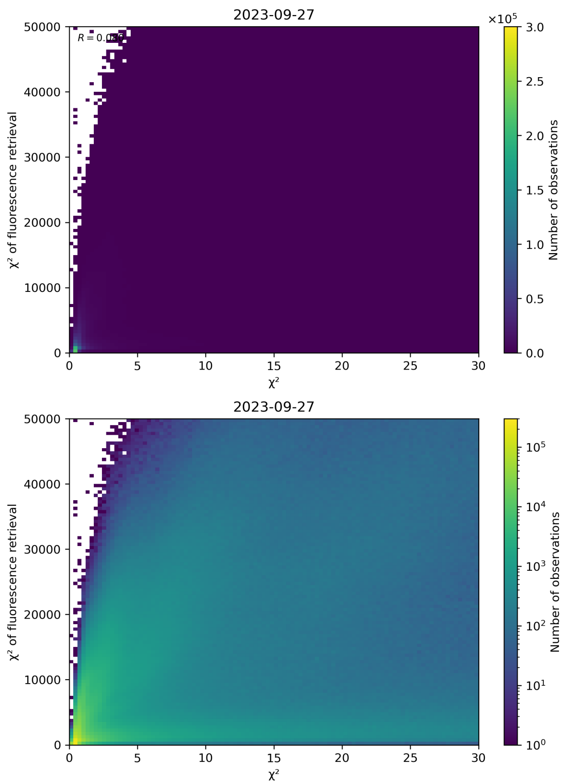
Figure 69: Scatter density plot of “ \chi^2 ” against “ \chi^2 of fluorescence retrieval” for 2023-09-26 to 2023-09-28.
