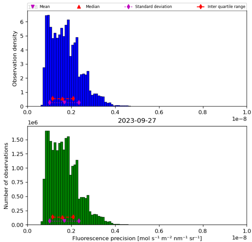
Figure 41: Histogram of “Fluorescence precision” for 2023-09-26 to 2023-09-28
