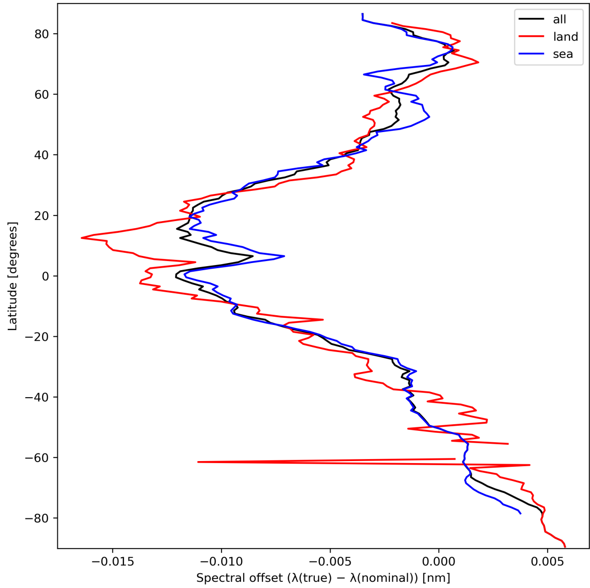
Figure 28: Zonal average of “Spectral offset ( \lambda(\text{true}) - \lambda(\text{nominal}) )” for 2023-09-26 to 2023-09-28.
