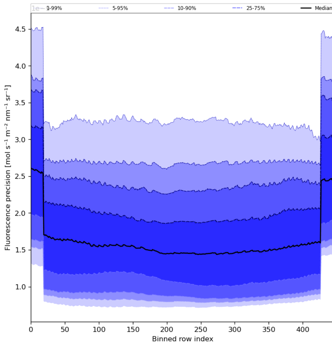
Figure 58: Along track statistics of “Fluorescence precision” for 2023-09-26 to 2023-09-28
