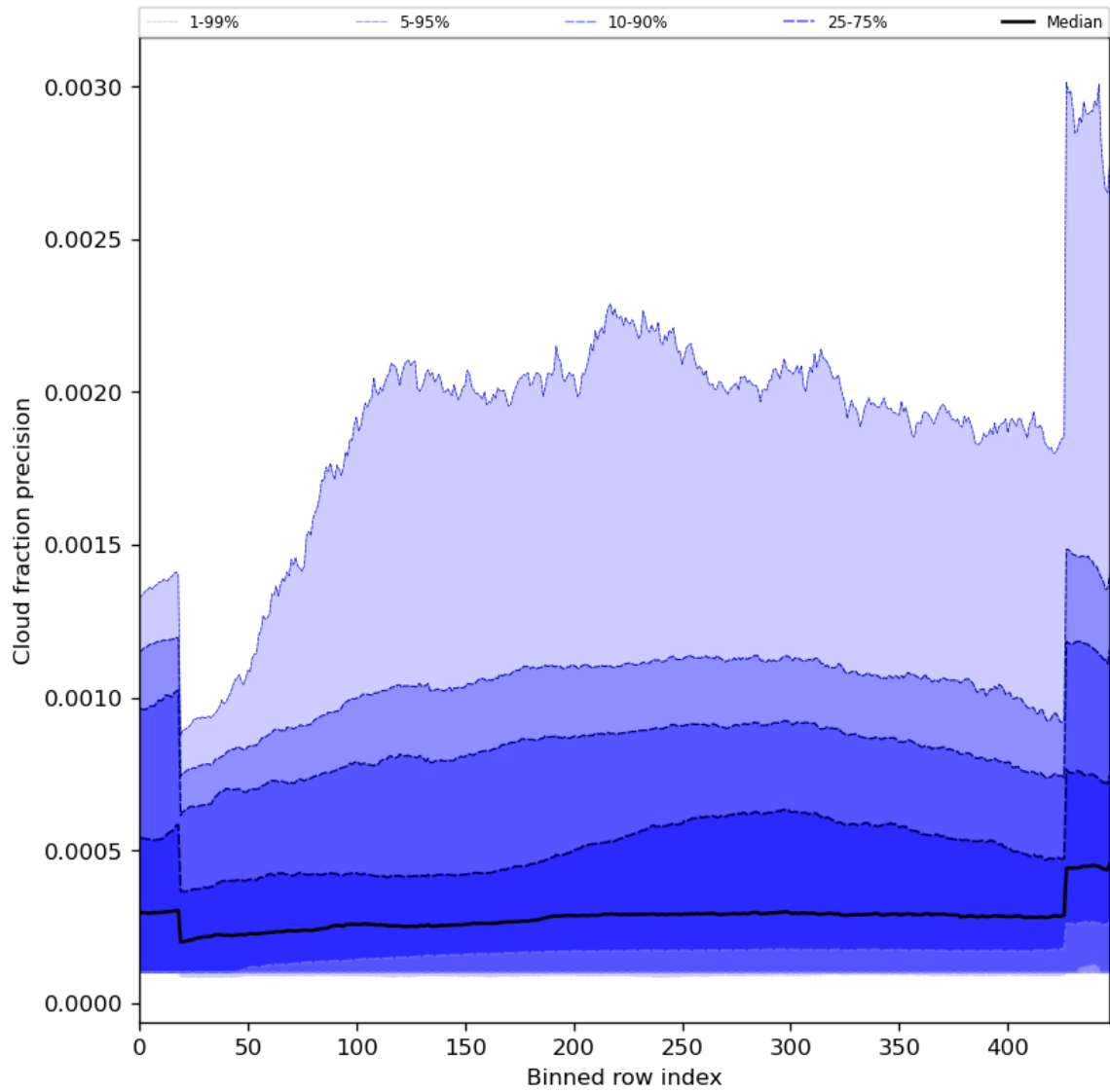
Figure 50: Along track statistics of “Cloud fraction precision” for 2023-09-26 to 2023-09-28
