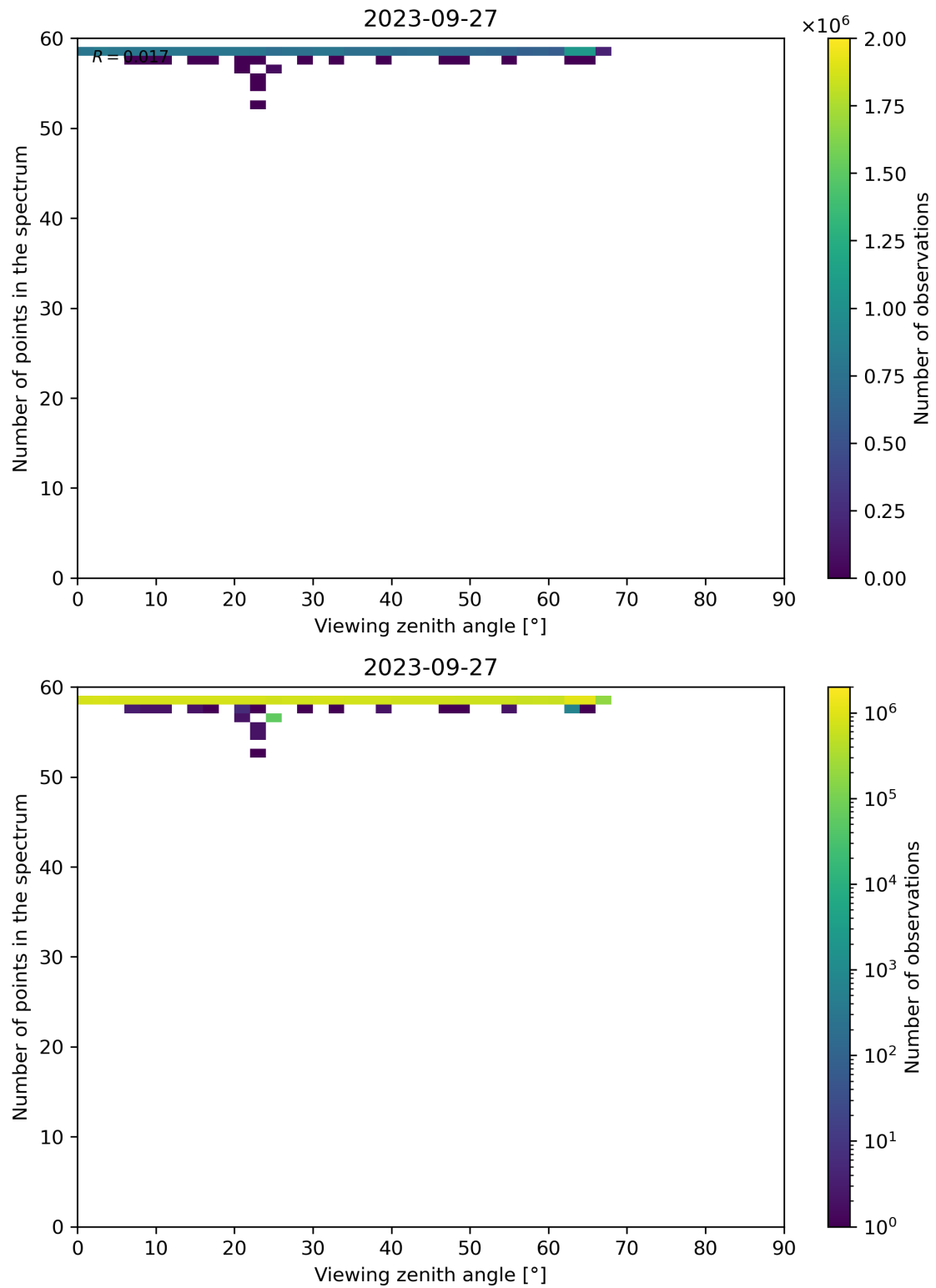
Figure 137: Scatter density plot of “Viewing zenith angle” against “Number of points in the spectrum” for 2023-09-26 to 2023-09-28.
