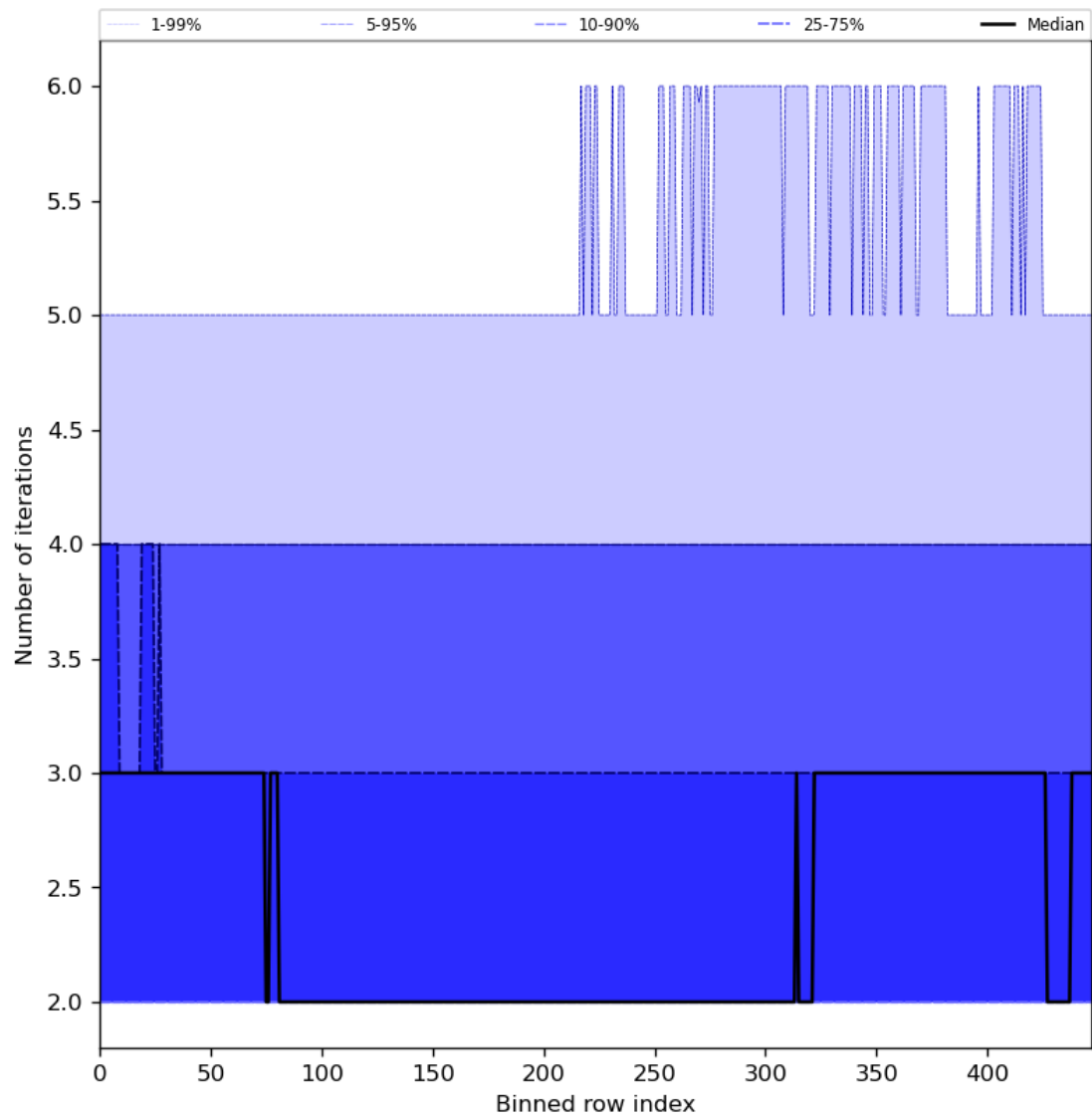
Figure 56: Along track statistics of “Number of iterations” for 2023-09-26 to 2023-09-28
