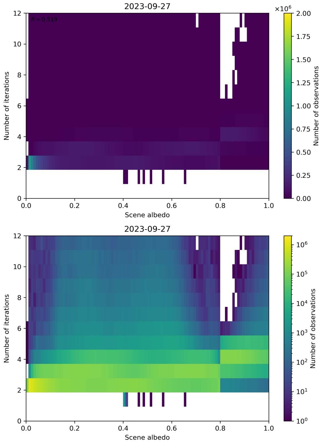
Figure 115: Scatter density plot of “Scene albedo” against “Number of iterations” for 2023-09-26 to 2023-09-28.
