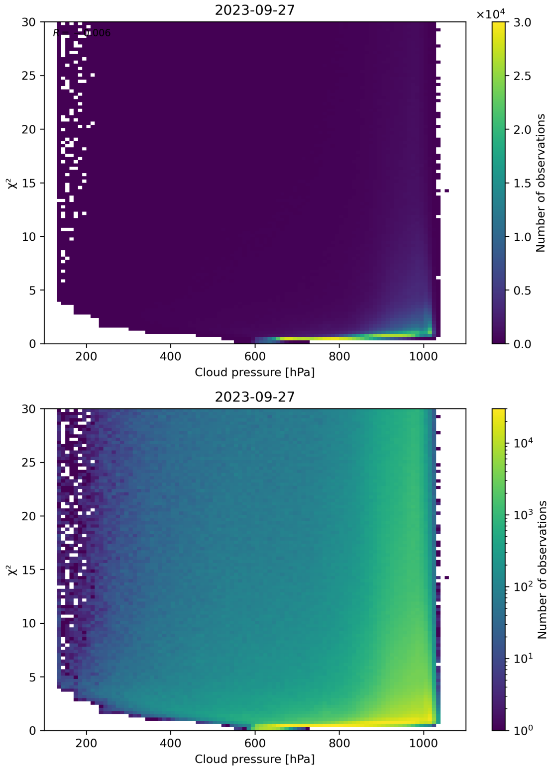
Figure 85: Scatter density plot of “Cloud pressure” against “ \chi^2 ” for 2023-09-26 to 2023-09-28.
