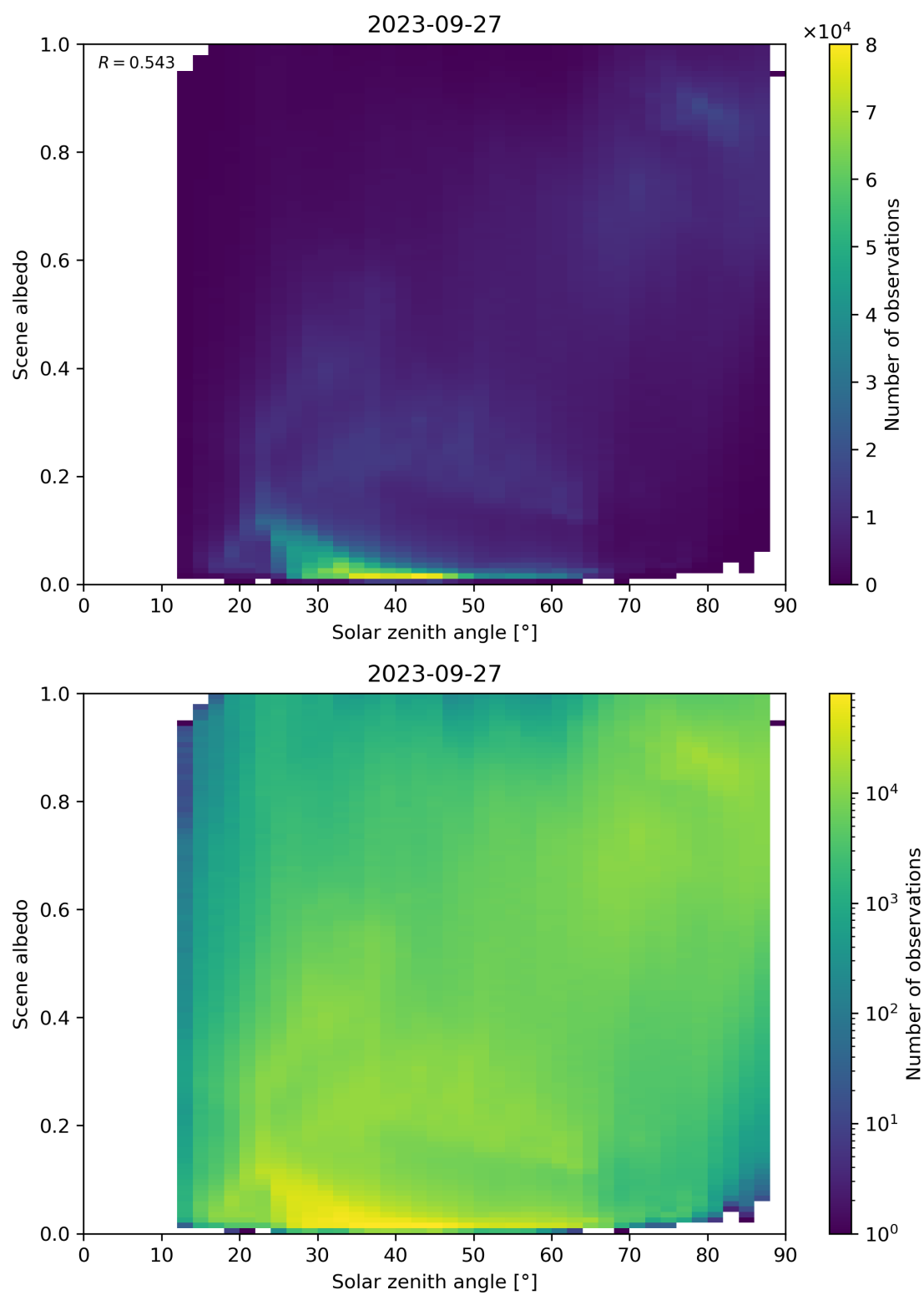
Figure 127: Scatter density plot of “Solar zenith angle” against “Scene albedo” for 2023-09-26 to 2023-09-28.
