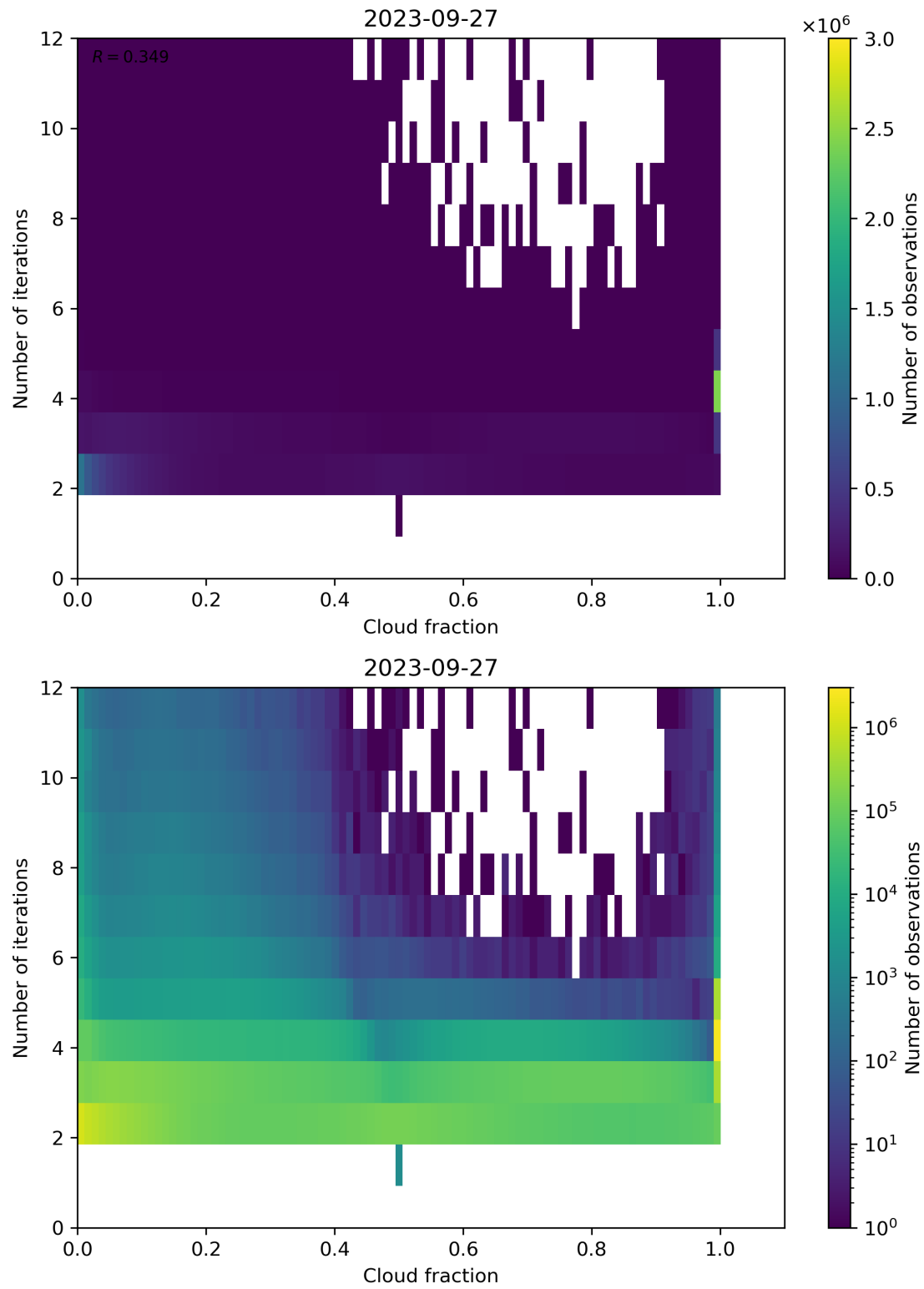
Figure 80: Scatter density plot of “Cloud fraction” against “Number of iterations” for 2023-09-26 to 2023-09-28.
