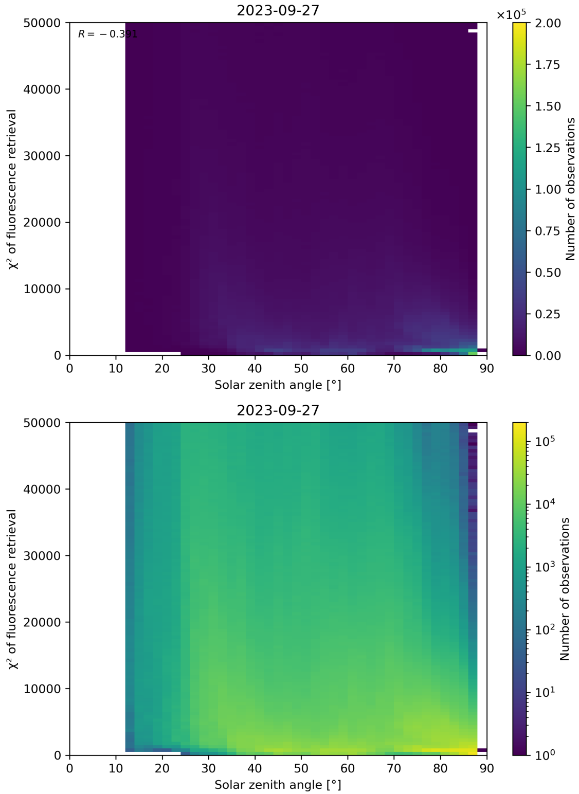
Figure 120: Scatter density plot of “Solar zenith angle” against “ \chi^2 of fluorescence retrieval” for 2023-09-26 to 2023-09-28.
