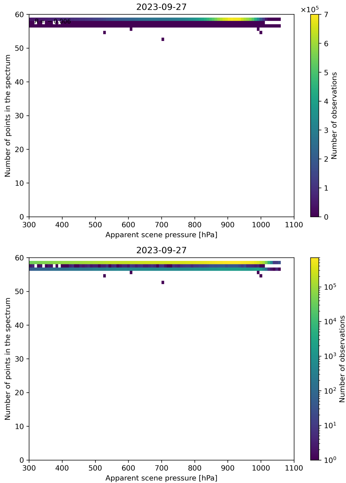
Figure 67: Scatter density plot of “Apparent scene pressure” against “Number of points in the spectrum” for 2023-09-26 to 2023-09-28.
