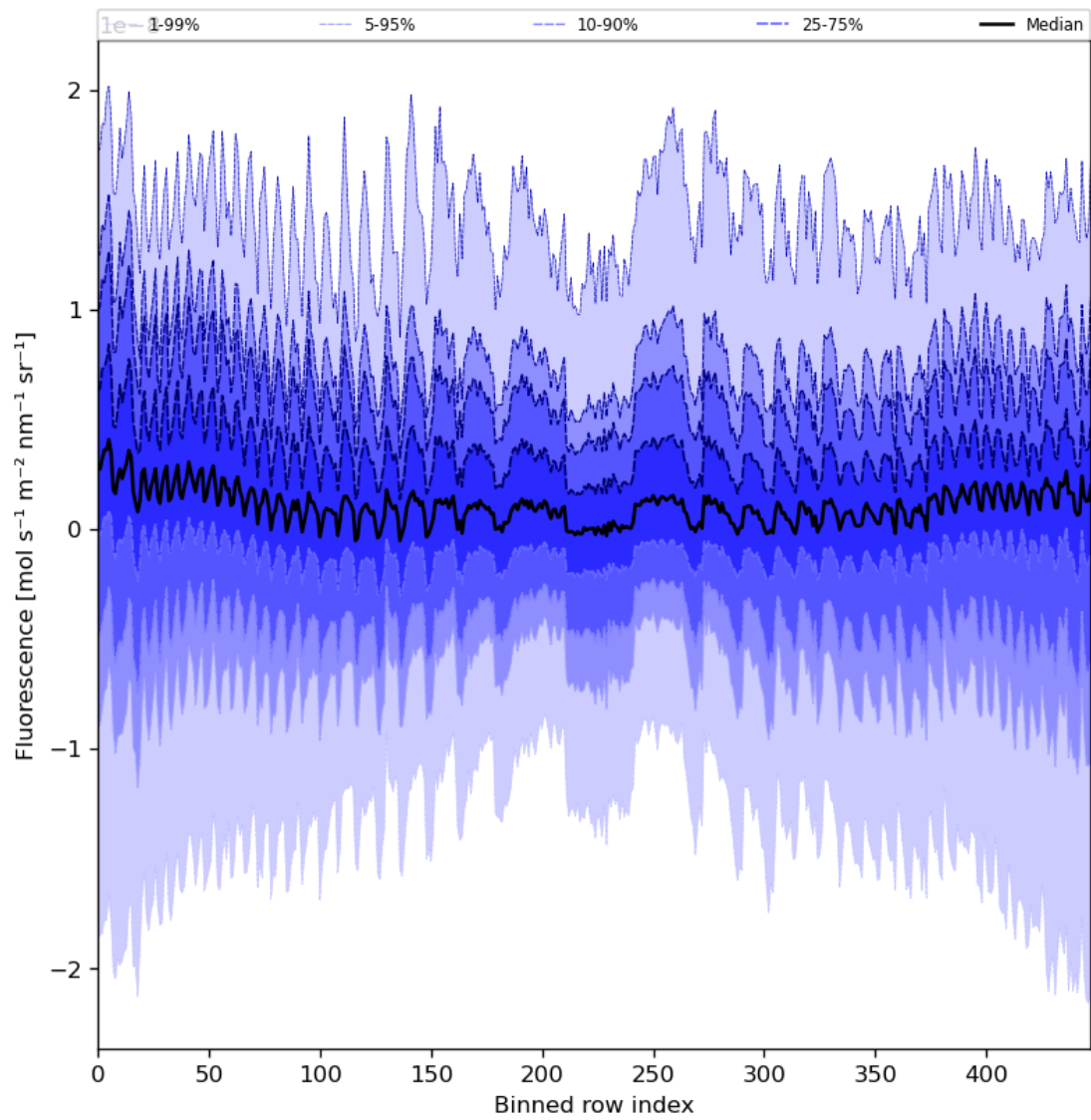
Figure 57: Along track statistics of “Fluorescence” for 2023-09-26 to 2023-09-28
