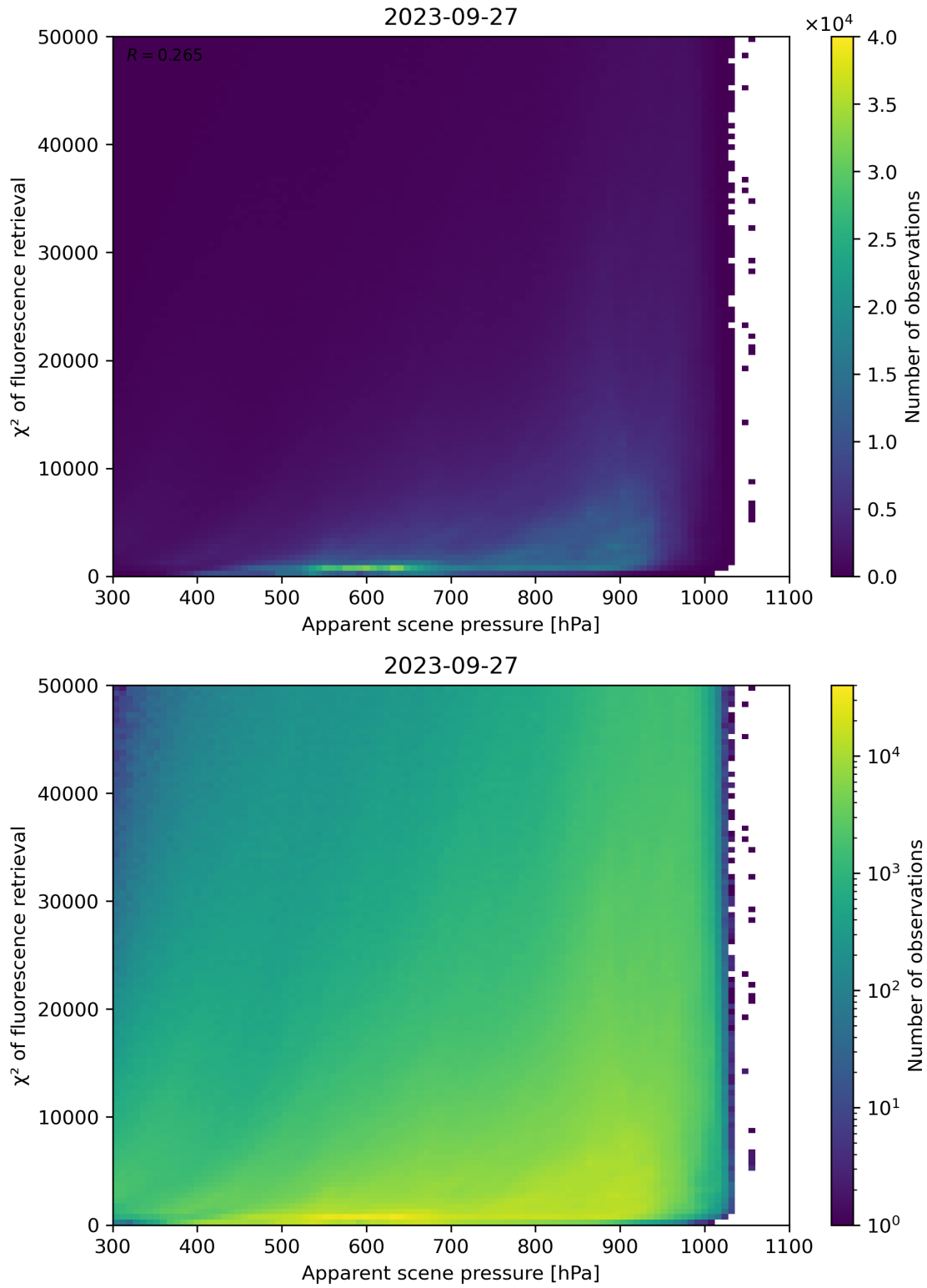
Figure 64: Scatter density plot of “Apparent scene pressure” against “ \chi^2 of fluorescence retrieval” for 2023-09-26 to 2023-09-28.
