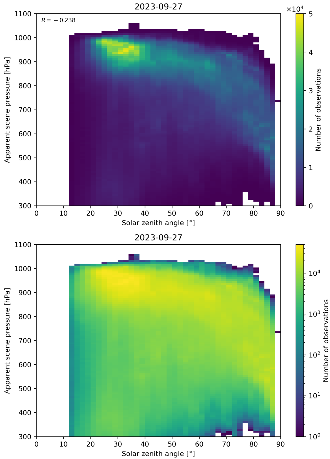
Figure 118: Scatter density plot of “Solar zenith angle” against “Apparent scene pressure” for 2023-09-26 to 2023-09-28.
