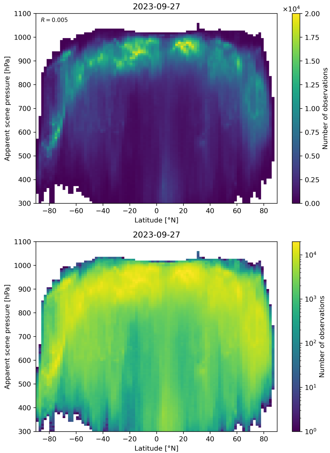
Figure 96: Scatter density plot of “Latitude” against “Apparent scene pressure” for 2023-09-26 to 2023-09-28.
