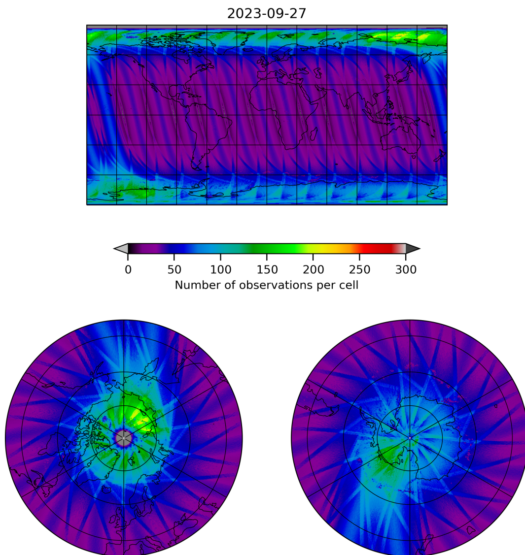
Figure 11: Map of the number of observations for 2023-09-26 to 2023-09-28
