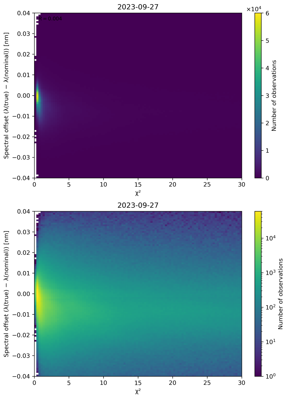
Figure 75: Scatter density plot of “ \chi^2 ” against “Spectral offset ( \lambda(\text{true}) - \lambda(\text{nominal}) )” for 2023-09-26 to 2023-09-28.
