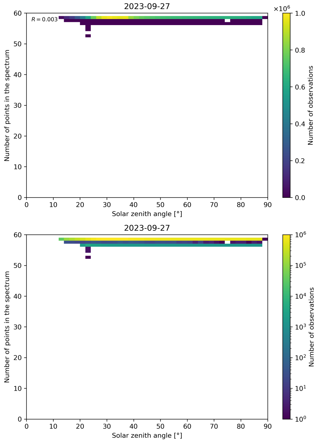
Figure 126: Scatter density plot of “Solar zenith angle” against “Number of points in the spectrum” for 2023-09-26 to 2023-09-28.
