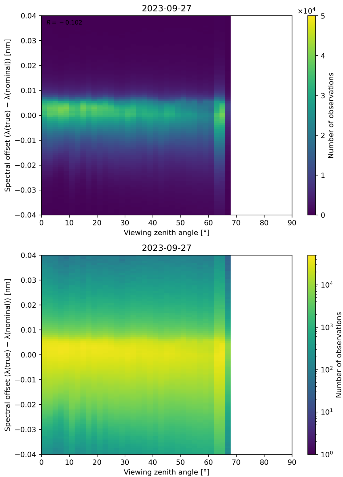
Figure 140: Scatter density plot of “Viewing zenith angle” against “Spectral offset ( \lambda(\text{true}) - \lambda(\text{nominal}) )” for 2023-09-26 to 2023-09-28.
