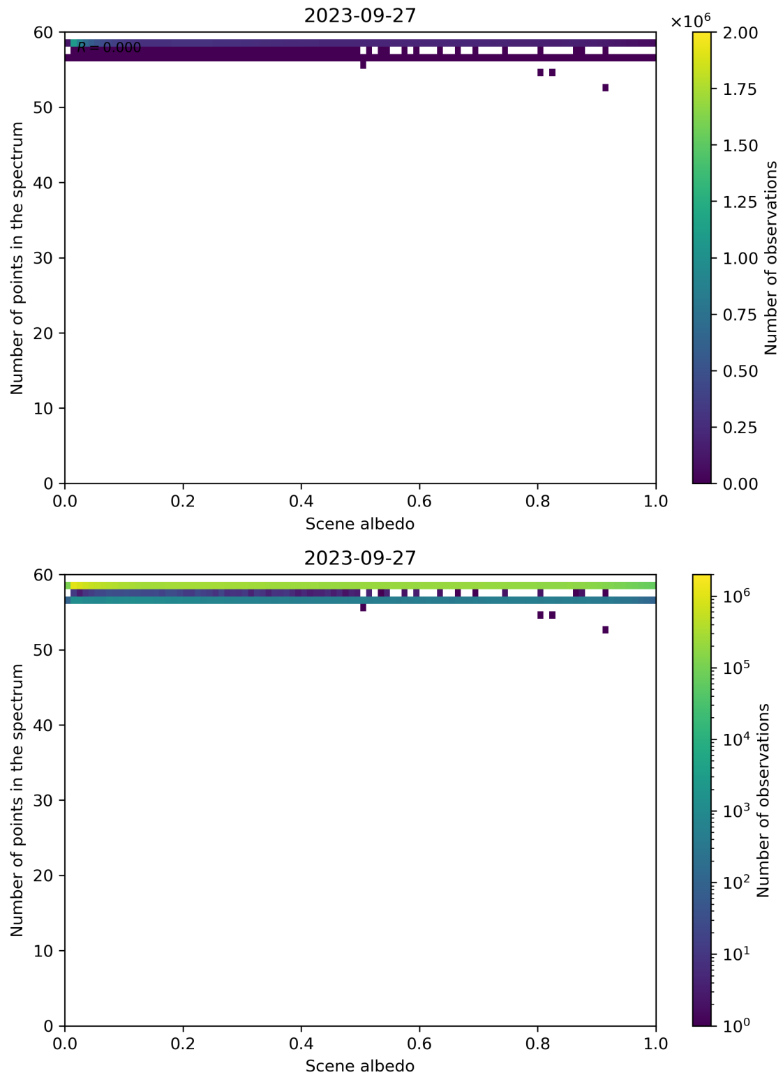
Figure 116: Scatter density plot of “Scene albedo” against “Number of points in the spectrum” for 2023-09-26 to 2023-09-28.
