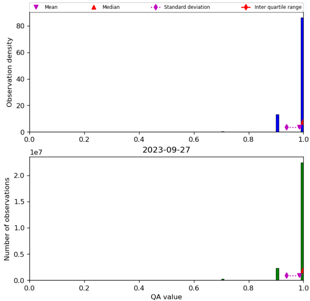
Figure 29: Histogram of “QA value” for 2023-09-26 to 2023-09-28
