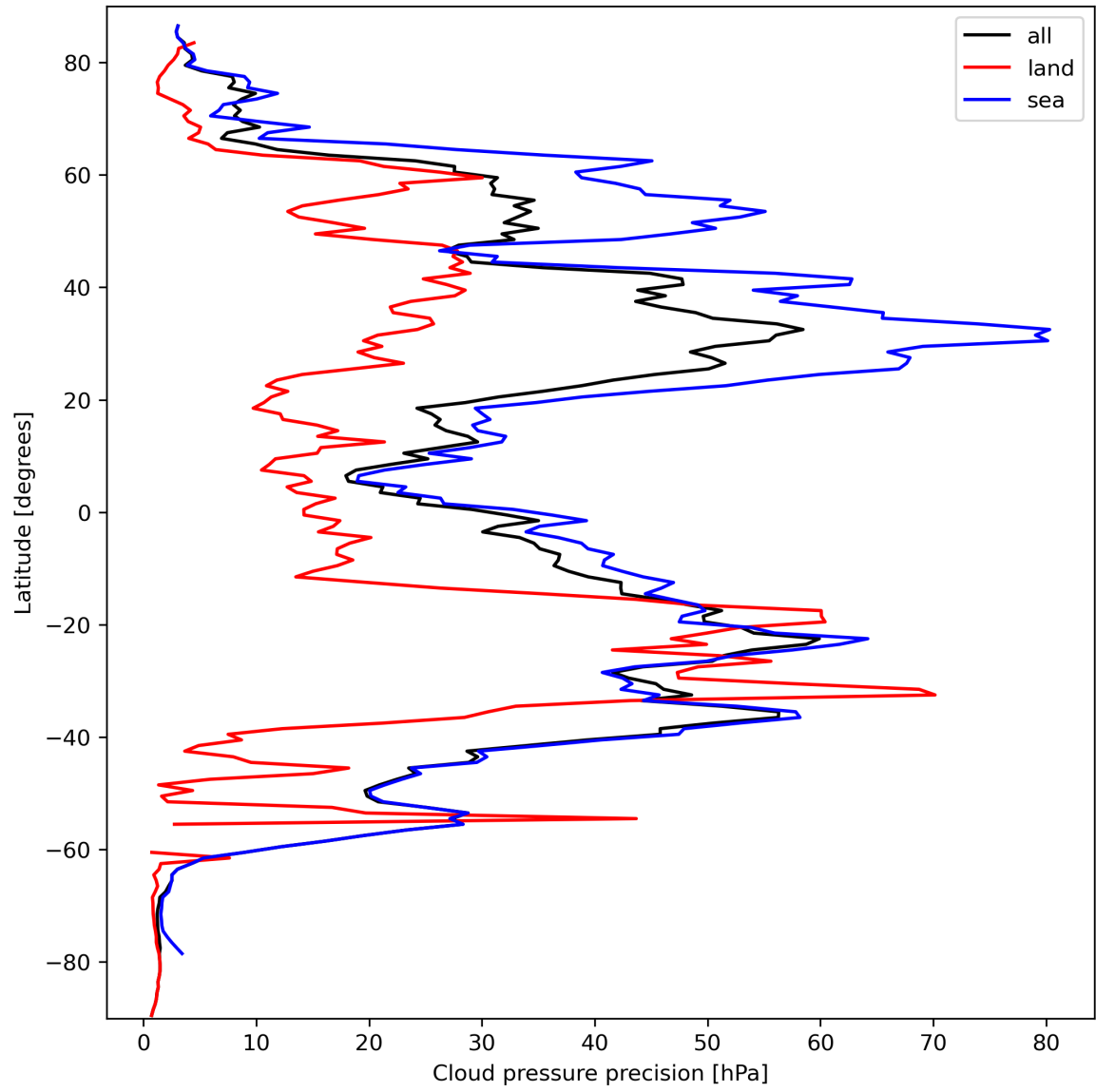
Figure 14: Zonal average of “Cloud pressure precision” for 2023-09-26 to 2023-09-28.
