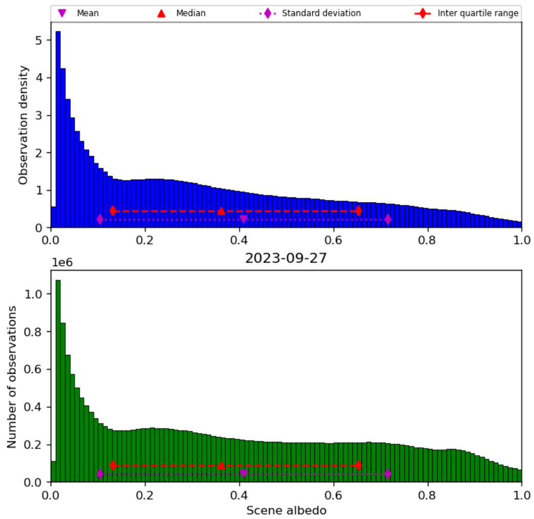
Figure 34: Histogram of “Scene albedo” for 2023-09-26 to 2023-09-28
