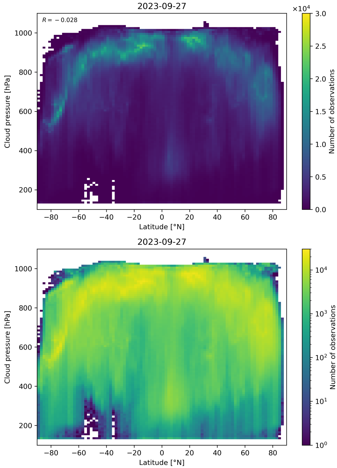
Figure 100: Scatter density plot of “Latitude” against “Cloud pressure” for 2023-09-26 to 2023-09-28.
