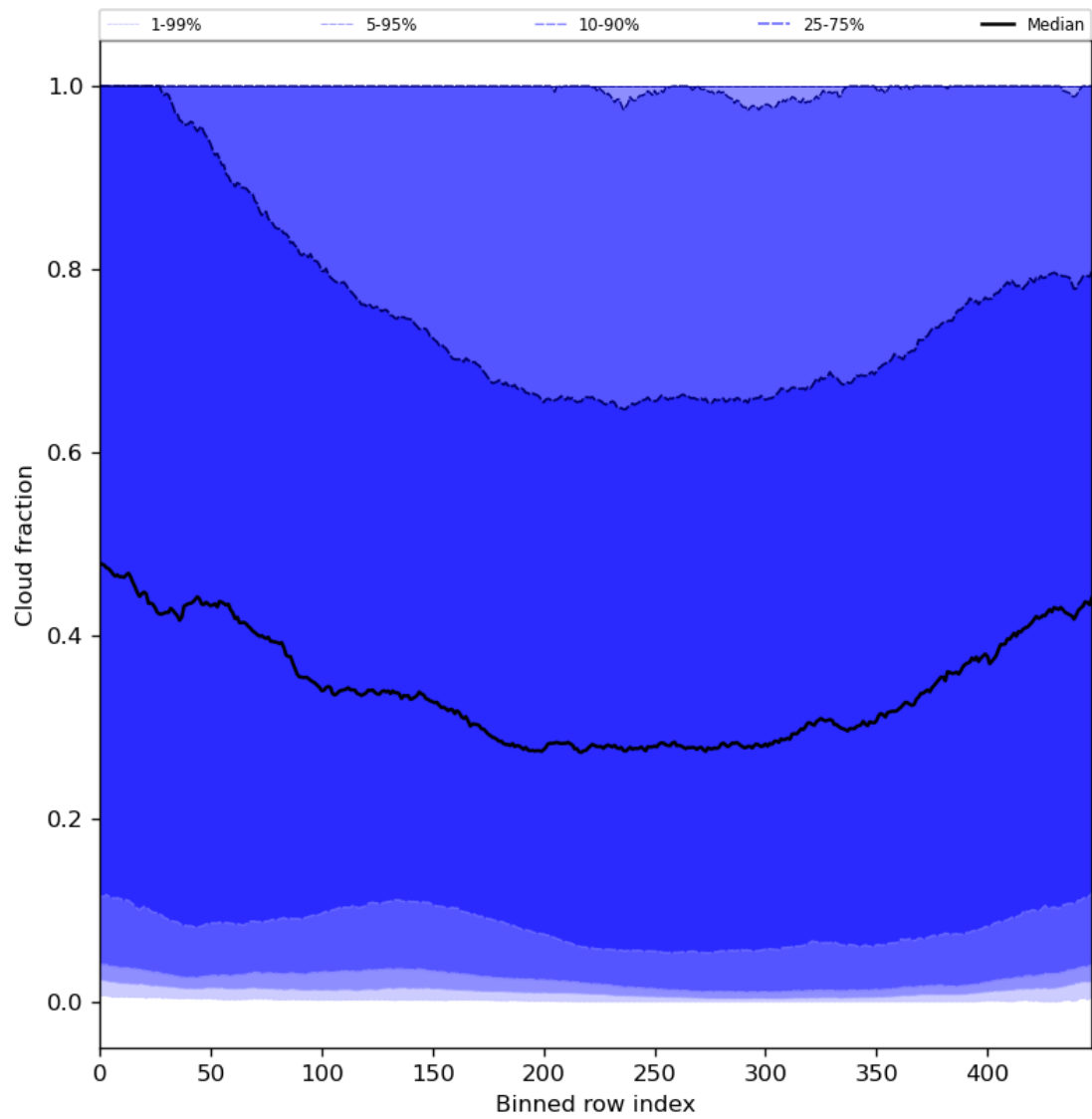
Figure 49: Along track statistics of “Cloud fraction” for 2023-09-26 to 2023-09-28
