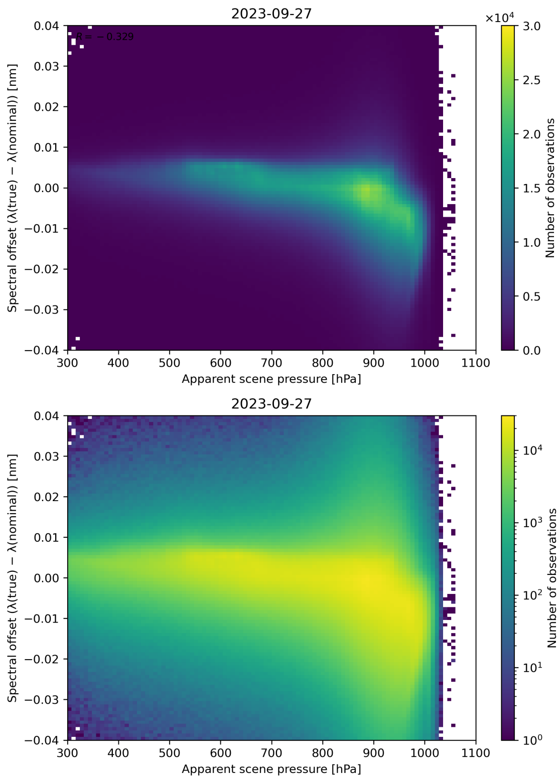
Figure 68: Scatter density plot of “Apparent scene pressure” against “Spectral offset ( \lambda(\text{true}) - \lambda(\text{nominal}) )” for 2023-09-26 to 2023-09-28.
