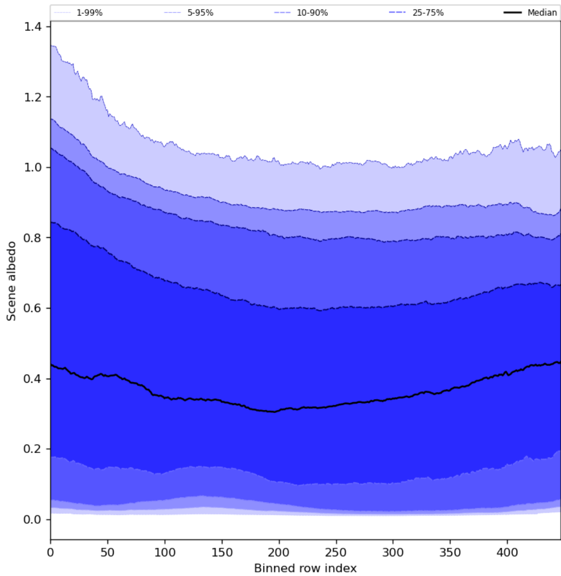
Figure 51: Along track statistics of “Scene albedo” for 2023-09-26 to 2023-09-28
