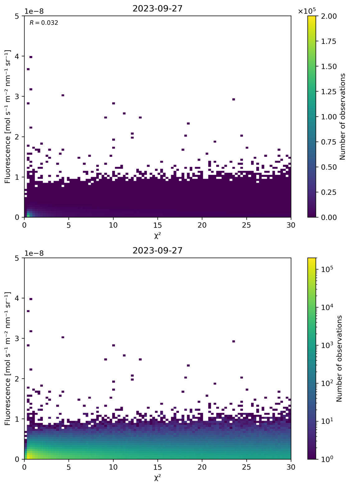
Figure 70: Scatter density plot of “ \chi^2 ” against “Fluorescence” for 2023-09-26 to 2023-09-28.
