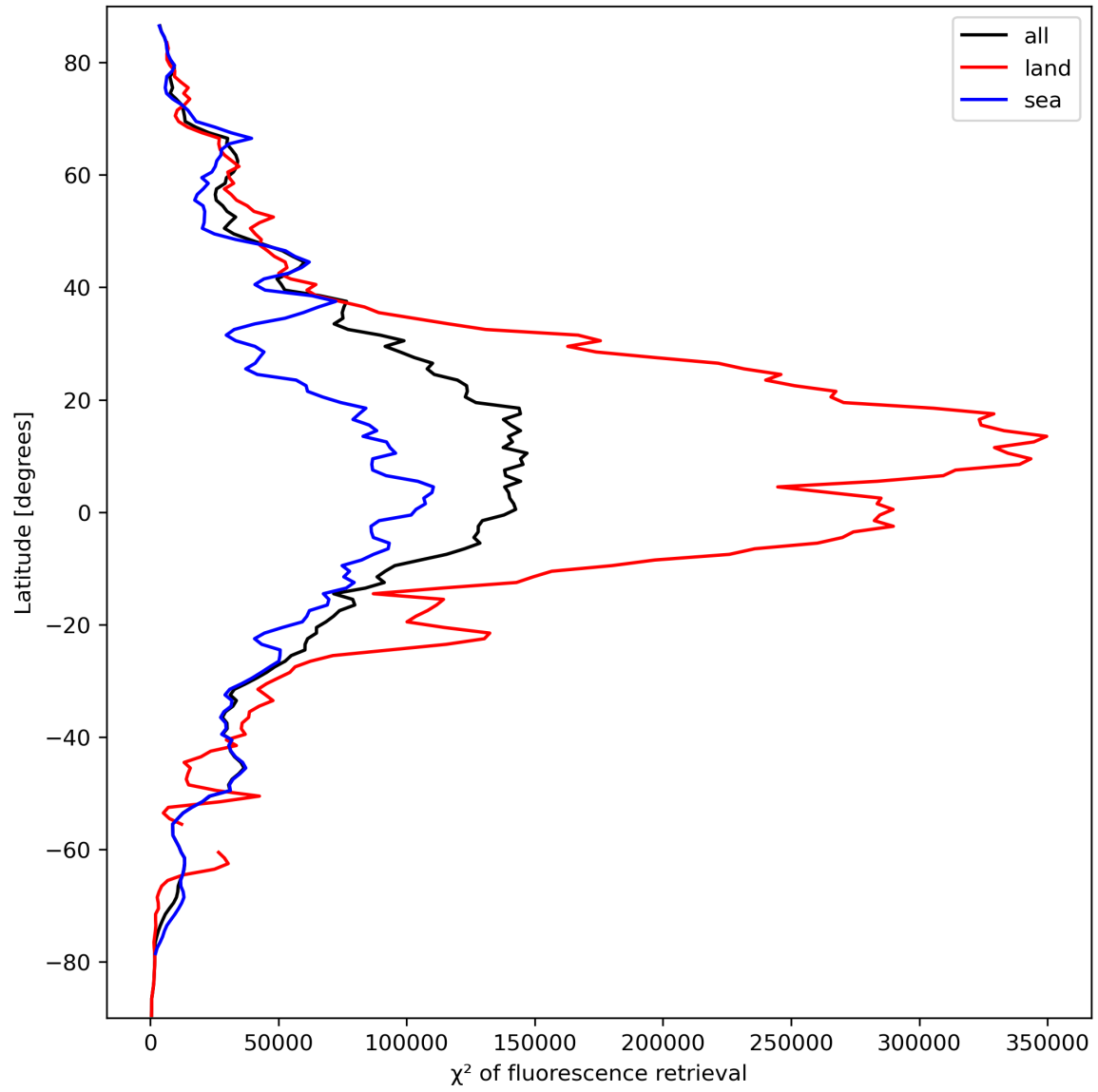
Figure 25: Zonal average of “ \chi^2 of fluorescence retrieval” for 2023-09-26 to 2023-09-28.
