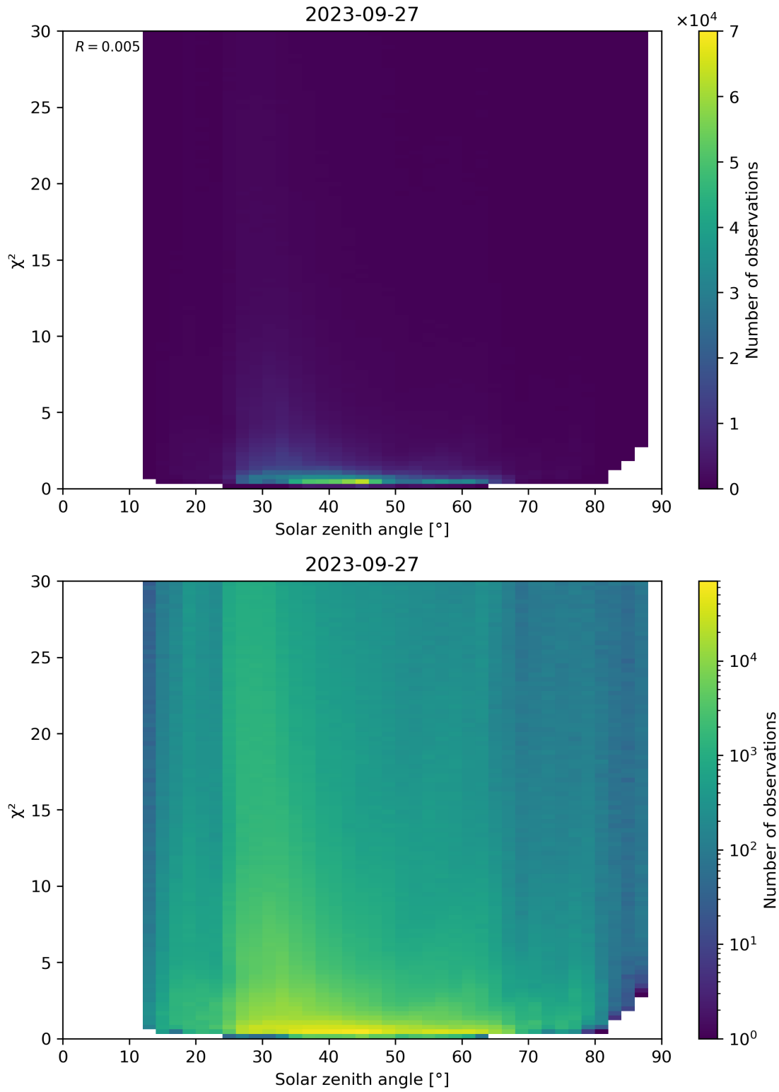
Figure 119: Scatter density plot of “Solar zenith angle” against “ \chi^2 ” for 2023-09-26 to 2023-09-28.
