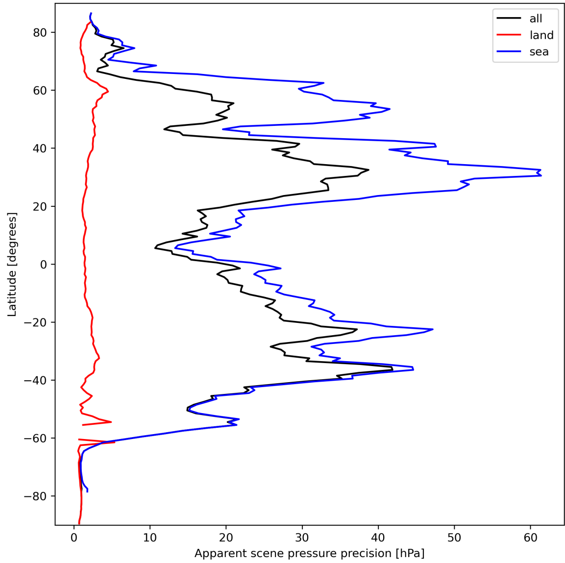
Figure 20: Zonal average of “Apparent scene pressure precision” for 2023-09-26 to 2023-09-28.
