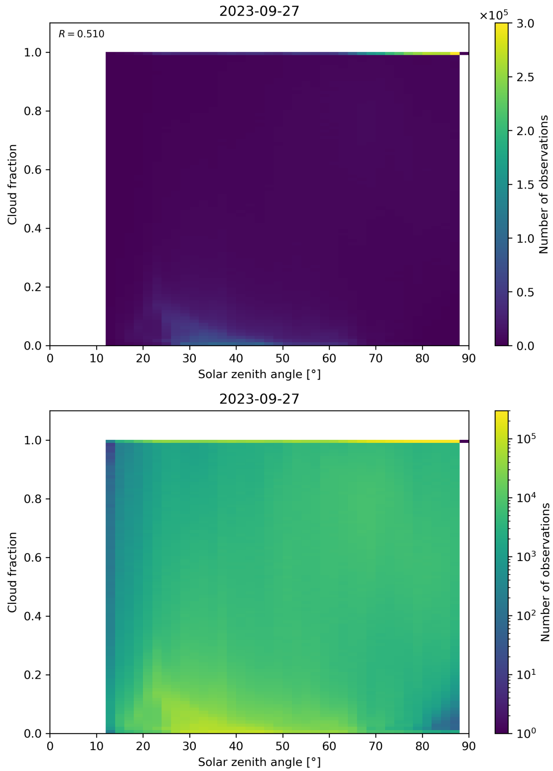
Figure 121: Scatter density plot of “Solar zenith angle” against “Cloud fraction” for 2023-09-26 to 2023-09-28.
