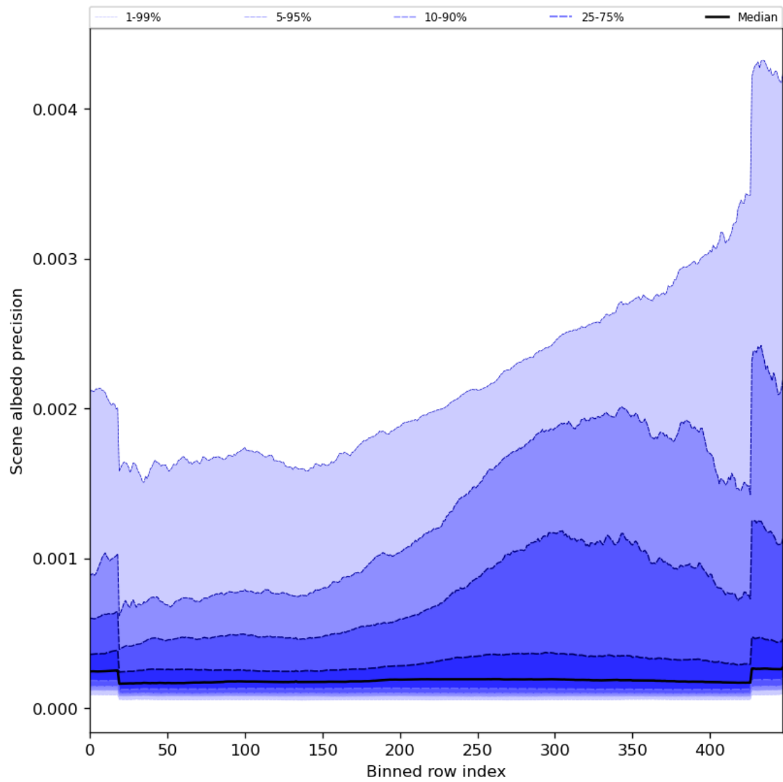
Figure 52: Along track statistics of “Scene albedo precision” for 2023-09-26 to 2023-09-28
