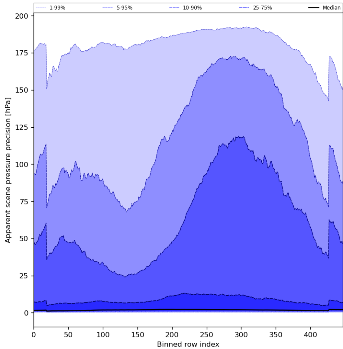
Figure 54: Along track statistics of “Apparent scene pressure precision” for 2023-09-26 to 2023-09-28
