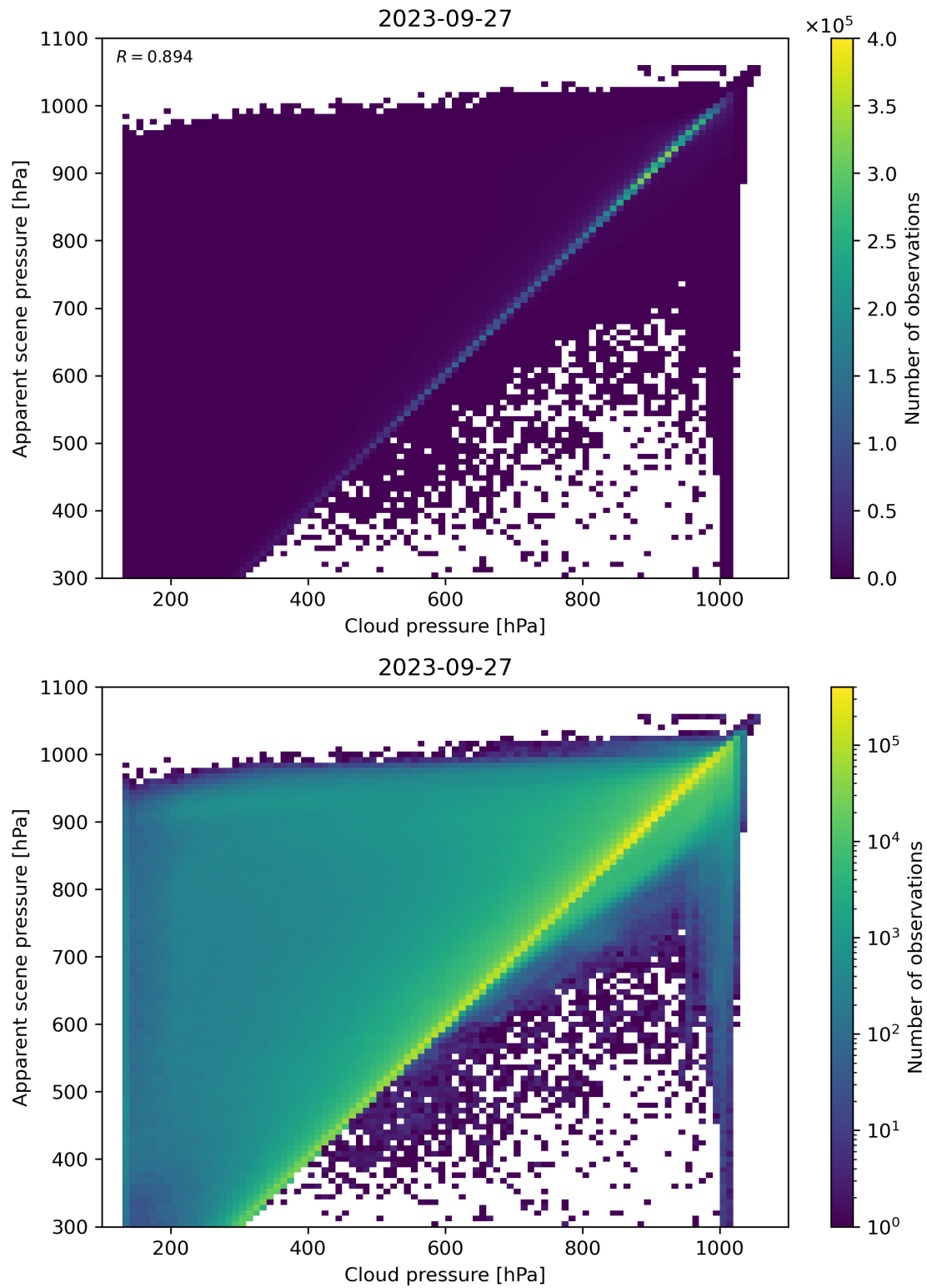
Figure 84: Scatter density plot of “Cloud pressure” against “Apparent scene pressure” for 2023-09-26 to 2023-09-28.
