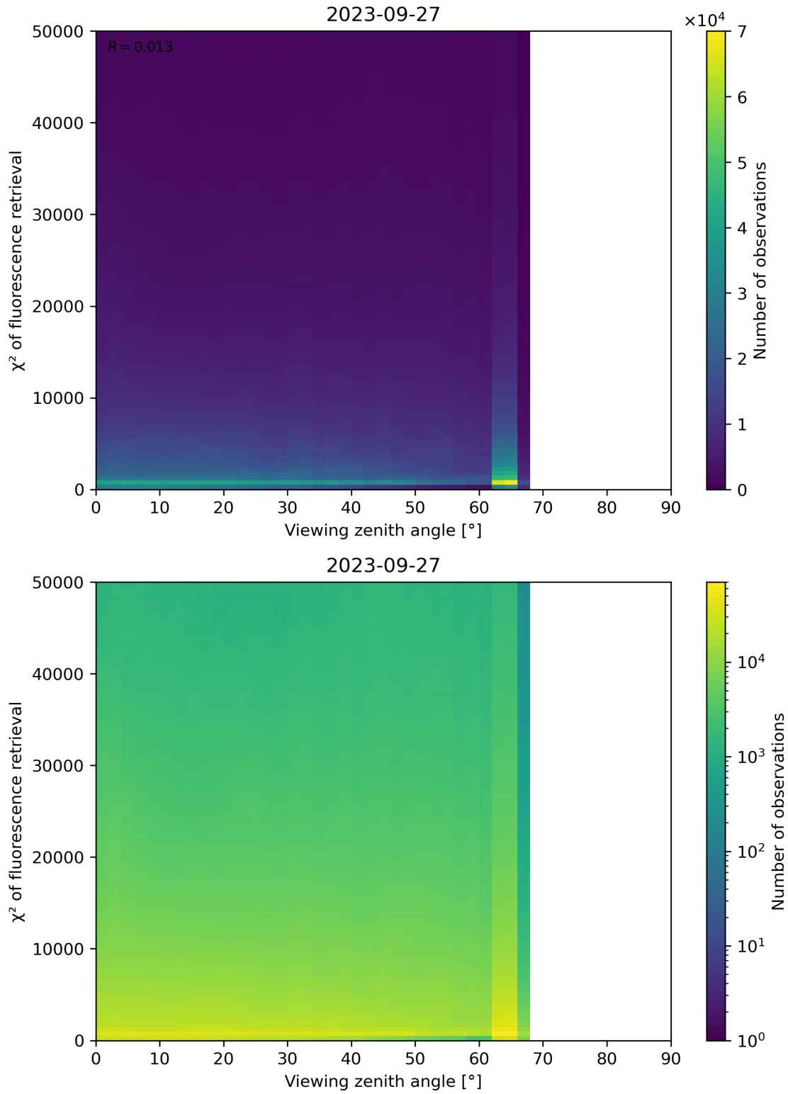
Figure 131: Scatter density plot of “Viewing zenith angle” against “ \chi^2 of fluorescence retrieval” for 2023-09-26 to 2023-09-28.
