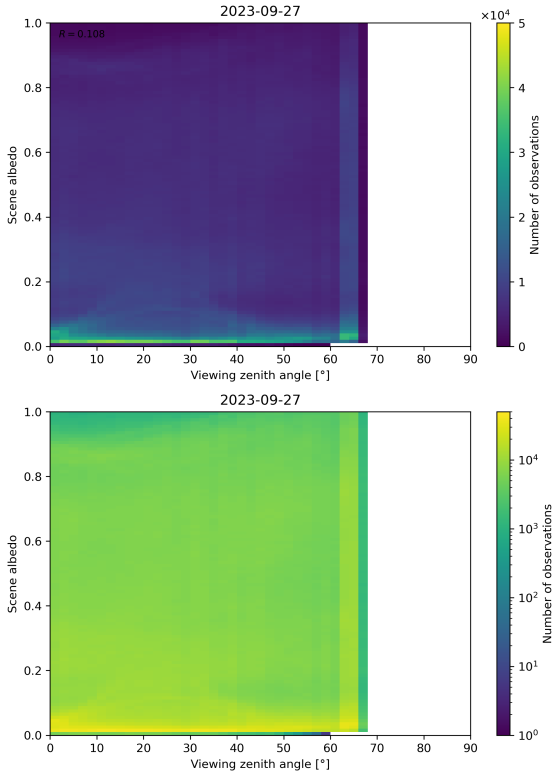
Figure 138: Scatter density plot of “Viewing zenith angle” against “Scene albedo” for 2023-09-26 to 2023-09-28.
