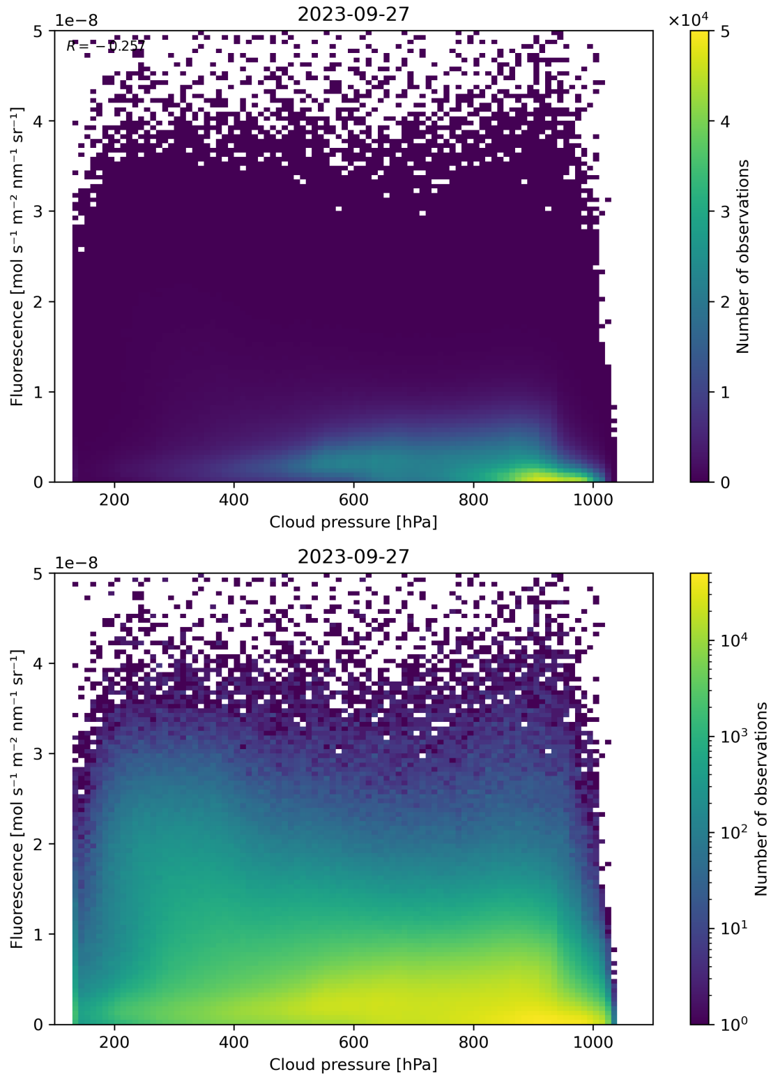
Figure 88: Scatter density plot of “Cloud pressure” against “Fluorescence” for 2023-09-26 to 2023-09-28.
