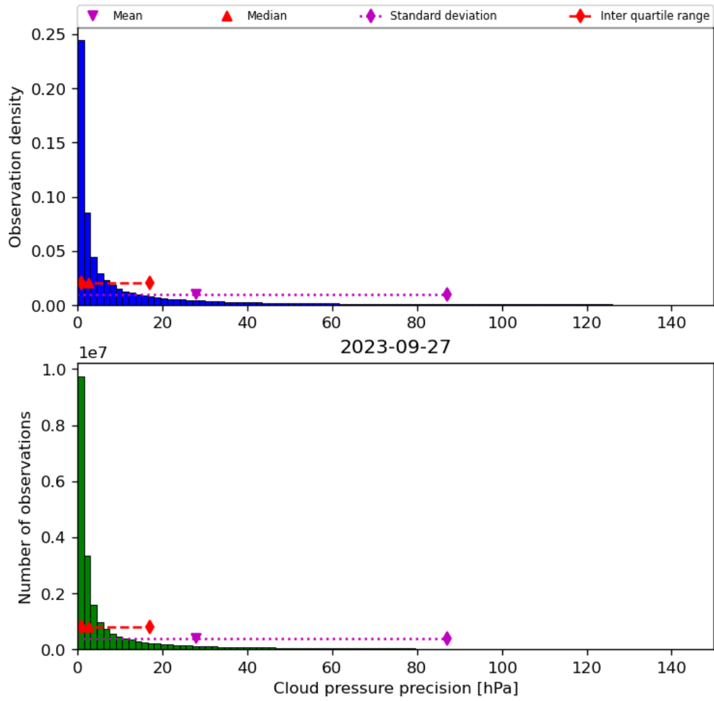
Figure 31: Histogram of “Cloud pressure precision” for 2023-09-26 to 2023-09-28
