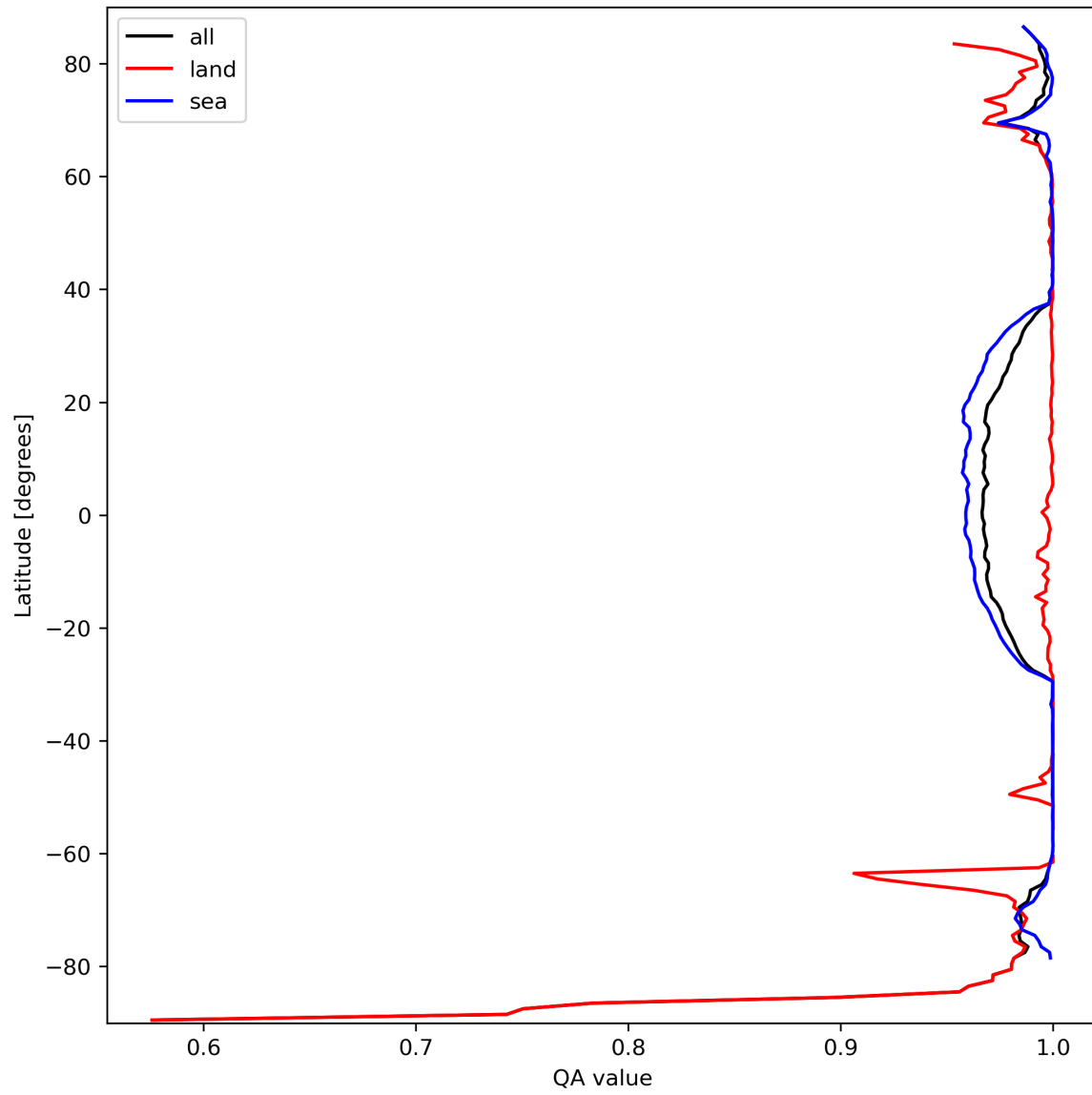
Figure 12: Zonal average of “QA value” for 2023-09-26 to 2023-09-28.
