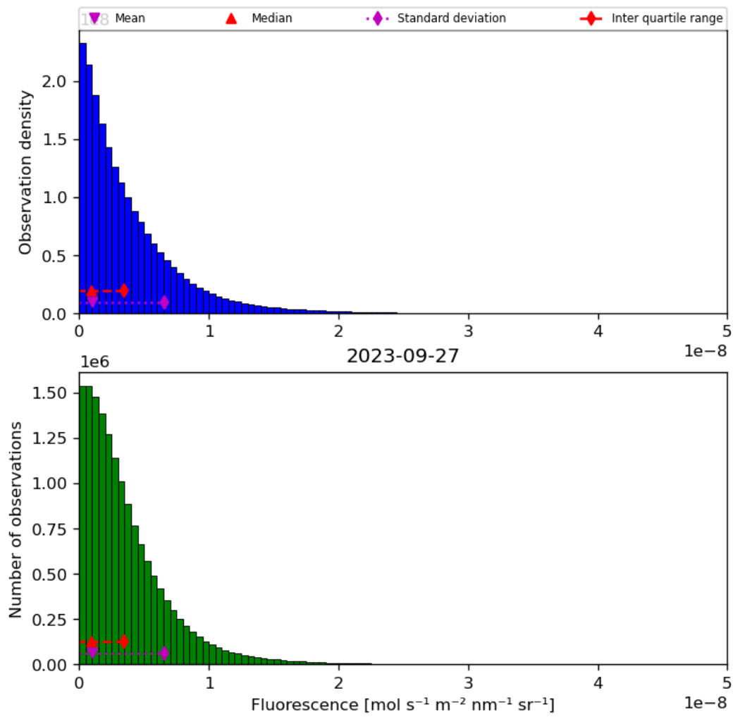
Figure 40: Histogram of “Fluorescence” for 2023-09-26 to 2023-09-28
