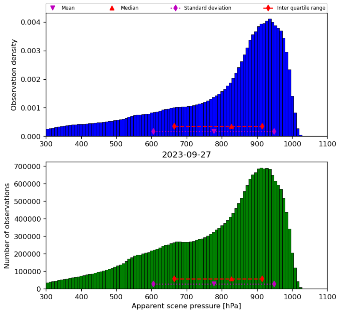
Figure 36: Histogram of “Apparent scene pressure” for 2023-09-26 to 2023-09-28
