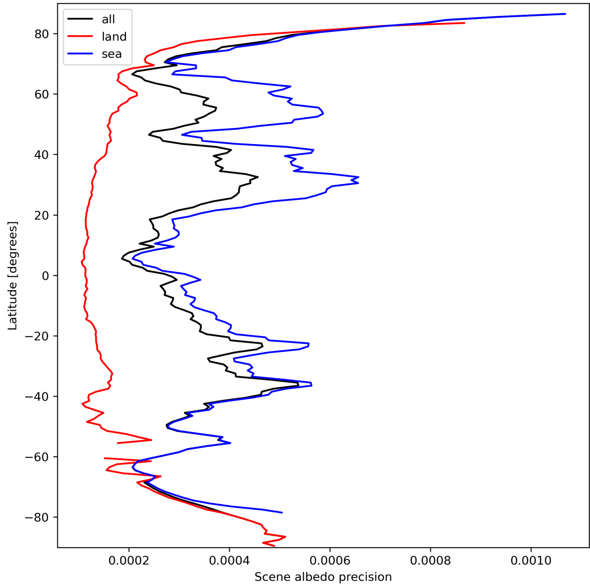
Figure 18: Zonal average of “Scene albedo precision” for 2023-09-26 to 2023-09-28.
