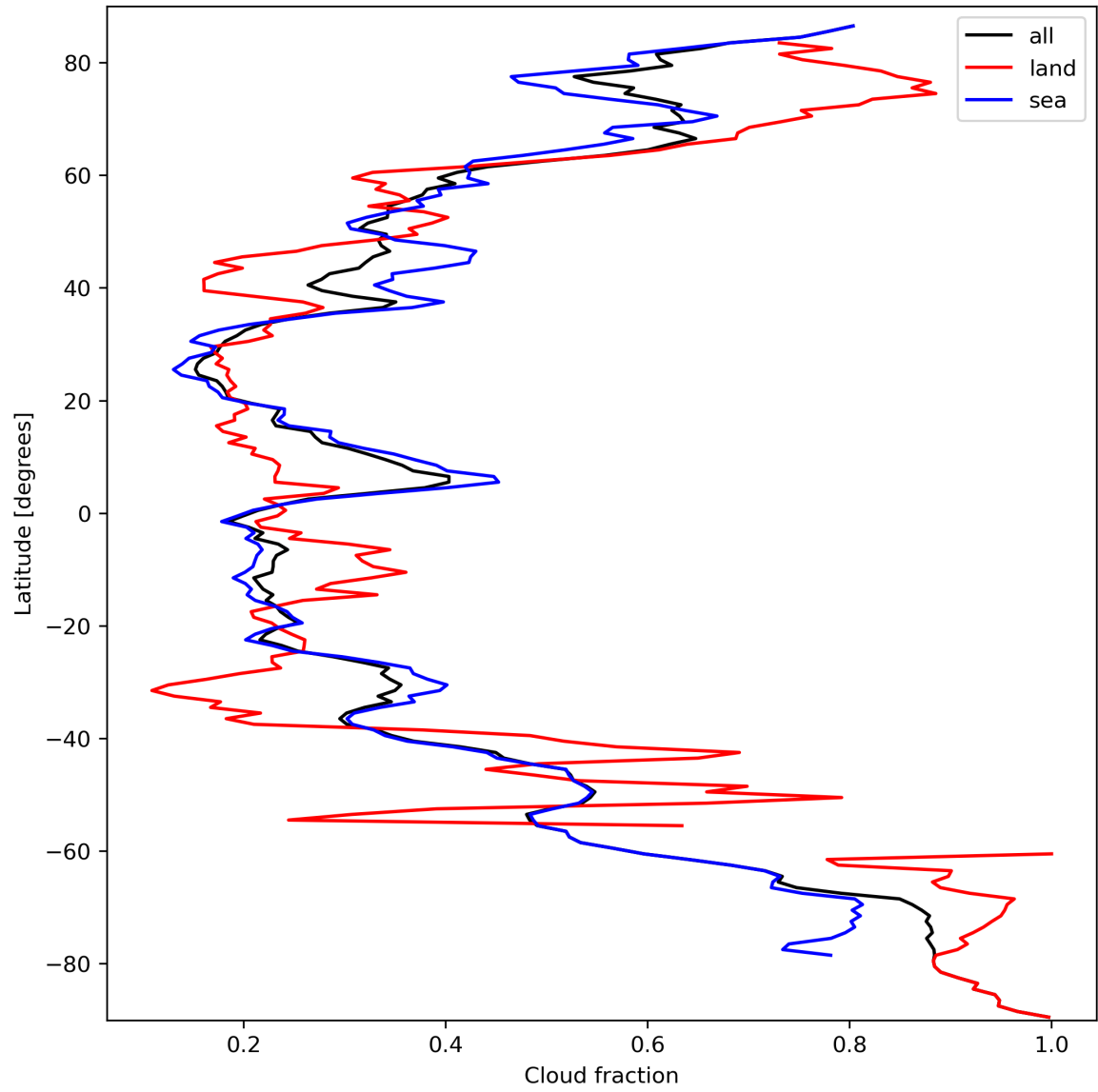
Figure 15: Zonal average of “Cloud fraction” for 2023-09-26 to 2023-09-28.
