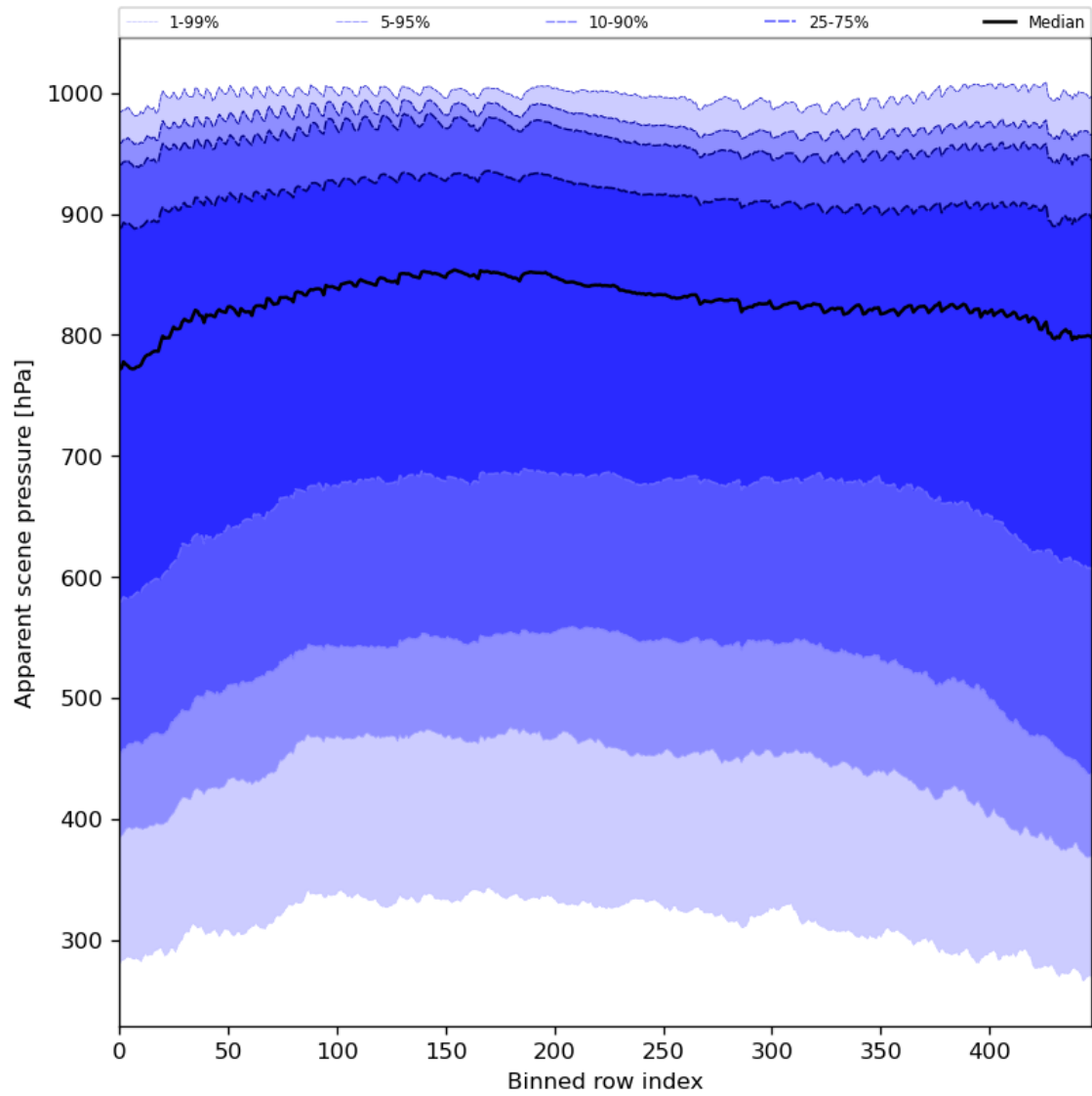
Figure 53: Along track statistics of “Apparent scene pressure” for 2023-09-26 to 2023-09-28
