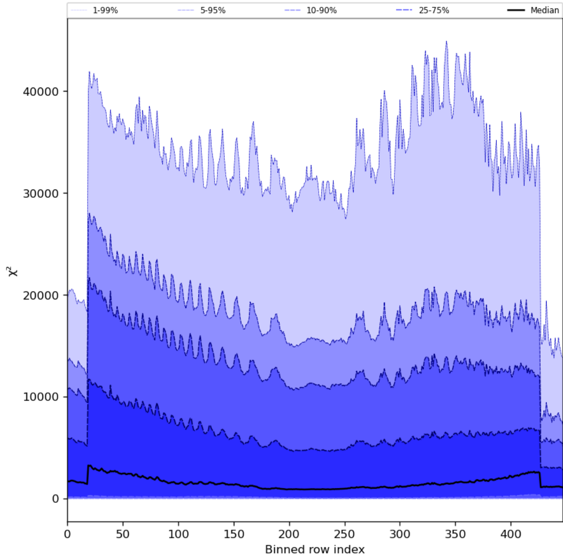
Figure 55: Along track statistics of " \chi^2 " for 2023-09-26 to 2023-09-28
