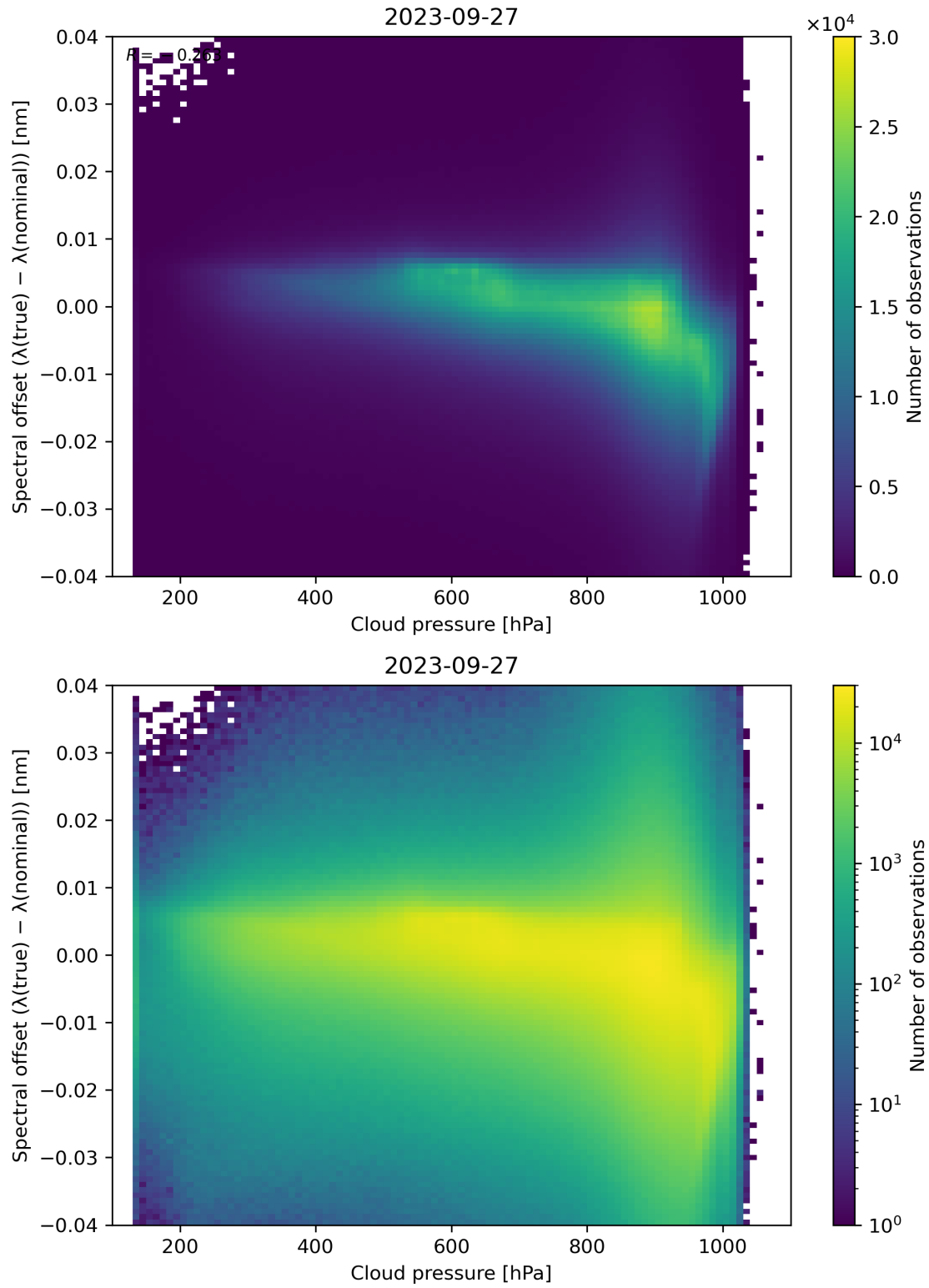
Figure 92: Scatter density plot of “Cloud pressure” against “Spectral offset ( \lambda(\text{true}) - \lambda(\text{nominal}) )” for 2023-09-26 to 2023-09-28.
