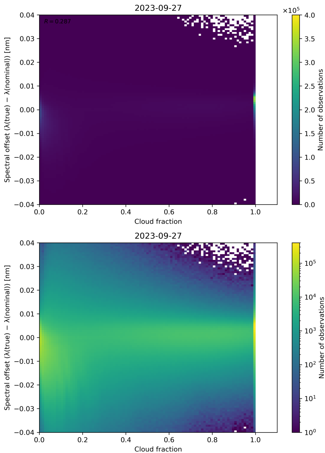
Figure 83: Scatter density plot of “Cloud fraction” against “Spectral offset ( \lambda(\text{true}) - \lambda(\text{nominal}) )” for 2023-09-26 to 2023-09-28.
