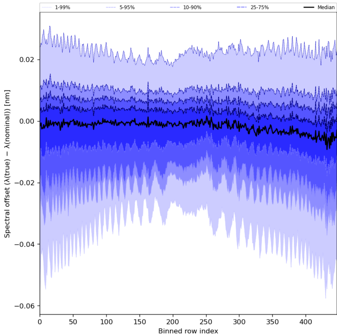
Figure 62: Along track statistics of “Spectral offset ( \lambda(\text{true}) - \lambda(\text{nominal}) )” for 2023-09-26 to 2023-09-28
