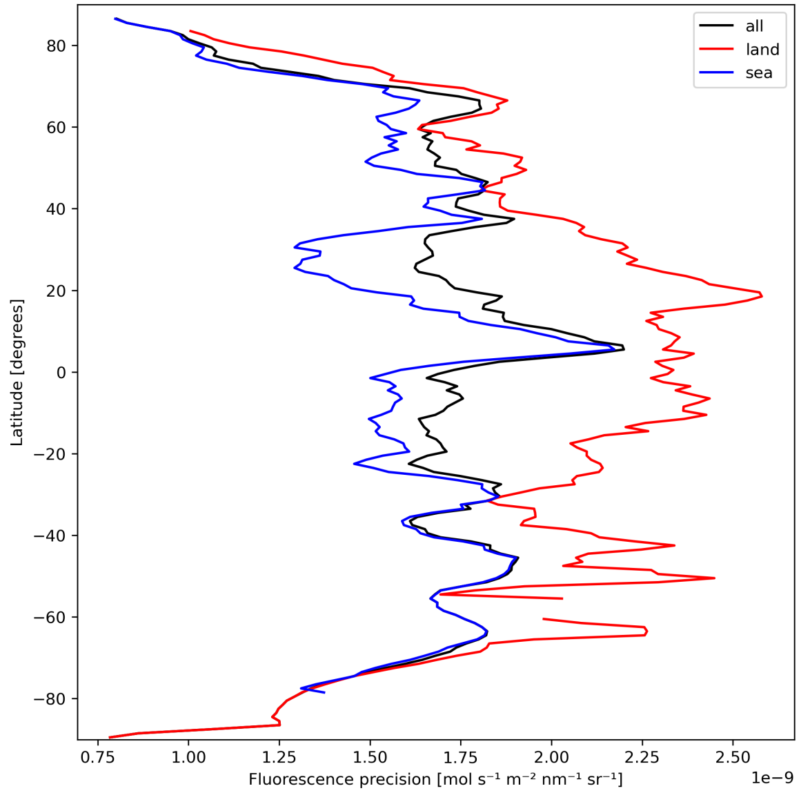
Figure 24: Zonal average of “Fluorescence precision” for 2023-09-26 to 2023-09-28.
