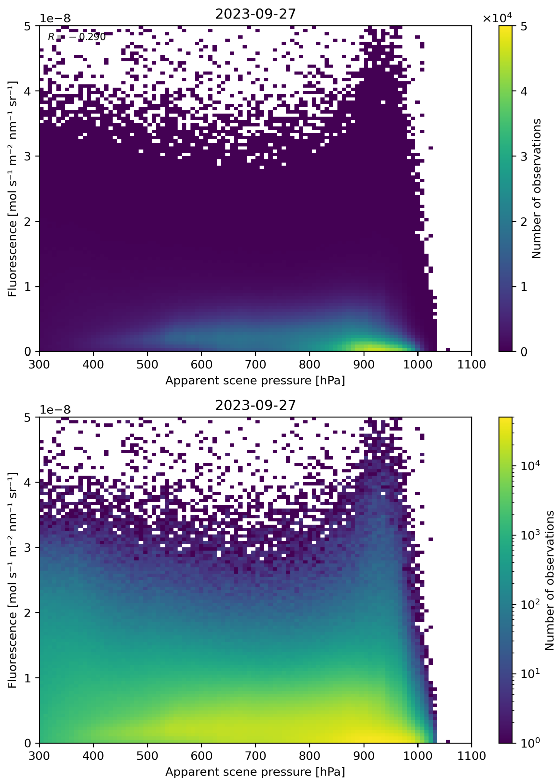
Figure 65: Scatter density plot of “Apparent scene pressure” against “Fluorescence” for 2023-09-26 to 2023-09-28.
