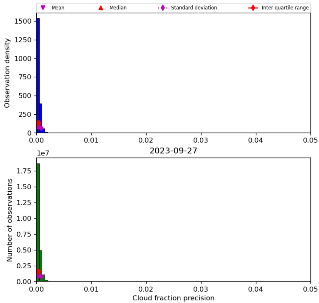
Figure 33: Histogram of “Cloud fraction precision” for 2023-09-26 to 2023-09-28
