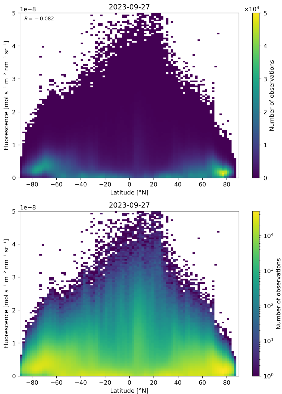
Figure 101: Scatter density plot of “Latitude” against “Fluorescence” for 2023-09-26 to 2023-09-28.
