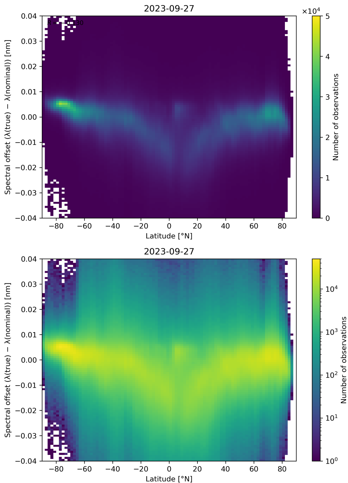
Figure 105: Scatter density plot of “Latitude” against “Spectral offset ( \lambda(\text{true}) - \lambda(\text{nominal}) )” for 2023-09-26 to 2023-09-28.
