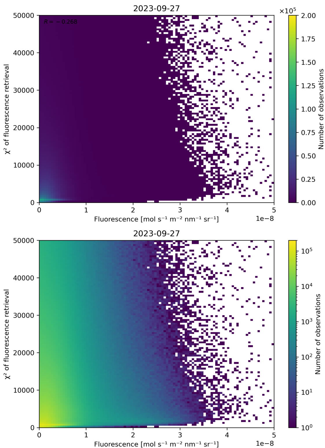
Figure 93: Scatter density plot of “Fluorescence” against “ \chi^2 of fluorescence retrieval” for 2023-09-26 to 2023-09-28.
