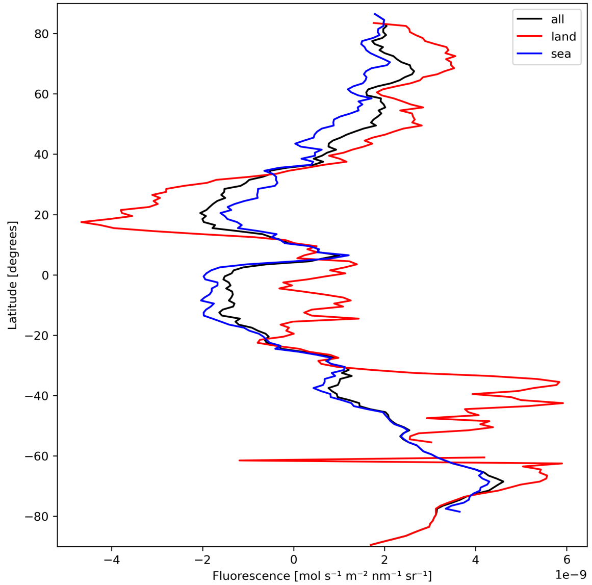
Figure 23: Zonal average of “Fluorescence” for 2023-09-26 to 2023-09-28.
