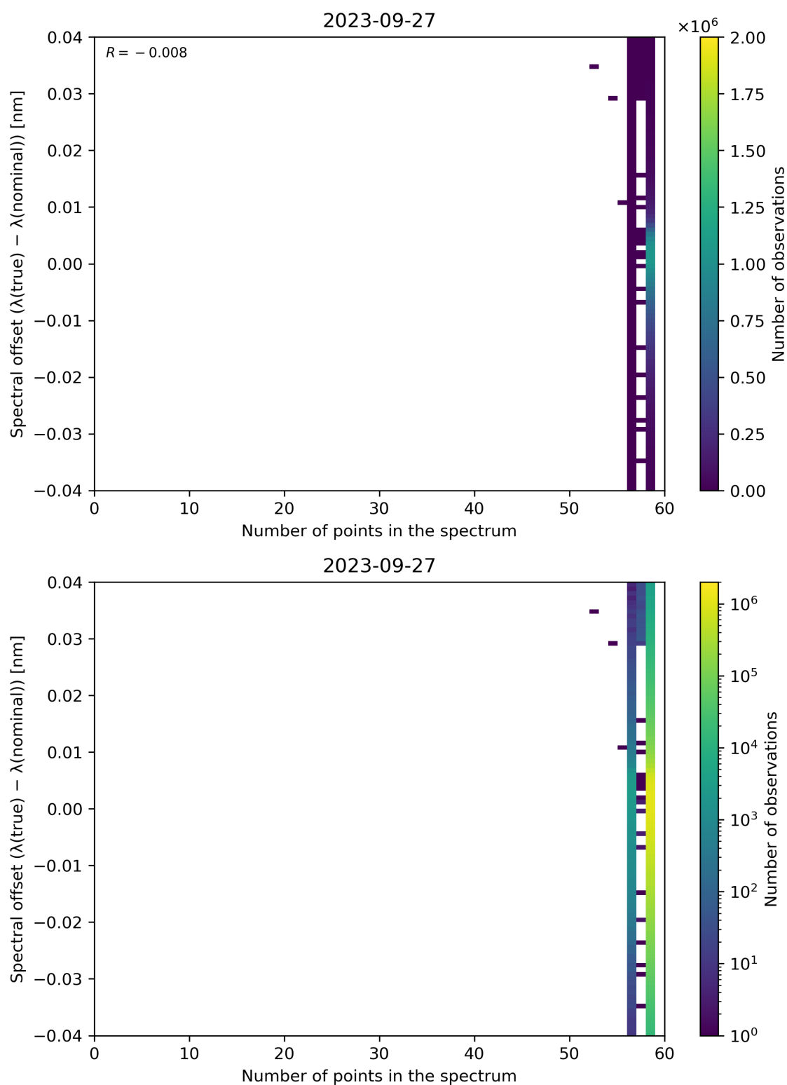
Figure 110: Scatter density plot of “Number of points in the spectrum” against “Spectral offset ( \lambda(\text{true}) - \lambda(\text{nominal}) )” for 2023-09-26 to 2023-09-28.
