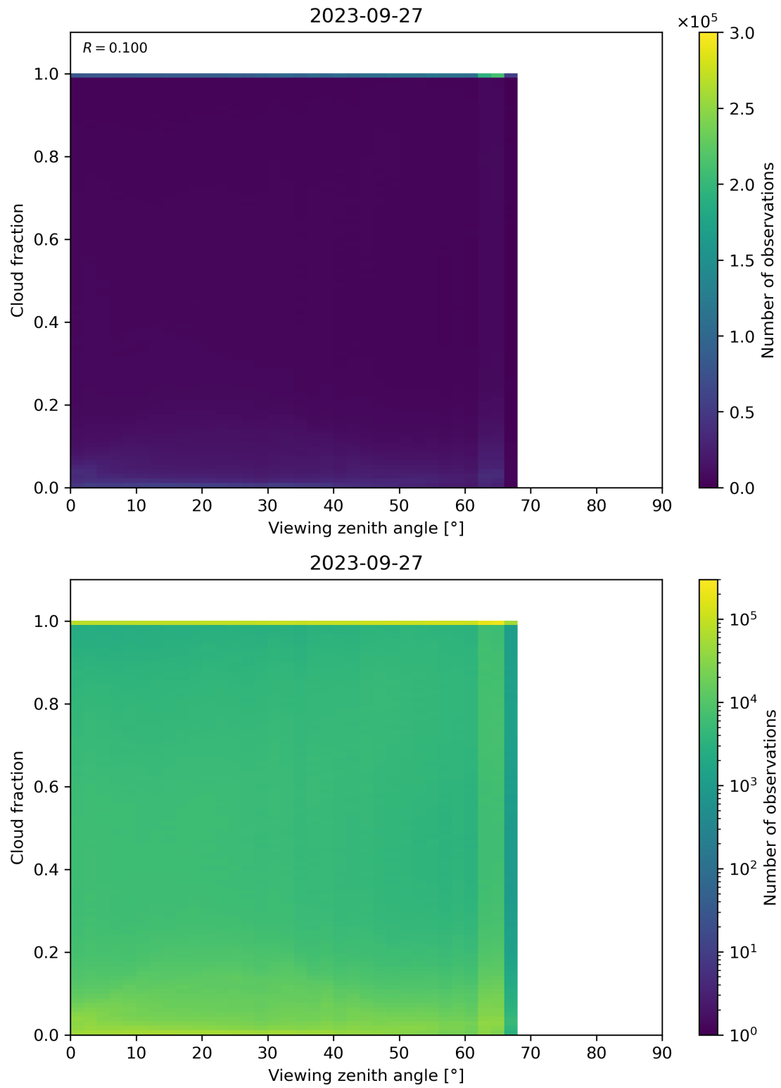
Figure 132: Scatter density plot of “Viewing zenith angle” against “Cloud fraction” for 2023-09-26 to 2023-09-28.
