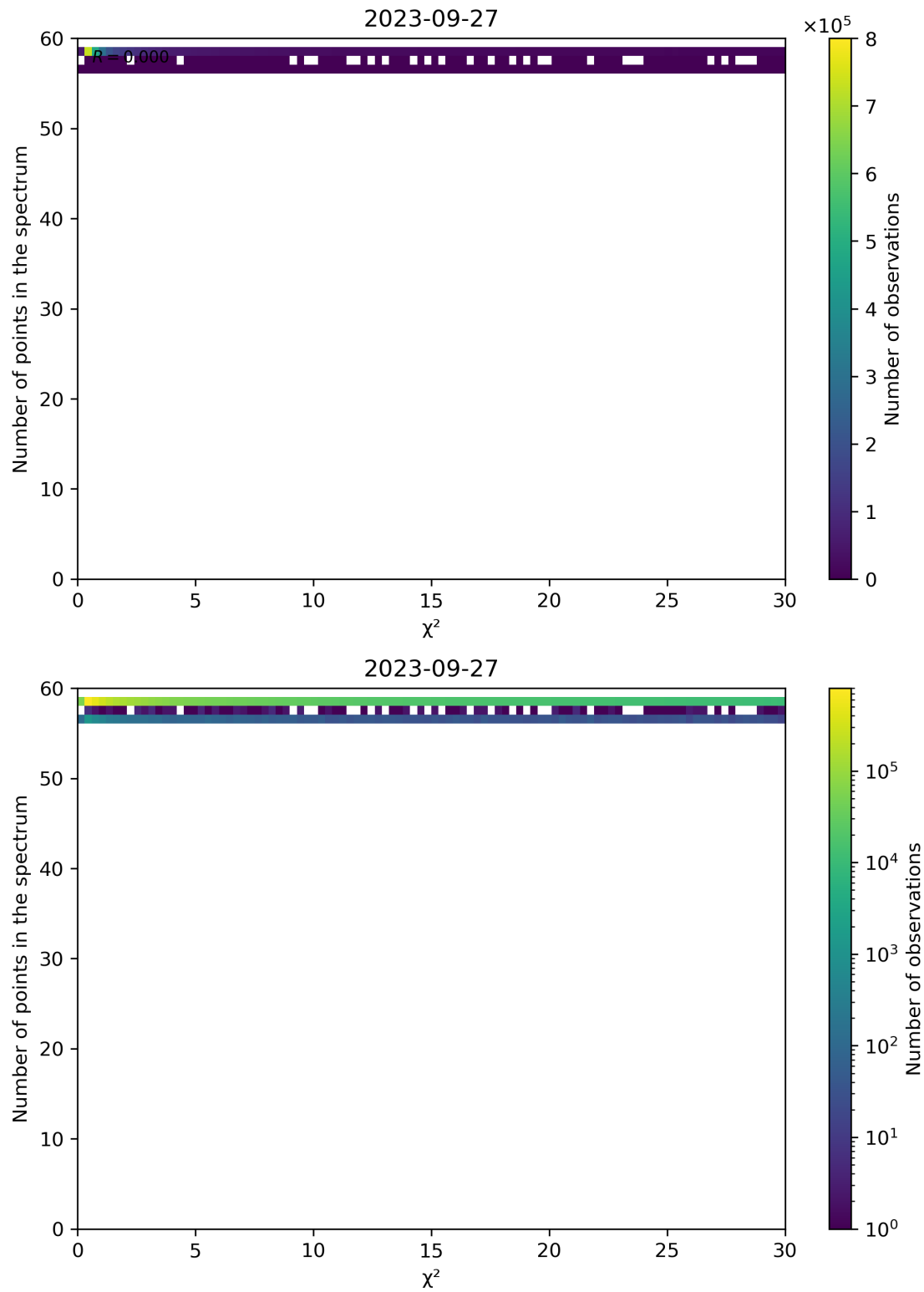
Figure 74: Scatter density plot of “ \chi^2 ” against “Number of points in the spectrum” for 2023-09-26 to 2023-09-28.
