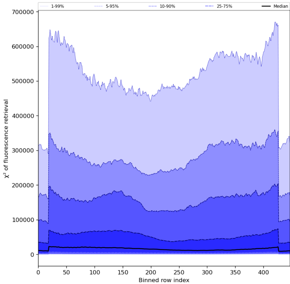
Figure 59: Along track statistics of “ \chi^2 of fluorescence retrieval” for 2023-09-26 to 2023-09-28
