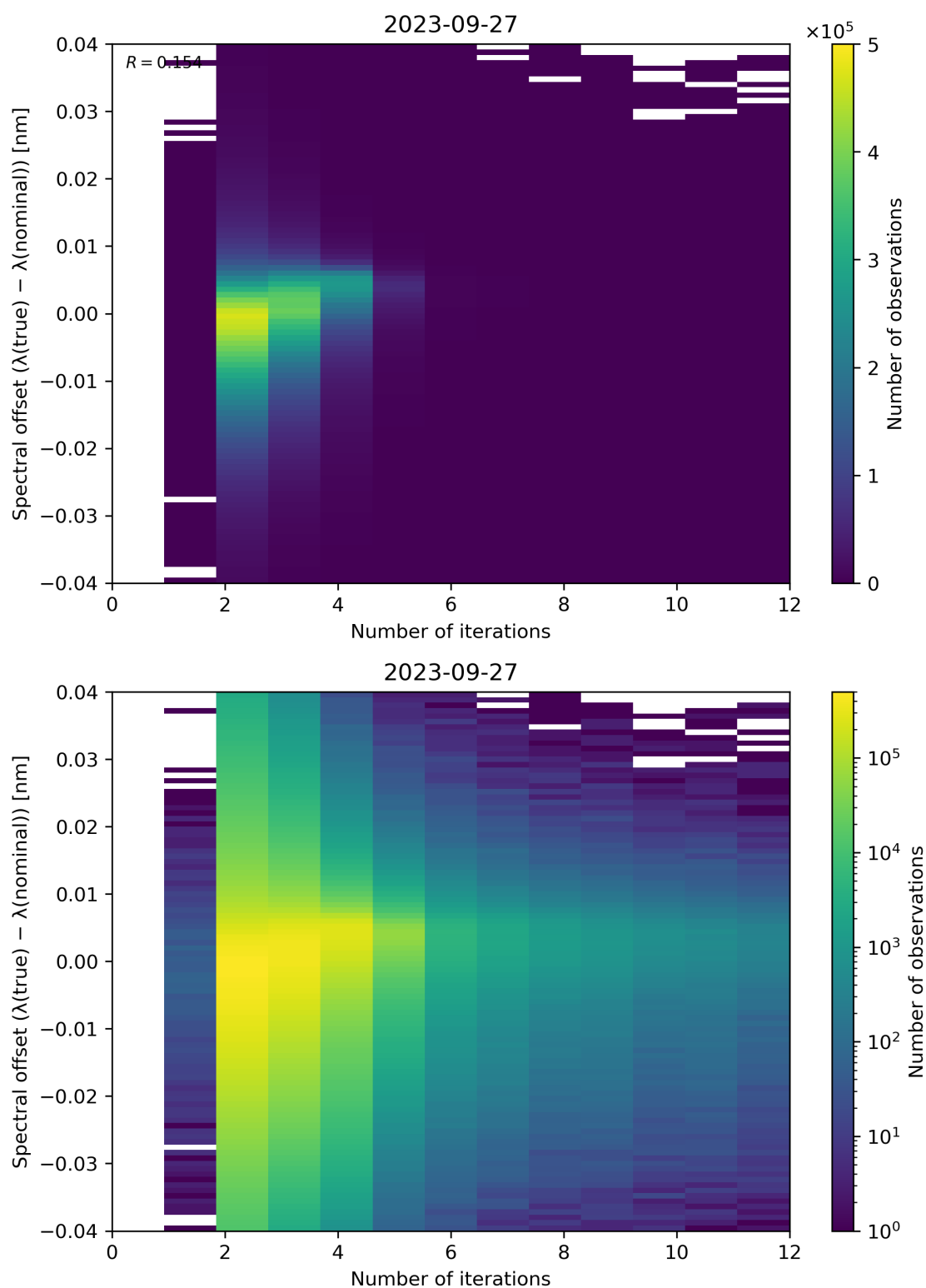
Figure 109: Scatter density plot of “Number of iterations” against “Spectral offset ( \lambda(\text{true}) - \lambda(\text{nominal}) )” for 2023-09-26 to 2023-09-28.
