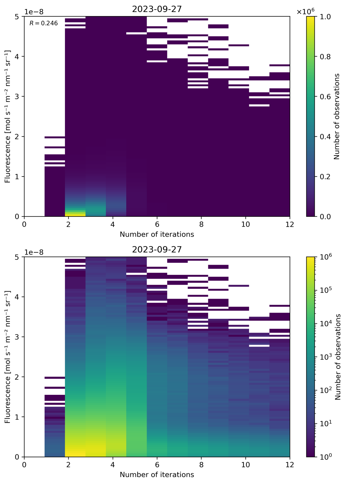
Figure 107: Scatter density plot of “Number of iterations” against “Fluorescence” for 2023-09-26 to 2023-09-28.
