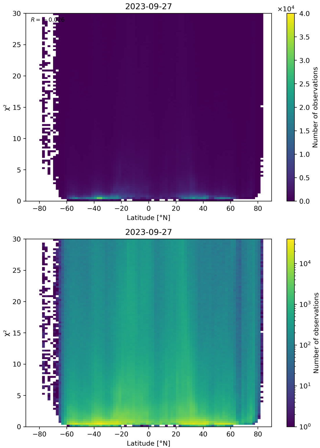
Figure 97: Scatter density plot of “Latitude” against “ \chi^2 ” for 2023-09-26 to 2023-09-28.
