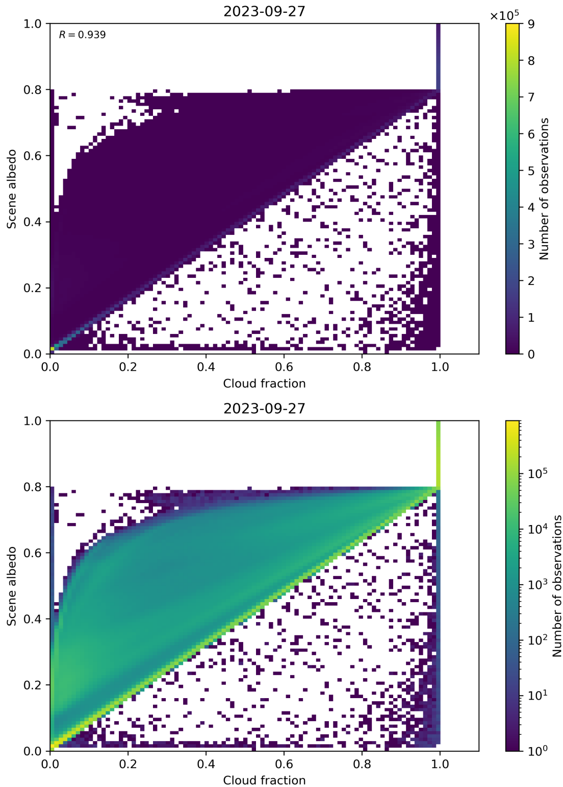
Figure 82: Scatter density plot of “Cloud fraction” against “Scene albedo” for 2023-09-26 to 2023-09-28.
