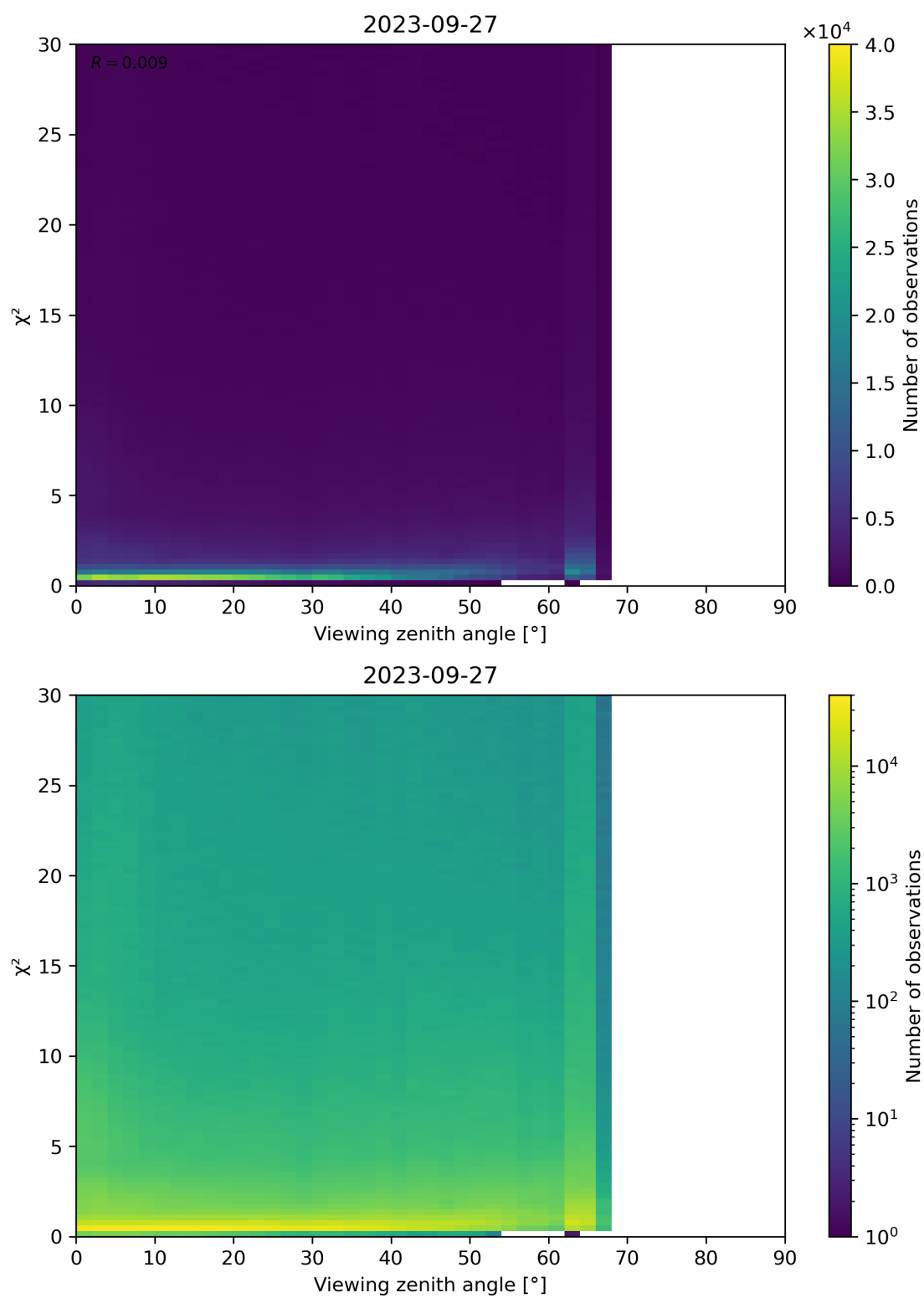
Figure 130: Scatter density plot of “Viewing zenith angle” against “ \chi^2 ” for 2023-09-26 to 2023-09-28.
