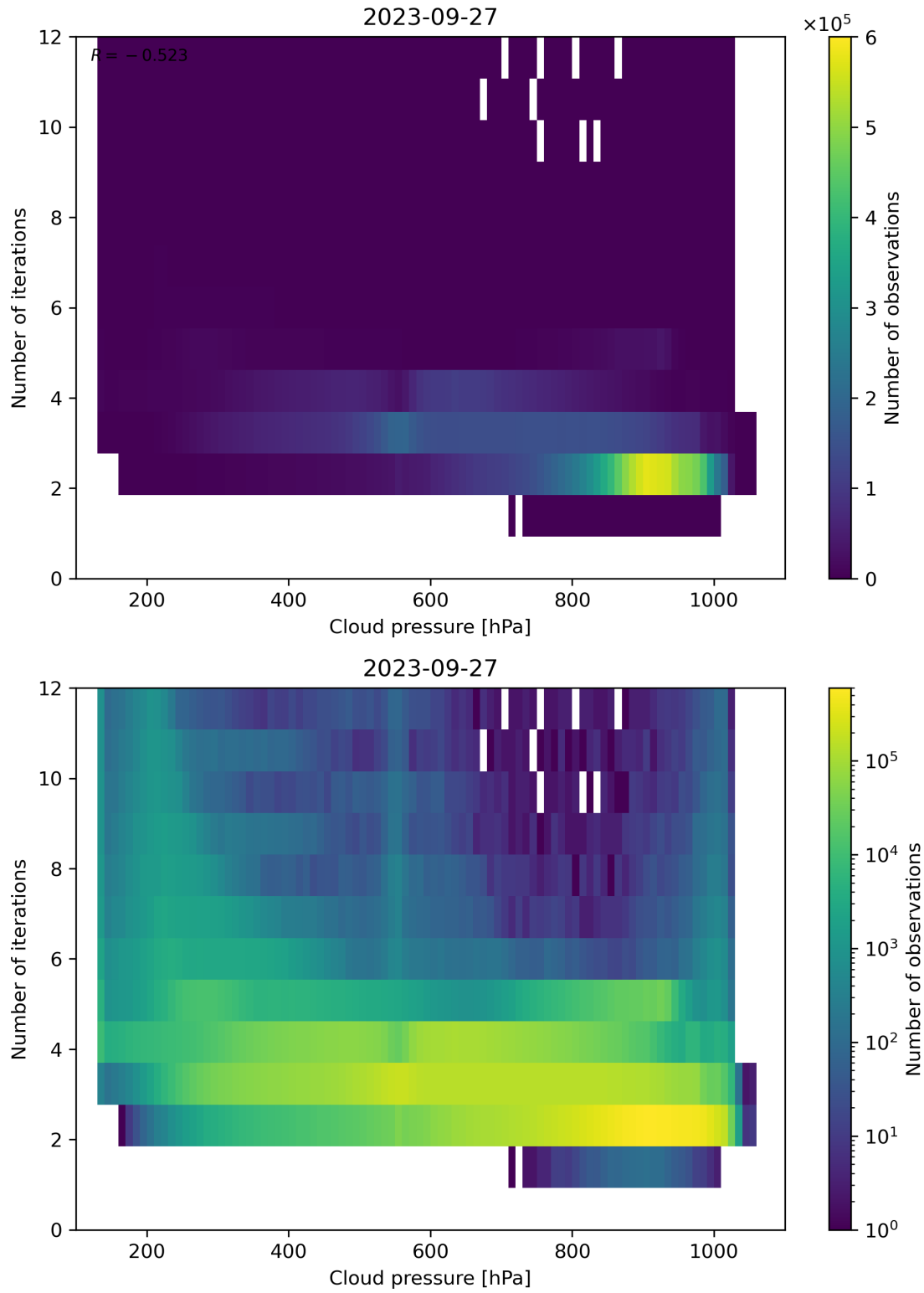
Figure 89: Scatter density plot of “Cloud pressure” against “Number of iterations” for 2023-09-26 to 2023-09-28.
