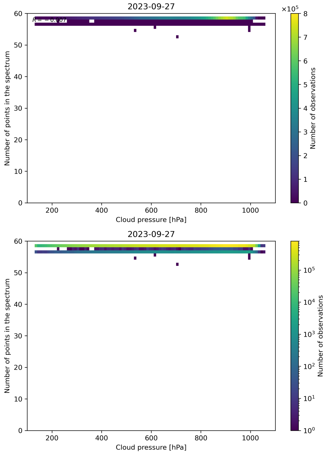
Figure 90: Scatter density plot of “Cloud pressure” against “Number of points in the spectrum” for 2023-09-26 to 2023-09-28.
