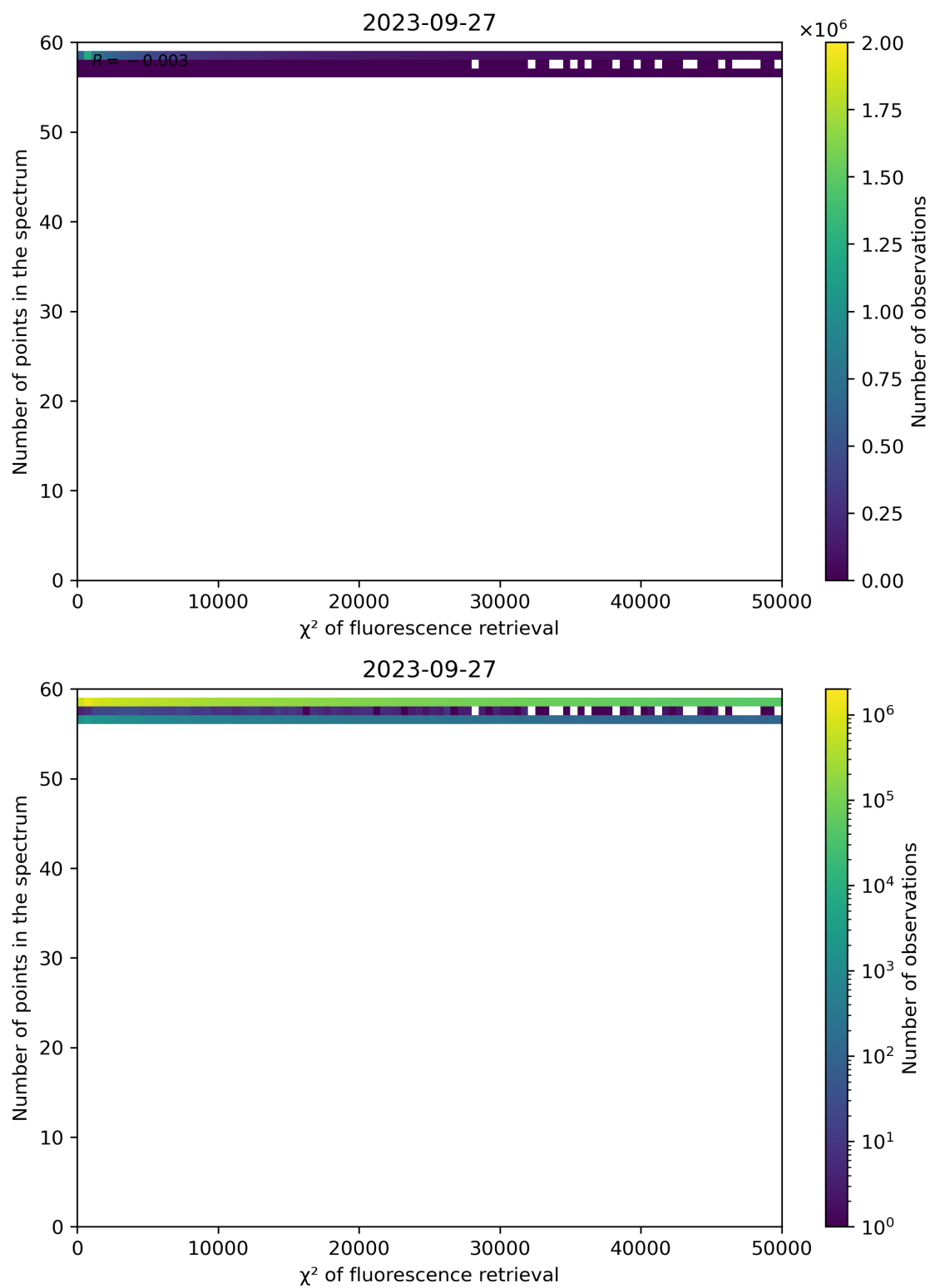
Figure 71: Scatter density plot of “ \chi^2 of fluorescence retrieval” against “Number of points in the spectrum” for 2023-09-26 to 2023-09-28.
