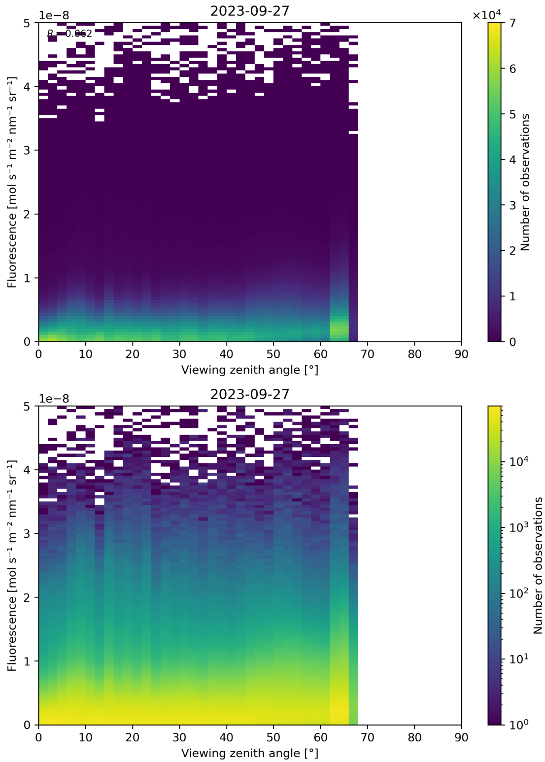
Figure 134: Scatter density plot of “Viewing zenith angle” against “Fluorescence” for 2023-09-26 to 2023-09-28.
