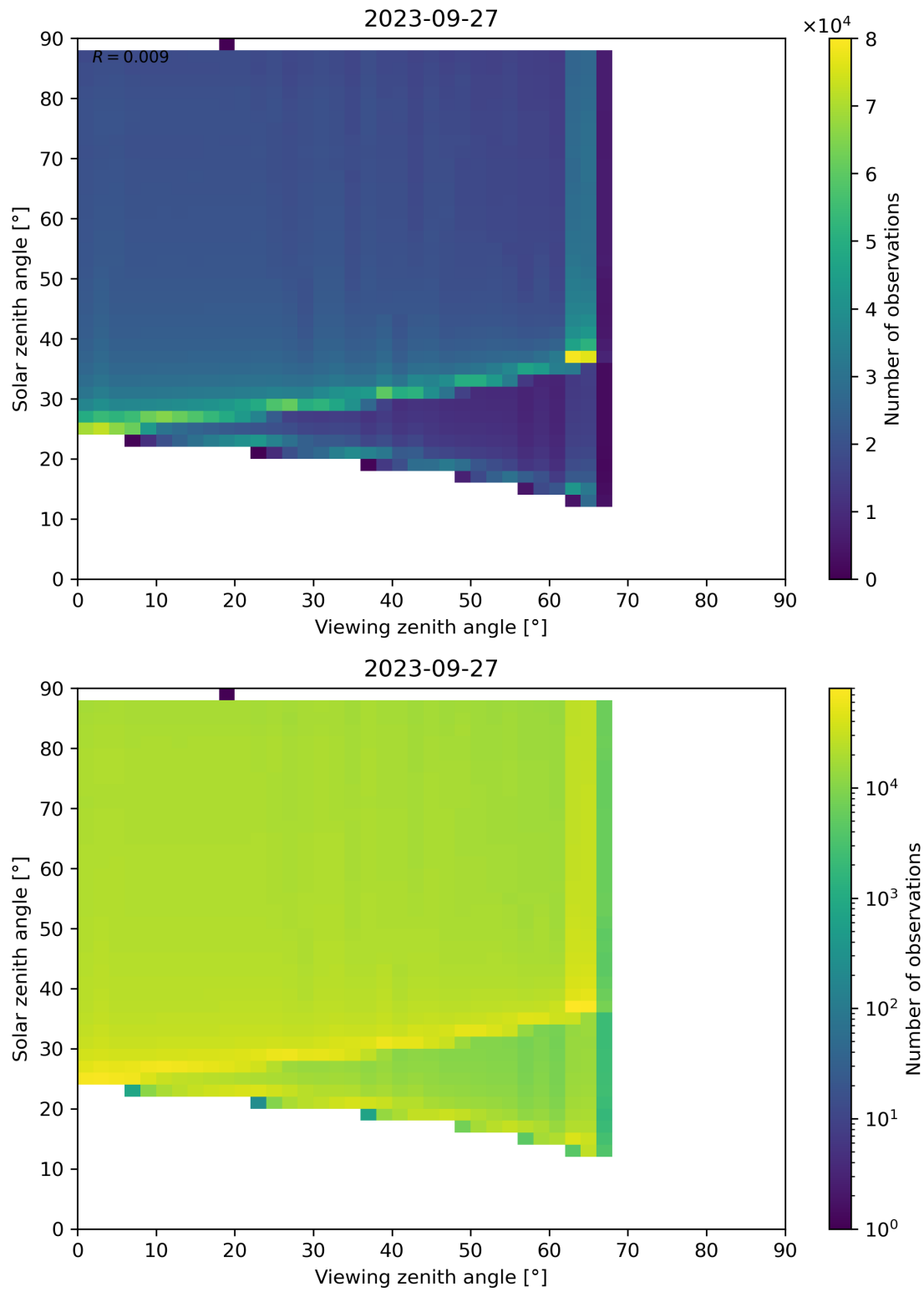
Figure 139: Scatter density plot of “Viewing zenith angle” against “Solar zenith angle” for 2023-09-26 to 2023-09-28.
