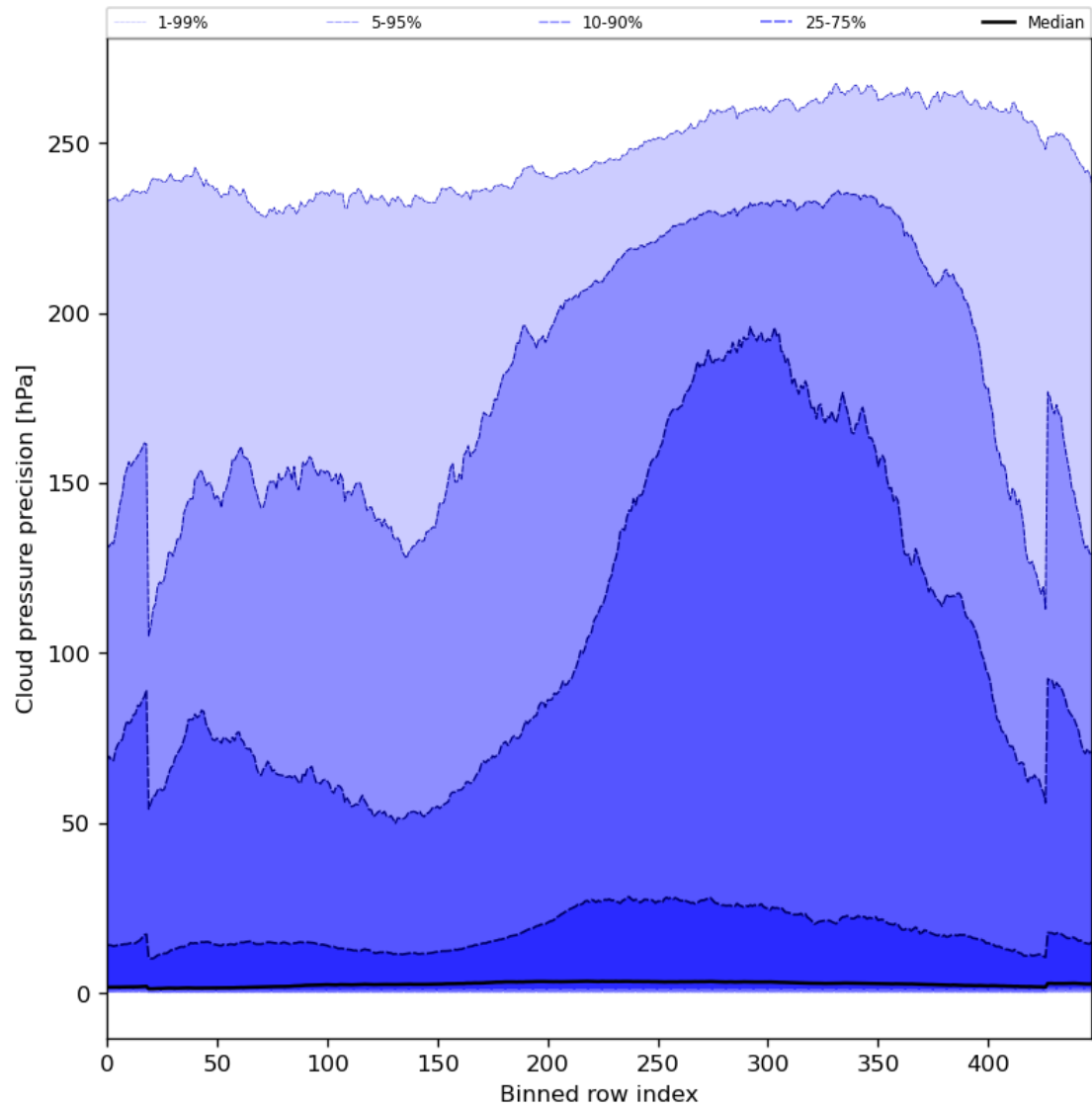
Figure 48: Along track statistics of “Cloud pressure precision” for 2023-09-26 to 2023-09-28
