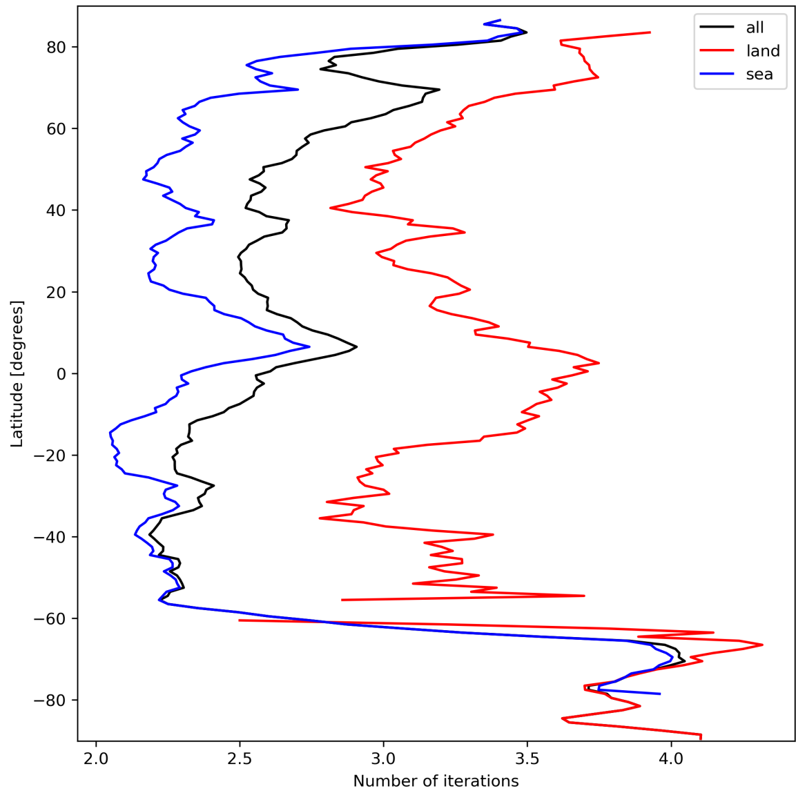
Figure 22: Zonal average of “Number of iterations” for 2023-09-26 to 2023-09-28.
