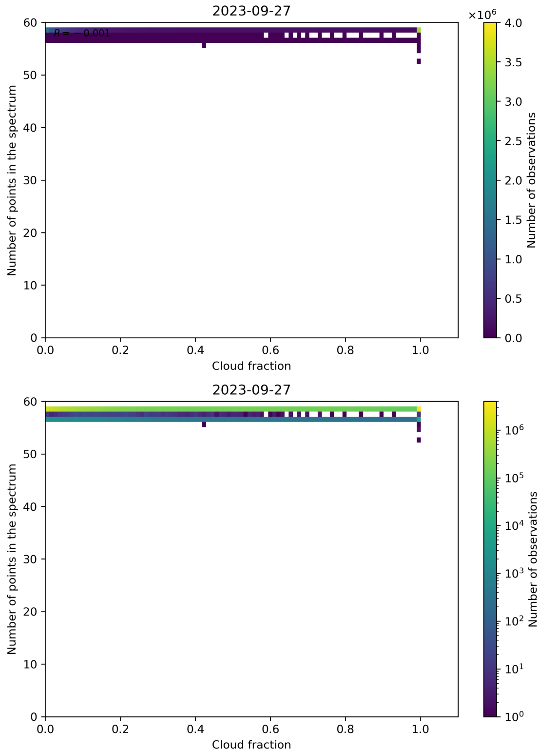
Figure 81: Scatter density plot of “Cloud fraction” against “Number of points in the spectrum” for 2023-09-26 to 2023-09-28.
