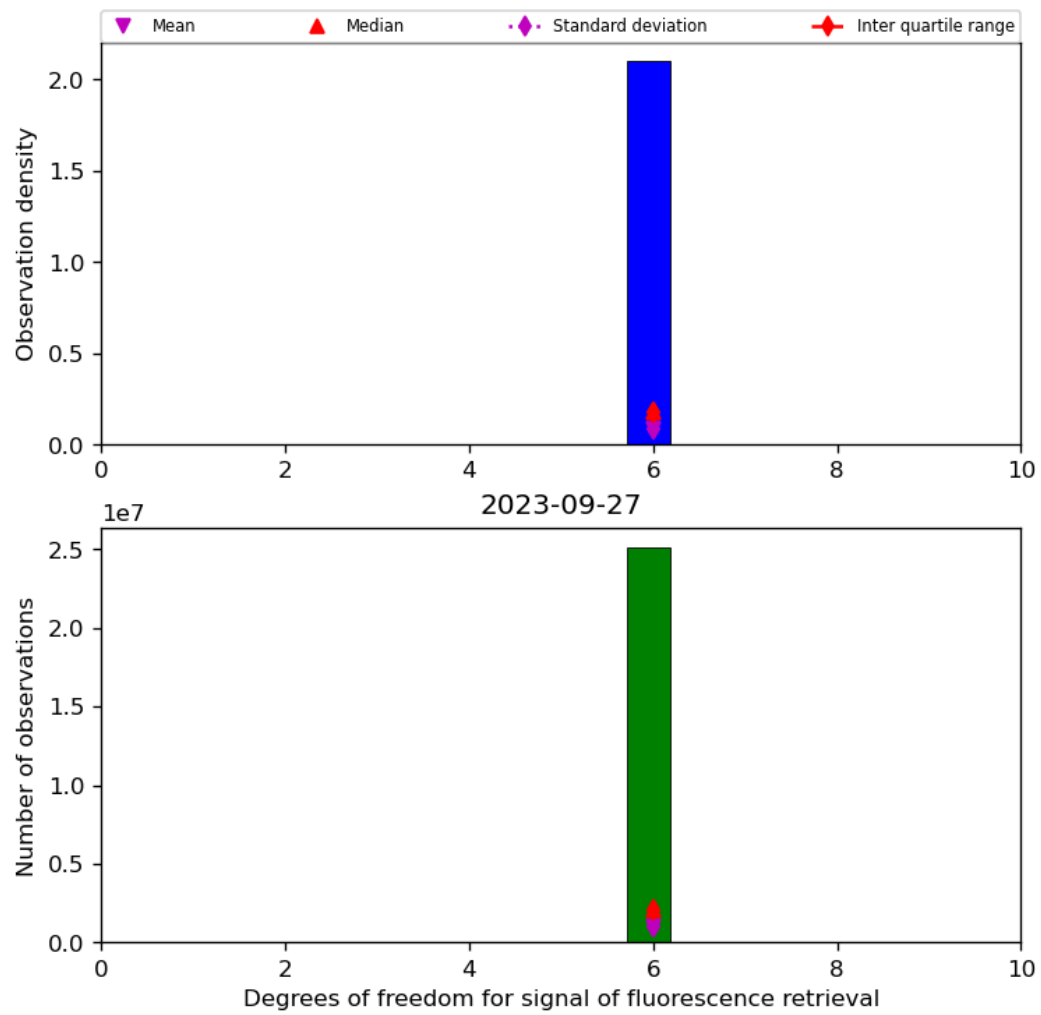
Figure 43: Histogram of “Degrees of freedom for signal of fluorescence retrieval” for 2023-09-26 to 2023-09-28
