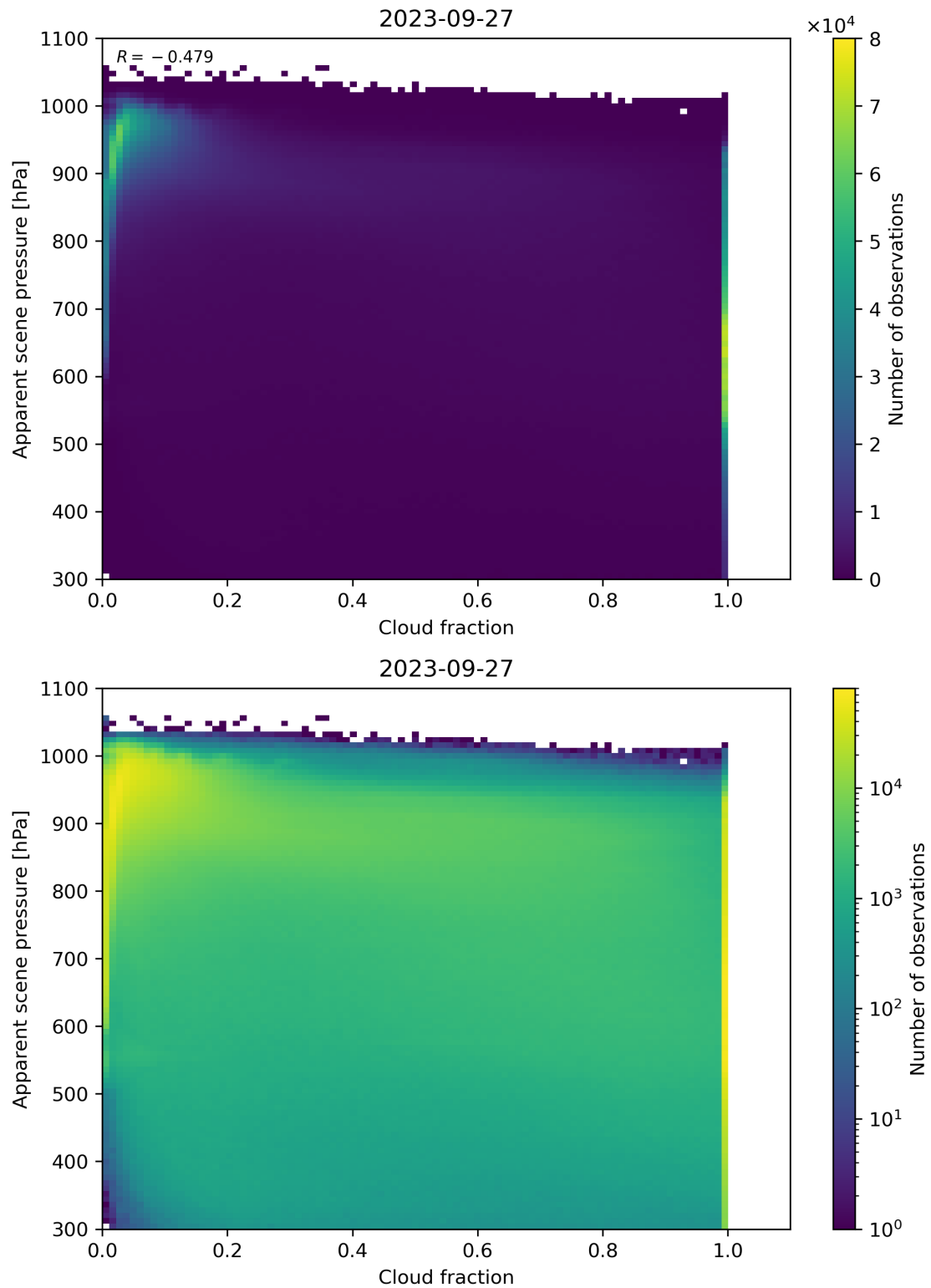
Figure 76: Scatter density plot of “Cloud fraction” against “Apparent scene pressure” for 2023-09-26 to 2023-09-28.
