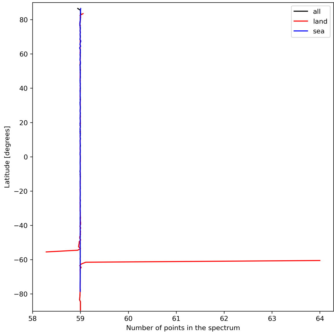
Figure 27: Zonal average of “Number of points in the spectrum” for 2023-09-26 to 2023-09-28.
