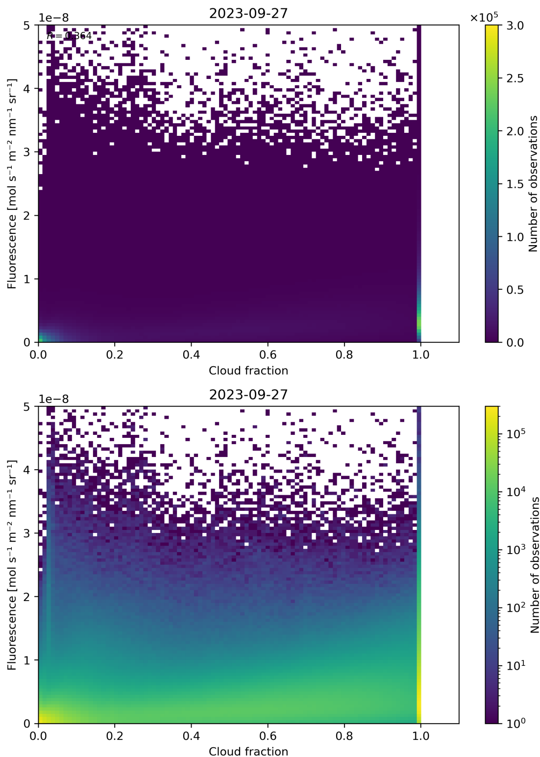
Figure 79: Scatter density plot of “Cloud fraction” against “Fluorescence” for 2023-09-26 to 2023-09-28.
