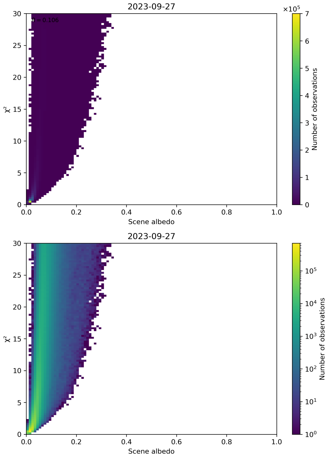
Figure 112: Scatter density plot of “Scene albedo” against “ \chi^2 ” for 2023-09-26 to 2023-09-28.
