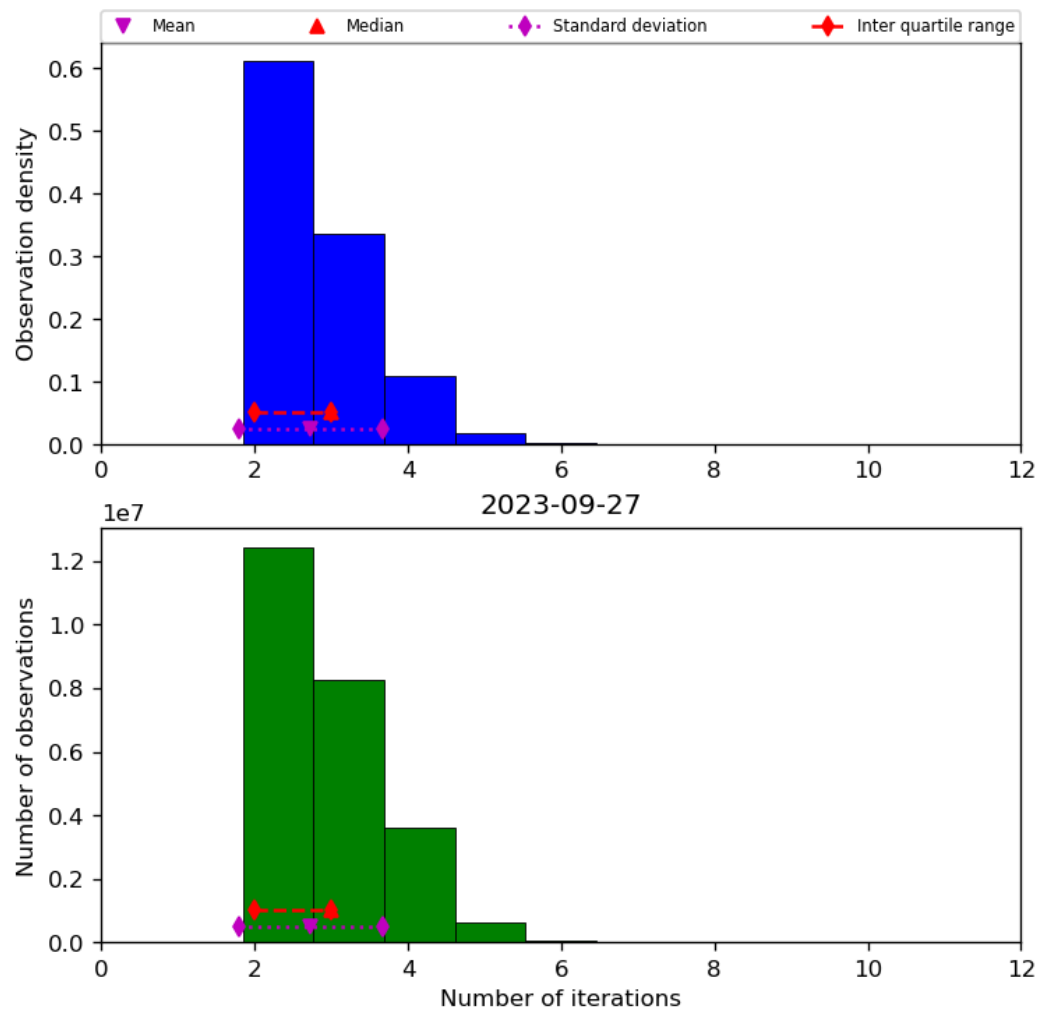
Figure 39: Histogram of “Number of iterations” for 2023-09-26 to 2023-09-28
