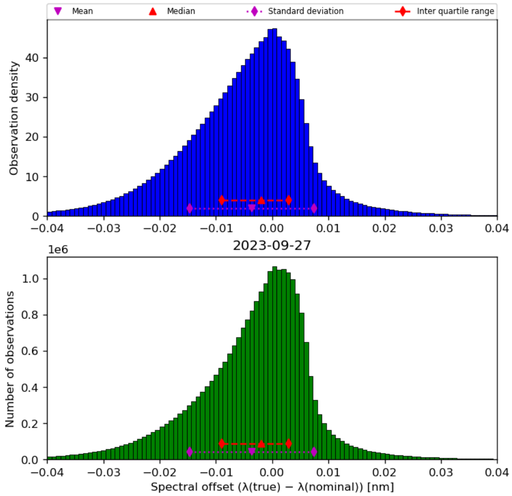
Figure 45: Histogram of “Spectral offset ( \lambda(\text{true}) - \lambda(\text{nominal}) )” for 2023-09-26 to 2023-09-28
