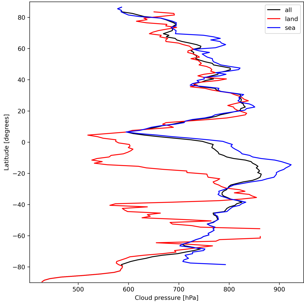
Figure 13: Zonal average of “Cloud pressure” for 2023-09-26 to 2023-09-28.
