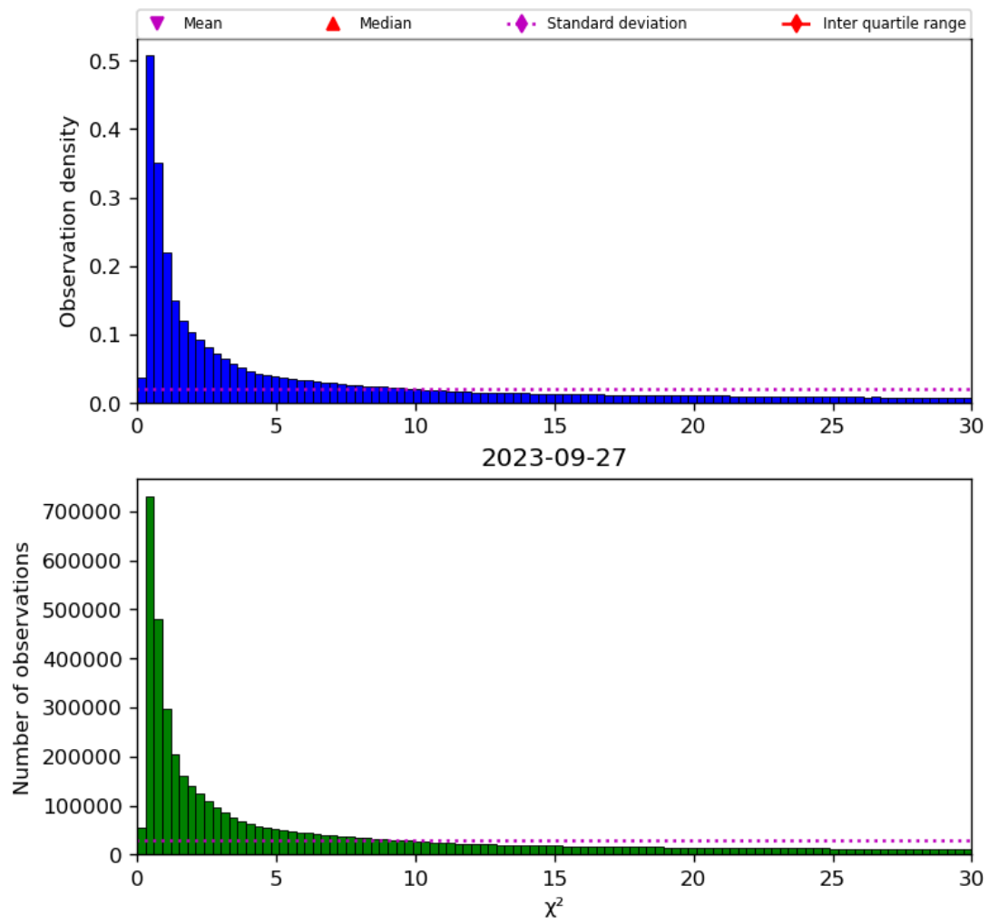
Figure 38: Histogram of " \chi^2 " for 2023-09-26 to 2023-09-28
