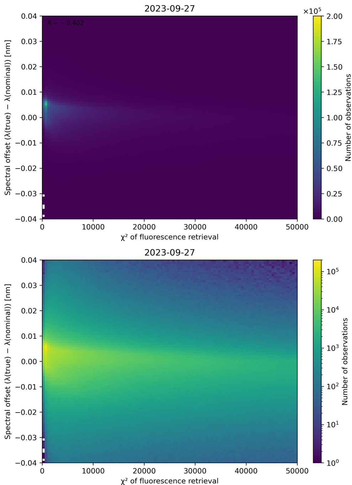
Figure 72: Scatter density plot of " \chi^2 of fluorescence retrieval" against "Spectral offset ( \lambda(\text{true}) - \lambda(\text{nominal})) " for 2023-09-26 to 2023-09-28.
