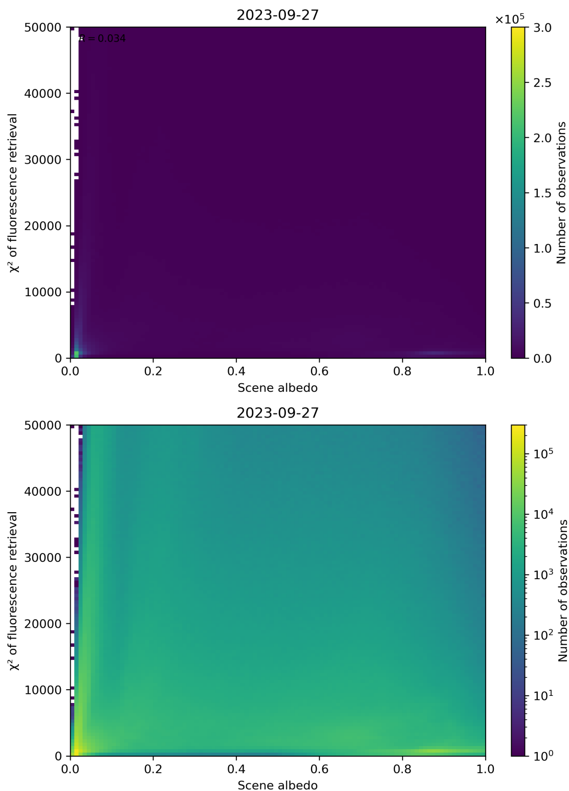
Figure 113: Scatter density plot of “Scene albedo” against “ \chi^2 of fluorescence retrieval” for 2023-09-26 to 2023-09-28.
