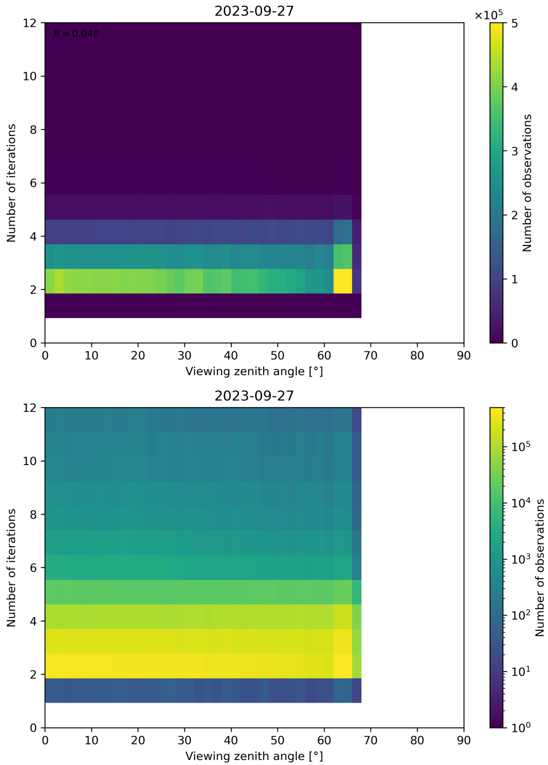
Figure 136: Scatter density plot of “Viewing zenith angle” against “Number of iterations” for 2023-09-26 to 2023-09-28.
