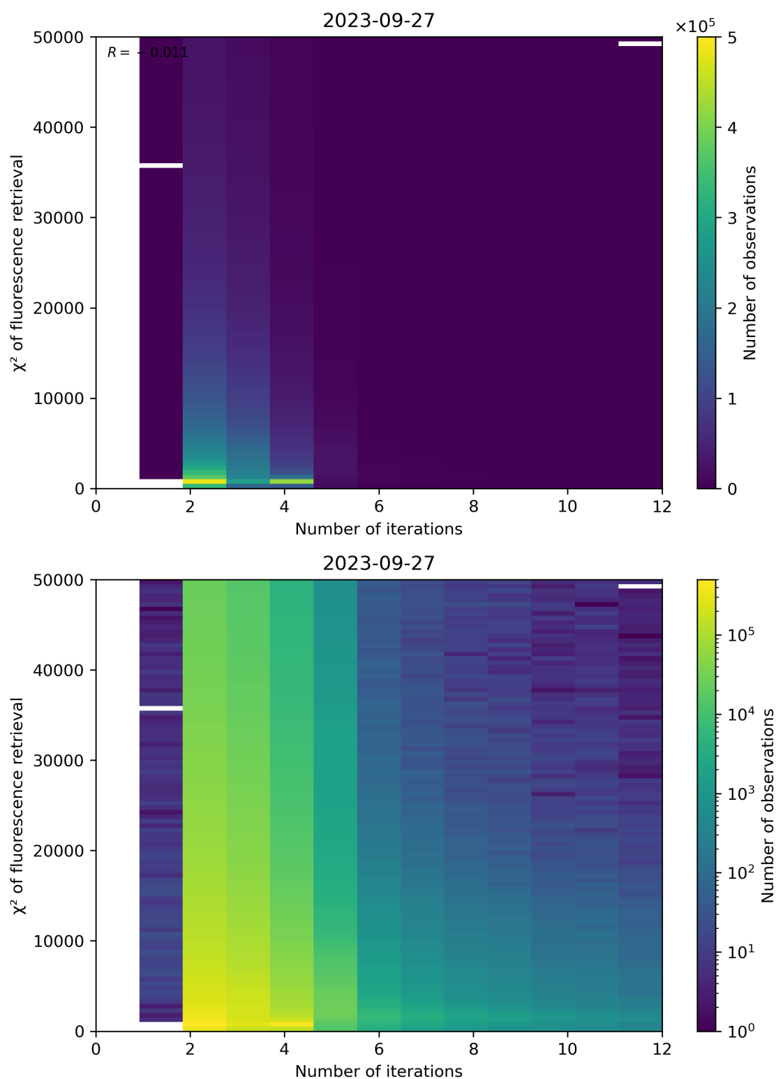
Figure 106: Scatter density plot of “Number of iterations” against “ \chi^2 of fluorescence retrieval” for 2023-09-26 to 2023-09-28.
