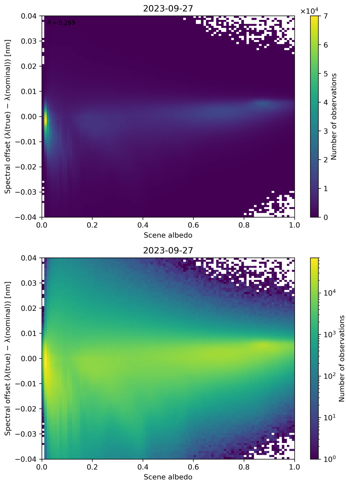
Figure 117: Scatter density plot of “Scene albedo” against “Spectral offset ( \lambda(\text{true}) - \lambda(\text{nominal}) )” for 2023-09-26 to 2023-09-28.
