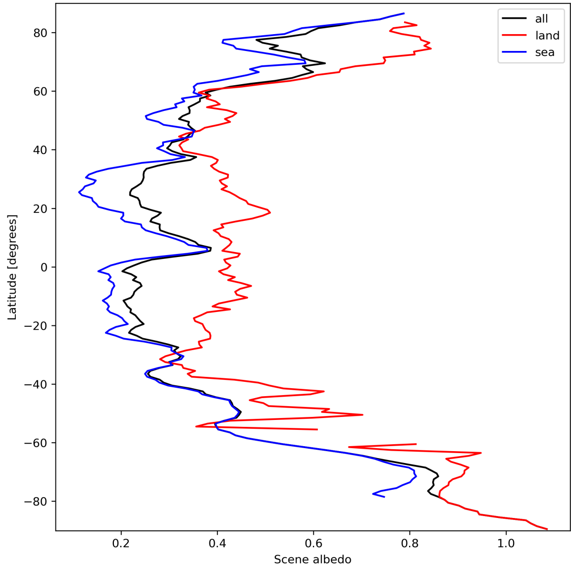
Figure 17: Zonal average of “Scene albedo” for 2023-09-26 to 2023-09-28.
