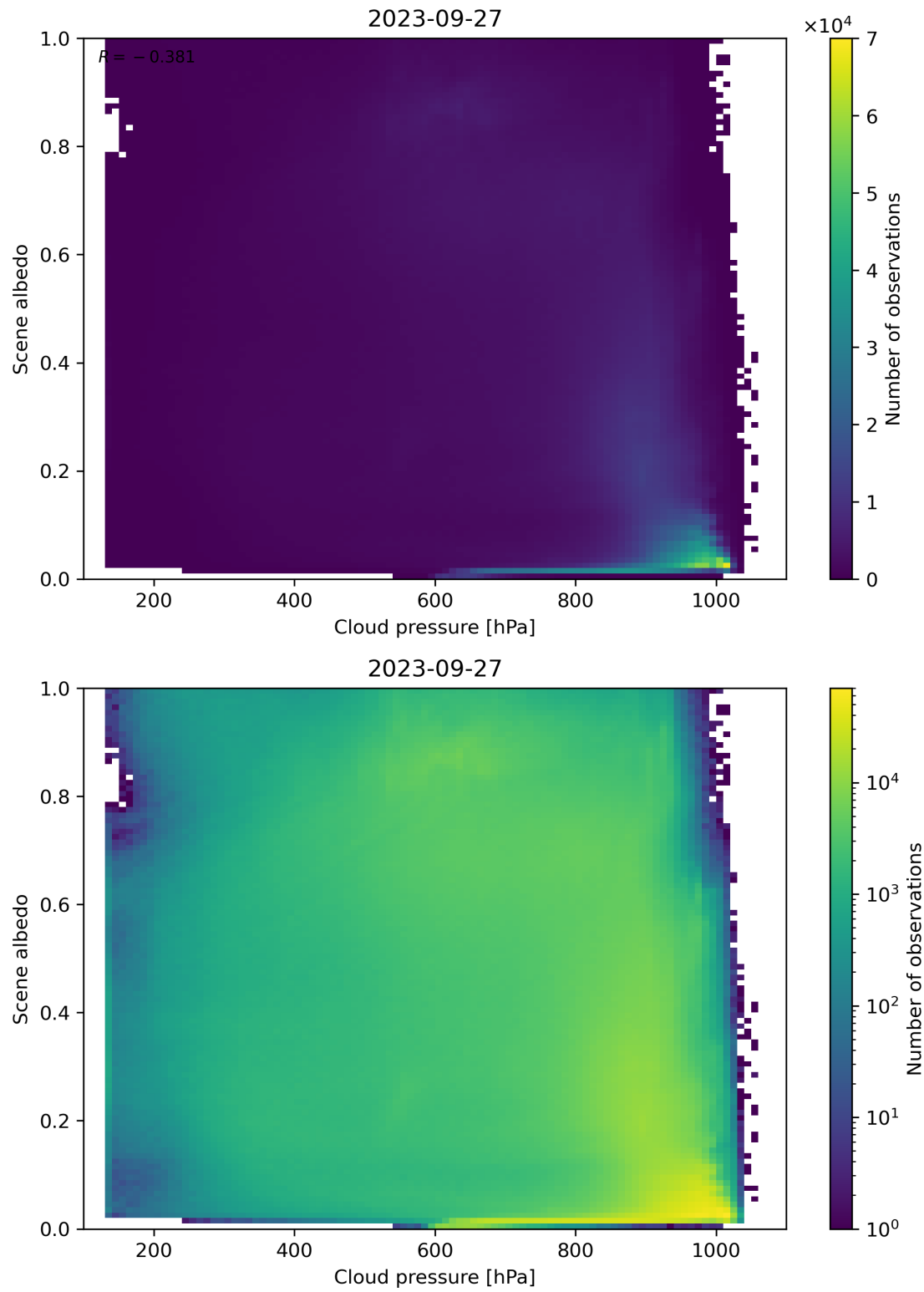
Figure 91: Scatter density plot of “Cloud pressure” against “Scene albedo” for 2023-09-26 to 2023-09-28.
