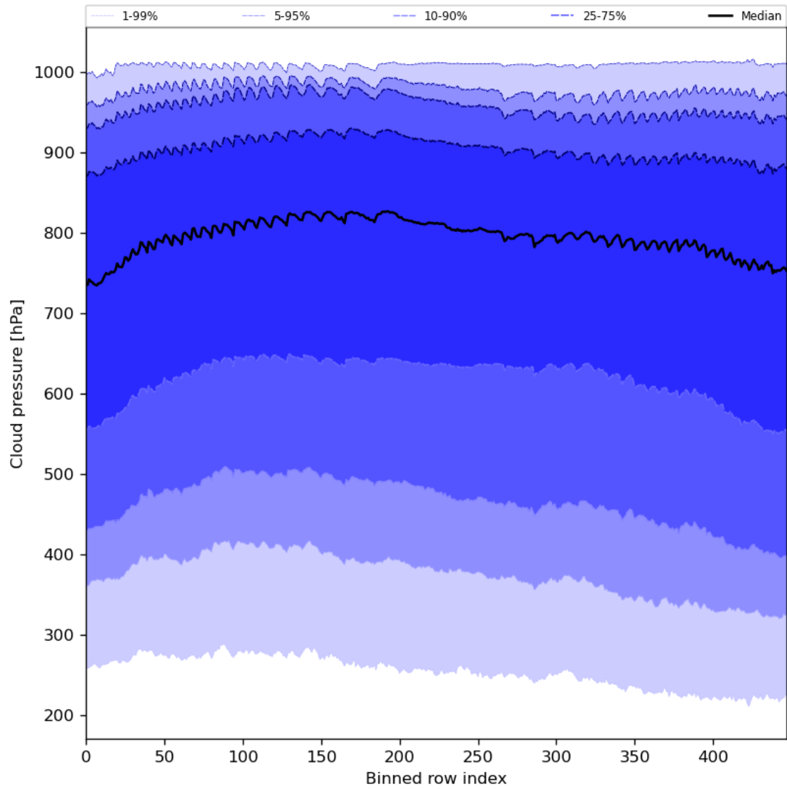
Figure 47: Along track statistics of “Cloud pressure” for 2023-09-26 to 2023-09-28
