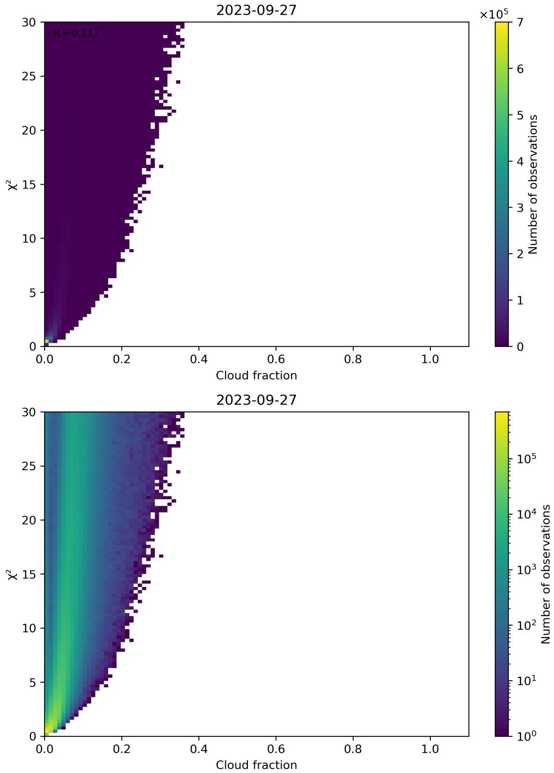
Figure 77: Scatter density plot of “Cloud fraction” against “ \chi^2 ” for 2023-09-26 to 2023-09-28.
