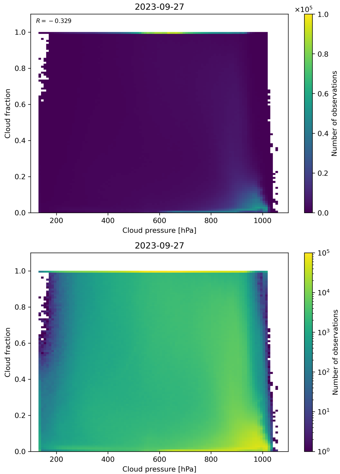
Figure 87: Scatter density plot of “Cloud pressure” against “Cloud fraction” for 2023-09-26 to 2023-09-28.
