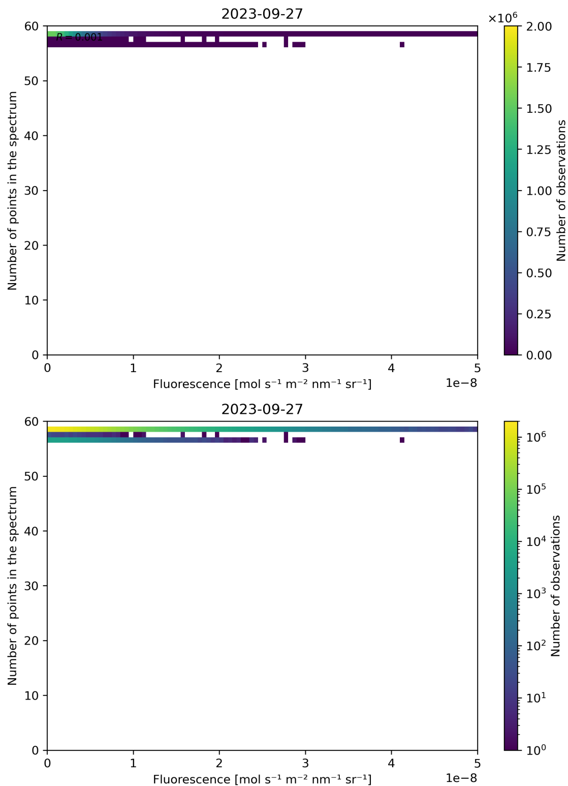
Figure 94: Scatter density plot of “Fluorescence” against “Number of points in the spectrum” for 2023-09-26 to 2023-09-28.
