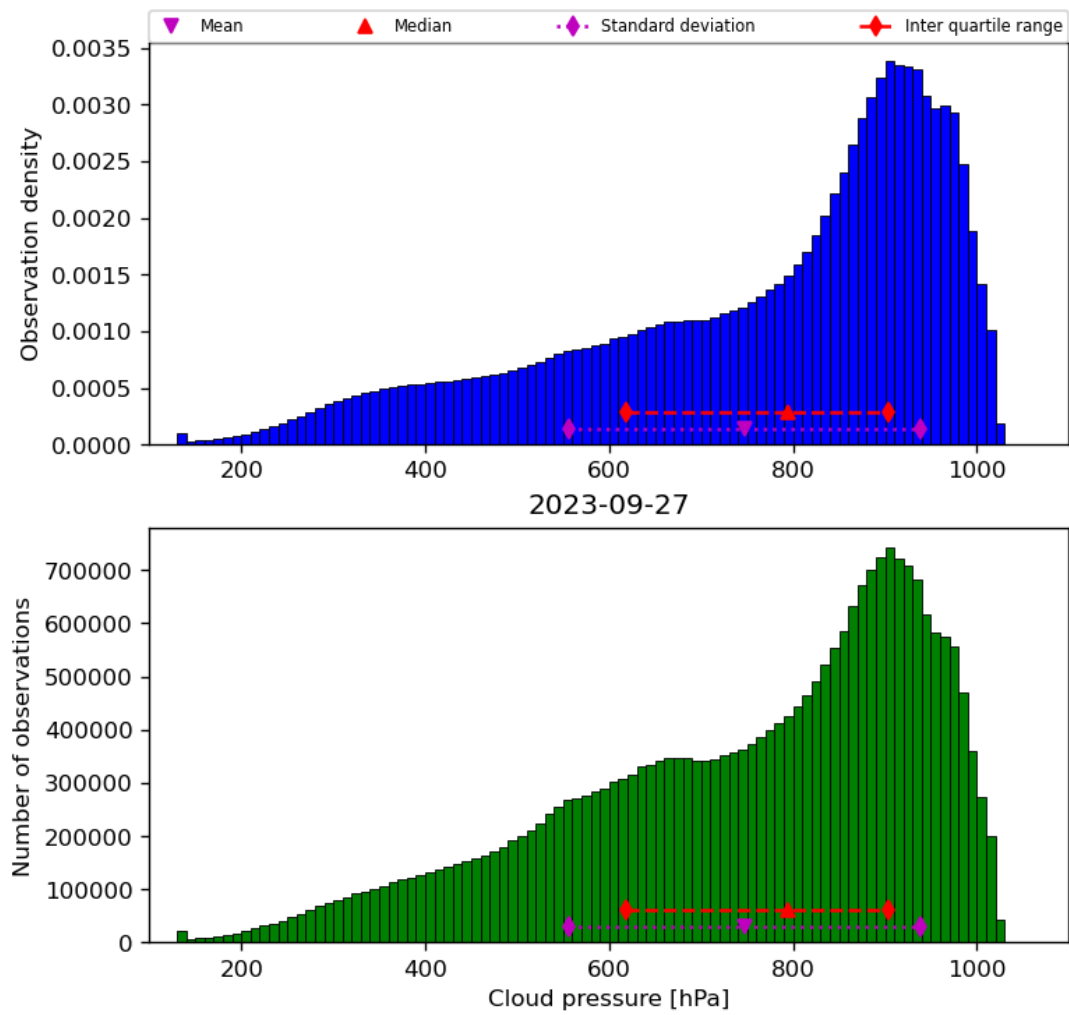
Figure 30: Histogram of “Cloud pressure” for 2023-09-26 to 2023-09-28
