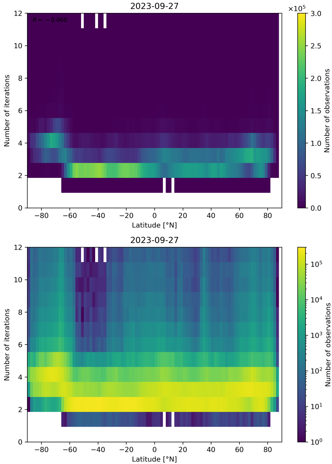
Figure 102: Scatter density plot of “Latitude” against “Number of iterations” for 2023-09-26 to 2023-09-28.
