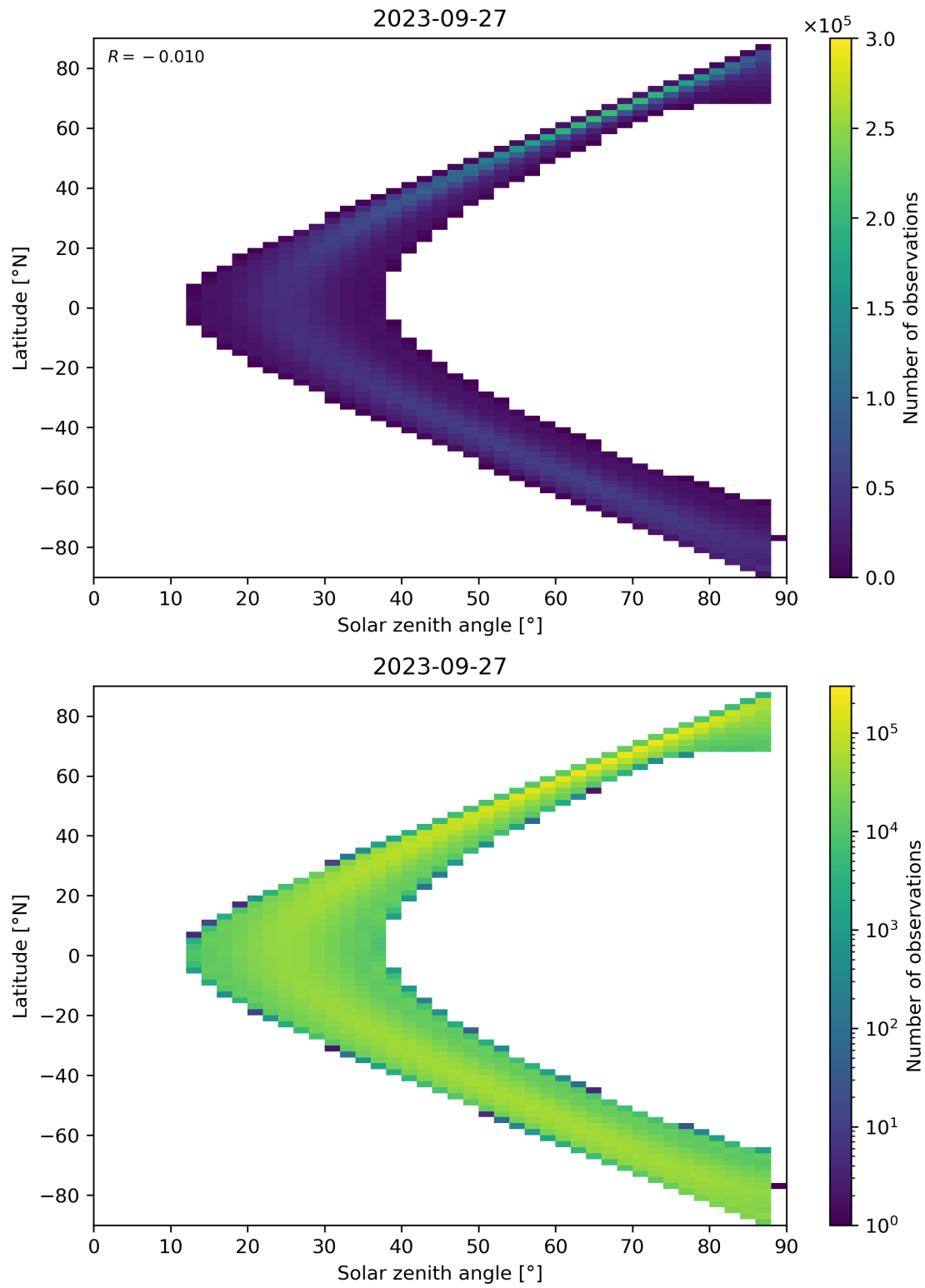
Figure 124: Scatter density plot of “Solar zenith angle” against “Latitude” for 2023-09-26 to 2023-09-28.
