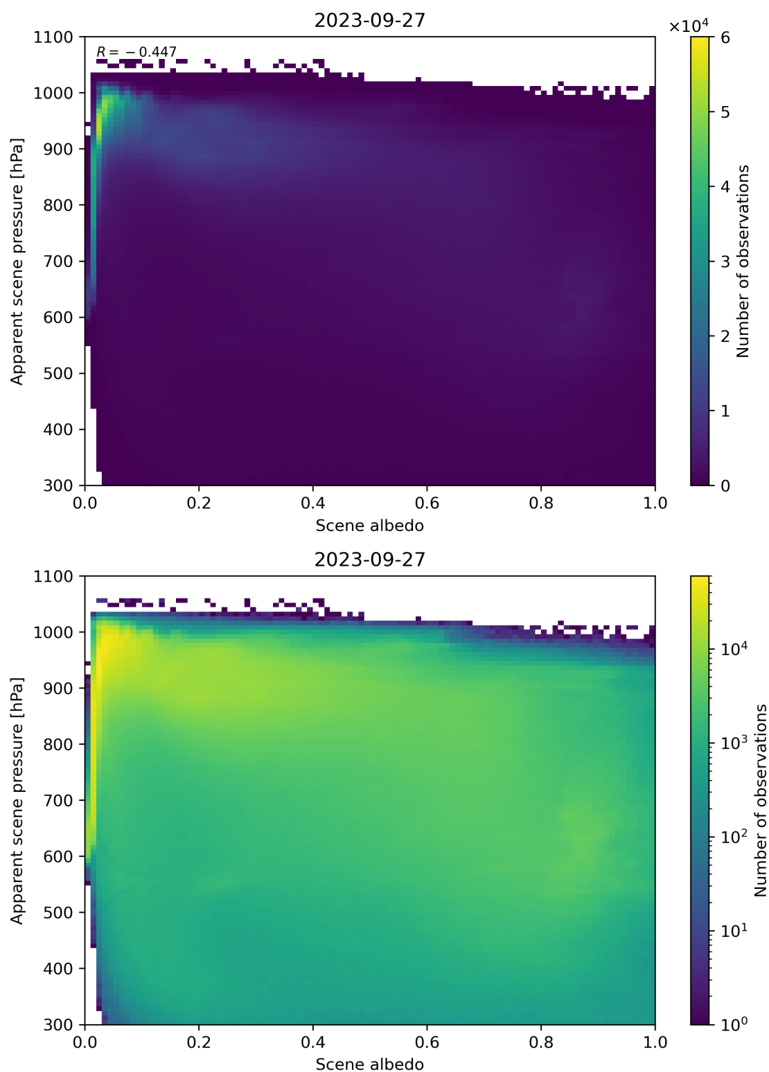
Figure 111: Scatter density plot of “Scene albedo” against “Apparent scene pressure” for 2023-09-26 to 2023-09-28.
