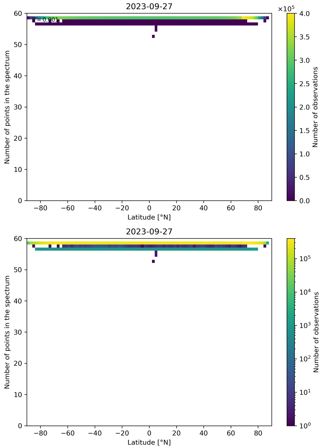
Figure 103: Scatter density plot of “Latitude” against “Number of points in the spectrum” for 2023-09-26 to 2023-09-28.
