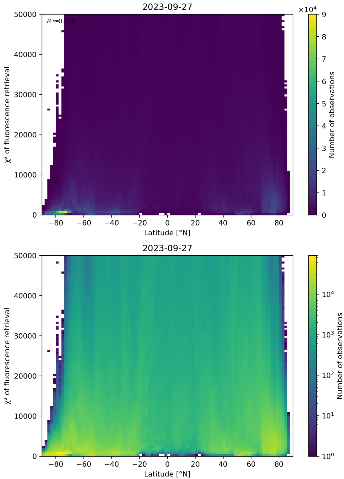
Figure 98: Scatter density plot of “Latitude” against “ \chi^2 of fluorescence retrieval” for 2023-09-26 to 2023-09-28.
