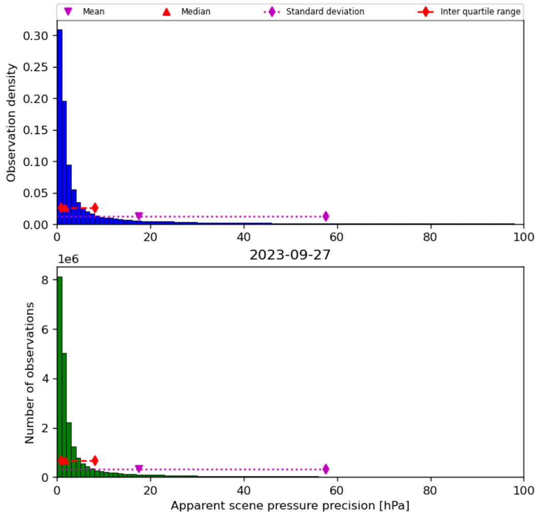
Figure 37: Histogram of “Apparent scene pressure precision” for 2023-09-26 to 2023-09-28
