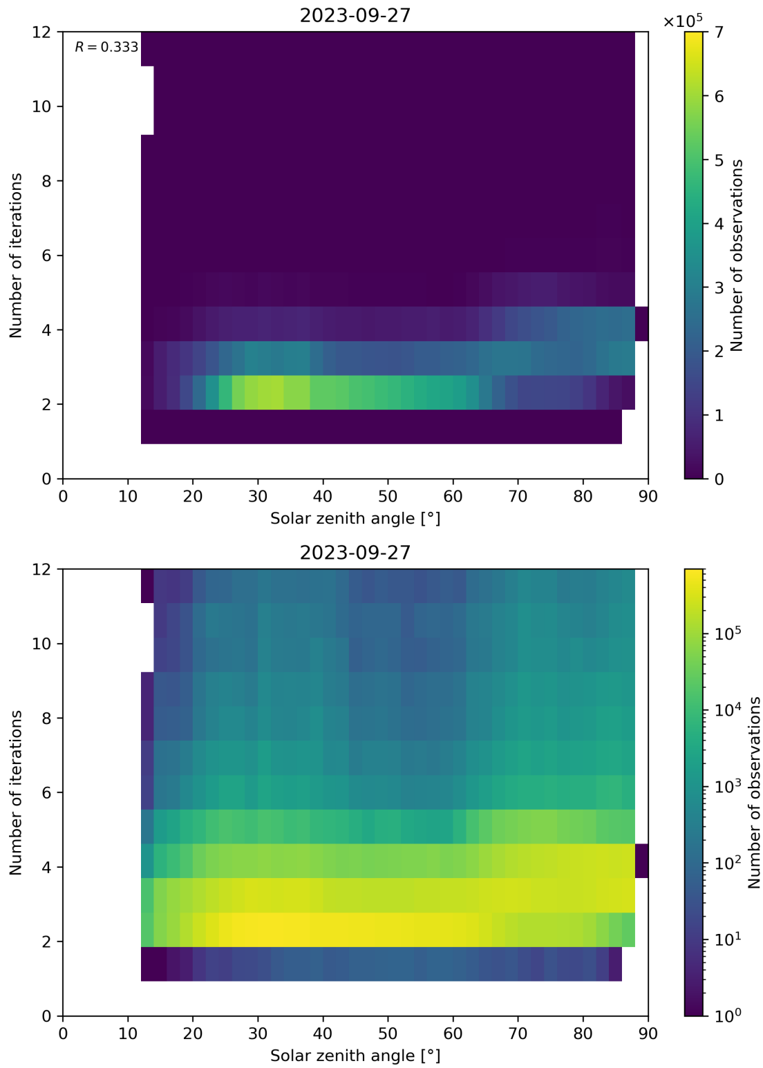
Figure 125: Scatter density plot of “Solar zenith angle” against “Number of iterations” for 2023-09-26 to 2023-09-28.
