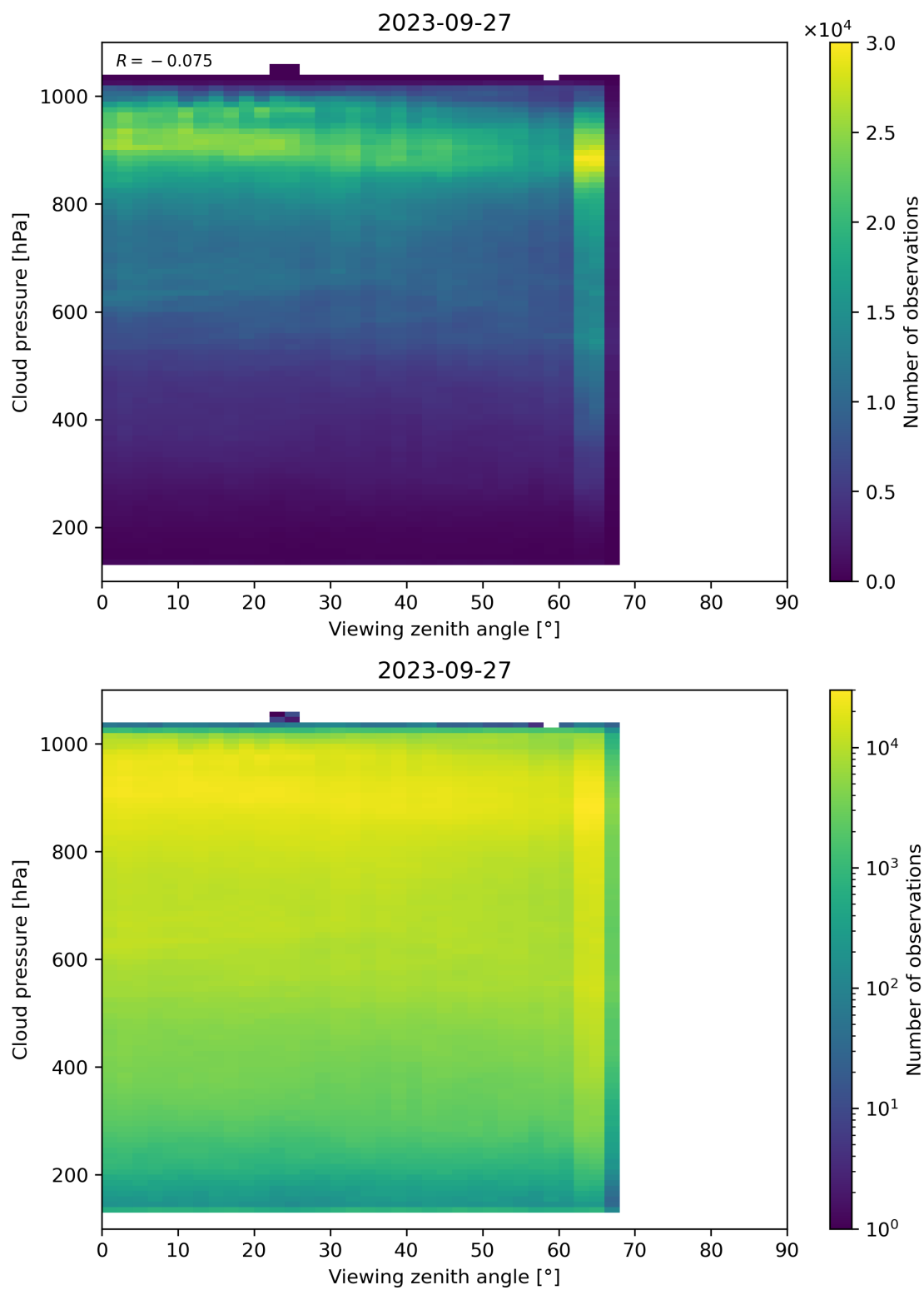
Figure 133: Scatter density plot of “Viewing zenith angle” against “Cloud pressure” for 2023-09-26 to 2023-09-28.
