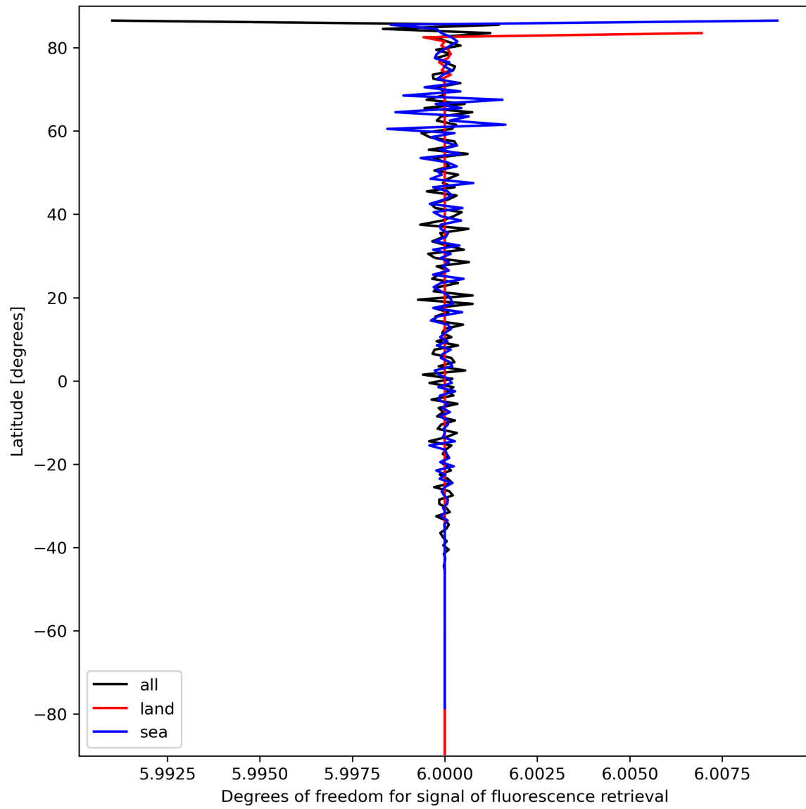
Figure 26: Zonal average of “Degrees of freedom for signal of fluorescence retrieval” for 2023-09-26 to 2023-09-28.
