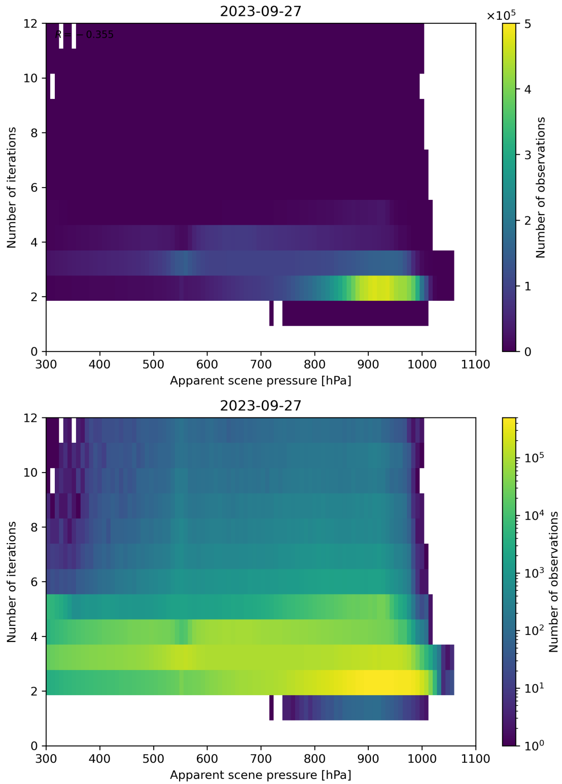
Figure 66: Scatter density plot of “Apparent scene pressure” against “Number of iterations” for 2023-09-26 to 2023-09-28.
