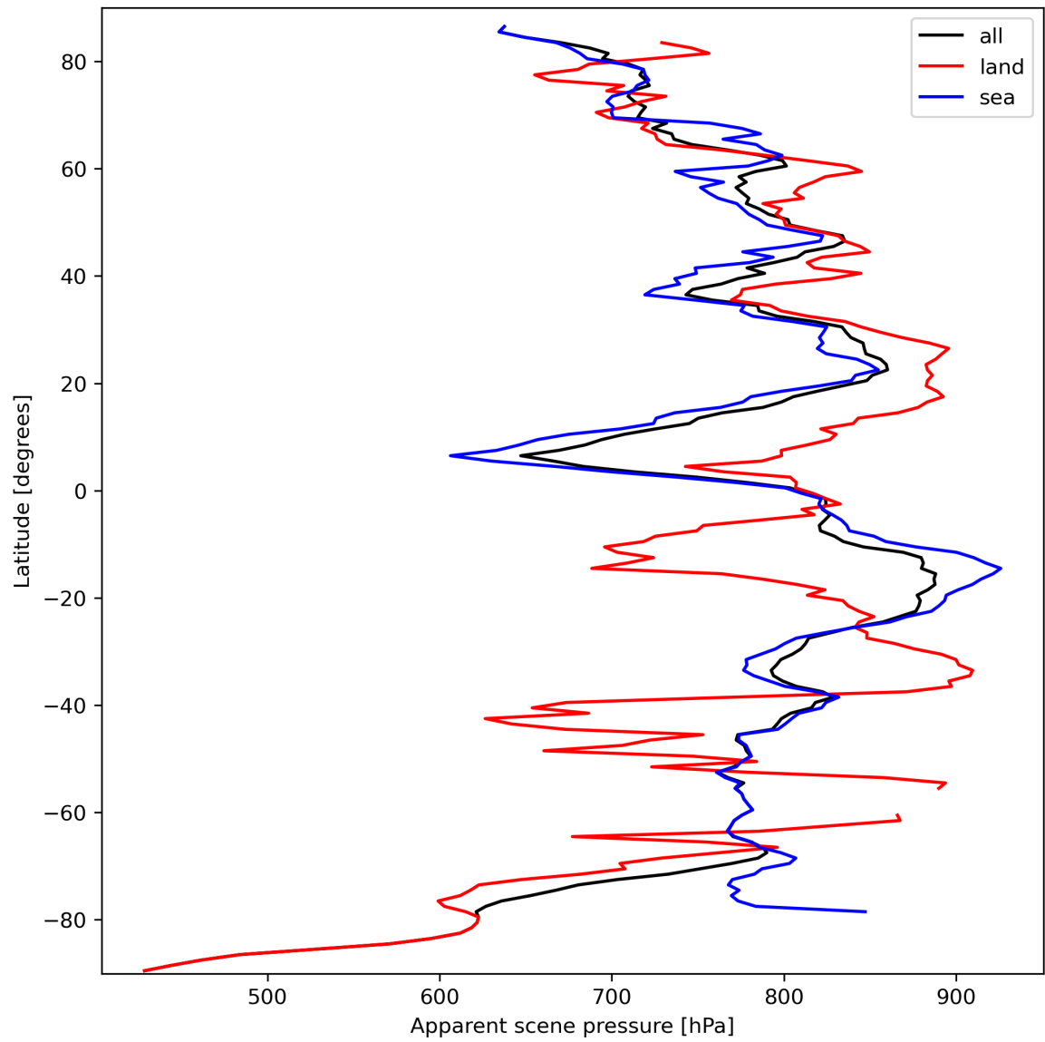
Figure 19: Zonal average of “Apparent scene pressure” for 2023-09-26 to 2023-09-28.
