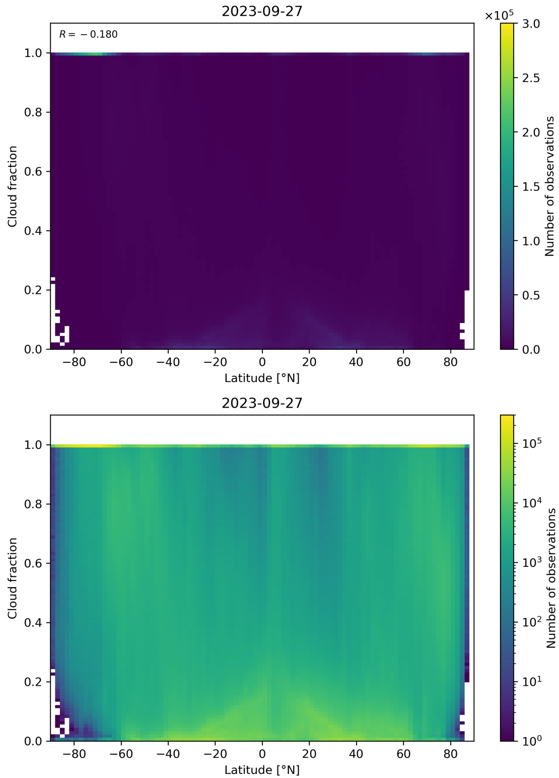
Figure 99: Scatter density plot of “Latitude” against “Cloud fraction” for 2023-09-26 to 2023-09-28.
