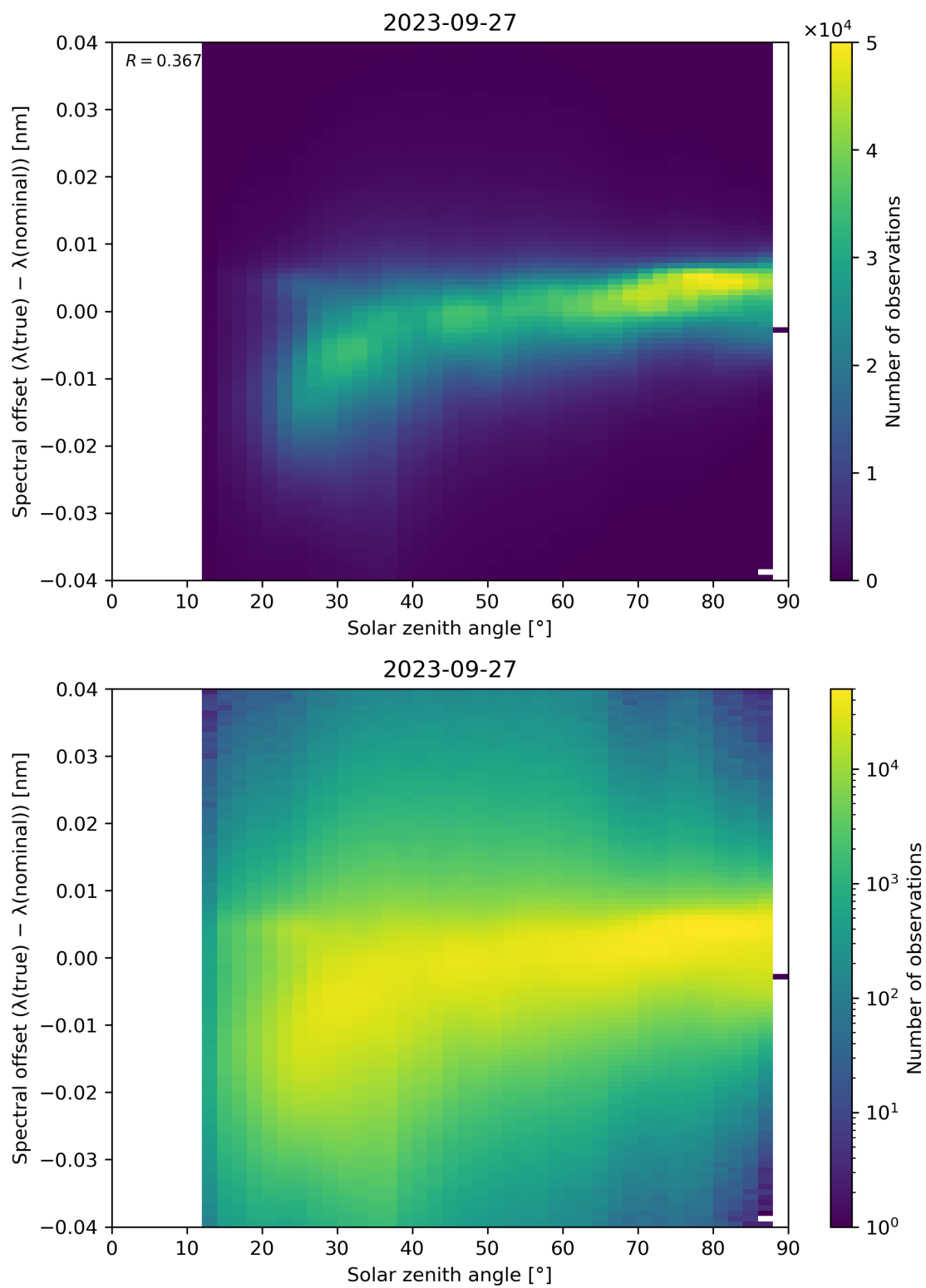
Figure 128: Scatter density plot of “Solar zenith angle” against “Spectral offset ( \lambda(\text{true}) - \lambda(\text{nominal}) )” for 2023-09-26 to 2023-09-28.
