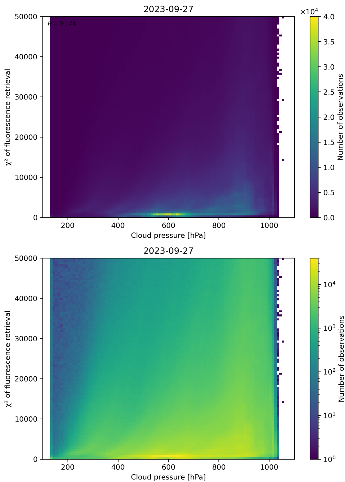
Figure 86: Scatter density plot of “Cloud pressure” against “ \chi^2 of fluorescence retrieval” for 2023-09-26 to 2023-09-28.
