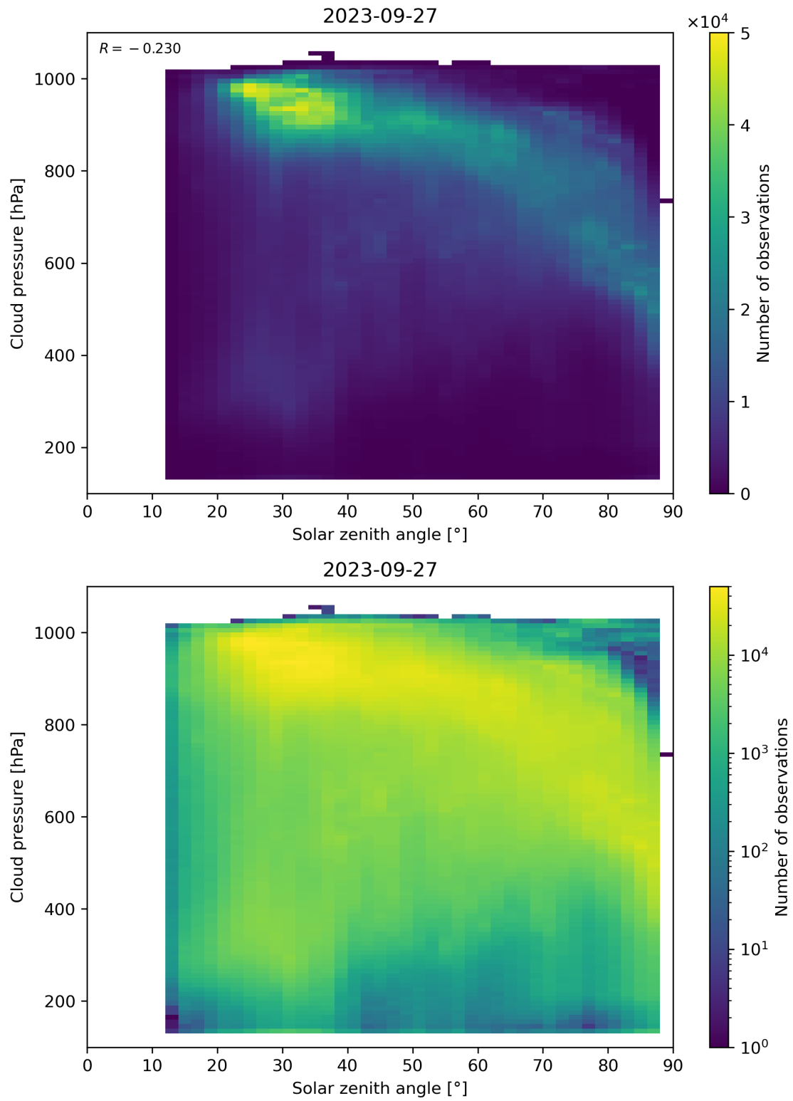
Figure 122: Scatter density plot of “Solar zenith angle” against “Cloud pressure” for 2023-09-26 to 2023-09-28.
