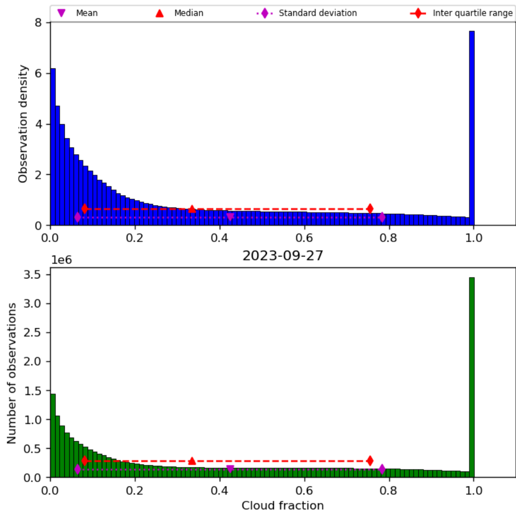
Figure 32: Histogram of “Cloud fraction” for 2023-09-26 to 2023-09-28
