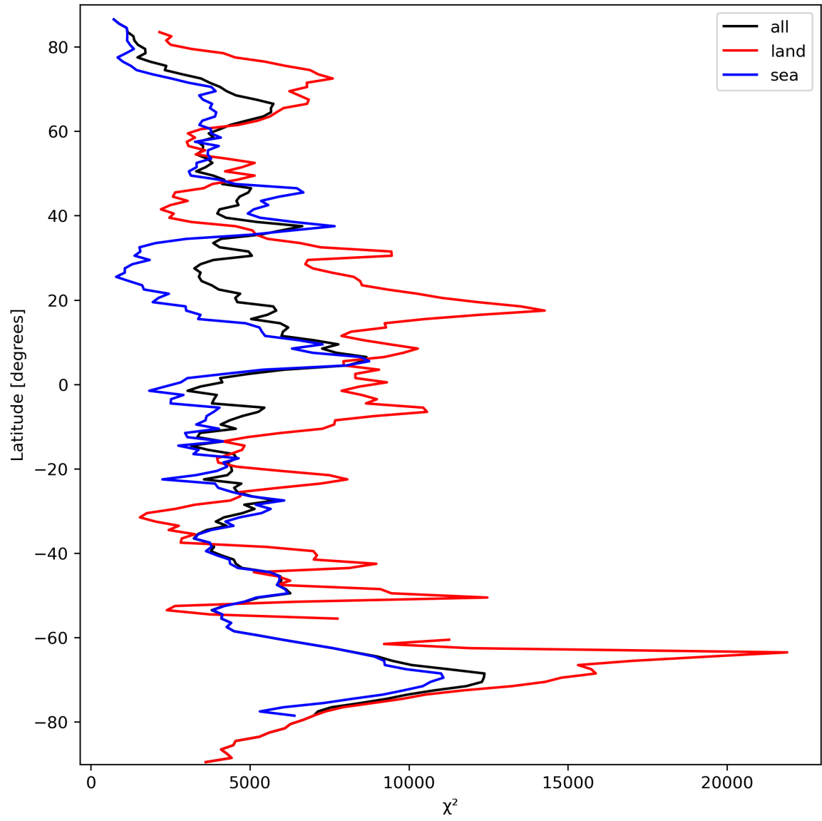
Figure 21: Zonal average of “ \chi^2 ” for 2023-09-26 to 2023-09-28.
