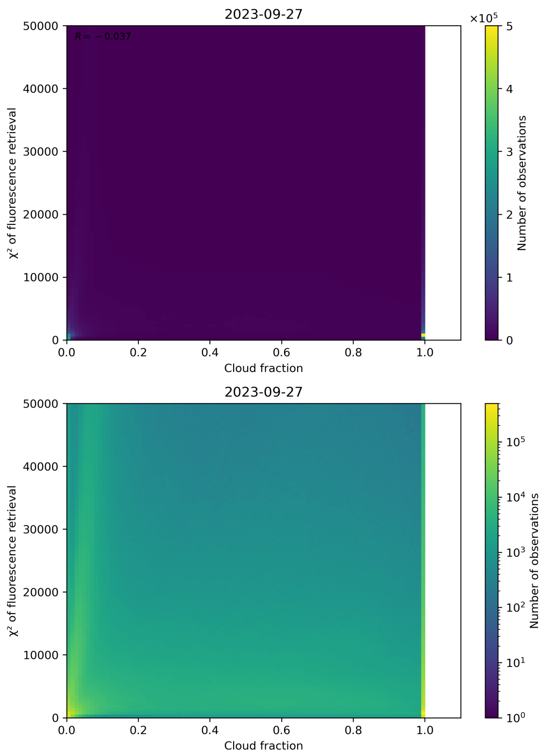
Figure 78: Scatter density plot of “Cloud fraction” against “ \chi^2 of fluorescence retrieval” for 2023-09-26 to 2023-09-28.
