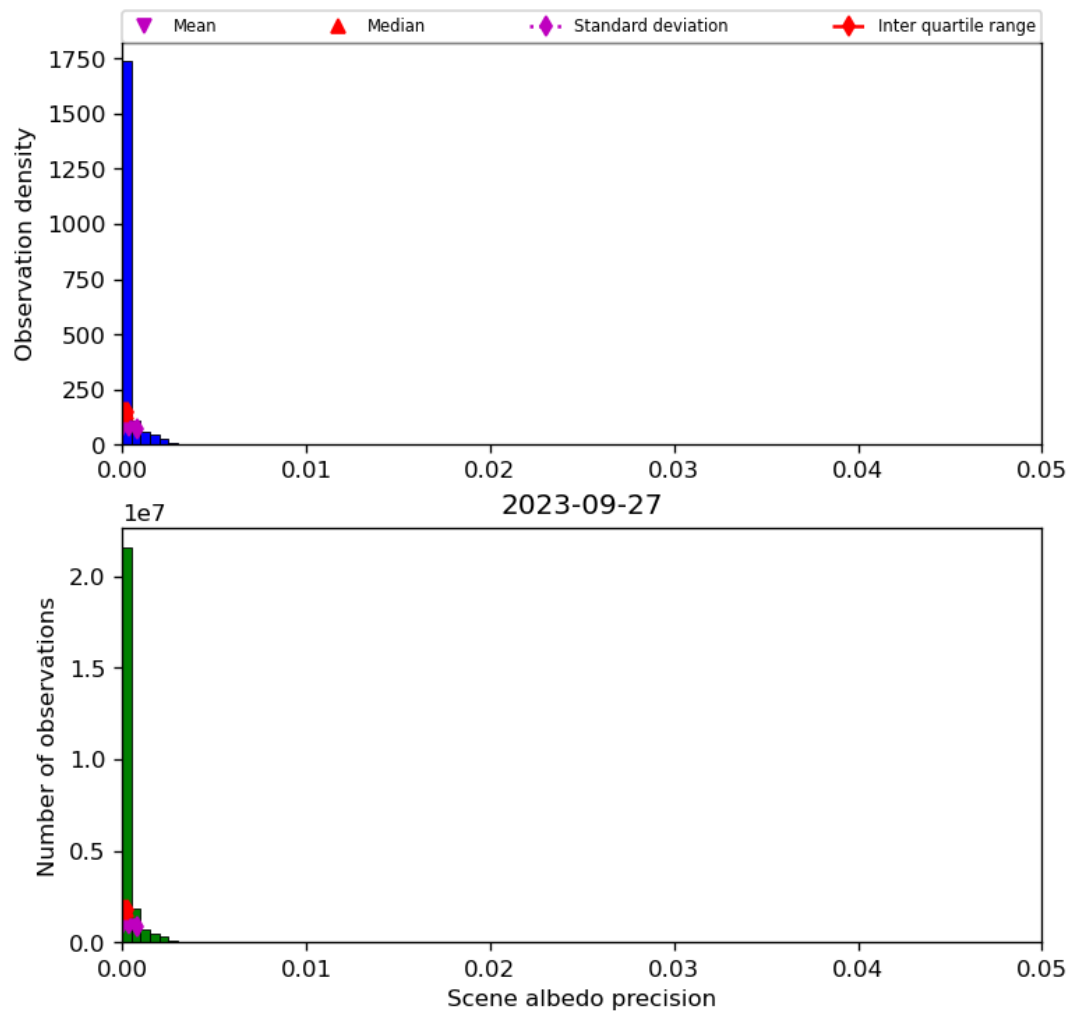
Figure 35: Histogram of “Scene albedo precision” for 2023-09-26 to 2023-09-28
