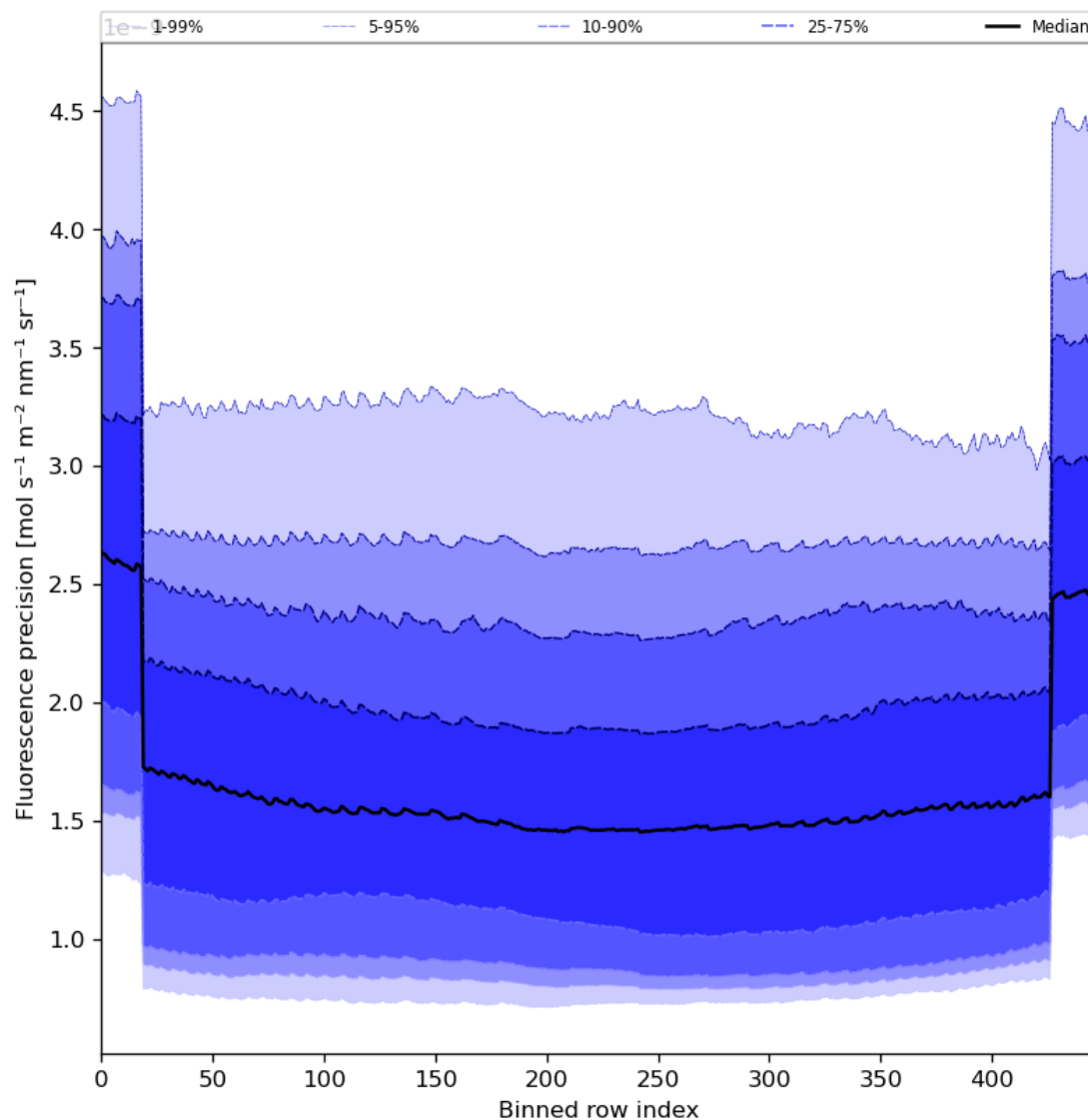
Figure 58: Along track statistics of “Fluorescence precision” for 2023-09-27 to 2023-09-29
