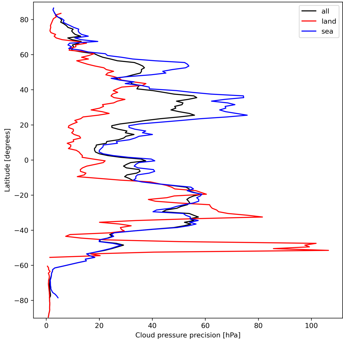
Figure 14: Zonal average of “Cloud pressure precision” for 2023-09-27 to 2023-09-29.
