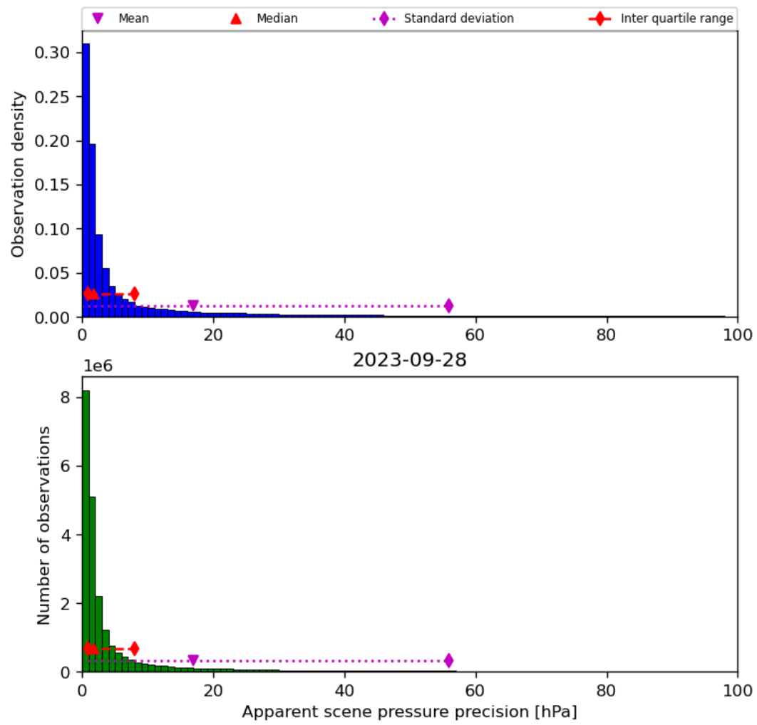
Figure 37: Histogram of “Apparent scene pressure precision” for 2023-09-27 to 2023-09-29
