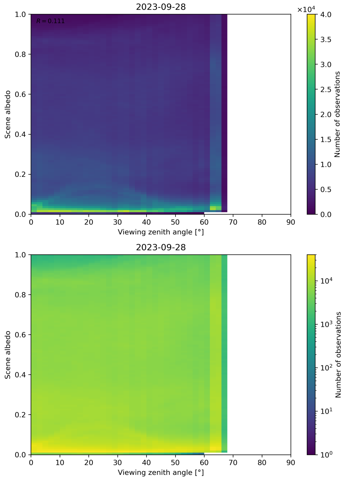
Figure 138: Scatter density plot of “Viewing zenith angle” against “Scene albedo” for 2023-09-27 to 2023-09-29.
