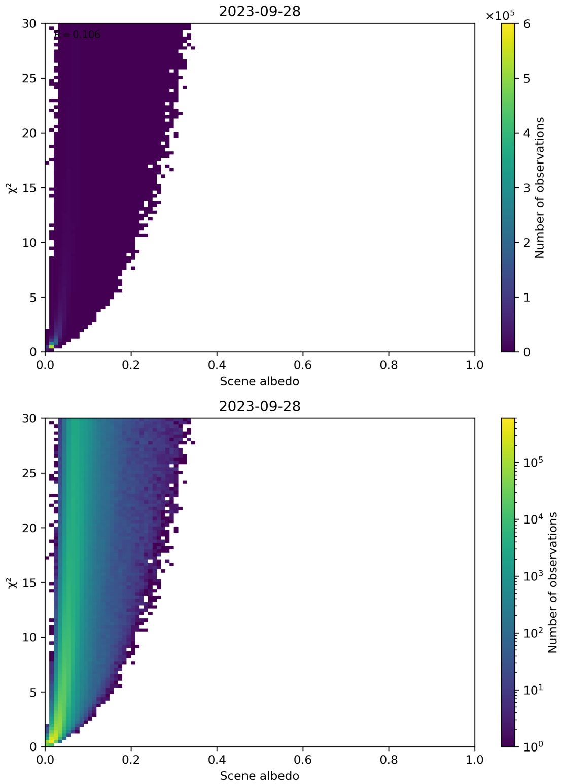
Figure 112: Scatter density plot of “Scene albedo” against “ \chi^2 ” for 2023-09-27 to 2023-09-29.
