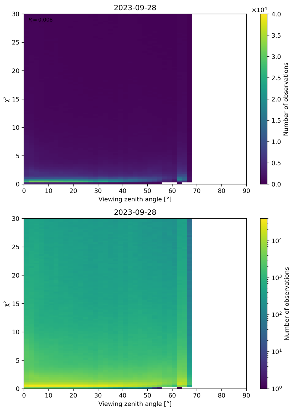
Figure 130: Scatter density plot of “Viewing zenith angle” against “ \chi^2 ” for 2023-09-27 to 2023-09-29.
