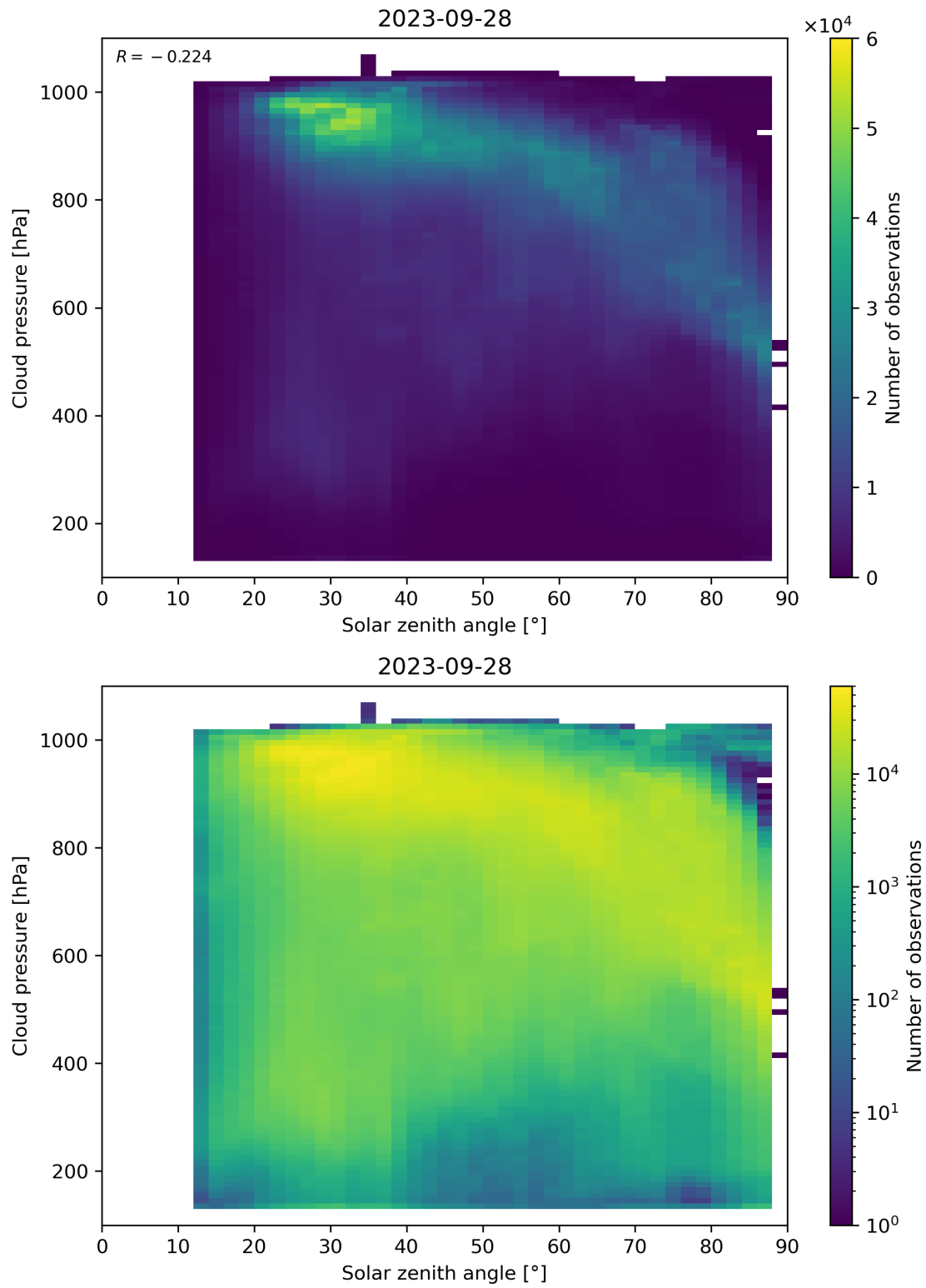
Figure 122: Scatter density plot of “Solar zenith angle” against “Cloud pressure” for 2023-09-27 to 2023-09-29.
