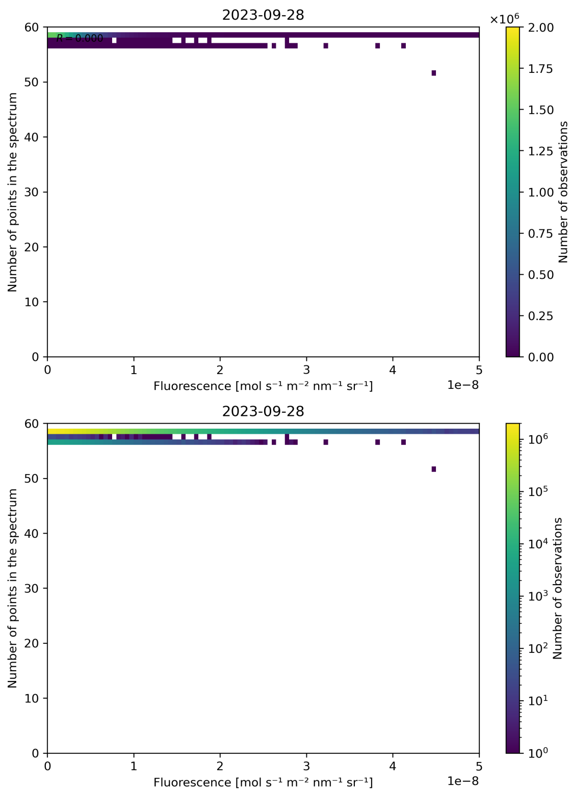
Figure 94: Scatter density plot of “Fluorescence” against “Number of points in the spectrum” for 2023-09-27 to 2023-09-29.
