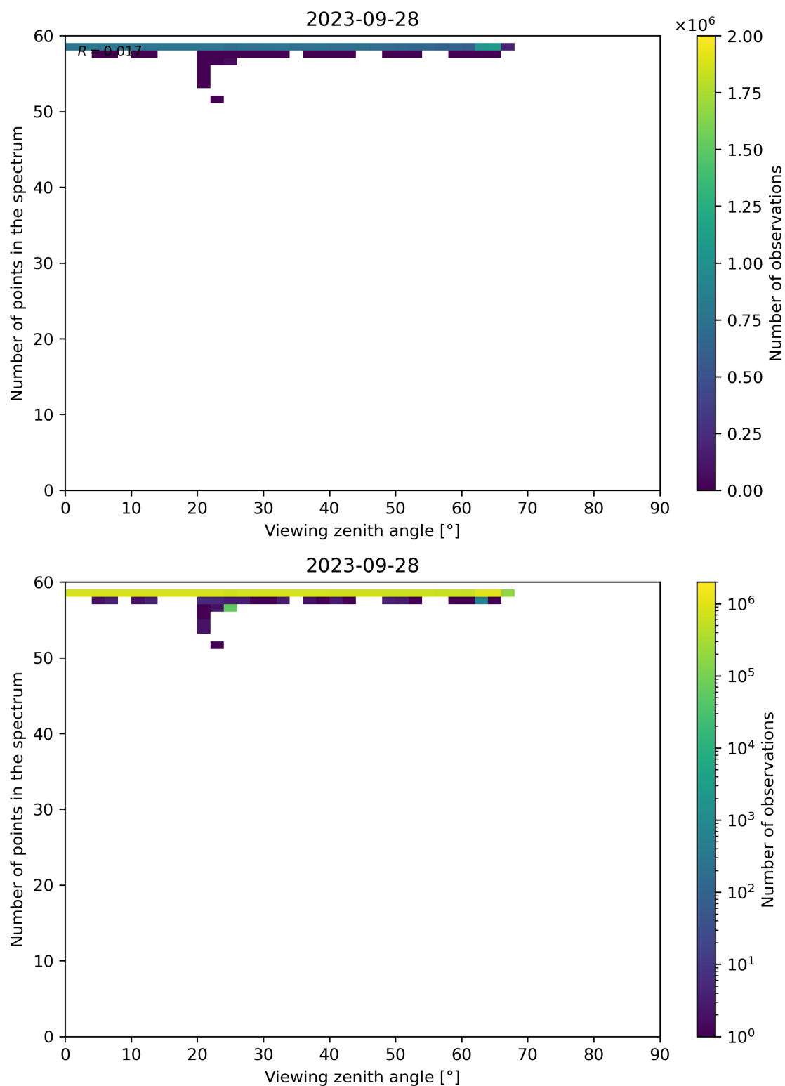
Figure 137: Scatter density plot of “Viewing zenith angle” against “Number of points in the spectrum” for 2023-09-27 to 2023-09-29.
