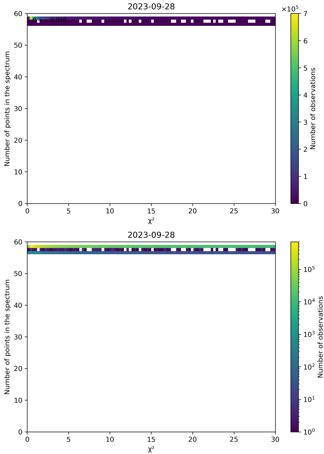
Figure 74: Scatter density plot of " \chi^2 " against "Number of points in the spectrum" for 2023-09-27 to 2023-09-29.
