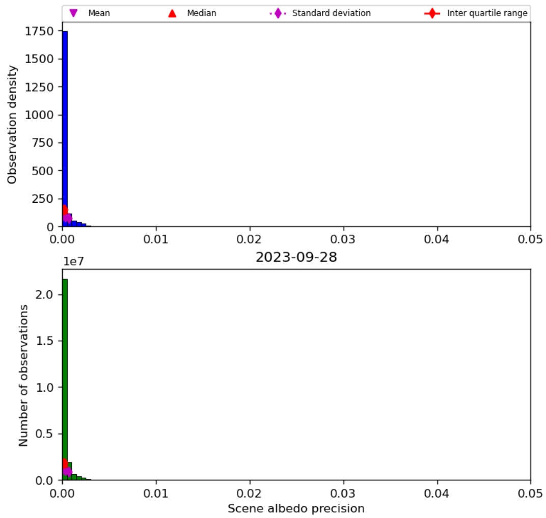
Figure 35: Histogram of “Scene albedo precision” for 2023-09-27 to 2023-09-29
