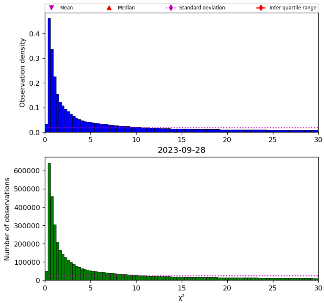
Figure 38: Histogram of “ \chi^2 ” for 2023-09-27 to 2023-09-29
