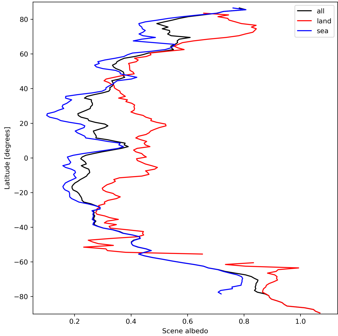
Figure 17: Zonal average of “Scene albedo” for 2023-09-27 to 2023-09-29.
