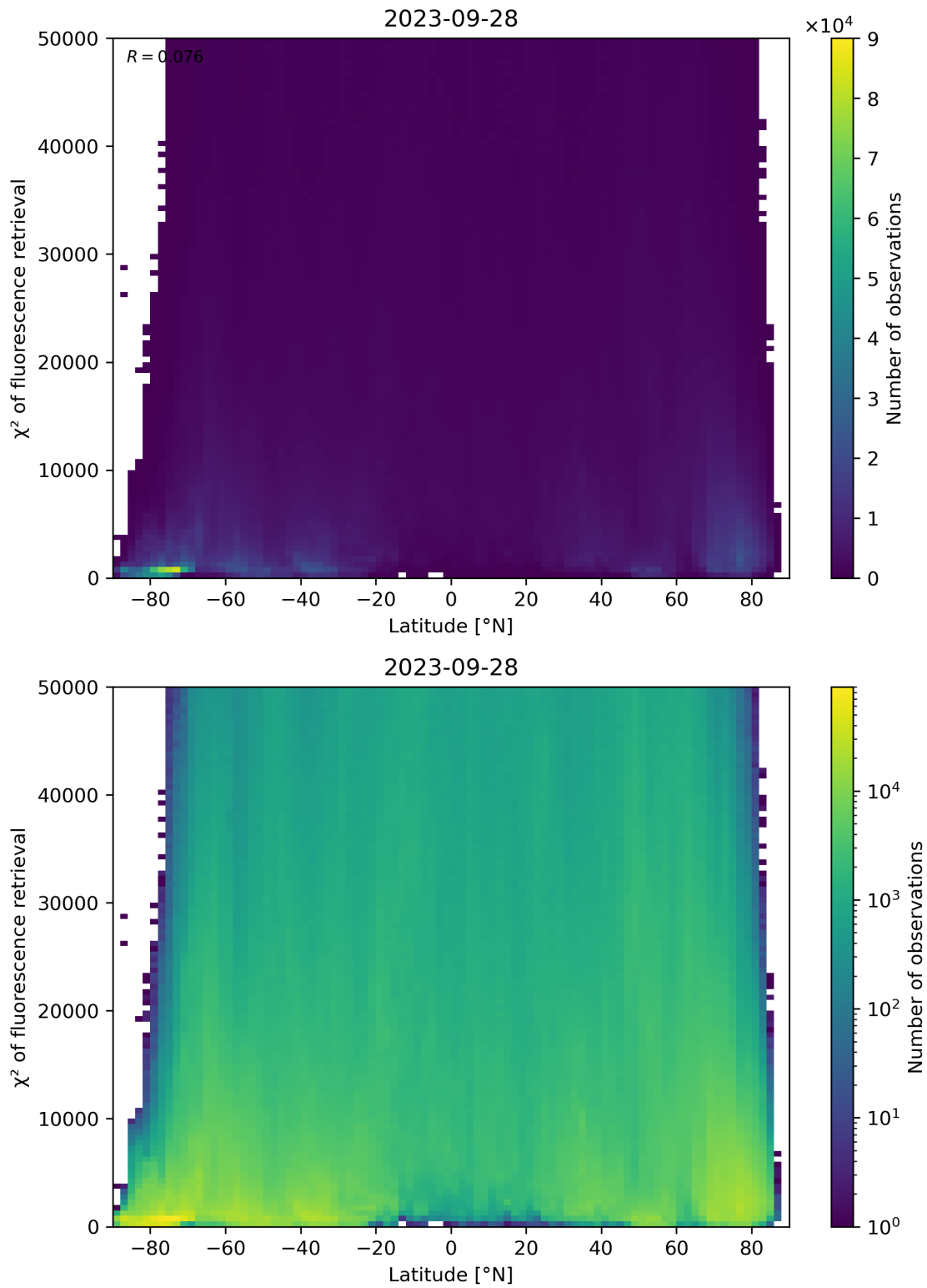
Figure 98: Scatter density plot of “Latitude” against “ \chi^2 of fluorescence retrieval” for 2023-09-27 to 2023-09-29.
