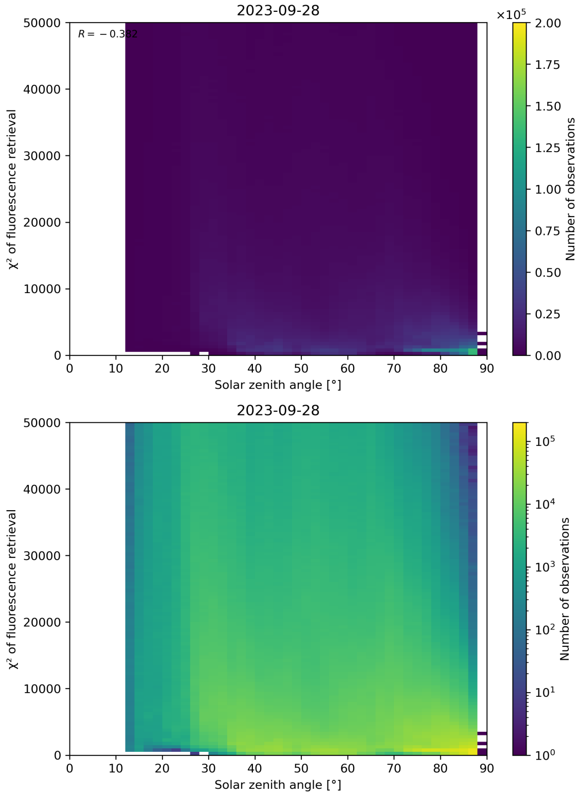
Figure 120: Scatter density plot of “Solar zenith angle” against “ \chi^2 of fluorescence retrieval” for 2023-09-27 to 2023-09-29.
