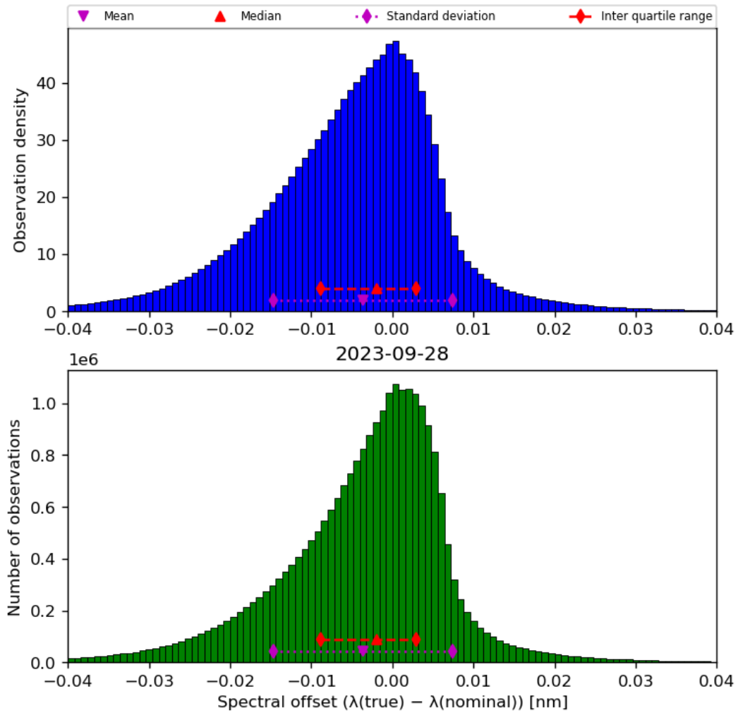
Figure 45: Histogram of “Spectral offset ( \lambda(\text{true}) - \lambda(\text{nominal}) )” for 2023-09-27 to 2023-09-29
