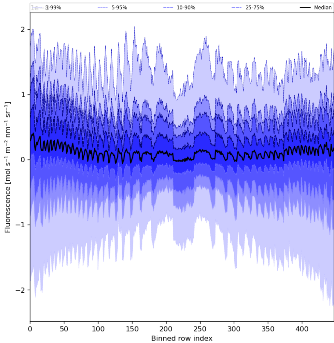
Figure 57: Along track statistics of “Fluorescence” for 2023-09-27 to 2023-09-29
