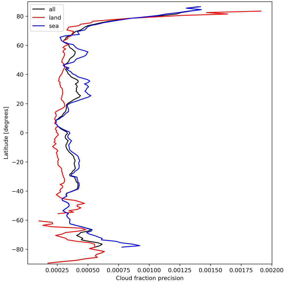
Figure 16: Zonal average of “Cloud fraction precision” for 2023-09-27 to 2023-09-29.
