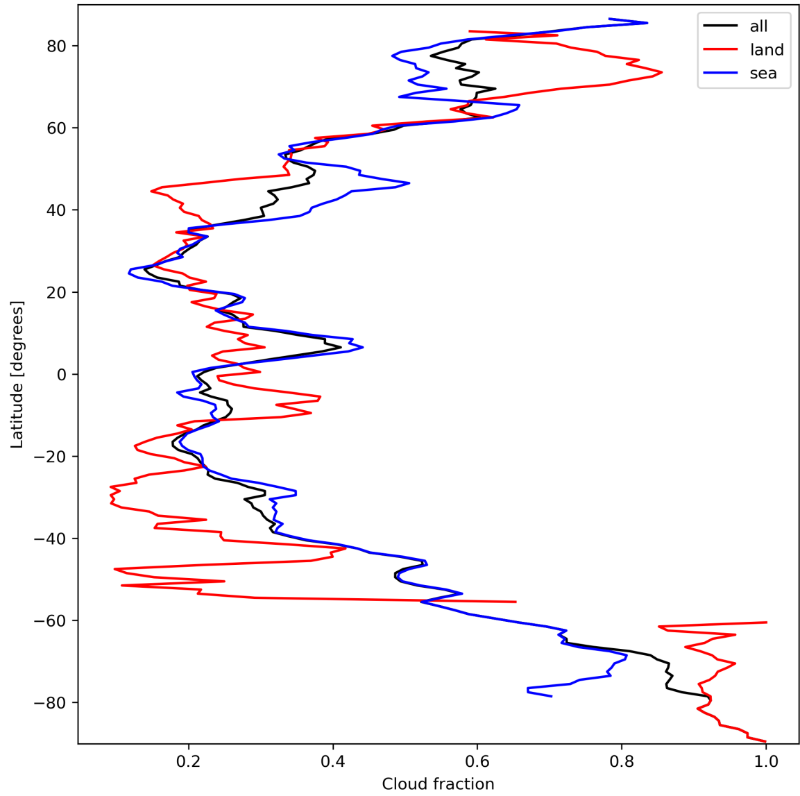
Figure 15: Zonal average of “Cloud fraction” for 2023-09-27 to 2023-09-29.
