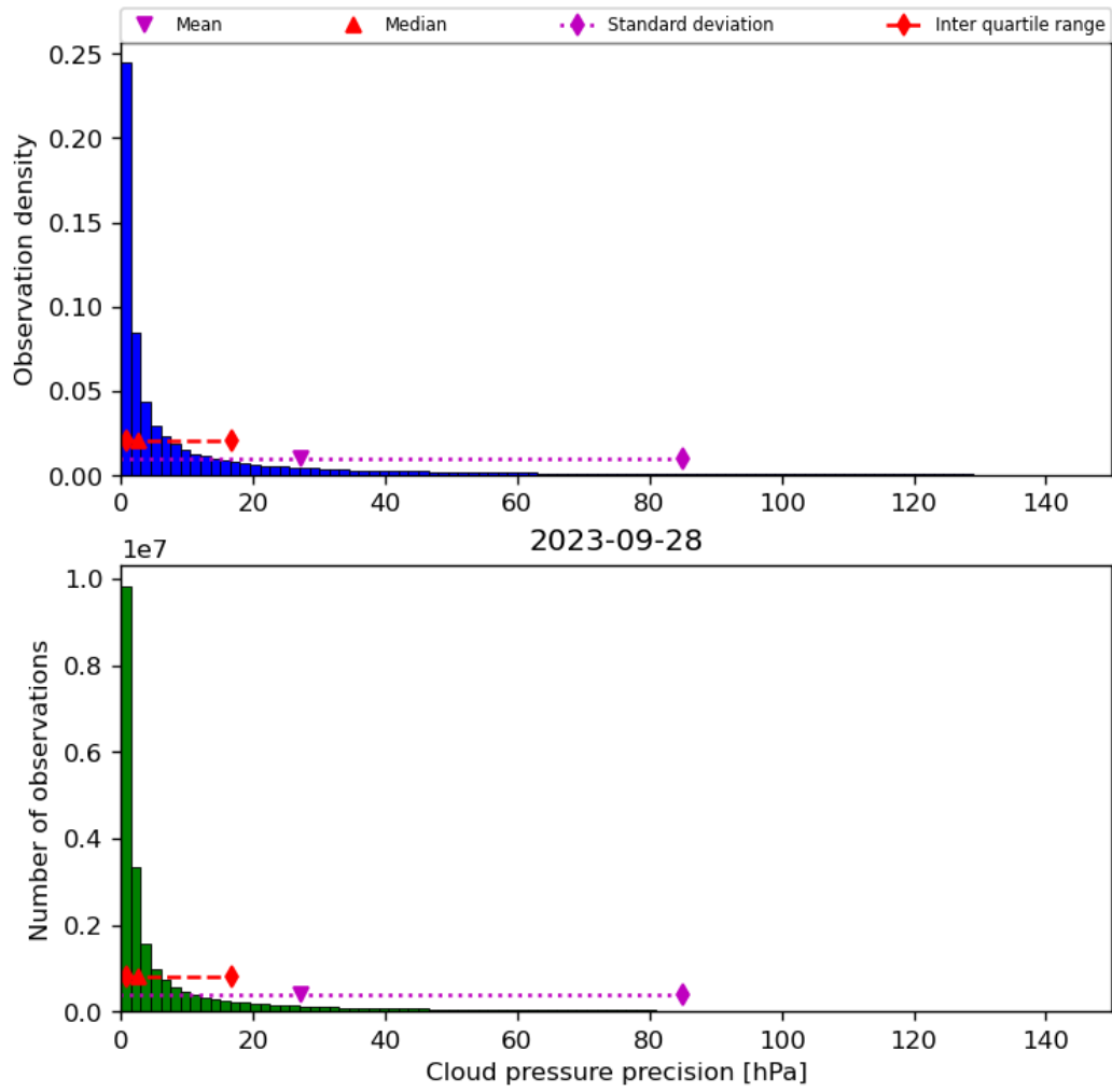
Figure 31: Histogram of “Cloud pressure precision” for 2023-09-27 to 2023-09-29
