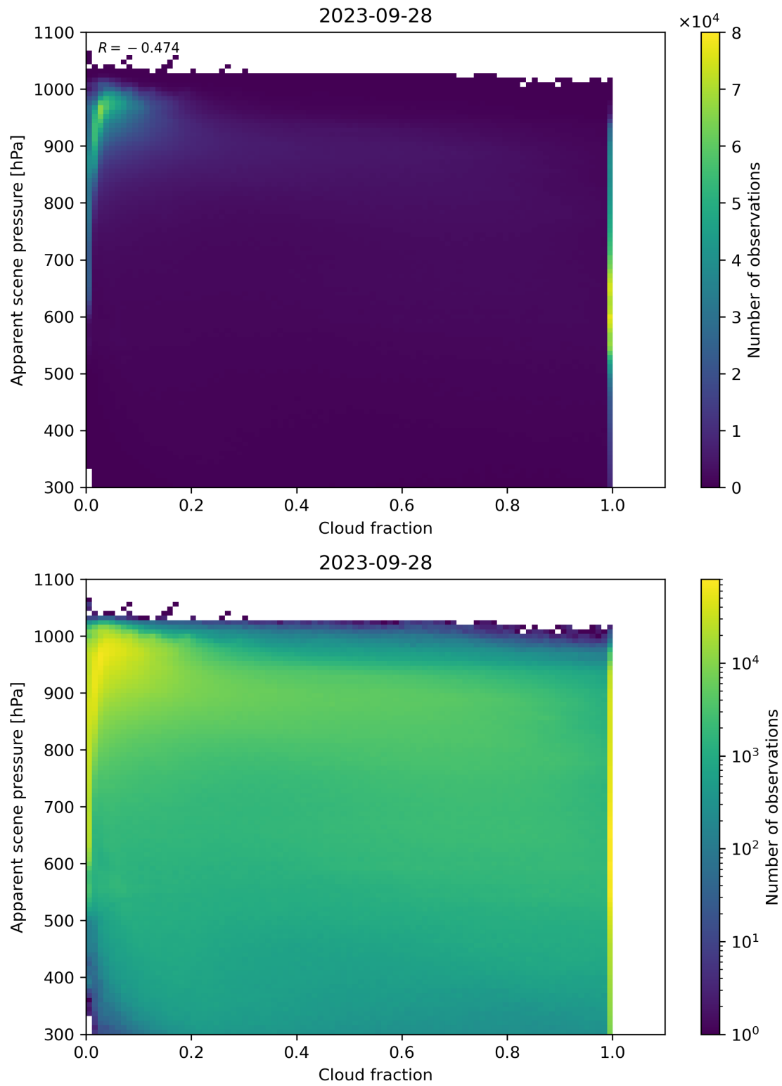
Figure 76: Scatter density plot of “Cloud fraction” against “Apparent scene pressure” for 2023-09-27 to 2023-09-29.
