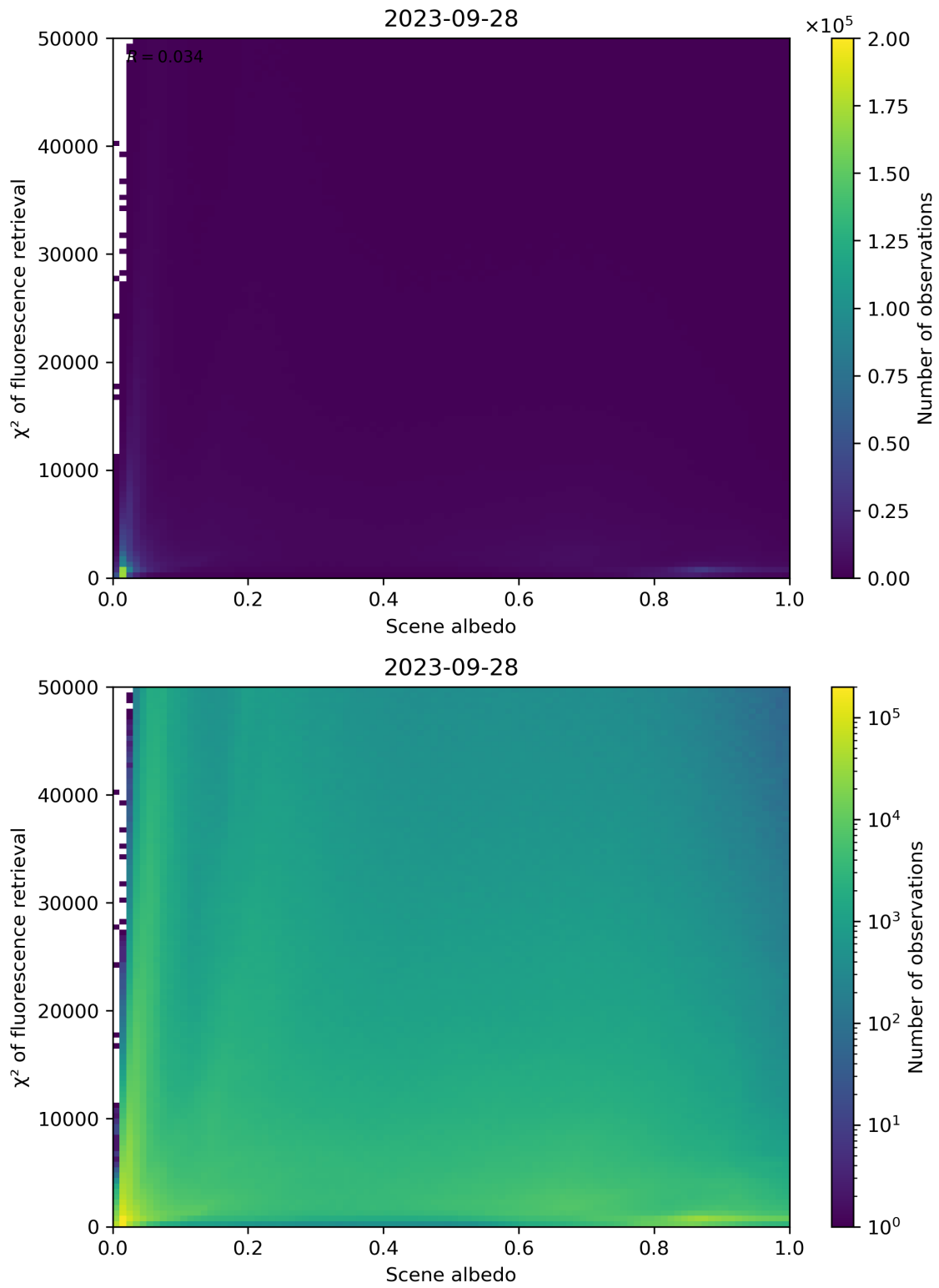
Figure 113: Scatter density plot of “Scene albedo” against “ \chi^2 of fluorescence retrieval” for 2023-09-27 to 2023-09-29.
