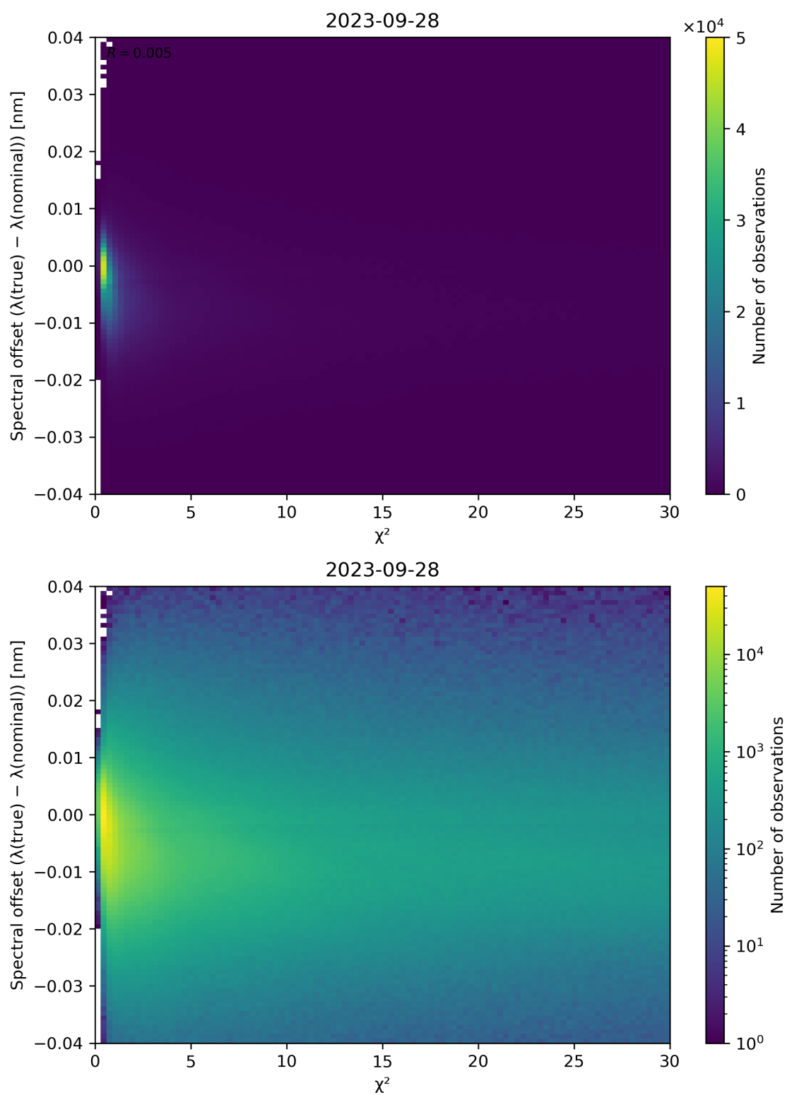
Figure 75: Scatter density plot of “ \chi^2 ” against “Spectral offset ( \lambda(\text{true}) - \lambda(\text{nominal}) )” for 2023-09-27 to 2023-09-29.
