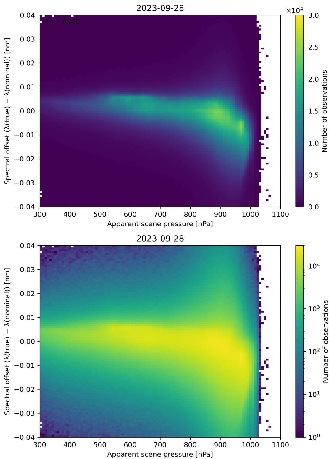
Figure 68: Scatter density plot of “Apparent scene pressure” against “Spectral offset ( \lambda(\text{true}) - \lambda(\text{nominal}) )” for 2023-09-27 to 2023-09-29.
