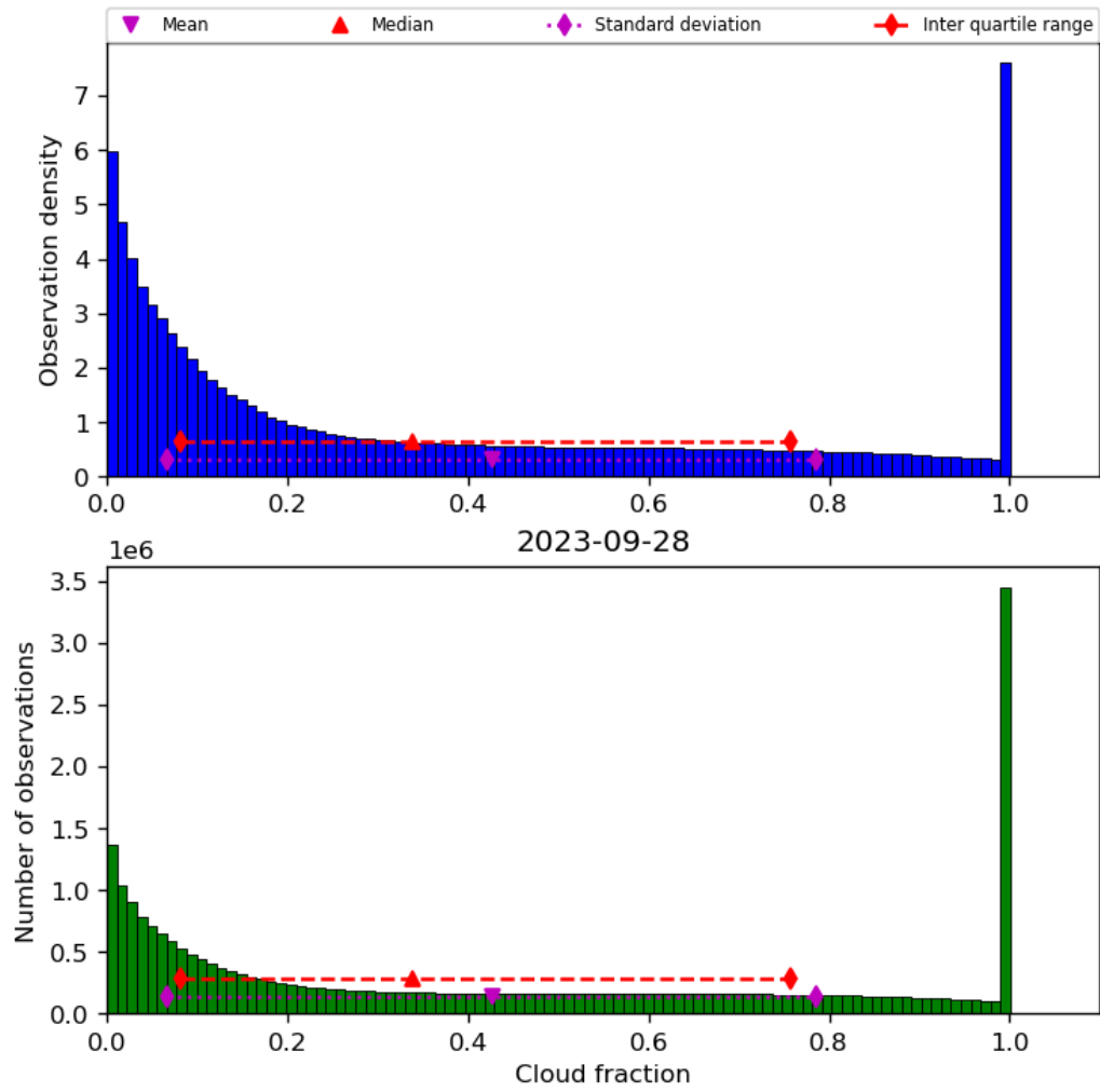
Figure 32: Histogram of “Cloud fraction” for 2023-09-27 to 2023-09-29
