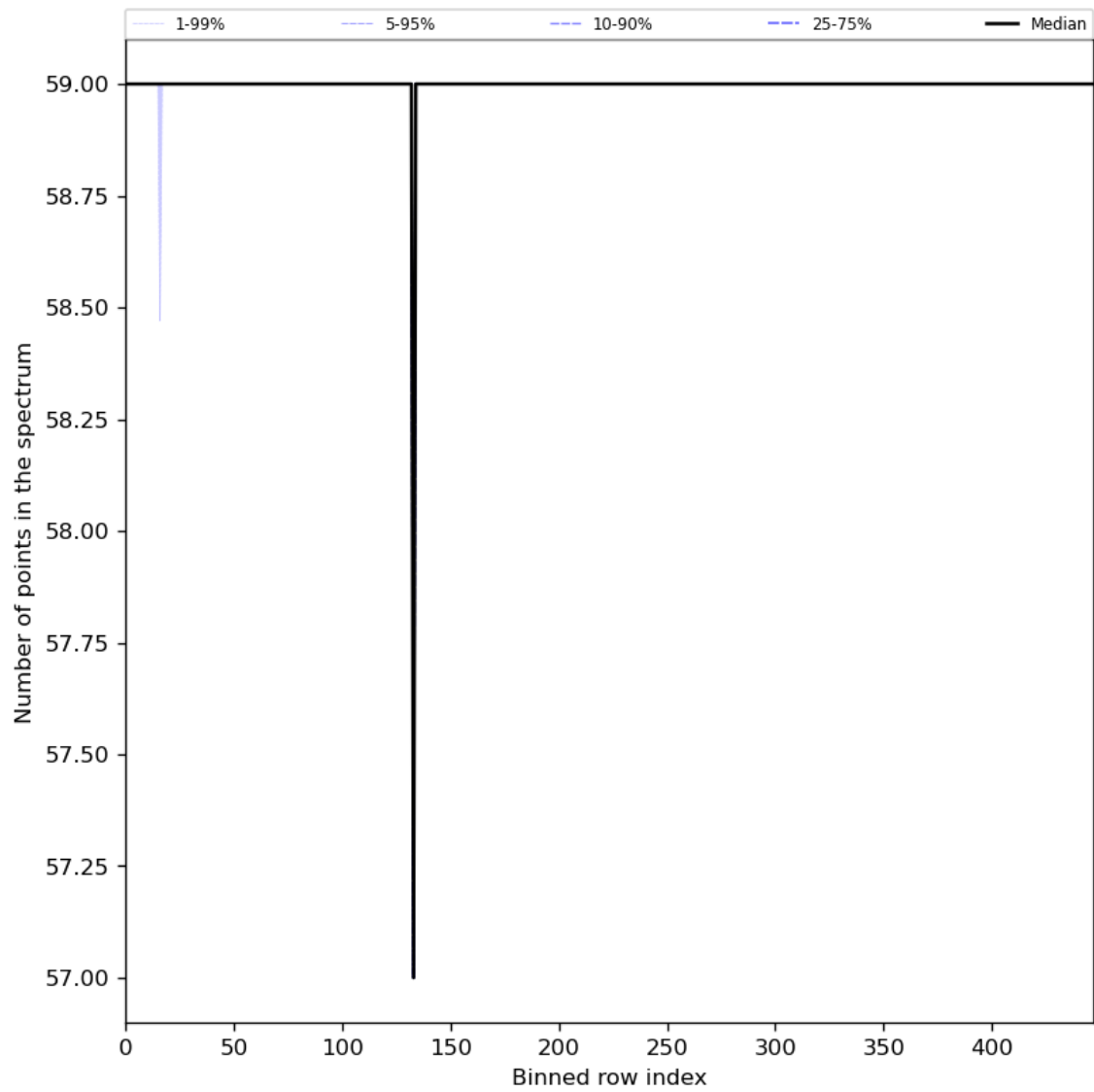
Figure 61: Along track statistics of “Number of points in the spectrum” for 2023-09-27 to 2023-09-29
