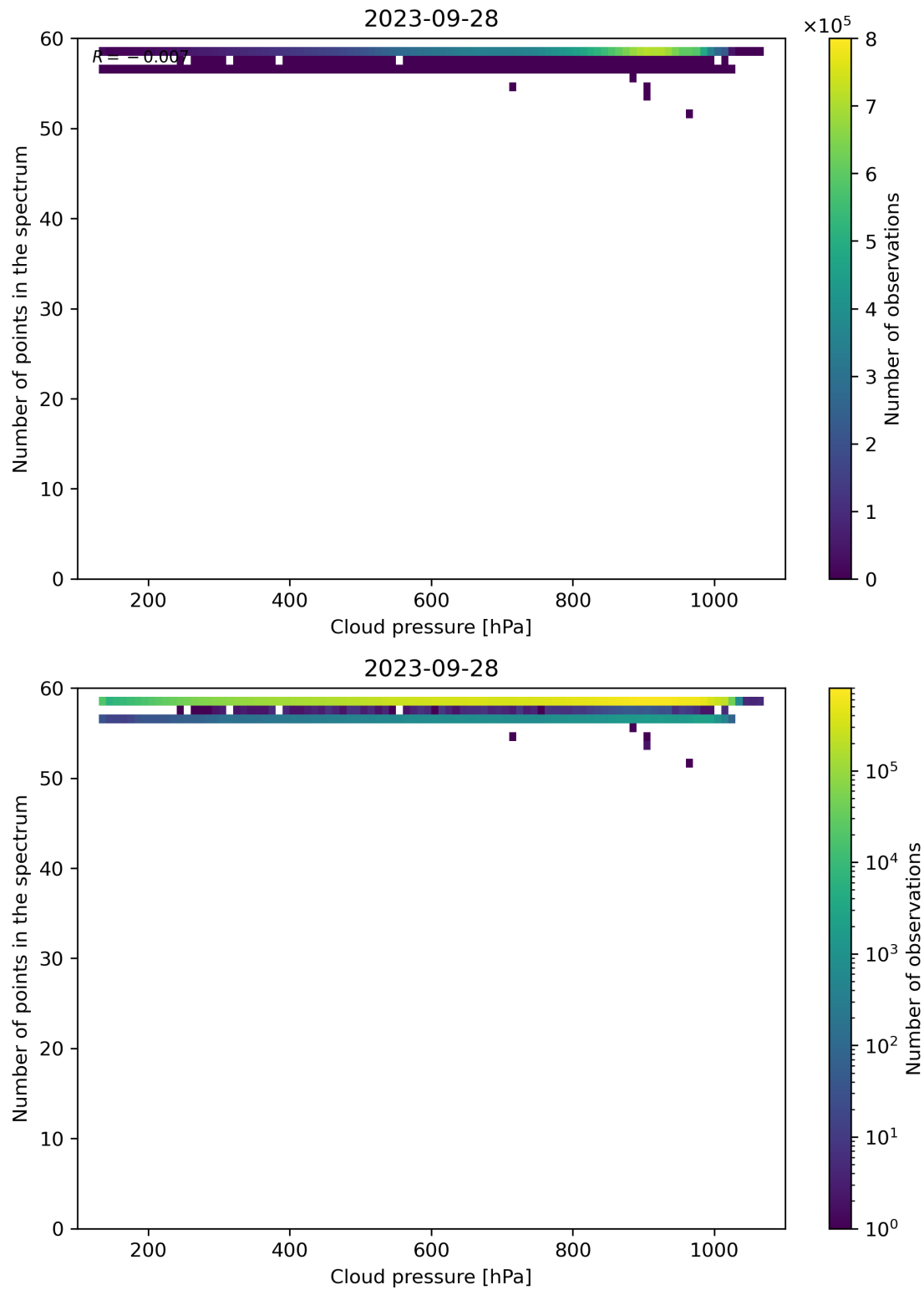
Figure 90: Scatter density plot of “Cloud pressure” against “Number of points in the spectrum” for 2023-09-27 to 2023-09-29.
