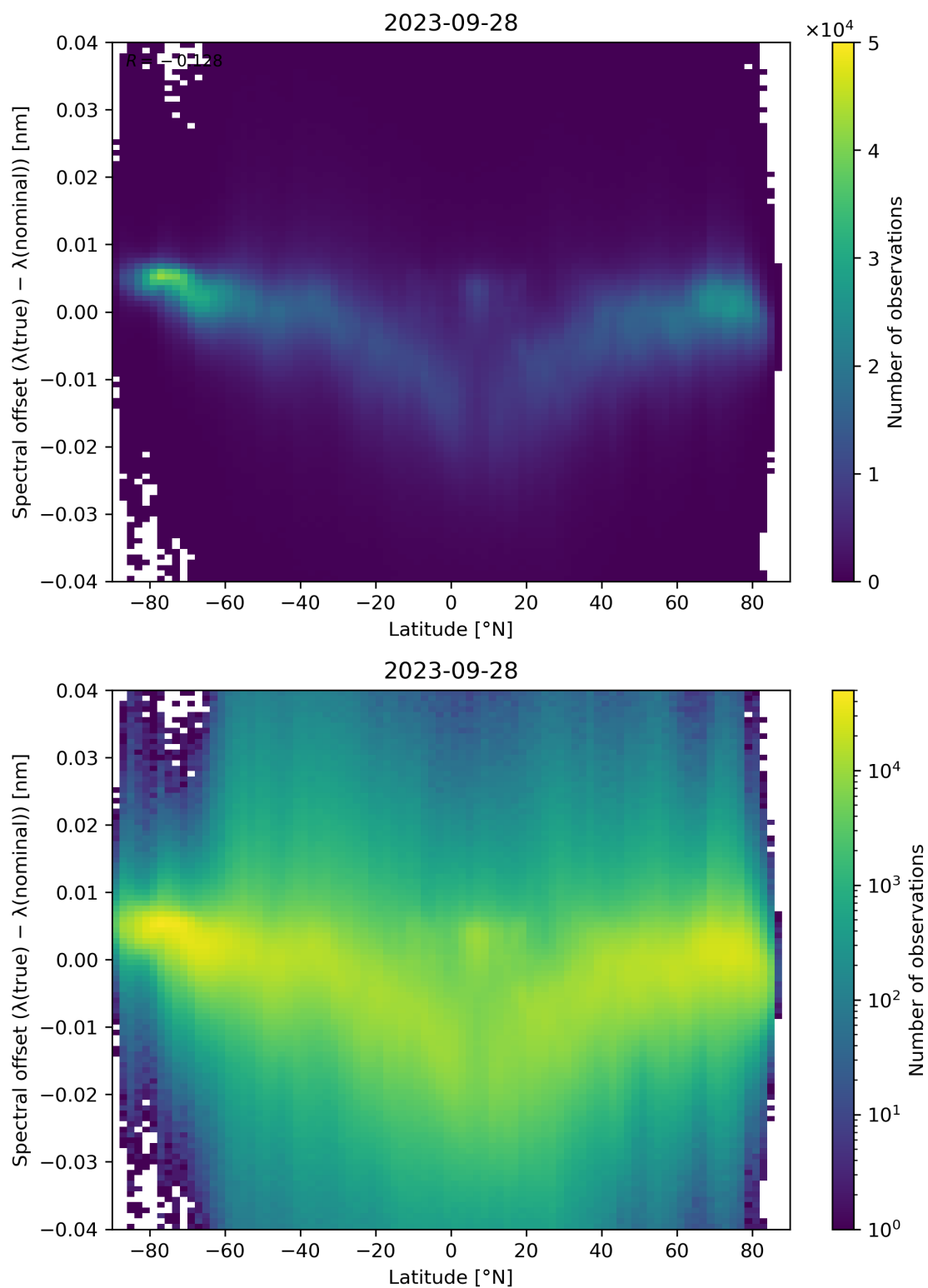
Figure 105: Scatter density plot of “Latitude” against “Spectral offset ( \lambda(\text{true}) - \lambda(\text{nominal}) )” for 2023-09-27 to 2023-09-29.
