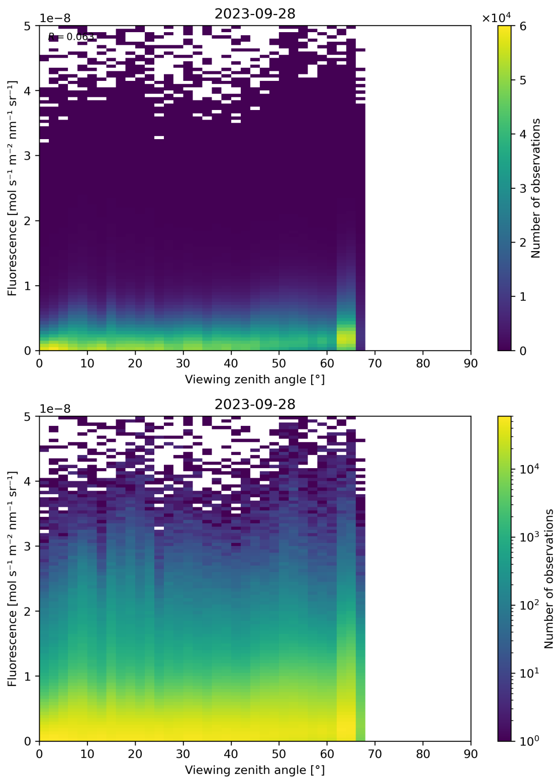
Figure 134: Scatter density plot of “Viewing zenith angle” against “Fluorescence” for 2023-09-27 to 2023-09-29.
