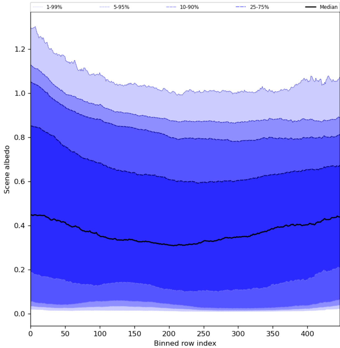
Figure 51: Along track statistics of “Scene albedo” for 2023-09-27 to 2023-09-29
