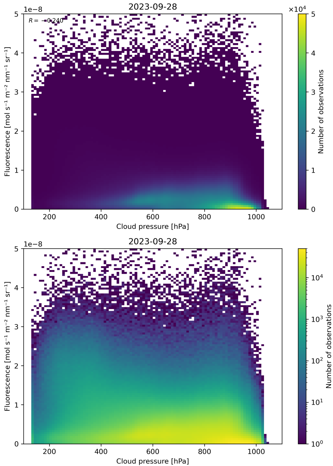
Figure 88: Scatter density plot of “Cloud pressure” against “Fluorescence” for 2023-09-27 to 2023-09-29.
