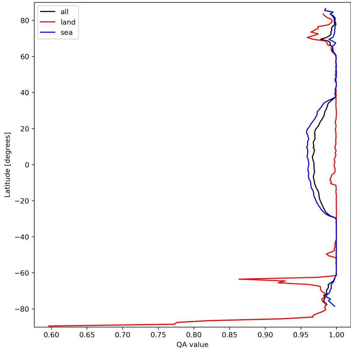
Figure 12: Zonal average of “QA value” for 2023-09-27 to 2023-09-29.
