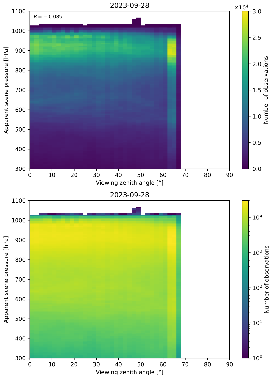
Figure 129: Scatter density plot of “Viewing zenith angle” against “Apparent scene pressure” for 2023-09-27 to 2023-09-29.
