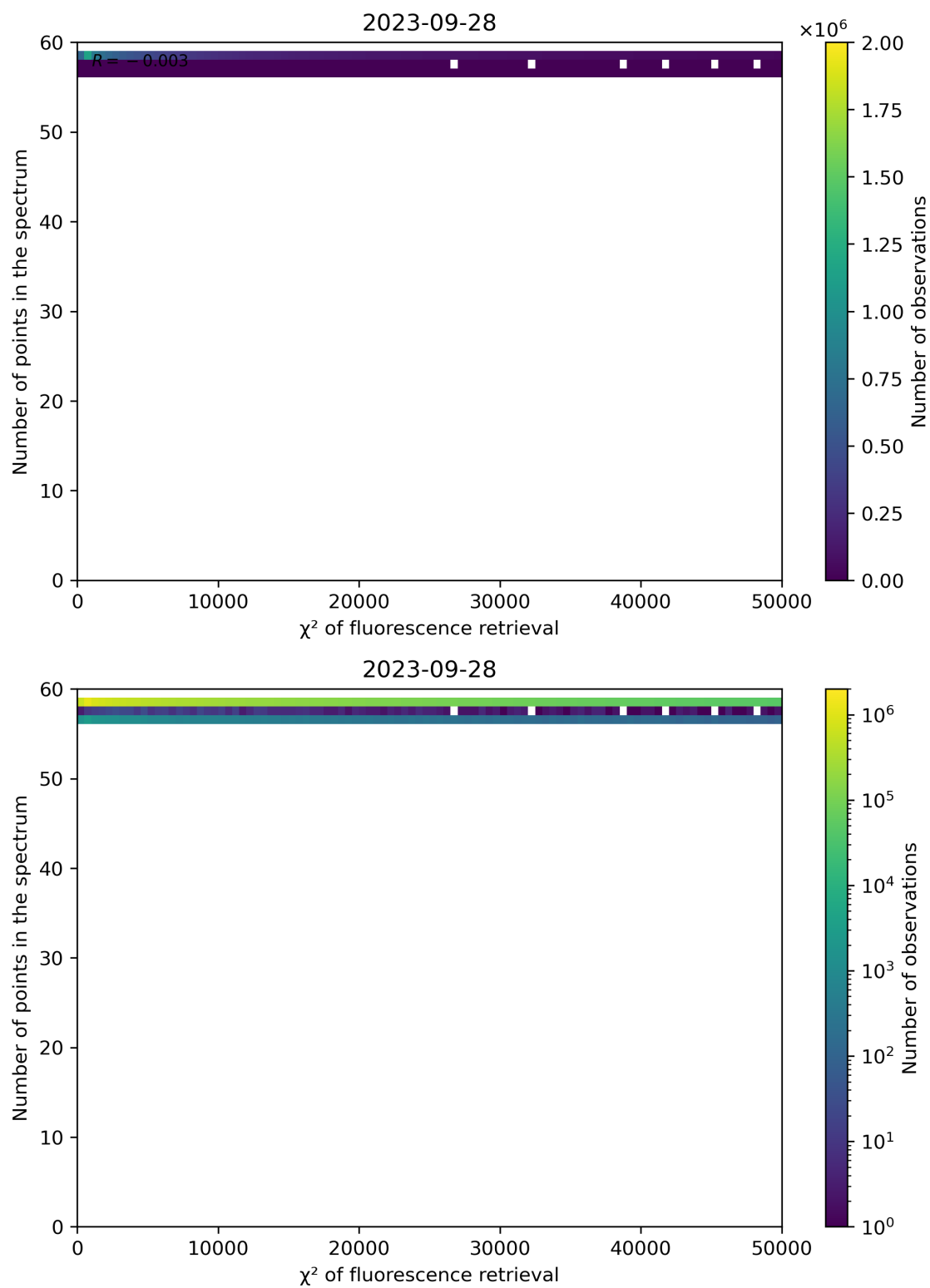
Figure 71: Scatter density plot of " \chi^2 of fluorescence retrieval" against "Number of points in the spectrum" for 2023-09-27 to 2023-09-29.
