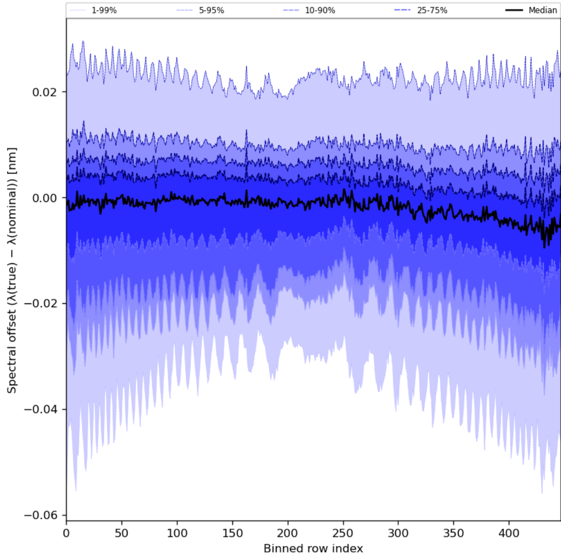
Figure 62: Along track statistics of “Spectral offset ( \lambda(\text{true}) - \lambda(\text{nominal}) )” for 2023-09-27 to 2023-09-29
