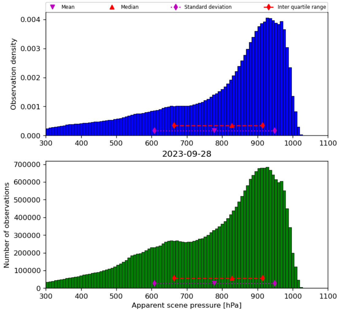
Figure 36: Histogram of “Apparent scene pressure” for 2023-09-27 to 2023-09-29
