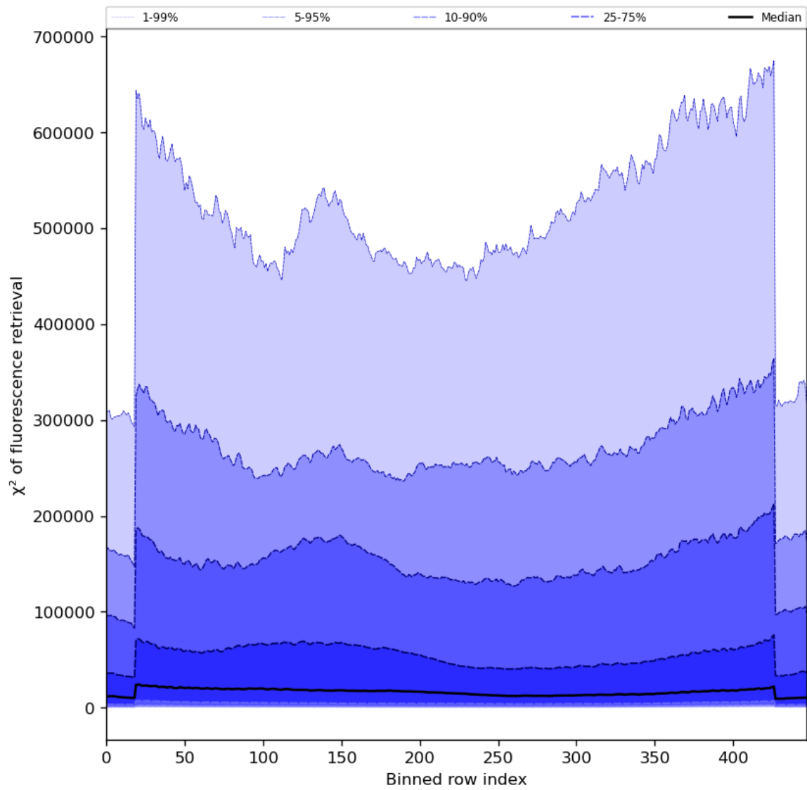
Figure 59: Along track statistics of “ \chi^2 of fluorescence retrieval” for 2023-09-27 to 2023-09-29
