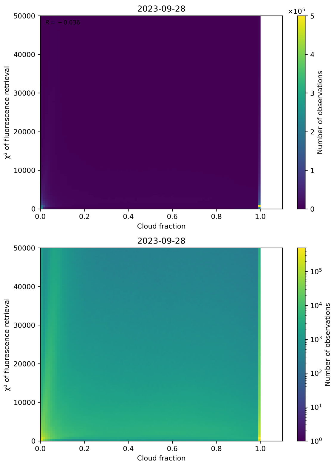
Figure 78: Scatter density plot of “Cloud fraction” against “ \chi^2 of fluorescence retrieval” for 2023-09-27 to 2023-09-29.
