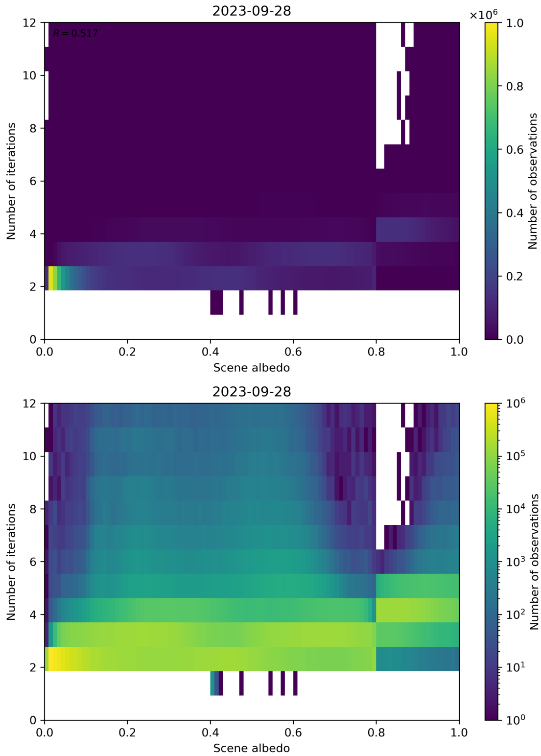
Figure 115: Scatter density plot of “Scene albedo” against “Number of iterations” for 2023-09-27 to 2023-09-29.
