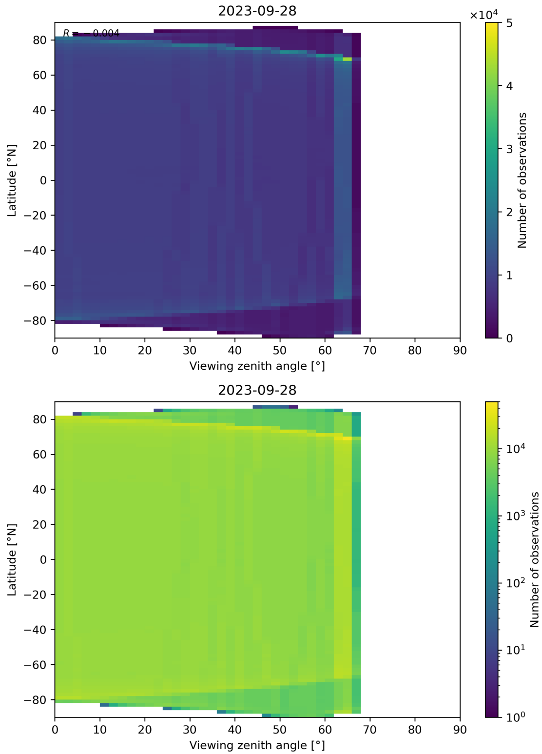
Figure 135: Scatter density plot of “Viewing zenith angle” against “Latitude” for 2023-09-27 to 2023-09-29.
