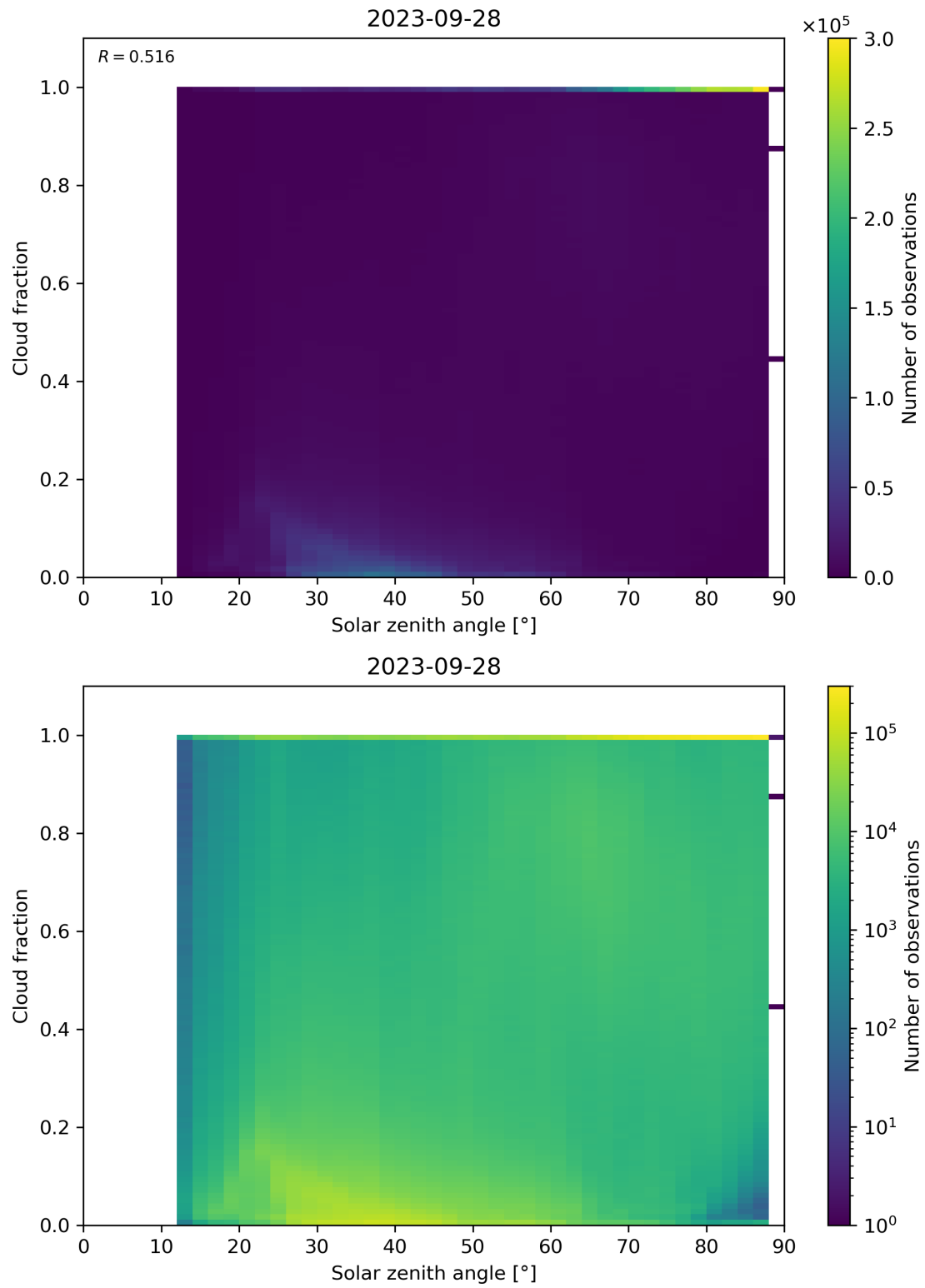
Figure 121: Scatter density plot of “Solar zenith angle” against “Cloud fraction” for 2023-09-27 to 2023-09-29.
