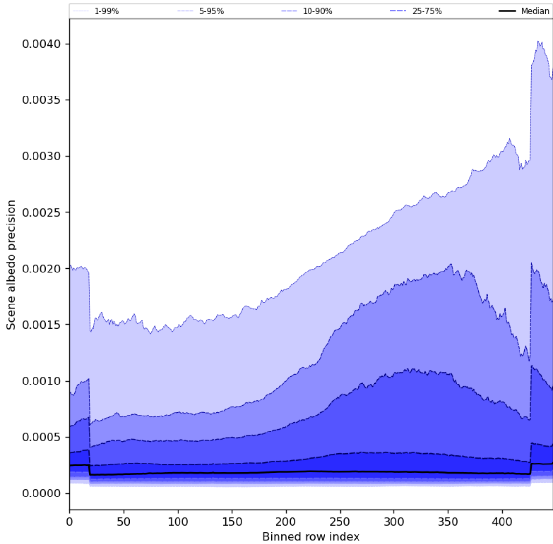
Figure 52: Along track statistics of “Scene albedo precision” for 2023-09-27 to 2023-09-29
