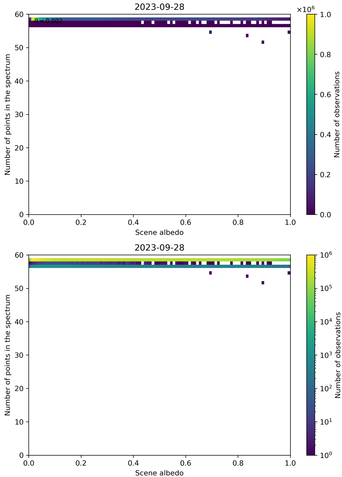
Figure 116: Scatter density plot of “Scene albedo” against “Number of points in the spectrum” for 2023-09-27 to 2023-09-29.
