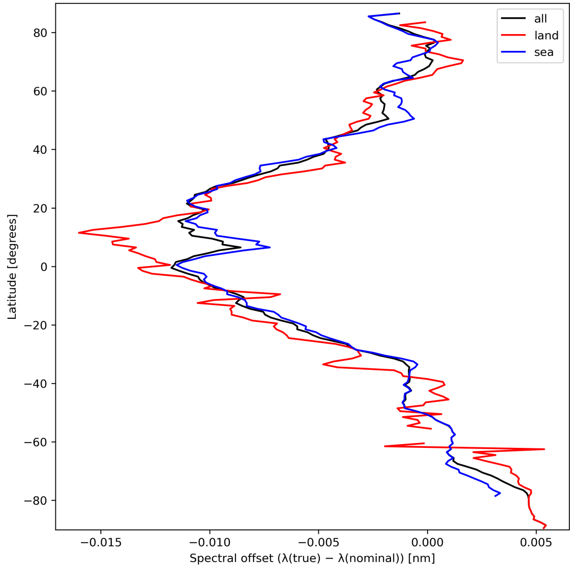
Figure 28: Zonal average of “Spectral offset ( \lambda(\text{true}) - \lambda(\text{nominal}) )” for 2023-09-27 to 2023-09-29.
