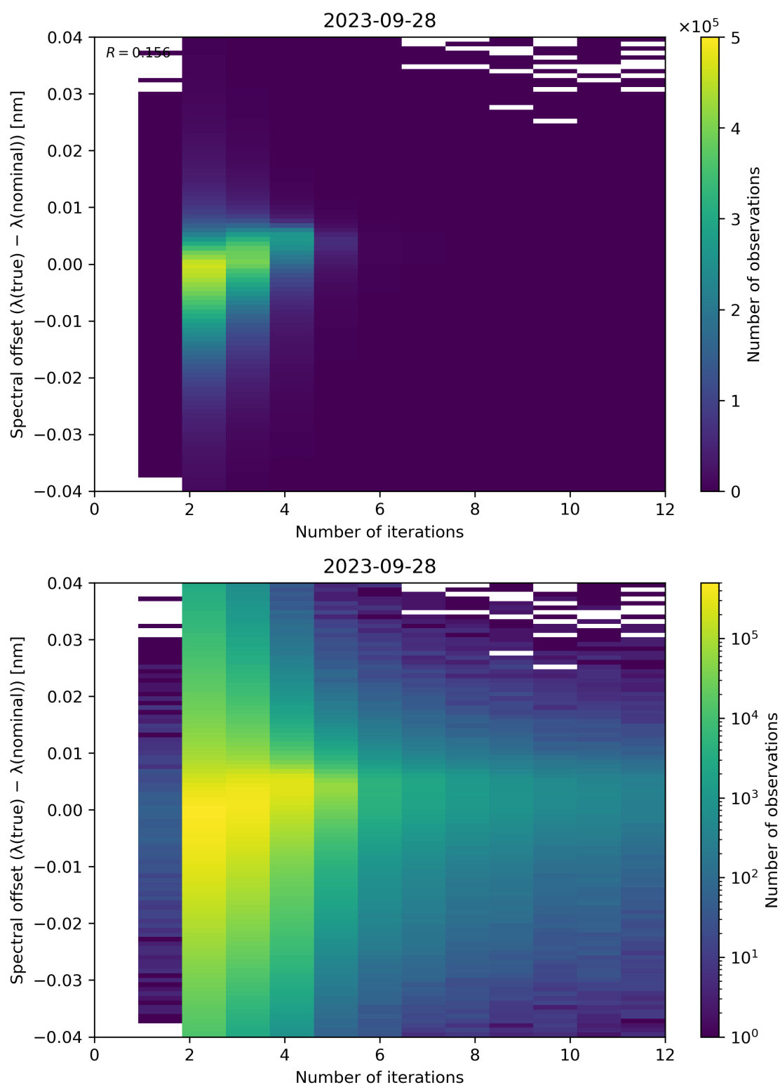
Figure 109: Scatter density plot of “Number of iterations” against “Spectral offset ( \lambda(\text{true}) - \lambda(\text{nominal}) )” for 2023-09-27 to 2023-09-29.
