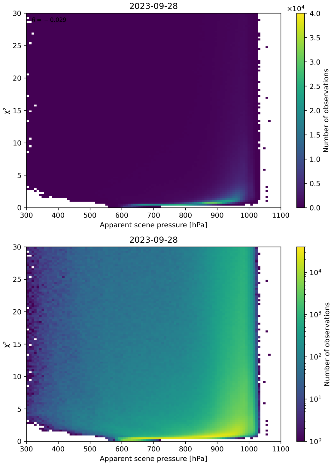
Figure 63: Scatter density plot of “Apparent scene pressure” against “ \chi^2 ” for 2023-09-27 to 2023-09-29.
