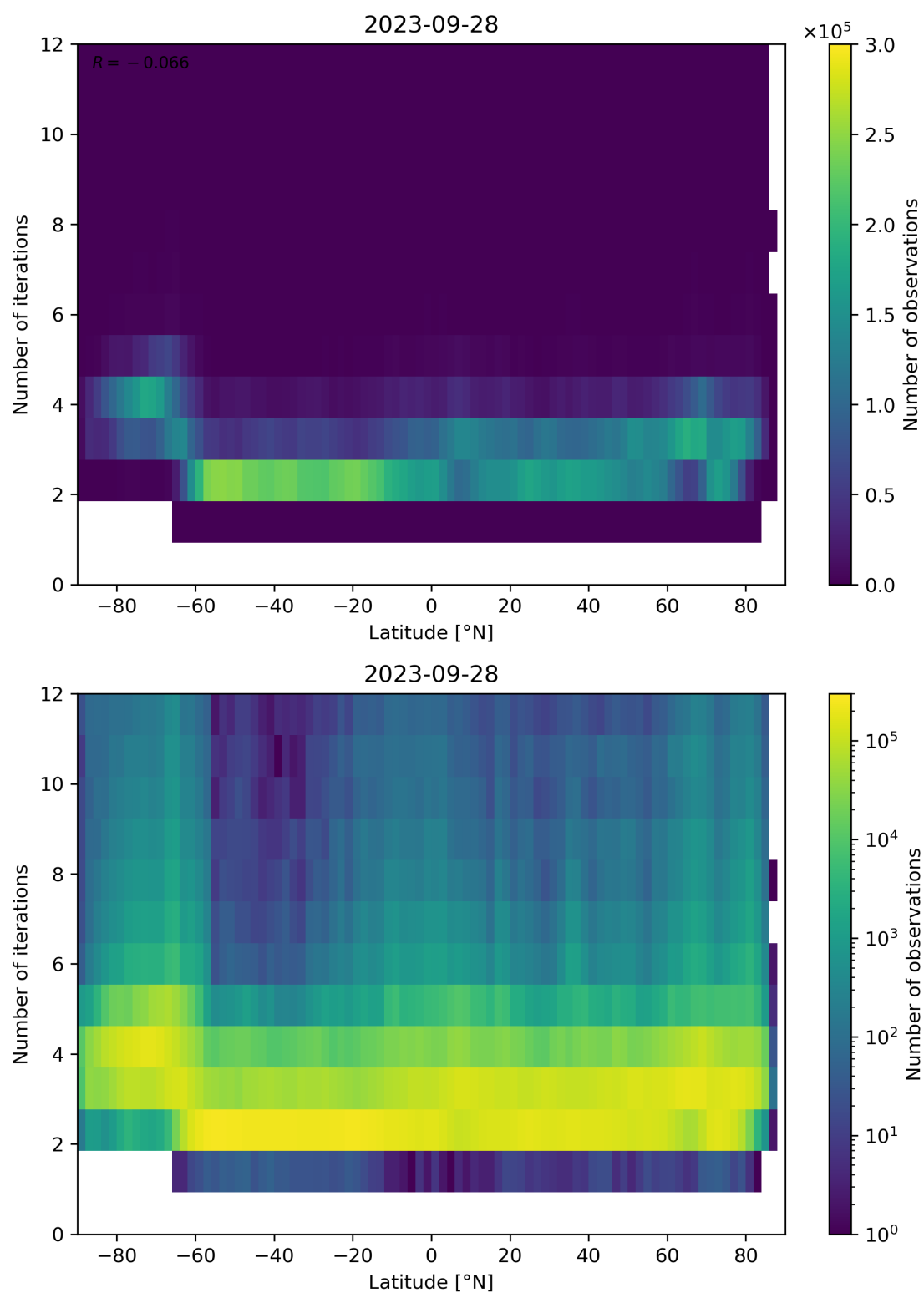
Figure 102: Scatter density plot of “Latitude” against “Number of iterations” for 2023-09-27 to 2023-09-29.
