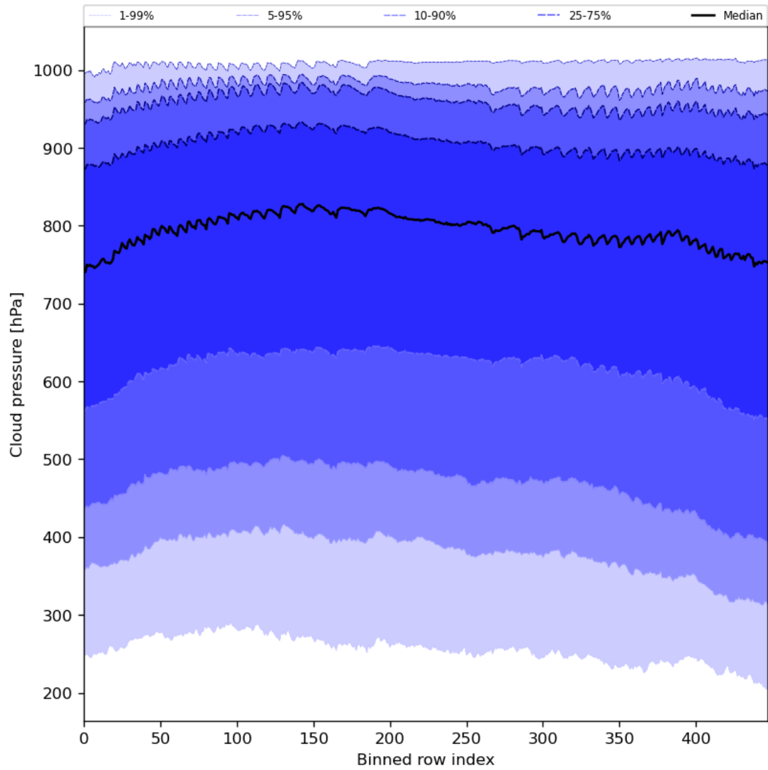
Figure 47: Along track statistics of “Cloud pressure” for 2023-09-27 to 2023-09-29
