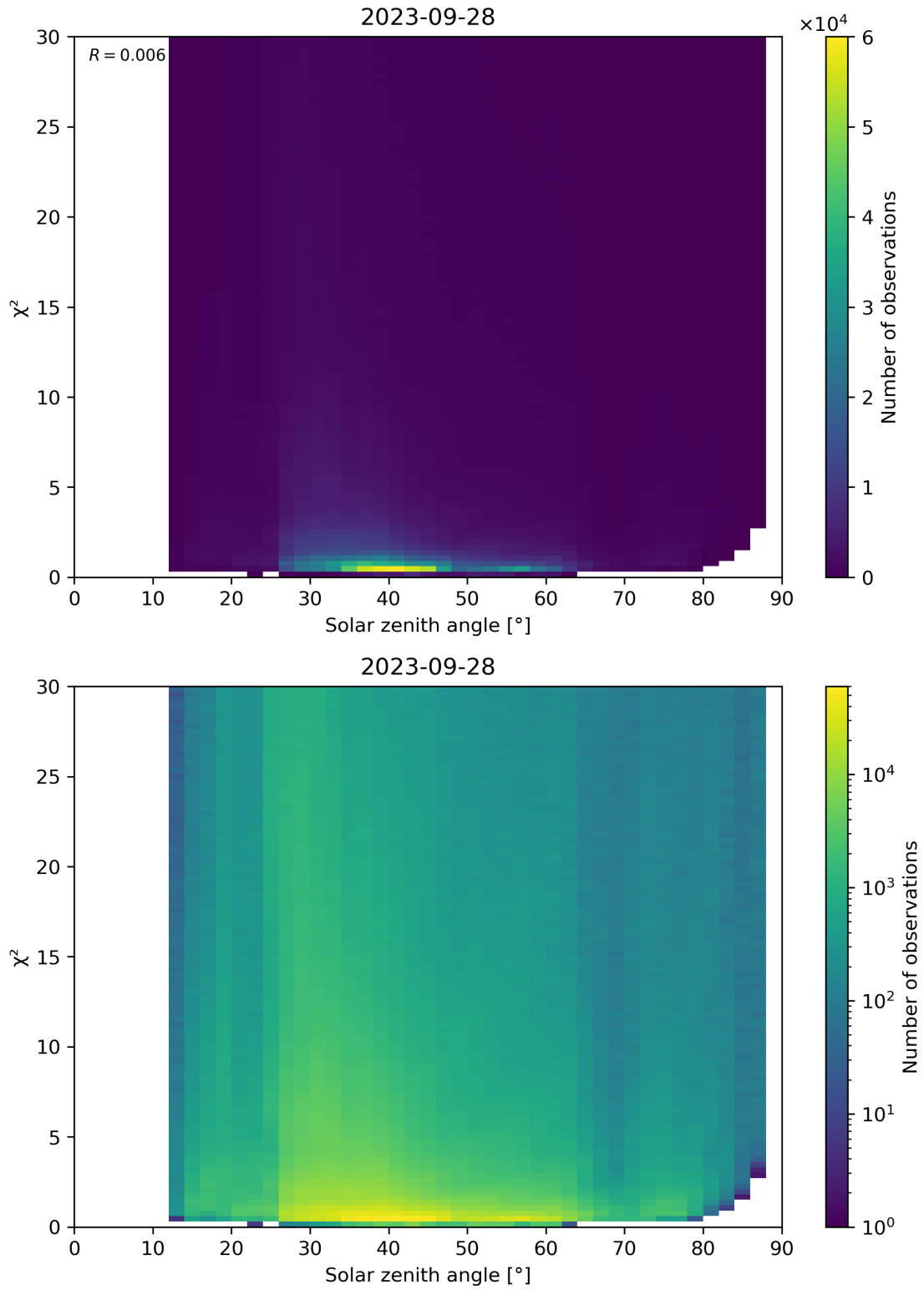
Figure 119: Scatter density plot of “Solar zenith angle” against “ \chi^2 ” for 2023-09-27 to 2023-09-29.
