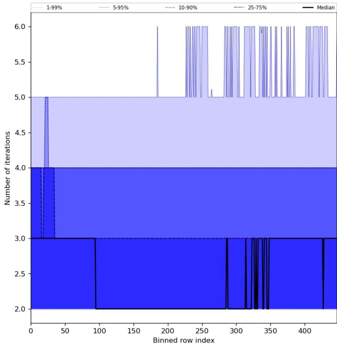
Figure 56: Along track statistics of “Number of iterations” for 2023-09-27 to 2023-09-29
