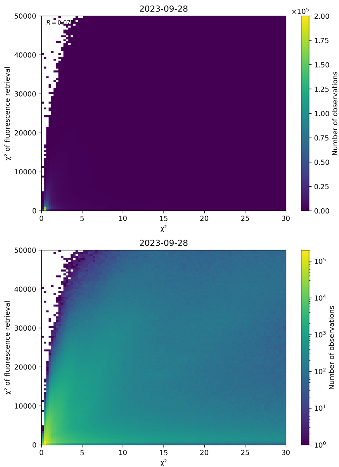
Figure 69: Scatter density plot of “ \chi^2 ” against “ \chi^2 of fluorescence retrieval” for 2023-09-27 to 2023-09-29.
