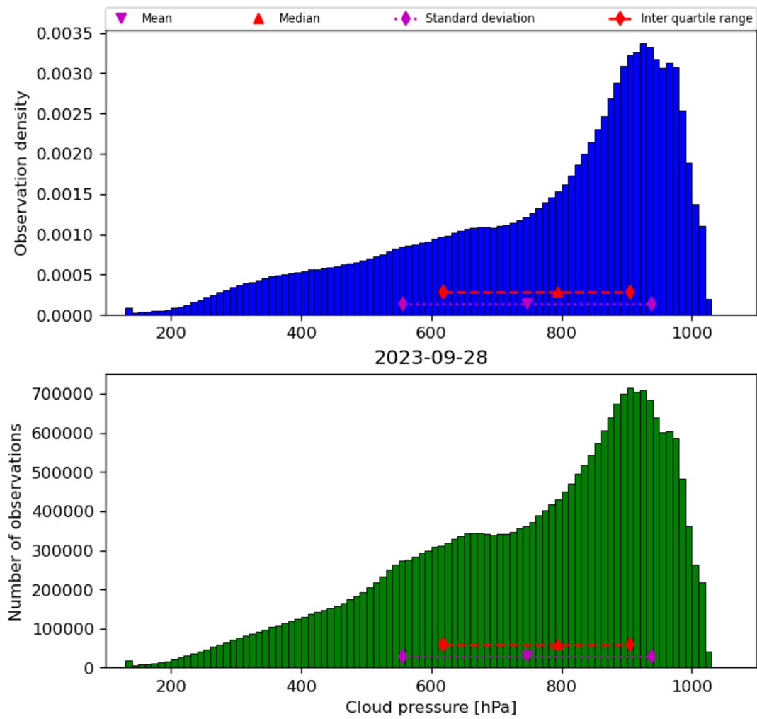
Figure 30: Histogram of “Cloud pressure” for 2023-09-27 to 2023-09-29
