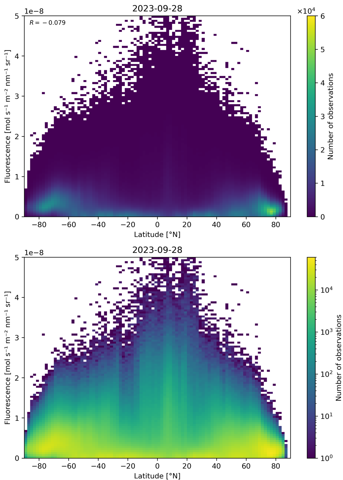
Figure 101: Scatter density plot of “Latitude” against “Fluorescence” for 2023-09-27 to 2023-09-29.
