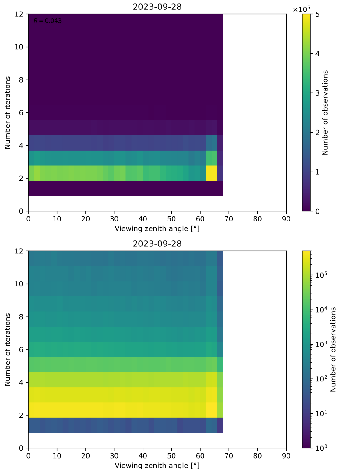
Figure 136: Scatter density plot of “Viewing zenith angle” against “Number of iterations” for 2023-09-27 to 2023-09-29.
