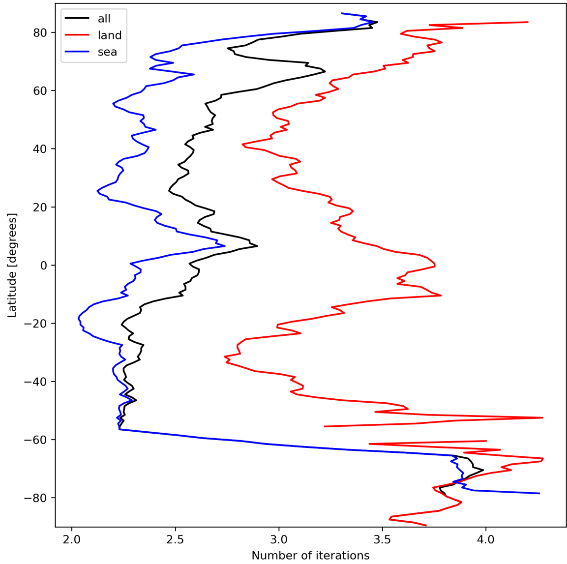
Figure 22: Zonal average of “Number of iterations” for 2023-09-27 to 2023-09-29.
