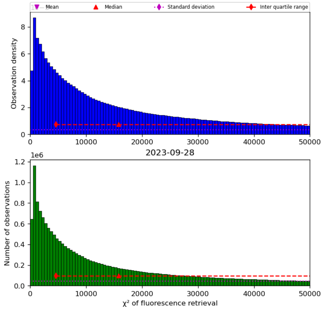
Figure 42: Histogram of “ \chi^2 of fluorescence retrieval” for 2023-09-27 to 2023-09-29
