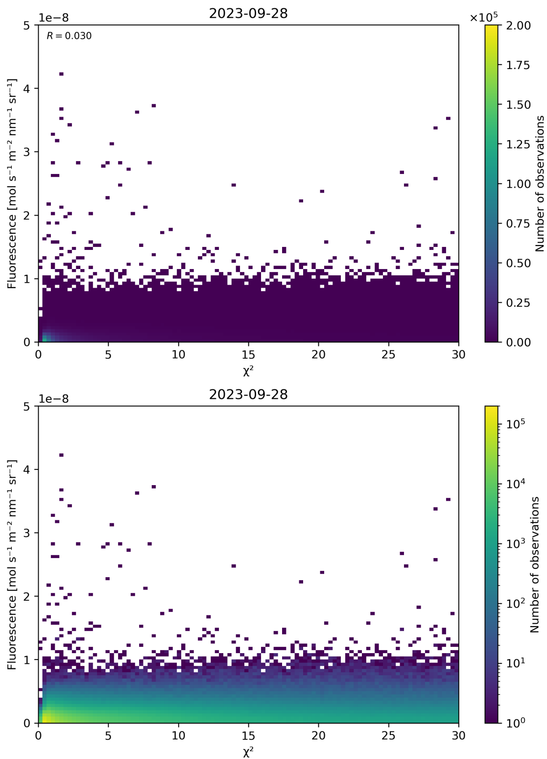
Figure 70: Scatter density plot of “ \chi^2 ” against “Fluorescence” for 2023-09-27 to 2023-09-29.
