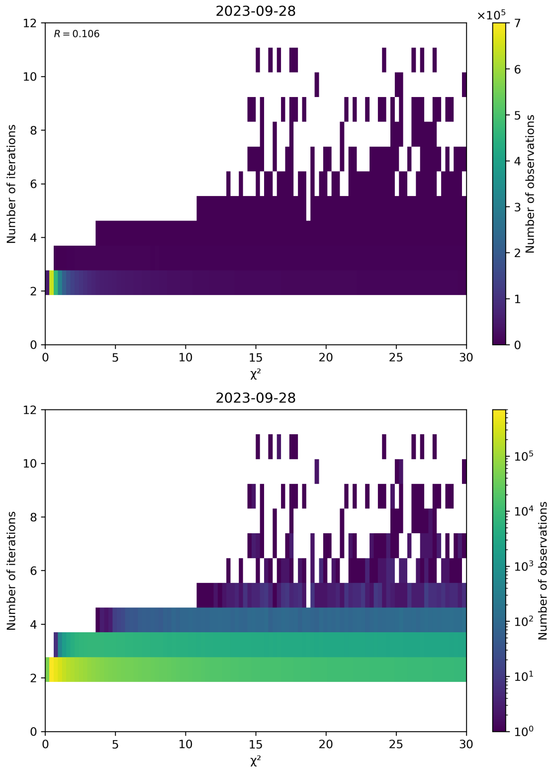
Figure 73: Scatter density plot of “ \chi^2 ” against “Number of iterations” for 2023-09-27 to 2023-09-29.
