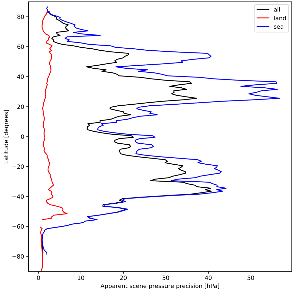
Figure 20: Zonal average of “Apparent scene pressure precision” for 2023-09-27 to 2023-09-29.
