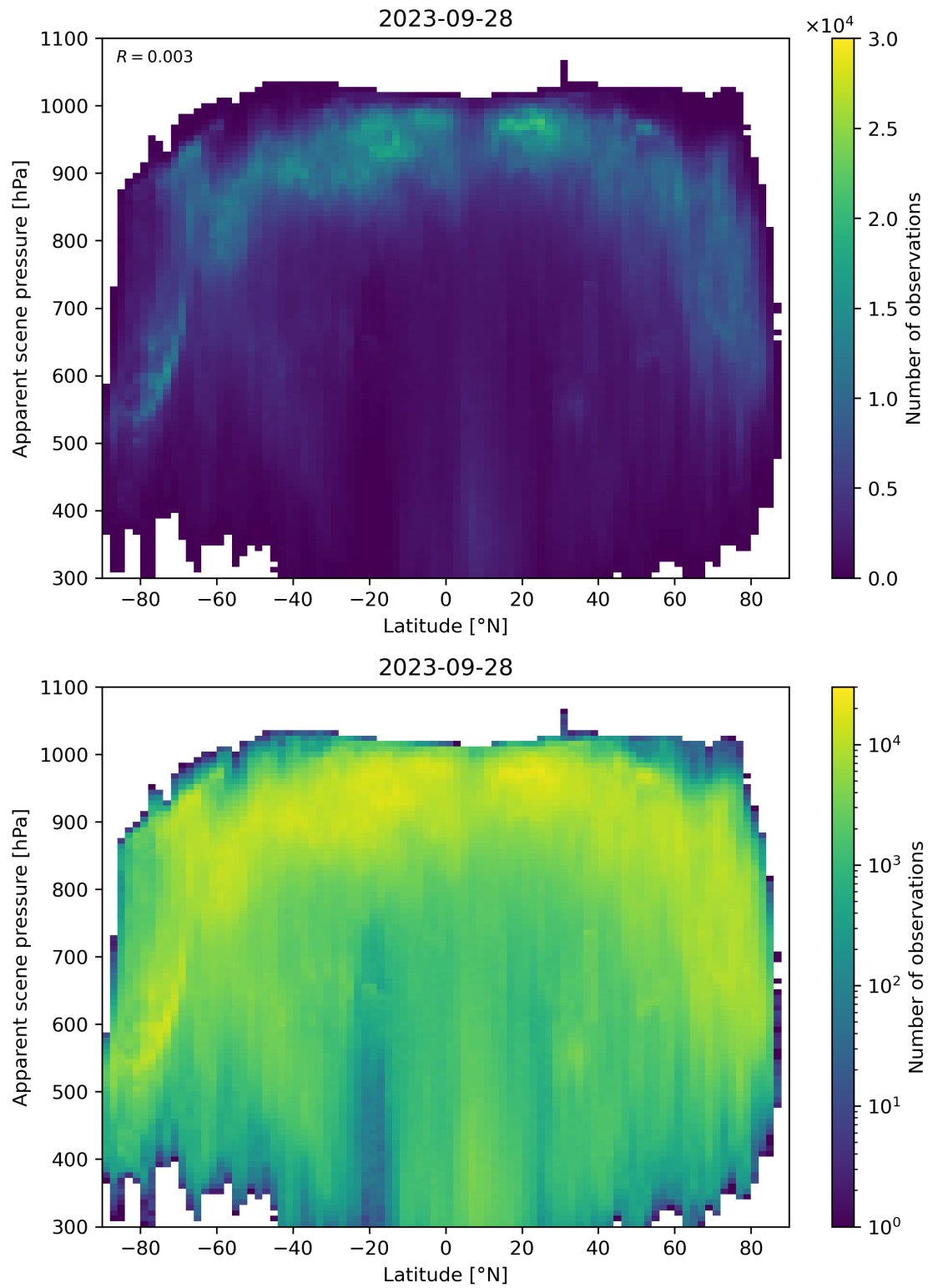
Figure 96: Scatter density plot of “Latitude” against “Apparent scene pressure” for 2023-09-27 to 2023-09-29.
