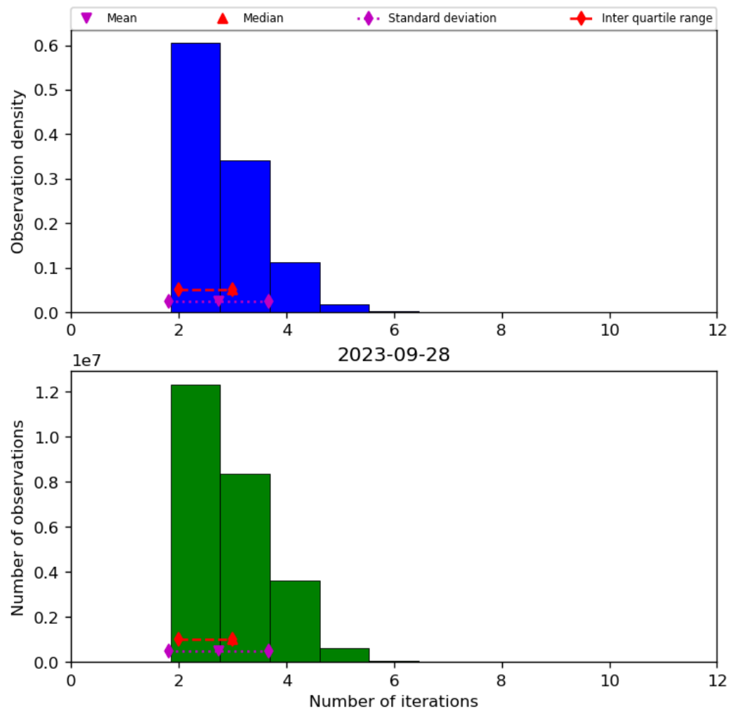
Figure 39: Histogram of “Number of iterations” for 2023-09-27 to 2023-09-29
