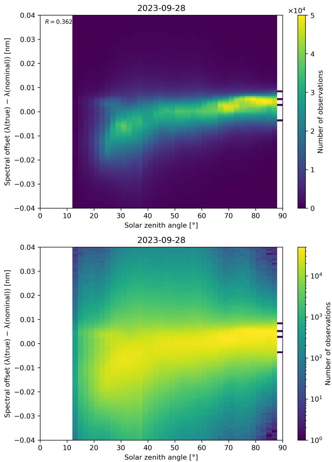
Figure 128: Scatter density plot of “Solar zenith angle” against “Spectral offset ( \lambda(\text{true}) - \lambda(\text{nominal}) )” for 2023-09-27 to 2023-09-29.
