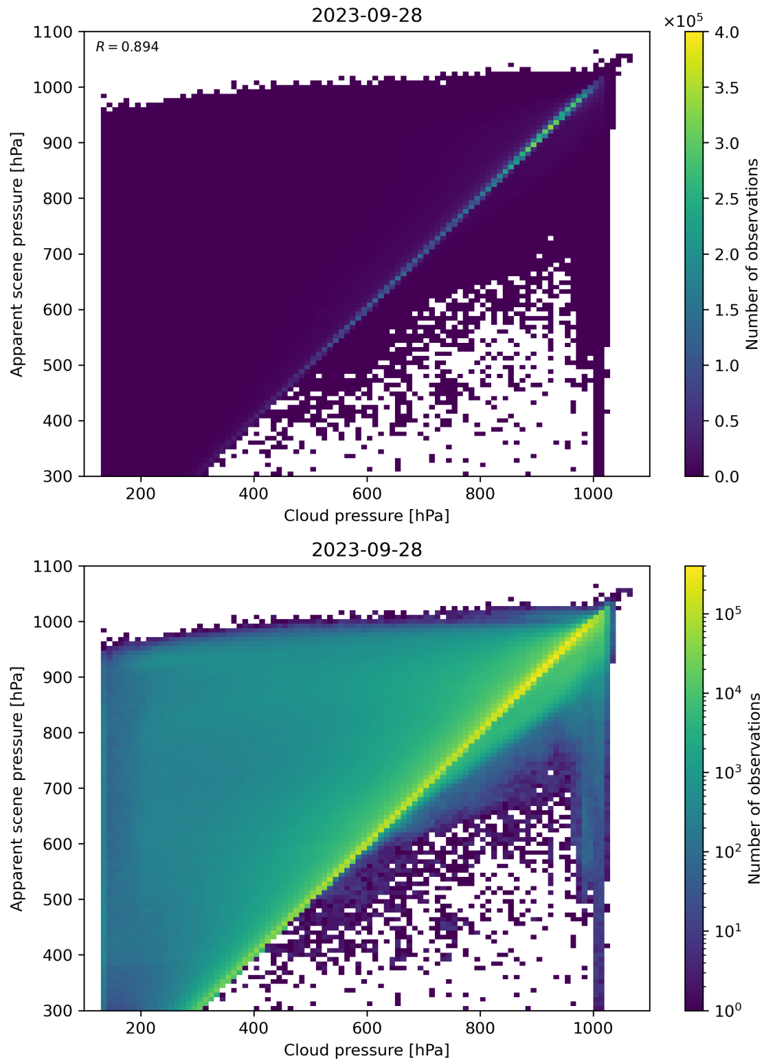
Figure 84: Scatter density plot of “Cloud pressure” against “Apparent scene pressure” for 2023-09-27 to 2023-09-29.
