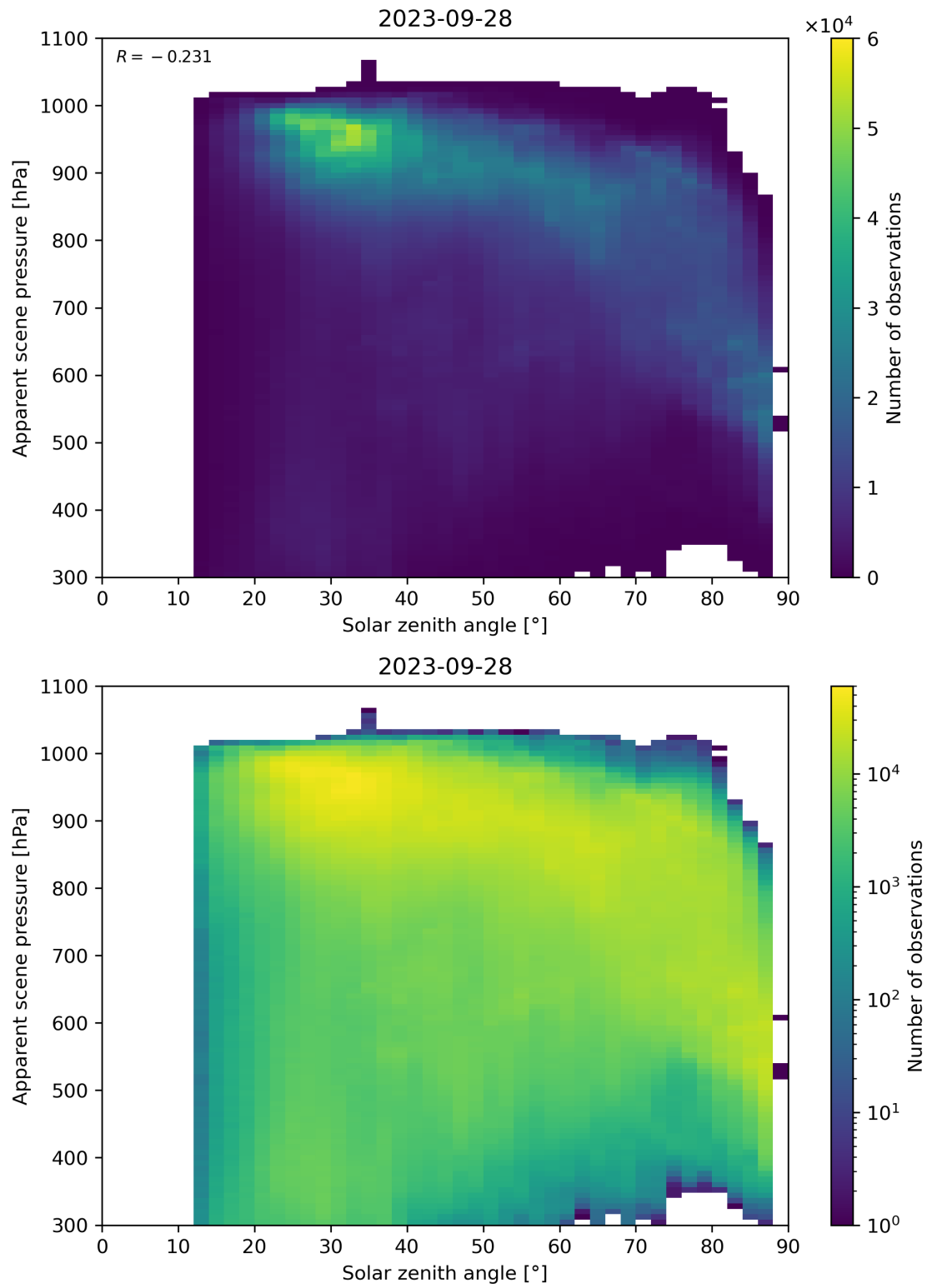
Figure 118: Scatter density plot of “Solar zenith angle” against “Apparent scene pressure” for 2023-09-27 to 2023-09-29.
