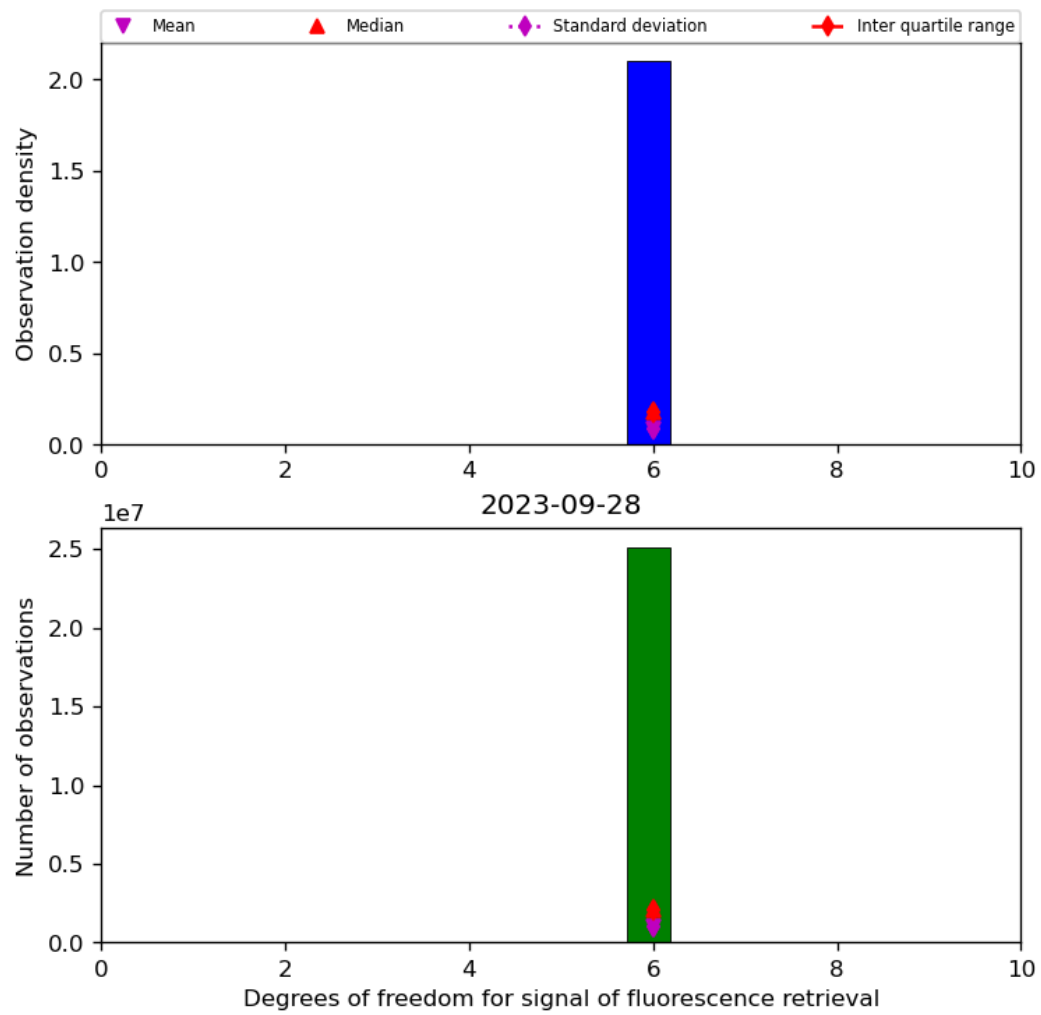
Figure 43: Histogram of “Degrees of freedom for signal of fluorescence retrieval” for 2023-09-27 to 2023-09-29
