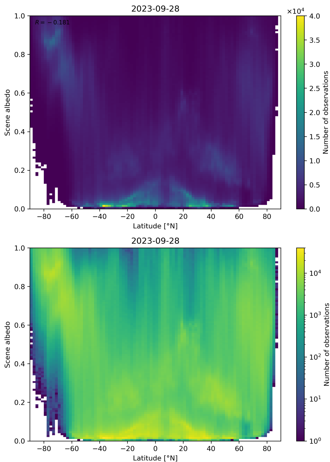
Figure 104: Scatter density plot of “Latitude” against “Scene albedo” for 2023-09-27 to 2023-09-29.
