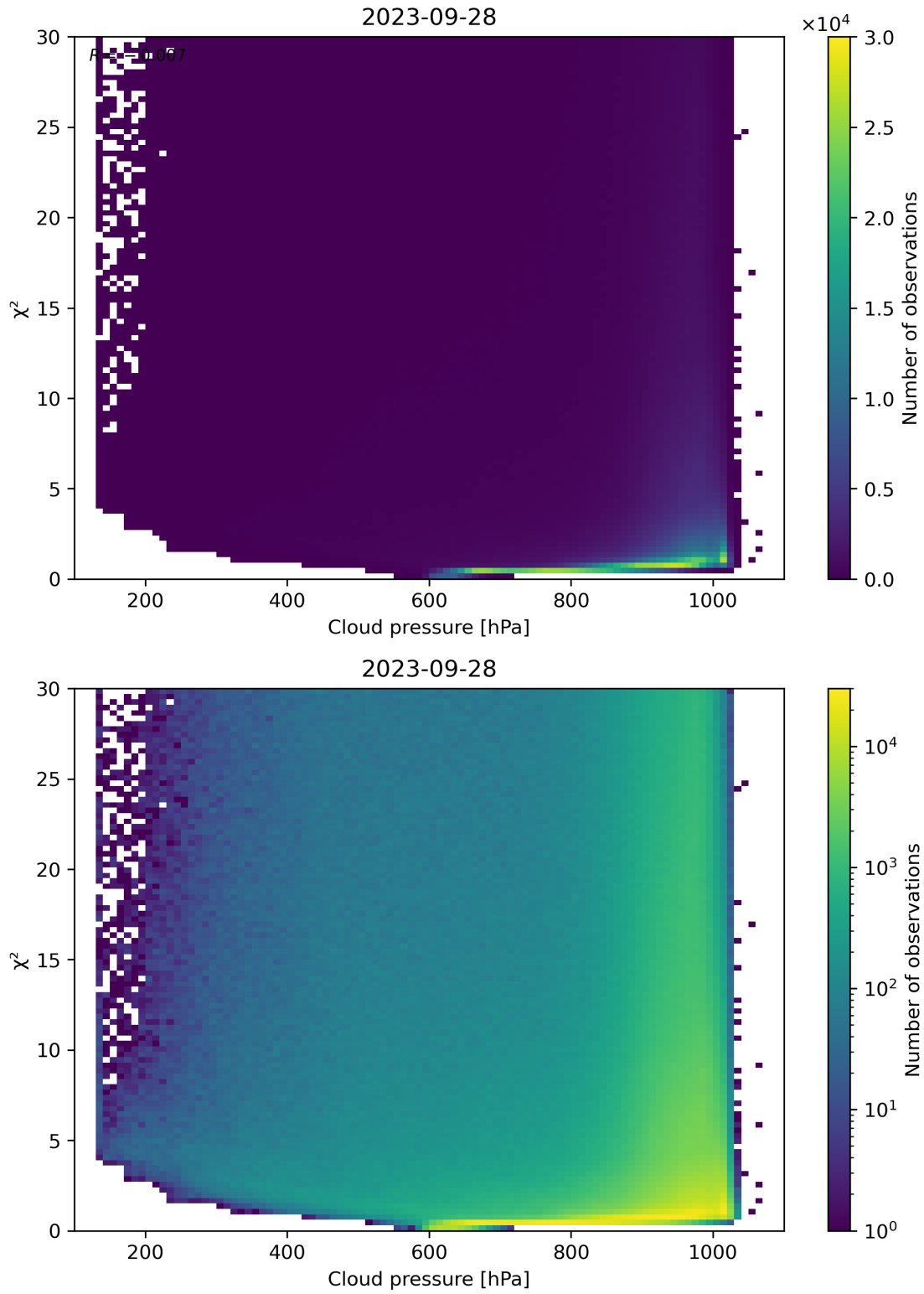
Figure 85: Scatter density plot of “Cloud pressure” against “ \chi^2 ” for 2023-09-27 to 2023-09-29.
