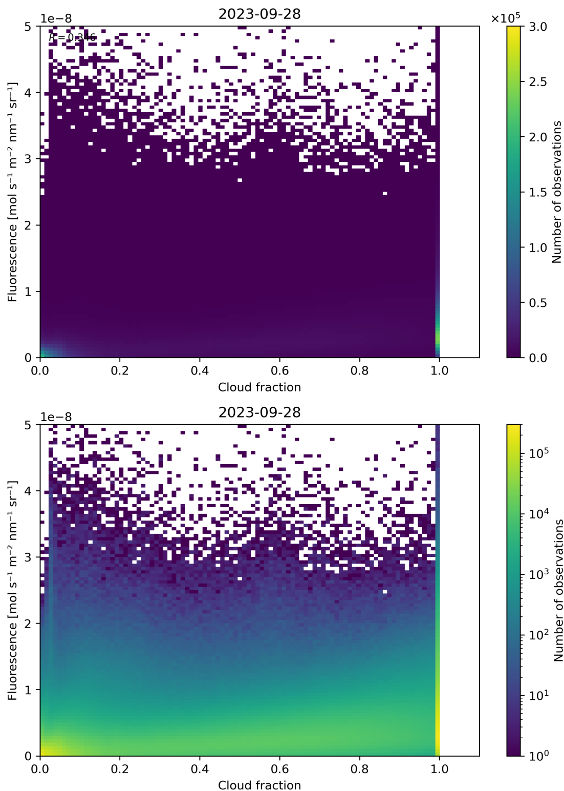
Figure 79: Scatter density plot of “Cloud fraction” against “Fluorescence” for 2023-09-27 to 2023-09-29.
