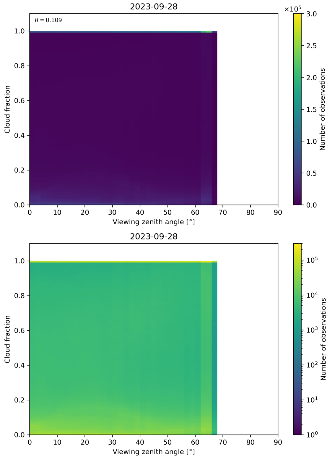
Figure 132: Scatter density plot of “Viewing zenith angle” against “Cloud fraction” for 2023-09-27 to 2023-09-29.
