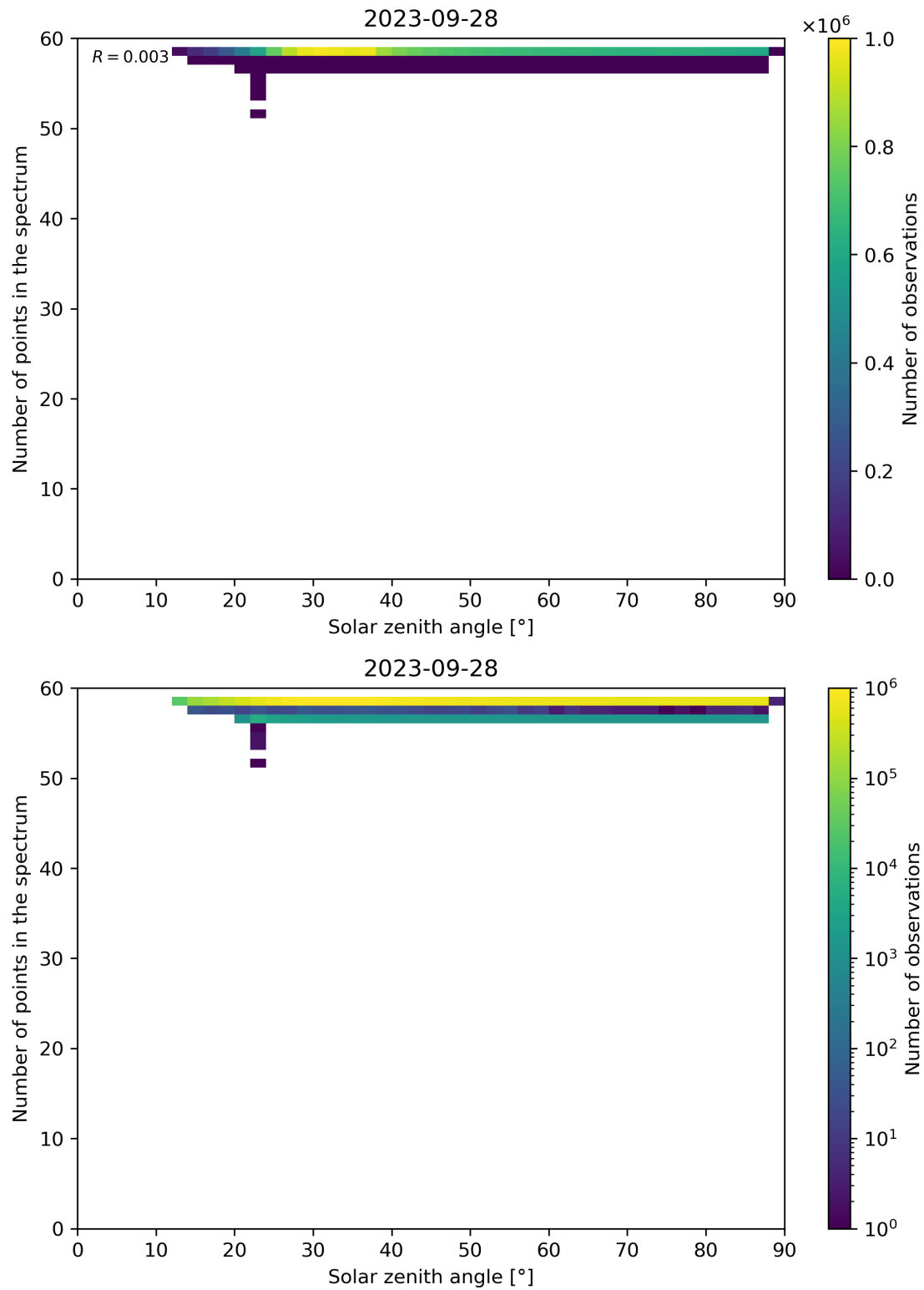
Figure 126: Scatter density plot of “Solar zenith angle” against “Number of points in the spectrum” for 2023-09-27 to 2023-09-29.
