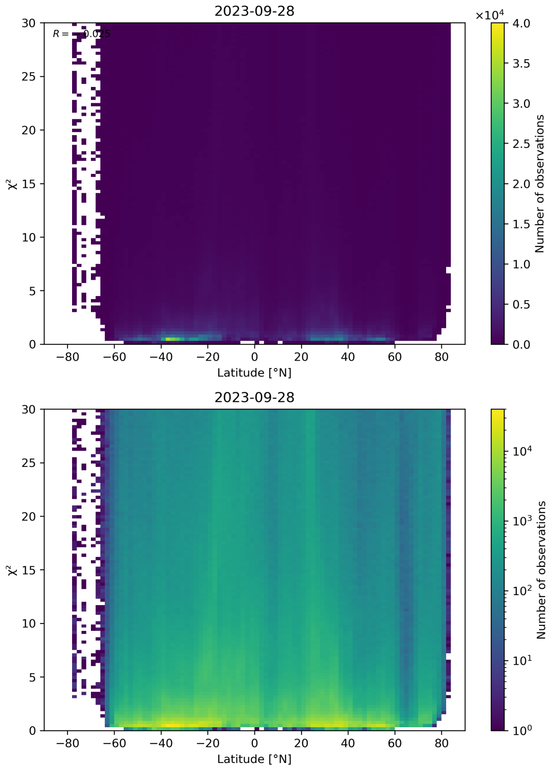
Figure 97: Scatter density plot of “Latitude” against “ \chi^2 ” for 2023-09-27 to 2023-09-29.
