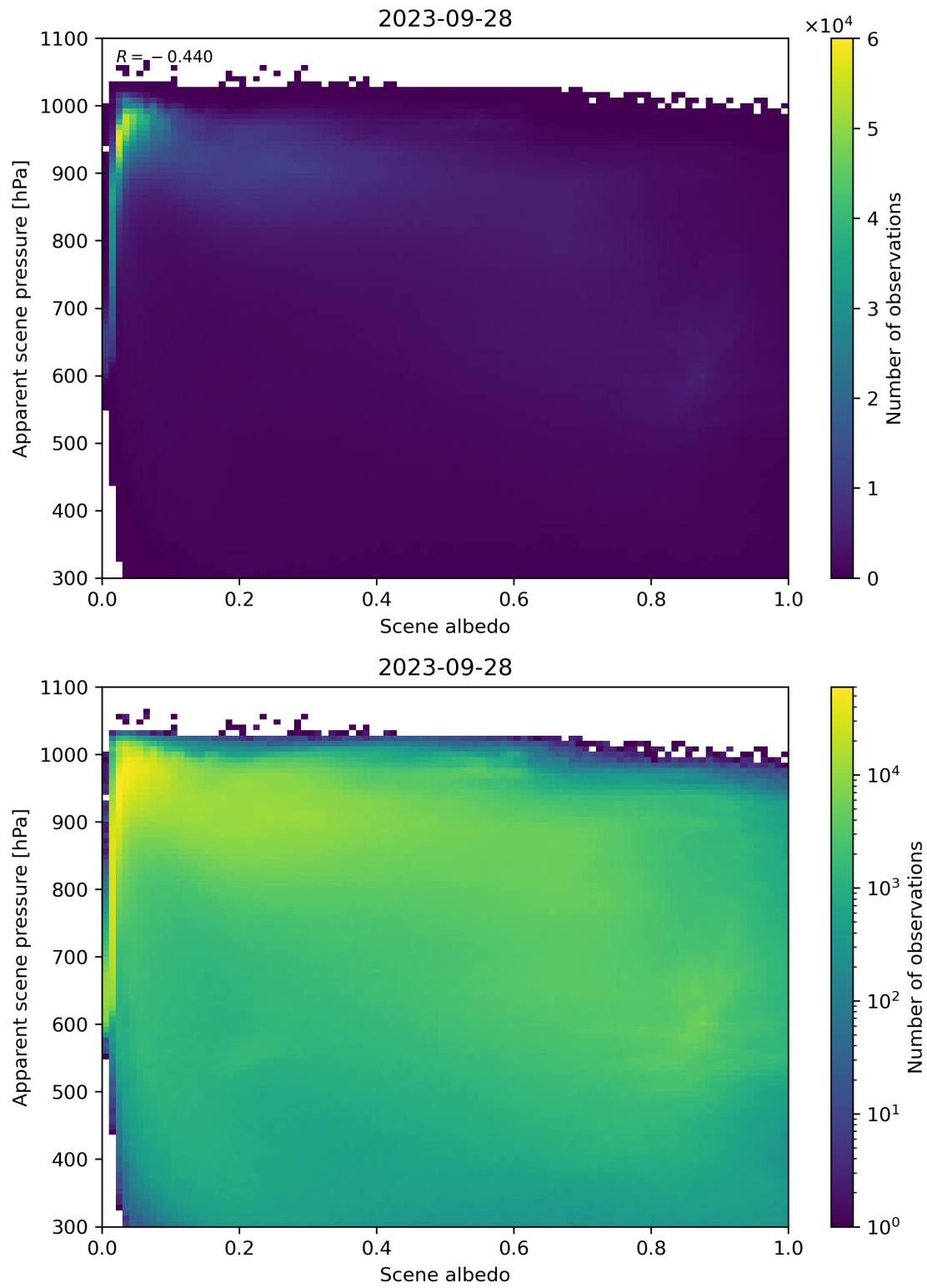
Figure 111: Scatter density plot of “Scene albedo” against “Apparent scene pressure” for 2023-09-27 to 2023-09-29.
