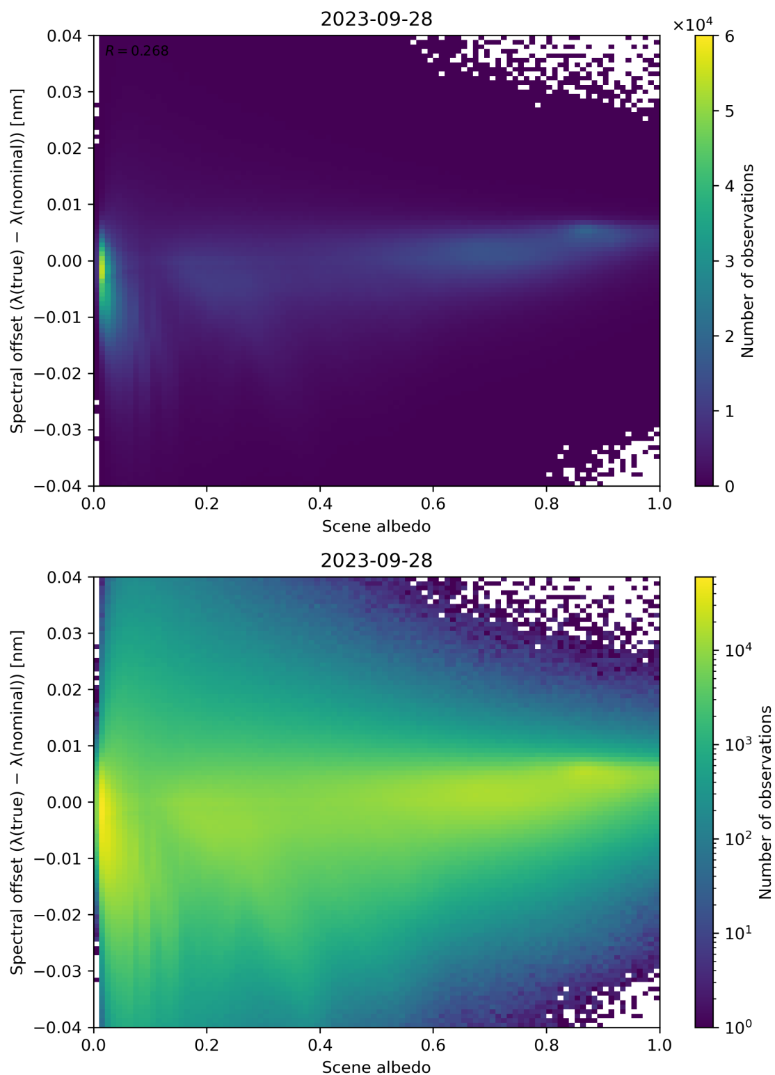
Figure 117: Scatter density plot of “Scene albedo” against “Spectral offset ( \lambda(\text{true}) - \lambda(\text{nominal}) )” for 2023-09-27 to 2023-09-29.
