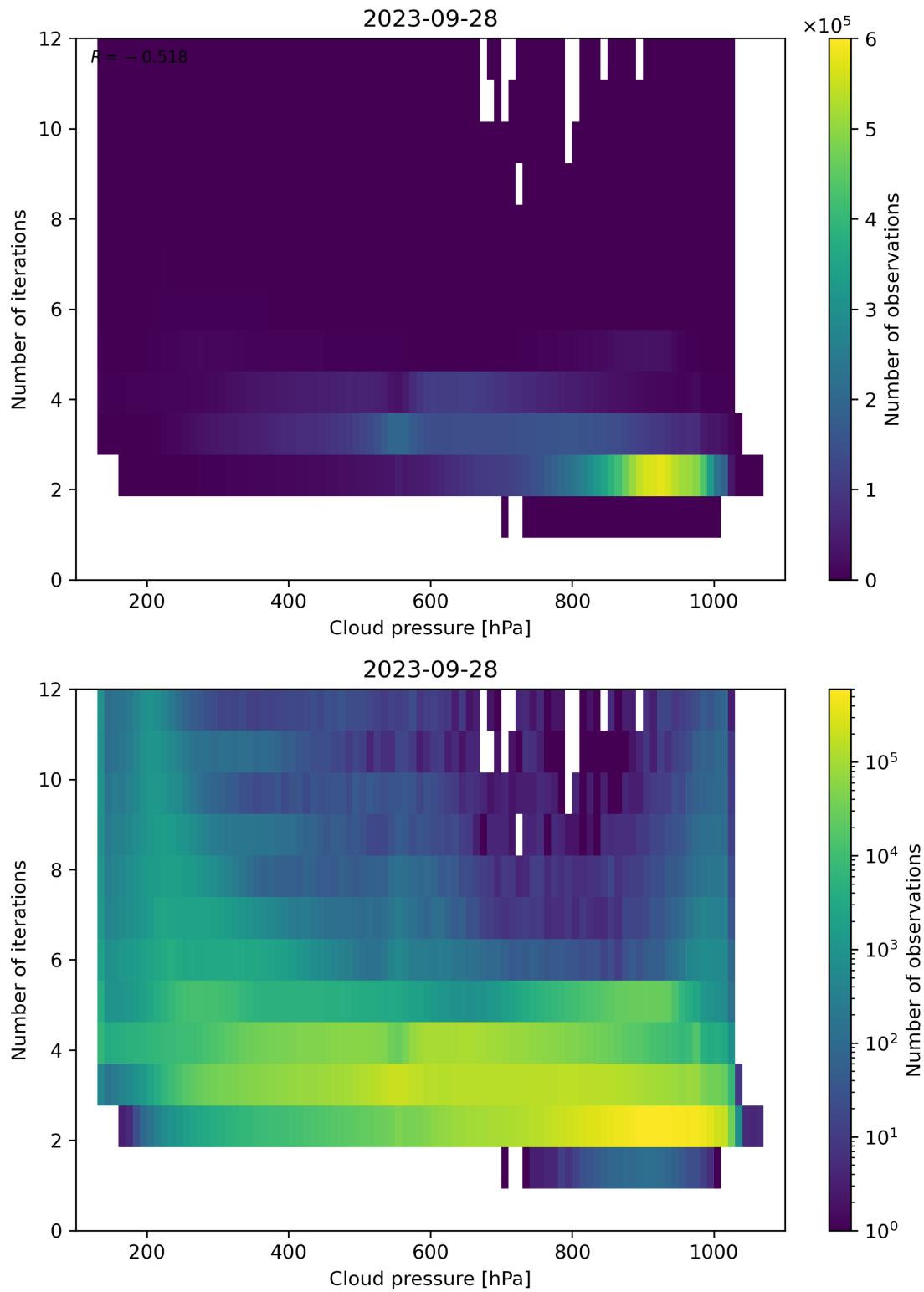
Figure 89: Scatter density plot of “Cloud pressure” against “Number of iterations” for 2023-09-27 to 2023-09-29.
