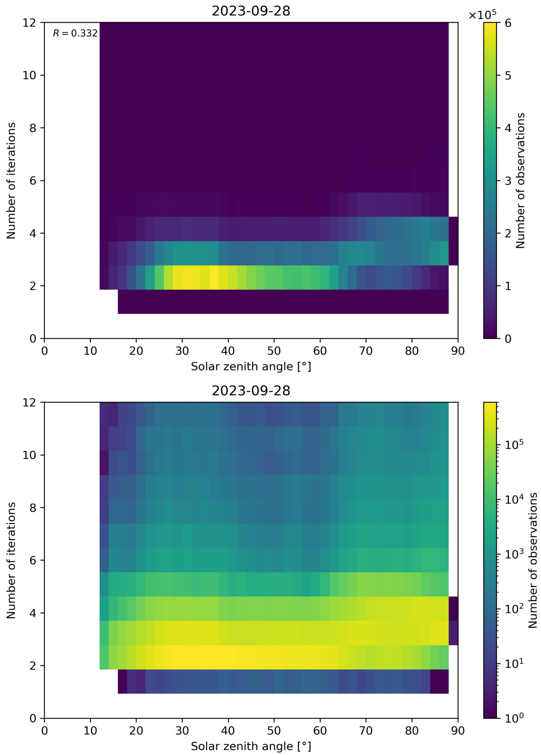
Figure 125: Scatter density plot of “Solar zenith angle” against “Number of iterations” for 2023-09-27 to 2023-09-29.
