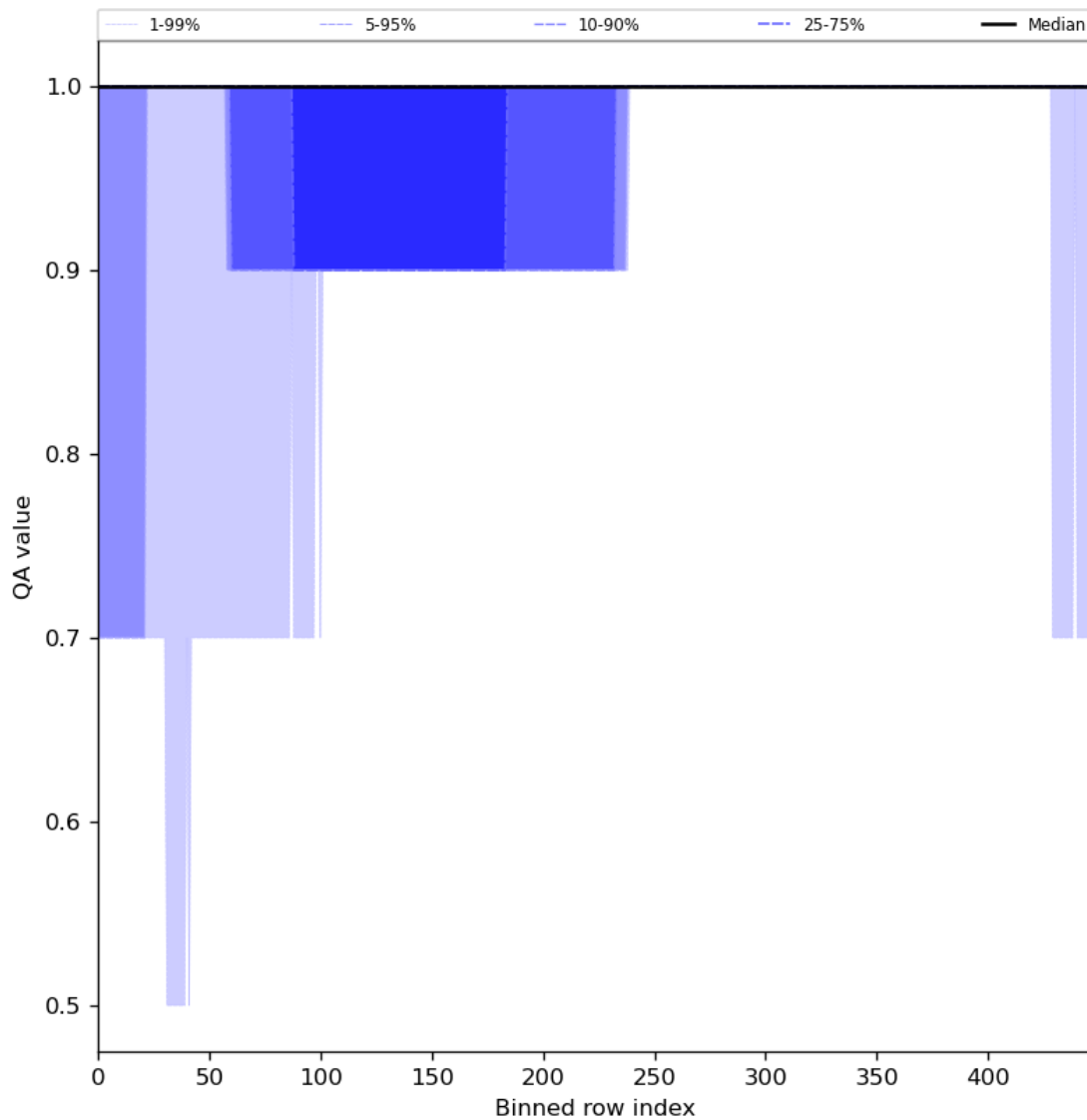
Figure 46: Along track statistics of “QA value” for 2023-09-27 to 2023-09-29
