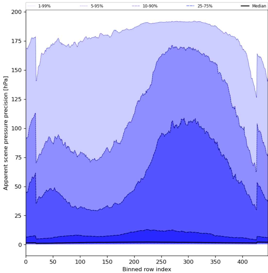
Figure 54: Along track statistics of “Apparent scene pressure precision” for 2023-09-27 to 2023-09-29
