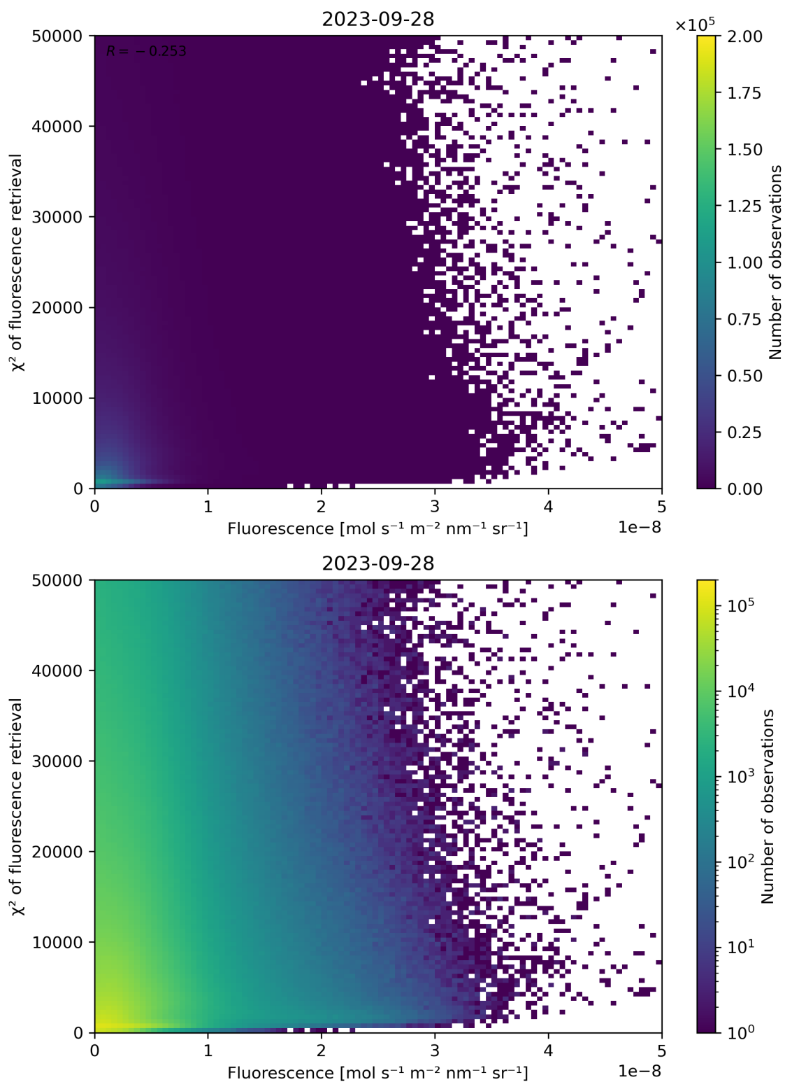
Figure 93: Scatter density plot of “Fluorescence” against “ \chi^2 of fluorescence retrieval” for 2023-09-27 to 2023-09-29.
