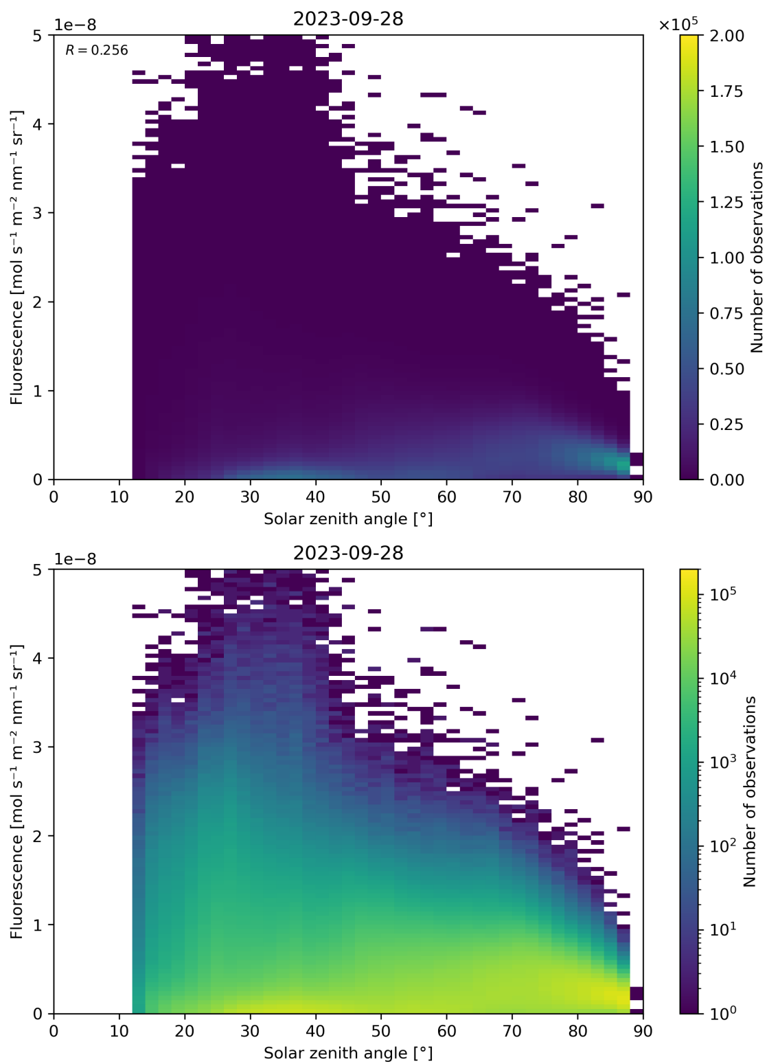
Figure 123: Scatter density plot of “Solar zenith angle” against “Fluorescence” for 2023-09-27 to 2023-09-29.
