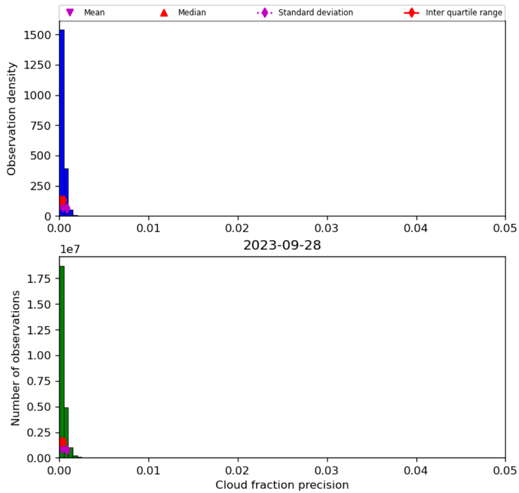
Figure 33: Histogram of “Cloud fraction precision” for 2023-09-27 to 2023-09-29
