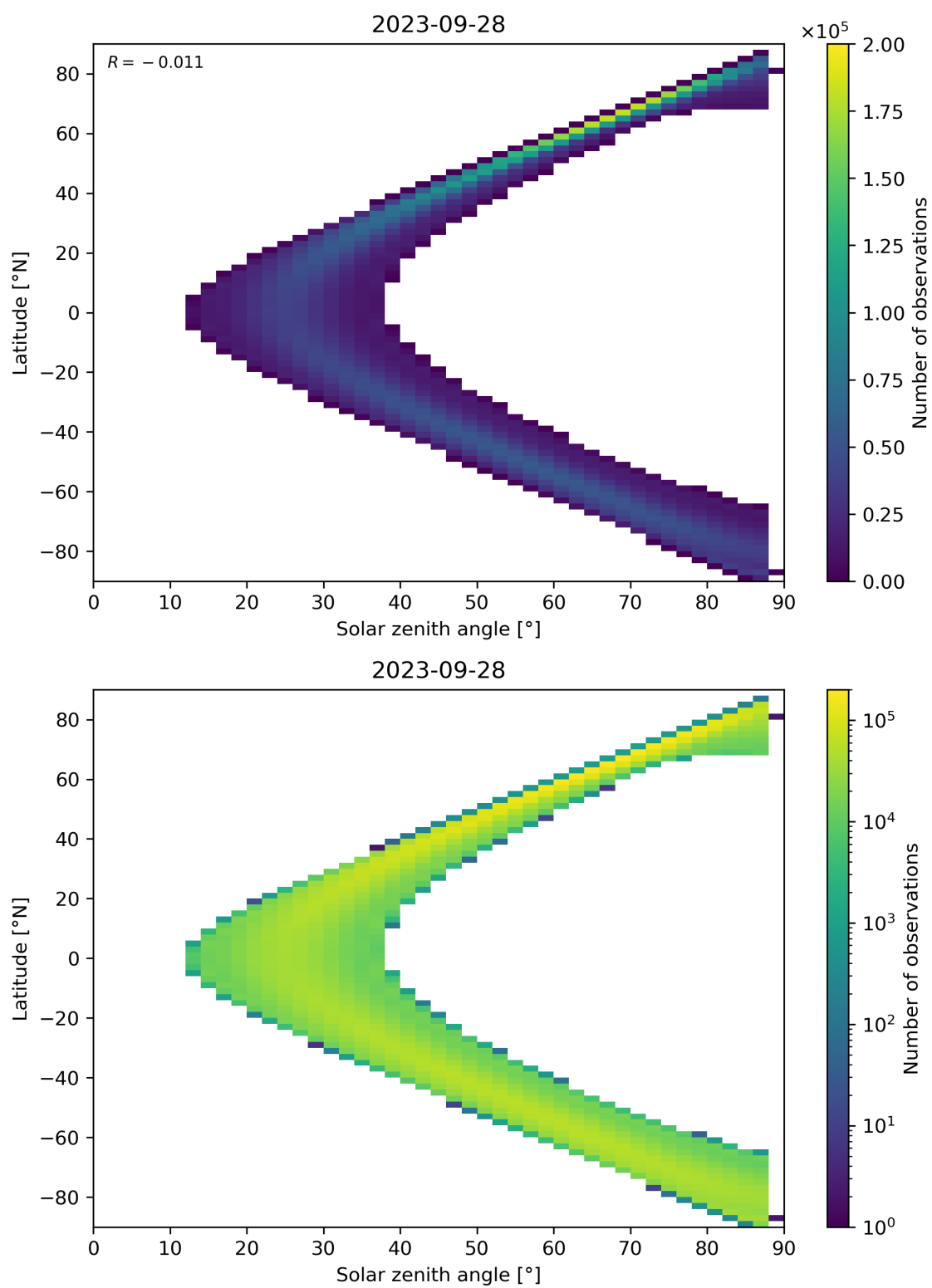
Figure 124: Scatter density plot of “Solar zenith angle” against “Latitude” for 2023-09-27 to 2023-09-29.
