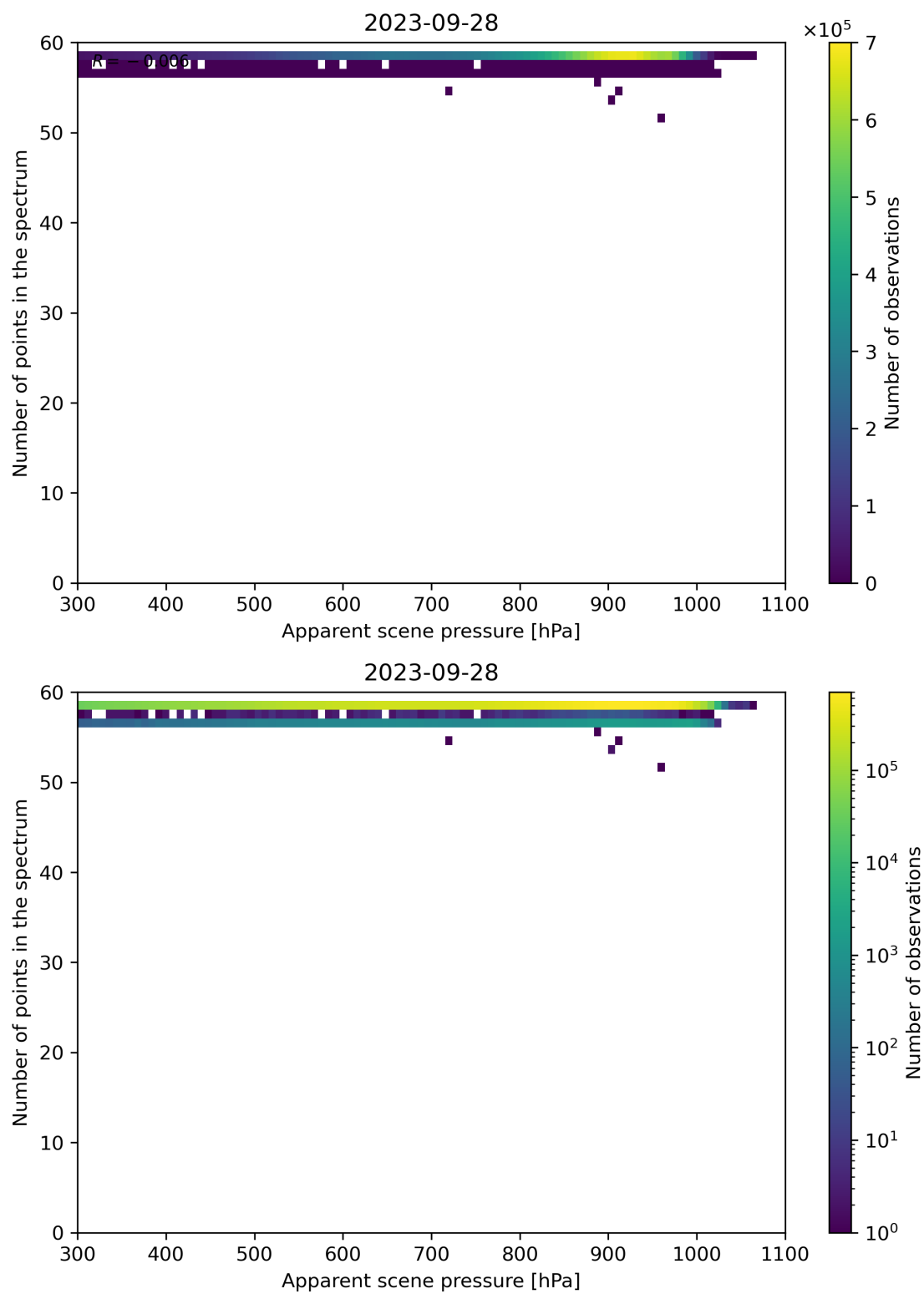
Figure 67: Scatter density plot of “Apparent scene pressure” against “Number of points in the spectrum” for 2023-09-27 to 2023-09-29.
