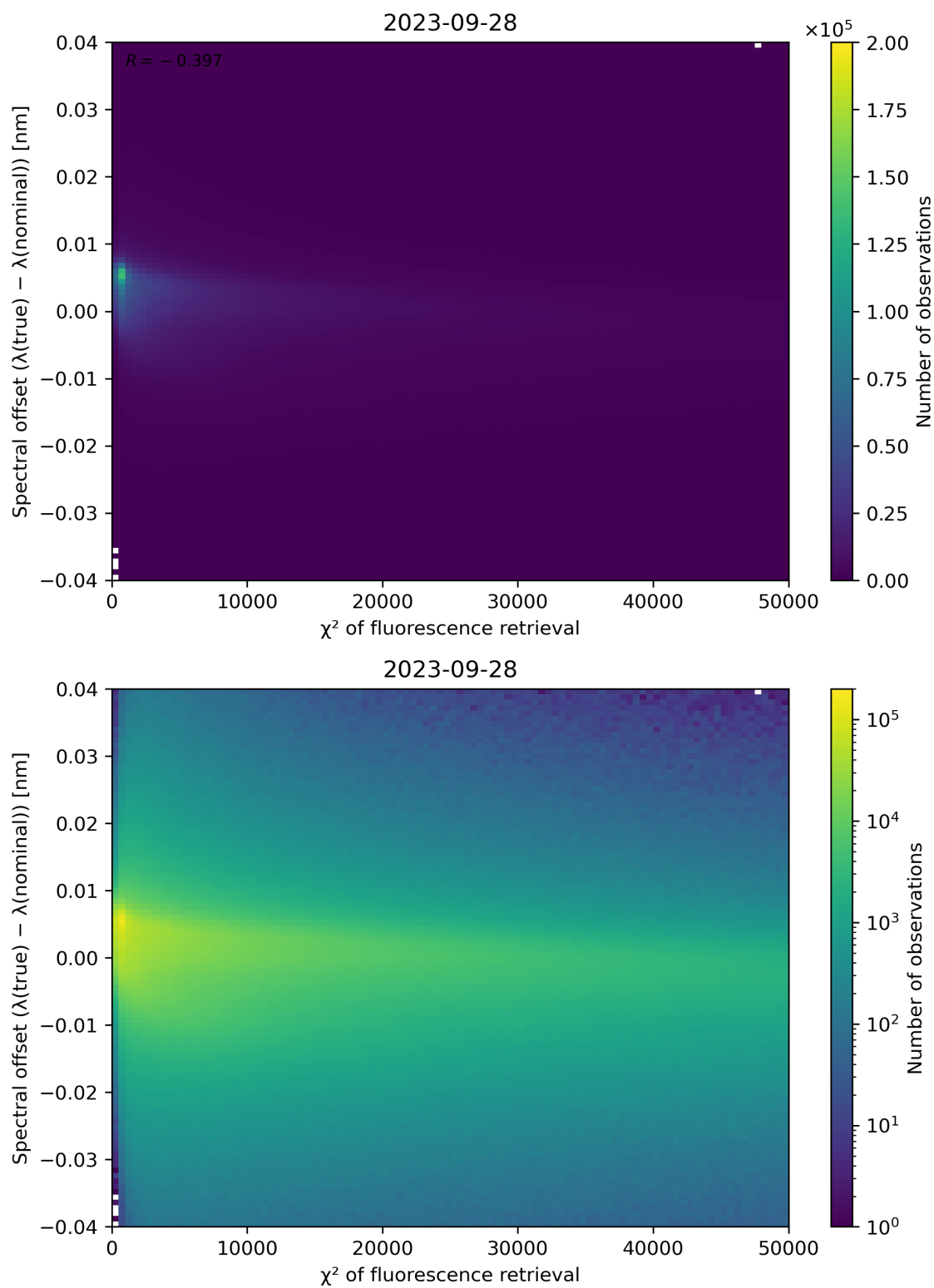
Figure 72: Scatter density plot of " \chi^2 of fluorescence retrieval" against "Spectral offset ( \lambda(\text{true}) - \lambda(\text{nominal}) )" for 2023-09-27 to 2023-09-29.
