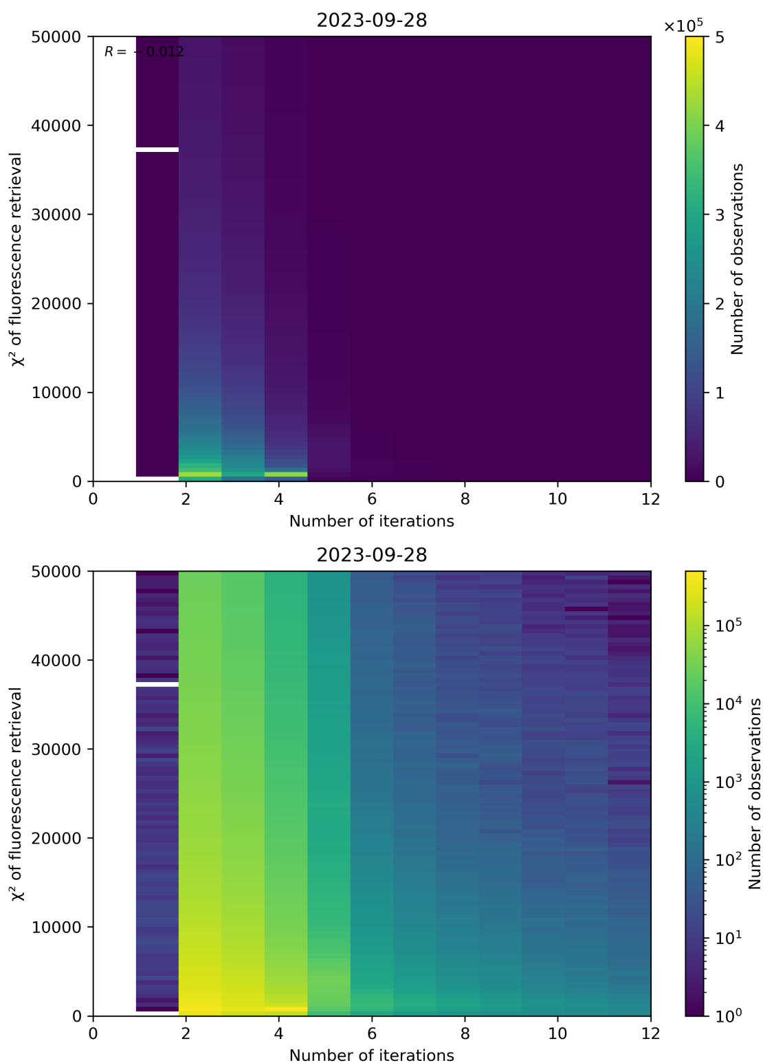
Figure 106: Scatter density plot of “Number of iterations” against “ \chi^2 of fluorescence retrieval” for 2023-09-27 to 2023-09-29.
