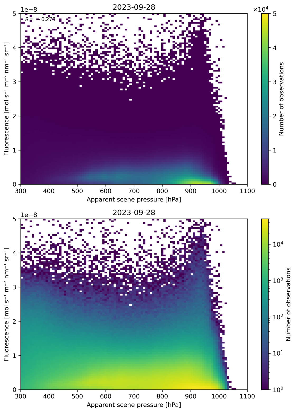
Figure 65: Scatter density plot of “Apparent scene pressure” against “Fluorescence” for 2023-09-27 to 2023-09-29.
