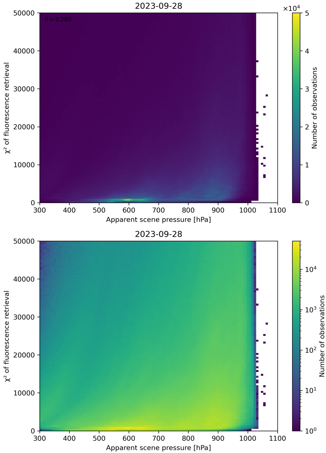
Figure 64: Scatter density plot of “Apparent scene pressure” against “ \chi^2 of fluorescence retrieval” for 2023-09-27 to 2023-09-29.
