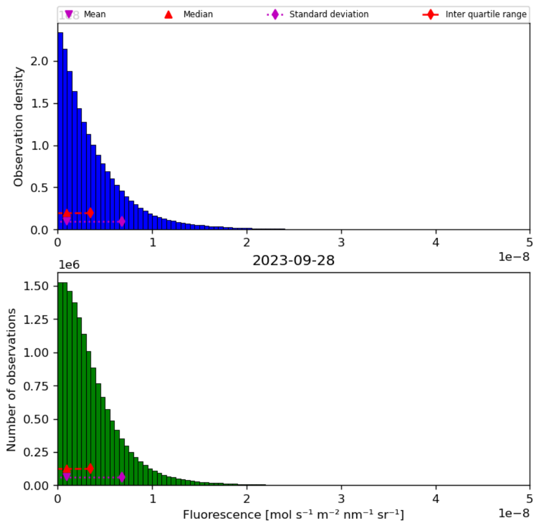
Figure 40: Histogram of “Fluorescence” for 2023-09-27 to 2023-09-29
