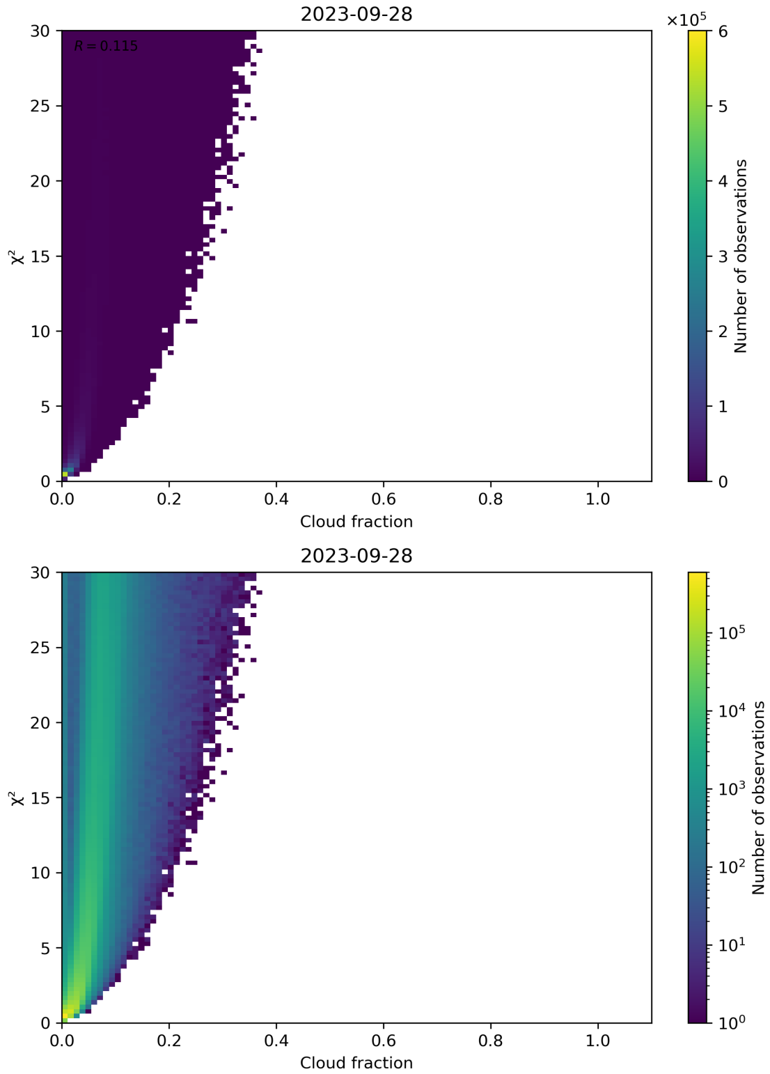
Figure 77: Scatter density plot of “Cloud fraction” against “ \chi^2 ” for 2023-09-27 to 2023-09-29.
