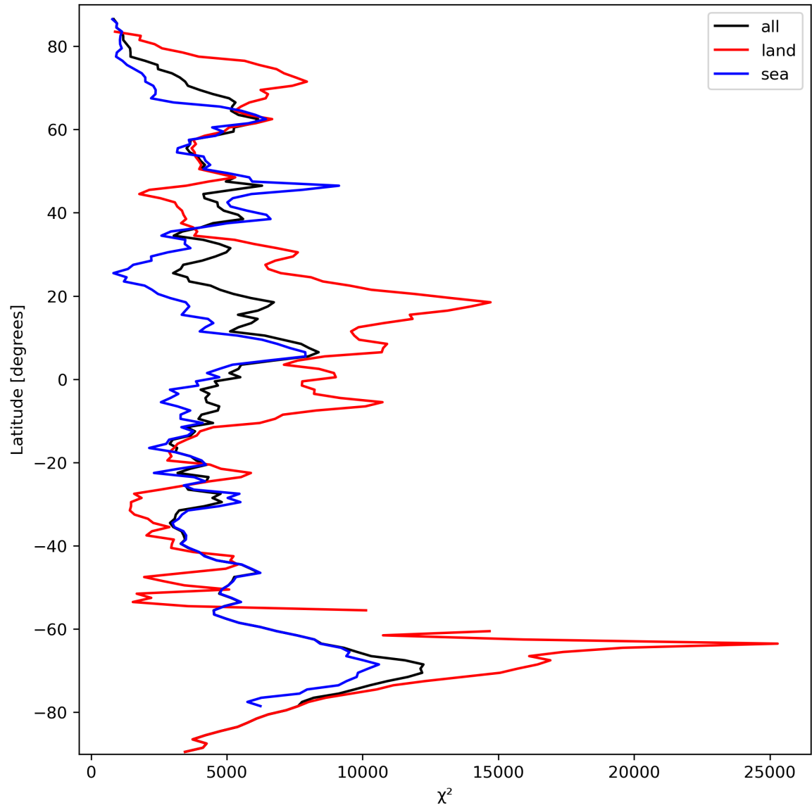
Figure 21: Zonal average of “ \chi^2 ” for 2023-09-27 to 2023-09-29.
