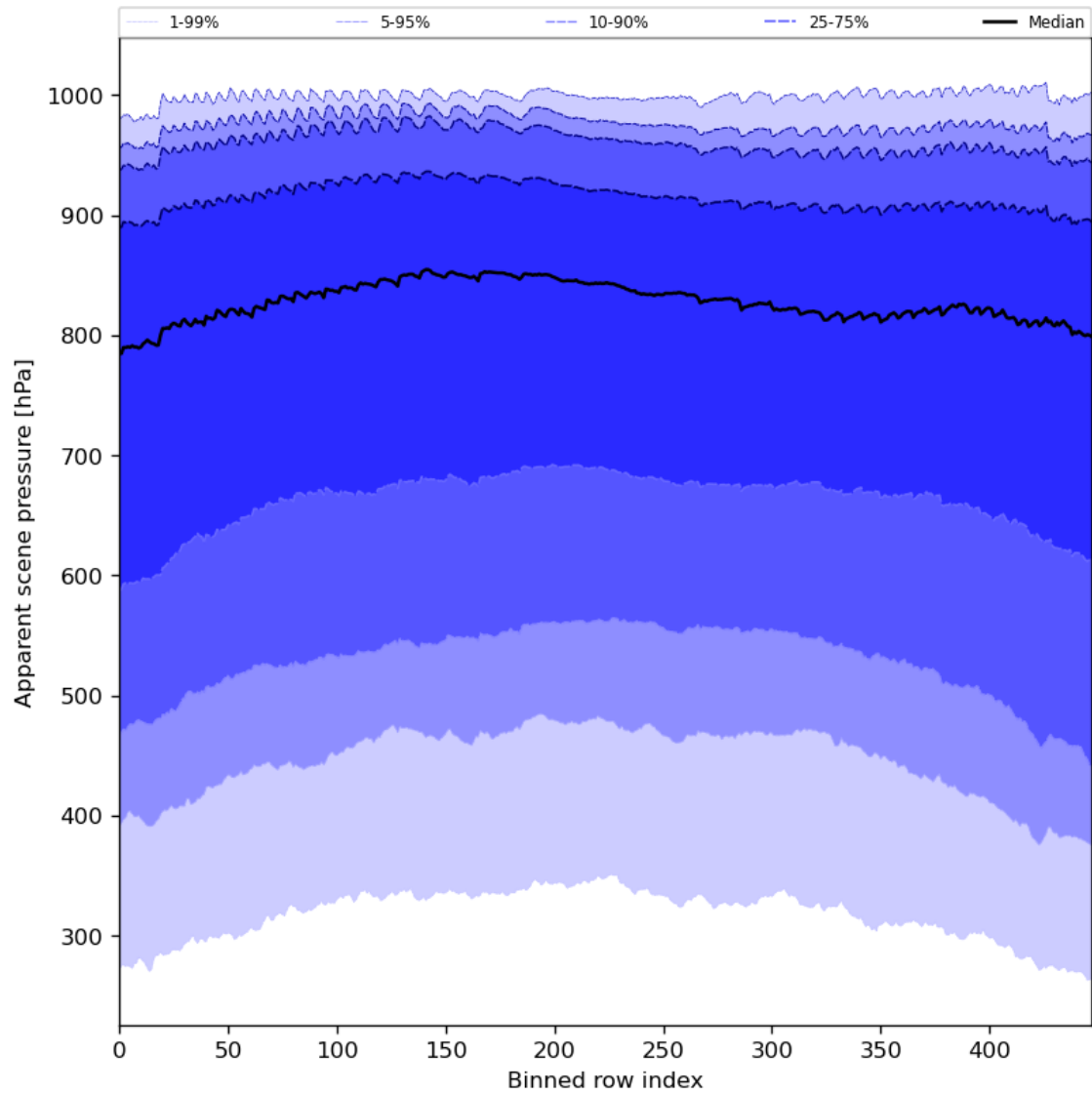
Figure 53: Along track statistics of “Apparent scene pressure” for 2023-09-27 to 2023-09-29
