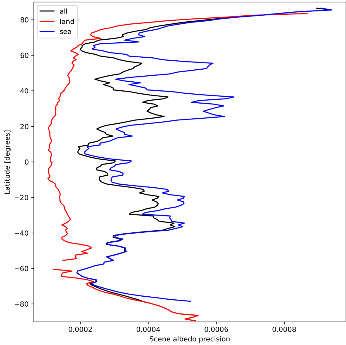
Figure 18: Zonal average of “Scene albedo precision” for 2023-09-27 to 2023-09-29.
