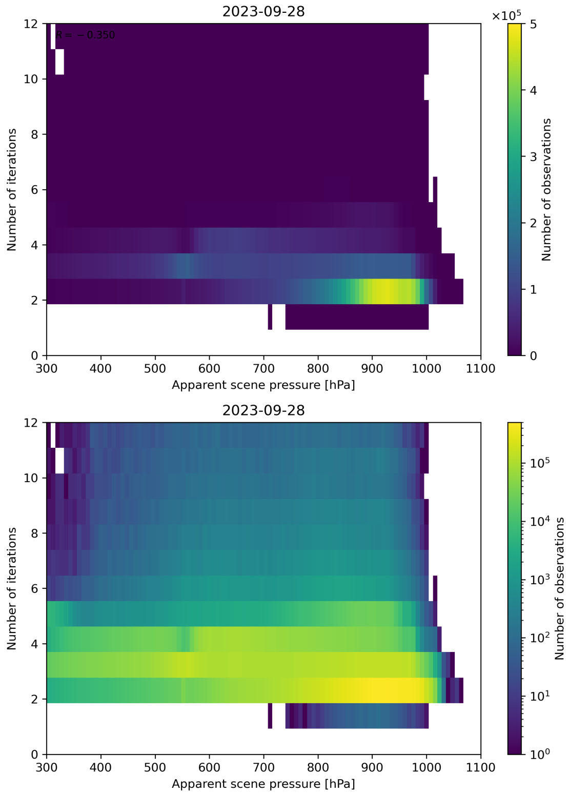
Figure 66: Scatter density plot of “Apparent scene pressure” against “Number of iterations” for 2023-09-27 to 2023-09-29.
