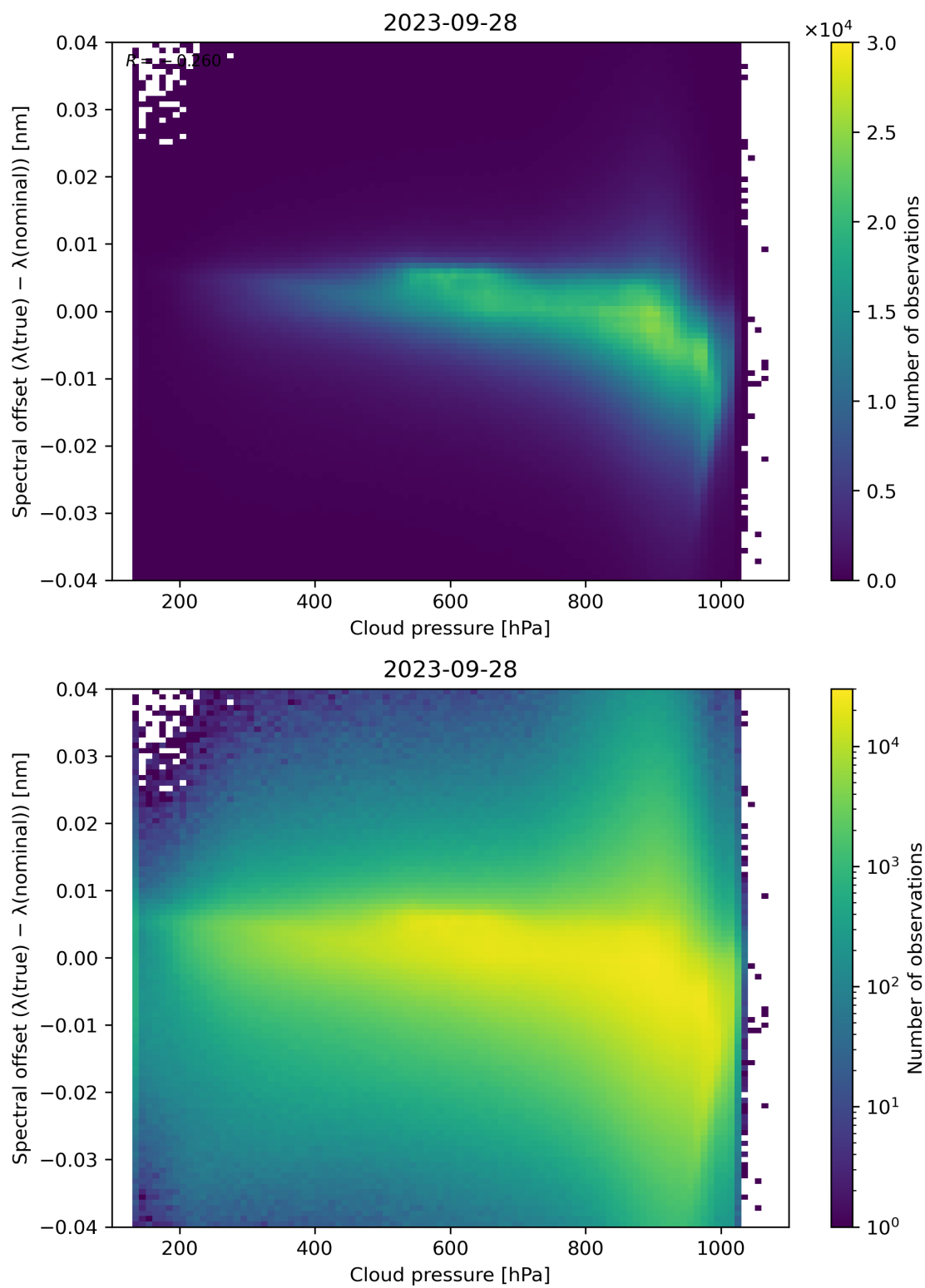
Figure 92: Scatter density plot of “Cloud pressure” against “Spectral offset ( \lambda(\text{true}) - \lambda(\text{nominal}) )” for 2023-09-27 to 2023-09-29.
