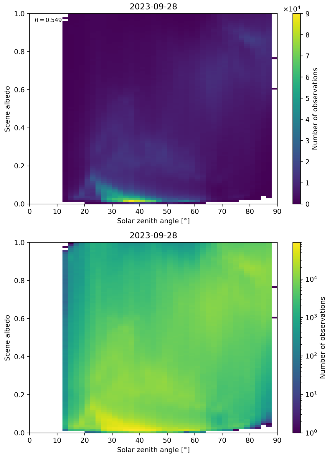
Figure 127: Scatter density plot of “Solar zenith angle” against “Scene albedo” for 2023-09-27 to 2023-09-29.
