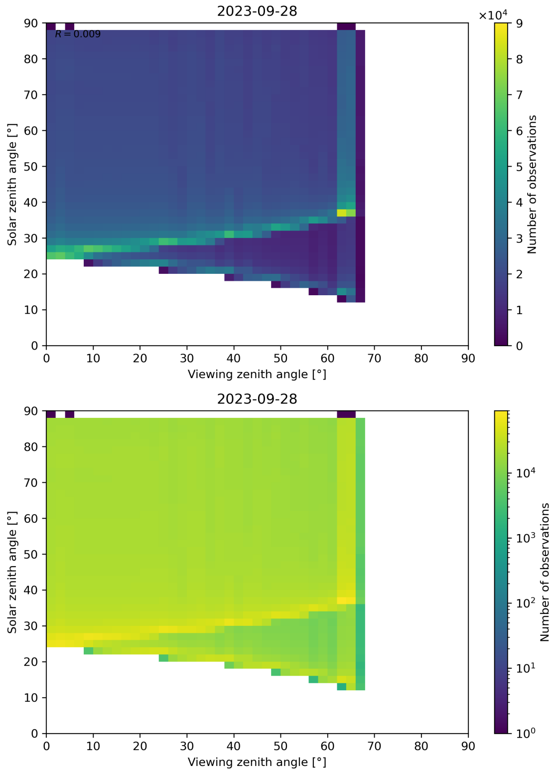
Figure 139: Scatter density plot of “Viewing zenith angle” against “Solar zenith angle” for 2023-09-27 to 2023-09-29.
