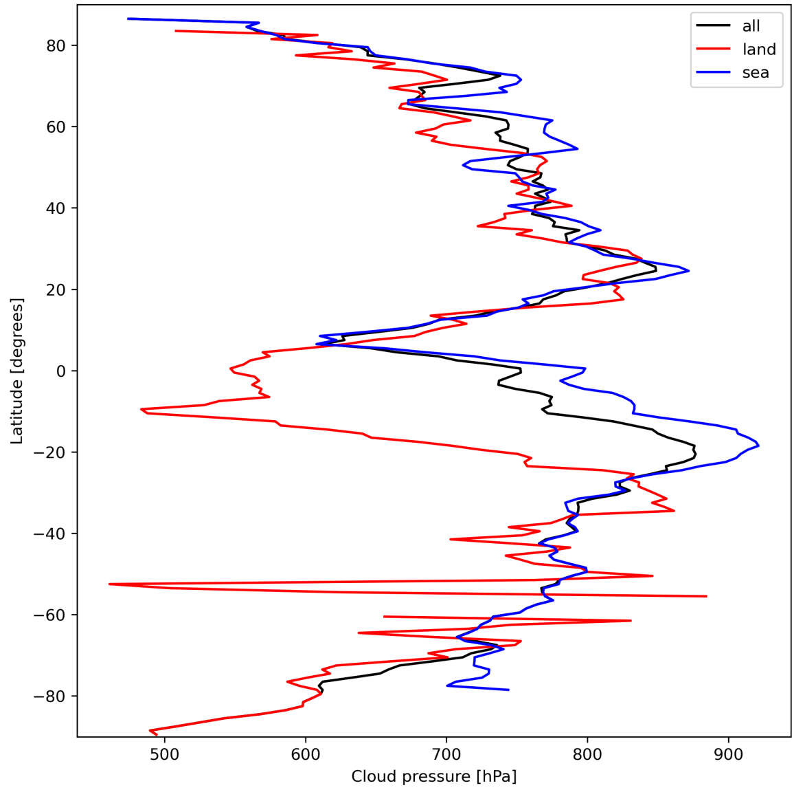
Figure 13: Zonal average of “Cloud pressure” for 2023-09-27 to 2023-09-29.
