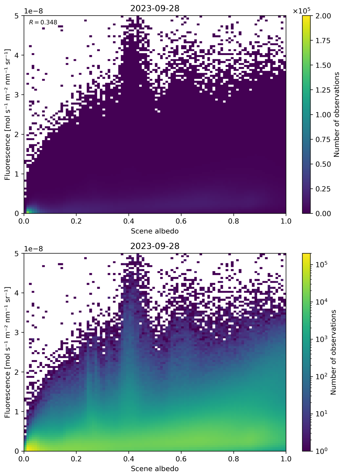
Figure 114: Scatter density plot of “Scene albedo” against “Fluorescence” for 2023-09-27 to 2023-09-29.
