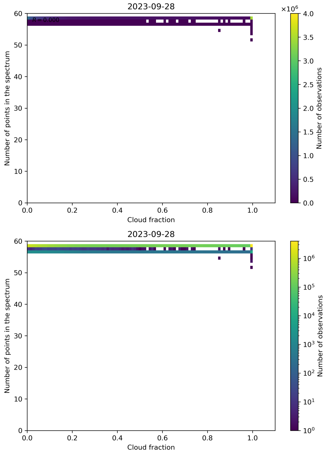
Figure 81: Scatter density plot of “Cloud fraction” against “Number of points in the spectrum” for 2023-09-27 to 2023-09-29.
