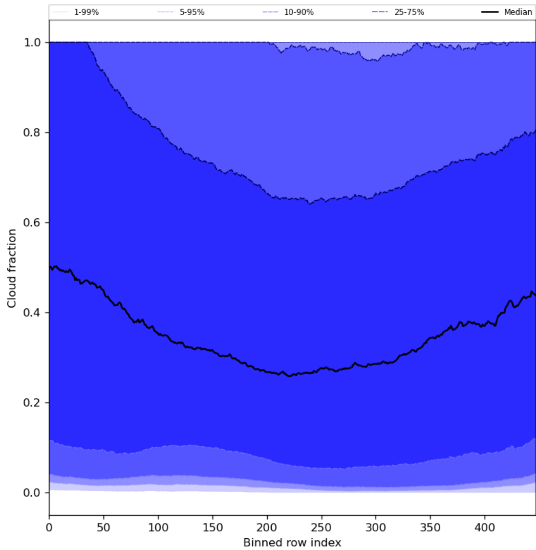
Figure 49: Along track statistics of “Cloud fraction” for 2023-09-27 to 2023-09-29
