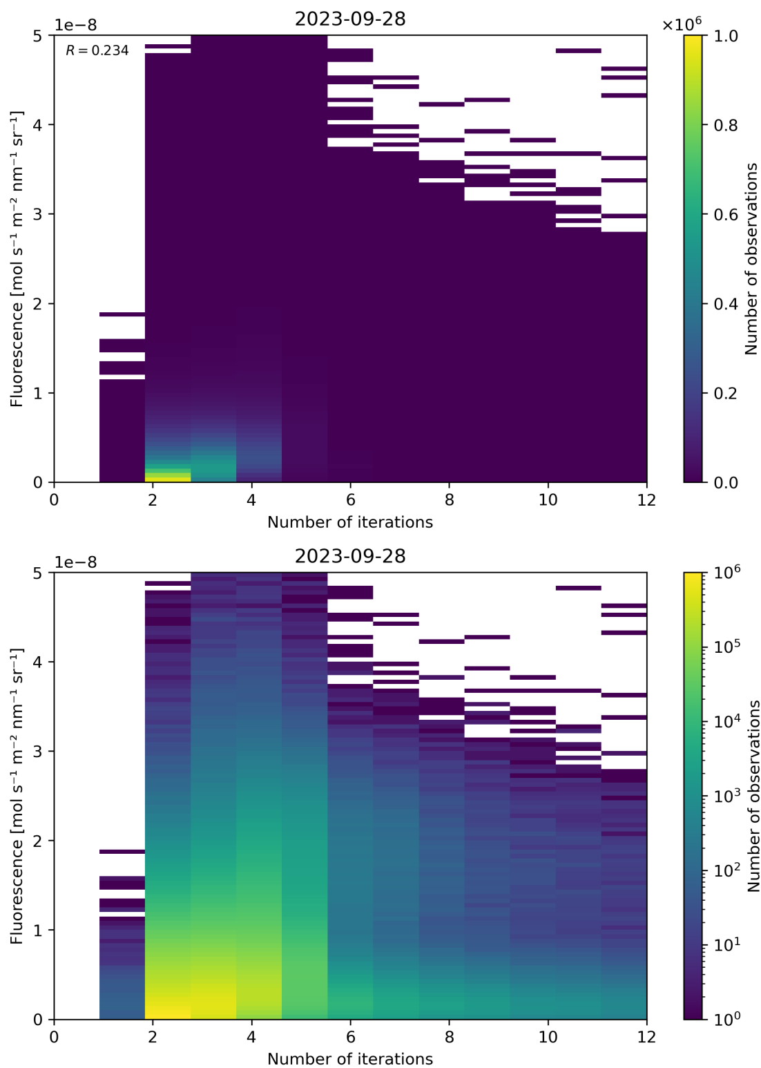
Figure 107: Scatter density plot of “Number of iterations” against “Fluorescence” for 2023-09-27 to 2023-09-29.
