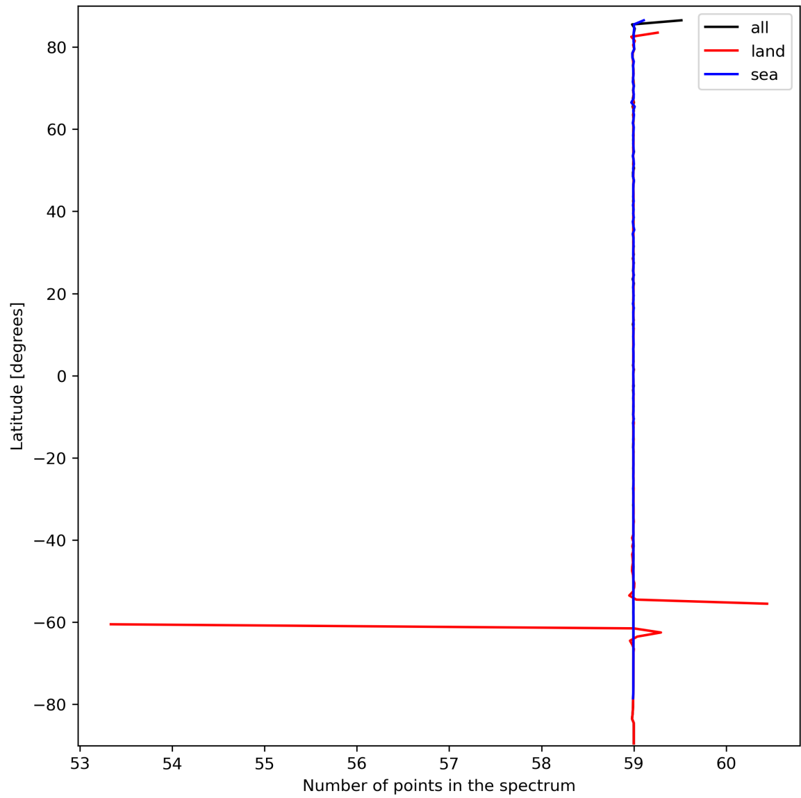
Figure 27: Zonal average of “Number of points in the spectrum” for 2023-09-27 to 2023-09-29.
