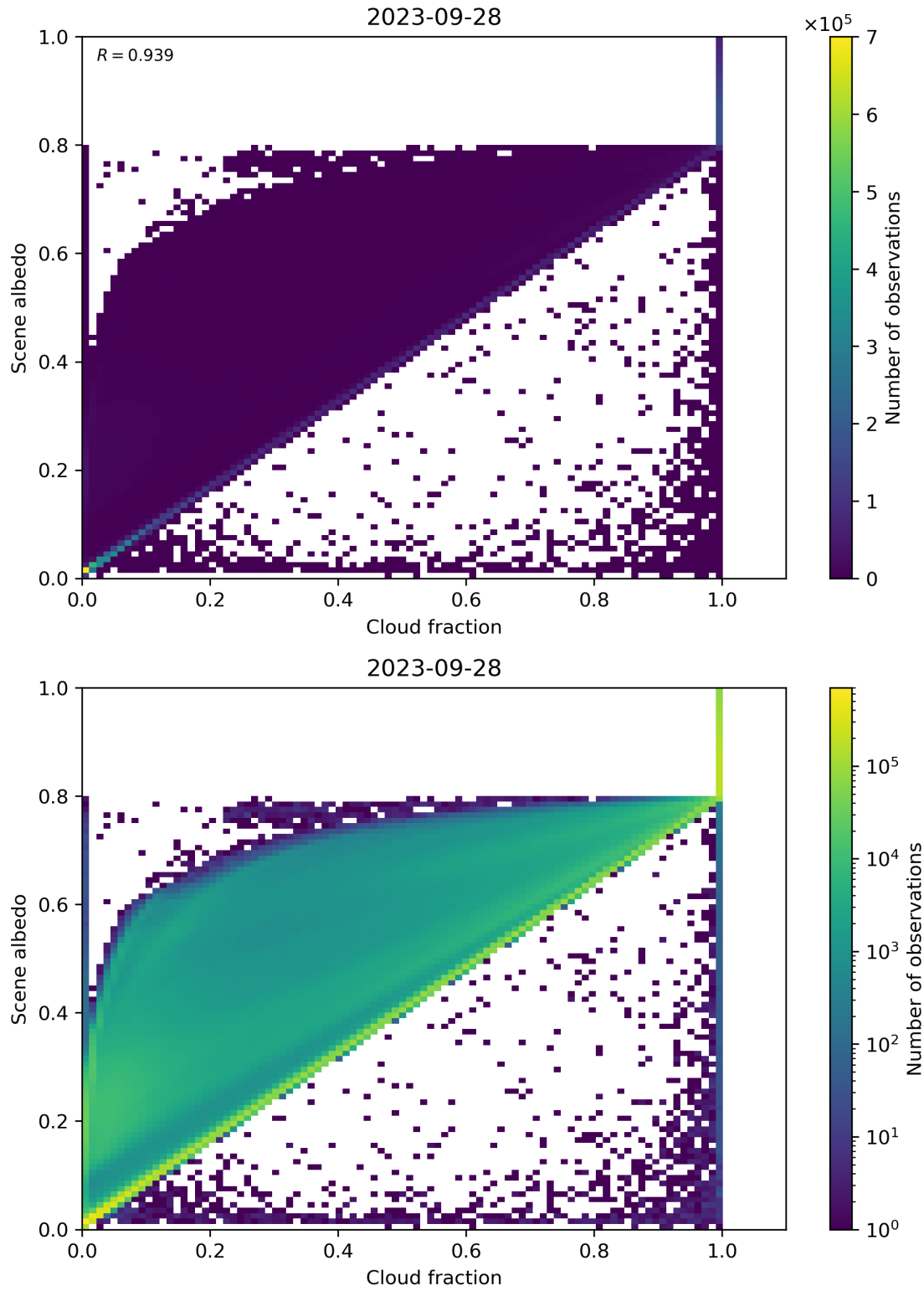
Figure 82: Scatter density plot of “Cloud fraction” against “Scene albedo” for 2023-09-27 to 2023-09-29.
