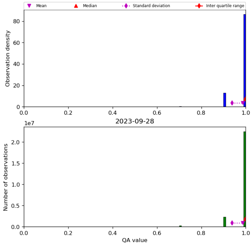
Figure 29: Histogram of “QA value” for 2023-09-27 to 2023-09-29
