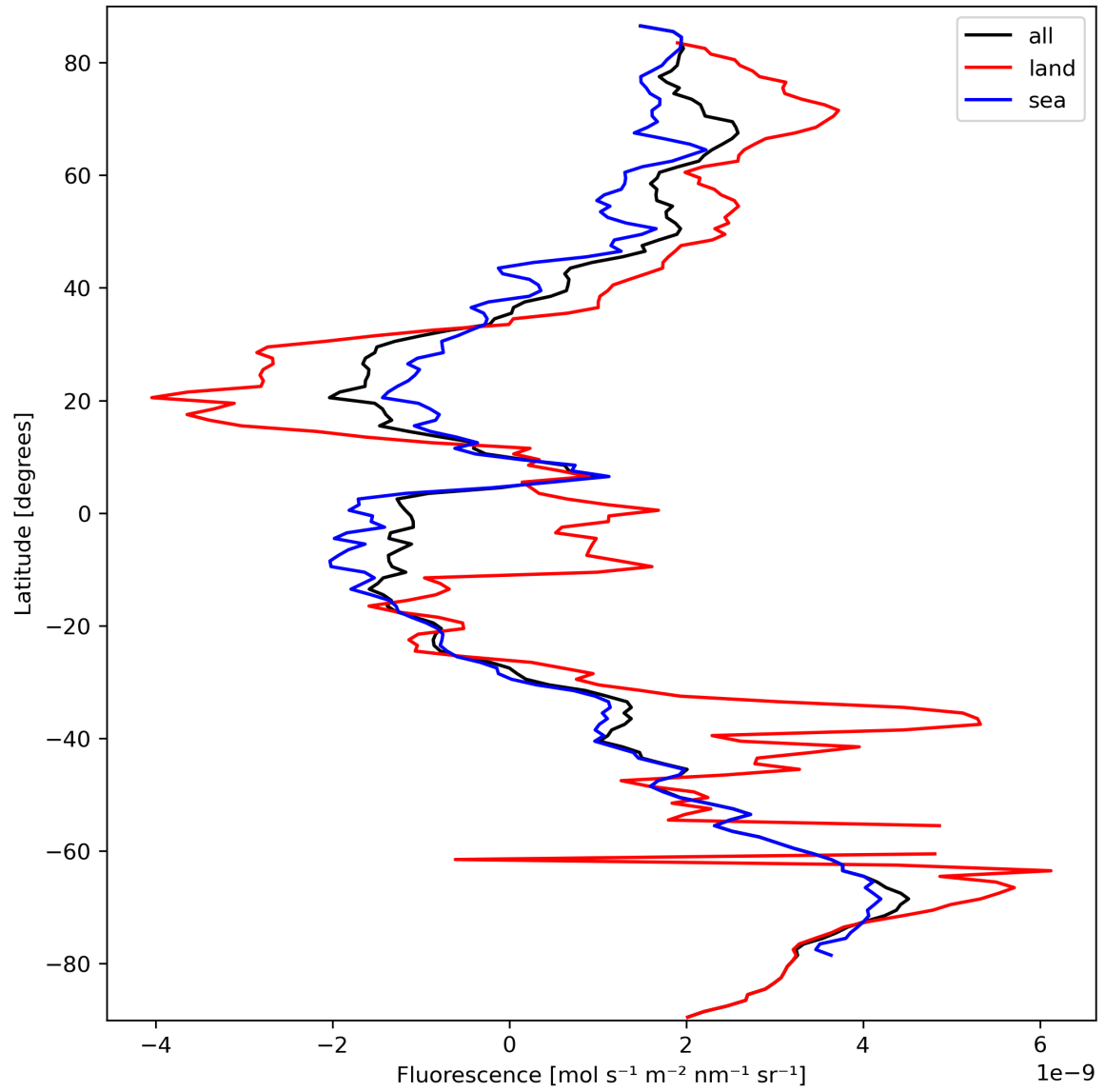
Figure 23: Zonal average of “Fluorescence” for 2023-09-27 to 2023-09-29.
