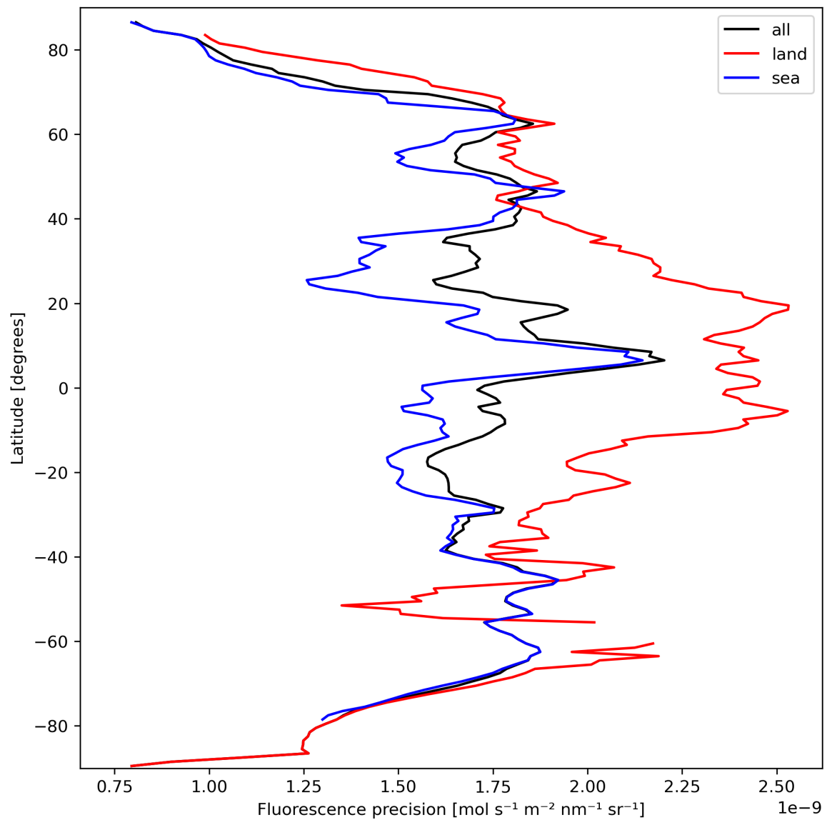
Figure 24: Zonal average of “Fluorescence precision” for 2023-09-27 to 2023-09-29.
