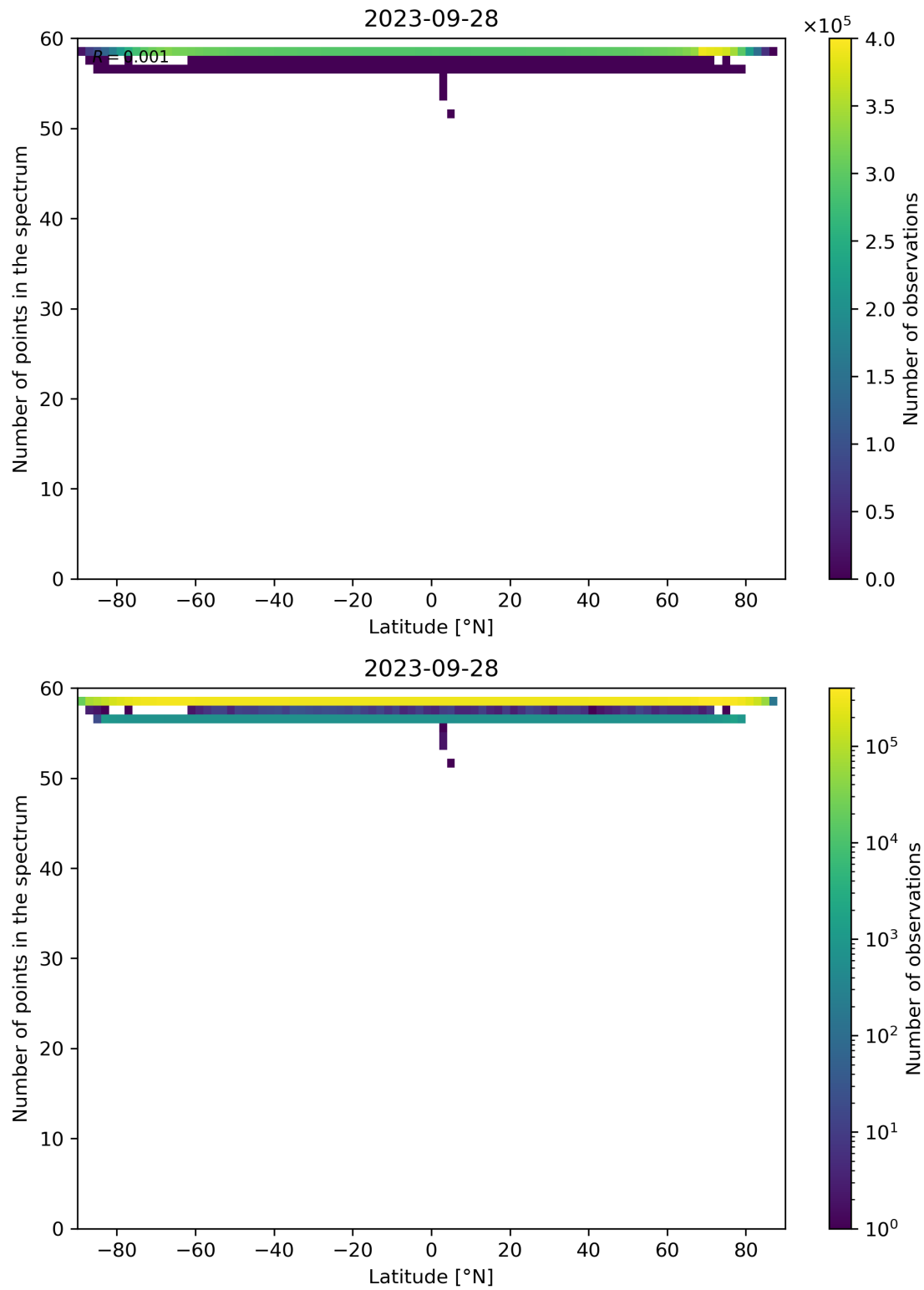
Figure 103: Scatter density plot of “Latitude” against “Number of points in the spectrum” for 2023-09-27 to 2023-09-29.
