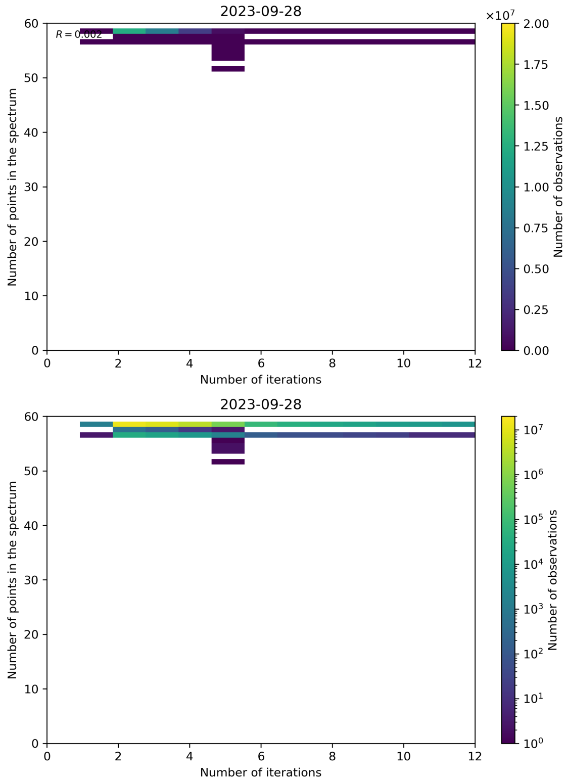
Figure 108: Scatter density plot of “Number of iterations” against “Number of points in the spectrum” for 2023-09-27 to 2023-09-29.
