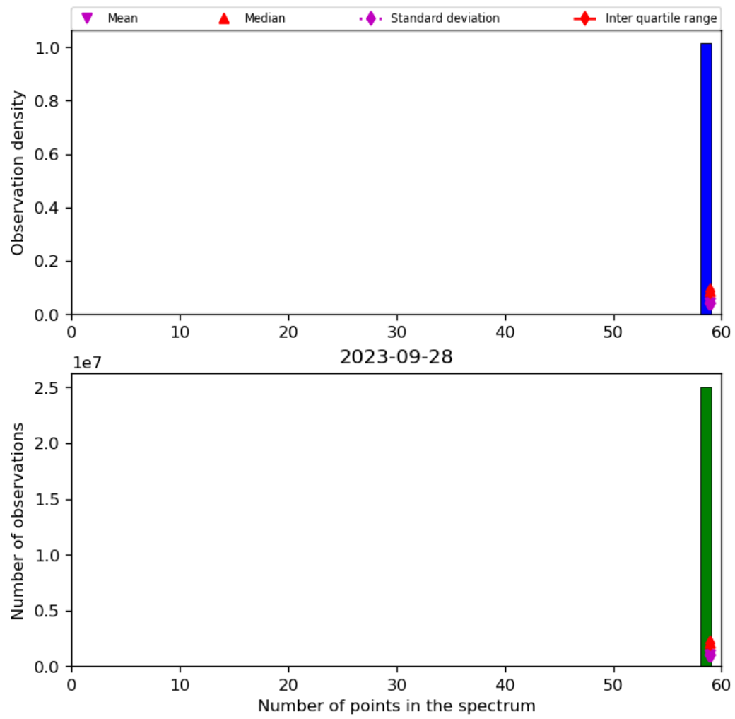
Figure 44: Histogram of “Number of points in the spectrum” for 2023-09-27 to 2023-09-29
