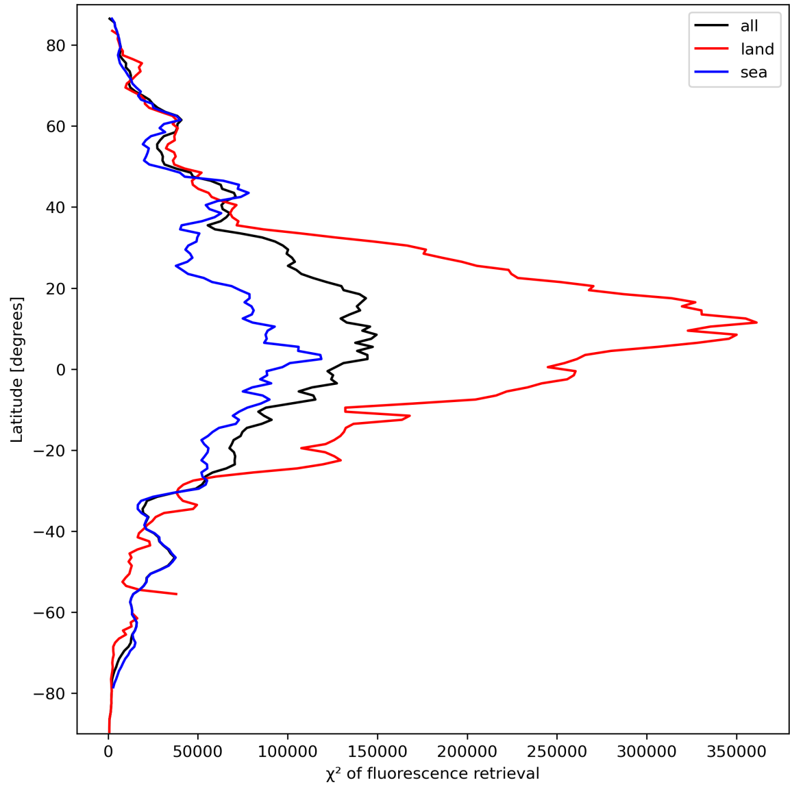
Figure 25: Zonal average of “ \chi^2 of fluorescence retrieval” for 2023-09-27 to 2023-09-29.
