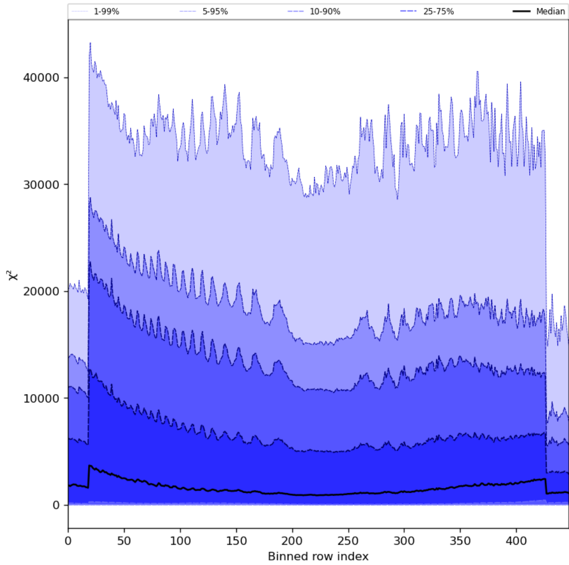
Figure 55: Along track statistics of “ \chi^2 ” for 2023-09-27 to 2023-09-29
