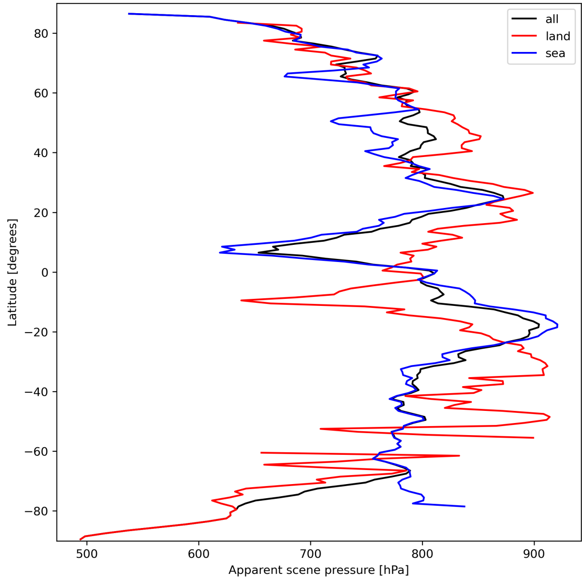
Figure 19: Zonal average of “Apparent scene pressure” for 2023-09-27 to 2023-09-29.
