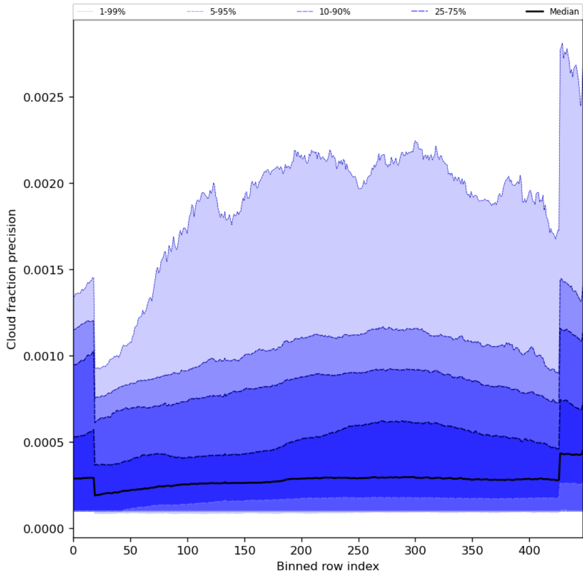
Figure 50: Along track statistics of “Cloud fraction precision” for 2023-09-27 to 2023-09-29
