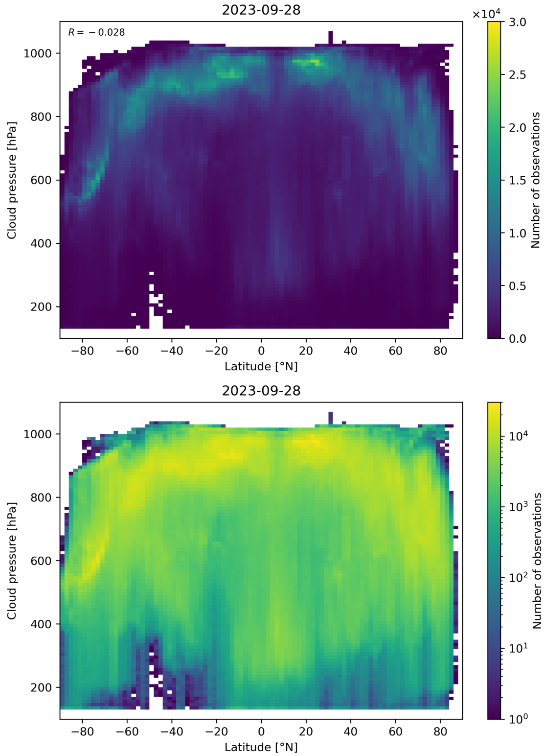
Figure 100: Scatter density plot of “Latitude” against “Cloud pressure” for 2023-09-27 to 2023-09-29.
