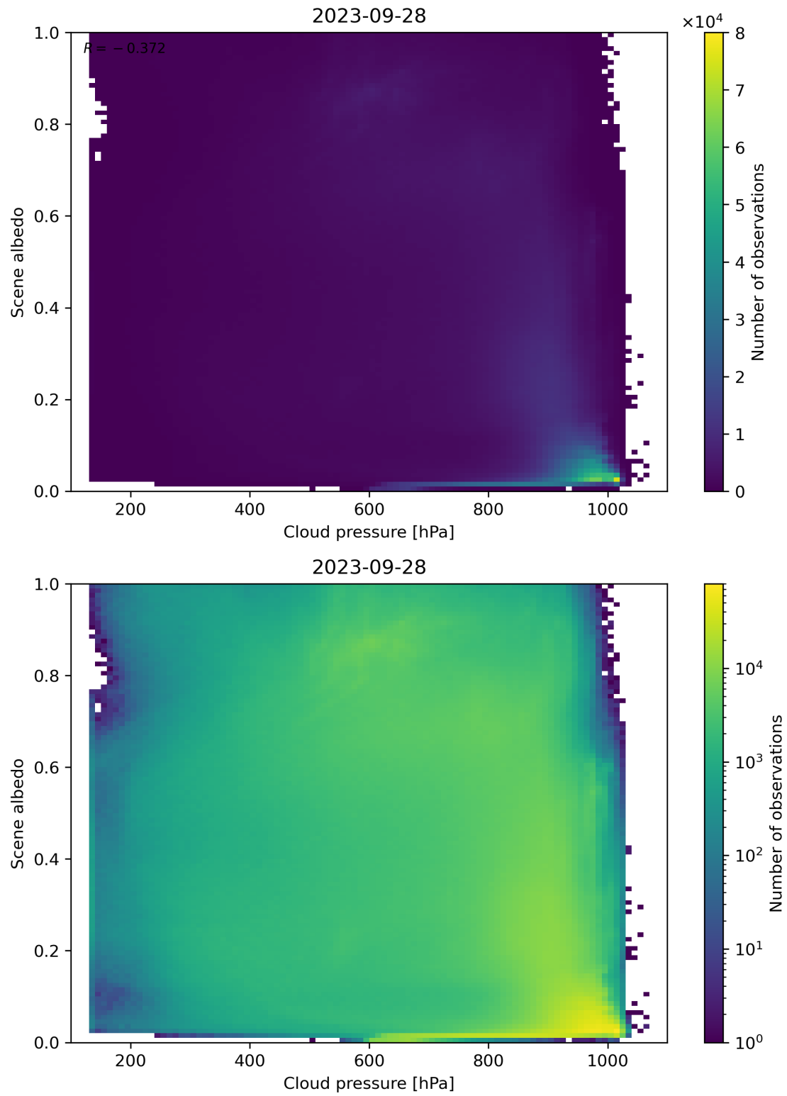
Figure 91: Scatter density plot of “Cloud pressure” against “Scene albedo” for 2023-09-27 to 2023-09-29.
