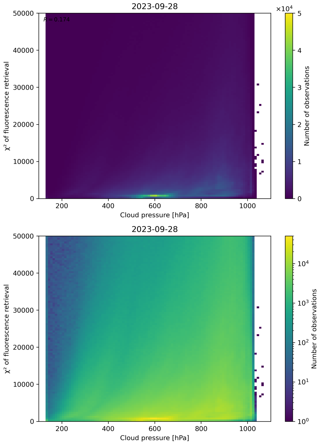
Figure 86: Scatter density plot of “Cloud pressure” against “ \chi^2 of fluorescence retrieval” for 2023-09-27 to 2023-09-29.
