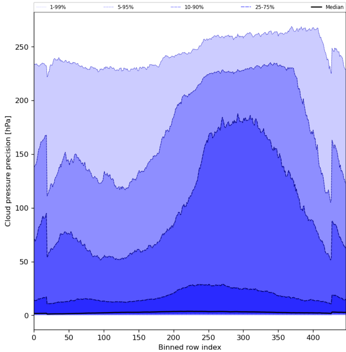
Figure 48: Along track statistics of “Cloud pressure precision” for 2023-09-27 to 2023-09-29
