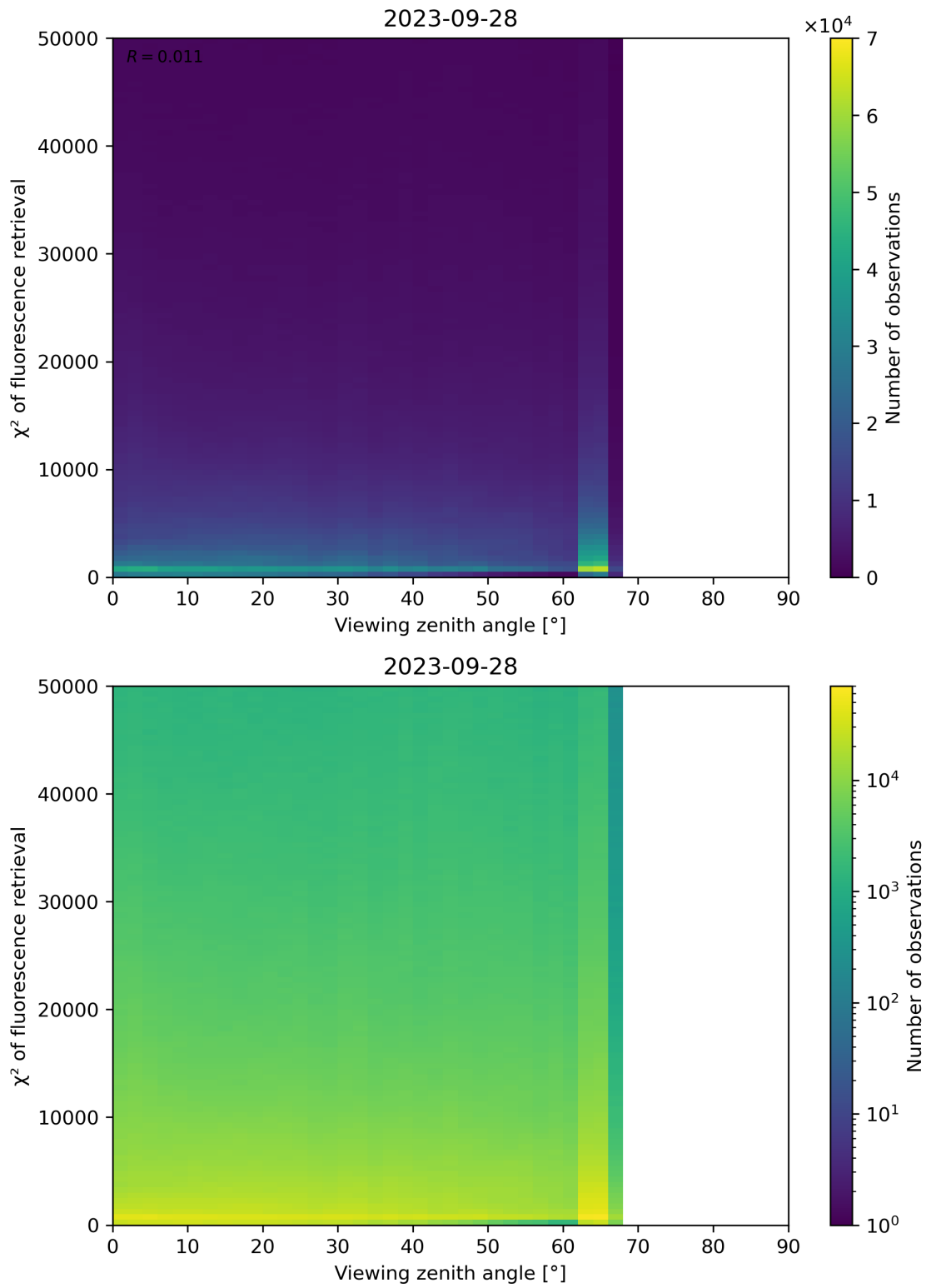
Figure 131: Scatter density plot of “Viewing zenith angle” against “ \chi^2 of fluorescence retrieval” for 2023-09-27 to 2023-09-29.
