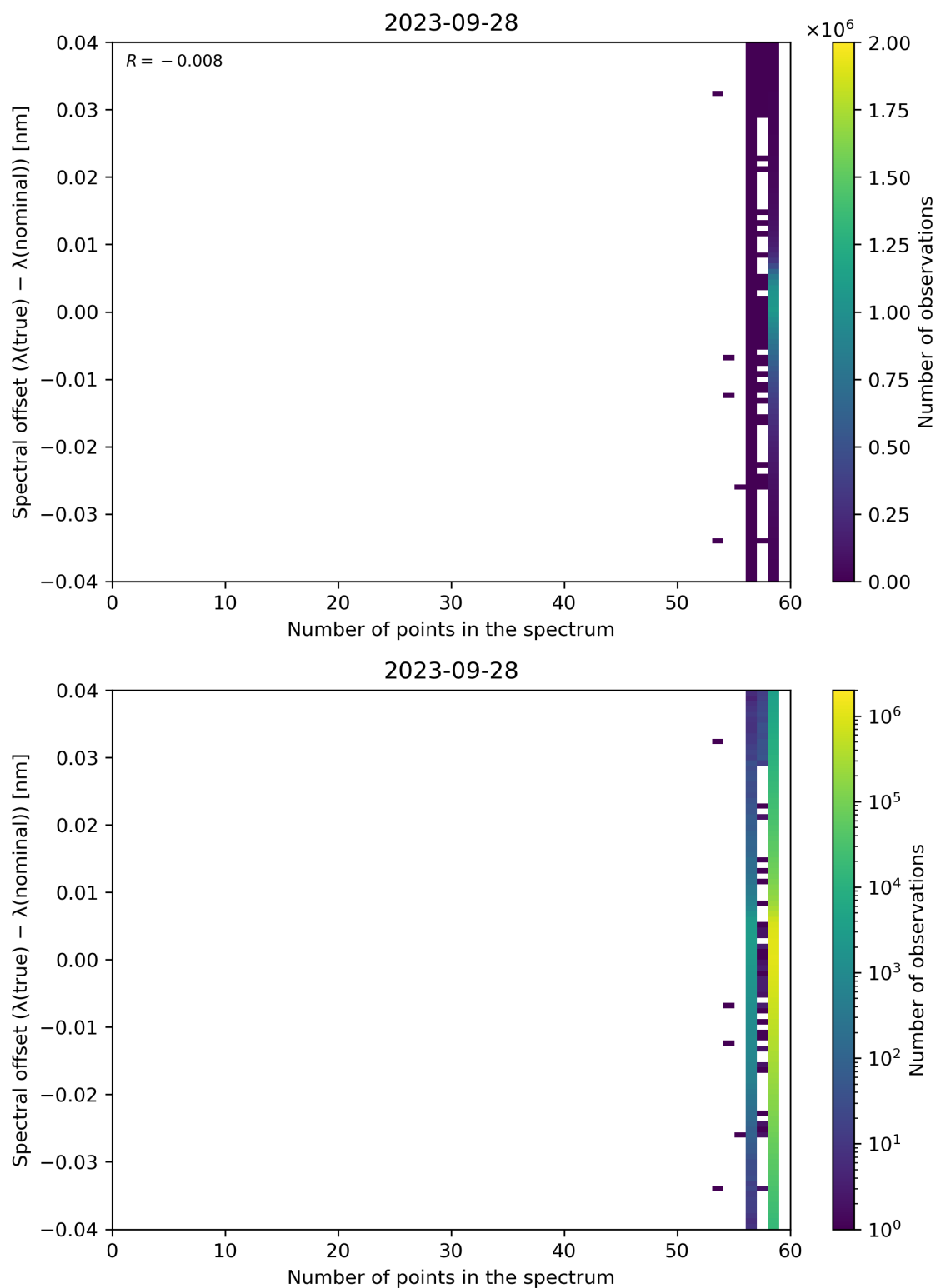
Figure 110: Scatter density plot of “Number of points in the spectrum” against “Spectral offset ( \lambda(\text{true}) - \lambda(\text{nominal}) )” for 2023-09-27 to 2023-09-29.
