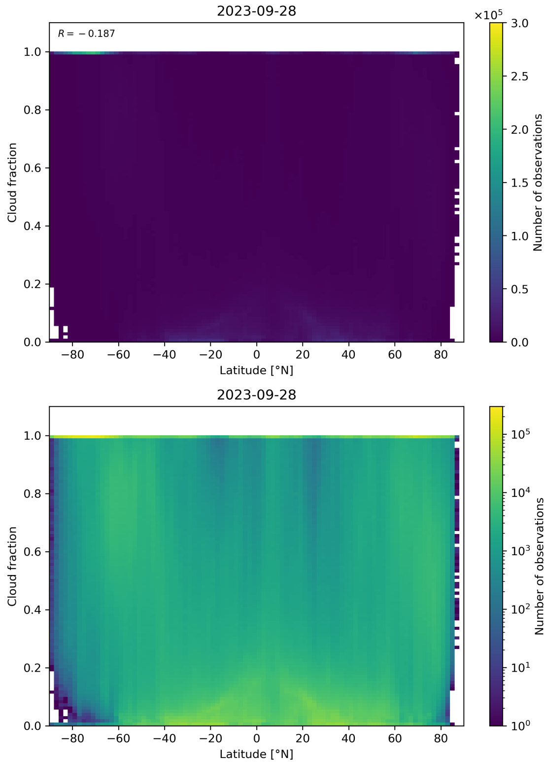
Figure 99: Scatter density plot of “Latitude” against “Cloud fraction” for 2023-09-27 to 2023-09-29.
