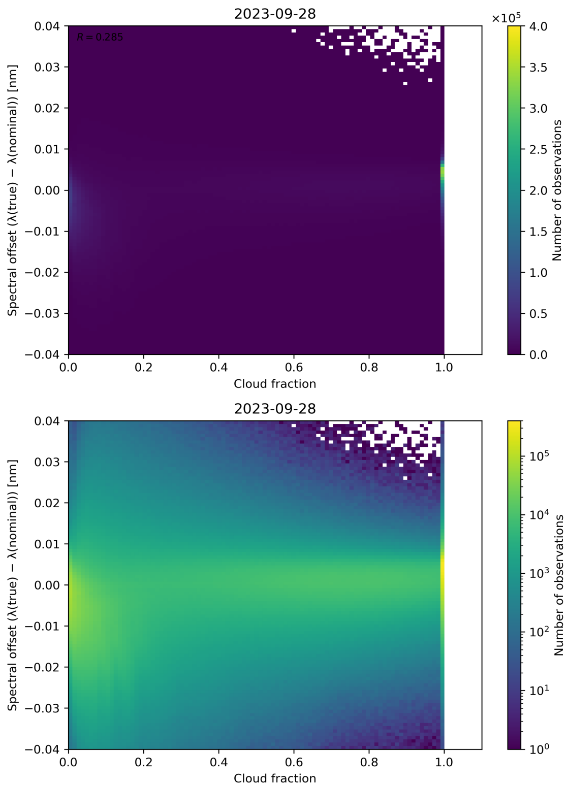
Figure 83: Scatter density plot of “Cloud fraction” against “Spectral offset ( \lambda(\text{true}) - \lambda(\text{nominal}) )” for 2023-09-27 to 2023-09-29.
