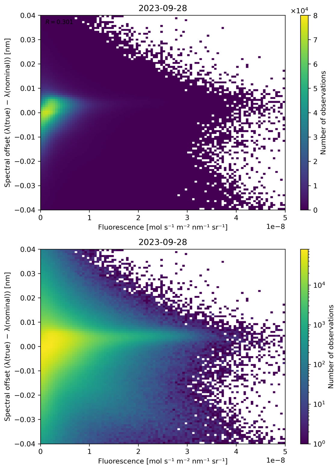
Figure 95: Scatter density plot of “Fluorescence” against “Spectral offset ( \lambda(\text{true}) - \lambda(\text{nominal}) )” for 2023-09-27 to 2023-09-29.
