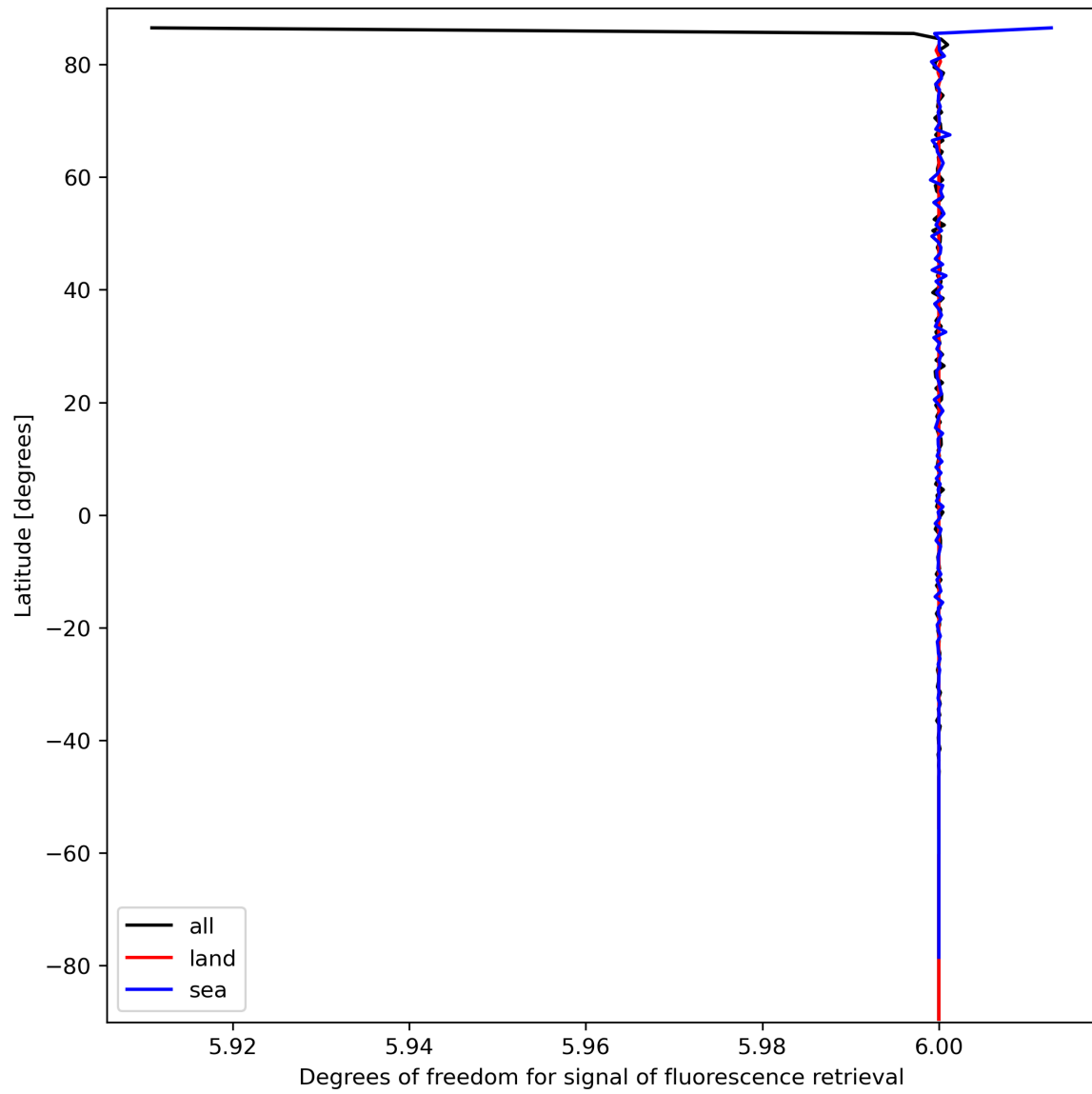
Figure 26: Zonal average of “Degrees of freedom for signal of fluorescence retrieval” for 2023-09-27 to 2023-09-29.
