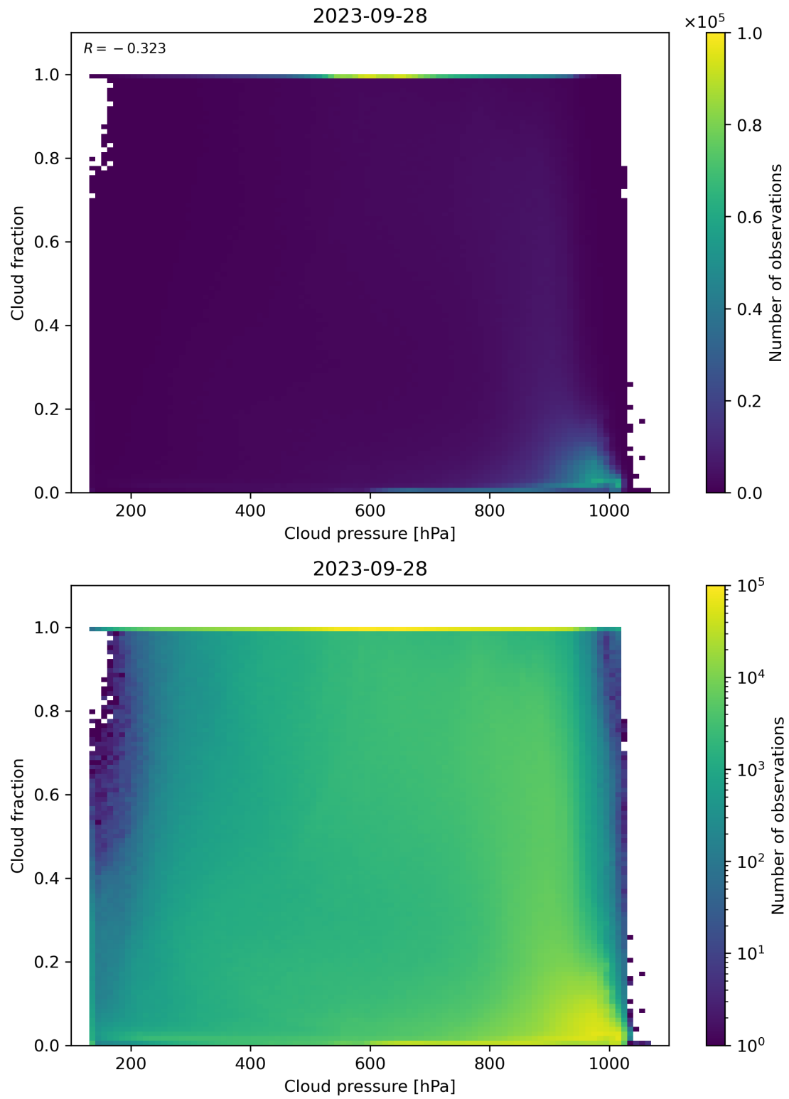
Figure 87: Scatter density plot of “Cloud pressure” against “Cloud fraction” for 2023-09-27 to 2023-09-29.
