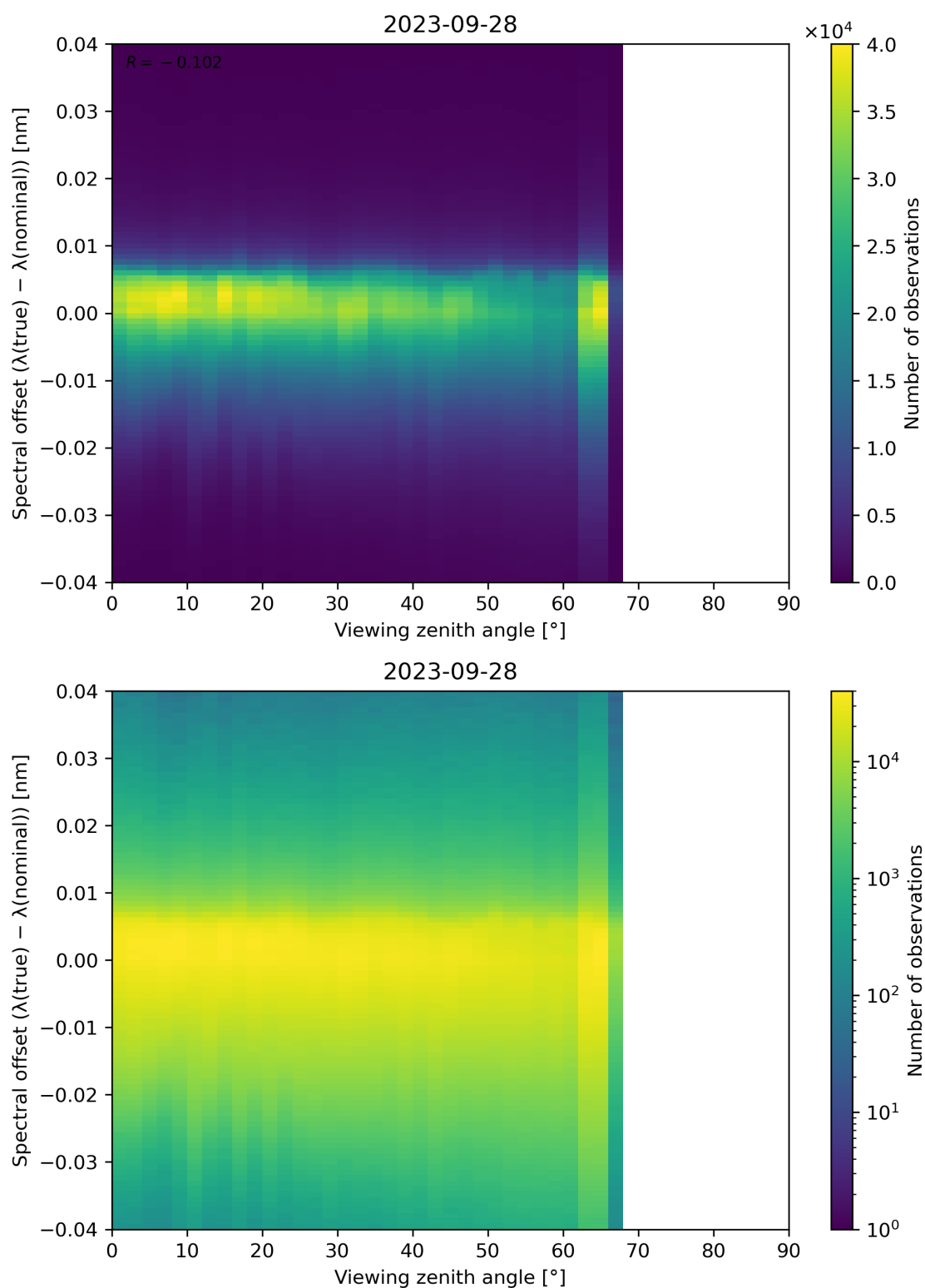
Figure 140: Scatter density plot of “Viewing zenith angle” against “Spectral offset ( \lambda(\text{true}) - \lambda(\text{nominal}) )” for 2023-09-27 to 2023-09-29.
