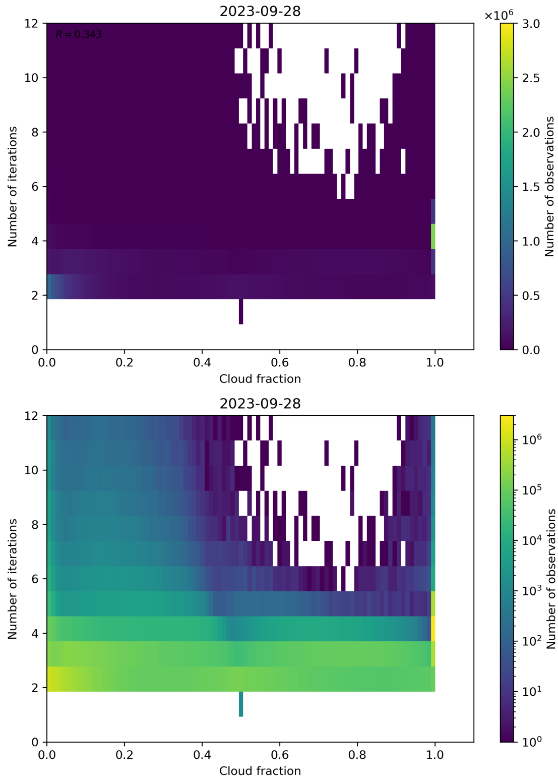
Figure 80: Scatter density plot of “Cloud fraction” against “Number of iterations” for 2023-09-27 to 2023-09-29.
