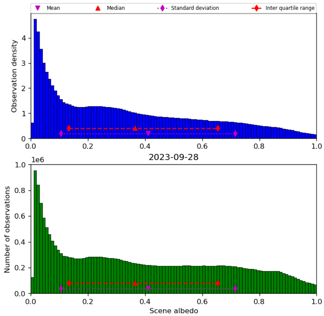
Figure 34: Histogram of “Scene albedo” for 2023-09-27 to 2023-09-29
