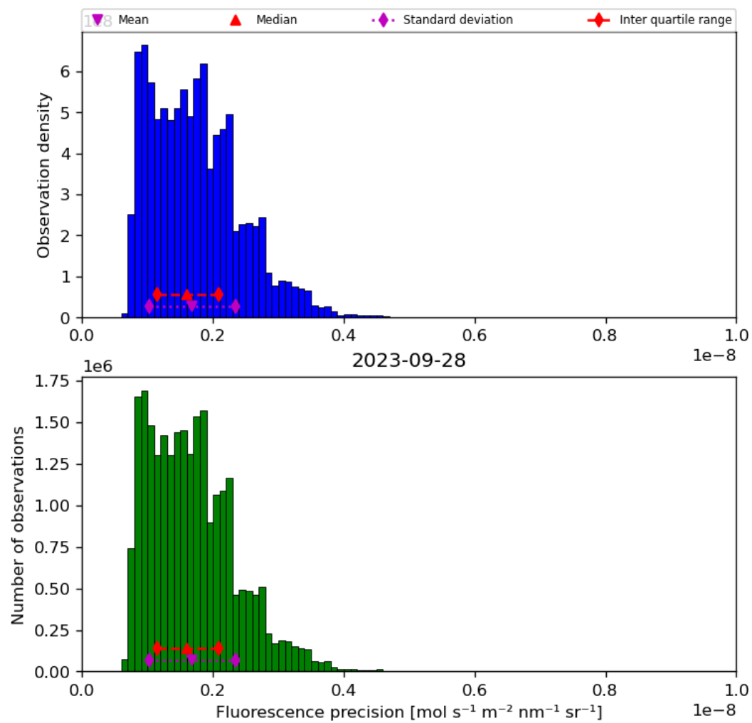
Figure 41: Histogram of “Fluorescence precision” for 2023-09-27 to 2023-09-29
