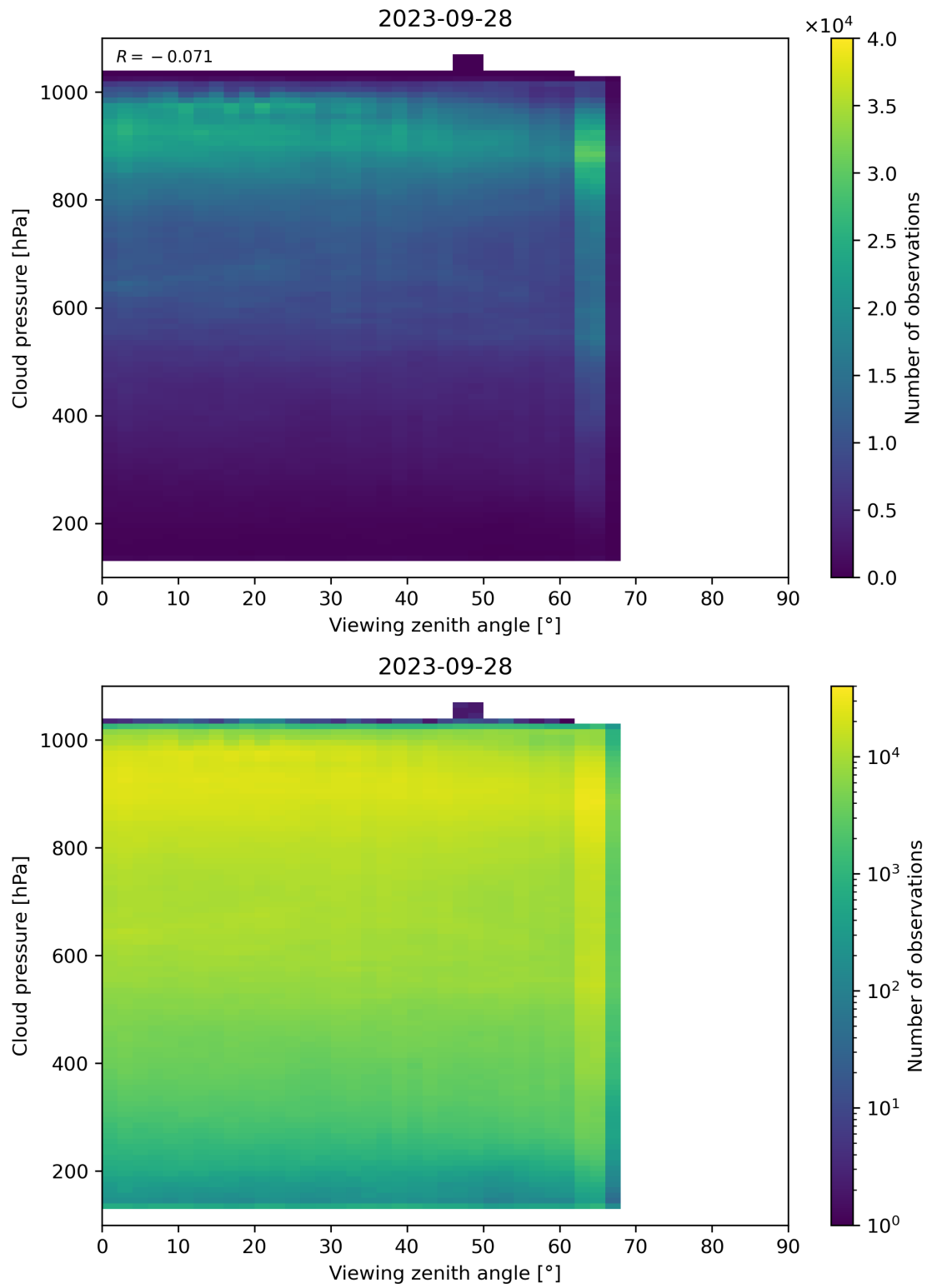
Figure 133: Scatter density plot of “Viewing zenith angle” against “Cloud pressure” for 2023-09-27 to 2023-09-29.
