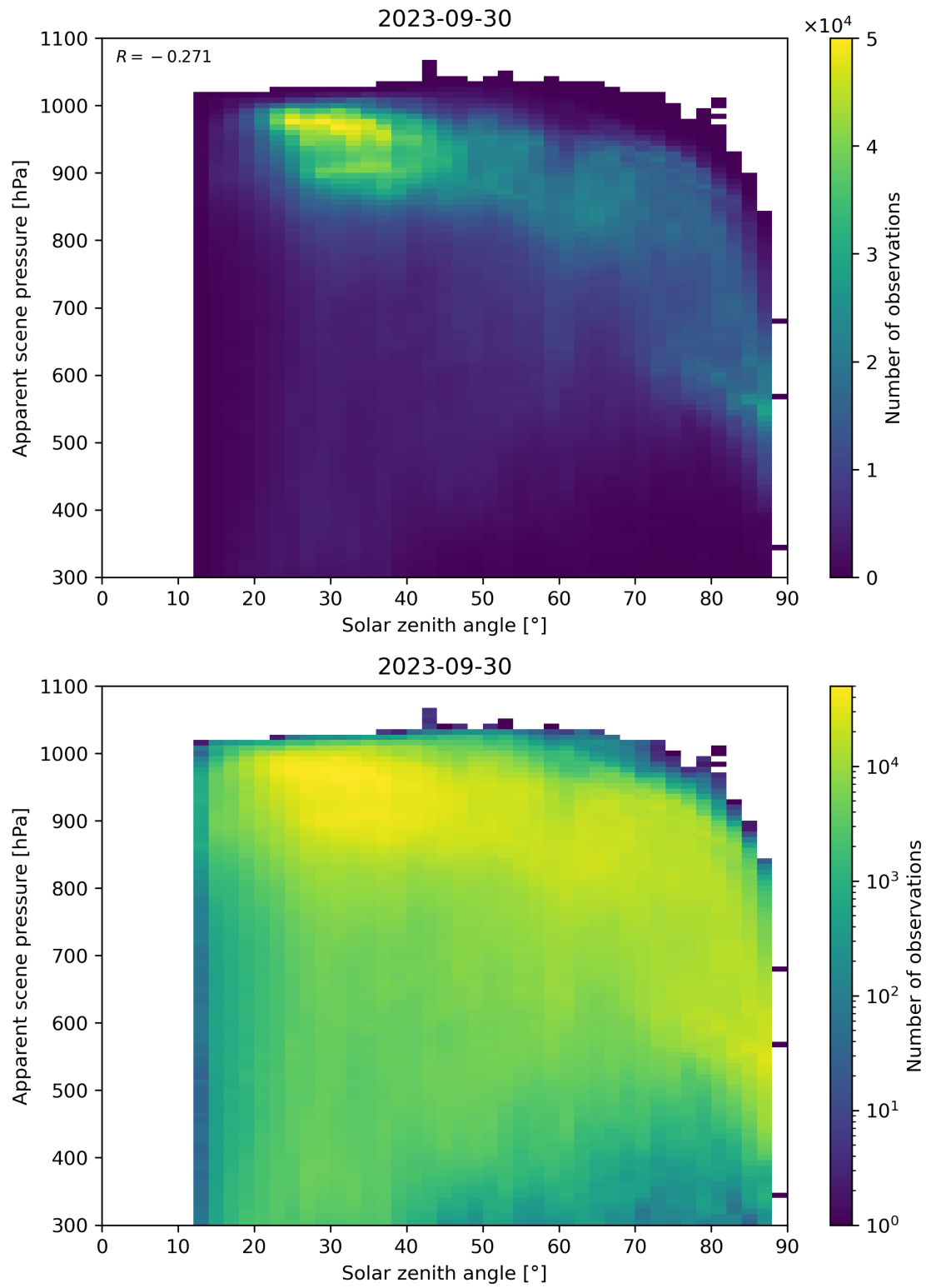
Figure 118: Scatter density plot of “Solar zenith angle” against “Apparent scene pressure” for 2023-09-29 to 2023-10-01.
