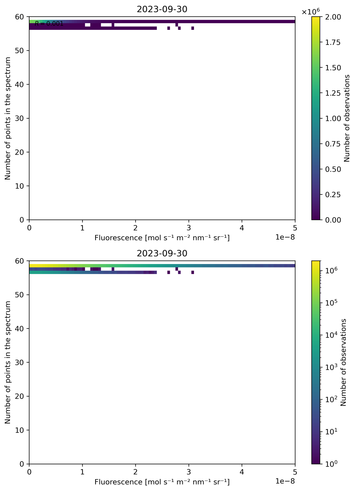
Figure 94: Scatter density plot of “Fluorescence” against “Number of points in the spectrum” for 2023-09-29 to 2023-10-01.
