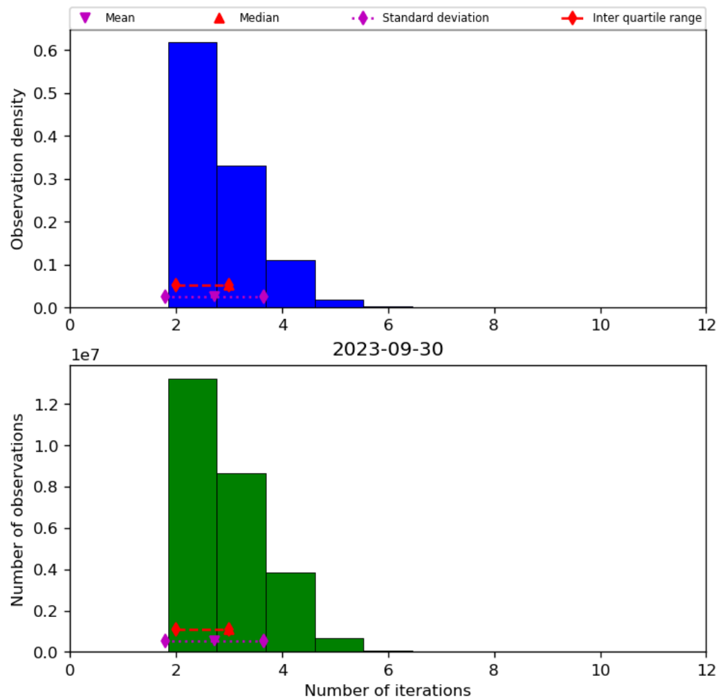
Figure 39: Histogram of “Number of iterations” for 2023-09-29 to 2023-10-01
