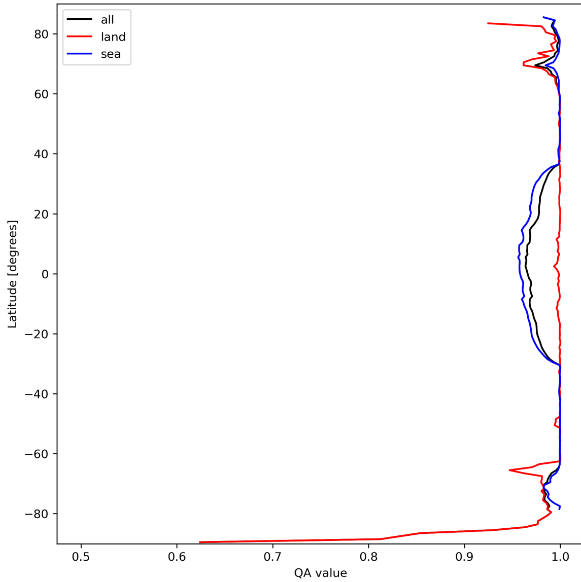
Figure 12: Zonal average of “QA value” for 2023-09-29 to 2023-10-01.
