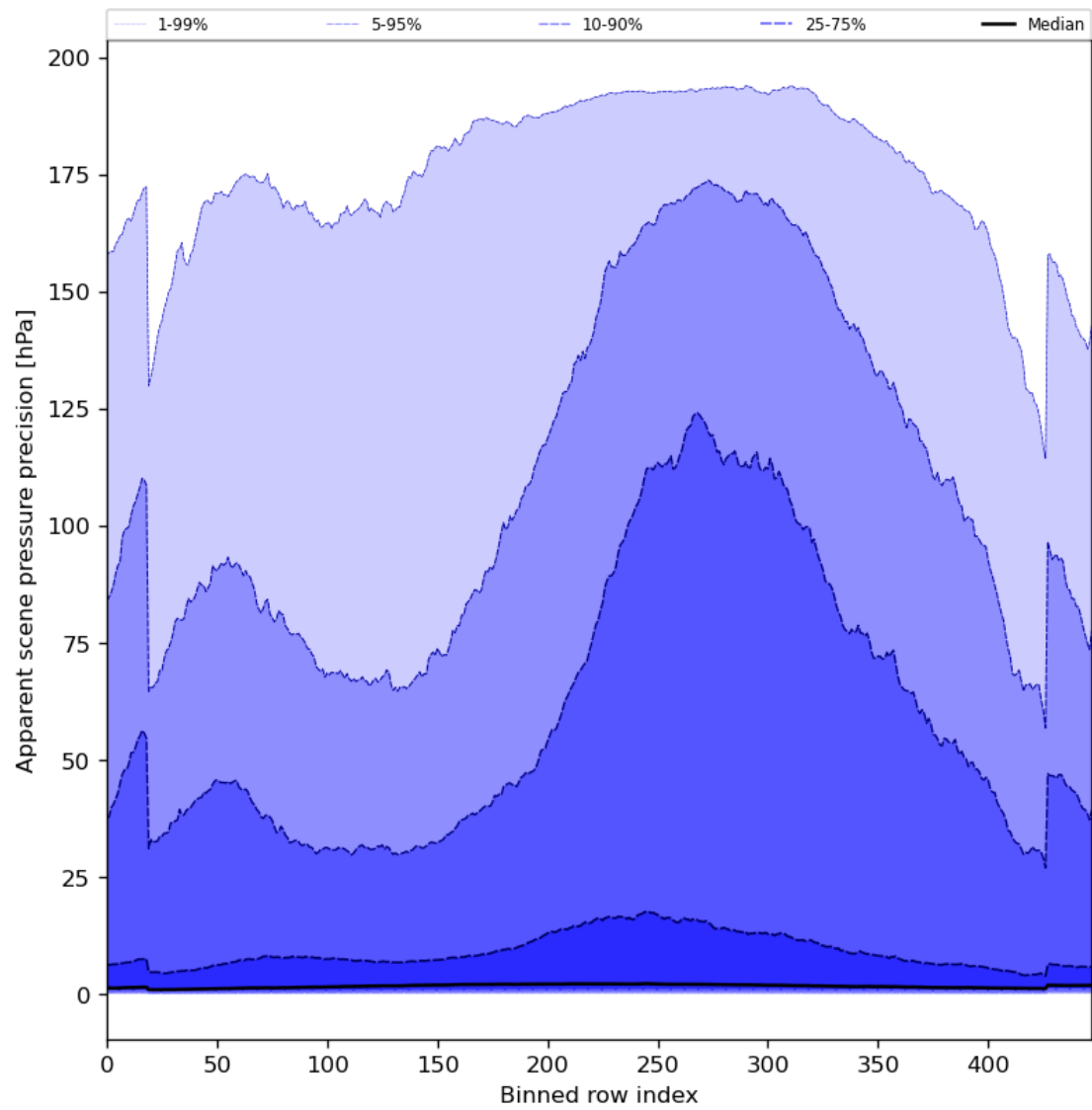
Figure 54: Along track statistics of “Apparent scene pressure precision” for 2023-09-29 to 2023-10-01
