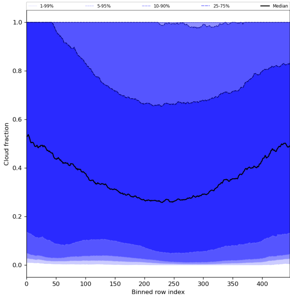
Figure 49: Along track statistics of “Cloud fraction” for 2023-09-29 to 2023-10-01
