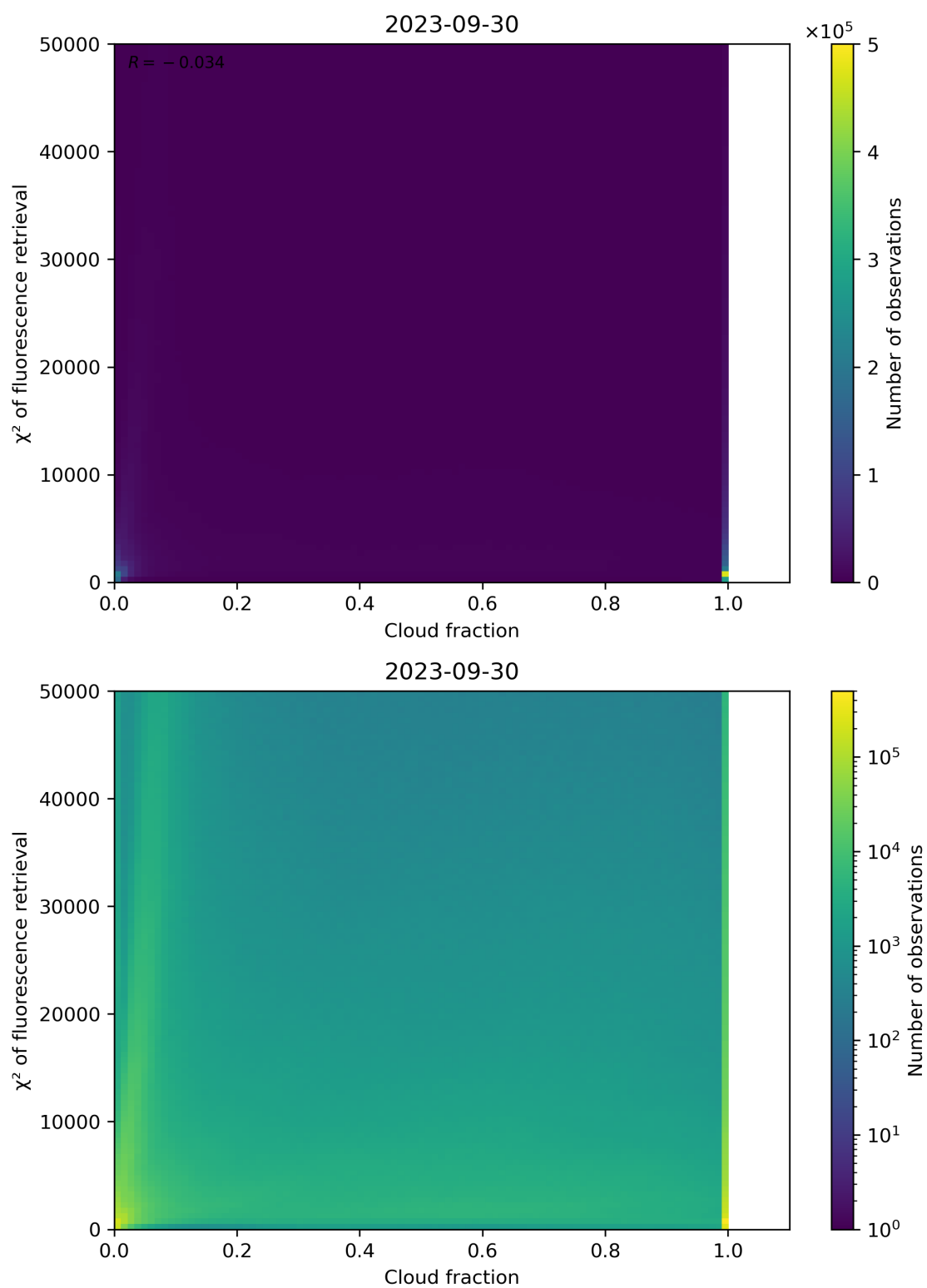
Figure 78: Scatter density plot of “Cloud fraction” against “ \chi^2 of fluorescence retrieval” for 2023-09-29 to 2023-10-01.
