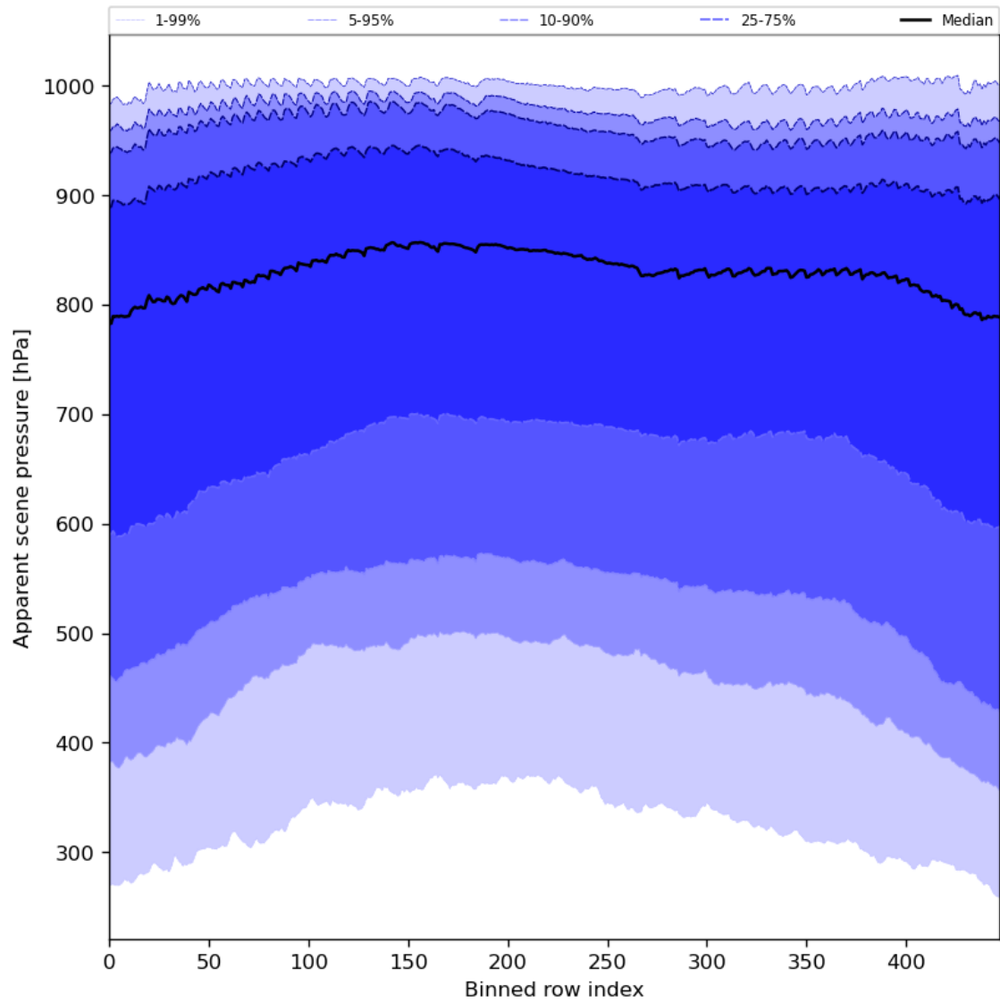
Figure 53: Along track statistics of “Apparent scene pressure” for 2023-09-29 to 2023-10-01
