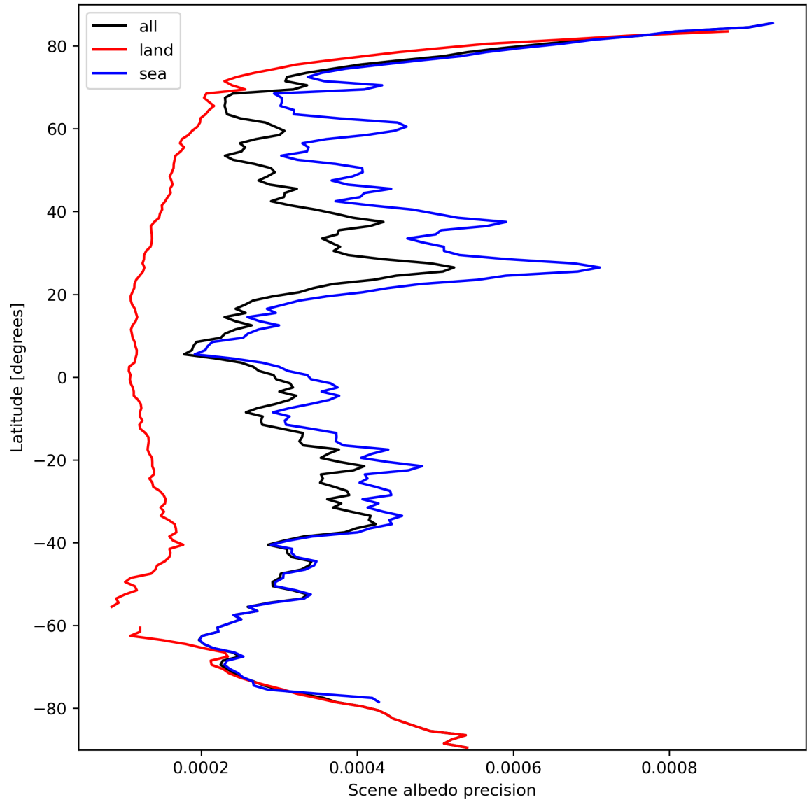
Figure 18: Zonal average of "Scene albedo precision" for 2023-09-29 to 2023-10-01.
