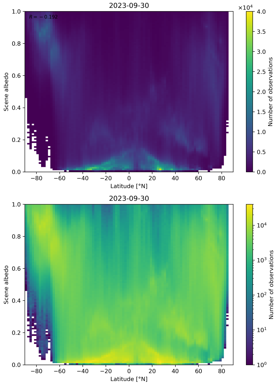
Figure 104: Scatter density plot of “Latitude” against “Scene albedo” for 2023-09-29 to 2023-10-01.
