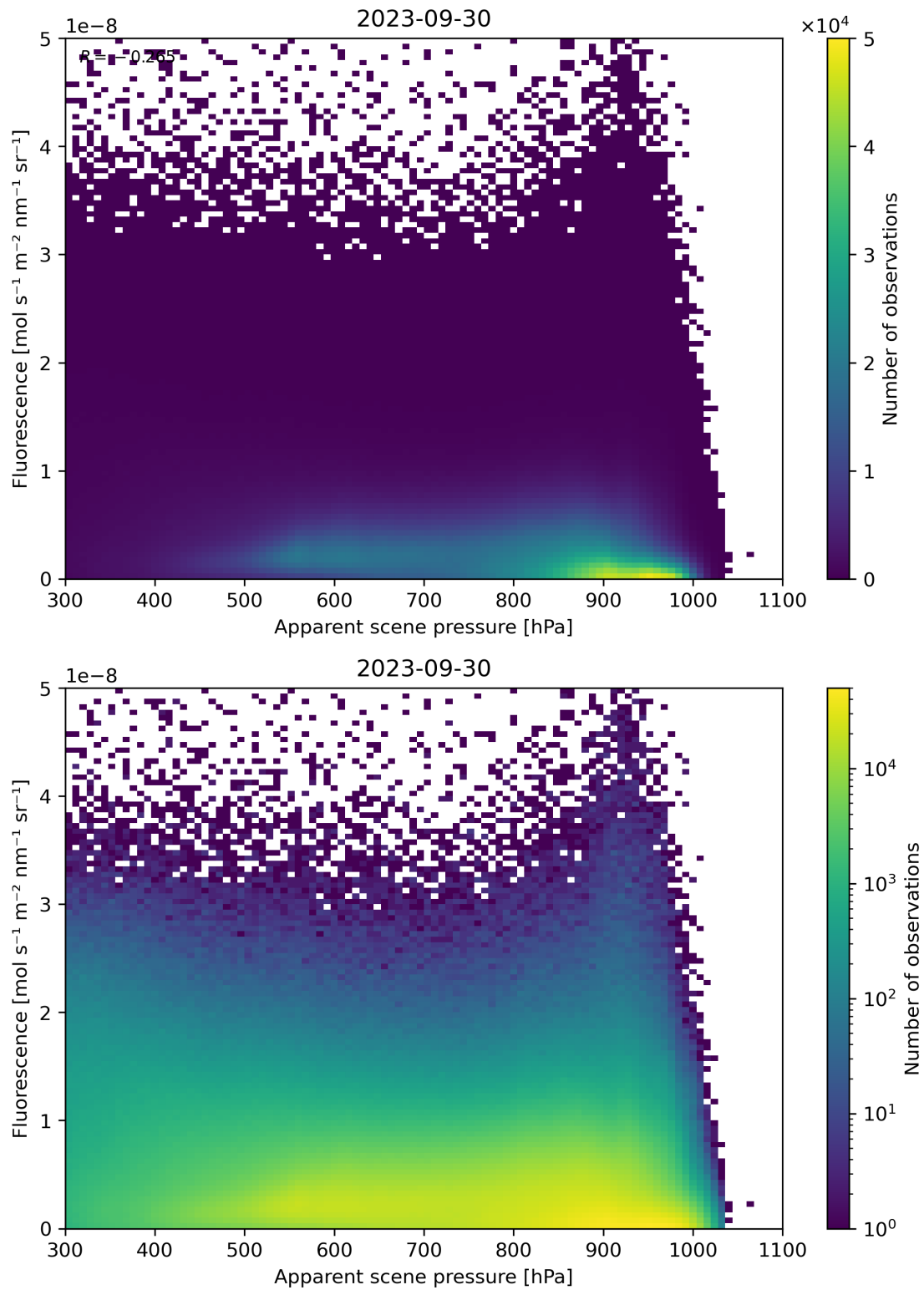
Figure 65: Scatter density plot of “Apparent scene pressure” against “Fluorescence” for 2023-09-29 to 2023-10-01.
