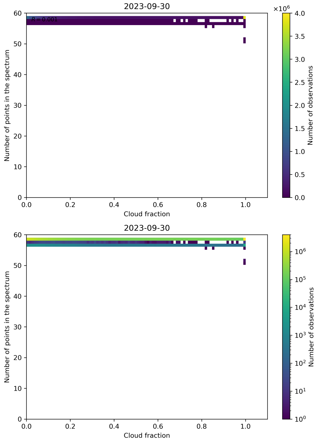
Figure 81: Scatter density plot of “Cloud fraction” against “Number of points in the spectrum” for 2023-09-29 to 2023-10-01.
