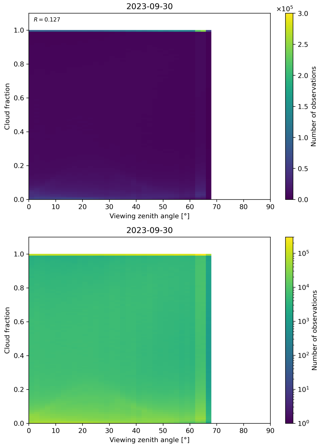
Figure 132: Scatter density plot of “Viewing zenith angle” against “Cloud fraction” for 2023-09-29 to 2023-10-01.
