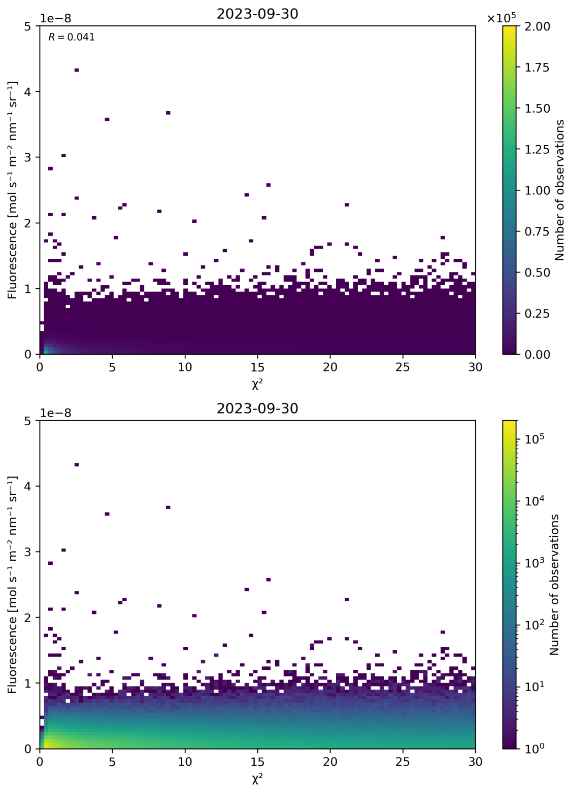
Figure 70: Scatter density plot of “ \chi^2 ” against “Fluorescence” for 2023-09-29 to 2023-10-01.
