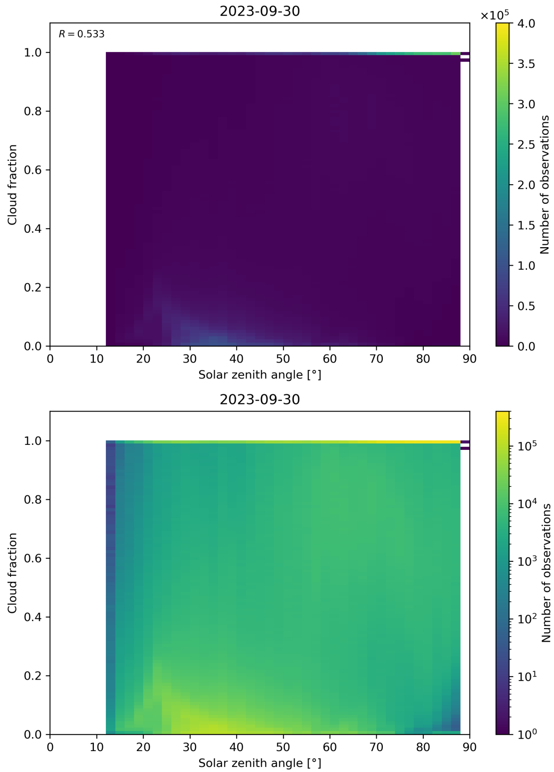
Figure 121: Scatter density plot of “Solar zenith angle” against “Cloud fraction” for 2023-09-29 to 2023-10-01.
