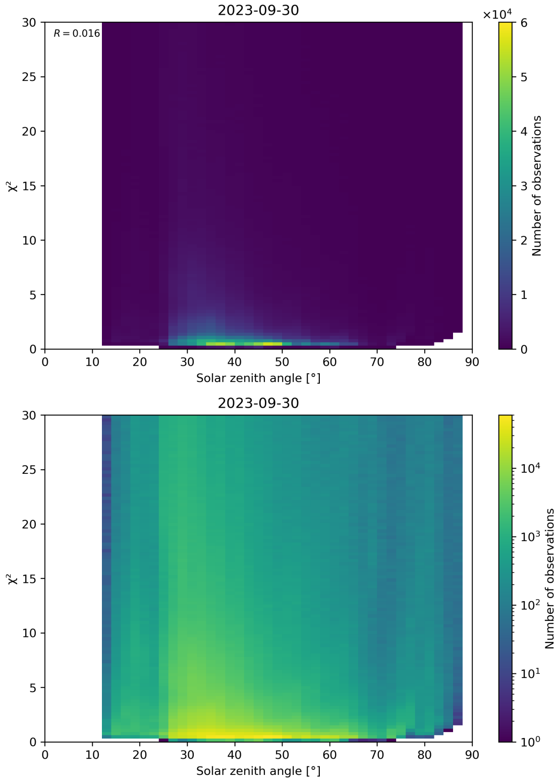
Figure 119: Scatter density plot of “Solar zenith angle” against “ \chi^2 ” for 2023-09-29 to 2023-10-01.
