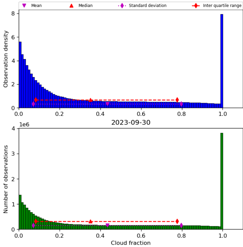
Figure 32: Histogram of “Cloud fraction” for 2023-09-29 to 2023-10-01
