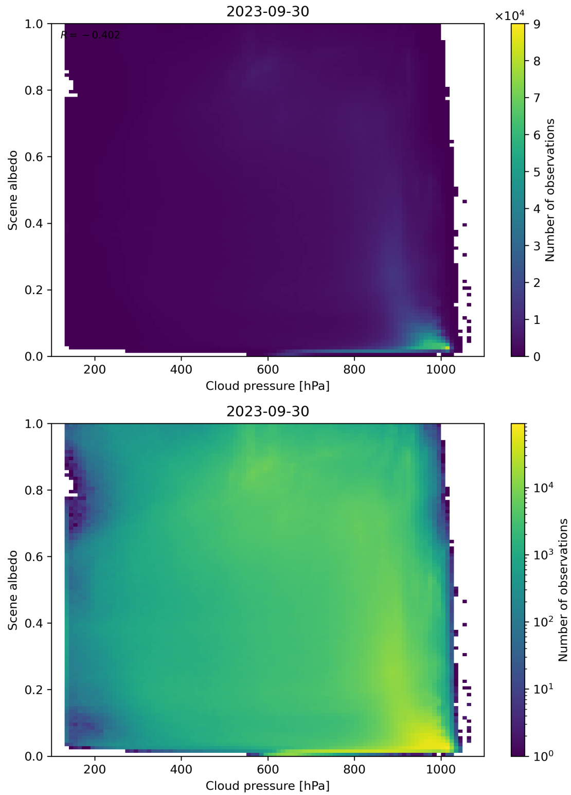
Figure 91: Scatter density plot of “Cloud pressure” against “Scene albedo” for 2023-09-29 to 2023-10-01.
