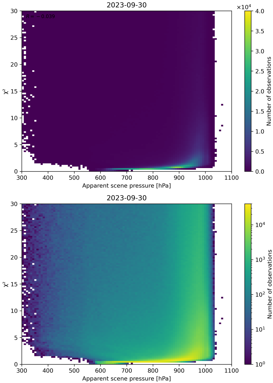
Figure 63: Scatter density plot of “Apparent scene pressure” against “ \chi^2 ” for 2023-09-29 to 2023-10-01.
