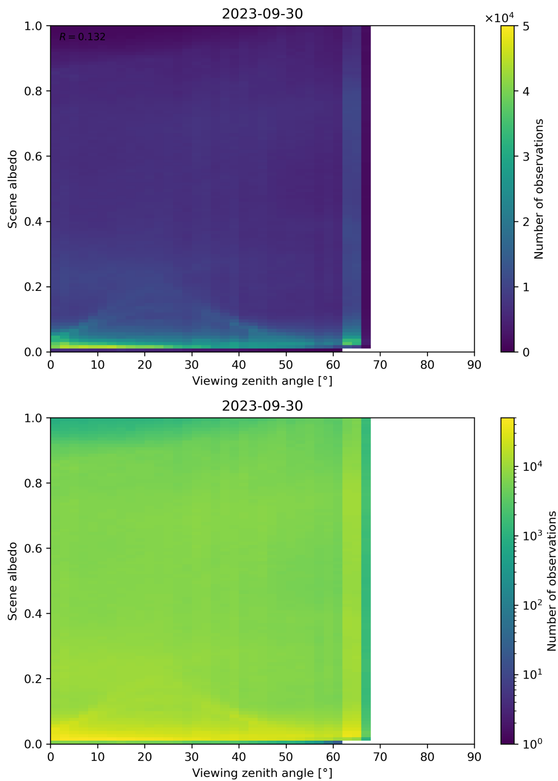
Figure 138: Scatter density plot of “Viewing zenith angle” against “Scene albedo” for 2023-09-29 to 2023-10-01.
