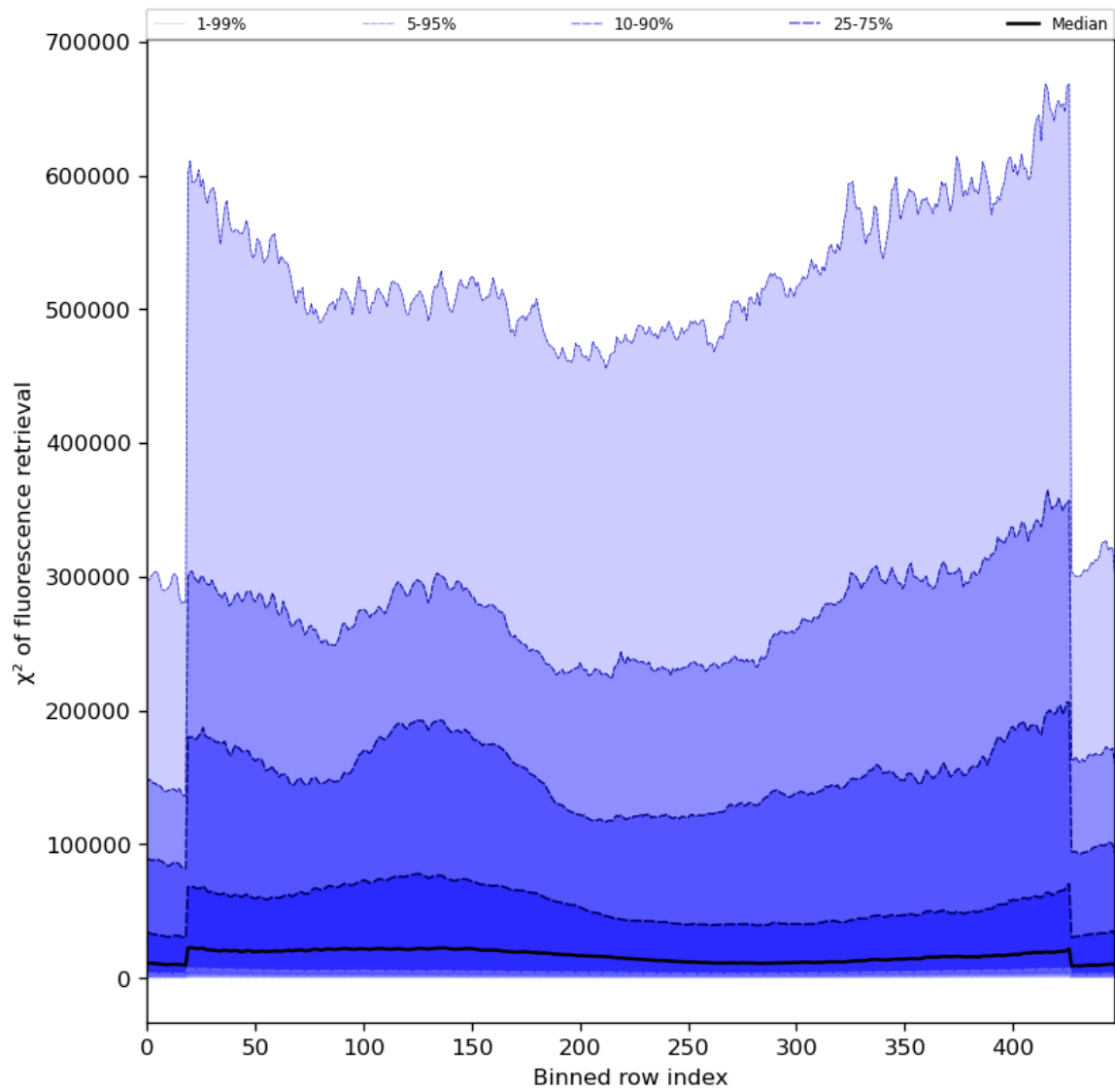
Figure 59: Along track statistics of “ \chi^2 of fluorescence retrieval” for 2023-09-29 to 2023-10-01
