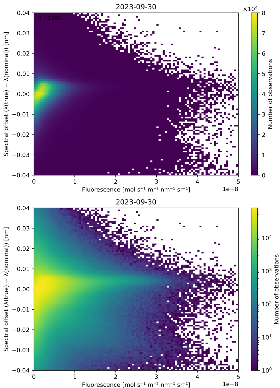
Figure 95: Scatter density plot of “Fluorescence” against “Spectral offset ( \lambda(\text{true}) - \lambda(\text{nominal}) )” for 2023-09-29 to 2023-10-01.
