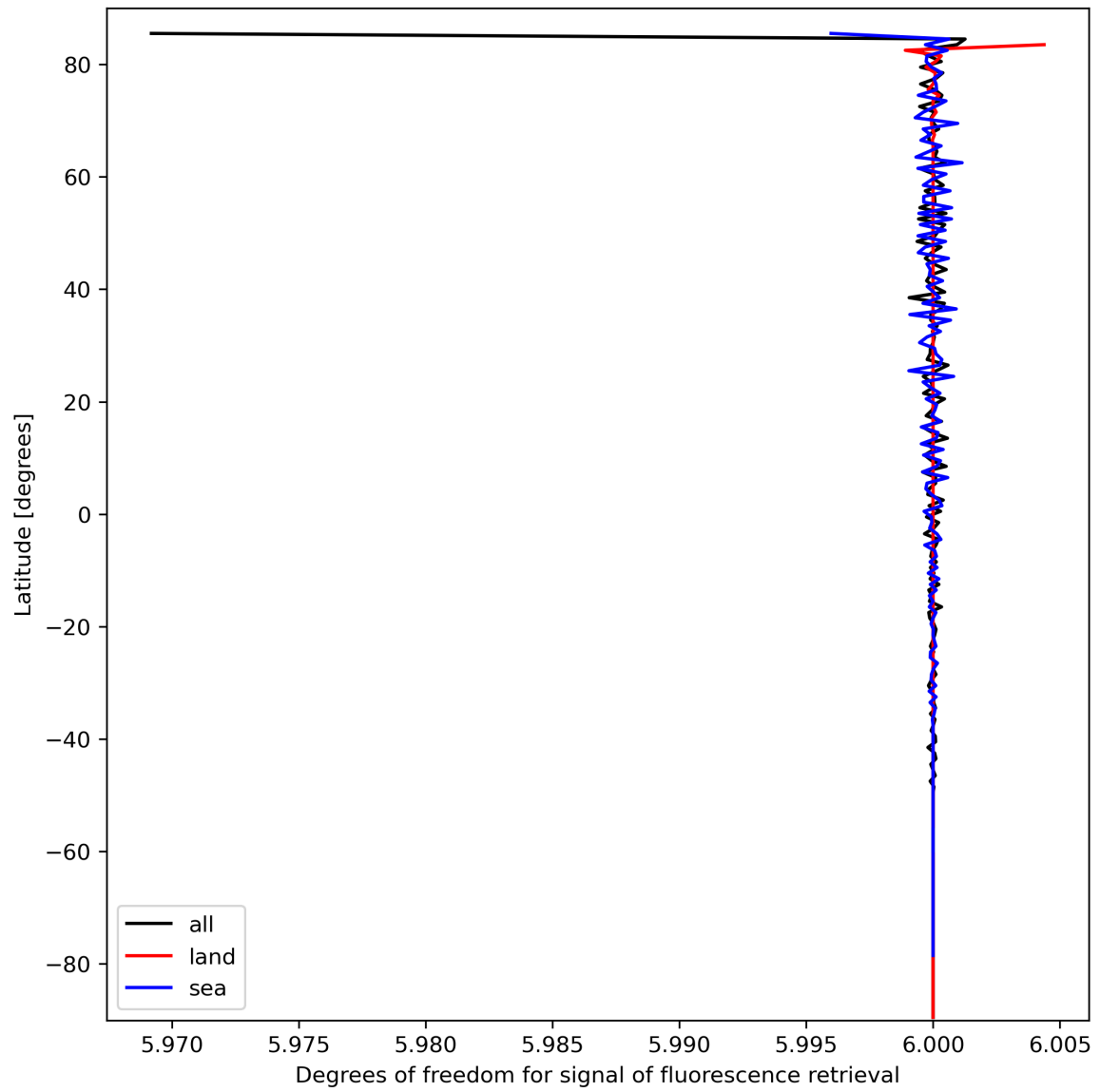
Figure 26: Zonal average of “Degrees of freedom for signal of fluorescence retrieval” for 2023-09-29 to 2023-10-01.
