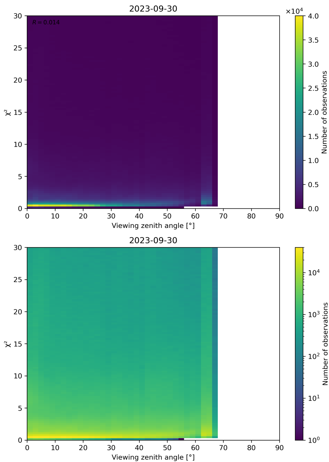
Figure 130: Scatter density plot of “Viewing zenith angle” against “ \chi^2 ” for 2023-09-29 to 2023-10-01.
