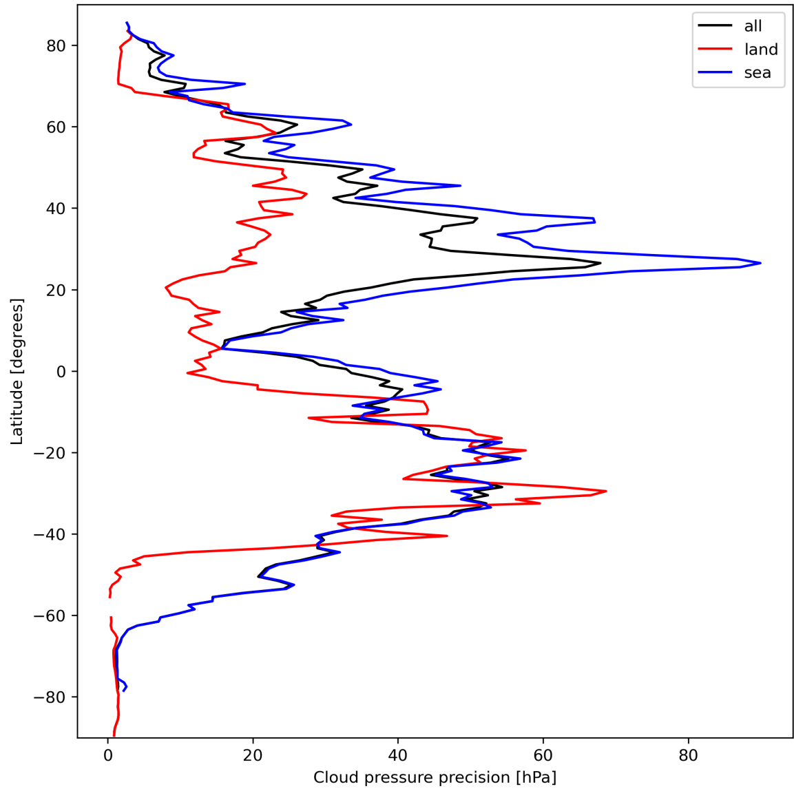
Figure 14: Zonal average of “Cloud pressure precision” for 2023-09-29 to 2023-10-01.
