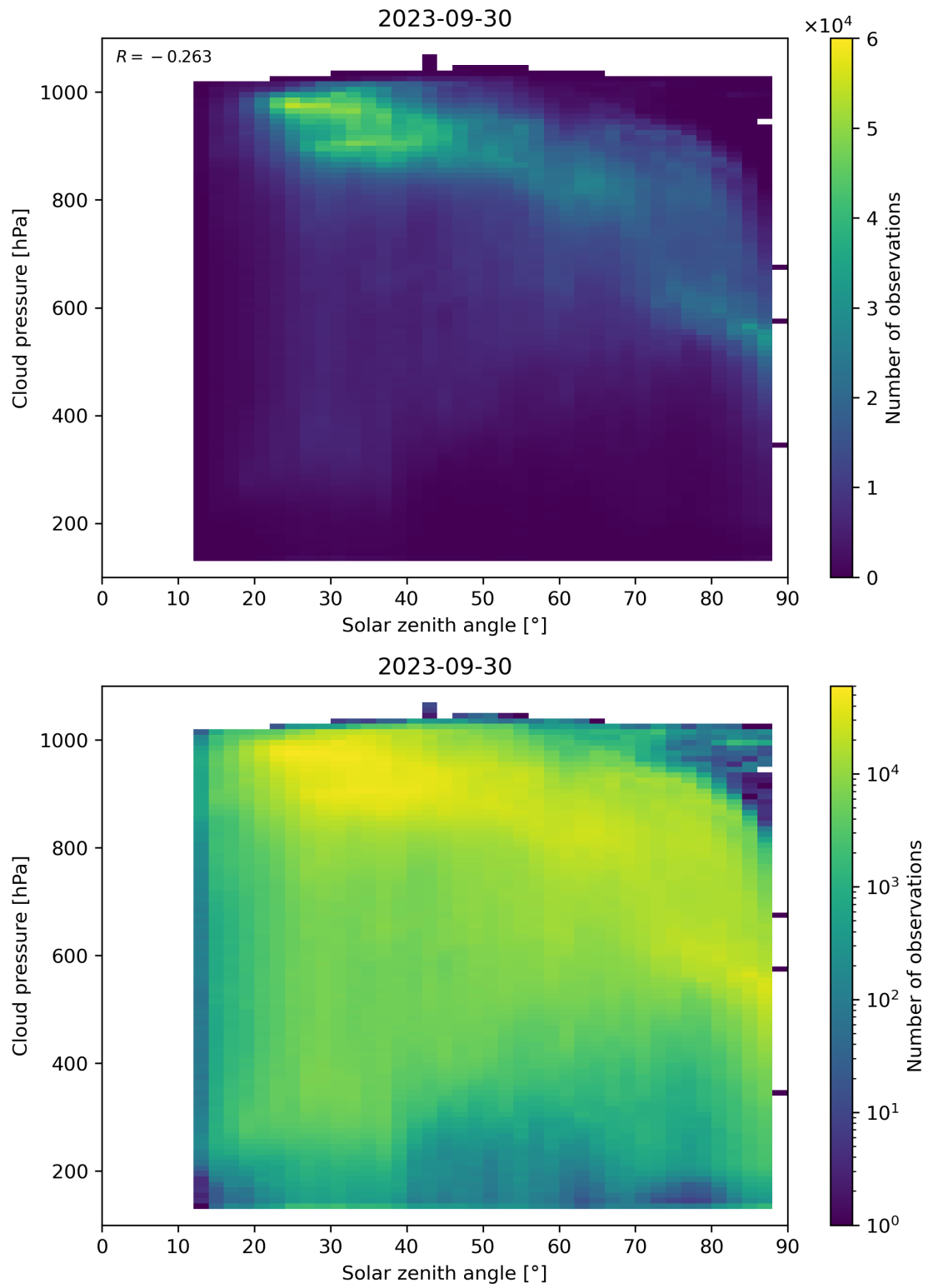
Figure 122: Scatter density plot of “Solar zenith angle” against “Cloud pressure” for 2023-09-29 to 2023-10-01.
