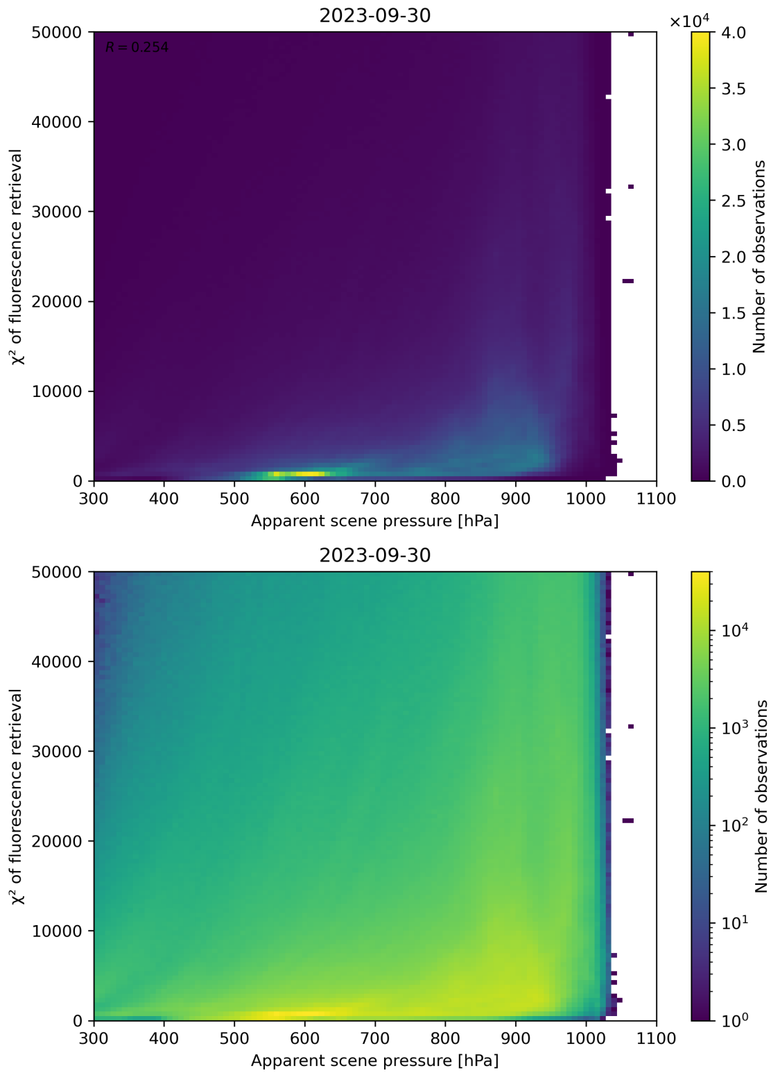
Figure 64: Scatter density plot of “Apparent scene pressure” against “ \chi^2 of fluorescence retrieval” for 2023-09-29 to 2023-10-01.
