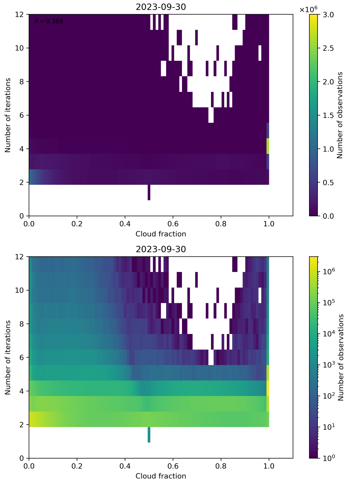
Figure 80: Scatter density plot of “Cloud fraction” against “Number of iterations” for 2023-09-29 to 2023-10-01.
