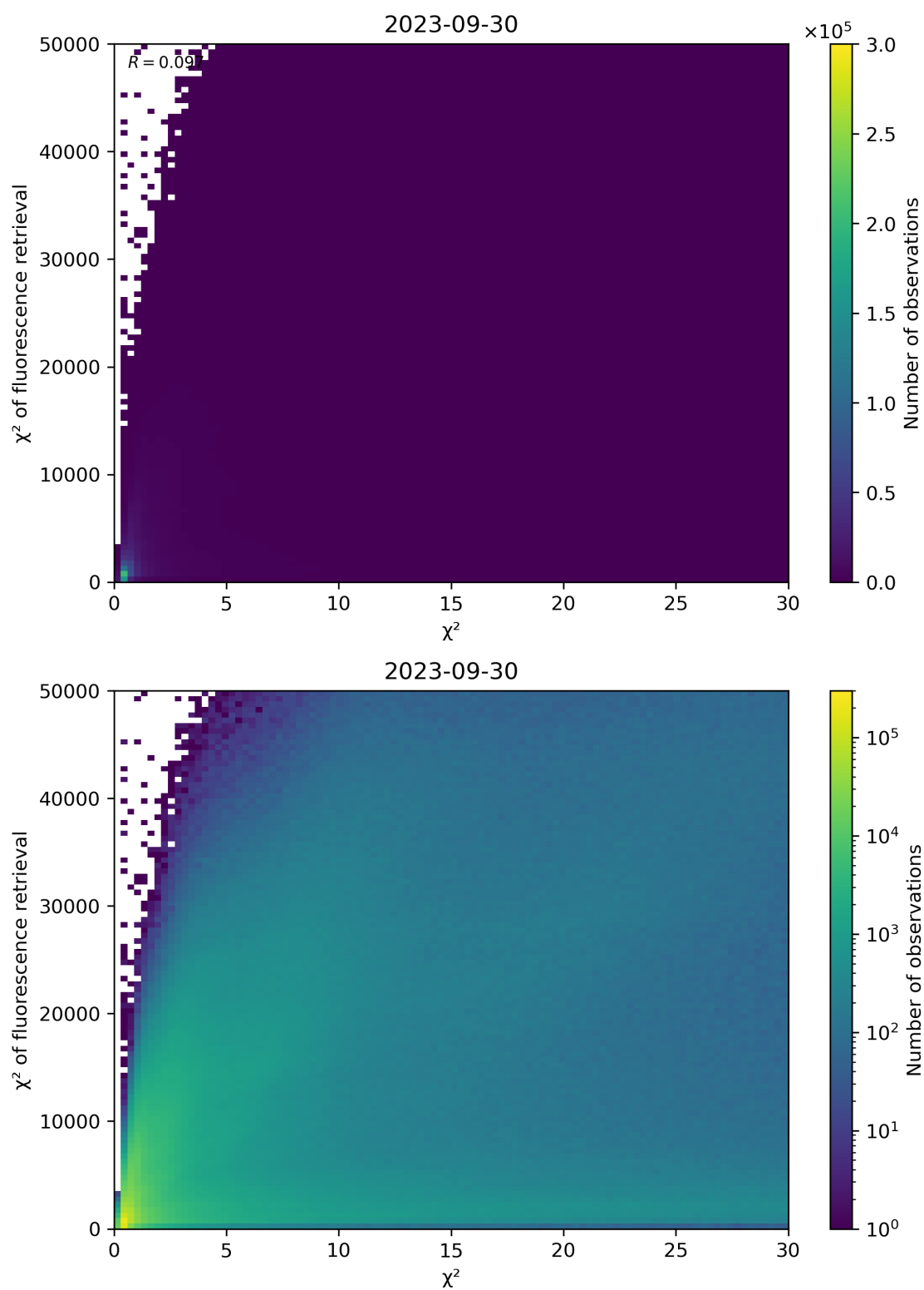
Figure 69: Scatter density plot of “ \chi^2 ” against “ \chi^2 of fluorescence retrieval” for 2023-09-29 to 2023-10-01.
