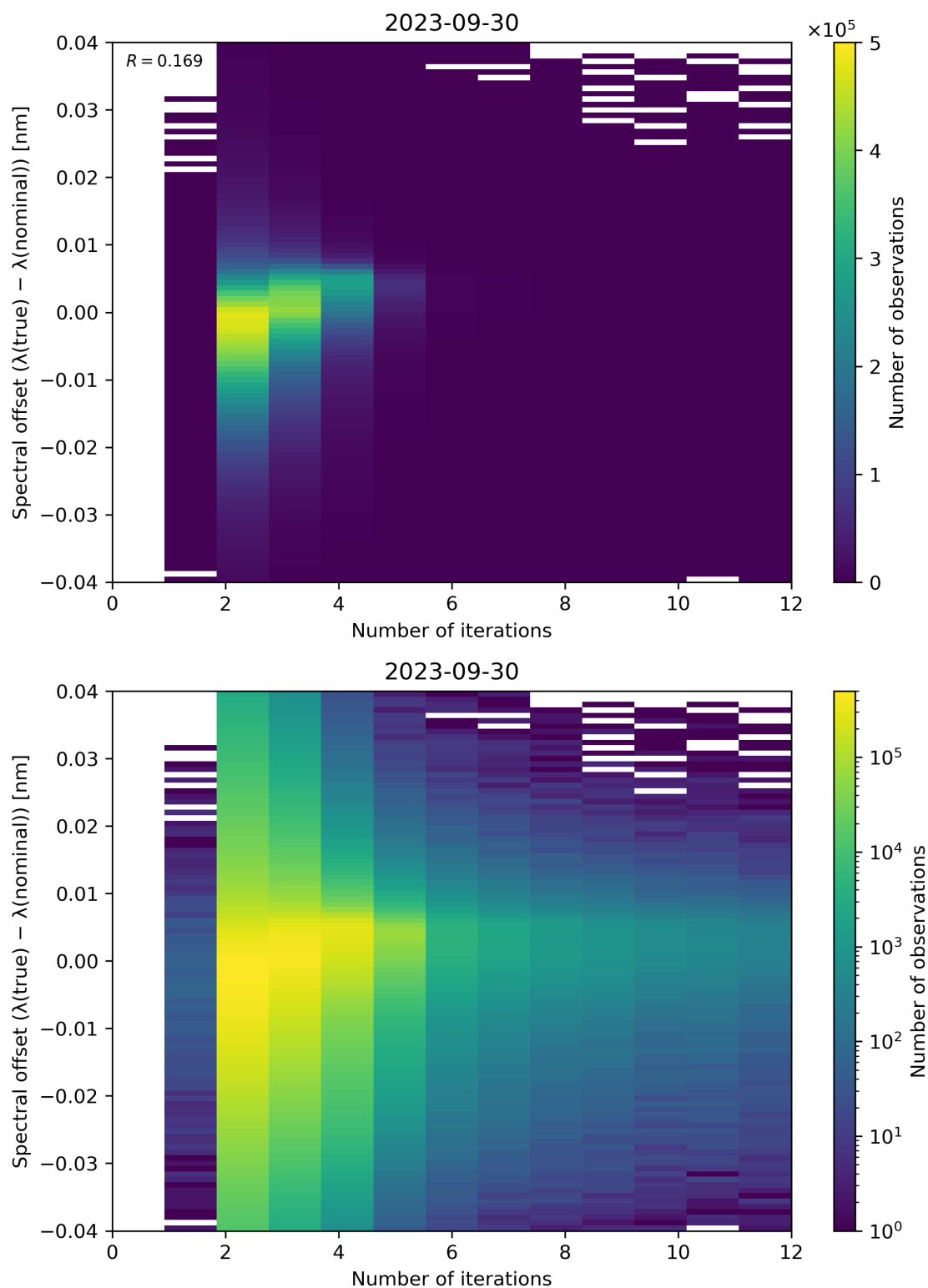
Figure 109: Scatter density plot of “Number of iterations” against “Spectral offset ( \lambda(\text{true}) - \lambda(\text{nominal}) )” for 2023-09-29 to 2023-10-01.
