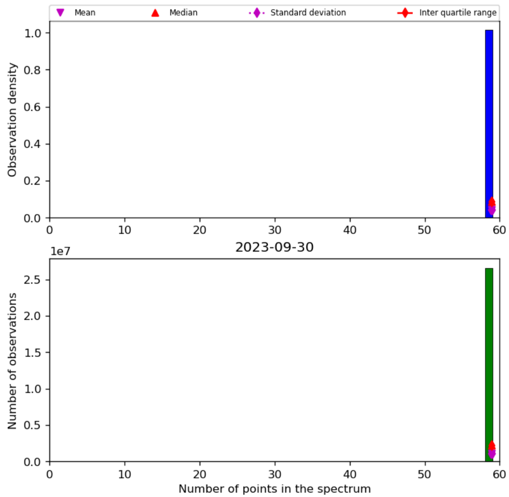
Figure 44: Histogram of "Number of points in the spectrum" for 2023-09-29 to 2023-10-01
