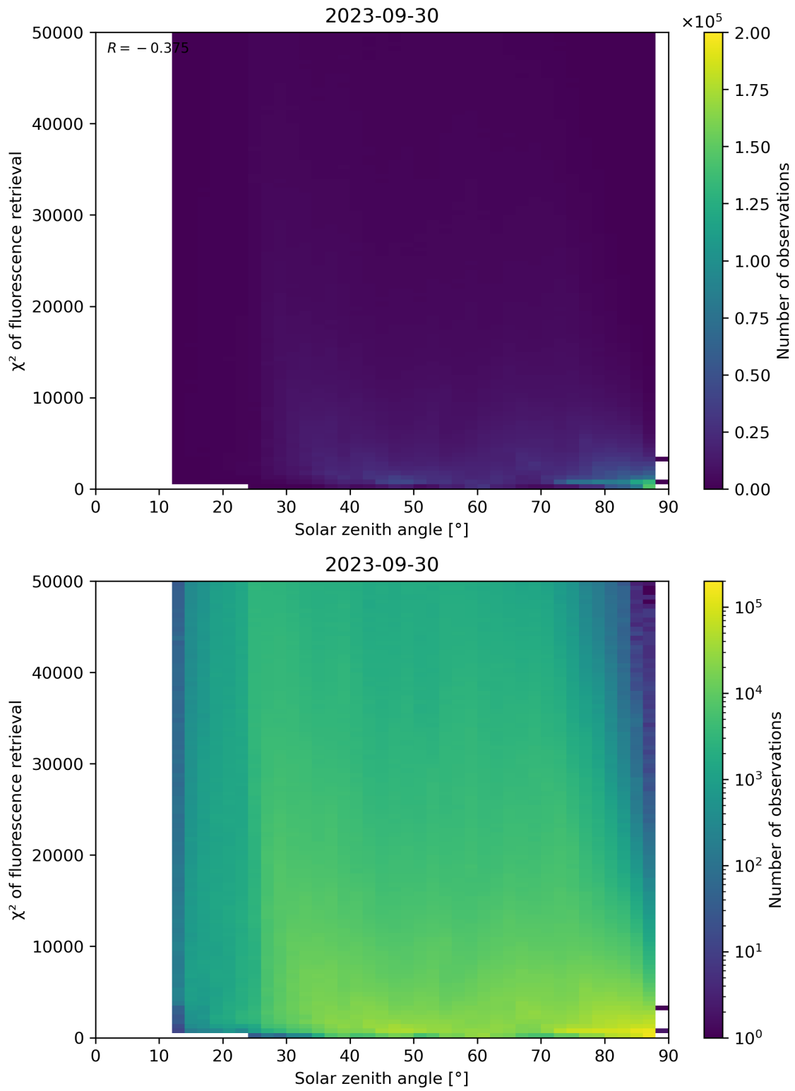
Figure 120: Scatter density plot of “Solar zenith angle” against “ \chi^2 of fluorescence retrieval” for 2023-09-29 to 2023-10-01.
