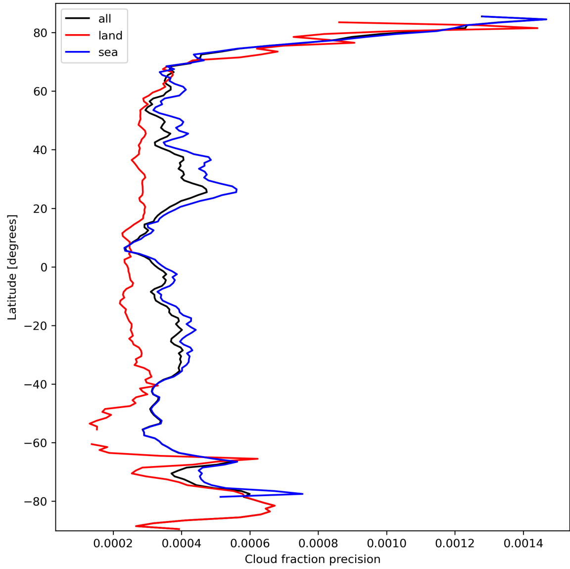
Figure 16: Zonal average of “Cloud fraction precision” for 2023-09-29 to 2023-10-01.
