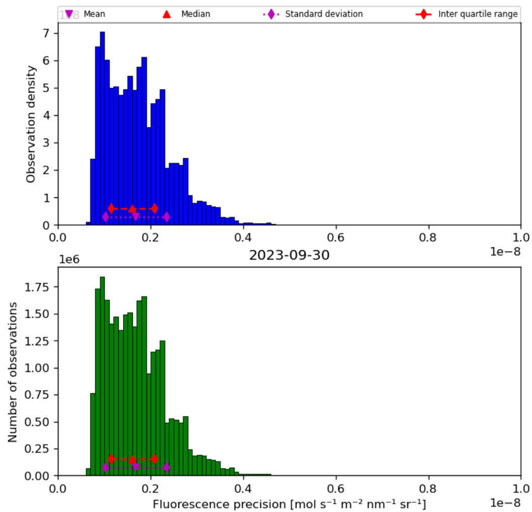
Figure 41: Histogram of “Fluorescence precision” for 2023-09-29 to 2023-10-01
