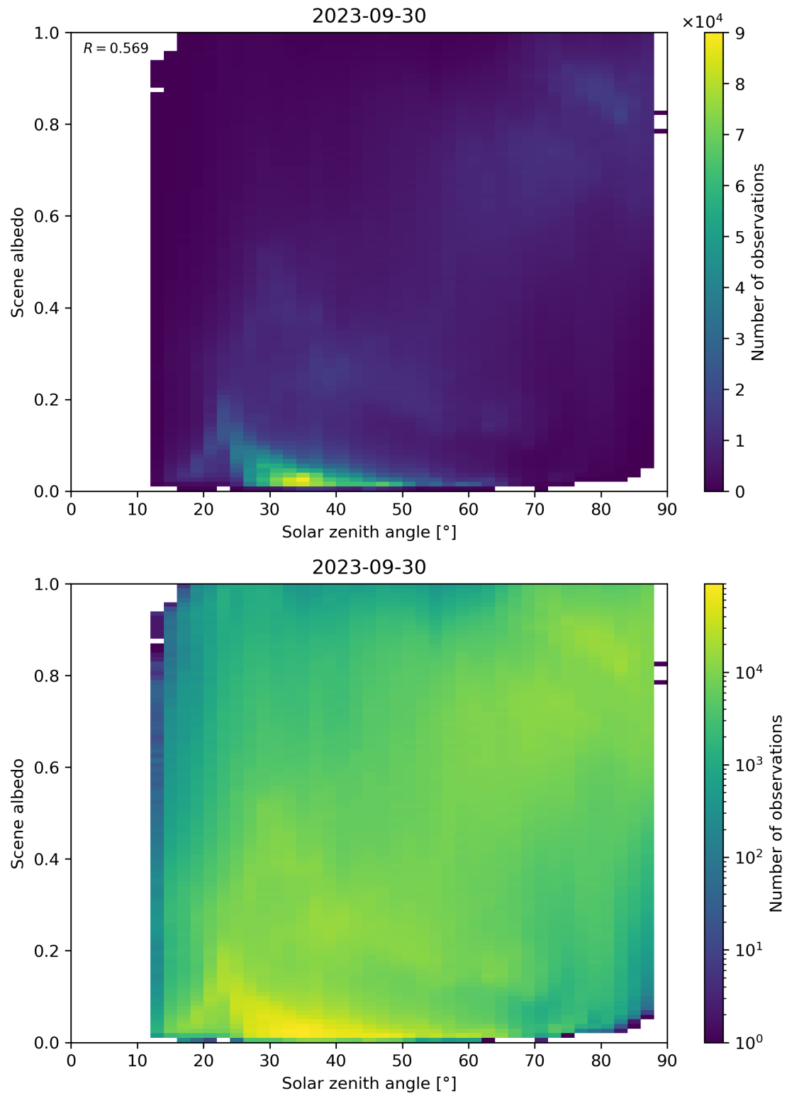
Figure 127: Scatter density plot of “Solar zenith angle” against “Scene albedo” for 2023-09-29 to 2023-10-01.
