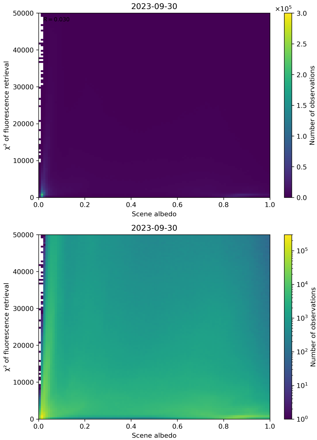
Figure 113: Scatter density plot of “Scene albedo” against “ \chi^2 of fluorescence retrieval” for 2023-09-29 to 2023-10-01.
