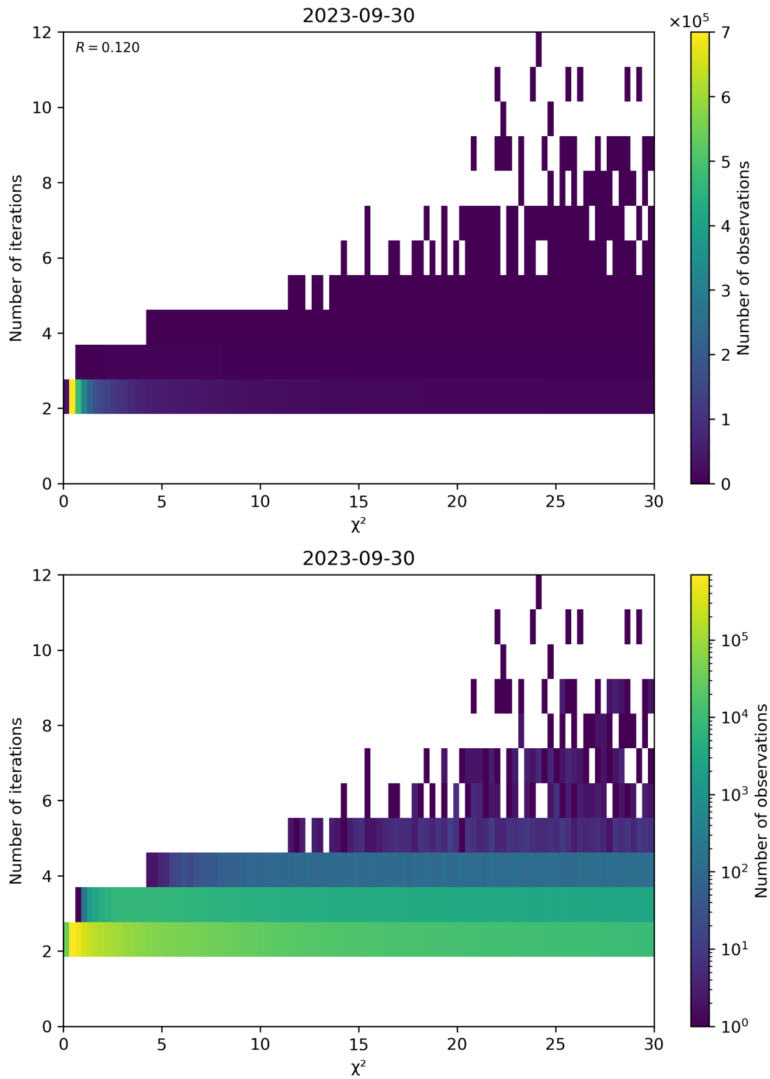
Figure 73: Scatter density plot of “ \chi^2 ” against “Number of iterations” for 2023-09-29 to 2023-10-01.
