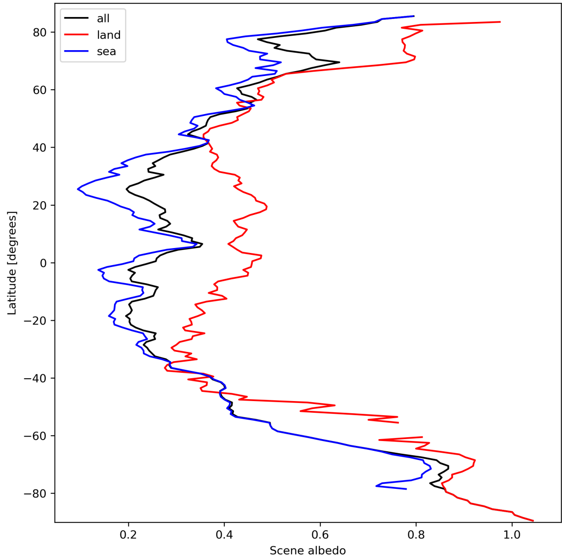
Figure 17: Zonal average of “Scene albedo” for 2023-09-29 to 2023-10-01.
