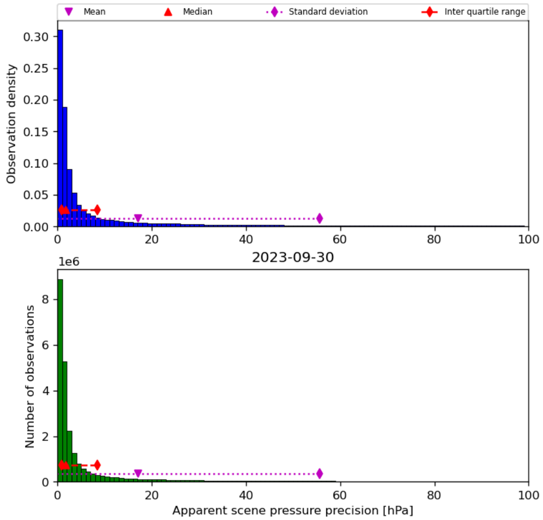
Figure 37: Histogram of “Apparent scene pressure precision” for 2023-09-29 to 2023-10-01
