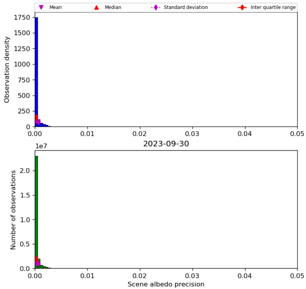
Figure 35: Histogram of “Scene albedo precision” for 2023-09-29 to 2023-10-01
