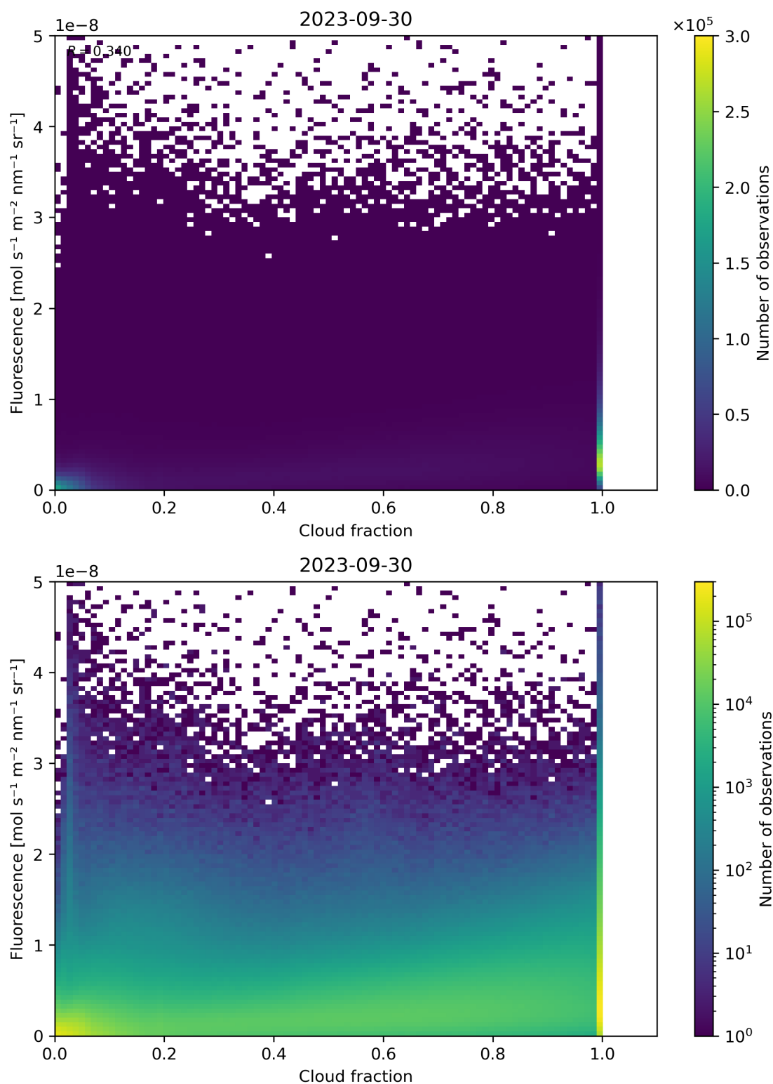
Figure 79: Scatter density plot of “Cloud fraction” against “Fluorescence” for 2023-09-29 to 2023-10-01.
