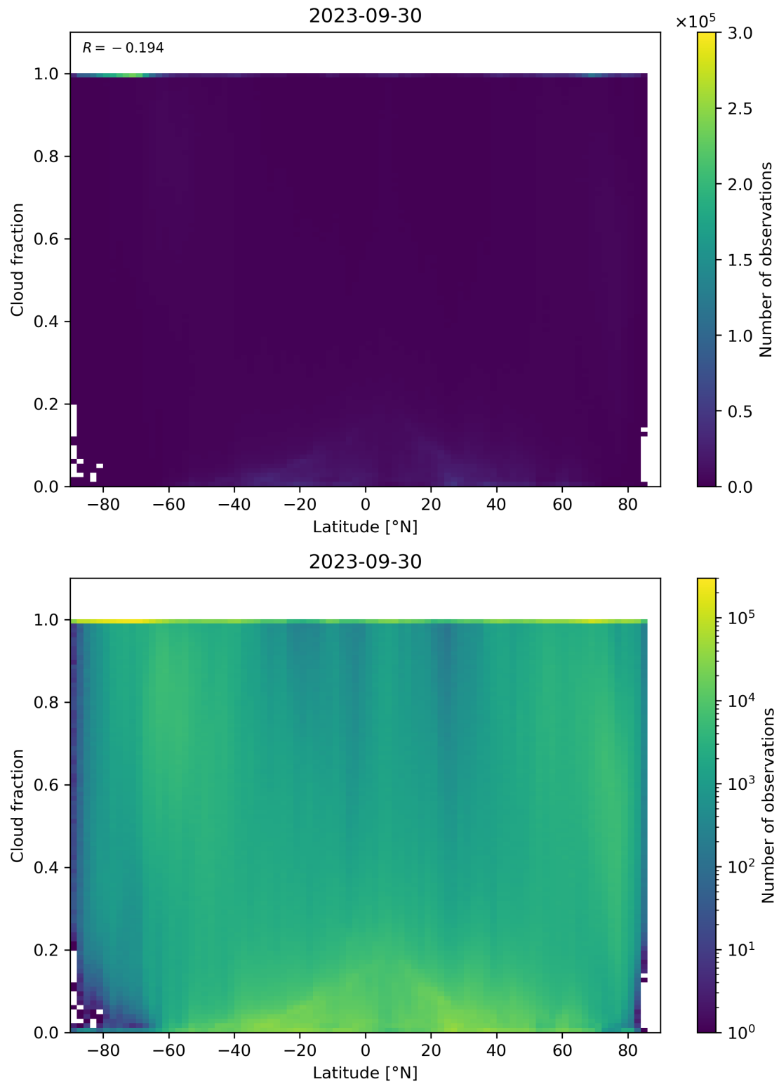
Figure 99: Scatter density plot of “Latitude” against “Cloud fraction” for 2023-09-29 to 2023-10-01.
