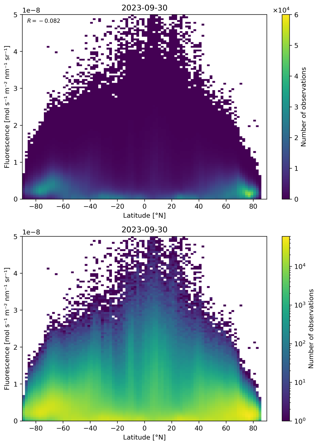
Figure 101: Scatter density plot of “Latitude” against “Fluorescence” for 2023-09-29 to 2023-10-01.
