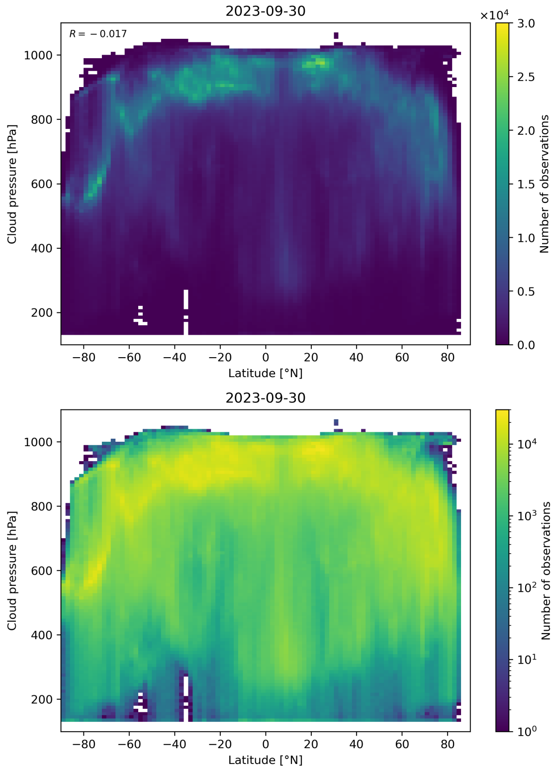
Figure 100: Scatter density plot of “Latitude” against “Cloud pressure” for 2023-09-29 to 2023-10-01.
