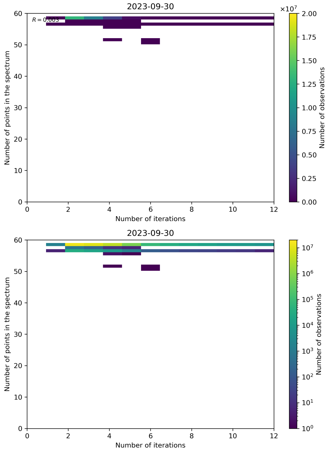
Figure 108: Scatter density plot of “Number of iterations” against “Number of points in the spectrum” for 2023-09-29 to 2023-10-01.
