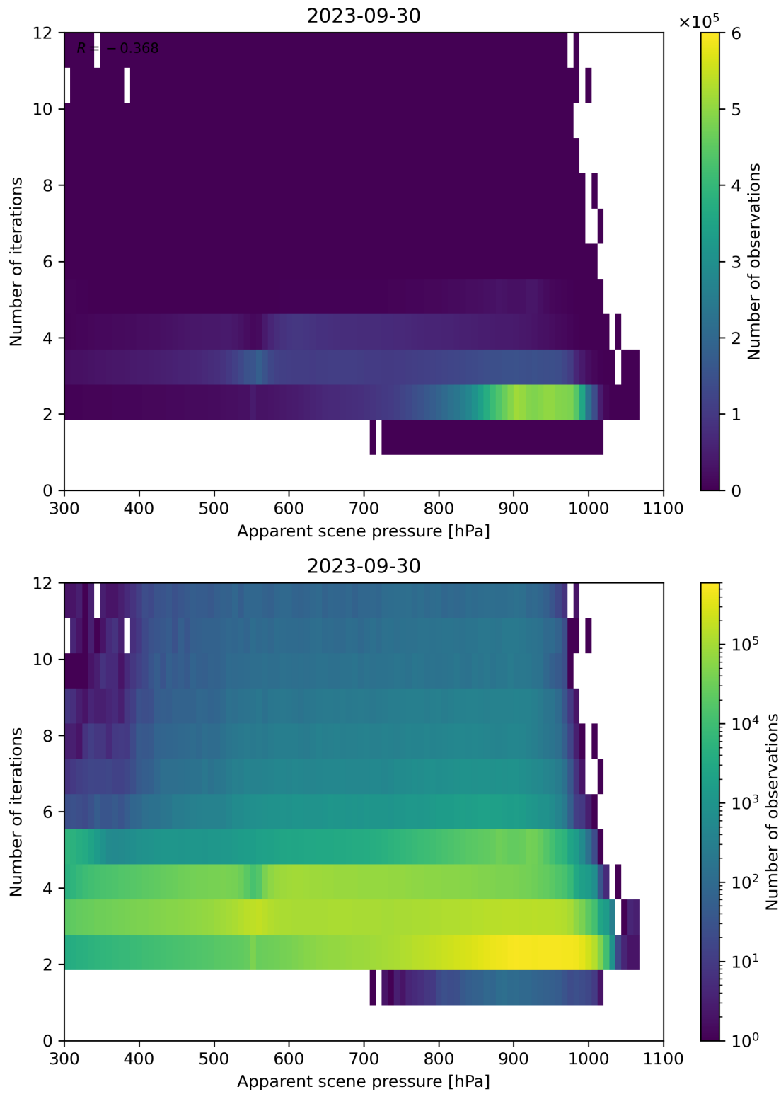
Figure 66: Scatter density plot of “Apparent scene pressure” against “Number of iterations” for 2023-09-29 to 2023-10-01.
