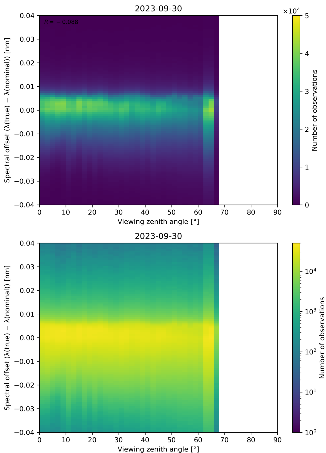
Figure 140: Scatter density plot of “Viewing zenith angle” against “Spectral offset ( \lambda(\text{true}) - \lambda(\text{nominal}) )” for 2023-09-29 to 2023-10-01.
