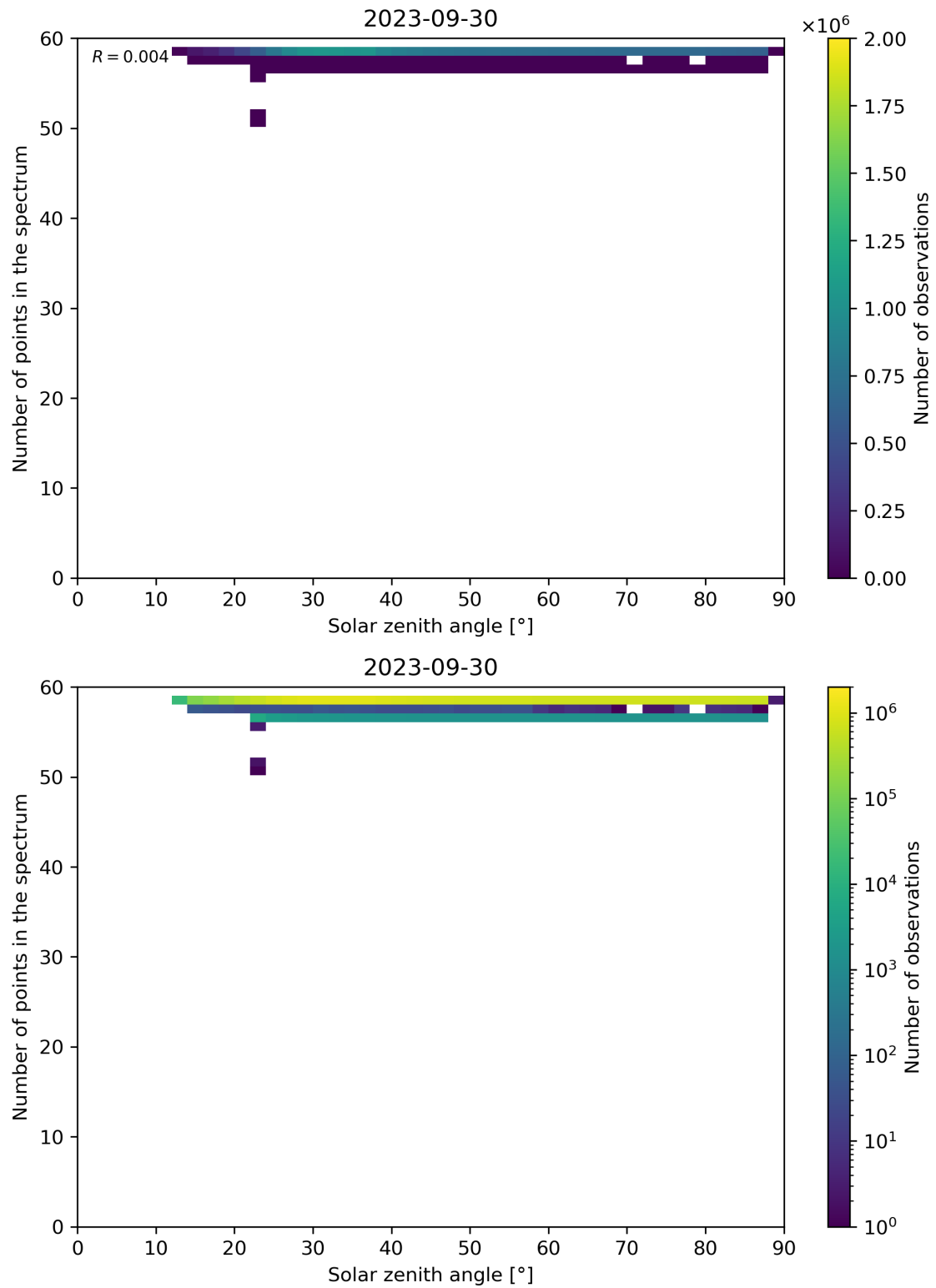
Figure 126: Scatter density plot of “Solar zenith angle” against “Number of points in the spectrum” for 2023-09-29 to 2023-10-01.
