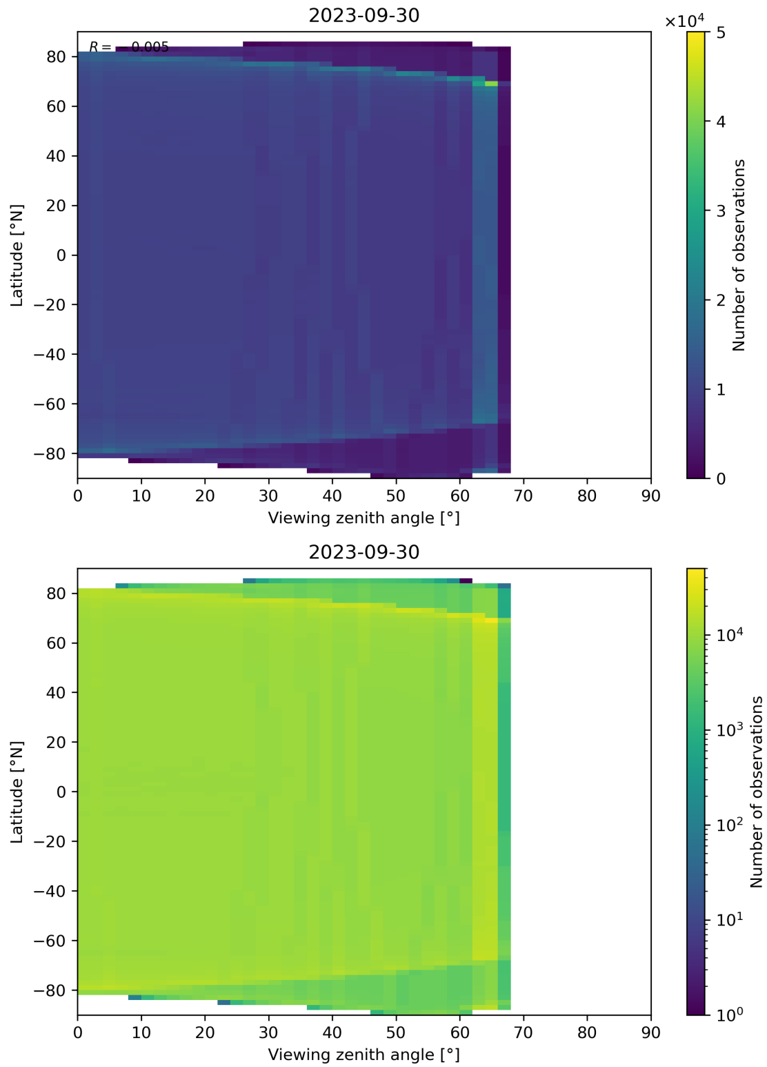
Figure 135: Scatter density plot of “Viewing zenith angle” against “Latitude” for 2023-09-29 to 2023-10-01.
