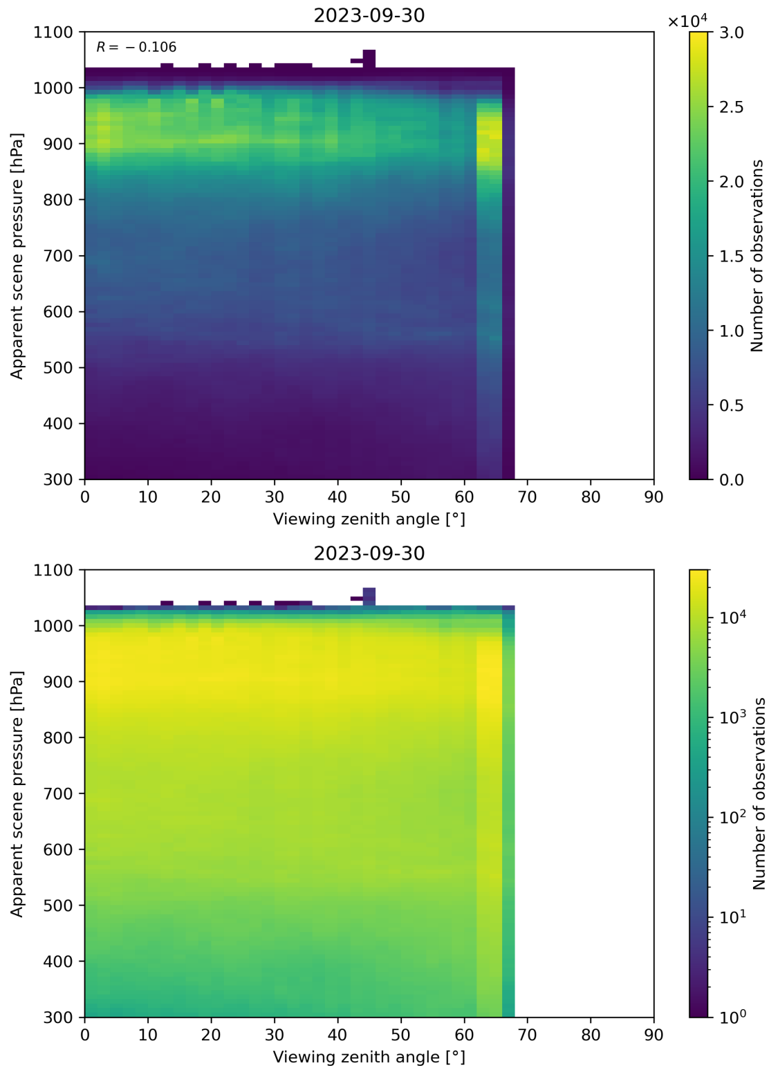
Figure 129: Scatter density plot of “Viewing zenith angle” against “Apparent scene pressure” for 2023-09-29 to 2023-10-01.
