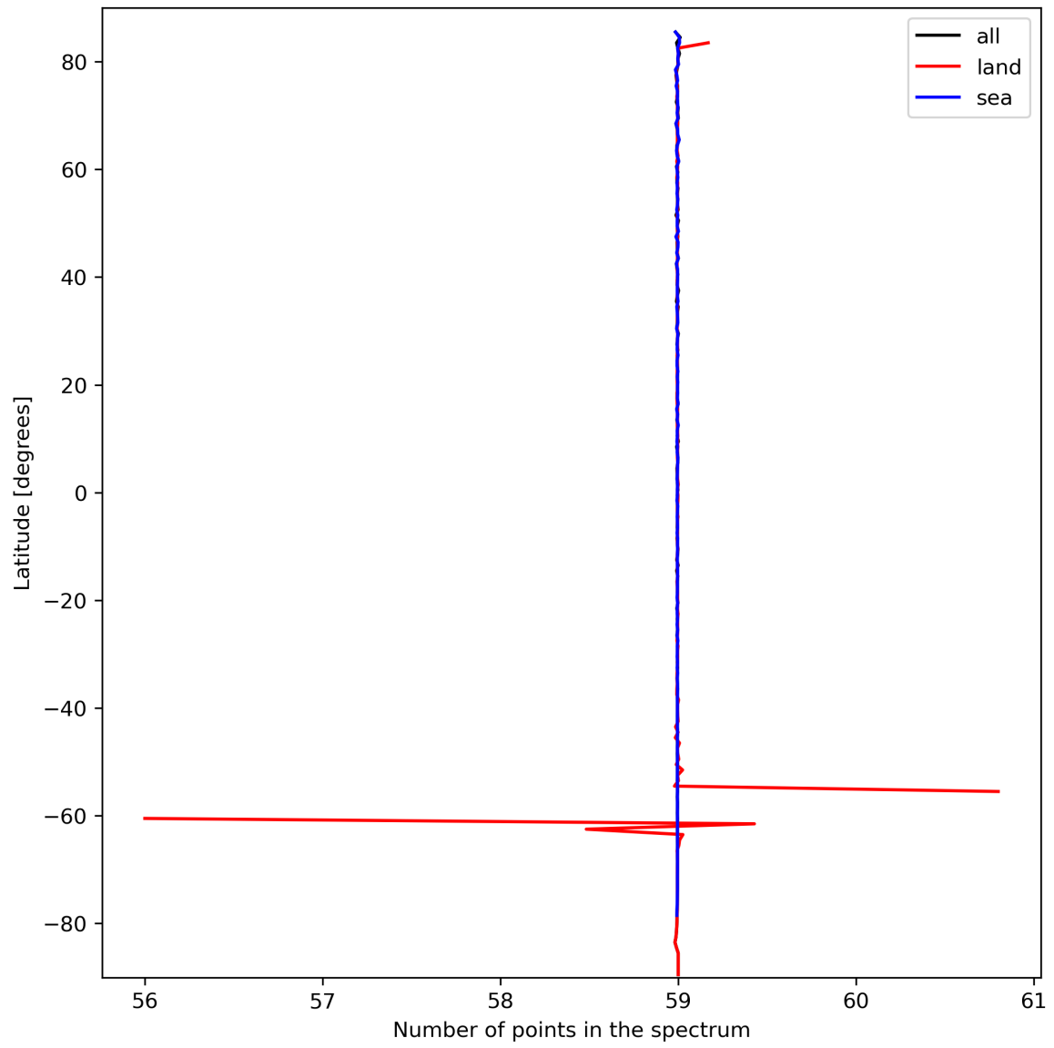
Figure 27: Zonal average of “Number of points in the spectrum” for 2023-09-29 to 2023-10-01.
