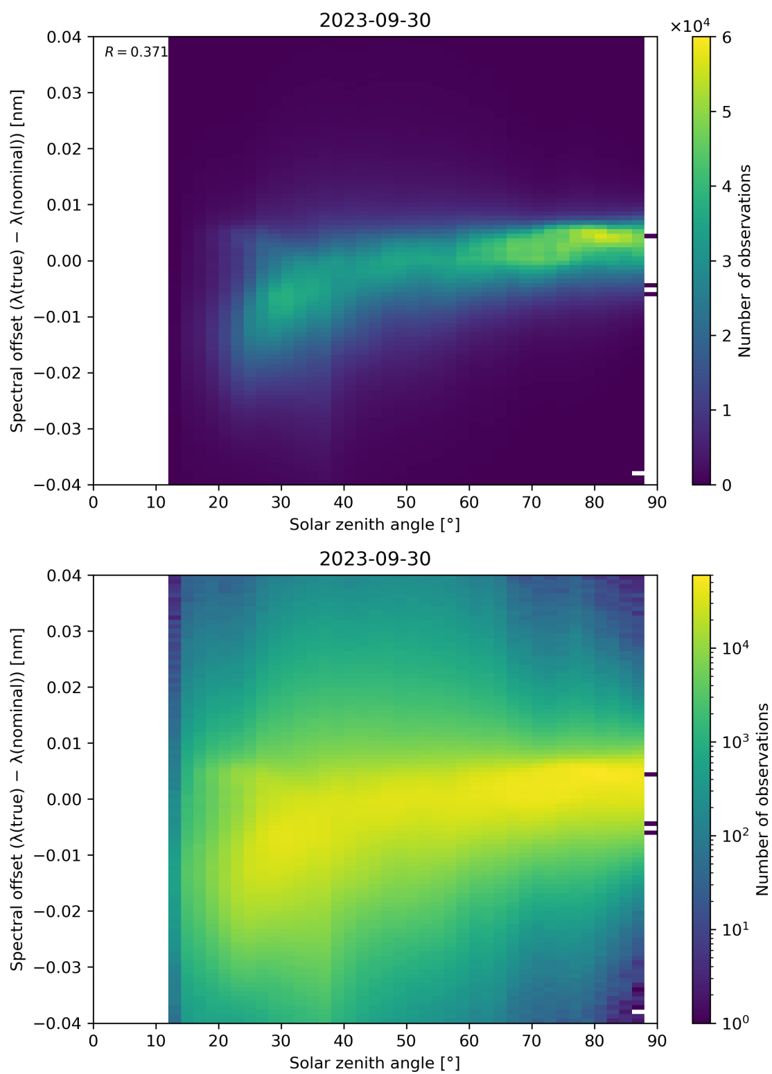
Figure 128: Scatter density plot of “Solar zenith angle” against “Spectral offset ( \lambda(\text{true}) - \lambda(\text{nominal}) )” for 2023-09-29 to 2023-10-01.
