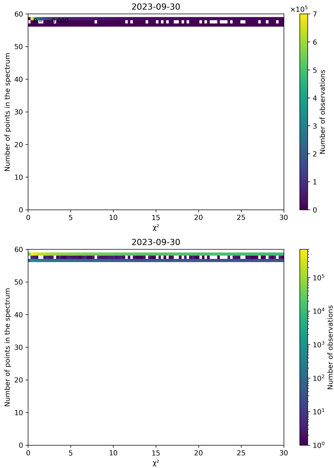
Figure 74: Scatter density plot of " \chi^2 " against "Number of points in the spectrum" for 2023-09-29 to 2023-10-01.
