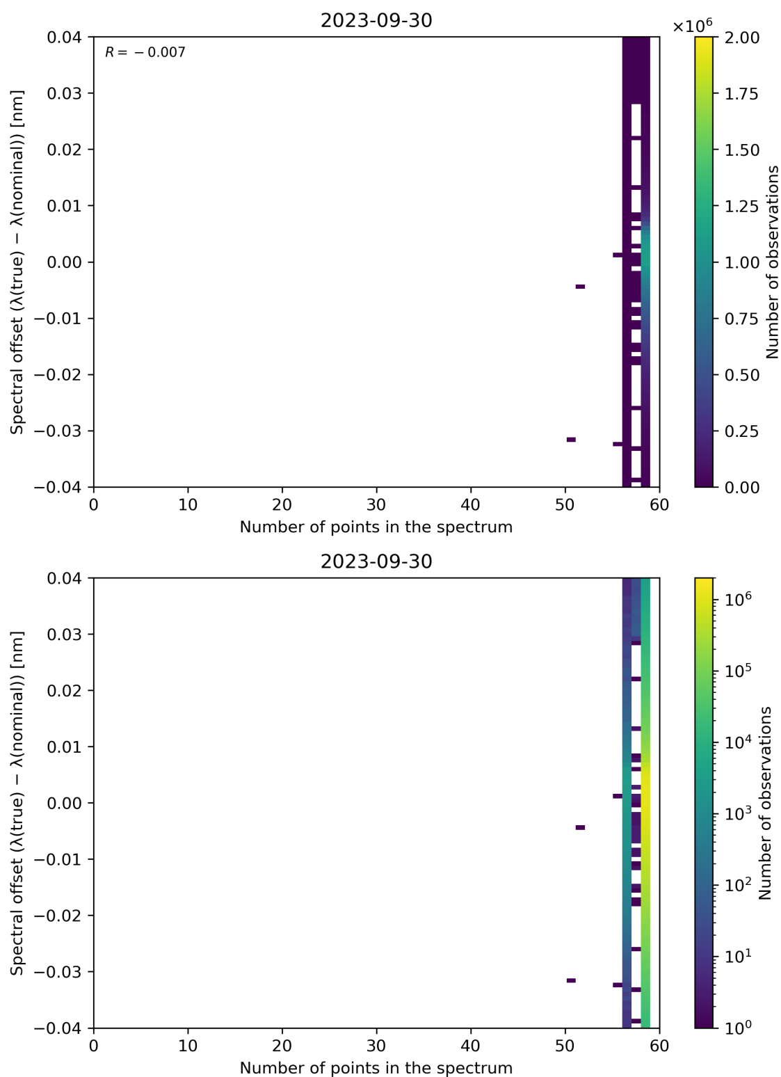
Figure 110: Scatter density plot of “Number of points in the spectrum” against “Spectral offset ( \lambda(\text{true}) - \lambda(\text{nominal}) )” for 2023-09-29 to 2023-10-01.
