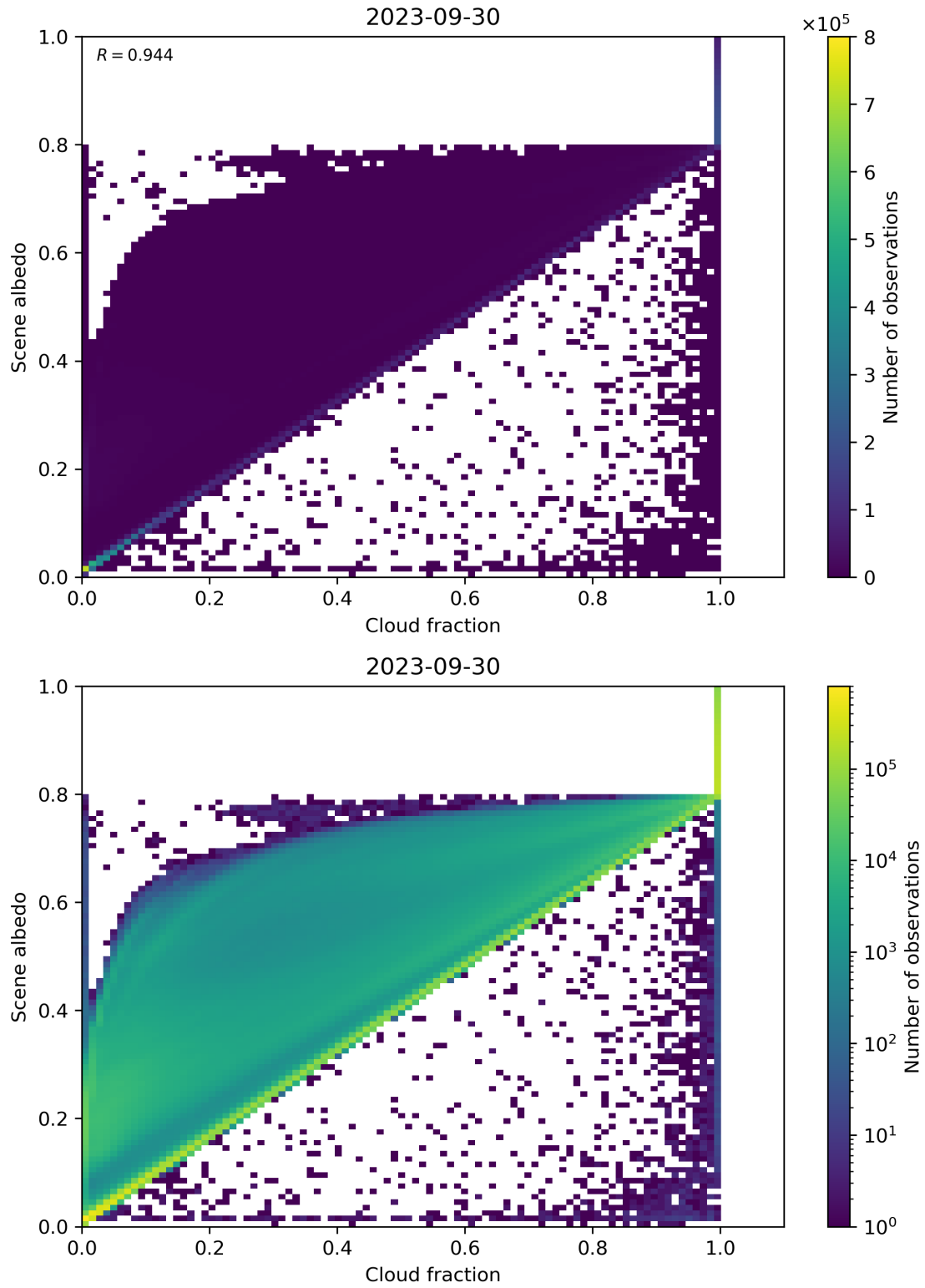
Figure 82: Scatter density plot of “Cloud fraction” against “Scene albedo” for 2023-09-29 to 2023-10-01.
