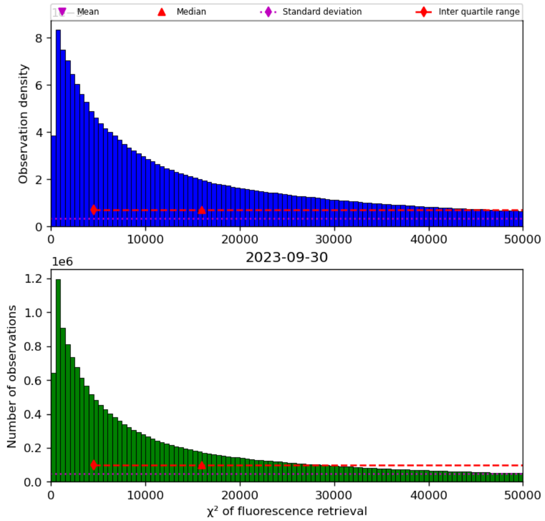
Figure 42: Histogram of “ \chi^2 of fluorescence retrieval” for 2023-09-29 to 2023-10-01
