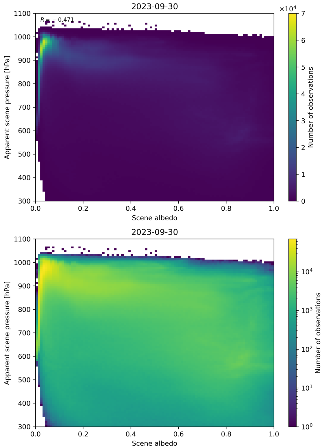
Figure 111: Scatter density plot of “Scene albedo” against “Apparent scene pressure” for 2023-09-29 to 2023-10-01.
