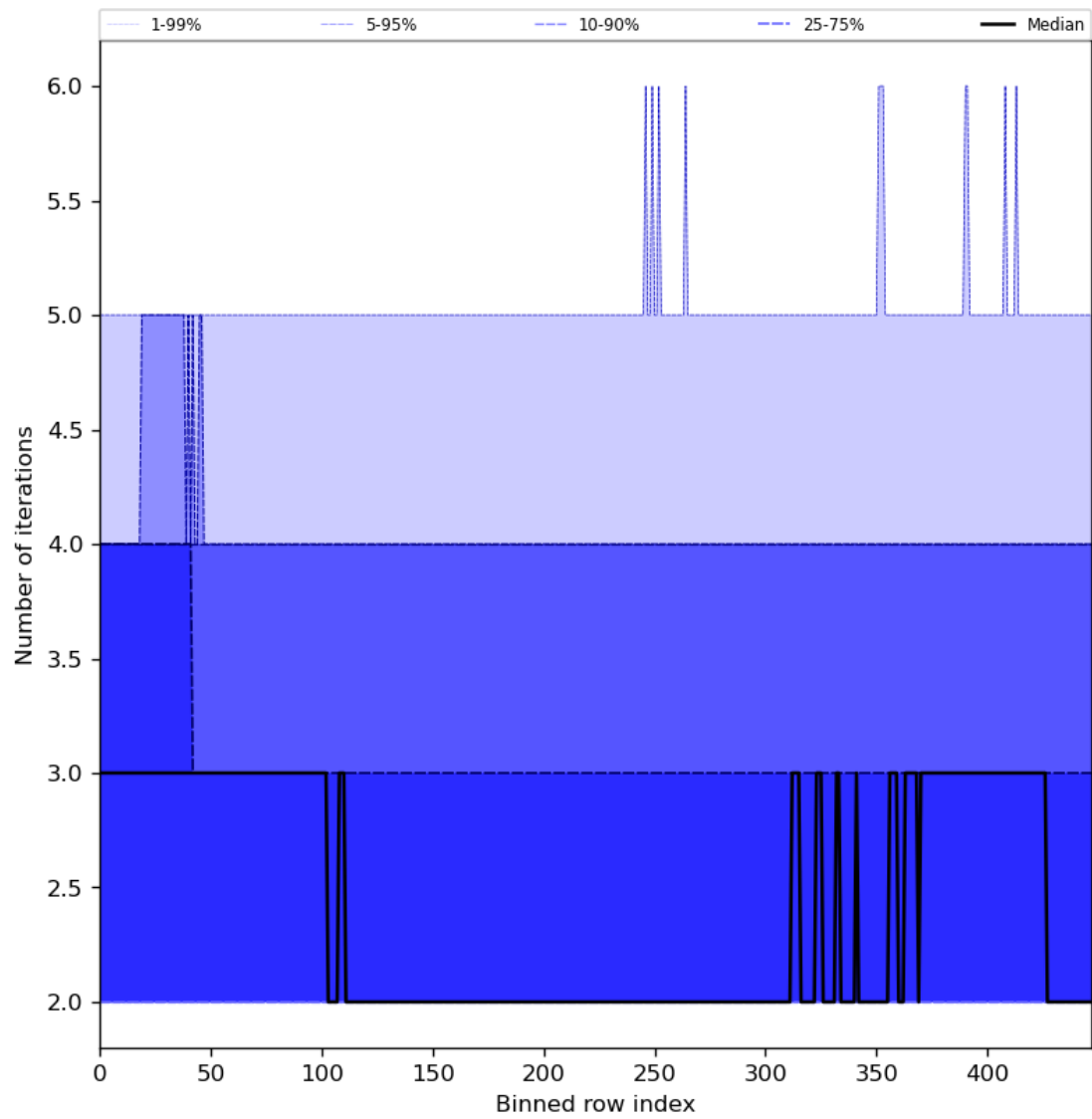
Figure 56: Along track statistics of "Number of iterations" for 2023-09-29 to 2023-10-01
