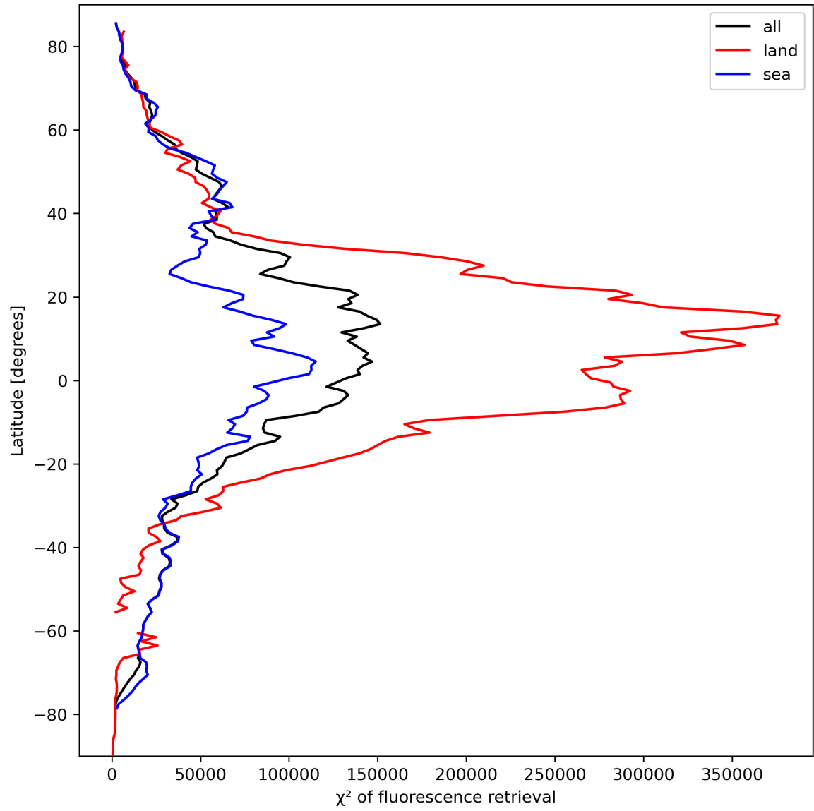
Figure 25: Zonal average of “ \chi^2 of fluorescence retrieval” for 2023-09-29 to 2023-10-01.
