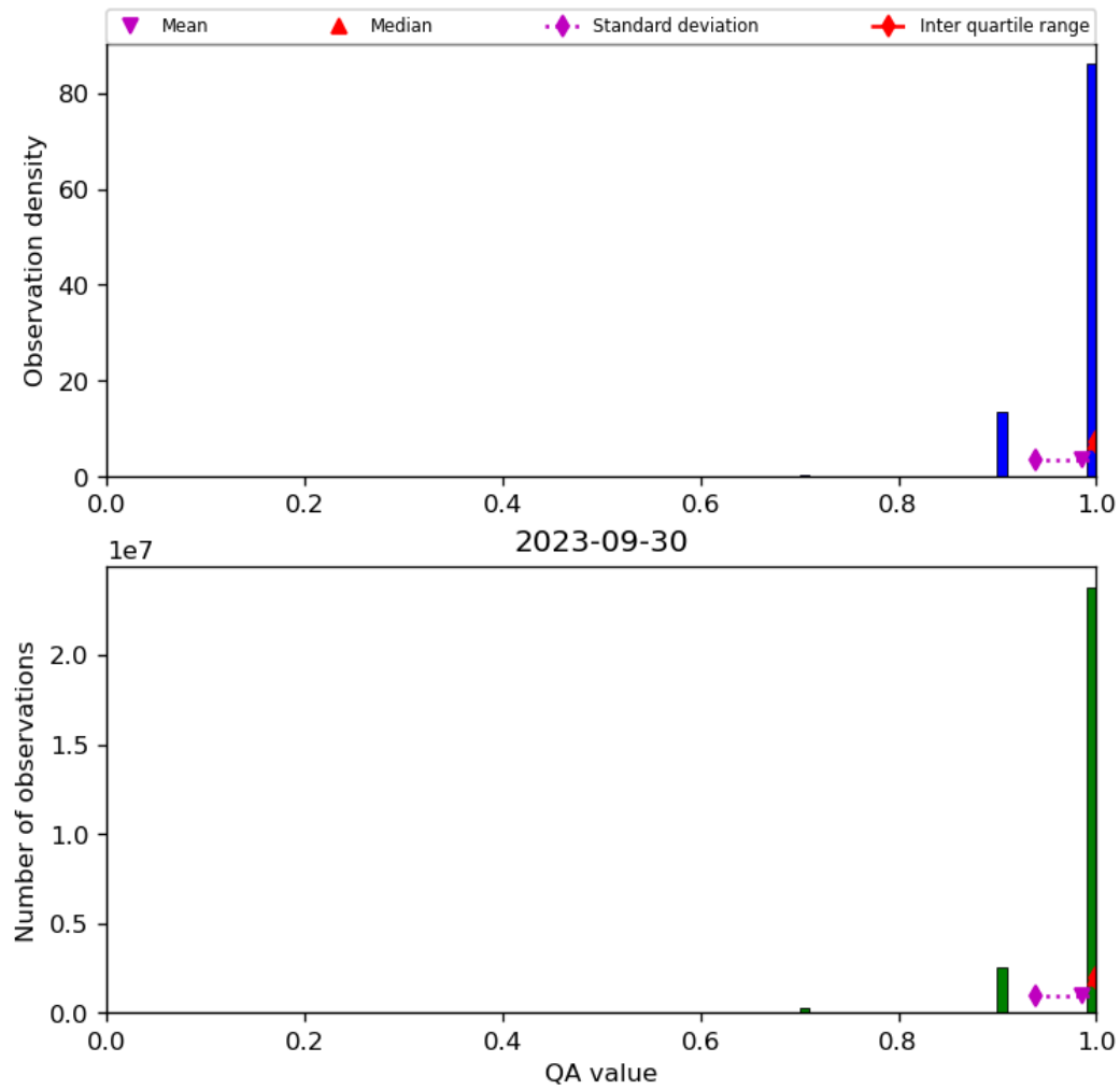
Figure 29: Histogram of “QA value” for 2023-09-29 to 2023-10-01
