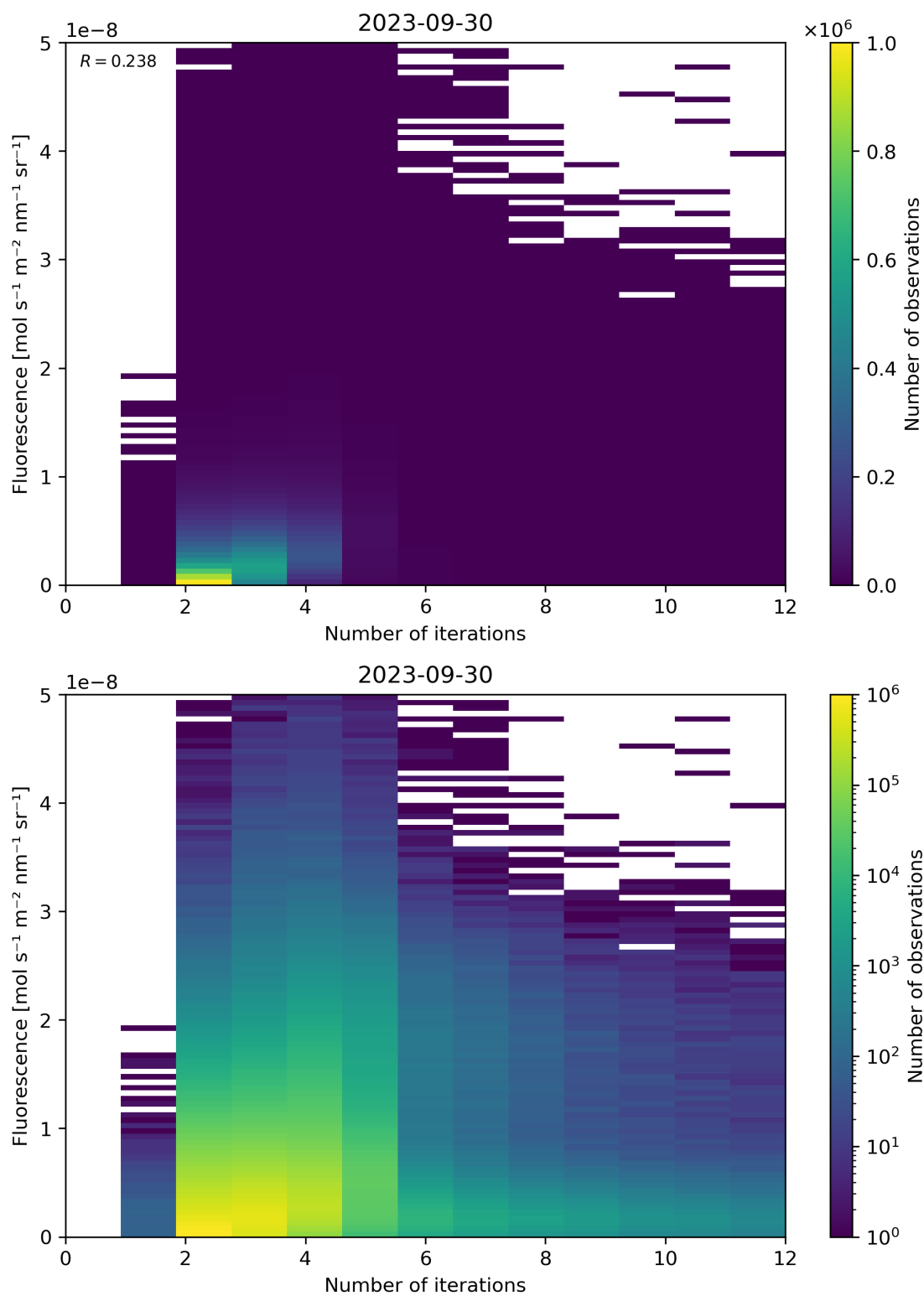
Figure 107: Scatter density plot of "Number of iterations" against "Fluorescence" for 2023-09-29 to 2023-10-01.
