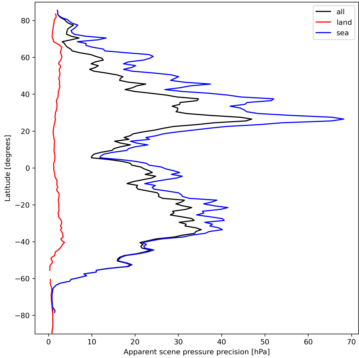
Figure 20: Zonal average of “Apparent scene pressure precision” for 2023-09-29 to 2023-10-01.
