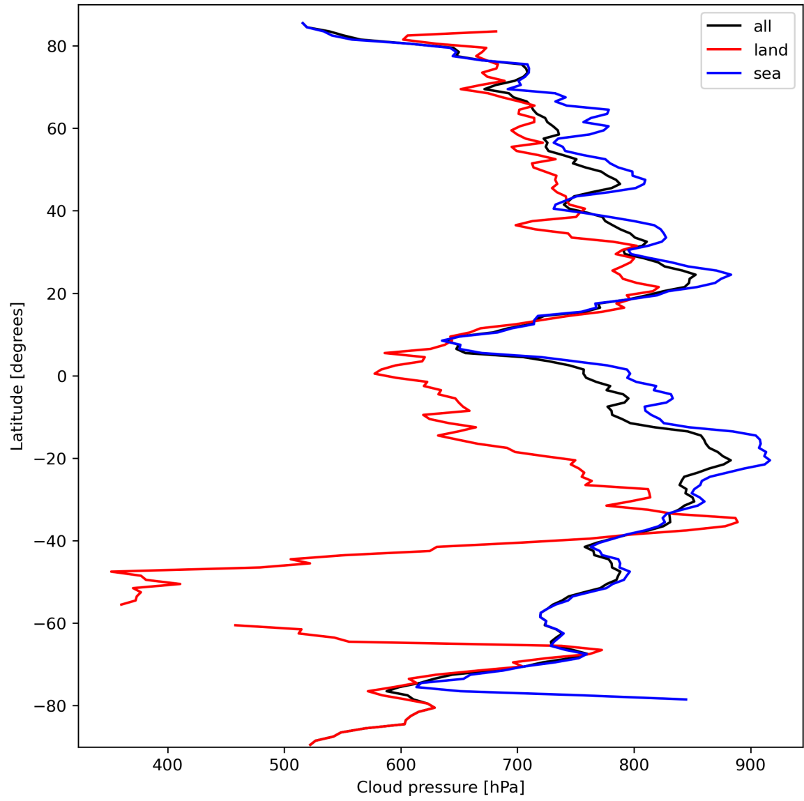
Figure 13: Zonal average of “Cloud pressure” for 2023-09-29 to 2023-10-01.
