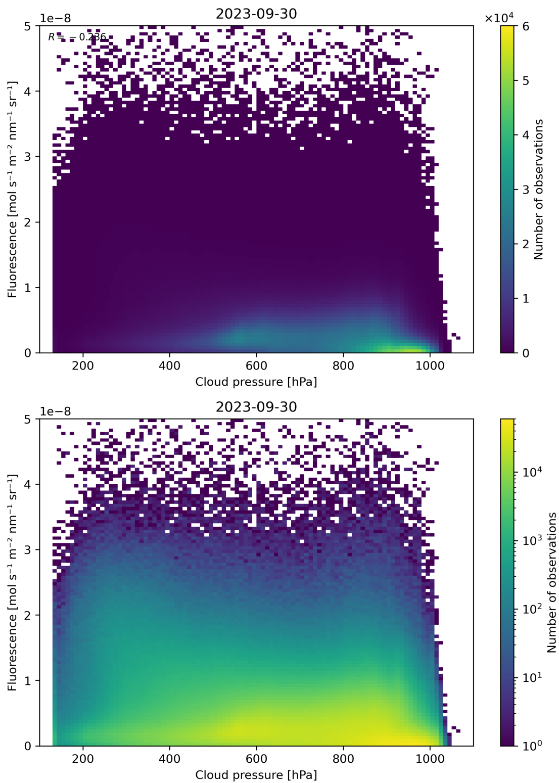
Figure 88: Scatter density plot of “Cloud pressure” against “Fluorescence” for 2023-09-29 to 2023-10-01.
