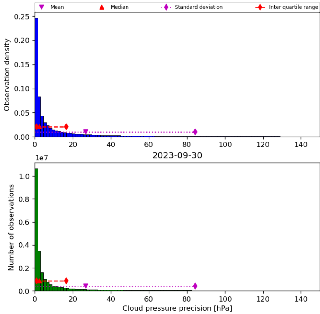
Figure 31: Histogram of “Cloud pressure precision” for 2023-09-29 to 2023-10-01
