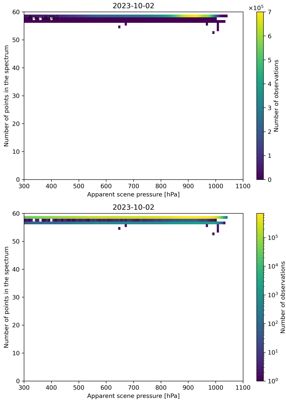
Figure 67: Scatter density plot of “Apparent scene pressure” against “Number of points in the spectrum” for 2023-10-01 to 2023-10-03.
