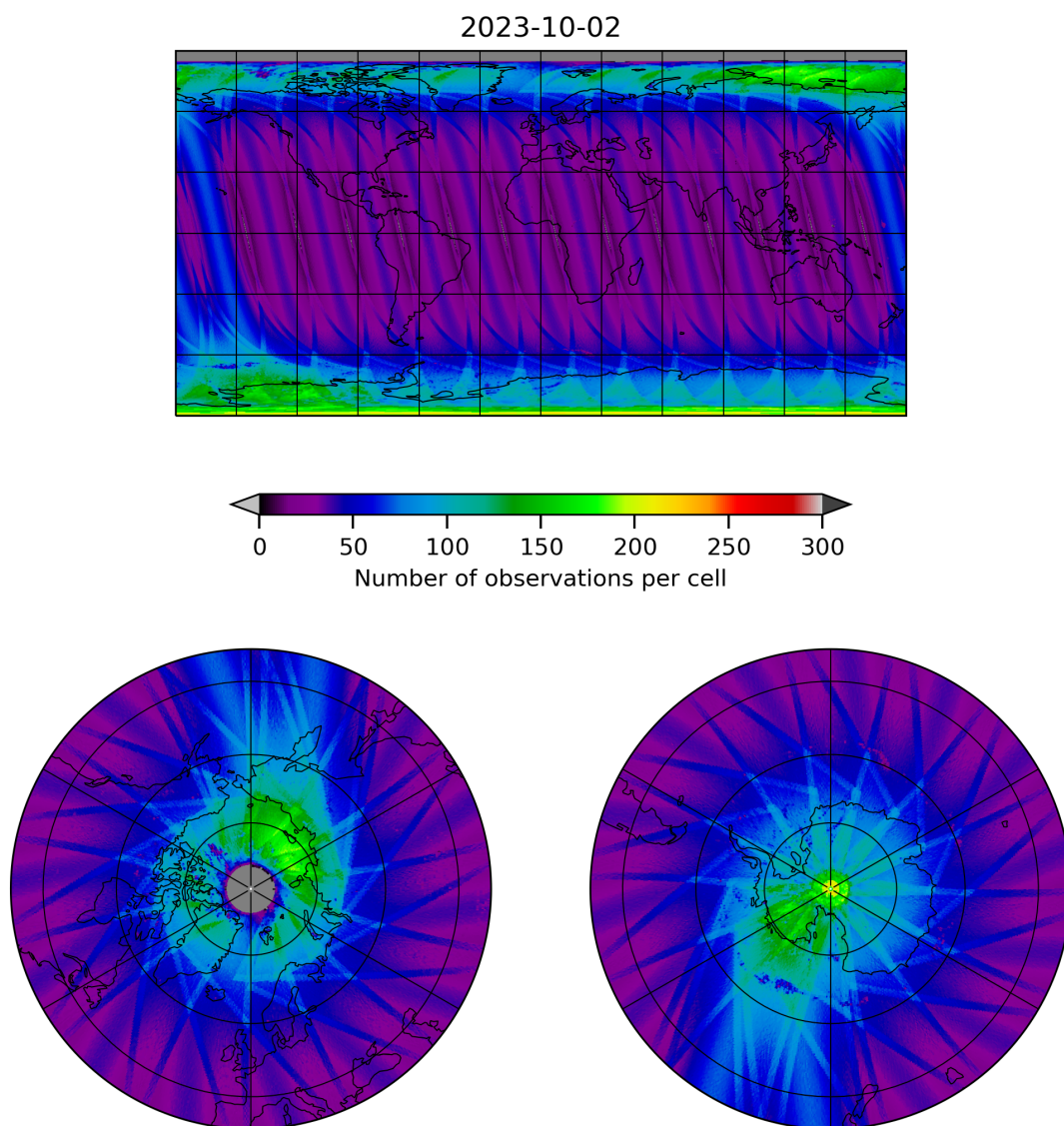
Figure 11: Map of the number of observations for 2023-10-01 to 2023-10-03
