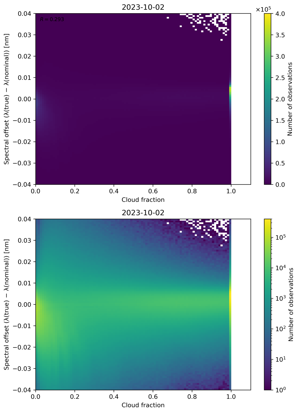
Figure 83: Scatter density plot of “Cloud fraction” against “Spectral offset ( \lambda(\text{true}) - \lambda(\text{nominal}) )” for 2023-10-01 to 2023-10-03.
