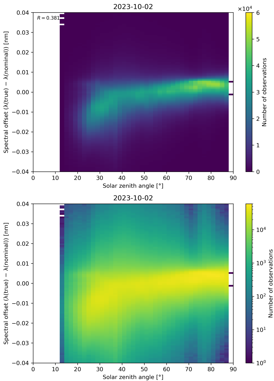
Figure 128: Scatter density plot of “Solar zenith angle” against “Spectral offset ( \lambda(\text{true}) - \lambda(\text{nominal}) )” for 2023-10-01 to 2023-10-03.
