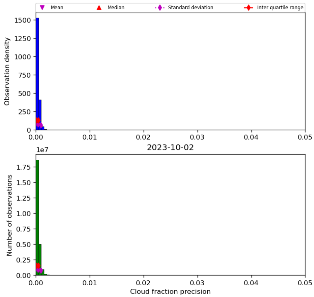
Figure 33: Histogram of “Cloud fraction precision” for 2023-10-01 to 2023-10-03
