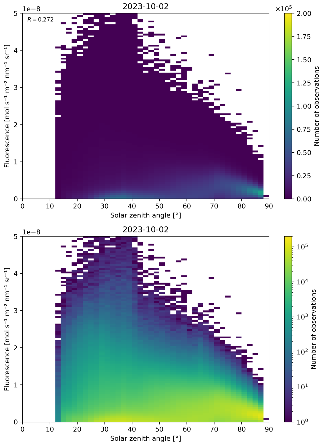
Figure 123: Scatter density plot of “Solar zenith angle” against “Fluorescence” for 2023-10-01 to 2023-10-03.
