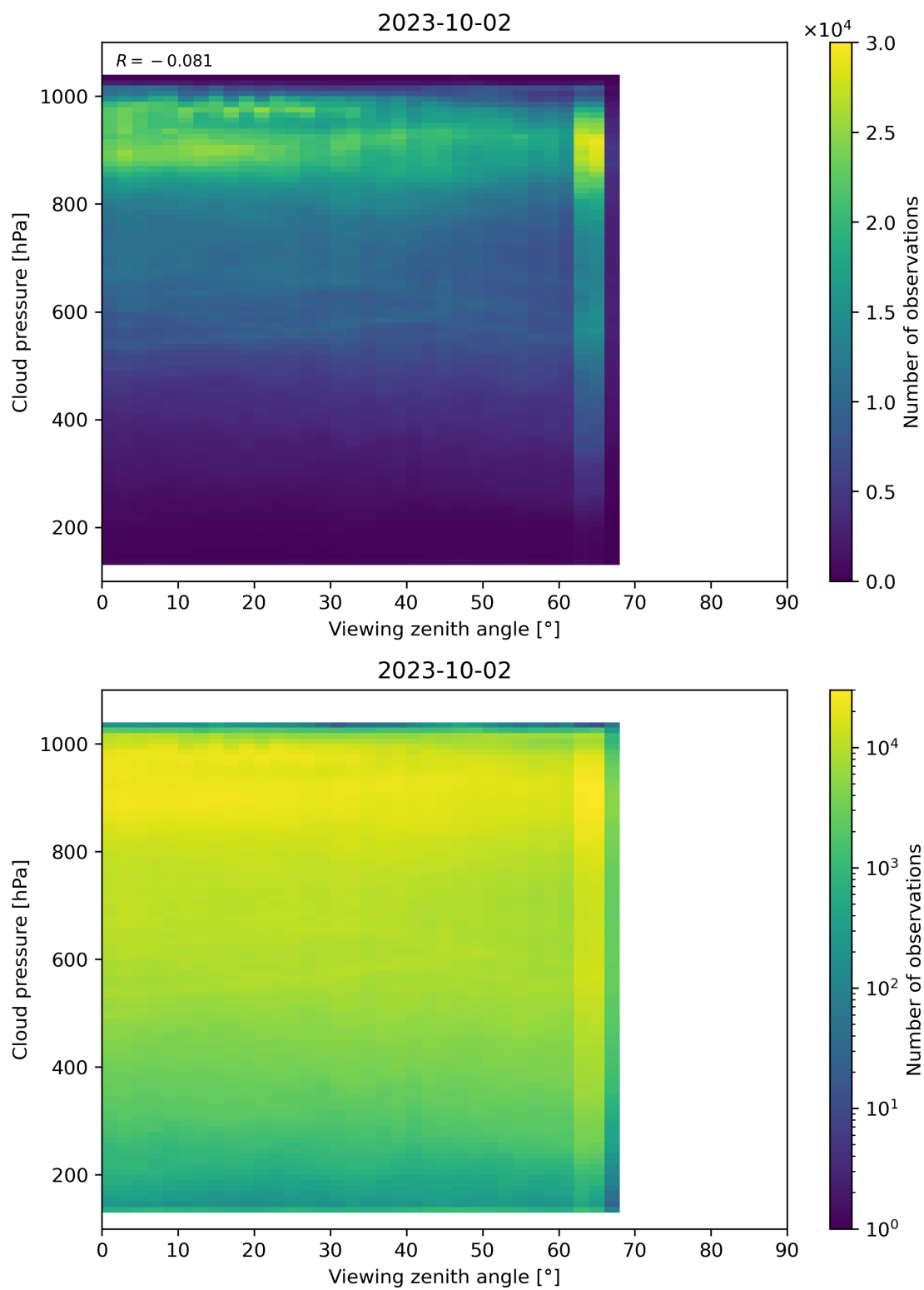
Figure 133: Scatter density plot of “Viewing zenith angle” against “Cloud pressure” for 2023-10-01 to 2023-10-03.
