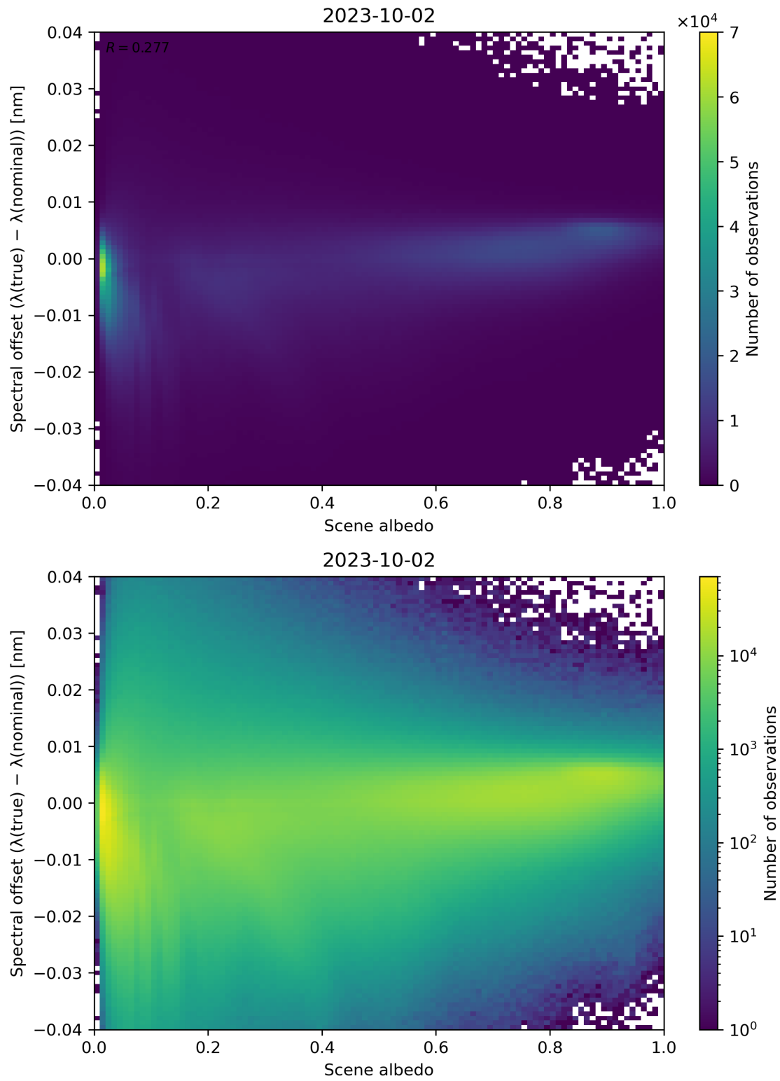
Figure 117: Scatter density plot of “Scene albedo” against “Spectral offset ( \lambda(\text{true}) - \lambda(\text{nominal}) )” for 2023-10-01 to 2023-10-03.
