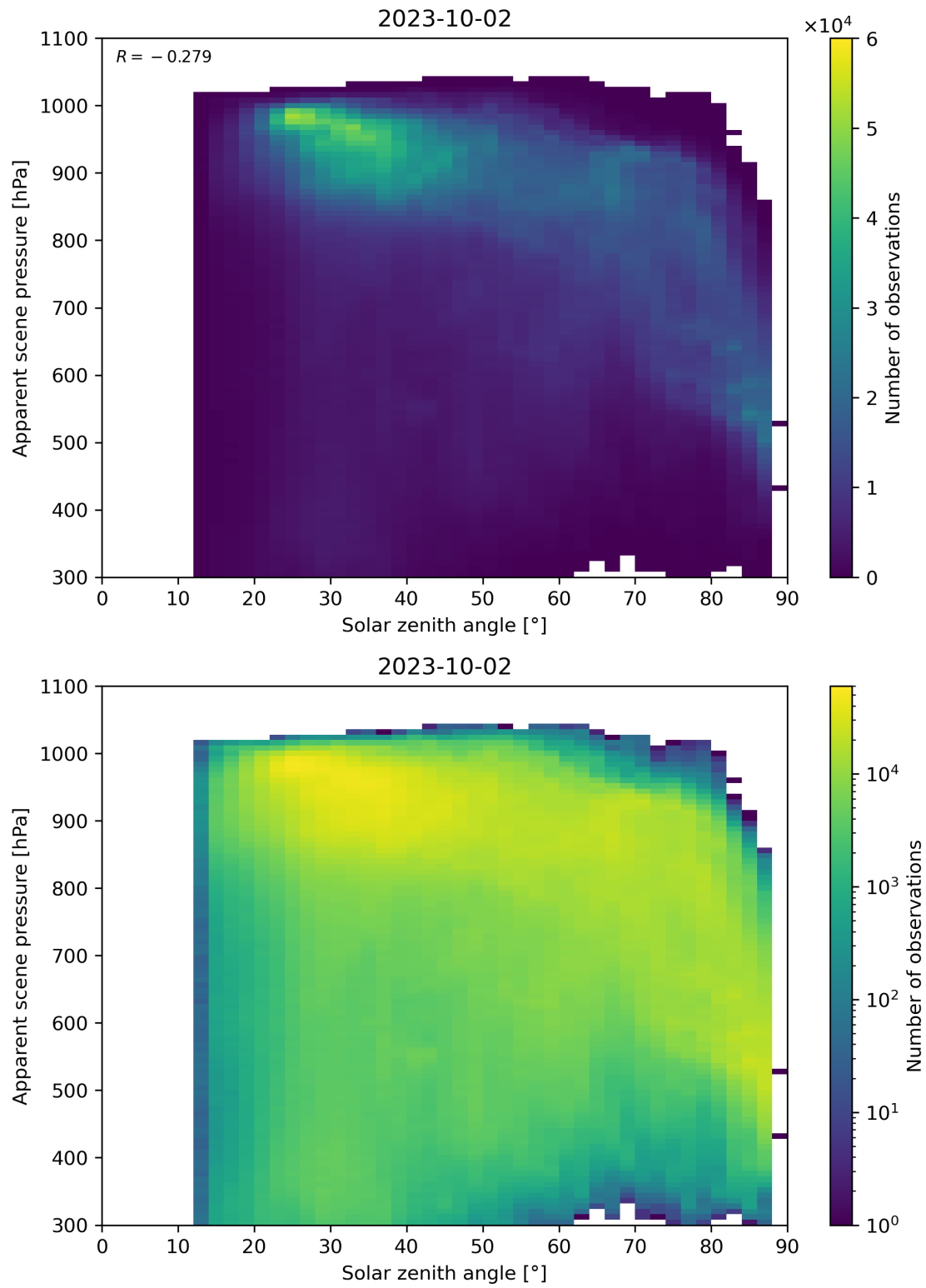
Figure 118: Scatter density plot of “Solar zenith angle” against “Apparent scene pressure” for 2023-10-01 to 2023-10-03.
