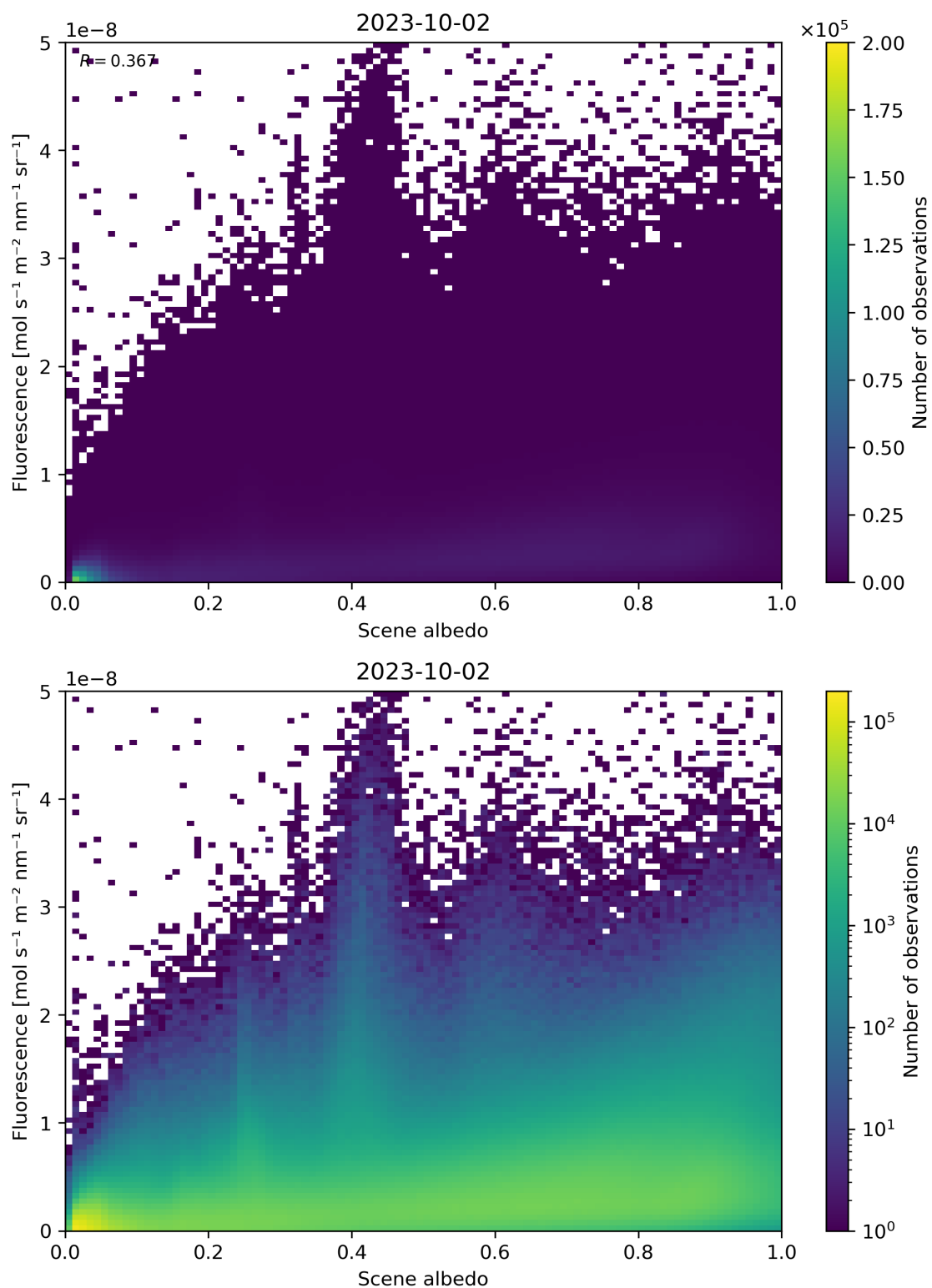
Figure 114: Scatter density plot of “Scene albedo” against “Fluorescence” for 2023-10-01 to 2023-10-03.
