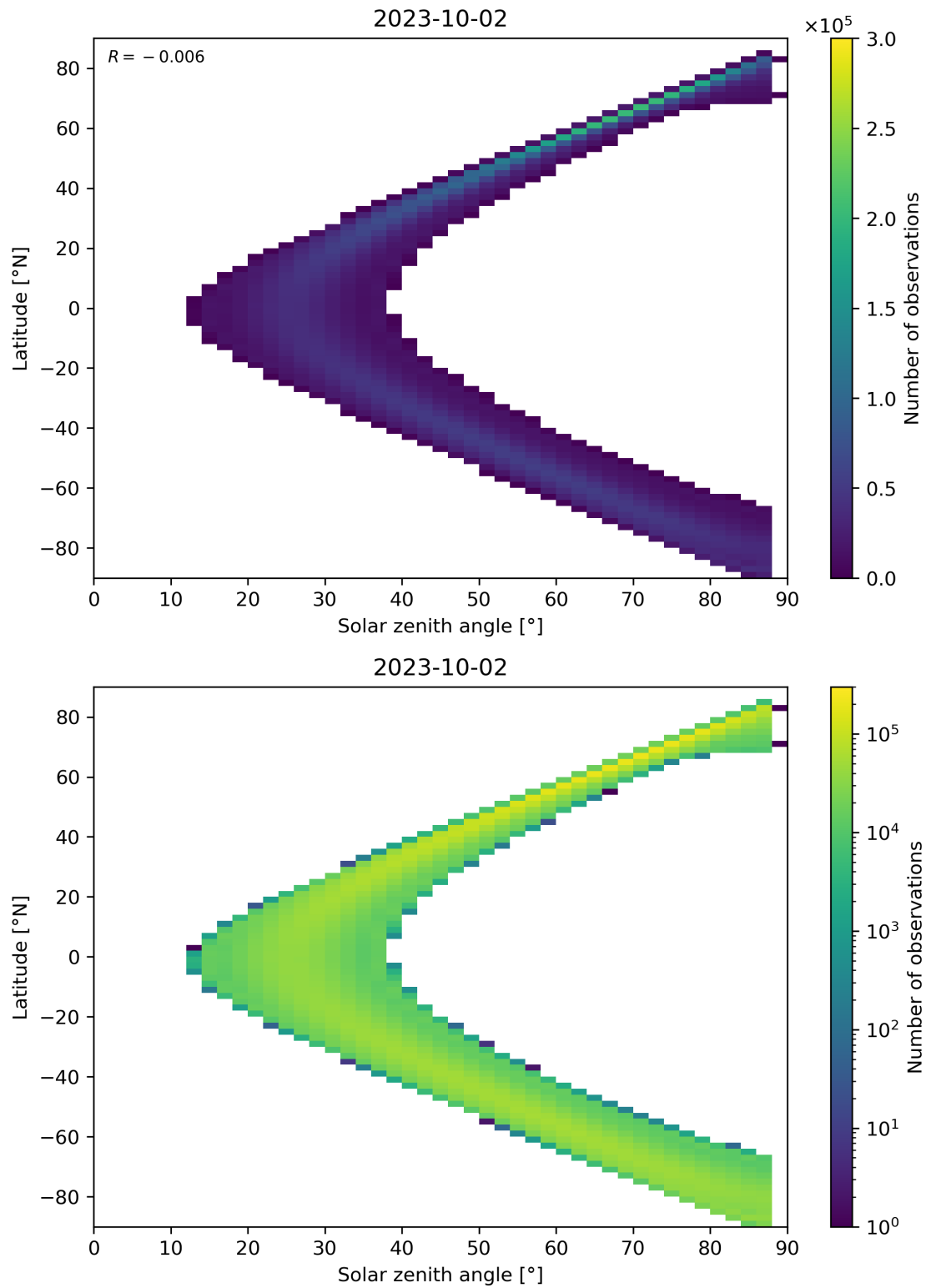
Figure 124: Scatter density plot of “Solar zenith angle” against “Latitude” for 2023-10-01 to 2023-10-03.
