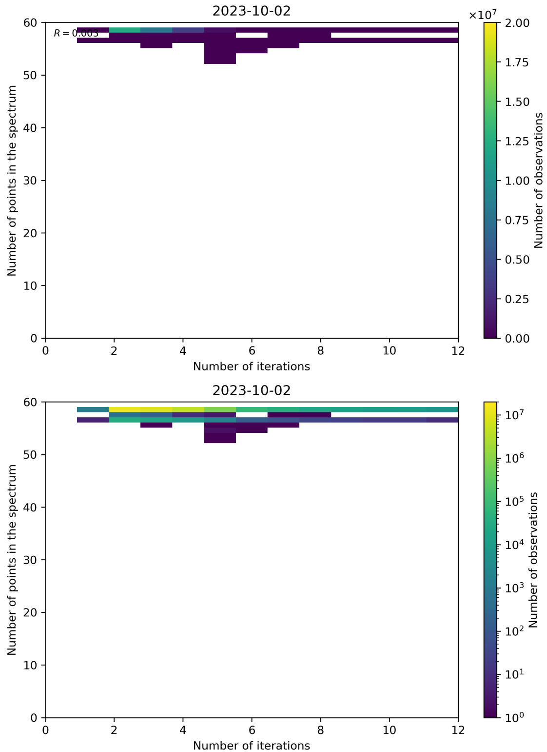
Figure 108: Scatter density plot of “Number of iterations” against “Number of points in the spectrum” for 2023-10-01 to 2023-10-03.
