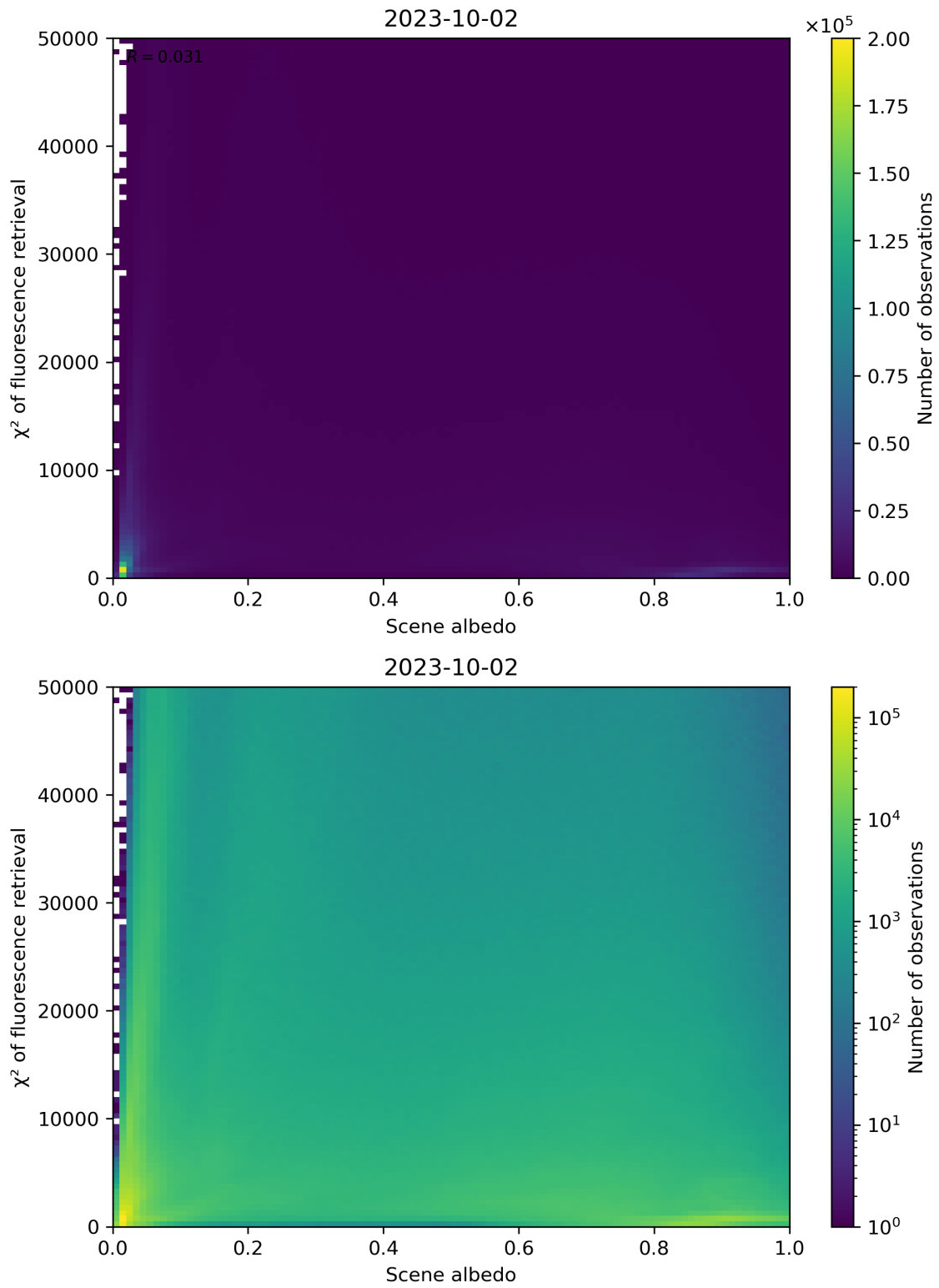
Figure 113: Scatter density plot of “Scene albedo” against “ \chi^2 of fluorescence retrieval” for 2023-10-01 to 2023-10-03.
