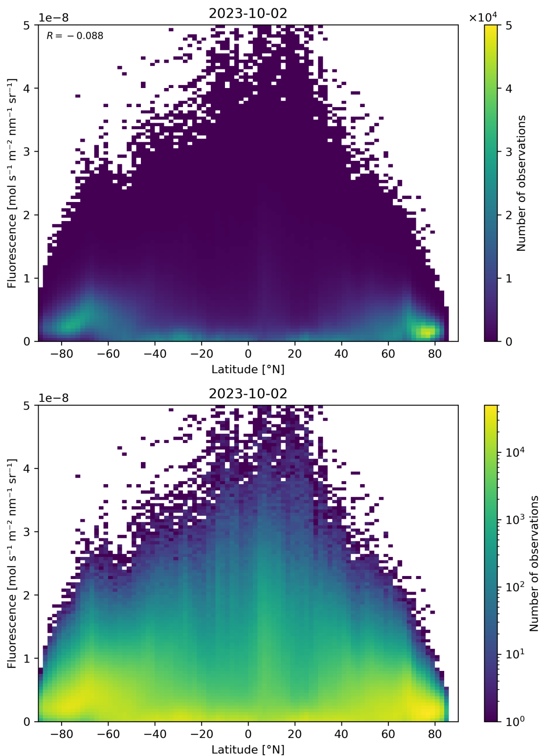
Figure 101: Scatter density plot of “Latitude” against “Fluorescence” for 2023-10-01 to 2023-10-03.
