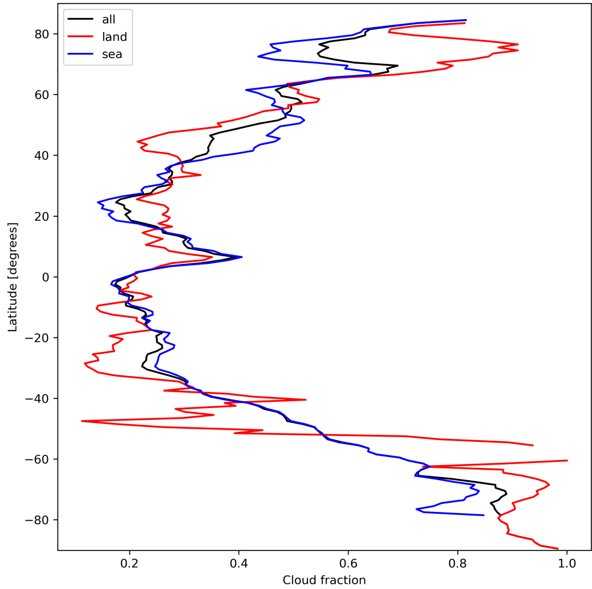
Figure 15: Zonal average of “Cloud fraction” for 2023-10-01 to 2023-10-03.
