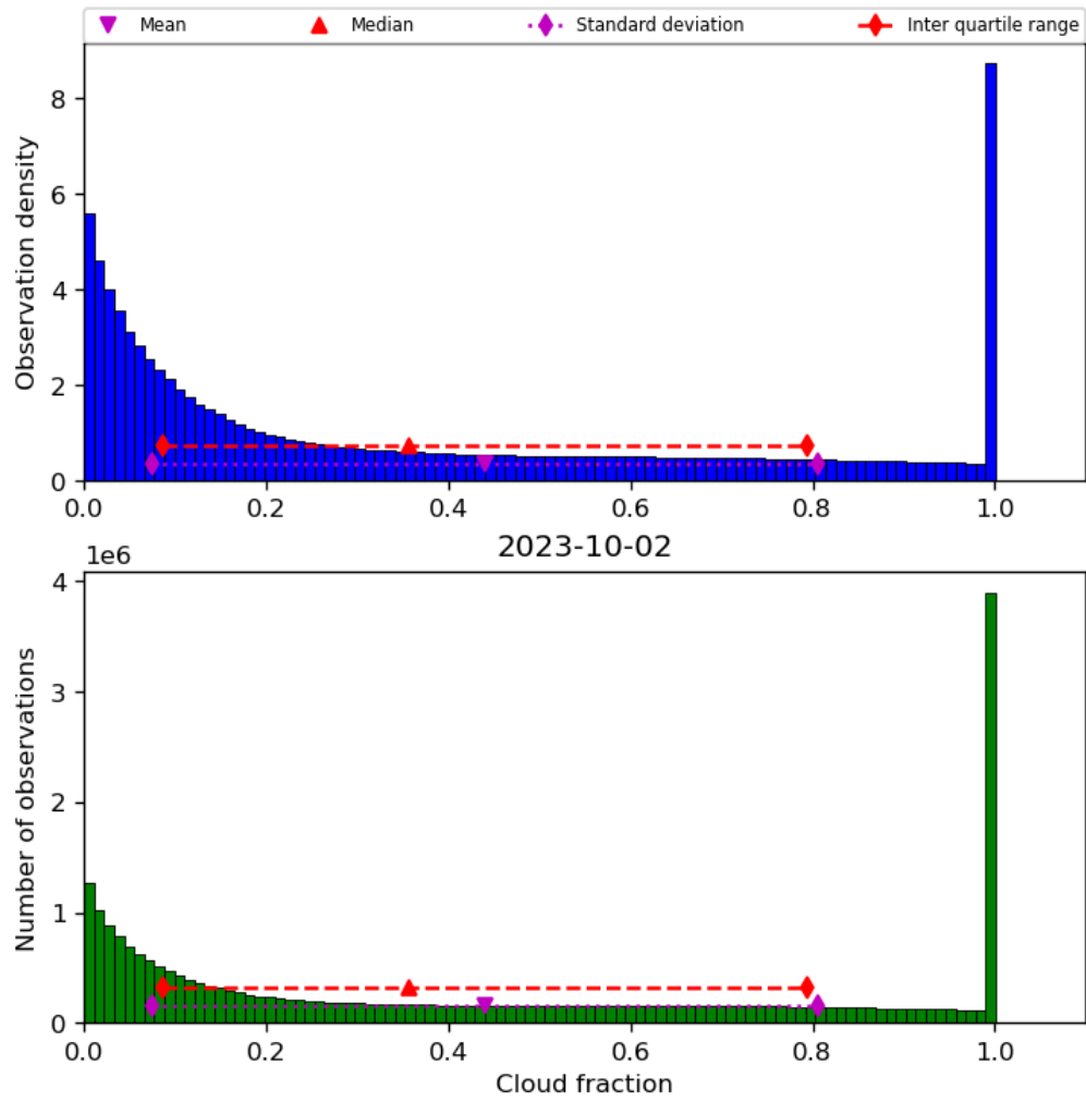
Figure 32: Histogram of “Cloud fraction” for 2023-10-01 to 2023-10-03
