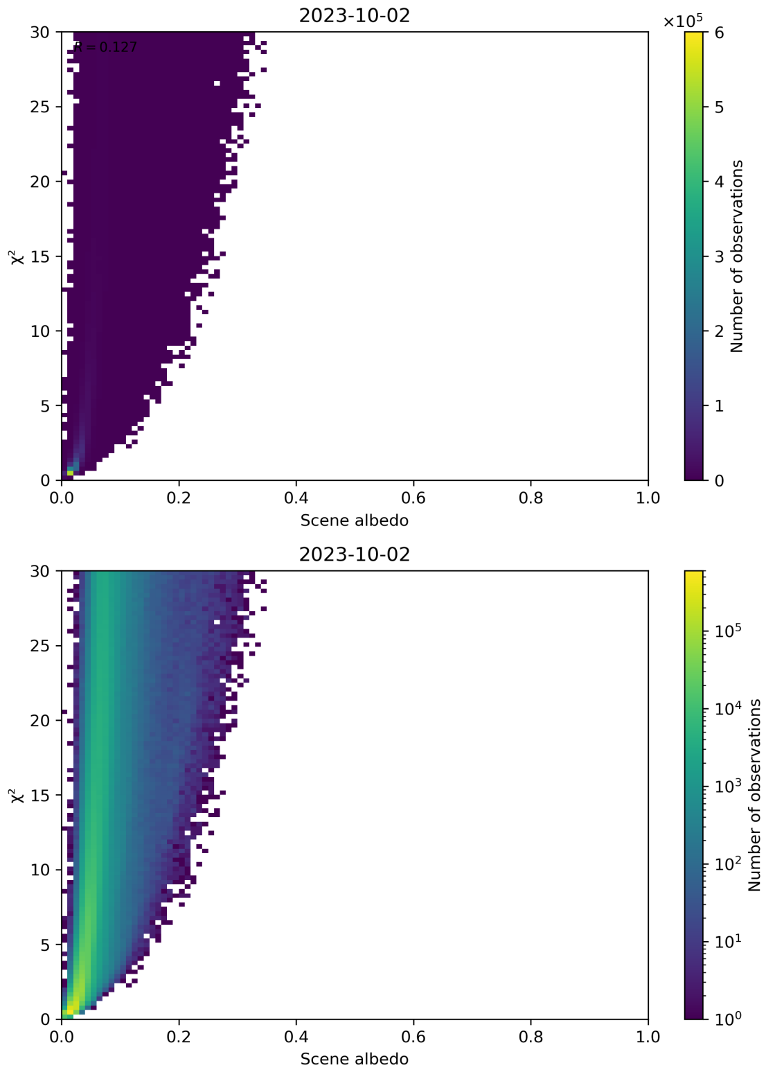
Figure 112: Scatter density plot of “Scene albedo” against “ \chi^2 ” for 2023-10-01 to 2023-10-03.
