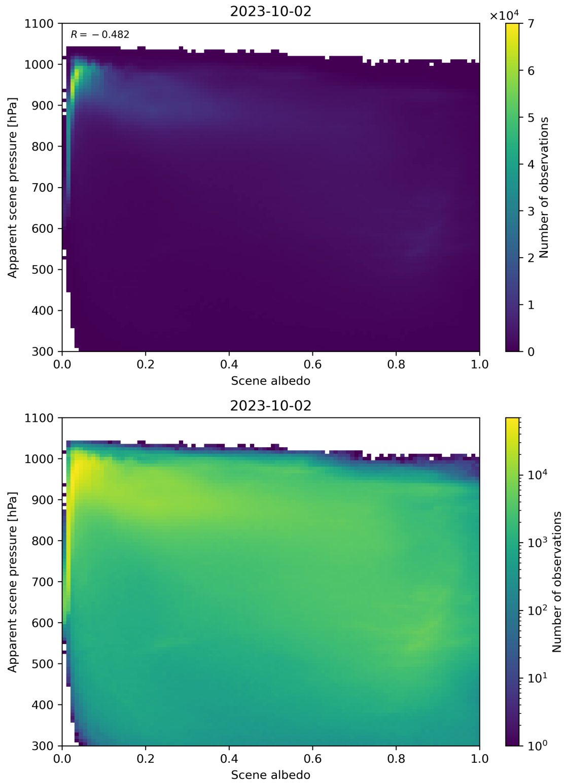
Figure 111: Scatter density plot of “Scene albedo” against “Apparent scene pressure” for 2023-10-01 to 2023-10-03.
