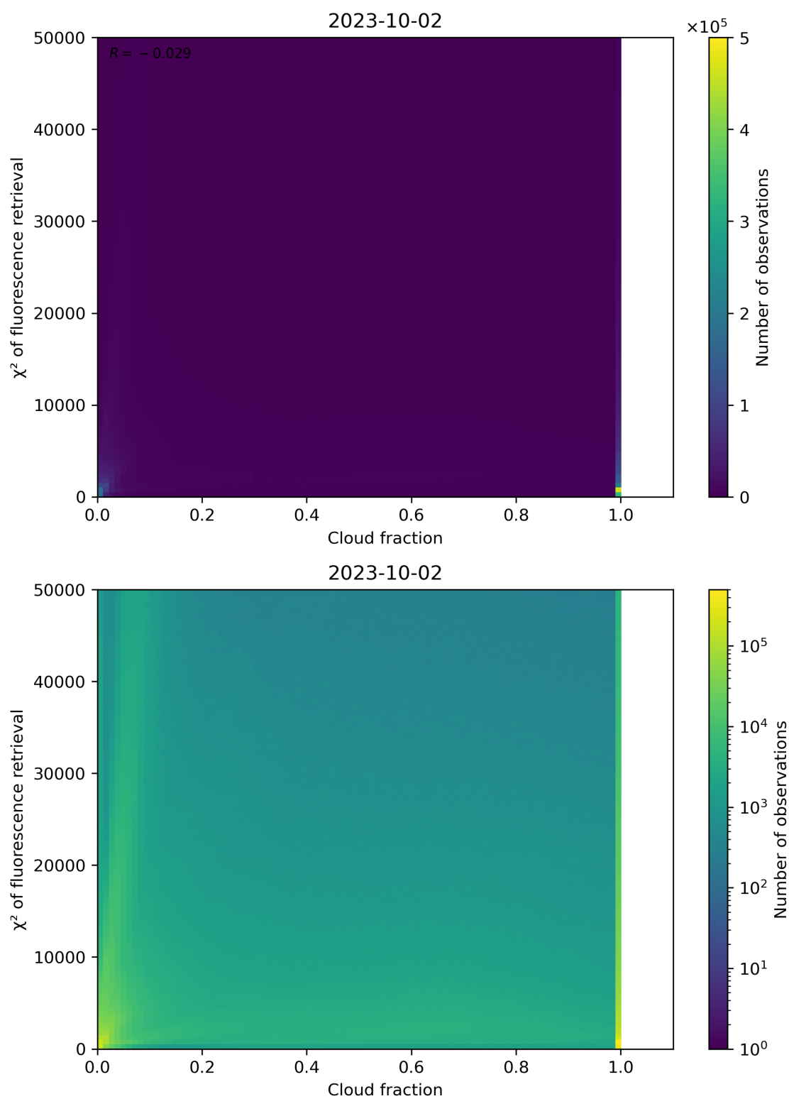
Figure 78: Scatter density plot of “Cloud fraction” against “ \chi^2 of fluorescence retrieval” for 2023-10-01 to 2023-10-03.
