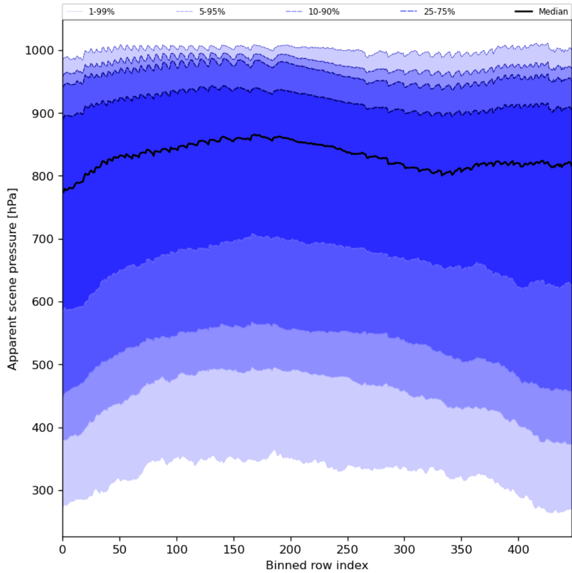
Figure 53: Along track statistics of “Apparent scene pressure” for 2023-10-01 to 2023-10-03
