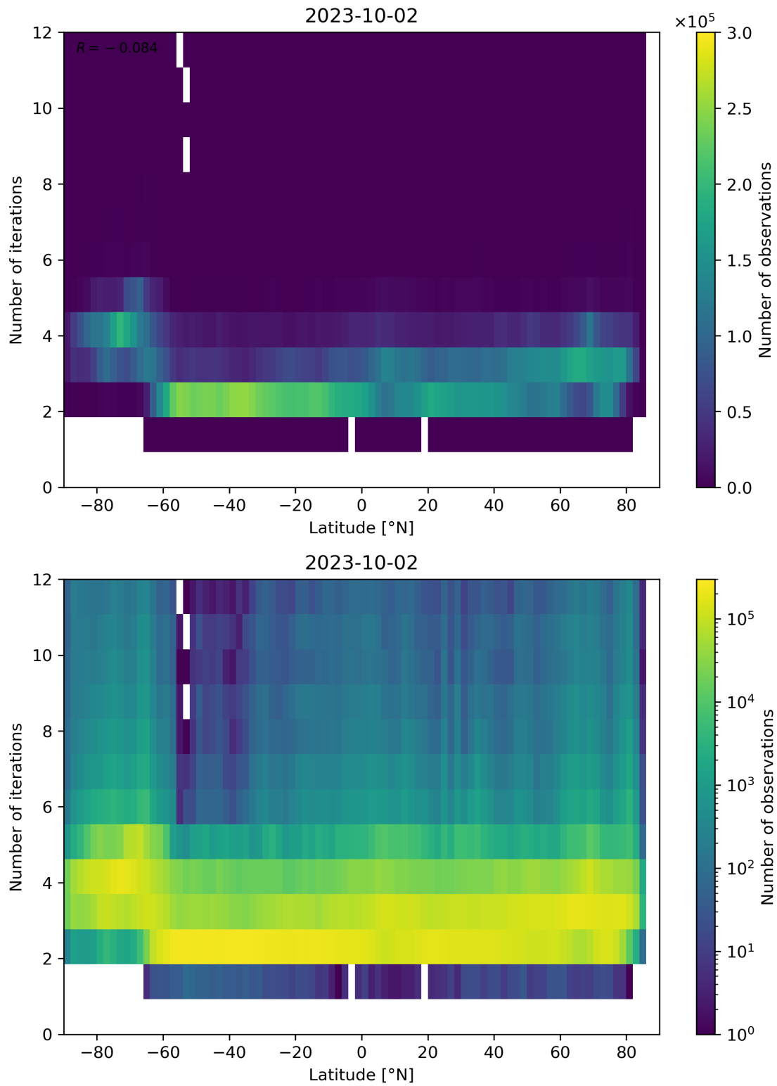
Figure 102: Scatter density plot of “Latitude” against “Number of iterations” for 2023-10-01 to 2023-10-03.
