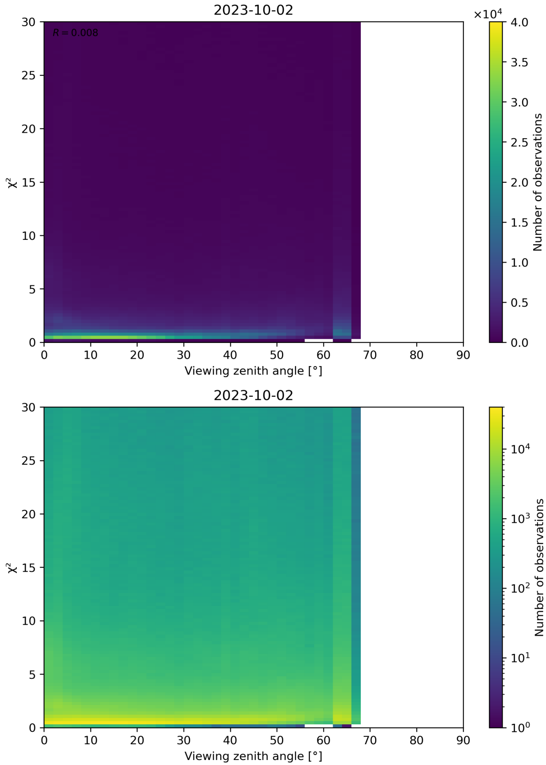
Figure 130: Scatter density plot of “Viewing zenith angle” against “ \chi^2 ” for 2023-10-01 to 2023-10-03.
