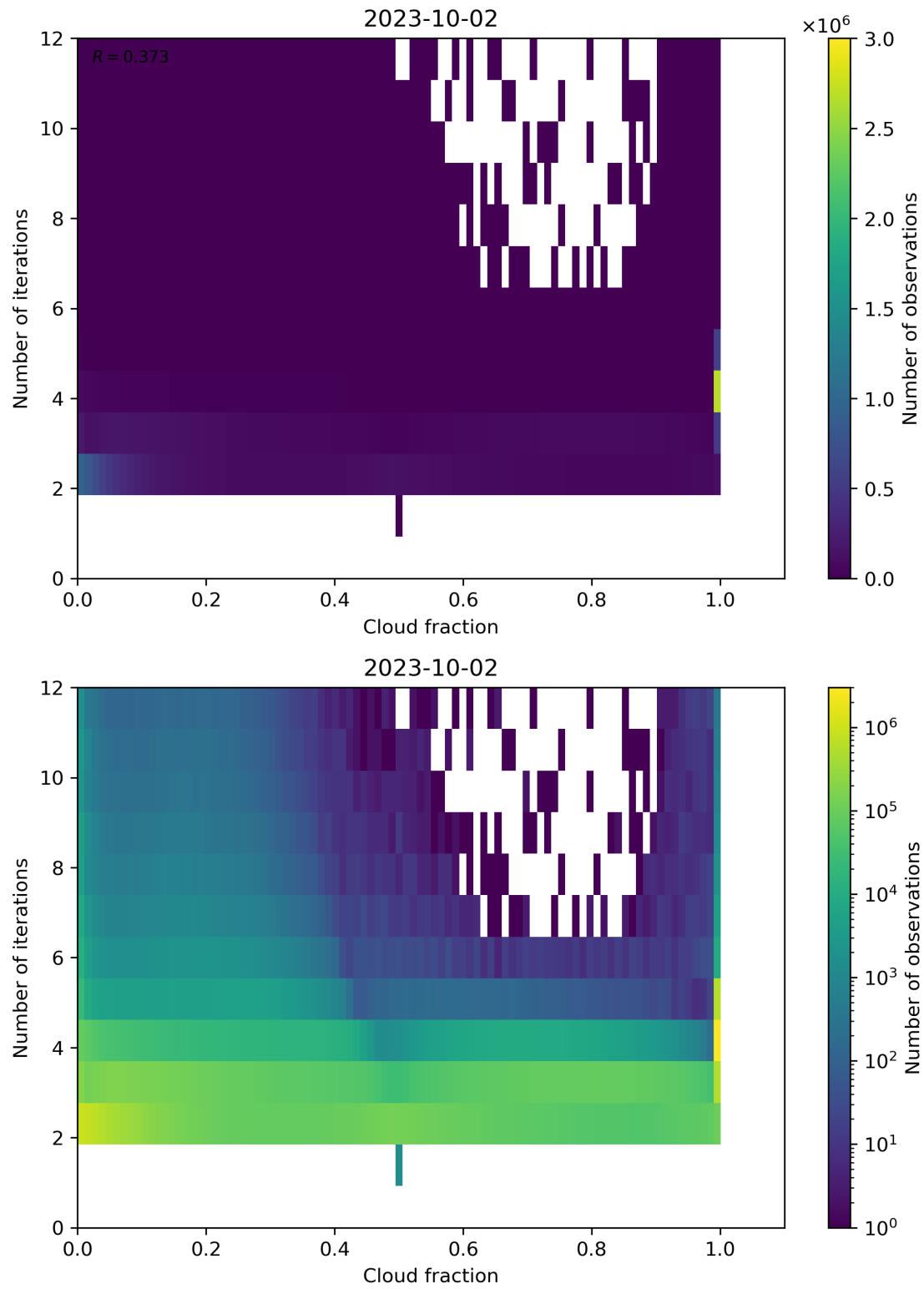
Figure 80: Scatter density plot of “Cloud fraction” against “Number of iterations” for 2023-10-01 to 2023-10-03.
