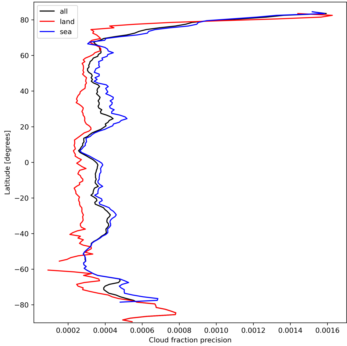
Figure 16: Zonal average of “Cloud fraction precision” for 2023-10-01 to 2023-10-03.
