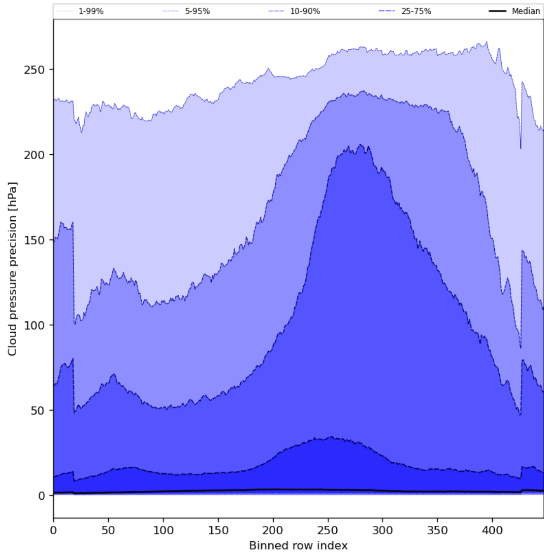
Figure 48: Along track statistics of “Cloud pressure precision” for 2023-10-01 to 2023-10-03
