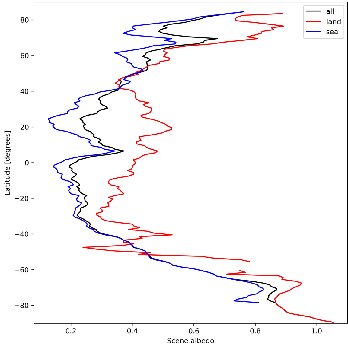
Figure 17: Zonal average of “Scene albedo” for 2023-10-01 to 2023-10-03.
