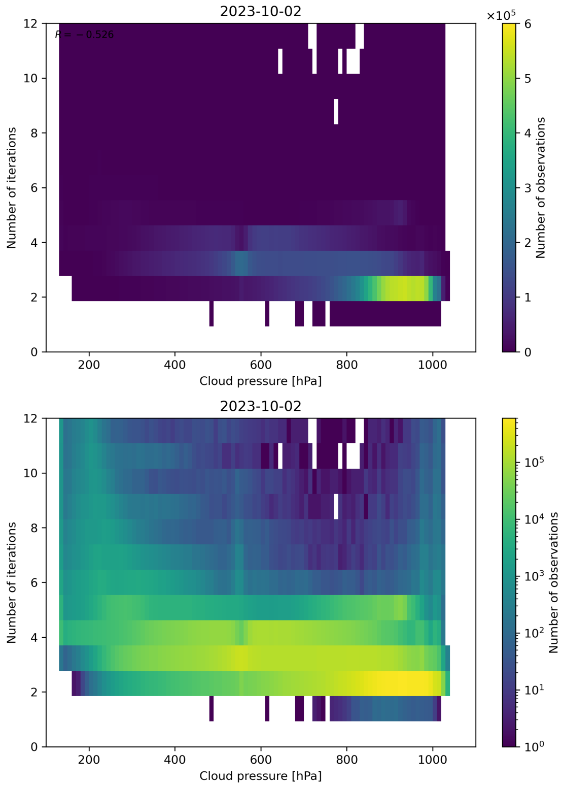
Figure 89: Scatter density plot of “Cloud pressure” against “Number of iterations” for 2023-10-01 to 2023-10-03.
