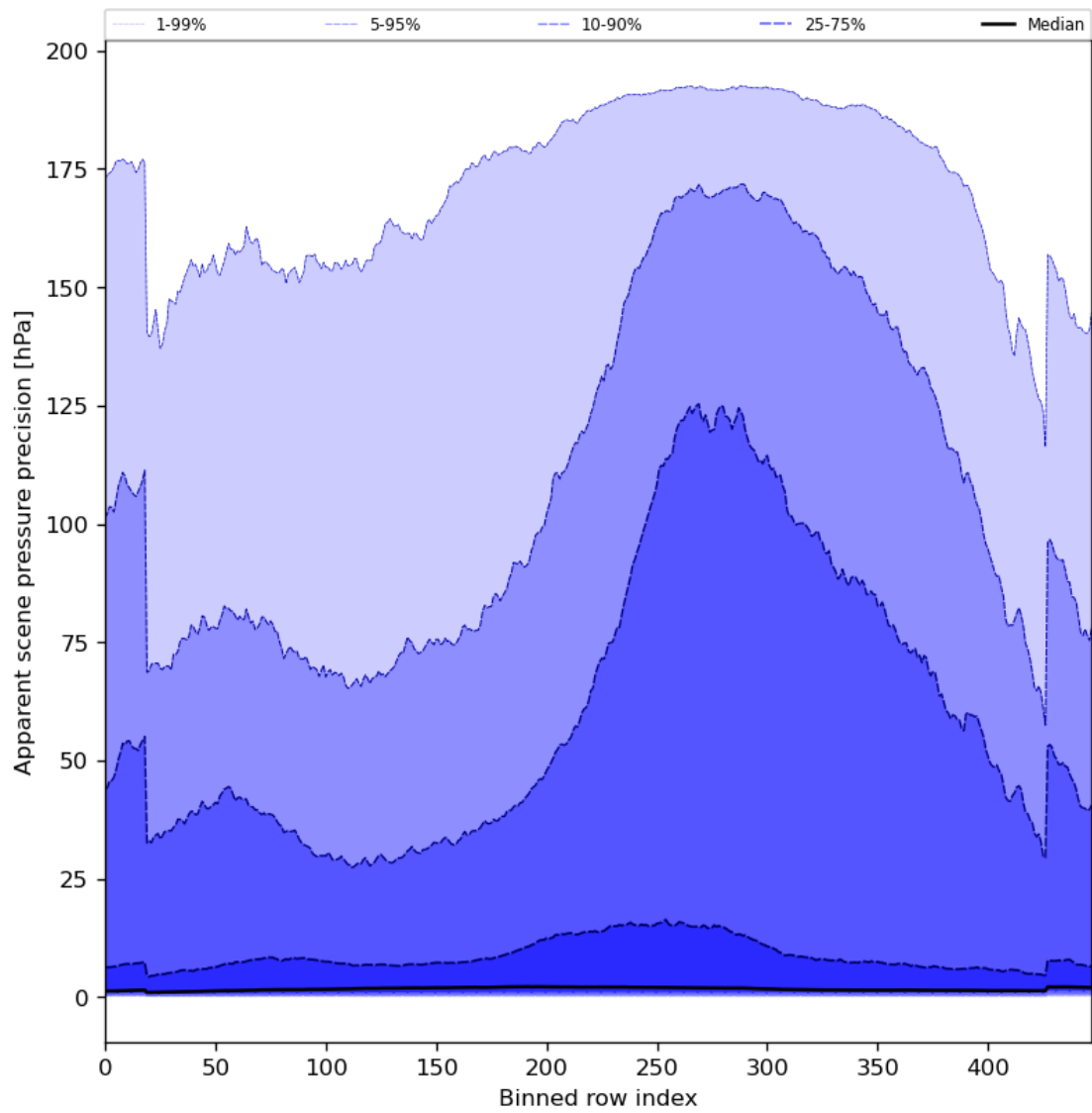
Figure 54: Along track statistics of “Apparent scene pressure precision” for 2023-10-01 to 2023-10-03
