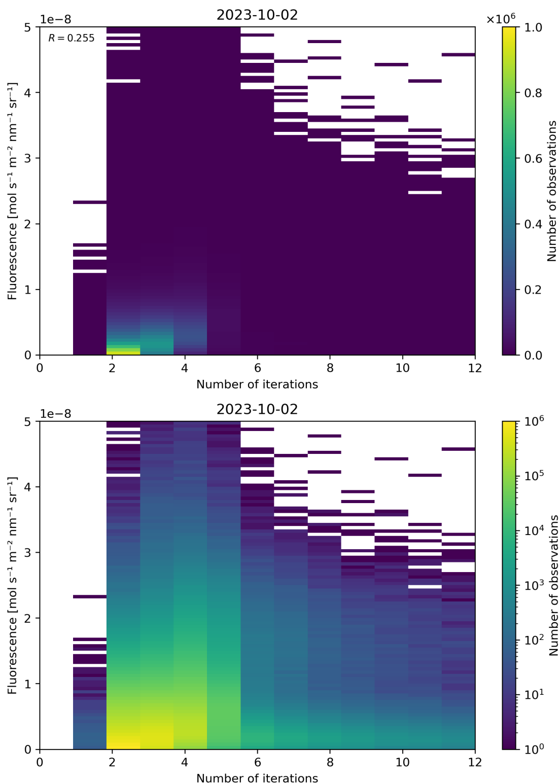
Figure 107: Scatter density plot of "Number of iterations" against "Fluorescence" for 2023-10-01 to 2023-10-03.
