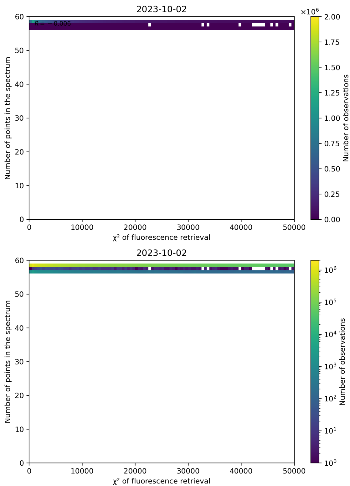
Figure 71: Scatter density plot of " \chi^2 of fluorescence retrieval" against "Number of points in the spectrum" for 2023-10-01 to 2023-10-03.
