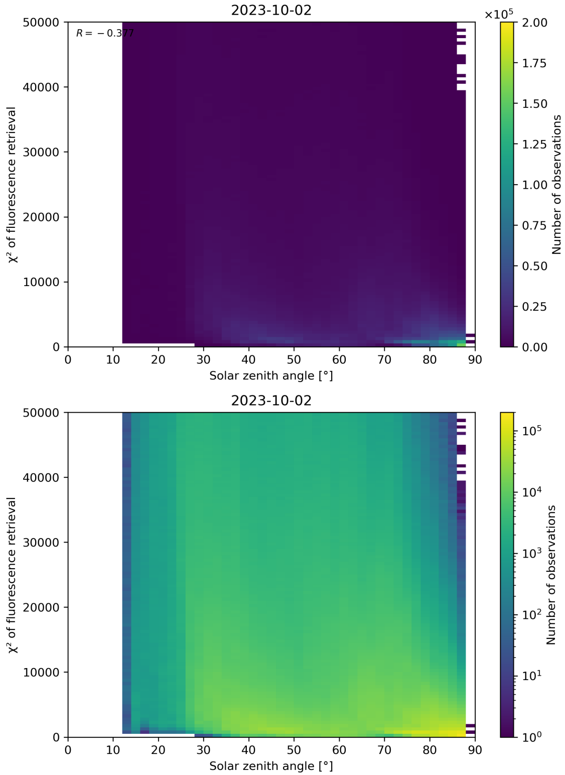
Figure 120: Scatter density plot of “Solar zenith angle” against “ \chi^2 of fluorescence retrieval” for 2023-10-01 to 2023-10-03.
