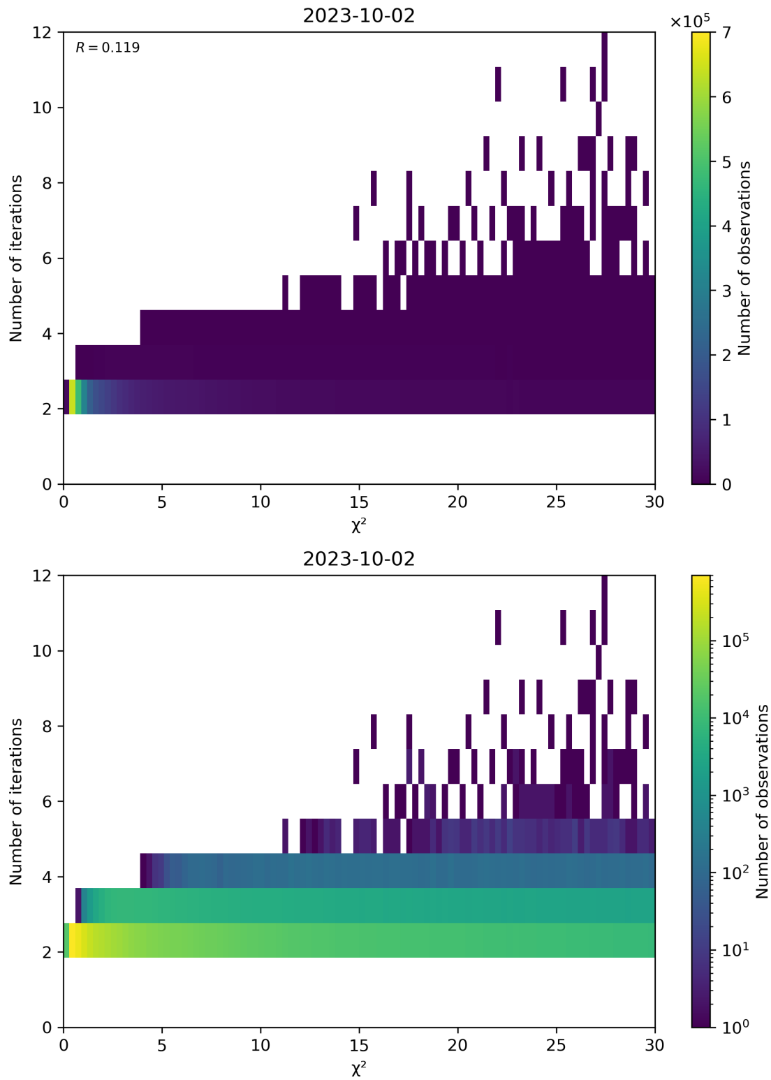
Figure 73: Scatter density plot of “ \chi^2 ” against “Number of iterations” for 2023-10-01 to 2023-10-03.
