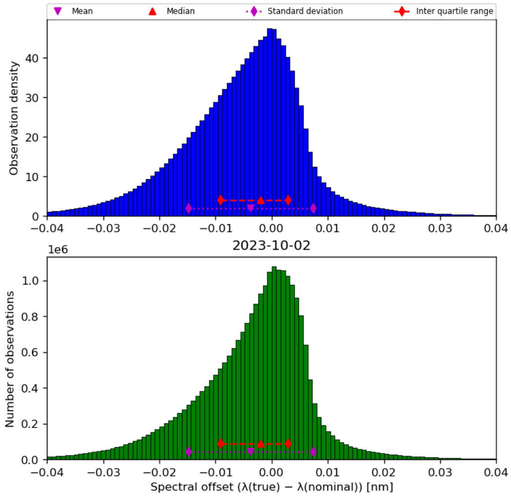
Figure 45: Histogram of “Spectral offset ( \lambda(\text{true}) - \lambda(\text{nominal}) )” for 2023-10-01 to 2023-10-03
