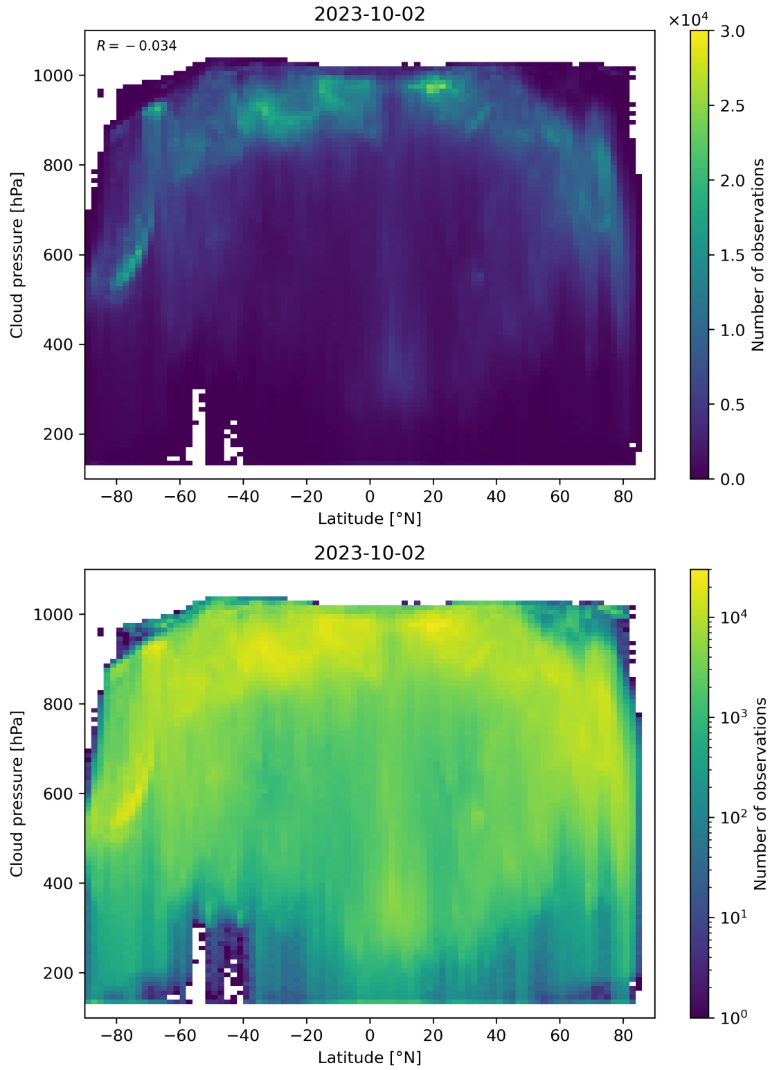
Figure 100: Scatter density plot of “Latitude” against “Cloud pressure” for 2023-10-01 to 2023-10-03.
