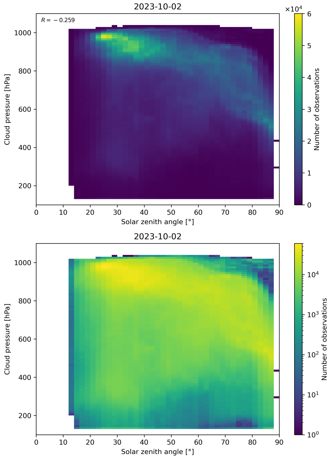
Figure 122: Scatter density plot of “Solar zenith angle” against “Cloud pressure” for 2023-10-01 to 2023-10-03.
