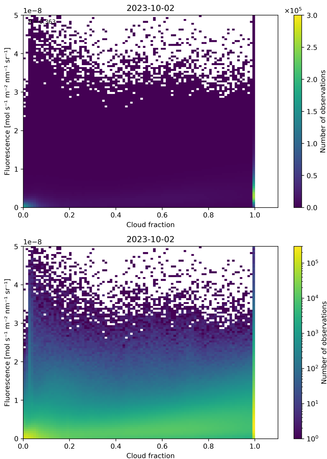
Figure 79: Scatter density plot of “Cloud fraction” against “Fluorescence” for 2023-10-01 to 2023-10-03.
