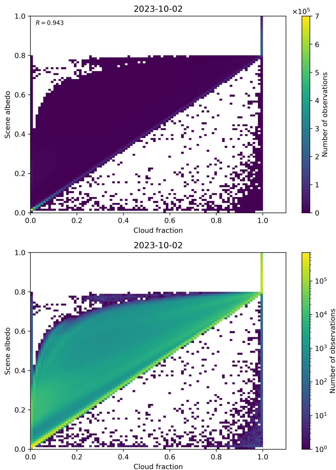
Figure 82: Scatter density plot of “Cloud fraction” against “Scene albedo” for 2023-10-01 to 2023-10-03.
