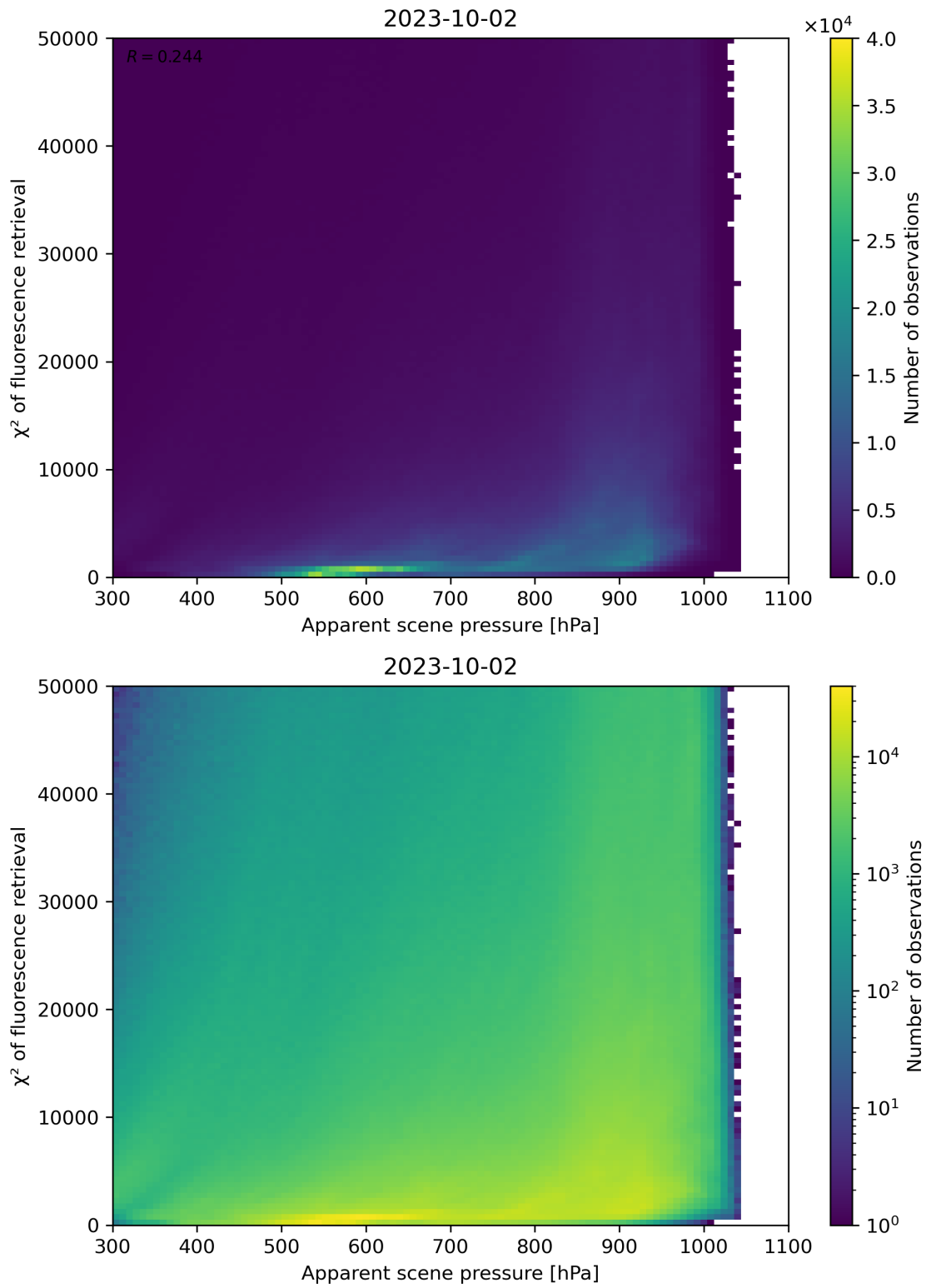
Figure 64: Scatter density plot of “Apparent scene pressure” against “ \chi^2 of fluorescence retrieval” for 2023-10-01 to 2023-10-03.
