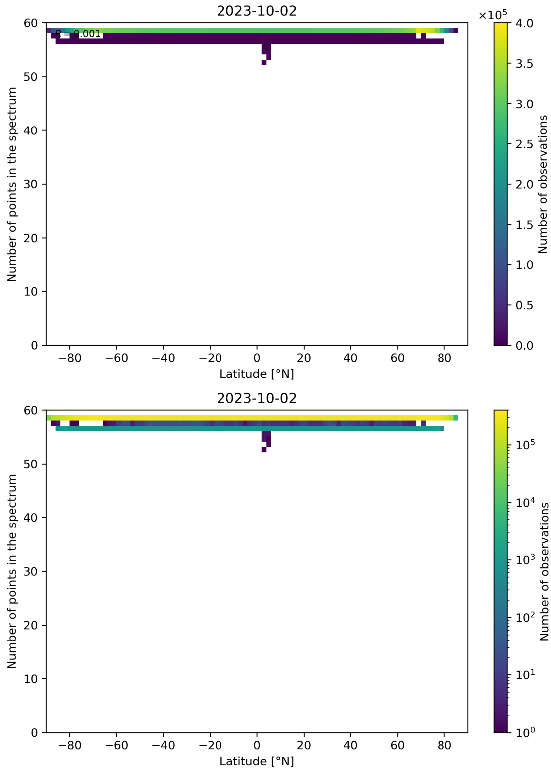
Figure 103: Scatter density plot of “Latitude” against “Number of points in the spectrum” for 2023-10-01 to 2023-10-03.
