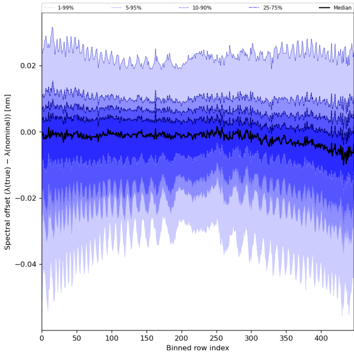
Figure 62: Along track statistics of “Spectral offset ( \lambda(\text{true}) - \lambda(\text{nominal}) )” for 2023-10-01 to 2023-10-03
