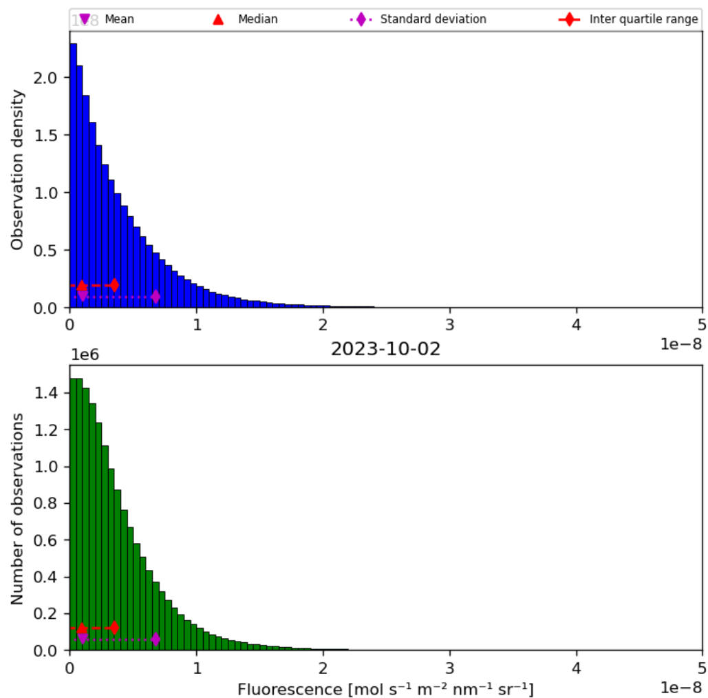
Figure 40: Histogram of “Fluorescence” for 2023-10-01 to 2023-10-03
