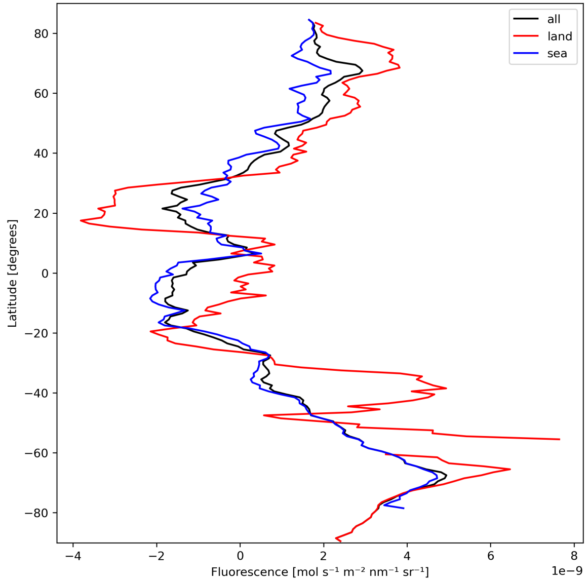
Figure 23: Zonal average of “Fluorescence” for 2023-10-01 to 2023-10-03.
