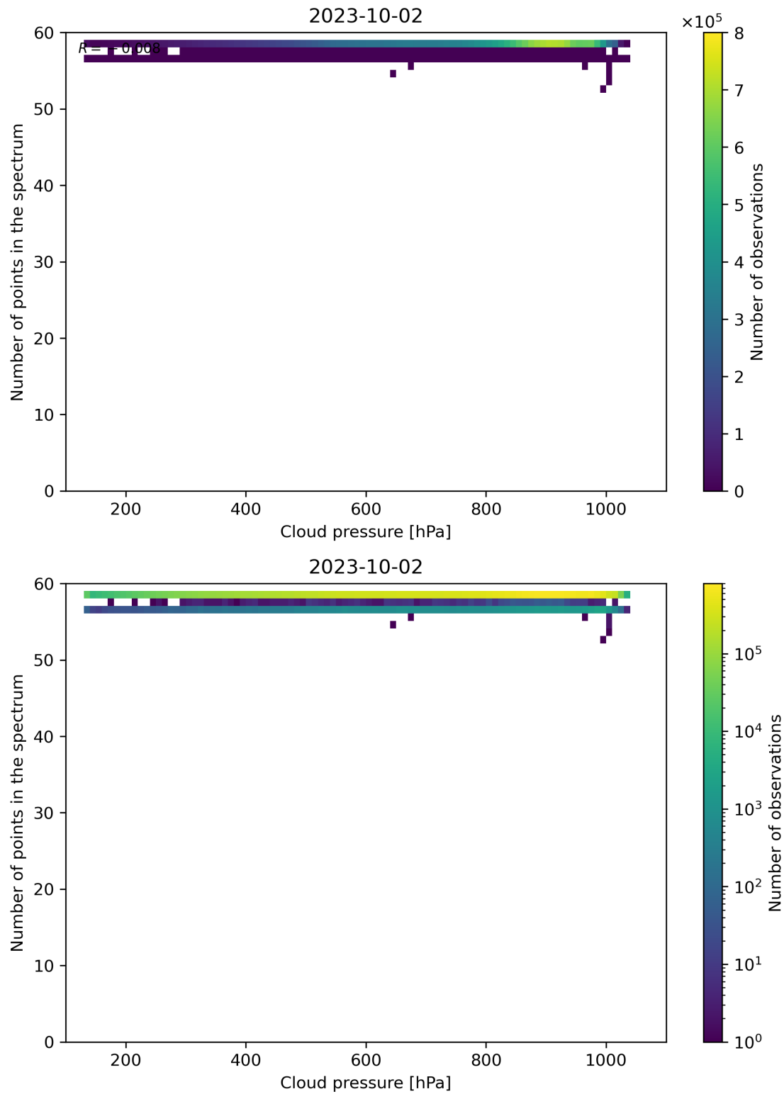
Figure 90: Scatter density plot of “Cloud pressure” against “Number of points in the spectrum” for 2023-10-01 to 2023-10-03.
