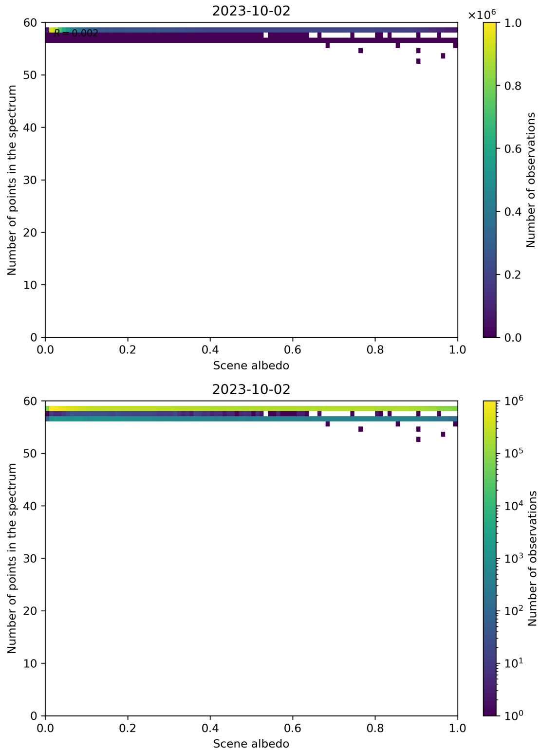
Figure 116: Scatter density plot of “Scene albedo” against “Number of points in the spectrum” for 2023-10-01 to 2023-10-03.
