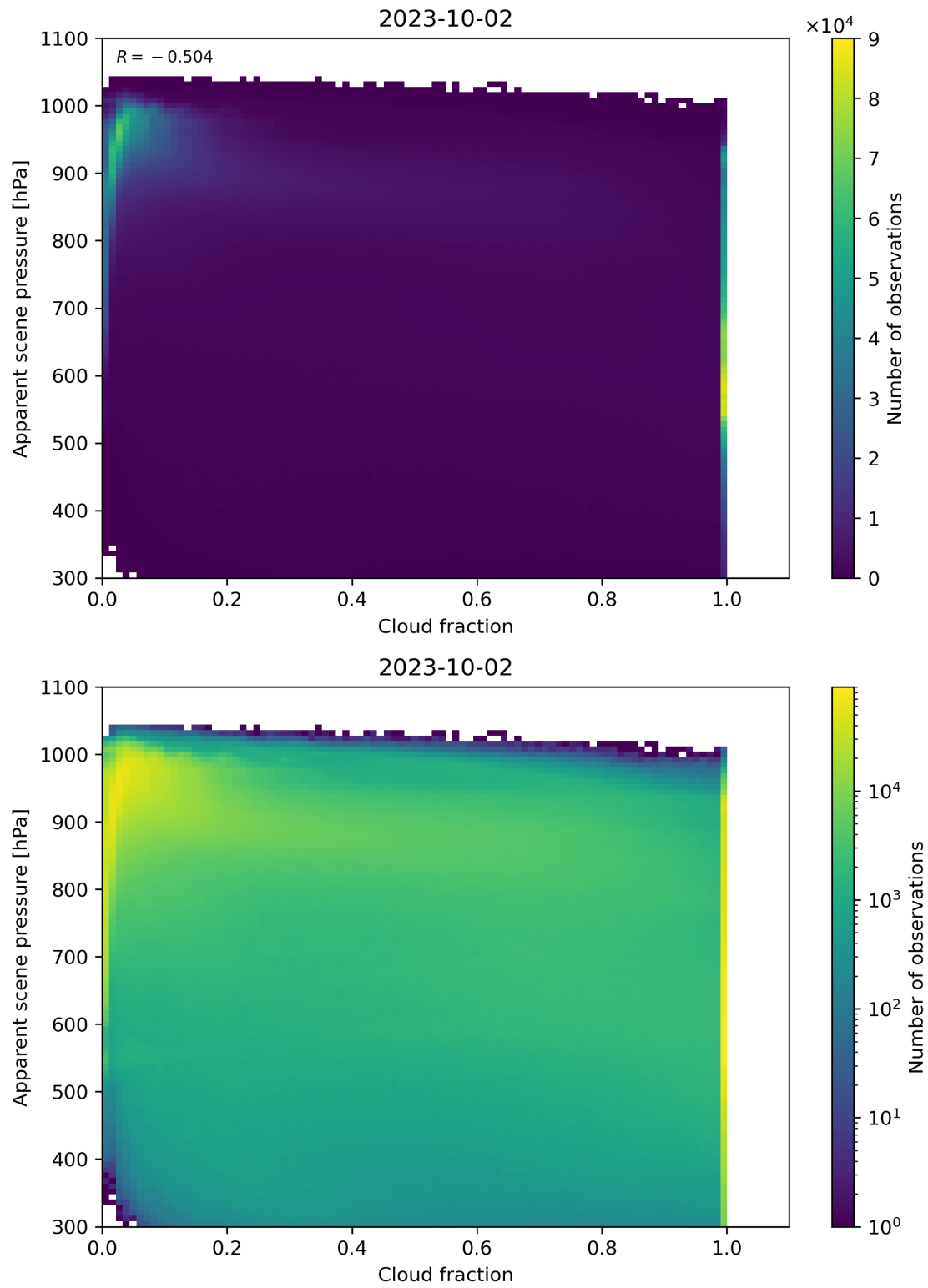
Figure 76: Scatter density plot of “Cloud fraction” against “Apparent scene pressure” for 2023-10-01 to 2023-10-03.
