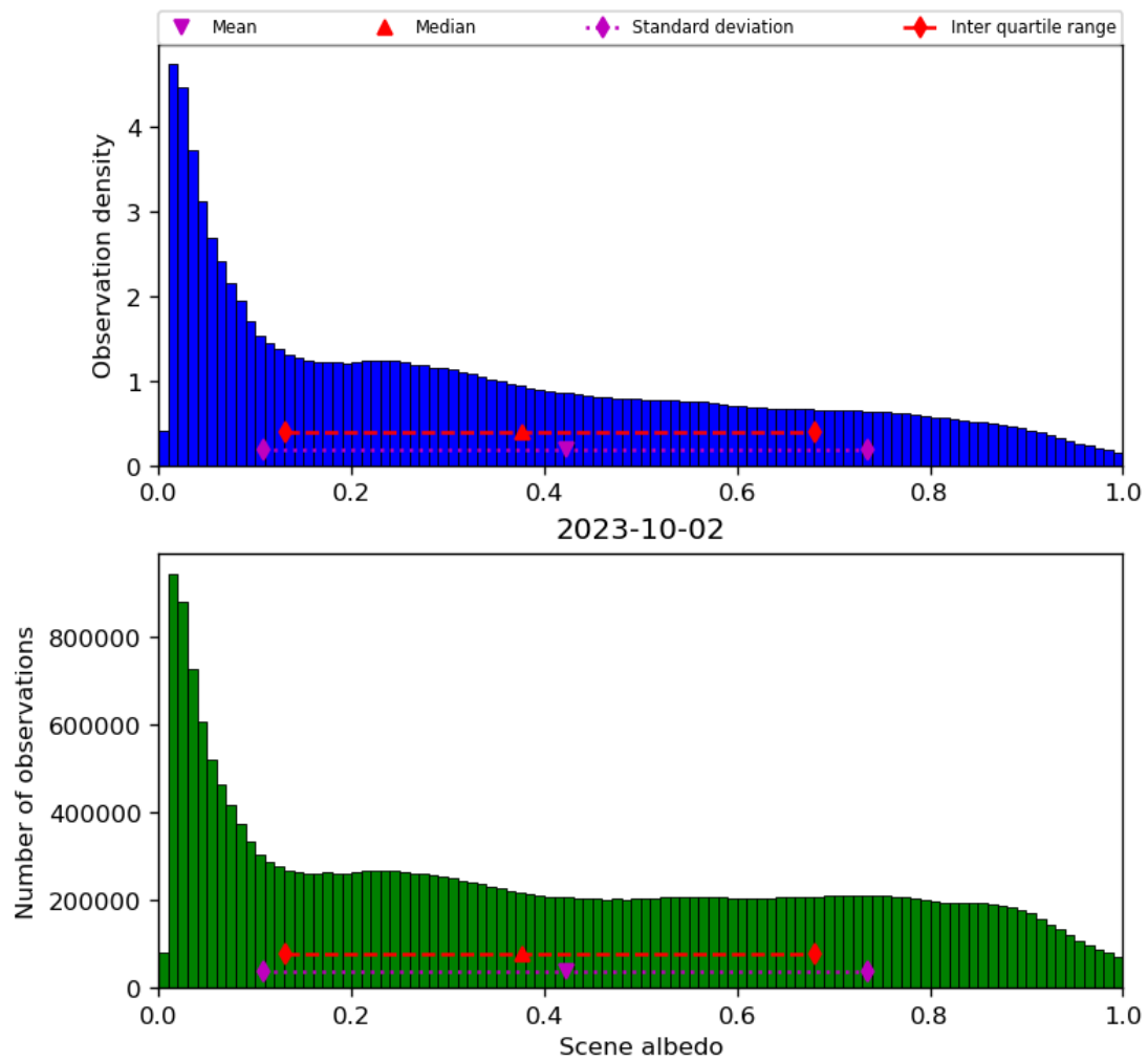
Figure 34: Histogram of “Scene albedo” for 2023-10-01 to 2023-10-03
