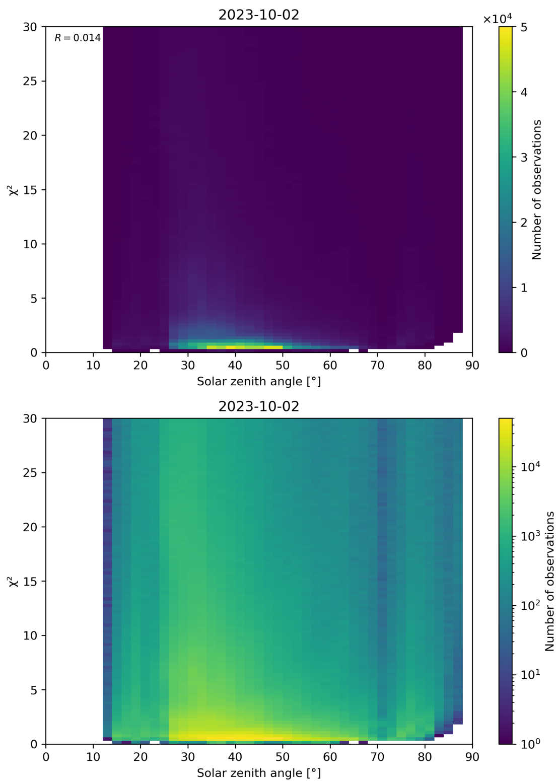
Figure 119: Scatter density plot of “Solar zenith angle” against “ \chi^2 ” for 2023-10-01 to 2023-10-03.
