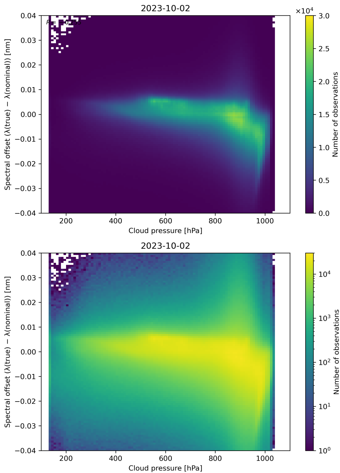
Figure 92: Scatter density plot of “Cloud pressure” against “Spectral offset ( \lambda(\text{true}) - \lambda(\text{nominal}) )” for 2023-10-01 to 2023-10-03.
