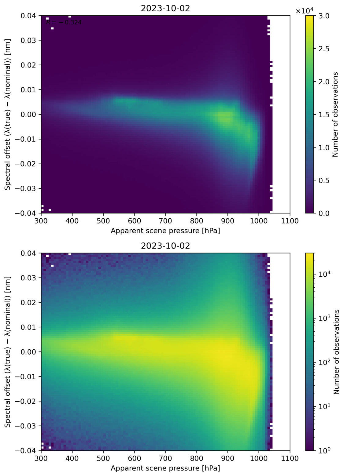
Figure 68: Scatter density plot of “Apparent scene pressure” against “Spectral offset ( \lambda(\text{true}) - \lambda(\text{nominal}) )” for 2023-10-01 to 2023-10-03.
