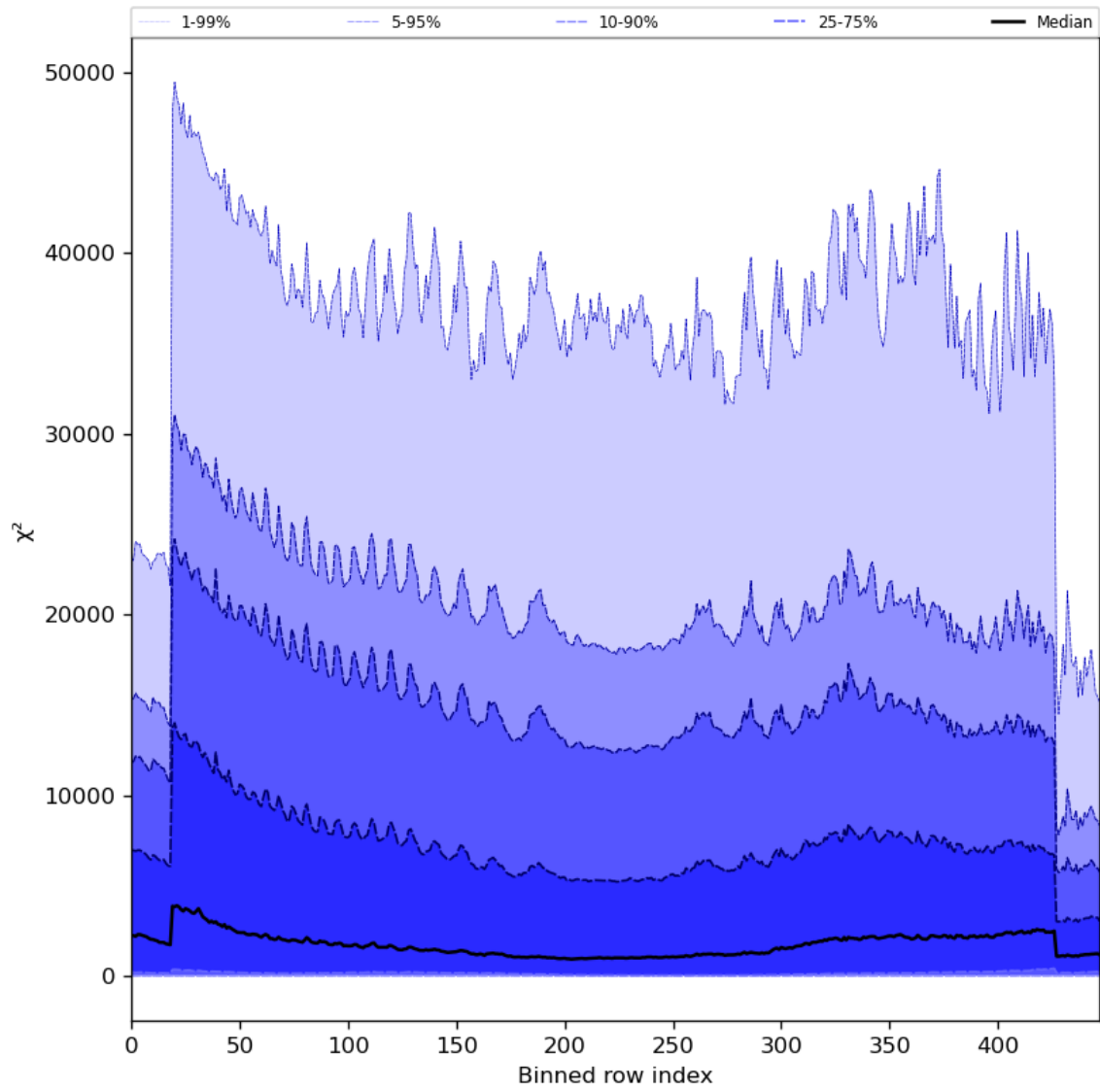
Figure 55: Along track statistics of “ \chi^2 ” for 2023-10-01 to 2023-10-03
