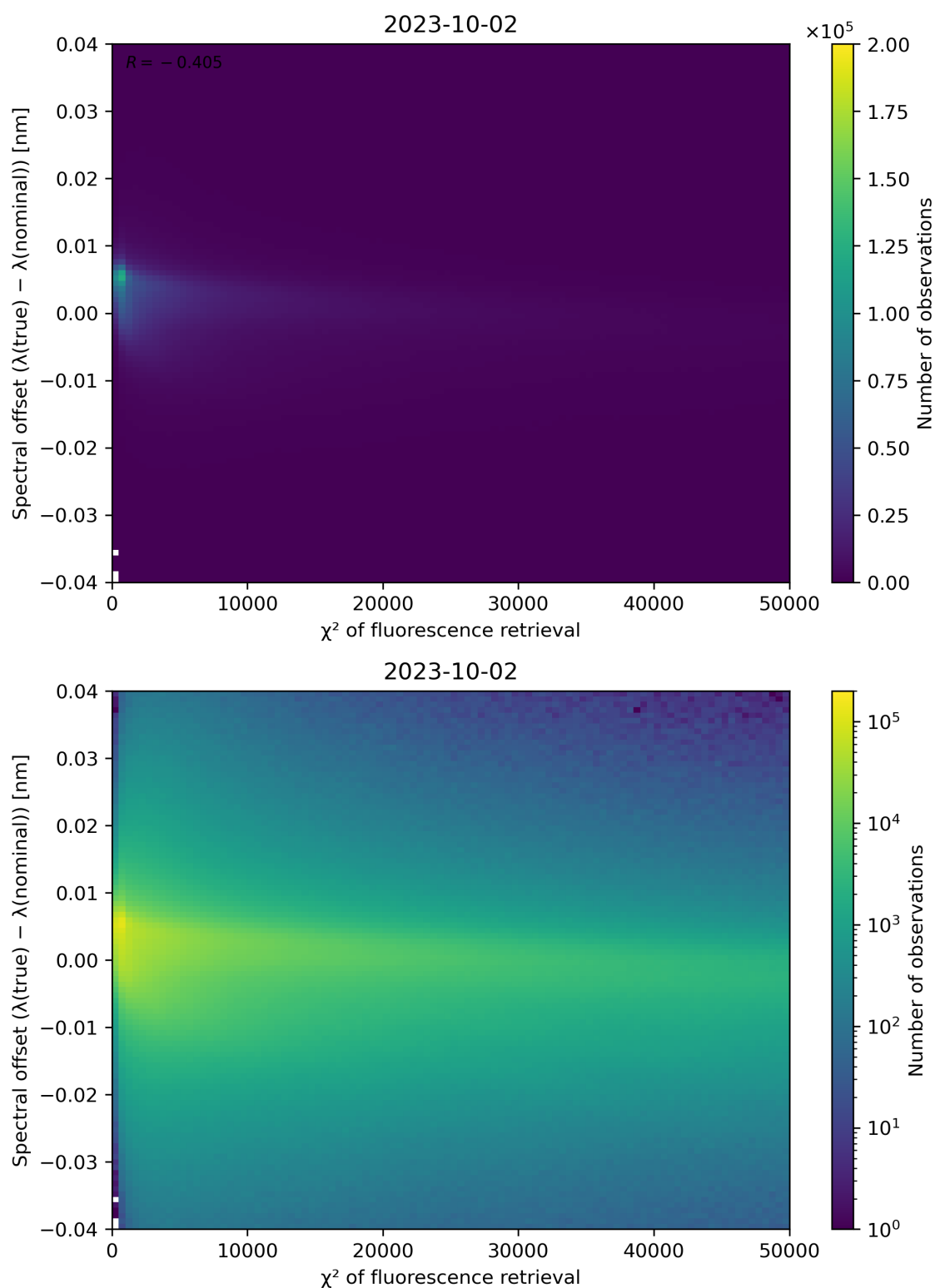
Figure 72: Scatter density plot of " \chi^2 of fluorescence retrieval" against "Spectral offset ( \lambda(\text{true}) - \lambda(\text{nominal})) " for 2023-10-01 to 2023-10-03.
