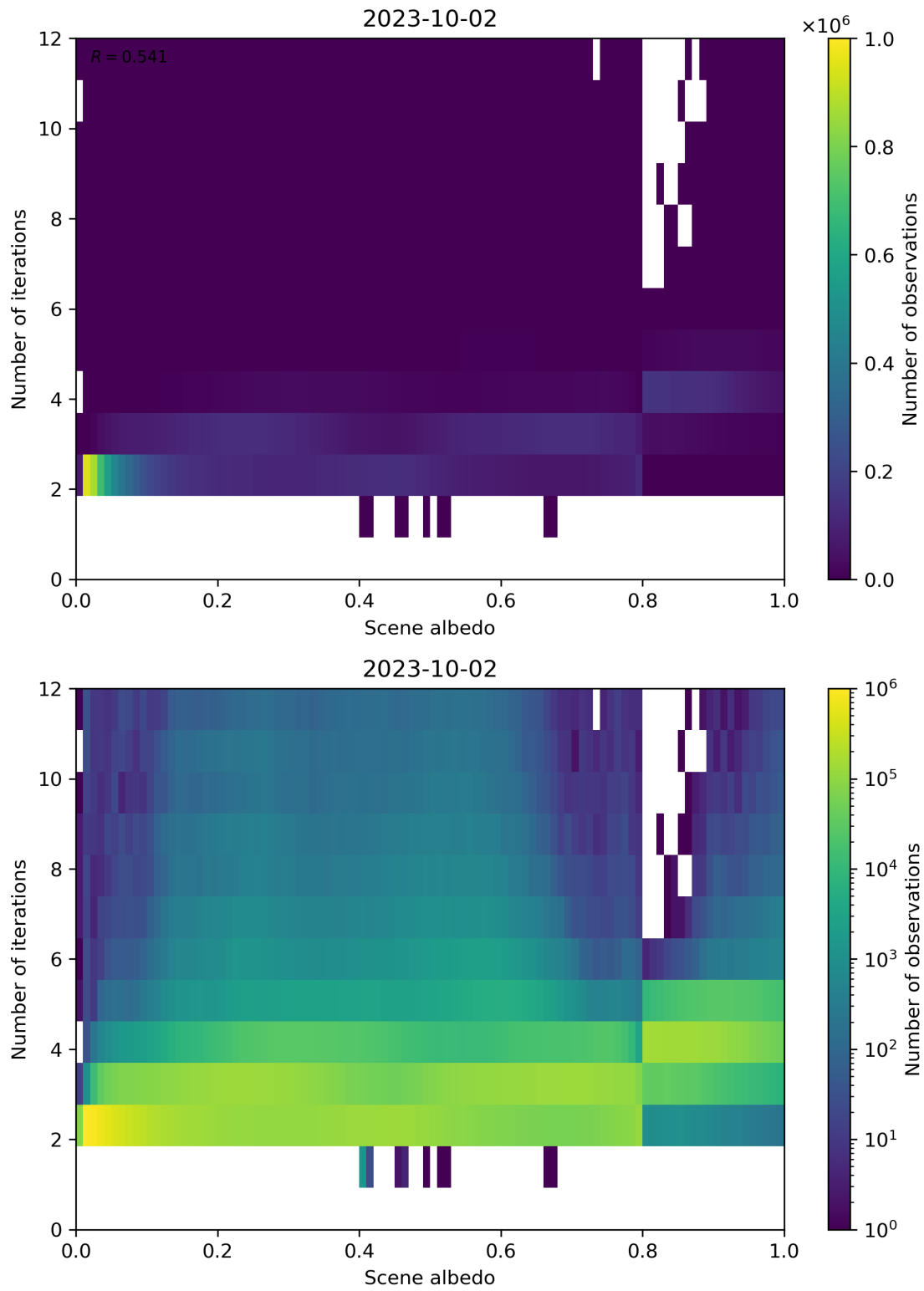
Figure 115: Scatter density plot of “Scene albedo” against “Number of iterations” for 2023-10-01 to 2023-10-03.
