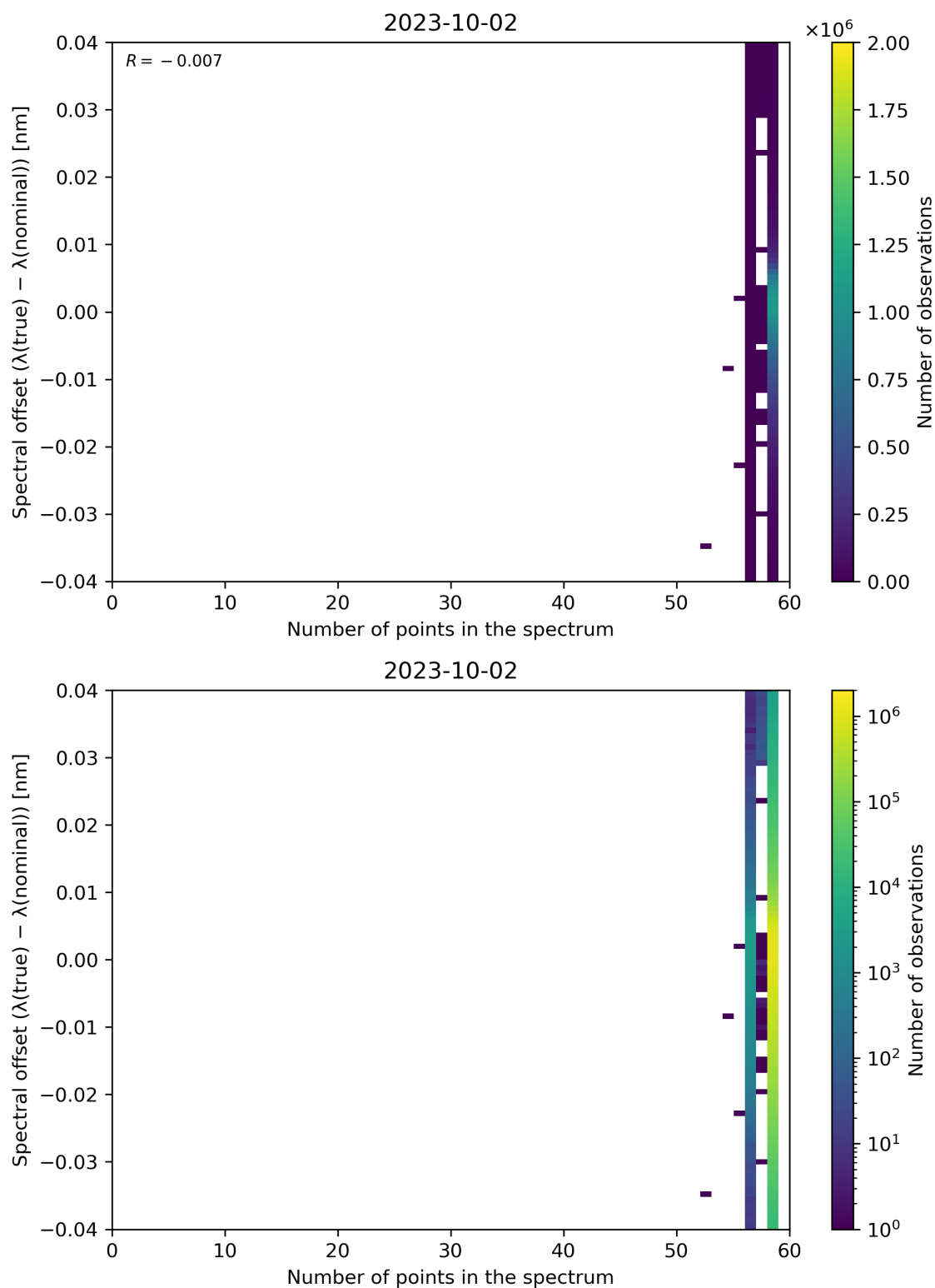
Figure 110: Scatter density plot of “Number of points in the spectrum” against “Spectral offset ( \lambda(\text{true}) - \lambda(\text{nominal}) )” for 2023-10-01 to 2023-10-03.
