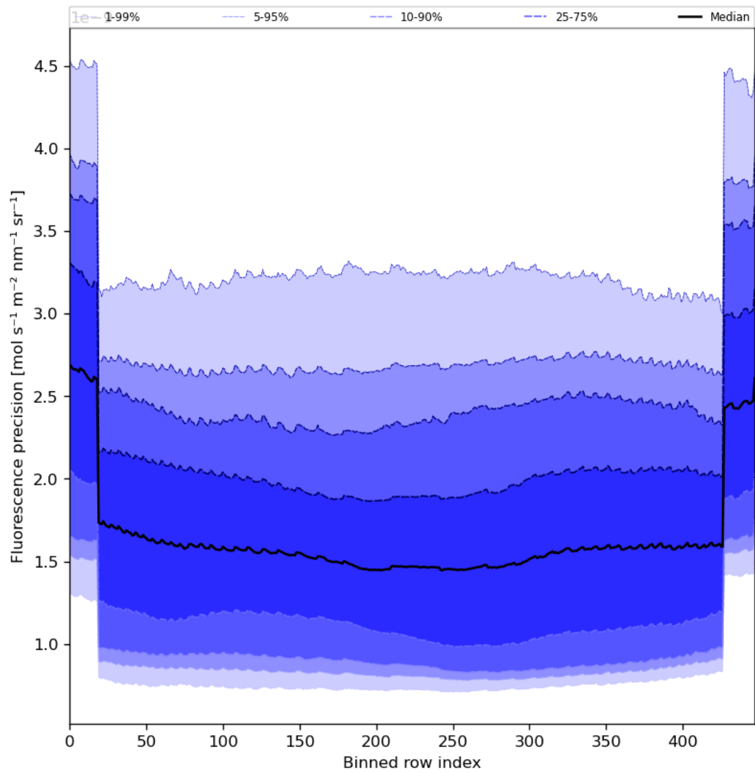
Figure 58: Along track statistics of “Fluorescence precision” for 2023-10-01 to 2023-10-03
