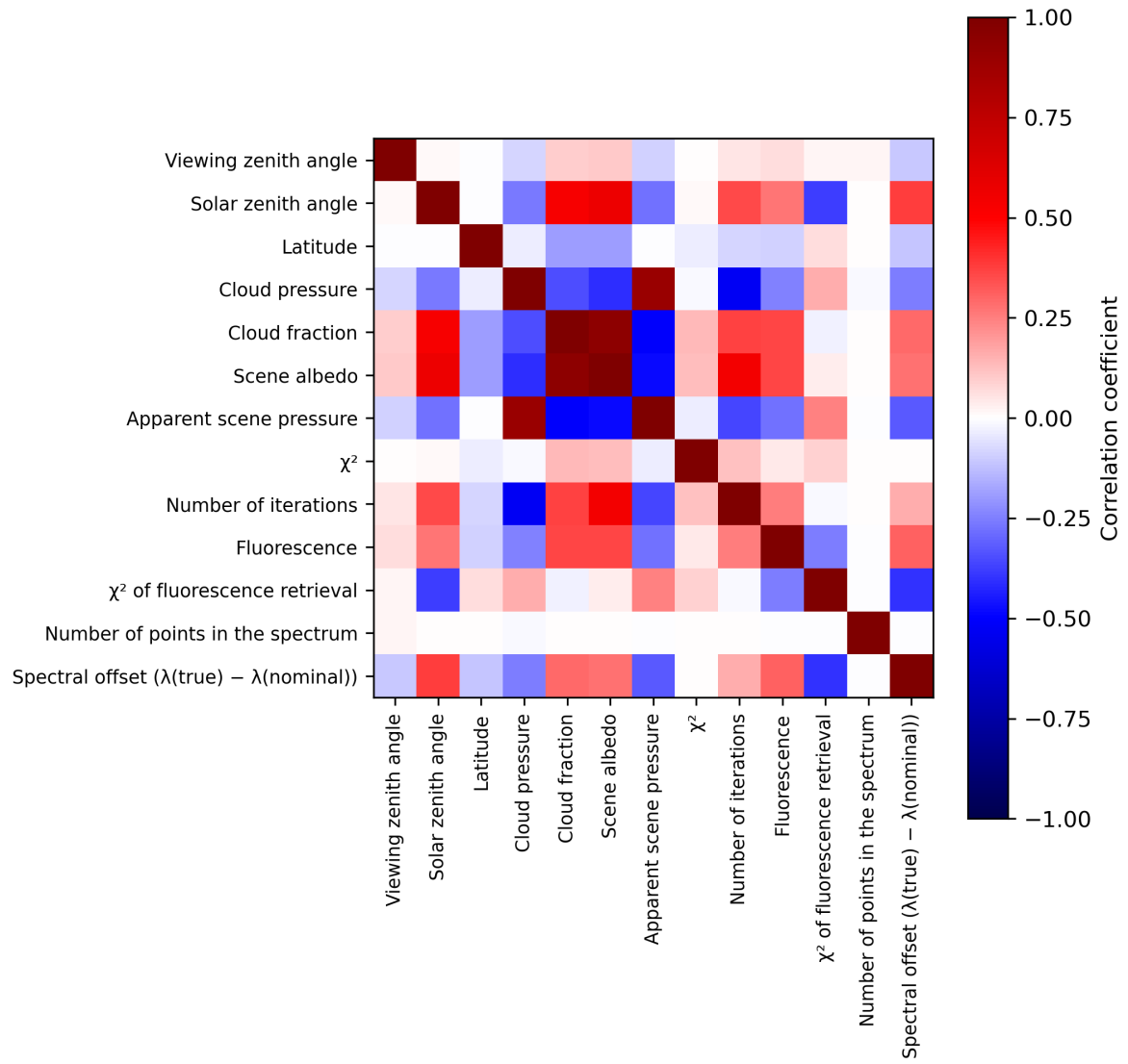
Figure 2: Map of correlation matrix for 2023-10-01 to 2023-10-03.
