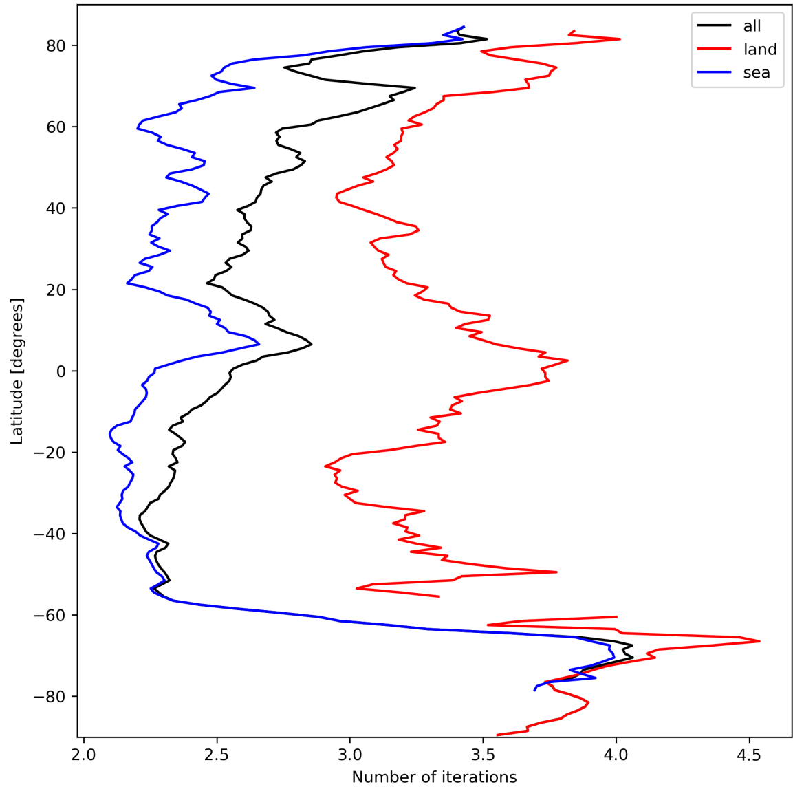
Figure 22: Zonal average of “Number of iterations” for 2023-10-01 to 2023-10-03.
