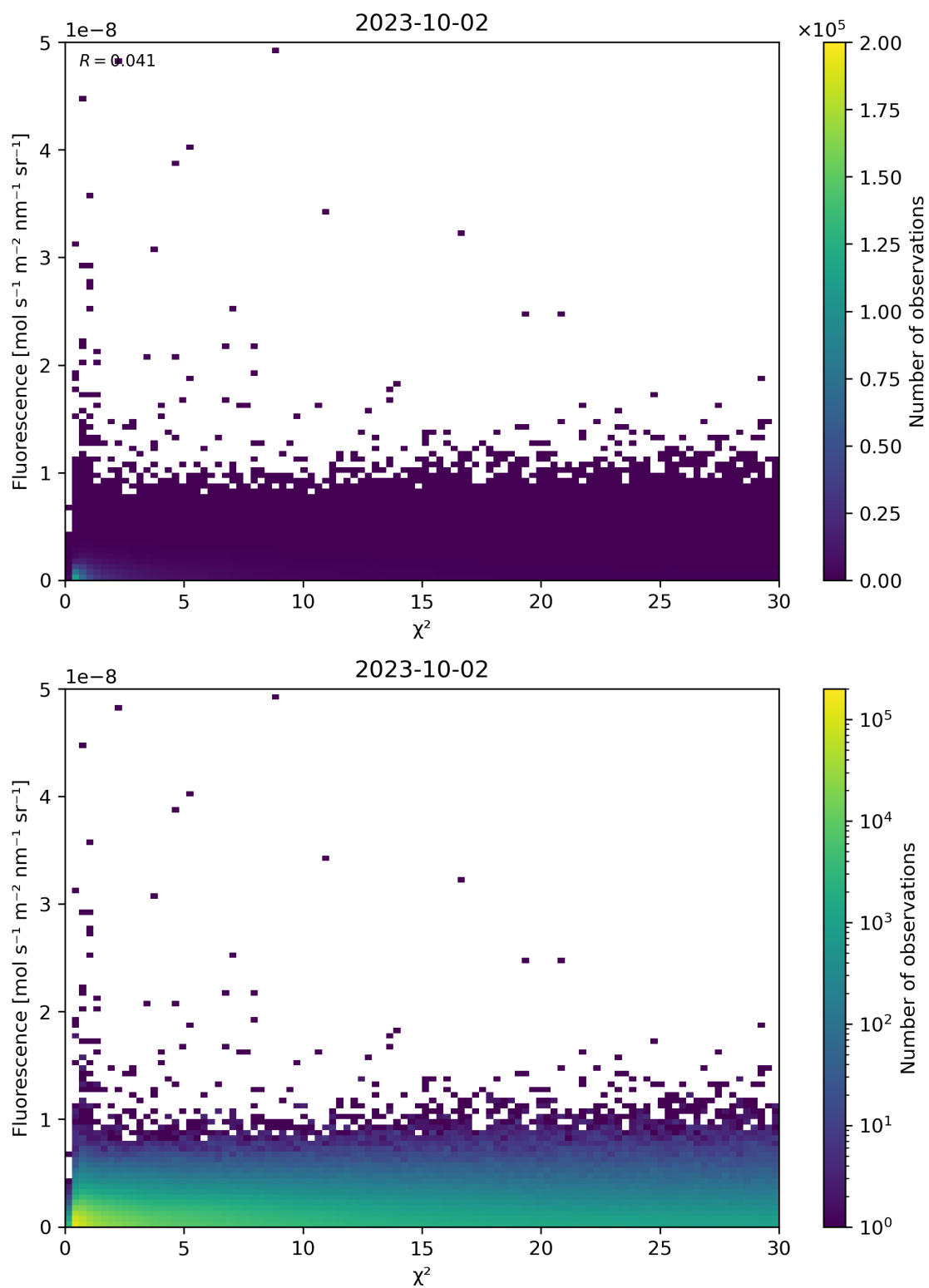
Figure 70: Scatter density plot of “ \chi^2 ” against “Fluorescence” for 2023-10-01 to 2023-10-03.
