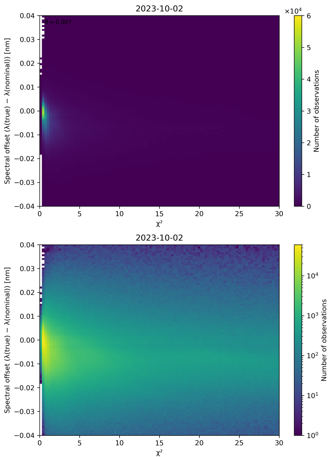
Figure 75: Scatter density plot of “ \chi^2 ” against “Spectral offset ( \lambda(\text{true}) - \lambda(\text{nominal}) )” for 2023-10-01 to 2023-10-03.
