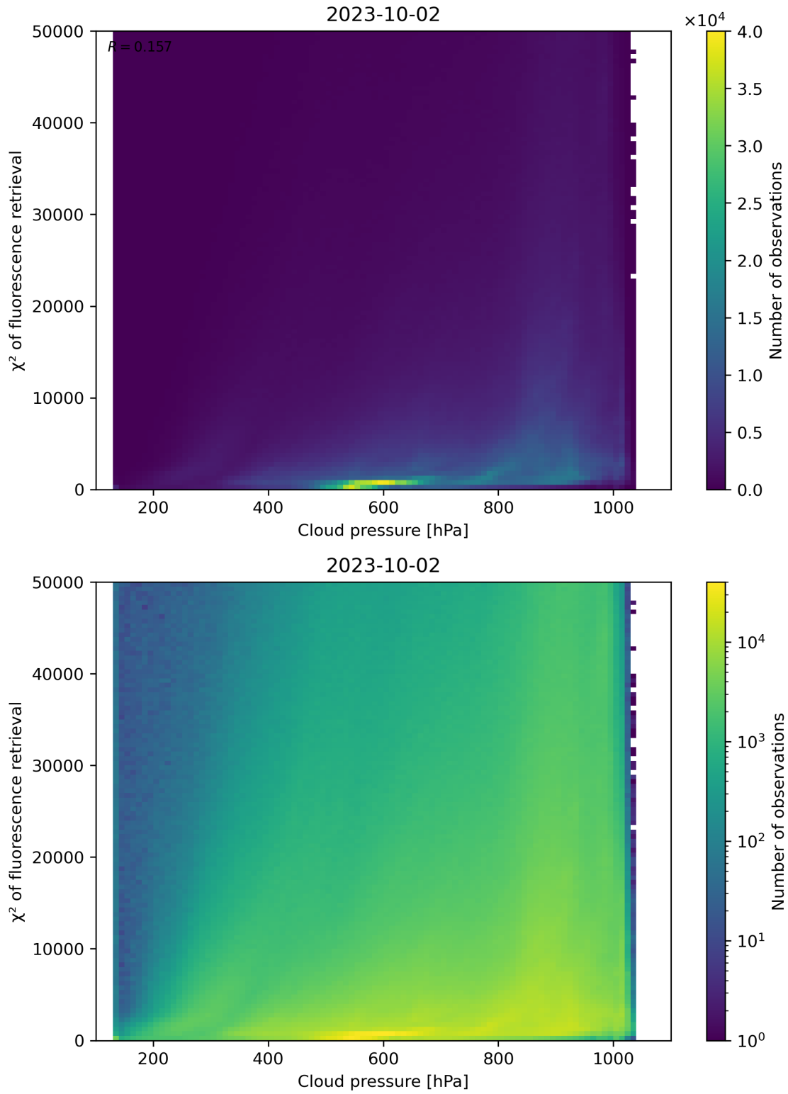
Figure 86: Scatter density plot of “Cloud pressure” against “ \chi^2 of fluorescence retrieval” for 2023-10-01 to 2023-10-03.
