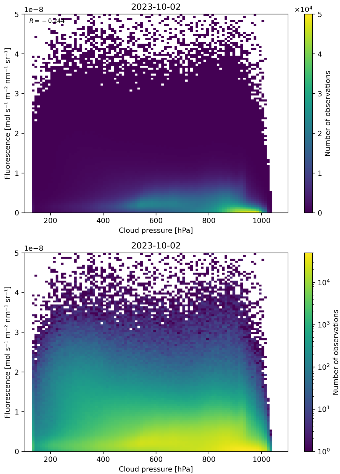
Figure 88: Scatter density plot of “Cloud pressure” against “Fluorescence” for 2023-10-01 to 2023-10-03.
