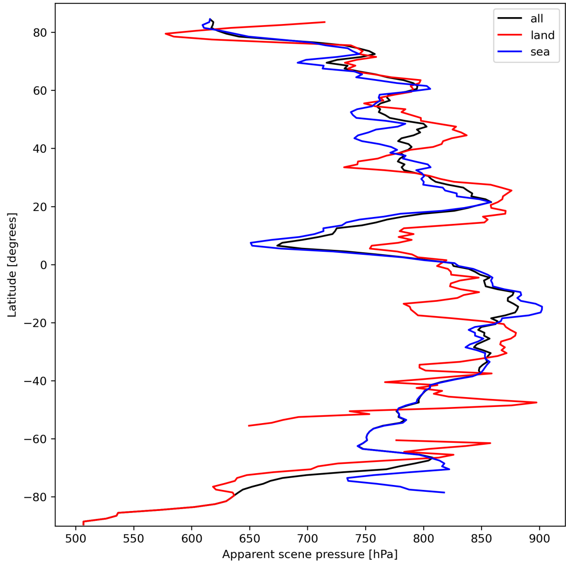
Figure 19: Zonal average of “Apparent scene pressure” for 2023-10-01 to 2023-10-03.
