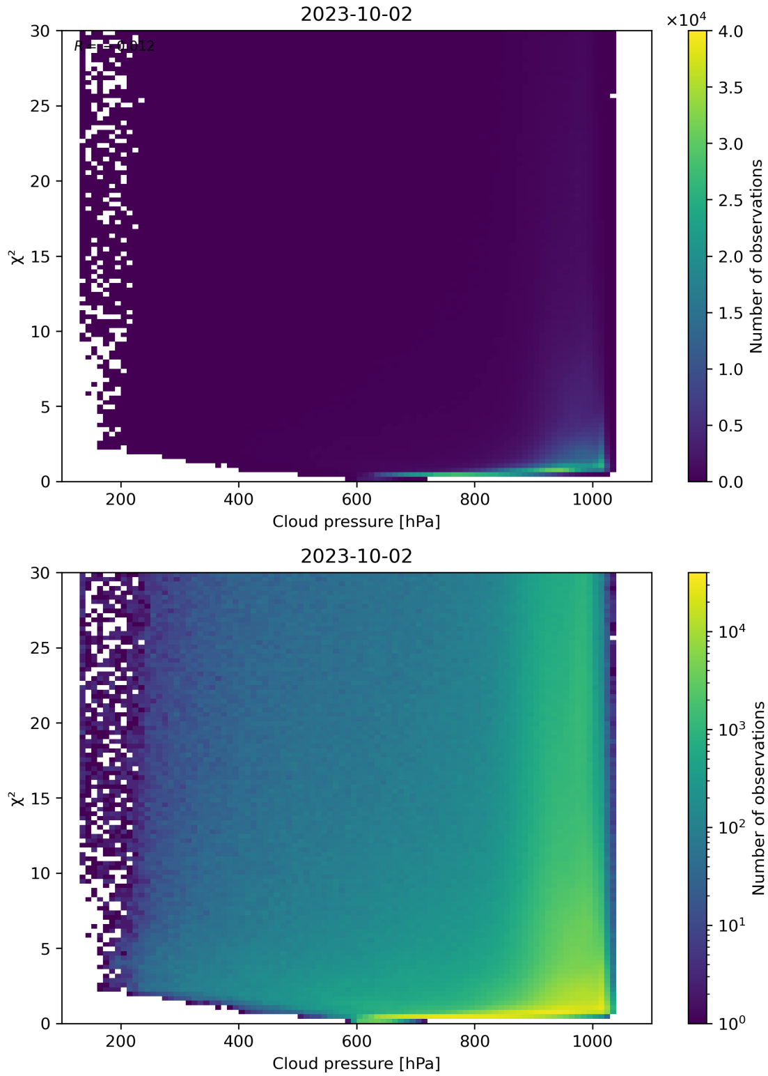
Figure 85: Scatter density plot of “Cloud pressure” against “ \chi^2 ” for 2023-10-01 to 2023-10-03.
