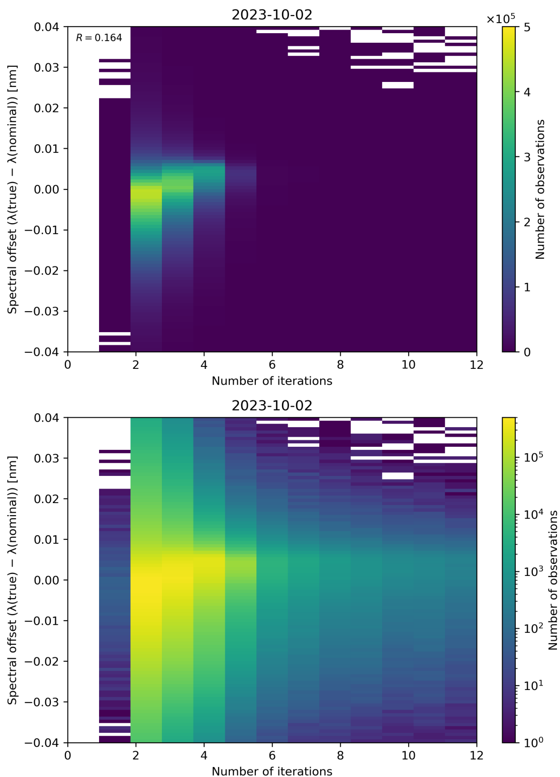
Figure 109: Scatter density plot of “Number of iterations” against “Spectral offset ( \lambda(\text{true}) - \lambda(\text{nominal}) )” for 2023-10-01 to 2023-10-03.
