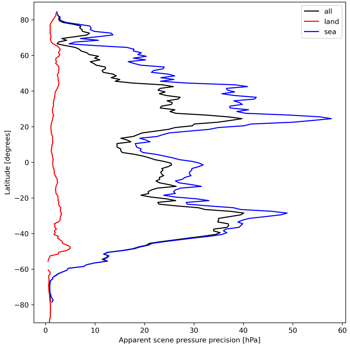
Figure 20: Zonal average of “Apparent scene pressure precision” for 2023-10-01 to 2023-10-03.
