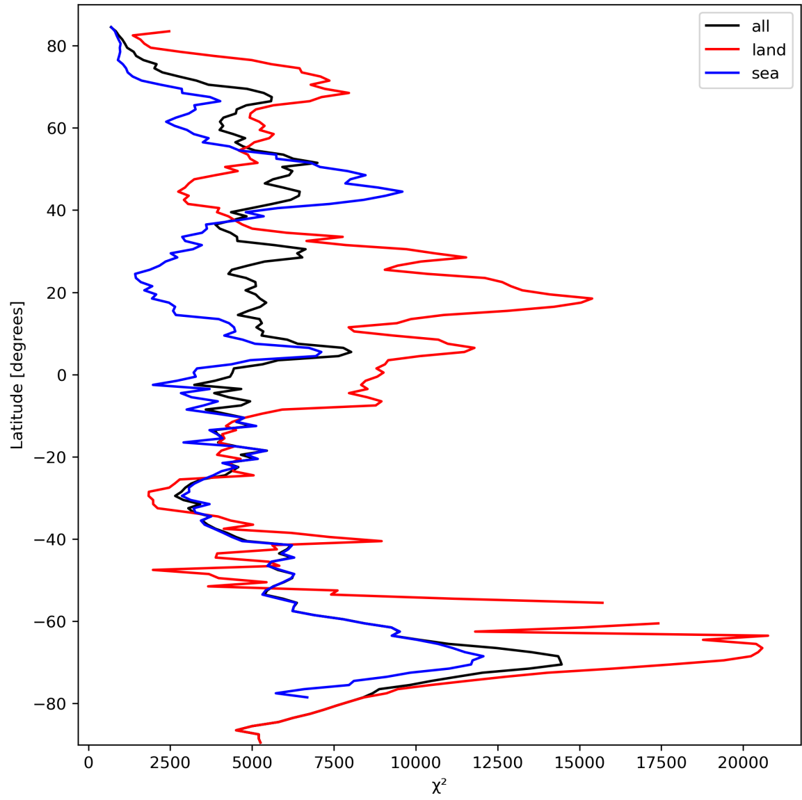
Figure 21: Zonal average of “ \chi^2 ” for 2023-10-01 to 2023-10-03.
