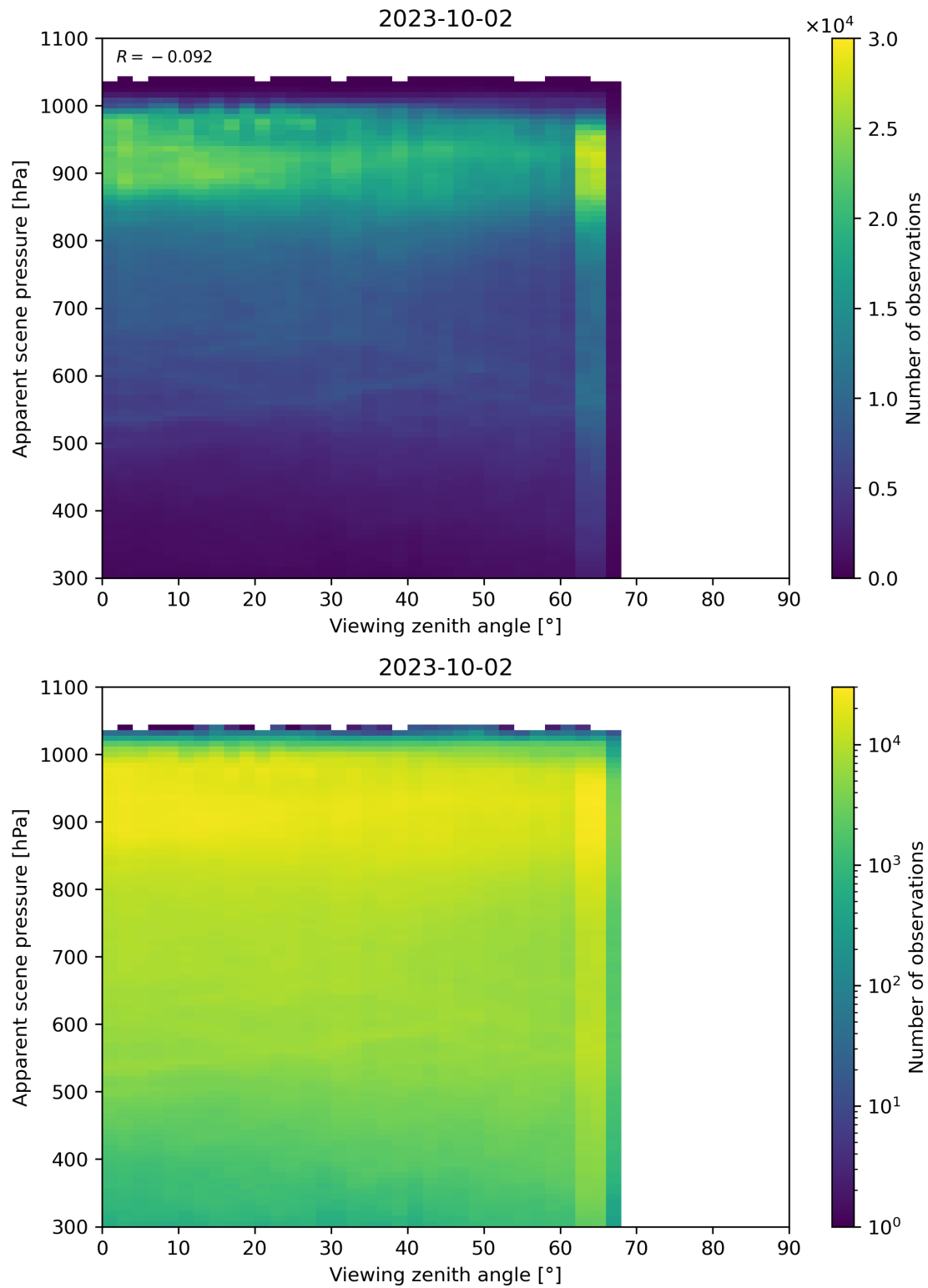
Figure 129: Scatter density plot of “Viewing zenith angle” against “Apparent scene pressure” for 2023-10-01 to 2023-10-03.
