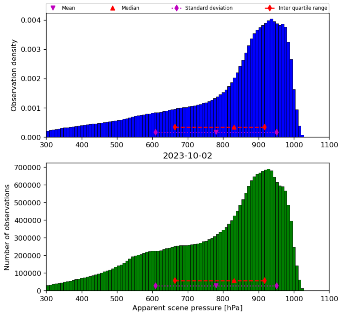
Figure 36: Histogram of “Apparent scene pressure” for 2023-10-01 to 2023-10-03
