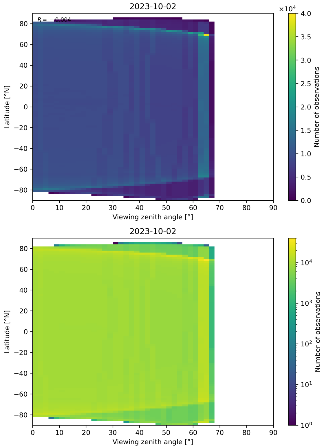
Figure 135: Scatter density plot of “Viewing zenith angle” against “Latitude” for 2023-10-01 to 2023-10-03.
