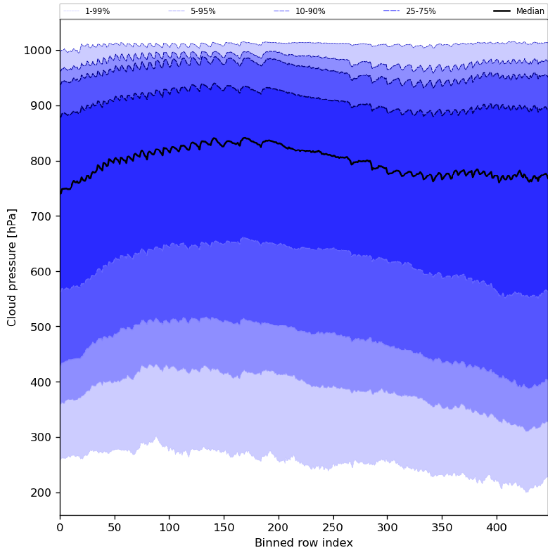
Figure 47: Along track statistics of “Cloud pressure” for 2023-10-01 to 2023-10-03
