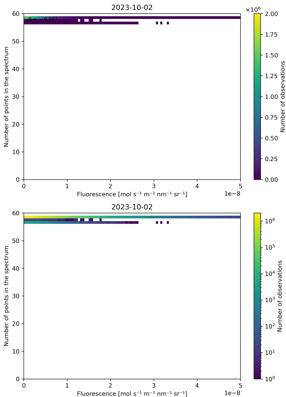
Figure 94: Scatter density plot of “Fluorescence” against “Number of points in the spectrum” for 2023-10-01 to 2023-10-03.
