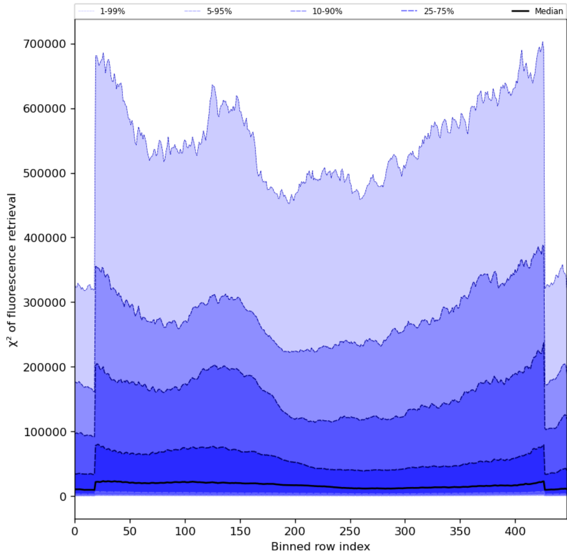
Figure 59: Along track statistics of “ \chi^2 of fluorescence retrieval” for 2023-10-01 to 2023-10-03
