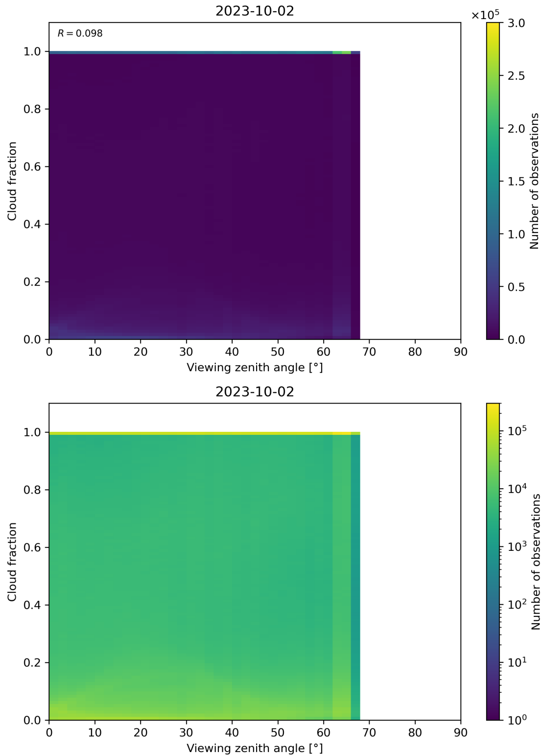
Figure 132: Scatter density plot of “Viewing zenith angle” against “Cloud fraction” for 2023-10-01 to 2023-10-03.
