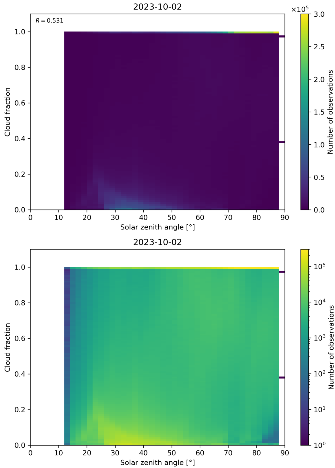
Figure 121: Scatter density plot of “Solar zenith angle” against “Cloud fraction” for 2023-10-01 to 2023-10-03.
