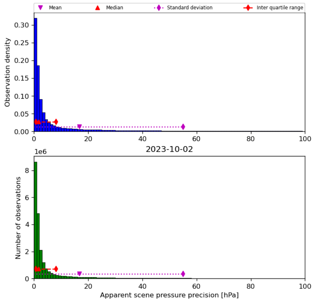
Figure 37: Histogram of “Apparent scene pressure precision” for 2023-10-01 to 2023-10-03
