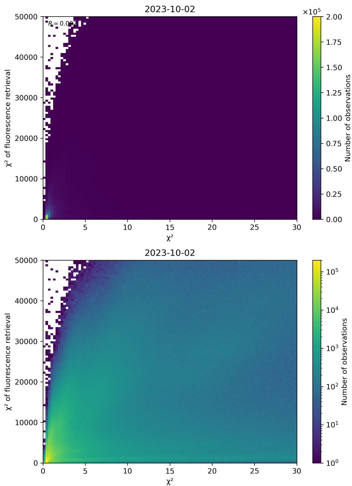
Figure 69: Scatter density plot of “ \chi^2 ” against “ \chi^2 of fluorescence retrieval” for 2023-10-01 to 2023-10-03.
