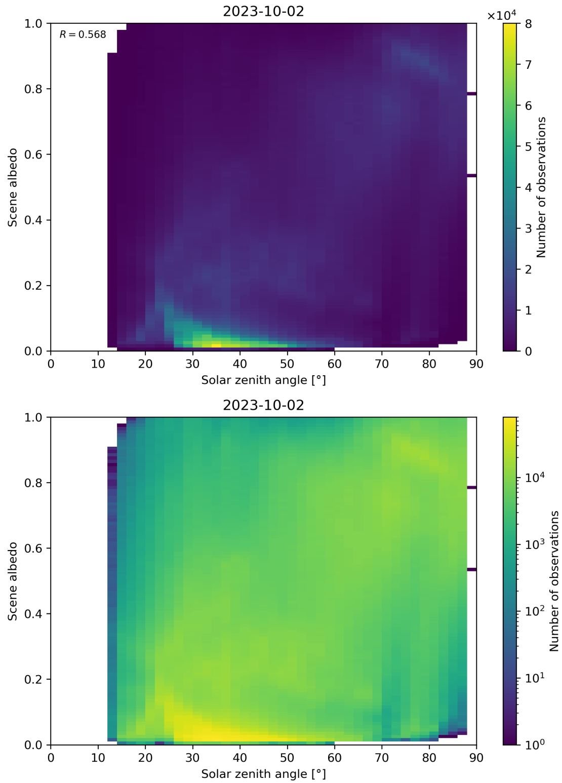
Figure 127: Scatter density plot of “Solar zenith angle” against “Scene albedo” for 2023-10-01 to 2023-10-03.
