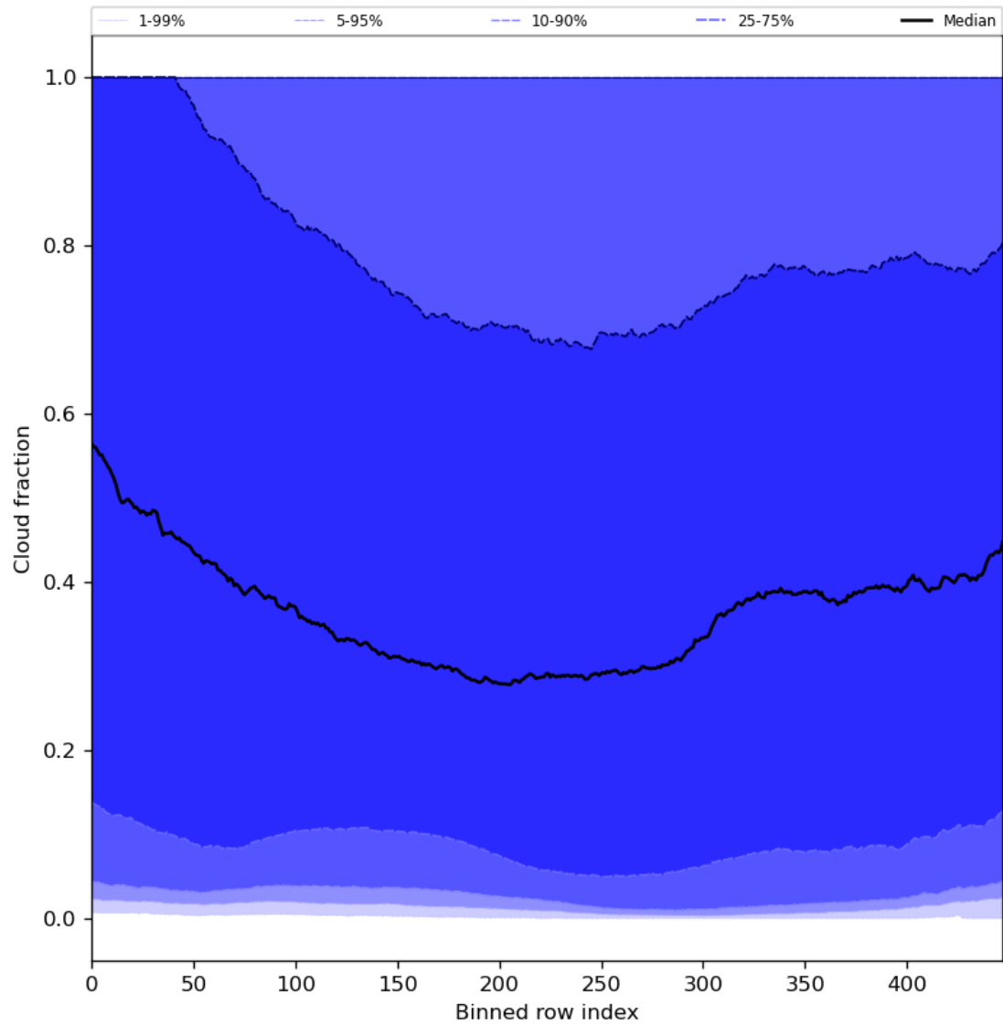
Figure 49: Along track statistics of “Cloud fraction” for 2023-10-01 to 2023-10-03
