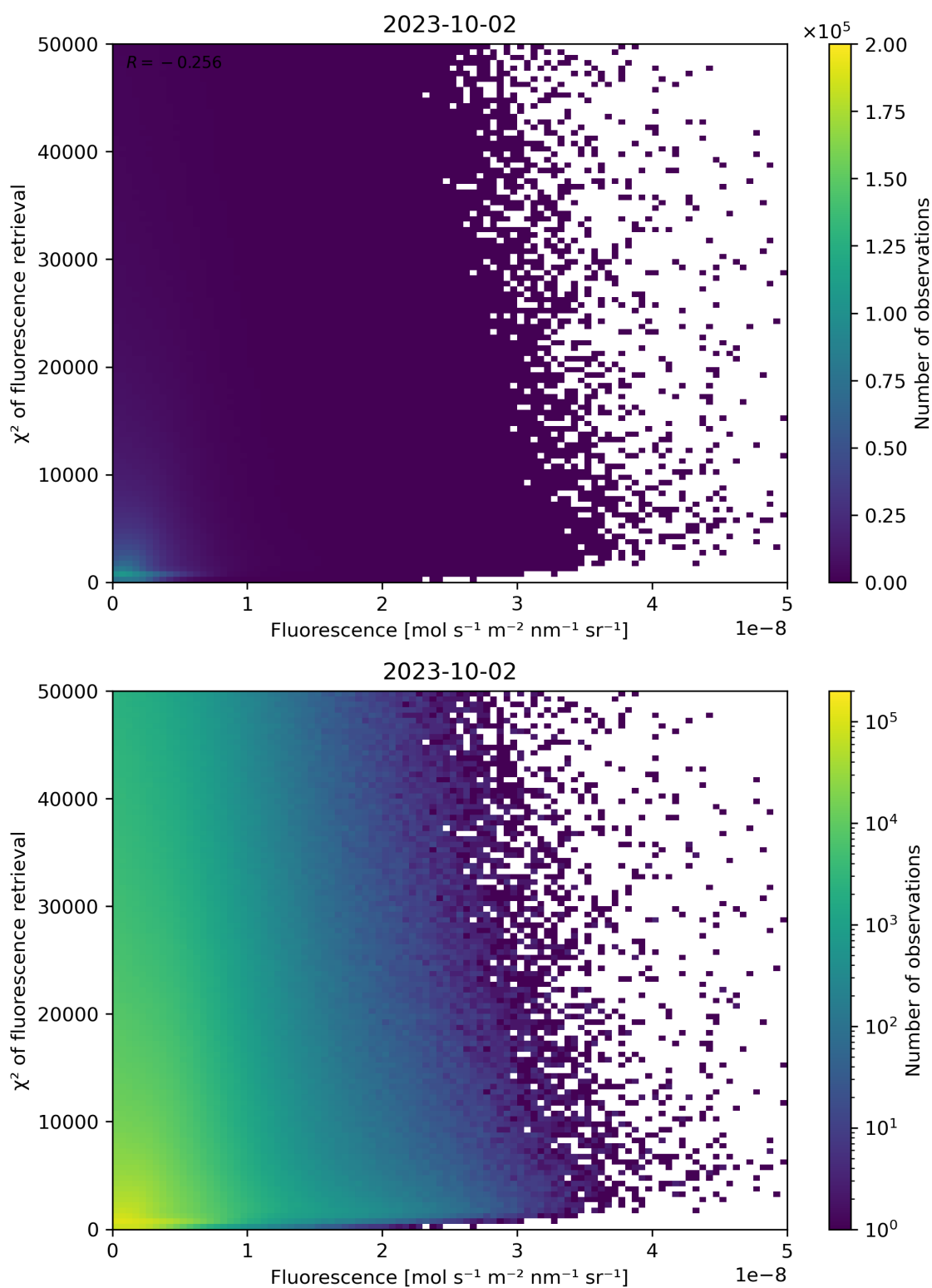
Figure 93: Scatter density plot of “Fluorescence” against “ \chi^2 of fluorescence retrieval” for 2023-10-01 to 2023-10-03.
