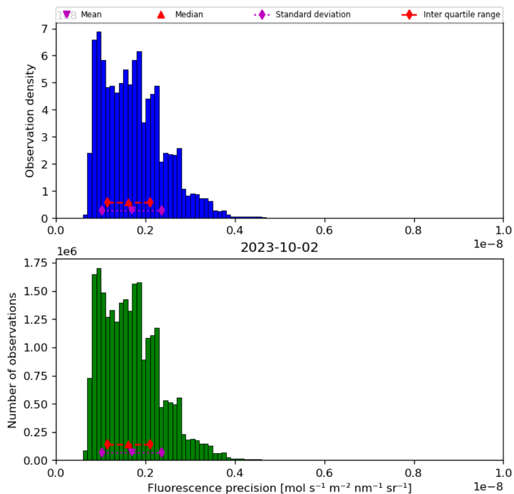
Figure 41: Histogram of “Fluorescence precision” for 2023-10-01 to 2023-10-03
