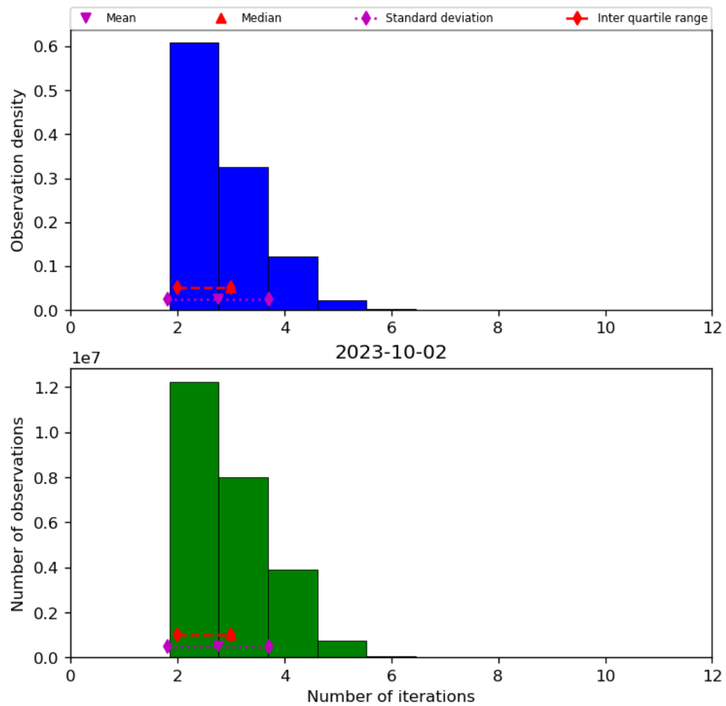
Figure 39: Histogram of “Number of iterations” for 2023-10-01 to 2023-10-03
