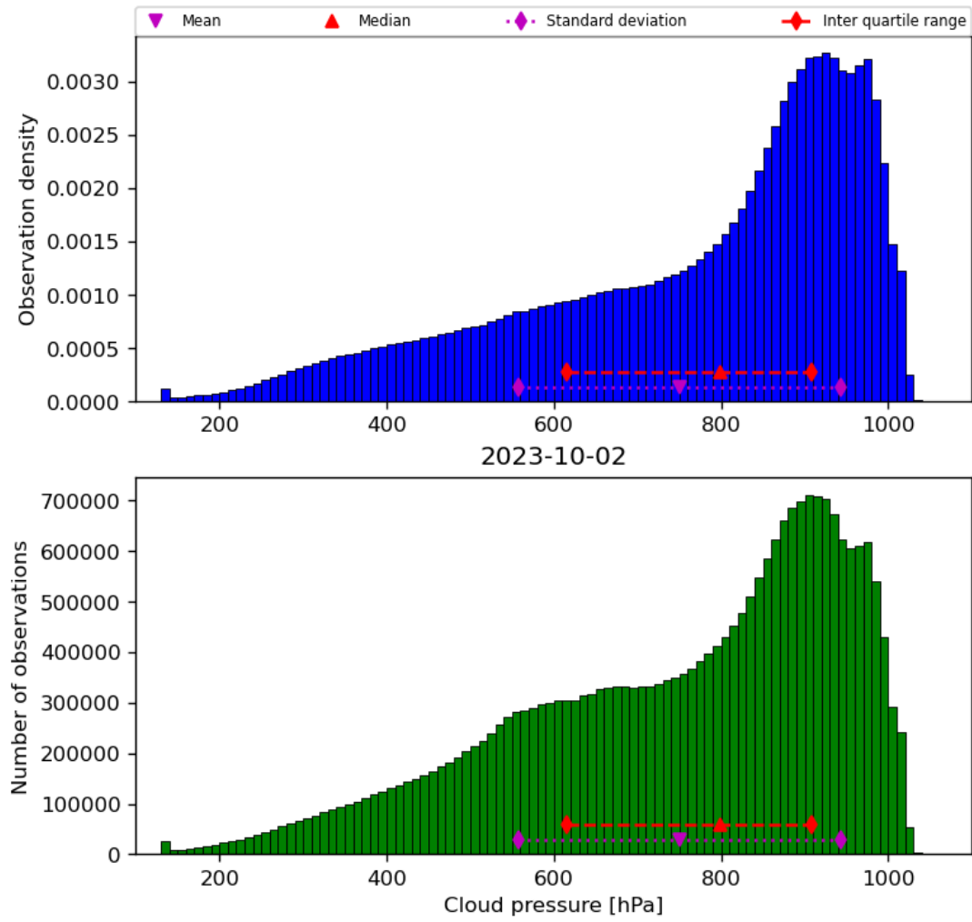
Figure 30: Histogram of “Cloud pressure” for 2023-10-01 to 2023-10-03
