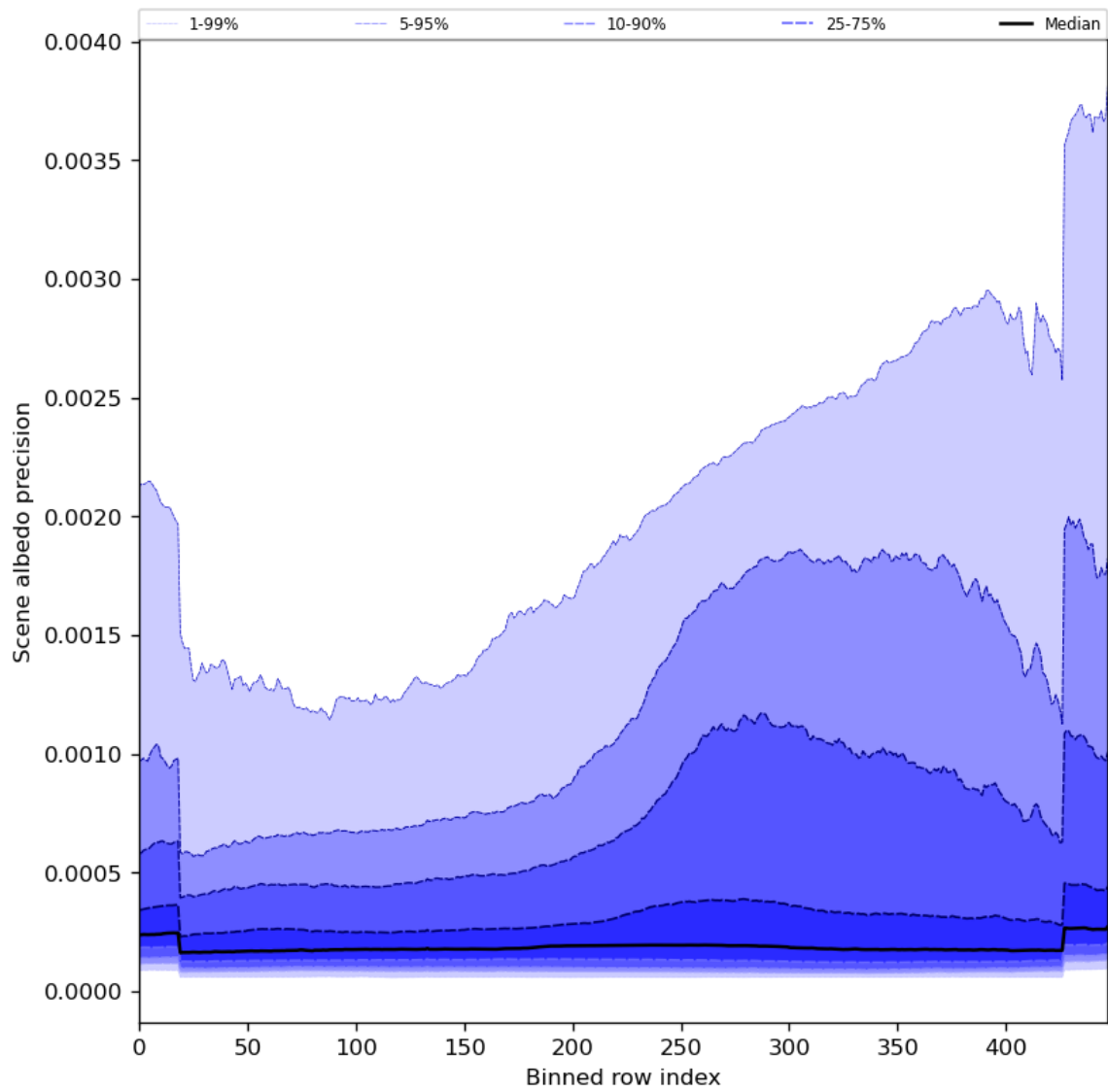
Figure 52: Along track statistics of “Scene albedo precision” for 2023-10-01 to 2023-10-03
