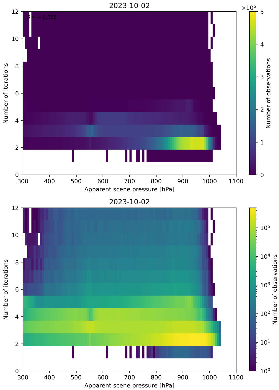
Figure 66: Scatter density plot of “Apparent scene pressure” against “Number of iterations” for 2023-10-01 to 2023-10-03.
