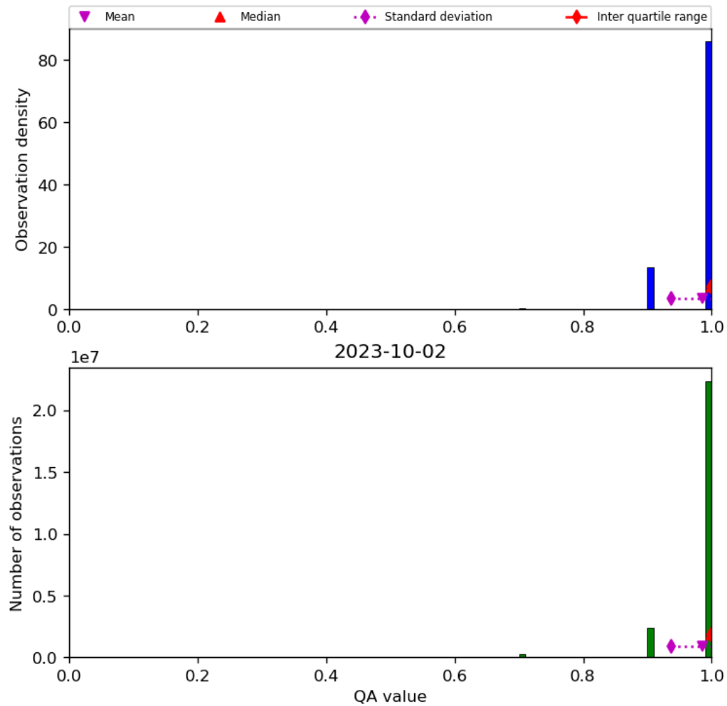
Figure 29: Histogram of “QA value” for 2023-10-01 to 2023-10-03
