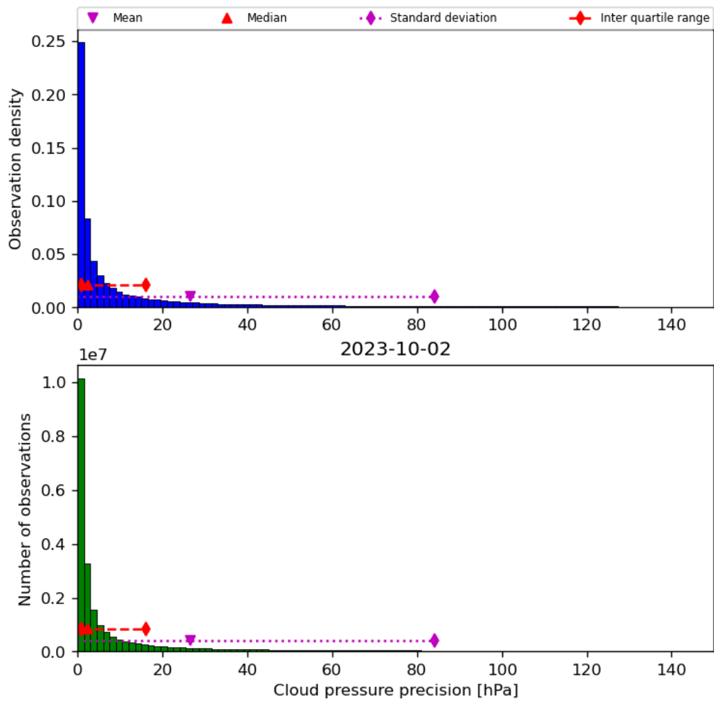
Figure 31: Histogram of “Cloud pressure precision” for 2023-10-01 to 2023-10-03
