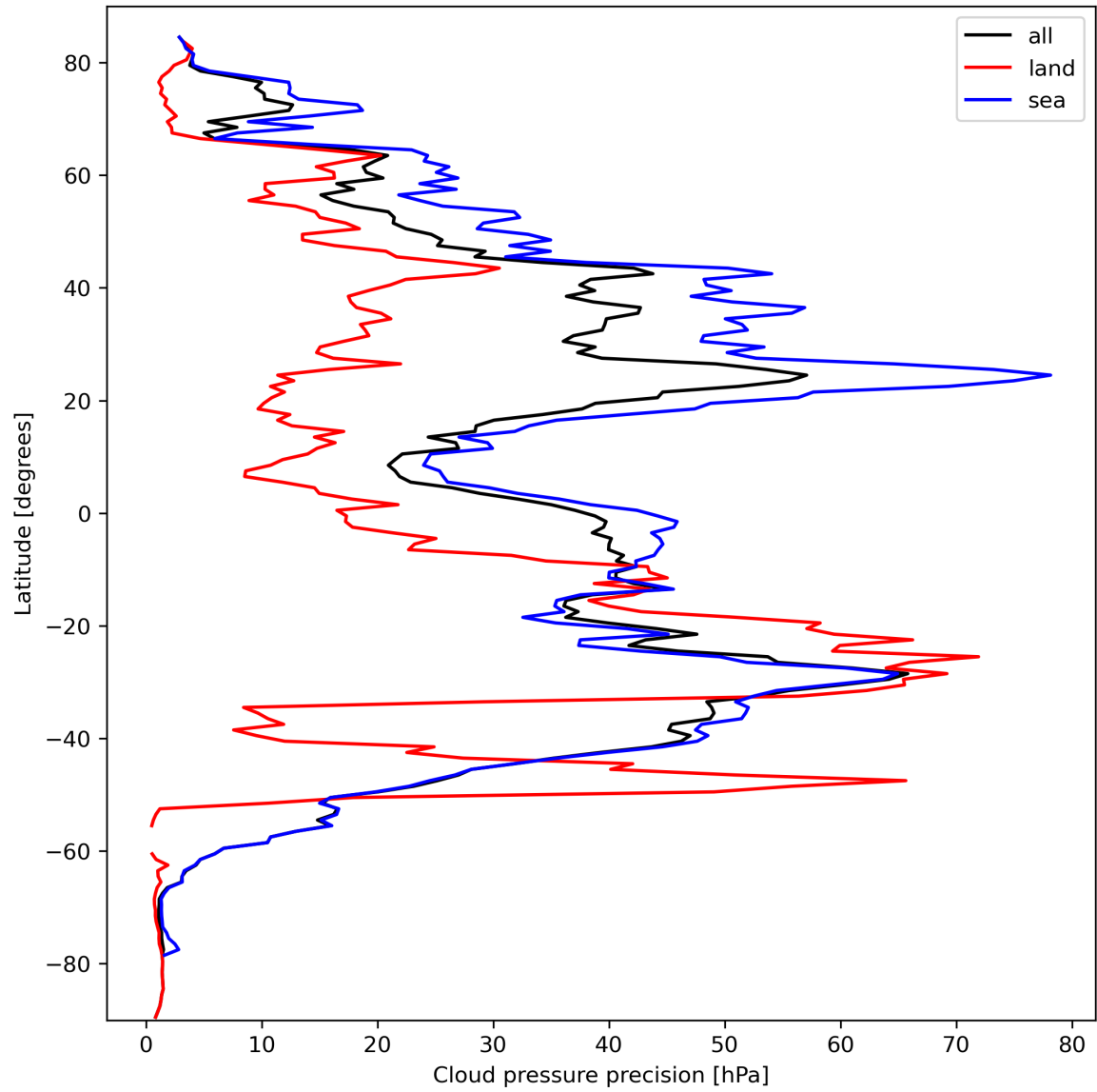
Figure 14: Zonal average of “Cloud pressure precision” for 2023-10-01 to 2023-10-03.
