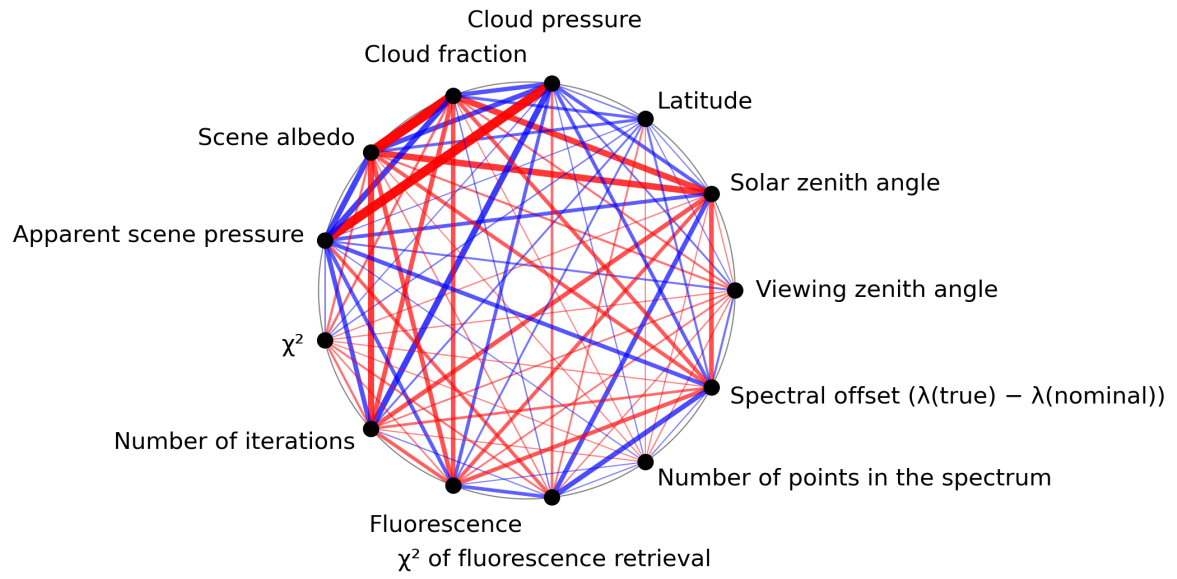
Figure 1: Map of correlation graph for 2023-10-01 to 2023-10-03.
