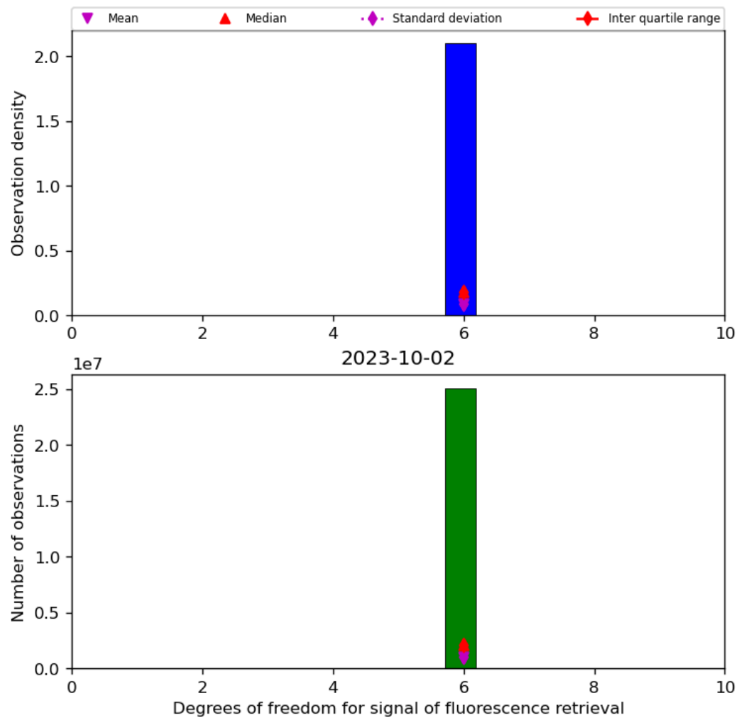
Figure 43: Histogram of “Degrees of freedom for signal of fluorescence retrieval” for 2023-10-01 to 2023-10-03
