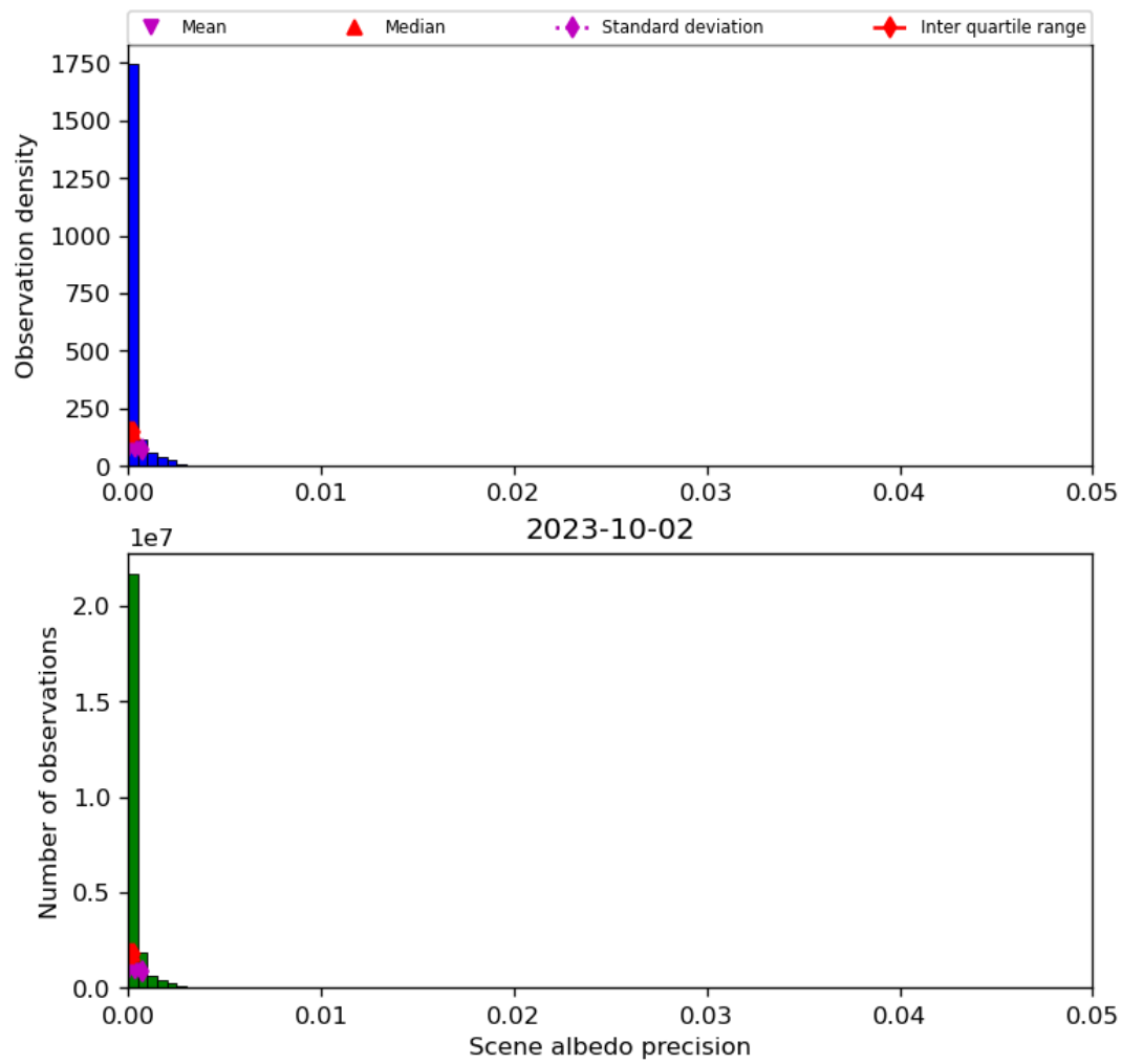
Figure 35: Histogram of “Scene albedo precision” for 2023-10-01 to 2023-10-03
