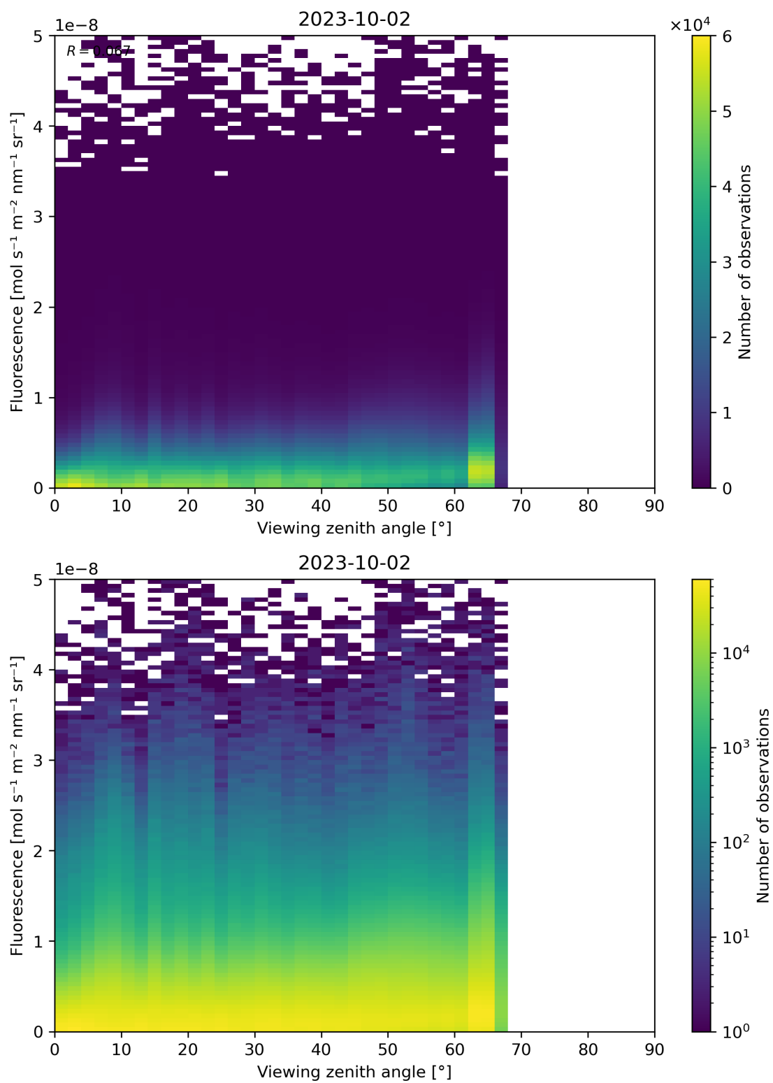
Figure 134: Scatter density plot of “Viewing zenith angle” against “Fluorescence” for 2023-10-01 to 2023-10-03.
