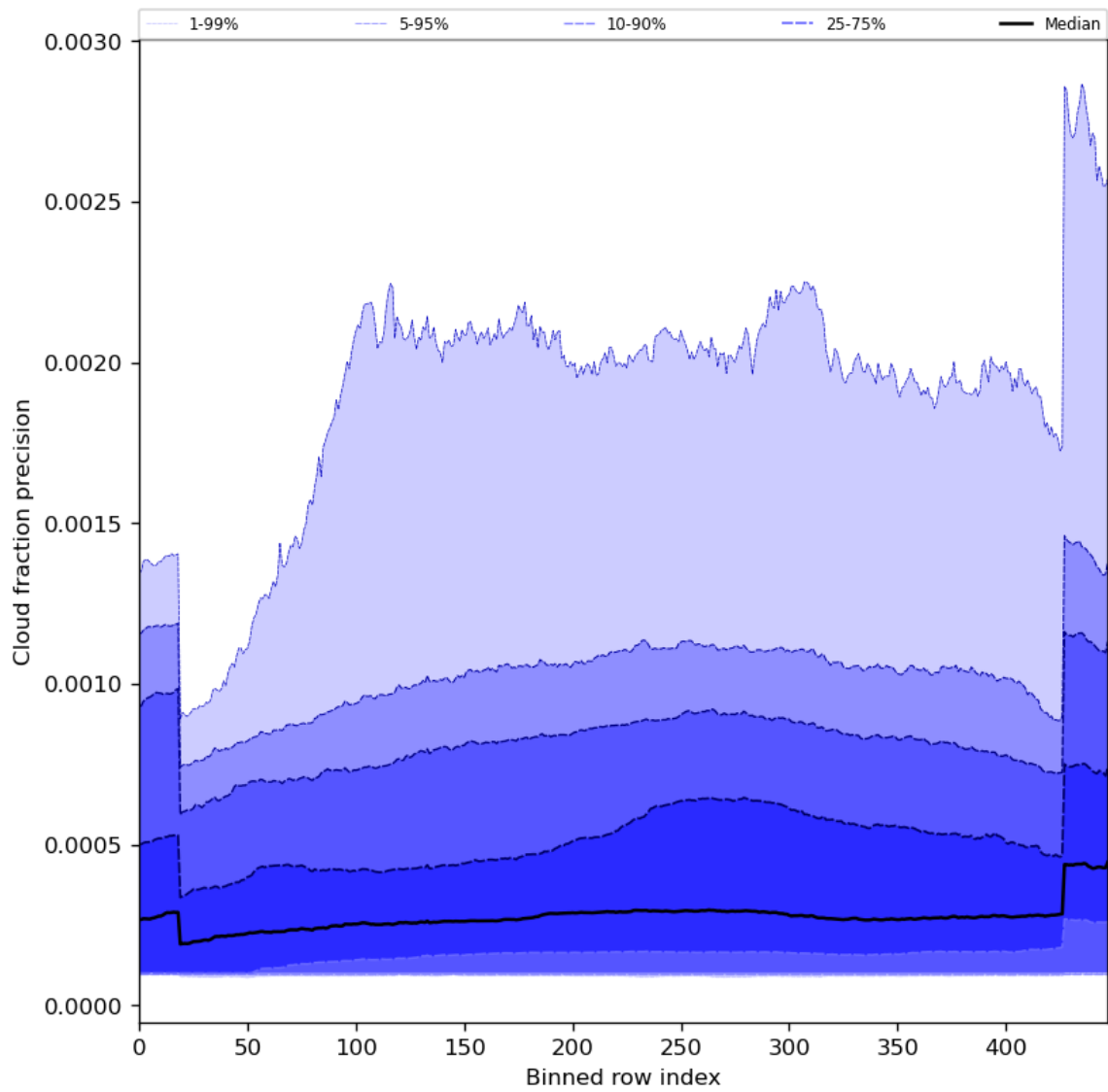
Figure 50: Along track statistics of “Cloud fraction precision” for 2023-10-01 to 2023-10-03
