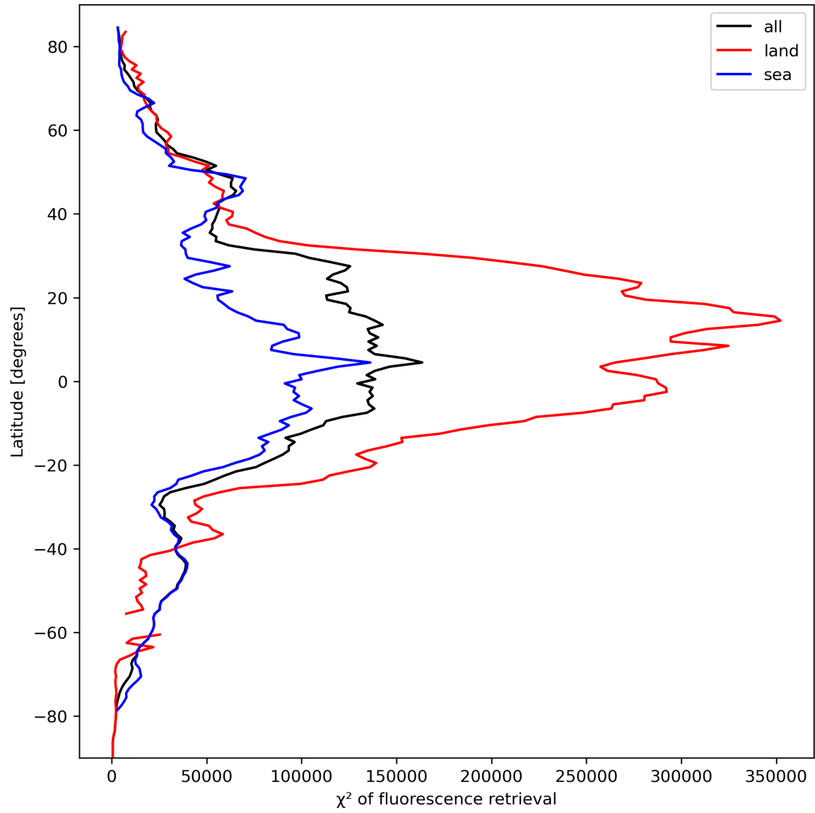
Figure 25: Zonal average of “ \chi^2 of fluorescence retrieval” for 2023-10-01 to 2023-10-03.
