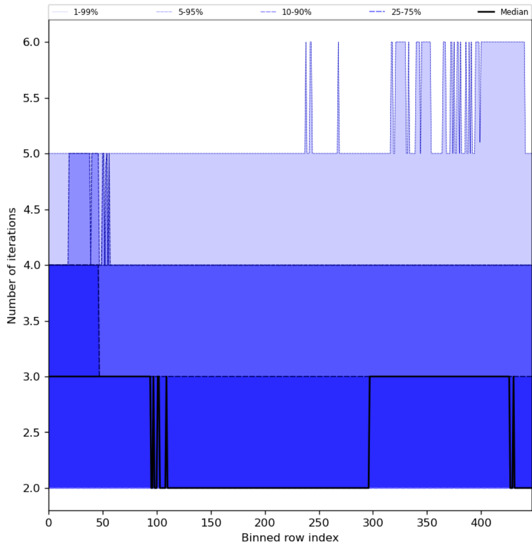
Figure 56: Along track statistics of "Number of iterations" for 2023-10-01 to 2023-10-03
