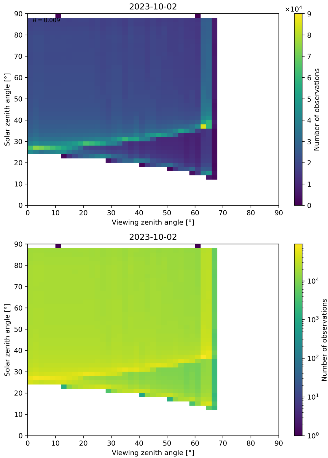
Figure 139: Scatter density plot of “Viewing zenith angle” against “Solar zenith angle” for 2023-10-01 to 2023-10-03.
