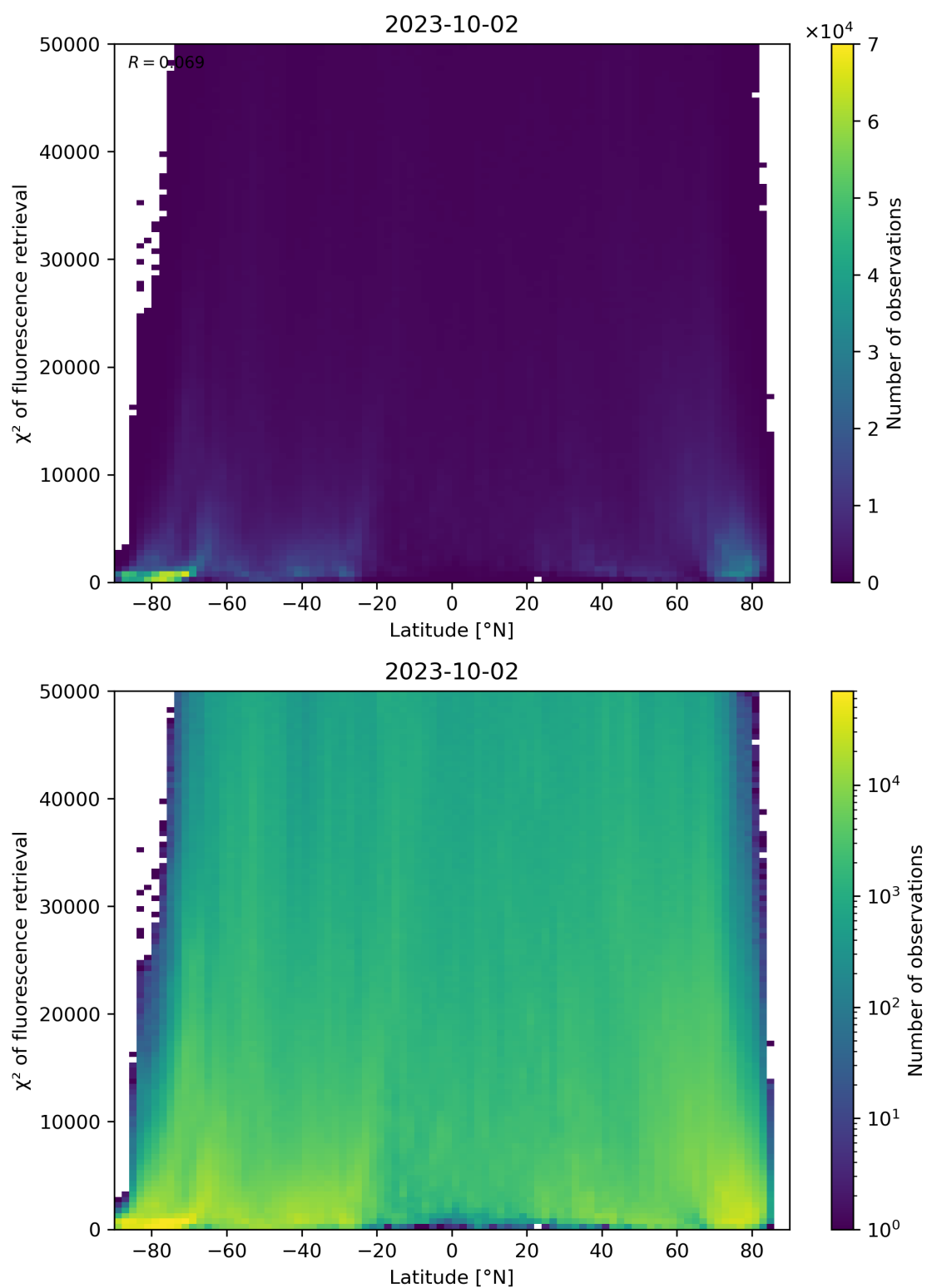
Figure 98: Scatter density plot of “Latitude” against “ \chi^2 of fluorescence retrieval” for 2023-10-01 to 2023-10-03.
