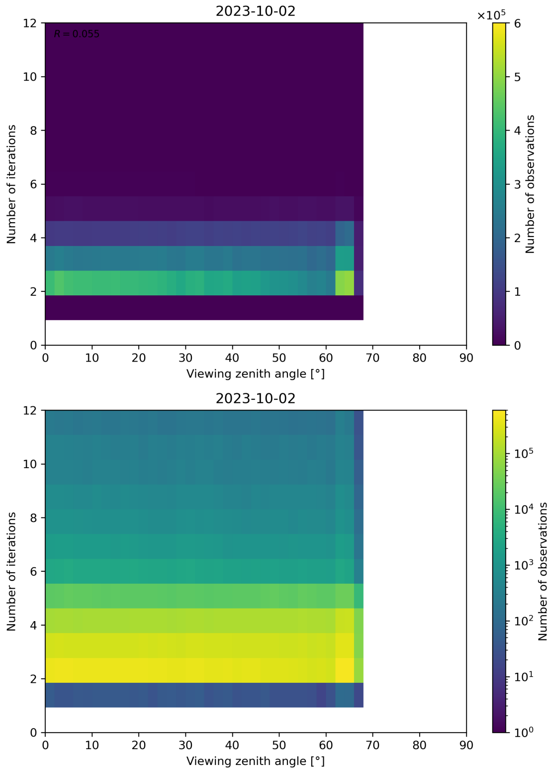
Figure 136: Scatter density plot of “Viewing zenith angle” against “Number of iterations” for 2023-10-01 to 2023-10-03.
