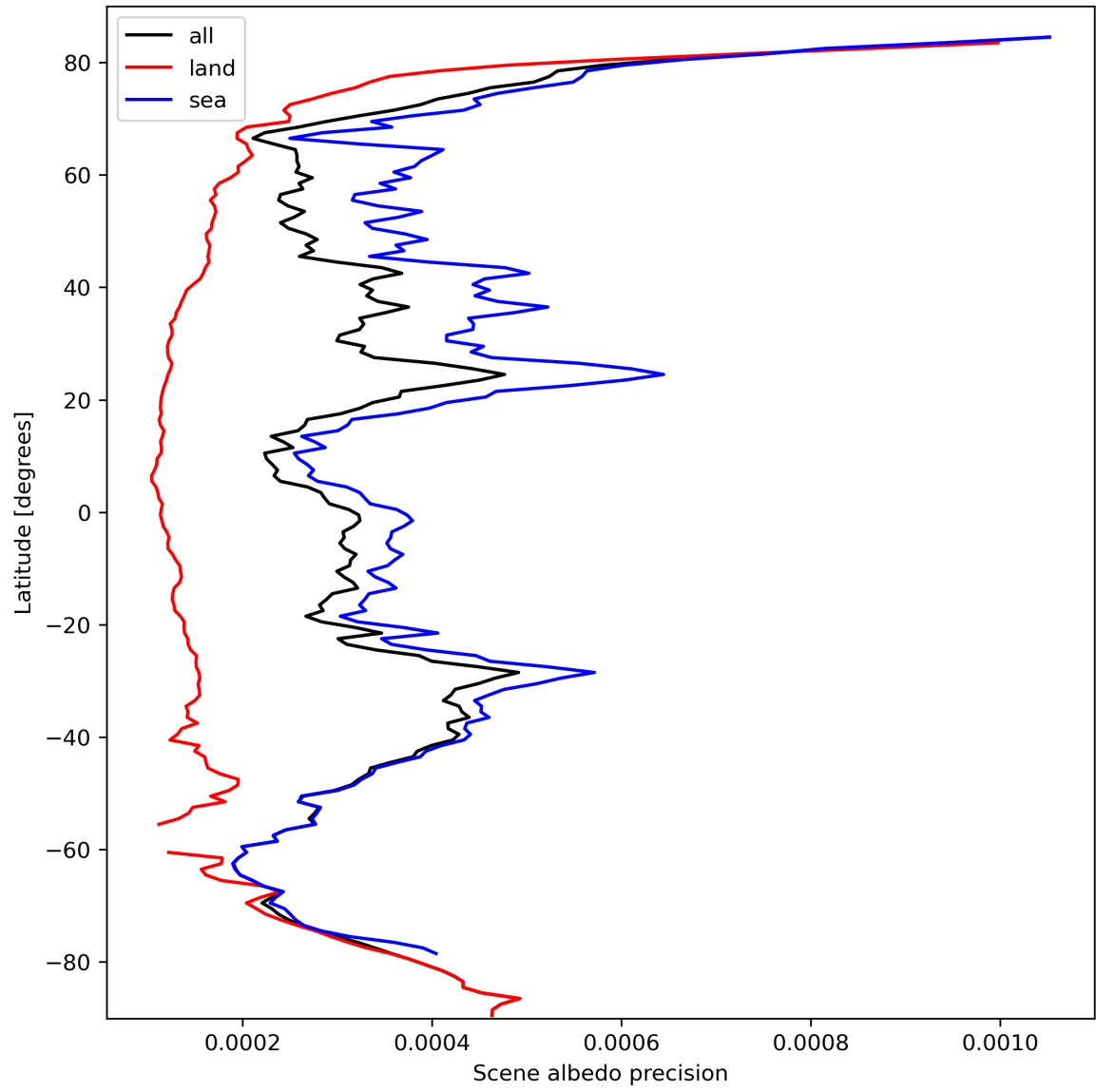
Figure 18: Zonal average of “Scene albedo precision” for 2023-10-01 to 2023-10-03.
