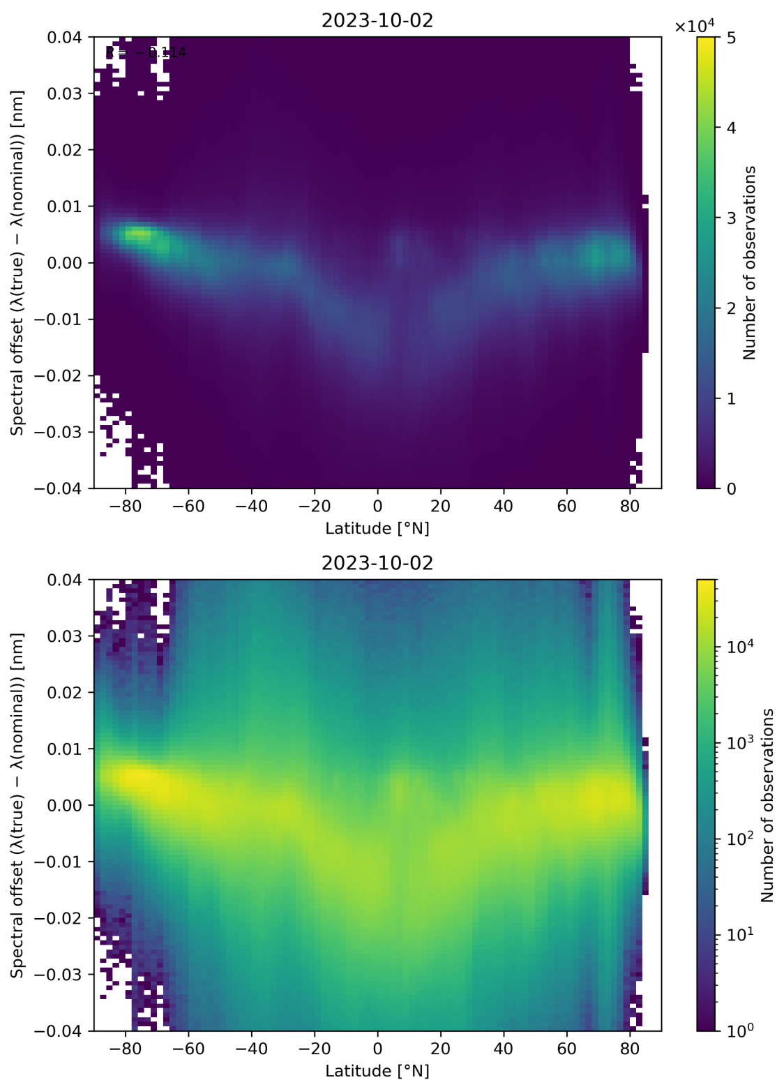
Figure 105: Scatter density plot of “Latitude” against “Spectral offset ( \lambda(\text{true}) - \lambda(\text{nominal}) )” for 2023-10-01 to 2023-10-03.
