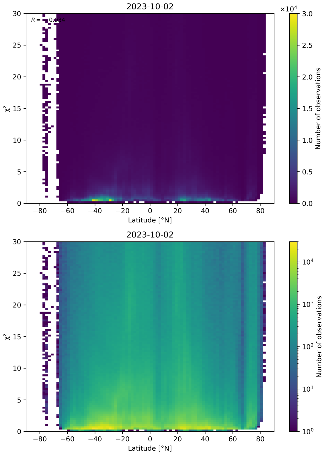
Figure 97: Scatter density plot of “Latitude” against “ \chi^2 ” for 2023-10-01 to 2023-10-03.
