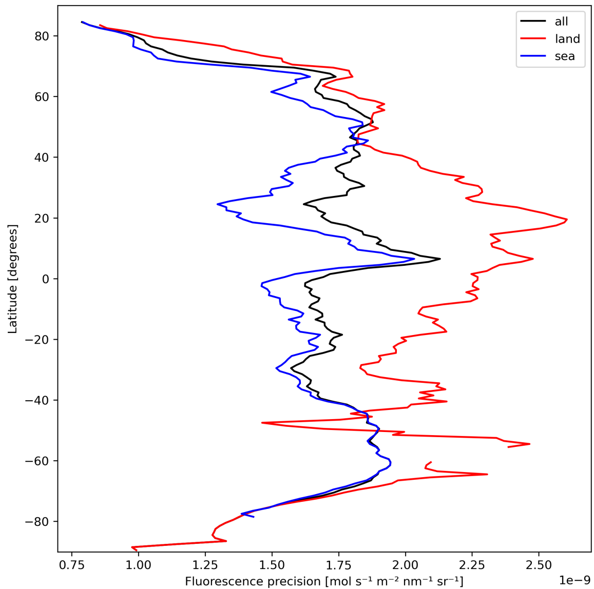
Figure 24: Zonal average of “Fluorescence precision” for 2023-10-01 to 2023-10-03.
