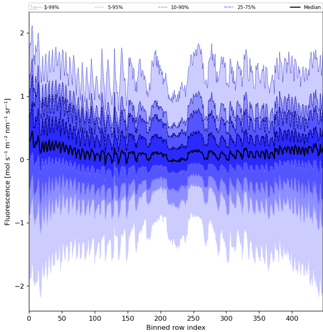
Figure 57: Along track statistics of “Fluorescence” for 2023-10-01 to 2023-10-03
