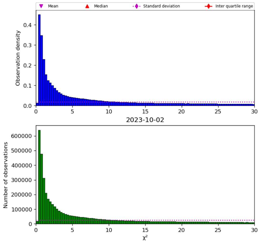
Figure 38: Histogram of “ \chi^2 ” for 2023-10-01 to 2023-10-03
