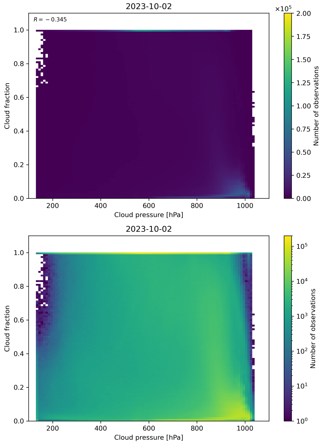
Figure 87: Scatter density plot of “Cloud pressure” against “Cloud fraction” for 2023-10-01 to 2023-10-03.
