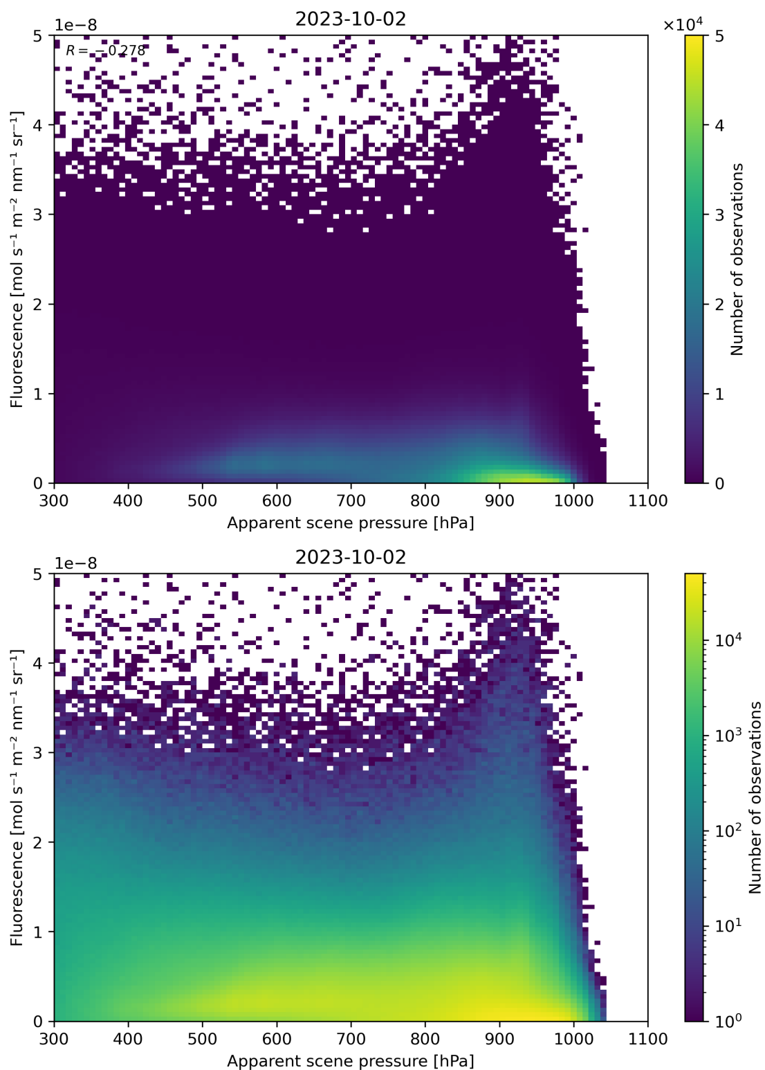
Figure 65: Scatter density plot of “Apparent scene pressure” against “Fluorescence” for 2023-10-01 to 2023-10-03.
