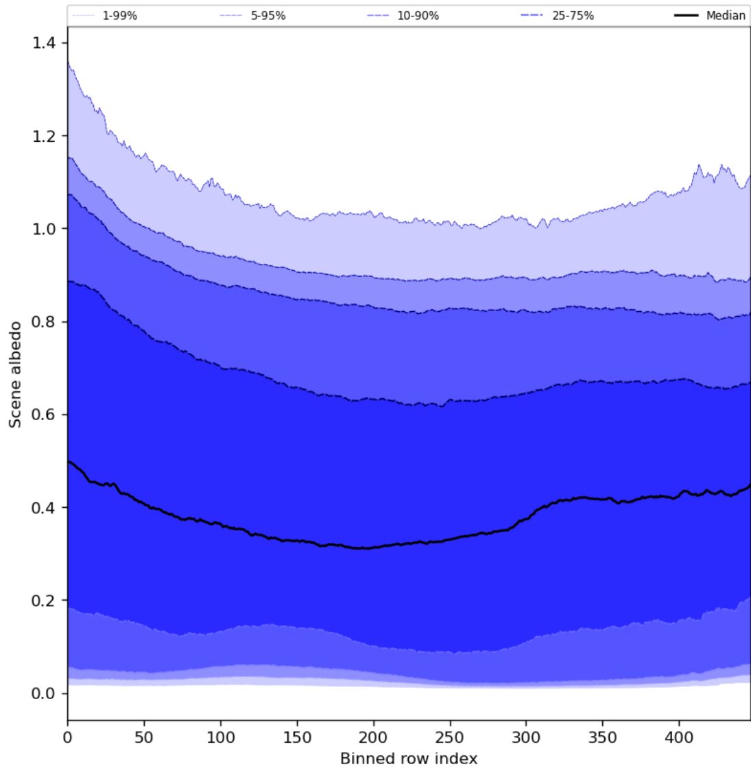
Figure 51: Along track statistics of “Scene albedo” for 2023-10-01 to 2023-10-03
