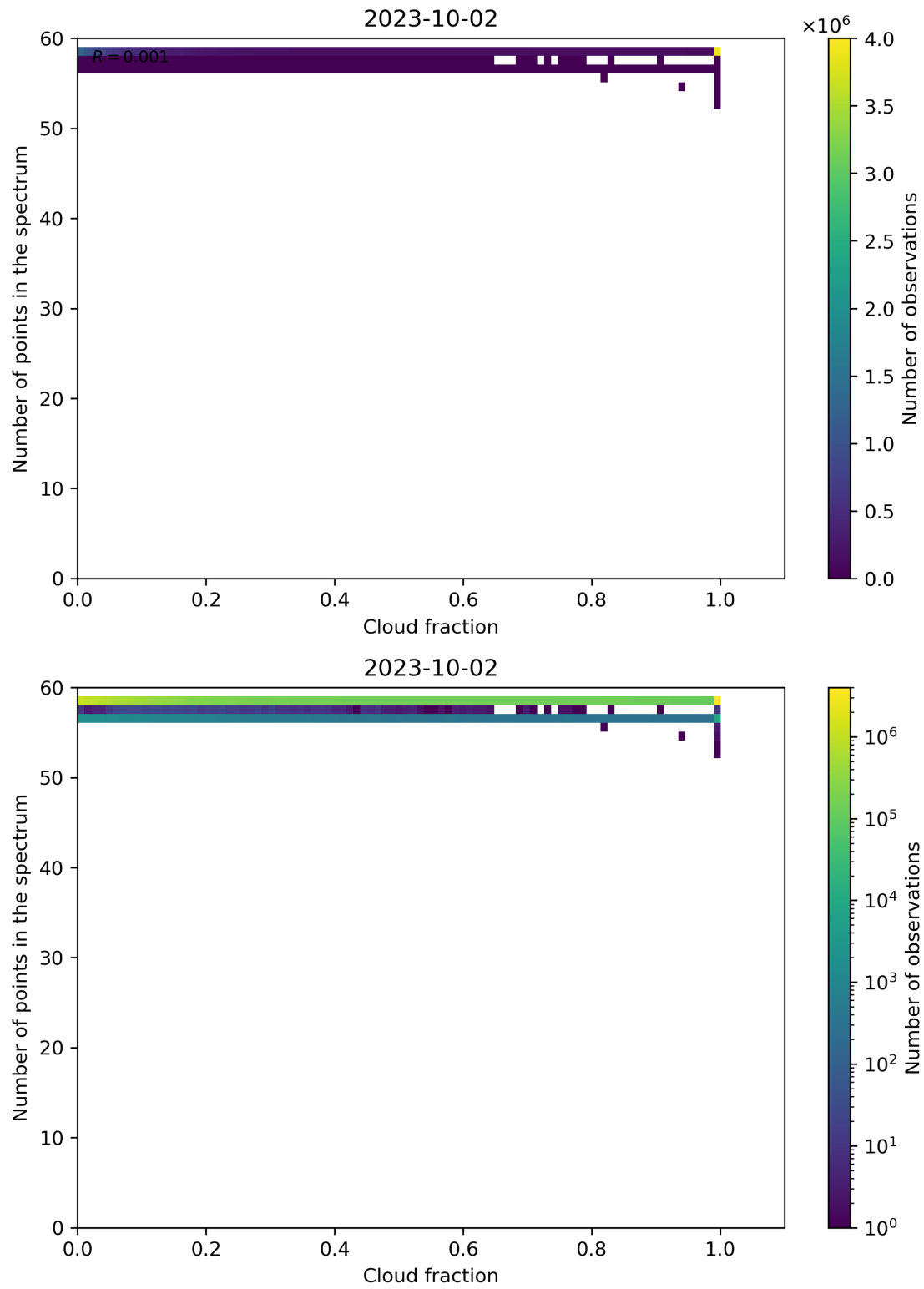
Figure 81: Scatter density plot of “Cloud fraction” against “Number of points in the spectrum” for 2023-10-01 to 2023-10-03.
