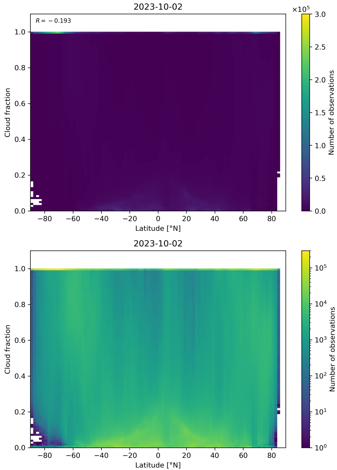
Figure 99: Scatter density plot of “Latitude” against “Cloud fraction” for 2023-10-01 to 2023-10-03.
