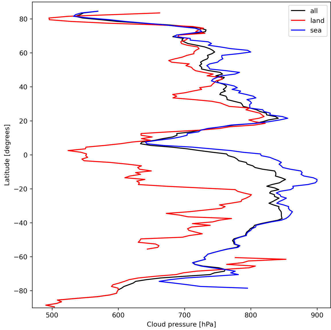
Figure 13: Zonal average of “Cloud pressure” for 2023-10-01 to 2023-10-03.
