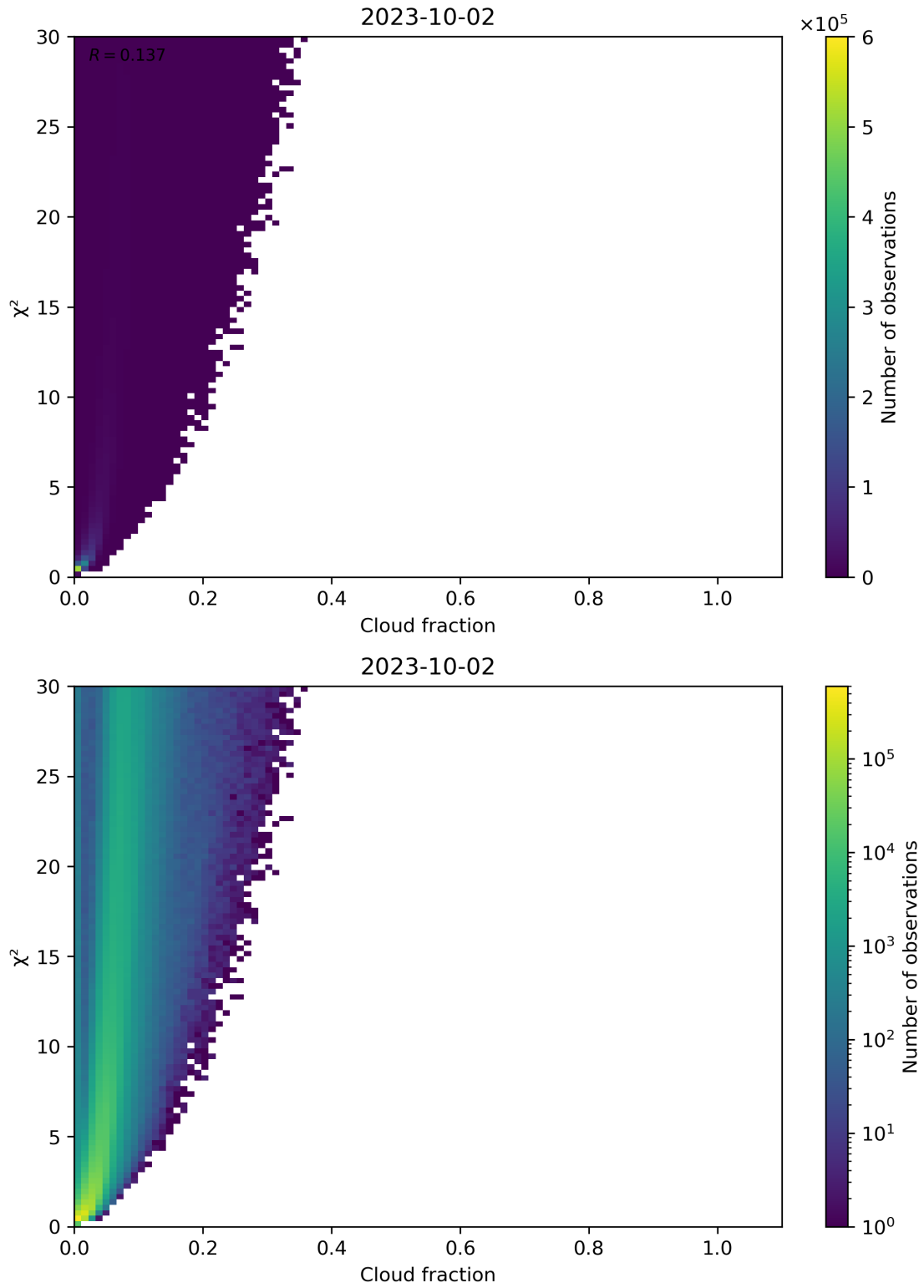
Figure 77: Scatter density plot of “Cloud fraction” against “ \chi^2 ” for 2023-10-01 to 2023-10-03.
