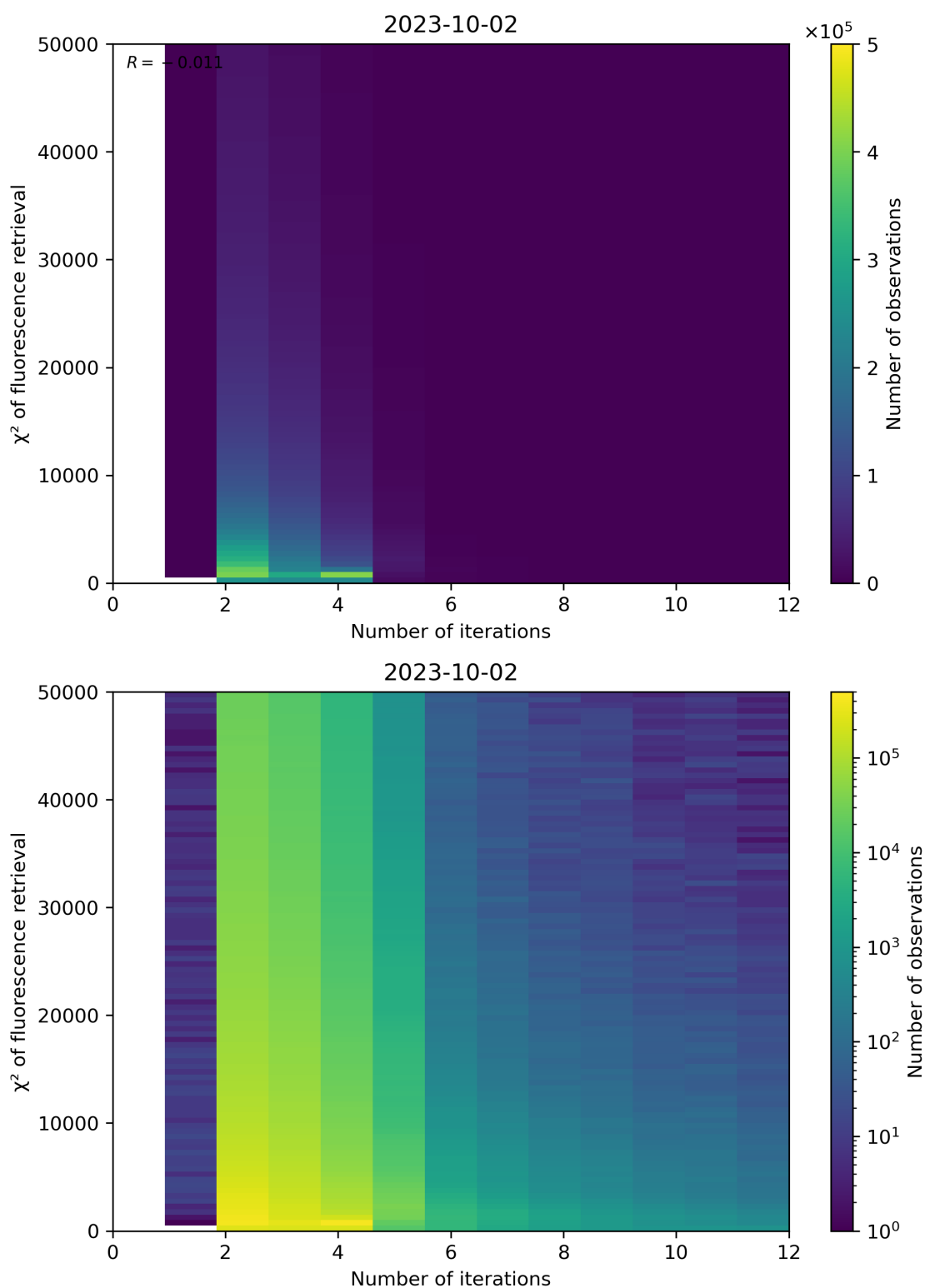
Figure 106: Scatter density plot of “Number of iterations” against “ \chi^2 of fluorescence retrieval” for 2023-10-01 to 2023-10-03.
