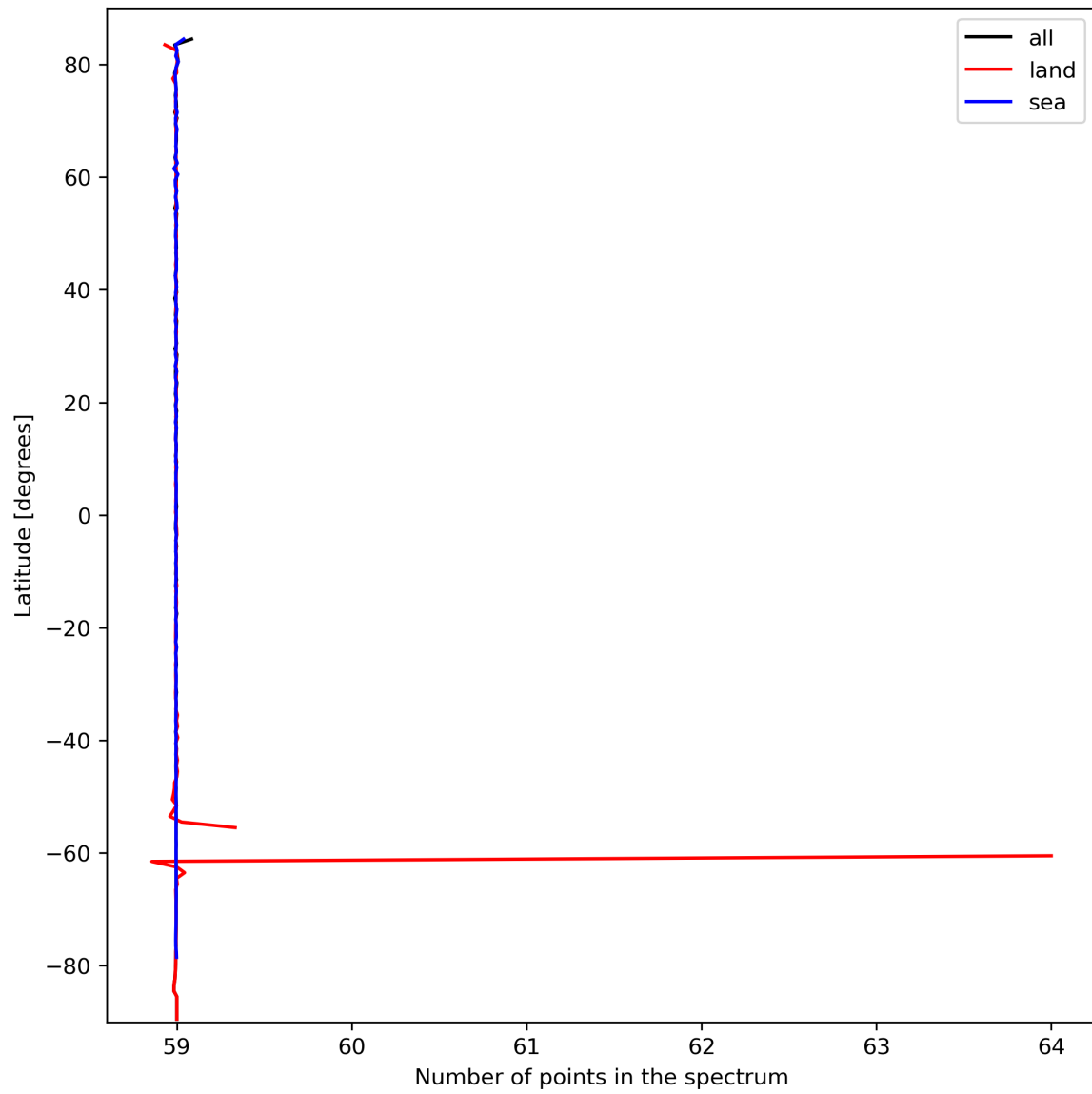
Figure 27: Zonal average of “Number of points in the spectrum” for 2023-10-01 to 2023-10-03.
