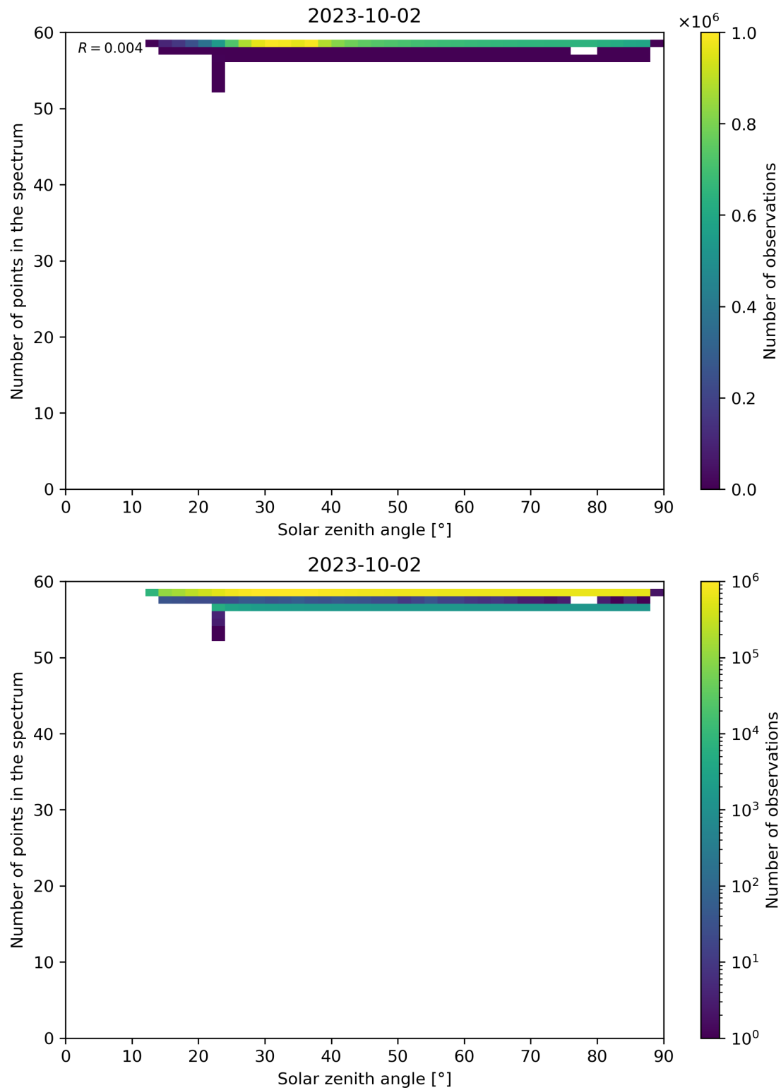
Figure 126: Scatter density plot of “Solar zenith angle” against “Number of points in the spectrum” for 2023-10-01 to 2023-10-03.
