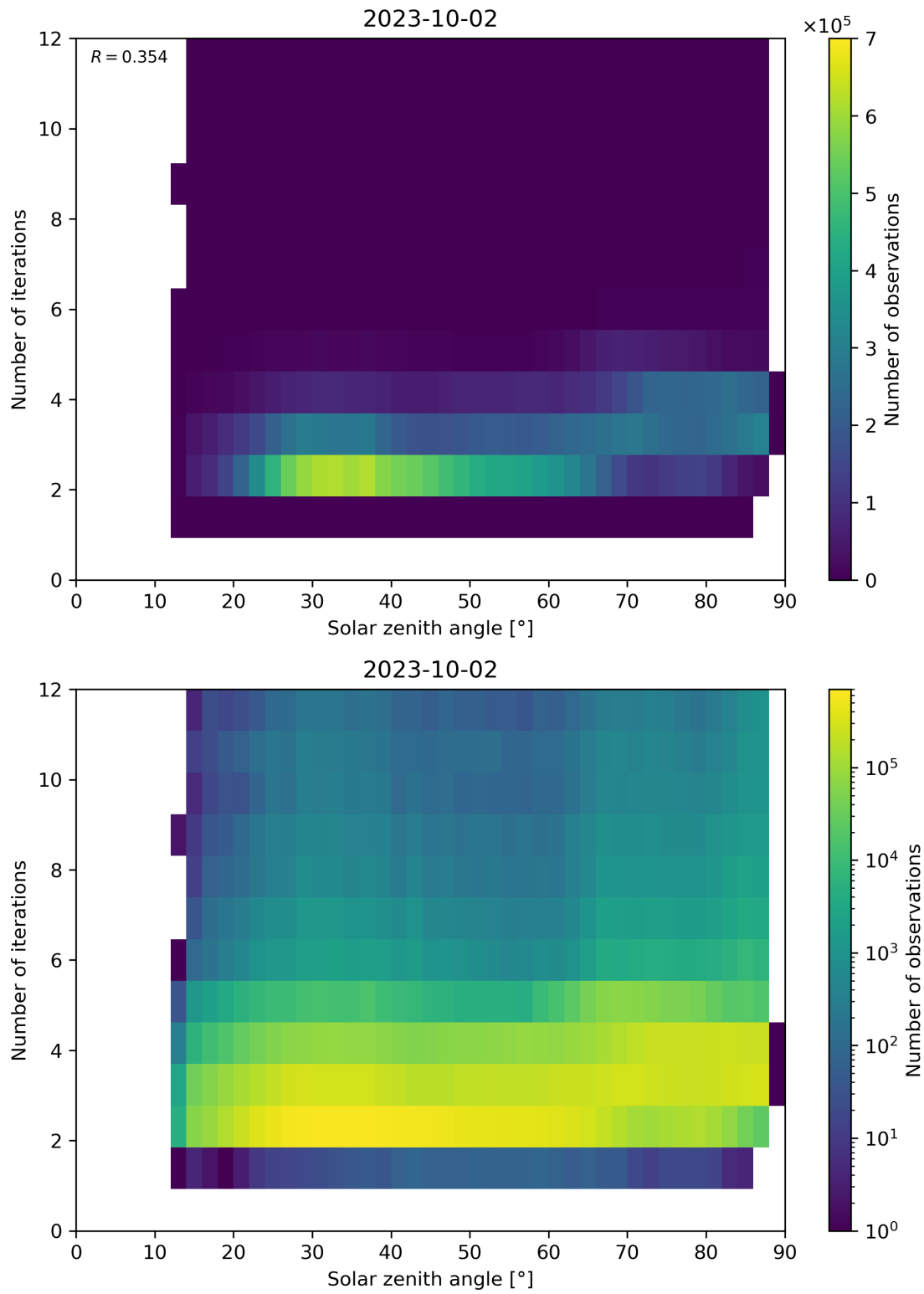
Figure 125: Scatter density plot of “Solar zenith angle” against “Number of iterations” for 2023-10-01 to 2023-10-03.
