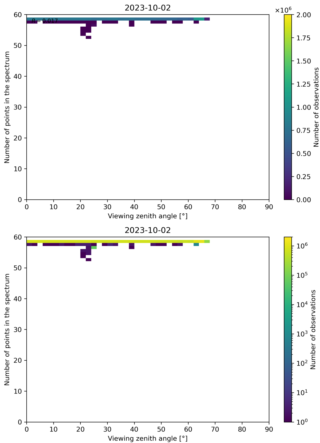
Figure 137: Scatter density plot of “Viewing zenith angle” against “Number of points in the spectrum” for 2023-10-01 to 2023-10-03.
