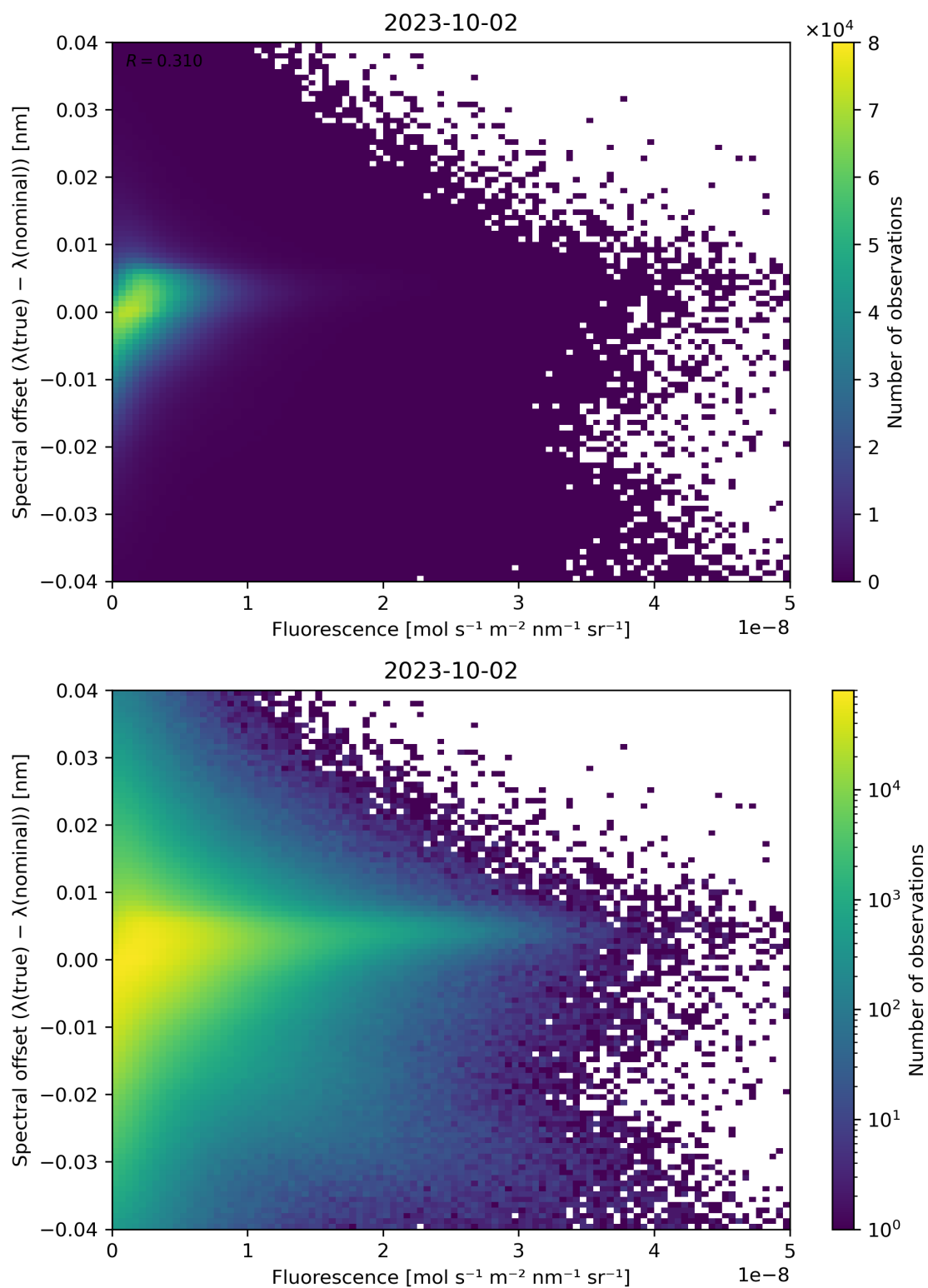
Figure 95: Scatter density plot of “Fluorescence” against “Spectral offset ( \lambda(\text{true}) - \lambda(\text{nominal}) )” for 2023-10-01 to 2023-10-03.
