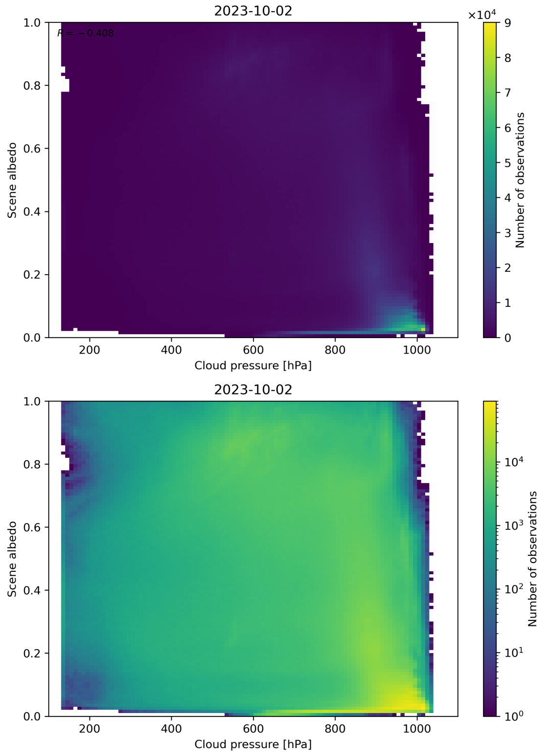
Figure 91: Scatter density plot of “Cloud pressure” against “Scene albedo” for 2023-10-01 to 2023-10-03.
