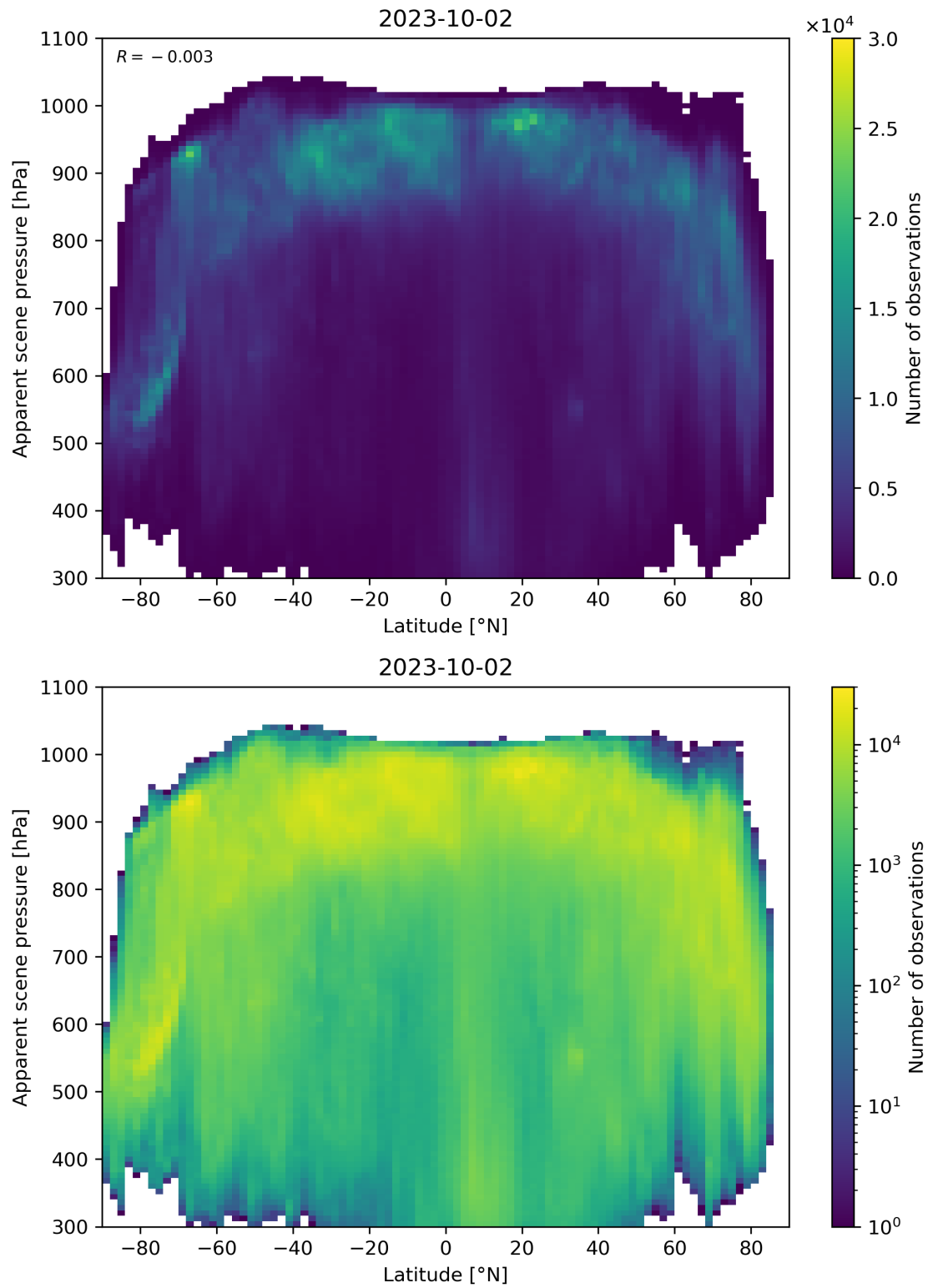
Figure 96: Scatter density plot of “Latitude” against “Apparent scene pressure” for 2023-10-01 to 2023-10-03.
