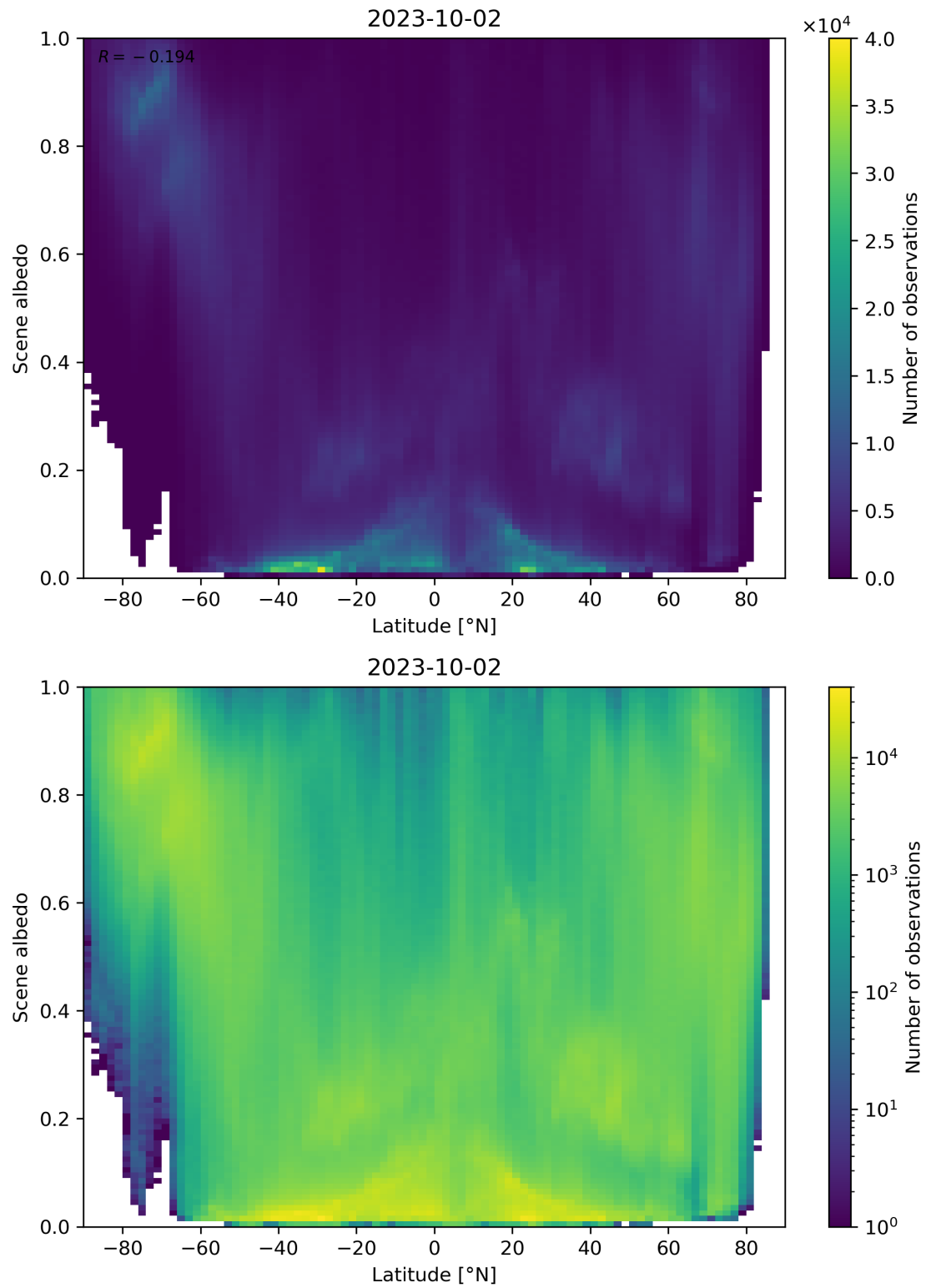
Figure 104: Scatter density plot of “Latitude” against “Scene albedo” for 2023-10-01 to 2023-10-03.
