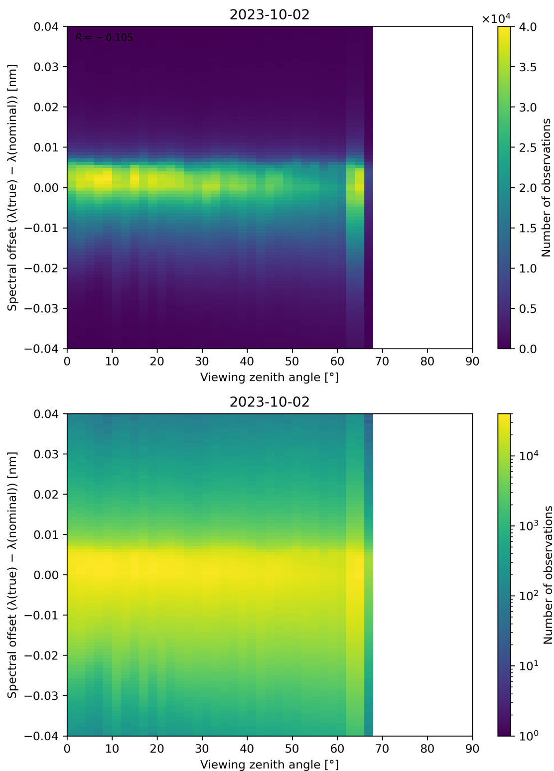
Figure 140: Scatter density plot of “Viewing zenith angle” against “Spectral offset ( \lambda(\text{true}) - \lambda(\text{nominal}) )” for 2023-10-01 to 2023-10-03.
