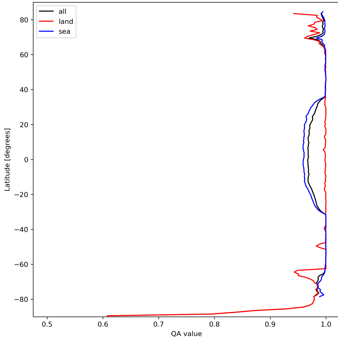
Figure 12: Zonal average of “QA value” for 2023-10-01 to 2023-10-03.
