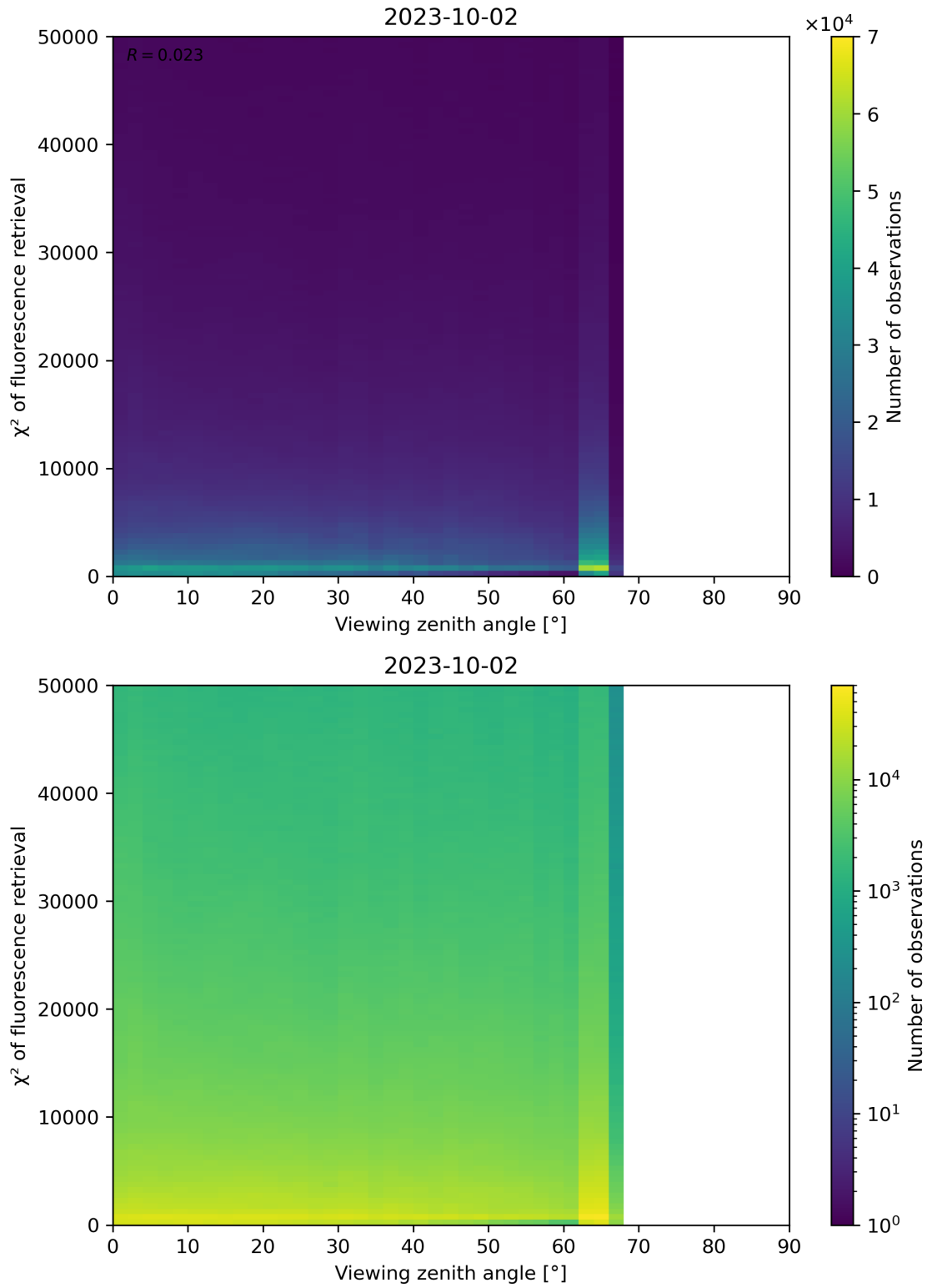
Figure 131: Scatter density plot of “Viewing zenith angle” against “ \chi^2 of fluorescence retrieval” for 2023-10-01 to 2023-10-03.
