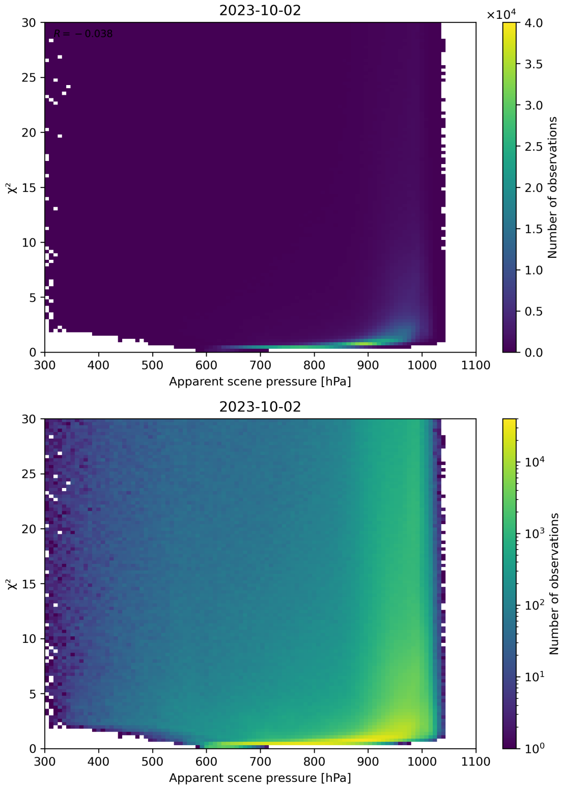
Figure 63: Scatter density plot of “Apparent scene pressure” against “ \chi^2 ” for 2023-10-01 to 2023-10-03.
