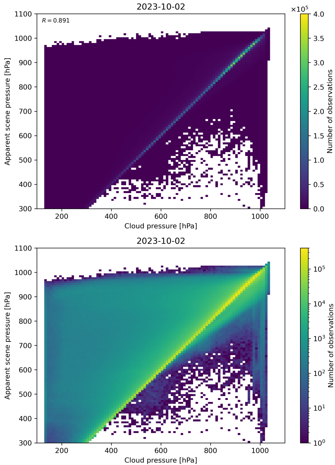
Figure 84: Scatter density plot of “Cloud pressure” against “Apparent scene pressure” for 2023-10-01 to 2023-10-03.
