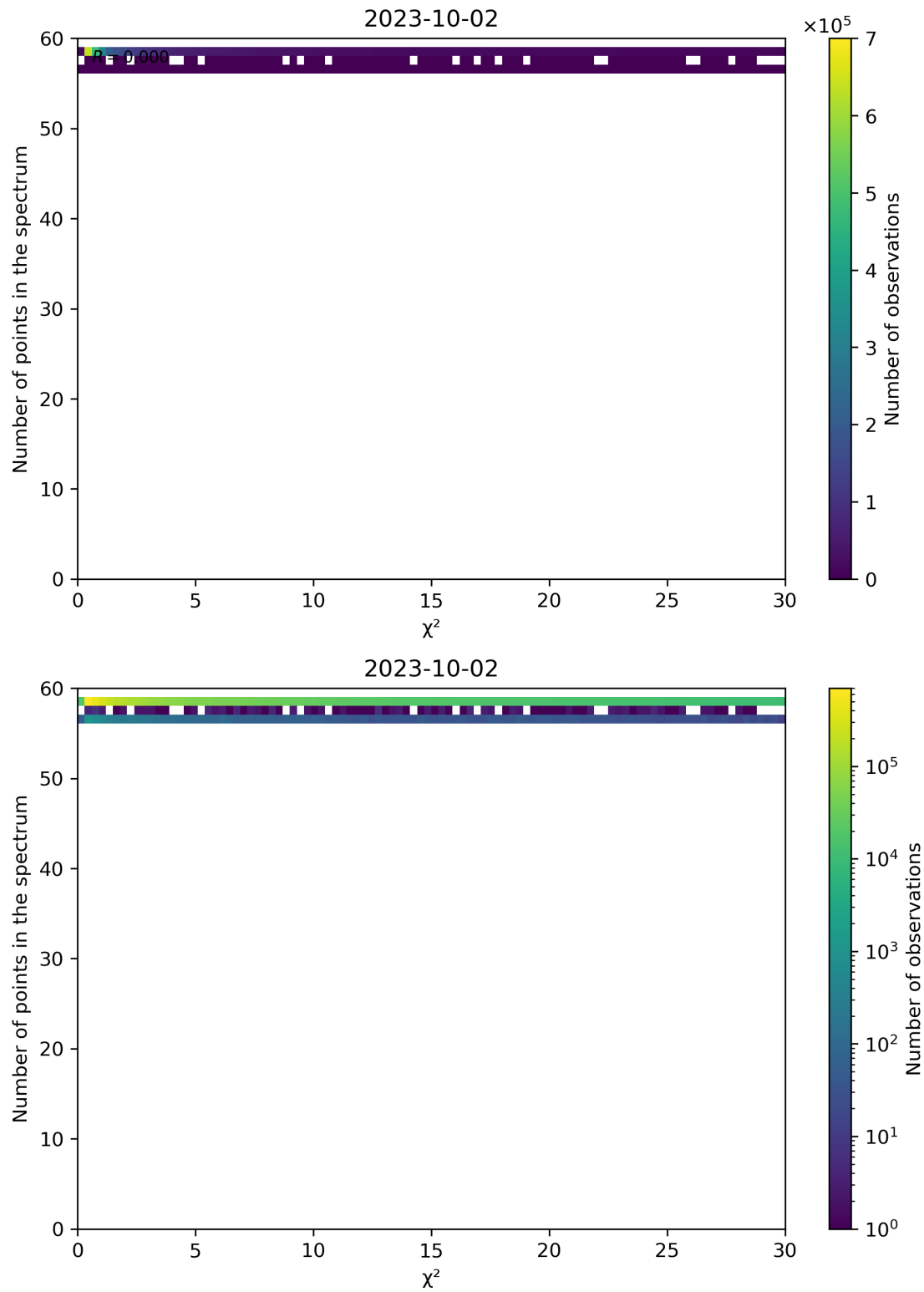
Figure 74: Scatter density plot of " \chi^2 " against "Number of points in the spectrum" for 2023-10-01 to 2023-10-03.
