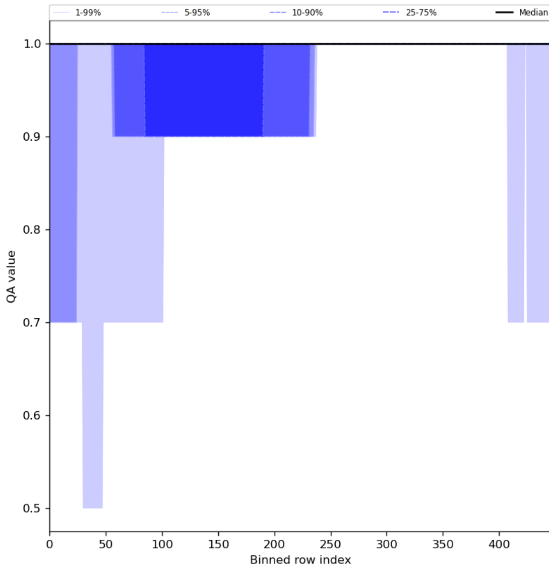
Figure 46: Along track statistics of “QA value” for 2023-10-01 to 2023-10-03
