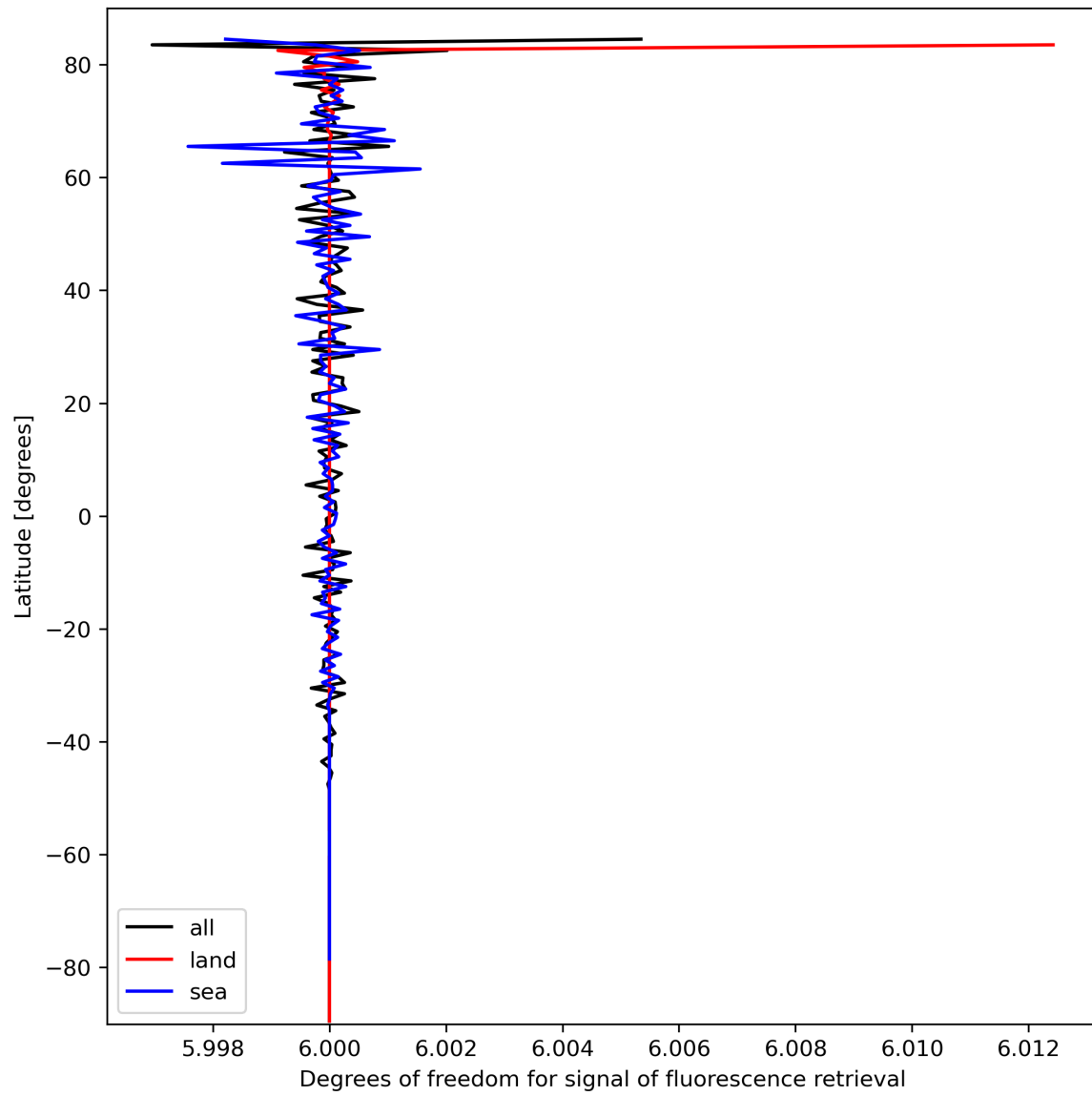
Figure 26: Zonal average of “Degrees of freedom for signal of fluorescence retrieval” for 2023-10-01 to 2023-10-03.
