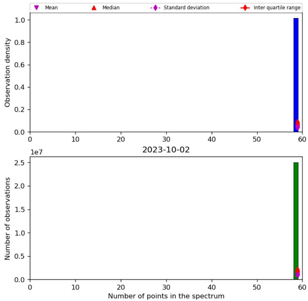
Figure 44: Histogram of “Number of points in the spectrum” for 2023-10-01 to 2023-10-03
