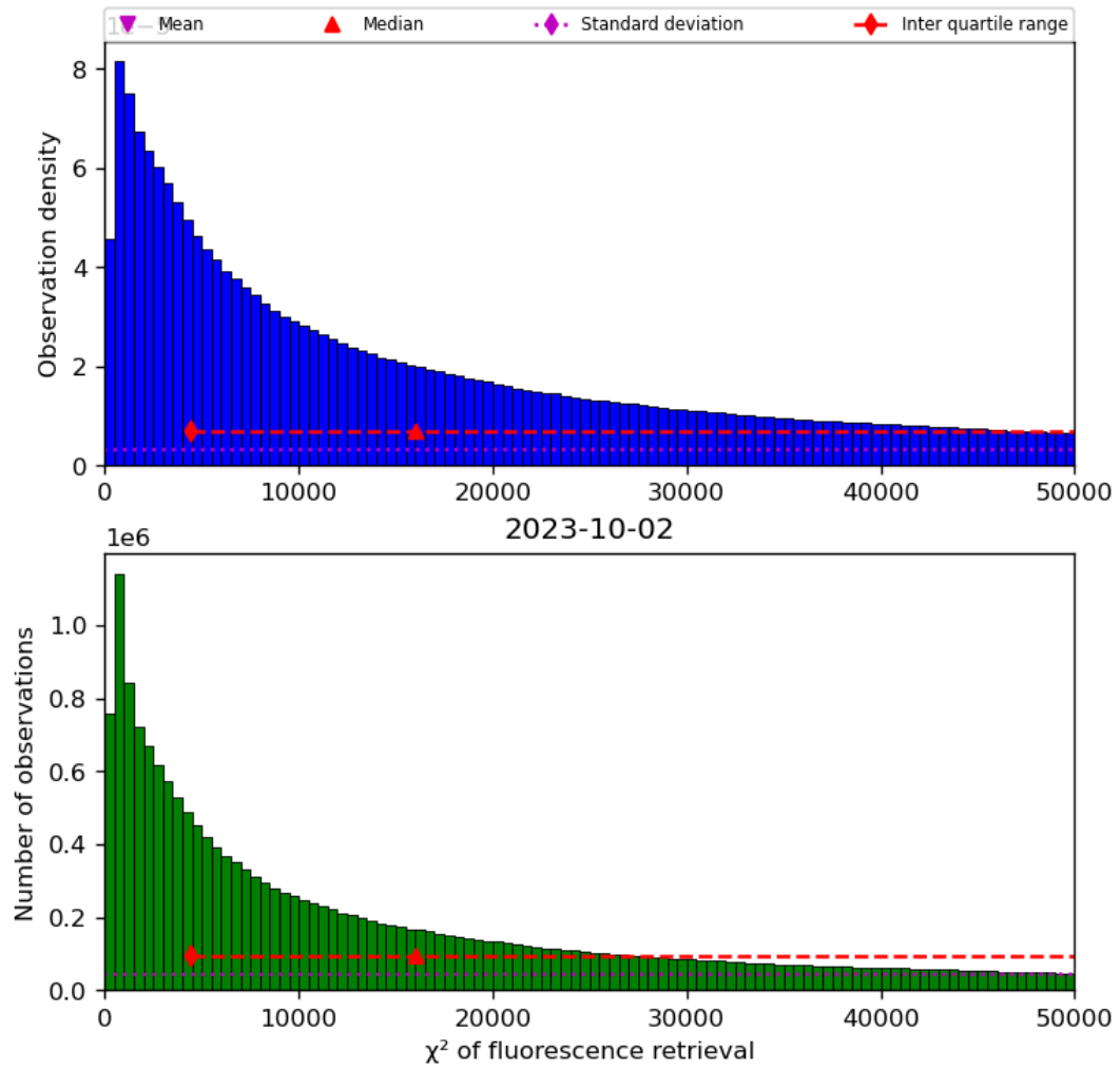
Figure 42: Histogram of “ \chi^2 of fluorescence retrieval” for 2023-10-01 to 2023-10-03
