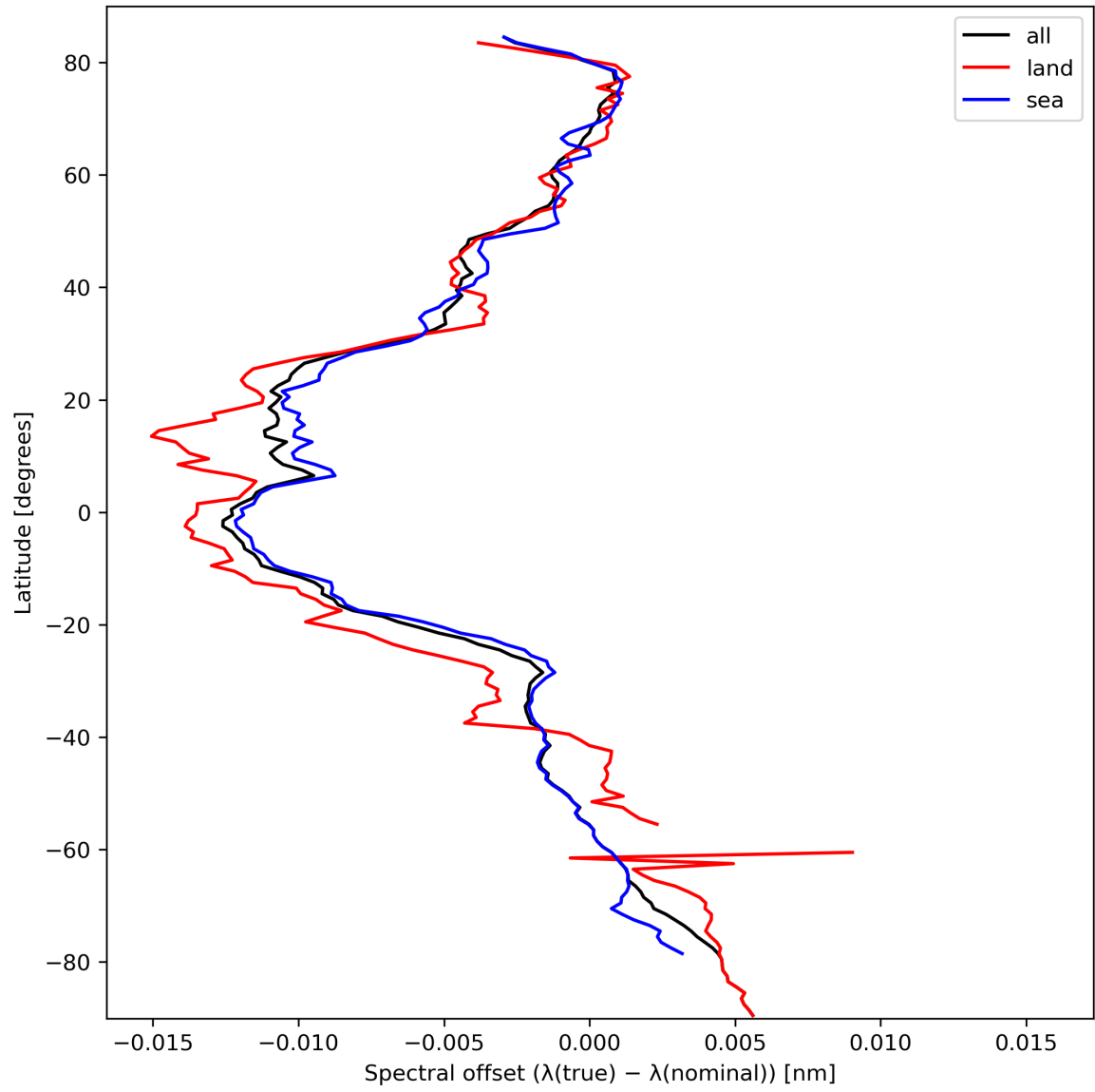
Figure 28: Zonal average of “Spectral offset ( \lambda(\text{true}) - \lambda(\text{nominal}) )” for 2023-10-01 to 2023-10-03.
