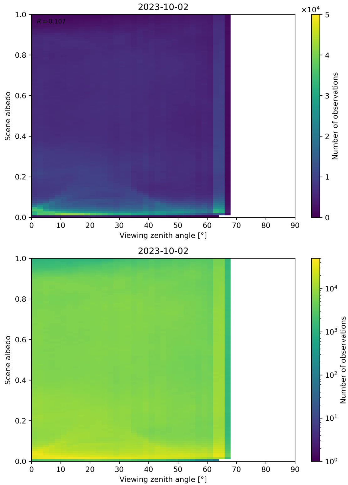
Figure 138: Scatter density plot of “Viewing zenith angle” against “Scene albedo” for 2023-10-01 to 2023-10-03.
