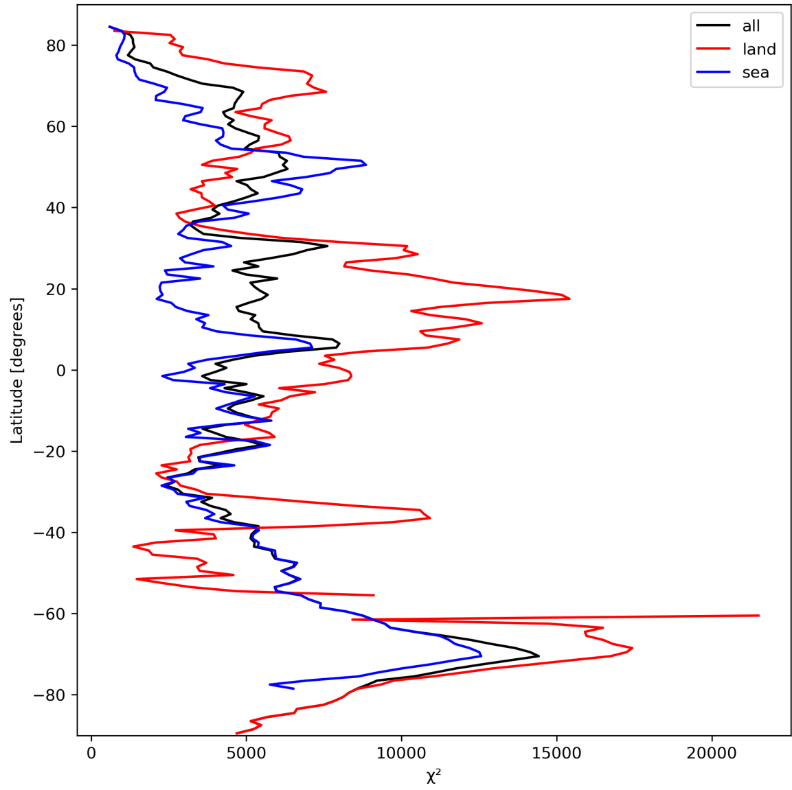
Figure 21: Zonal average of “ \chi^2 ” for 2023-10-02 to 2023-10-04.
