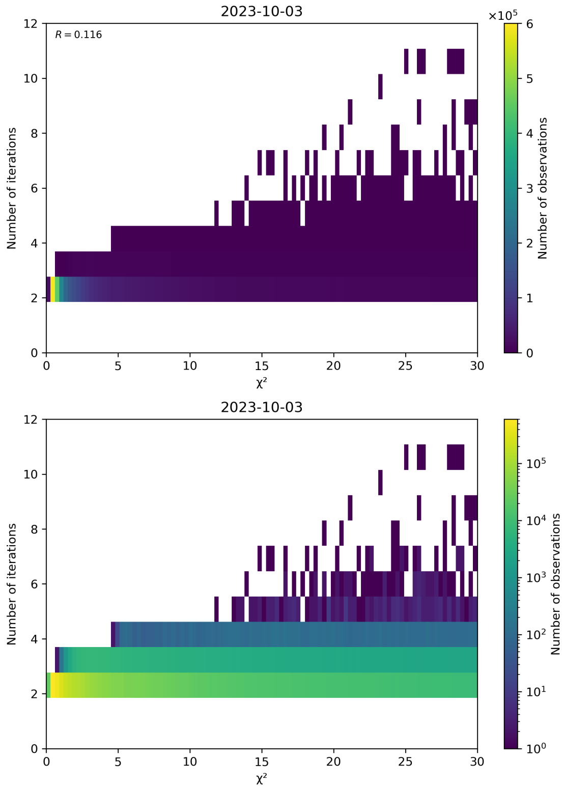
Figure 73: Scatter density plot of “ \chi^2 ” against “Number of iterations” for 2023-10-02 to 2023-10-04.
