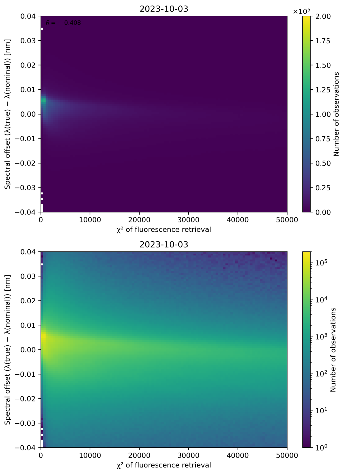
Figure 72: Scatter density plot of " \chi^2 of fluorescence retrieval" against "Spectral offset ( \lambda(\text{true}) - \lambda(\text{nominal}) )" for 2023-10-02 to 2023-10-04.
