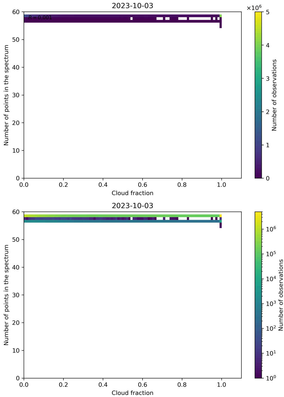
Figure 81: Scatter density plot of “Cloud fraction” against “Number of points in the spectrum” for 2023-10-02 to 2023-10-04.
