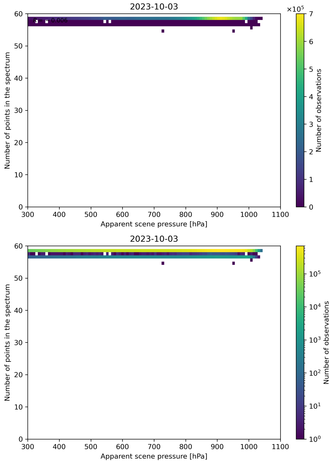
Figure 67: Scatter density plot of “Apparent scene pressure” against “Number of points in the spectrum” for 2023-10-02 to 2023-10-04.
