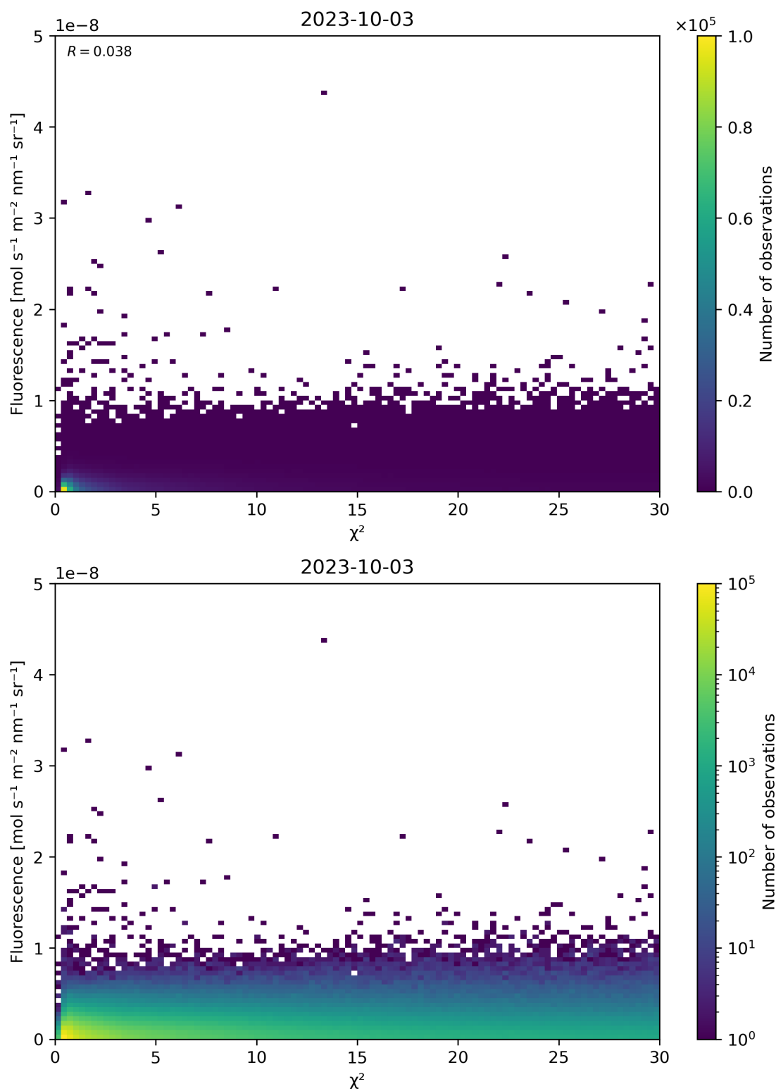
Figure 70: Scatter density plot of “ \chi^2 ” against “Fluorescence” for 2023-10-02 to 2023-10-04.
