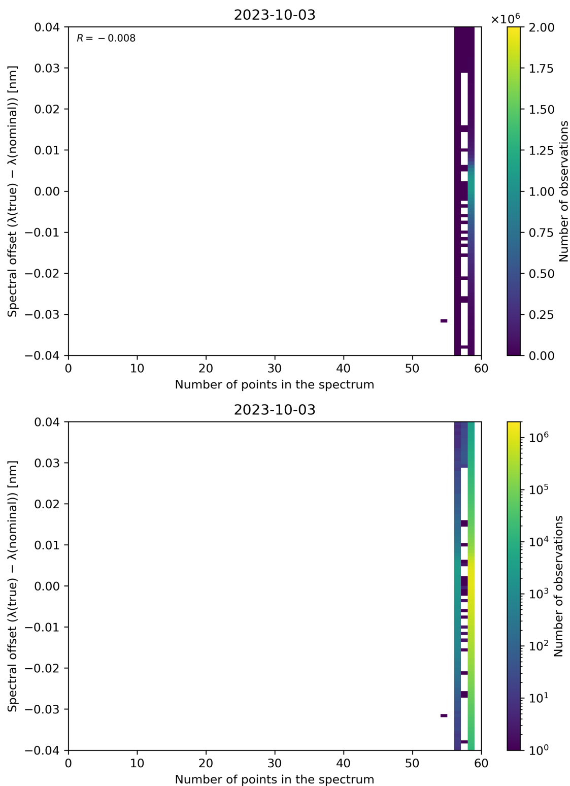
Figure 110: Scatter density plot of “Number of points in the spectrum” against “Spectral offset ( \lambda(\text{true}) - \lambda(\text{nominal}) )” for 2023-10-02 to 2023-10-04.
