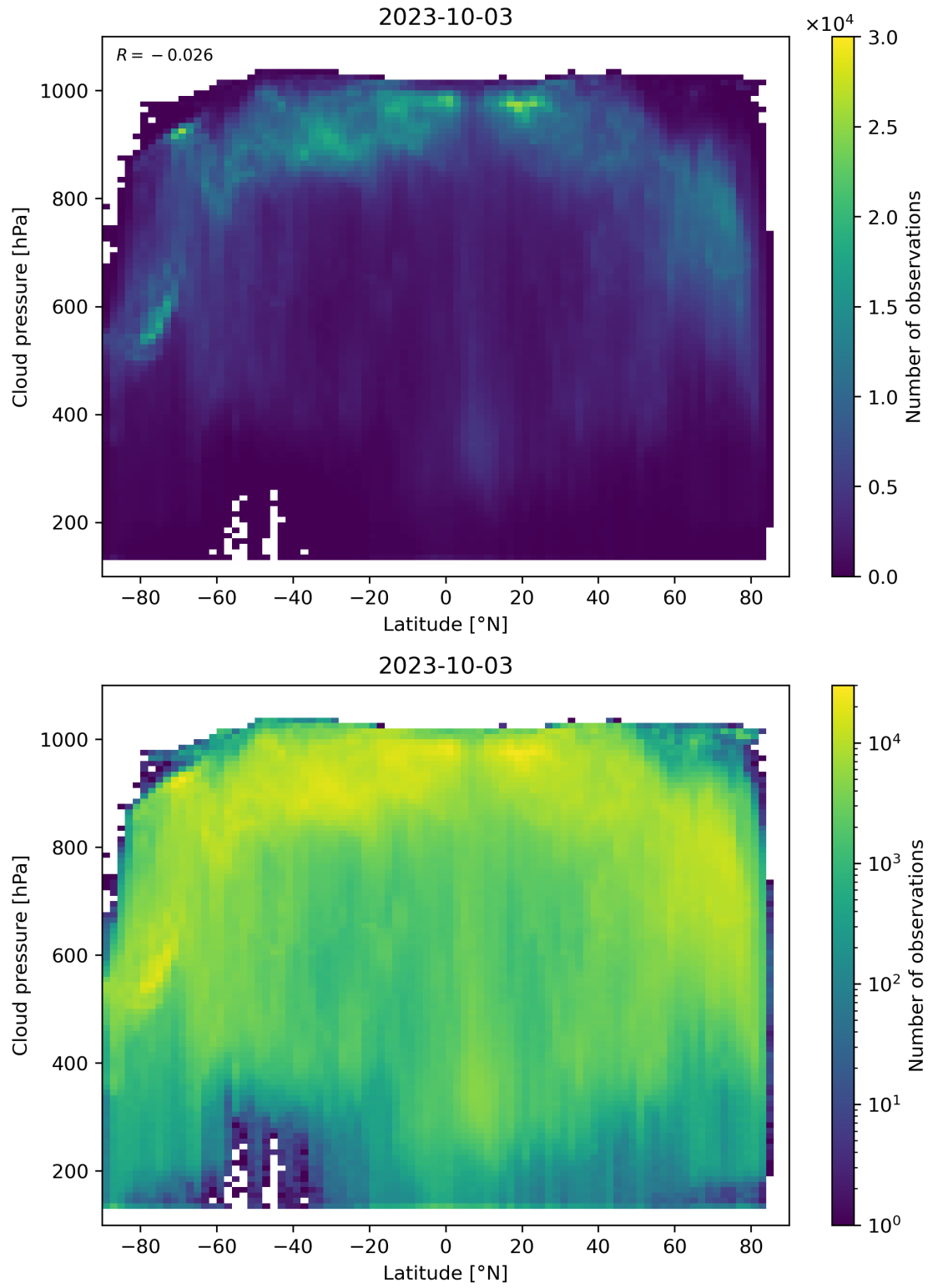
Figure 100: Scatter density plot of “Latitude” against “Cloud pressure” for 2023-10-02 to 2023-10-04.
