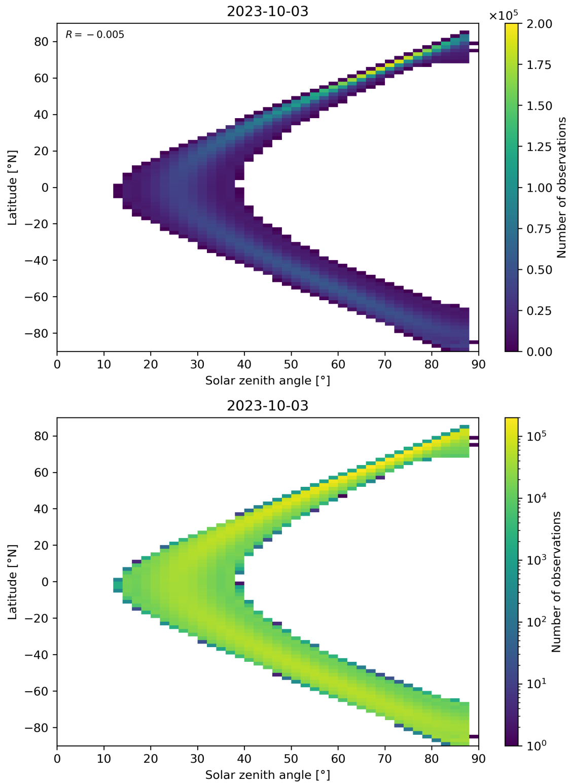
Figure 124: Scatter density plot of “Solar zenith angle” against “Latitude” for 2023-10-02 to 2023-10-04.
