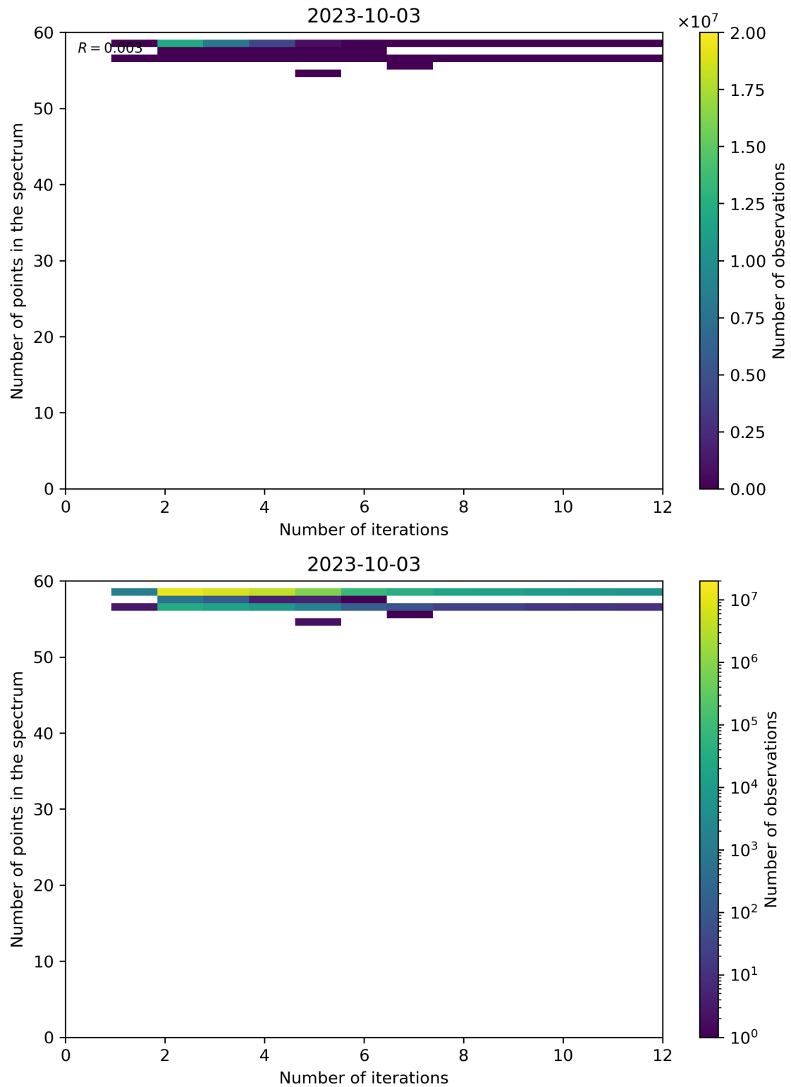
Figure 108: Scatter density plot of “Number of iterations” against “Number of points in the spectrum” for 2023-10-02 to 2023-10-04.
