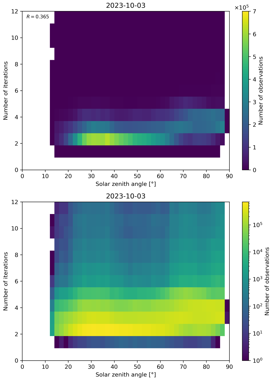
Figure 125: Scatter density plot of “Solar zenith angle” against “Number of iterations” for 2023-10-02 to 2023-10-04.
