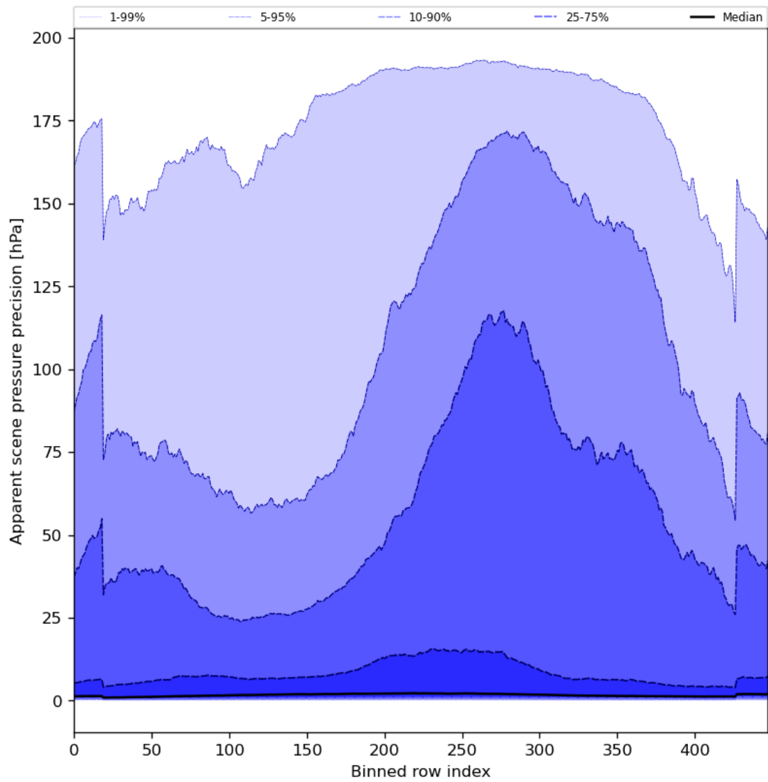
Figure 54: Along track statistics of “Apparent scene pressure precision” for 2023-10-02 to 2023-10-04
