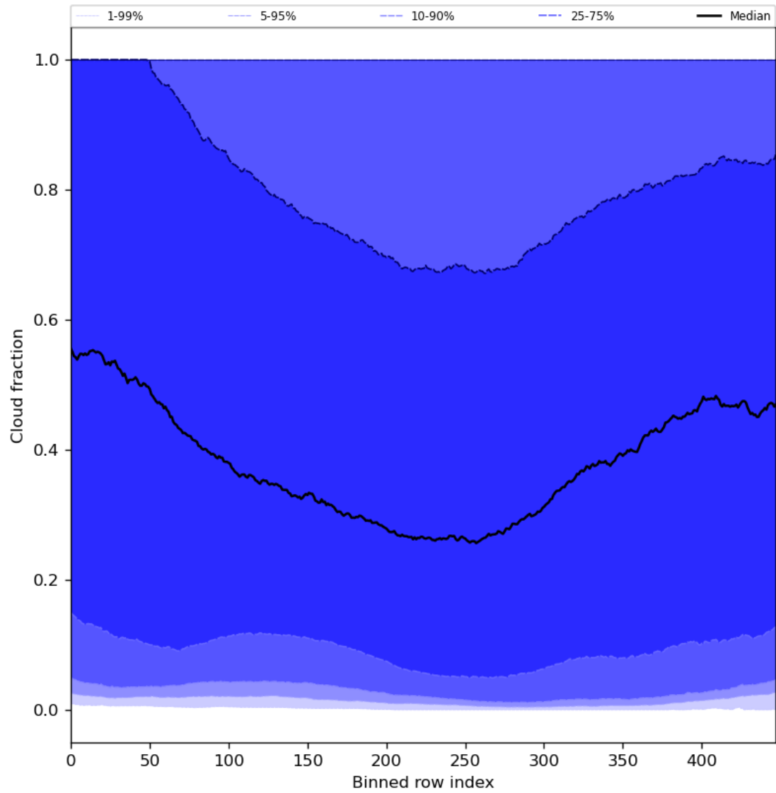
Figure 49: Along track statistics of “Cloud fraction” for 2023-10-02 to 2023-10-04
