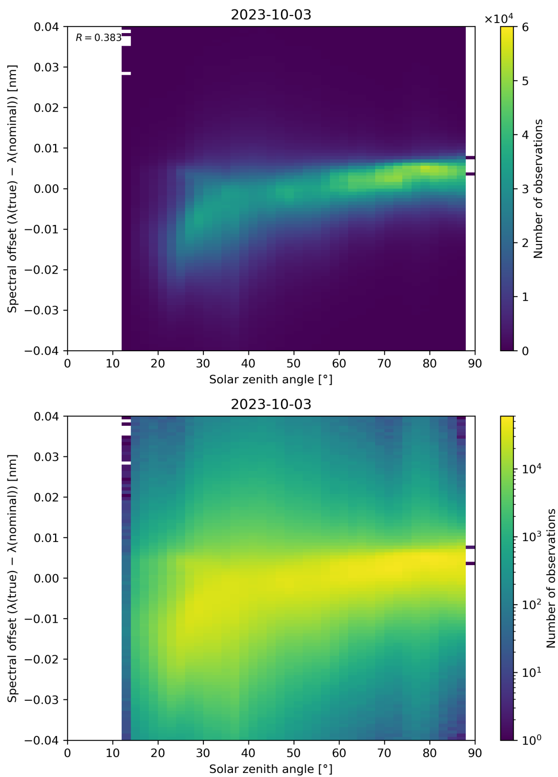
Figure 128: Scatter density plot of “Solar zenith angle” against “Spectral offset ( \lambda(\text{true}) - \lambda(\text{nominal}) )” for 2023-10-02 to 2023-10-04.
