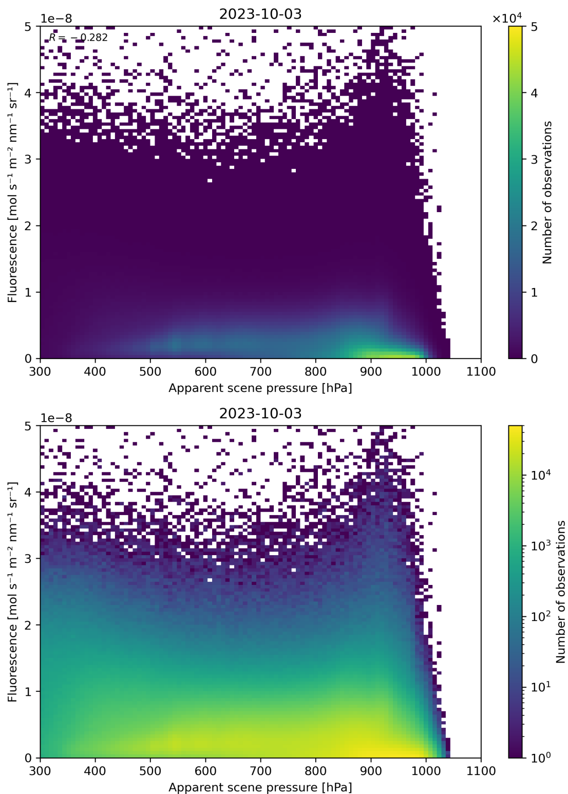
Figure 65: Scatter density plot of “Apparent scene pressure” against “Fluorescence” for 2023-10-02 to 2023-10-04.
