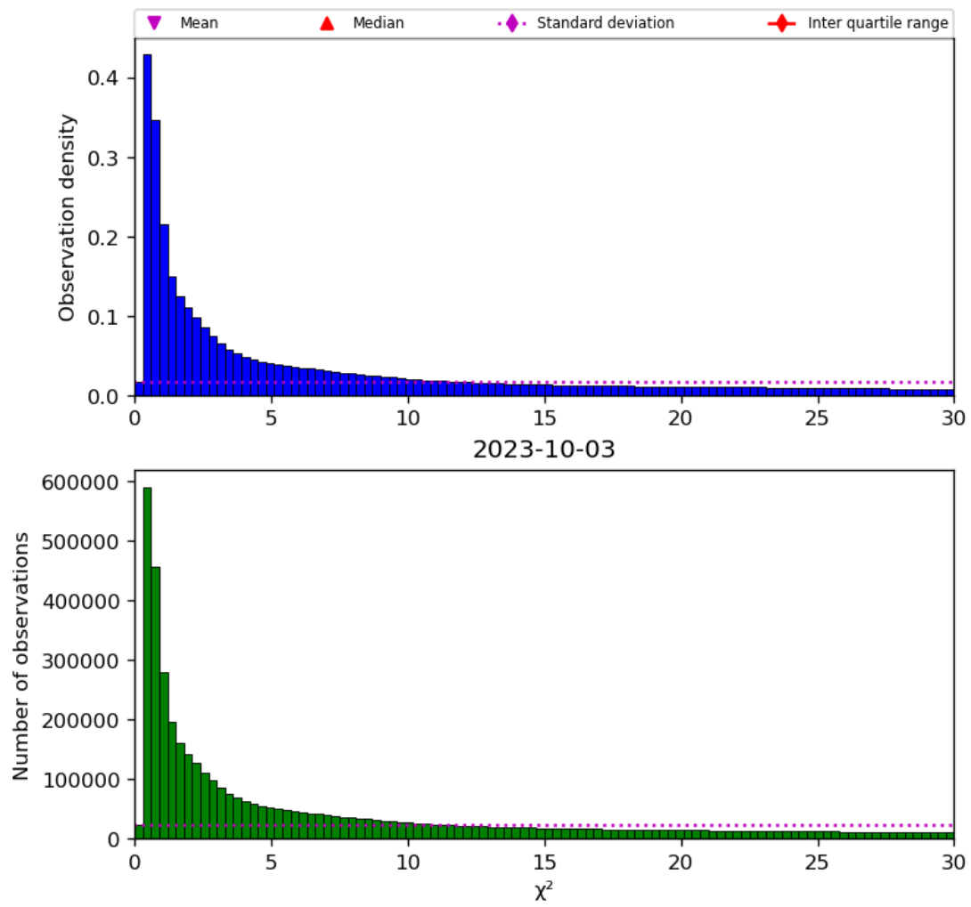
Figure 38: Histogram of " \chi^2 " for 2023-10-02 to 2023-10-04
