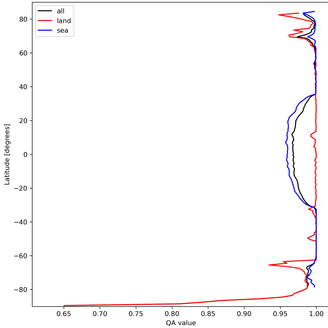
Figure 12: Zonal average of “QA value” for 2023-10-02 to 2023-10-04.
