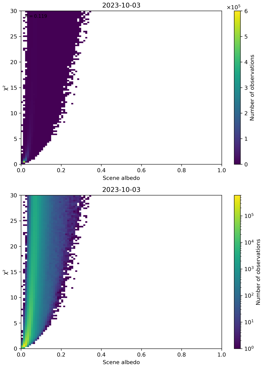
Figure 112: Scatter density plot of “Scene albedo” against “ \chi^2 ” for 2023-10-02 to 2023-10-04.
