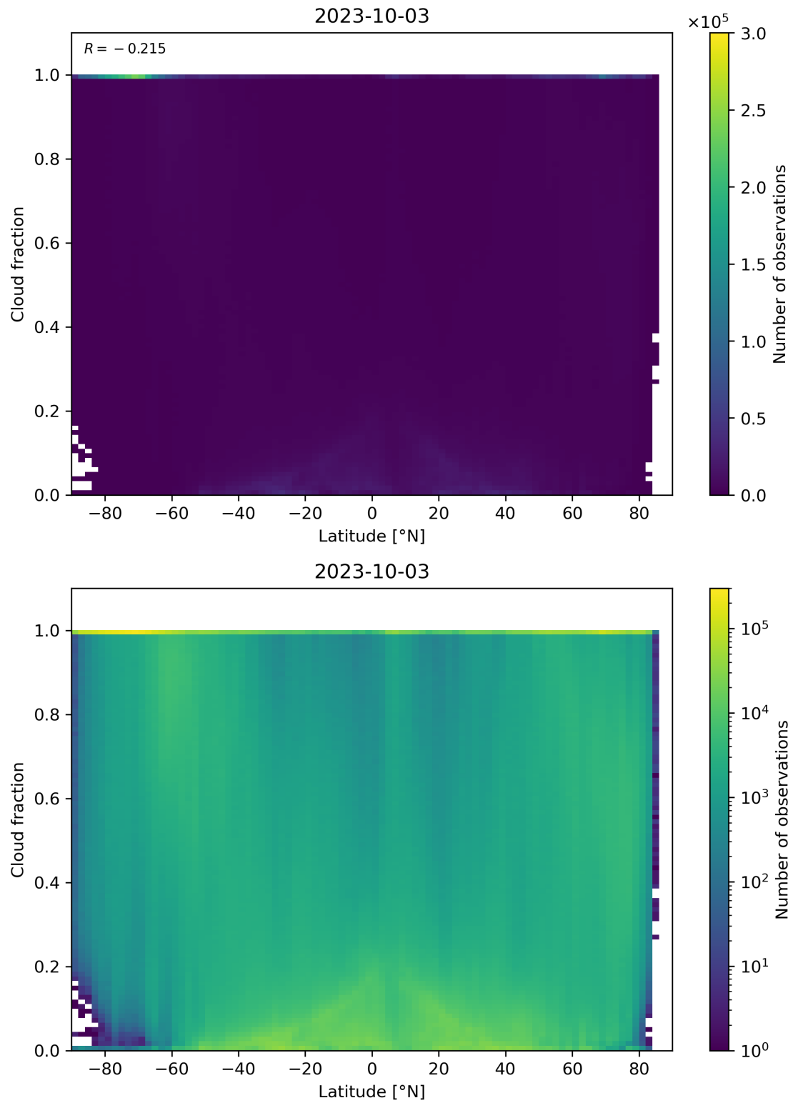
Figure 99: Scatter density plot of “Latitude” against “Cloud fraction” for 2023-10-02 to 2023-10-04.
