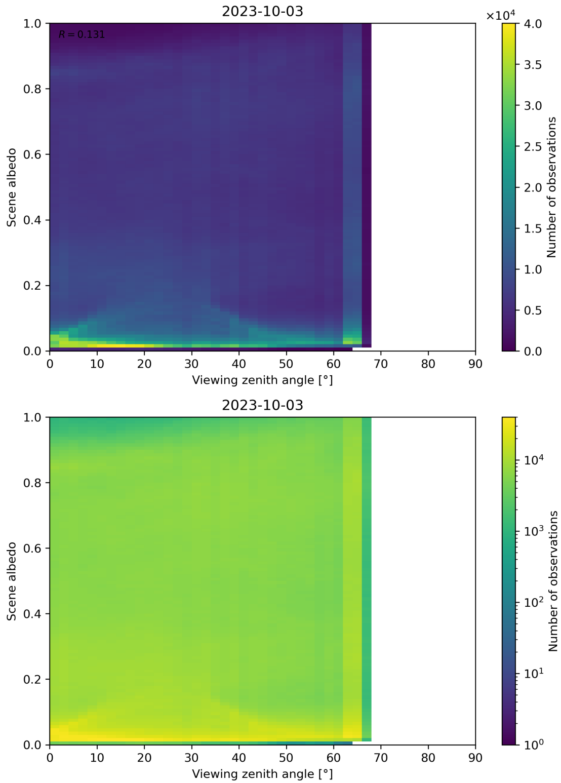
Figure 138: Scatter density plot of “Viewing zenith angle” against “Scene albedo” for 2023-10-02 to 2023-10-04.
