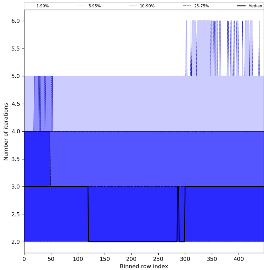
Figure 56: Along track statistics of "Number of iterations" for 2023-10-02 to 2023-10-04
