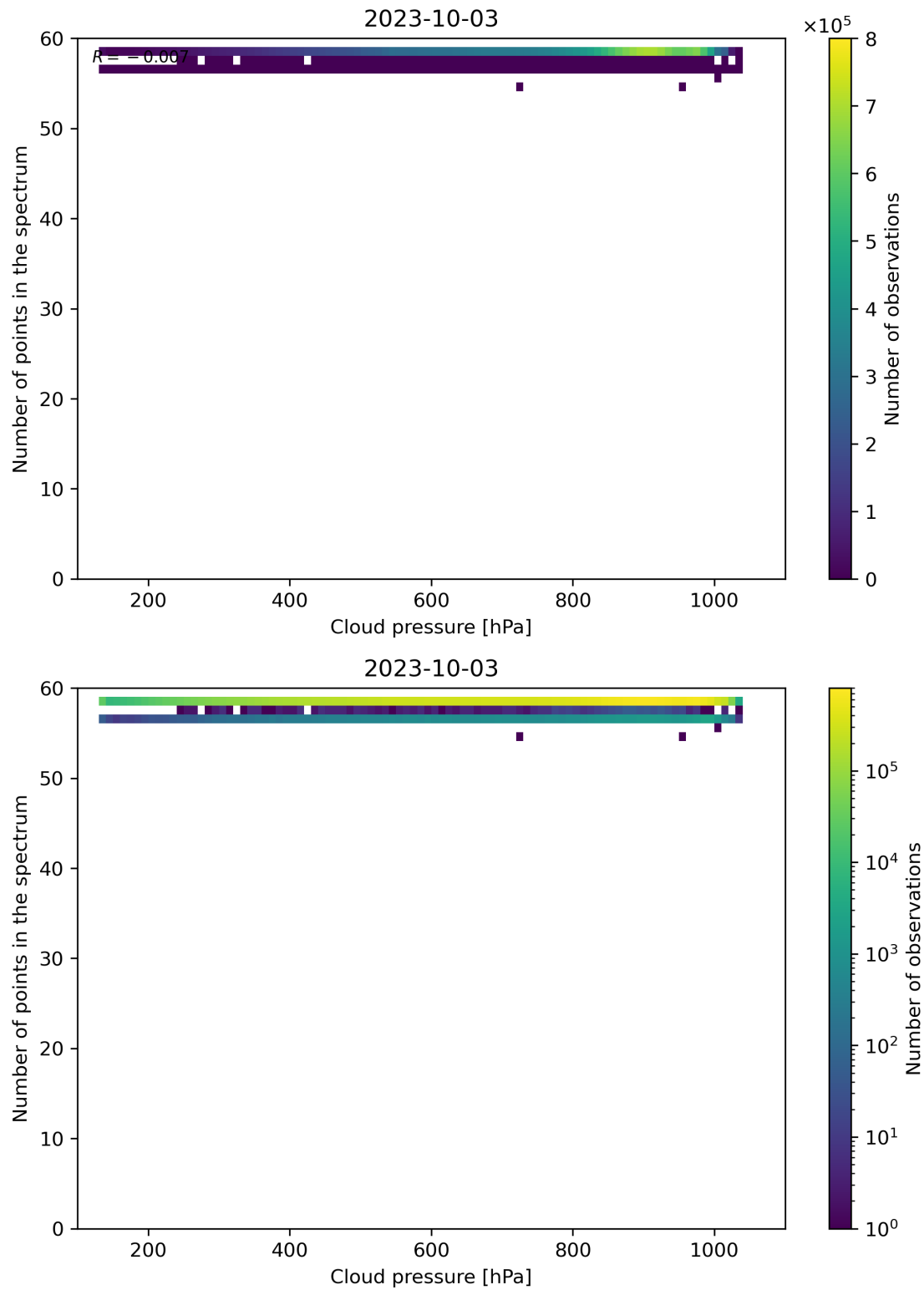
Figure 90: Scatter density plot of “Cloud pressure” against “Number of points in the spectrum” for 2023-10-02 to 2023-10-04.
