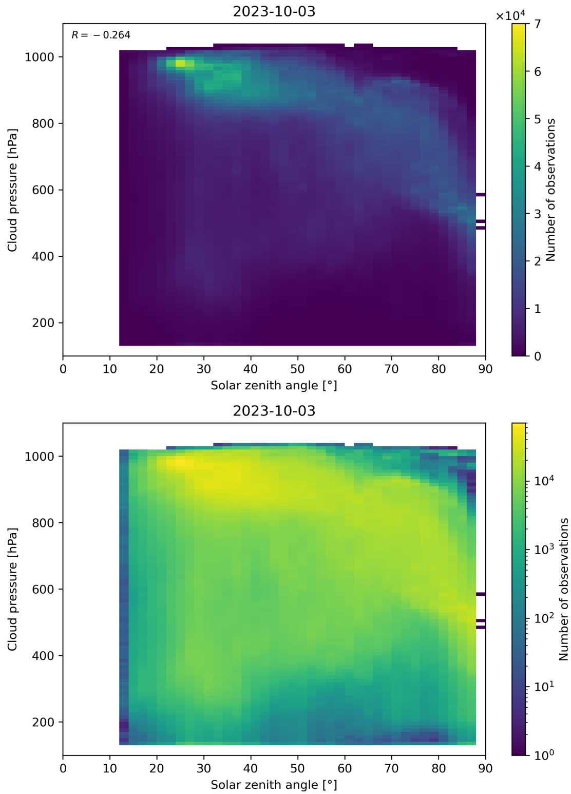
Figure 122: Scatter density plot of “Solar zenith angle” against “Cloud pressure” for 2023-10-02 to 2023-10-04.
