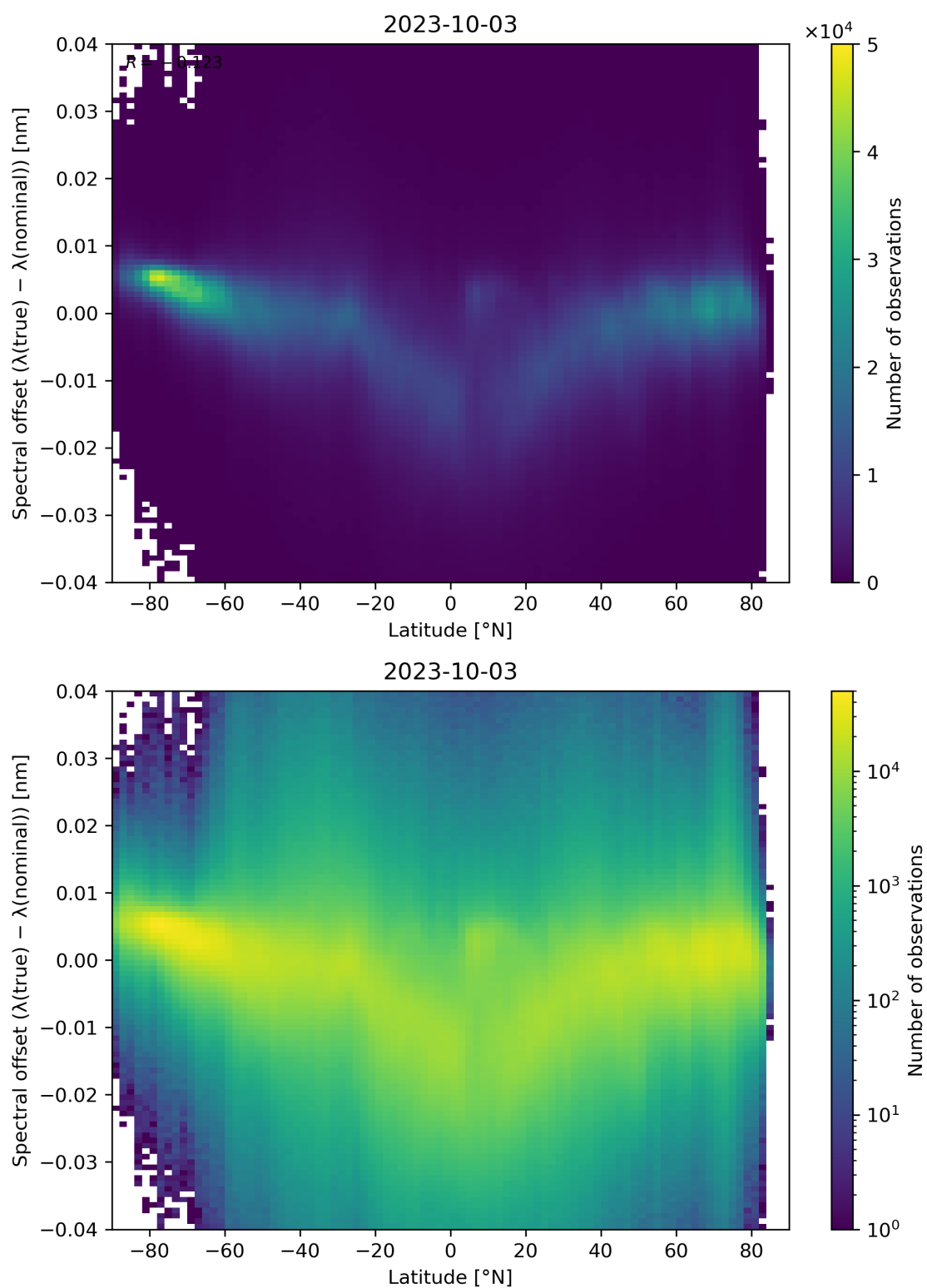
Figure 105: Scatter density plot of “Latitude” against “Spectral offset ( \lambda(\text{true}) - \lambda(\text{nominal}) )” for 2023-10-02 to 2023-10-04.
