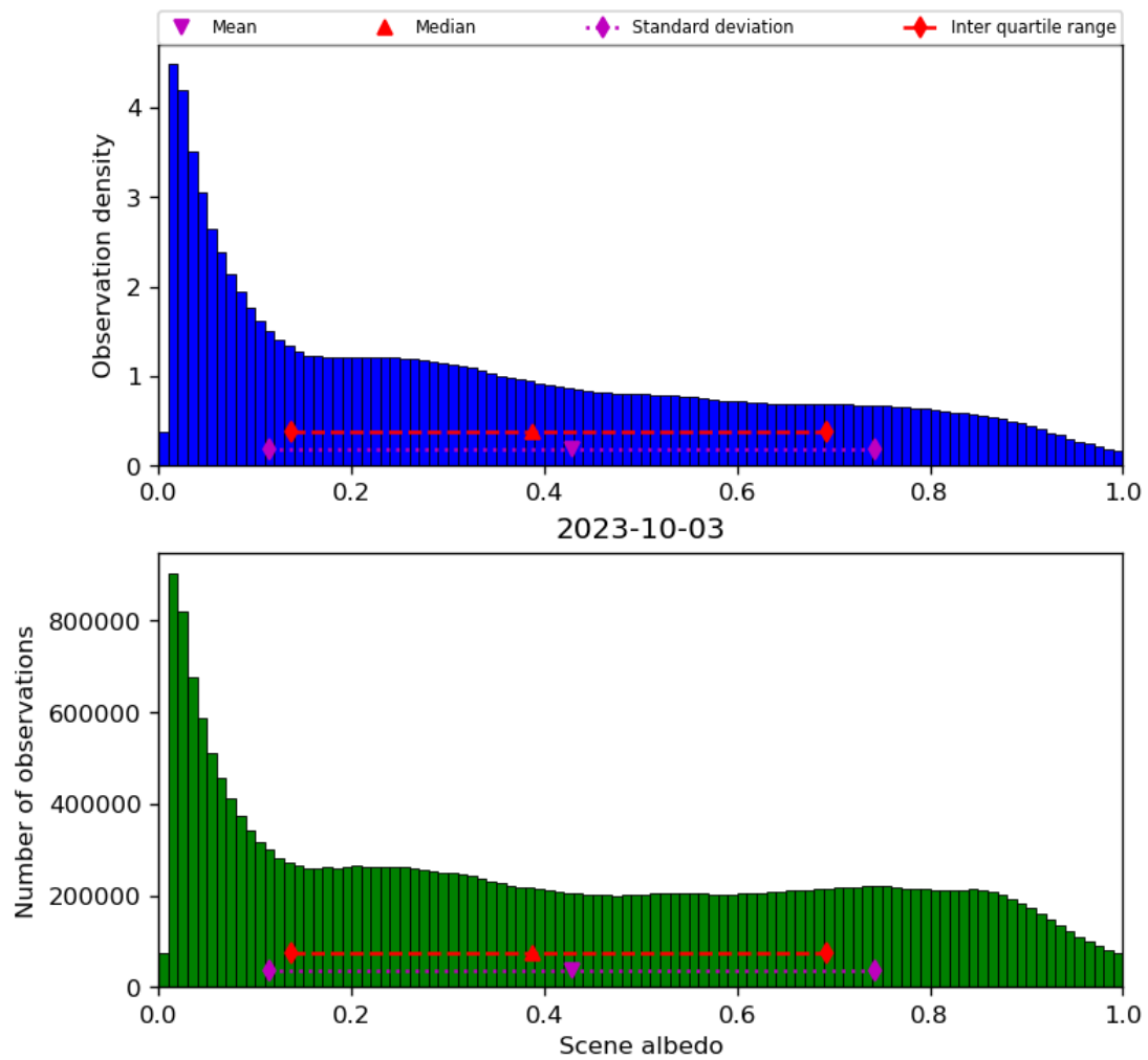
Figure 34: Histogram of “Scene albedo” for 2023-10-02 to 2023-10-04
