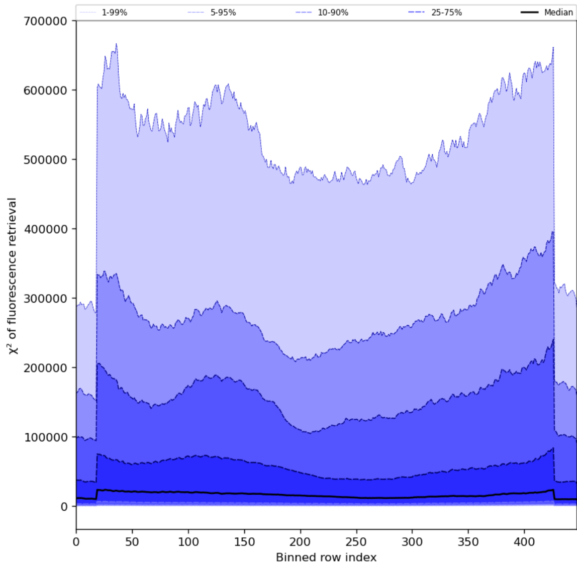
Figure 59: Along track statistics of “ \chi^2 of fluorescence retrieval” for 2023-10-02 to 2023-10-04
