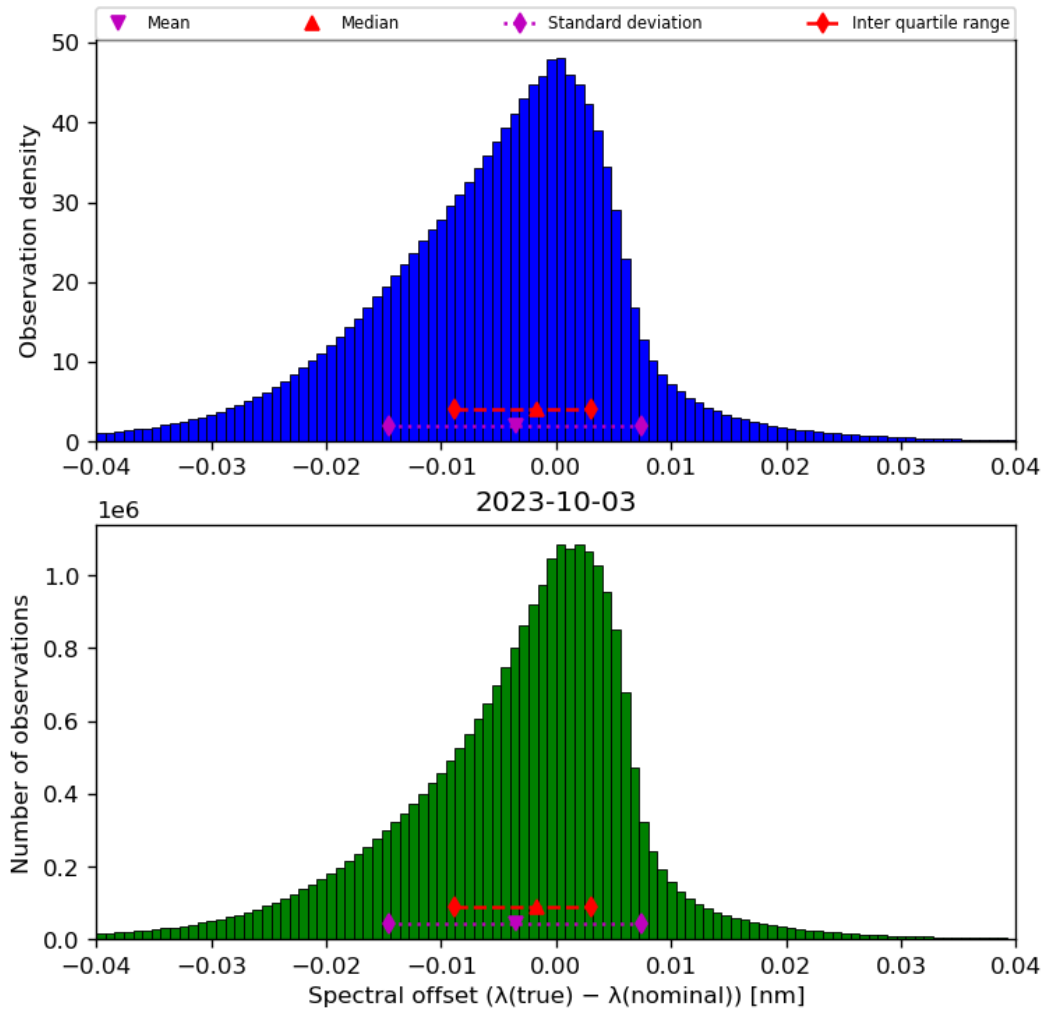
Figure 45: Histogram of “Spectral offset ( \lambda(\text{true}) - \lambda(\text{nominal}) )” for 2023-10-02 to 2023-10-04
