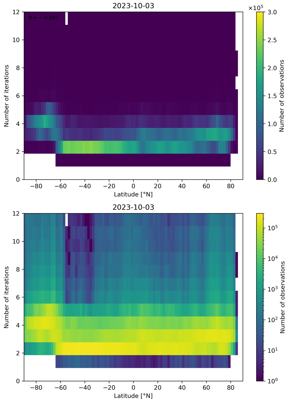
Figure 102: Scatter density plot of “Latitude” against “Number of iterations” for 2023-10-02 to 2023-10-04.
