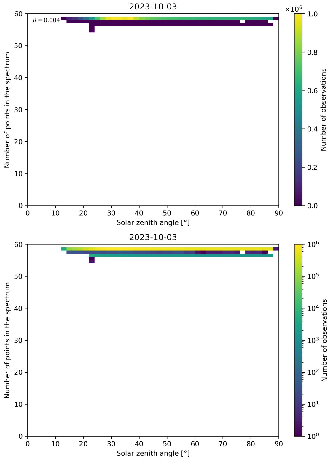
Figure 126: Scatter density plot of “Solar zenith angle” against “Number of points in the spectrum” for 2023-10-02 to 2023-10-04.
