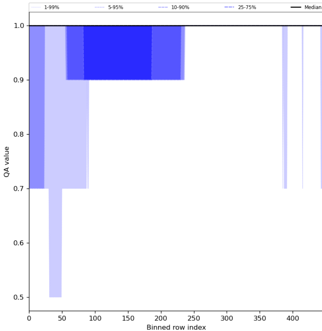
Figure 46: Along track statistics of “QA value” for 2023-10-02 to 2023-10-04
