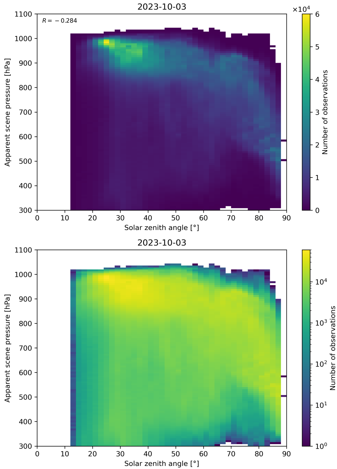
Figure 118: Scatter density plot of “Solar zenith angle” against “Apparent scene pressure” for 2023-10-02 to 2023-10-04.
