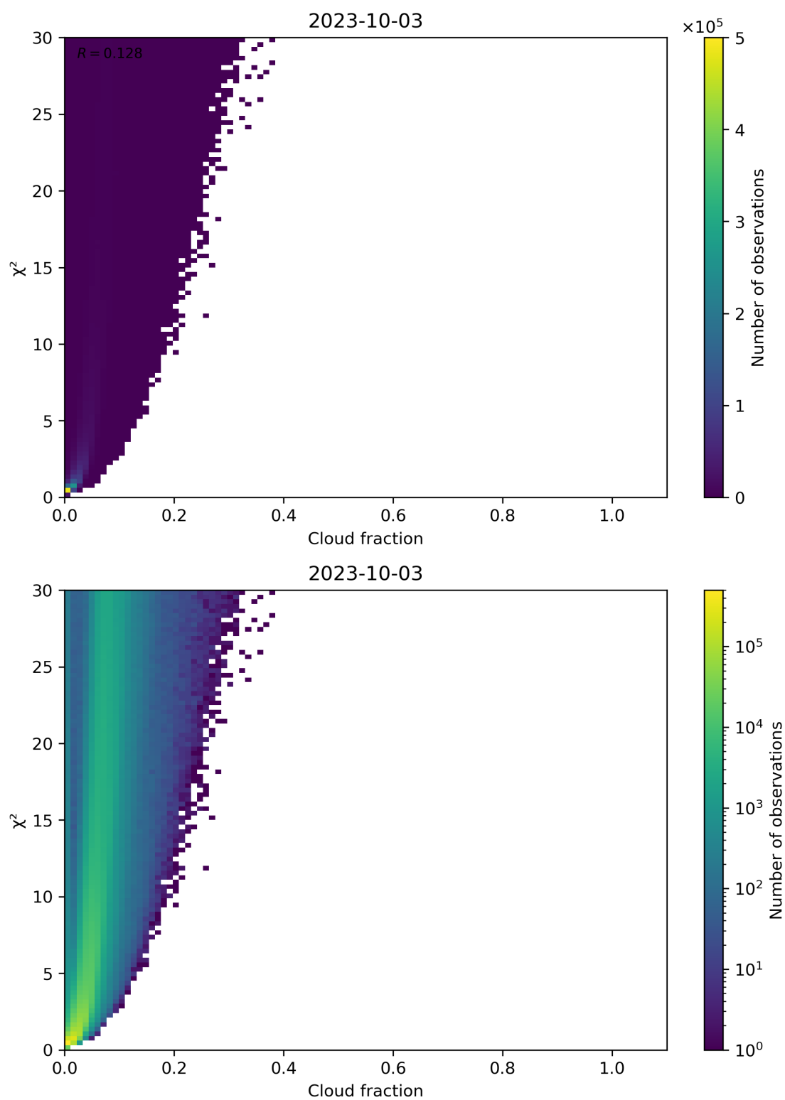
Figure 77: Scatter density plot of “Cloud fraction” against “ \chi^2 ” for 2023-10-02 to 2023-10-04.
