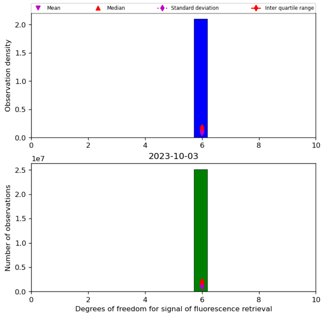
Figure 43: Histogram of “Degrees of freedom for signal of fluorescence retrieval” for 2023-10-02 to 2023-10-04
