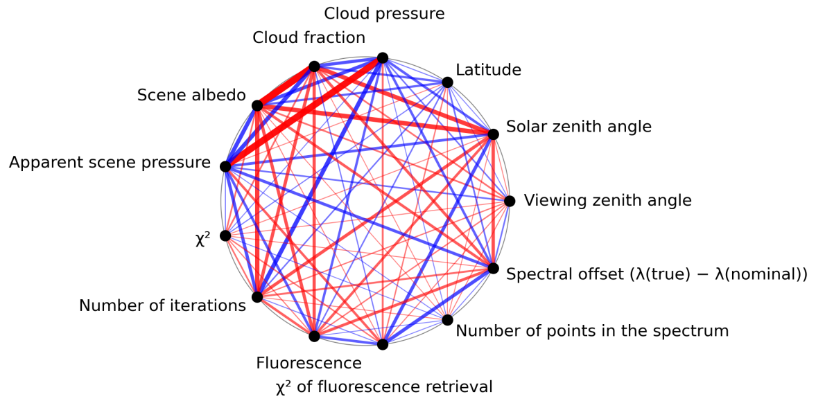
Figure 1: Map of correlation graph for 2023-10-02 to 2023-10-04.
