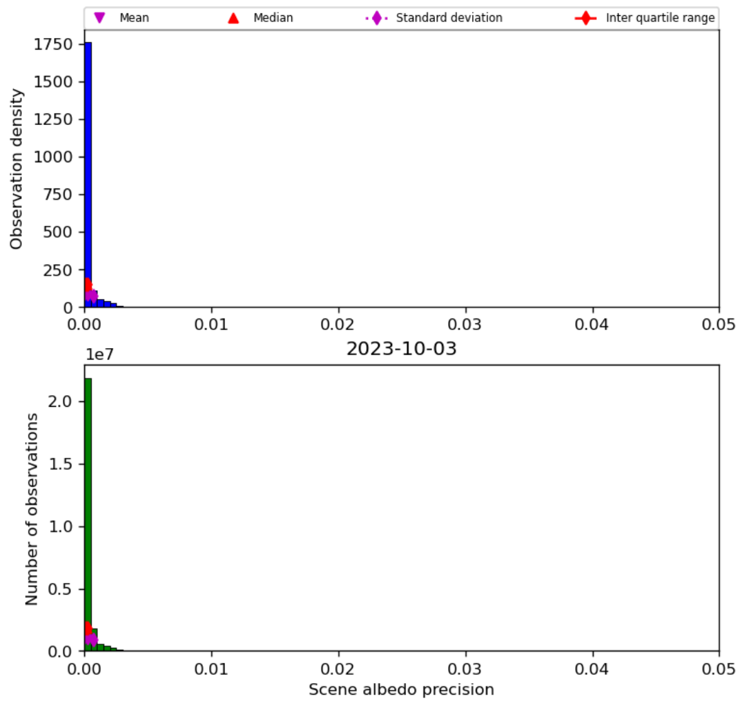
Figure 35: Histogram of “Scene albedo precision” for 2023-10-02 to 2023-10-04
