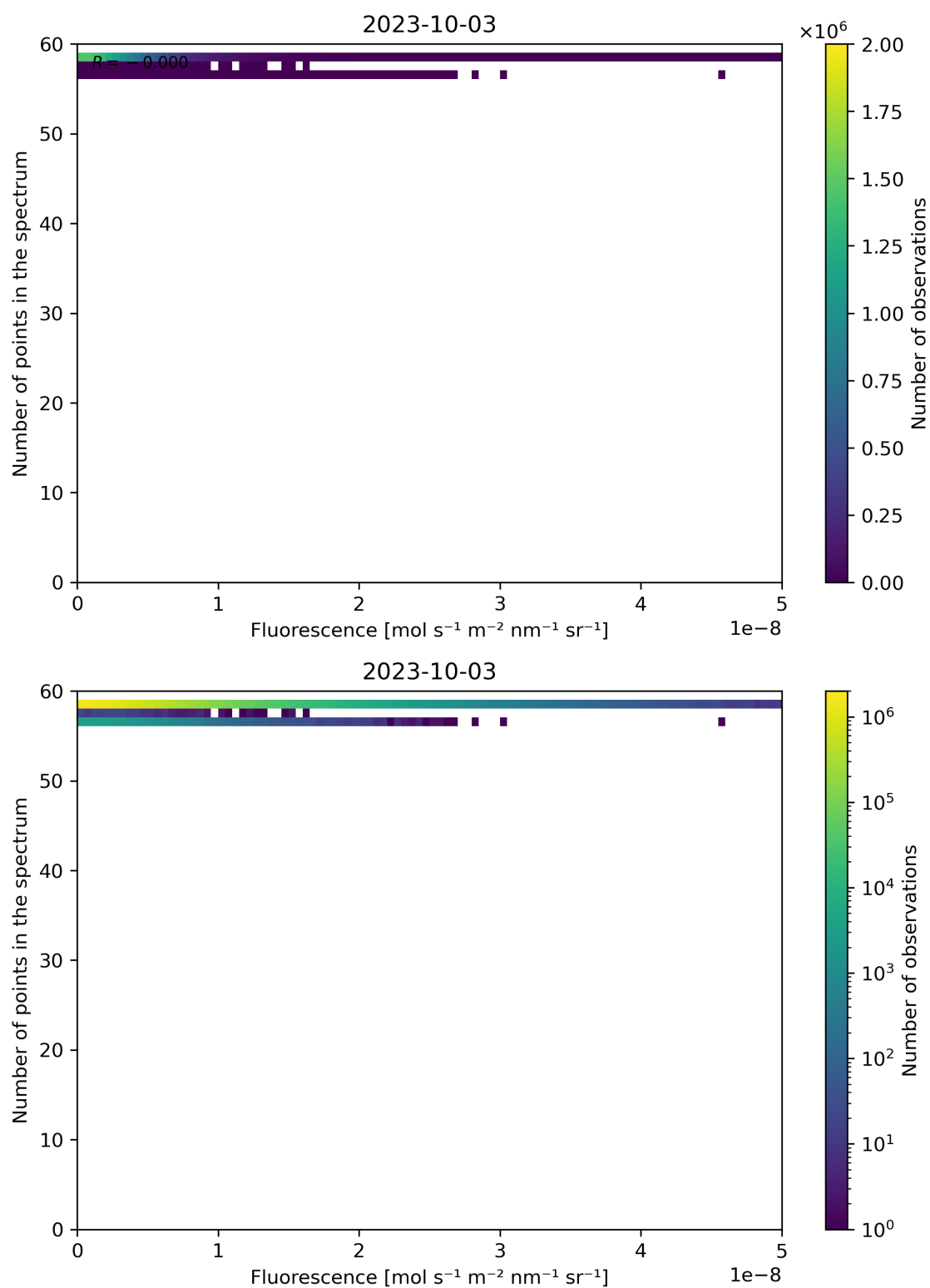
Figure 94: Scatter density plot of “Fluorescence” against “Number of points in the spectrum” for 2023-10-02 to 2023-10-04.
