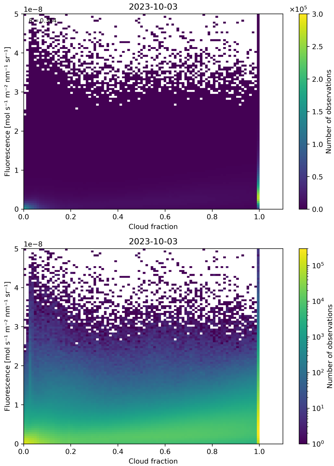
Figure 79: Scatter density plot of “Cloud fraction” against “Fluorescence” for 2023-10-02 to 2023-10-04.
