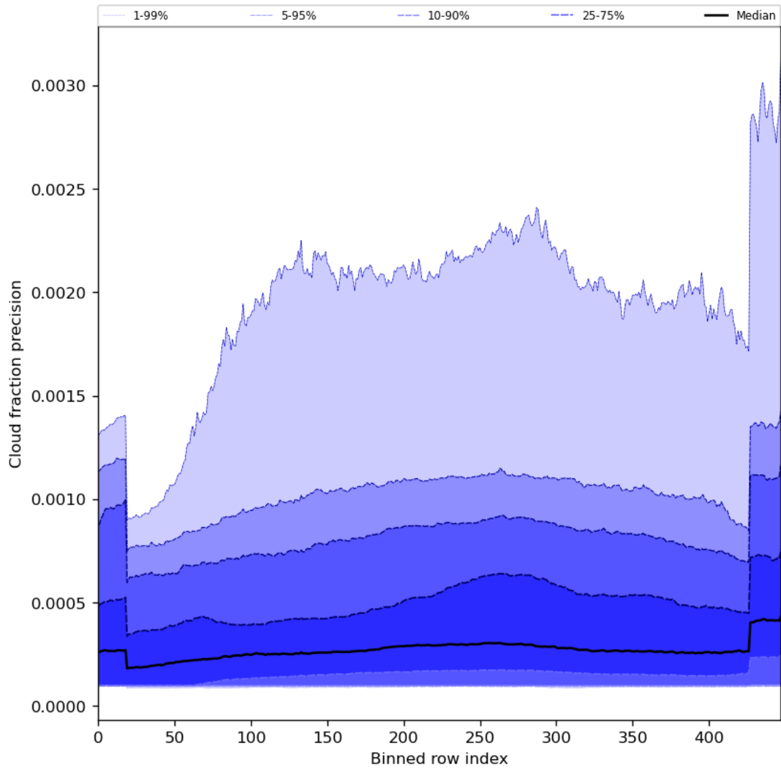
Figure 50: Along track statistics of “Cloud fraction precision” for 2023-10-02 to 2023-10-04
