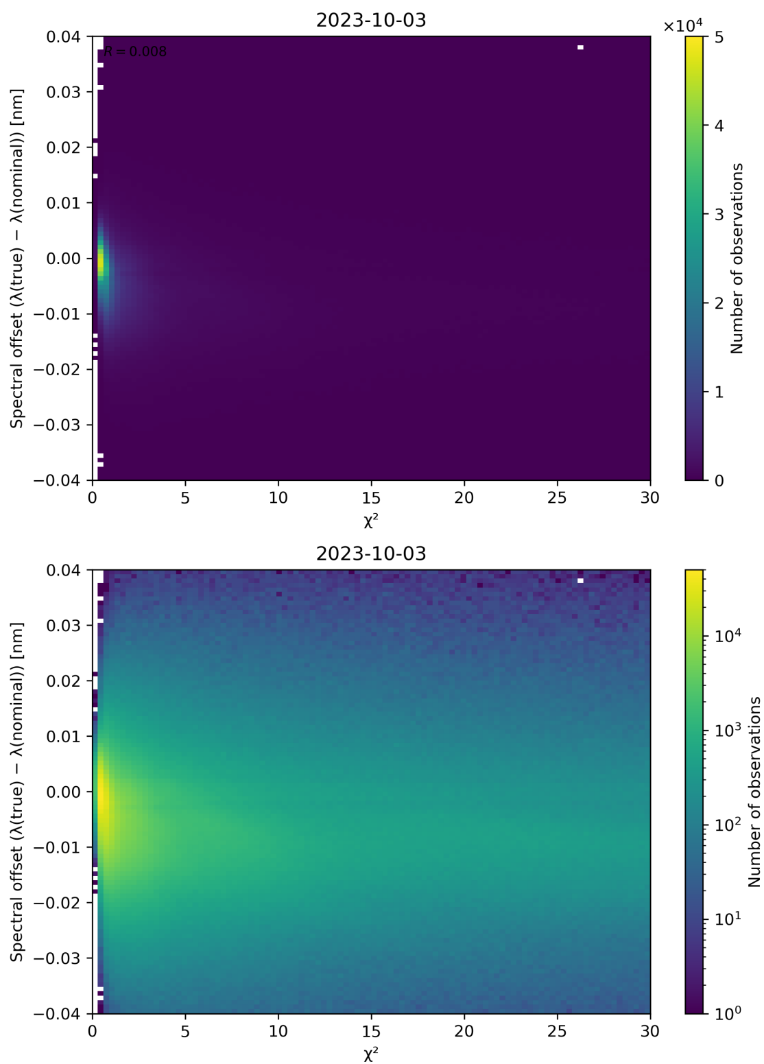
Figure 75: Scatter density plot of “ \chi^2 ” against “Spectral offset ( \lambda(\text{true}) - \lambda(\text{nominal}) )” for 2023-10-02 to 2023-10-04.
