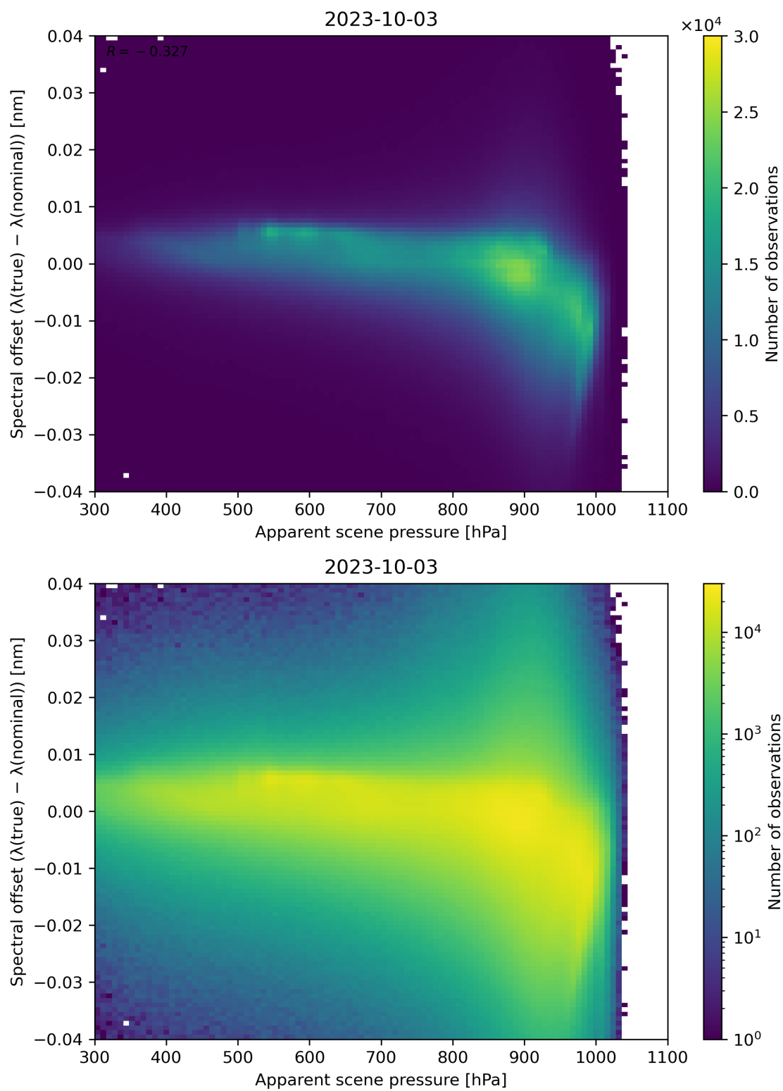
Figure 68: Scatter density plot of “Apparent scene pressure” against “Spectral offset ( \lambda(\text{true}) - \lambda(\text{nominal}) )” for 2023-10-02 to 2023-10-04.
