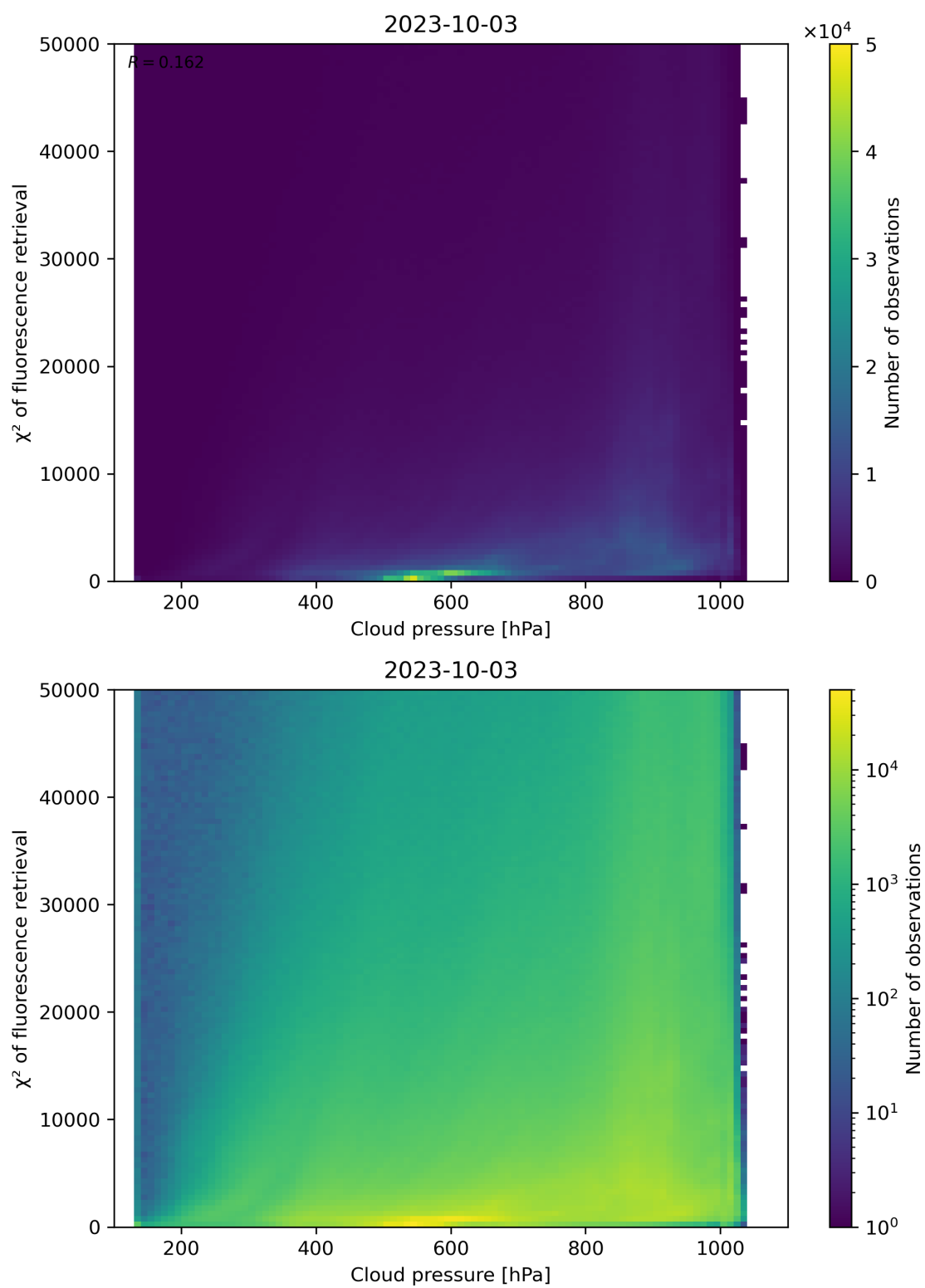
Figure 86: Scatter density plot of “Cloud pressure” against “ \chi^2 of fluorescence retrieval” for 2023-10-02 to 2023-10-04.
