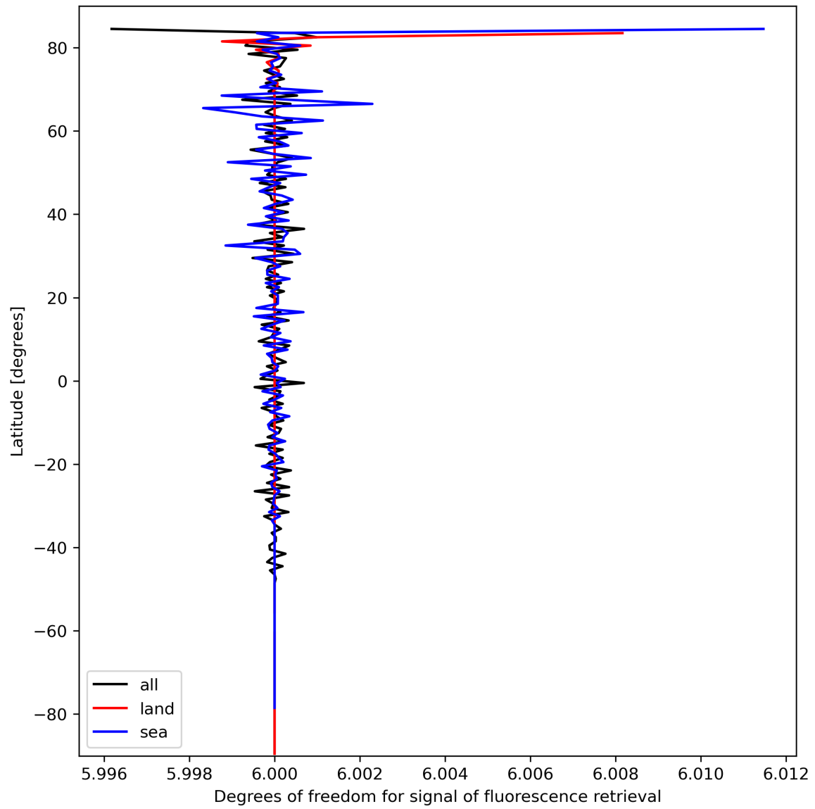
Figure 26: Zonal average of “Degrees of freedom for signal of fluorescence retrieval” for 2023-10-02 to 2023-10-04.
