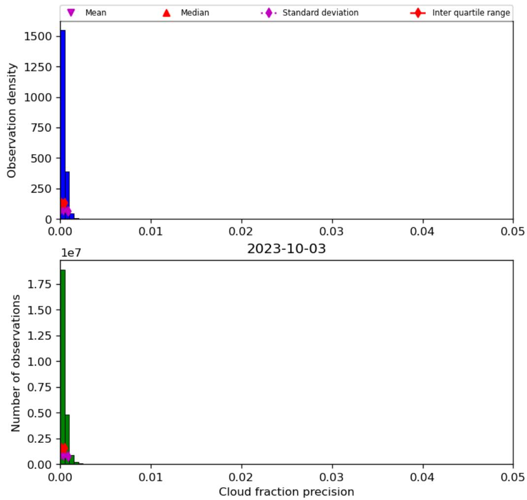
Figure 33: Histogram of “Cloud fraction precision” for 2023-10-02 to 2023-10-04
