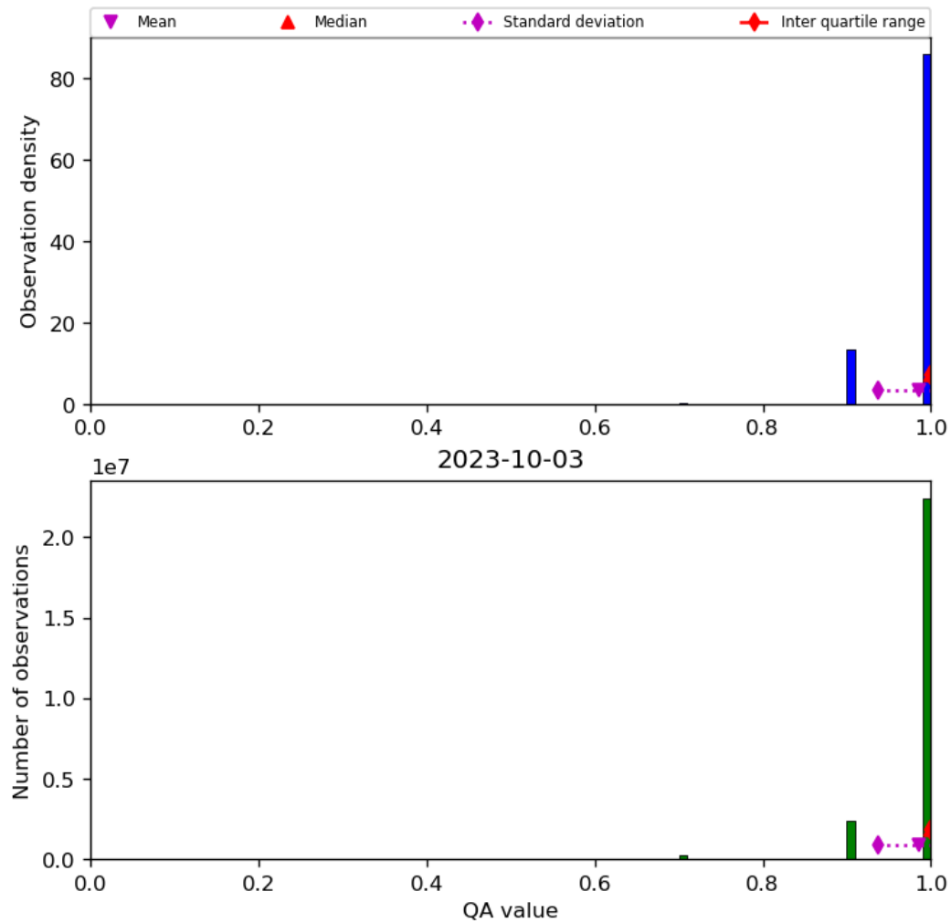
Figure 29: Histogram of “QA value” for 2023-10-02 to 2023-10-04
