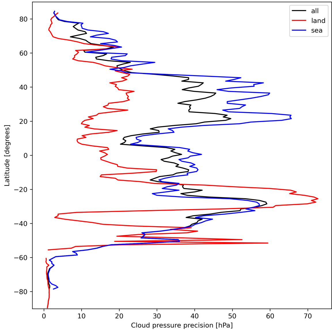
Figure 14: Zonal average of “Cloud pressure precision” for 2023-10-02 to 2023-10-04.
