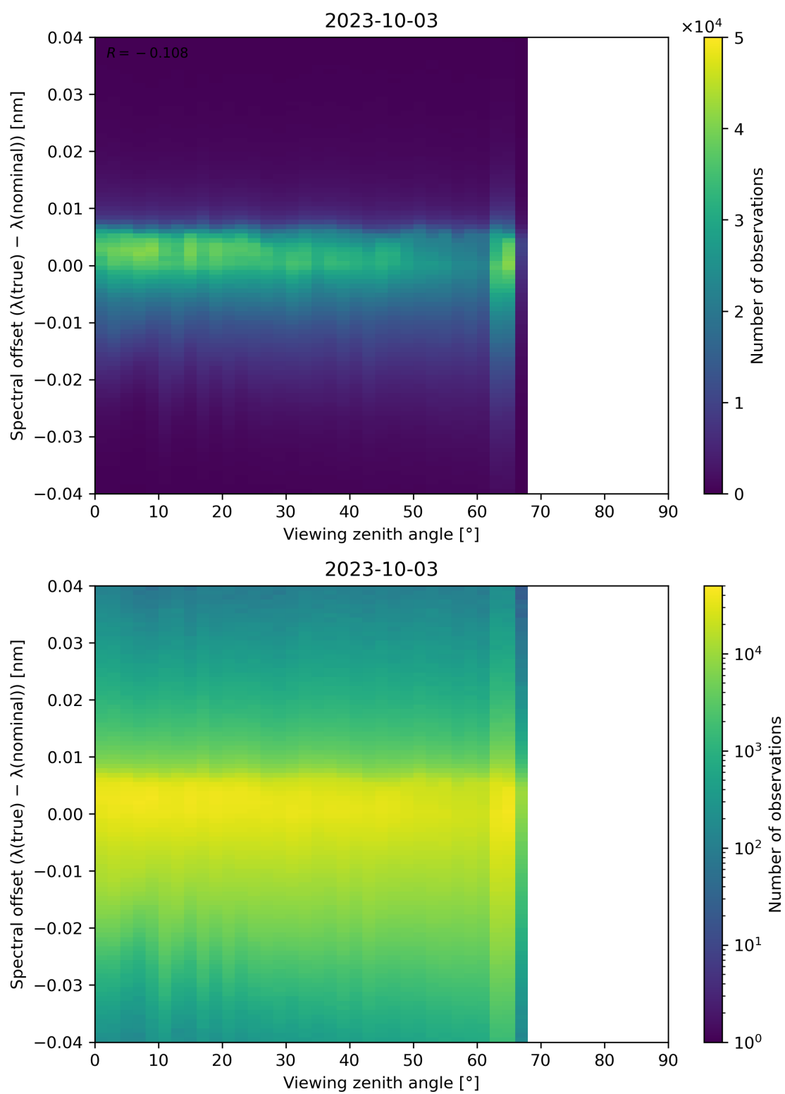
Figure 140: Scatter density plot of “Viewing zenith angle” against “Spectral offset ( \lambda(\text{true}) - \lambda(\text{nominal}) )” for 2023-10-02 to 2023-10-04.
