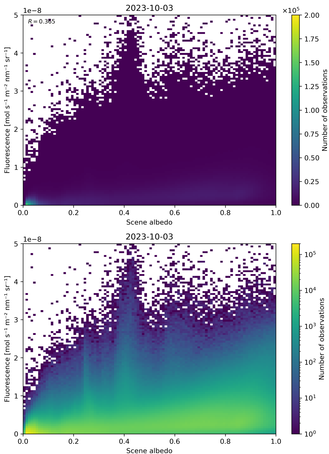
Figure 114: Scatter density plot of “Scene albedo” against “Fluorescence” for 2023-10-02 to 2023-10-04.
