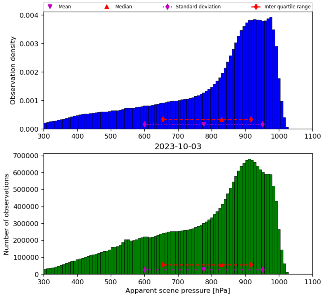
Figure 36: Histogram of “Apparent scene pressure” for 2023-10-02 to 2023-10-04
