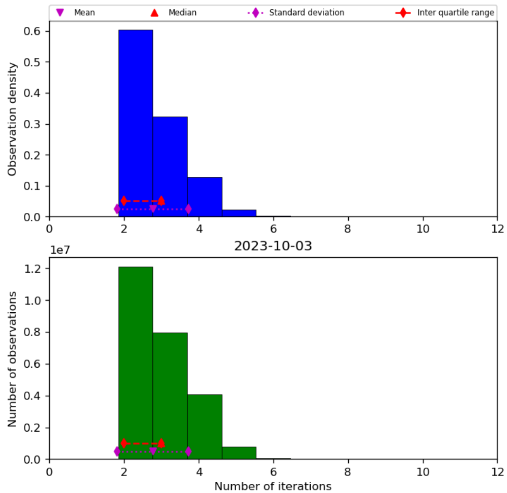
Figure 39: Histogram of “Number of iterations” for 2023-10-02 to 2023-10-04
