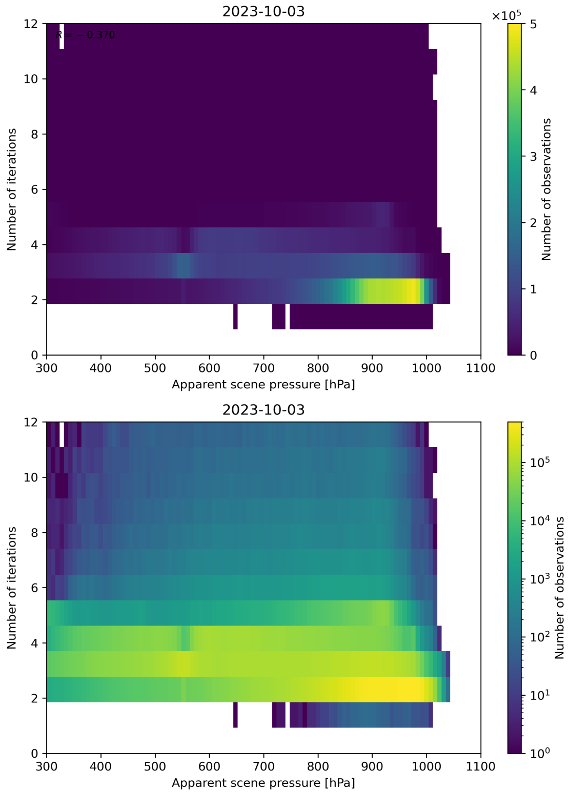
Figure 66: Scatter density plot of “Apparent scene pressure” against “Number of iterations” for 2023-10-02 to 2023-10-04.
