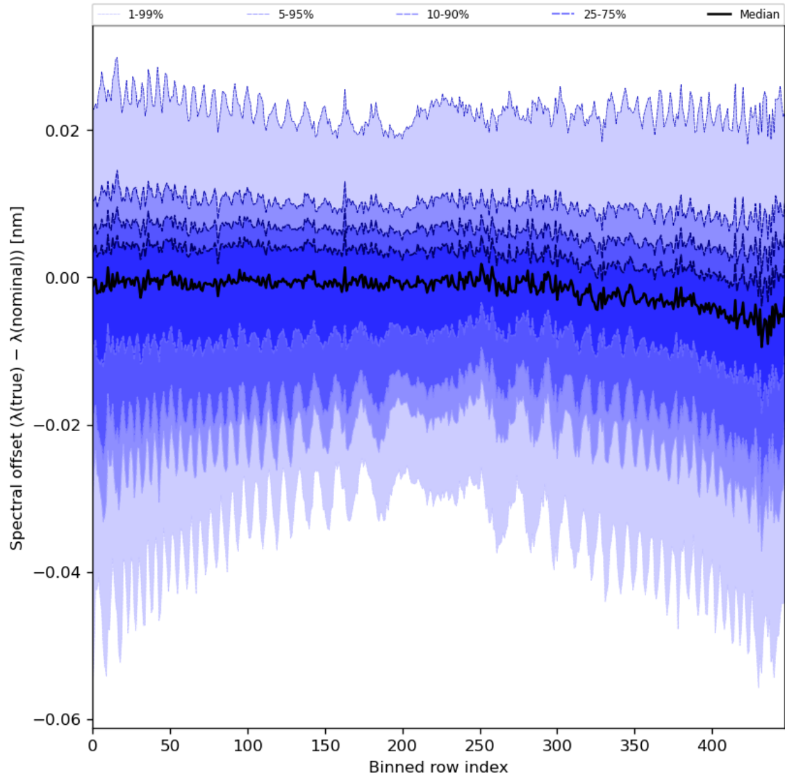
Figure 62: Along track statistics of “Spectral offset ( \lambda(\text{true}) - \lambda(\text{nominal}) )” for 2023-10-02 to 2023-10-04
