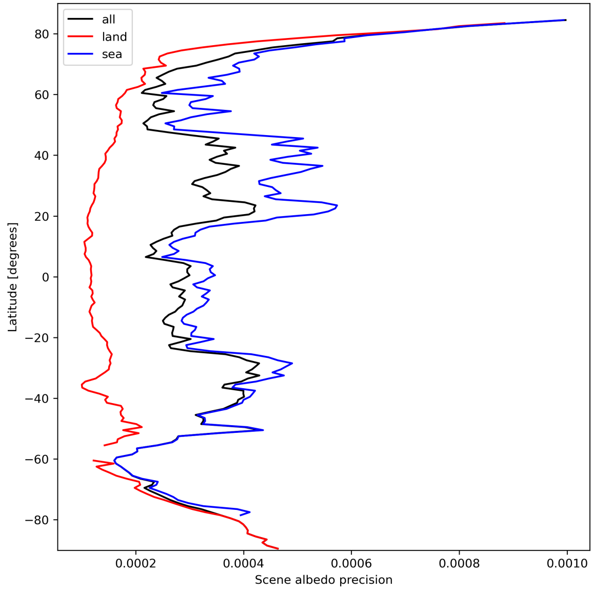
Figure 18: Zonal average of "Scene albedo precision" for 2023-10-02 to 2023-10-04.
