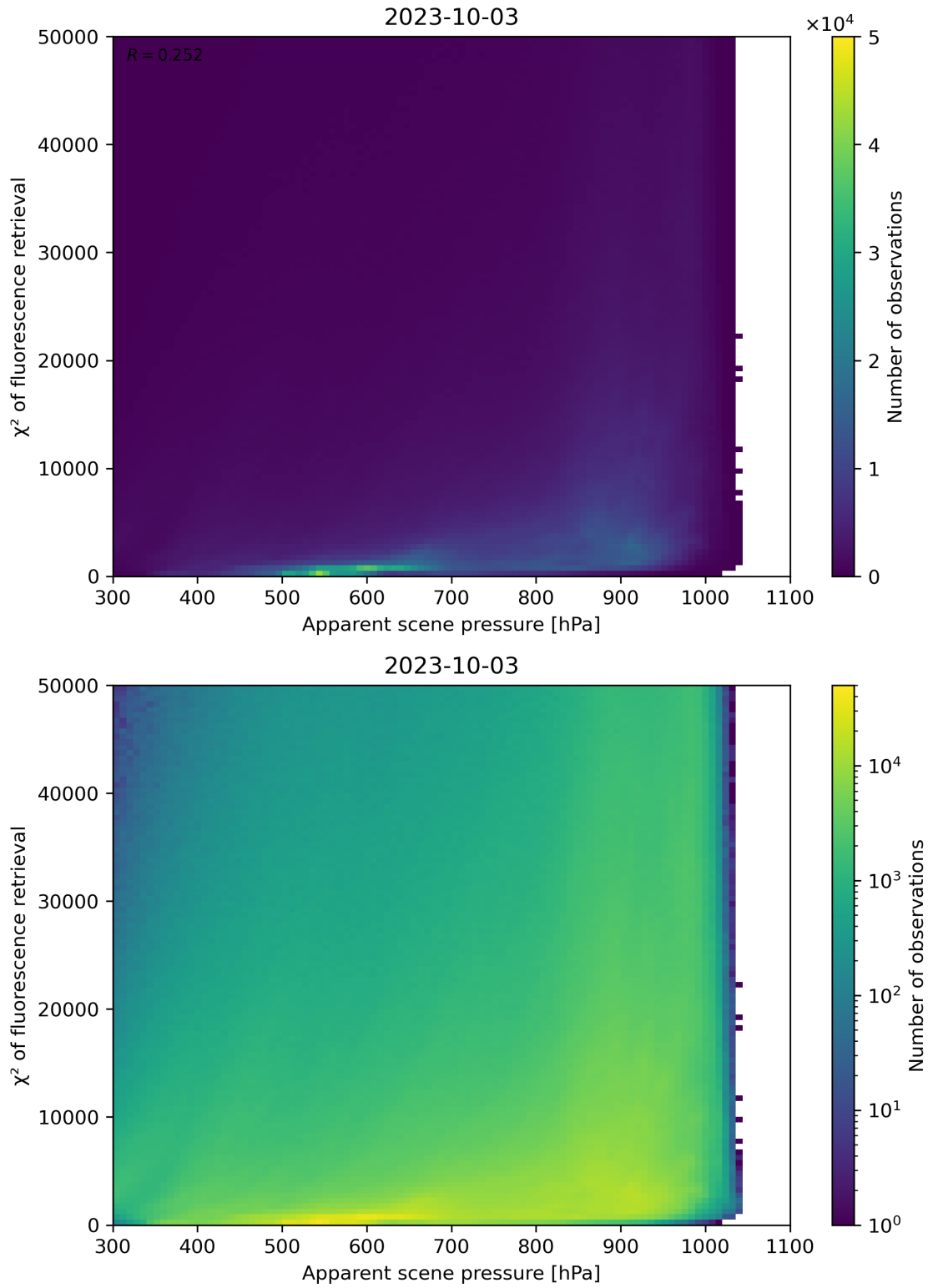
Figure 64: Scatter density plot of “Apparent scene pressure” against “ \chi^2 of fluorescence retrieval” for 2023-10-02 to 2023-10-04.
