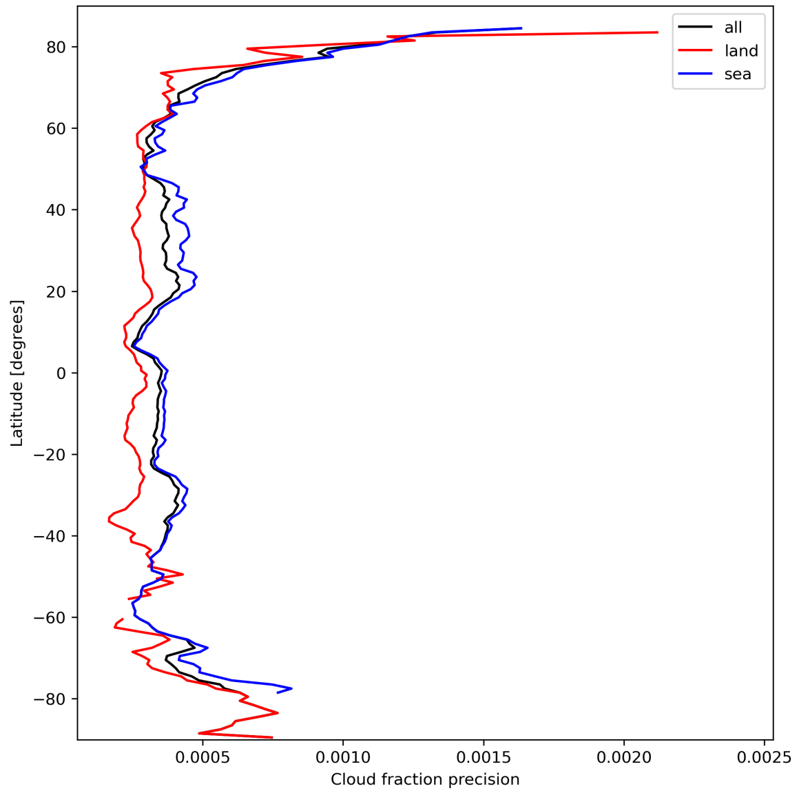
Figure 16: Zonal average of “Cloud fraction precision” for 2023-10-02 to 2023-10-04.
