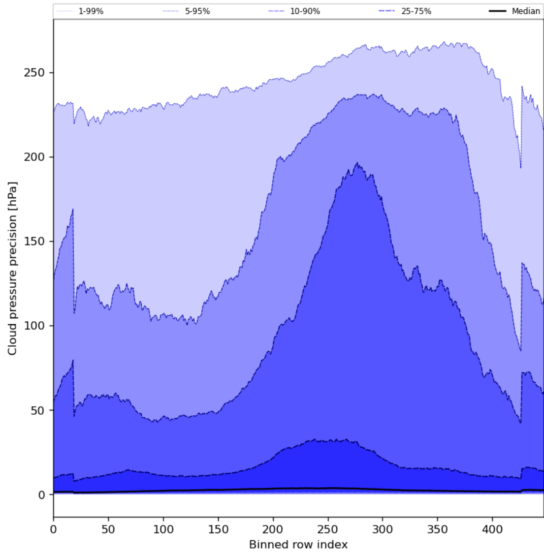
Figure 48: Along track statistics of “Cloud pressure precision” for 2023-10-02 to 2023-10-04
