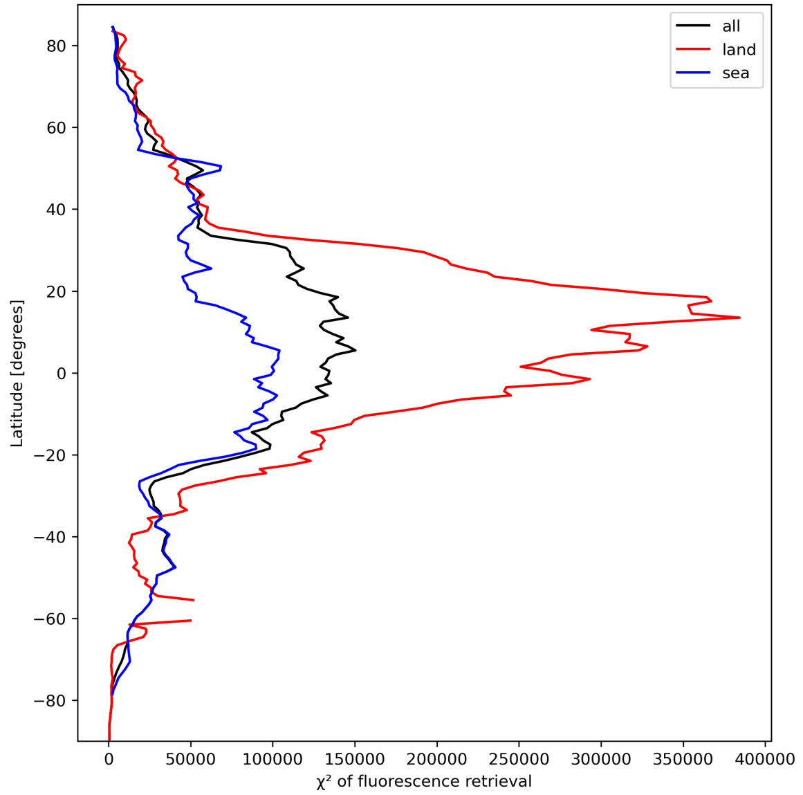
Figure 25: Zonal average of “ \chi^2 of fluorescence retrieval” for 2023-10-02 to 2023-10-04.
