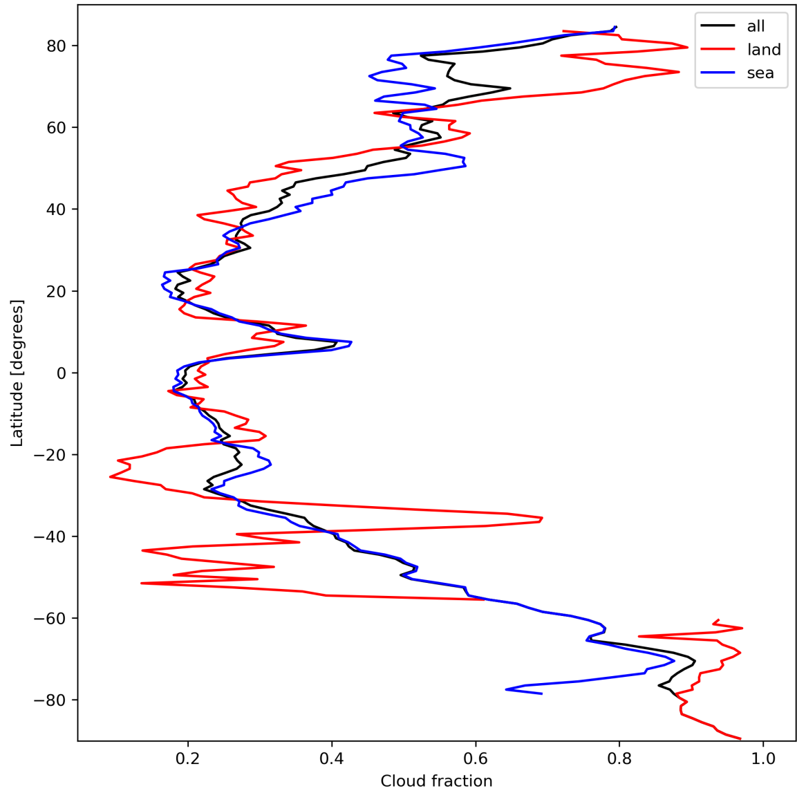
Figure 15: Zonal average of “Cloud fraction” for 2023-10-02 to 2023-10-04.
