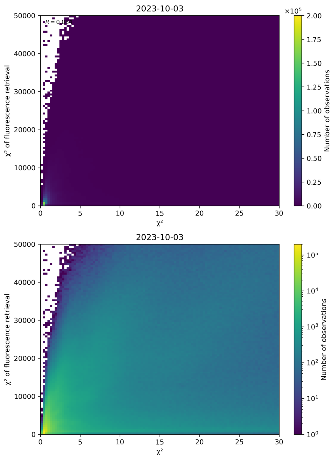
Figure 69: Scatter density plot of “ \chi^2 ” against “ \chi^2 of fluorescence retrieval” for 2023-10-02 to 2023-10-04.
