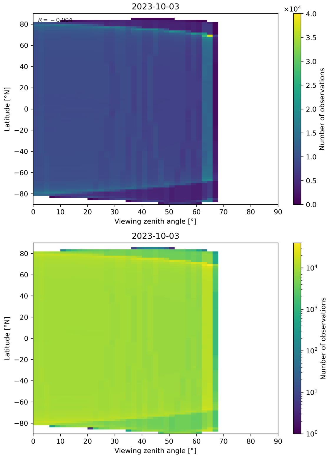
Figure 135: Scatter density plot of “Viewing zenith angle” against “Latitude” for 2023-10-02 to 2023-10-04.
