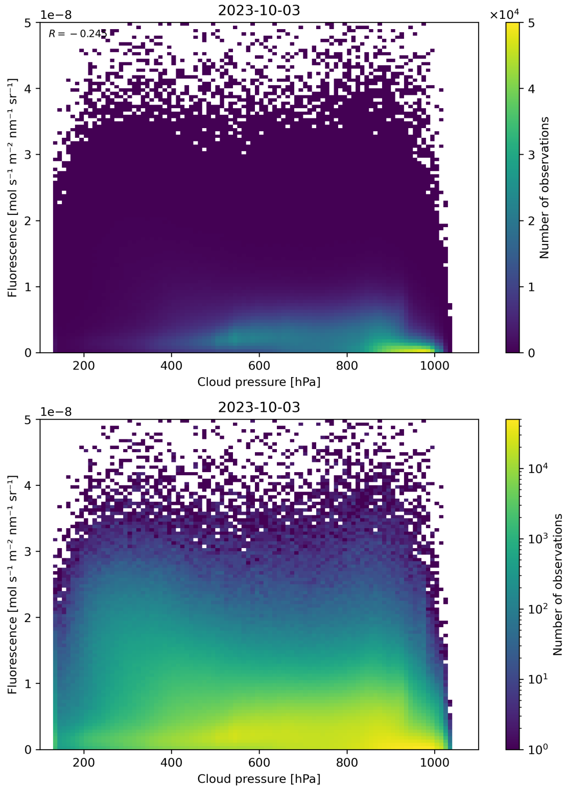
Figure 88: Scatter density plot of “Cloud pressure” against “Fluorescence” for 2023-10-02 to 2023-10-04.
