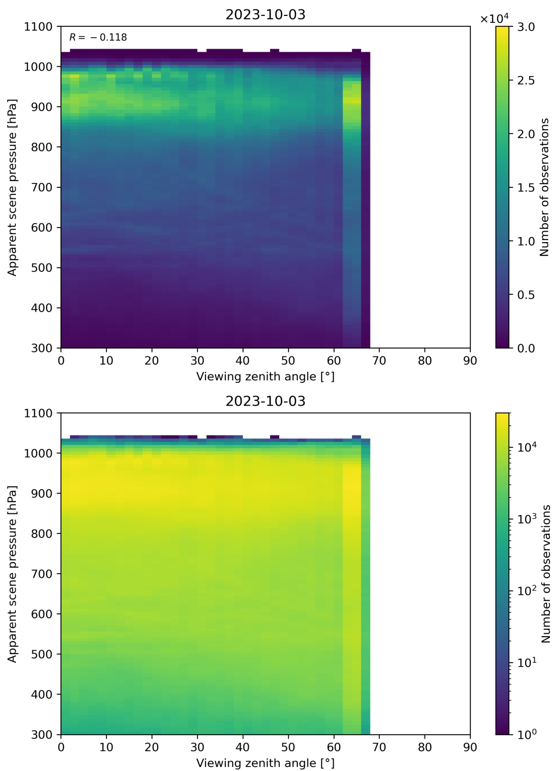
Figure 129: Scatter density plot of “Viewing zenith angle” against “Apparent scene pressure” for 2023-10-02 to 2023-10-04.
