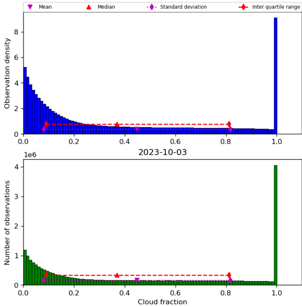
Figure 32: Histogram of “Cloud fraction” for 2023-10-02 to 2023-10-04
