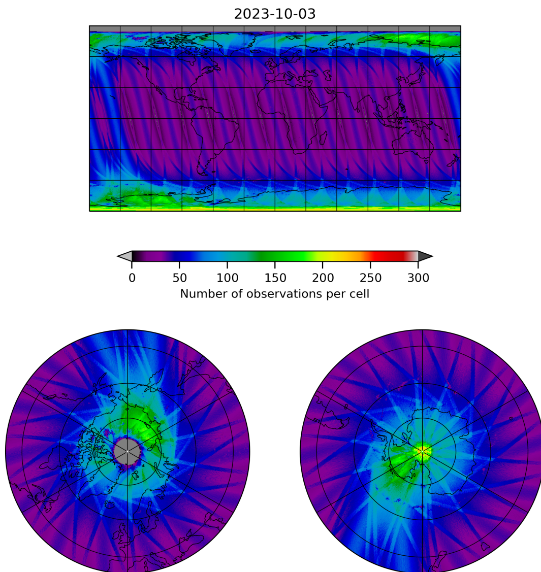
Figure 11: Map of the number of observations for 2023-10-02 to 2023-10-04
