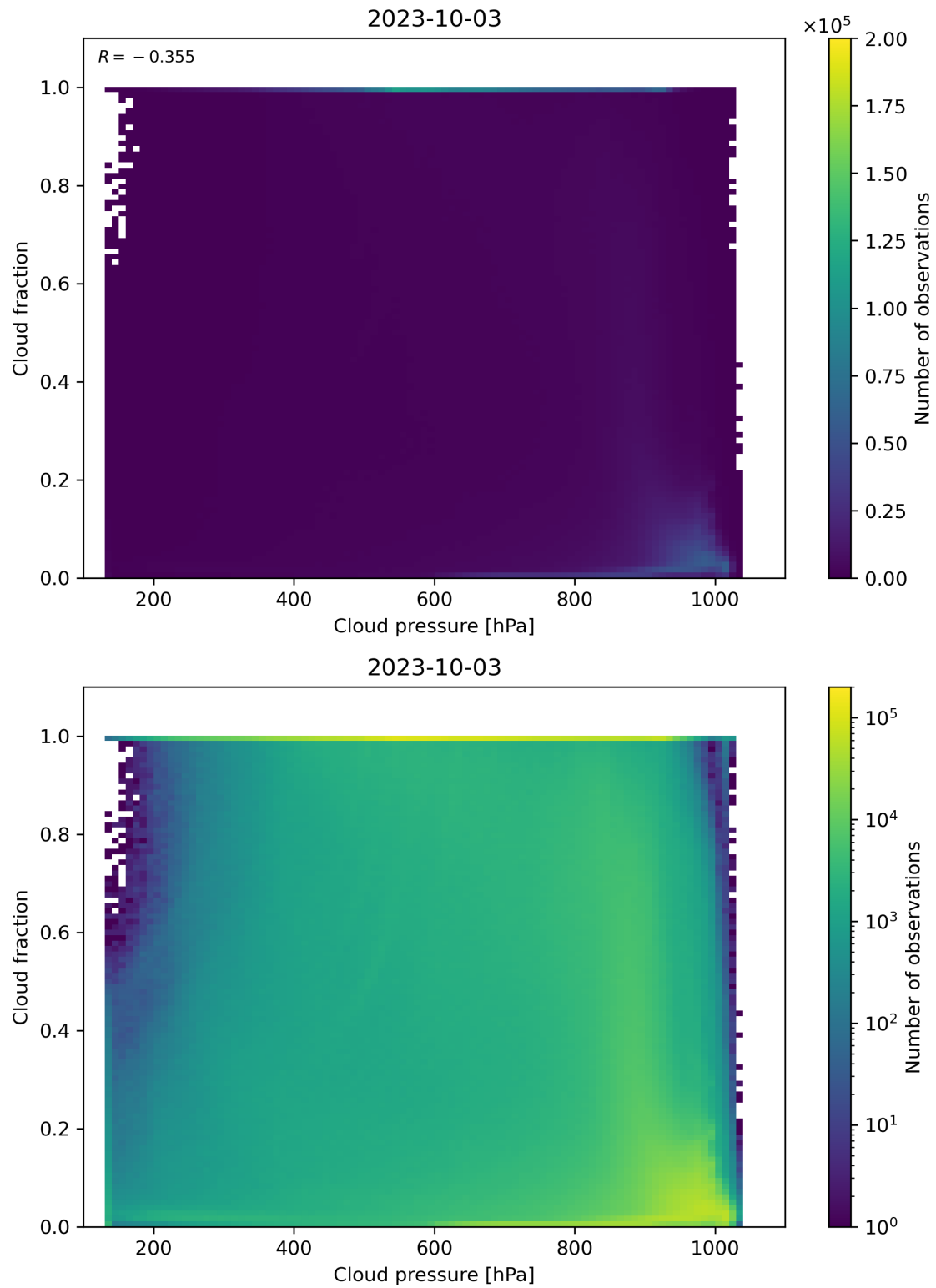
Figure 87: Scatter density plot of “Cloud pressure” against “Cloud fraction” for 2023-10-02 to 2023-10-04.
