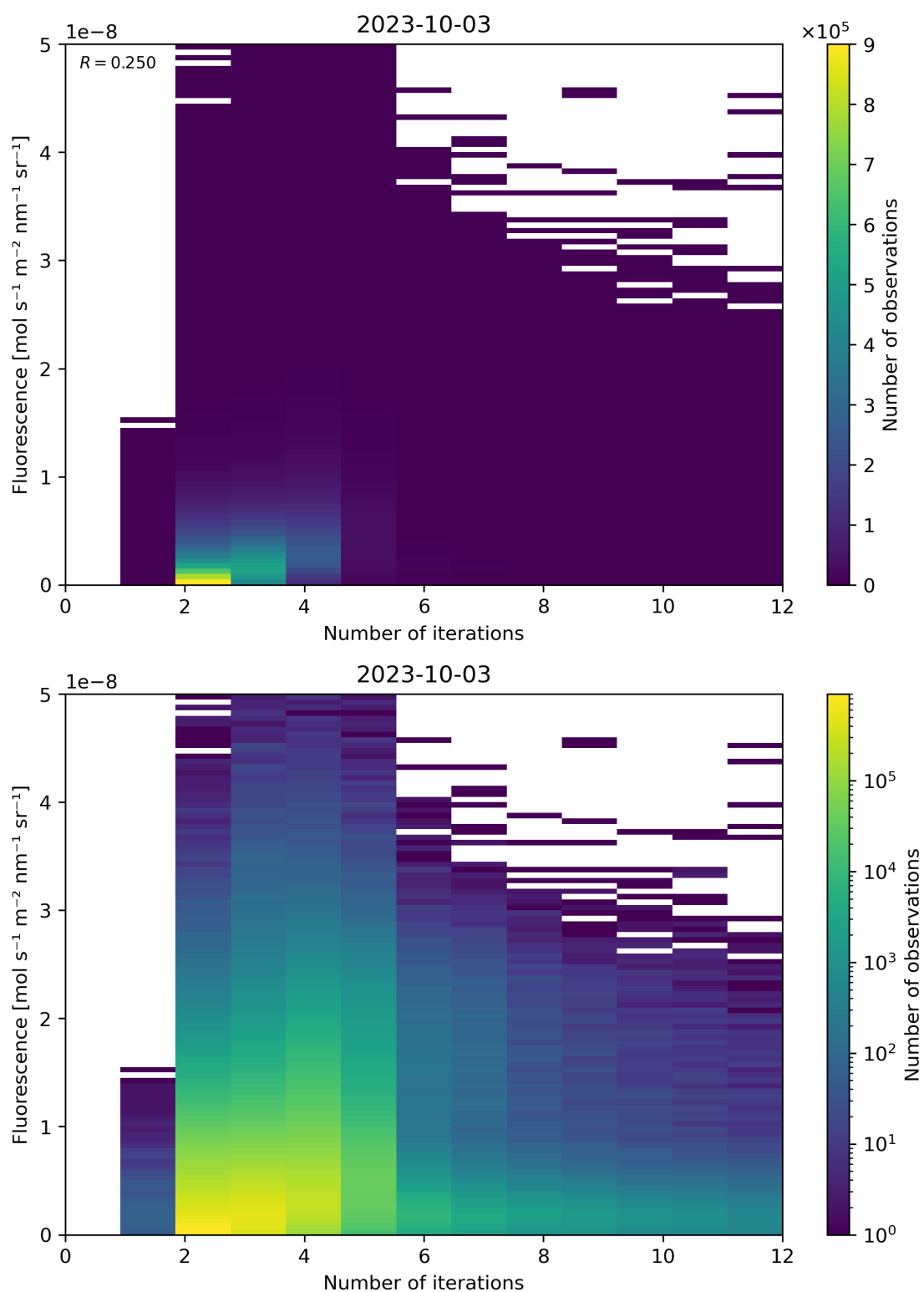
Figure 107: Scatter density plot of “Number of iterations” against “Fluorescence” for 2023-10-02 to 2023-10-04.
