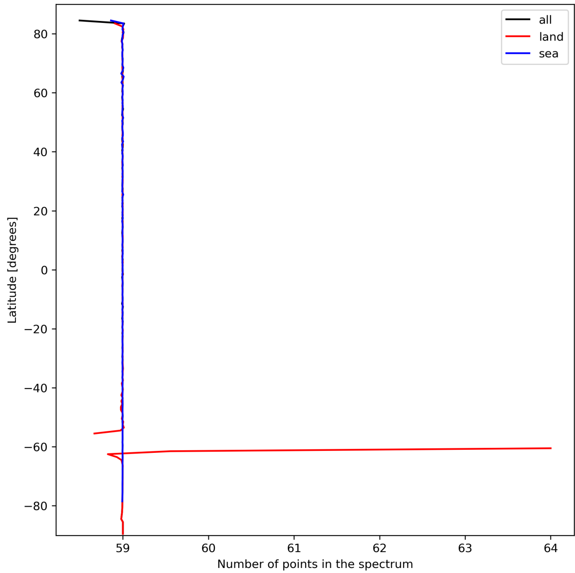
Figure 27: Zonal average of “Number of points in the spectrum” for 2023-10-02 to 2023-10-04.
