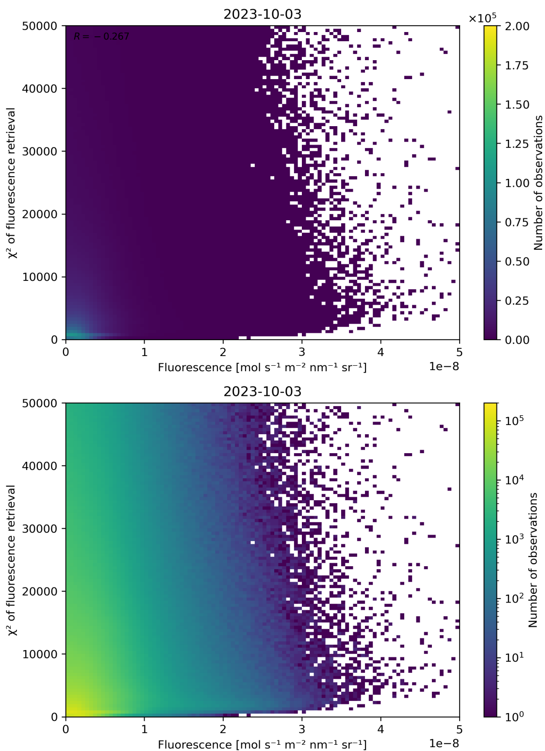
Figure 93: Scatter density plot of “Fluorescence” against “ \chi^2 of fluorescence retrieval” for 2023-10-02 to 2023-10-04.
