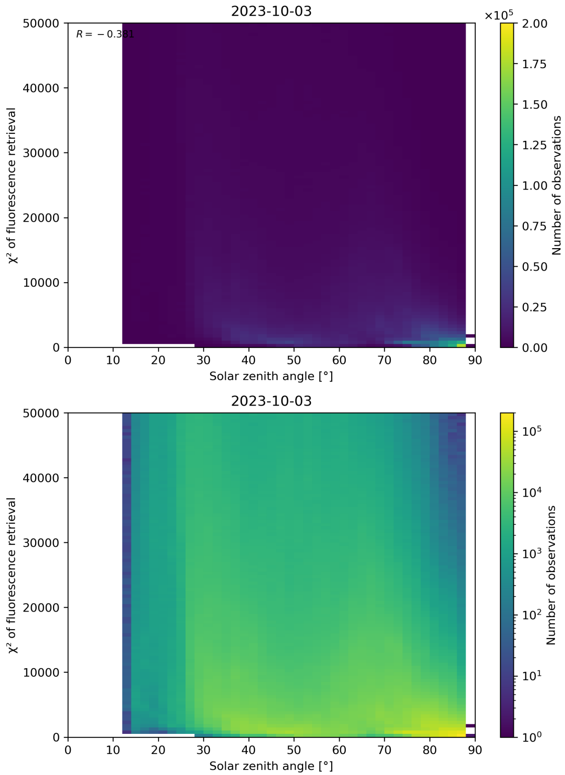
Figure 120: Scatter density plot of “Solar zenith angle” against “ \chi^2 of fluorescence retrieval” for 2023-10-02 to 2023-10-04.
