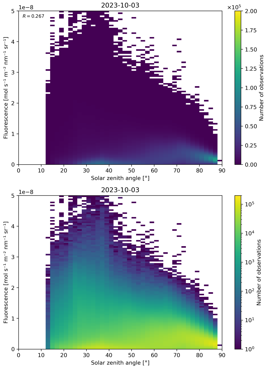
Figure 123: Scatter density plot of “Solar zenith angle” against “Fluorescence” for 2023-10-02 to 2023-10-04.
