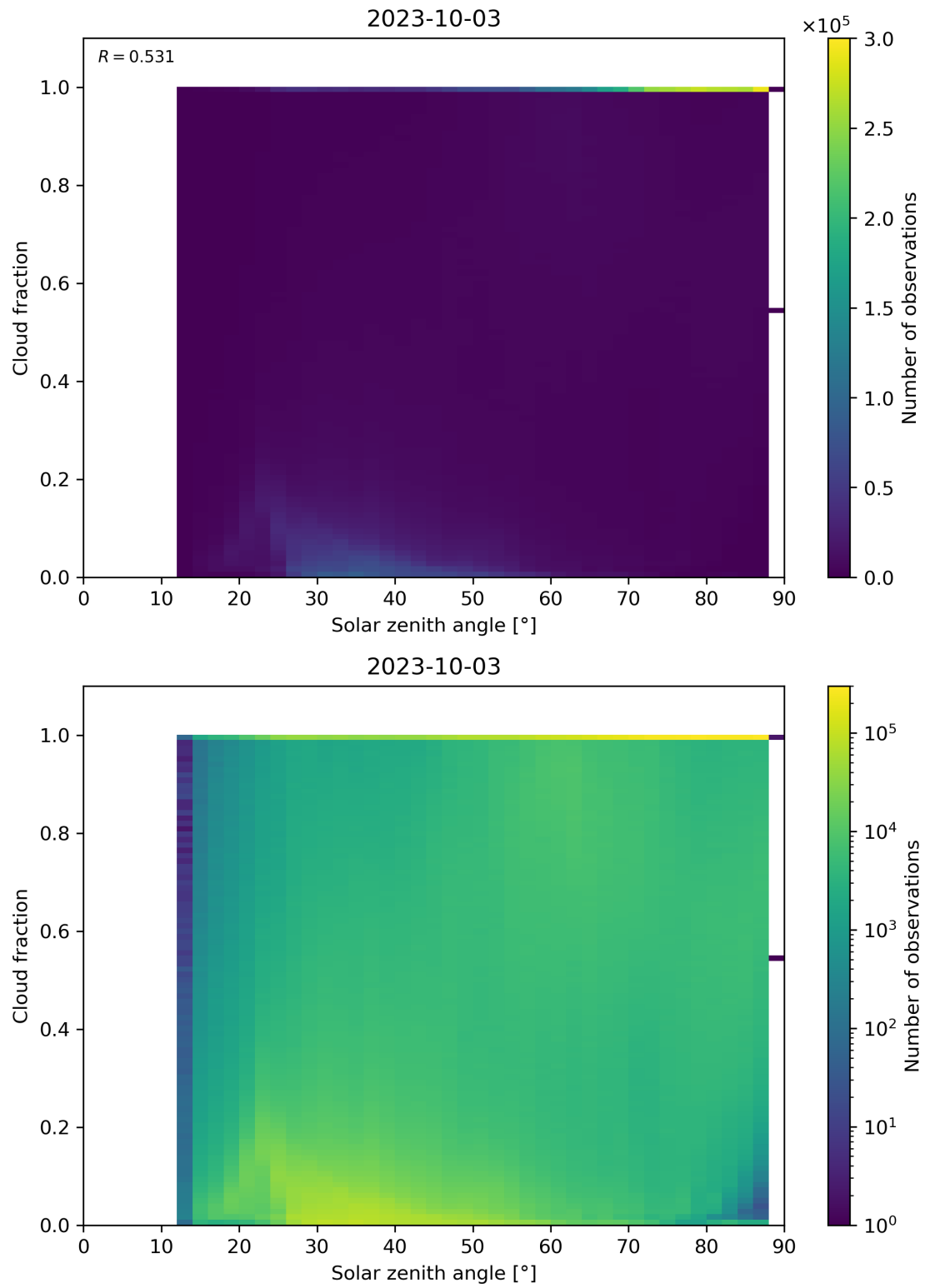
Figure 121: Scatter density plot of “Solar zenith angle” against “Cloud fraction” for 2023-10-02 to 2023-10-04.
