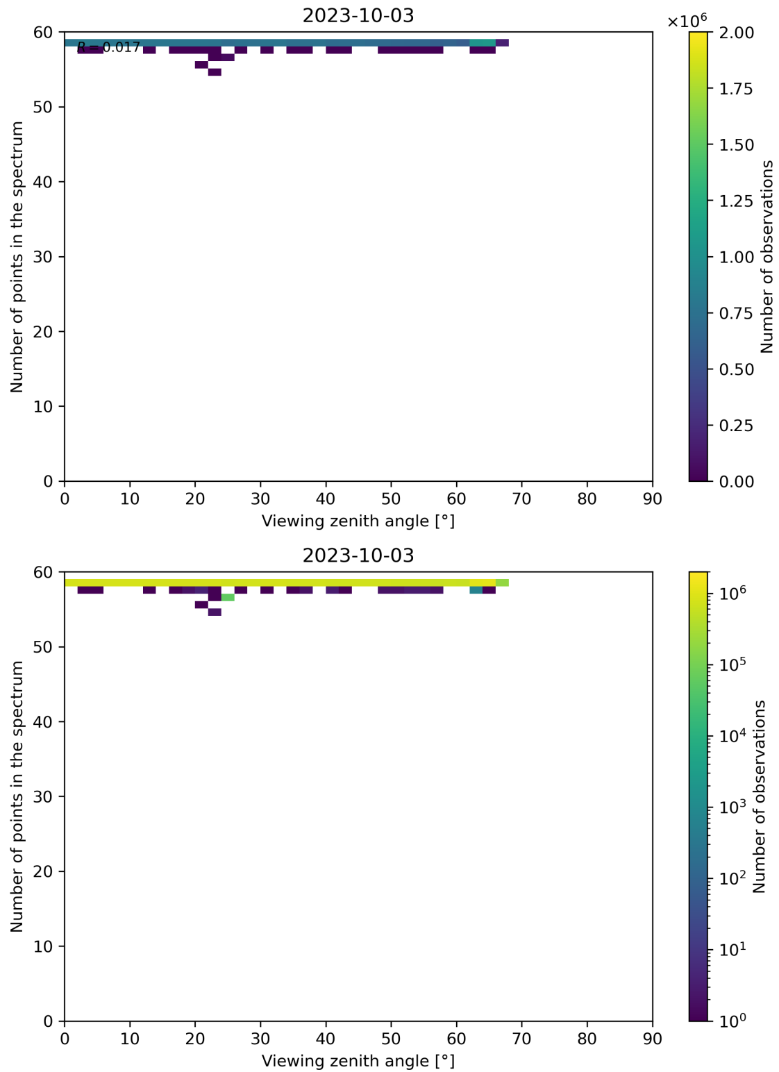
Figure 137: Scatter density plot of “Viewing zenith angle” against “Number of points in the spectrum” for 2023-10-02 to 2023-10-04.
