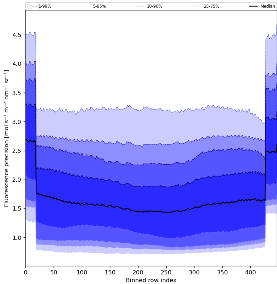
Figure 58: Along track statistics of “Fluorescence precision” for 2023-10-02 to 2023-10-04
