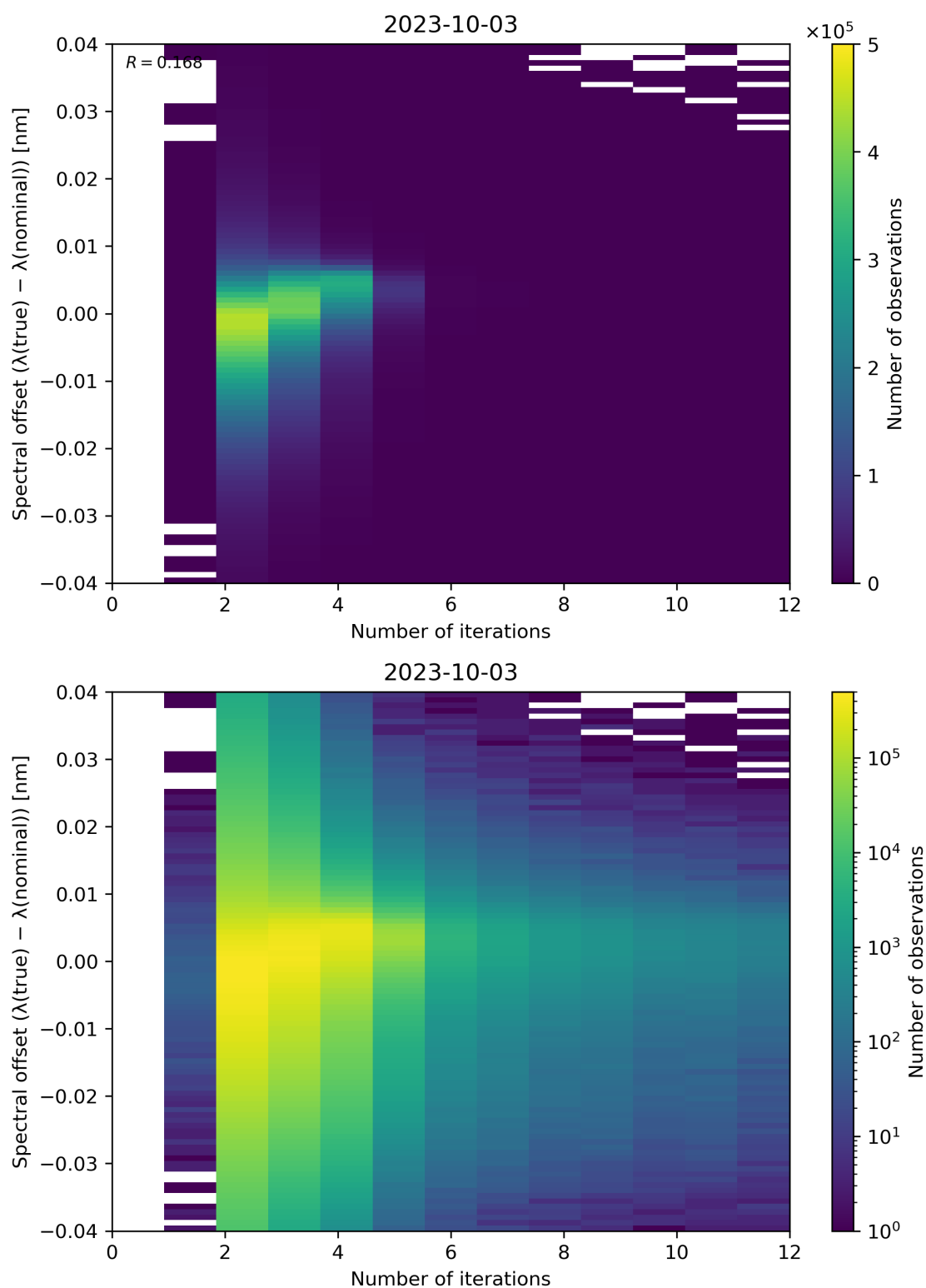
Figure 109: Scatter density plot of “Number of iterations” against “Spectral offset ( \lambda(\text{true}) - \lambda(\text{nominal}) )” for 2023-10-02 to 2023-10-04.
