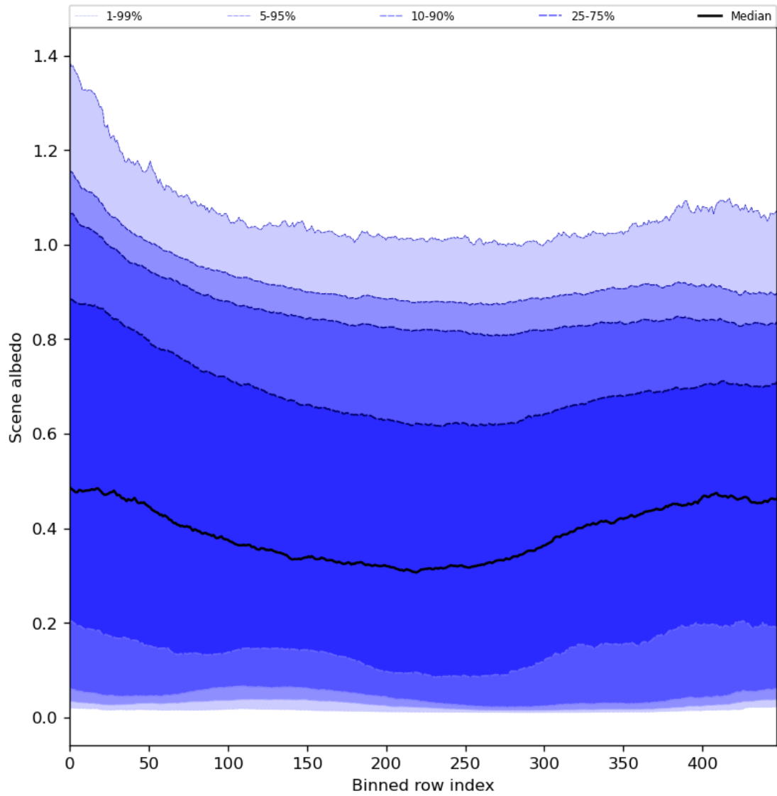
Figure 51: Along track statistics of “Scene albedo” for 2023-10-02 to 2023-10-04
