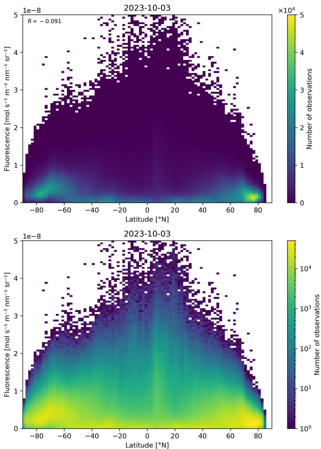
Figure 101: Scatter density plot of “Latitude” against “Fluorescence” for 2023-10-02 to 2023-10-04.
