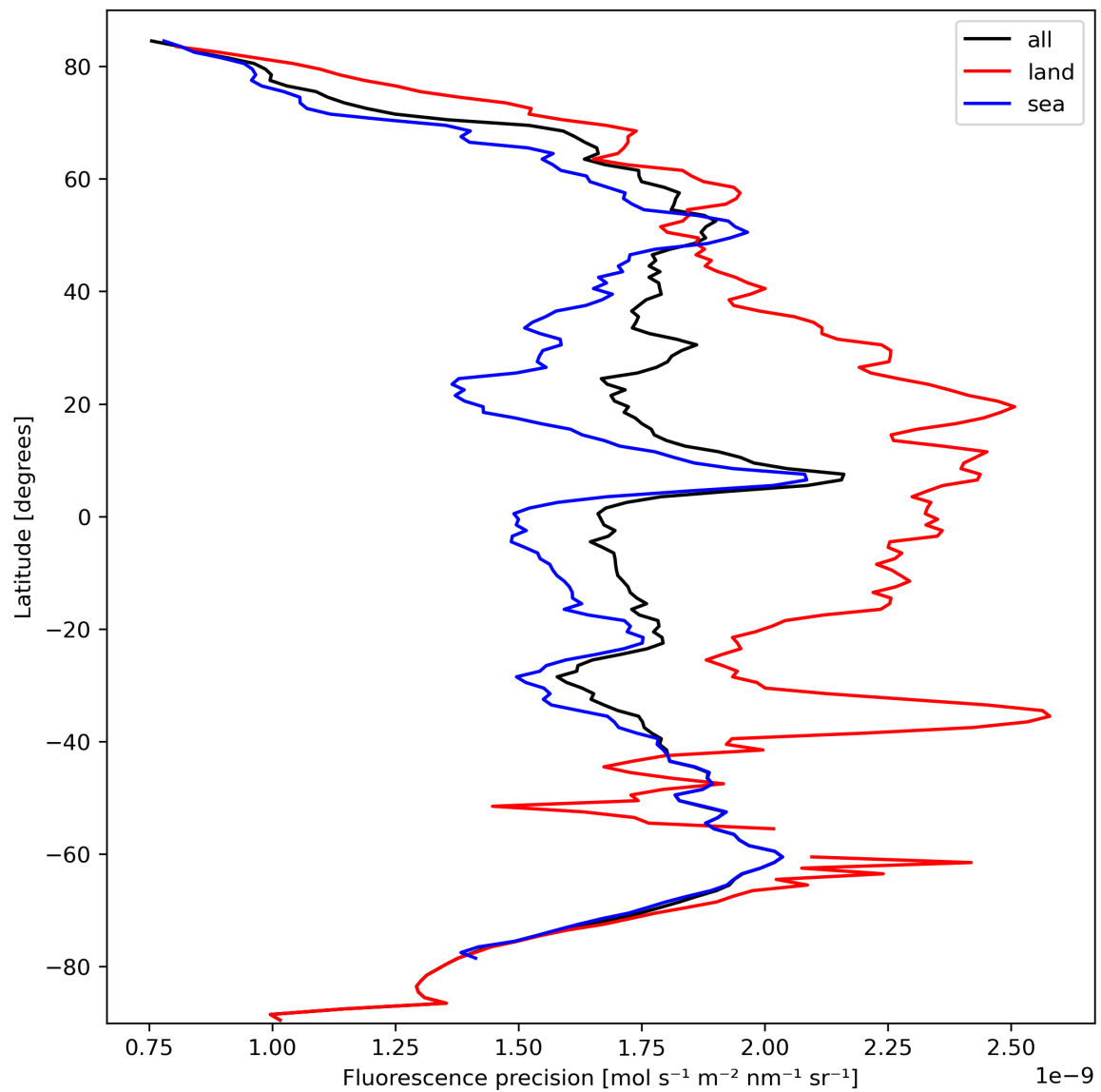
Figure 24: Zonal average of “Fluorescence precision” for 2023-10-02 to 2023-10-04.
