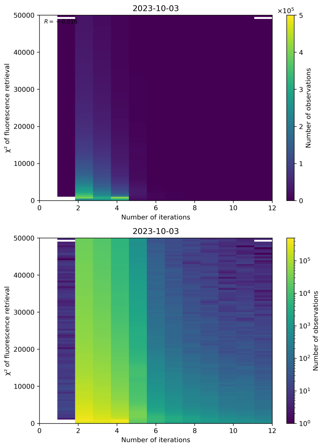
Figure 106: Scatter density plot of “Number of iterations” against “ \chi^2 of fluorescence retrieval” for 2023-10-02 to 2023-10-04.
