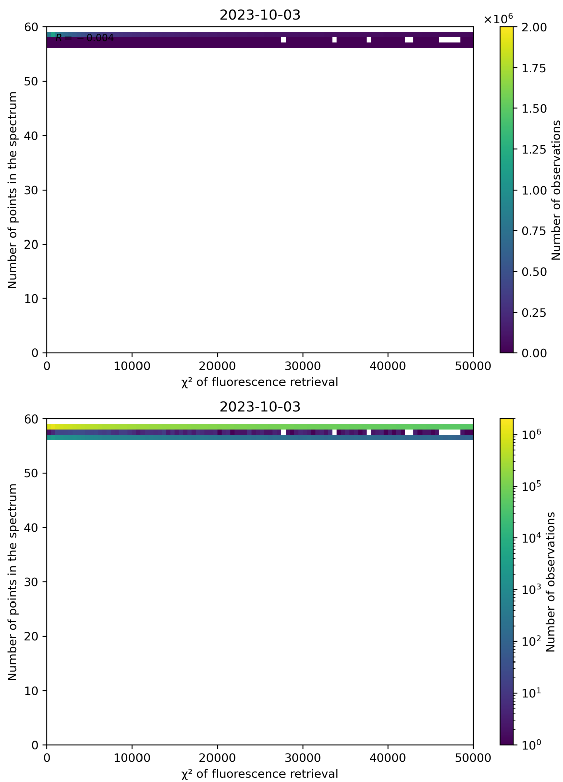
Figure 71: Scatter density plot of " \chi^2 of fluorescence retrieval" against "Number of points in the spectrum" for 2023-10-02 to 2023-10-04.
