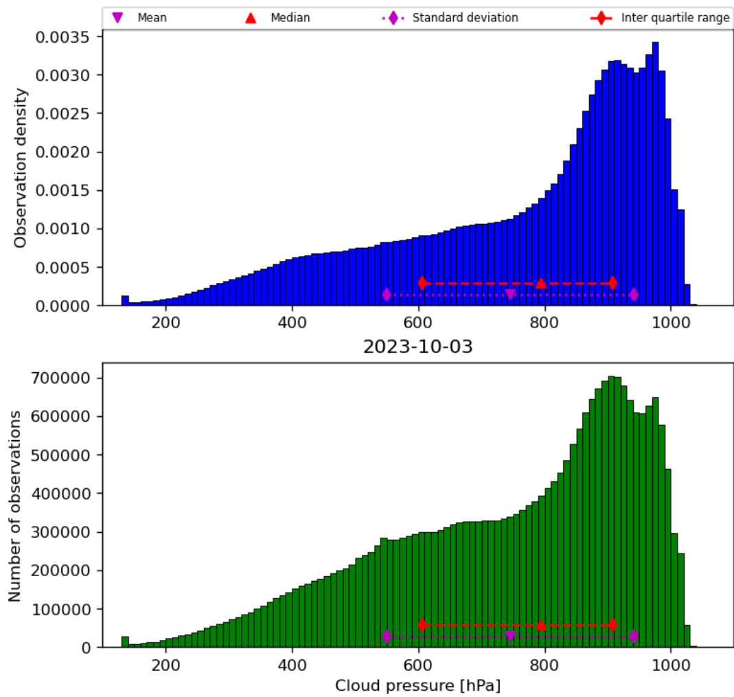
Figure 30: Histogram of “Cloud pressure” for 2023-10-02 to 2023-10-04
