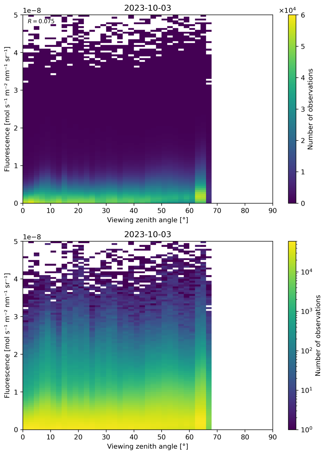
Figure 134: Scatter density plot of “Viewing zenith angle” against “Fluorescence” for 2023-10-02 to 2023-10-04.
