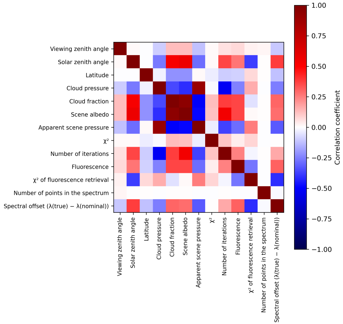
Figure 2: Map of correlation matrix for 2023-10-02 to 2023-10-04.
