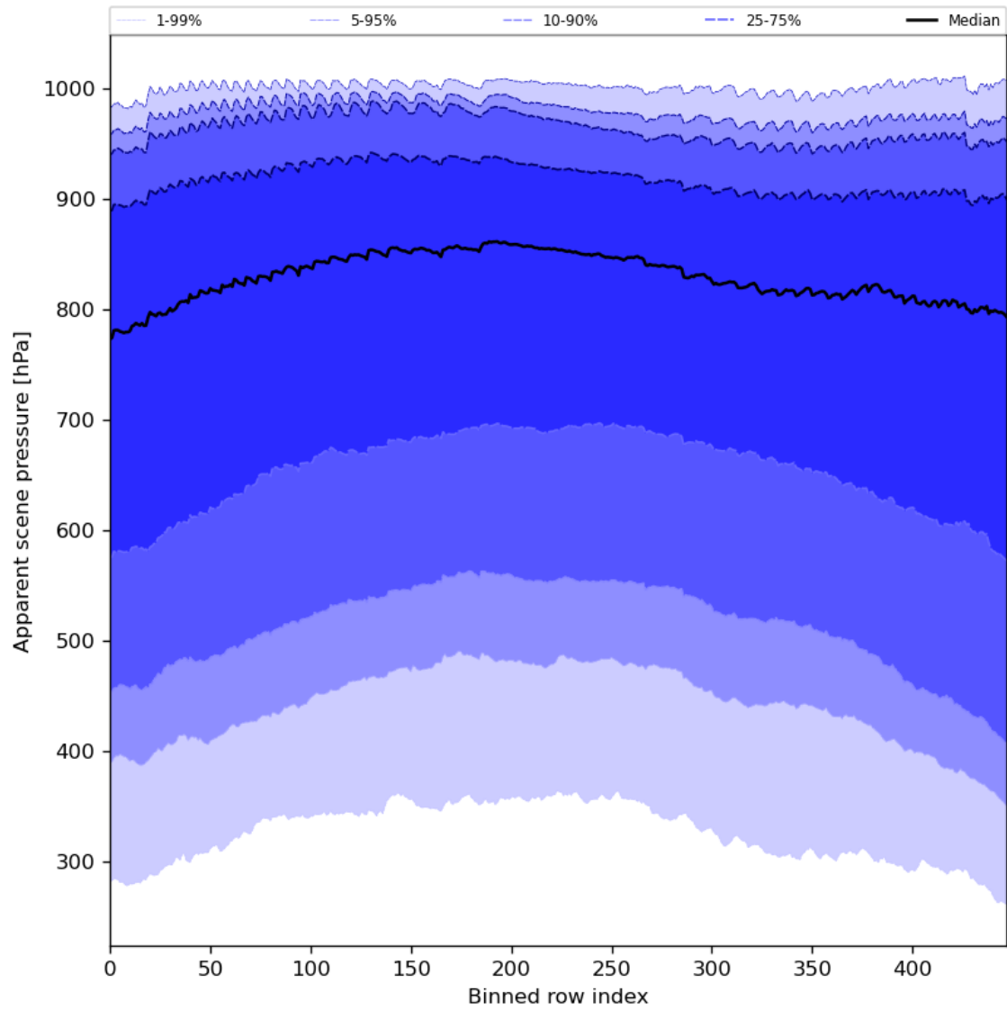
Figure 53: Along track statistics of “Apparent scene pressure” for 2023-10-02 to 2023-10-04
