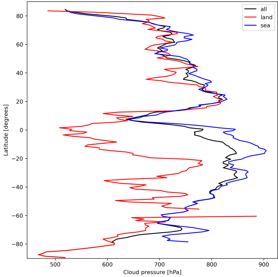
Figure 13: Zonal average of “Cloud pressure” for 2023-10-02 to 2023-10-04.
