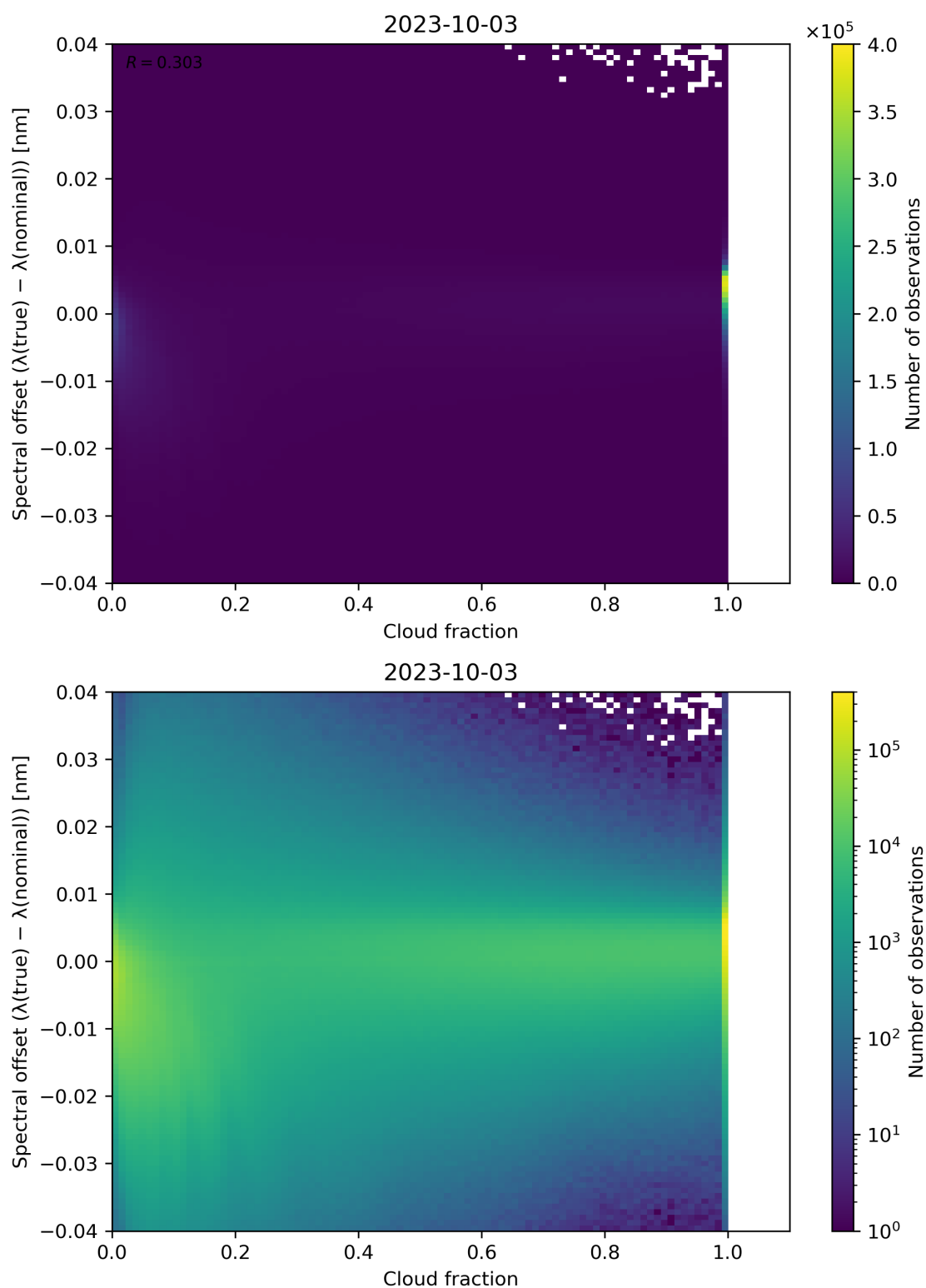
Figure 83: Scatter density plot of “Cloud fraction” against “Spectral offset ( \lambda(\text{true}) - \lambda(\text{nominal}) )” for 2023-10-02 to 2023-10-04.
