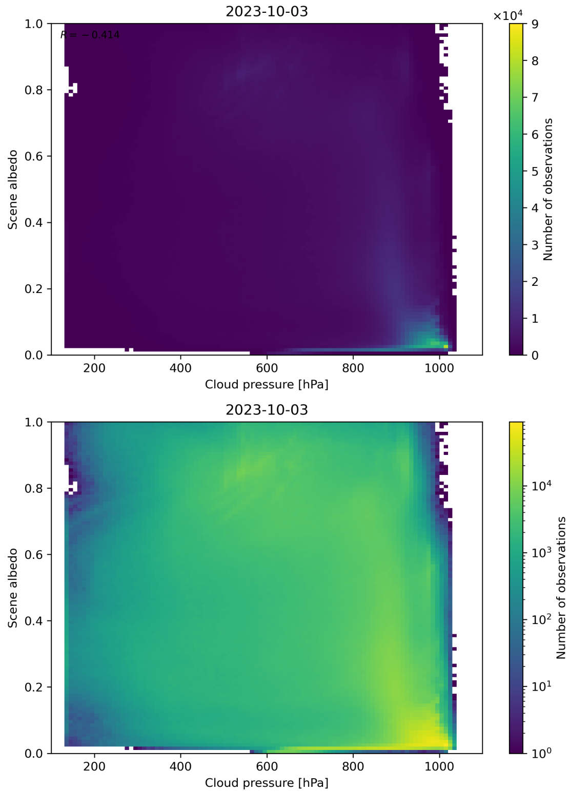
Figure 91: Scatter density plot of “Cloud pressure” against “Scene albedo” for 2023-10-02 to 2023-10-04.
