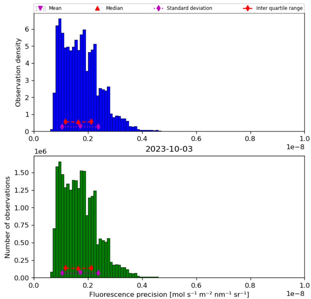
Figure 41: Histogram of “Fluorescence precision” for 2023-10-02 to 2023-10-04
