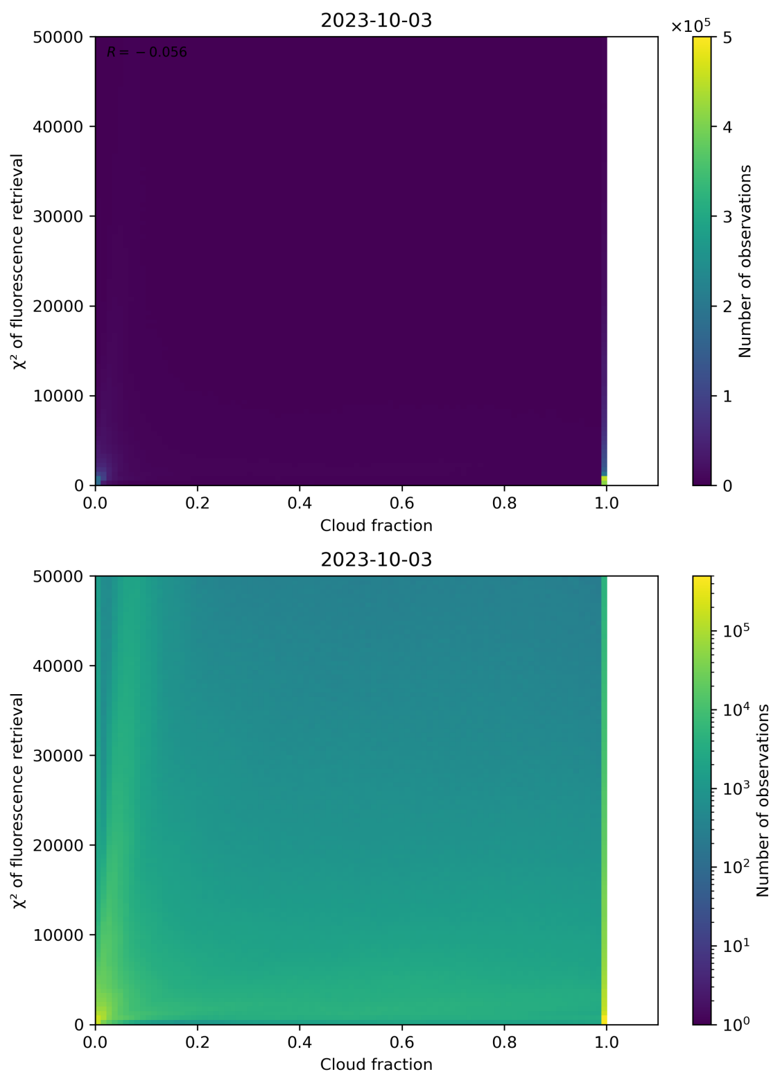
Figure 78: Scatter density plot of “Cloud fraction” against “ \chi^2 of fluorescence retrieval” for 2023-10-02 to 2023-10-04.
