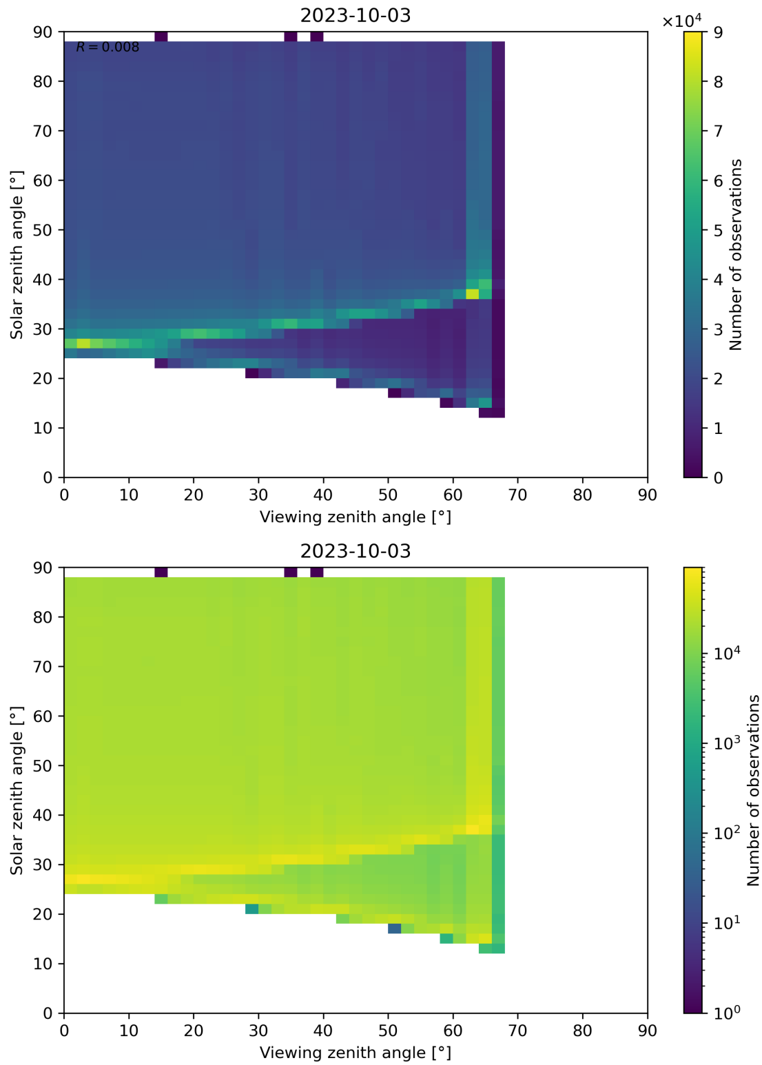
Figure 139: Scatter density plot of “Viewing zenith angle” against “Solar zenith angle” for 2023-10-02 to 2023-10-04.
