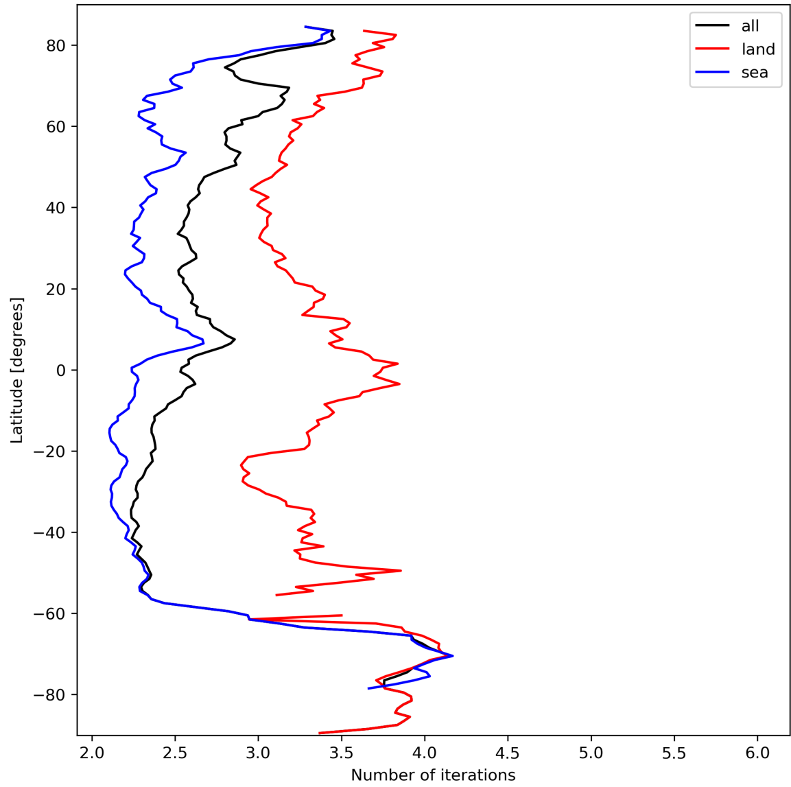
Figure 22: Zonal average of “Number of iterations” for 2023-10-02 to 2023-10-04.
