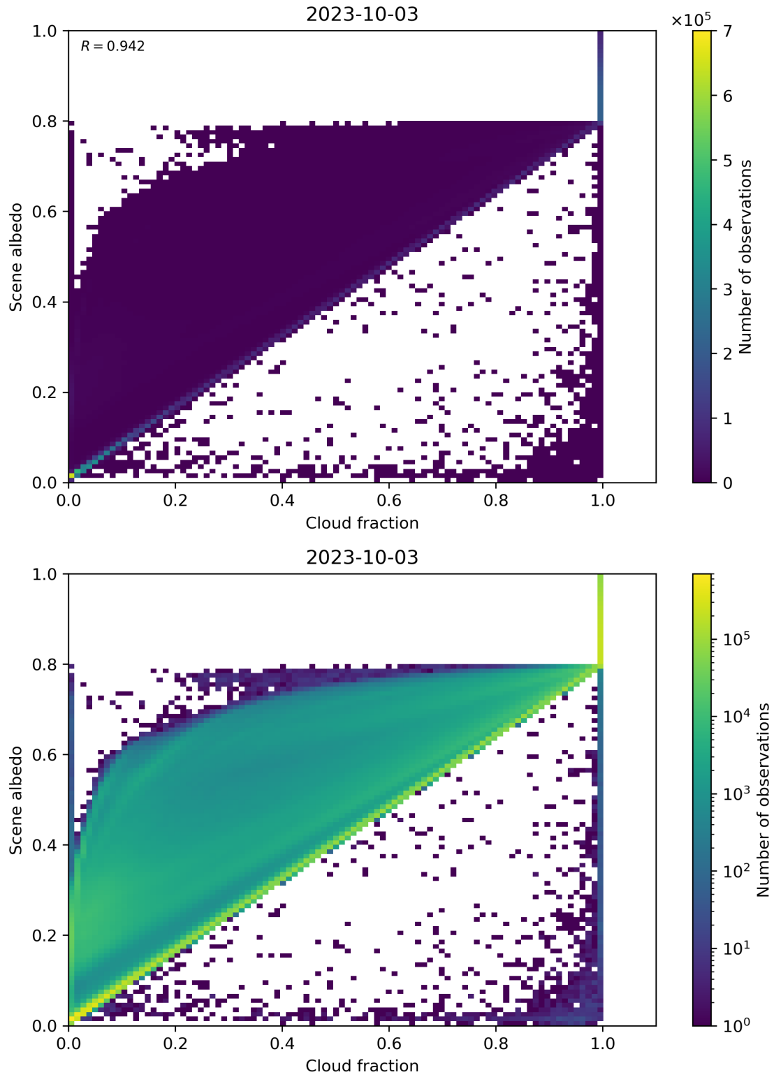
Figure 82: Scatter density plot of “Cloud fraction” against “Scene albedo” for 2023-10-02 to 2023-10-04.
