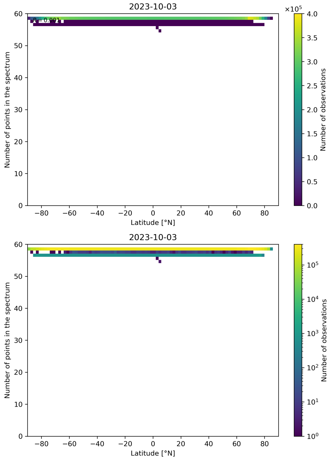
Figure 103: Scatter density plot of “Latitude” against “Number of points in the spectrum” for 2023-10-02 to 2023-10-04.
