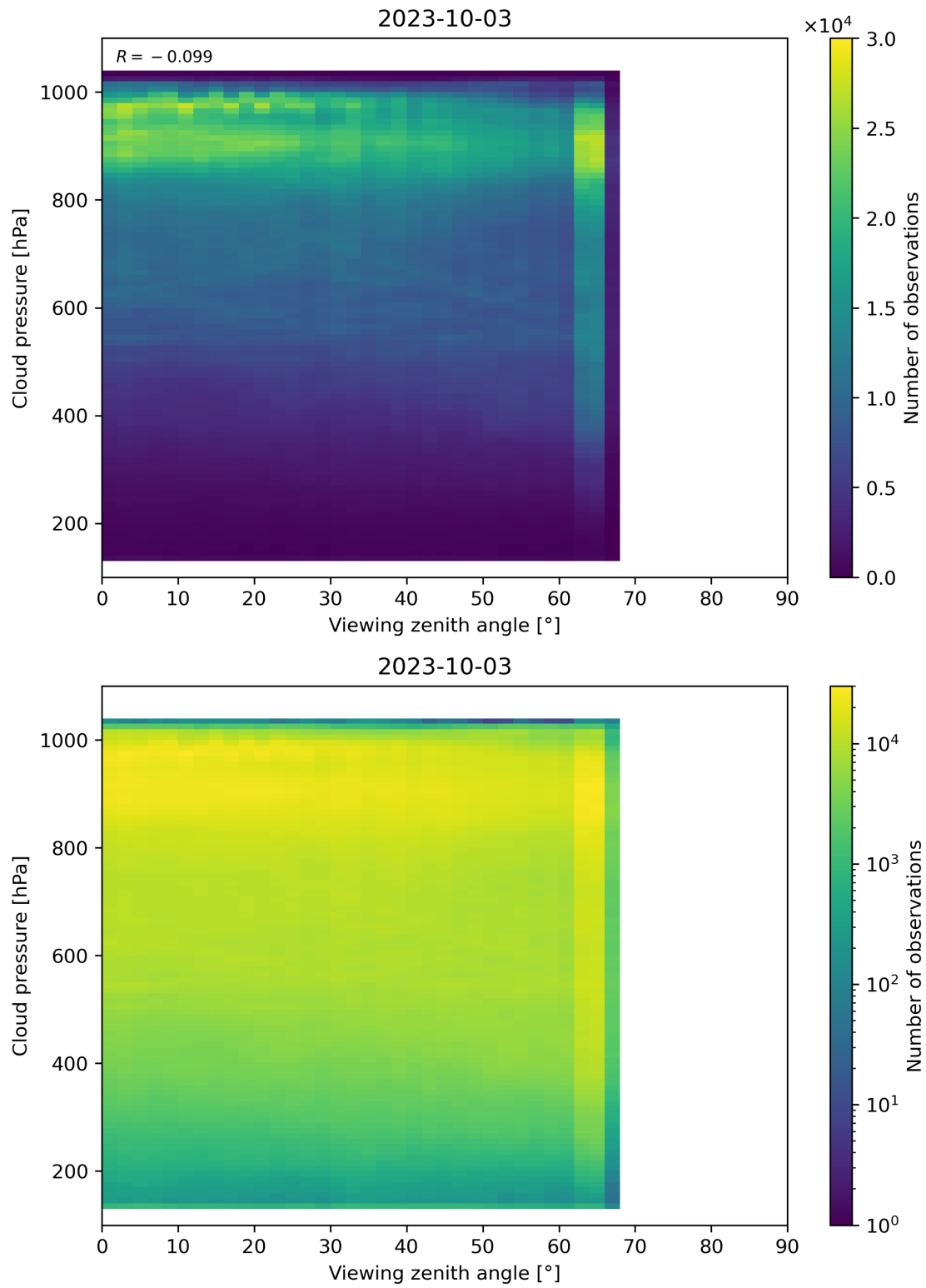
Figure 133: Scatter density plot of “Viewing zenith angle” against “Cloud pressure” for 2023-10-02 to 2023-10-04.
