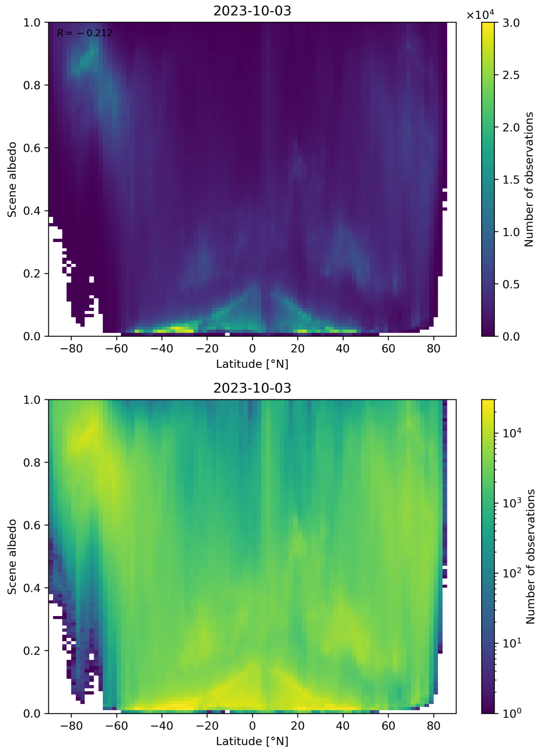
Figure 104: Scatter density plot of “Latitude” against “Scene albedo” for 2023-10-02 to 2023-10-04.
