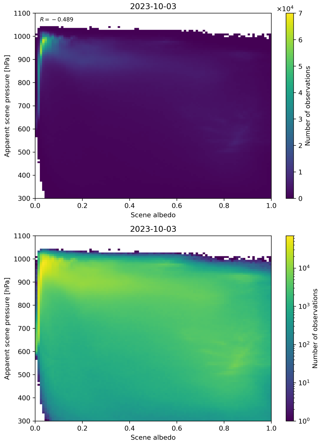
Figure 111: Scatter density plot of “Scene albedo” against “Apparent scene pressure” for 2023-10-02 to 2023-10-04.
