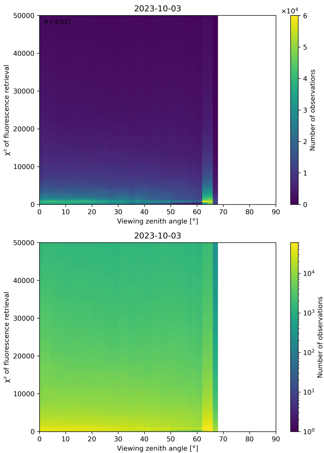
Figure 131: Scatter density plot of “Viewing zenith angle” against “ \chi^2 of fluorescence retrieval” for 2023-10-02 to 2023-10-04.
