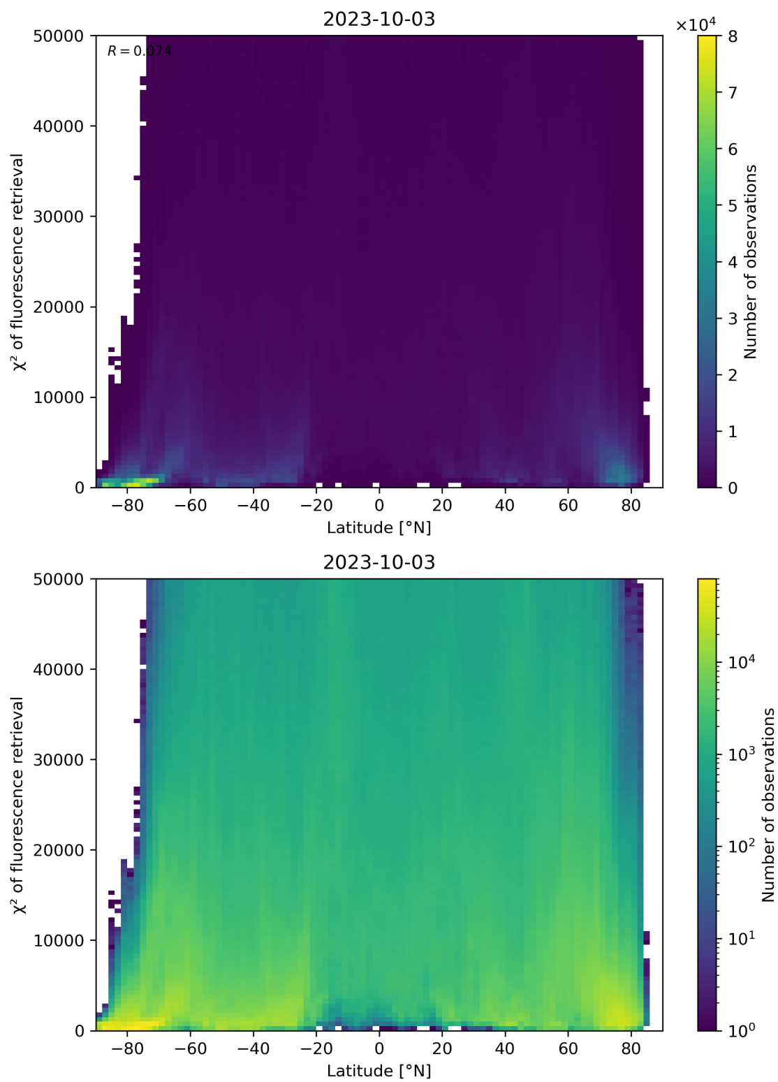
Figure 98: Scatter density plot of “Latitude” against “ \chi^2 of fluorescence retrieval” for 2023-10-02 to 2023-10-04.
