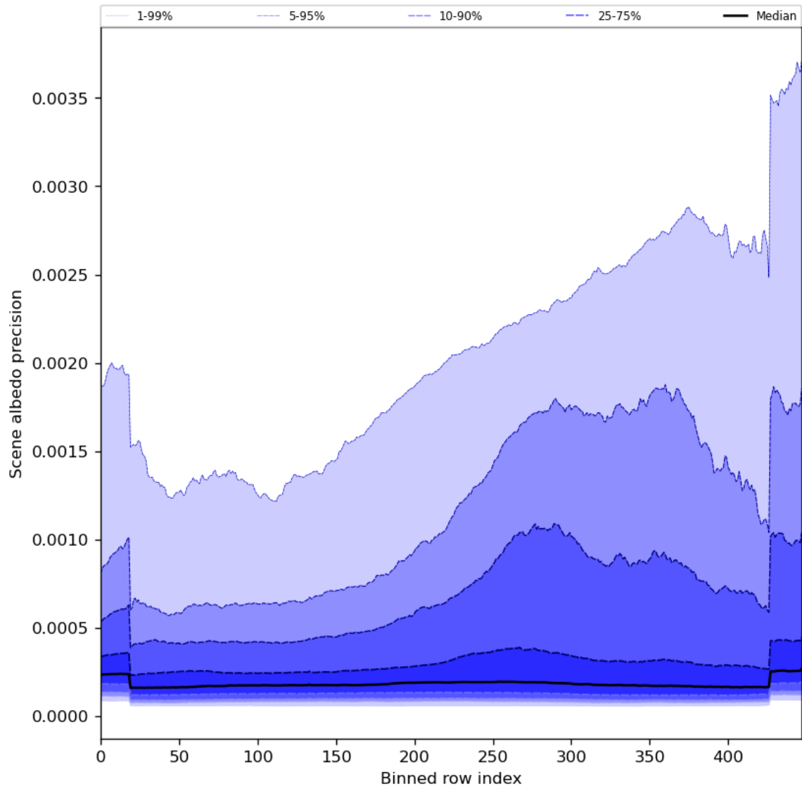
Figure 52: Along track statistics of “Scene albedo precision” for 2023-10-02 to 2023-10-04
