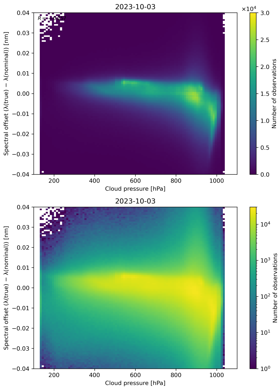
Figure 92: Scatter density plot of “Cloud pressure” against “Spectral offset ( \lambda(\text{true}) - \lambda(\text{nominal}) )” for 2023-10-02 to 2023-10-04.
