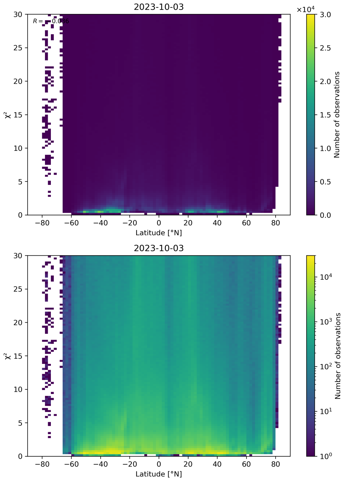
Figure 97: Scatter density plot of “Latitude” against “ \chi^2 ” for 2023-10-02 to 2023-10-04.
