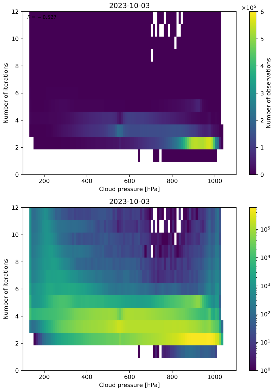
Figure 89: Scatter density plot of “Cloud pressure” against “Number of iterations” for 2023-10-02 to 2023-10-04.
