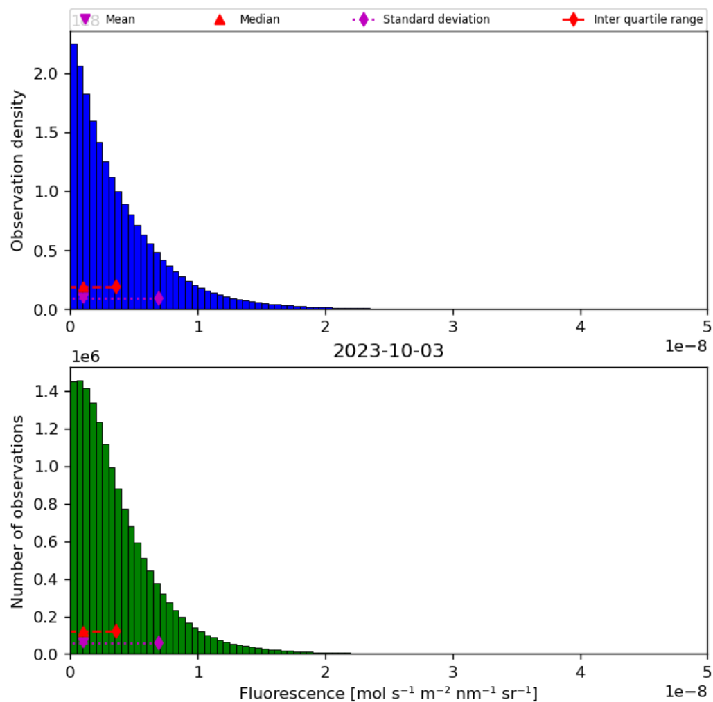
Figure 40: Histogram of “Fluorescence” for 2023-10-02 to 2023-10-04
