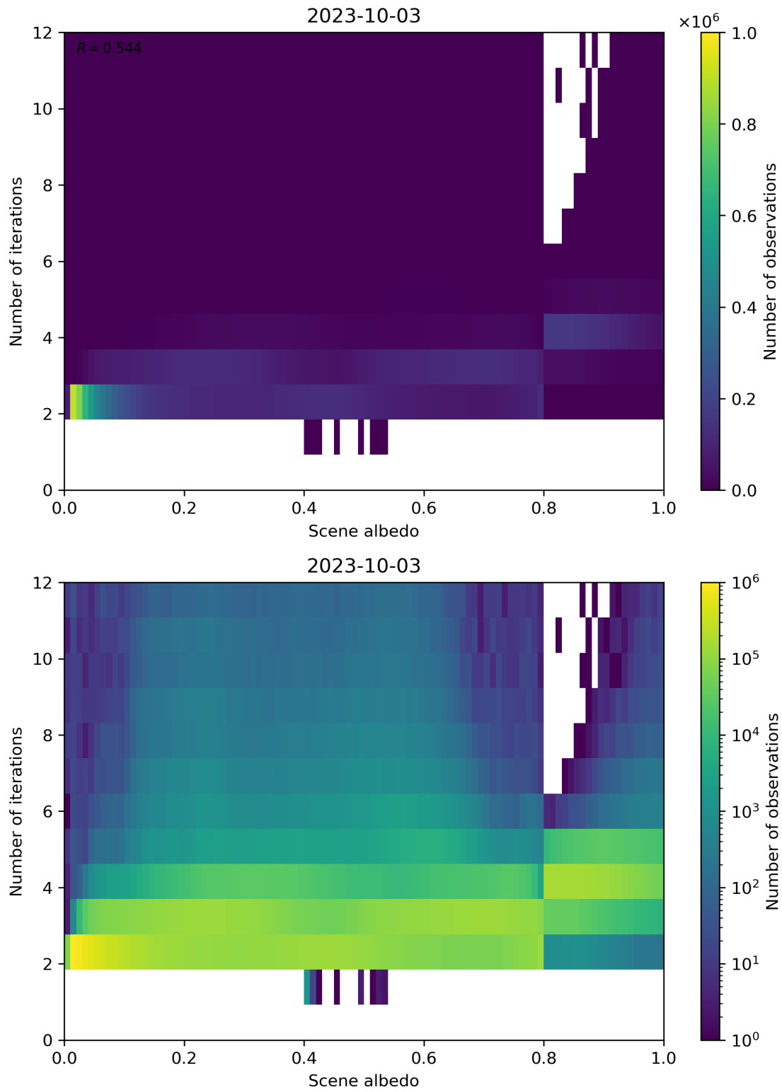
Figure 115: Scatter density plot of “Scene albedo” against “Number of iterations” for 2023-10-02 to 2023-10-04.
