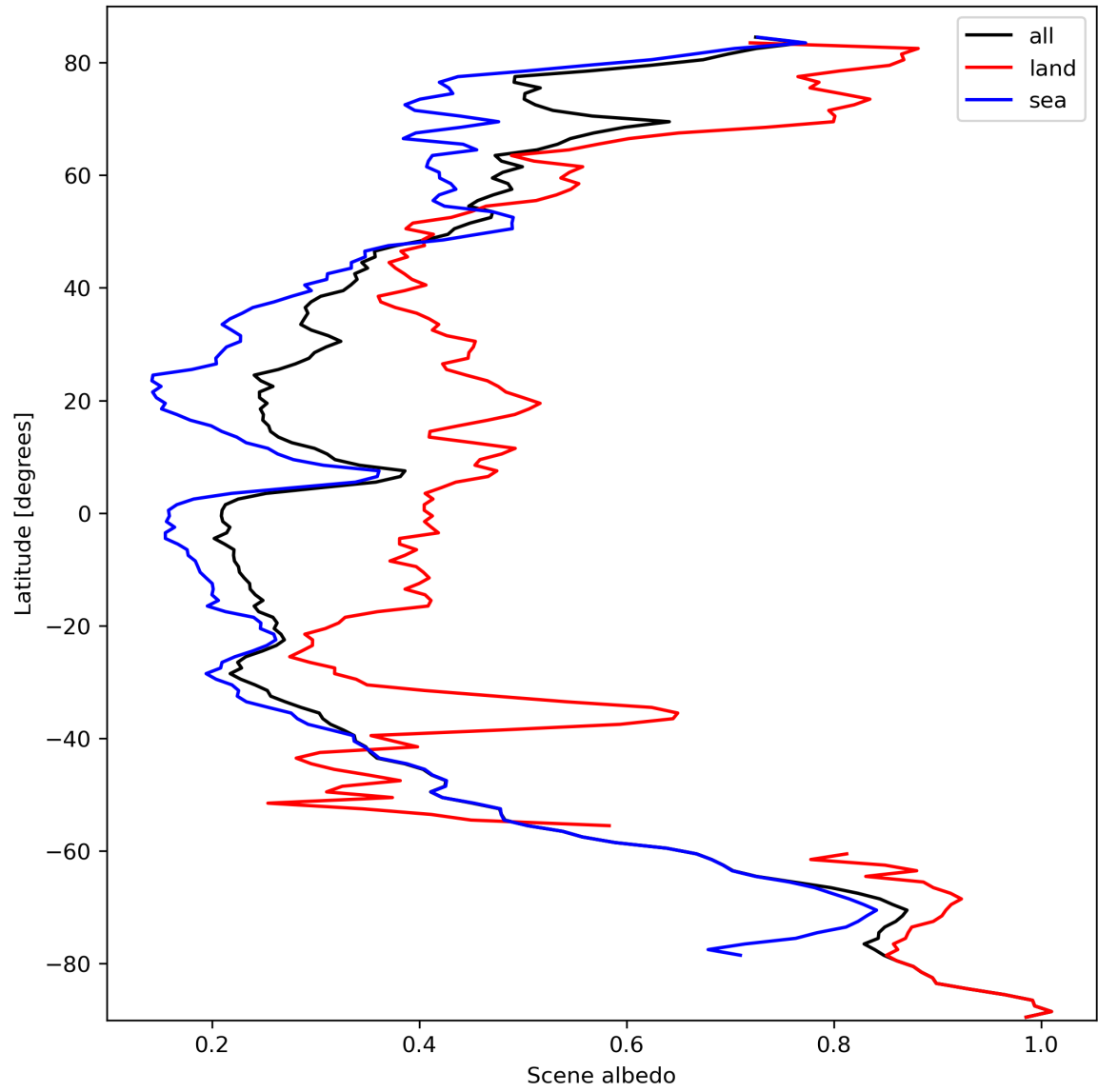
Figure 17: Zonal average of “Scene albedo” for 2023-10-02 to 2023-10-04.
