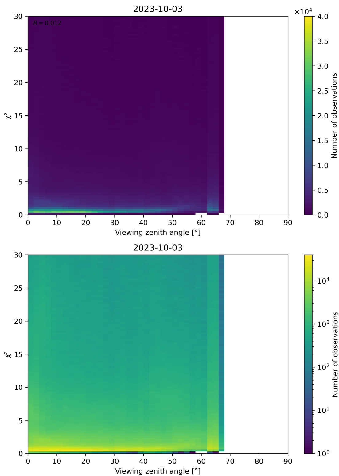
Figure 130: Scatter density plot of “Viewing zenith angle” against “ \chi^2 ” for 2023-10-02 to 2023-10-04.
