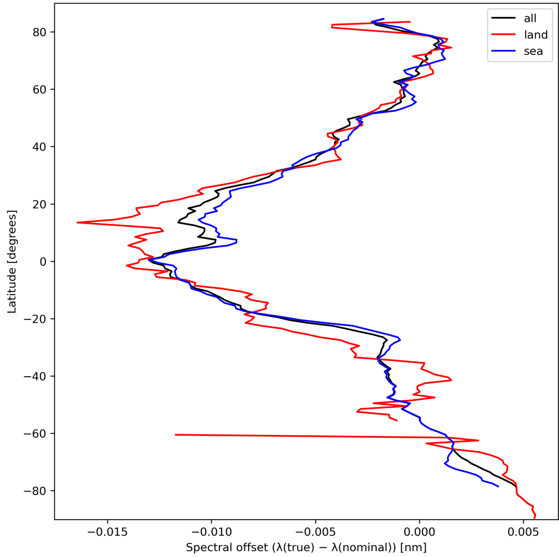
Figure 28: Zonal average of “Spectral offset ( \lambda(\text{true}) - \lambda(\text{nominal}) )” for 2023-10-02 to 2023-10-04.
