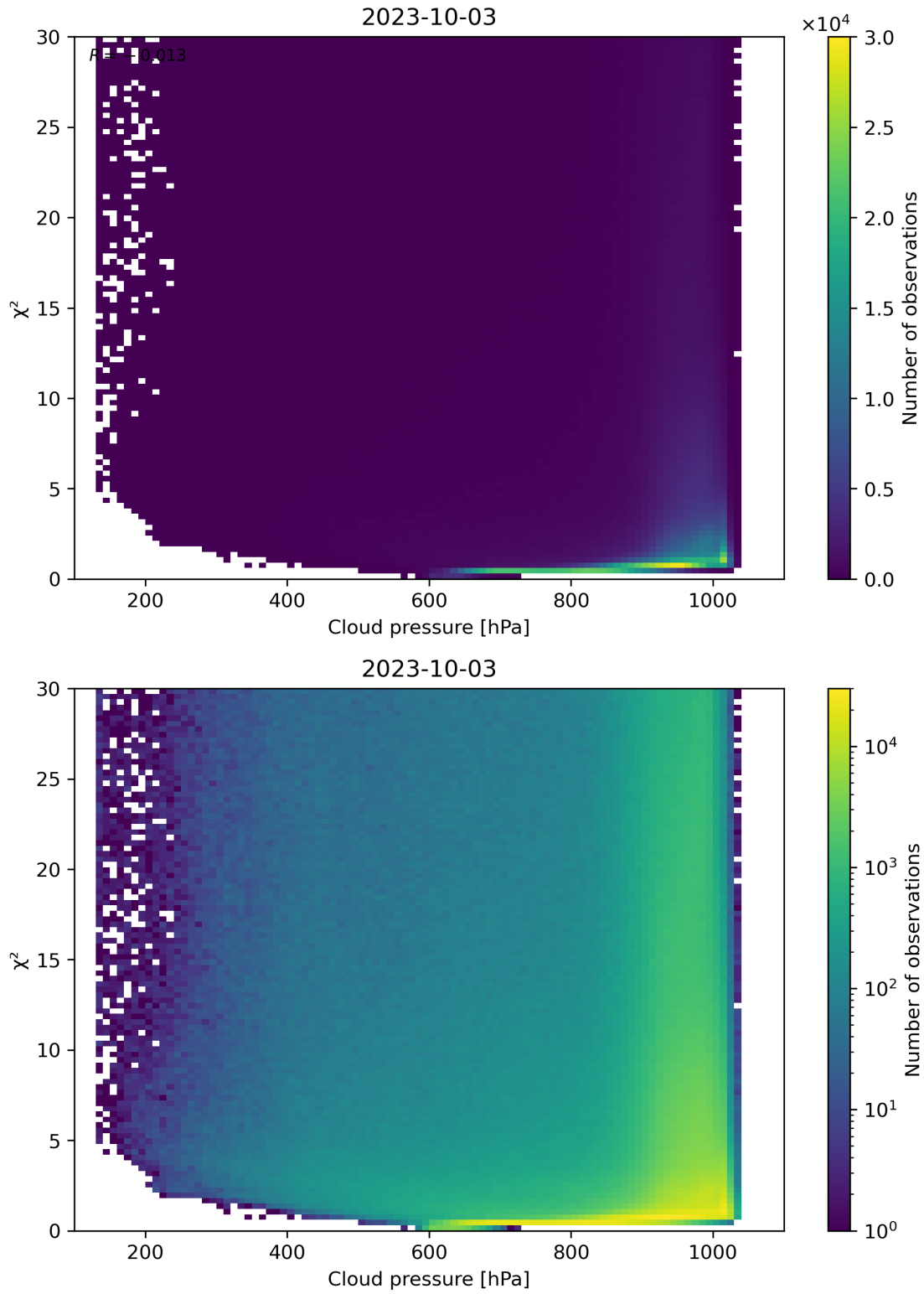
Figure 85: Scatter density plot of “Cloud pressure” against “ \chi^2 ” for 2023-10-02 to 2023-10-04.
