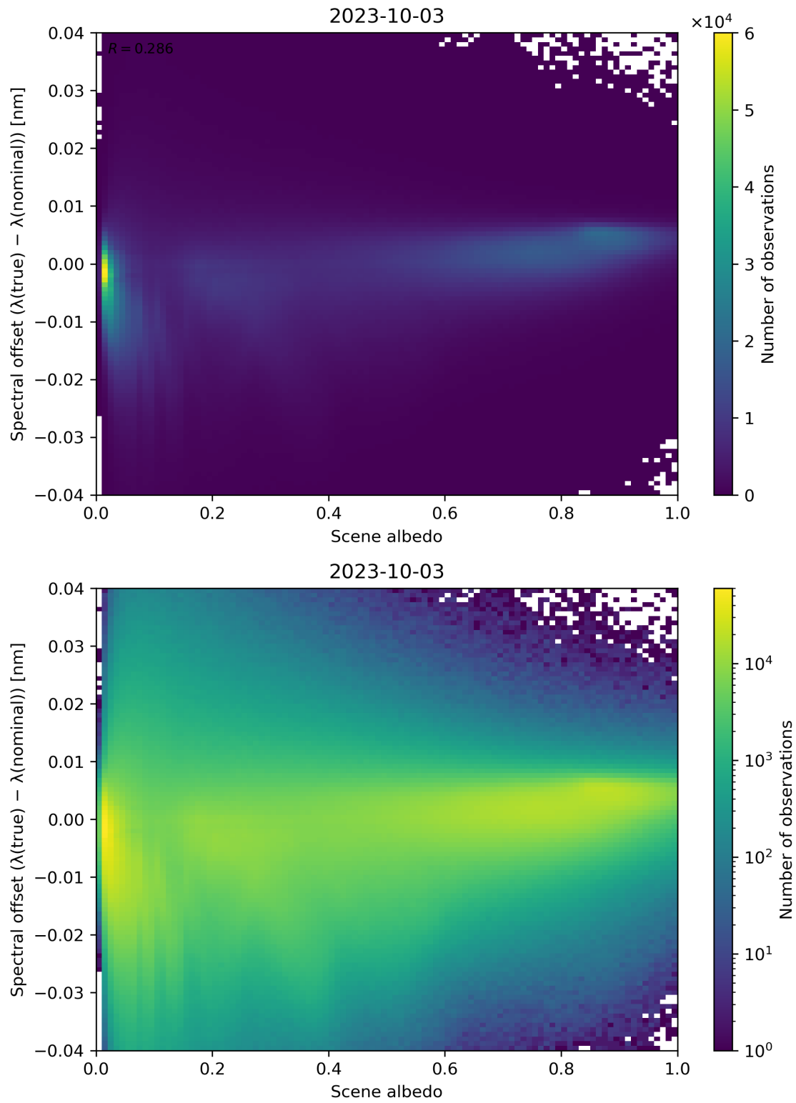
Figure 117: Scatter density plot of “Scene albedo” against “Spectral offset ( \lambda(\text{true}) - \lambda(\text{nominal}) )” for 2023-10-02 to 2023-10-04.
