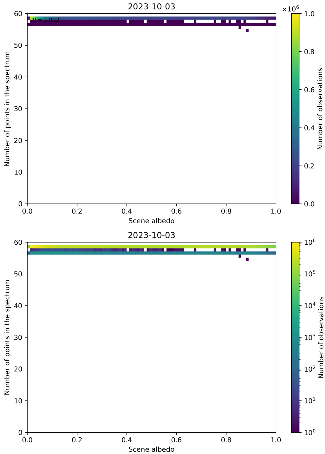
Figure 116: Scatter density plot of “Scene albedo” against “Number of points in the spectrum” for 2023-10-02 to 2023-10-04.
