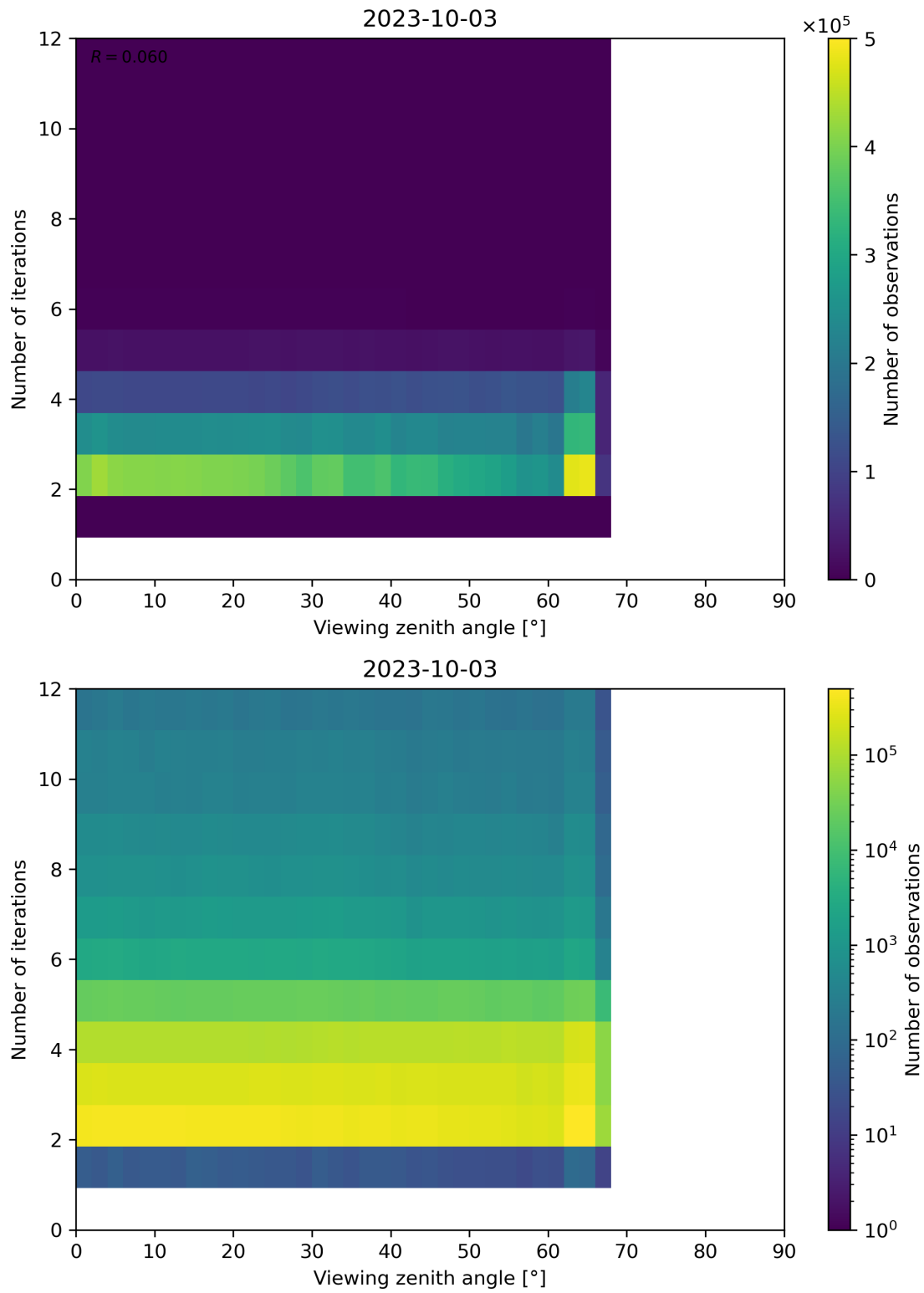
Figure 136: Scatter density plot of “Viewing zenith angle” against “Number of iterations” for 2023-10-02 to 2023-10-04.
