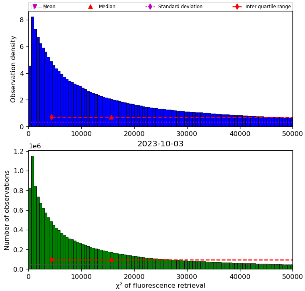
Figure 42: Histogram of “ \chi^2 of fluorescence retrieval” for 2023-10-02 to 2023-10-04
