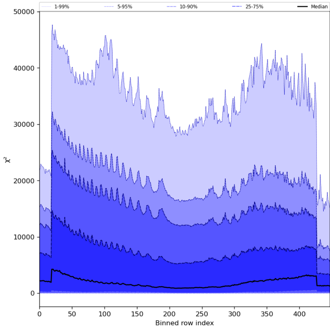
Figure 55: Along track statistics of “ \chi^2 ” for 2023-10-02 to 2023-10-04
