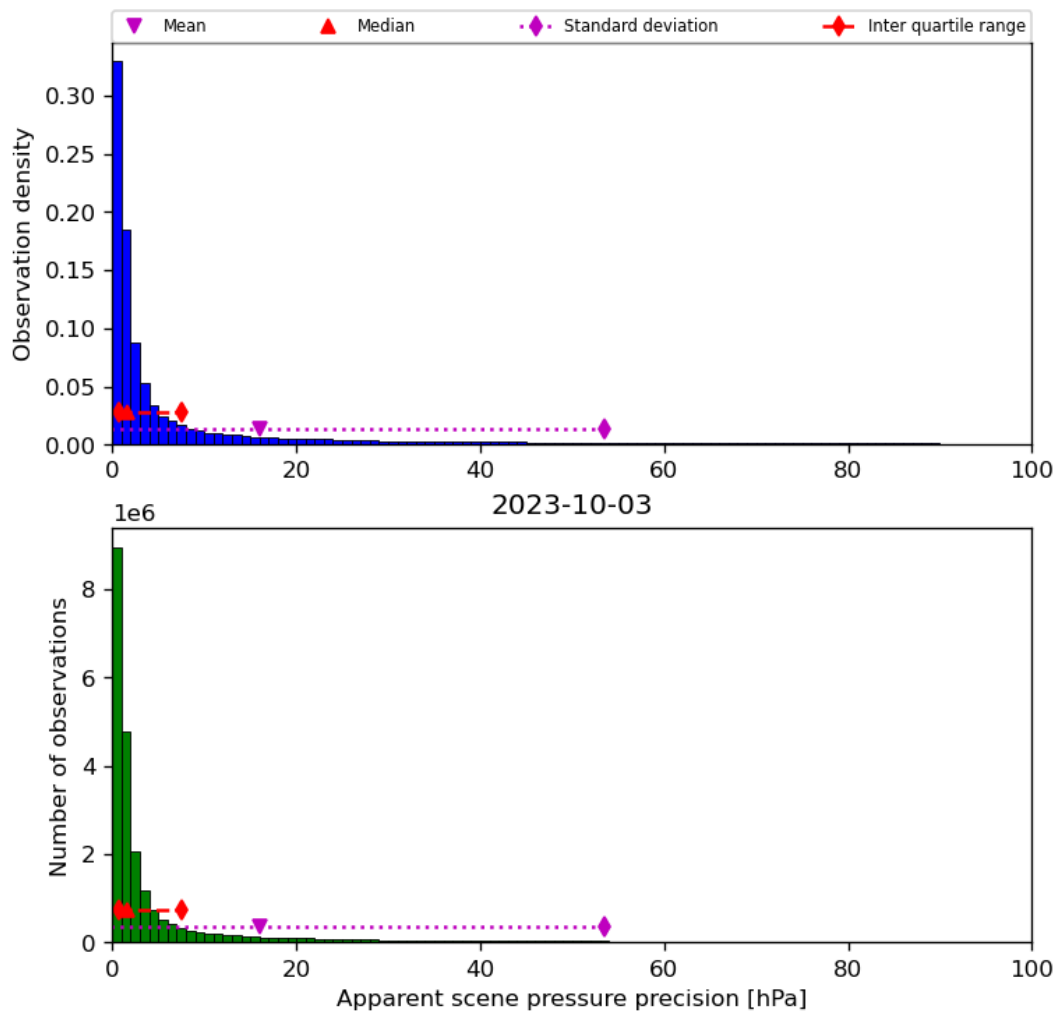
Figure 37: Histogram of “Apparent scene pressure precision” for 2023-10-02 to 2023-10-04
