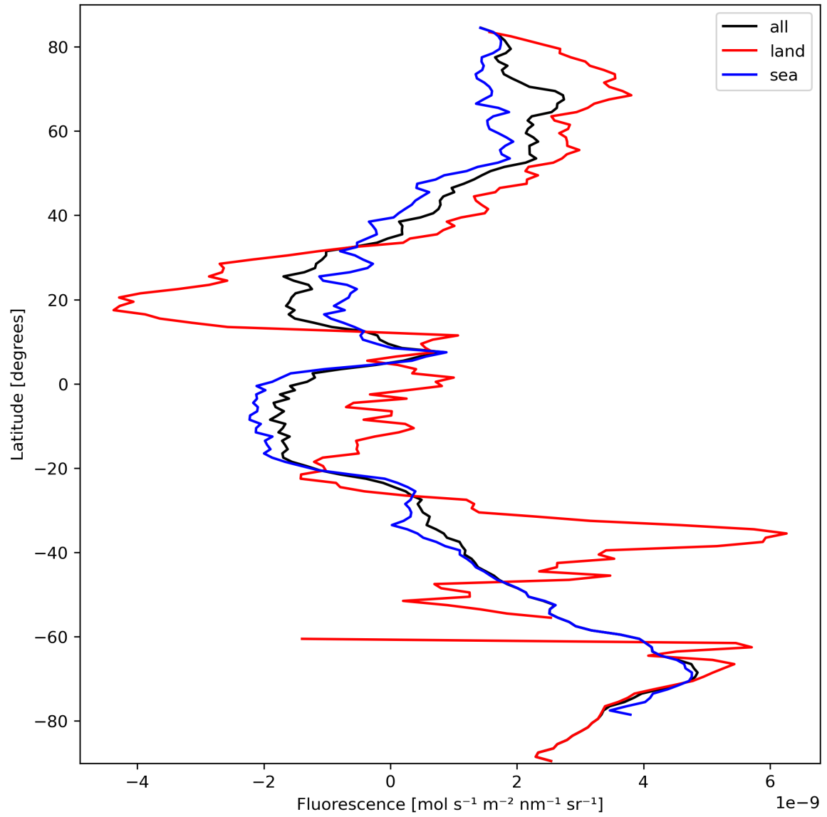
Figure 23: Zonal average of “Fluorescence” for 2023-10-02 to 2023-10-04.
