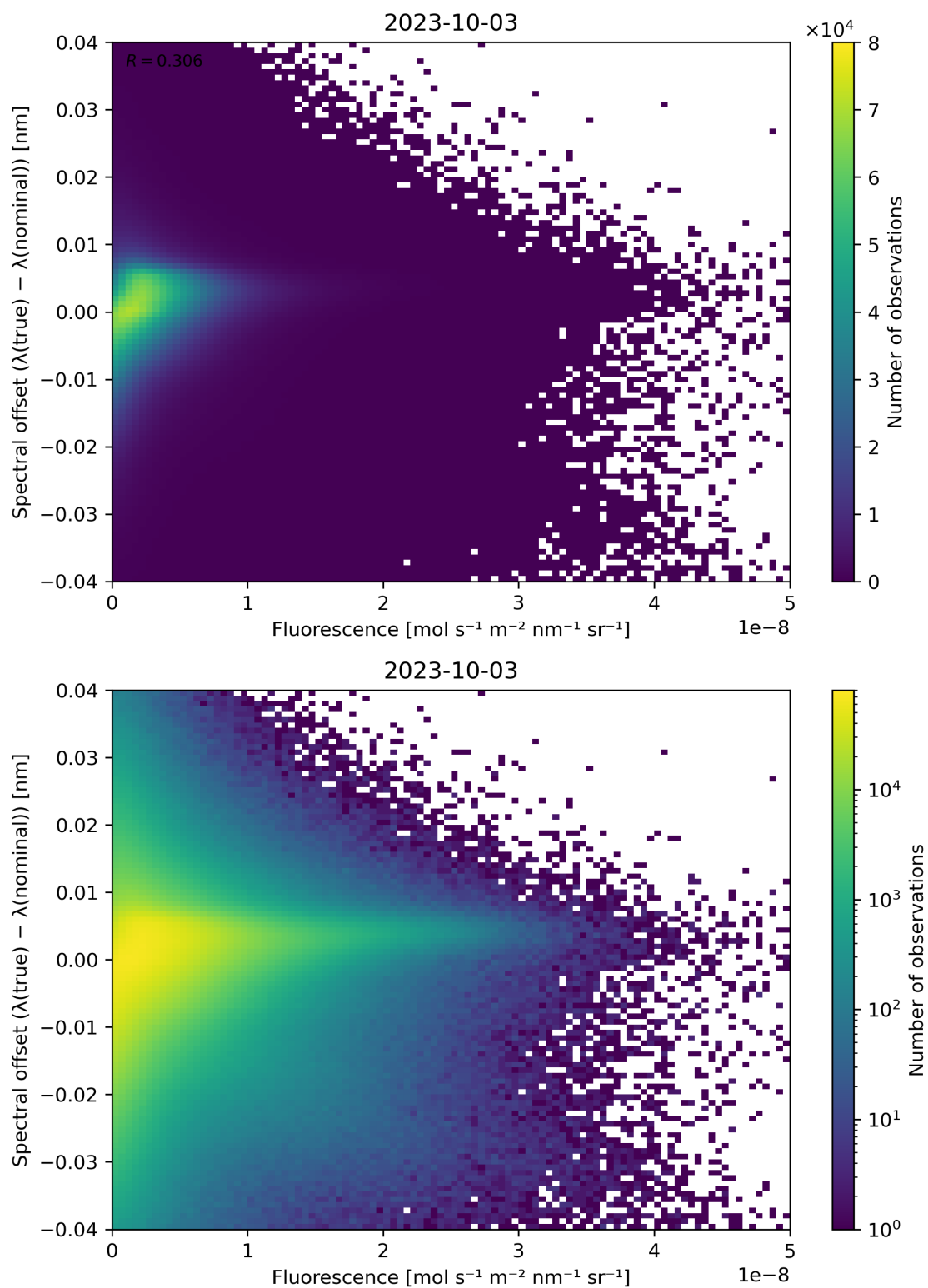
Figure 95: Scatter density plot of “Fluorescence” against “Spectral offset ( \lambda(\text{true}) - \lambda(\text{nominal}) )” for 2023-10-02 to 2023-10-04.
