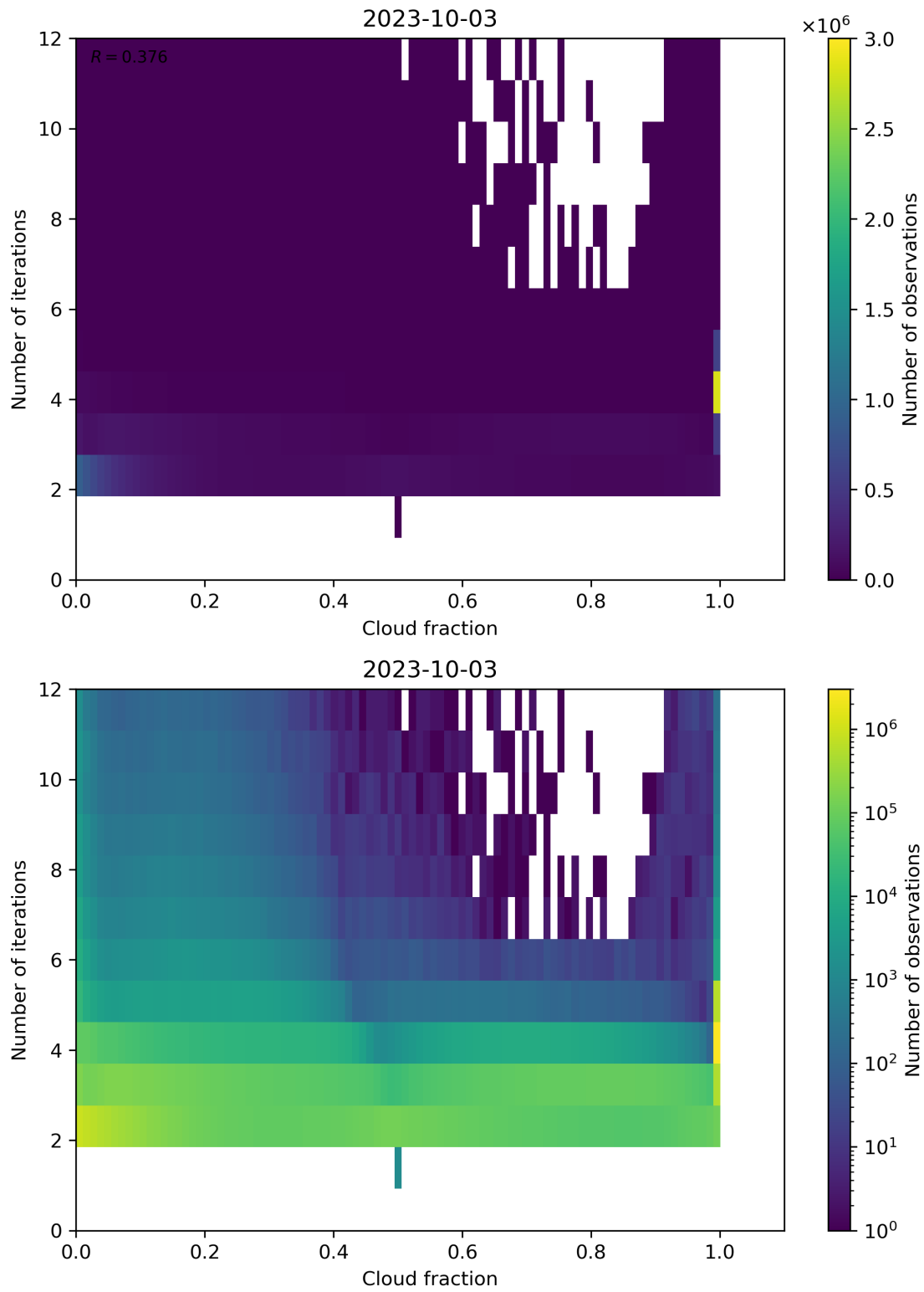
Figure 80: Scatter density plot of “Cloud fraction” against “Number of iterations” for 2023-10-02 to 2023-10-04.
