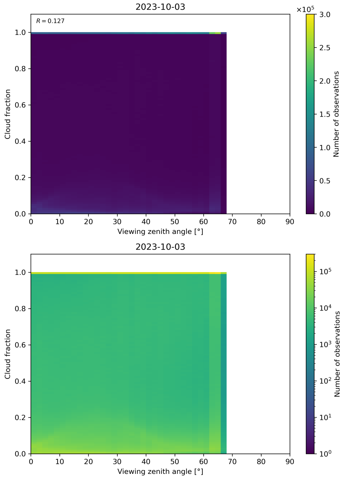
Figure 132: Scatter density plot of “Viewing zenith angle” against “Cloud fraction” for 2023-10-02 to 2023-10-04.
