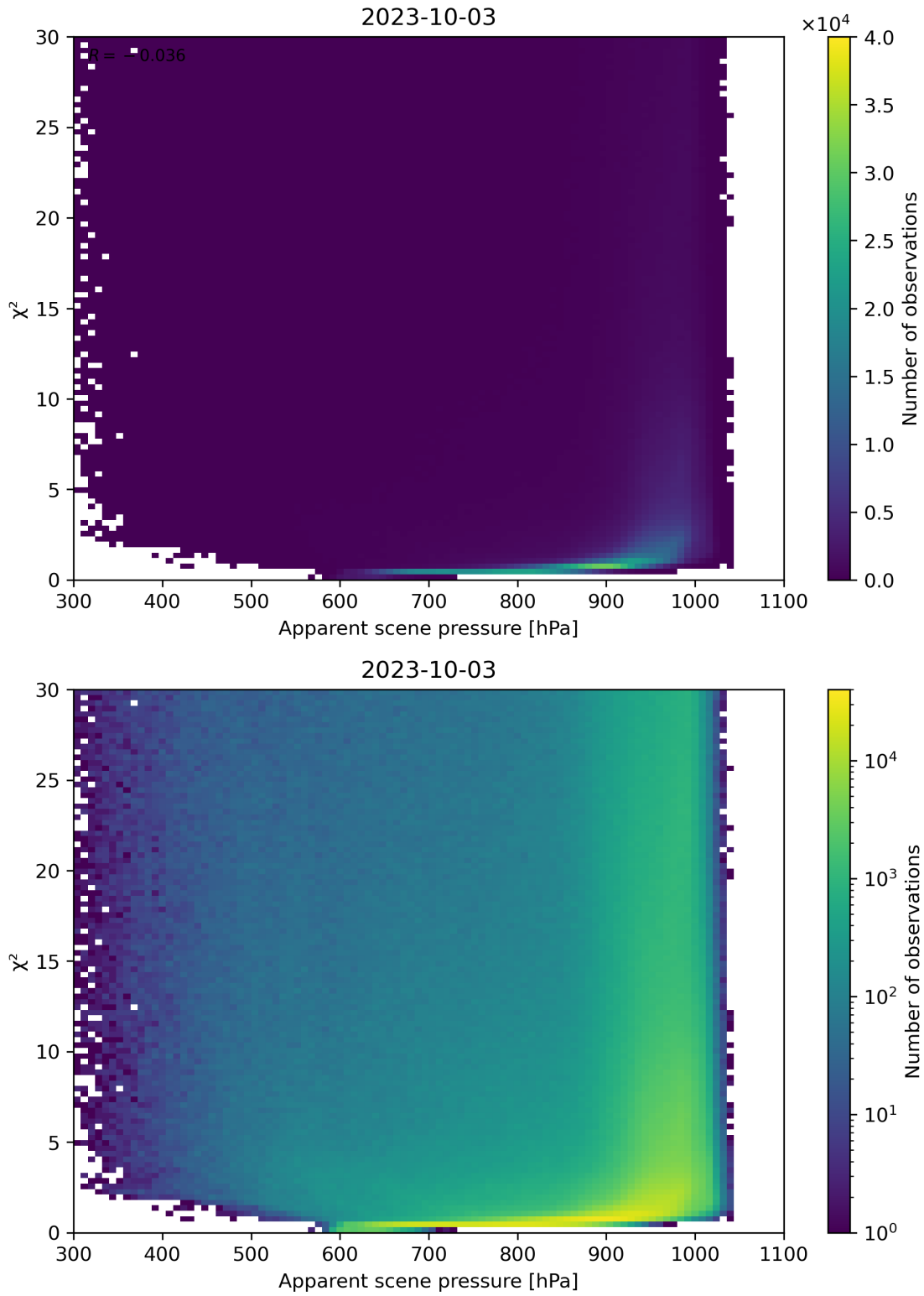
Figure 63: Scatter density plot of “Apparent scene pressure” against “ \chi^2 ” for 2023-10-02 to 2023-10-04.
