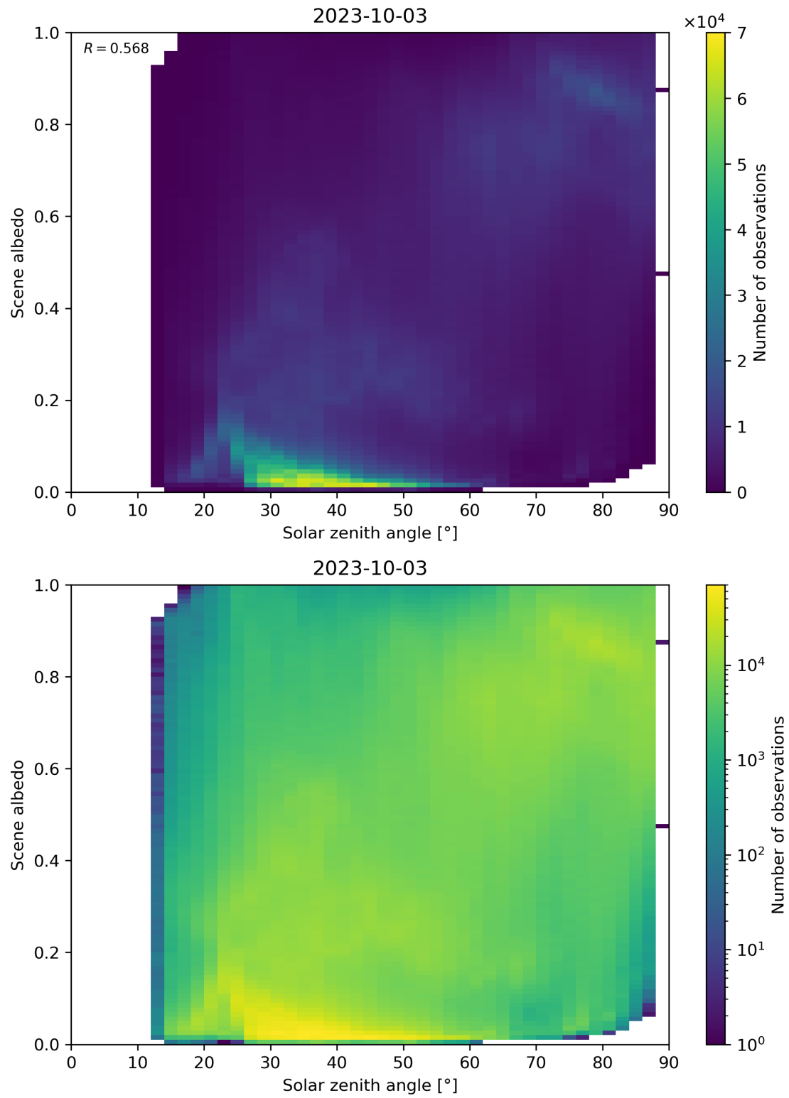
Figure 127: Scatter density plot of “Solar zenith angle” against “Scene albedo” for 2023-10-02 to 2023-10-04.
