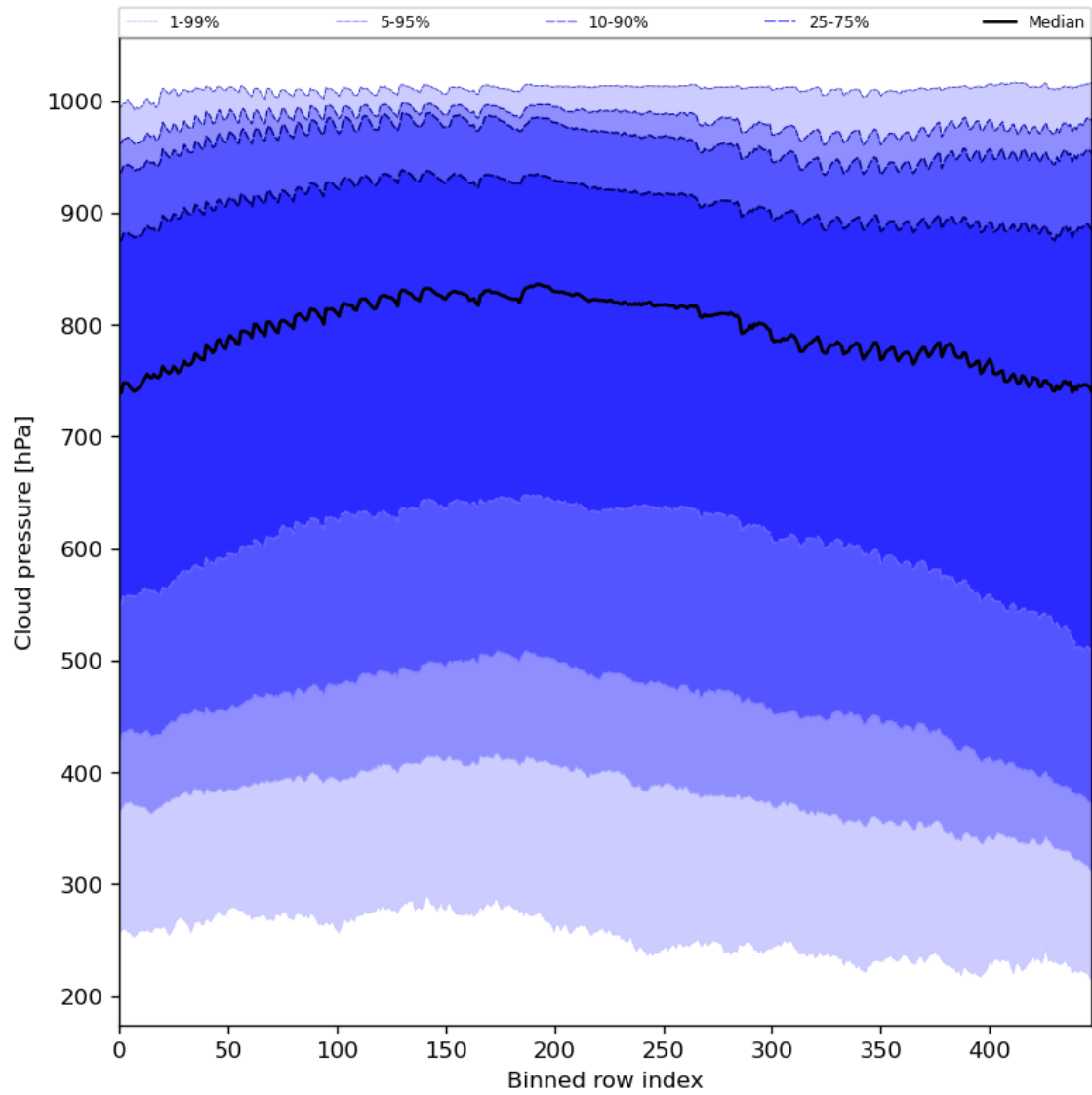
Figure 47: Along track statistics of “Cloud pressure” for 2023-10-02 to 2023-10-04
