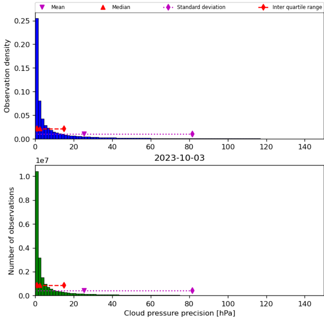
Figure 31: Histogram of “Cloud pressure precision” for 2023-10-02 to 2023-10-04
