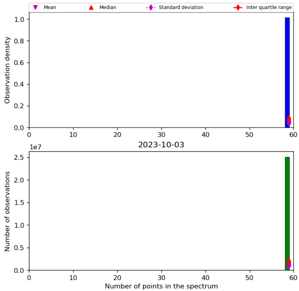
Figure 44: Histogram of “Number of points in the spectrum” for 2023-10-02 to 2023-10-04
