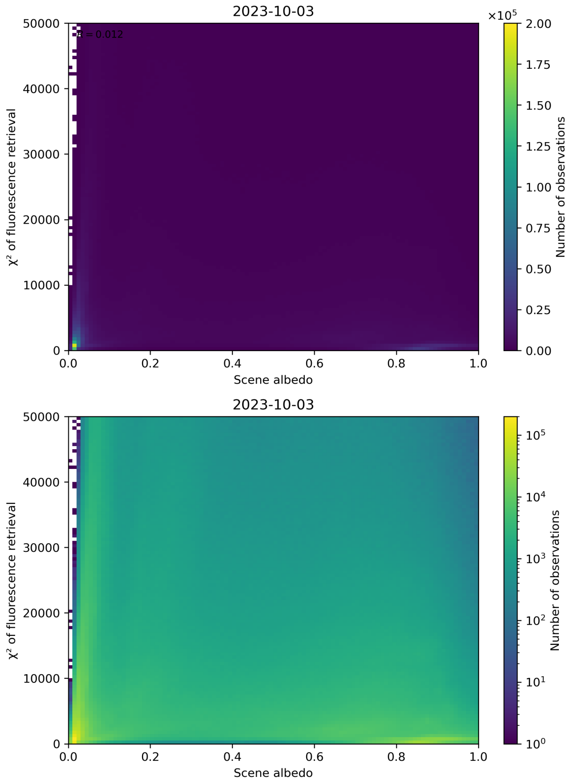
Figure 113: Scatter density plot of “Scene albedo” against “ \chi^2 of fluorescence retrieval” for 2023-10-02 to 2023-10-04.
