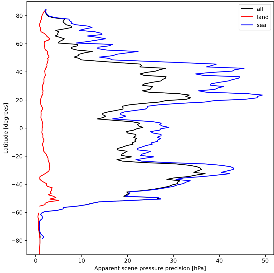
Figure 20: Zonal average of “Apparent scene pressure precision” for 2023-10-02 to 2023-10-04.
