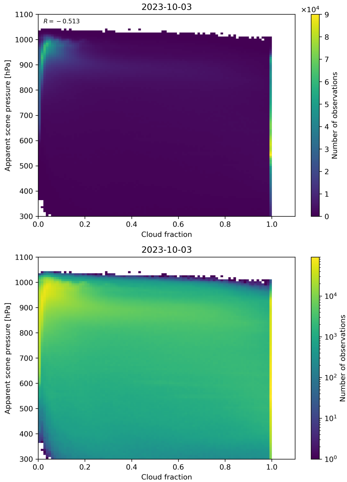
Figure 76: Scatter density plot of “Cloud fraction” against “Apparent scene pressure” for 2023-10-02 to 2023-10-04.
