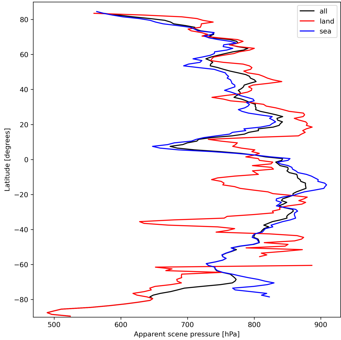
Figure 19: Zonal average of “Apparent scene pressure” for 2023-10-02 to 2023-10-04.
