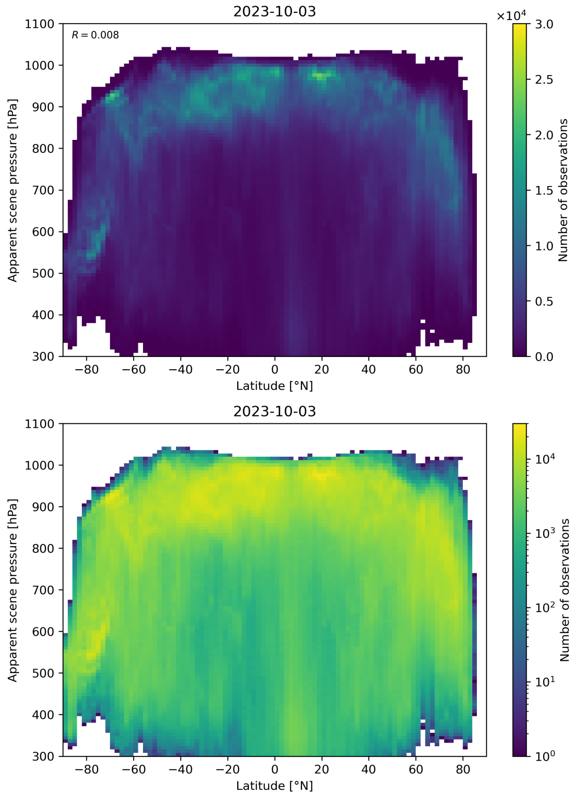
Figure 96: Scatter density plot of “Latitude” against “Apparent scene pressure” for 2023-10-02 to 2023-10-04.
