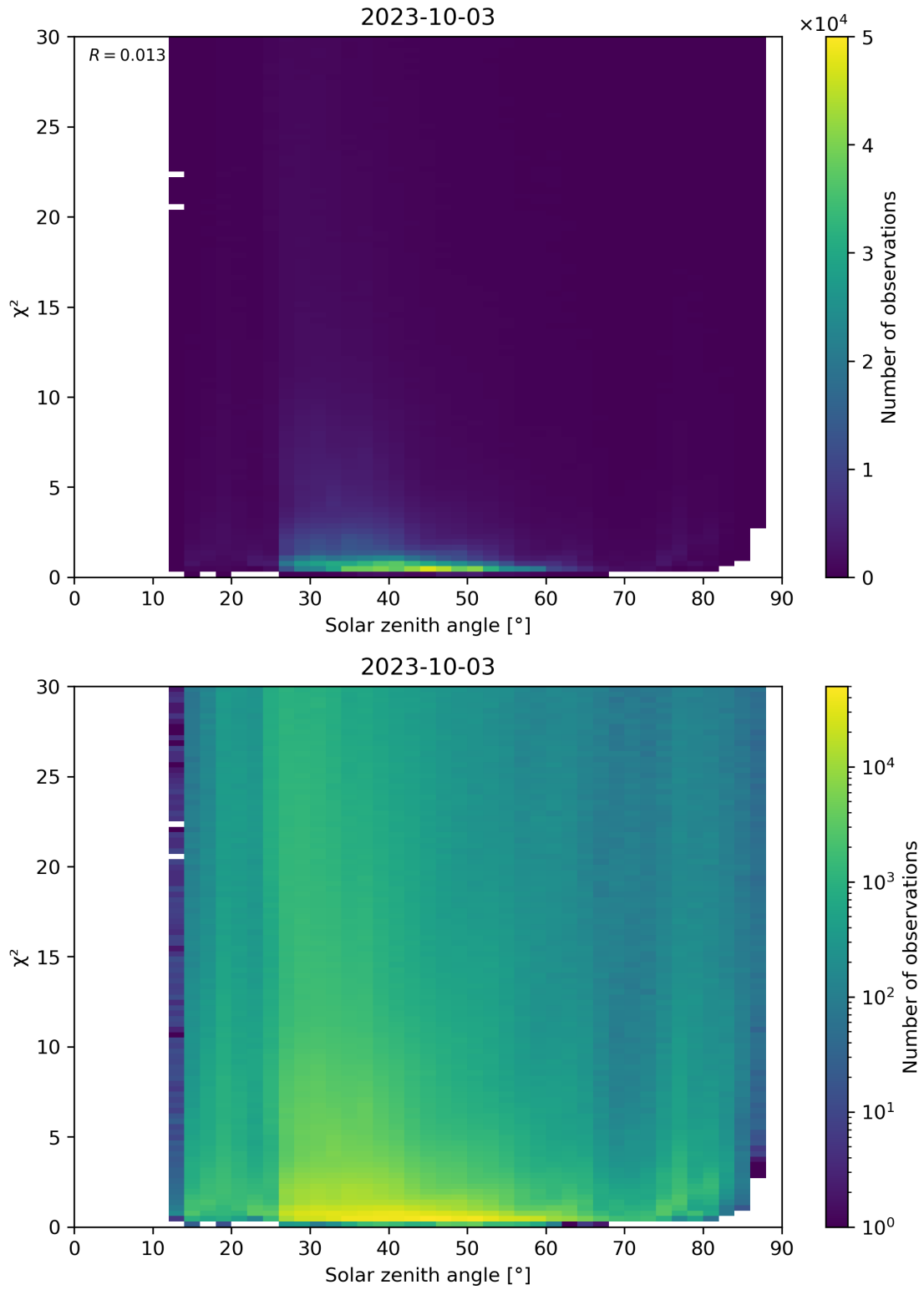
Figure 119: Scatter density plot of “Solar zenith angle” against “ \chi^2 ” for 2023-10-02 to 2023-10-04.
