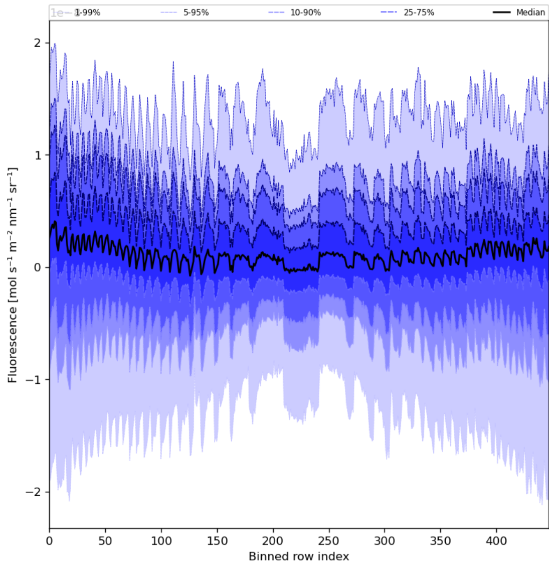
Figure 57: Along track statistics of “Fluorescence” for 2023-10-02 to 2023-10-04
