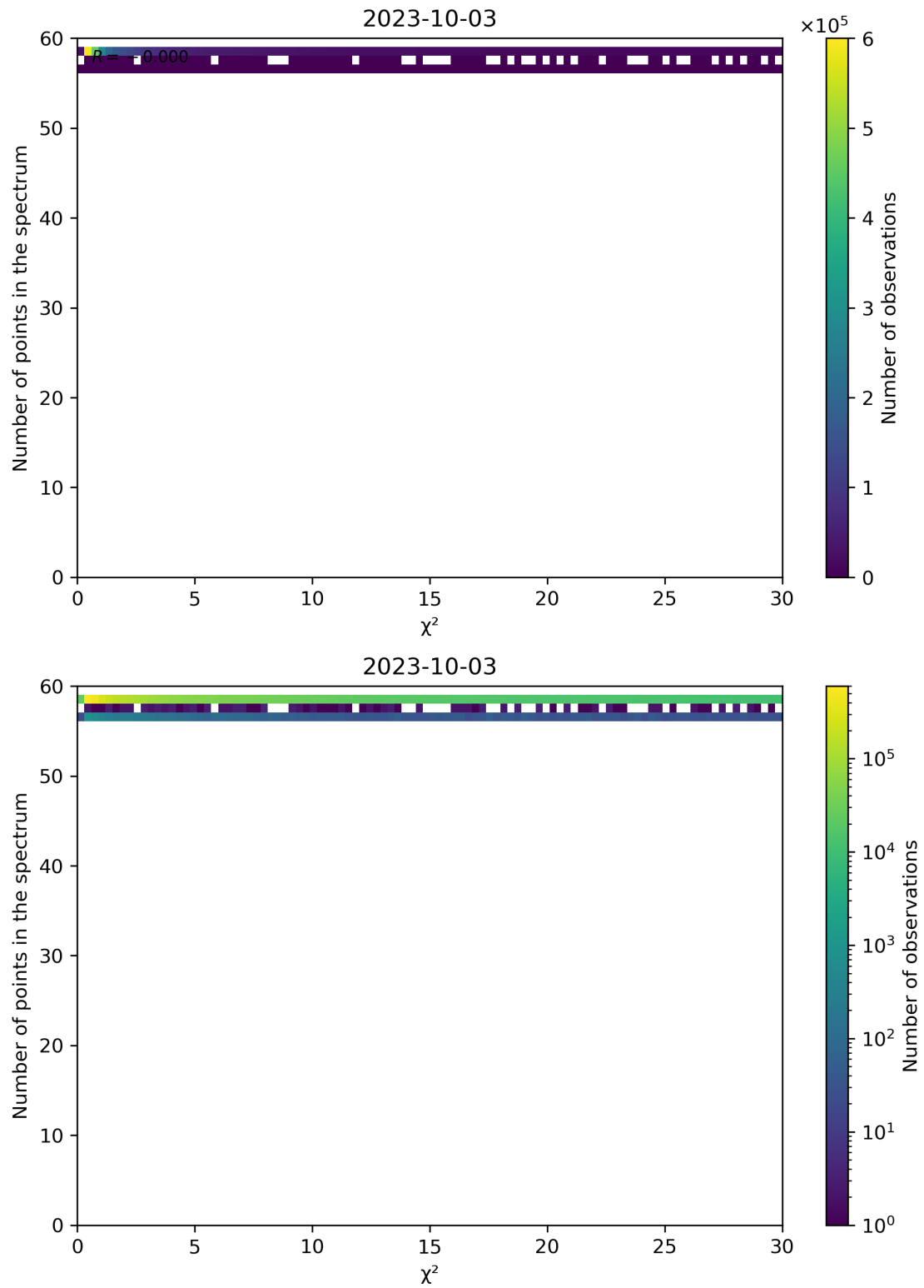
Figure 74: Scatter density plot of " \chi^2 " against "Number of points in the spectrum" for 2023-10-02 to 2023-10-04.
