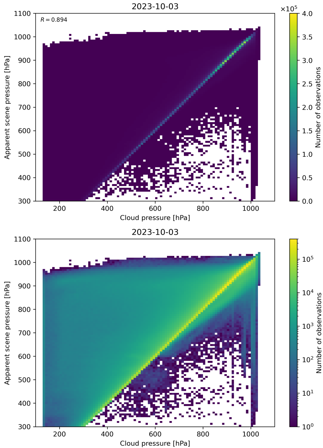
Figure 84: Scatter density plot of “Cloud pressure” against “Apparent scene pressure” for 2023-10-02 to 2023-10-04.
