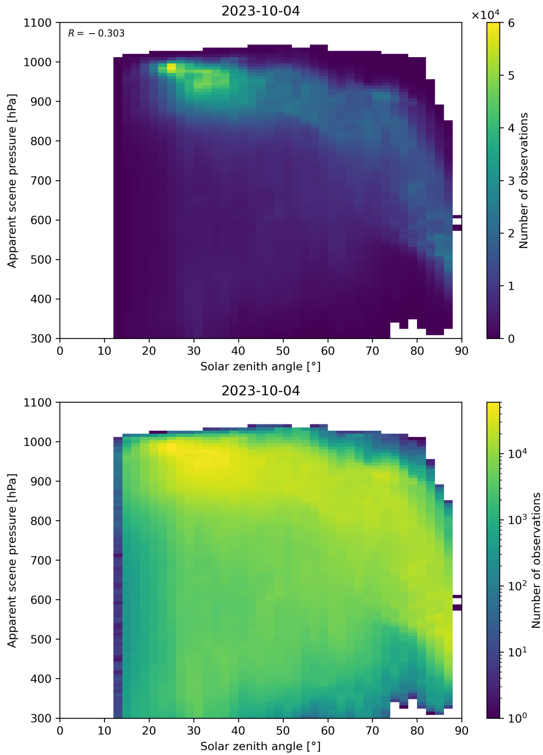
Figure 118: Scatter density plot of “Solar zenith angle” against “Apparent scene pressure” for 2023-10-03 to 2023-10-05.
