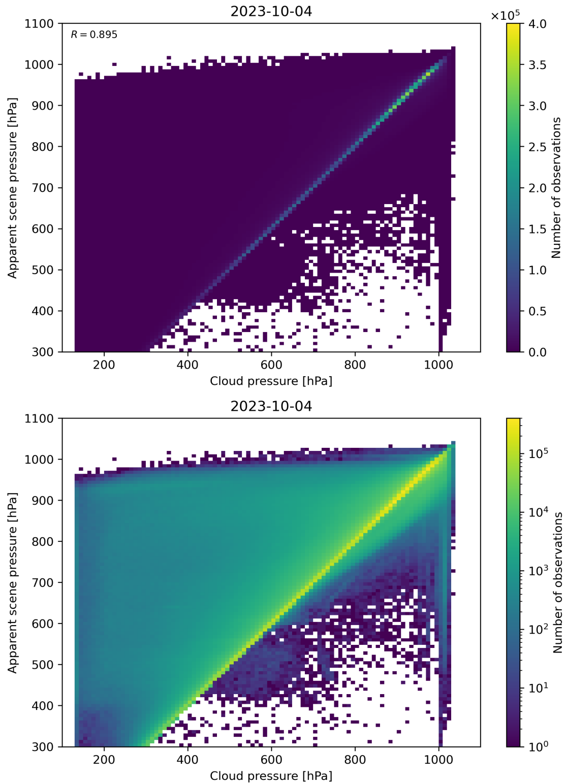
Figure 84: Scatter density plot of “Cloud pressure” against “Apparent scene pressure” for 2023-10-03 to 2023-10-05.
