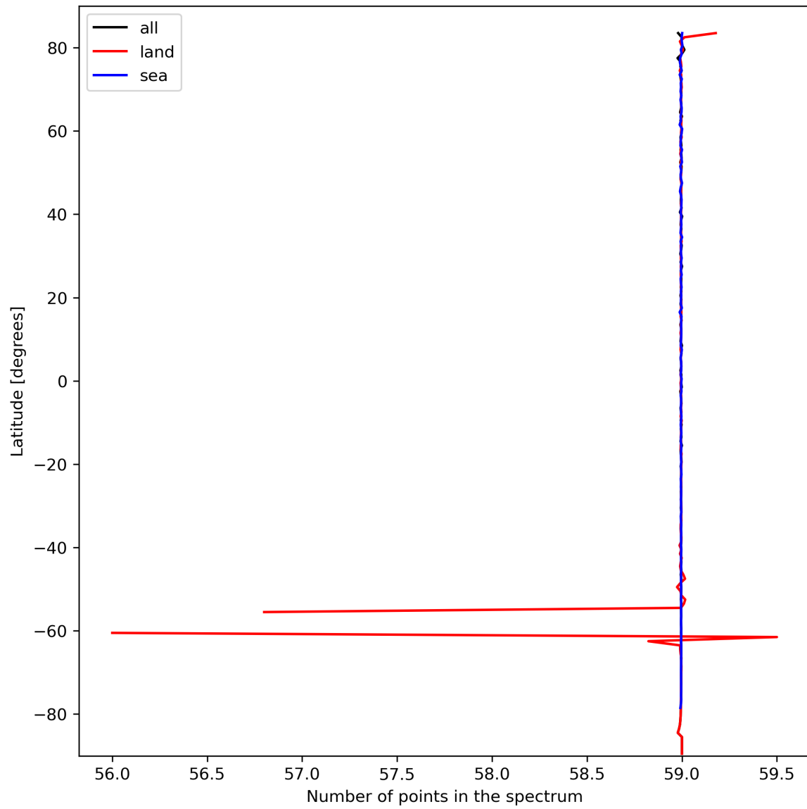
Figure 27: Zonal average of “Number of points in the spectrum” for 2023-10-03 to 2023-10-05.
