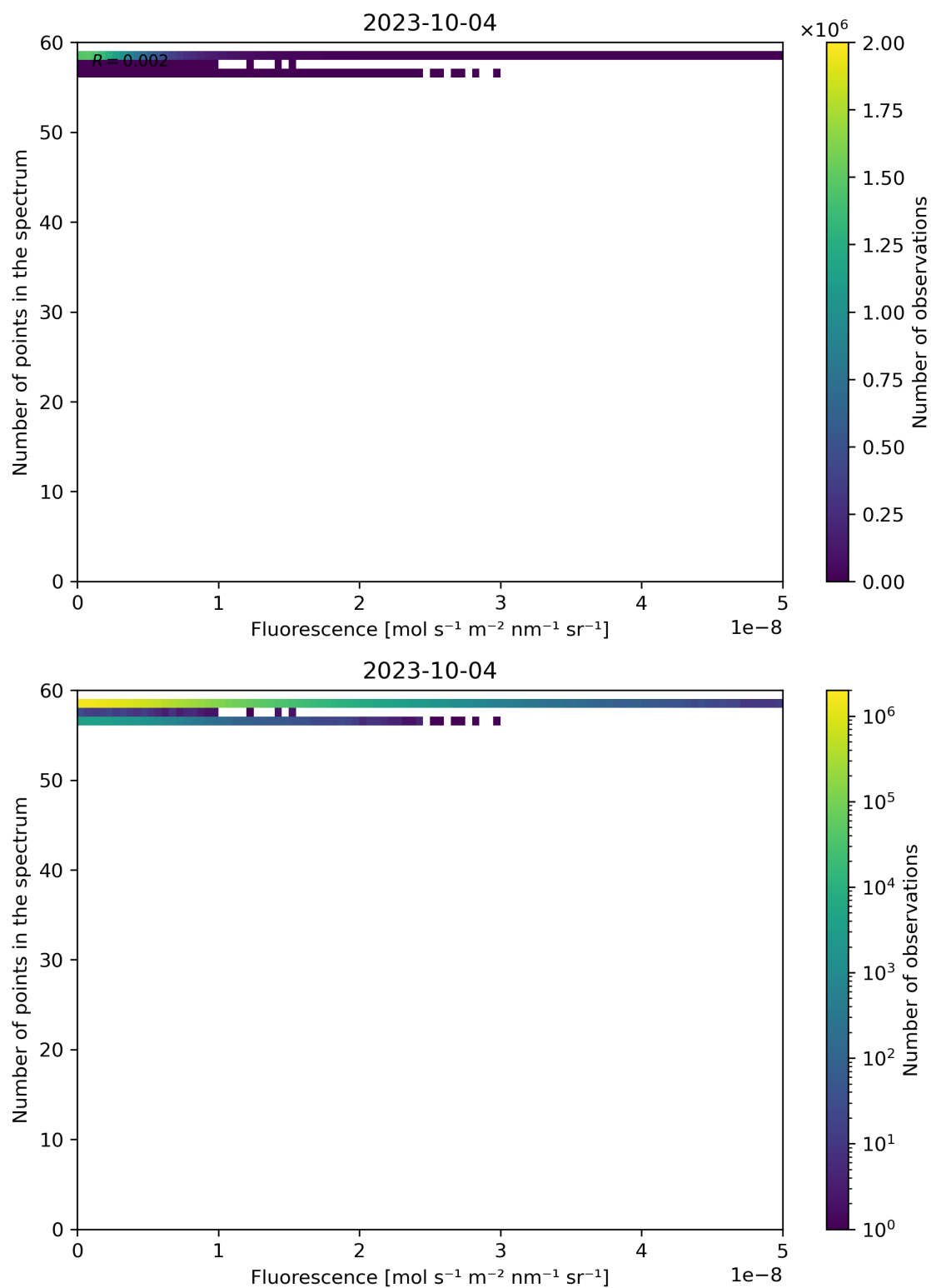
Figure 94: Scatter density plot of “Fluorescence” against “Number of points in the spectrum” for 2023-10-03 to 2023-10-05.
