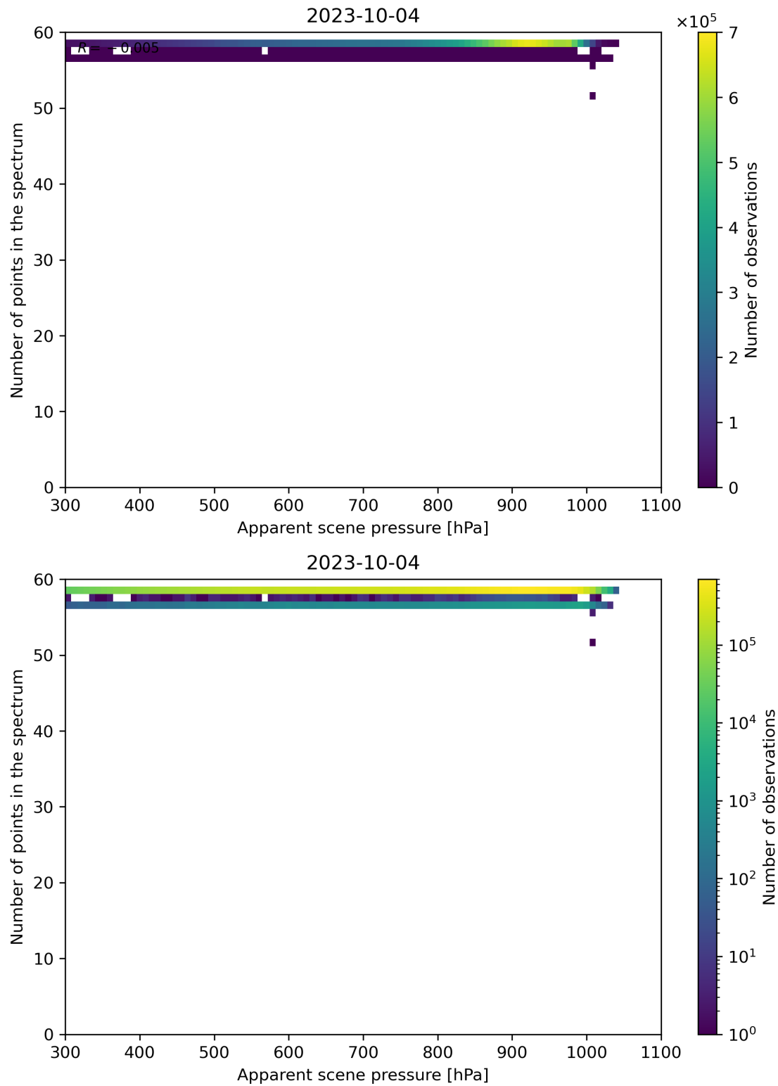
Figure 67: Scatter density plot of “Apparent scene pressure” against “Number of points in the spectrum” for 2023-10-03 to 2023-10-05.
