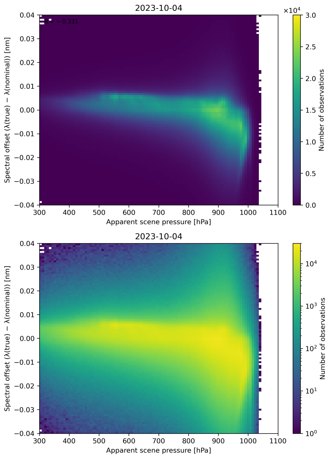
Figure 68: Scatter density plot of “Apparent scene pressure” against “Spectral offset ( \lambda(\text{true}) - \lambda(\text{nominal}) )” for 2023-10-03 to 2023-10-05.
