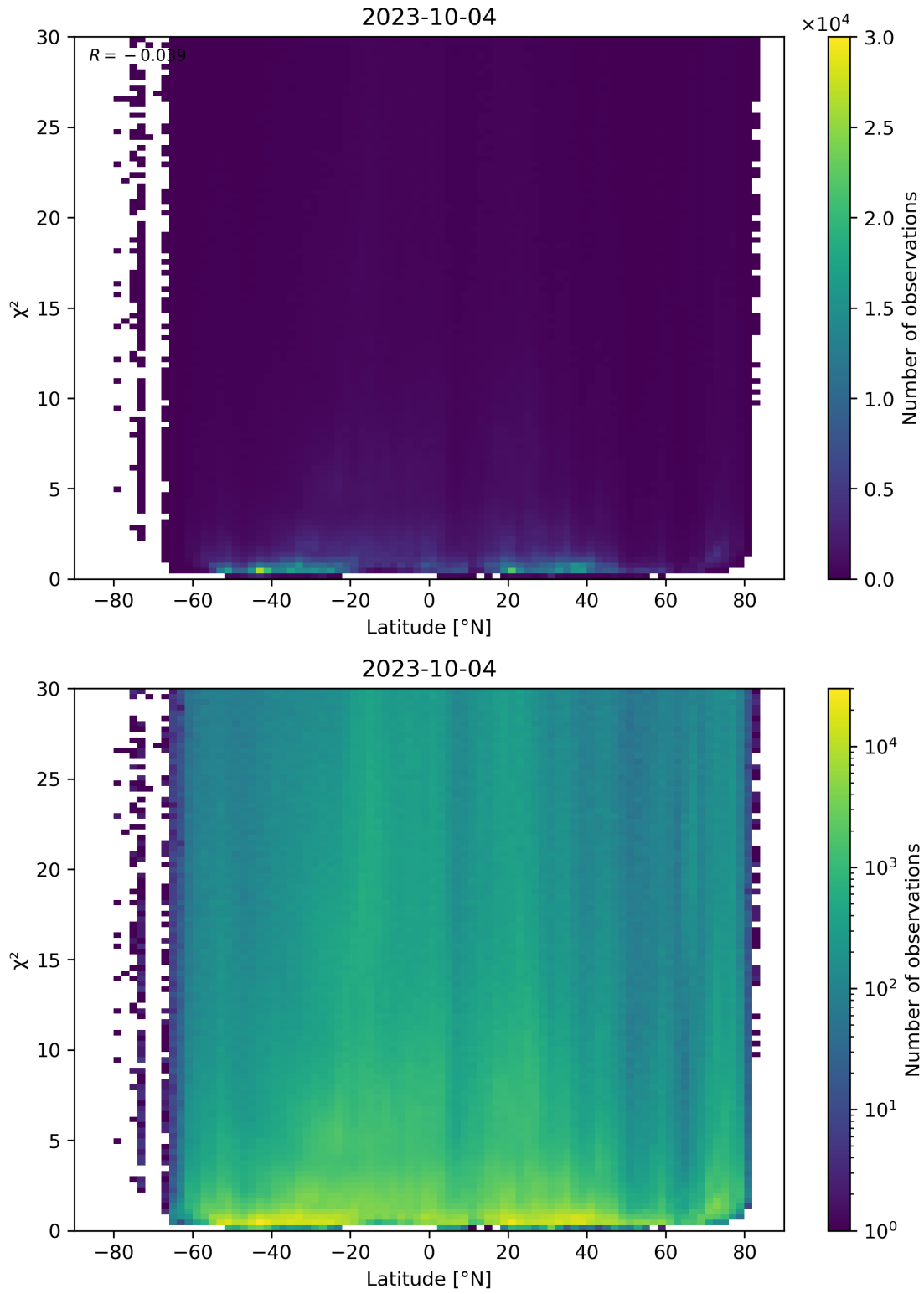
Figure 97: Scatter density plot of “Latitude” against “ \chi^2 ” for 2023-10-03 to 2023-10-05.
