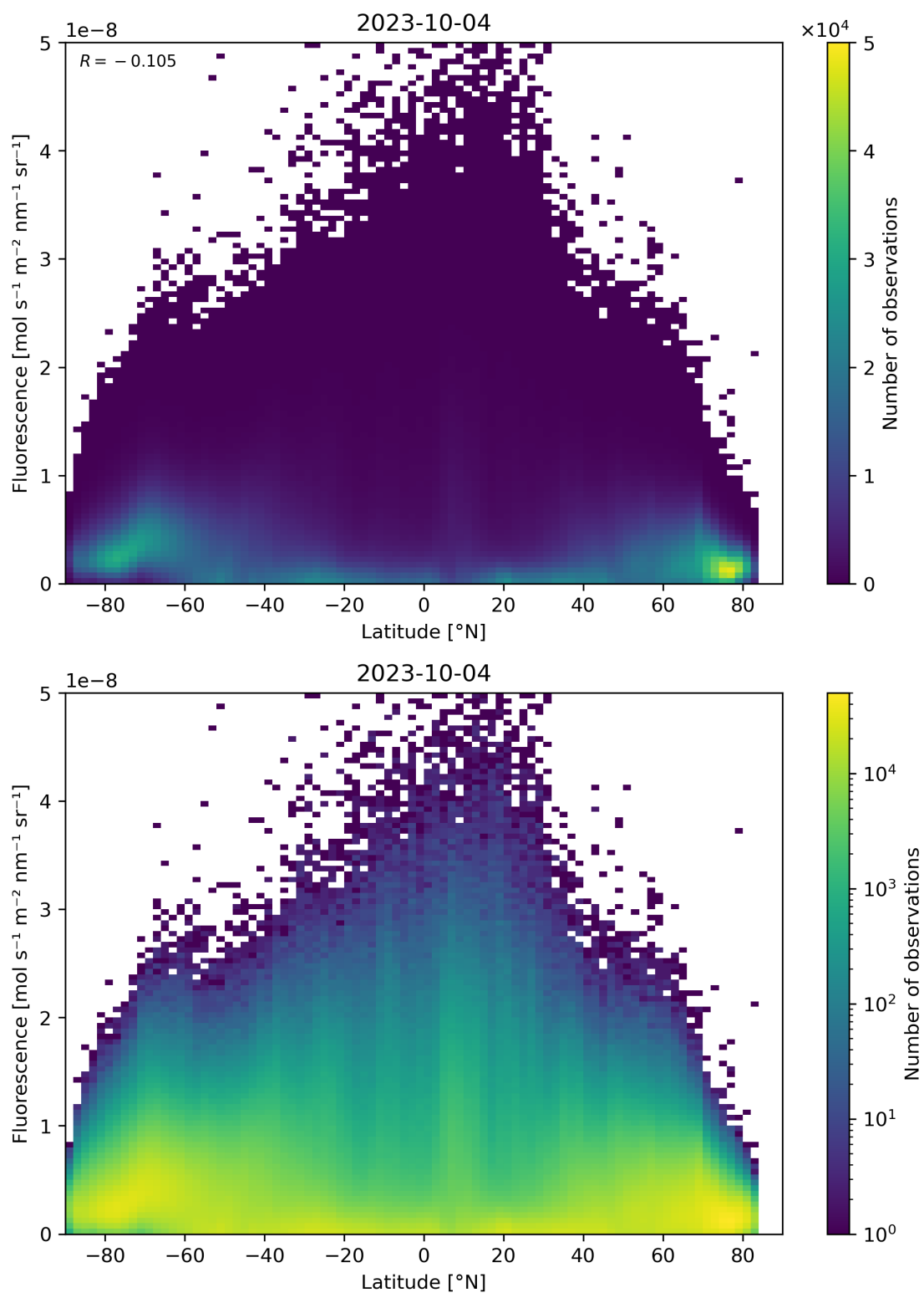
Figure 101: Scatter density plot of “Latitude” against “Fluorescence” for 2023-10-03 to 2023-10-05.
