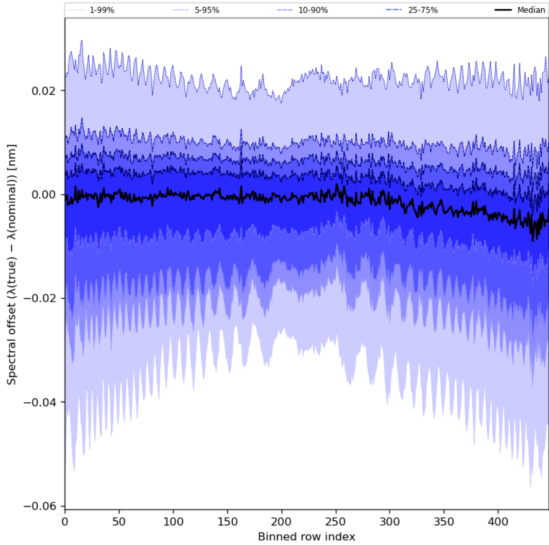
Figure 62: Along track statistics of “Spectral offset ( \lambda(\text{true}) - \lambda(\text{nominal}) )” for 2023-10-03 to 2023-10-05
