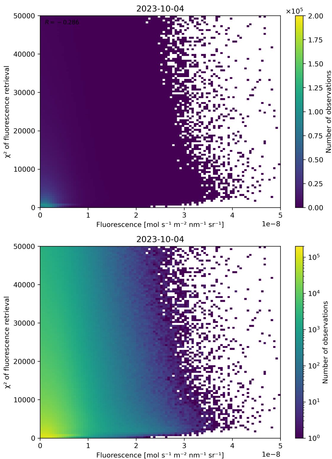
Figure 93: Scatter density plot of “Fluorescence” against “ \chi^2 of fluorescence retrieval” for 2023-10-03 to 2023-10-05.
