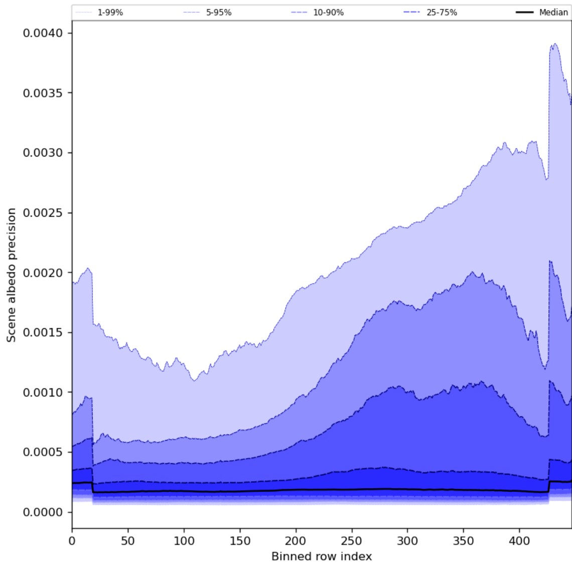
Figure 52: Along track statistics of “Scene albedo precision” for 2023-10-03 to 2023-10-05
