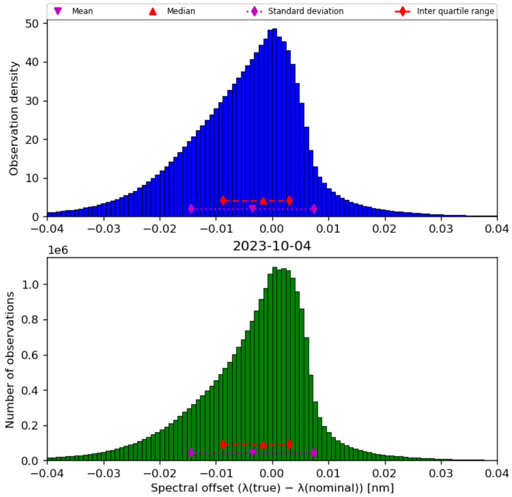
Figure 45: Histogram of “Spectral offset ( \lambda(\text{true}) - \lambda(\text{nominal}) )” for 2023-10-03 to 2023-10-05
