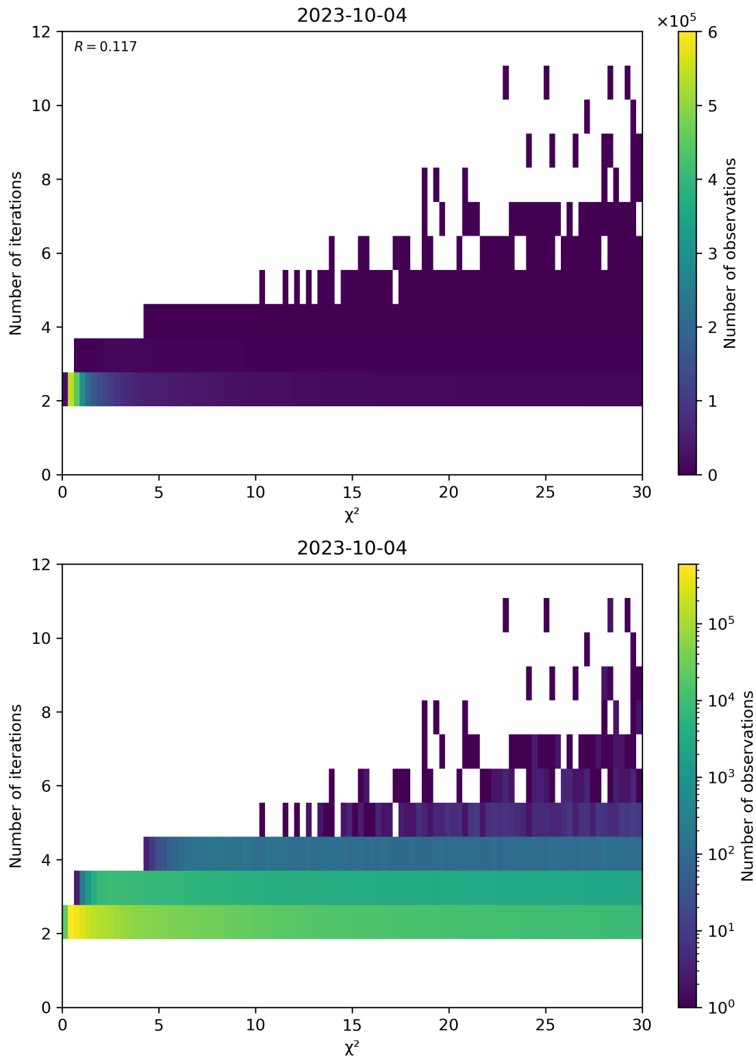
Figure 73: Scatter density plot of “ \chi^2 ” against “Number of iterations” for 2023-10-03 to 2023-10-05.
