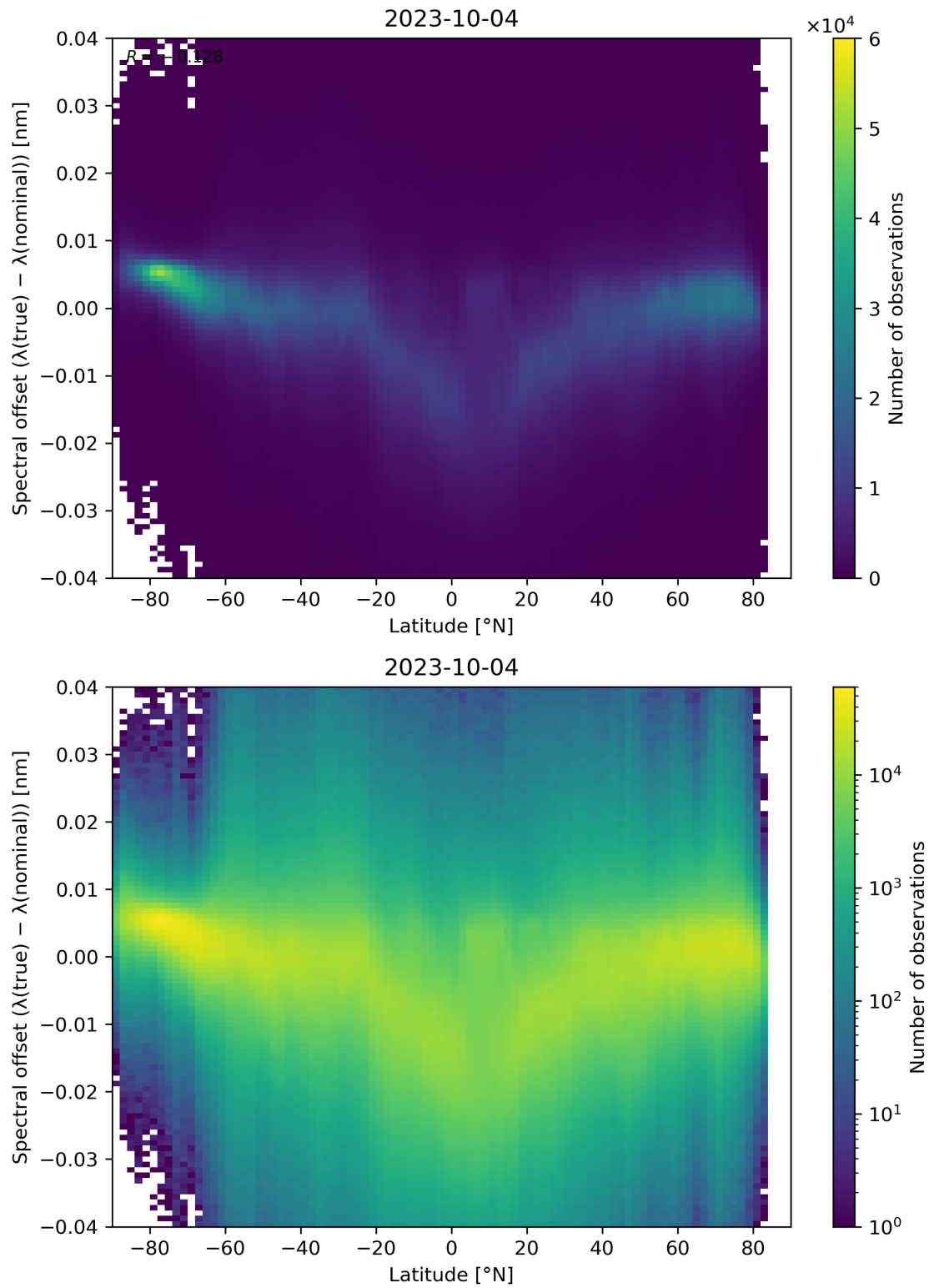
Figure 105: Scatter density plot of “Latitude” against “Spectral offset ( \lambda(\text{true}) - \lambda(\text{nominal}) )” for 2023-10-03 to 2023-10-05.
