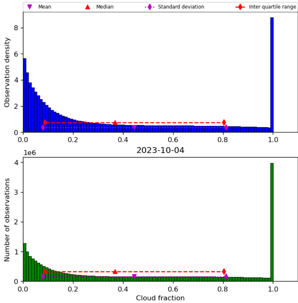
Figure 32: Histogram of “Cloud fraction” for 2023-10-03 to 2023-10-05
