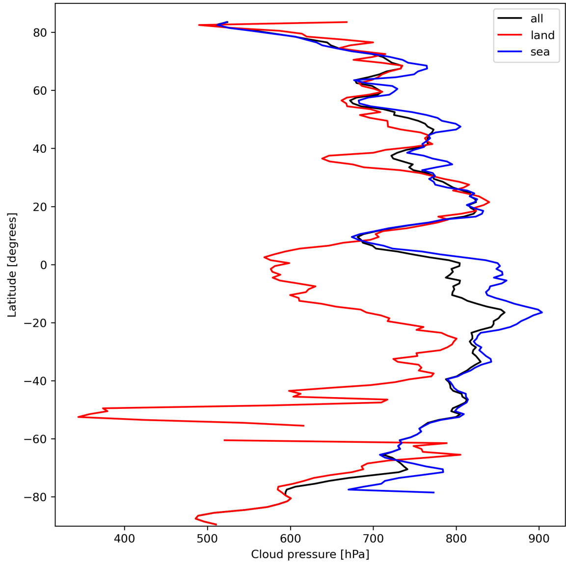
Figure 13: Zonal average of “Cloud pressure” for 2023-10-03 to 2023-10-05.
