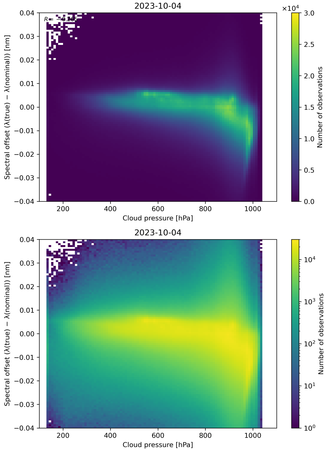
Figure 92: Scatter density plot of “Cloud pressure” against “Spectral offset ( \lambda(\text{true}) - \lambda(\text{nominal}) )” for 2023-10-03 to 2023-10-05.
