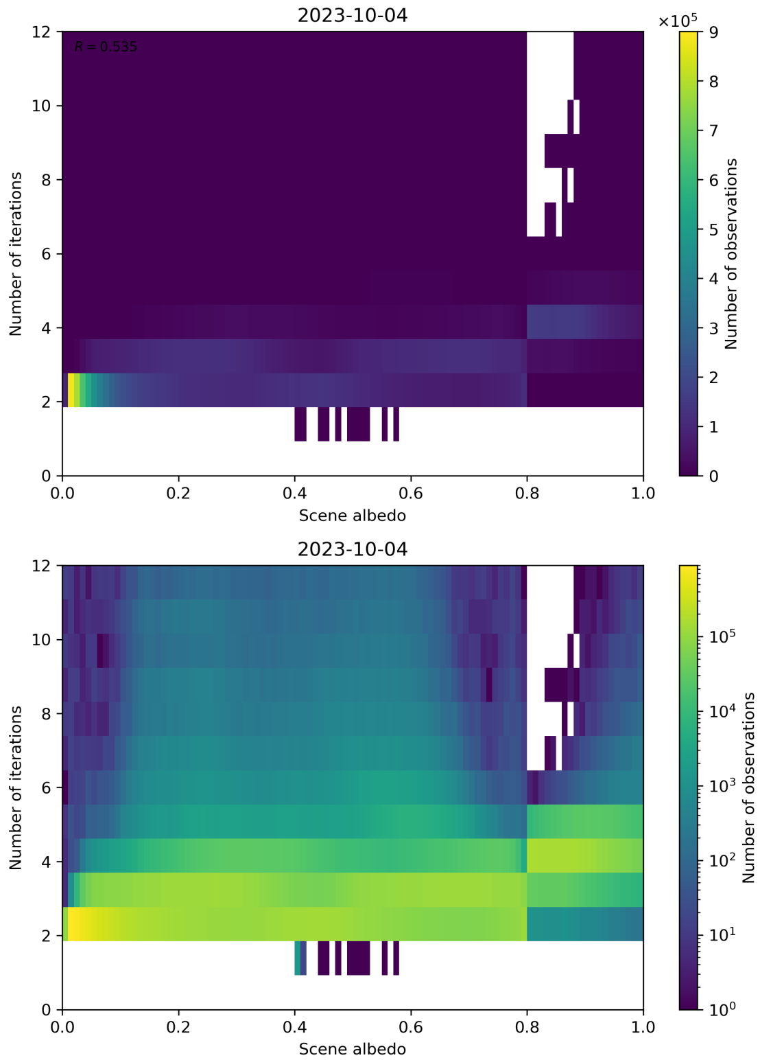
Figure 115: Scatter density plot of “Scene albedo” against “Number of iterations” for 2023-10-03 to 2023-10-05.
