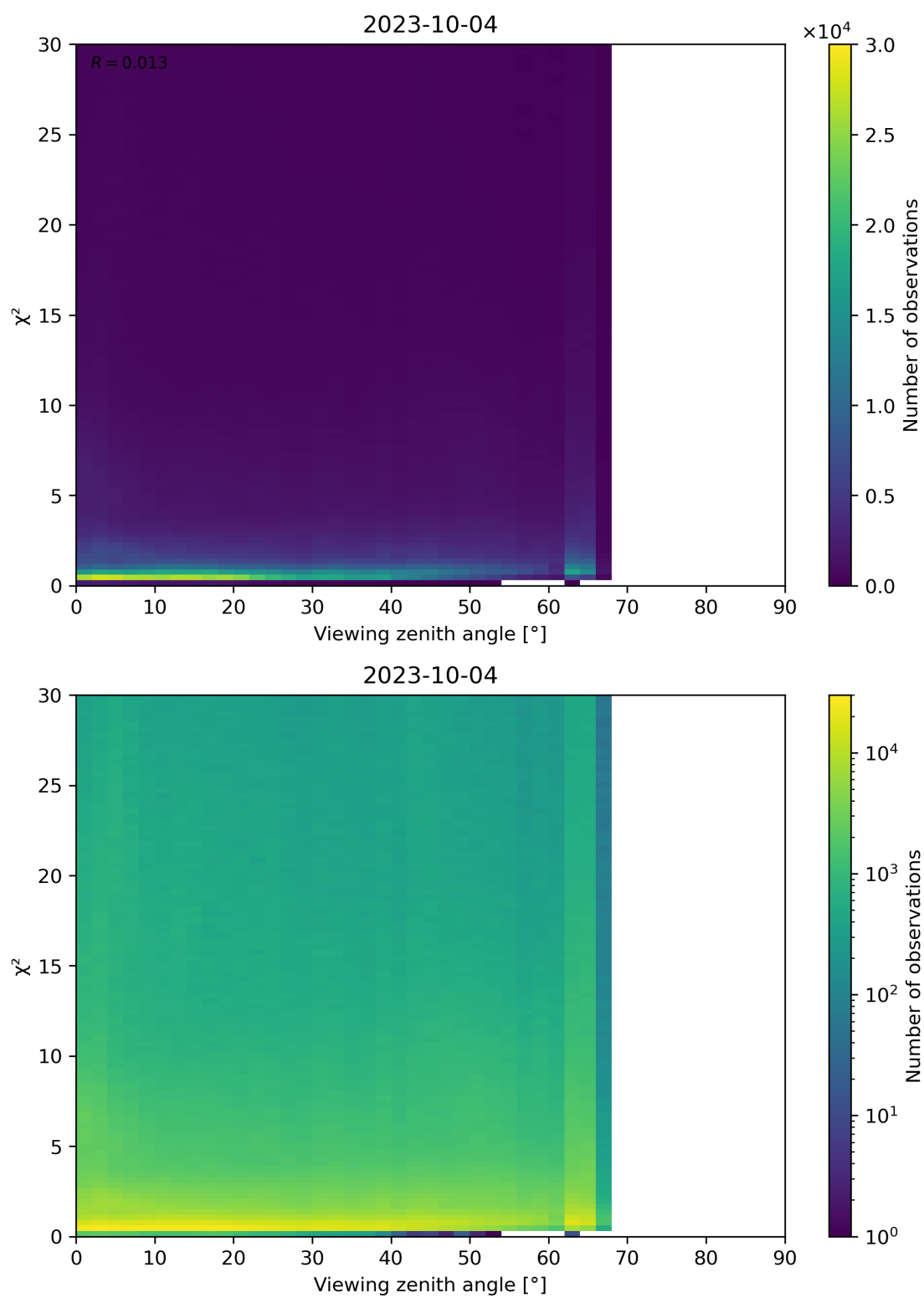
Figure 130: Scatter density plot of “Viewing zenith angle” against “ \chi^2 ” for 2023-10-03 to 2023-10-05.
