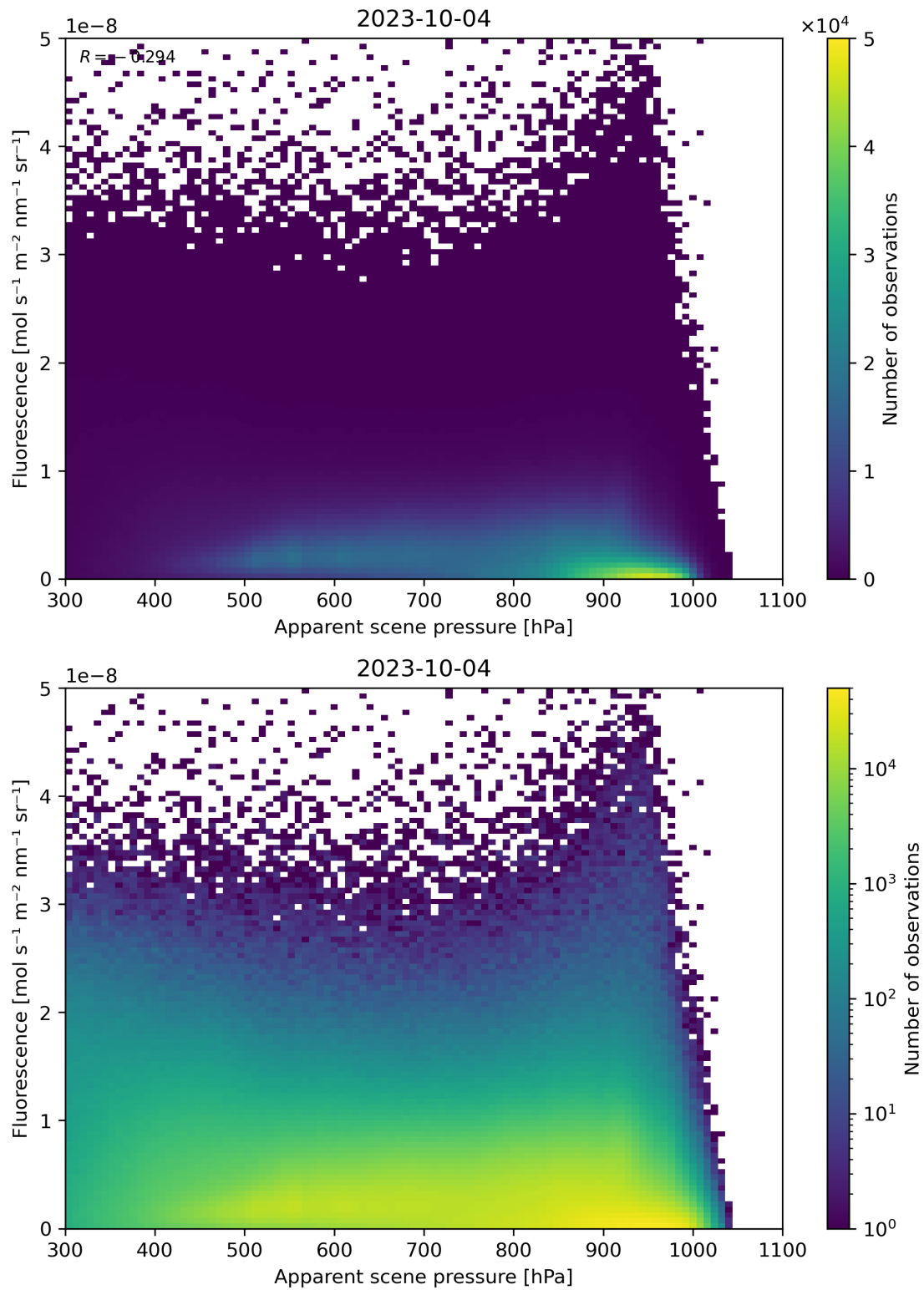
Figure 65: Scatter density plot of “Apparent scene pressure” against “Fluorescence” for 2023-10-03 to 2023-10-05.
