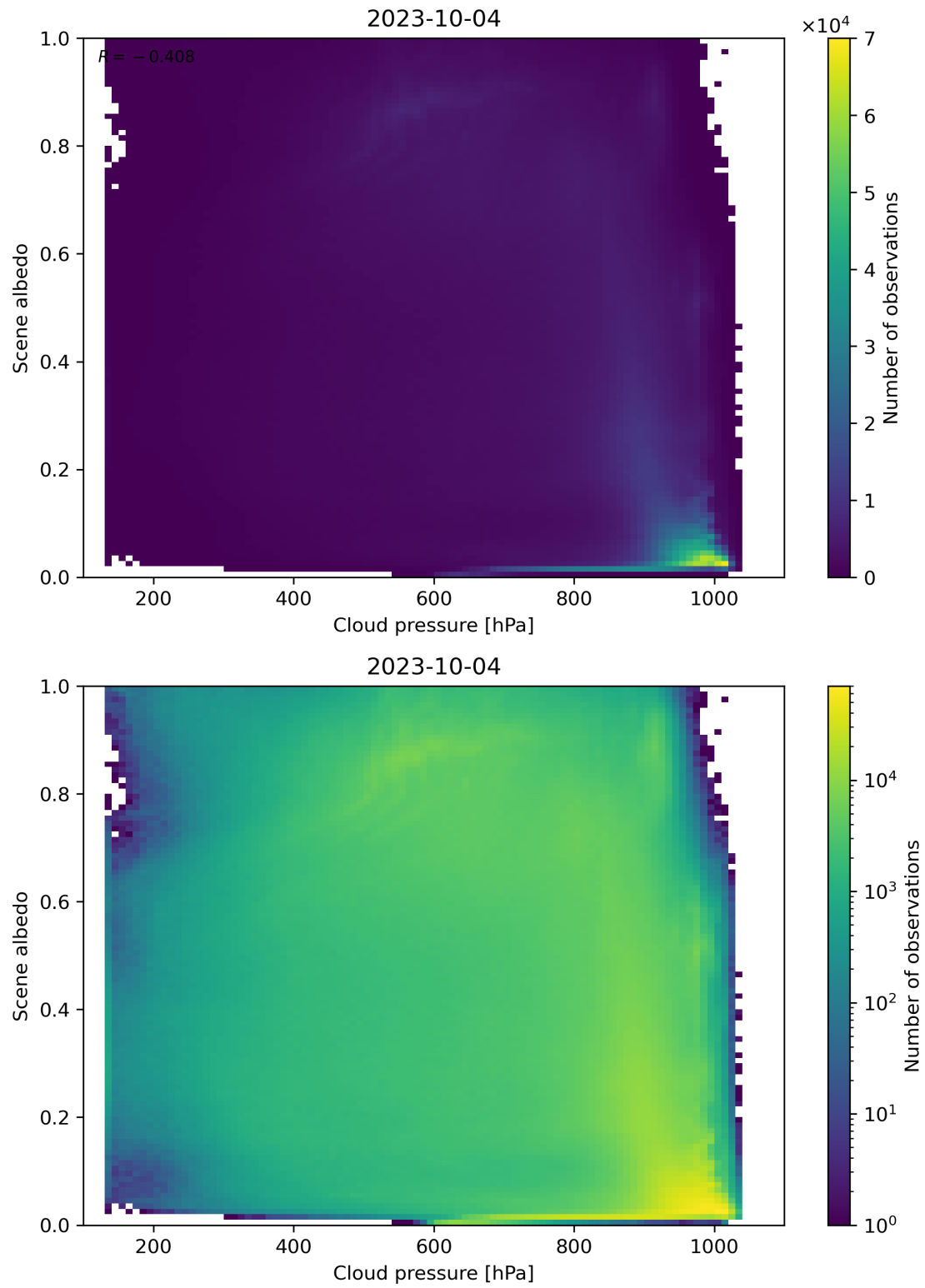
Figure 91: Scatter density plot of “Cloud pressure” against “Scene albedo” for 2023-10-03 to 2023-10-05.
