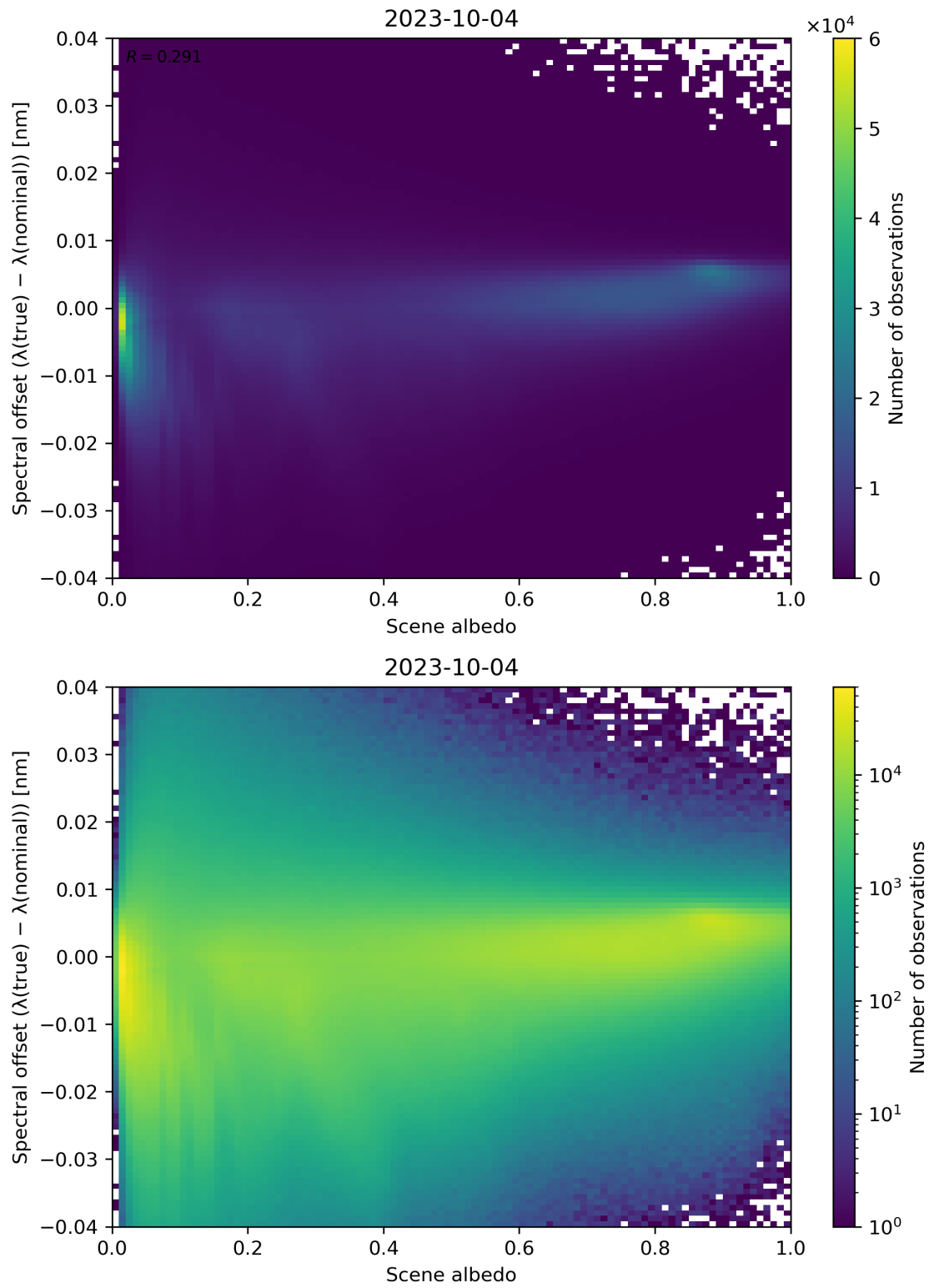
Figure 117: Scatter density plot of “Scene albedo” against “Spectral offset ( \lambda(\text{true}) - \lambda(\text{nominal}) )” for 2023-10-03 to 2023-10-05.
