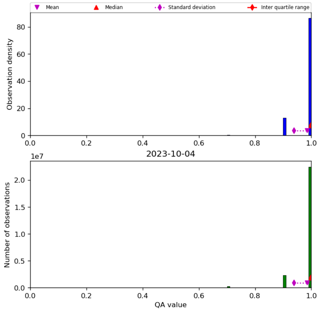
Figure 29: Histogram of “QA value” for 2023-10-03 to 2023-10-05
