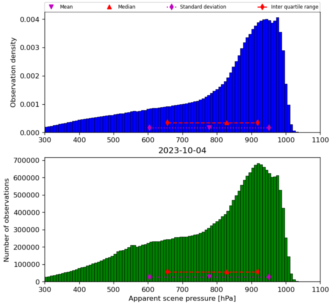
Figure 36: Histogram of “Apparent scene pressure” for 2023-10-03 to 2023-10-05
