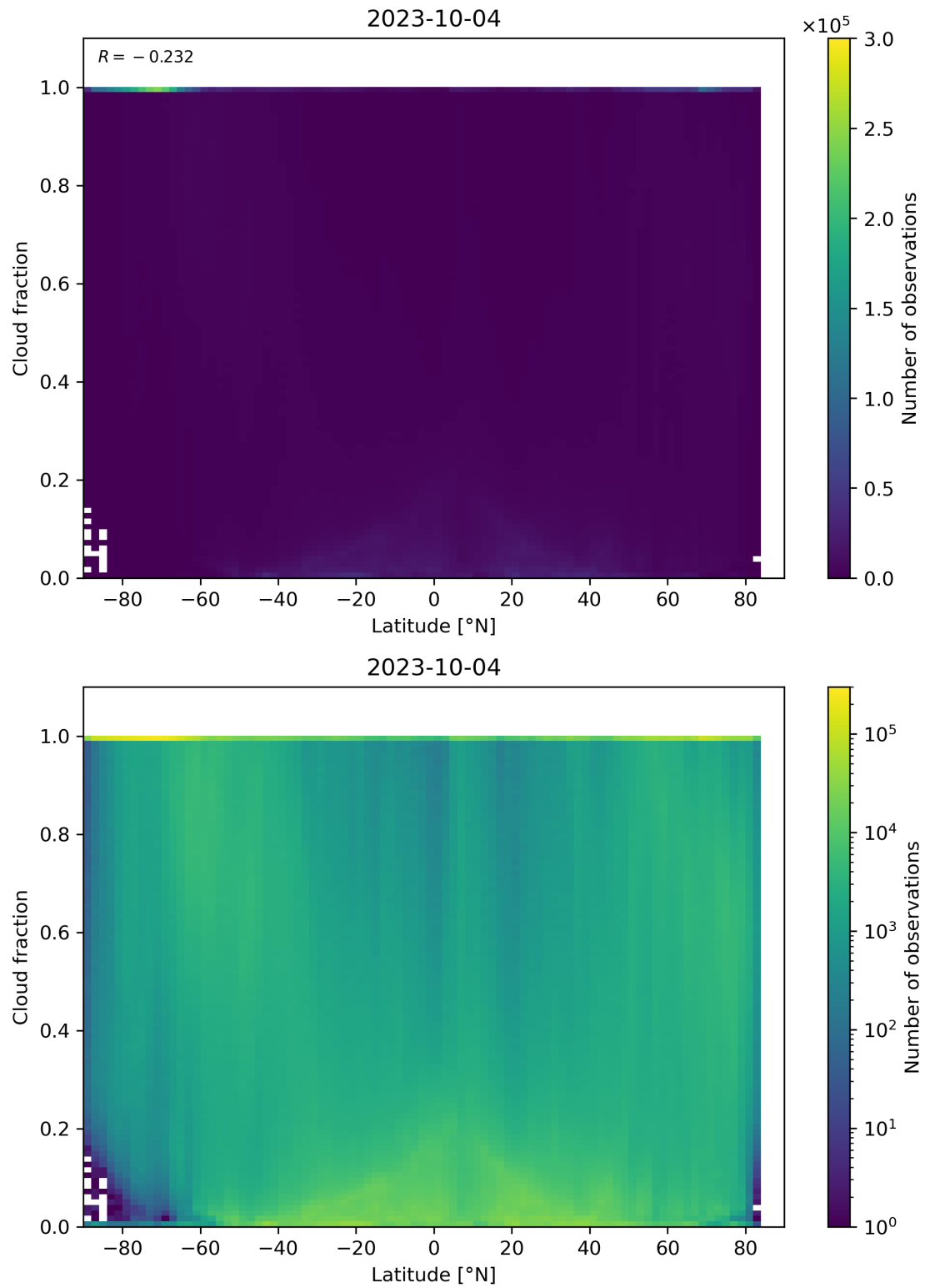
Figure 99: Scatter density plot of “Latitude” against “Cloud fraction” for 2023-10-03 to 2023-10-05.
