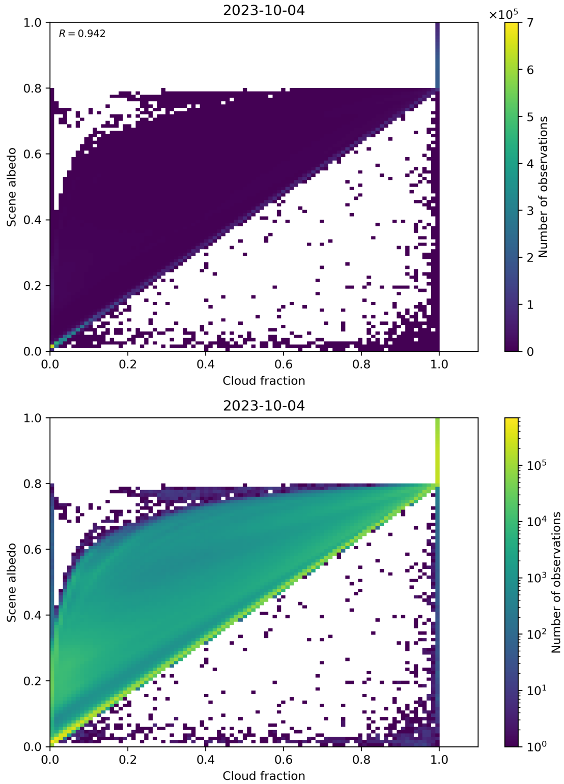
Figure 82: Scatter density plot of “Cloud fraction” against “Scene albedo” for 2023-10-03 to 2023-10-05.
