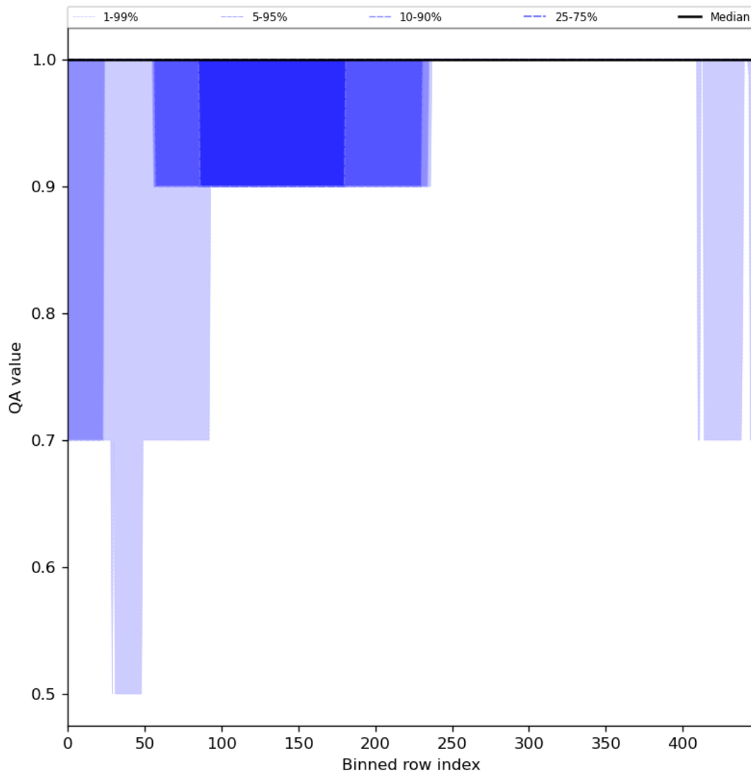
Figure 46: Along track statistics of “QA value” for 2023-10-03 to 2023-10-05
