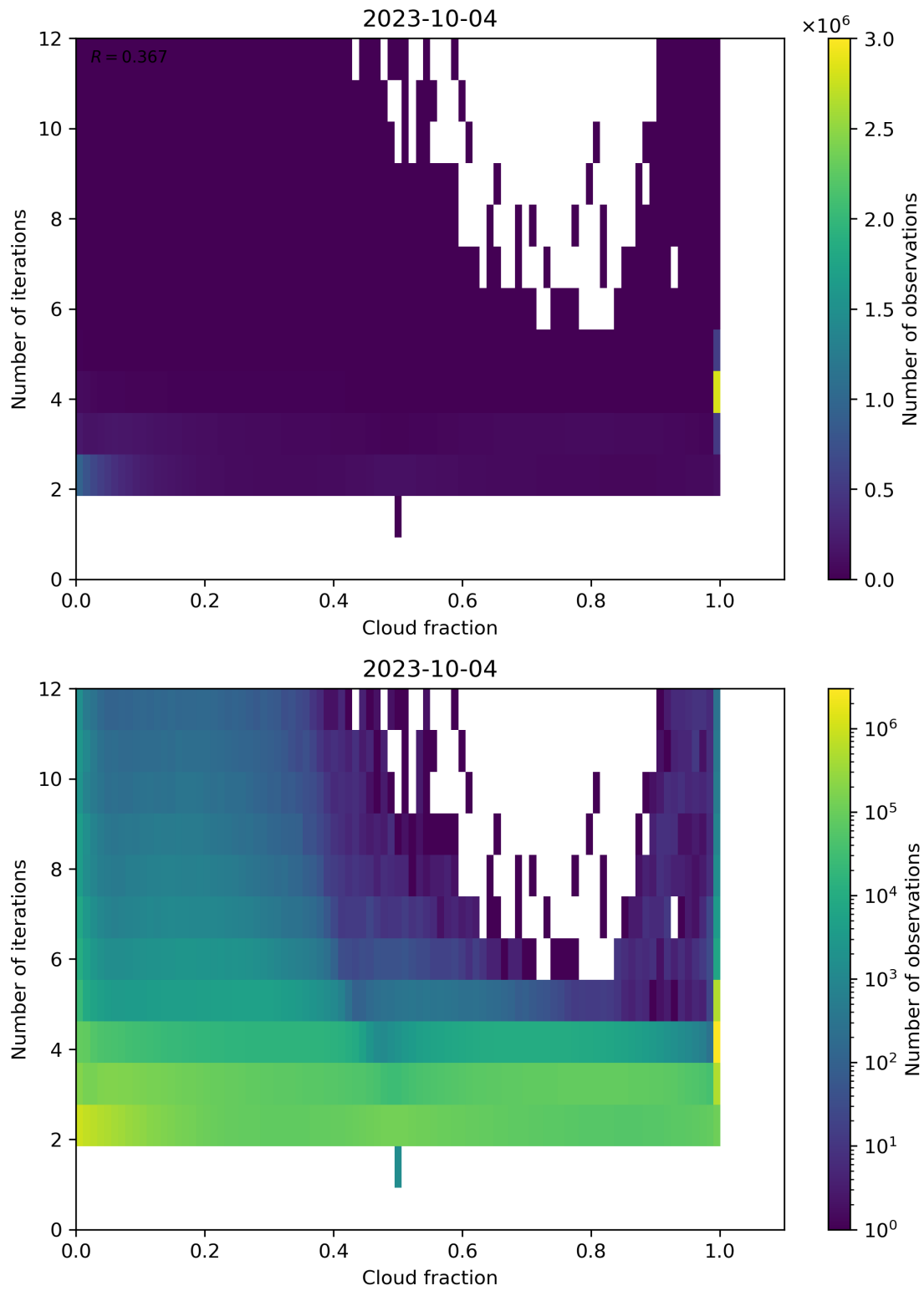
Figure 80: Scatter density plot of “Cloud fraction” against “Number of iterations” for 2023-10-03 to 2023-10-05.
