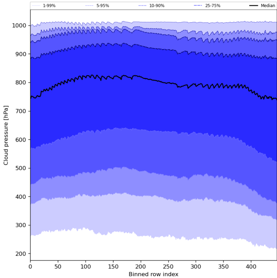
Figure 47: Along track statistics of “Cloud pressure” for 2023-10-03 to 2023-10-05
