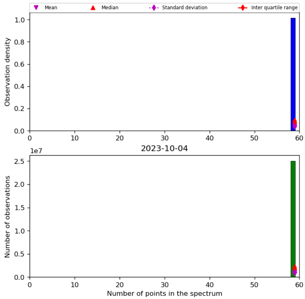
Figure 44: Histogram of “Number of points in the spectrum” for 2023-10-03 to 2023-10-05
