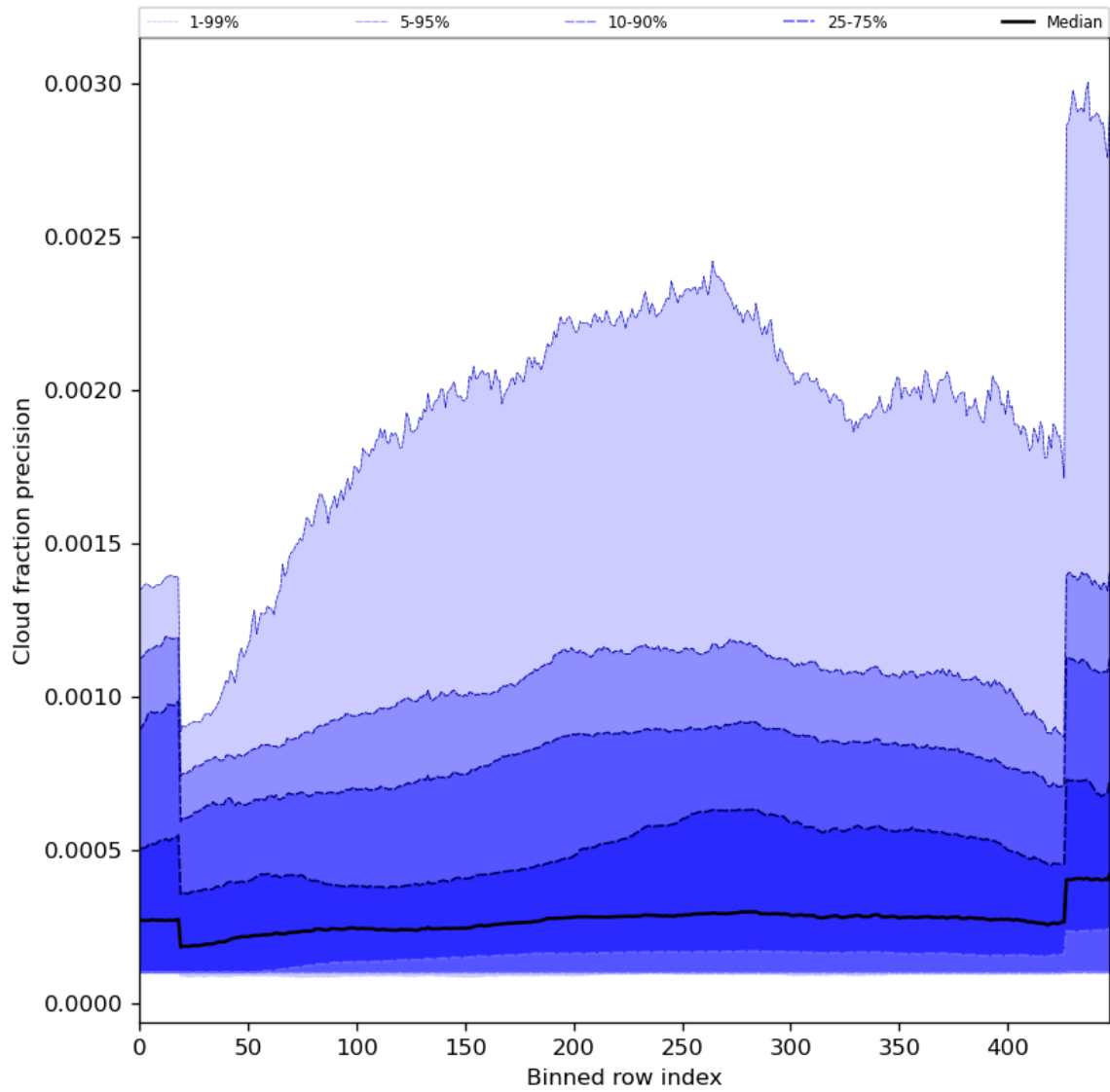
Figure 50: Along track statistics of “Cloud fraction precision” for 2023-10-03 to 2023-10-05
