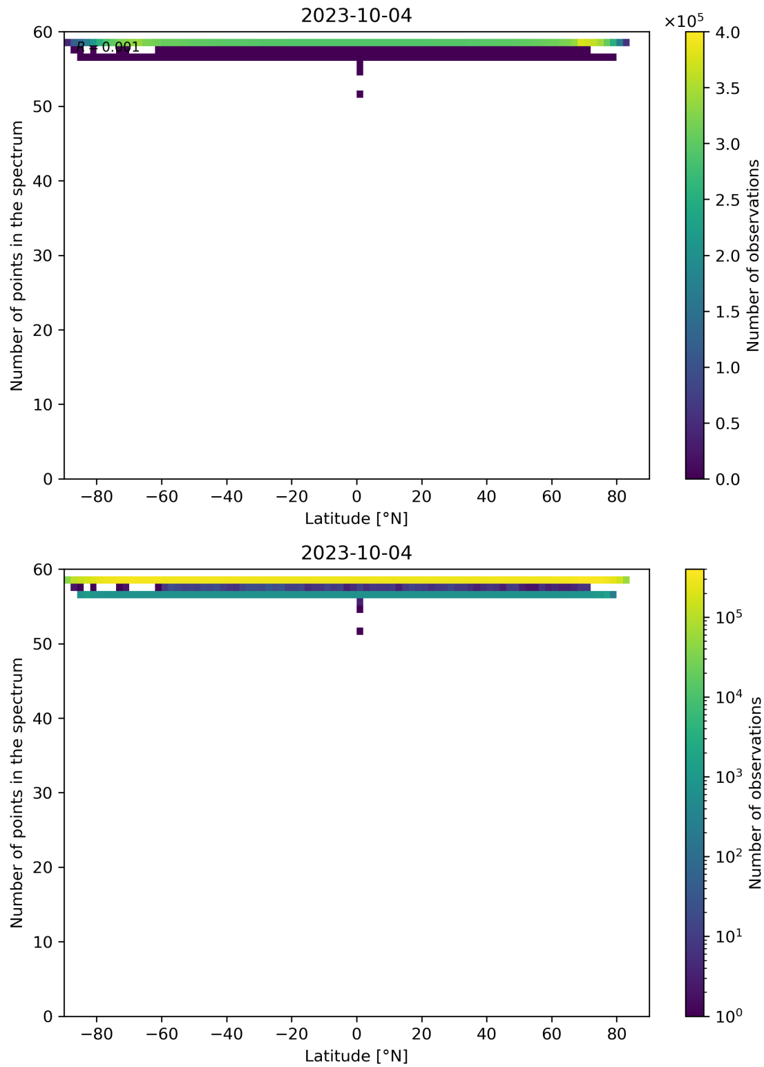
Figure 103: Scatter density plot of “Latitude” against “Number of points in the spectrum” for 2023-10-03 to 2023-10-05.
