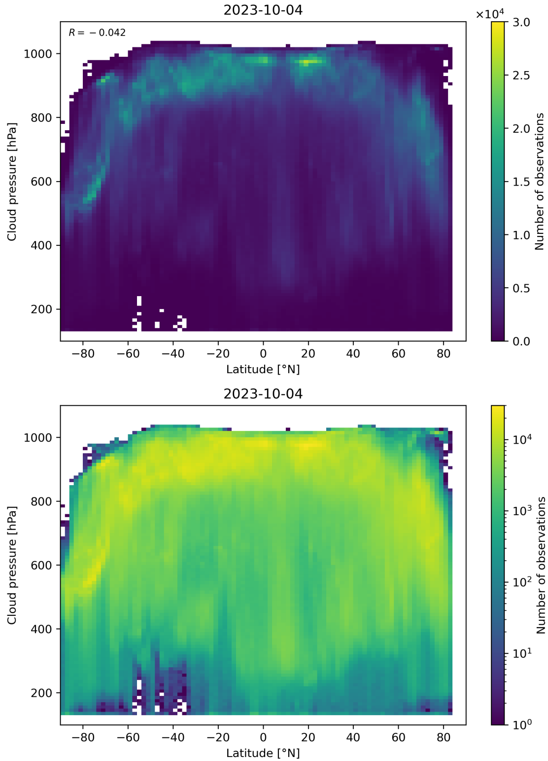
Figure 100: Scatter density plot of “Latitude” against “Cloud pressure” for 2023-10-03 to 2023-10-05.
