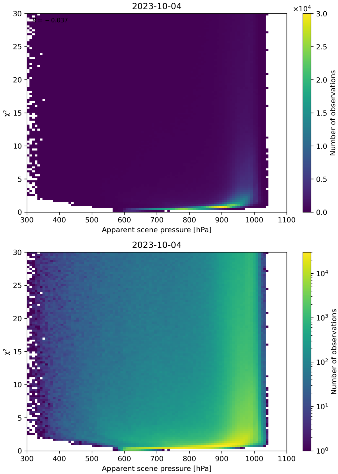
Figure 63: Scatter density plot of “Apparent scene pressure” against “ \chi^2 ” for 2023-10-03 to 2023-10-05.
