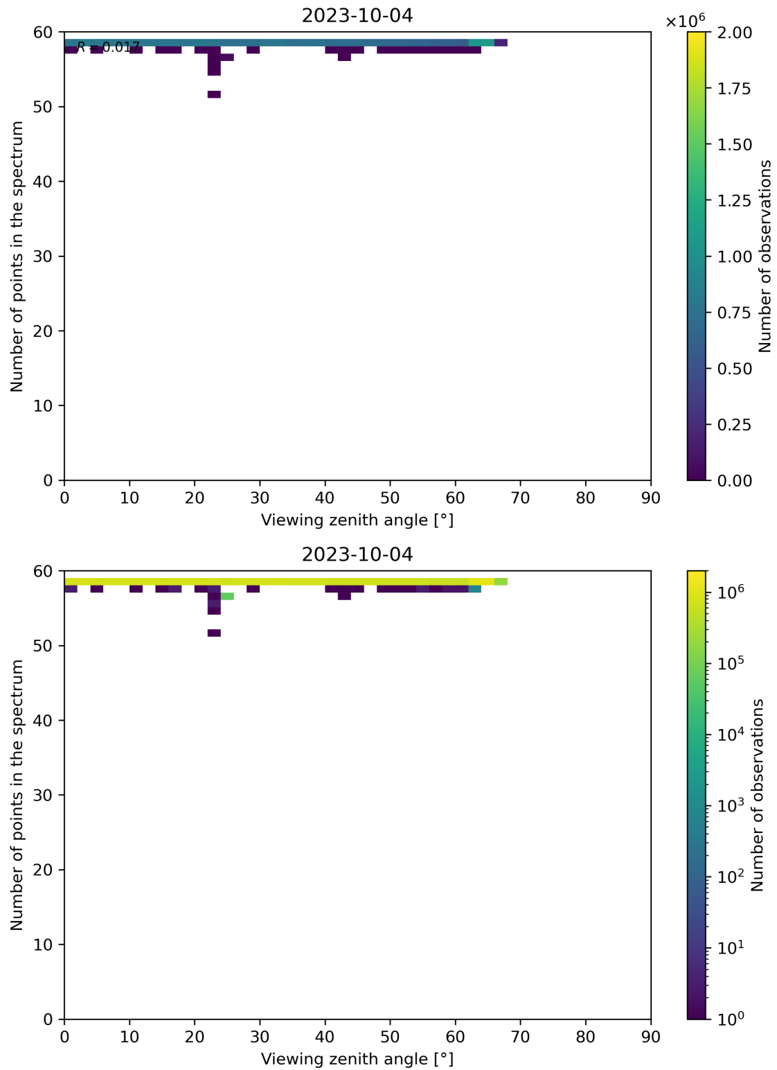
Figure 137: Scatter density plot of “Viewing zenith angle” against “Number of points in the spectrum” for 2023-10-03 to 2023-10-05.
