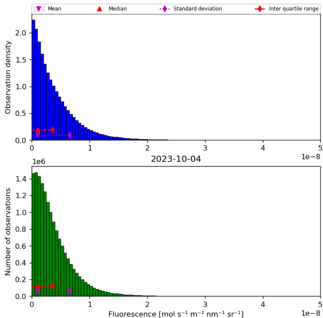
Figure 40: Histogram of “Fluorescence” for 2023-10-03 to 2023-10-05
