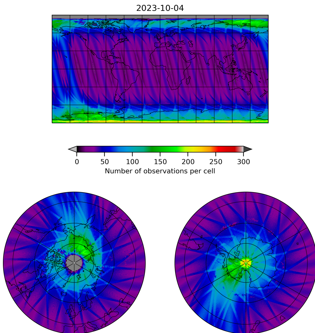
Figure 11: Map of the number of observations for 2023-10-03 to 2023-10-05
