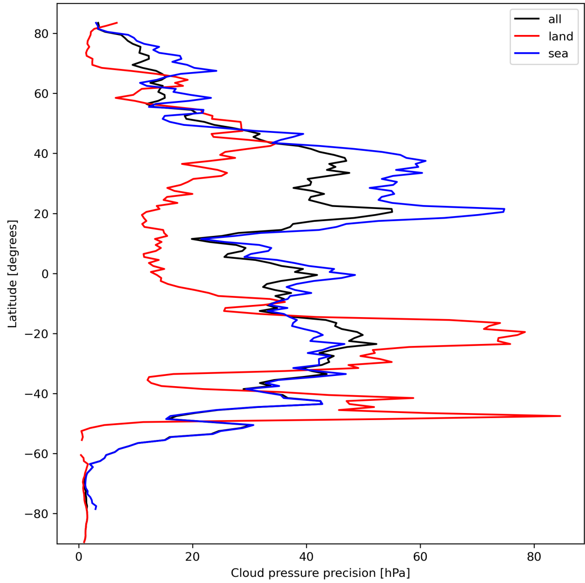
Figure 14: Zonal average of “Cloud pressure precision” for 2023-10-03 to 2023-10-05.
