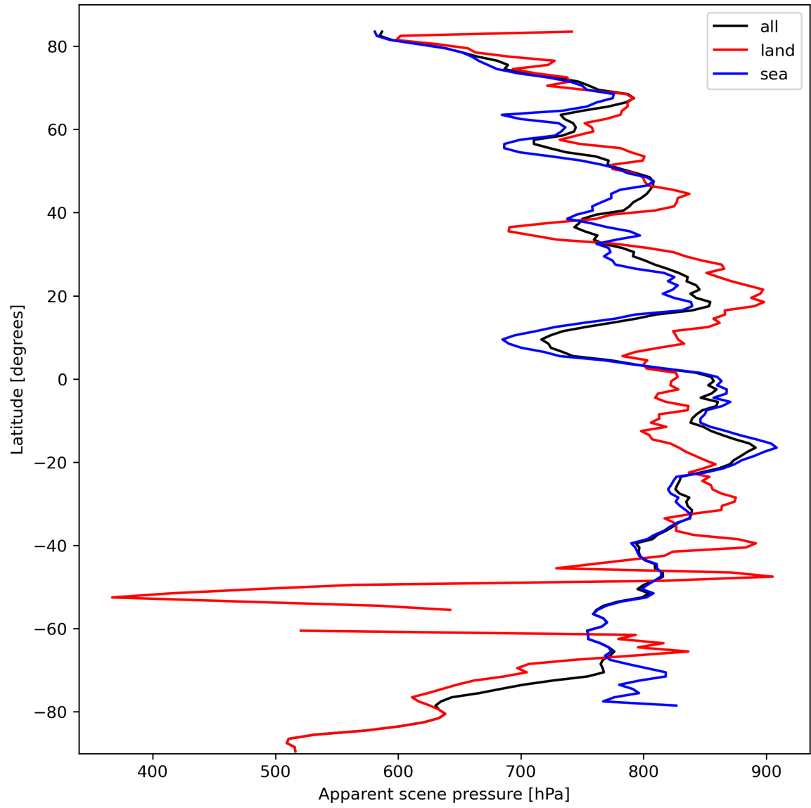
Figure 19: Zonal average of “Apparent scene pressure” for 2023-10-03 to 2023-10-05.
