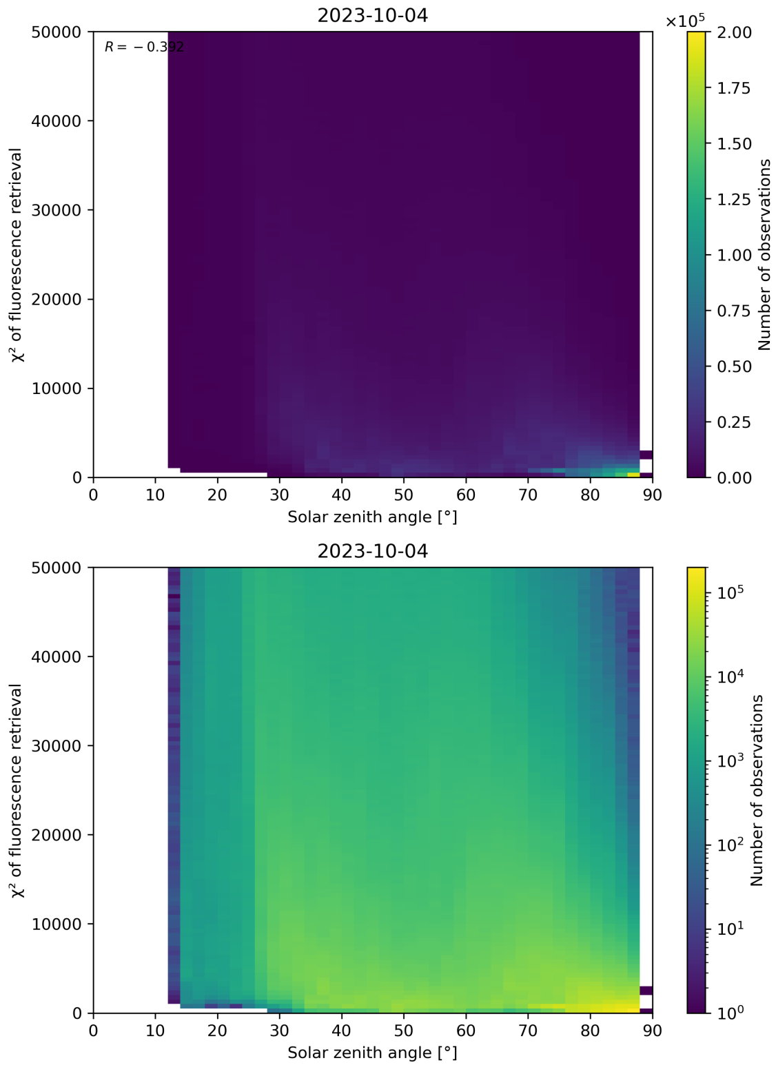
Figure 120: Scatter density plot of “Solar zenith angle” against “ \chi^2 of fluorescence retrieval” for 2023-10-03 to 2023-10-05.
