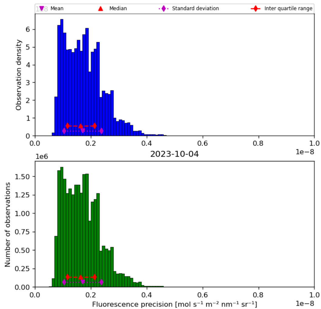
Figure 41: Histogram of “Fluorescence precision” for 2023-10-03 to 2023-10-05
