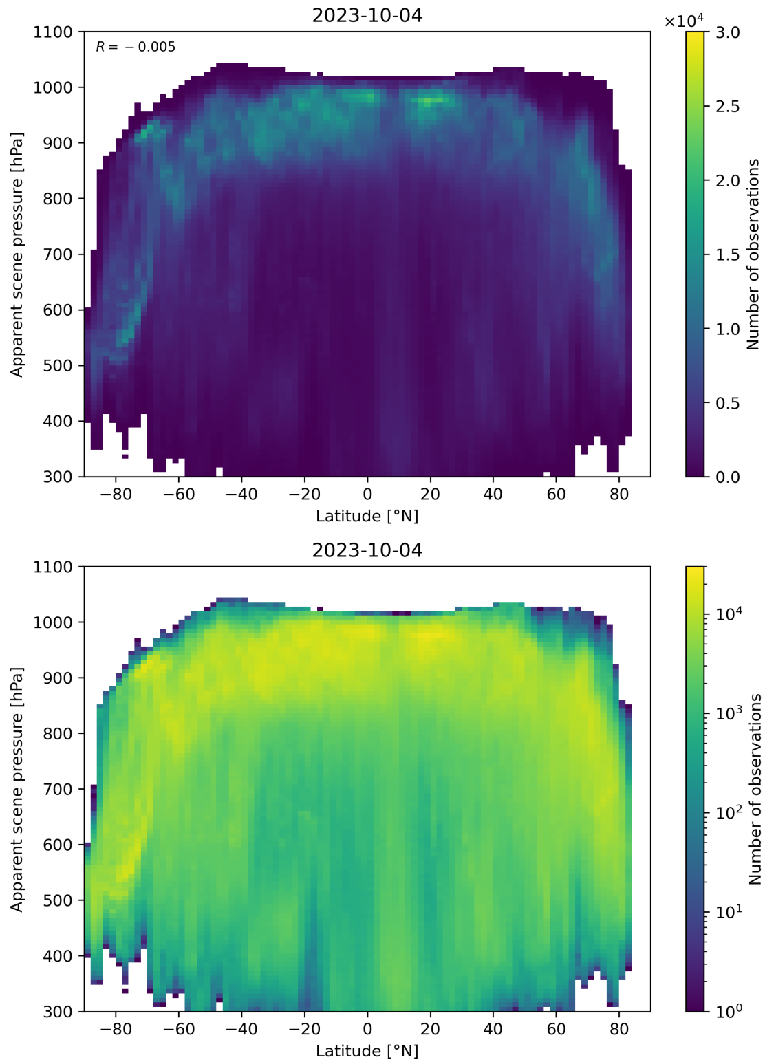
Figure 96: Scatter density plot of “Latitude” against “Apparent scene pressure” for 2023-10-03 to 2023-10-05.
