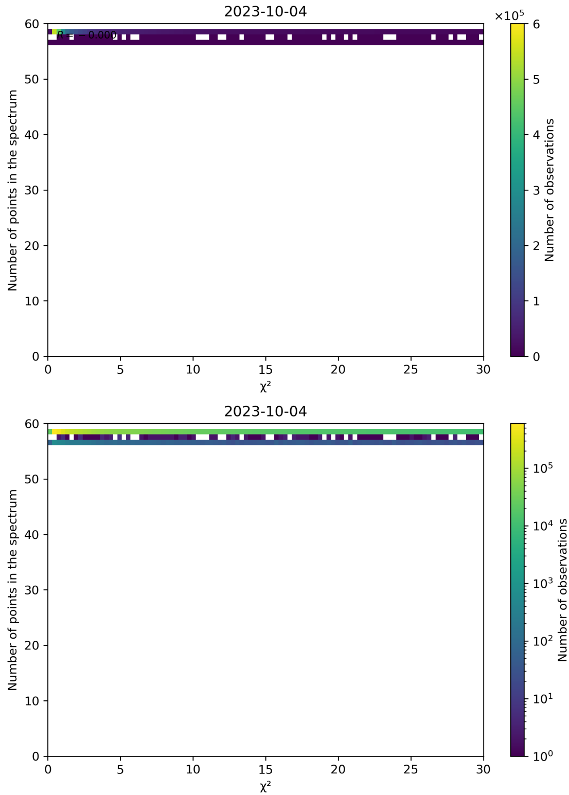
Figure 74: Scatter density plot of “ \chi^2 ” against “Number of points in the spectrum” for 2023-10-03 to 2023-10-05.
