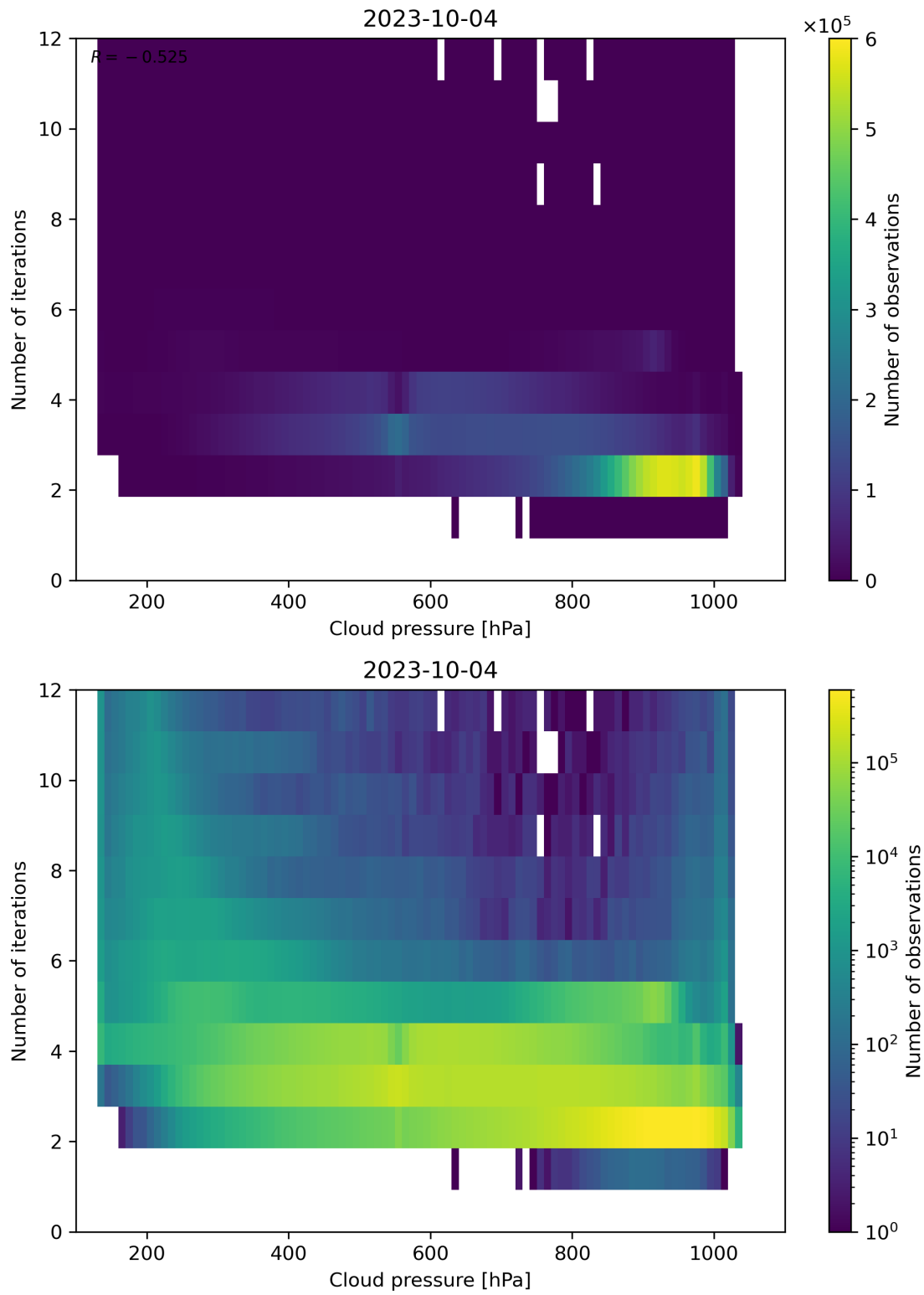
Figure 89: Scatter density plot of “Cloud pressure” against “Number of iterations” for 2023-10-03 to 2023-10-05.
