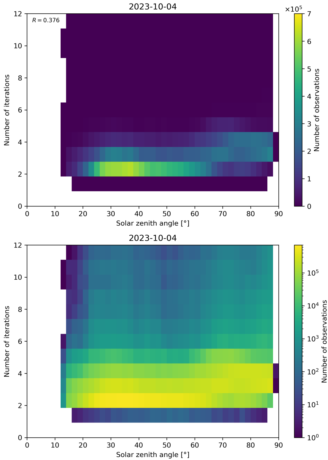
Figure 125: Scatter density plot of “Solar zenith angle” against “Number of iterations” for 2023-10-03 to 2023-10-05.
