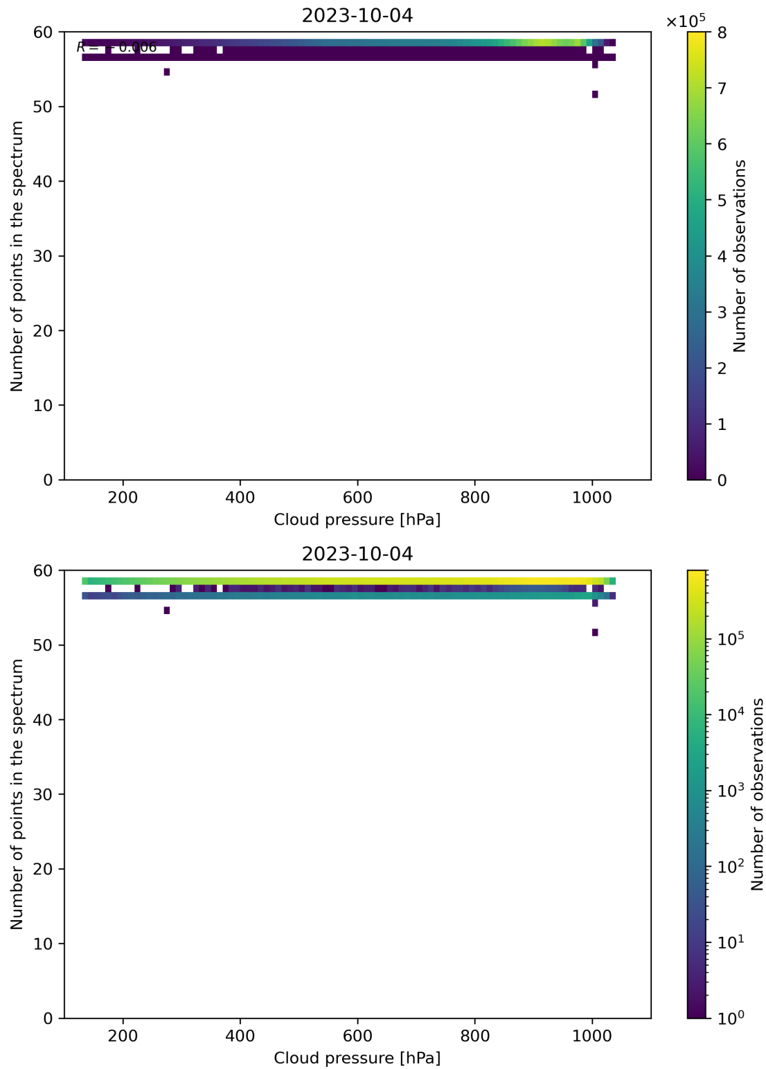
Figure 90: Scatter density plot of “Cloud pressure” against “Number of points in the spectrum” for 2023-10-03 to 2023-10-05.
