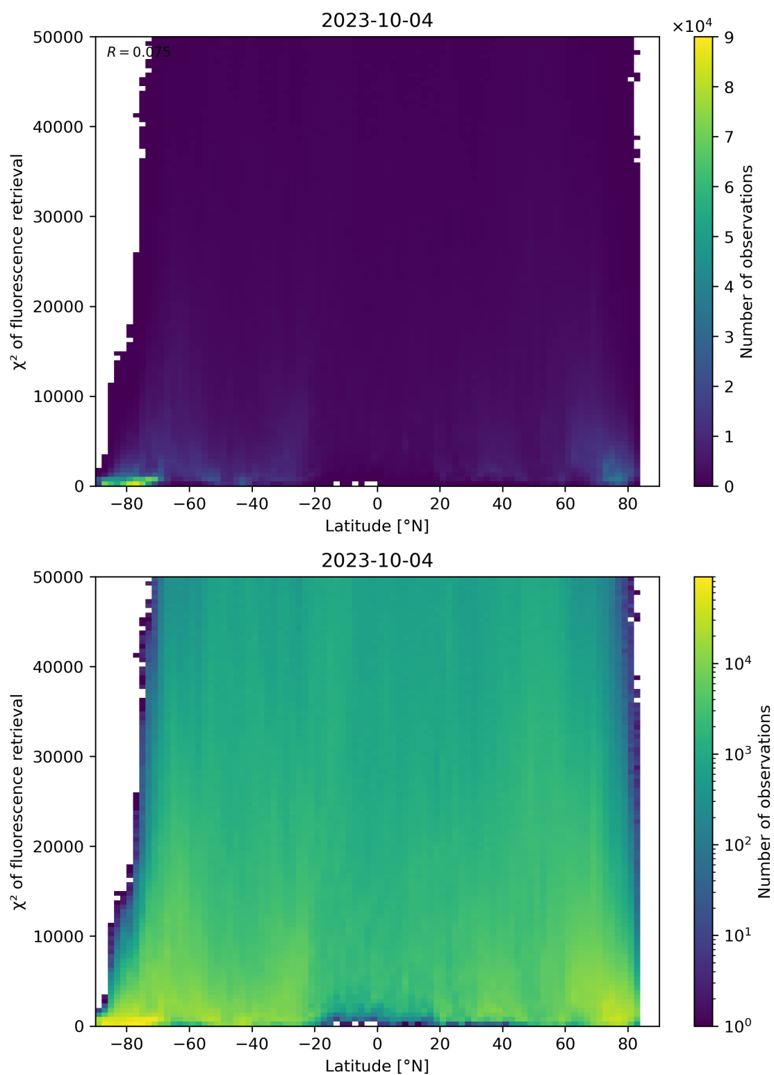
Figure 98: Scatter density plot of “Latitude” against “ \chi^2 of fluorescence retrieval” for 2023-10-03 to 2023-10-05.
