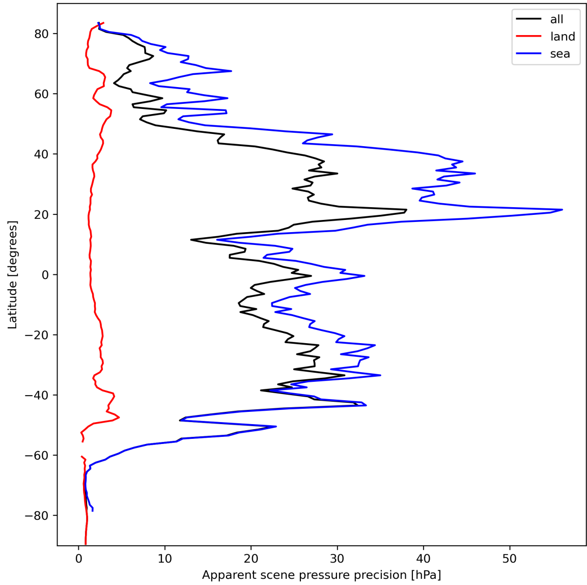
Figure 20: Zonal average of “Apparent scene pressure precision” for 2023-10-03 to 2023-10-05.
