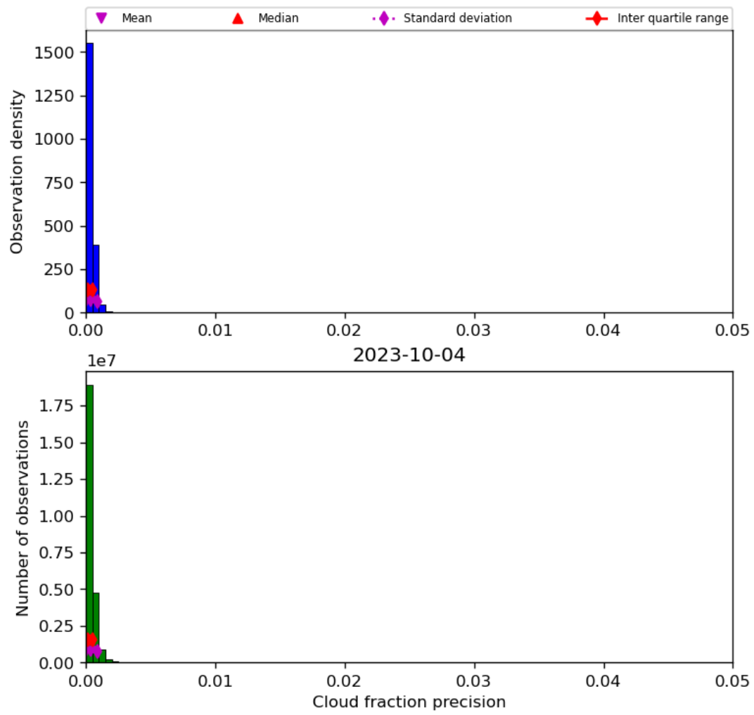
Figure 33: Histogram of “Cloud fraction precision” for 2023-10-03 to 2023-10-05
