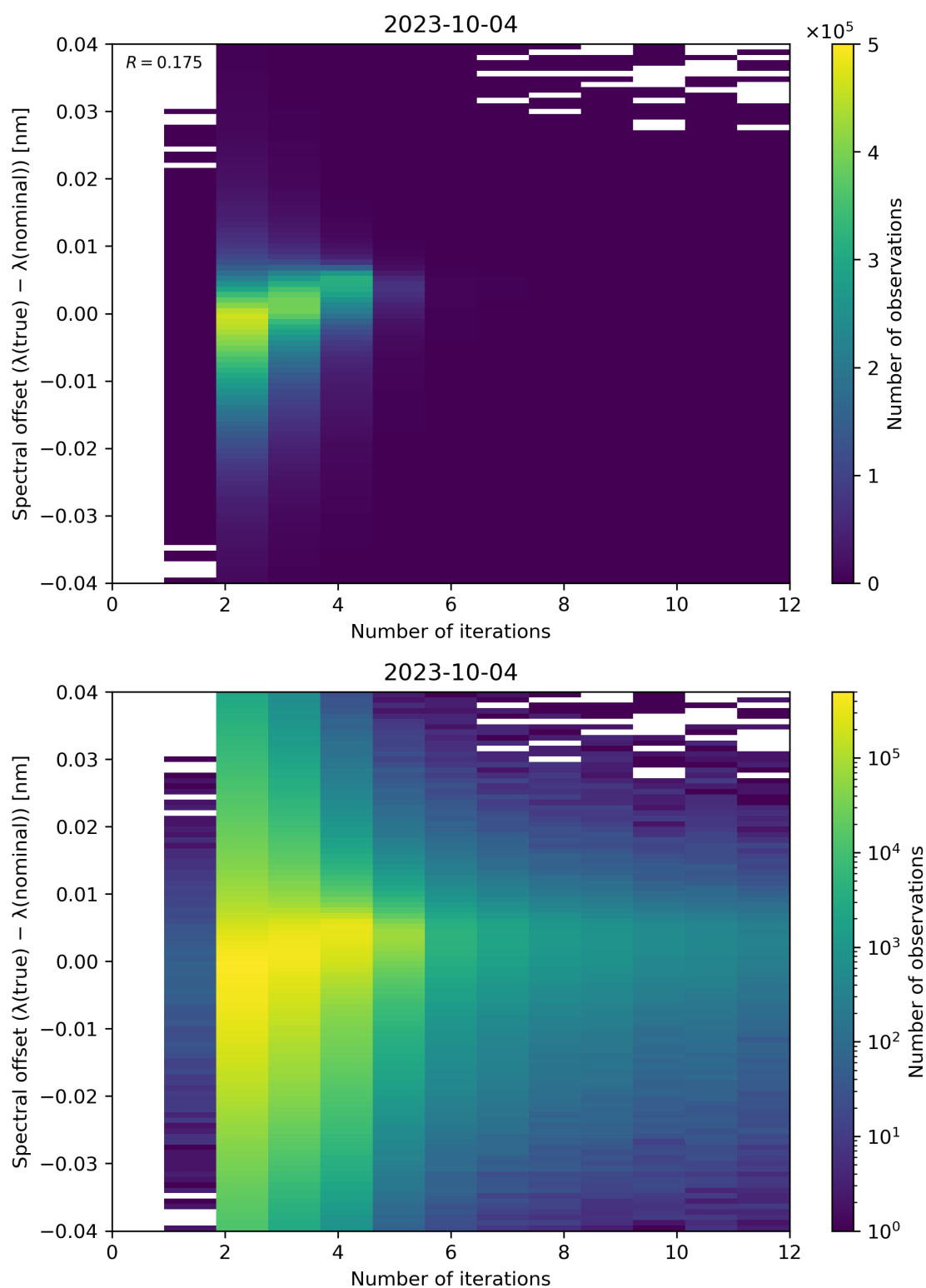
Figure 109: Scatter density plot of “Number of iterations” against “Spectral offset ( \lambda(\text{true}) - \lambda(\text{nominal}) )” for 2023-10-03 to 2023-10-05.
