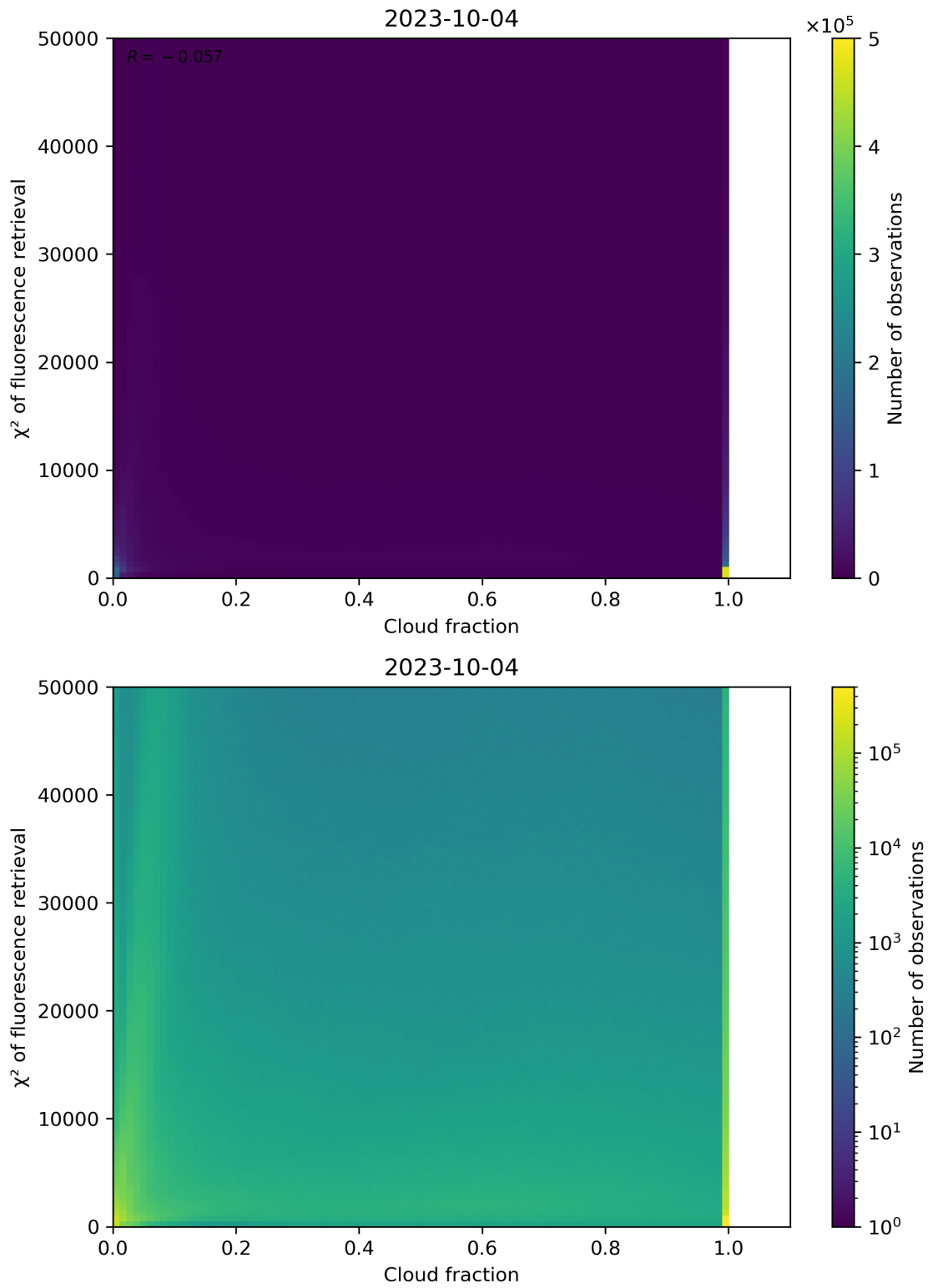
Figure 78: Scatter density plot of “Cloud fraction” against “ \chi^2 of fluorescence retrieval” for 2023-10-03 to 2023-10-05.
