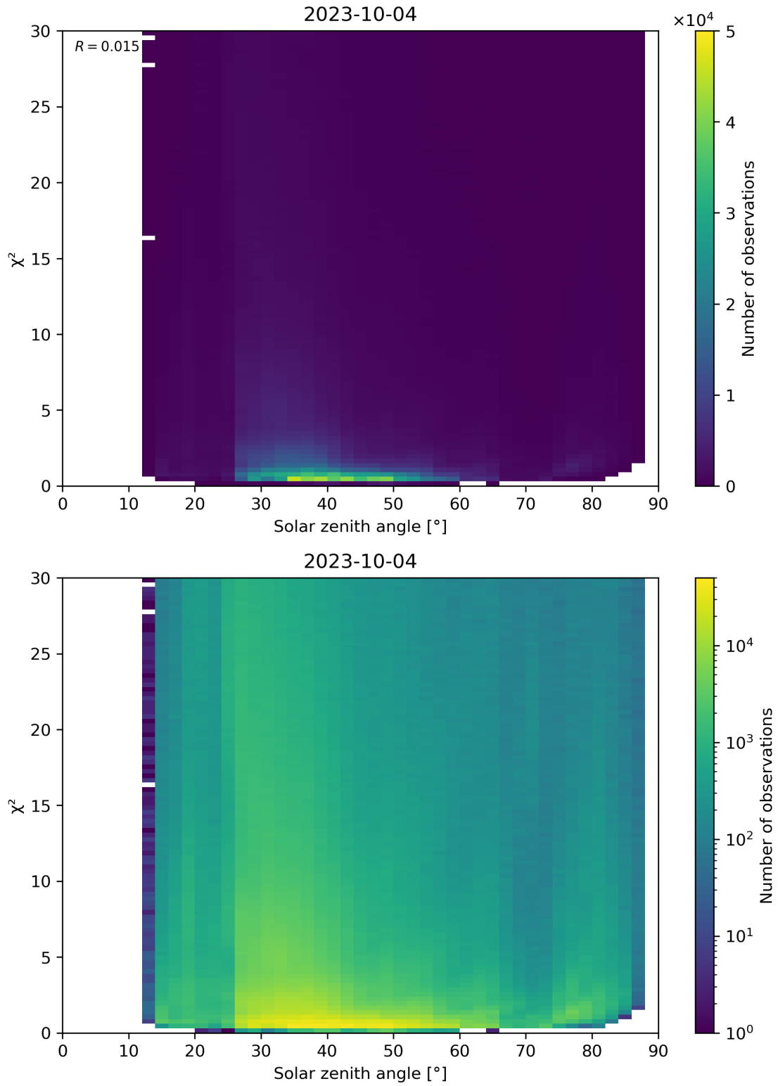
Figure 119: Scatter density plot of “Solar zenith angle” against “ \chi^2 ” for 2023-10-03 to 2023-10-05.
