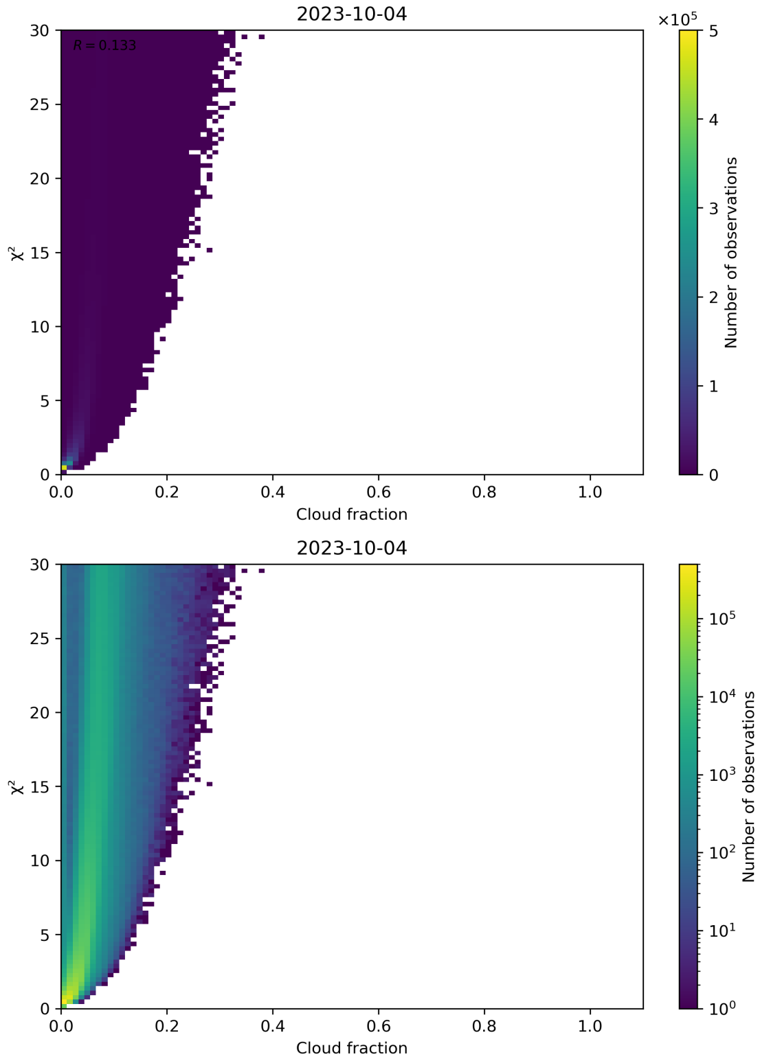
Figure 77: Scatter density plot of “Cloud fraction” against “ \chi^2 ” for 2023-10-03 to 2023-10-05.
