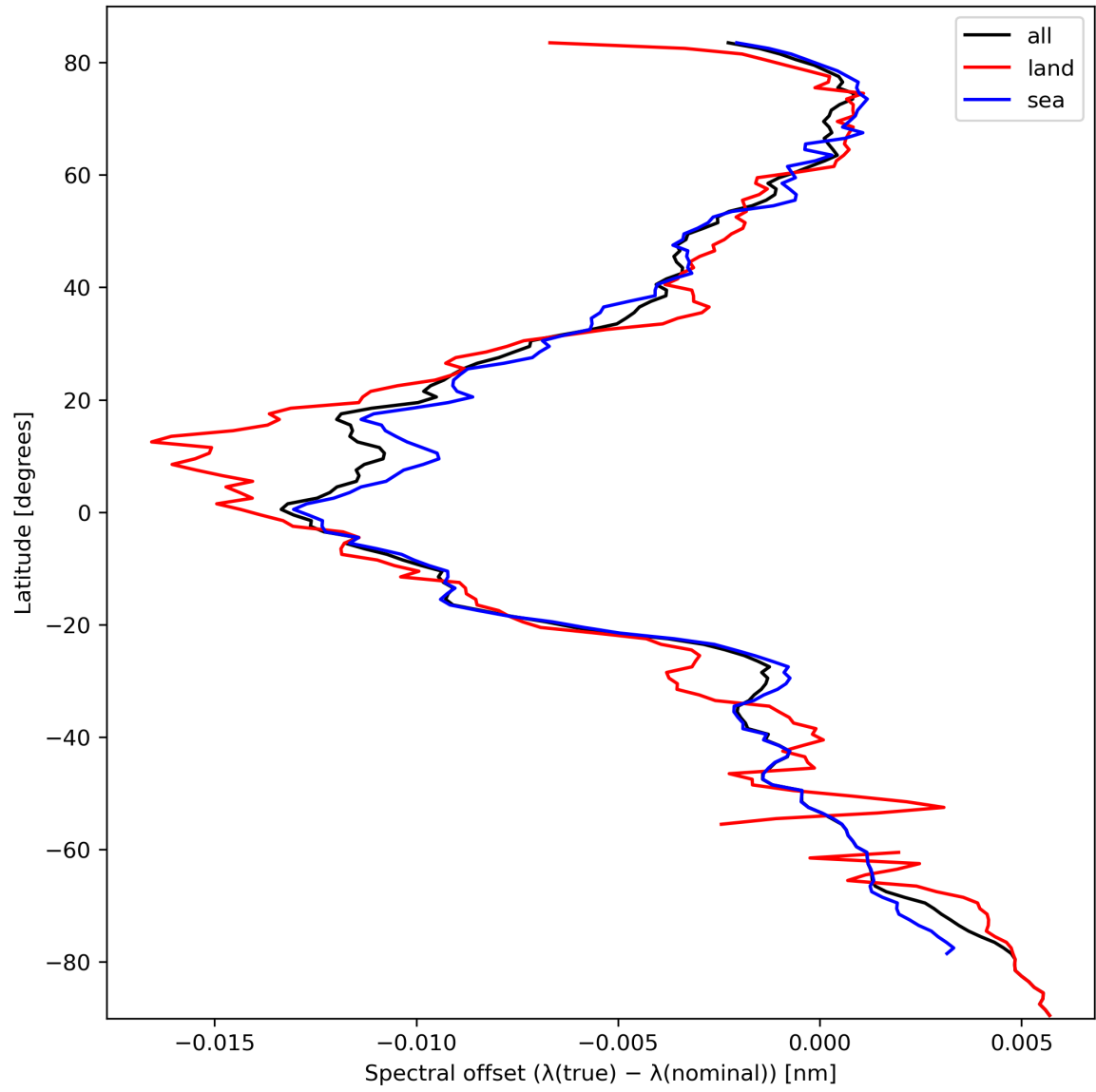
Figure 28: Zonal average of “Spectral offset ( \lambda(\text{true}) - \lambda(\text{nominal}) )” for 2023-10-03 to 2023-10-05.
