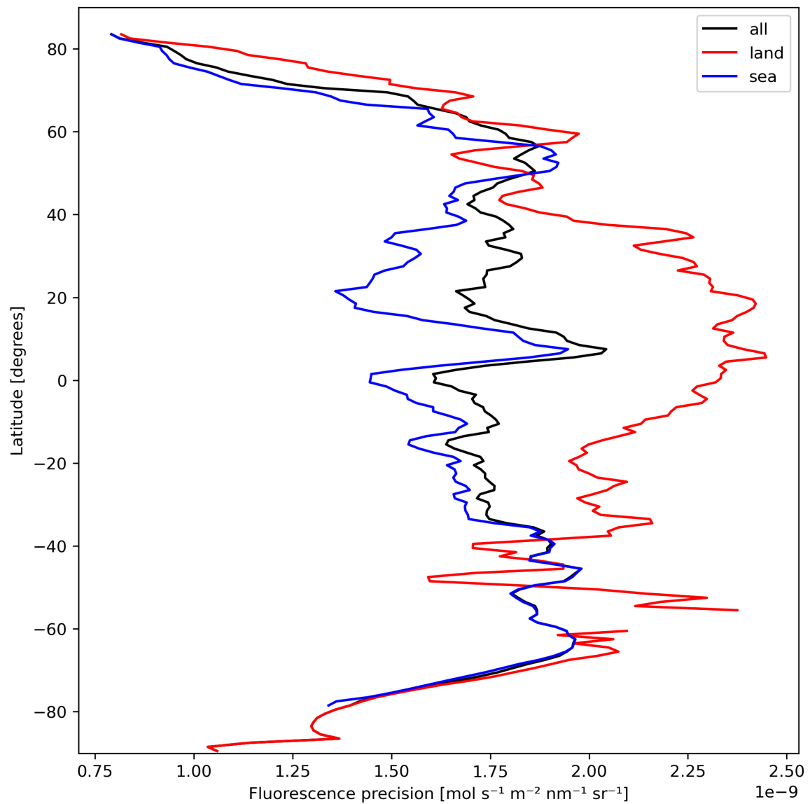
Figure 24: Zonal average of “Fluorescence precision” for 2023-10-03 to 2023-10-05.
