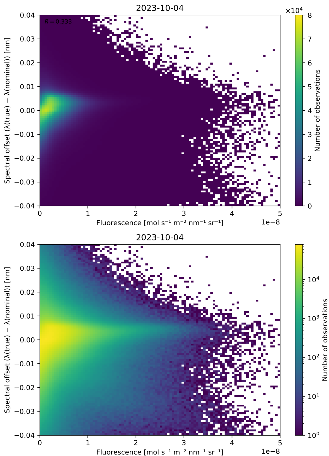
Figure 95: Scatter density plot of “Fluorescence” against “Spectral offset ( \lambda(\text{true}) - \lambda(\text{nominal}) )” for 2023-10-03 to 2023-10-05.
