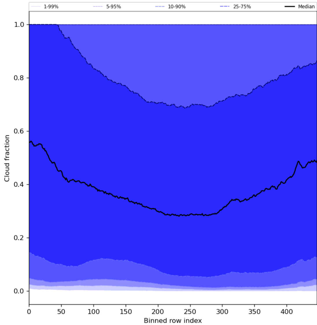
Figure 49: Along track statistics of “Cloud fraction” for 2023-10-03 to 2023-10-05
