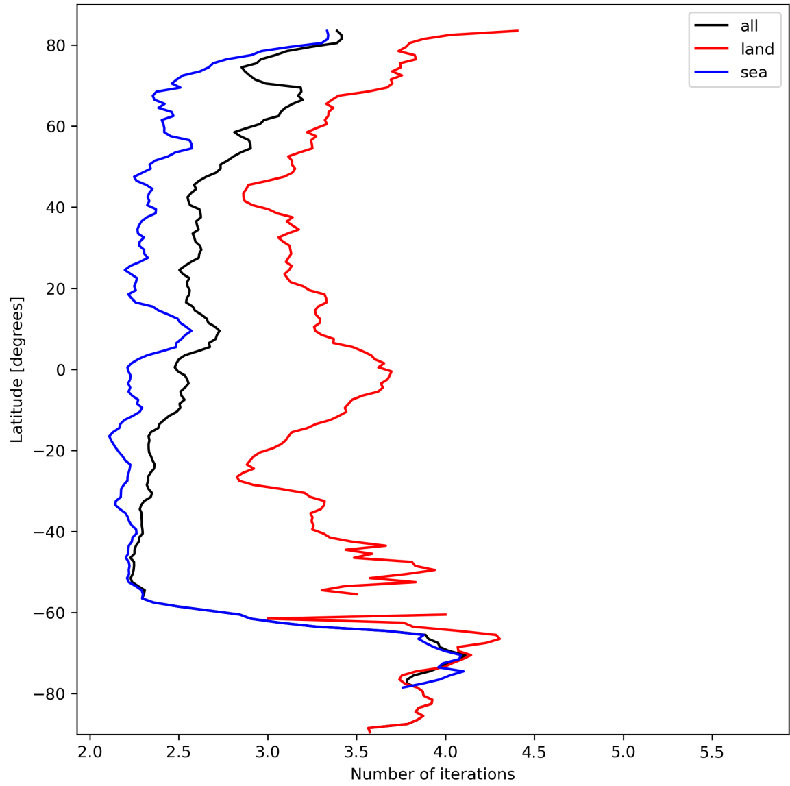
Figure 22: Zonal average of “Number of iterations” for 2023-10-03 to 2023-10-05.
