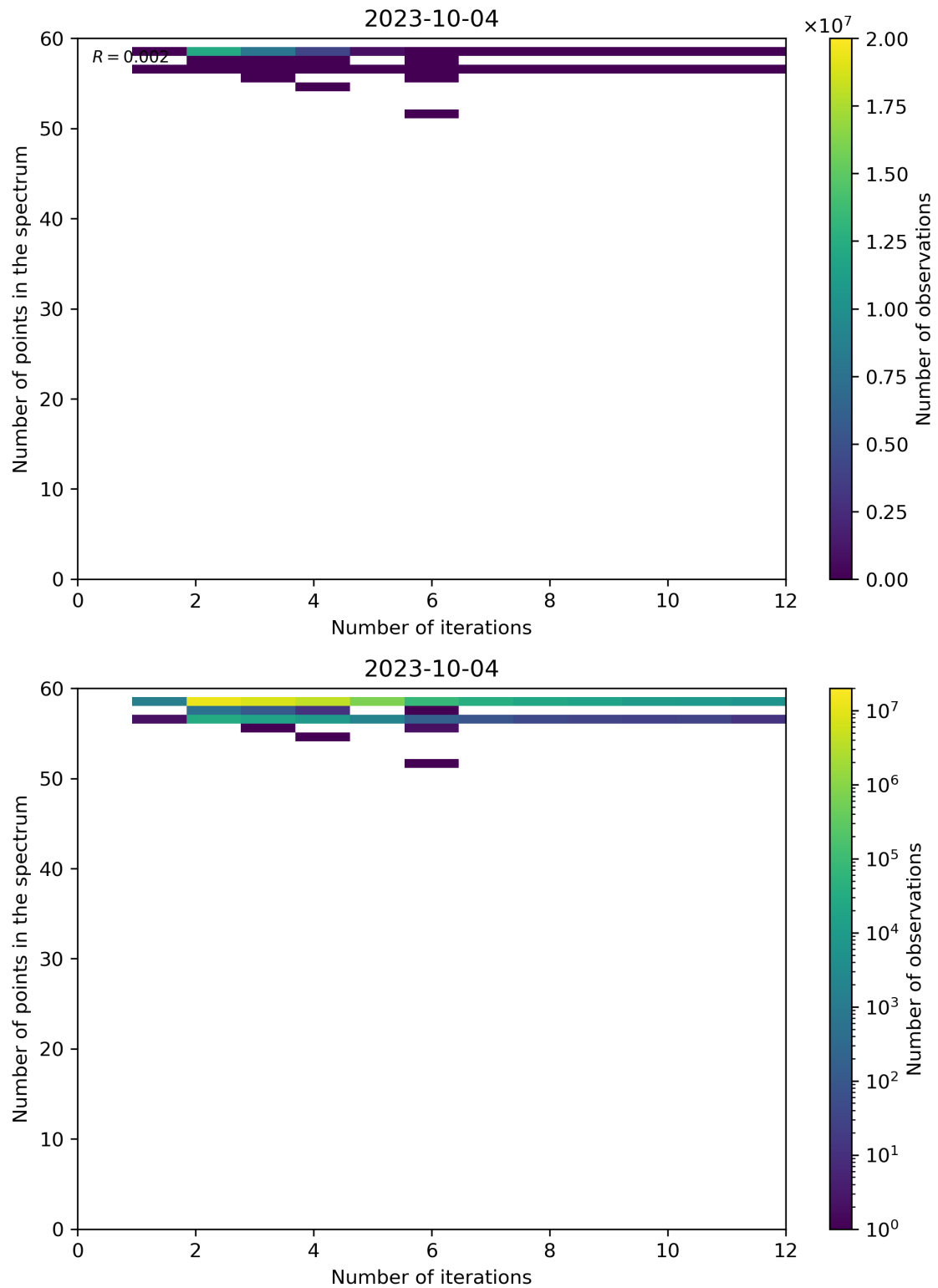
Figure 108: Scatter density plot of “Number of iterations” against “Number of points in the spectrum” for 2023-10-03 to 2023-10-05.
