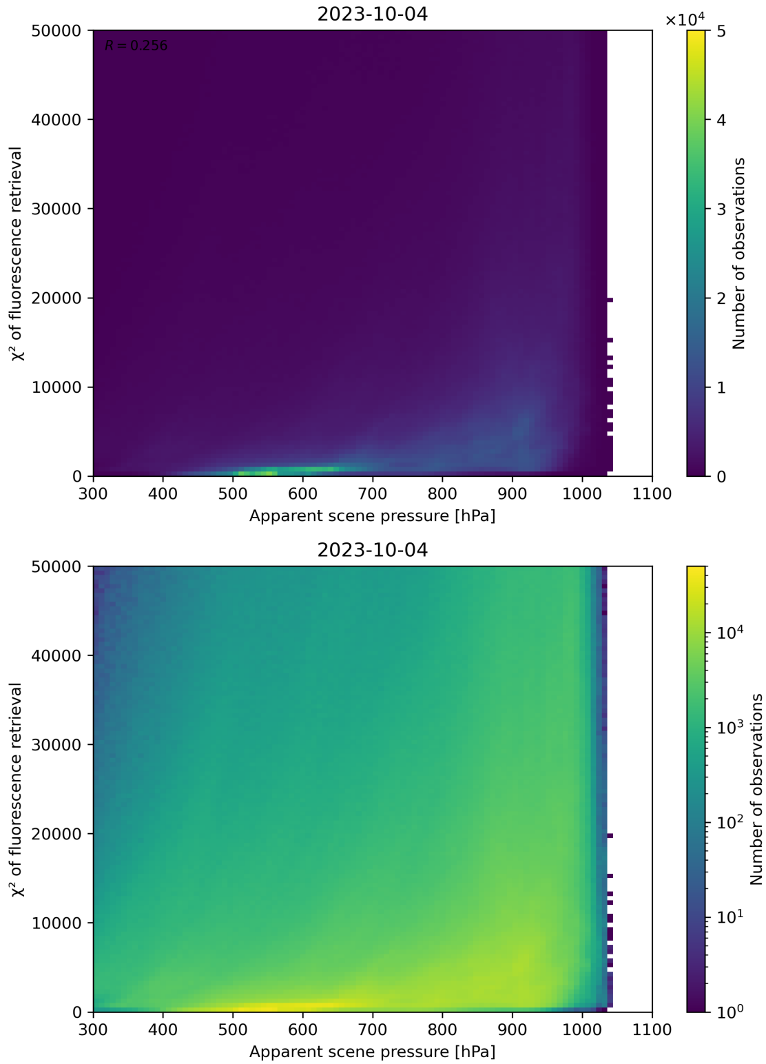
Figure 64: Scatter density plot of “Apparent scene pressure” against “ \chi^2 of fluorescence retrieval” for 2023-10-03 to 2023-10-05.
