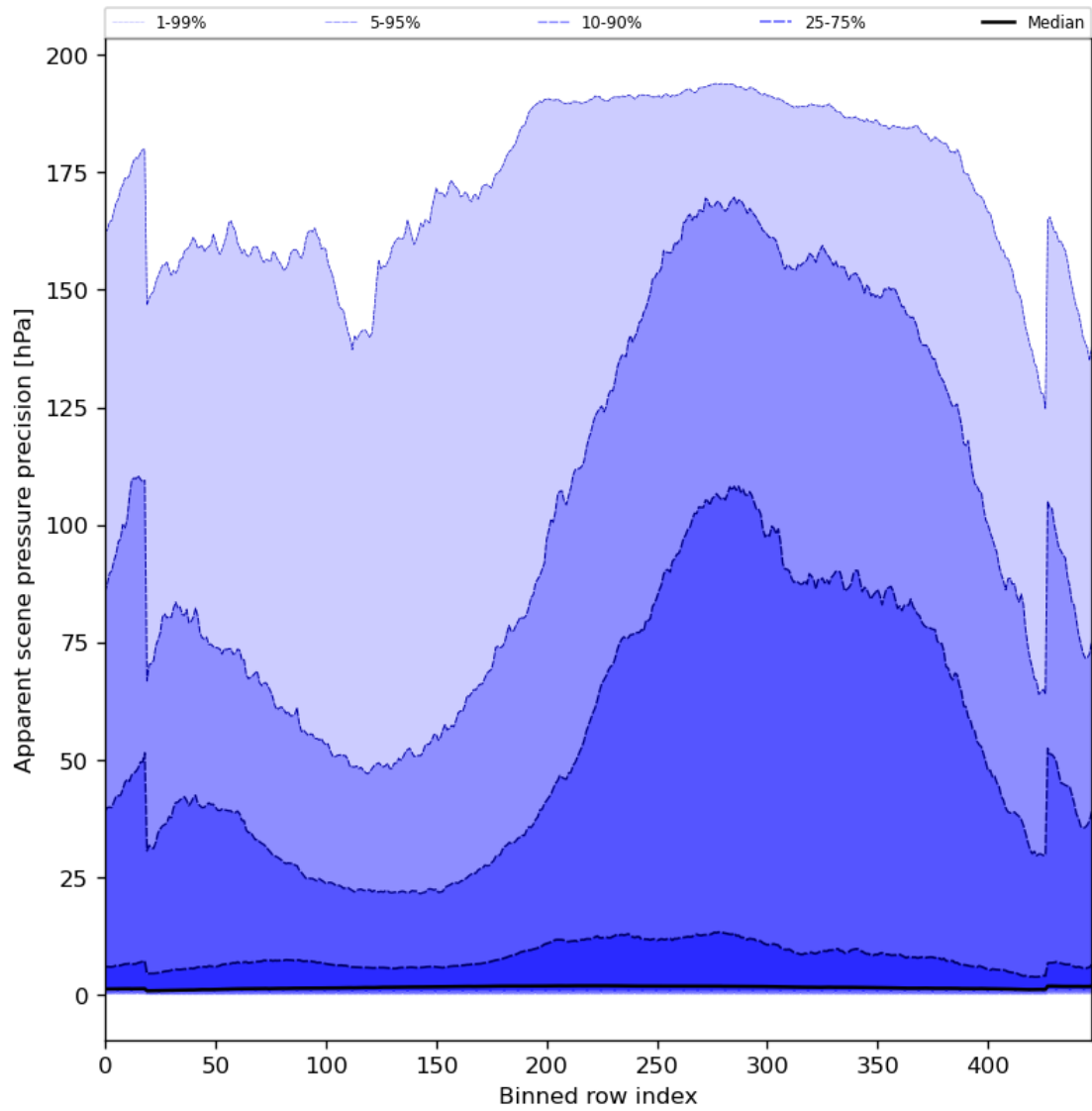
Figure 54: Along track statistics of “Apparent scene pressure precision” for 2023-10-03 to 2023-10-05
