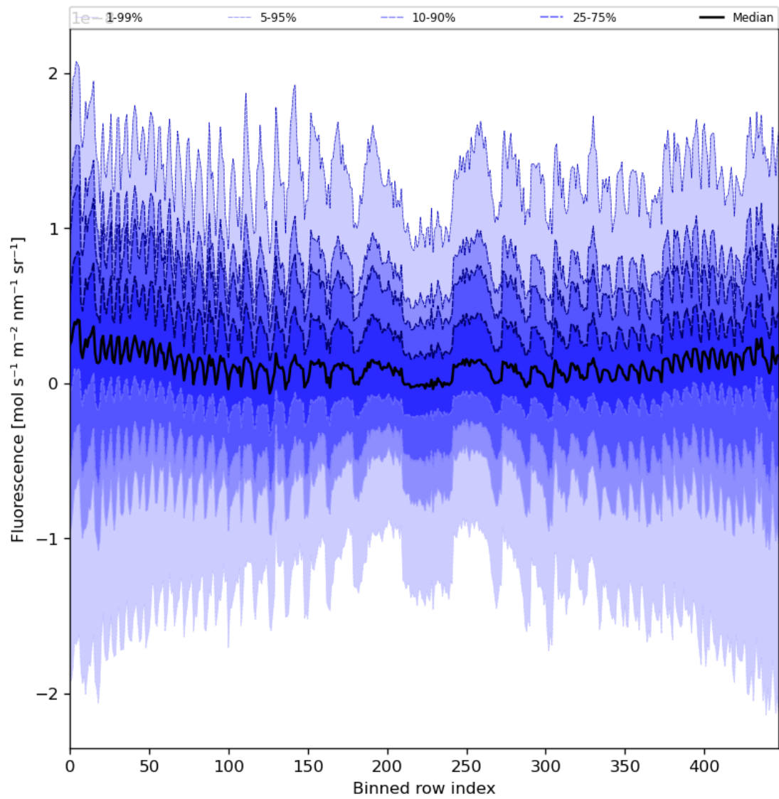
Figure 57: Along track statistics of “Fluorescence” for 2023-10-03 to 2023-10-05
