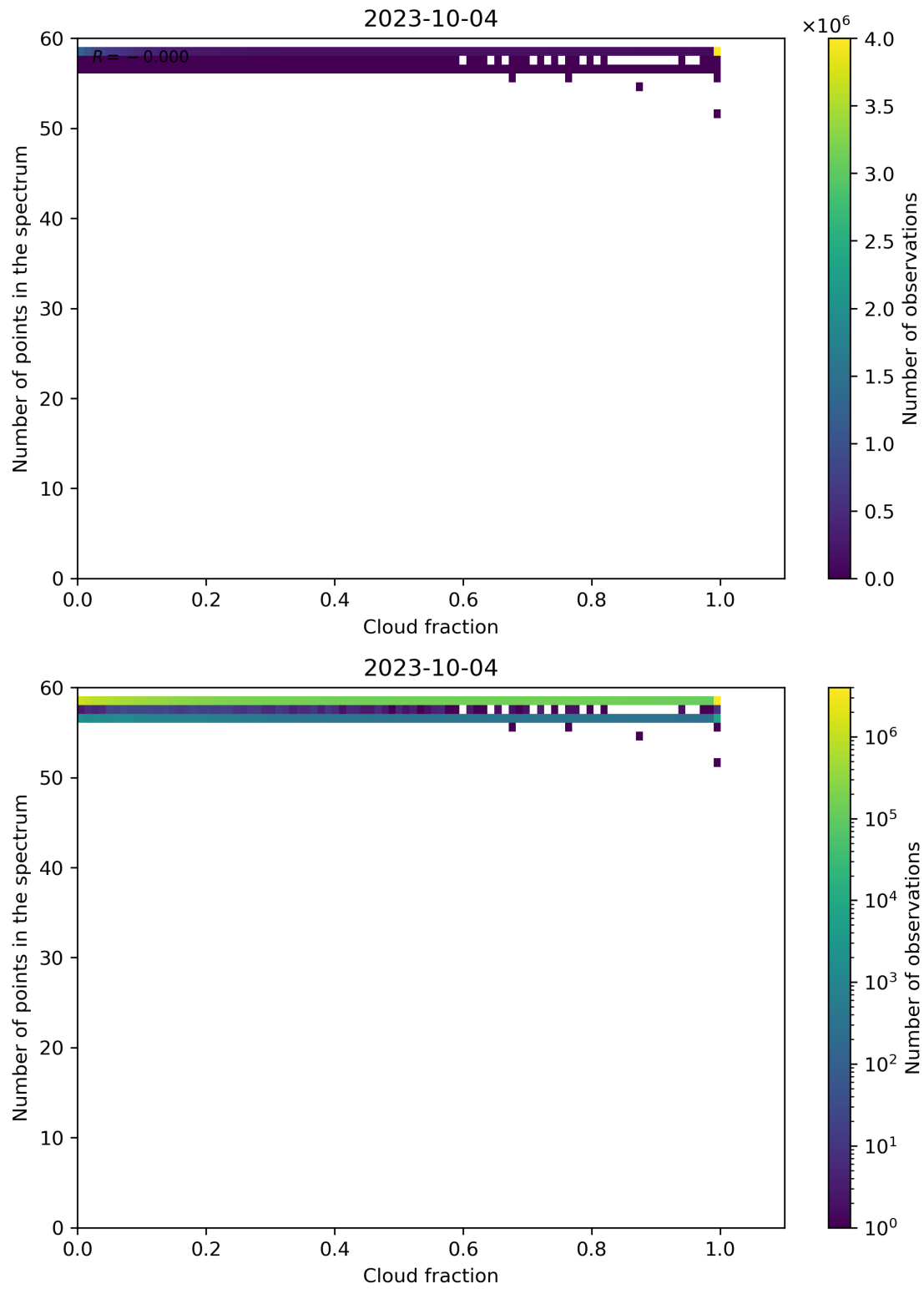
Figure 81: Scatter density plot of “Cloud fraction” against “Number of points in the spectrum” for 2023-10-03 to 2023-10-05.
