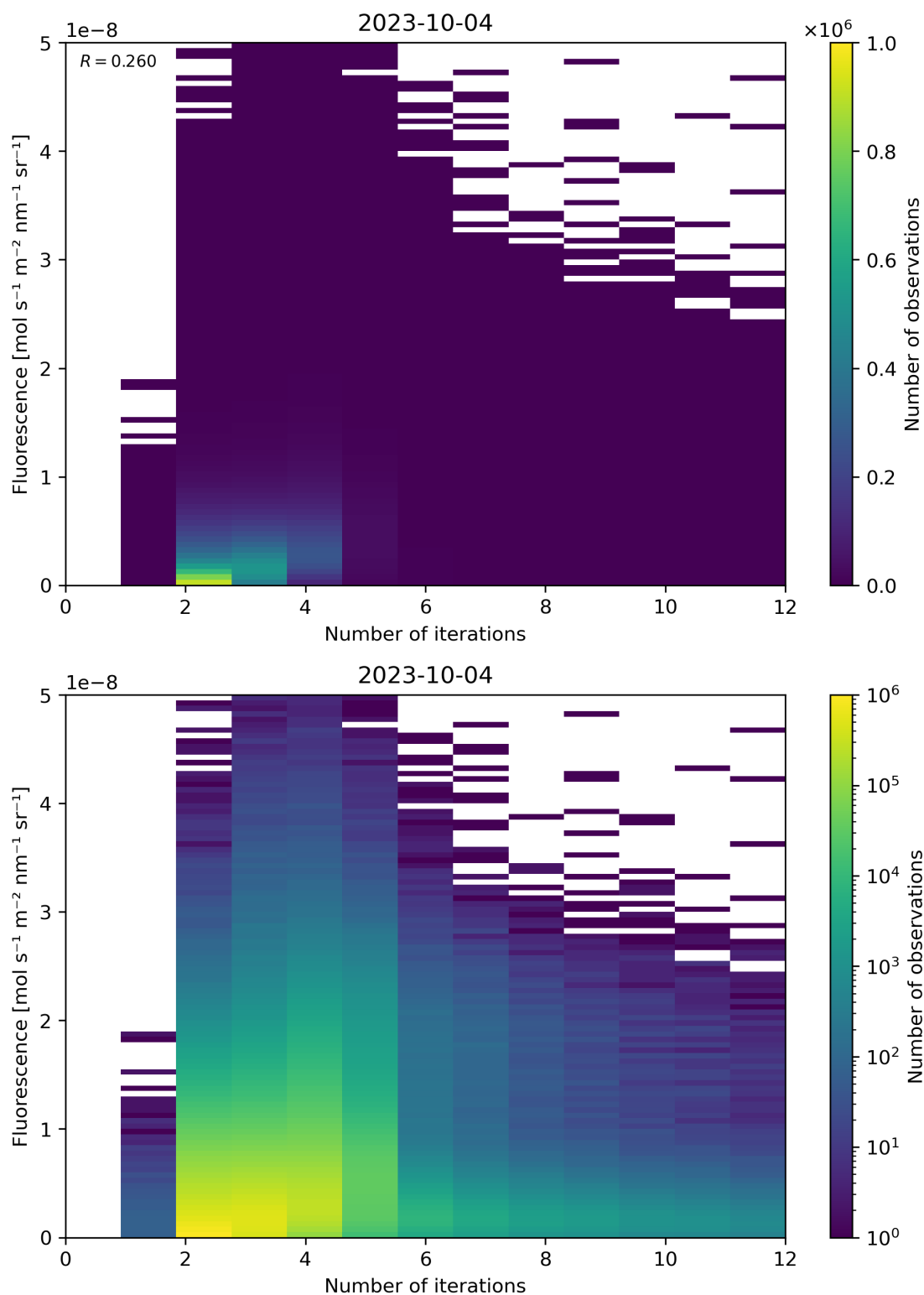
Figure 107: Scatter density plot of “Number of iterations” against “Fluorescence” for 2023-10-03 to 2023-10-05.
