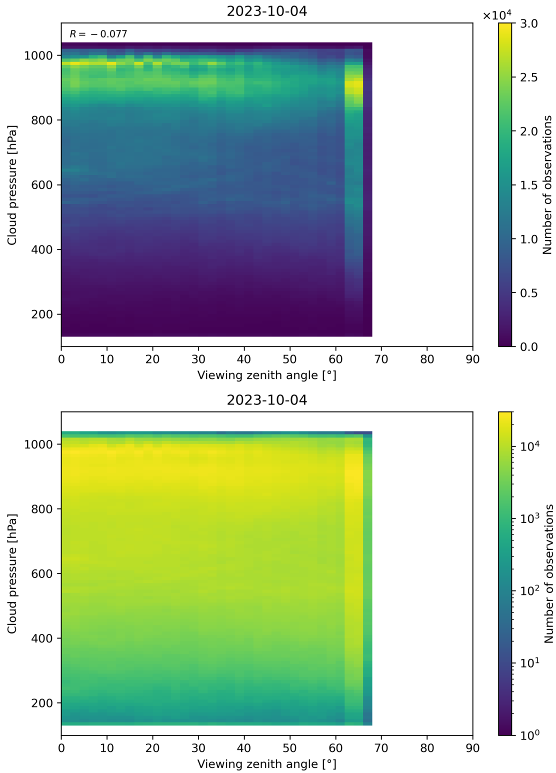
Figure 133: Scatter density plot of “Viewing zenith angle” against “Cloud pressure” for 2023-10-03 to 2023-10-05.
