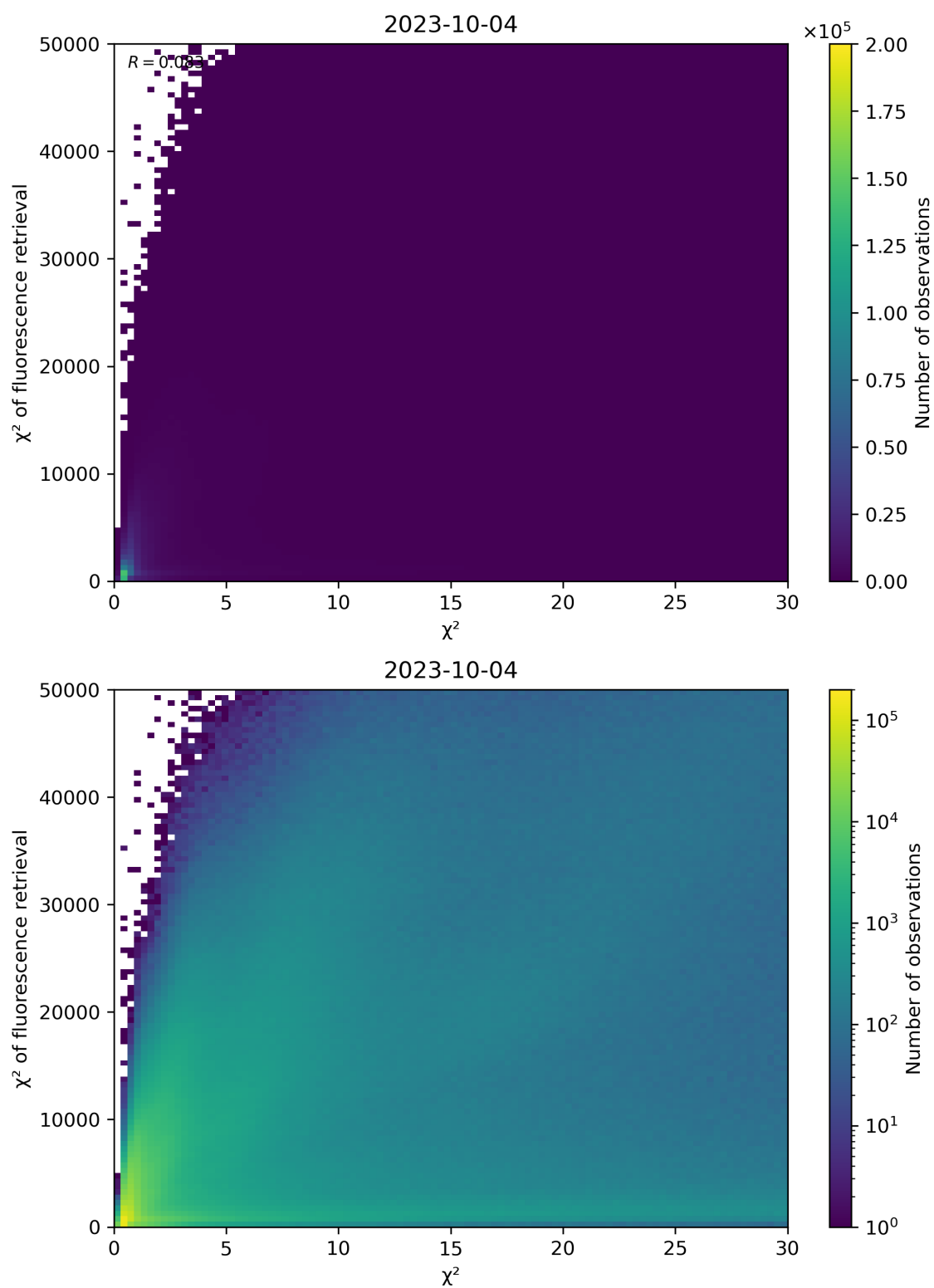
Figure 69: Scatter density plot of “ \chi^2 ” against “ \chi^2 of fluorescence retrieval” for 2023-10-03 to 2023-10-05.
