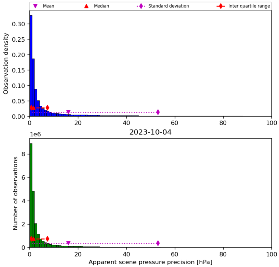
Figure 37: Histogram of “Apparent scene pressure precision” for 2023-10-03 to 2023-10-05
