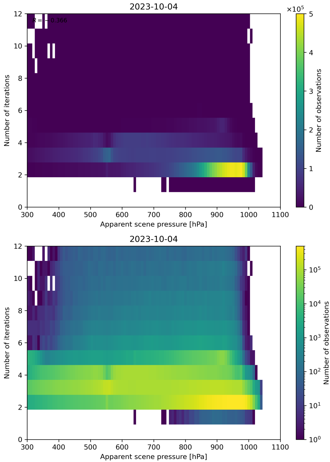
Figure 66: Scatter density plot of “Apparent scene pressure” against “Number of iterations” for 2023-10-03 to 2023-10-05.
