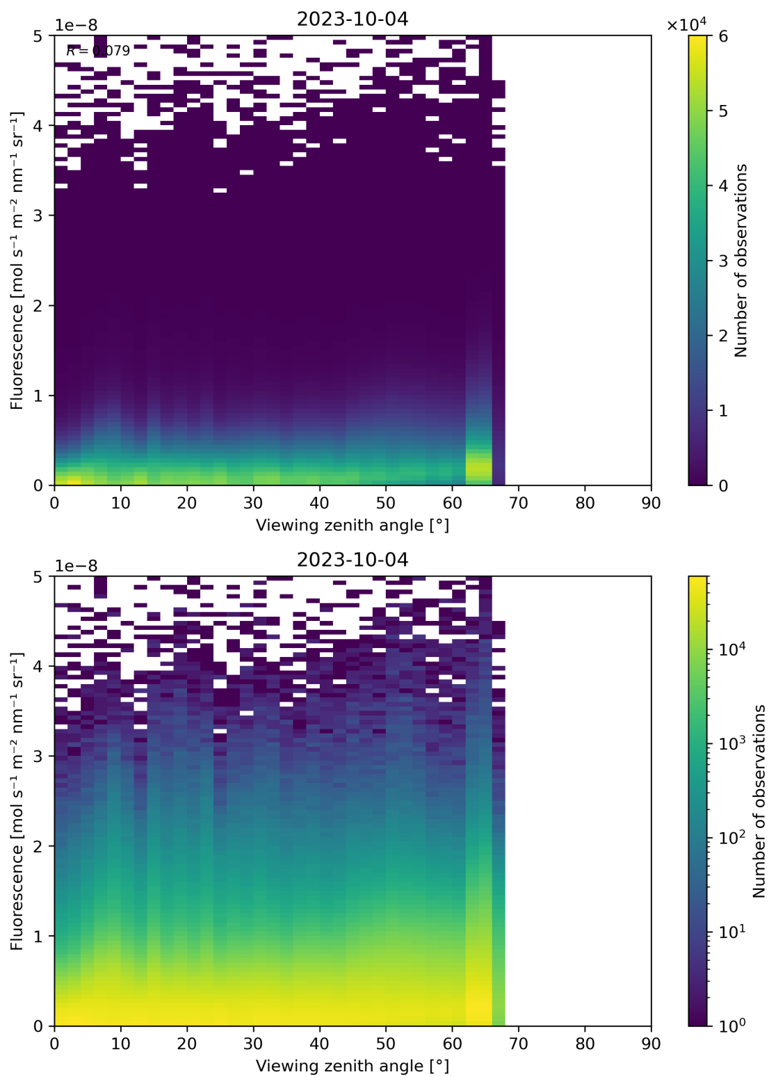
Figure 134: Scatter density plot of “Viewing zenith angle” against “Fluorescence” for 2023-10-03 to 2023-10-05.
