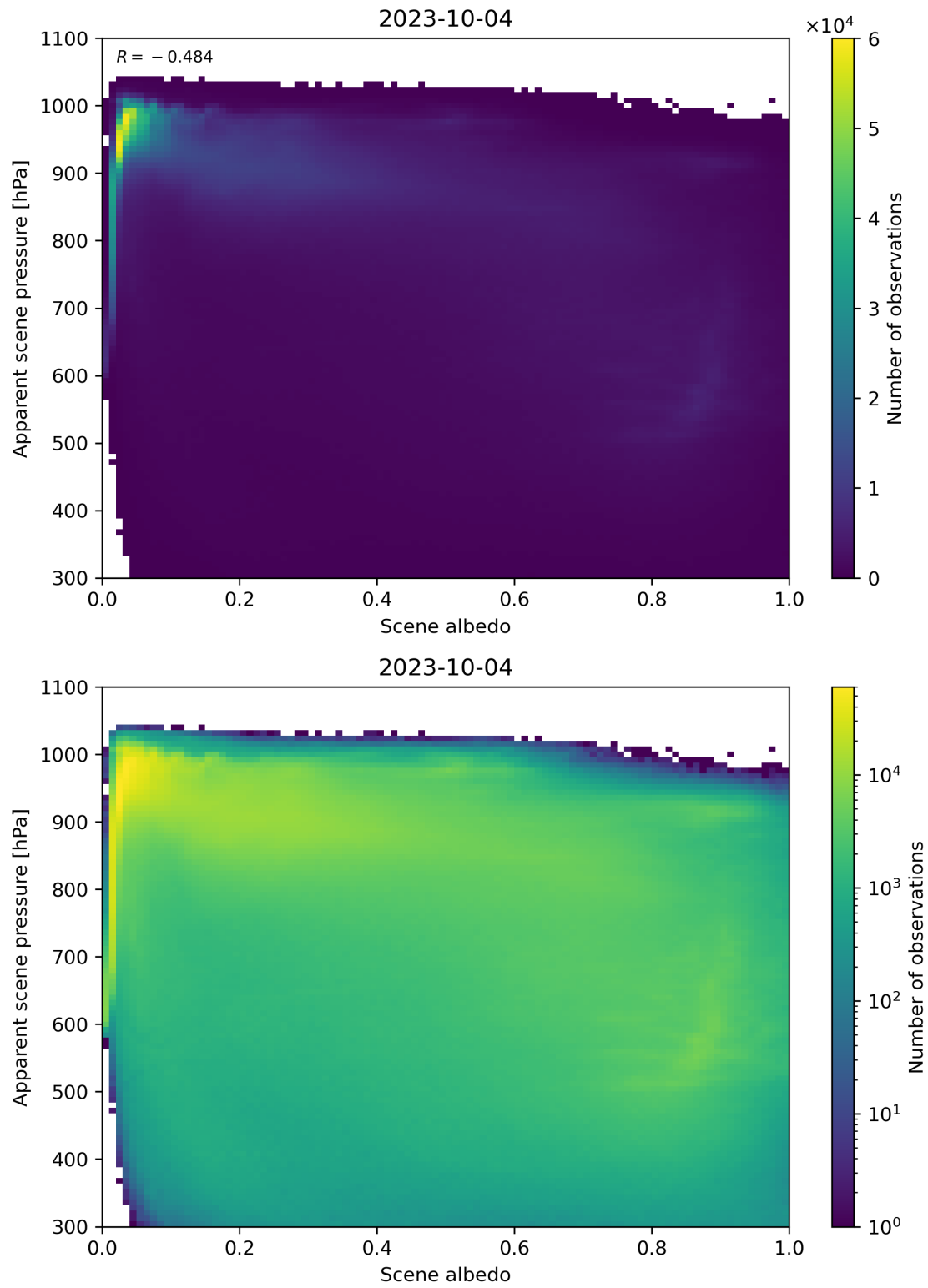
Figure 111: Scatter density plot of “Scene albedo” against “Apparent scene pressure” for 2023-10-03 to 2023-10-05.
