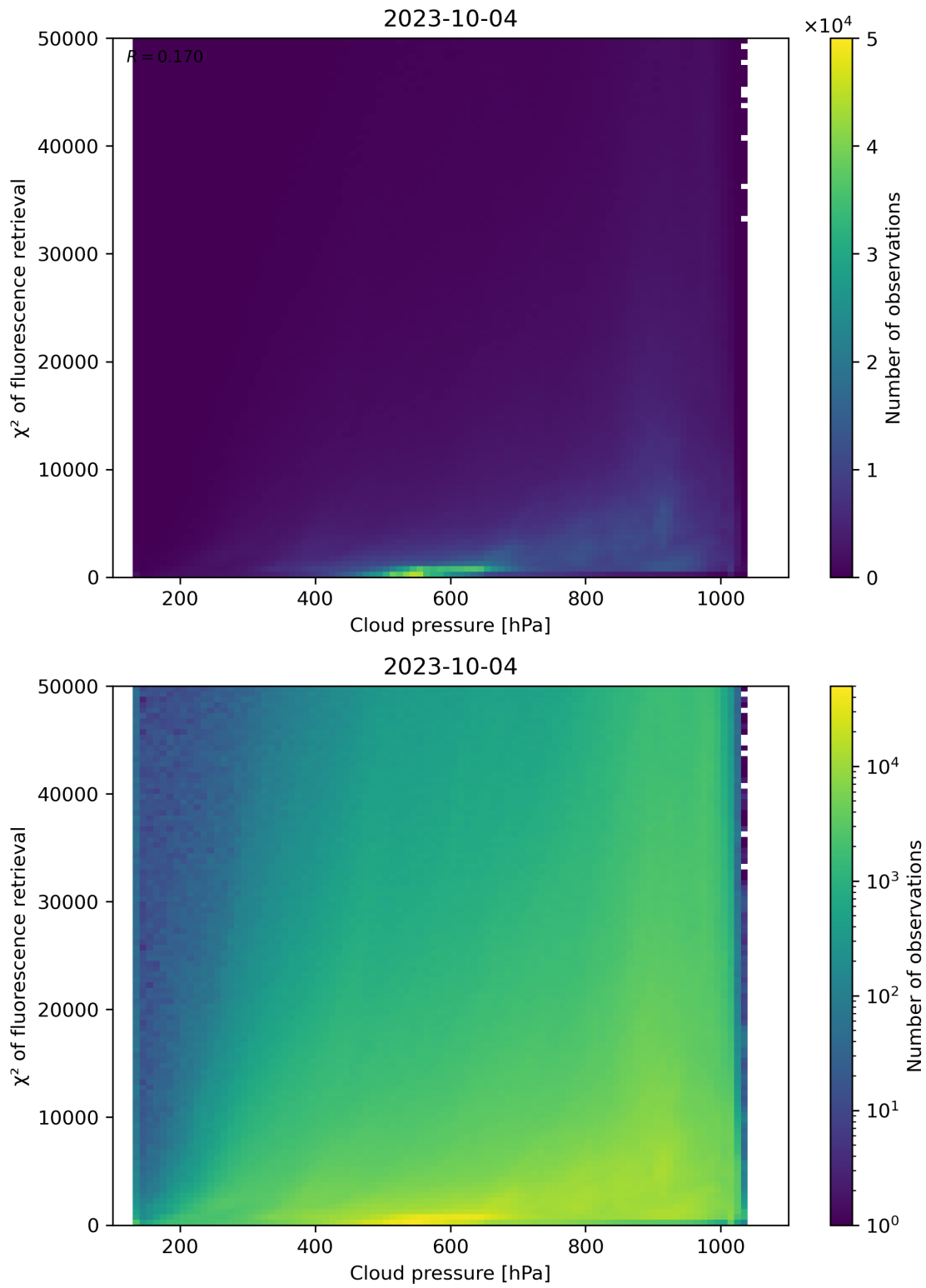
Figure 86: Scatter density plot of “Cloud pressure” against “ \chi^2 of fluorescence retrieval” for 2023-10-03 to 2023-10-05.
