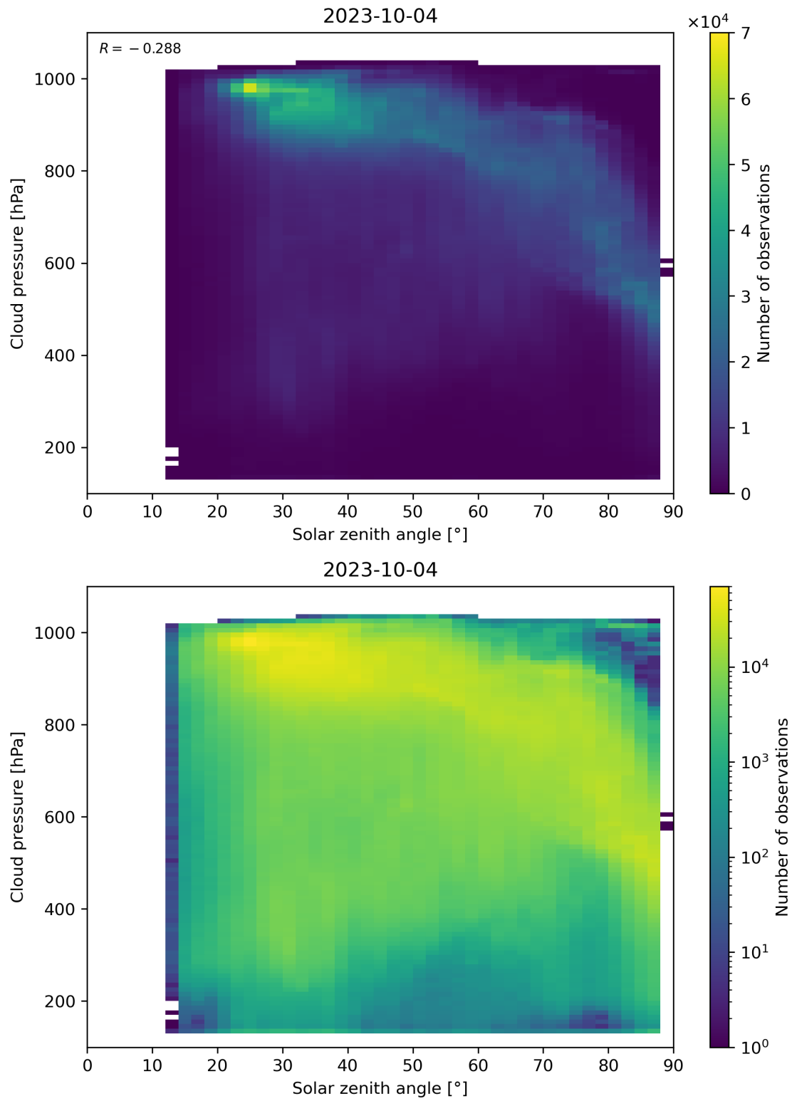
Figure 122: Scatter density plot of “Solar zenith angle” against “Cloud pressure” for 2023-10-03 to 2023-10-05.
