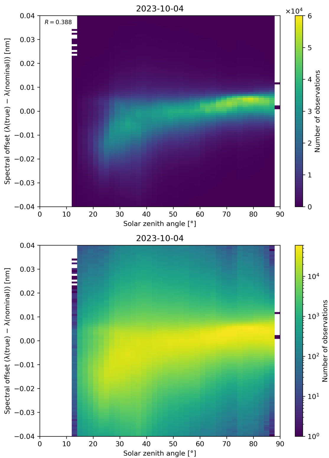
Figure 128: Scatter density plot of “Solar zenith angle” against “Spectral offset ( \lambda(\text{true}) - \lambda(\text{nominal}) )” for 2023-10-03 to 2023-10-05.
