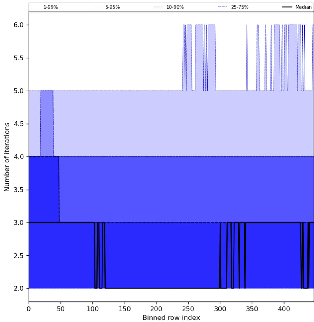
Figure 56: Along track statistics of “Number of iterations” for 2023-10-03 to 2023-10-05
