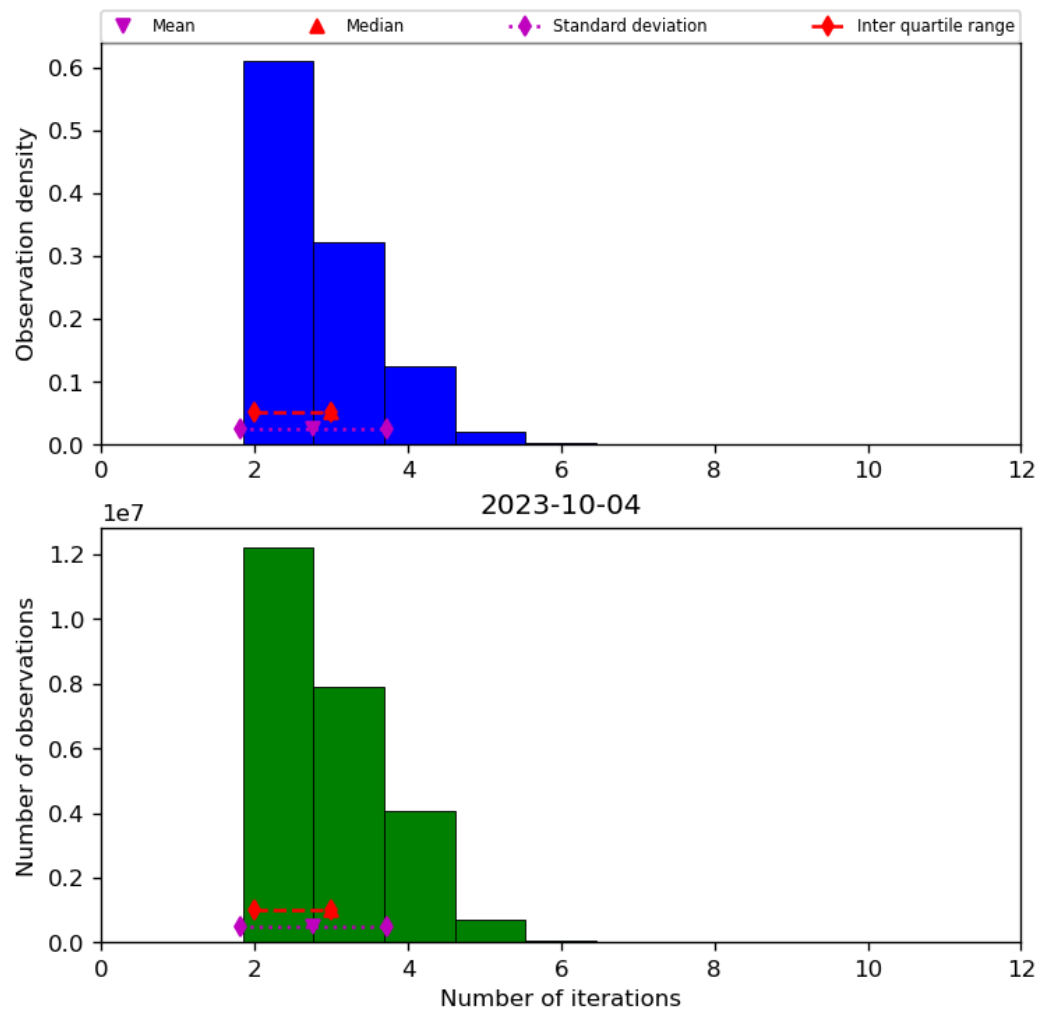
Figure 39: Histogram of “Number of iterations” for 2023-10-03 to 2023-10-05
