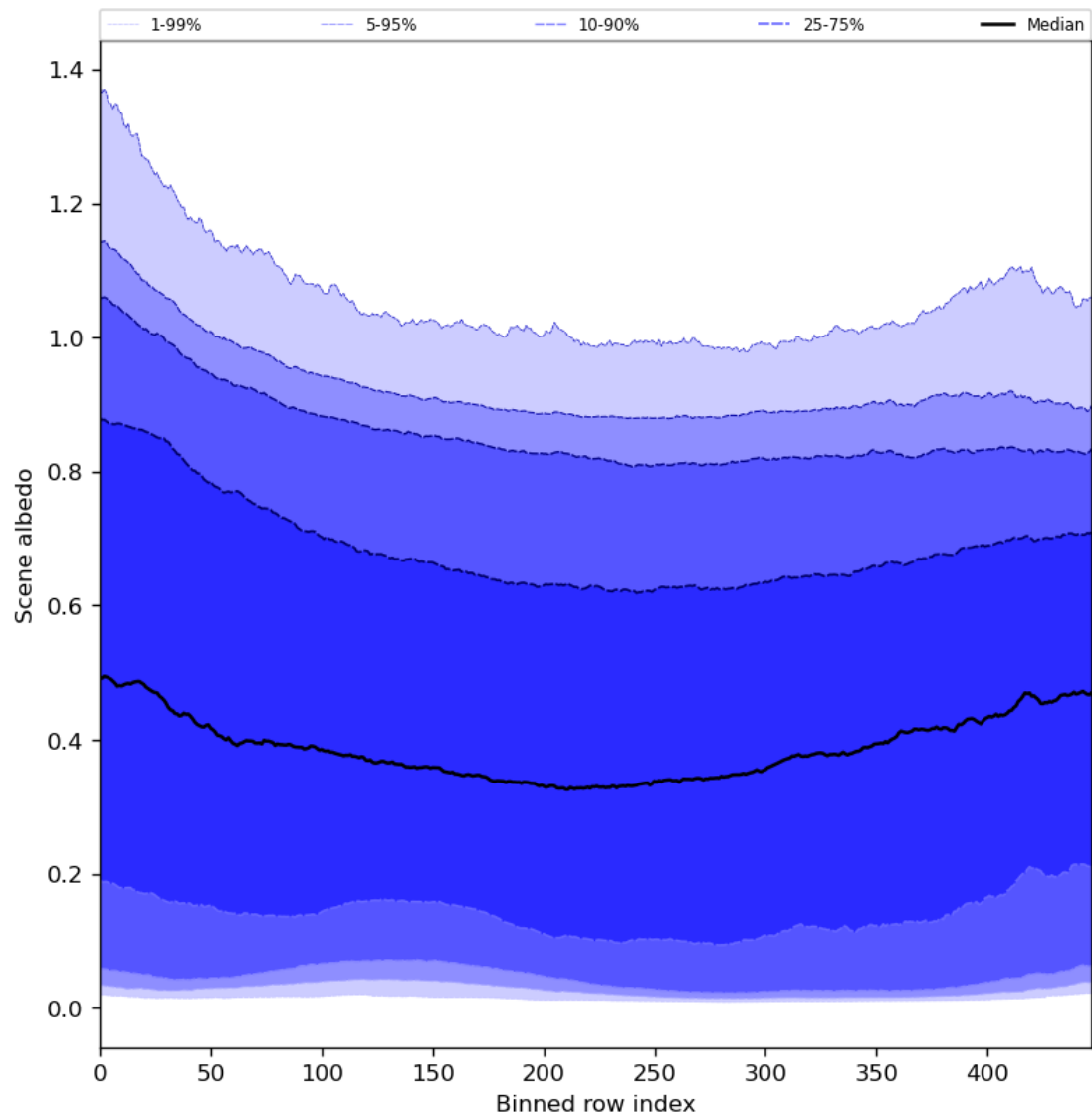
Figure 51: Along track statistics of “Scene albedo” for 2023-10-03 to 2023-10-05
