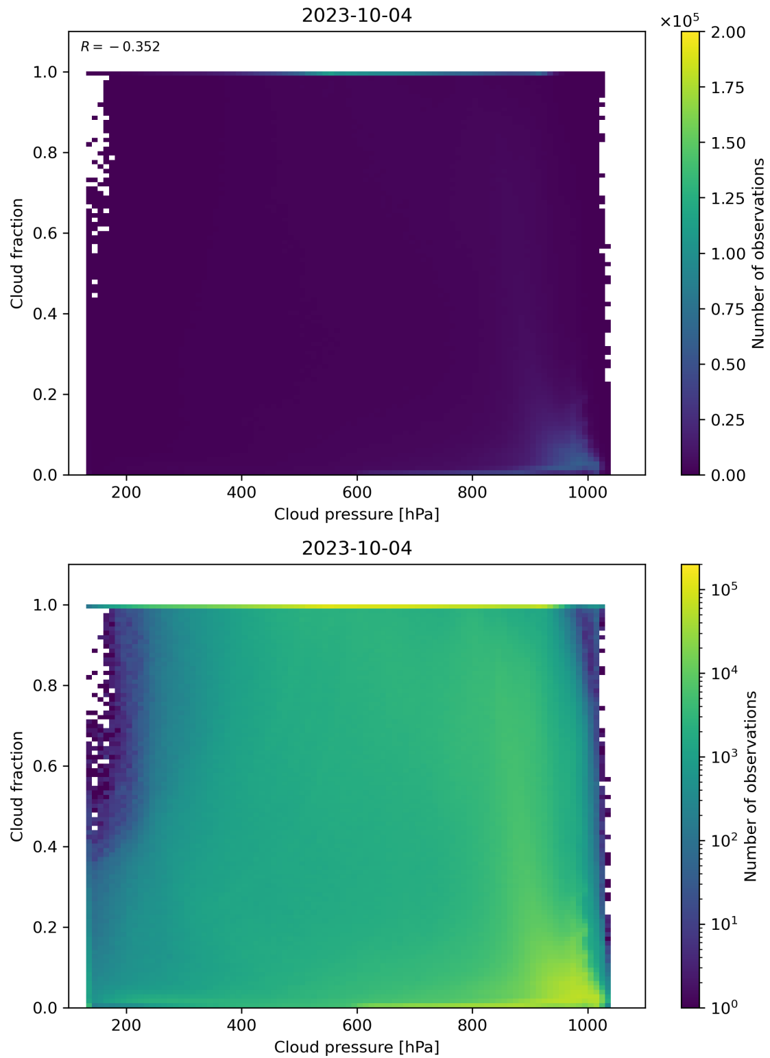
Figure 87: Scatter density plot of “Cloud pressure” against “Cloud fraction” for 2023-10-03 to 2023-10-05.
