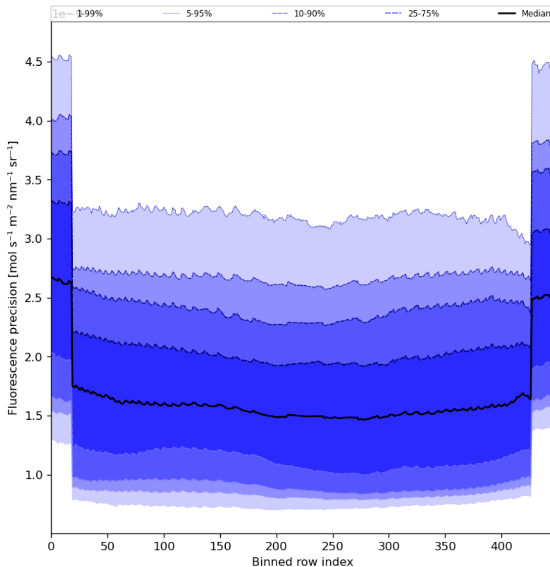
Figure 58: Along track statistics of “Fluorescence precision” for 2023-10-03 to 2023-10-05
