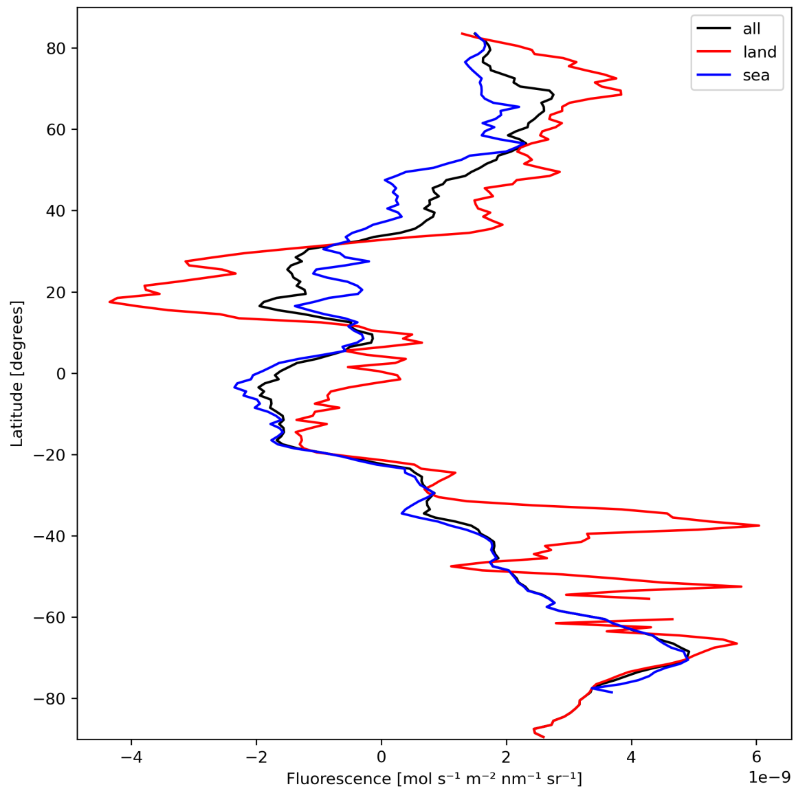
Figure 23: Zonal average of “Fluorescence” for 2023-10-03 to 2023-10-05.
