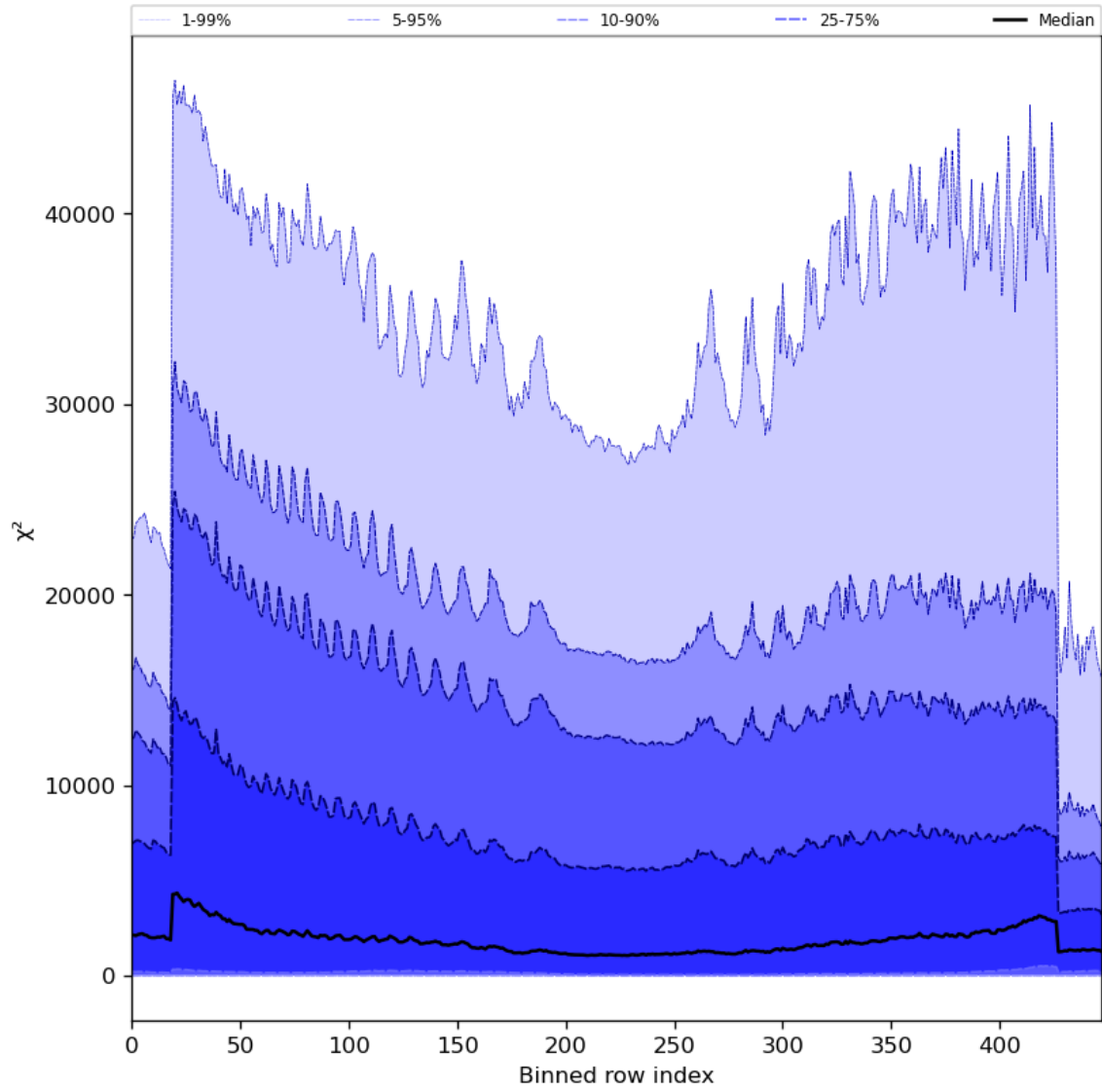
Figure 55: Along track statistics of “ \chi^2 ” for 2023-10-03 to 2023-10-05
