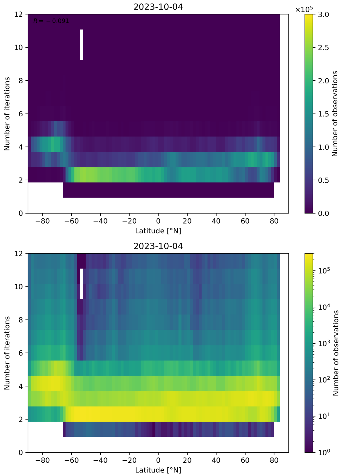
Figure 102: Scatter density plot of “Latitude” against “Number of iterations” for 2023-10-03 to 2023-10-05.
