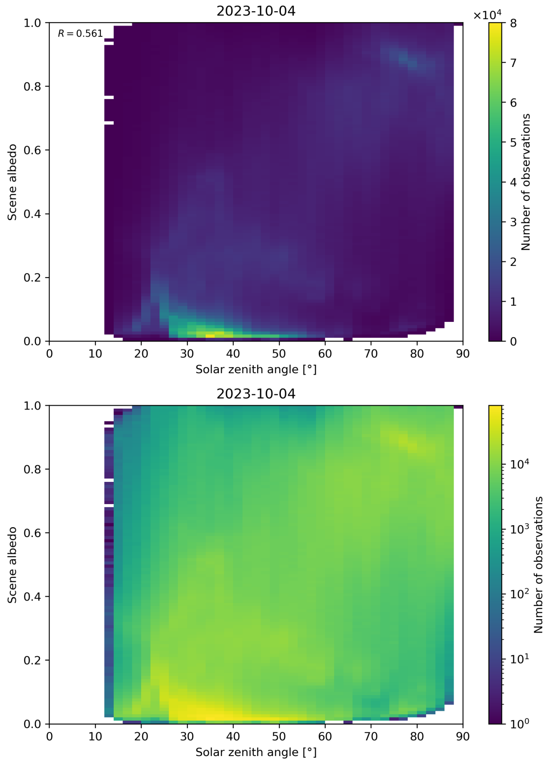
Figure 127: Scatter density plot of “Solar zenith angle” against “Scene albedo” for 2023-10-03 to 2023-10-05.
