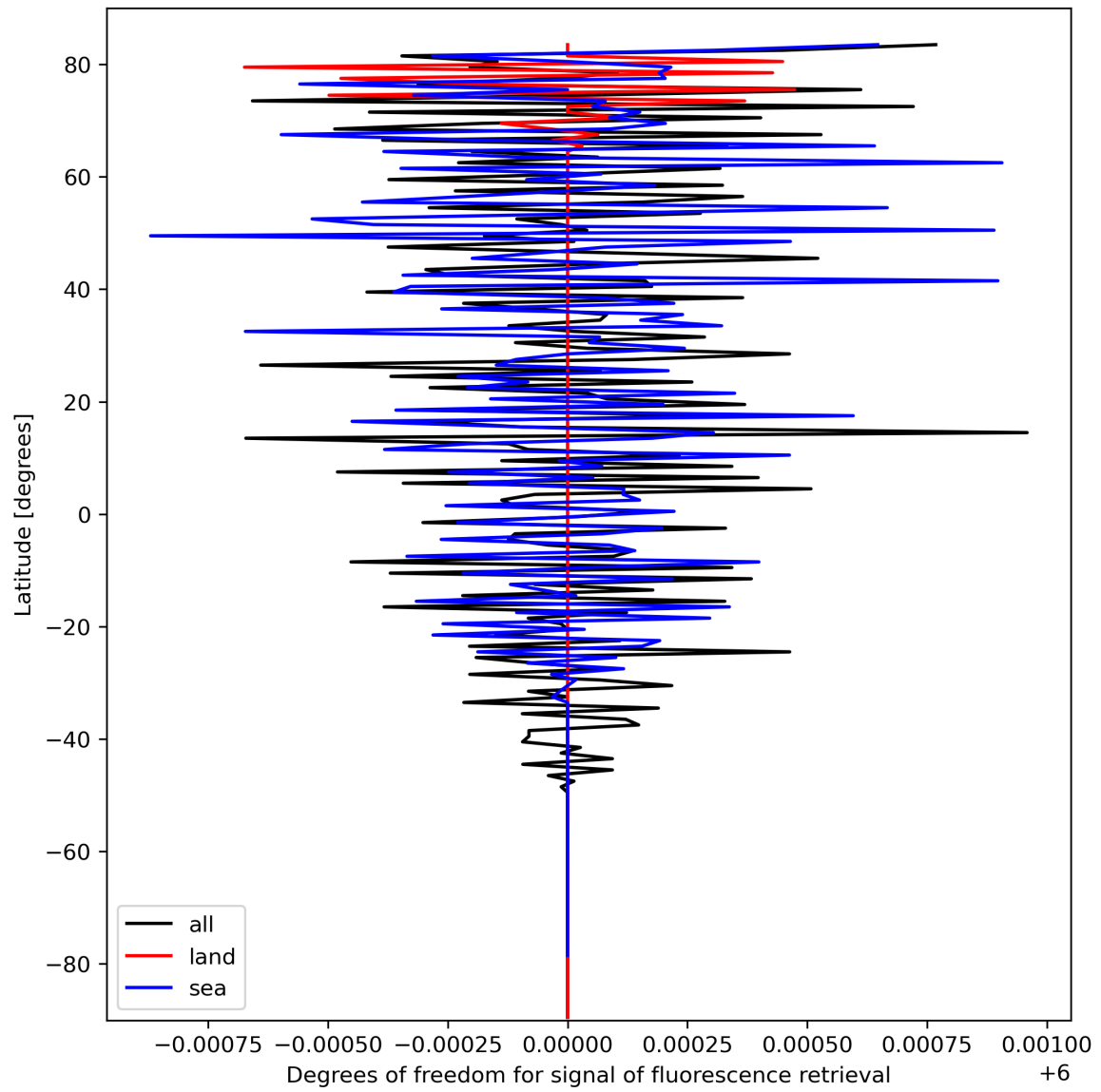
Figure 26: Zonal average of “Degrees of freedom for signal of fluorescence retrieval” for 2023-10-03 to 2023-10-05.
