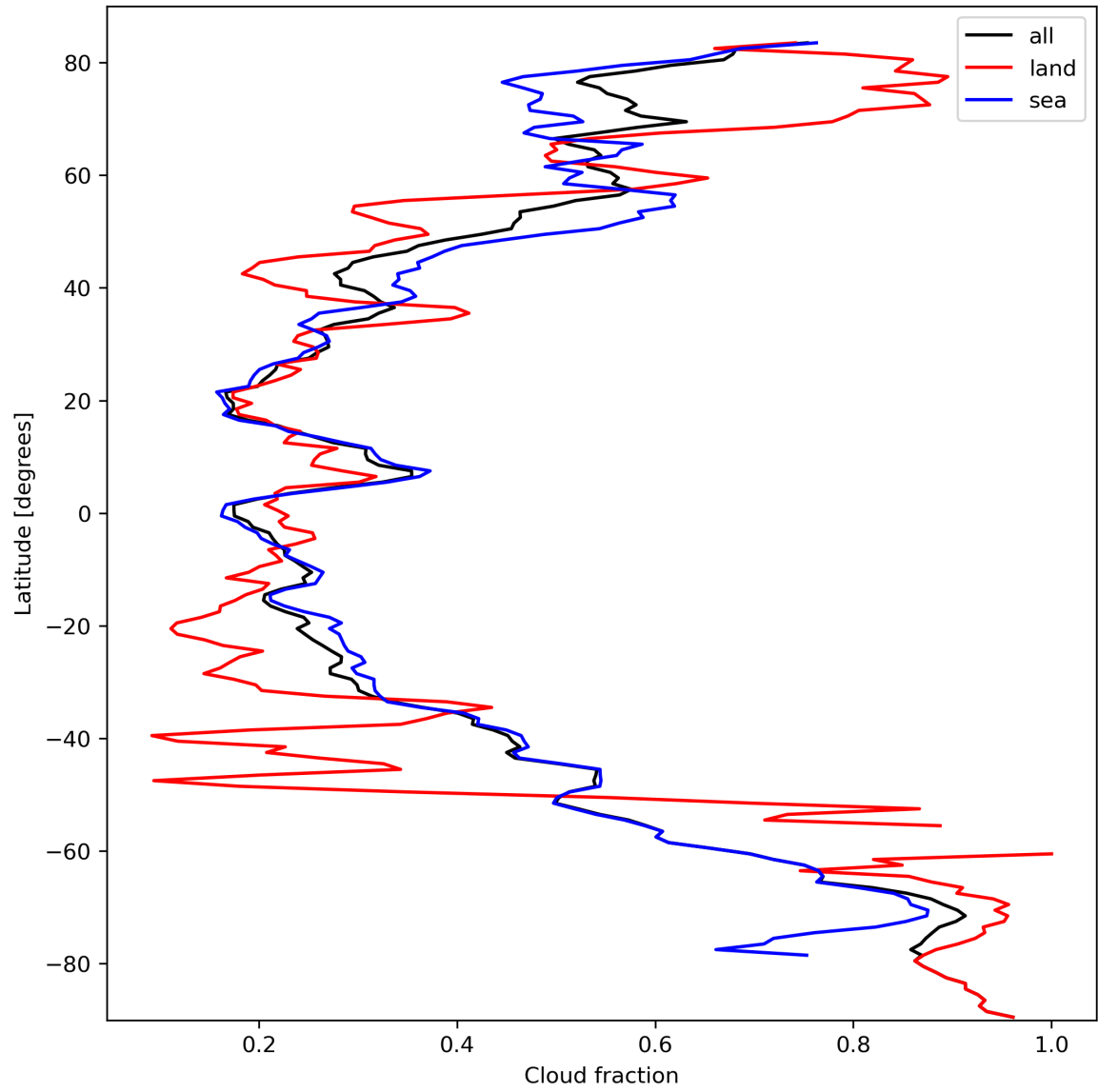
Figure 15: Zonal average of “Cloud fraction” for 2023-10-03 to 2023-10-05.
