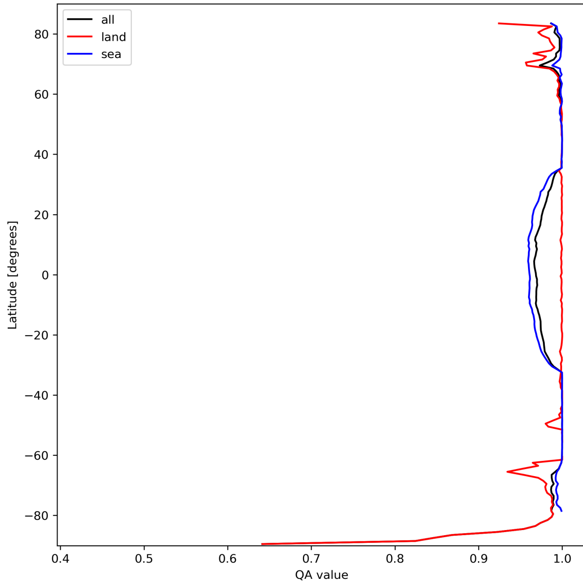
Figure 12: Zonal average of “QA value” for 2023-10-03 to 2023-10-05.
