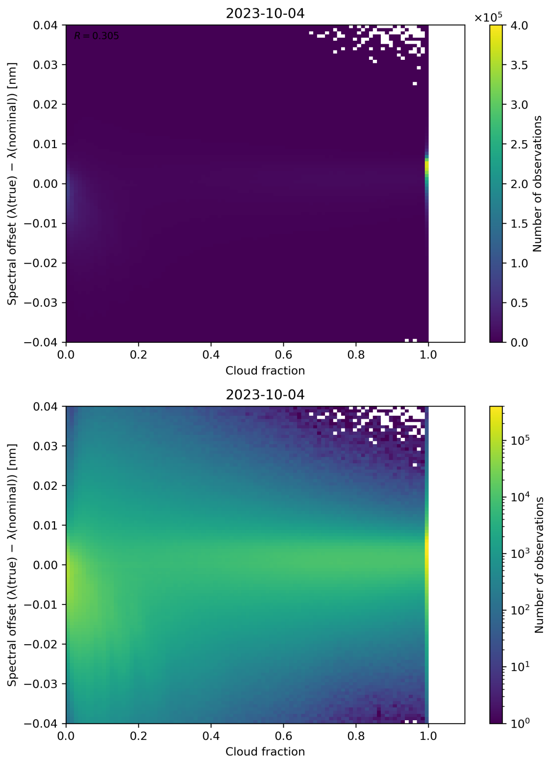
Figure 83: Scatter density plot of “Cloud fraction” against “Spectral offset ( \lambda(\text{true}) - \lambda(\text{nominal}) )” for 2023-10-03 to 2023-10-05.
