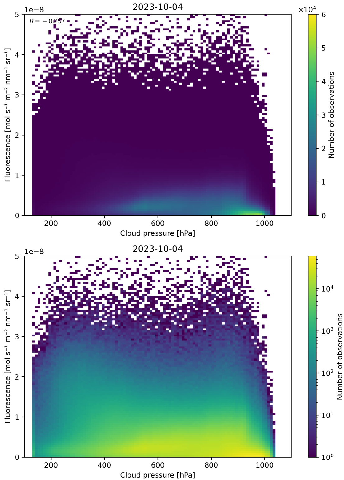
Figure 88: Scatter density plot of “Cloud pressure” against “Fluorescence” for 2023-10-03 to 2023-10-05.
