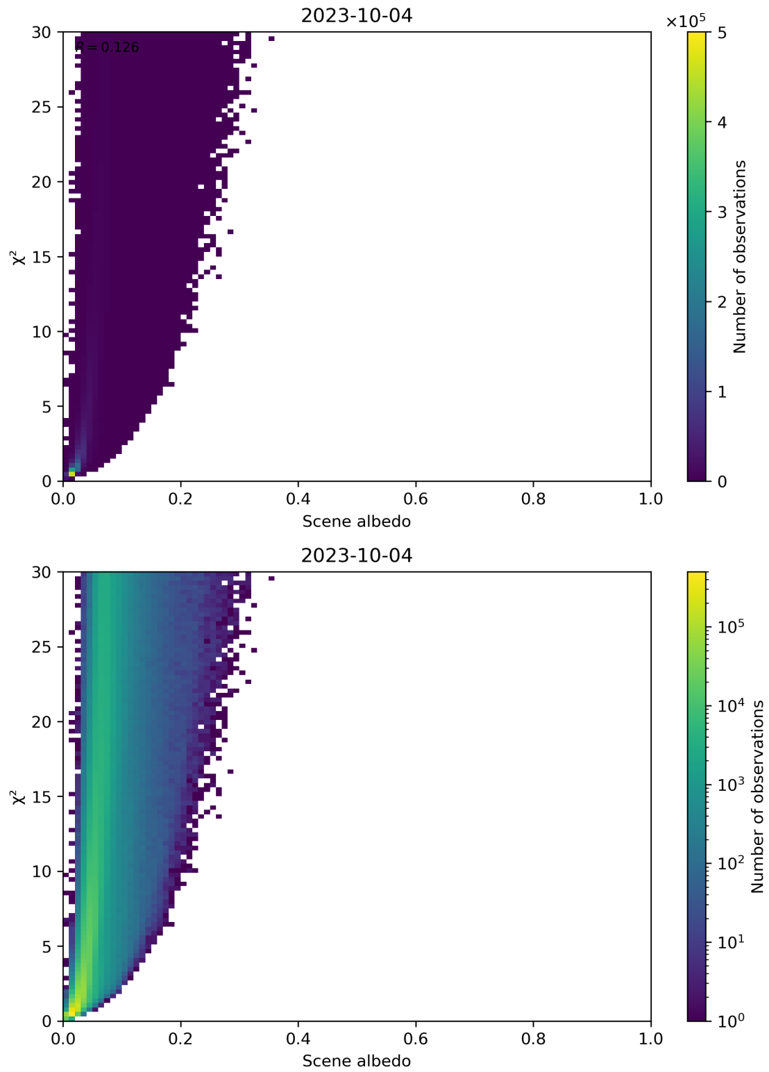
Figure 112: Scatter density plot of “Scene albedo” against “ \chi^2 ” for 2023-10-03 to 2023-10-05.
