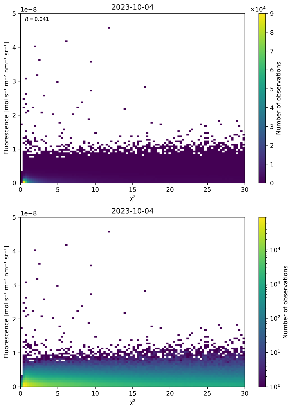
Figure 70: Scatter density plot of “ \chi^2 ” against “Fluorescence” for 2023-10-03 to 2023-10-05.
