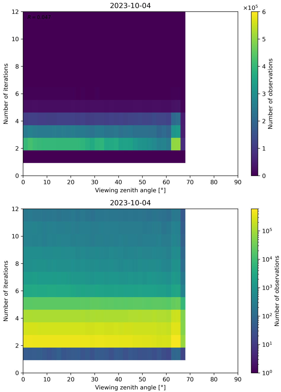
Figure 136: Scatter density plot of “Viewing zenith angle” against “Number of iterations” for 2023-10-03 to 2023-10-05.
