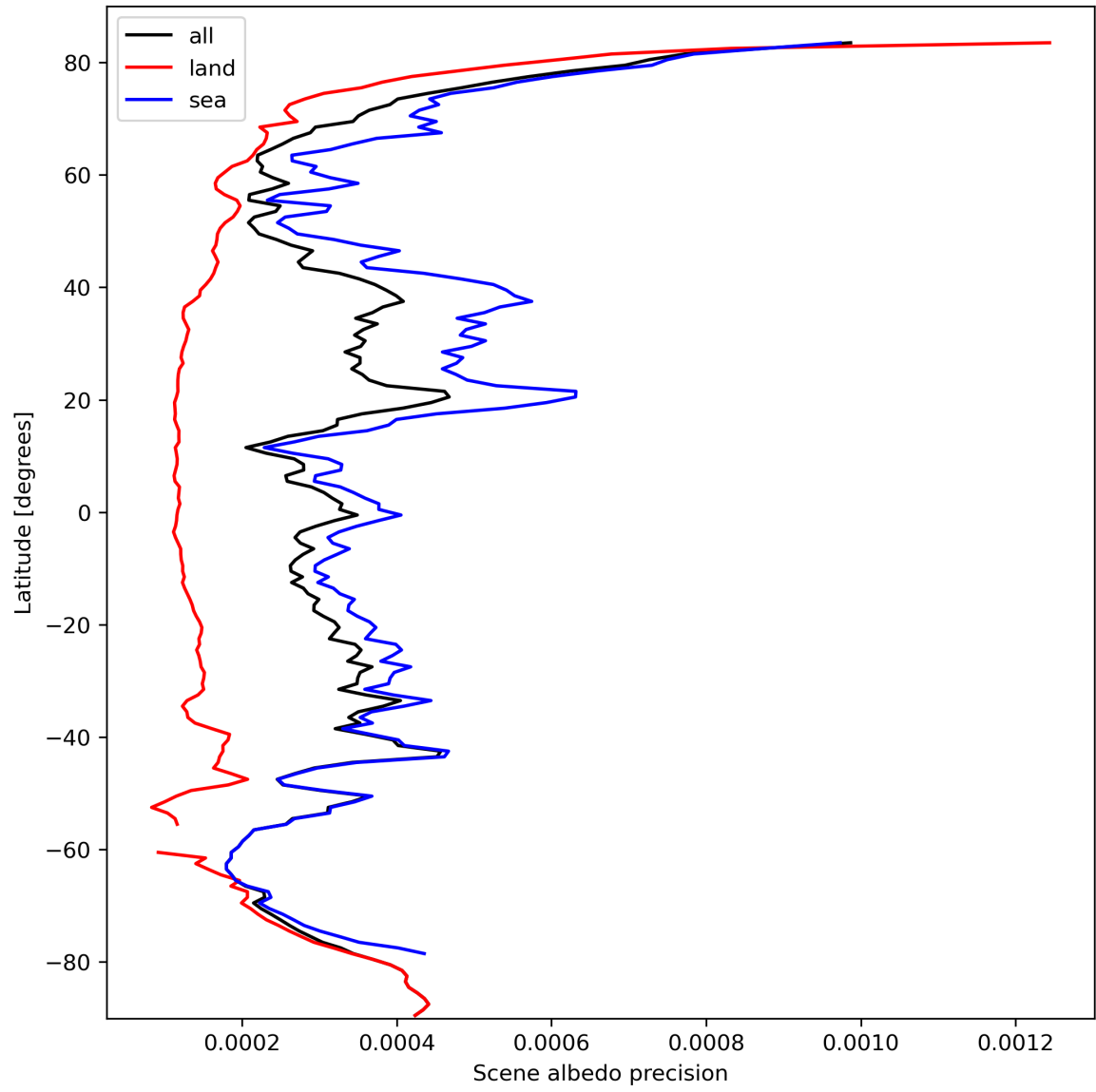
Figure 18: Zonal average of “Scene albedo precision” for 2023-10-03 to 2023-10-05.
