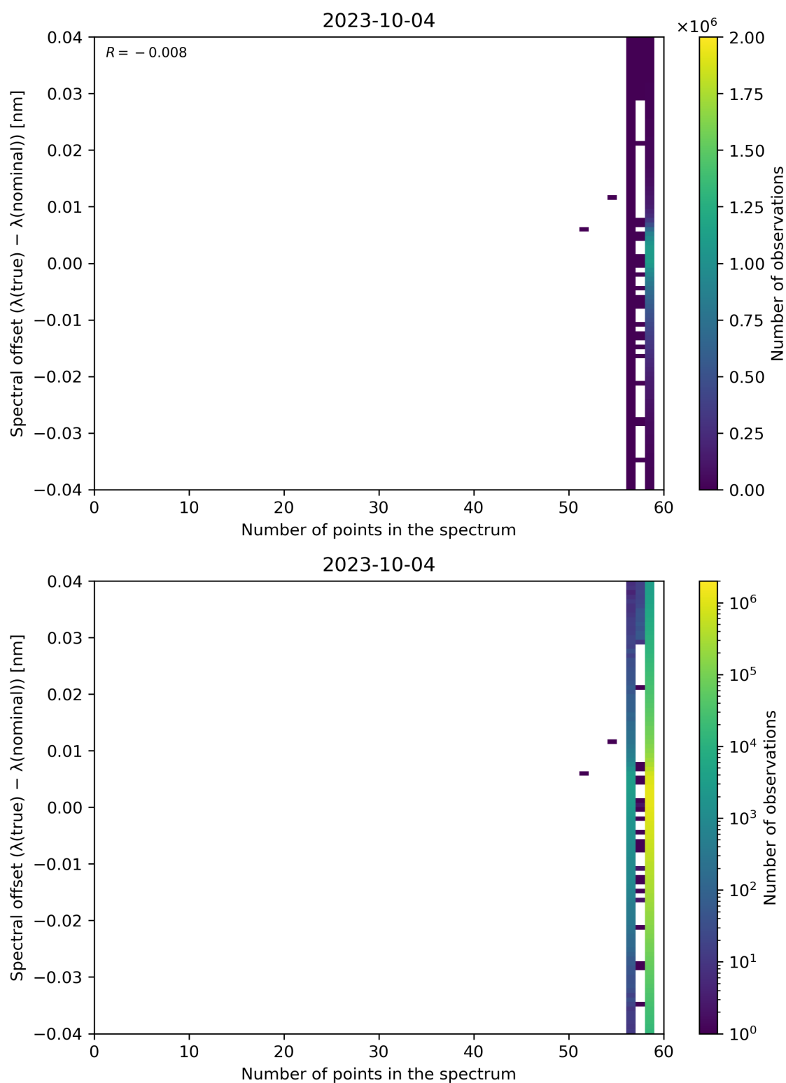
Figure 110: Scatter density plot of “Number of points in the spectrum” against “Spectral offset ( \lambda(\text{true}) - \lambda(\text{nominal}) )” for 2023-10-03 to 2023-10-05.
