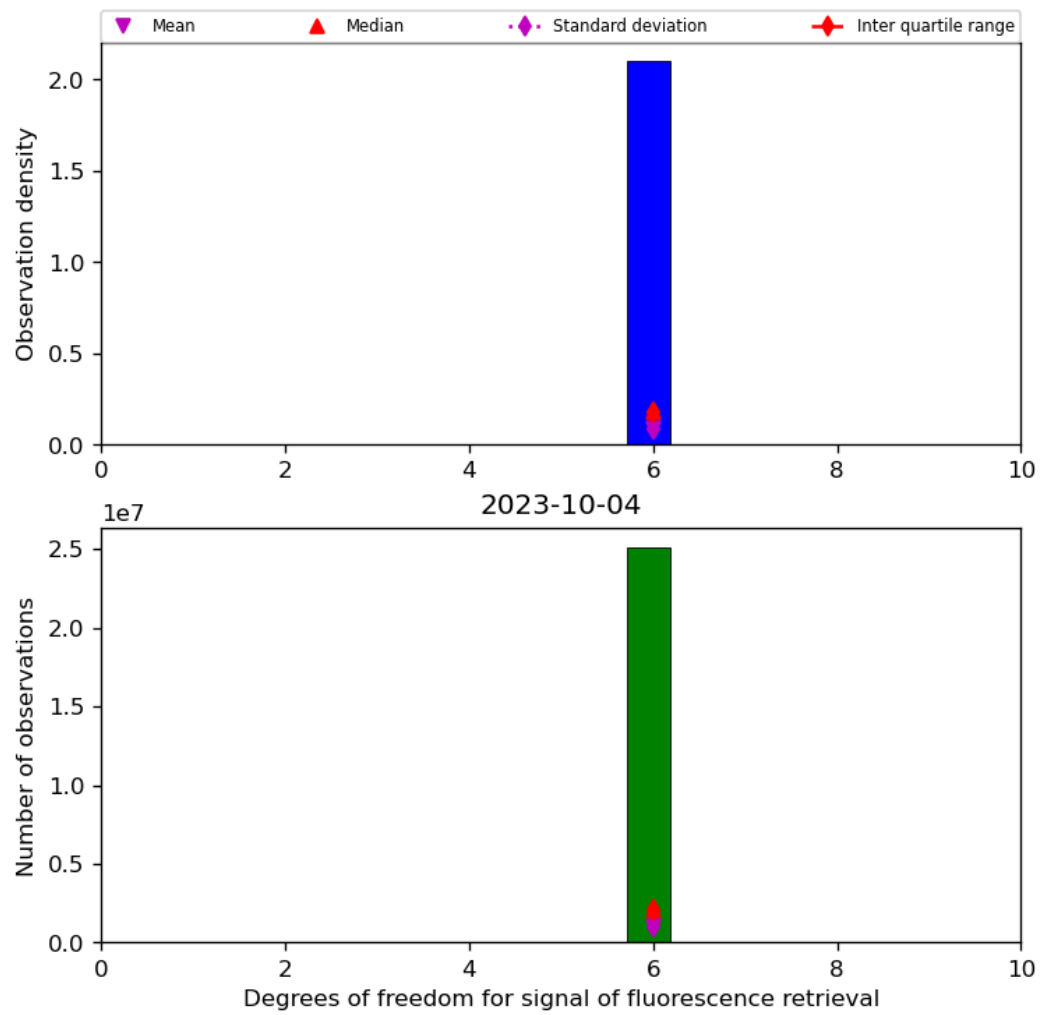
Figure 43: Histogram of “Degrees of freedom for signal of fluorescence retrieval” for 2023-10-03 to 2023-10-05
