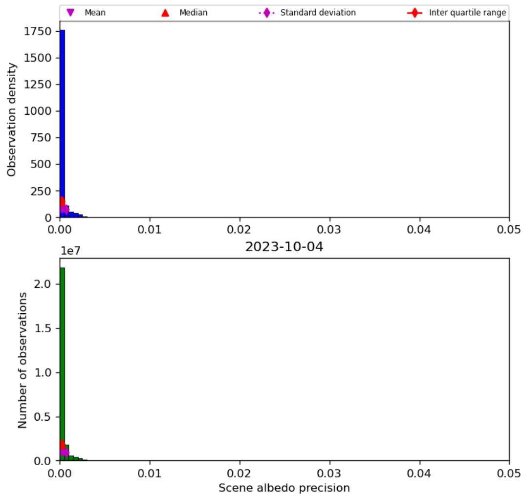
Figure 35: Histogram of “Scene albedo precision” for 2023-10-03 to 2023-10-05
