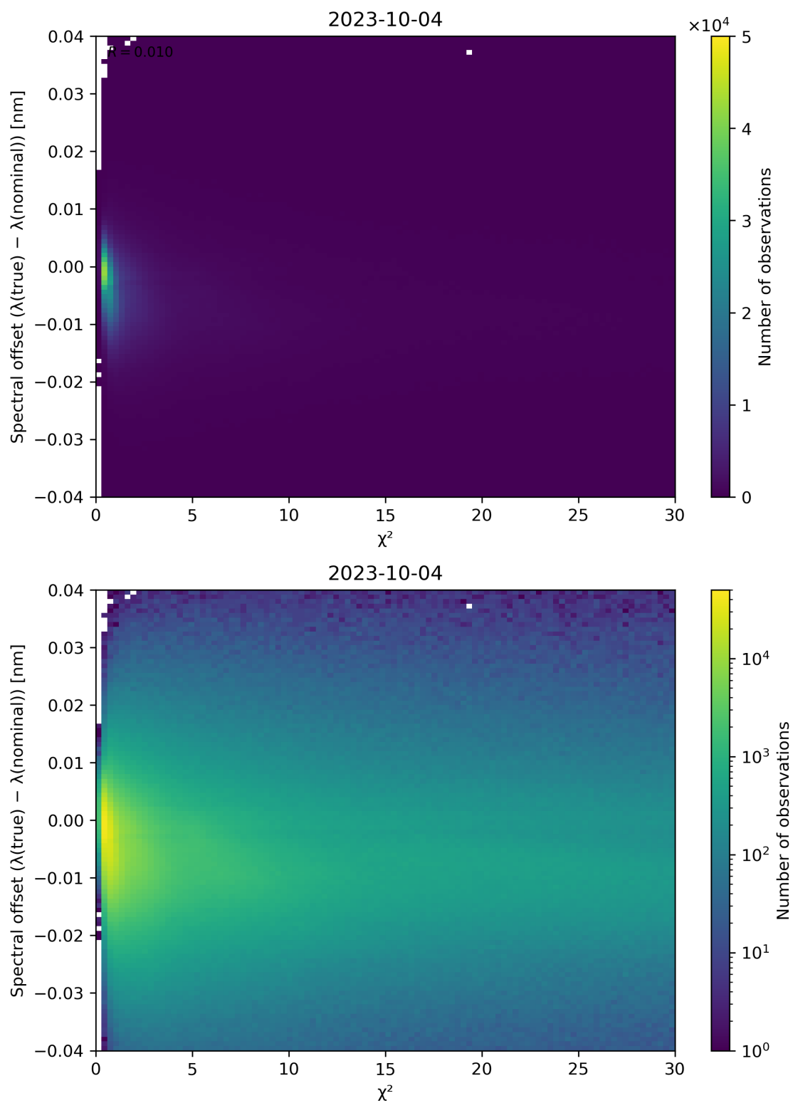
Figure 75: Scatter density plot of “ \chi^2 ” against “Spectral offset ( \lambda(\text{true}) - \lambda(\text{nominal}) )” for 2023-10-03 to 2023-10-05.
