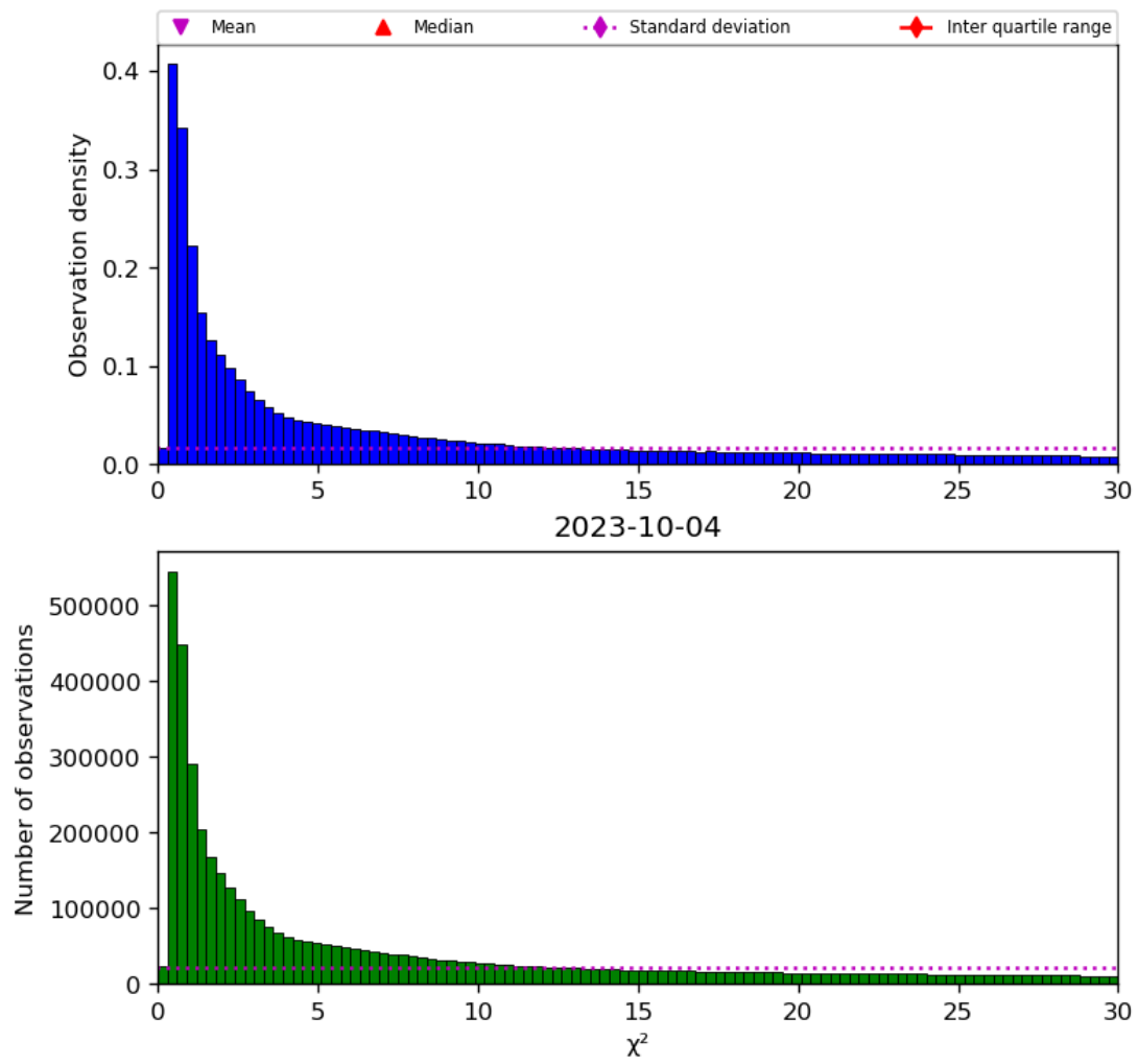
Figure 38: Histogram of “ \chi^2 ” for 2023-10-03 to 2023-10-05
