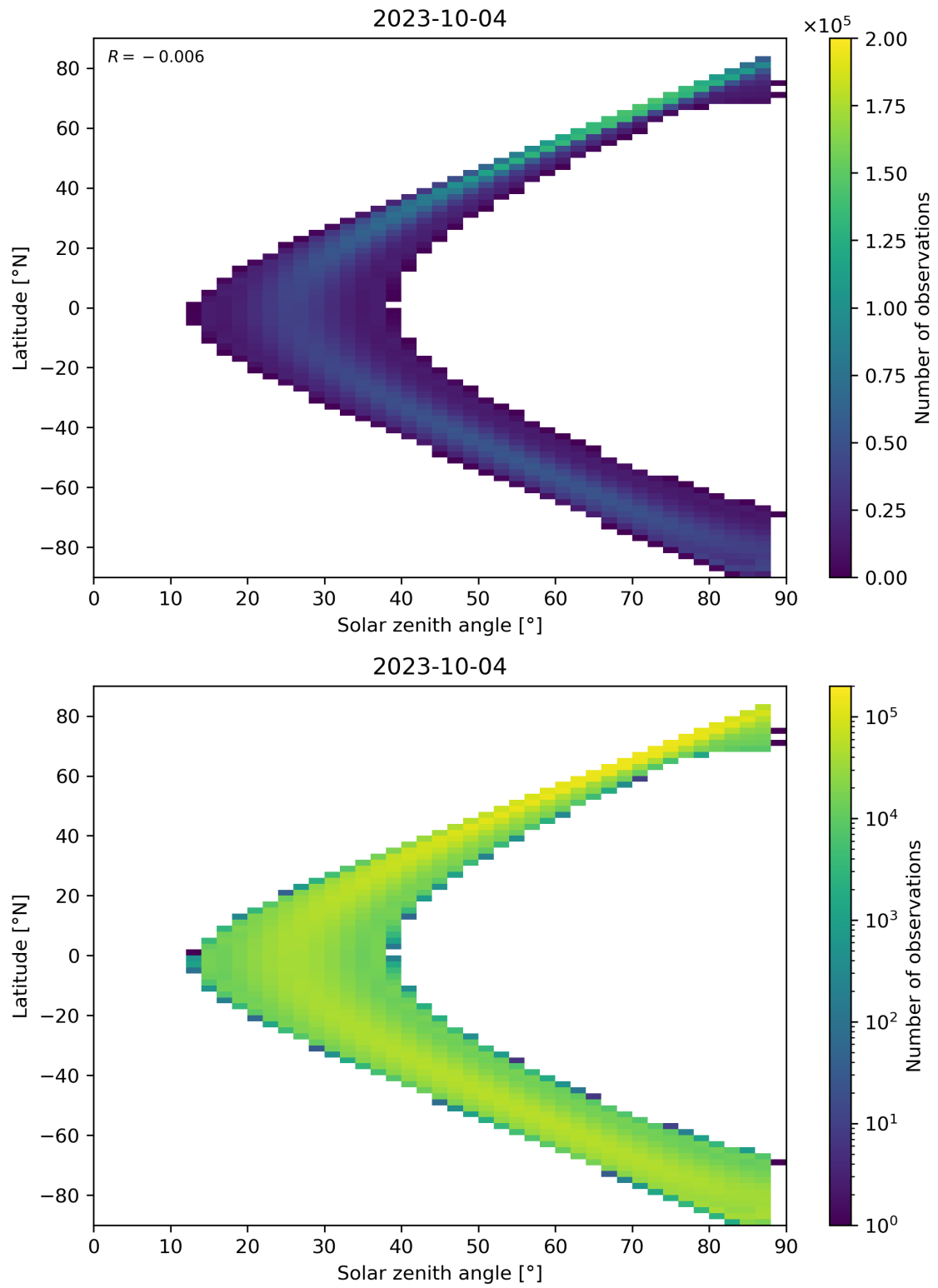
Figure 124: Scatter density plot of “Solar zenith angle” against “Latitude” for 2023-10-03 to 2023-10-05.
