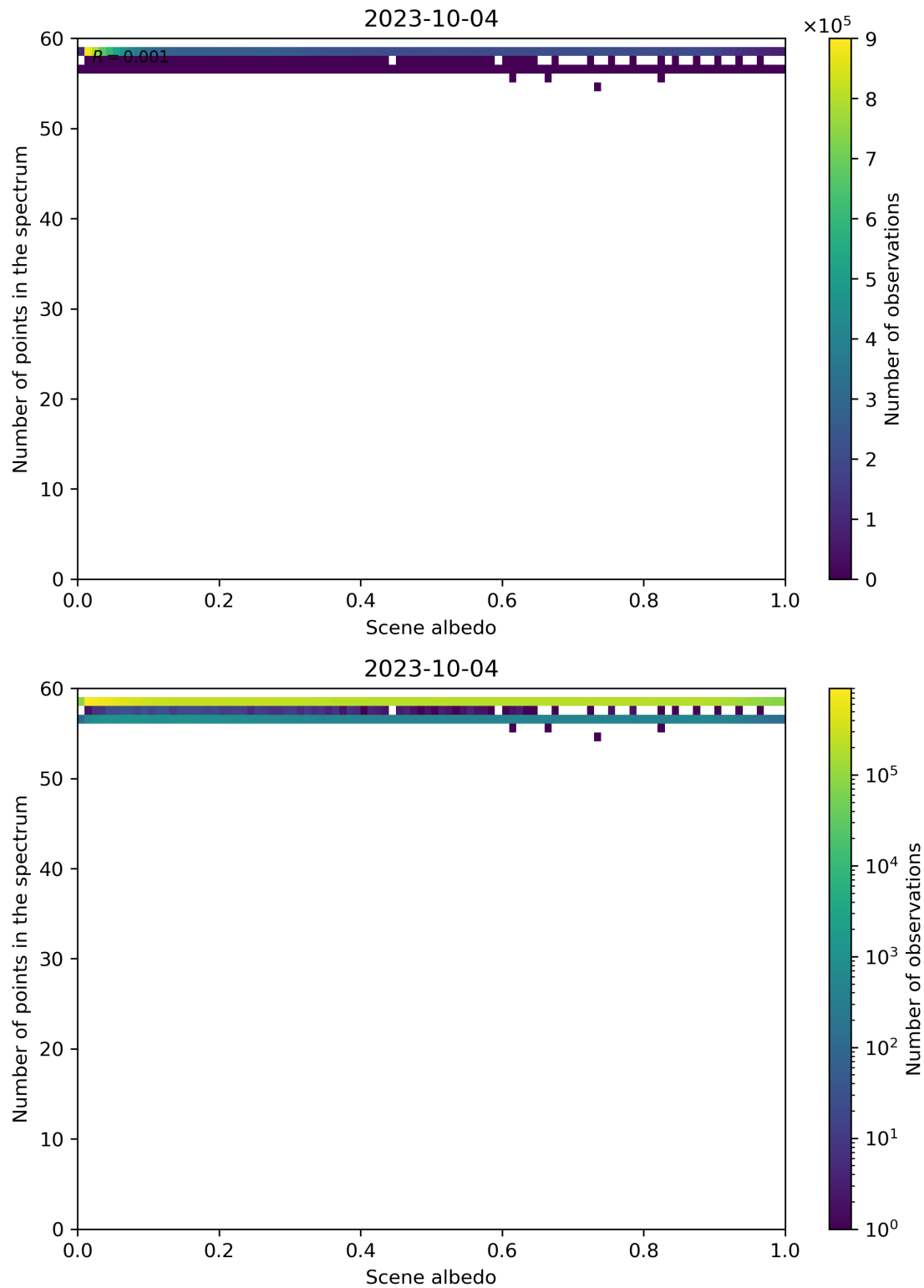
Figure 116: Scatter density plot of “Scene albedo” against “Number of points in the spectrum” for 2023-10-03 to 2023-10-05.
