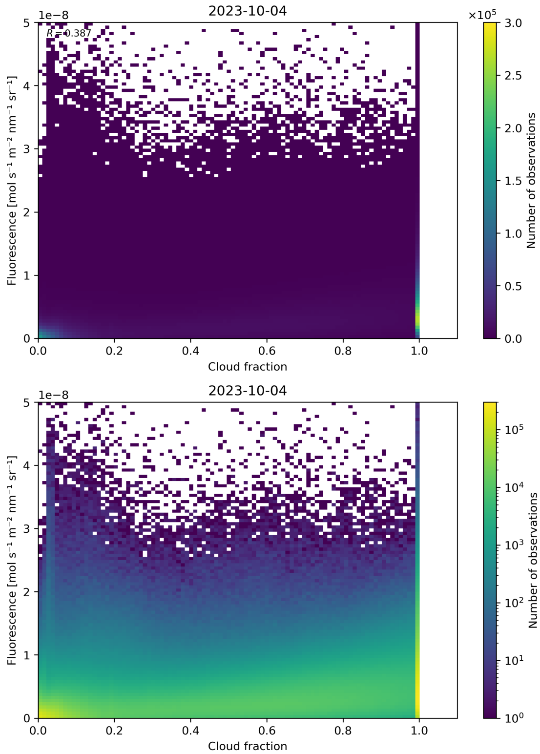
Figure 79: Scatter density plot of “Cloud fraction” against “Fluorescence” for 2023-10-03 to 2023-10-05.
