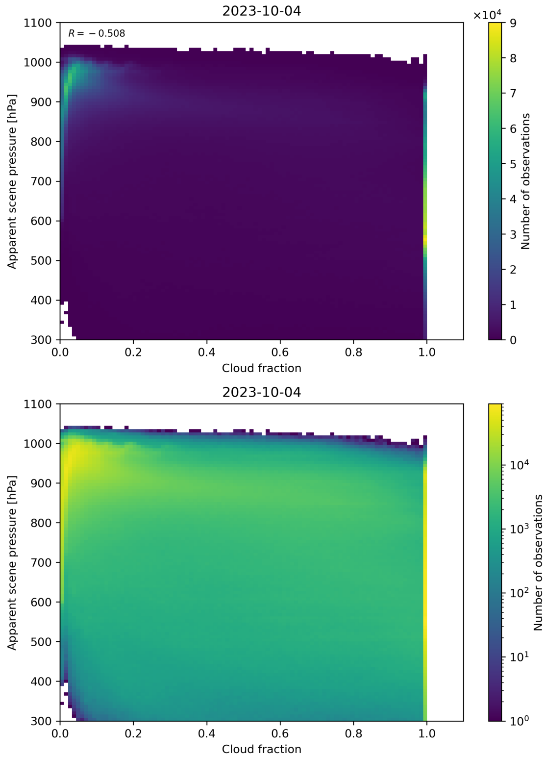
Figure 76: Scatter density plot of “Cloud fraction” against “Apparent scene pressure” for 2023-10-03 to 2023-10-05.
