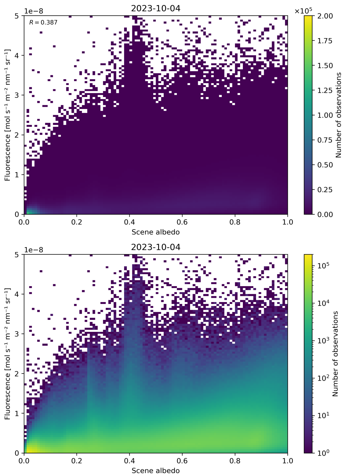
Figure 114: Scatter density plot of “Scene albedo” against “Fluorescence” for 2023-10-03 to 2023-10-05.
