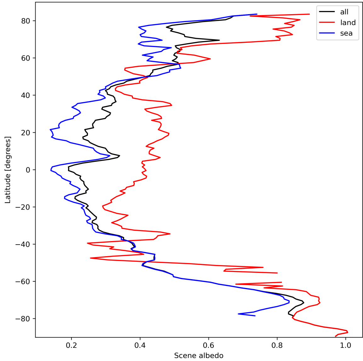
Figure 17: Zonal average of “Scene albedo” for 2023-10-03 to 2023-10-05.
