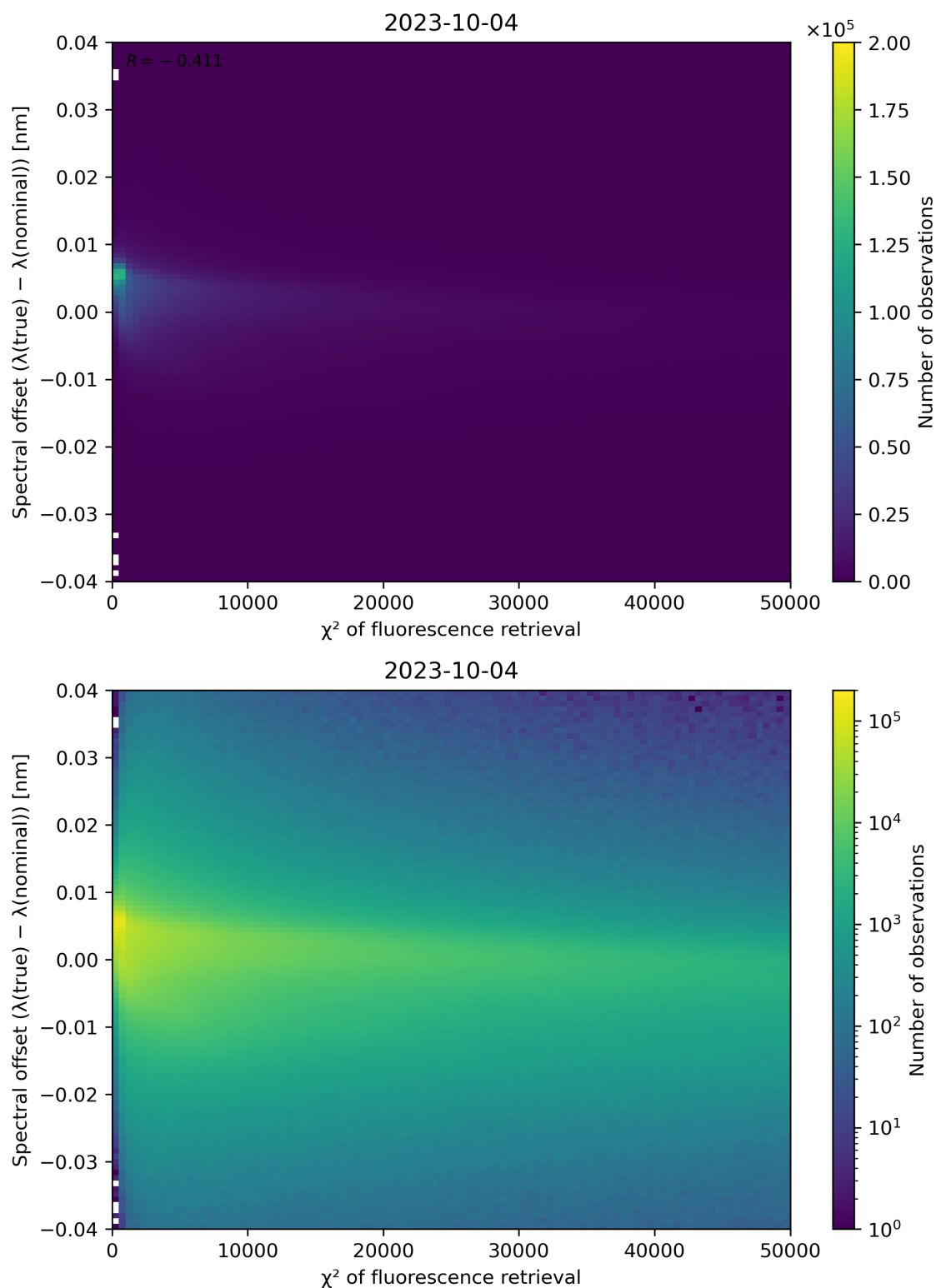
Figure 72: Scatter density plot of " \chi^2 of fluorescence retrieval" against "Spectral offset ( \lambda(\text{true}) - \lambda(\text{nominal})) " for 2023-10-03 to 2023-10-05.
