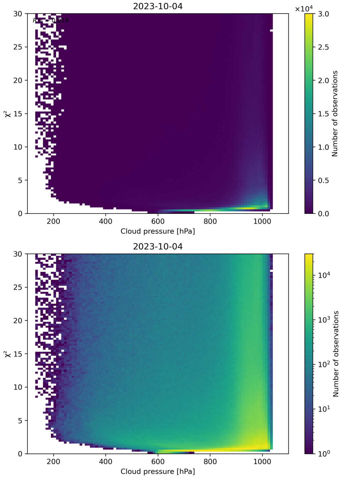
Figure 85: Scatter density plot of “Cloud pressure” against “ \chi^2 ” for 2023-10-03 to 2023-10-05.
