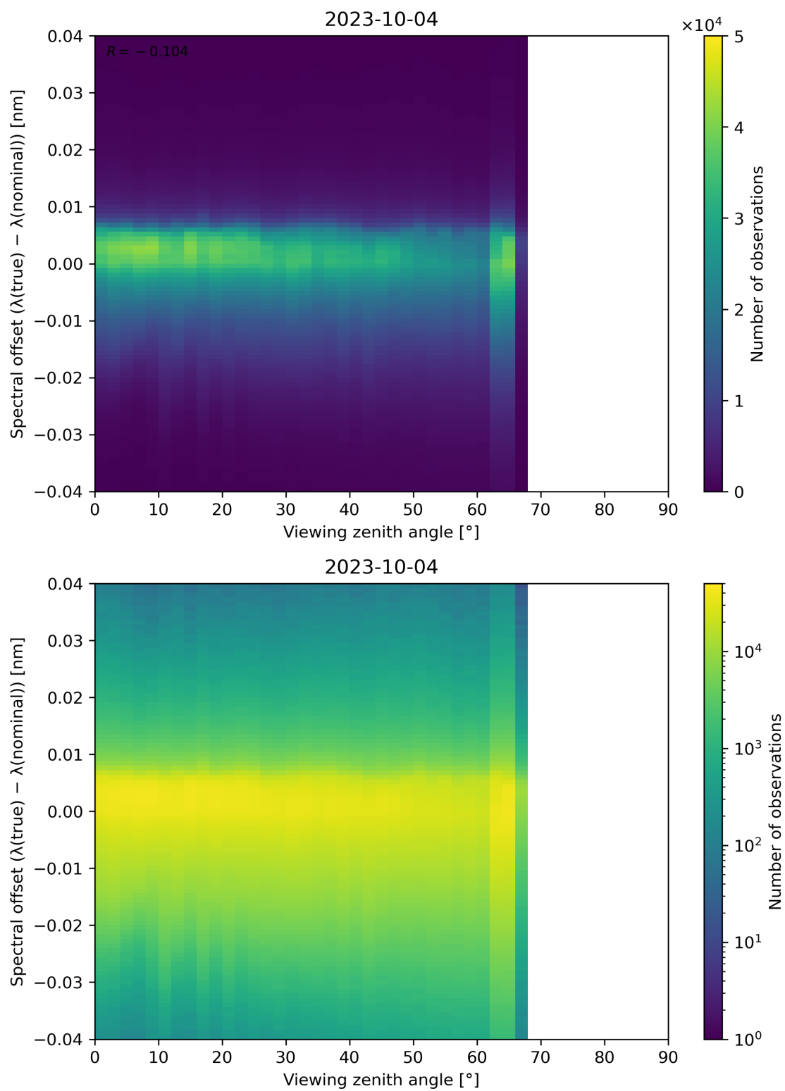
Figure 140: Scatter density plot of “Viewing zenith angle” against “Spectral offset ( \lambda(\text{true}) - \lambda(\text{nominal}) )” for 2023-10-03 to 2023-10-05.
