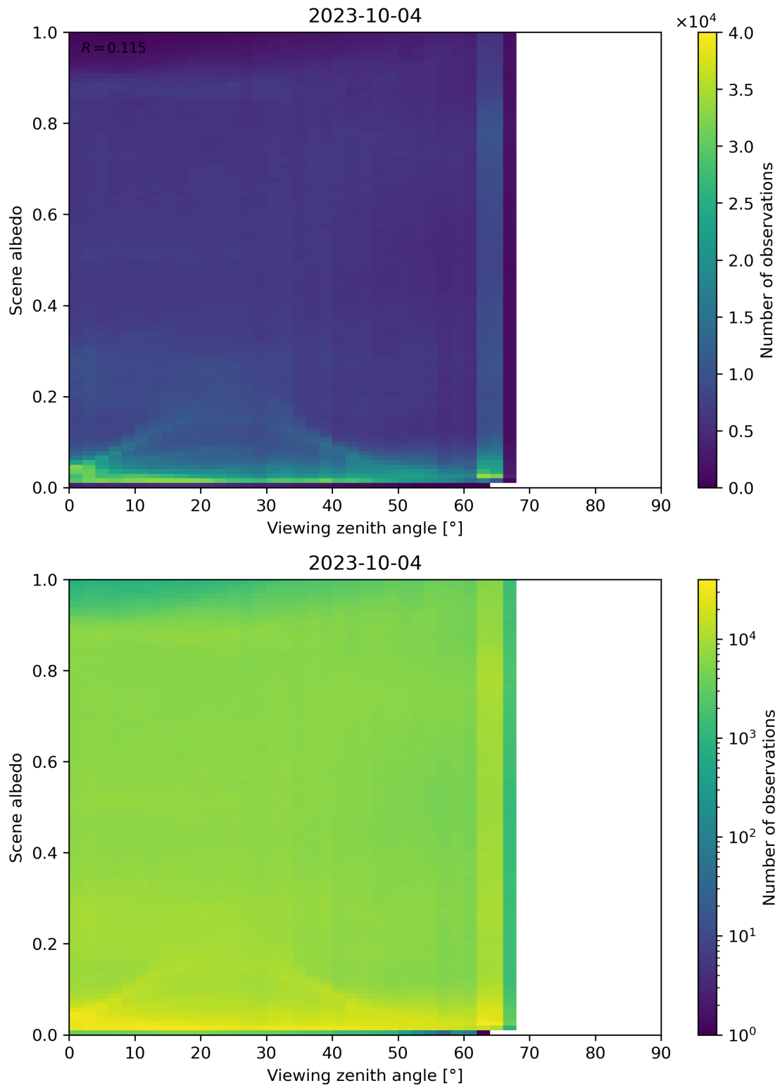
Figure 138: Scatter density plot of “Viewing zenith angle” against “Scene albedo” for 2023-10-03 to 2023-10-05.
