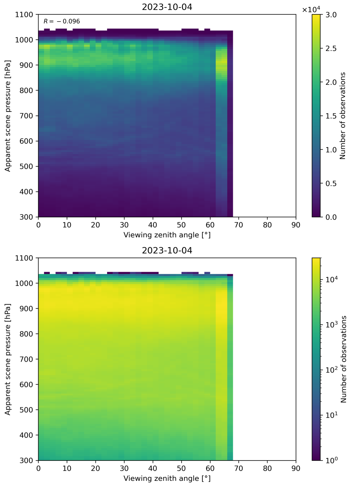
Figure 129: Scatter density plot of “Viewing zenith angle” against “Apparent scene pressure” for 2023-10-03 to 2023-10-05.
