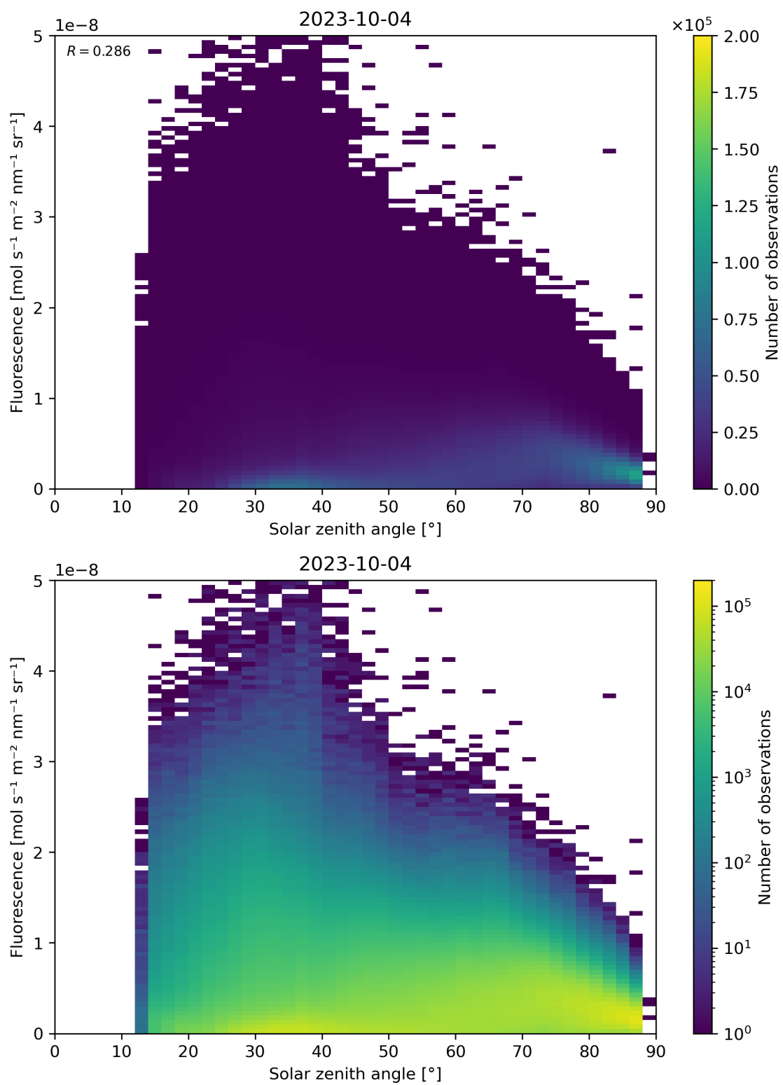
Figure 123: Scatter density plot of “Solar zenith angle” against “Fluorescence” for 2023-10-03 to 2023-10-05.
