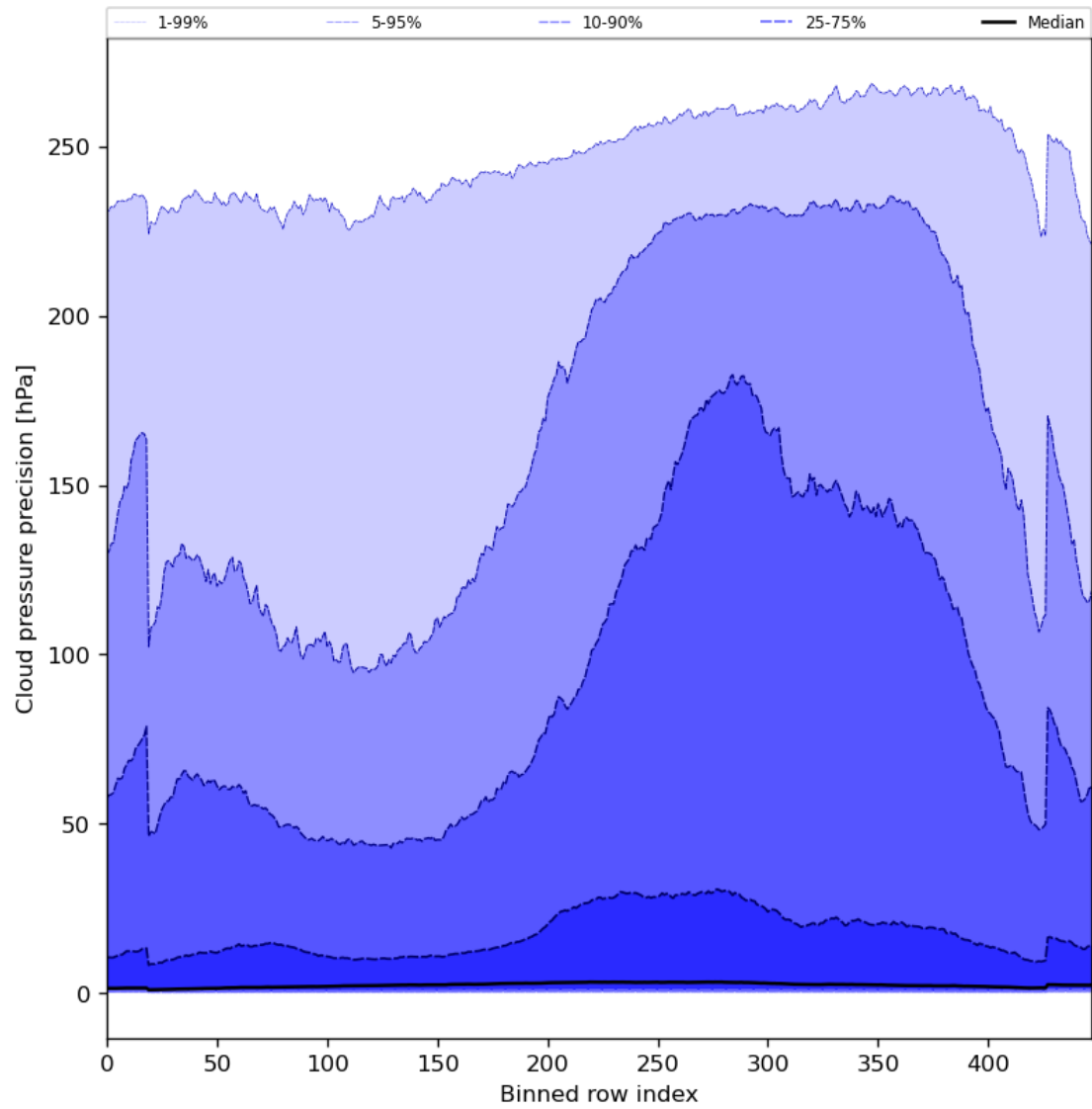
Figure 48: Along track statistics of “Cloud pressure precision” for 2023-10-03 to 2023-10-05
