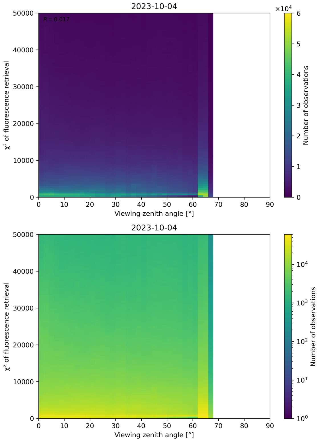
Figure 131: Scatter density plot of “Viewing zenith angle” against “ \chi^2 of fluorescence retrieval” for 2023-10-03 to 2023-10-05.
