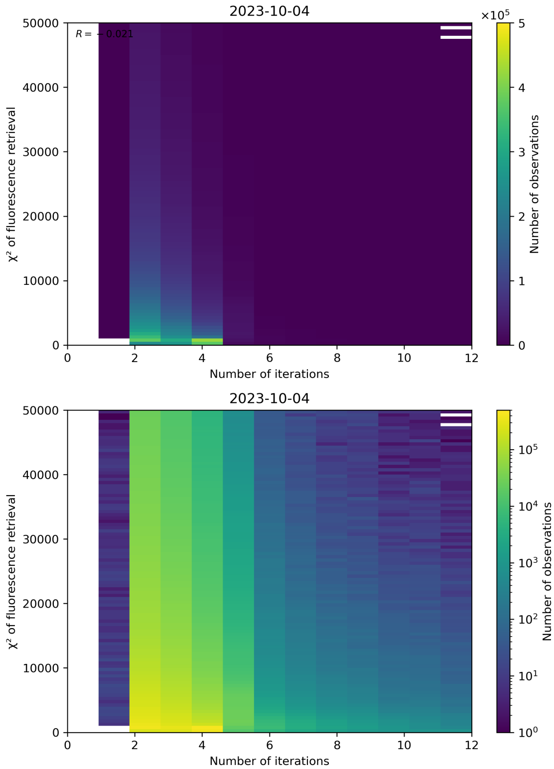
Figure 106: Scatter density plot of “Number of iterations” against “ \chi^2 of fluorescence retrieval” for 2023-10-03 to 2023-10-05.
