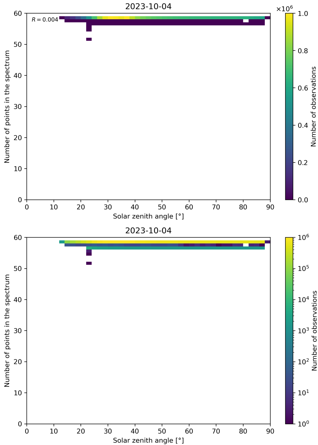
Figure 126: Scatter density plot of “Solar zenith angle” against “Number of points in the spectrum” for 2023-10-03 to 2023-10-05.
