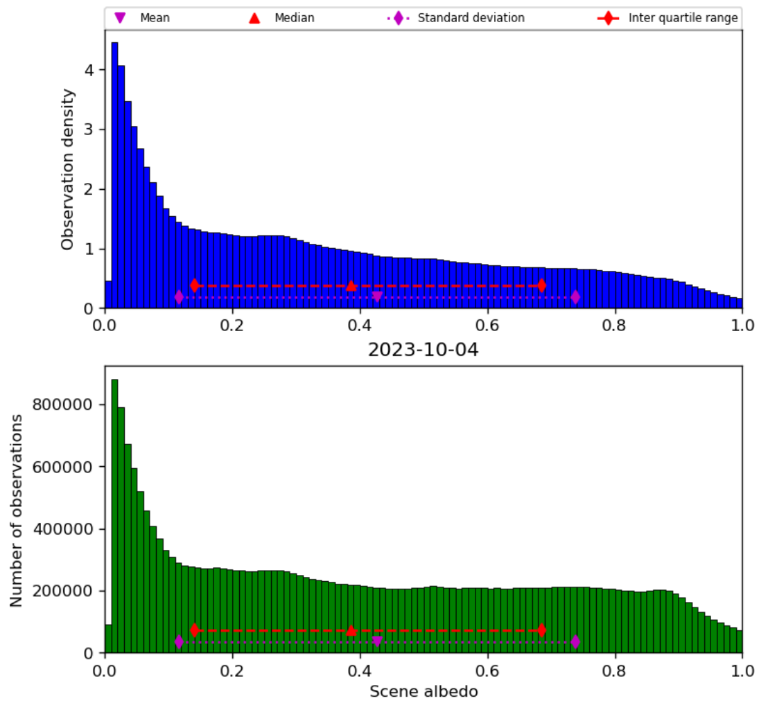
Figure 34: Histogram of “Scene albedo” for 2023-10-03 to 2023-10-05
