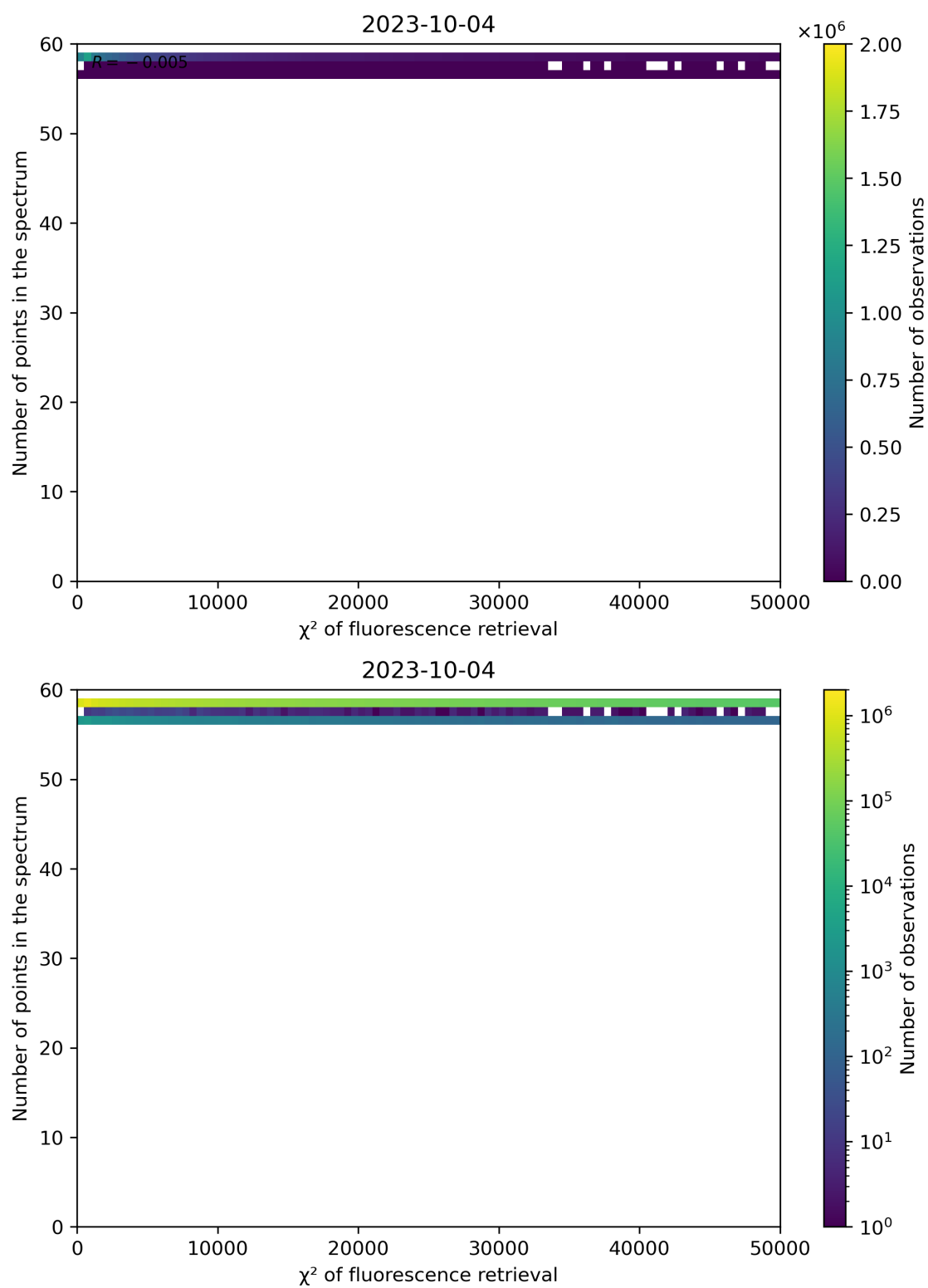
Figure 71: Scatter density plot of " \chi^2 of fluorescence retrieval" against "Number of points in the spectrum" for 2023-10-03 to 2023-10-05.
