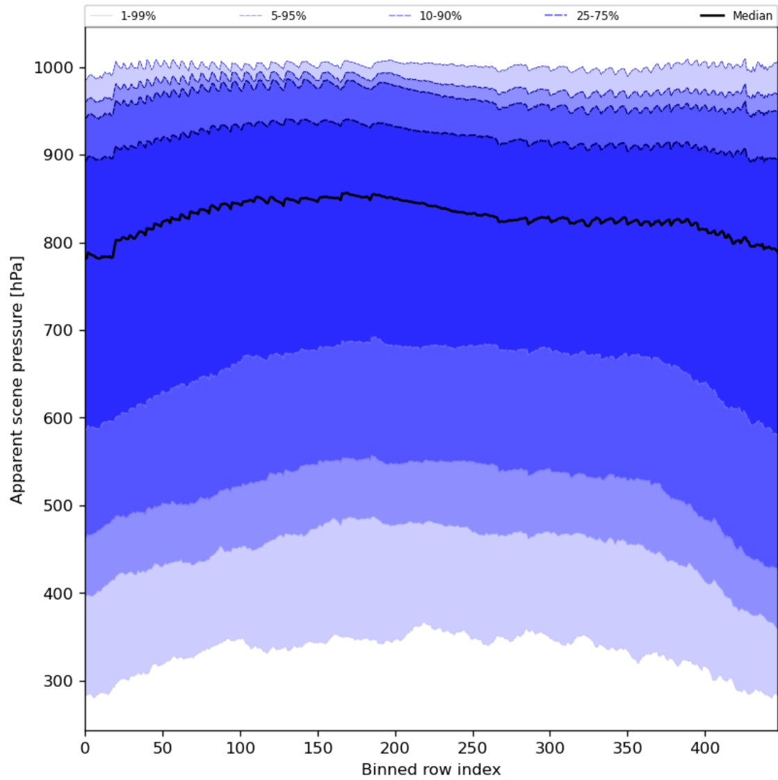
Figure 53: Along track statistics of “Apparent scene pressure” for 2023-10-03 to 2023-10-05
