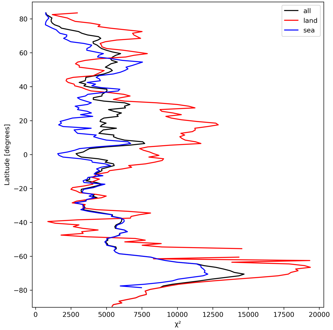
Figure 21: Zonal average of “ \chi^2 ” for 2023-10-03 to 2023-10-05.
