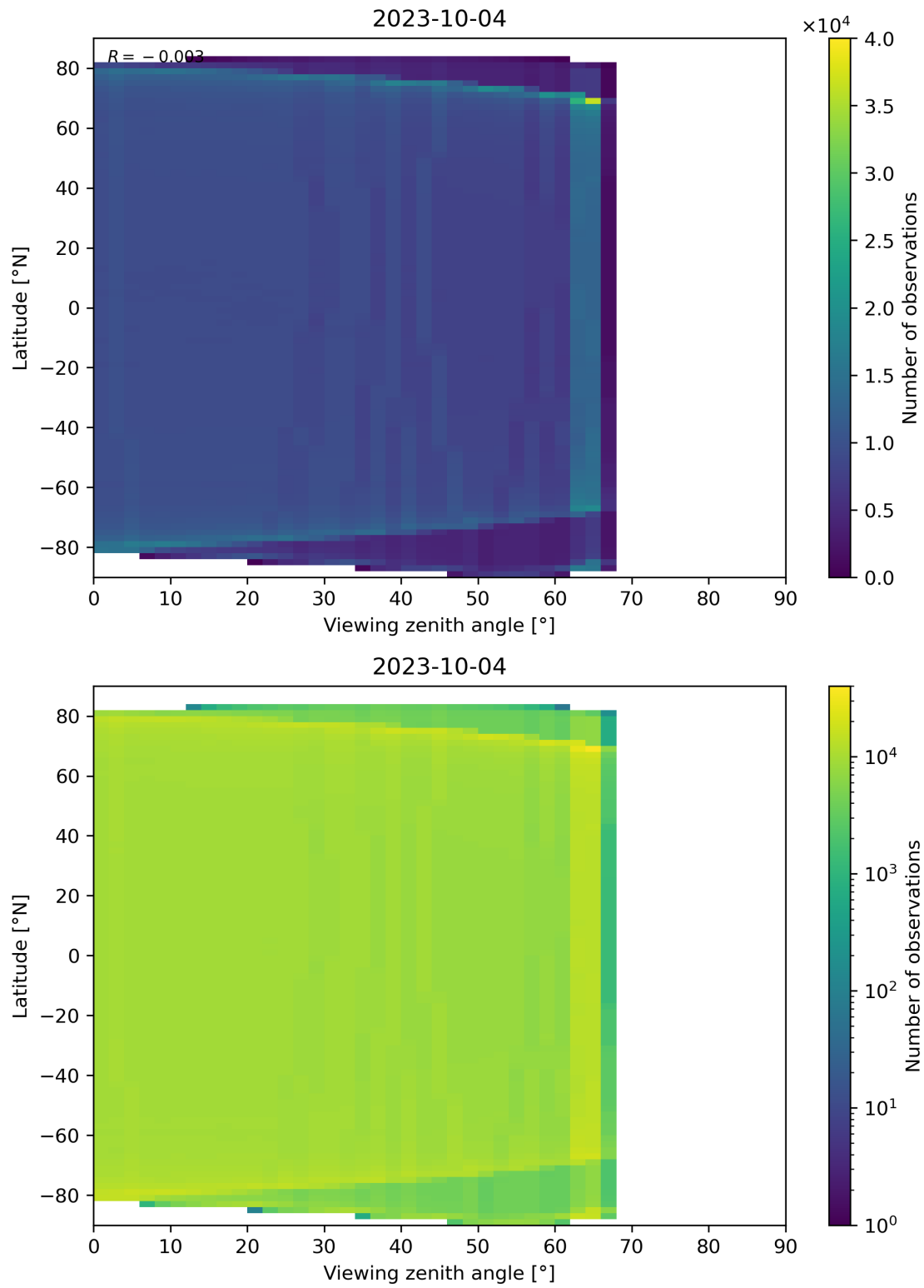
Figure 135: Scatter density plot of “Viewing zenith angle” against “Latitude” for 2023-10-03 to 2023-10-05.
