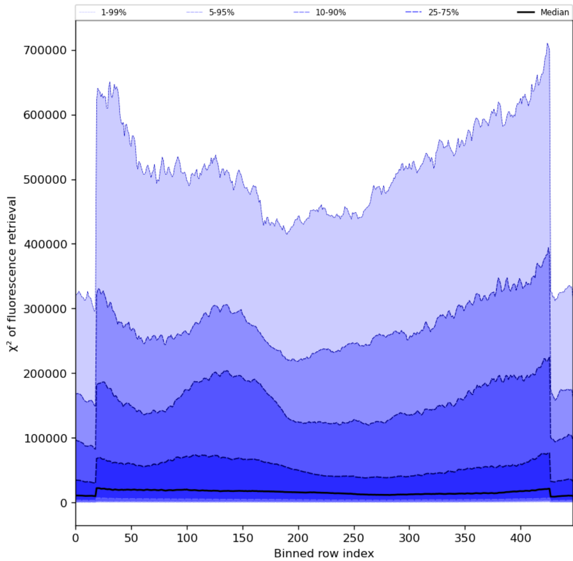
Figure 59: Along track statistics of “ \chi^2 of fluorescence retrieval” for 2023-10-03 to 2023-10-05
