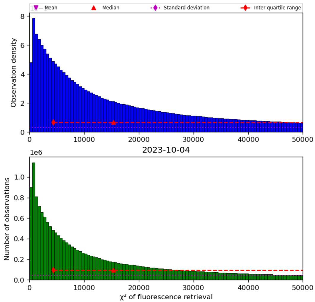
Figure 42: Histogram of “ \chi^2 of fluorescence retrieval” for 2023-10-03 to 2023-10-05
