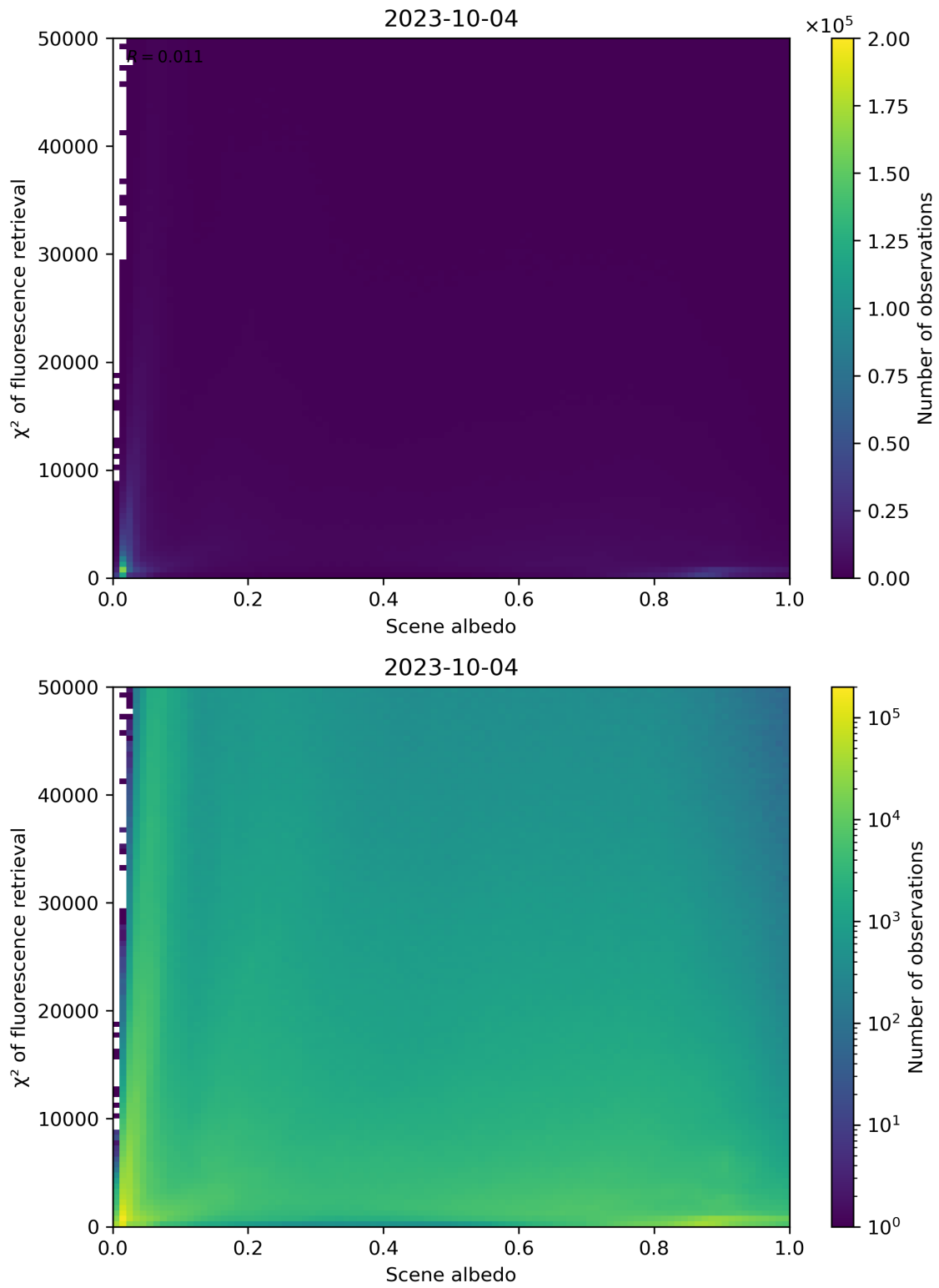
Figure 113: Scatter density plot of “Scene albedo” against “ \chi^2 of fluorescence retrieval” for 2023-10-03 to 2023-10-05.
