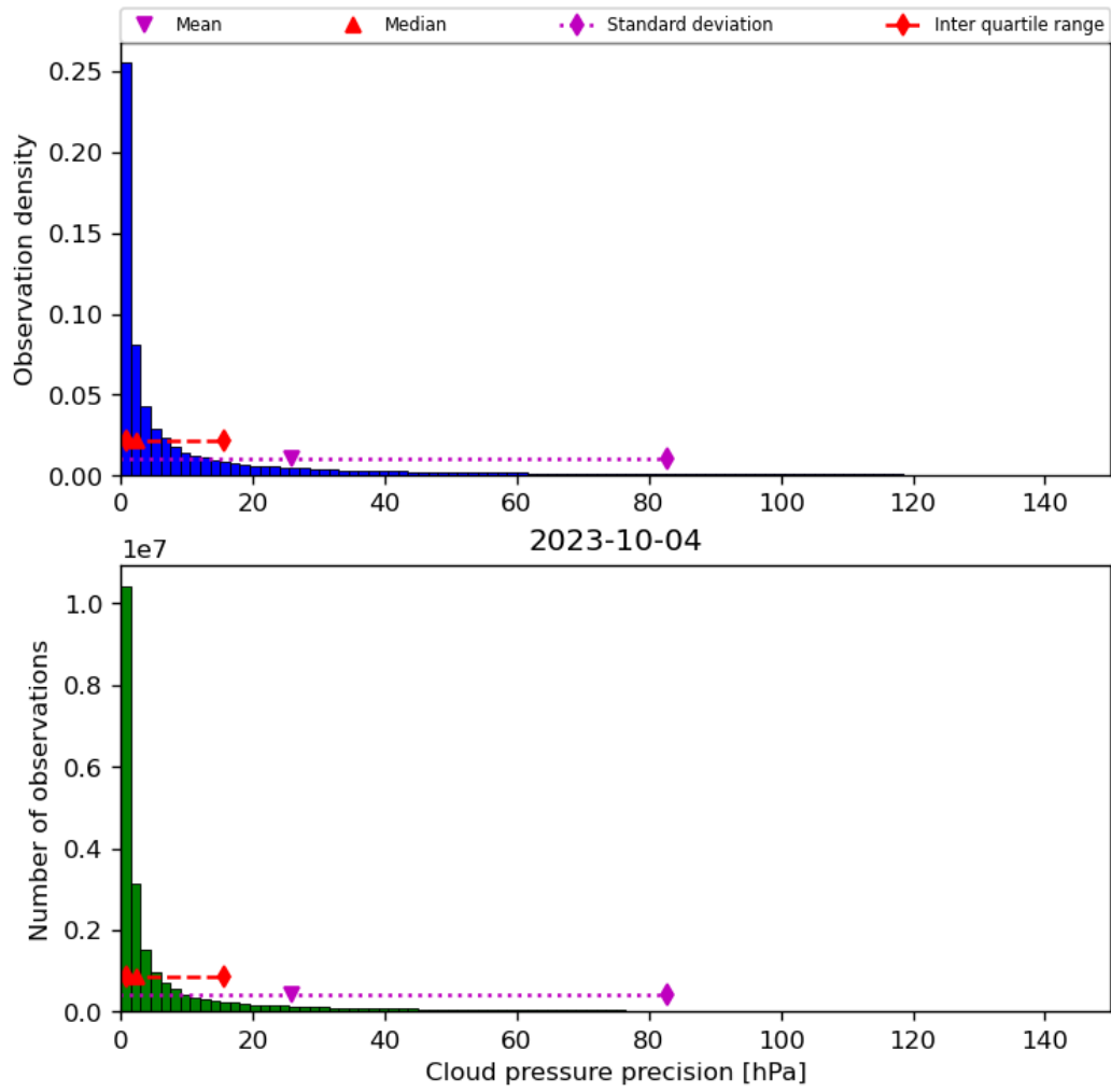
Figure 31: Histogram of “Cloud pressure precision” for 2023-10-03 to 2023-10-05
