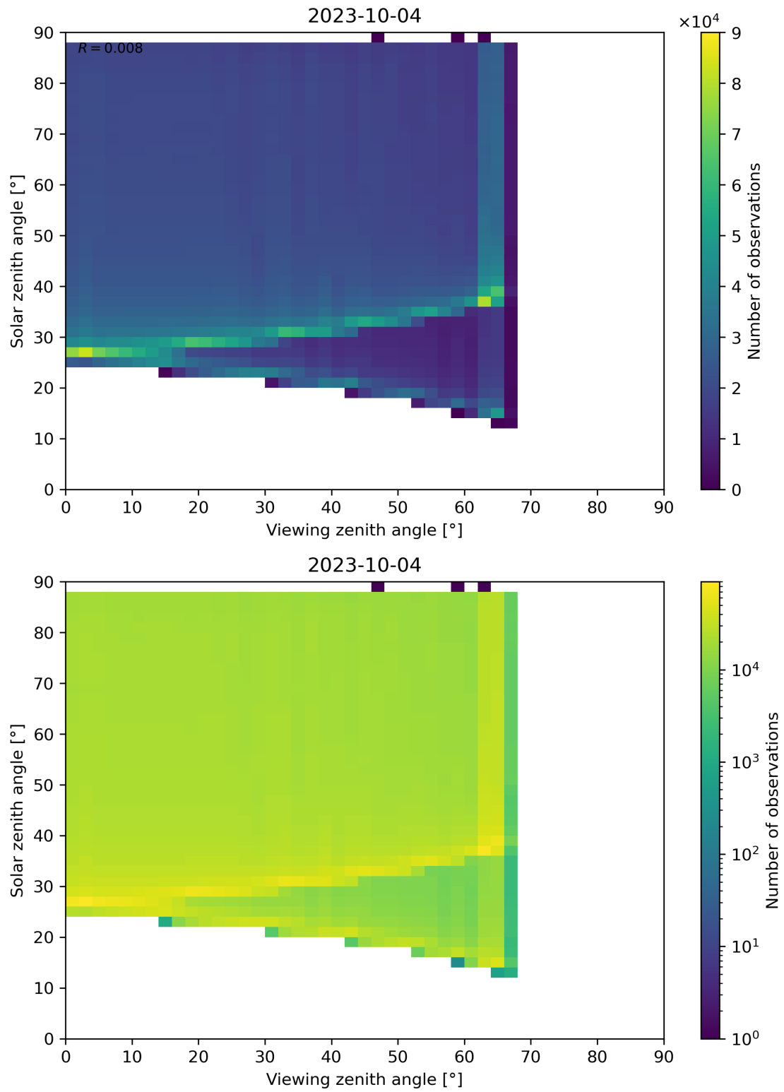
Figure 139: Scatter density plot of “Viewing zenith angle” against “Solar zenith angle” for 2023-10-03 to 2023-10-05.
