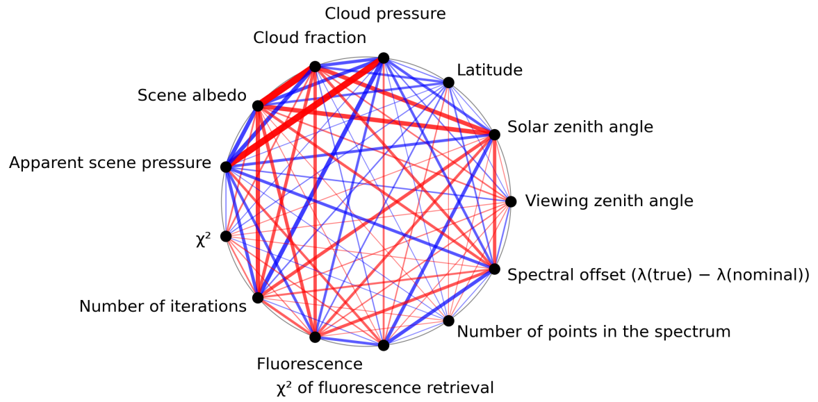
Figure 1: Map of correlation graph for 2023-10-03 to 2023-10-05.
