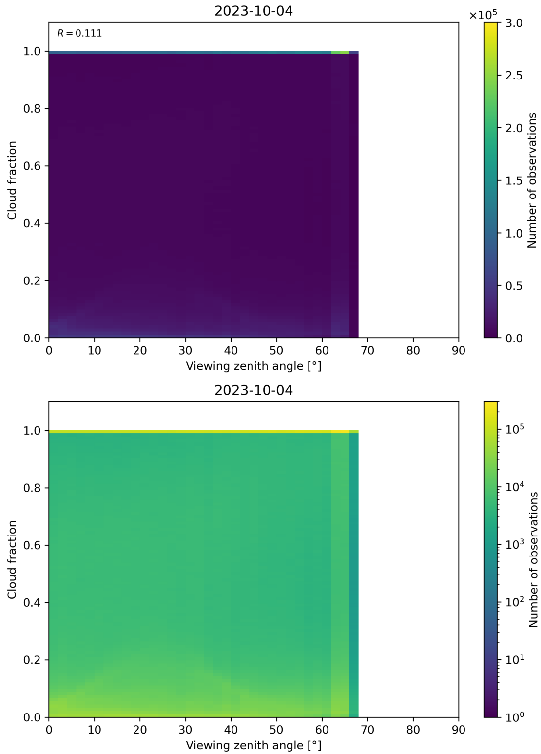
Figure 132: Scatter density plot of “Viewing zenith angle” against “Cloud fraction” for 2023-10-03 to 2023-10-05.
