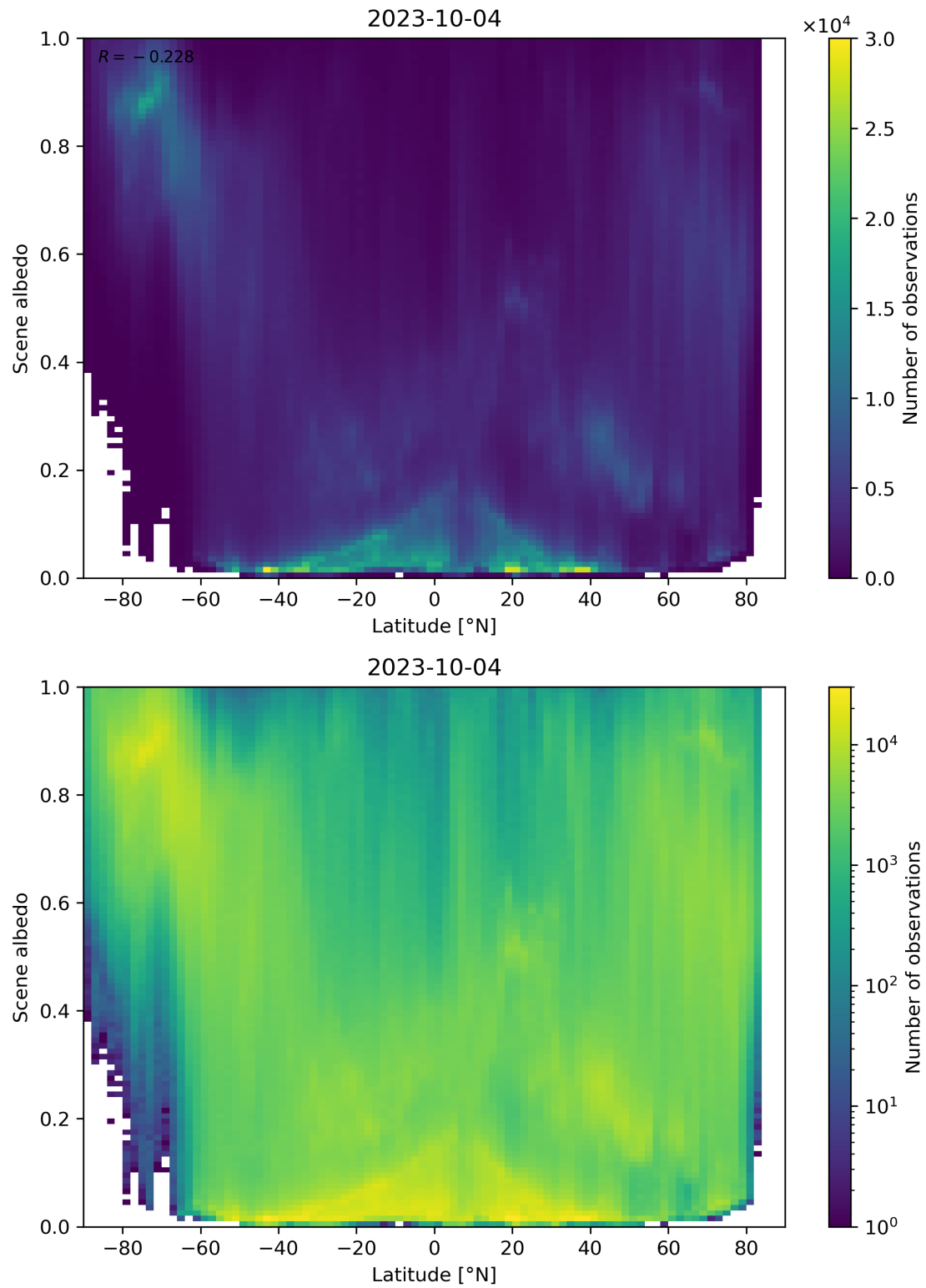
Figure 104: Scatter density plot of “Latitude” against “Scene albedo” for 2023-10-03 to 2023-10-05.
