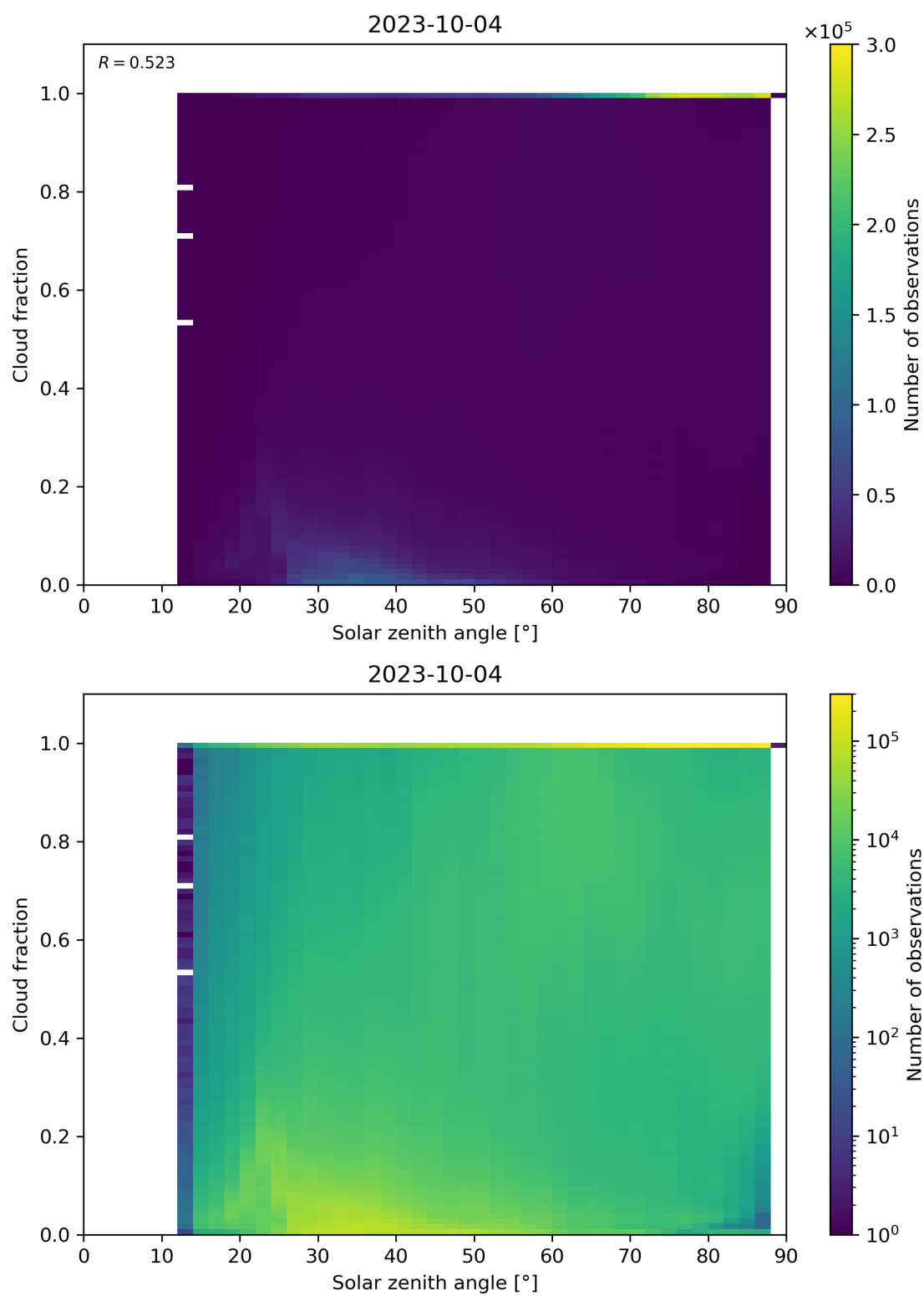
Figure 121: Scatter density plot of “Solar zenith angle” against “Cloud fraction” for 2023-10-03 to 2023-10-05.
