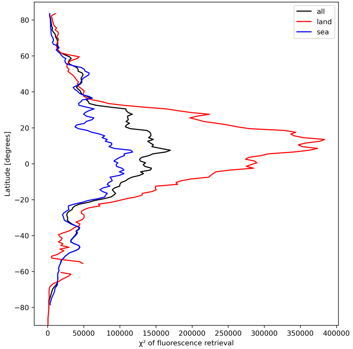
Figure 25: Zonal average of “ \chi^2 of fluorescence retrieval” for 2023-10-03 to 2023-10-05.
