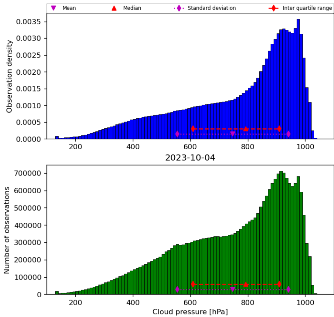
Figure 30: Histogram of “Cloud pressure” for 2023-10-03 to 2023-10-05
