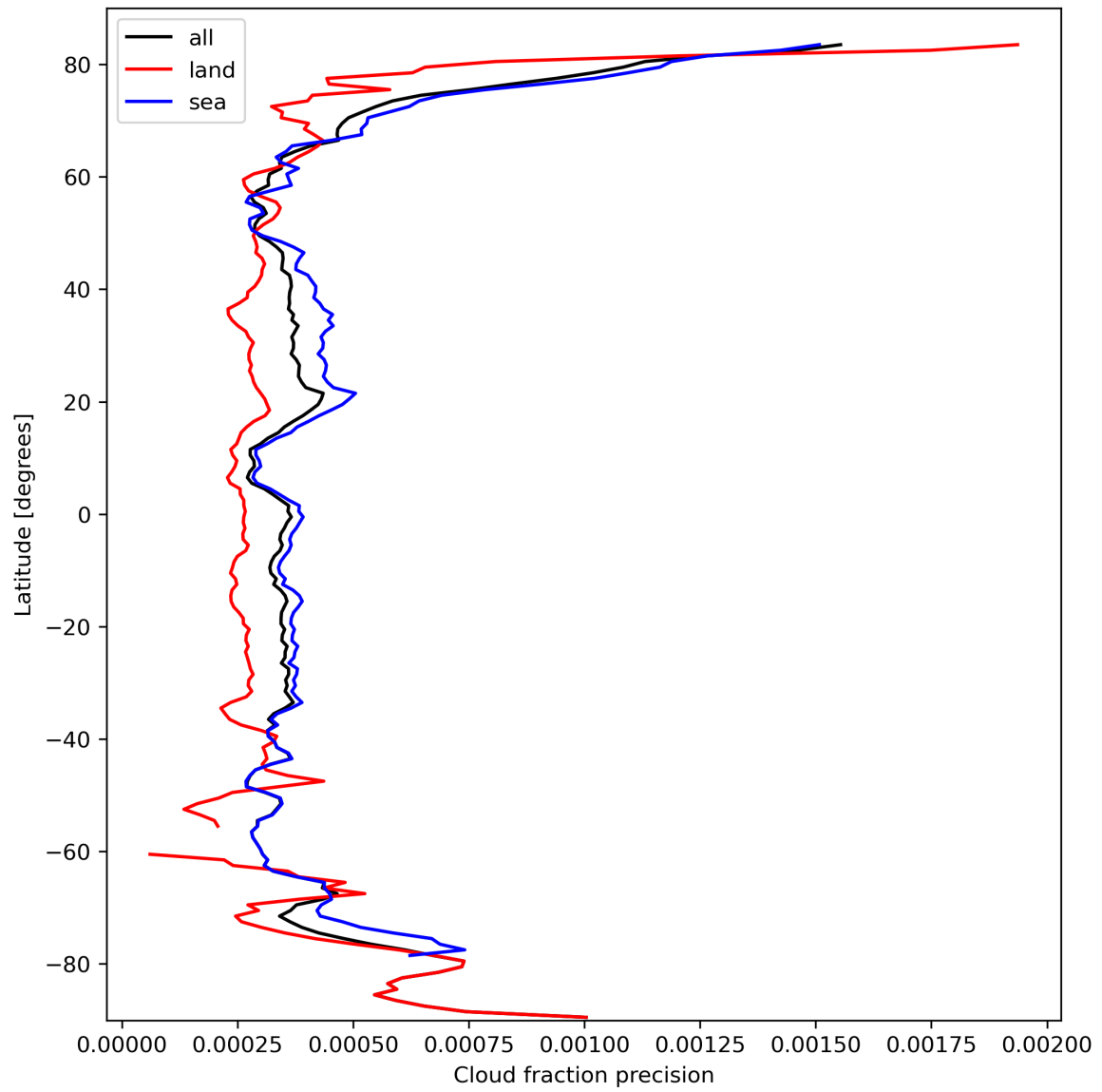
Figure 16: Zonal average of “Cloud fraction precision” for 2023-10-03 to 2023-10-05.
